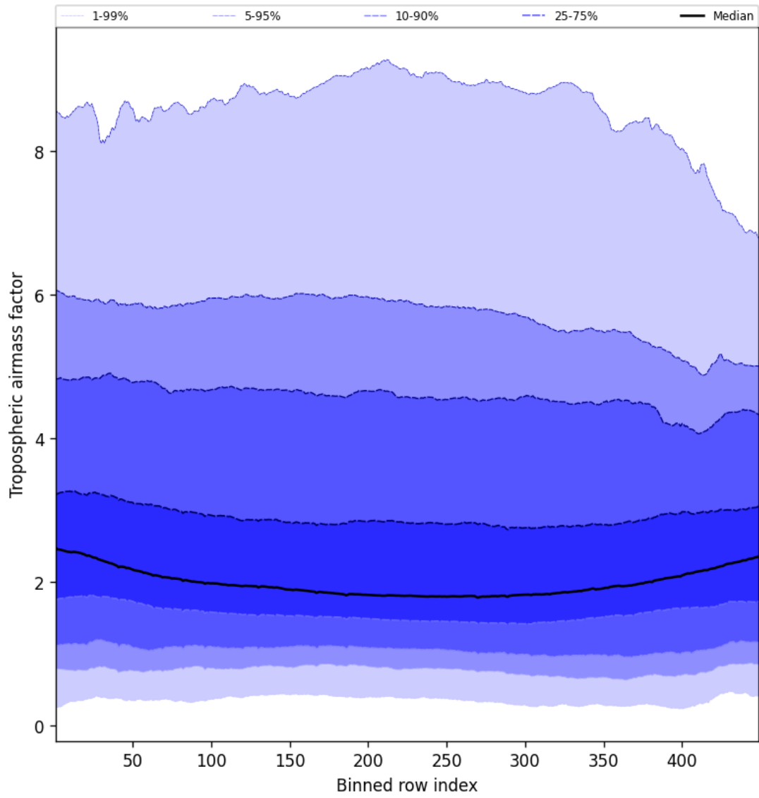
Figure 46: Along track statistics of “Tropospheric airmass factor” for 2025-09-20 to 2025-09-21
