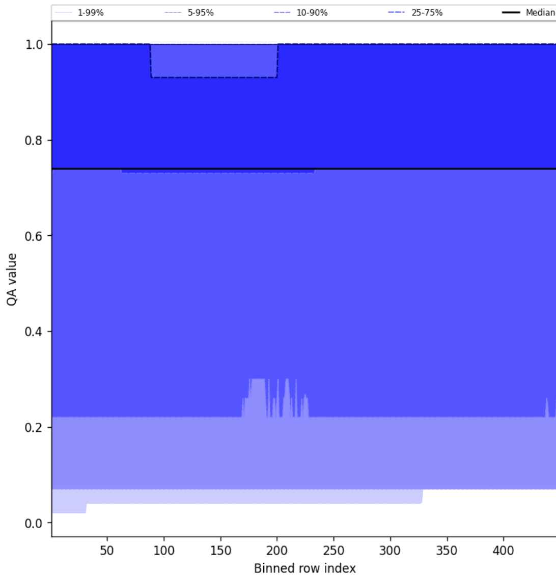
Figure 43: Along track statistics of “QA value” for 2025-09-20 to 2025-09-21
