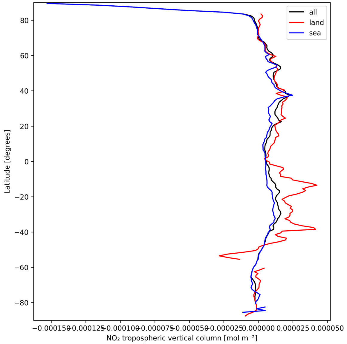
Figure 10: Zonal average of “NO 2 tropospheric vertical column” for 2025-09-20 to 2025-09-21.
