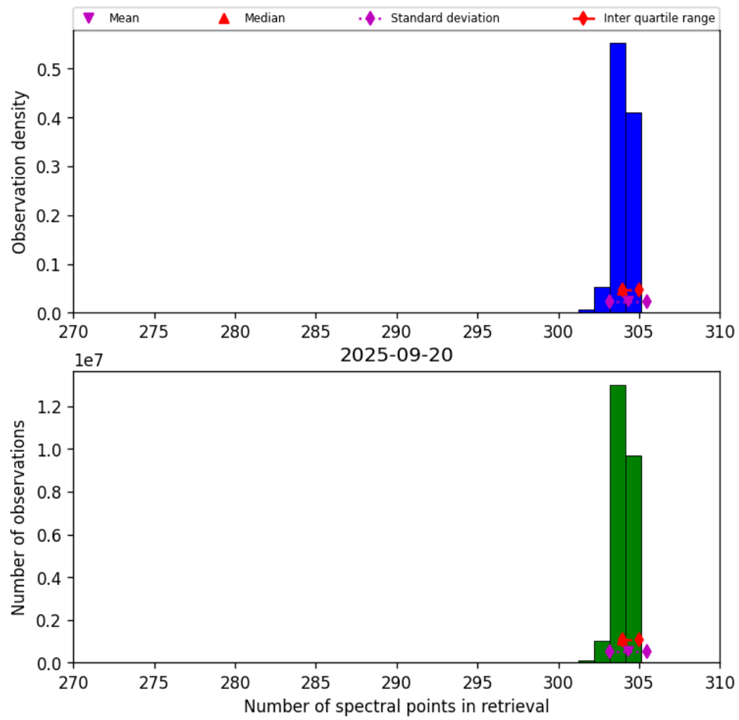
Figure 31: Histogram of “Number of spectral points in retrieval” for 2025-09-20 to 2025-09-21
