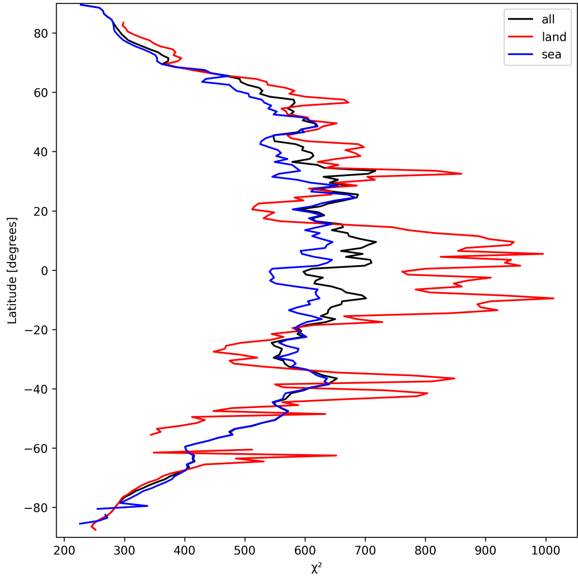
Figure 23: Zonal average of “ \chi^2 ” for 2025-09-20 to 2025-09-21.
