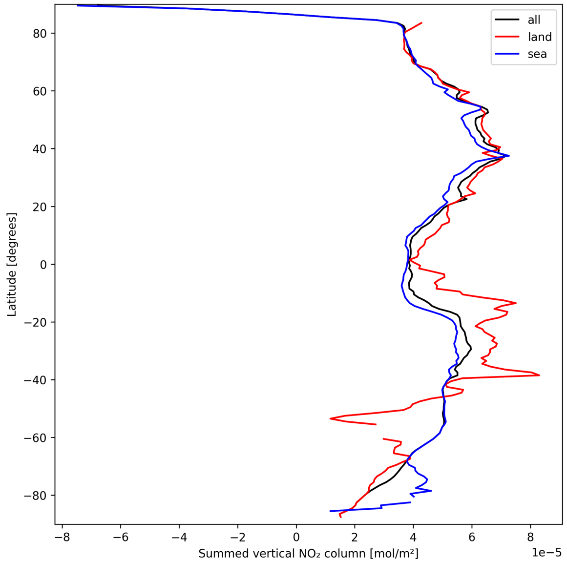
Figure 21: Zonal average of “Summed vertical NO 2 column” for 2025-09-20 to 2025-09-21.
