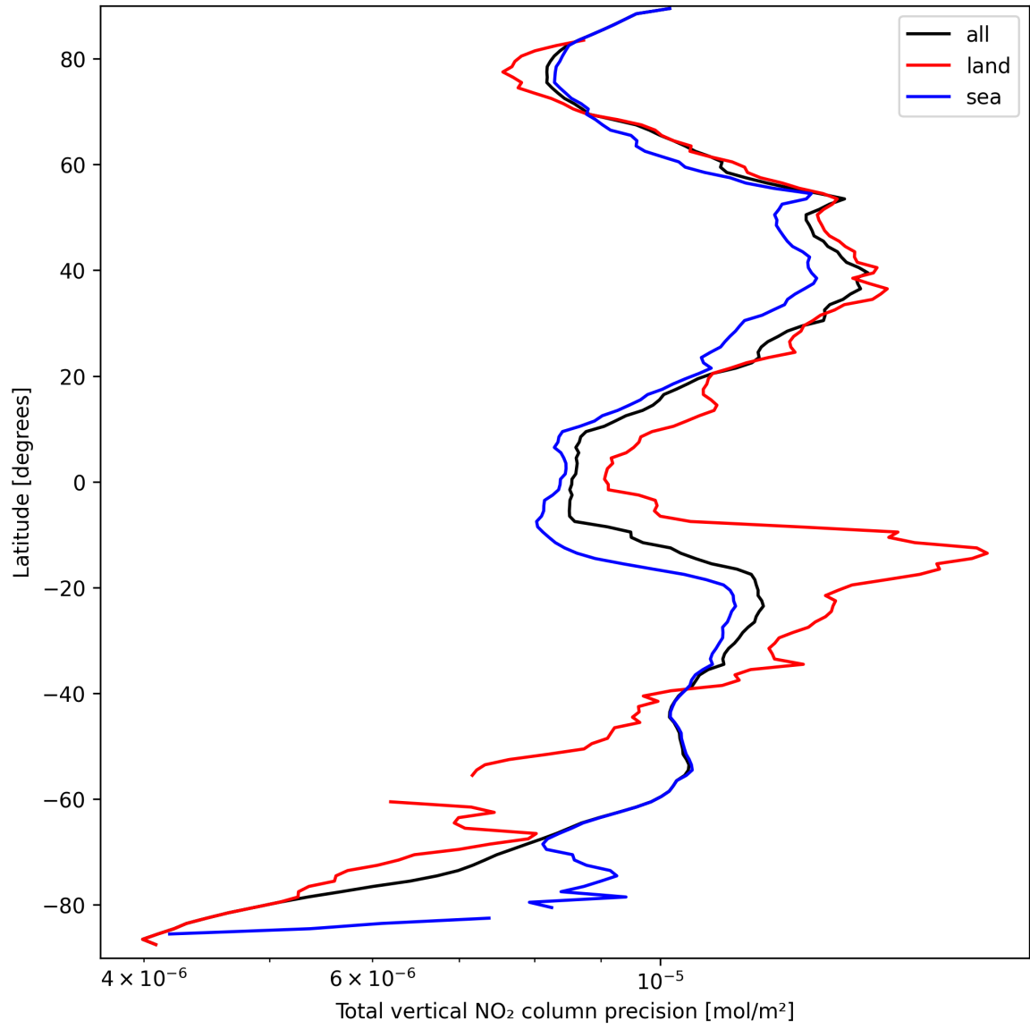
Figure 20: Zonal average of "Total vertical NO 2 column precision" for 2025-09-20 to 2025-09-21.
