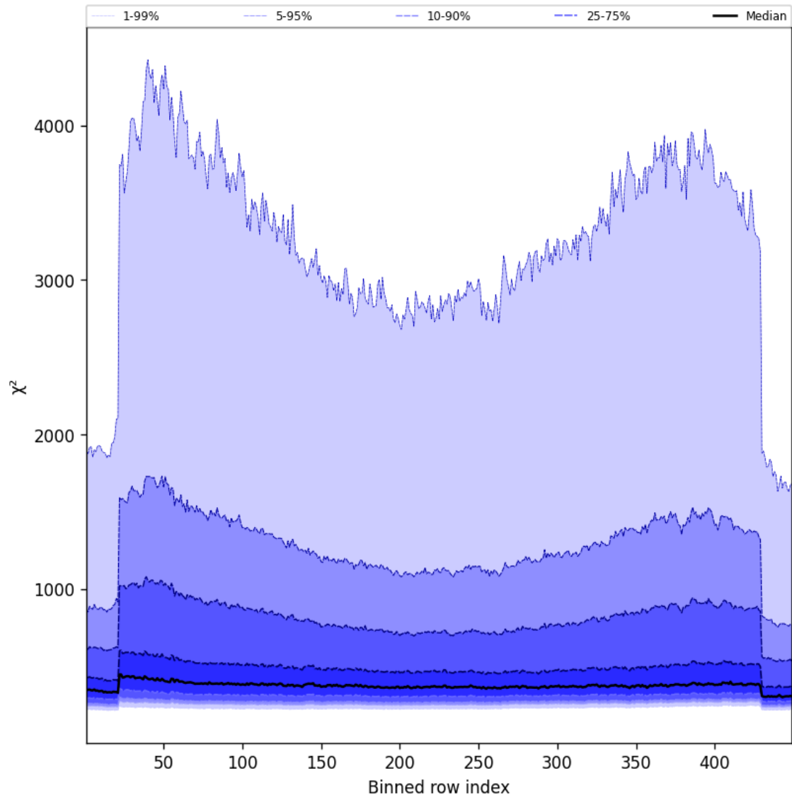
Figure 57: Along track statistics of “ \chi^2 ” for 2025-09-20 to 2025-09-21
