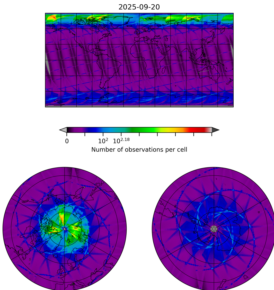
Figure 8: Map of the number of observations for 2025-09-20 to 2025-09-21
