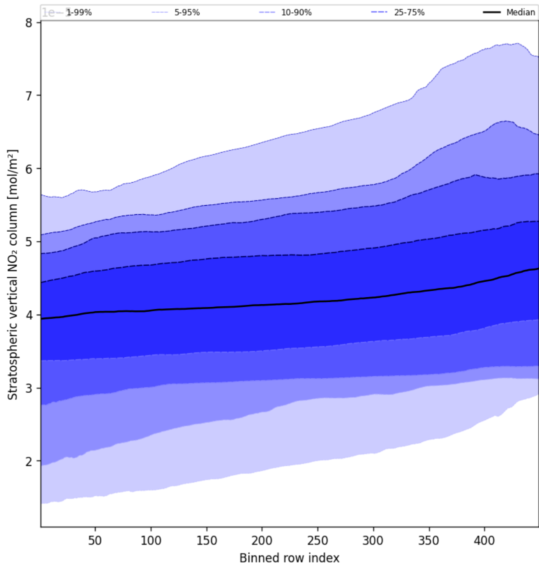
Figure 51: Along track statistics of “Stratospheric vertical NO 2 column” for 2025-09-20 to 2025-09-21
