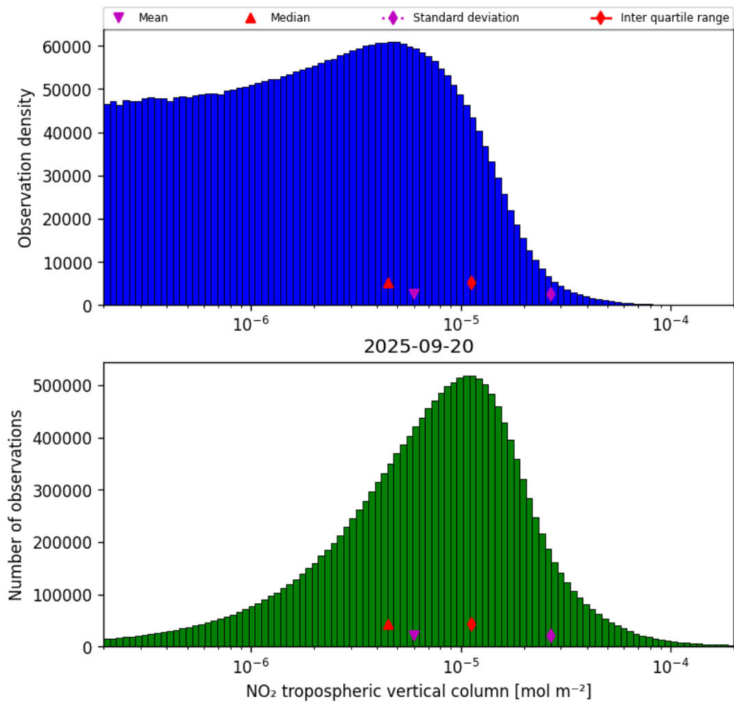
Figure 27: Histogram of “NO 2 tropospheric vertical column” for 2025-09-20 to 2025-09-21
