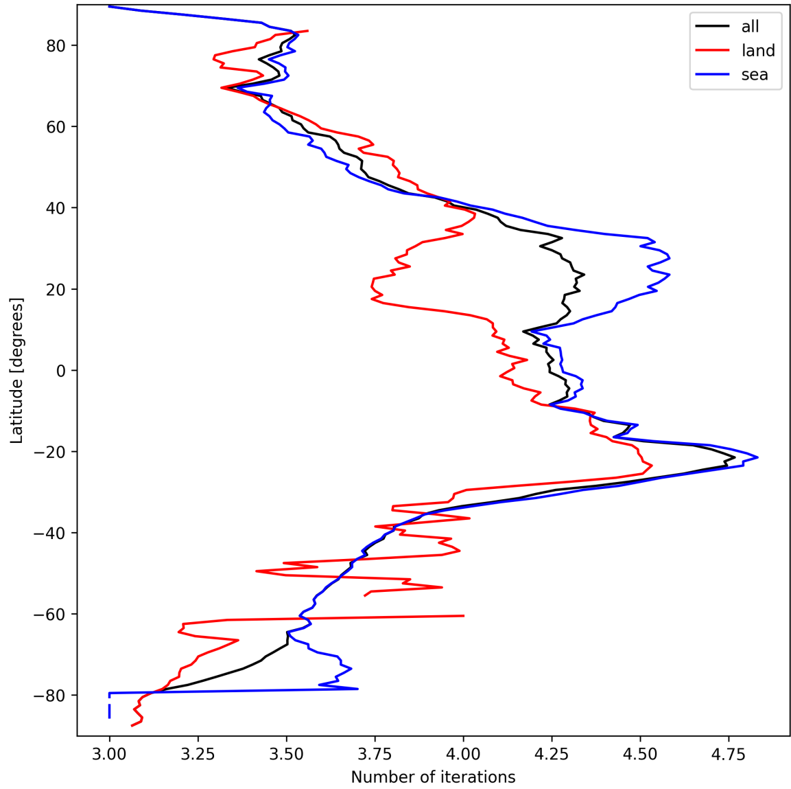
Figure 15: Zonal average of “Number of iterations” for 2025-09-20 to 2025-09-21.
