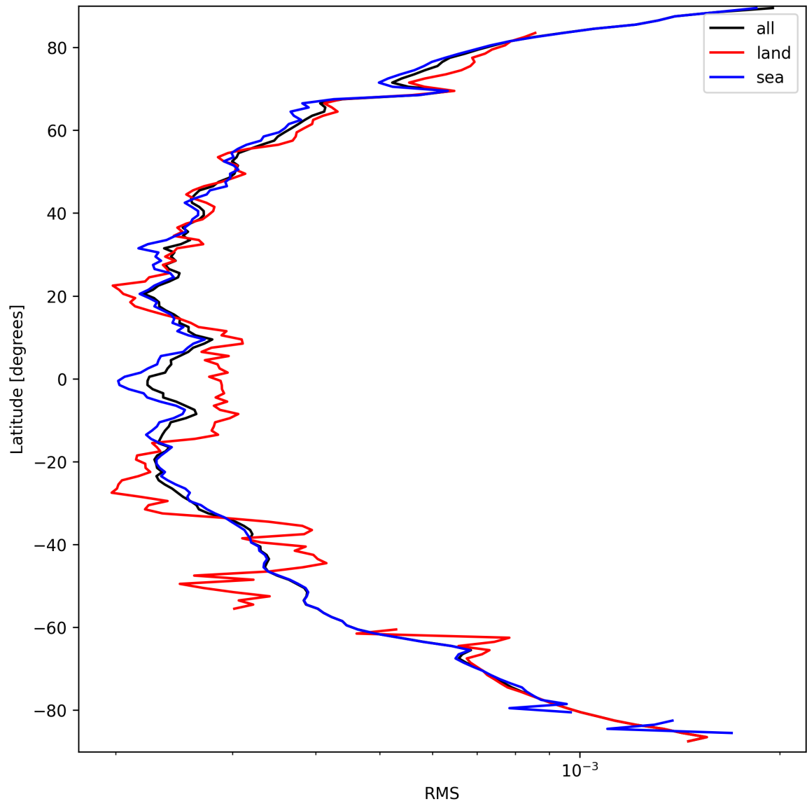
Figure 24: Zonal average of “RMS” for 2025-09-20 to 2025-09-21.
