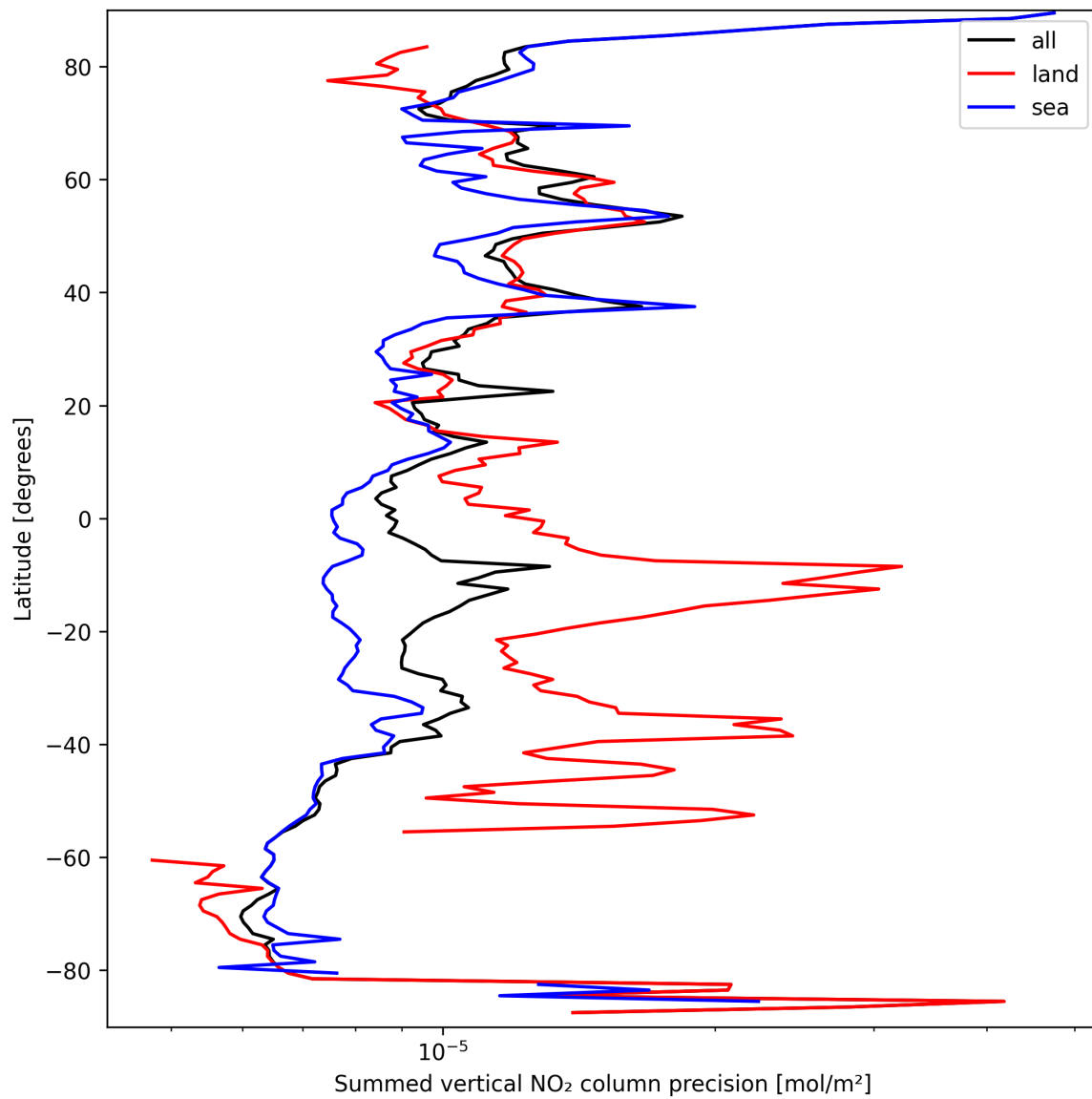
Figure 22: Zonal average of “Summed vertical NO 2 column precision” for 2025-09-20 to 2025-09-21.
