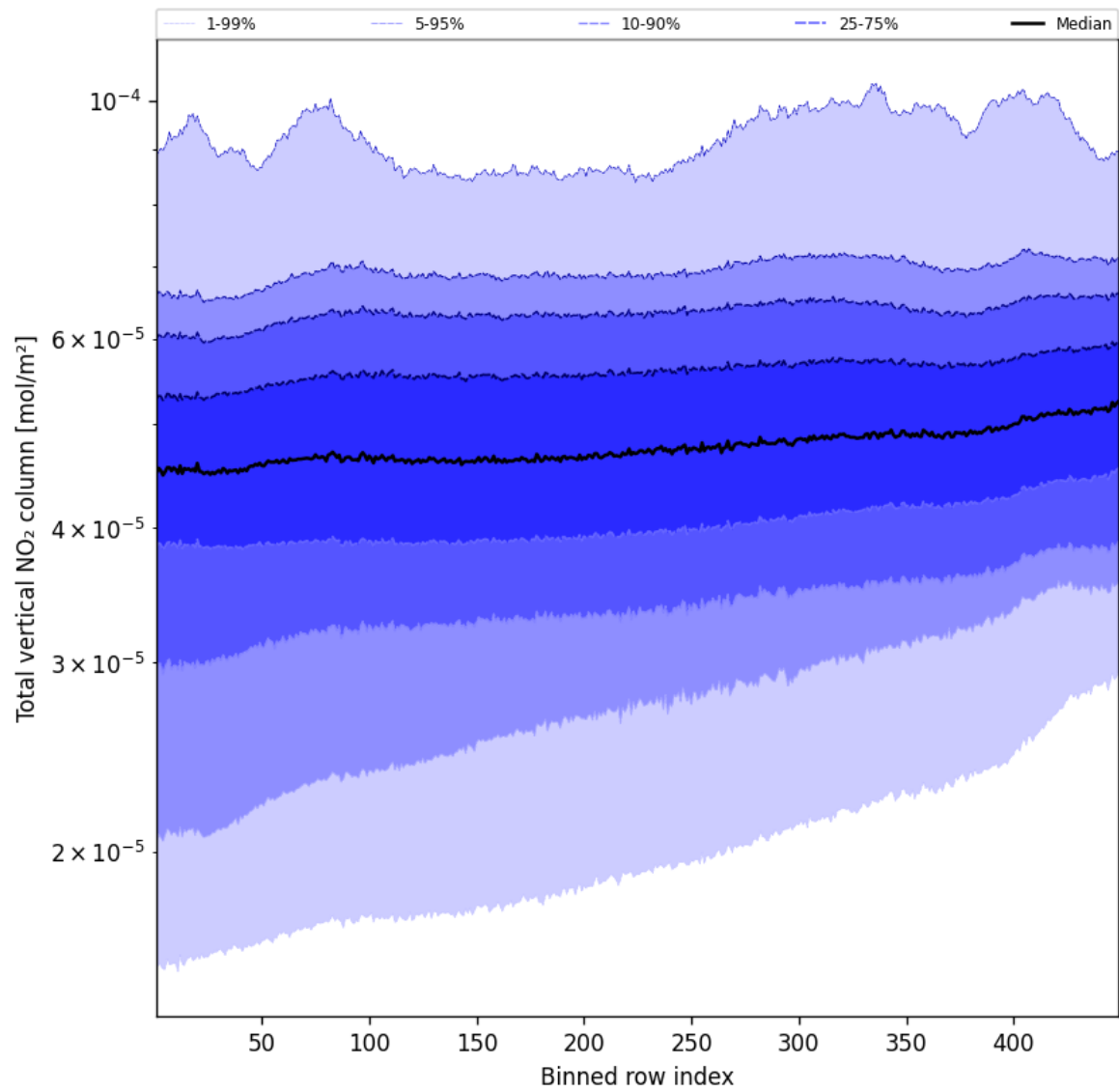
Figure 53: Along track statistics of “Total vertical NO 2 column” for 2025-09-20 to 2025-09-21
