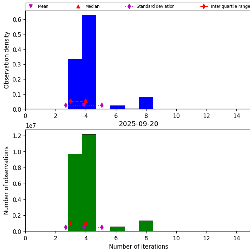
Figure 32: Histogram of “Number of iterations” for 2025-09-20 to 2025-09-21
