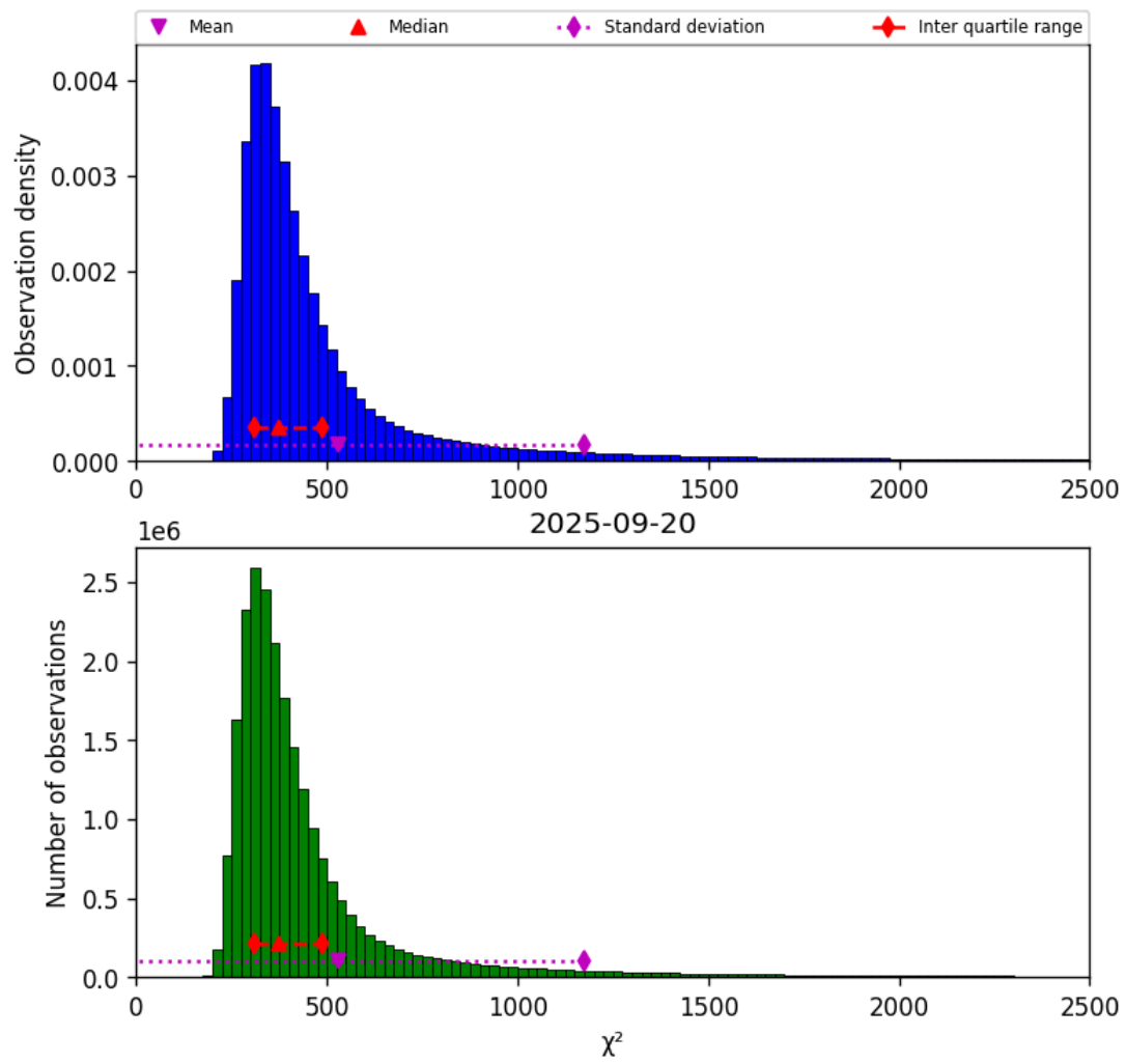
Figure 40: Histogram of “ \chi^2 ” for 2025-09-20 to 2025-09-21
