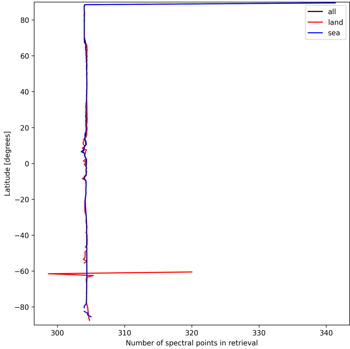
Figure 14: Zonal average of “Number of spectral points in retrieval” for 2025-09-20 to 2025-09-21.
