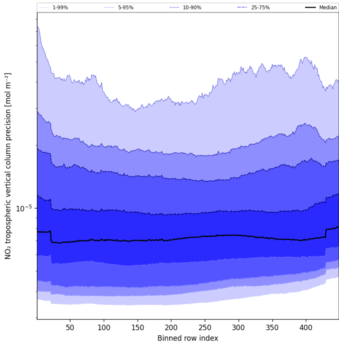
Figure 45: Along track statistics of “NO 2 tropospheric vertical column precision” for 2025-09-20 to 2025-09-21
