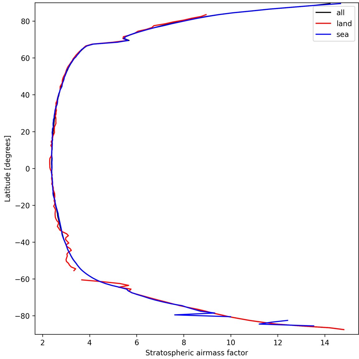
Figure 25: Zonal average of “Stratospheric airmass factor” for 2025-09-20 to 2025-09-21.
