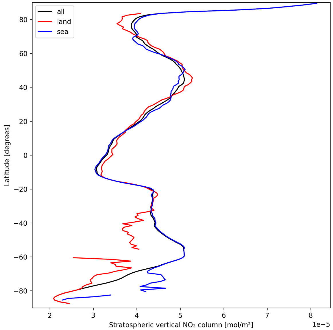
Figure 17: Zonal average of “Stratospheric vertical NO 2 column” for 2025-09-20 to 2025-09-21.
