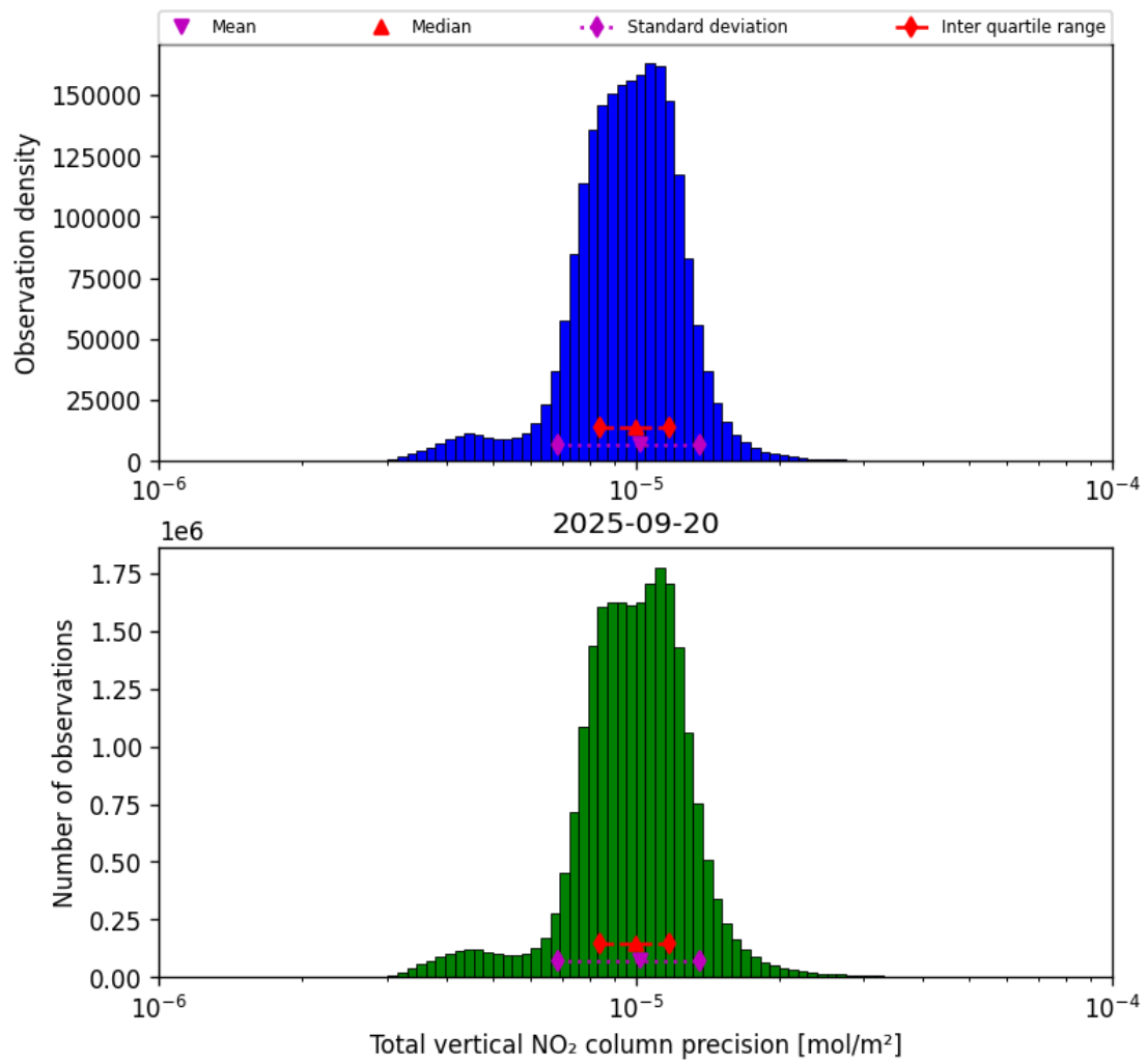
Figure 37: Histogram of “Total vertical NO 2 column precision” for 2025-09-20 to 2025-09-21
