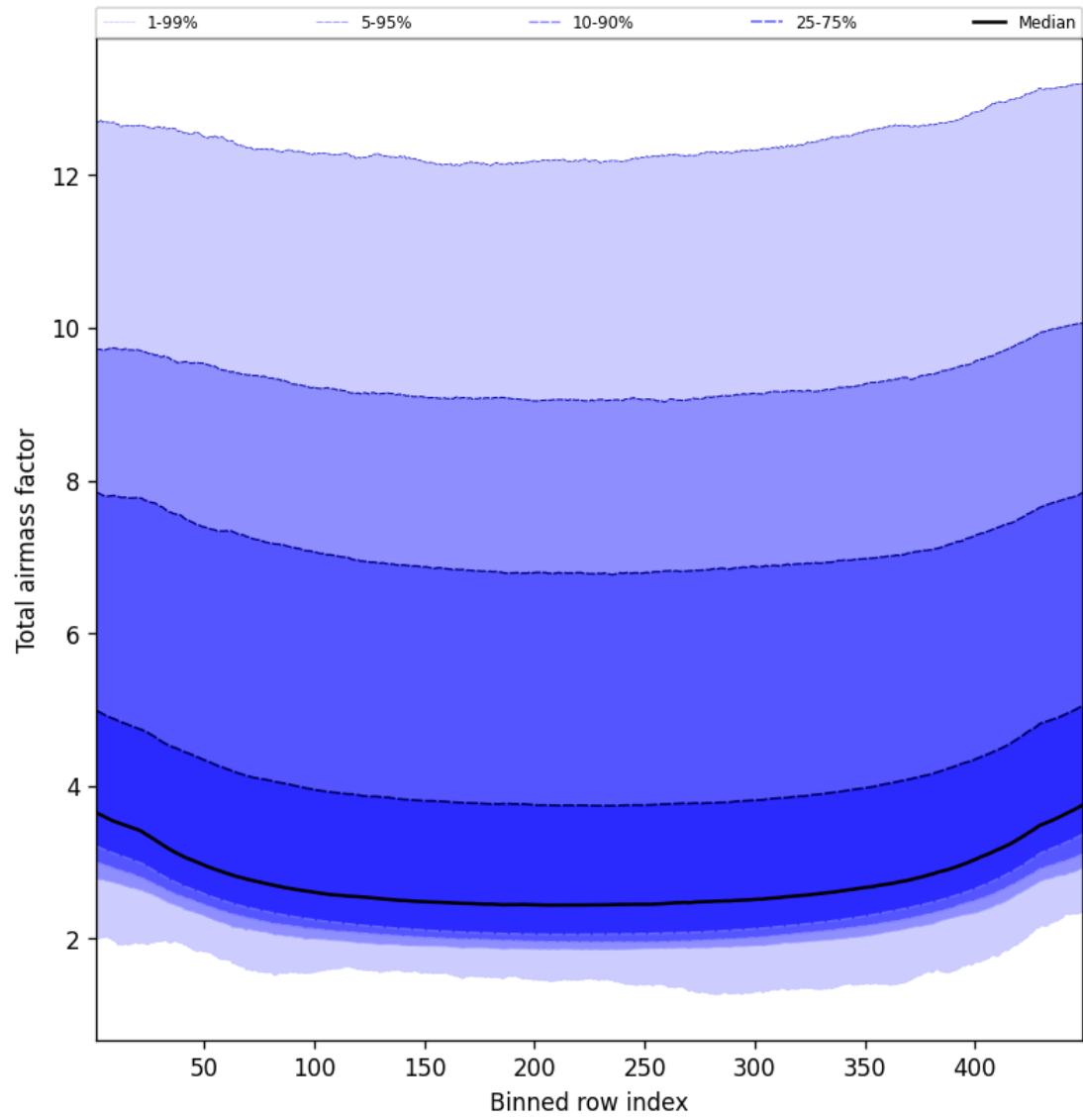
Figure 47: Along track statistics of “Total airmass factor” for 2025-09-20 to 2025-09-21
