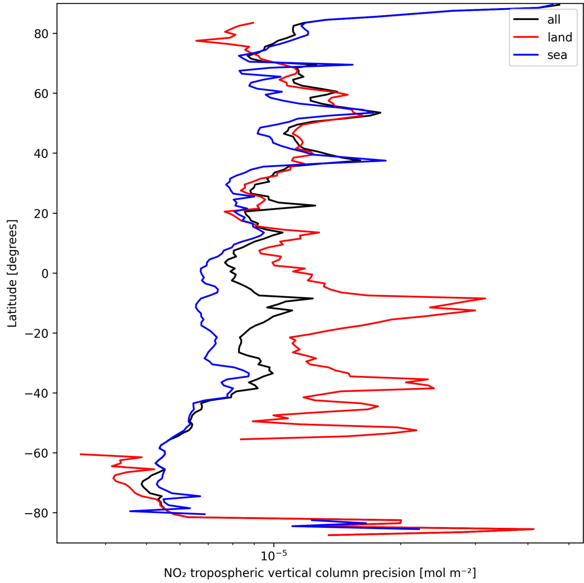
Figure 11: Zonal average of “NO 2 tropospheric vertical column precision” for 2025-09-20 to 2025-09-21.
