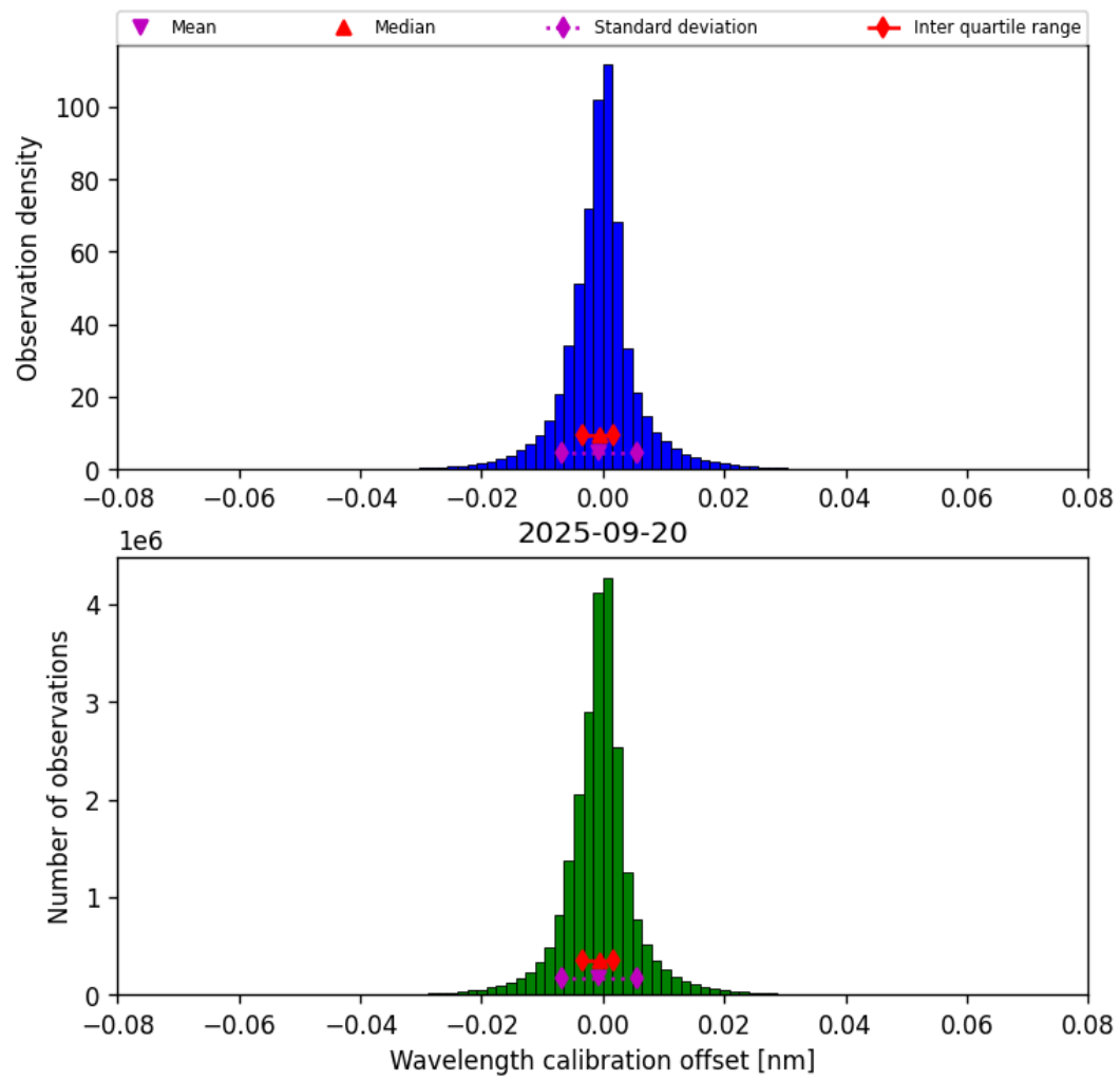
Figure 33: Histogram of “Wavelength calibration offset” for 2025-09-20 to 2025-09-21
