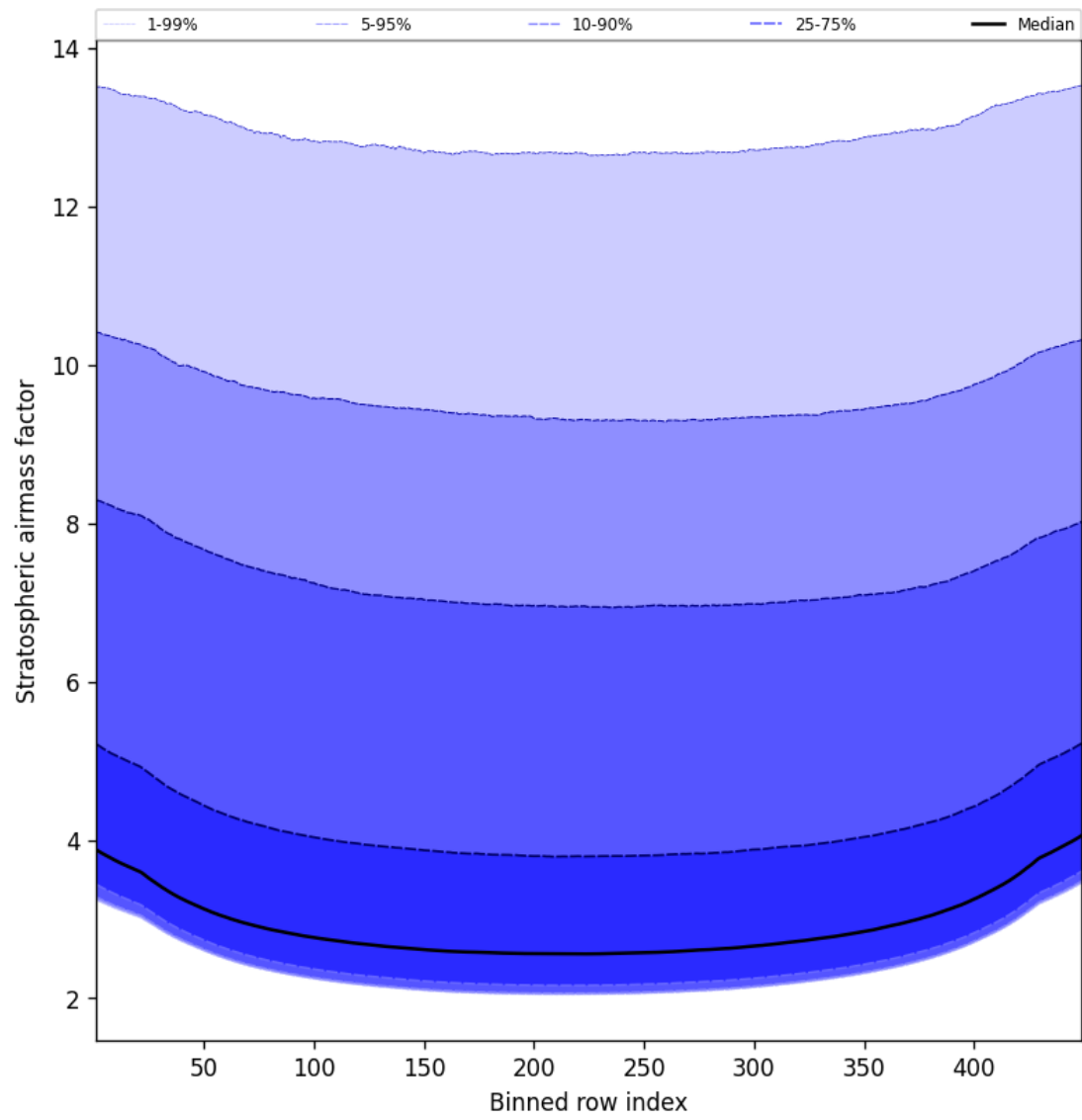
Figure 59: Along track statistics of “Stratospheric airmass factor” for 2025-09-20 to 2025-09-21
