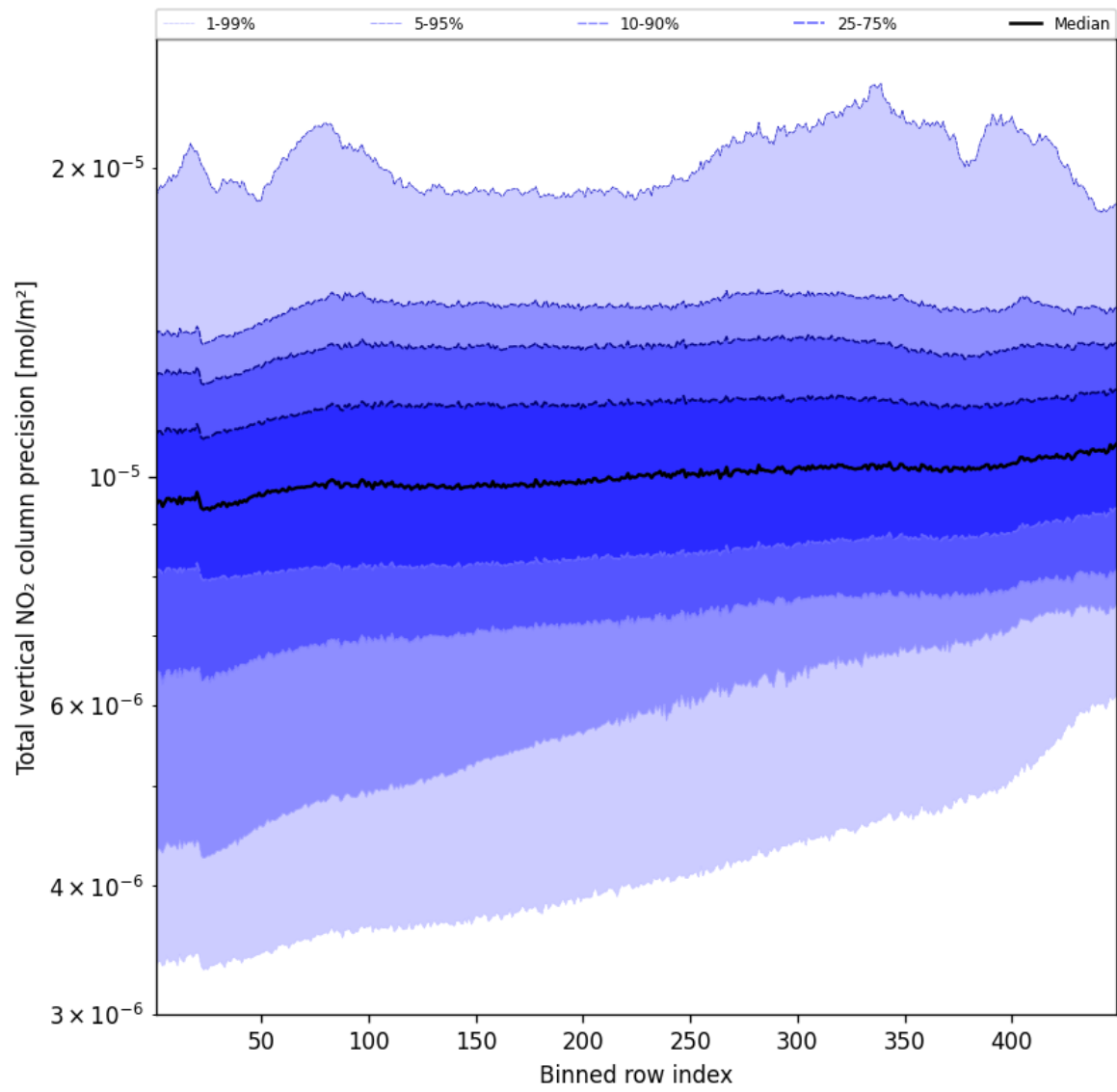
Figure 54: Along track statistics of “Total vertical NO 2 column precision” for 2025-09-20 to 2025-09-21
