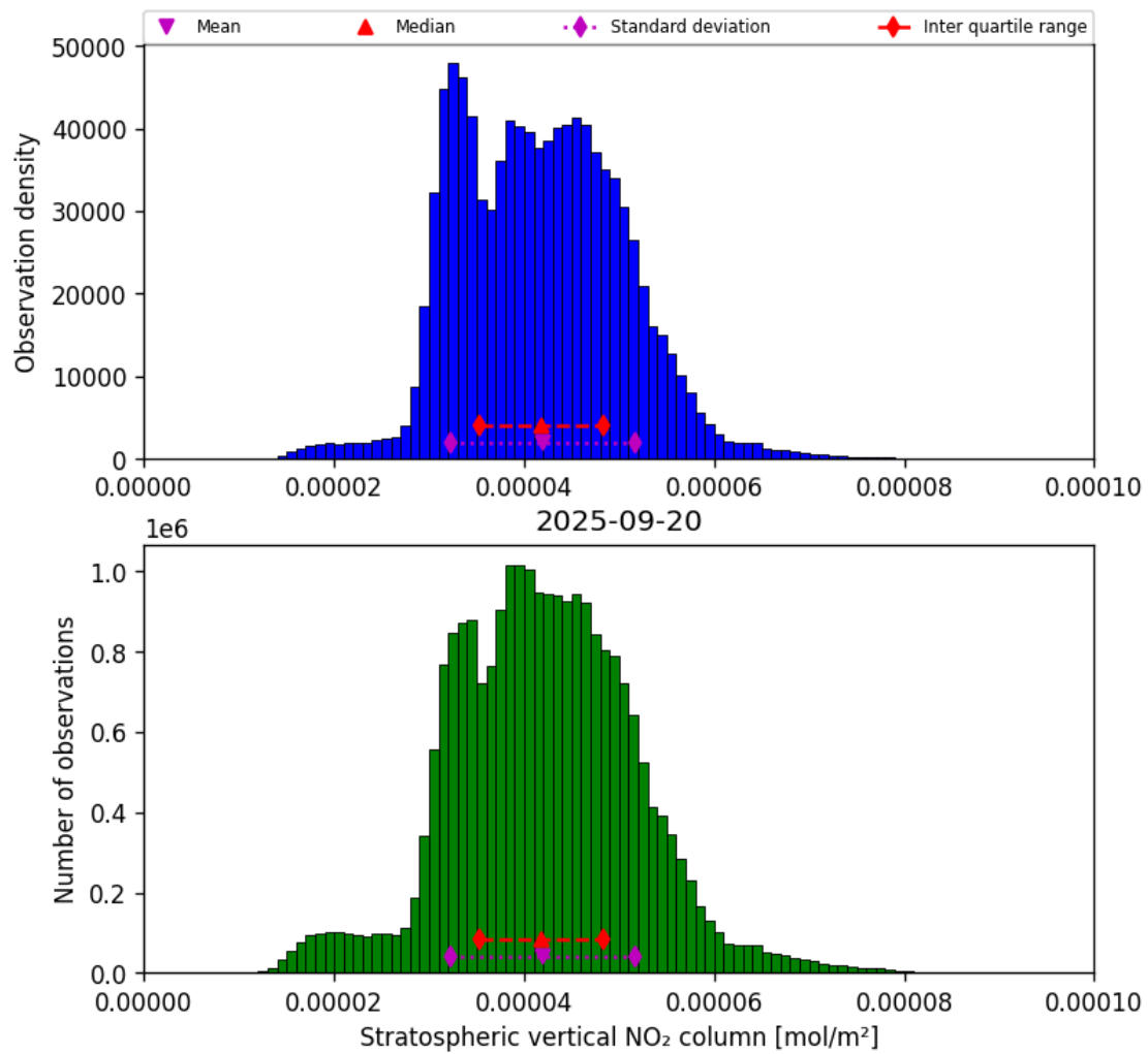
Figure 34: Histogram of “Stratospheric vertical NO 2 column” for 2025-09-20 to 2025-09-21
