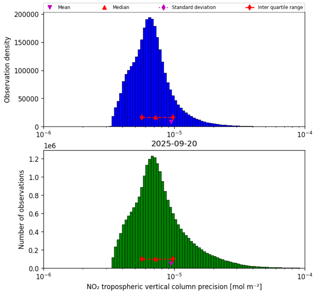
Figure 28: Histogram of “NO 2 tropospheric vertical column precision” for 2025-09-20 to 2025-09-21
