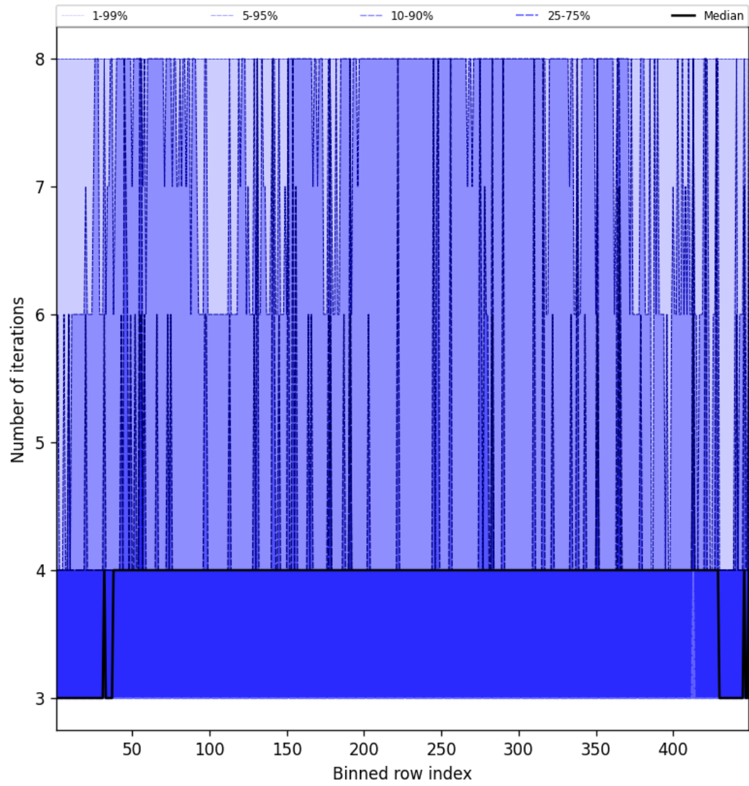
Figure 49: Along track statistics of “Number of iterations” for 2025-09-20 to 2025-09-21
