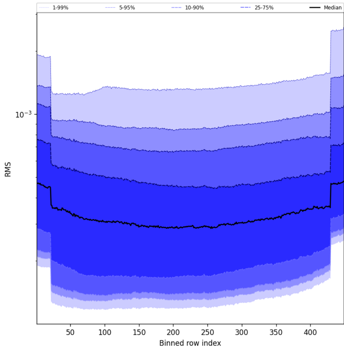
Figure 58: Along track statistics of “RMS” for 2025-09-20 to 2025-09-21
