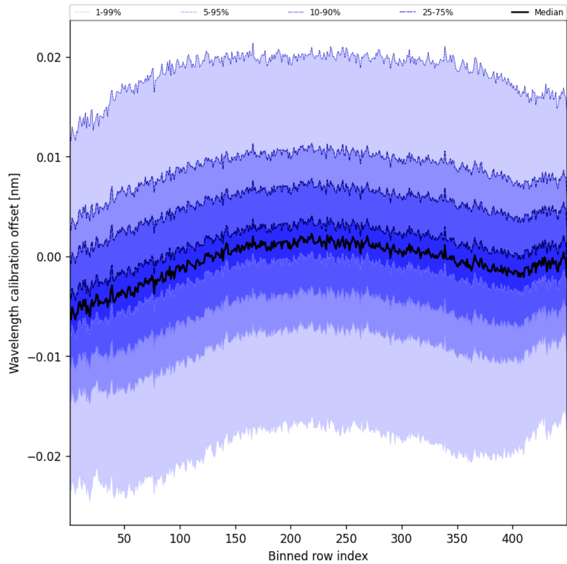
Figure 50: Along track statistics of “Wavelength calibration offset” for 2025-09-20 to 2025-09-21
