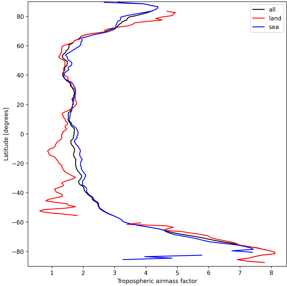
Figure 12: Zonal average of “Tropospheric air mass factor” for 2025-09-20 to 2025-09-21.
