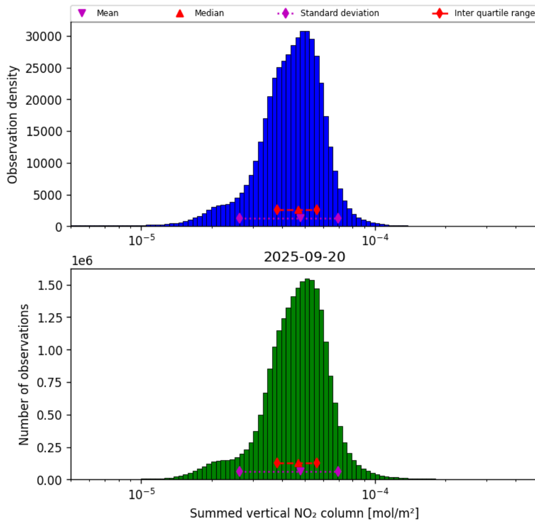
Figure 38: Histogram of "Summed vertical NO 2 column" for 2025-09-20 to 2025-09-21
