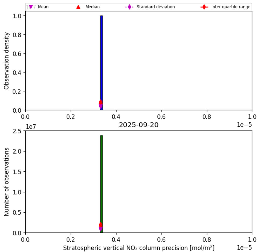
Figure 35: Histogram of “Stratospheric vertical NO 2 column precision” for 2025-09-20 to 2025-09-21
