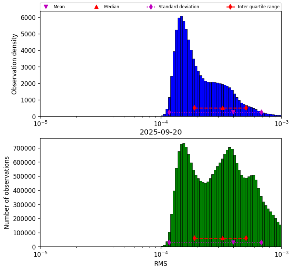
Figure 41: Histogram of “RMS” for 2025-09-20 to 2025-09-21
