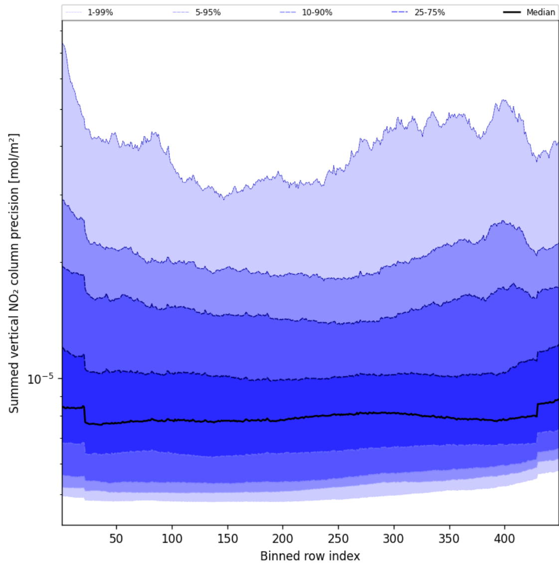
Figure 56: Along track statistics of “Summed vertical NO 2 column precision” for 2025-09-20 to 2025-09-21
