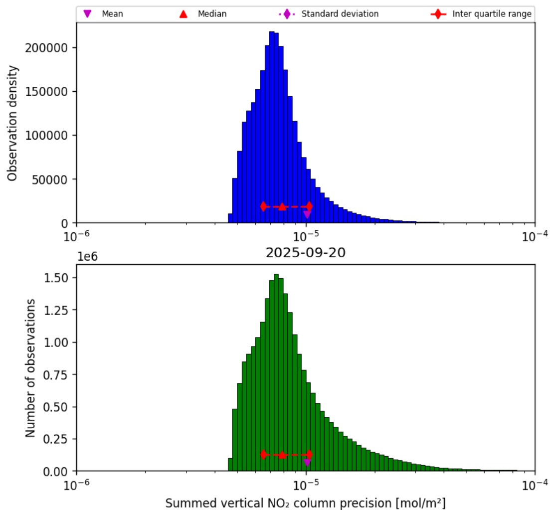
Figure 39: Histogram of “Summed vertical NO 2 column precision” for 2025-09-20 to 2025-09-21
