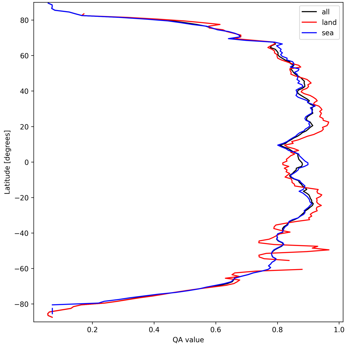
Figure 9: Zonal average of “QA value” for 2025-09-20 to 2025-09-21.
