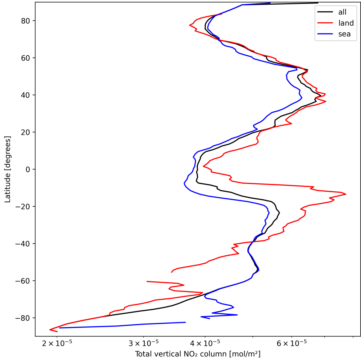
Figure 19: Zonal average of “Total vertical NO 2 column” for 2025-09-20 to 2025-09-21.
