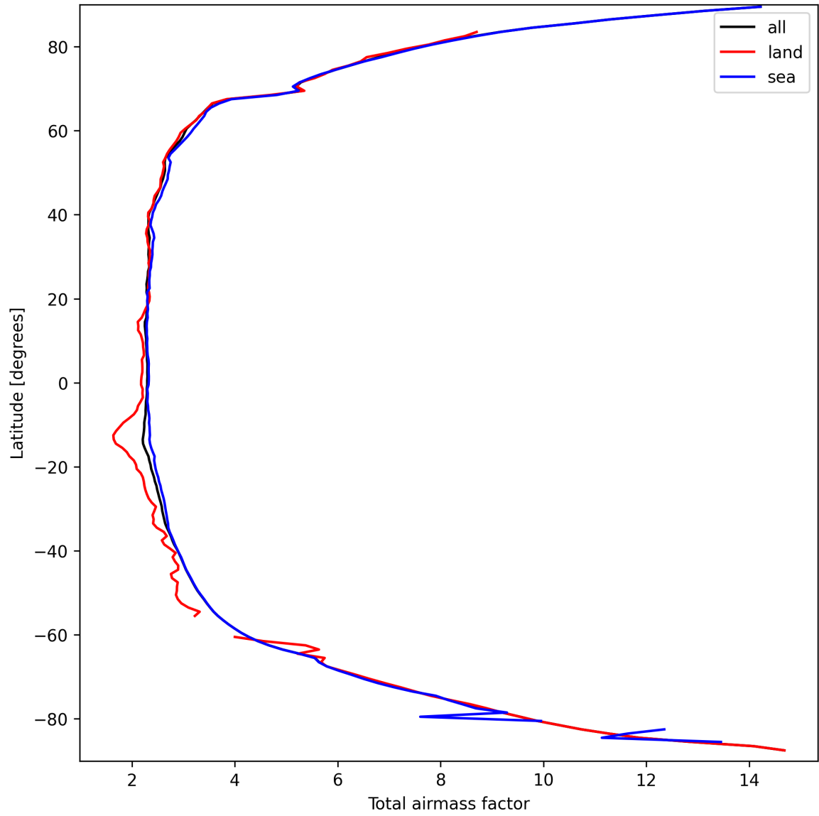
Figure 13: Zonal average of “Total airmass factor” for 2025-09-20 to 2025-09-21.
