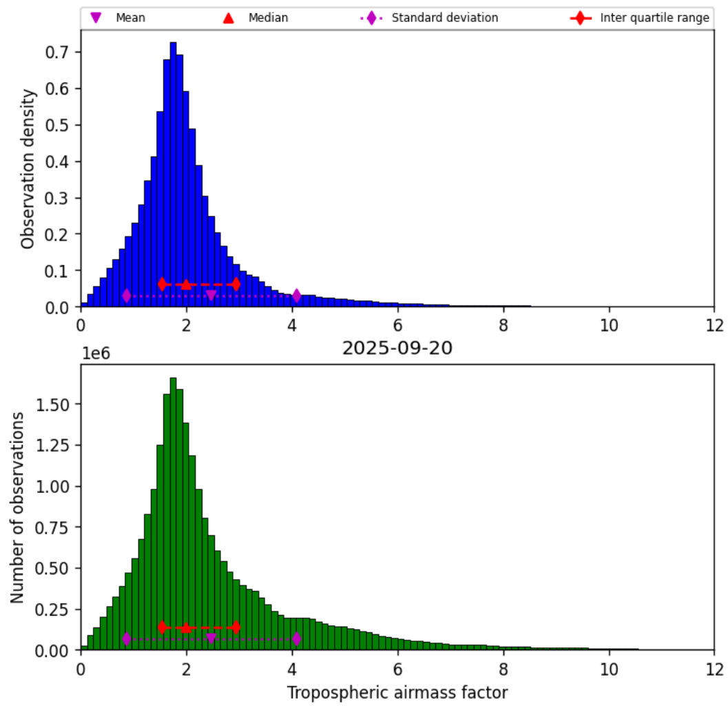
Figure 29: Histogram of “Tropospheric airmass factor” for 2025-09-20 to 2025-09-21
