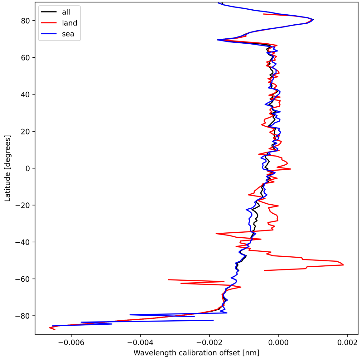
Figure 16: Zonal average of “Wavelength calibration offset” for 2025-09-20 to 2025-09-21.
