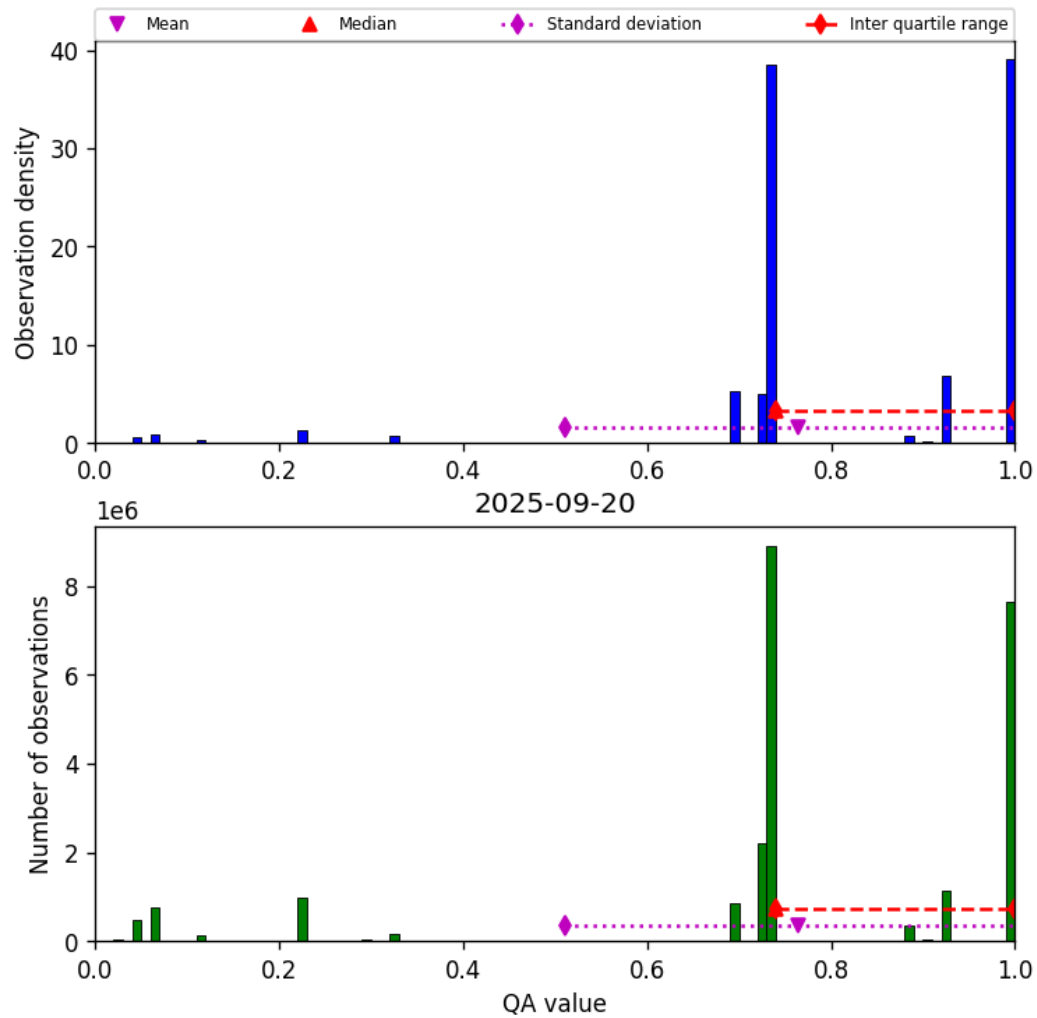
Figure 26: Histogram of “QA value” for 2025-09-20 to 2025-09-21
