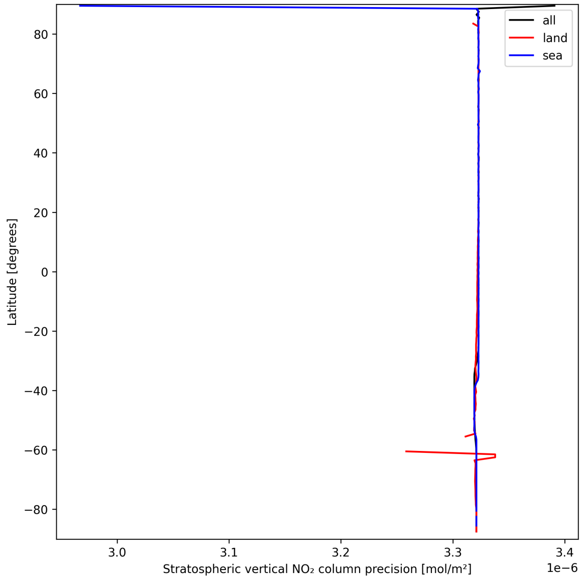
Figure 18: Zonal average of “Stratospheric vertical NO 2 column precision” for 2025-09-20 to 2025-09-21.
