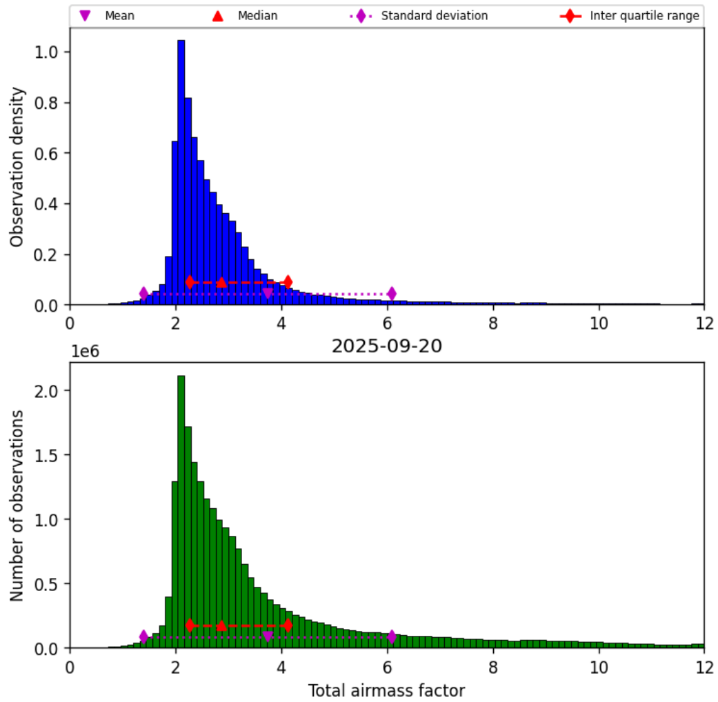
Figure 30: Histogram of “Total airmass factor” for 2025-09-20 to 2025-09-21
