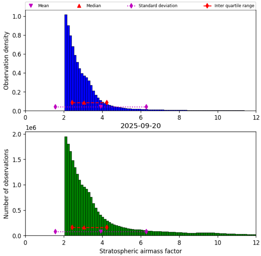
Figure 42: Histogram of “Stratospheric airmass factor” for 2025-09-20 to 2025-09-21
