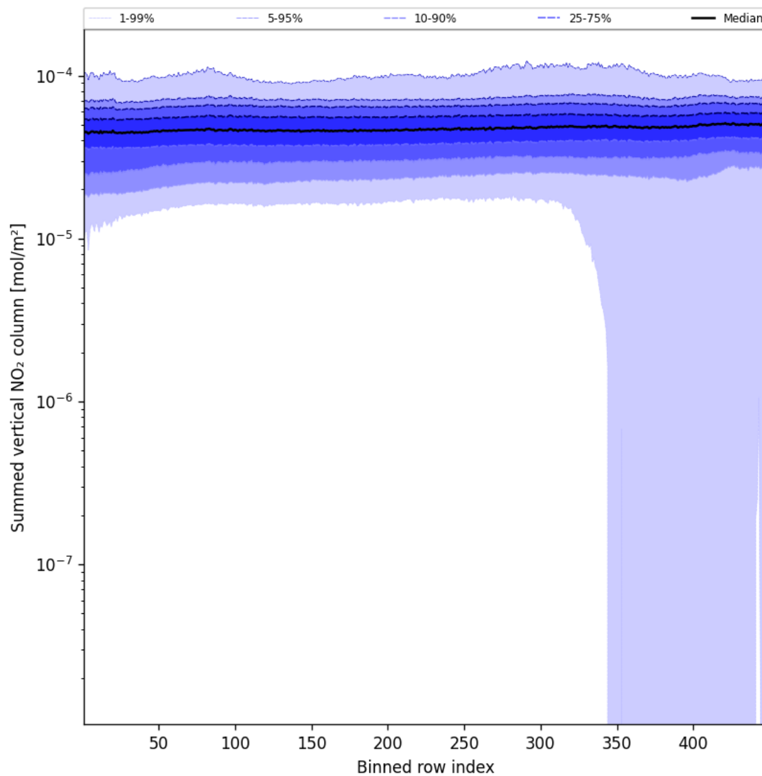
Figure 55: Along track statistics of “Summed vertical NO 2 column” for 2025-09-20 to 2025-09-21
