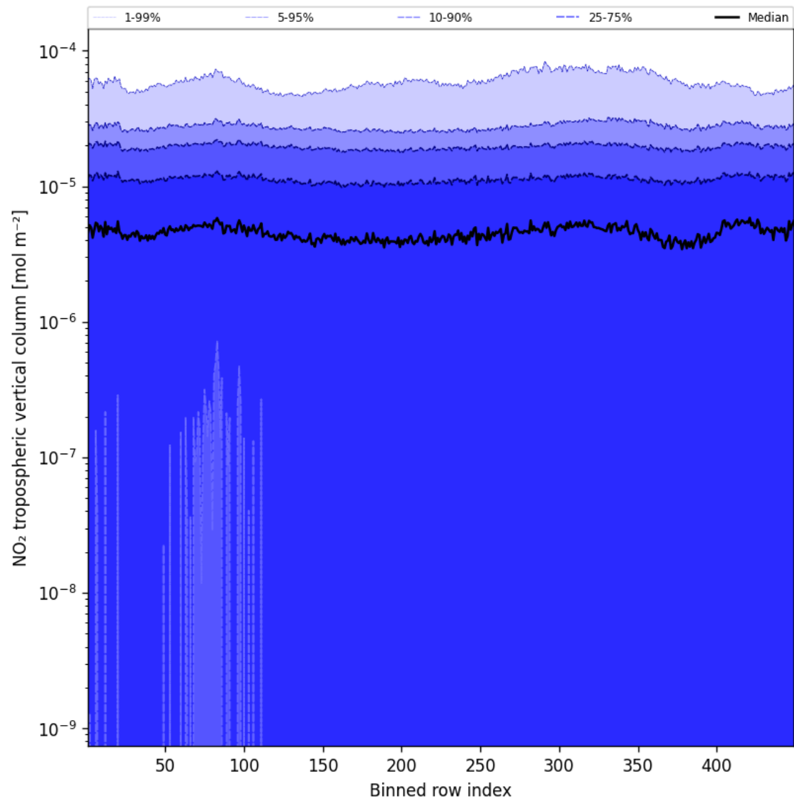
Figure 44: Along track statistics of "NO 2 tropospheric vertical column" for 2025-09-20 to 2025-09-21
