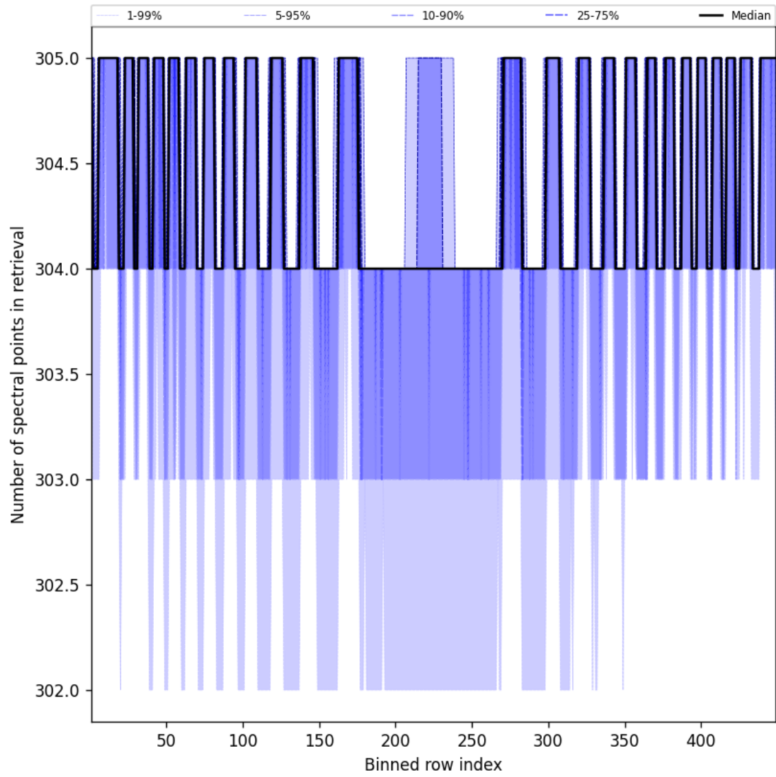
Figure 48: Along track statistics of “Number of spectral points in retrieval” for 2025-09-20 to 2025-09-21
