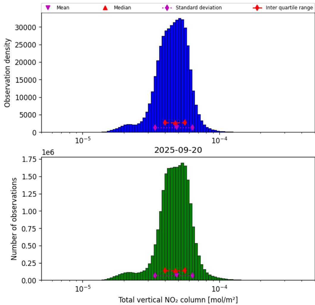
Figure 36: Histogram of “Total vertical NO 2 column” for 2025-09-20 to 2025-09-21
