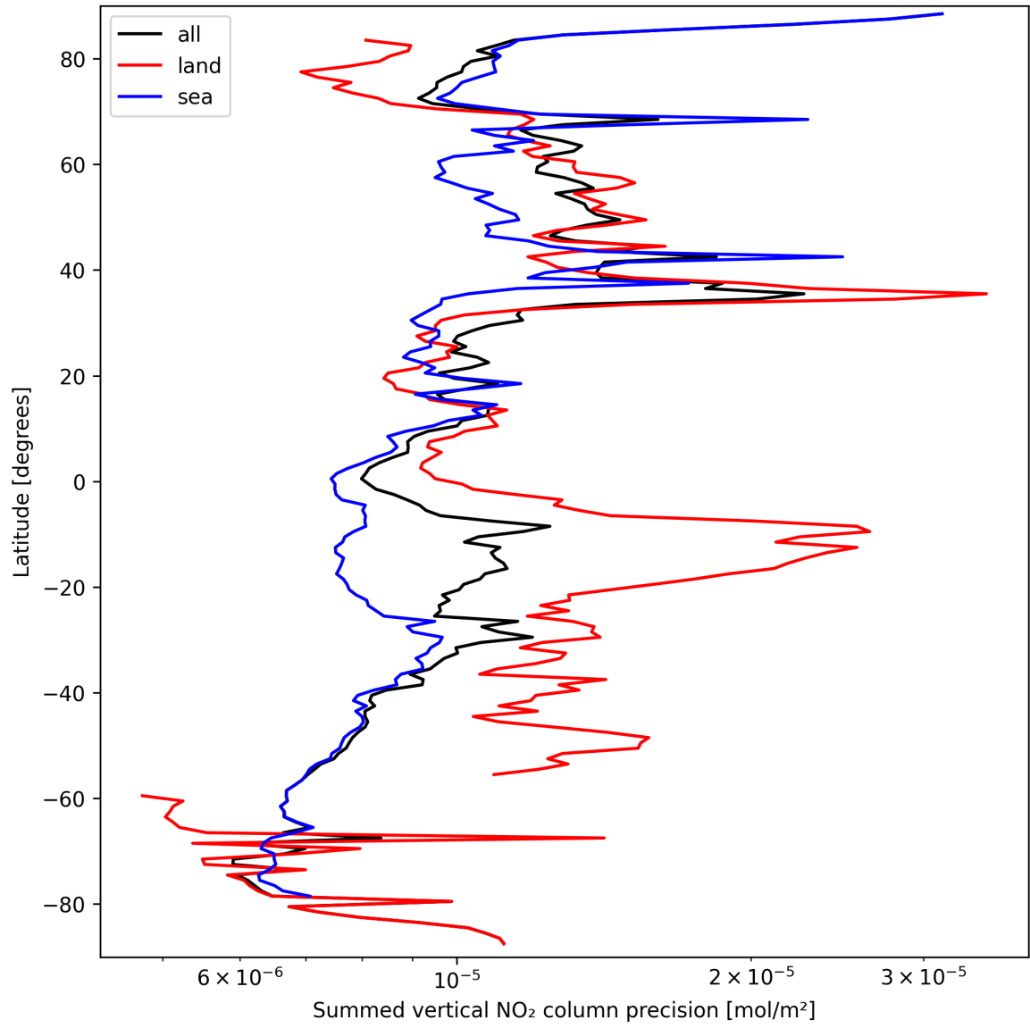
Figure 22: Zonal average of “Summed vertical NO 2 column precision” for 2025-09-21 to 2025-09-22.
