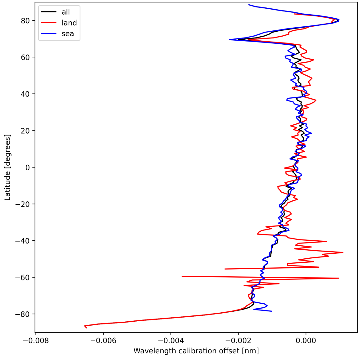
Figure 16: Zonal average of “Wavelength calibration offset” for 2025-09-21 to 2025-09-22.
