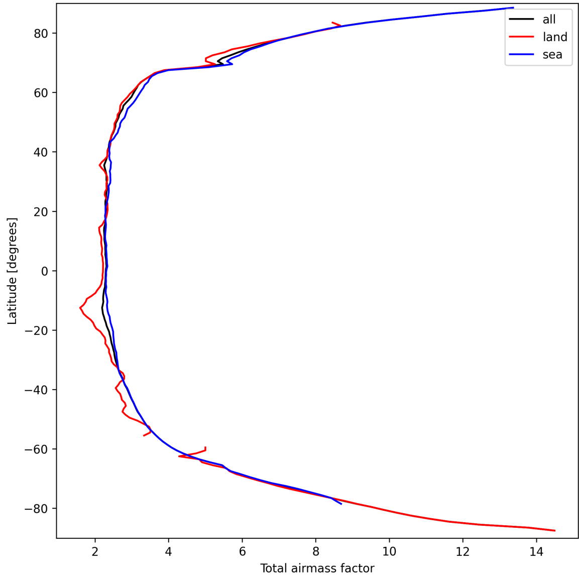
Figure 13: Zonal average of “Total airmass factor” for 2025-09-21 to 2025-09-22.
