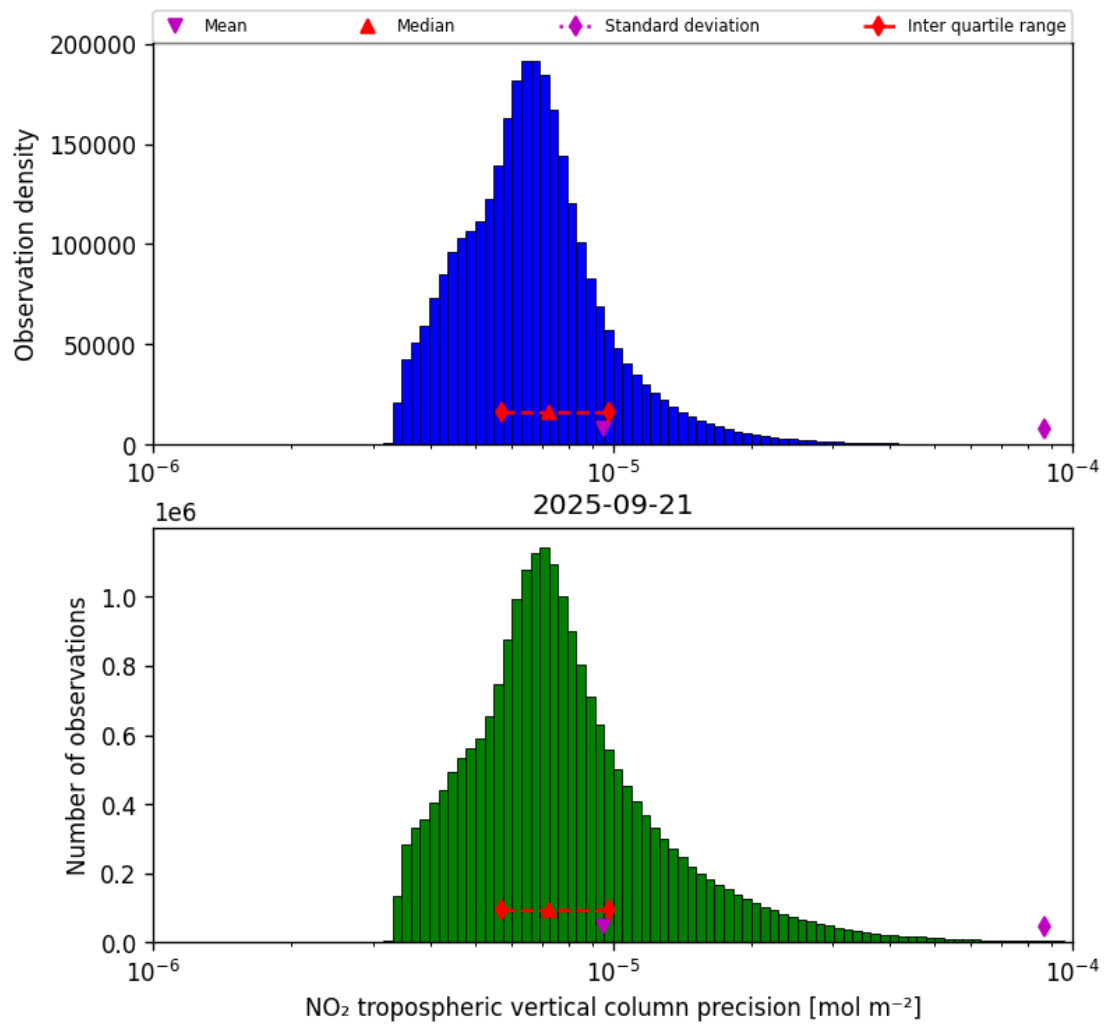
Figure 28: Histogram of “NO 2 tropospheric vertical column precision” for 2025-09-21 to 2025-09-22
