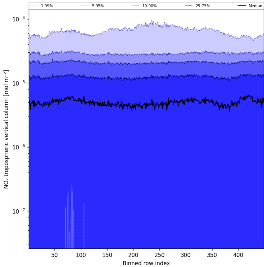
Figure 44: Along track statistics of “NO 2 tropospheric vertical column” for 2025-09-21 to 2025-09-22
