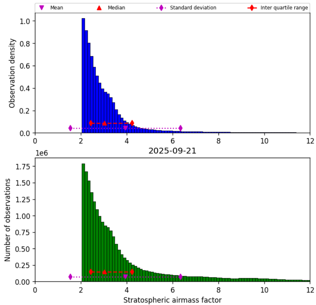
Figure 42: Histogram of “Stratospheric airmass factor” for 2025-09-21 to 2025-09-22
