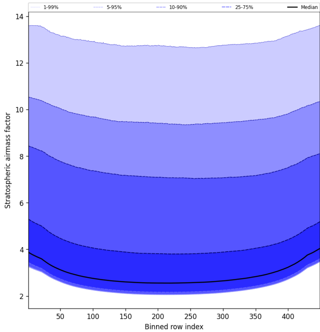
Figure 59: Along track statistics of “Stratospheric airmass factor” for 2025-09-21 to 2025-09-22
