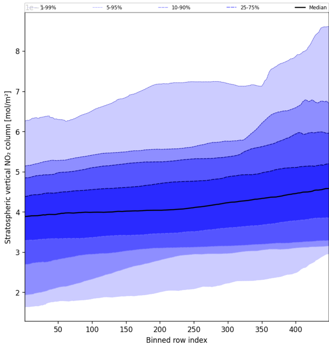
Figure 51: Along track statistics of “Stratospheric vertical NO 2 column” for 2025-09-21 to 2025-09-22
