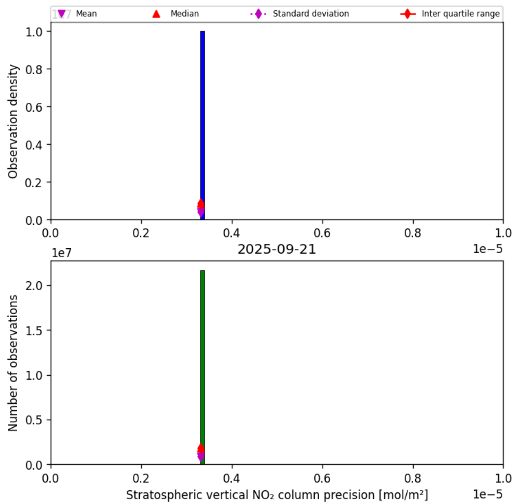
Figure 35: Histogram of “Stratospheric vertical NO 2 column precision” for 2025-09-21 to 2025-09-22
