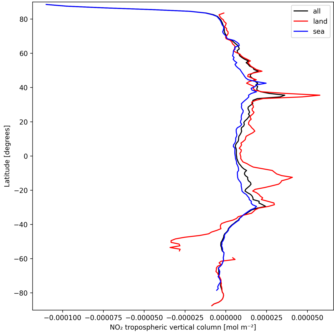
Figure 10: Zonal average of “NO 2 tropospheric vertical column” for 2025-09-21 to 2025-09-22.
