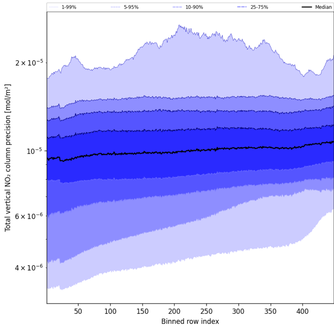
Figure 54: Along track statistics of “Total vertical NO 2 column precision” for 2025-09-21 to 2025-09-22
