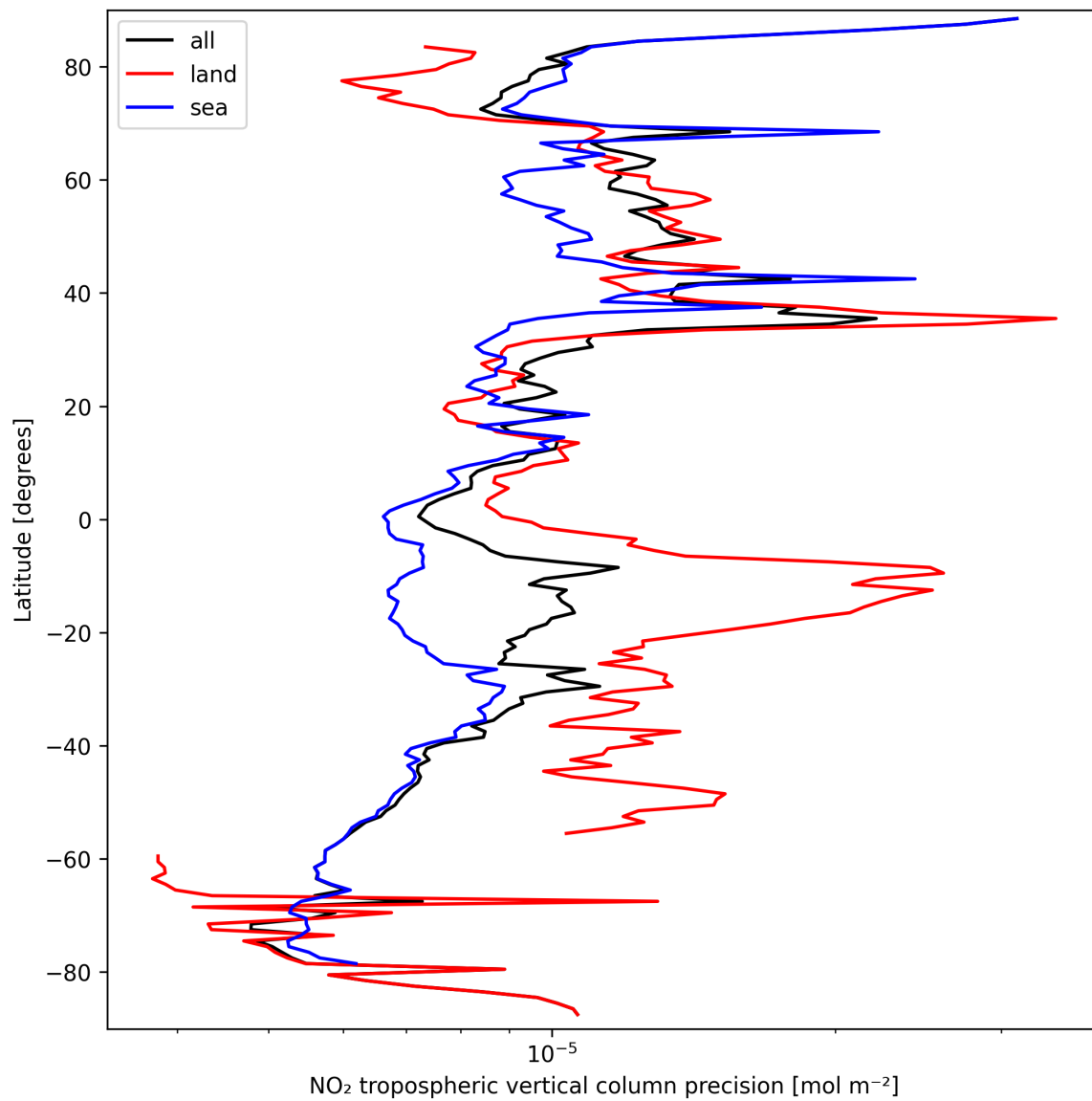
Figure 11: Zonal average of “NO 2 tropospheric vertical column precision” for 2025-09-21 to 2025-09-22.
