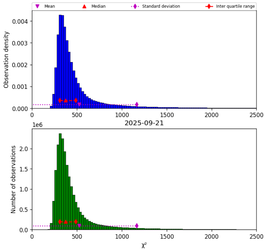
Figure 40: Histogram of “ \chi^2 ” for 2025-09-21 to 2025-09-22
