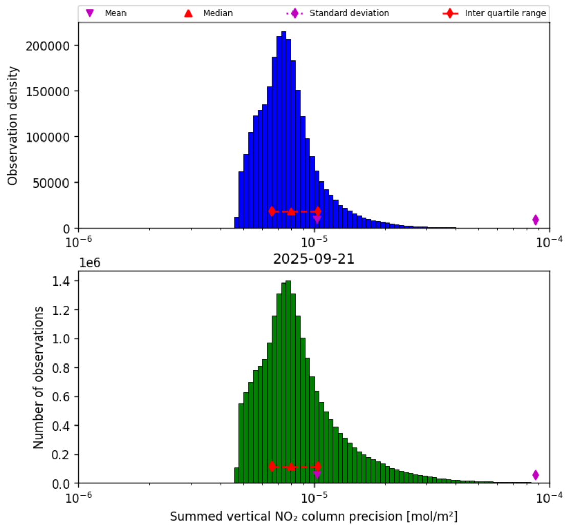
Figure 39: Histogram of “Summed vertical NO 2 column precision” for 2025-09-21 to 2025-09-22
