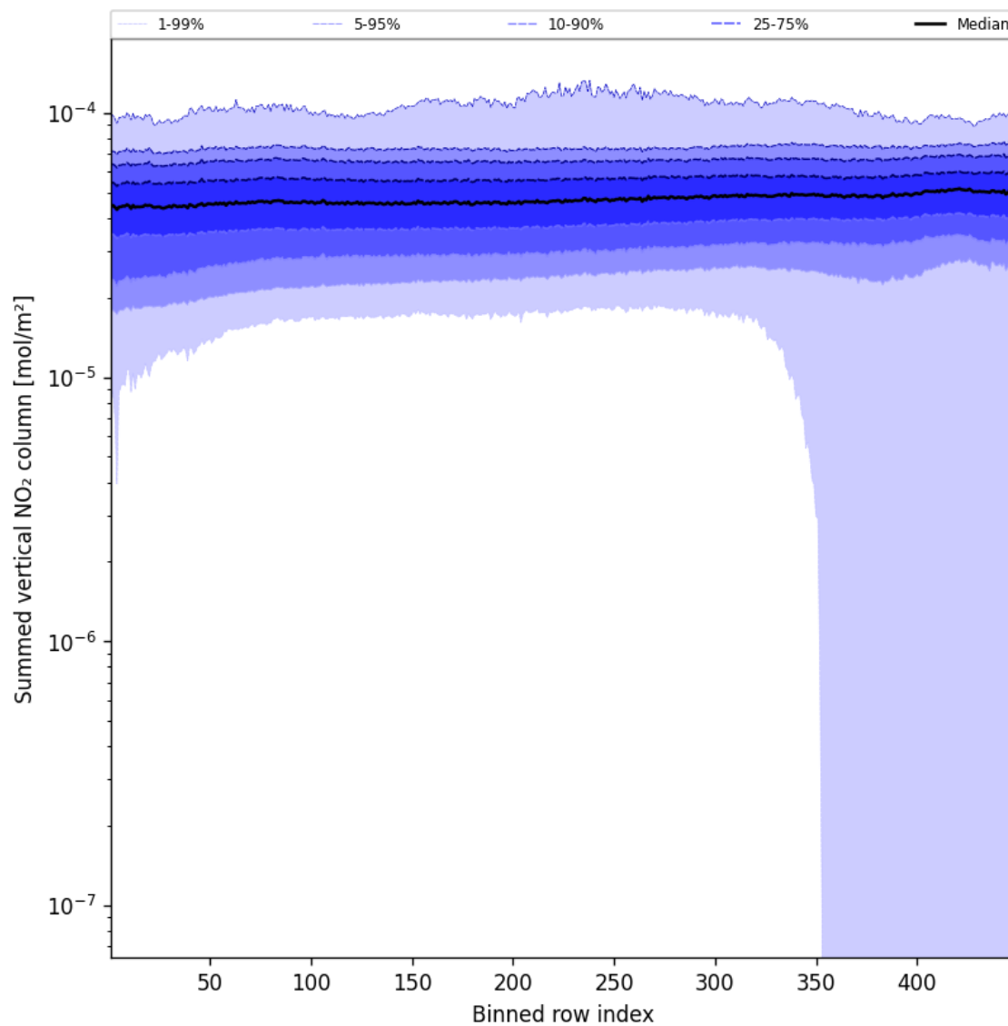
Figure 55: Along track statistics of “Summed vertical NO 2 column” for 2025-09-21 to 2025-09-22
