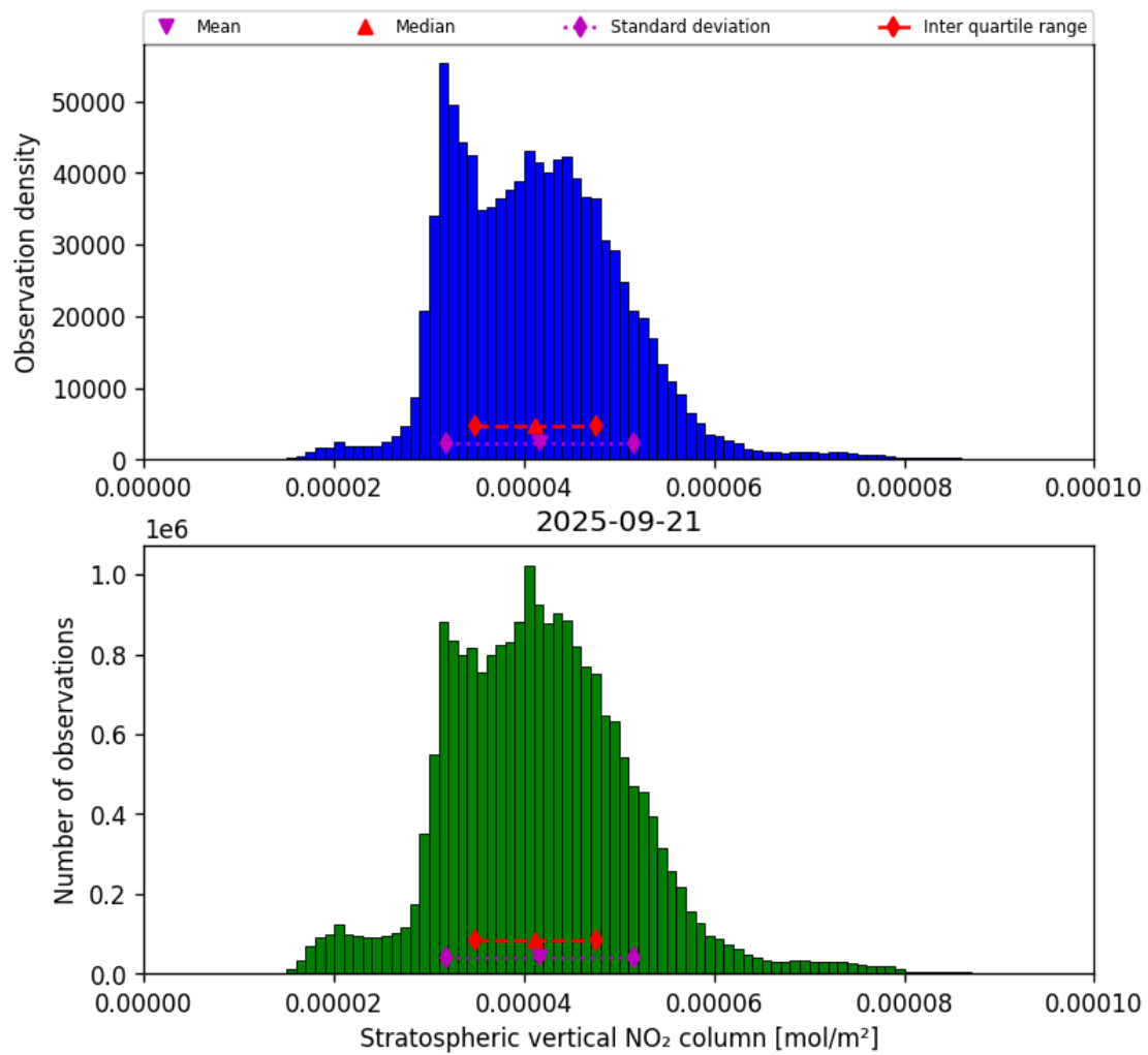
Figure 34: Histogram of “Stratospheric vertical NO 2 column” for 2025-09-21 to 2025-09-22
