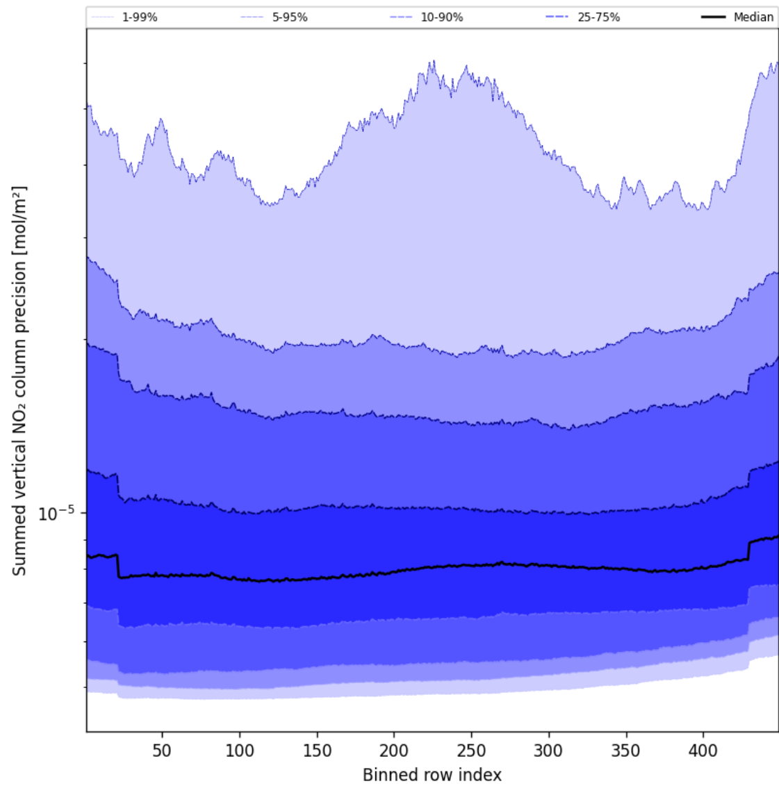
Figure 56: Along track statistics of “Summed vertical NO 2 column precision” for 2025-09-21 to 2025-09-22
