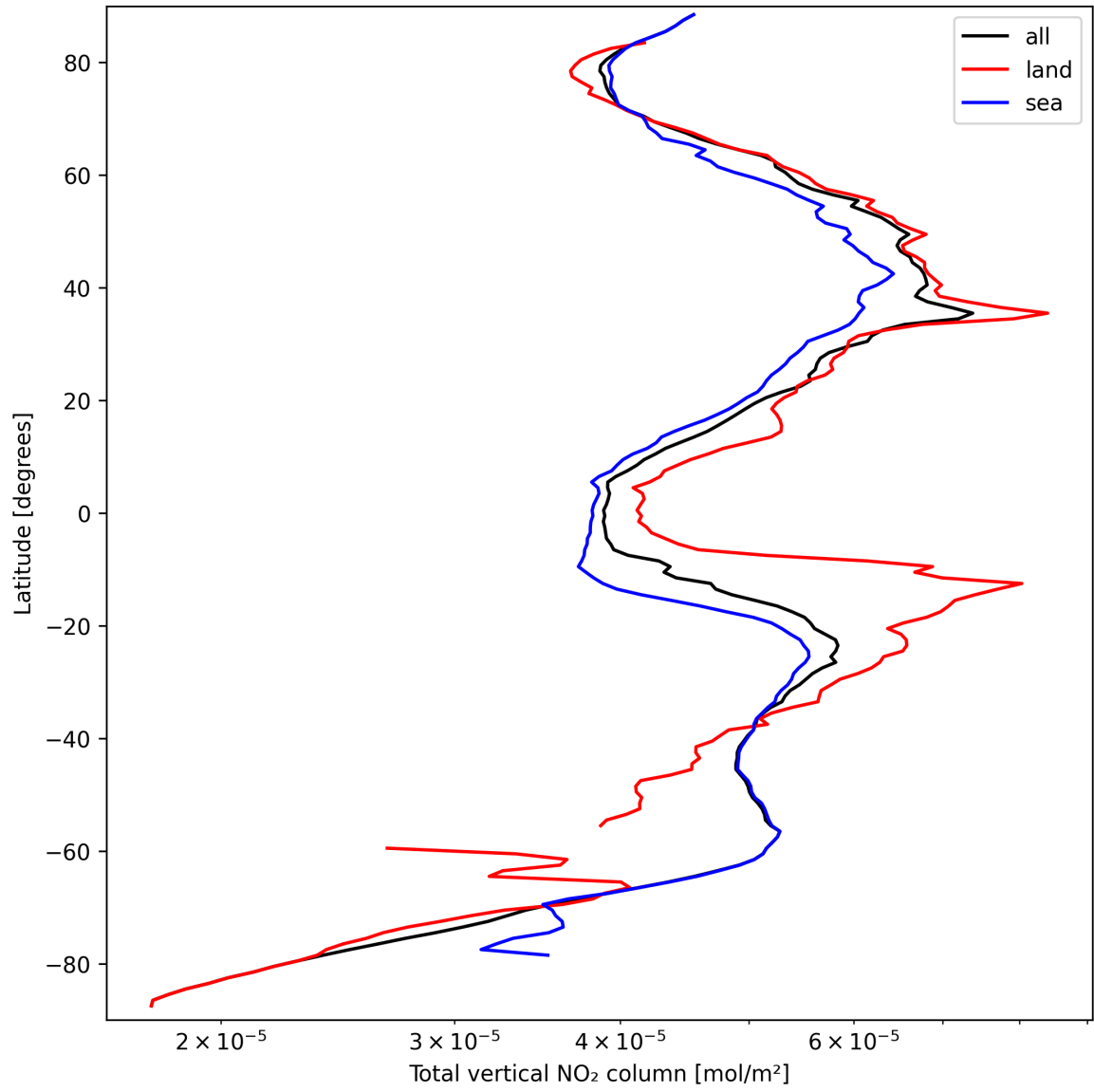
Figure 19: Zonal average of “Total vertical NO 2 column” for 2025-09-21 to 2025-09-22.
