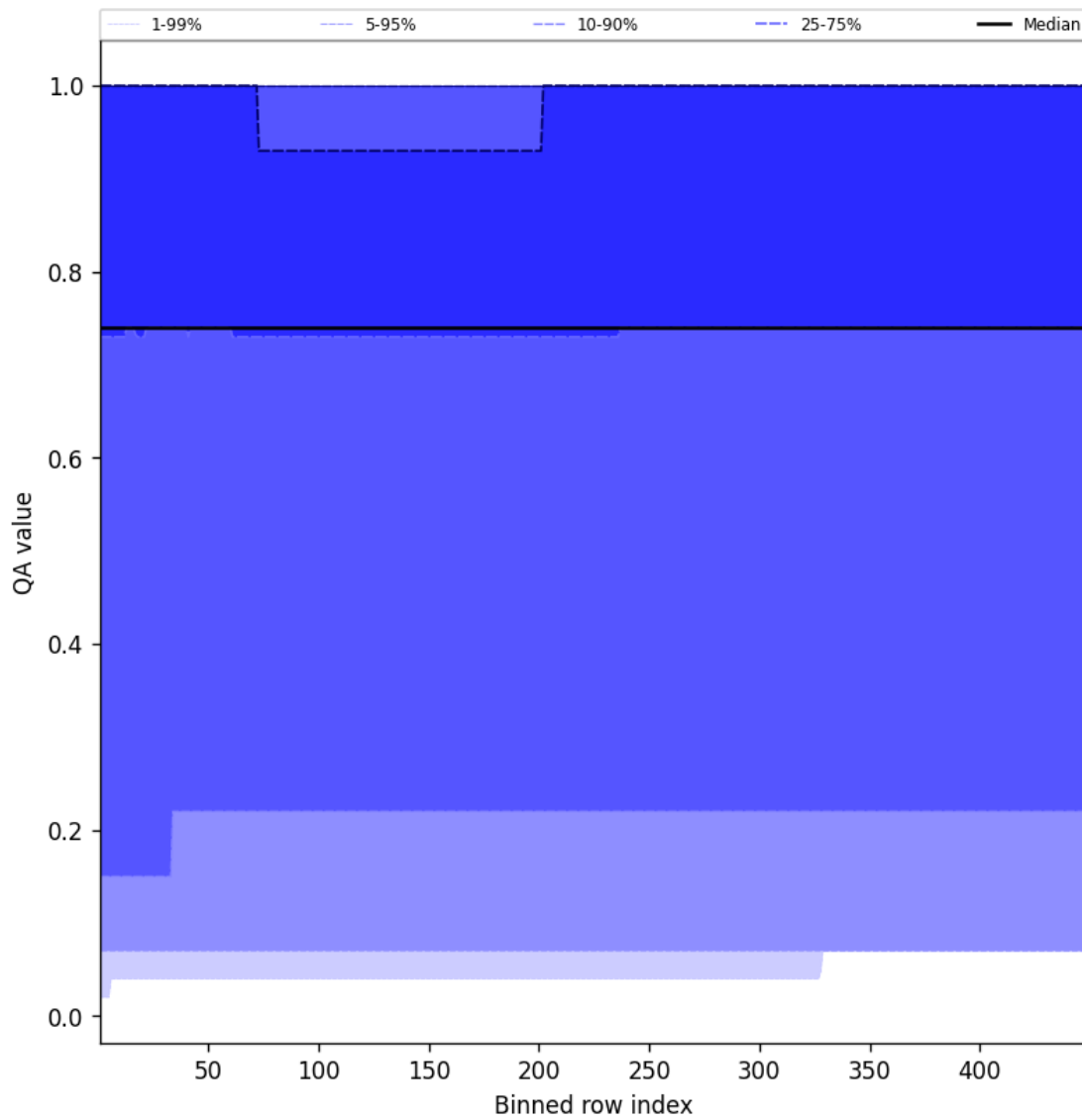
Figure 43: Along track statistics of “QA value” for 2025-09-21 to 2025-09-22
