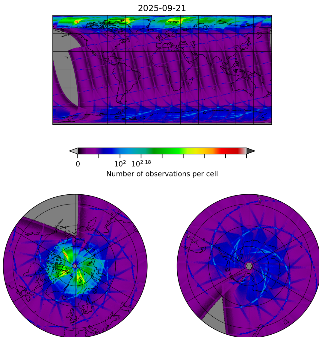
Figure 8: Map of the number of observations for 2025-09-21 to 2025-09-22
