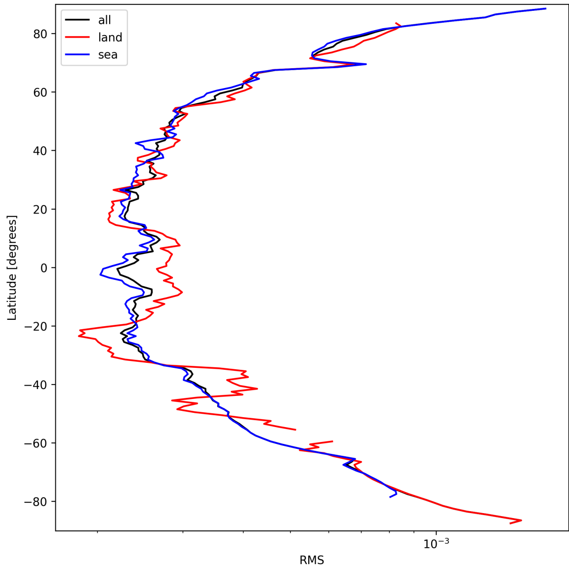
Figure 24: Zonal average of “RMS” for 2025-09-21 to 2025-09-22.
