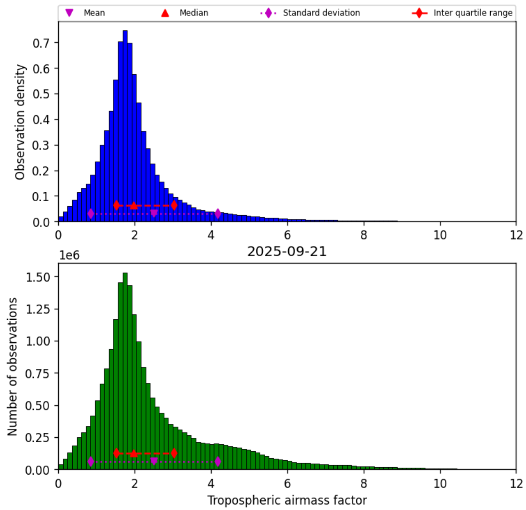
Figure 29: Histogram of “Tropospheric airmass factor” for 2025-09-21 to 2025-09-22
