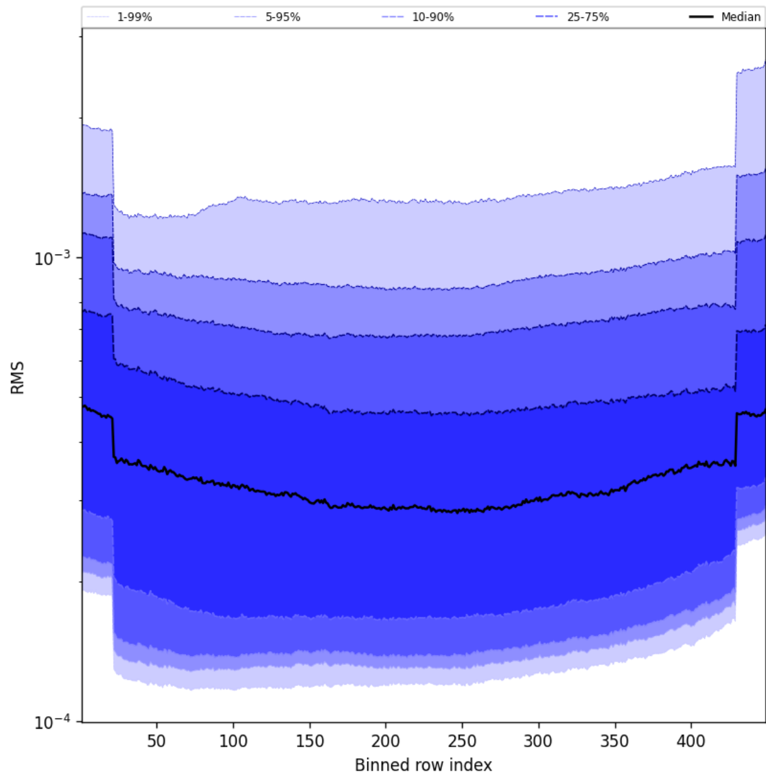
Figure 58: Along track statistics of “RMS” for 2025-09-21 to 2025-09-22
