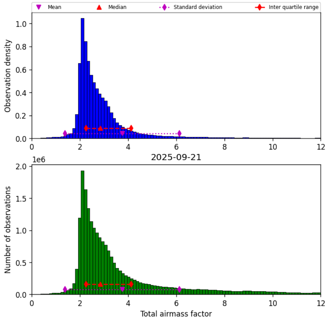
Figure 30: Histogram of “Total airmass factor” for 2025-09-21 to 2025-09-22
