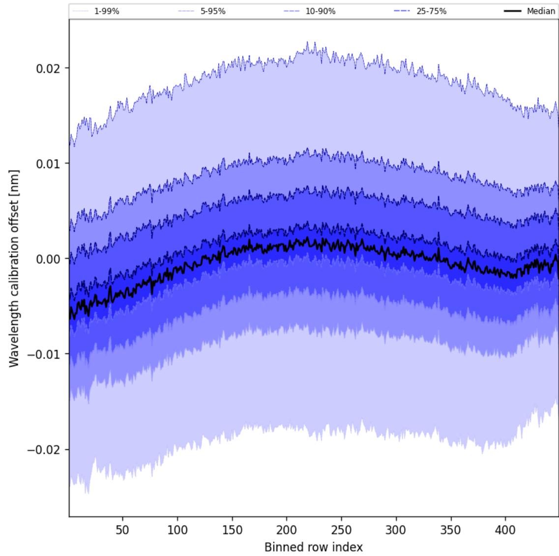
Figure 50: Along track statistics of “Wavelength calibration offset” for 2025-09-21 to 2025-09-22
