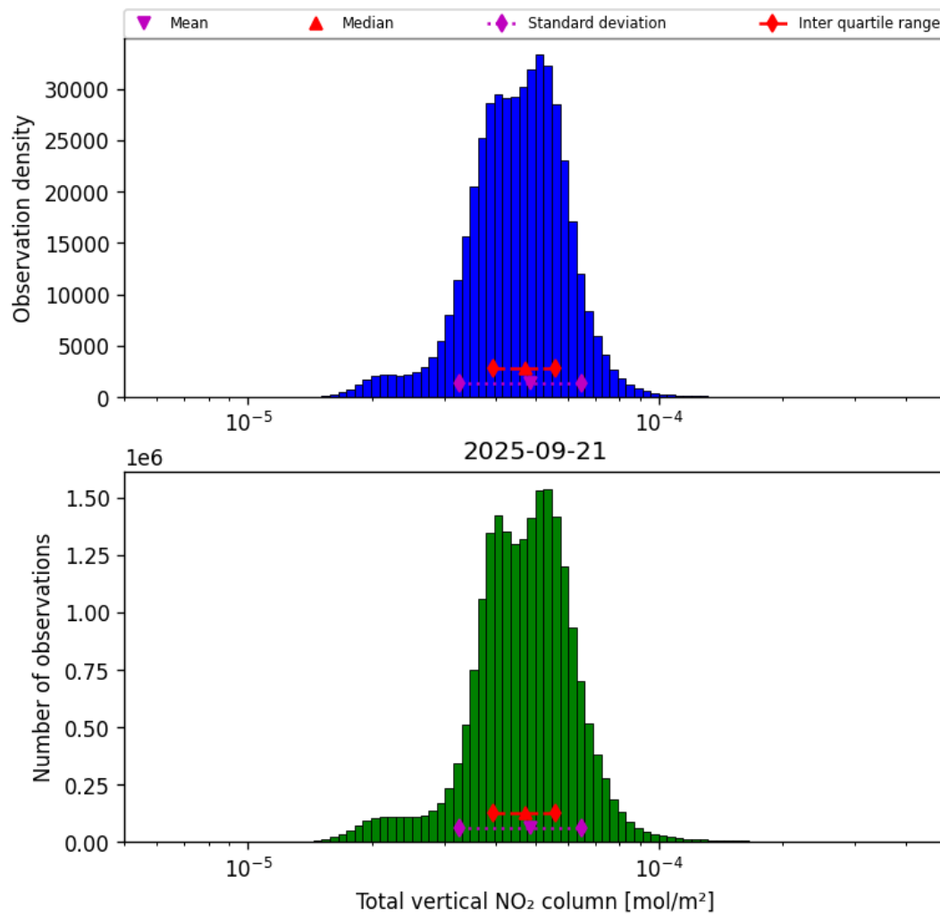
Figure 36: Histogram of “Total vertical NO 2 column” for 2025-09-21 to 2025-09-22
