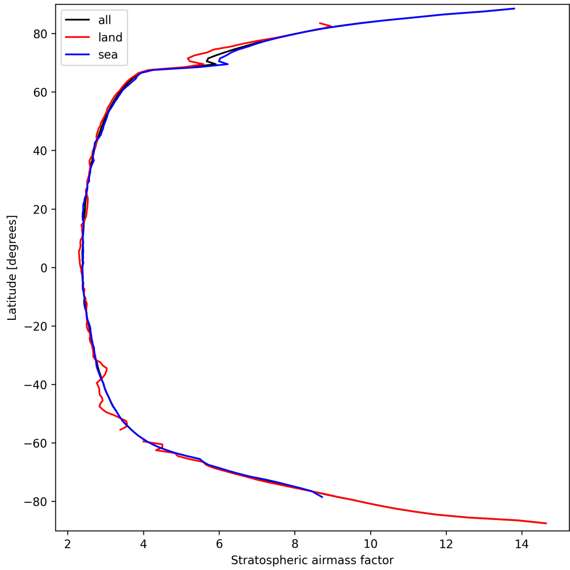
Figure 25: Zonal average of “Stratospheric airmass factor” for 2025-09-21 to 2025-09-22.
