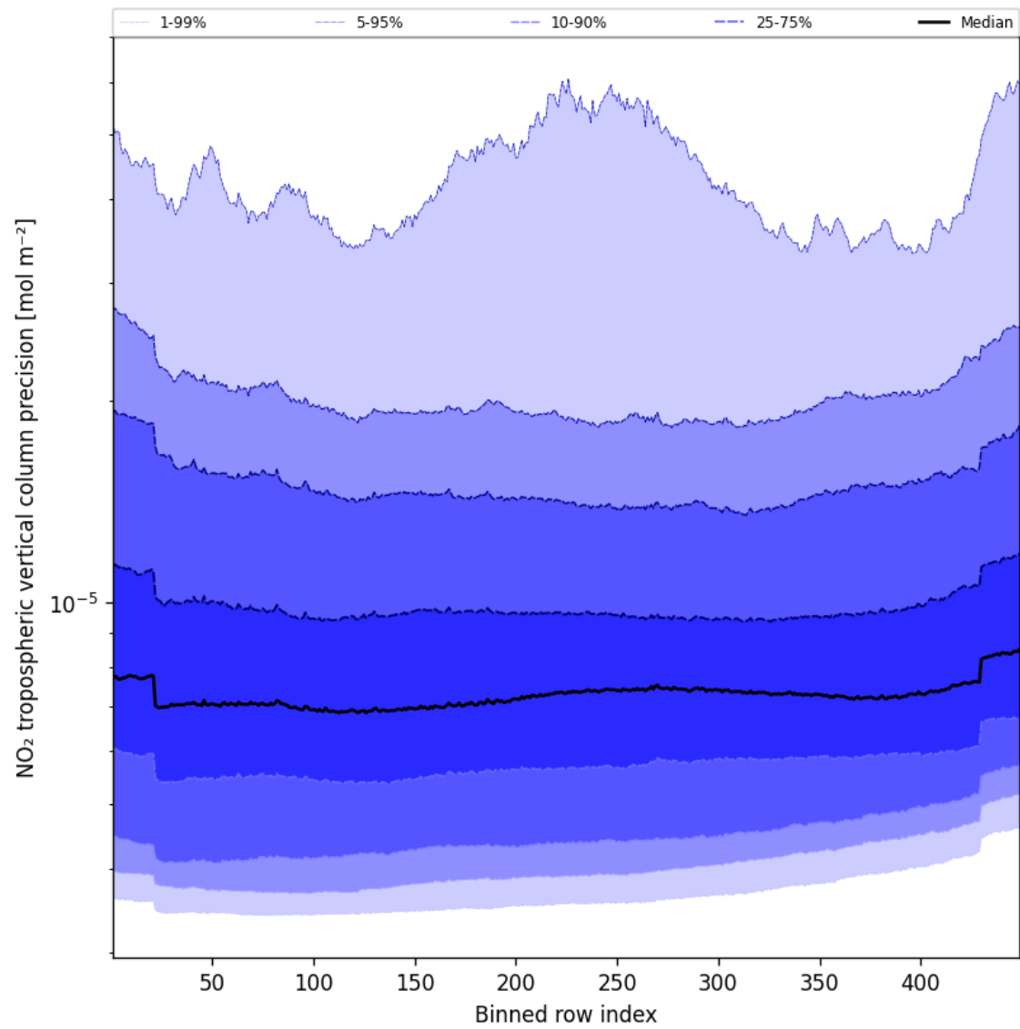
Figure 45: Along track statistics of “NO 2 tropospheric vertical column precision” for 2025-09-21 to 2025-09-22
