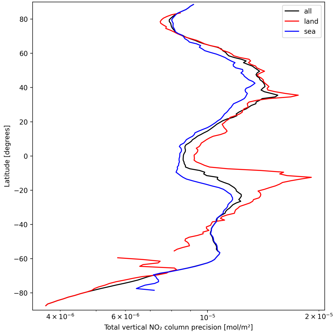
Figure 20: Zonal average of “Total vertical NO 2 column precision” for 2025-09-21 to 2025-09-22.
