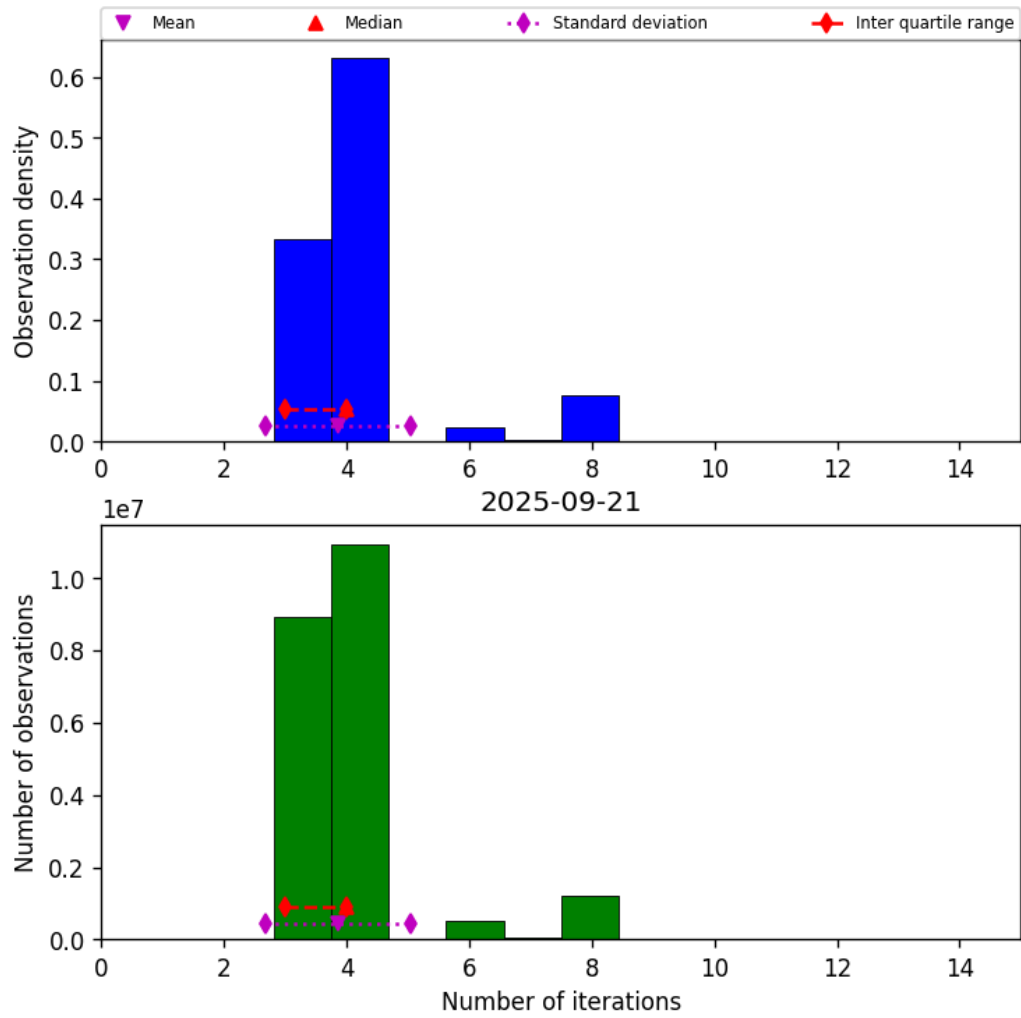
Figure 32: Histogram of “Number of iterations” for 2025-09-21 to 2025-09-22
