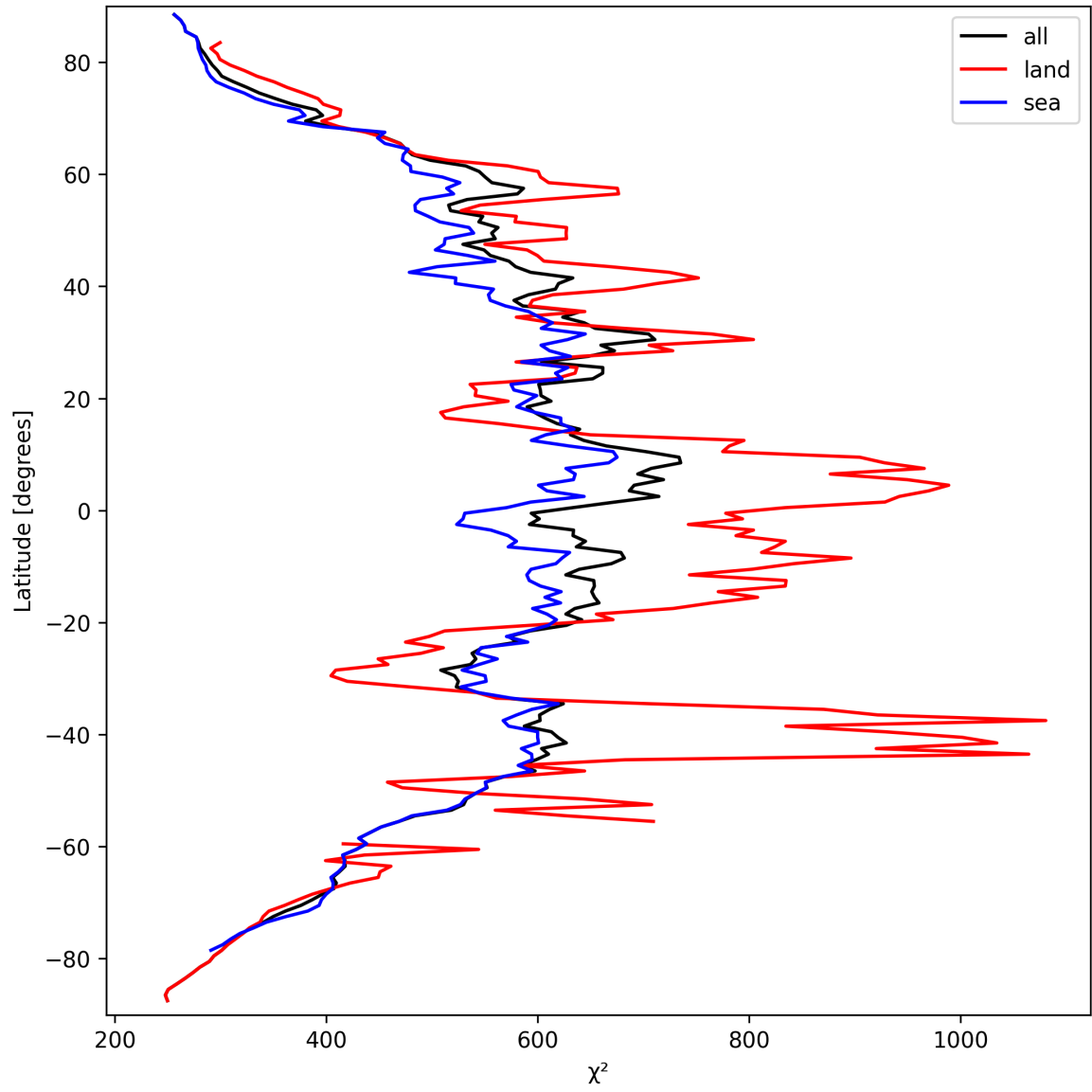
Figure 23: Zonal average of “ \chi^2 ” for 2025-09-21 to 2025-09-22.
