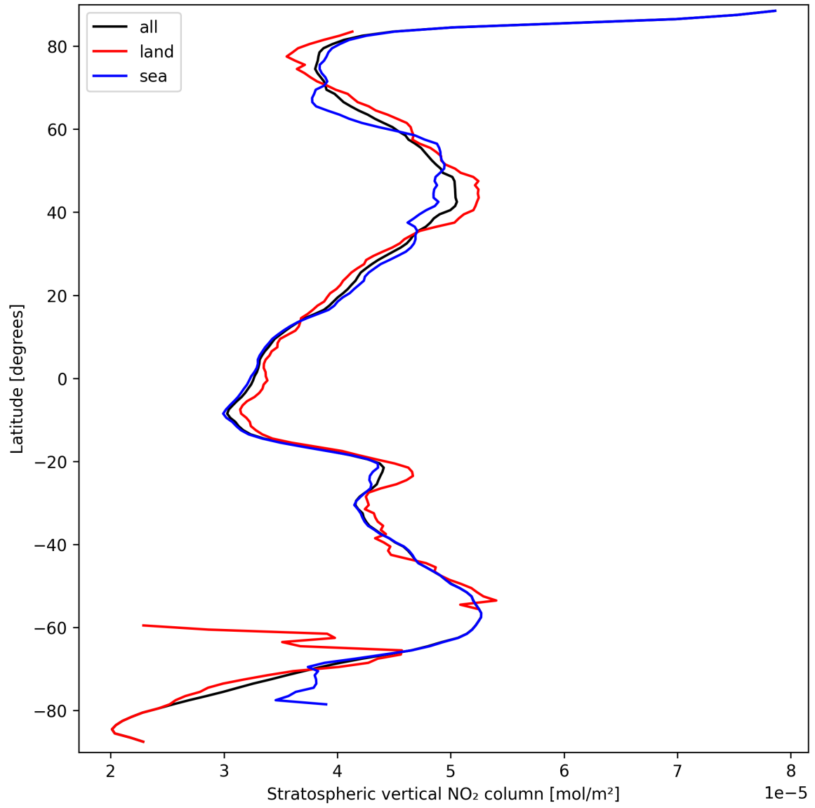
Figure 17: Zonal average of “Stratospheric vertical NO 2 column” for 2025-09-21 to 2025-09-22.
