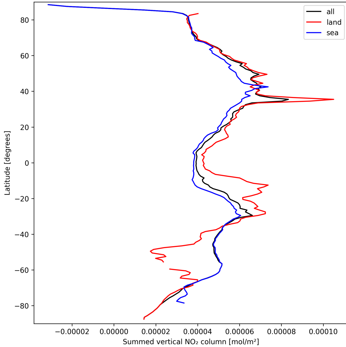
Figure 21: Zonal average of “Summed vertical NO 2 column” for 2025-09-21 to 2025-09-22.
