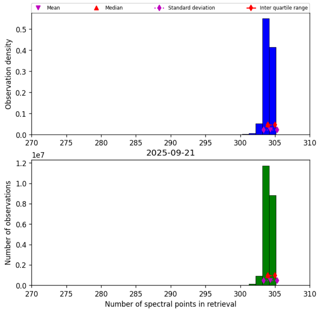
Figure 31: Histogram of “Number of spectral points in retrieval” for 2025-09-21 to 2025-09-22
