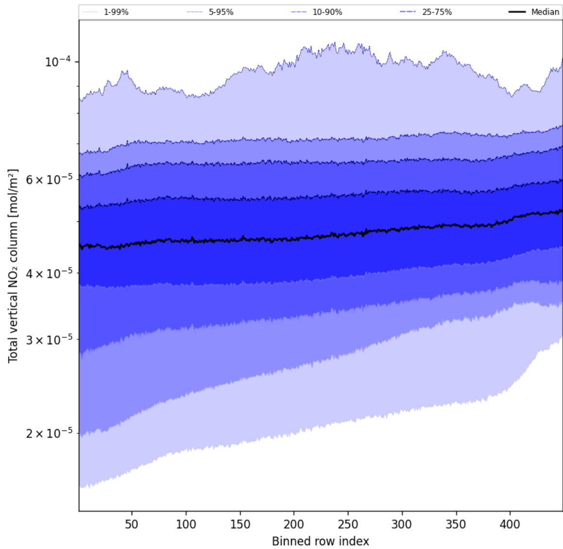
Figure 53: Along track statistics of “Total vertical NO 2 column” for 2025-09-21 to 2025-09-22
