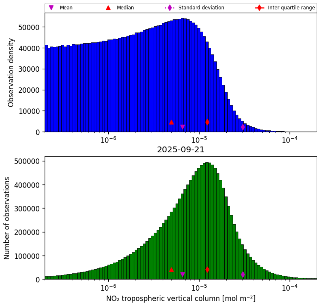
Figure 27: Histogram of “NO 2 tropospheric vertical column” for 2025-09-21 to 2025-09-22
