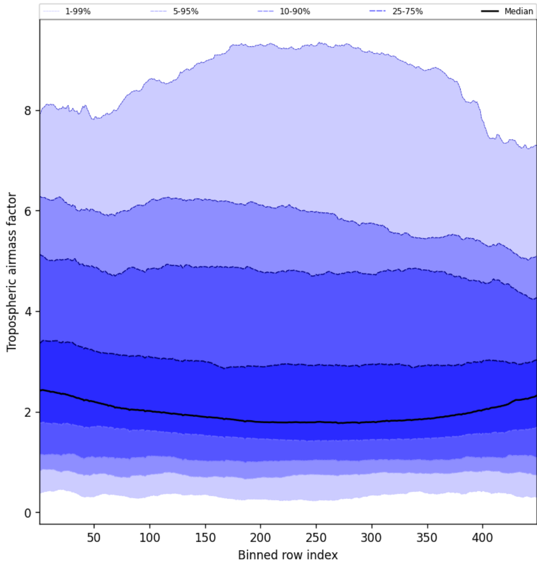
Figure 46: Along track statistics of “Tropospheric air mass factor” for 2025-09-21 to 2025-09-22
