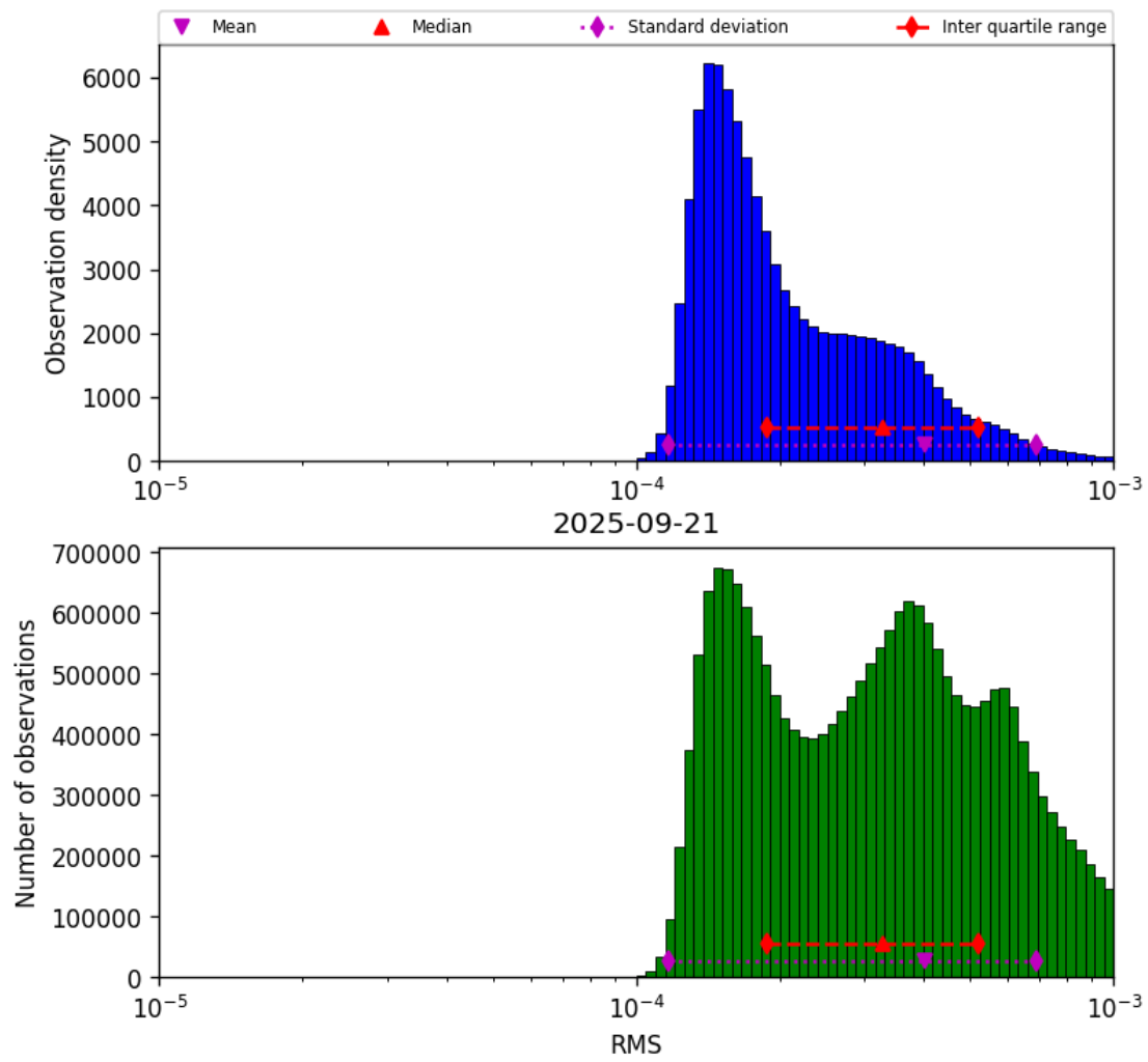
Figure 41: Histogram of “RMS” for 2025-09-21 to 2025-09-22
