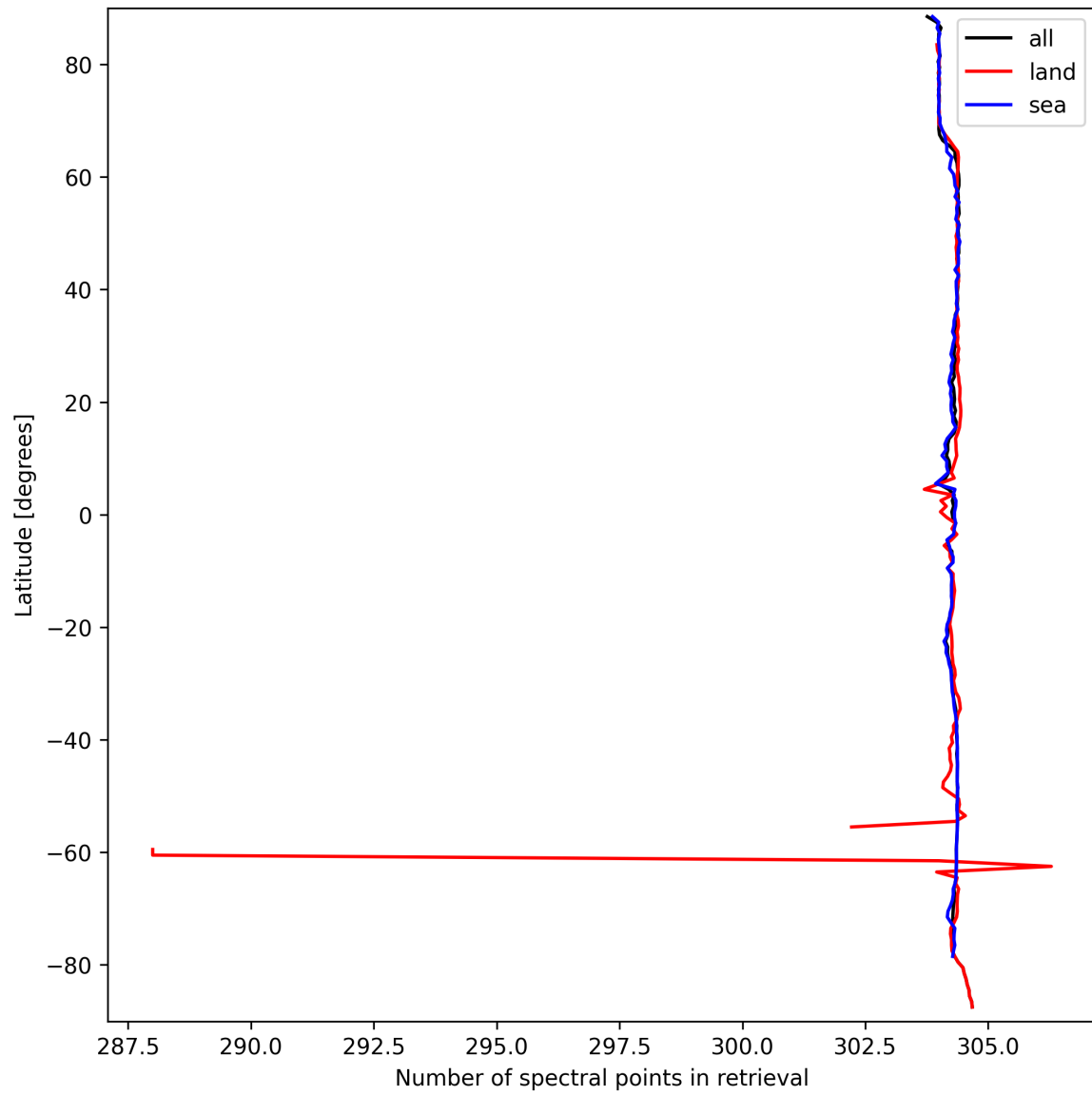
Figure 14: Zonal average of “Number of spectral points in retrieval” for 2025-09-21 to 2025-09-22.
