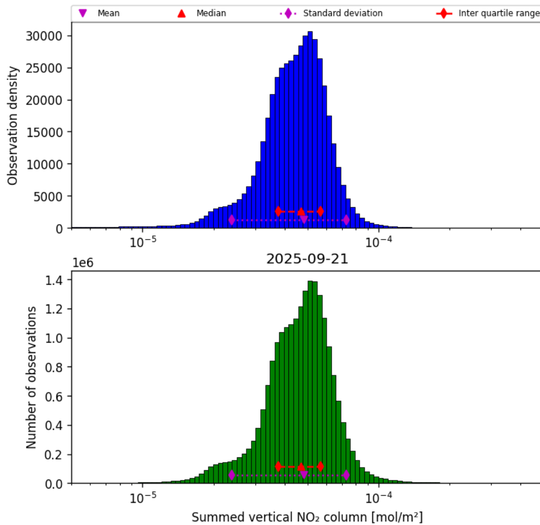
Figure 38: Histogram of "Summed vertical NO 2 column" for 2025-09-21 to 2025-09-22
