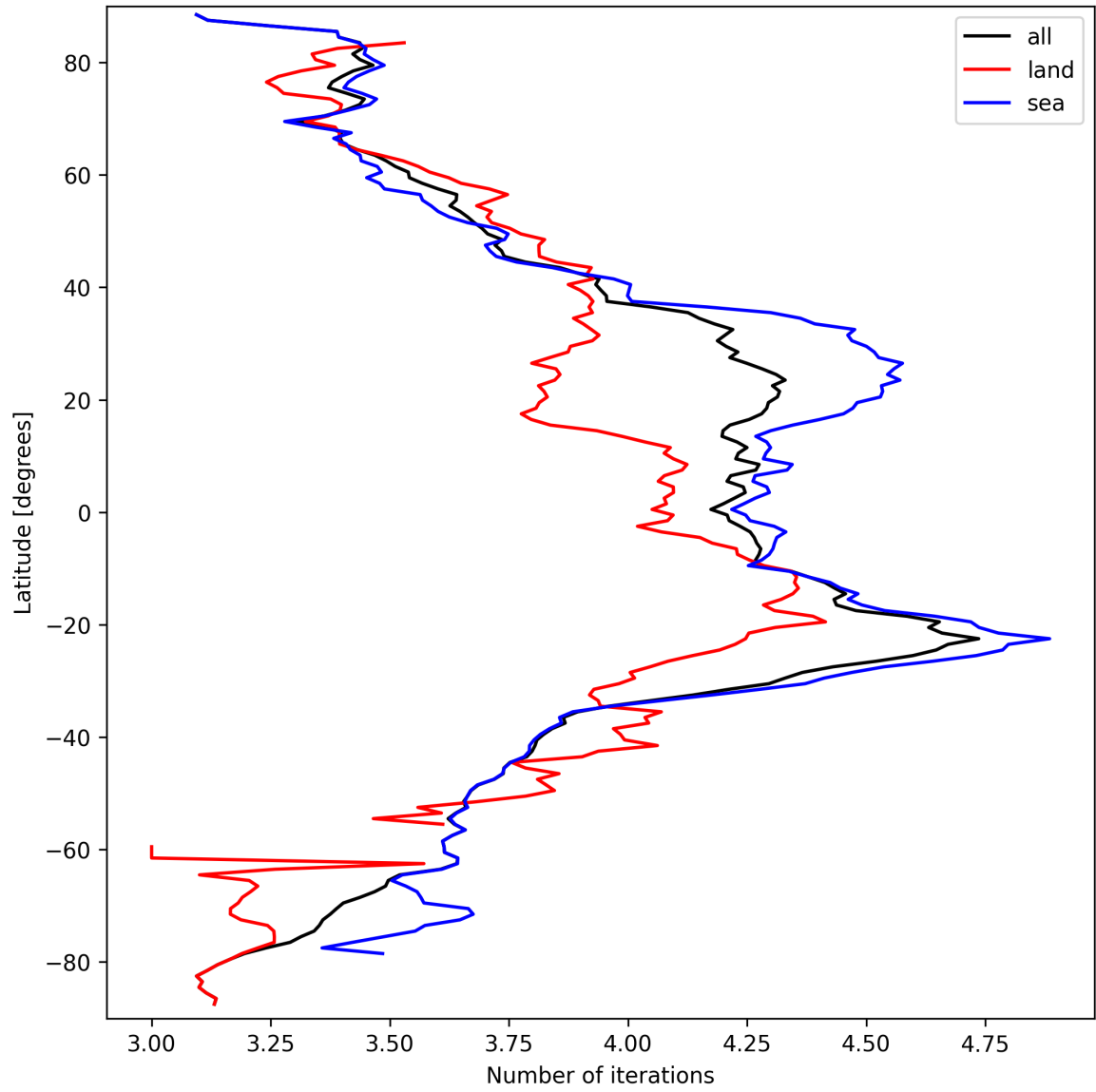
Figure 15: Zonal average of “Number of iterations” for 2025-09-21 to 2025-09-22.
