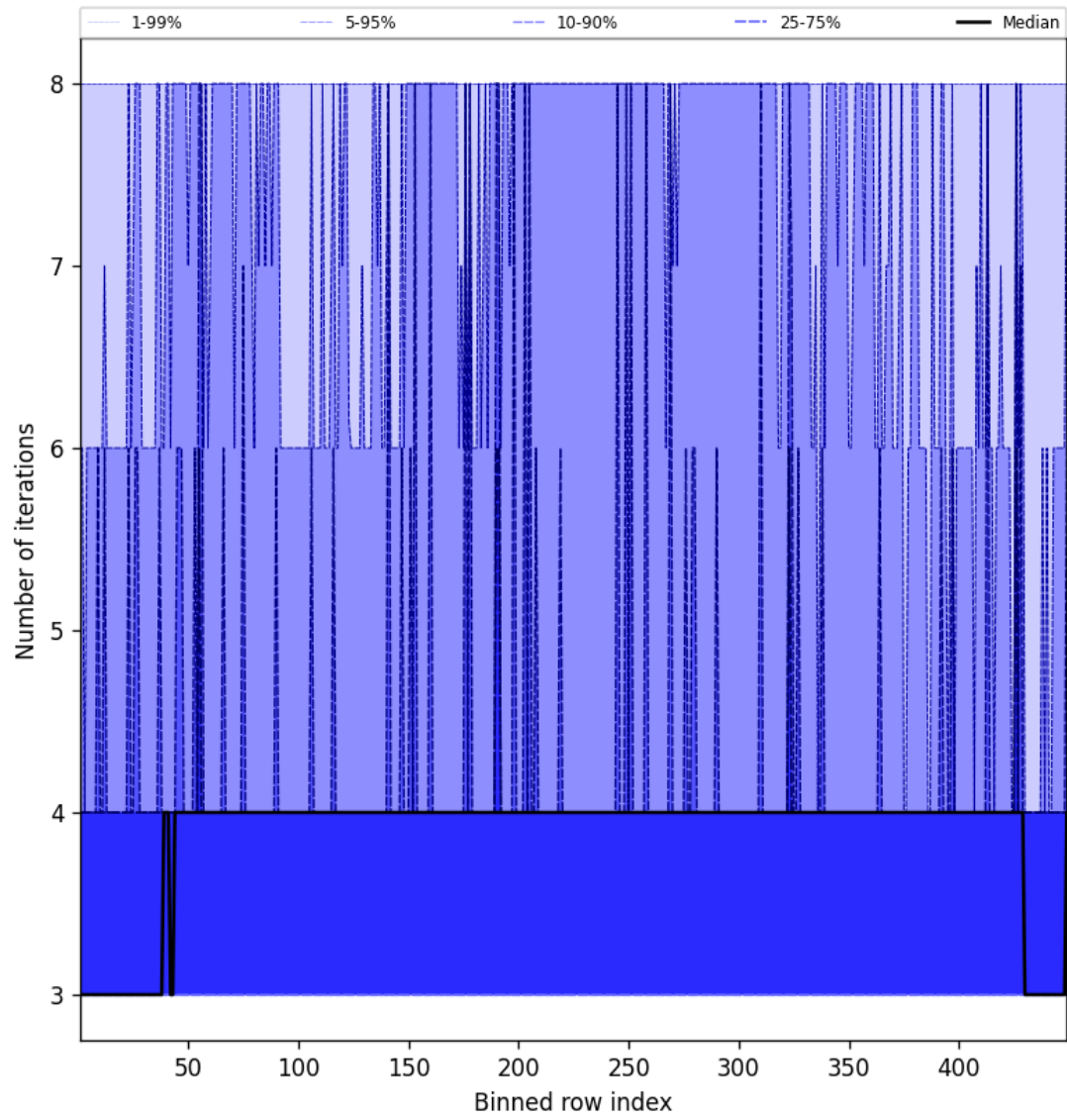
Figure 49: Along track statistics of “Number of iterations” for 2025-09-21 to 2025-09-22
