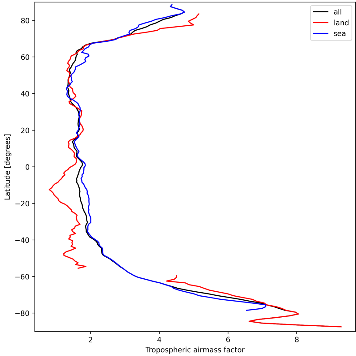
Figure 12: Zonal average of “Tropospheric airmass factor” for 2025-09-21 to 2025-09-22.
