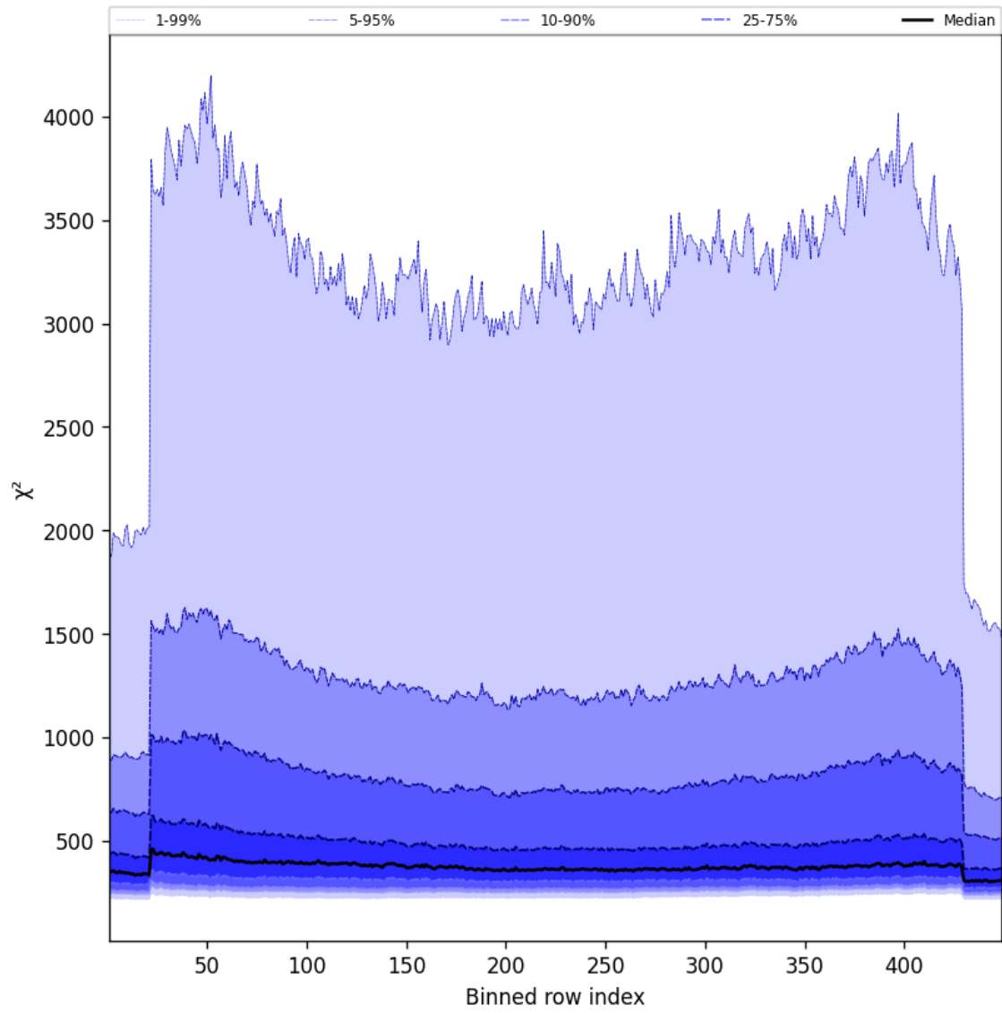
Figure 57: Along track statistics of “ \chi^2 ” for 2025-09-21 to 2025-09-22
