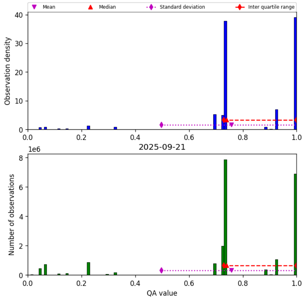
Figure 26: Histogram of “QA value” for 2025-09-21 to 2025-09-22
