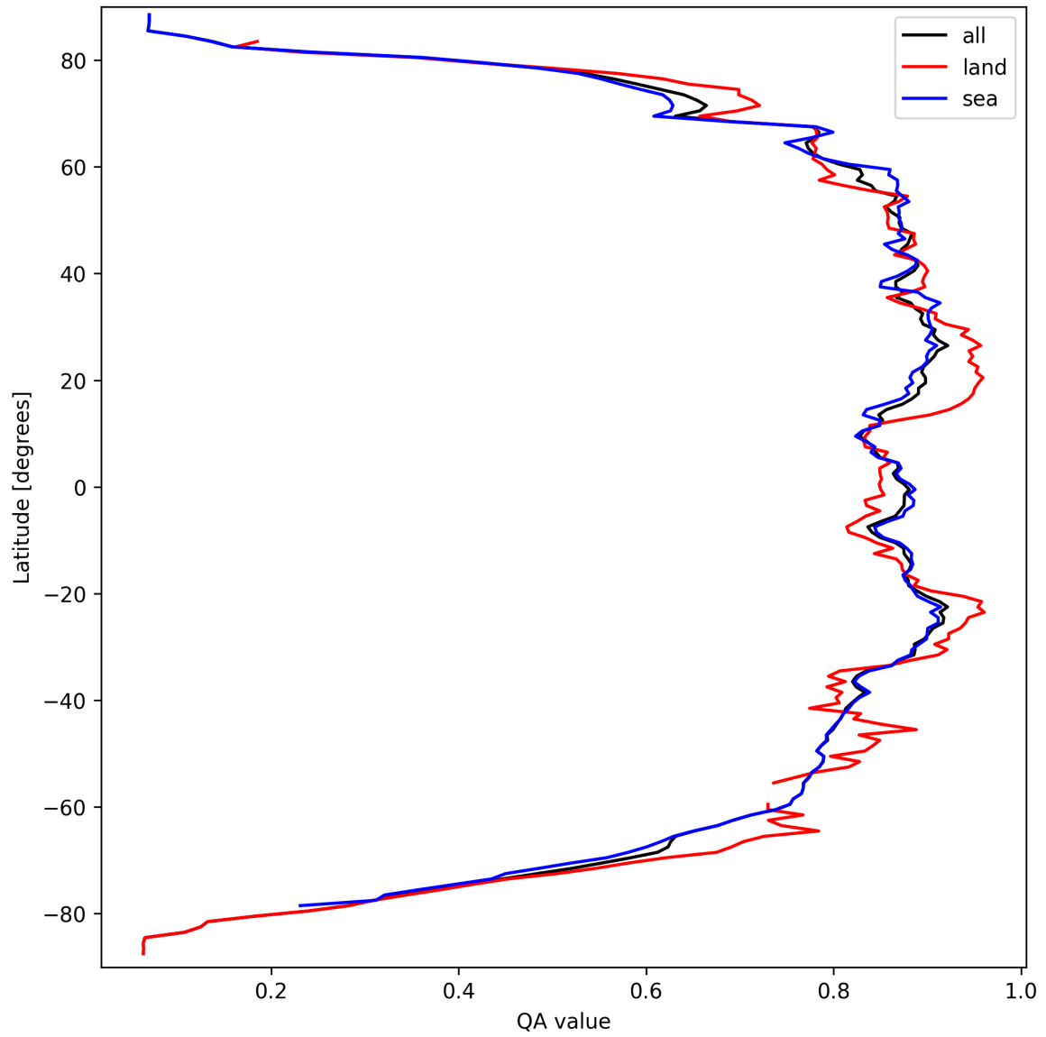
Figure 9: Zonal average of “QA value” for 2025-09-21 to 2025-09-22.
