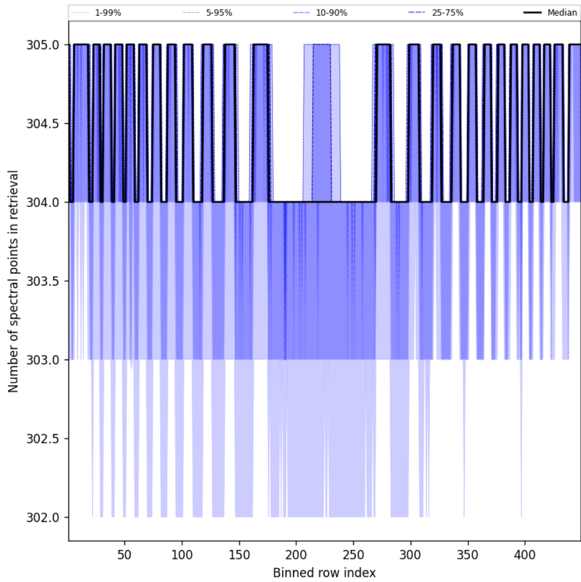
Figure 48: Along track statistics of “Number of spectral points in retrieval” for 2025-09-21 to 2025-09-22
