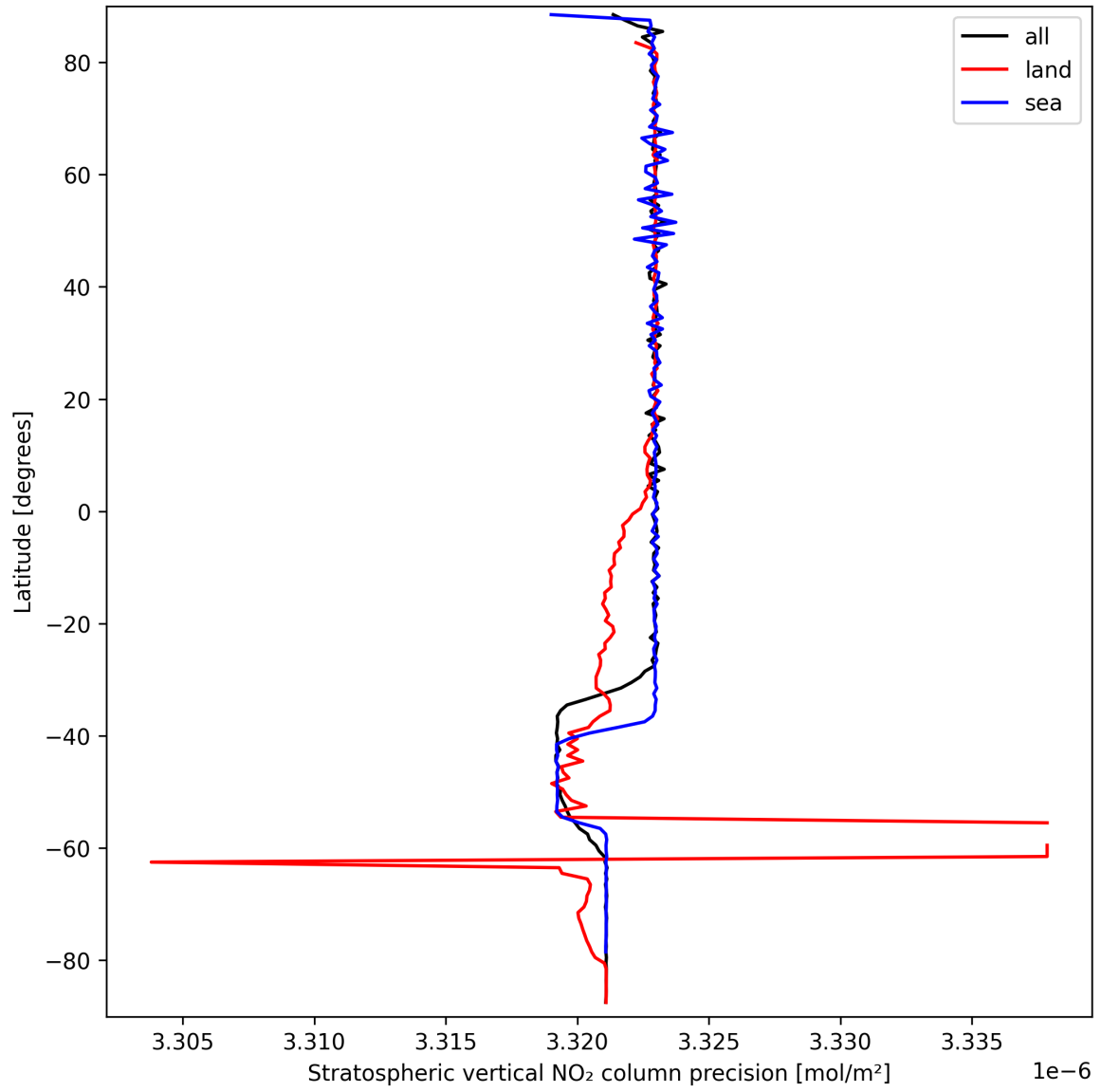
Figure 18: Zonal average of “Stratospheric vertical NO 2 column precision” for 2025-09-21 to 2025-09-22.
