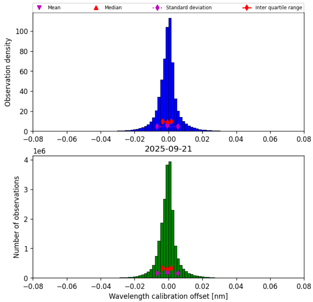
Figure 33: Histogram of “Wavelength calibration offset” for 2025-09-21 to 2025-09-22
