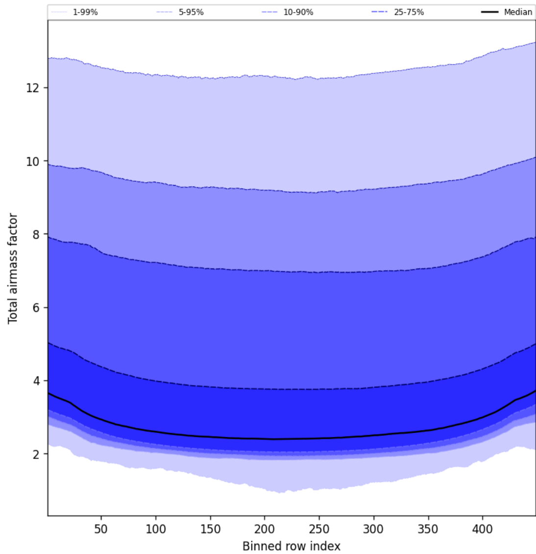
Figure 47: Along track statistics of “Total airmass factor” for 2025-09-21 to 2025-09-22
