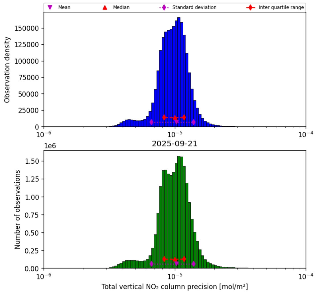
Figure 37: Histogram of “Total vertical NO 2 column precision” for 2025-09-21 to 2025-09-22
