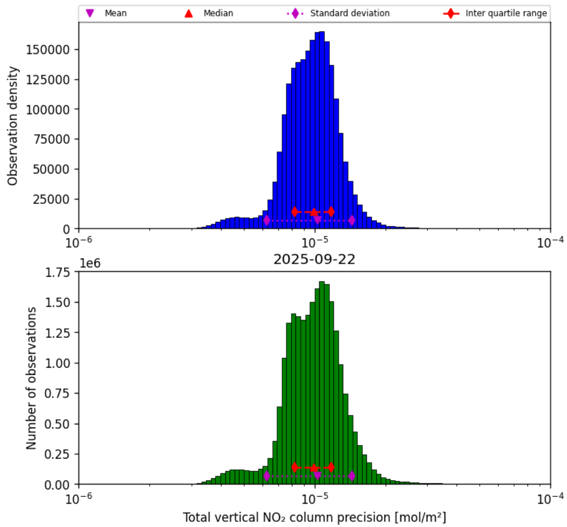
Figure 37: Histogram of “Total vertical NO 2 column precision” for 2025-09-22 to 2025-09-23
