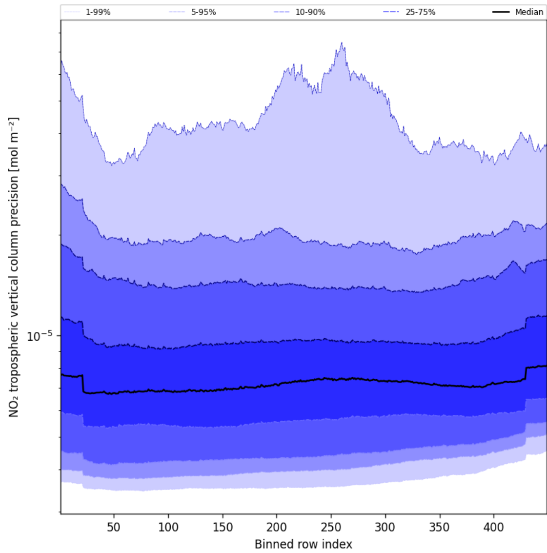
Figure 45: Along track statistics of “NO 2 tropospheric vertical column precision” for 2025-09-22 to 2025-09-23
