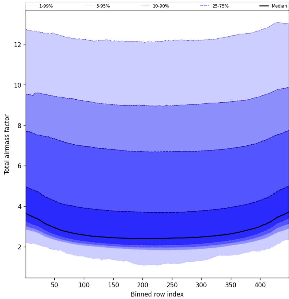
Figure 47: Along track statistics of “Total airmass factor” for 2025-09-22 to 2025-09-23
