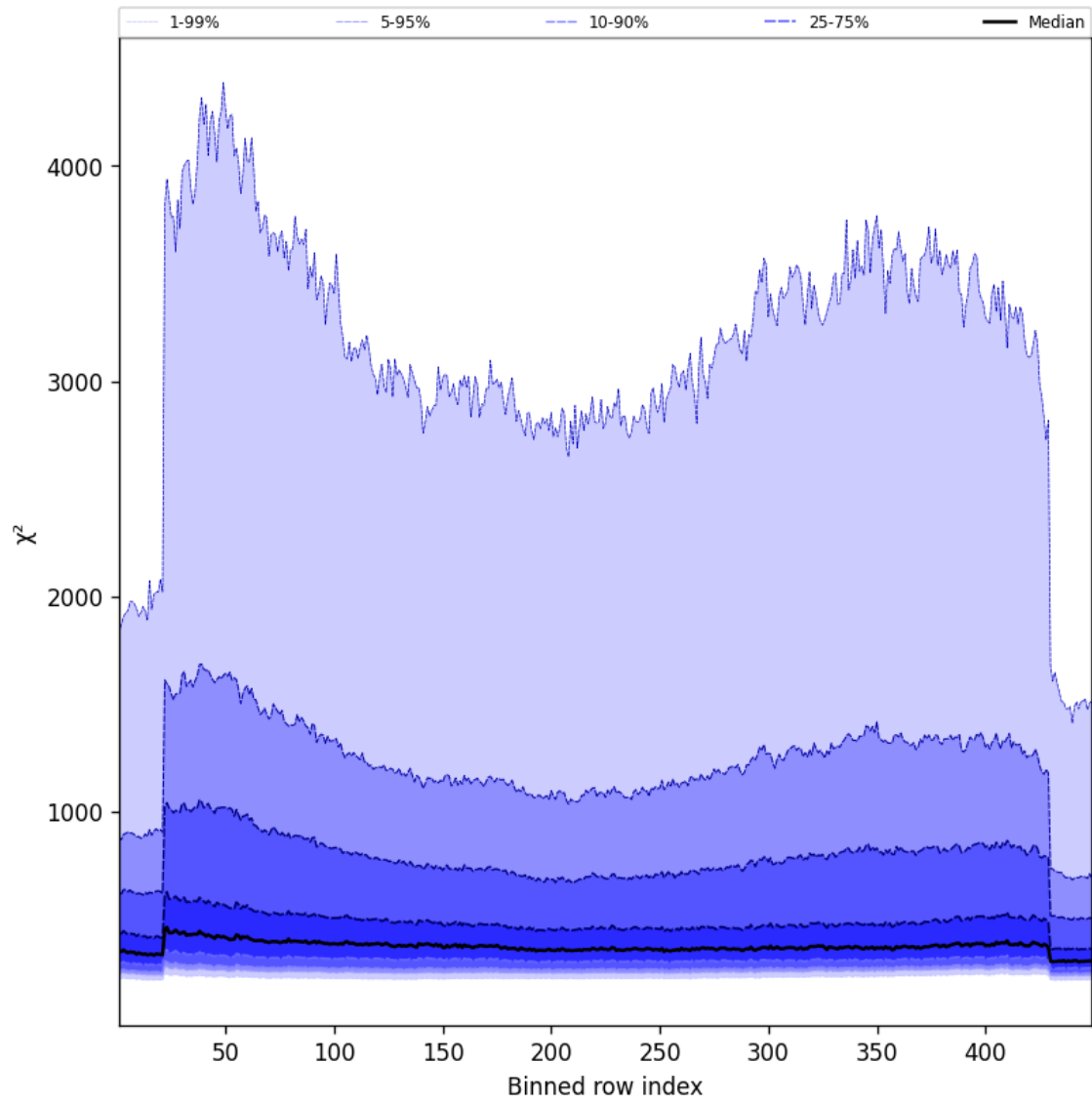
Figure 57: Along track statistics of “ \chi^2 ” for 2025-09-22 to 2025-09-23
