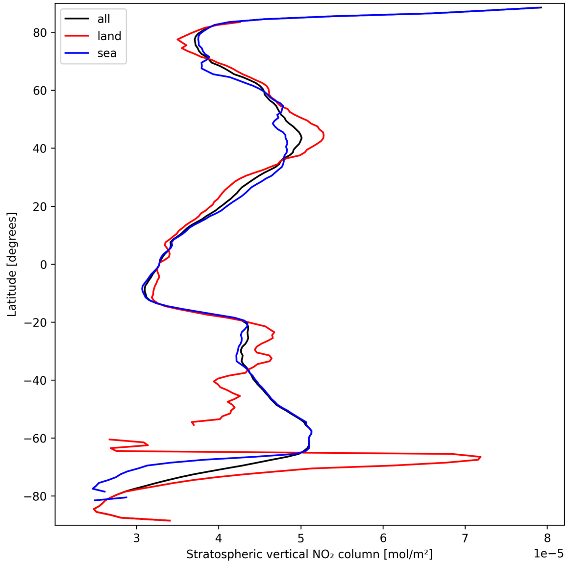
Figure 17: Zonal average of “Stratospheric vertical NO 2 column” for 2025-09-22 to 2025-09-23.
