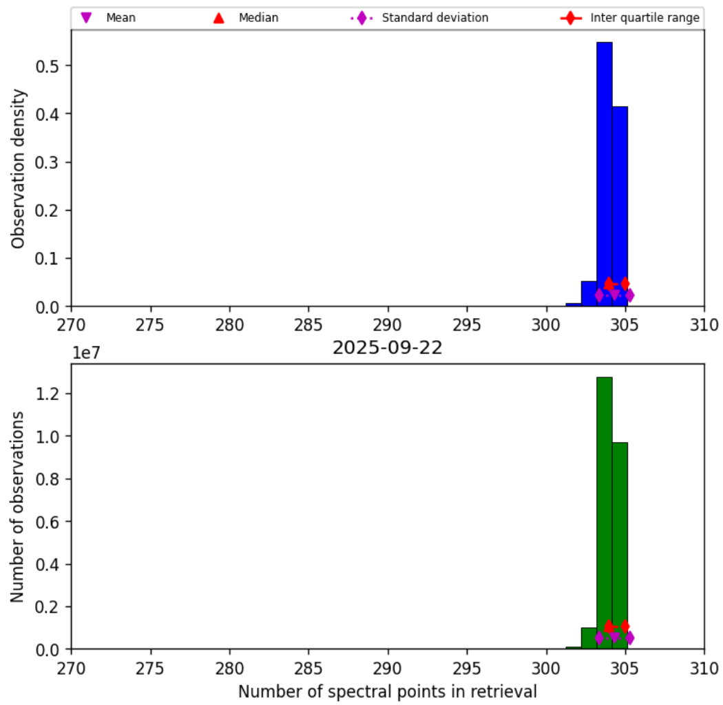
Figure 31: Histogram of “Number of spectral points in retrieval” for 2025-09-22 to 2025-09-23
