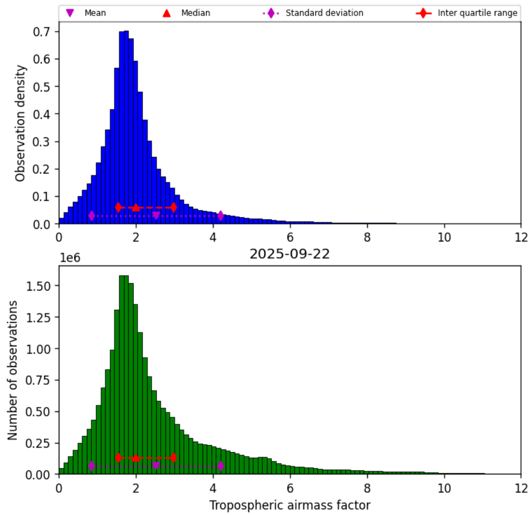
Figure 29: Histogram of “Tropospheric airmass factor” for 2025-09-22 to 2025-09-23
