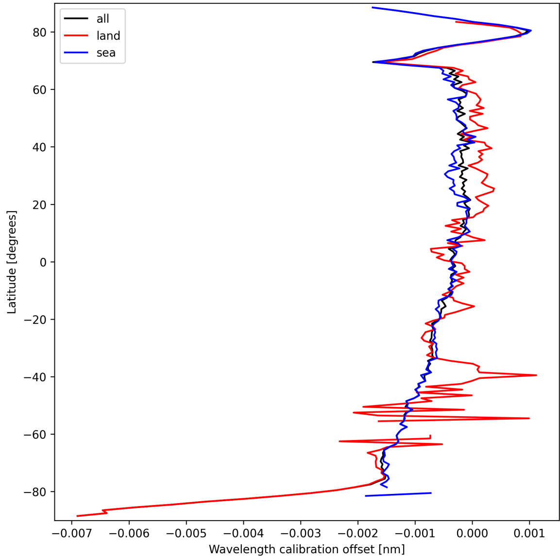
Figure 16: Zonal average of “Wavelength calibration offset” for 2025-09-22 to 2025-09-23.
