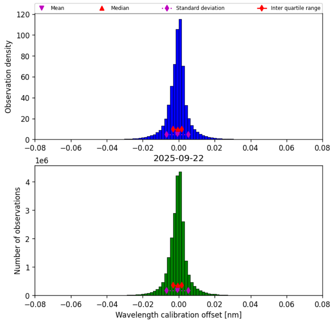
Figure 33: Histogram of “Wavelength calibration offset” for 2025-09-22 to 2025-09-23
