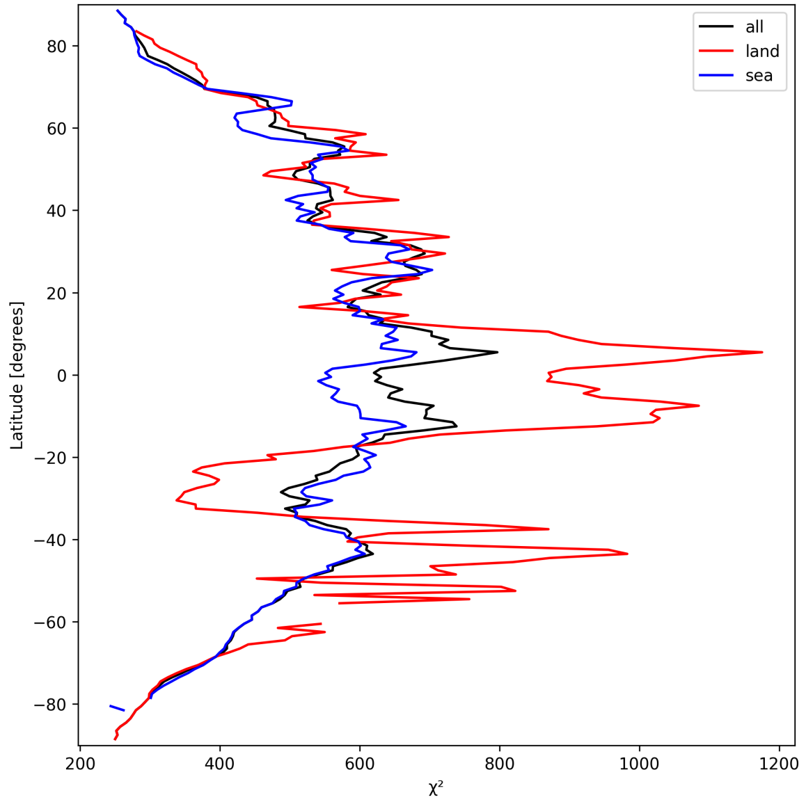
Figure 23: Zonal average of “ \chi^2 ” for 2025-09-22 to 2025-09-23.
