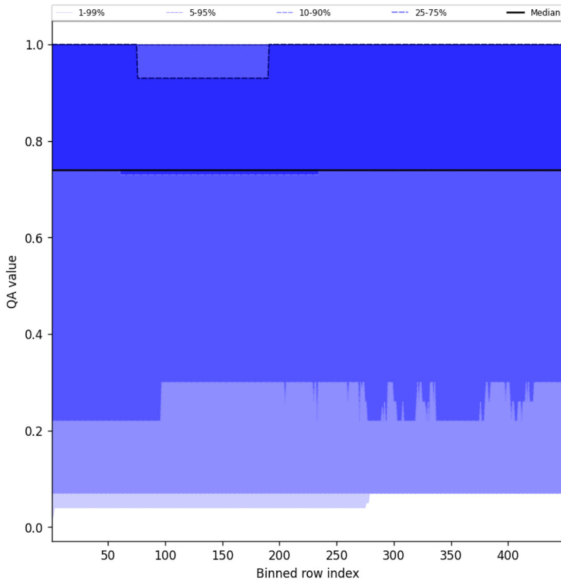
Figure 43: Along track statistics of “QA value” for 2025-09-22 to 2025-09-23
