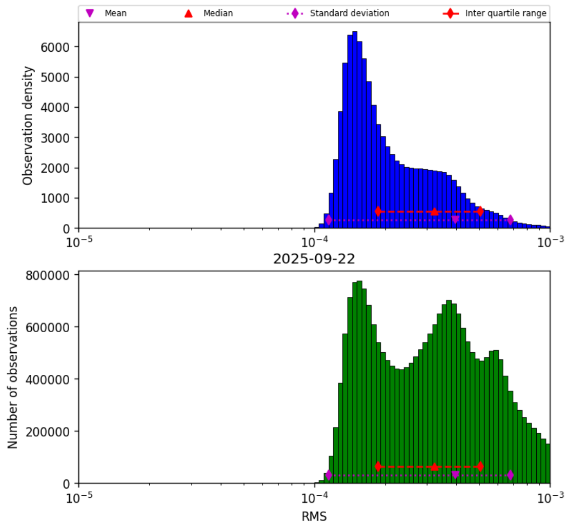
Figure 41: Histogram of “RMS” for 2025-09-22 to 2025-09-23
