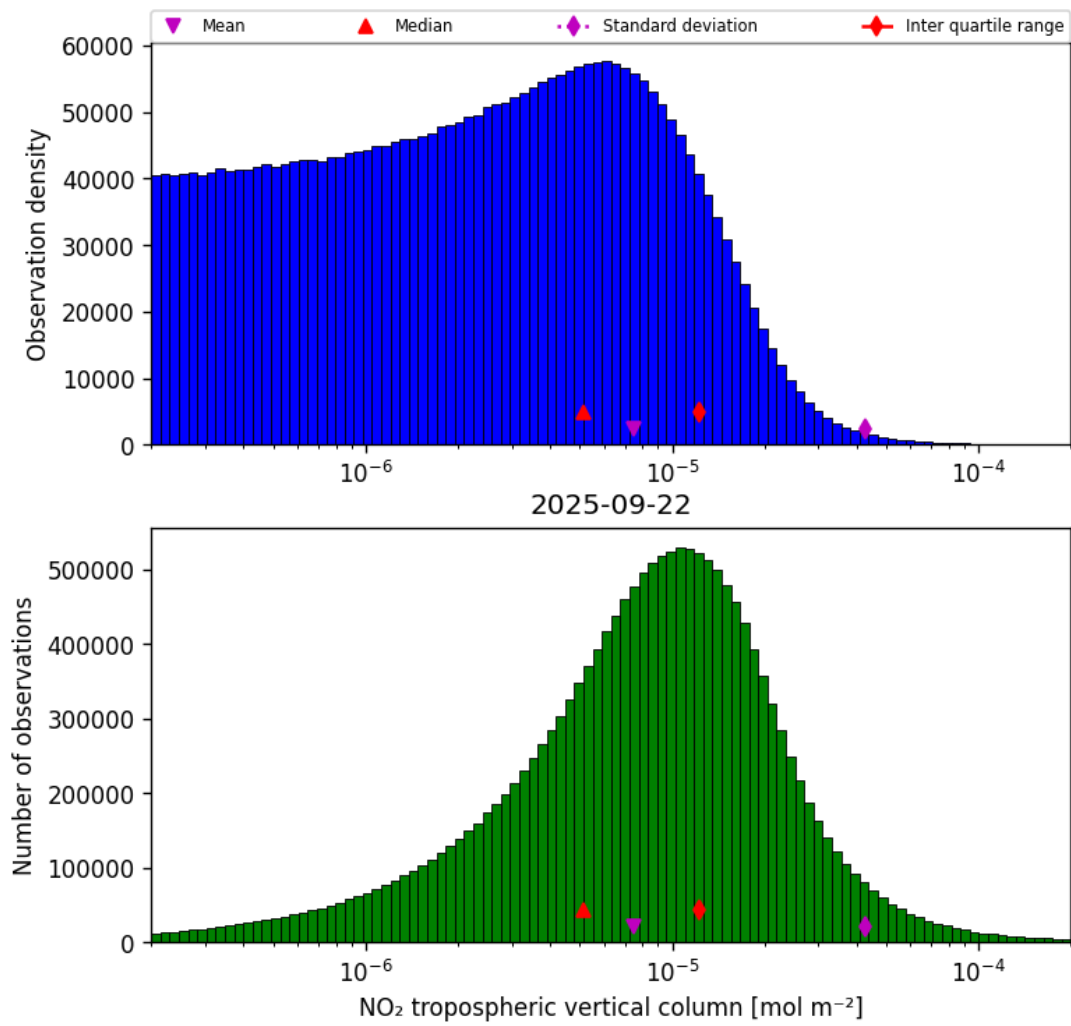
Figure 27: Histogram of “NO 2 tropospheric vertical column” for 2025-09-22 to 2025-09-23
