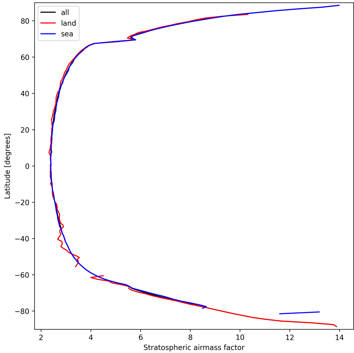
Figure 25: Zonal average of “Stratospheric air mass factor” for 2025-09-22 to 2025-09-23.
