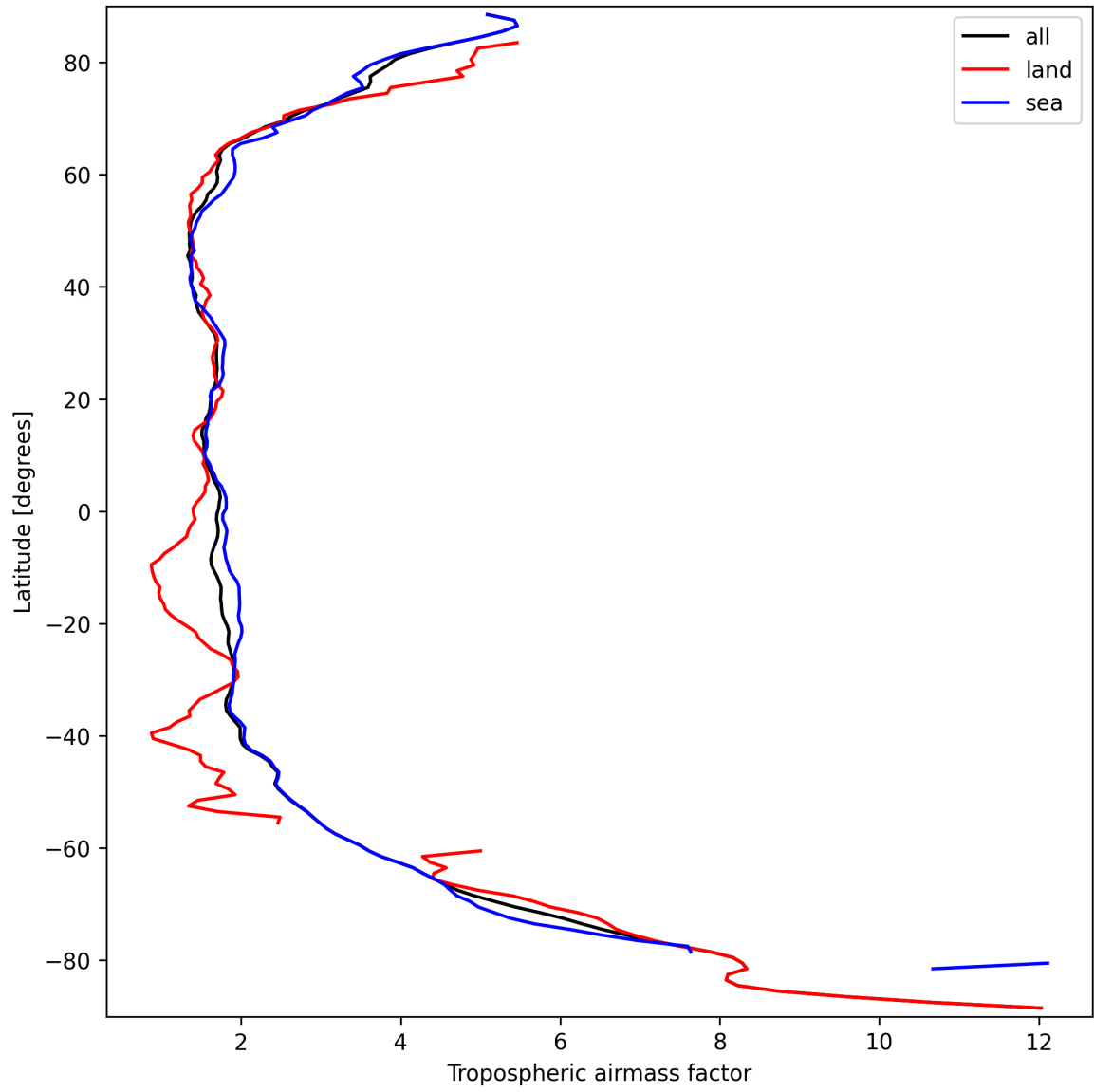
Figure 12: Zonal average of “Tropospheric airmass factor” for 2025-09-22 to 2025-09-23.
