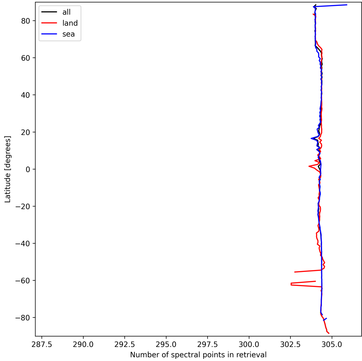
Figure 14: Zonal average of “Number of spectral points in retrieval” for 2025-09-22 to 2025-09-23.
