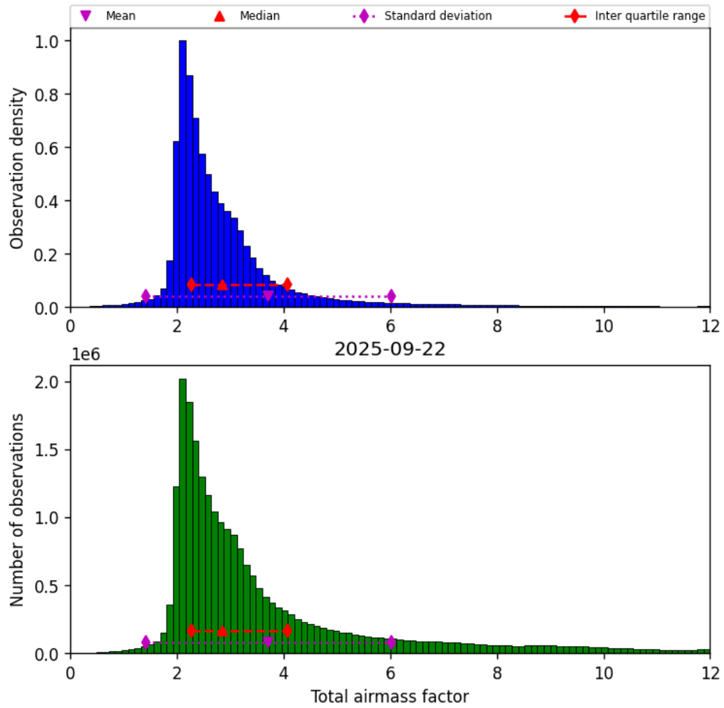
Figure 30: Histogram of “Total airmass factor” for 2025-09-22 to 2025-09-23
