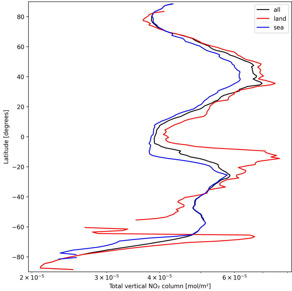
Figure 19: Zonal average of “Total vertical NO 2 column” for 2025-09-22 to 2025-09-23.
