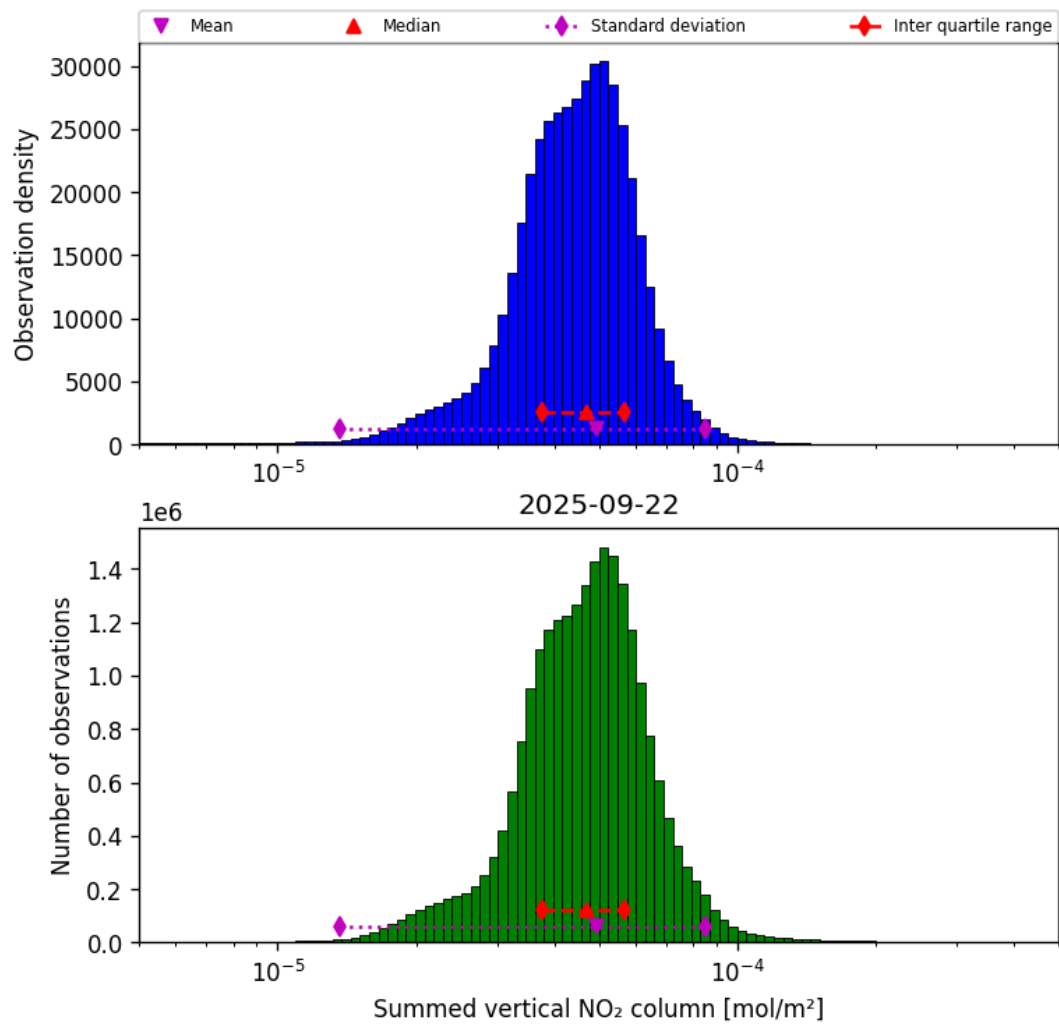
Figure 38: Histogram of “Summed vertical NO 2 column” for 2025-09-22 to 2025-09-23
