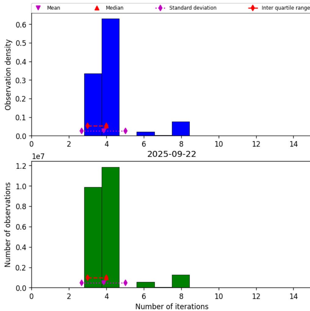
Figure 32: Histogram of “Number of iterations” for 2025-09-22 to 2025-09-23
