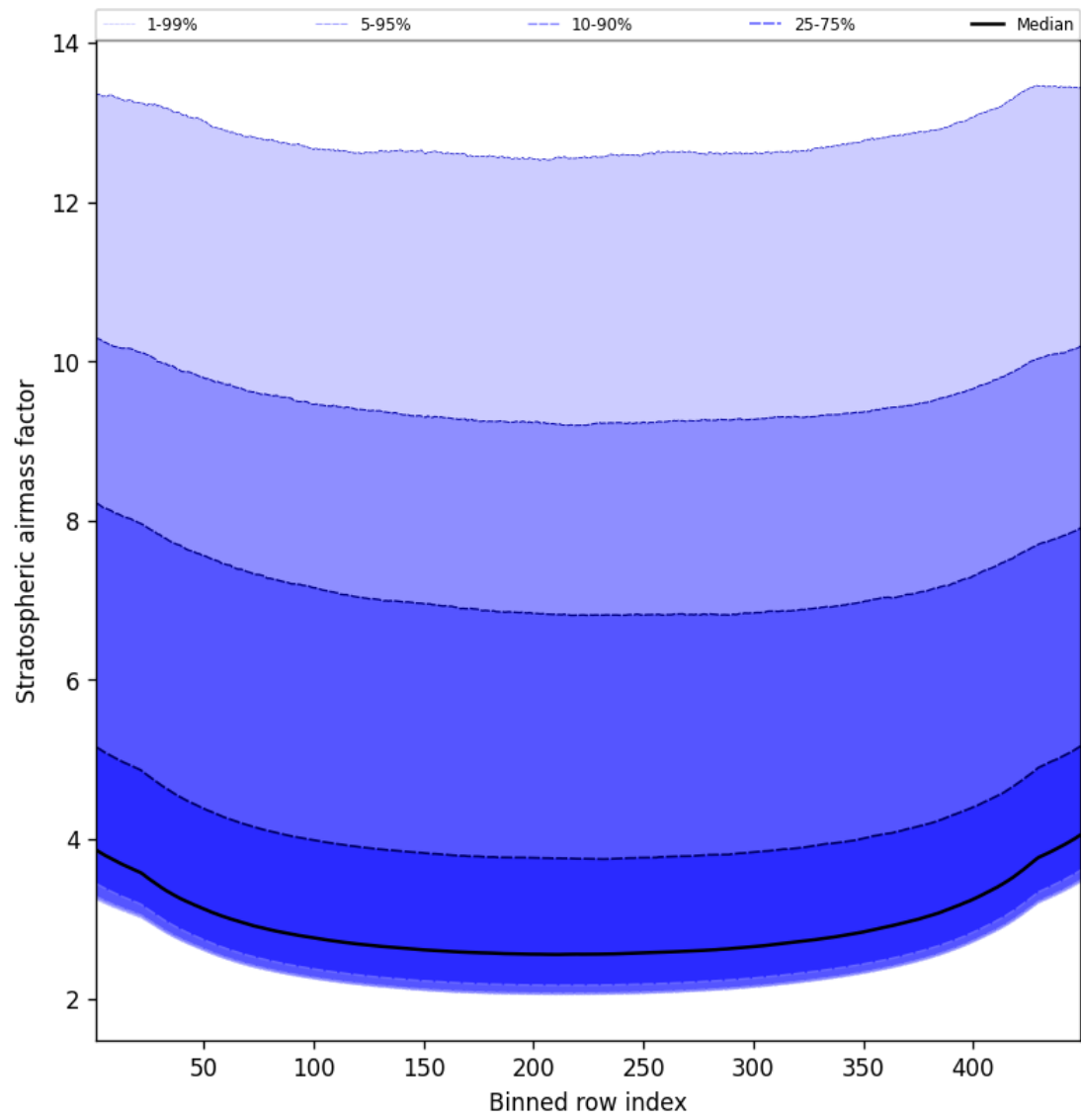
Figure 59: Along track statistics of “Stratospheric airmass factor” for 2025-09-22 to 2025-09-23
