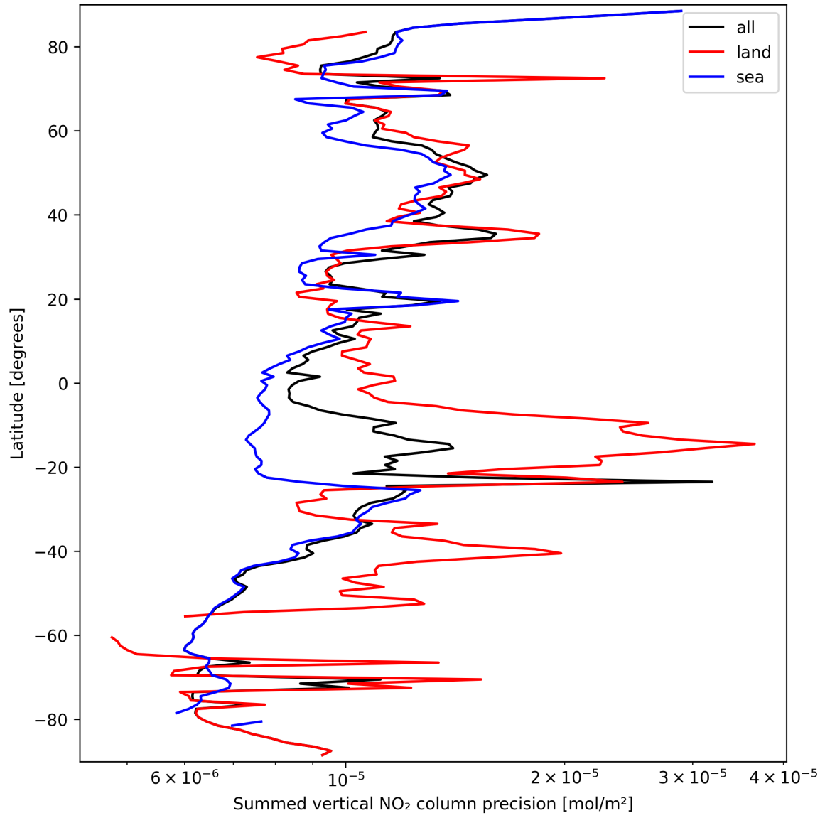
Figure 22: Zonal average of “Summed vertical NO 2 column precision” for 2025-09-22 to 2025-09-23.
