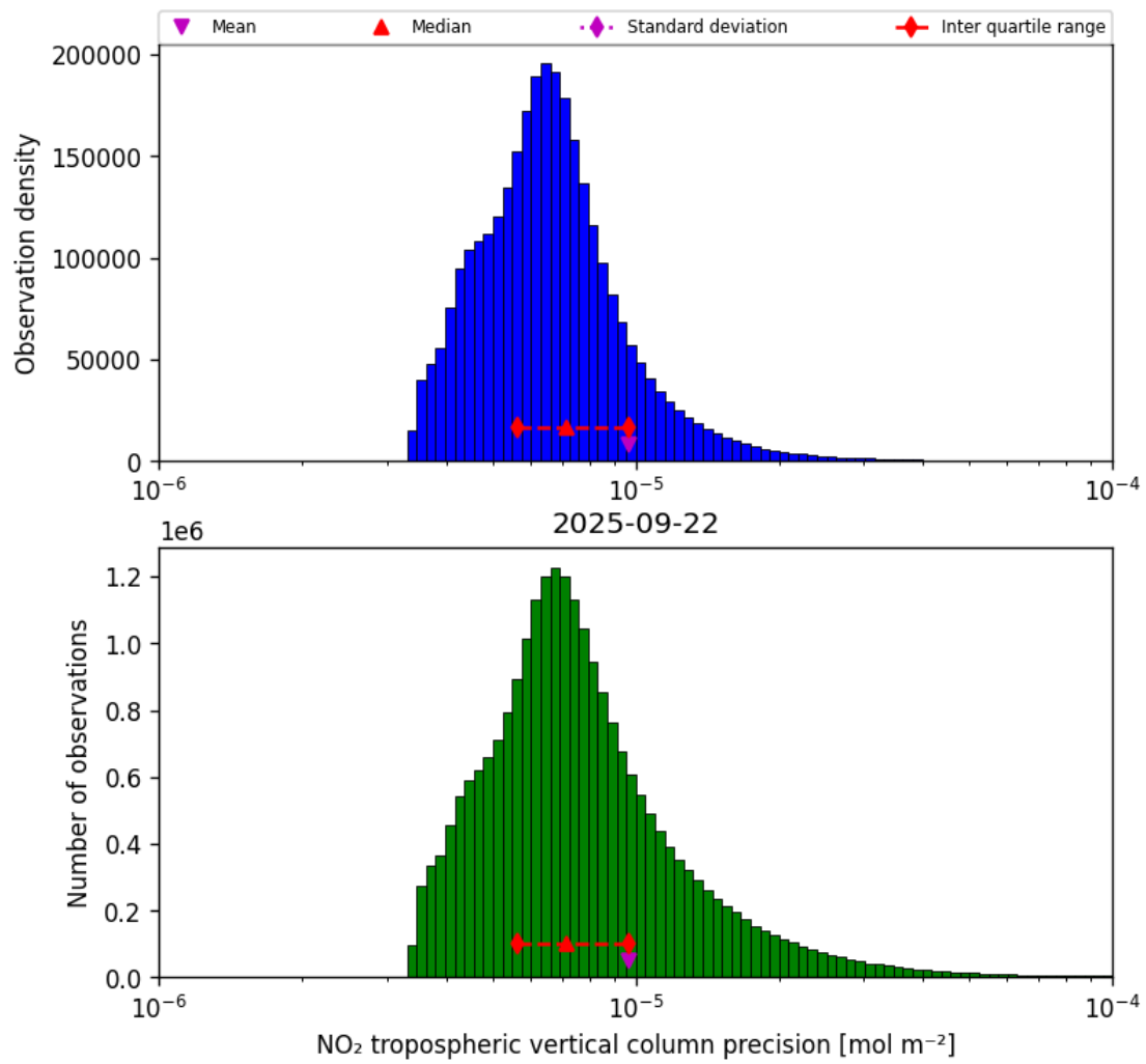
Figure 28: Histogram of “NO 2 tropospheric vertical column precision” for 2025-09-22 to 2025-09-23
