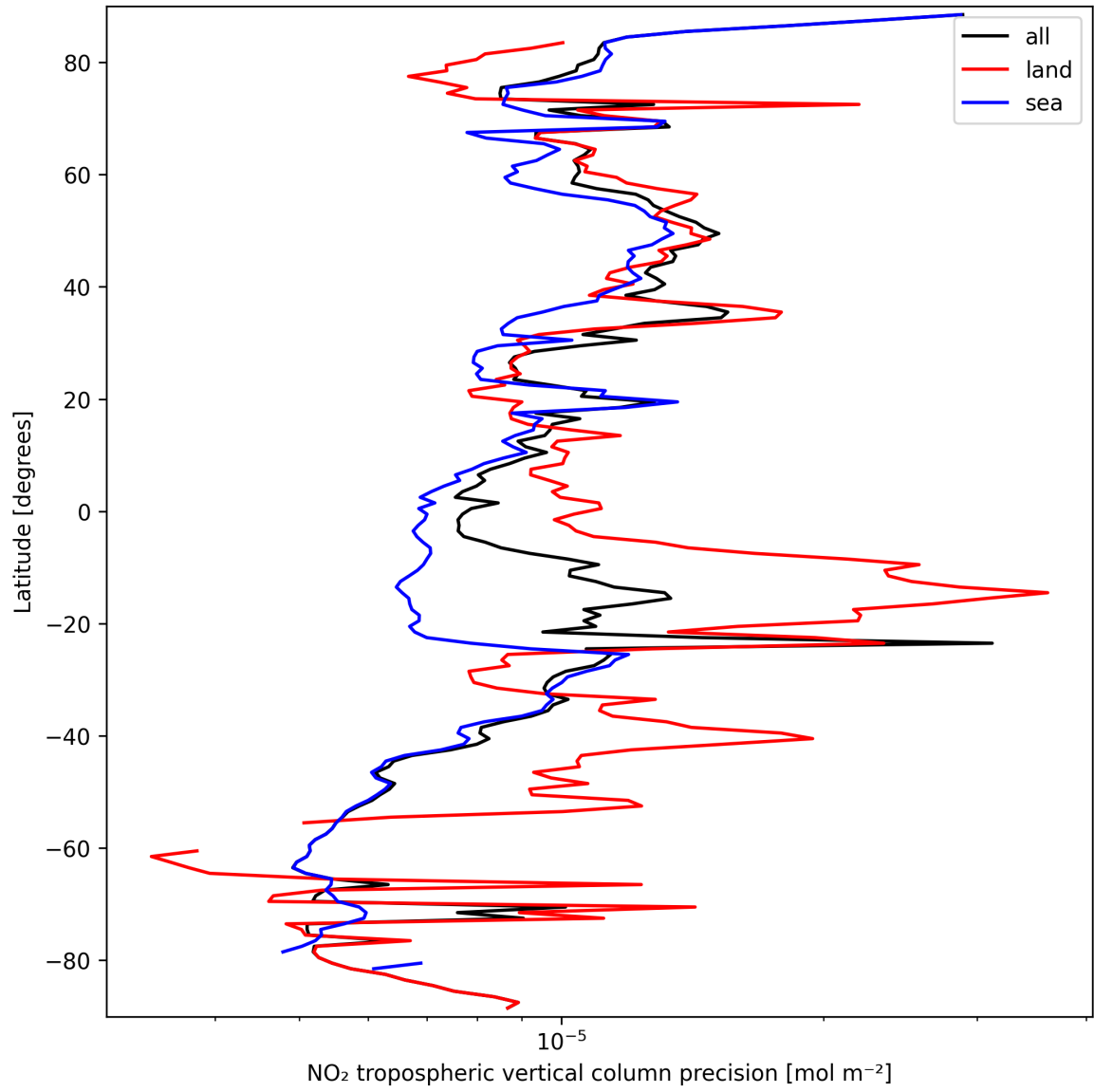
Figure 11: Zonal average of “NO 2 tropospheric vertical column precision” for 2025-09-22 to 2025-09-23.
