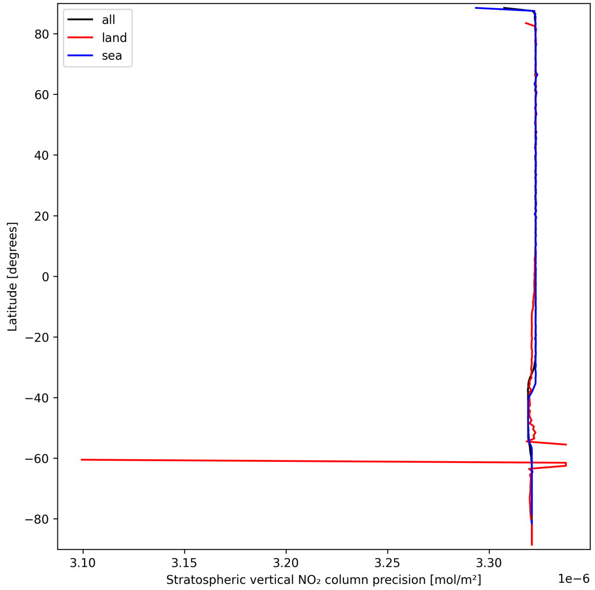
Figure 18: Zonal average of “Stratospheric vertical NO 2 column precision” for 2025-09-22 to 2025-09-23.
