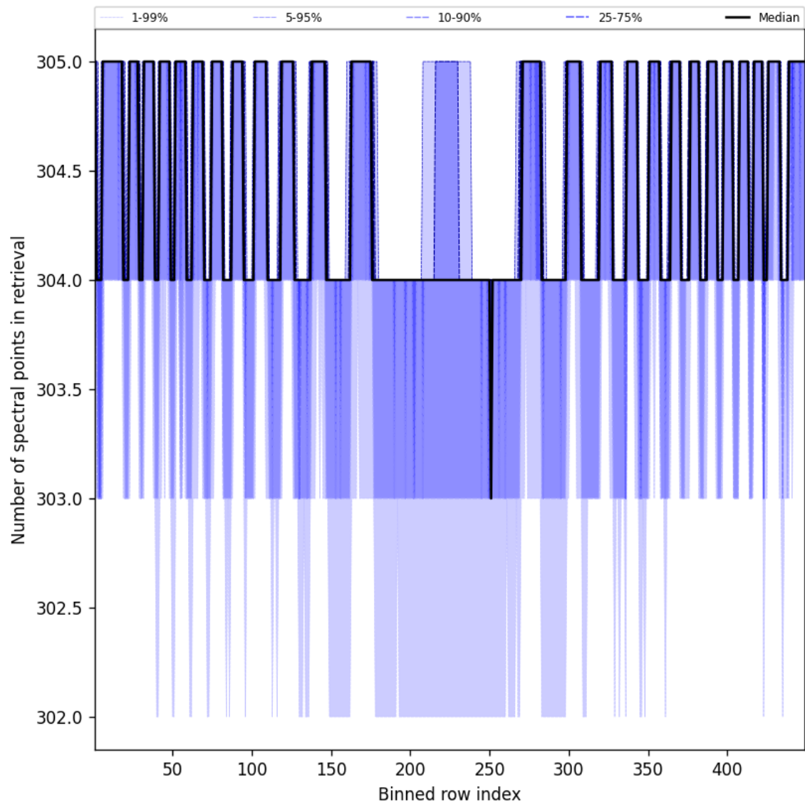
Figure 48: Along track statistics of “Number of spectral points in retrieval” for 2025-09-22 to 2025-09-23
