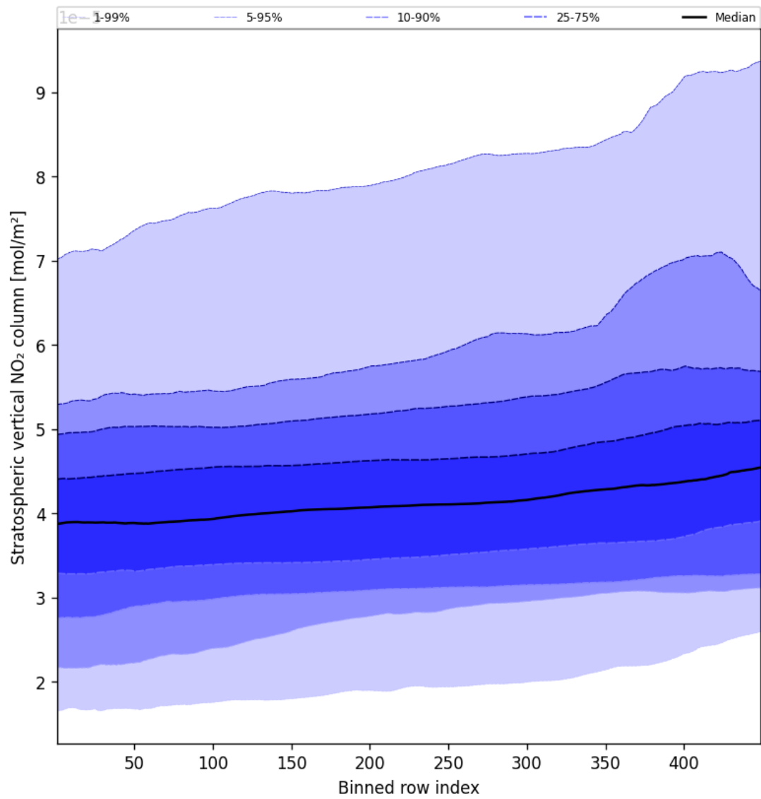
Figure 51: Along track statistics of “Stratospheric vertical NO 2 column” for 2025-09-22 to 2025-09-23
