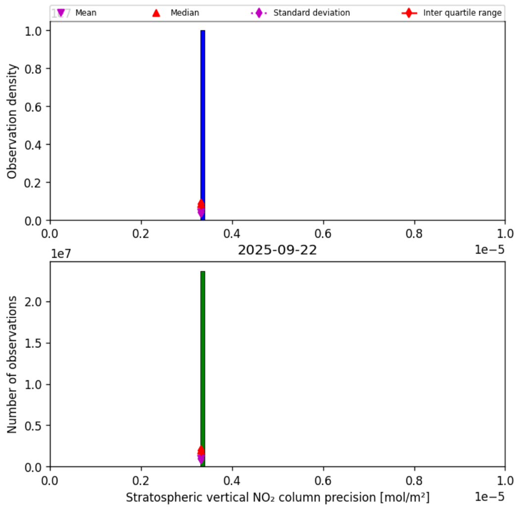
Figure 35: Histogram of “Stratospheric vertical NO 2 column precision” for 2025-09-22 to 2025-09-23
