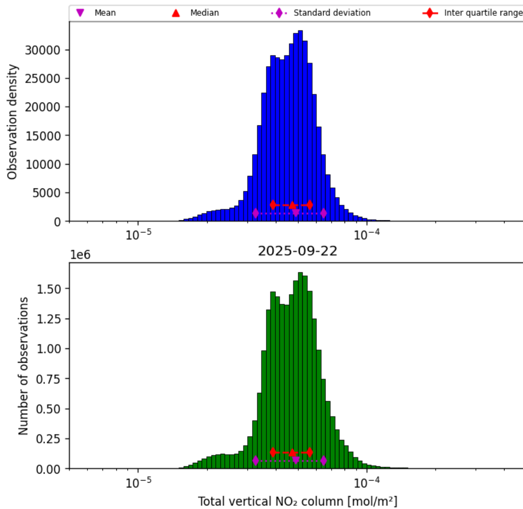
Figure 36: Histogram of “Total vertical NO 2 column” for 2025-09-22 to 2025-09-23
