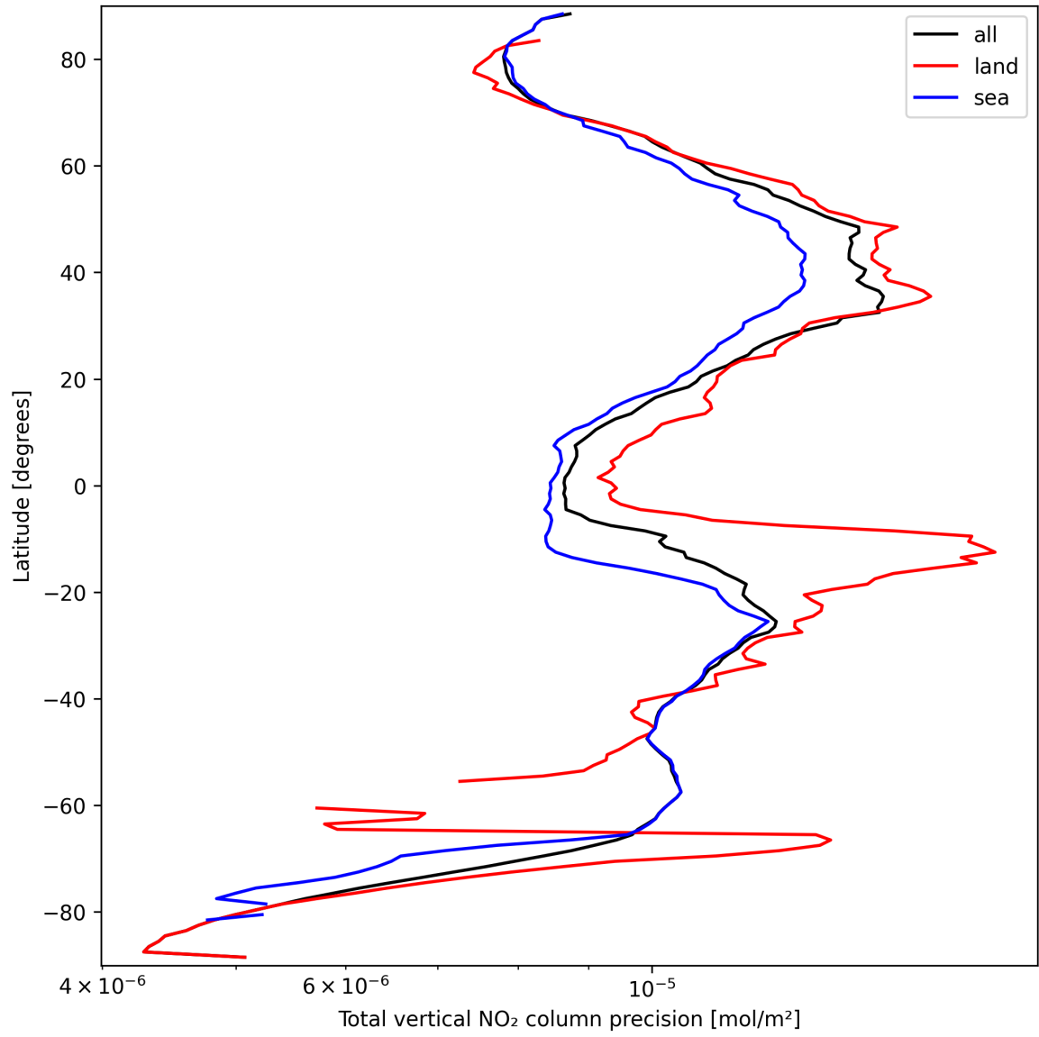
Figure 20: Zonal average of “Total vertical NO 2 column precision” for 2025-09-22 to 2025-09-23.
