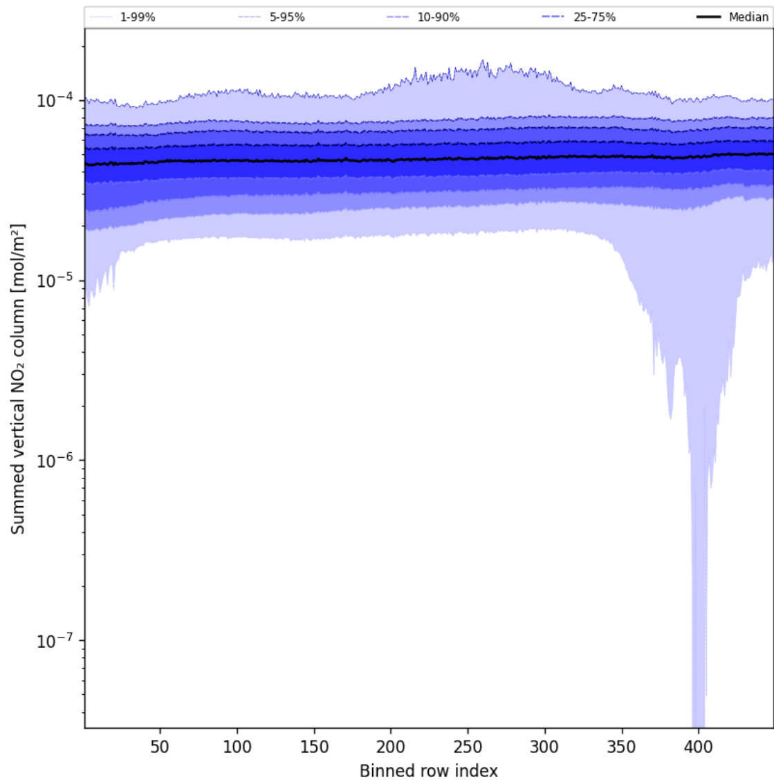
Figure 55: Along track statistics of “Summed vertical NO 2 column” for 2025-09-22 to 2025-09-23
