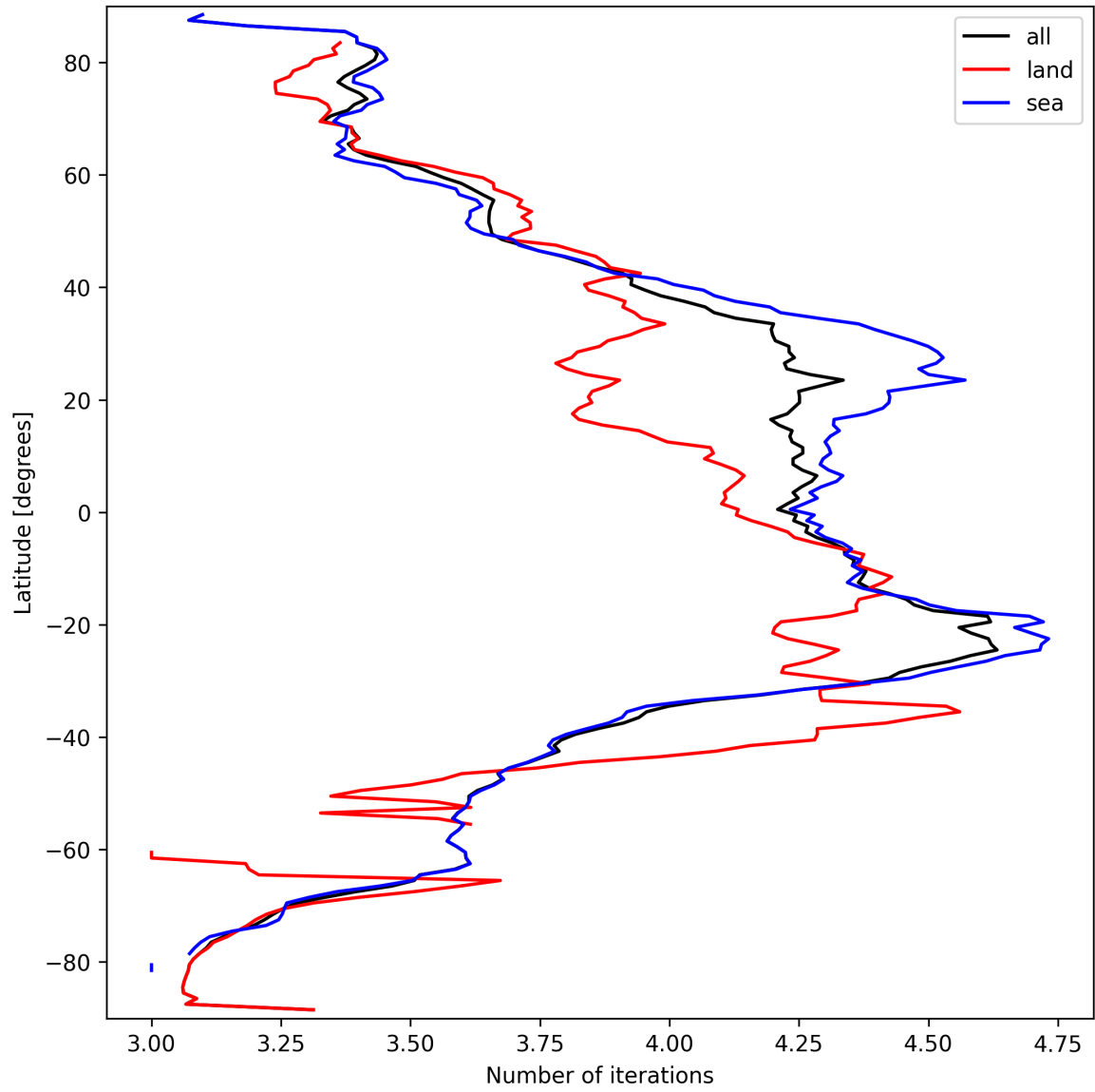
Figure 15: Zonal average of “Number of iterations” for 2025-09-22 to 2025-09-23.
