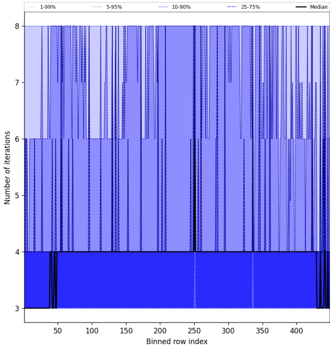
Figure 49: Along track statistics of “Number of iterations” for 2025-09-22 to 2025-09-23
