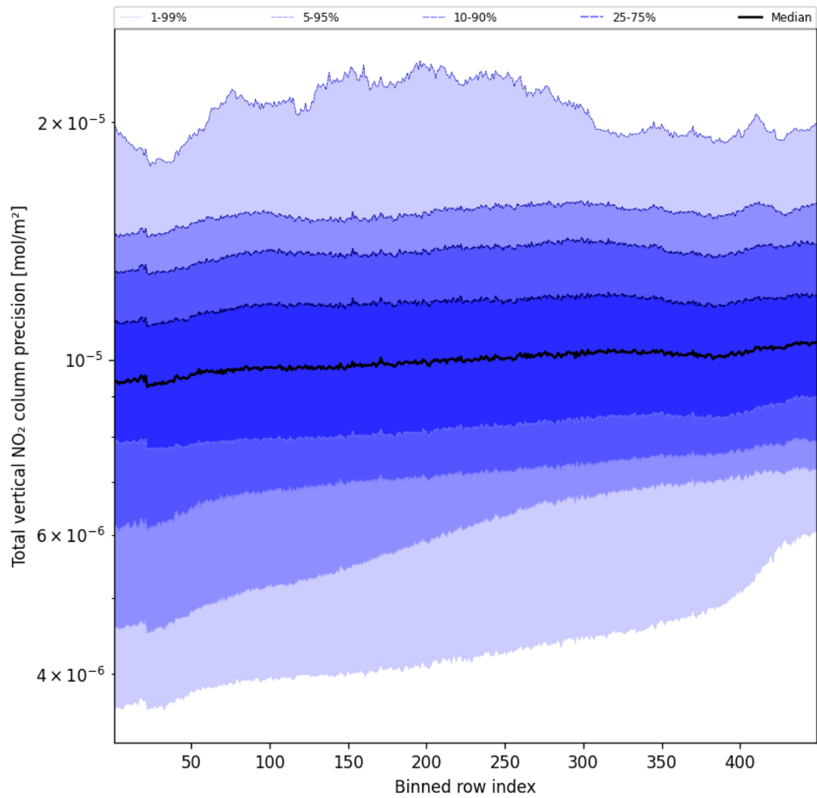
Figure 54: Along track statistics of “Total vertical NO 2 column precision” for 2025-09-22 to 2025-09-23
