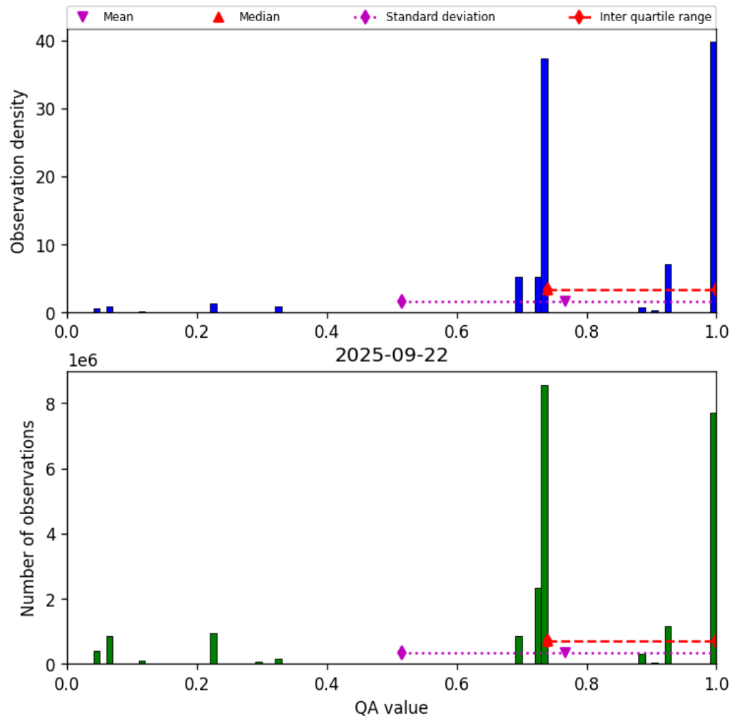
Figure 26: Histogram of “QA value” for 2025-09-22 to 2025-09-23
