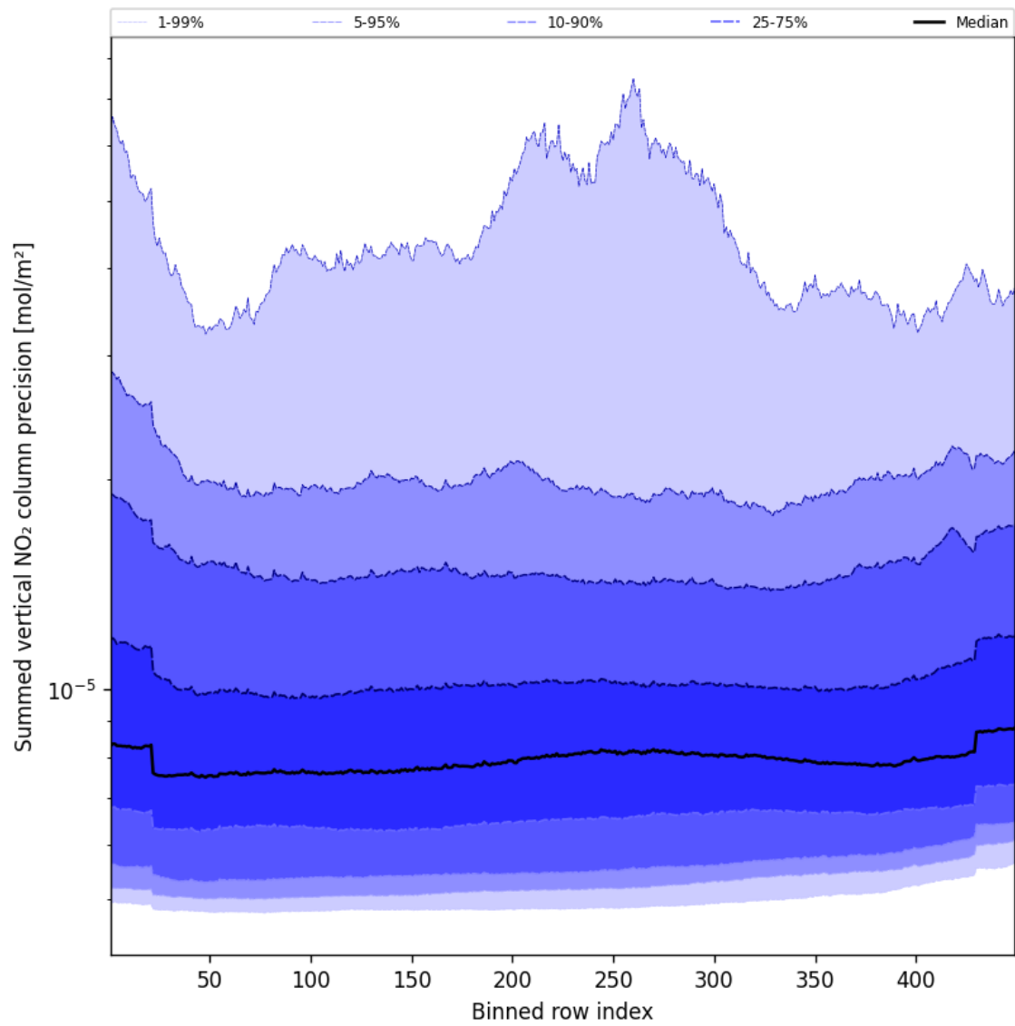
Figure 56: Along track statistics of “Summed vertical NO 2 column precision” for 2025-09-22 to 2025-09-23
