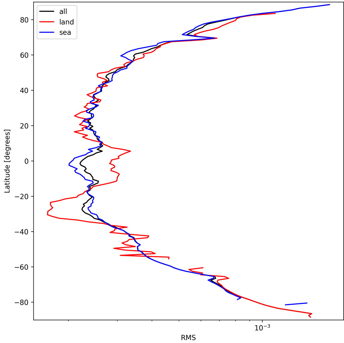
Figure 24: Zonal average of “RMS” for 2025-09-22 to 2025-09-23.
