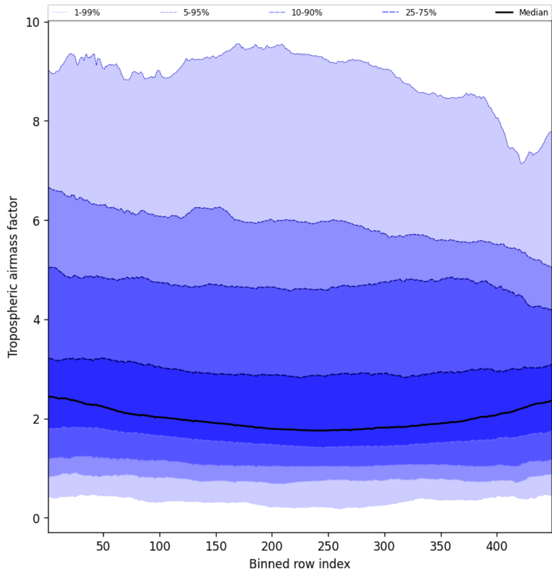
Figure 46: Along track statistics of “Tropospheric air mass factor” for 2025-09-22 to 2025-09-23
