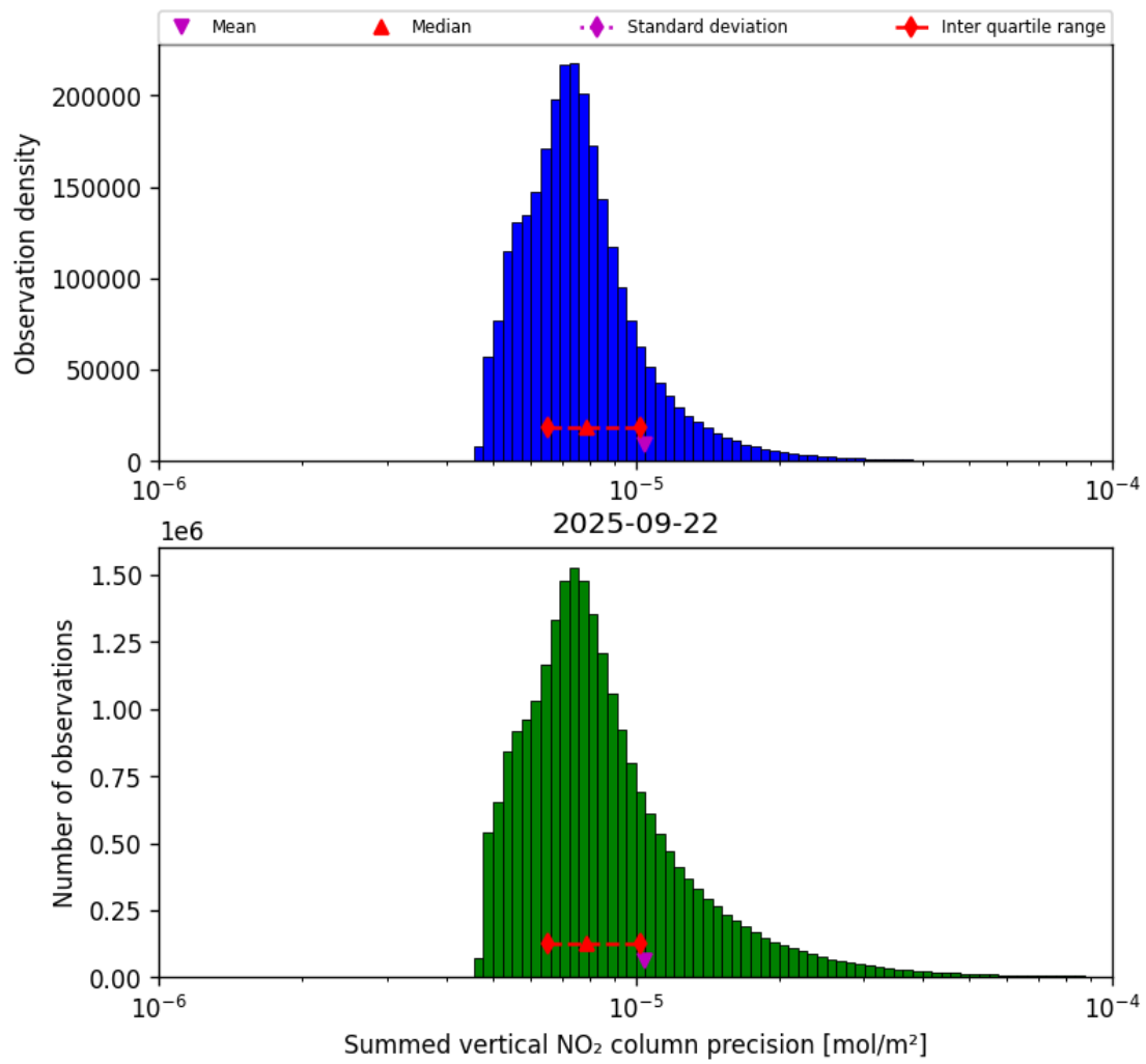
Figure 39: Histogram of “Summed vertical NO 2 column precision” for 2025-09-22 to 2025-09-23
