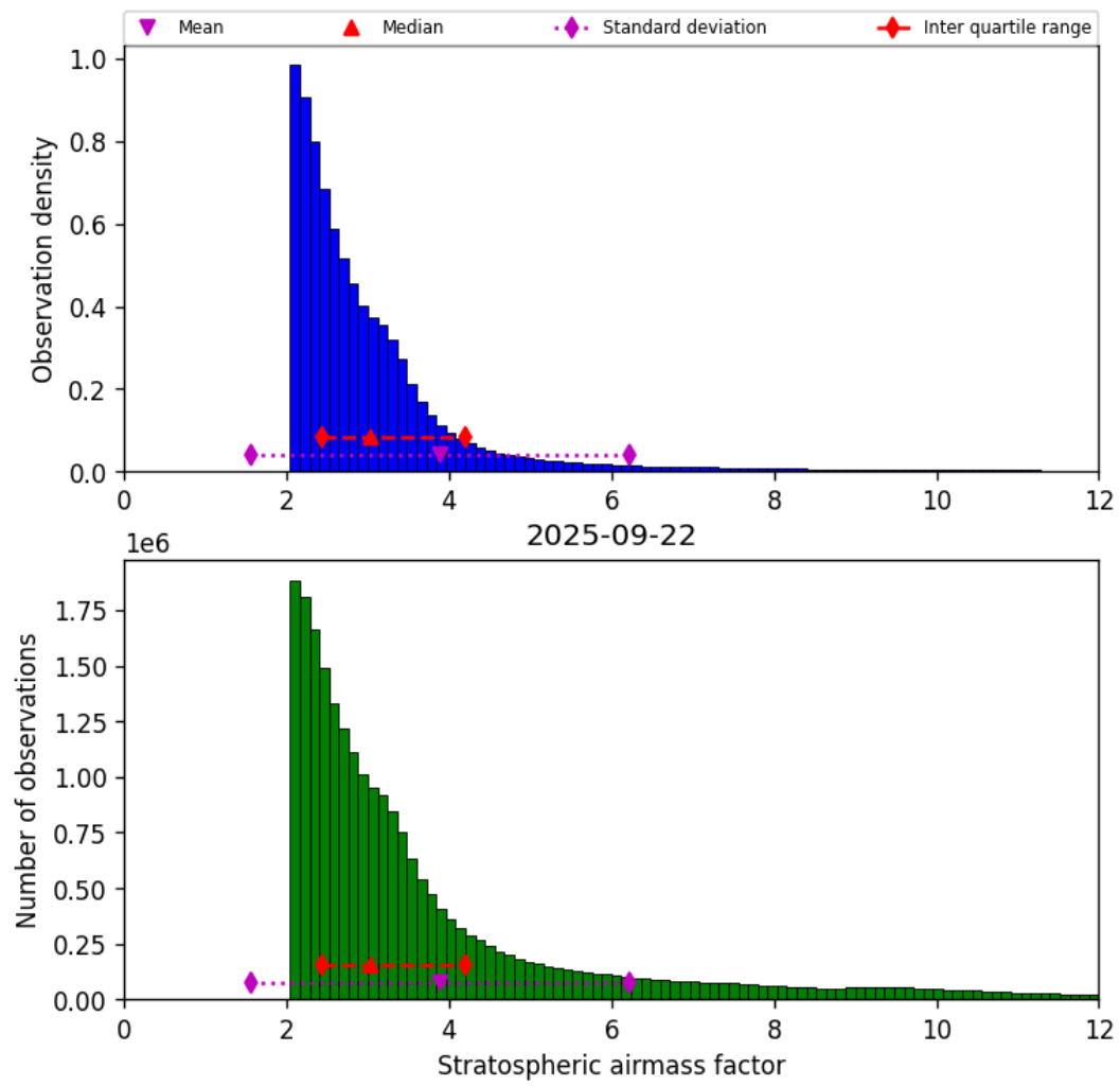
Figure 42: Histogram of “Stratospheric airmass factor” for 2025-09-22 to 2025-09-23
