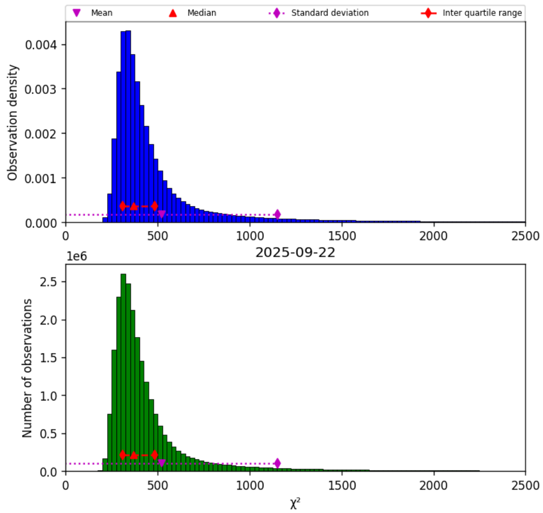
Figure 40: Histogram of “ \chi^2 ” for 2025-09-22 to 2025-09-23
