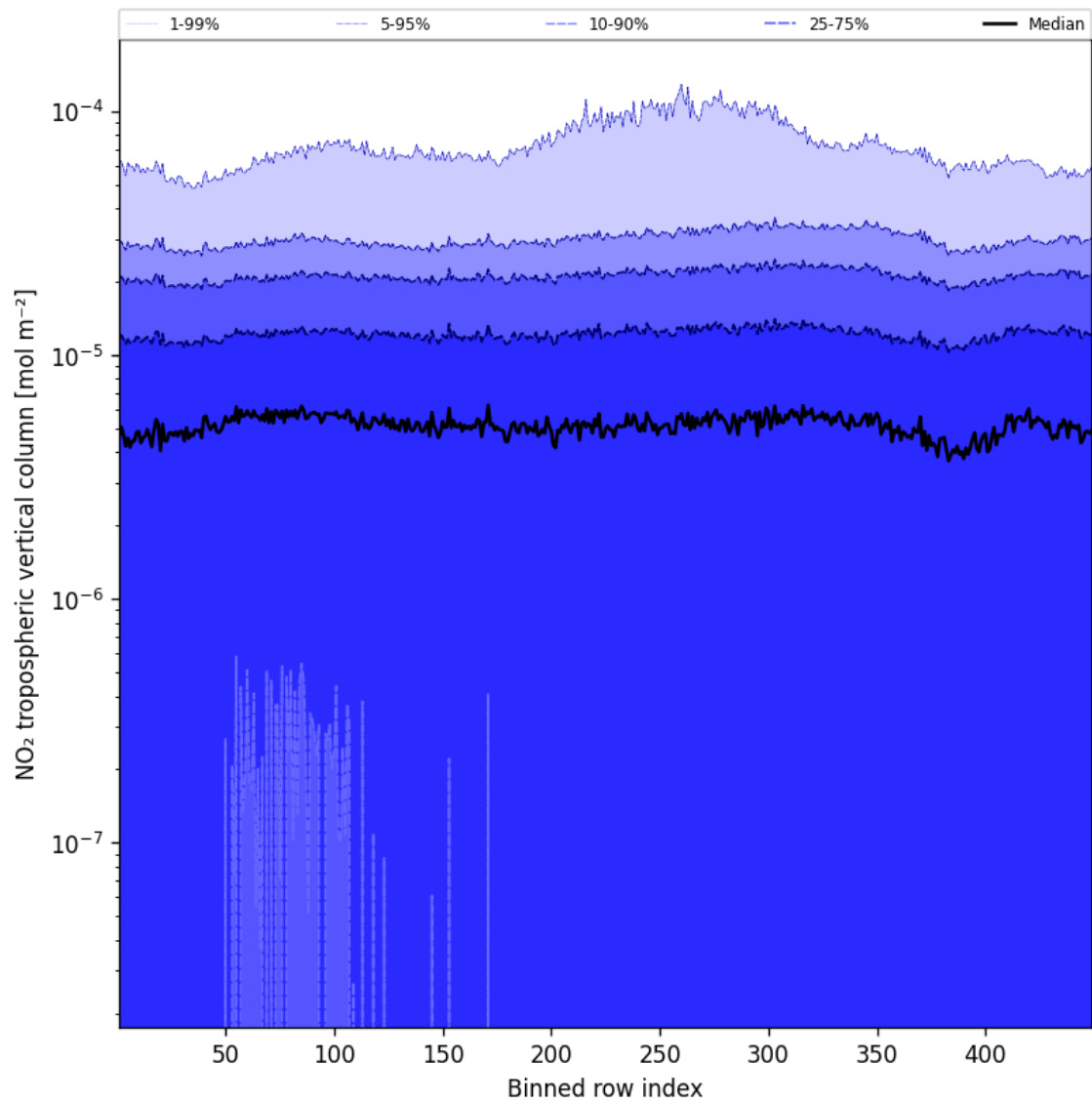
Figure 44: Along track statistics of “NO 2 tropospheric vertical column” for 2025-09-22 to 2025-09-23
