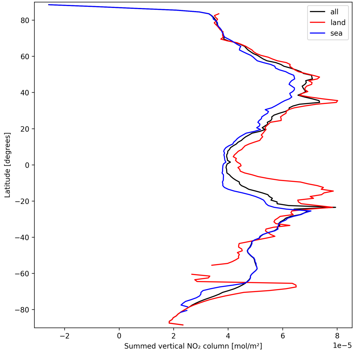
Figure 21: Zonal average of “Summed vertical NO 2 column” for 2025-09-22 to 2025-09-23.
