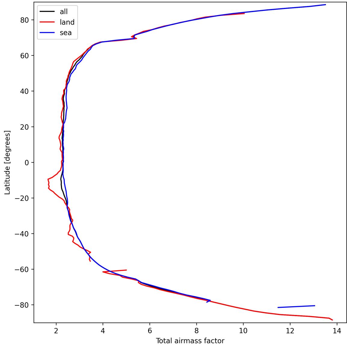
Figure 13: Zonal average of “Total airmass factor” for 2025-09-22 to 2025-09-23.
