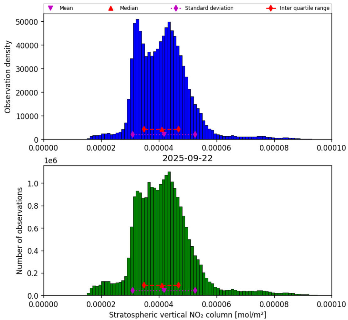
Figure 34: Histogram of “Stratospheric vertical NO 2 column” for 2025-09-22 to 2025-09-23
