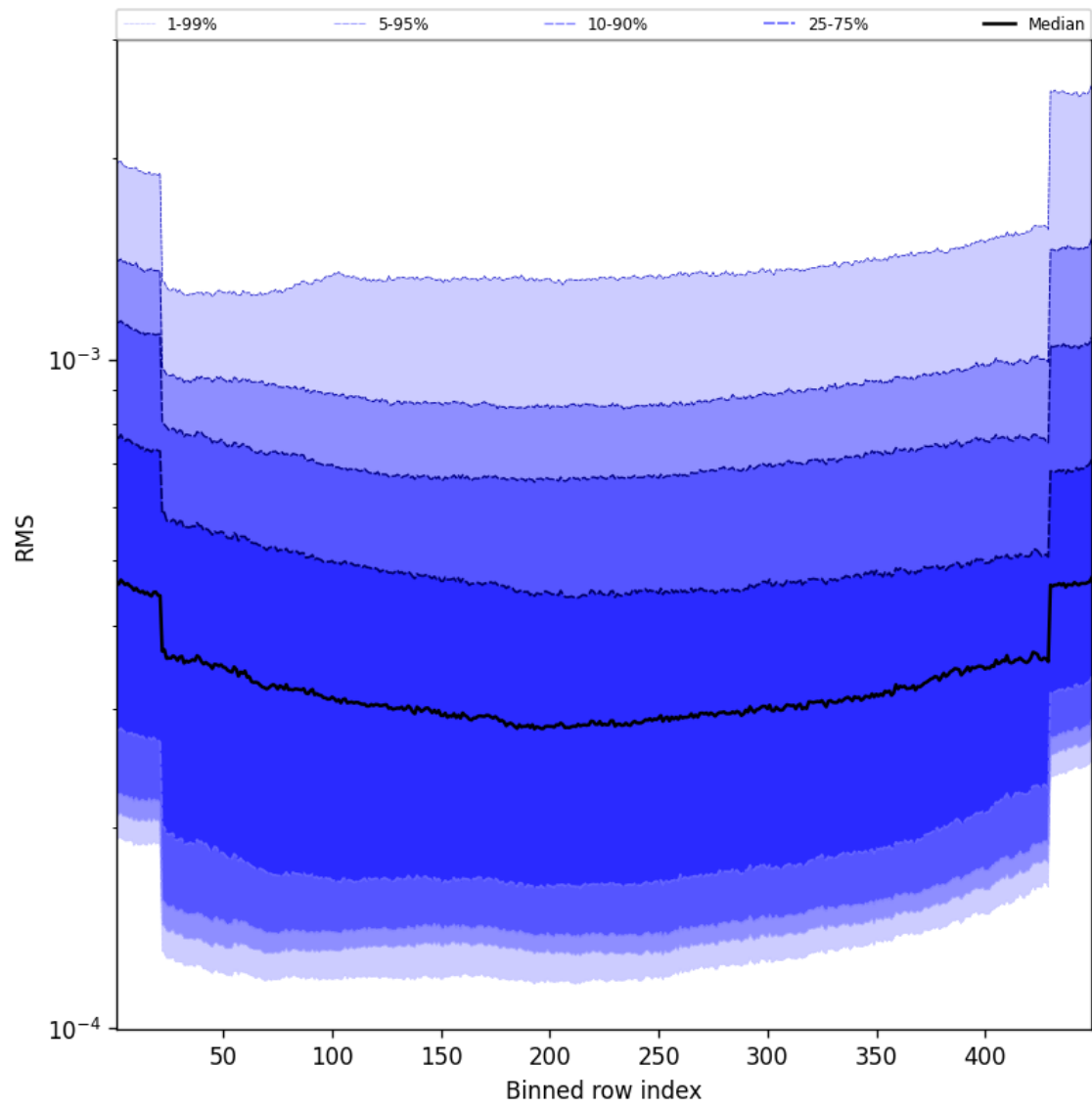
Figure 58: Along track statistics of “RMS” for 2025-09-22 to 2025-09-23
