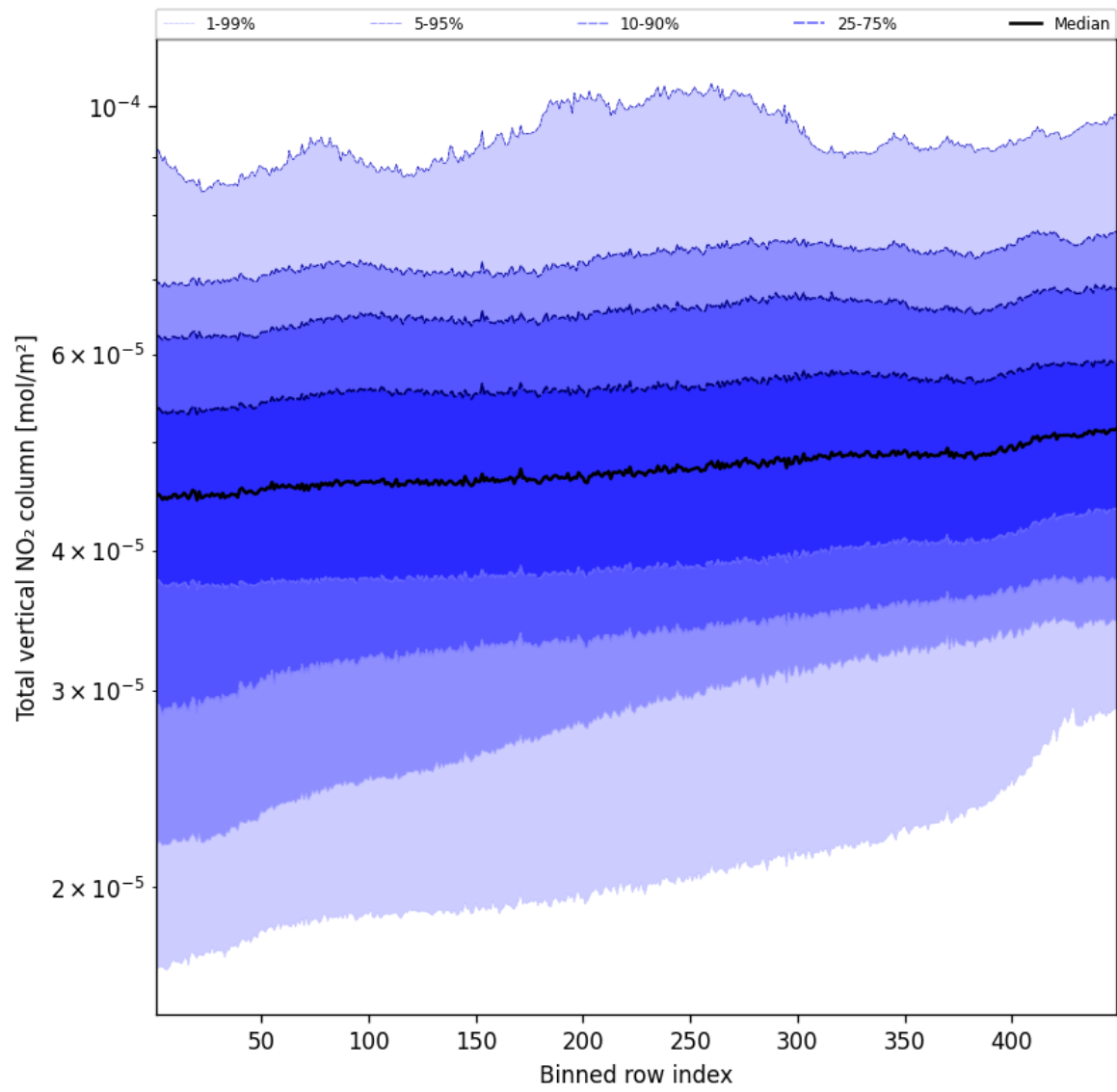
Figure 53: Along track statistics of “Total vertical NO 2 column” for 2025-09-22 to 2025-09-23
