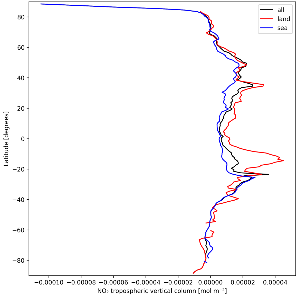
Figure 10: Zonal average of “NO 2 tropospheric vertical column” for 2025-09-22 to 2025-09-23.
