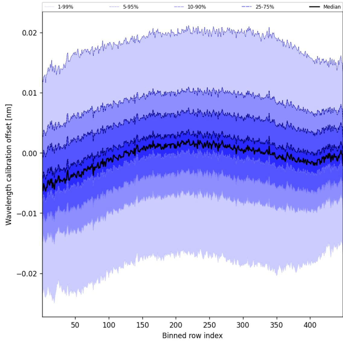
Figure 50: Along track statistics of “Wavelength calibration offset” for 2025-09-22 to 2025-09-23
