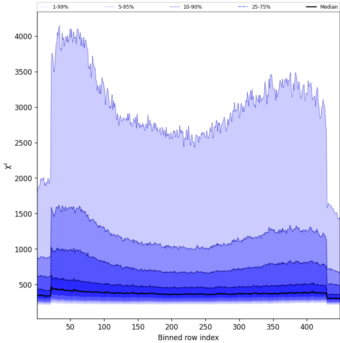
Figure 57: Along track statistics of “ \chi^2 ” for 2025-09-24 to 2025-09-25
