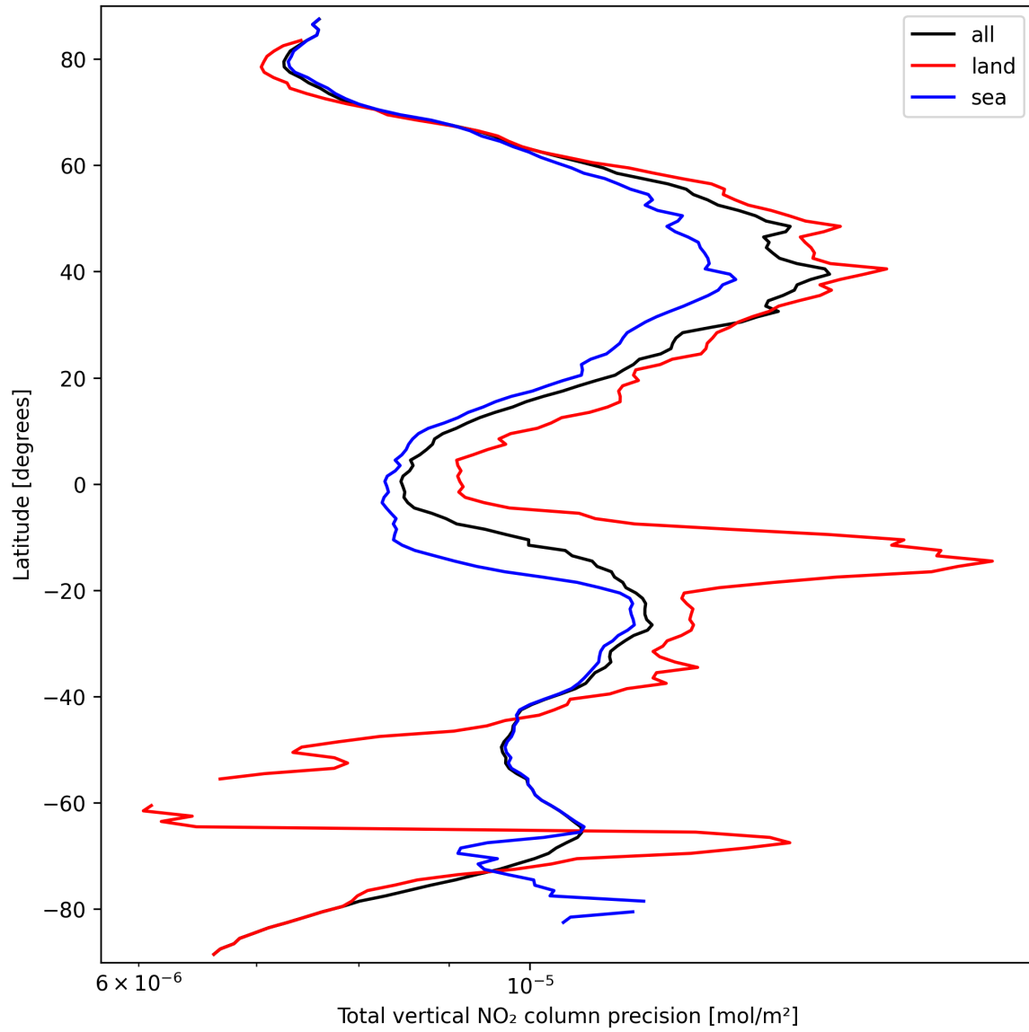
Figure 20: Zonal average of “Total vertical NO 2 column precision” for 2025-09-24 to 2025-09-25.
