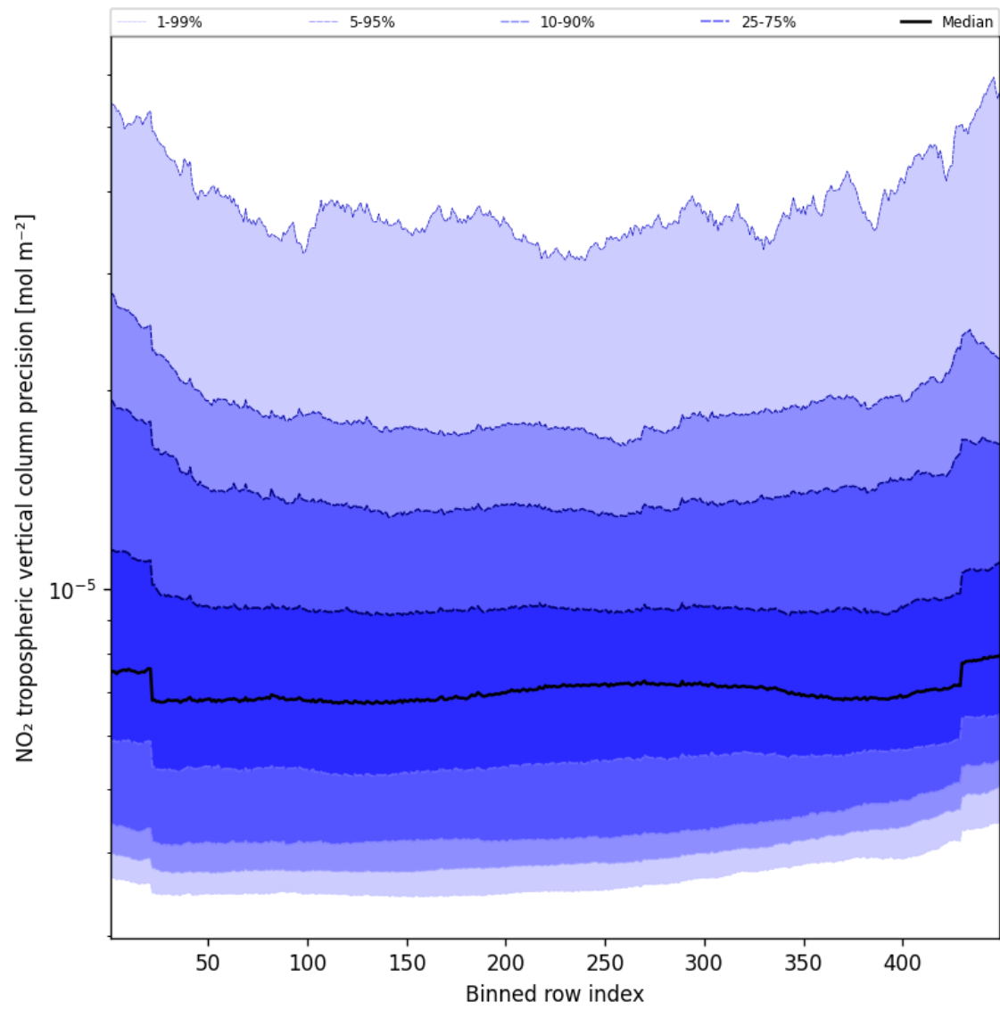
Figure 45: Along track statistics of “NO 2 tropospheric vertical column precision” for 2025-09-24 to 2025-09-25
