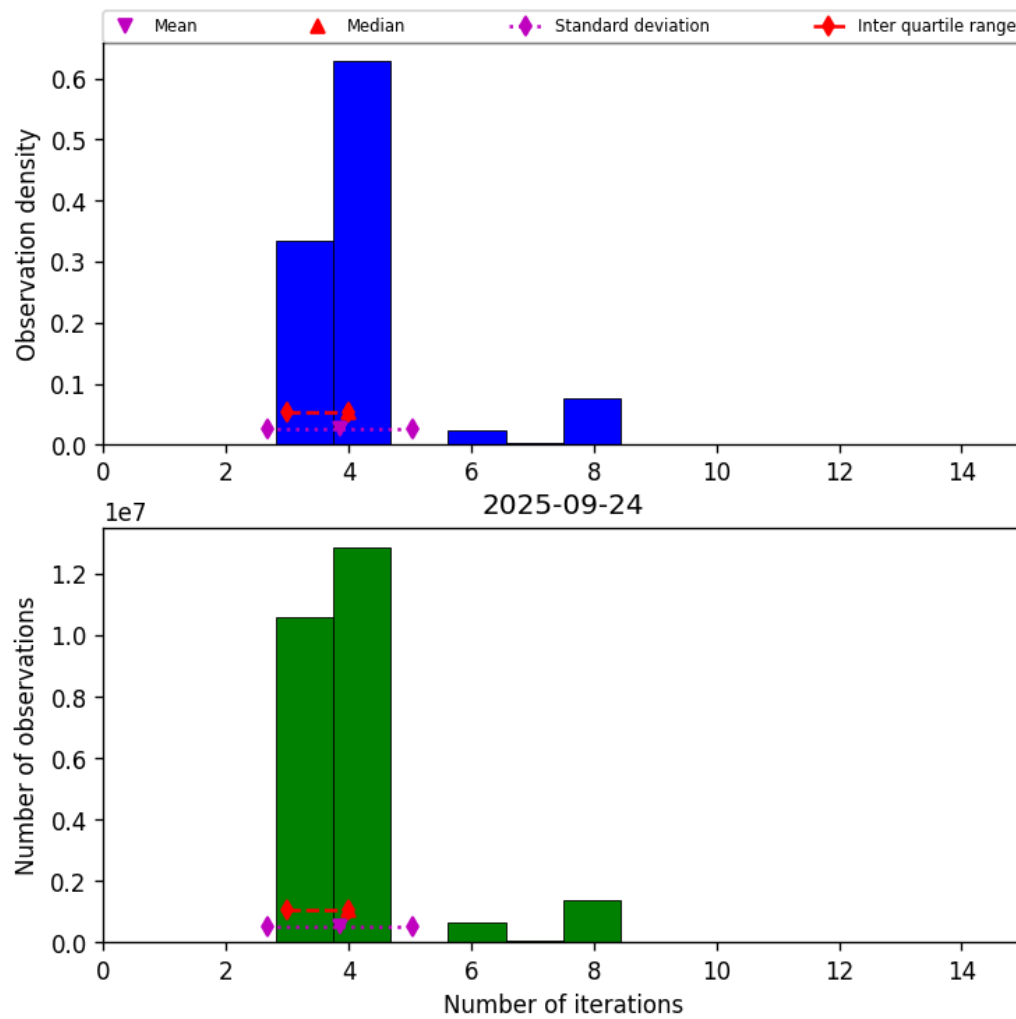
Figure 32: Histogram of “Number of iterations” for 2025-09-24 to 2025-09-25
