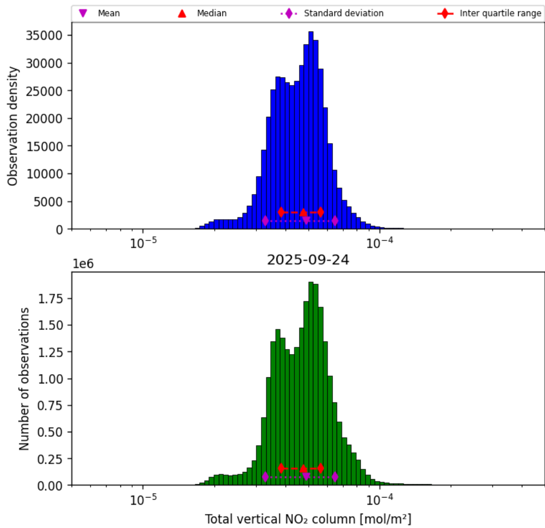
Figure 36: Histogram of “Total vertical NO 2 column” for 2025-09-24 to 2025-09-25
