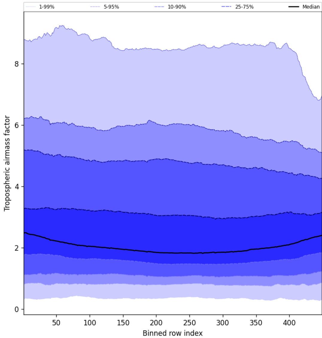
Figure 46: Along track statistics of “Tropospheric airmass factor” for 2025-09-24 to 2025-09-25
