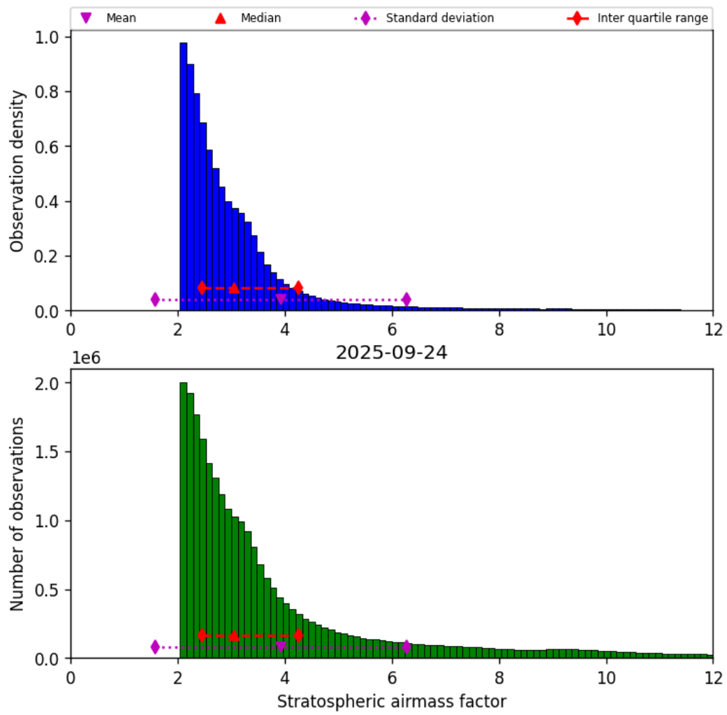
Figure 42: Histogram of “Stratospheric airmass factor” for 2025-09-24 to 2025-09-25
