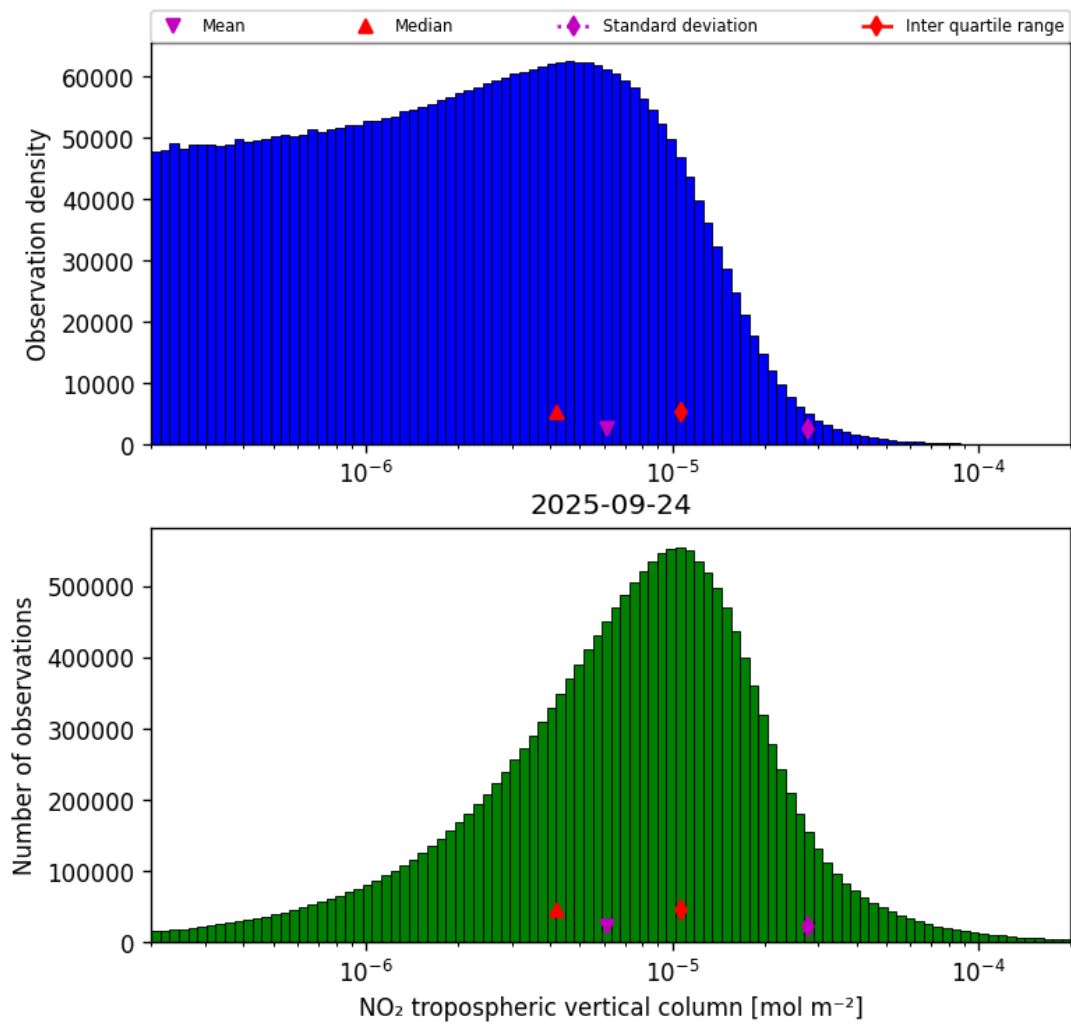
Figure 27: Histogram of “NO 2 tropospheric vertical column” for 2025-09-24 to 2025-09-25
