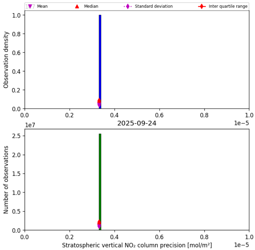
Figure 35: Histogram of “Stratospheric vertical NO 2 column precision” for 2025-09-24 to 2025-09-25
