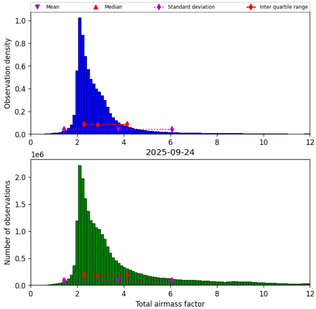
Figure 30: Histogram of “Total airmass factor” for 2025-09-24 to 2025-09-25
