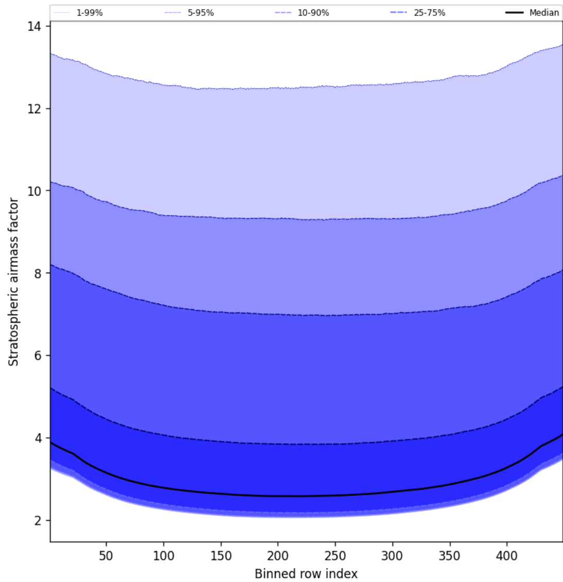
Figure 59: Along track statistics of “Stratospheric airmass factor” for 2025-09-24 to 2025-09-25
