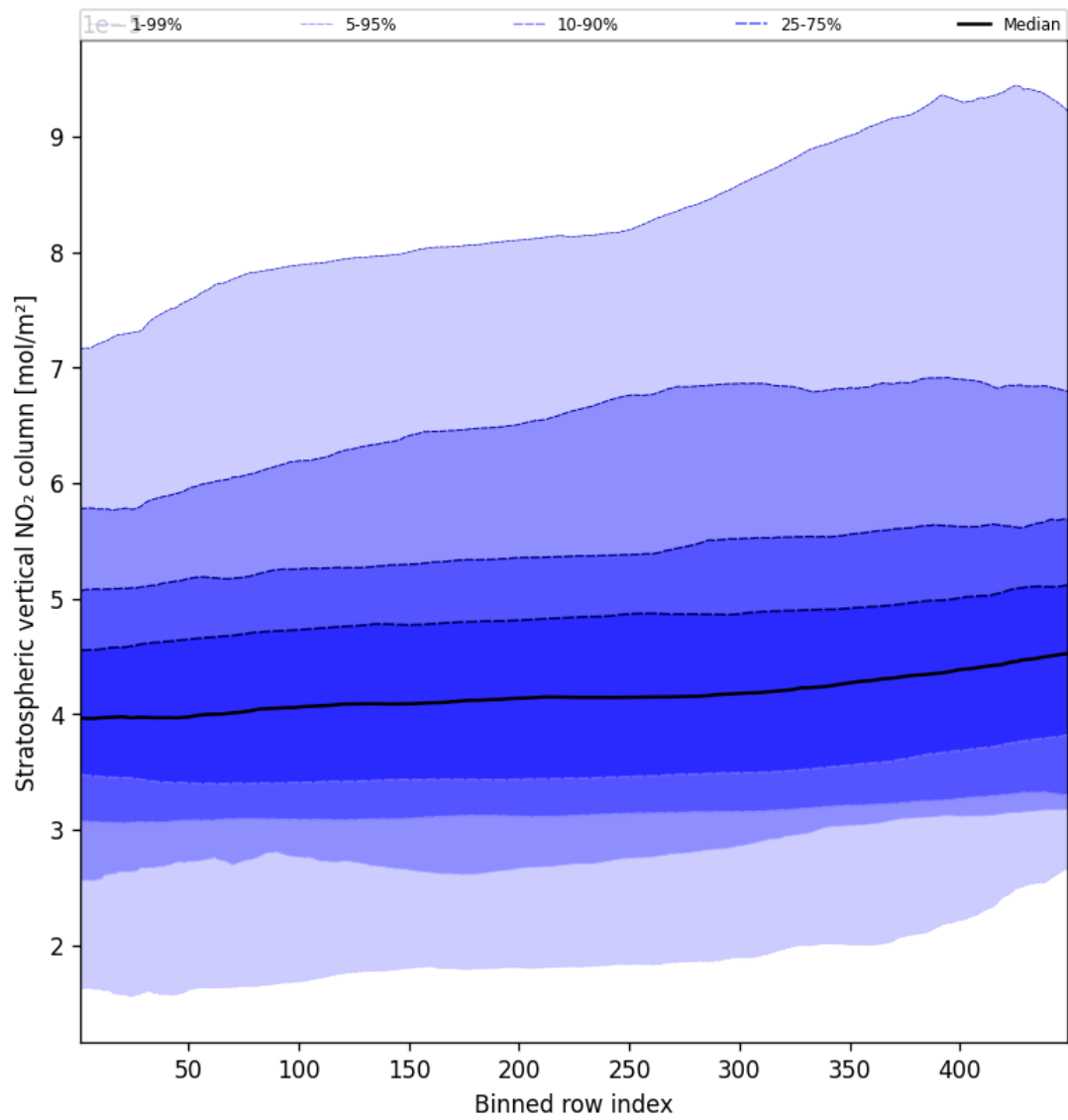
Figure 51: Along track statistics of “Stratospheric vertical NO 2 column” for 2025-09-24 to 2025-09-25
