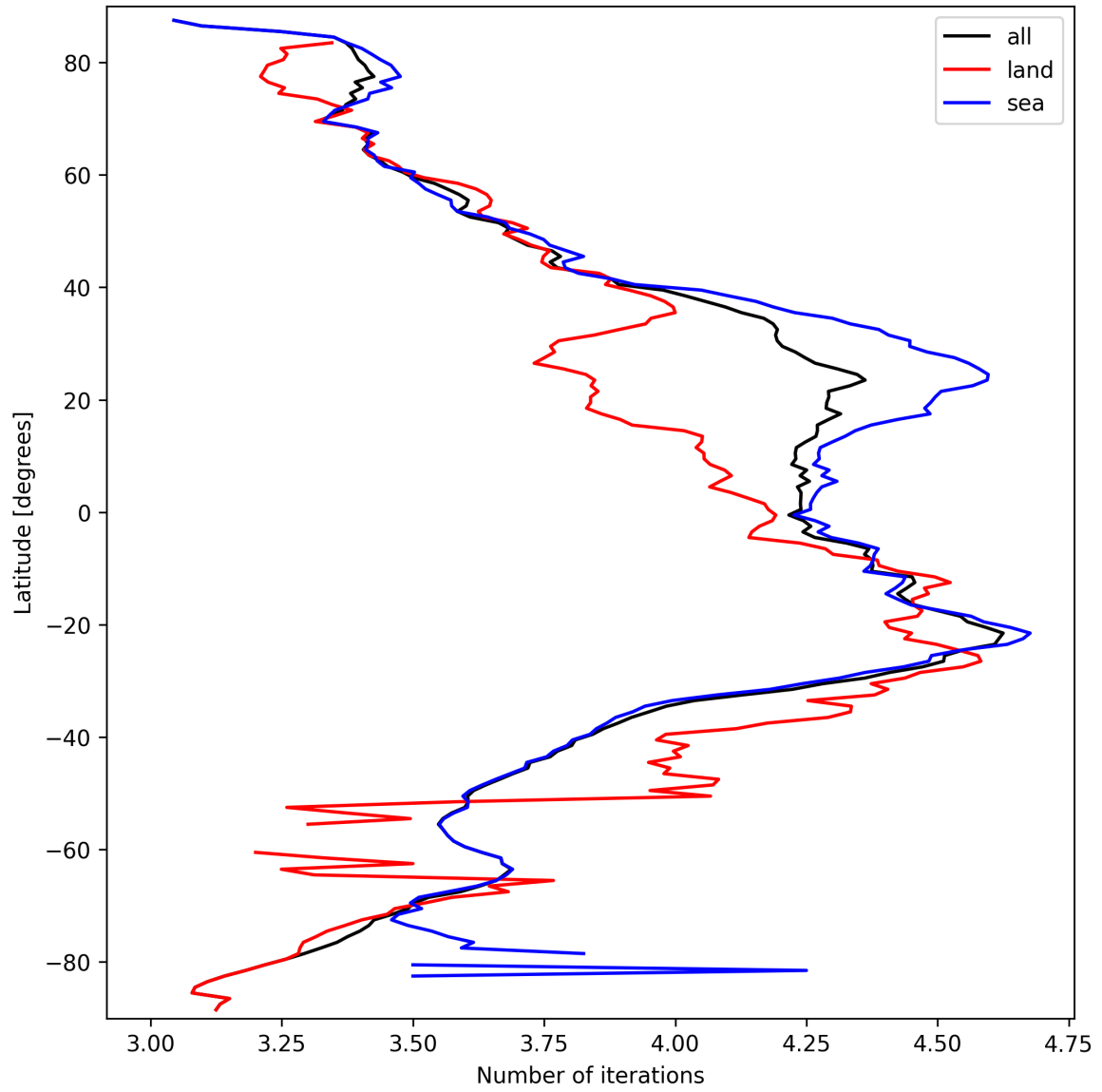
Figure 15: Zonal average of “Number of iterations” for 2025-09-24 to 2025-09-25.
