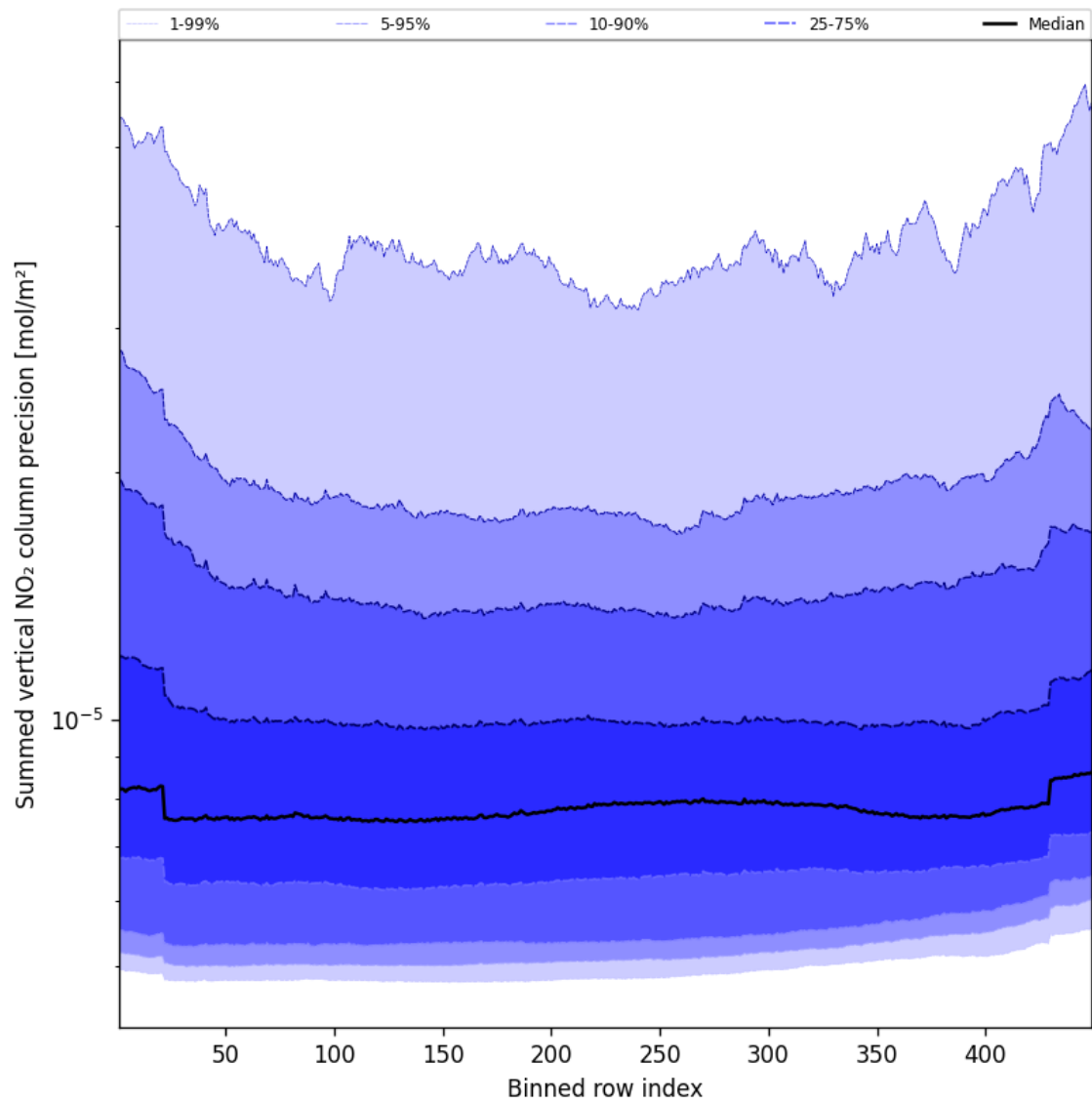
Figure 56: Along track statistics of “Summed vertical NO 2 column precision” for 2025-09-24 to 2025-09-25
