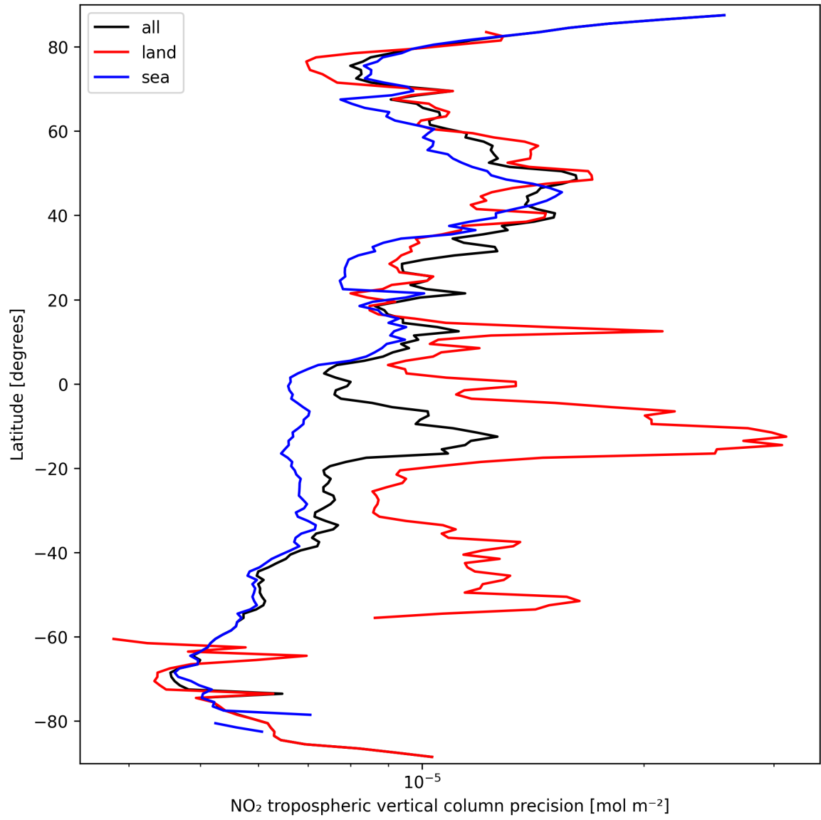
Figure 11: Zonal average of “NO 2 tropospheric vertical column precision” for 2025-09-24 to 2025-09-25.
