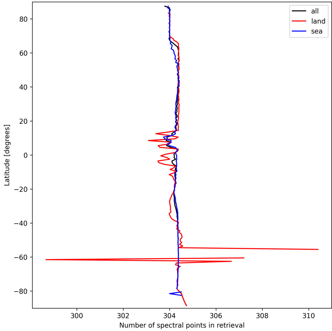
Figure 14: Zonal average of “Number of spectral points in retrieval” for 2025-09-24 to 2025-09-25.
