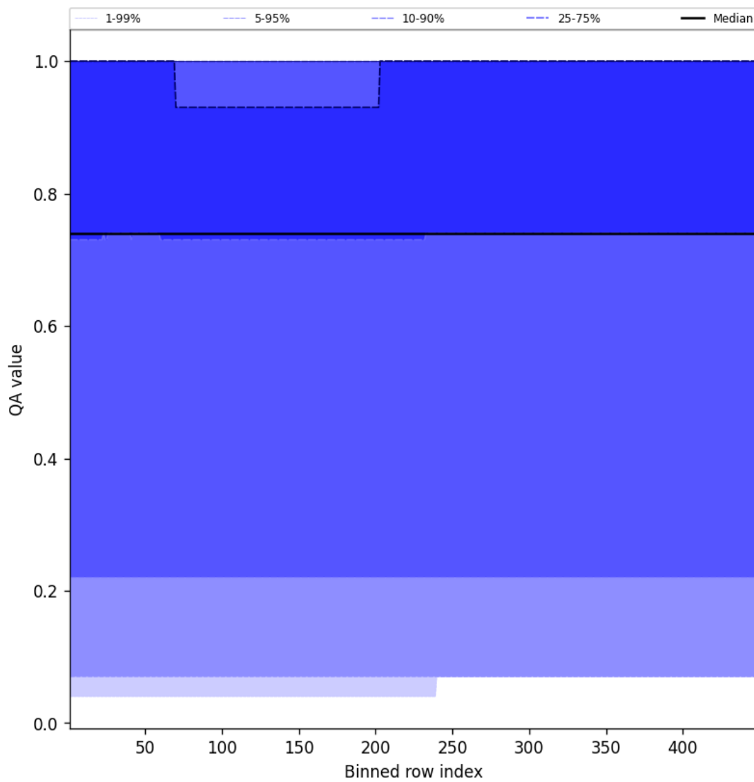
Figure 43: Along track statistics of “QA value” for 2025-09-24 to 2025-09-25
