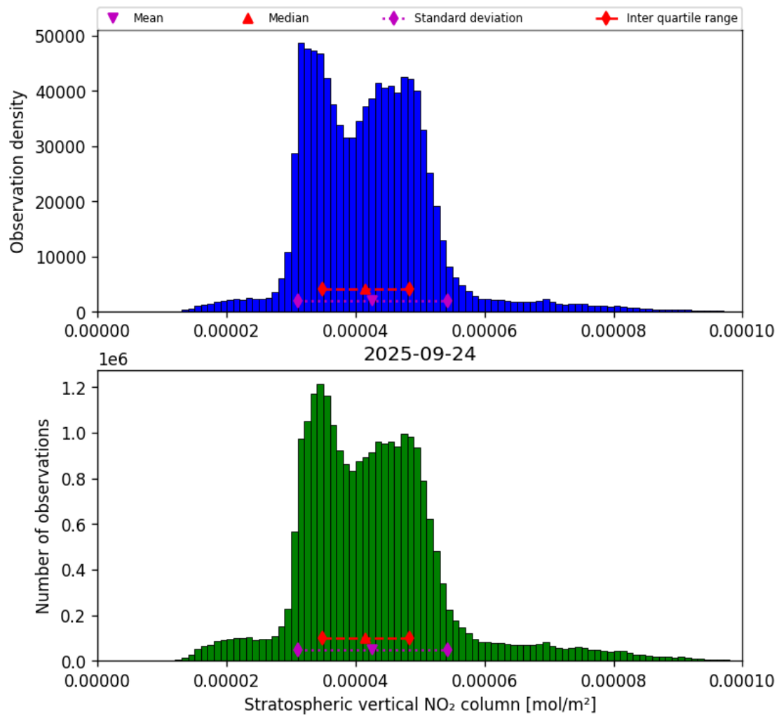
Figure 34: Histogram of “Stratospheric vertical NO 2 column” for 2025-09-24 to 2025-09-25
