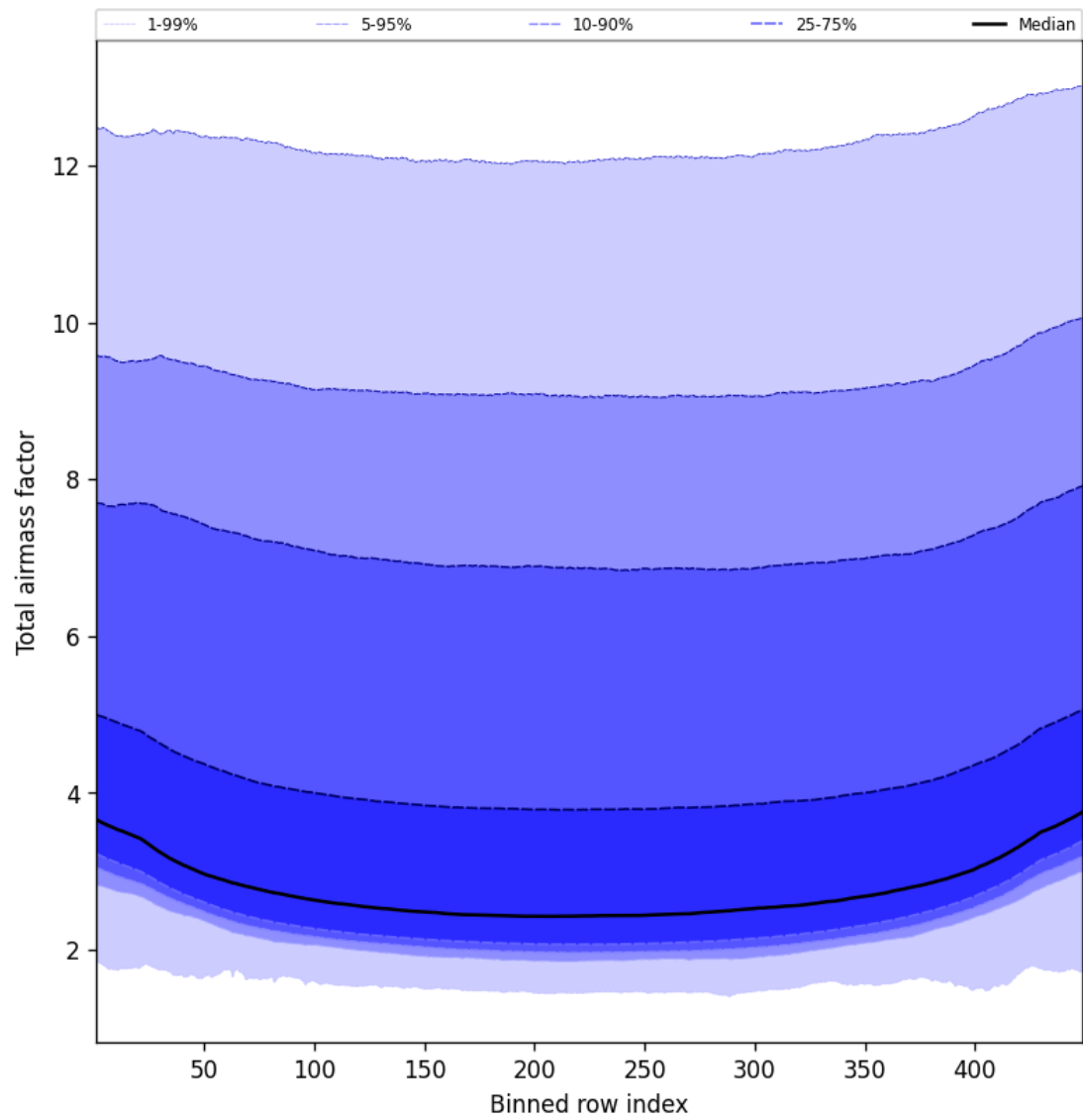
Figure 47: Along track statistics of “Total airmass factor” for 2025-09-24 to 2025-09-25
