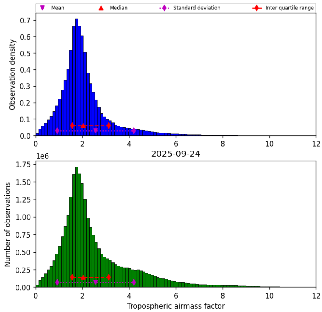
Figure 29: Histogram of “Tropospheric airmass factor” for 2025-09-24 to 2025-09-25
