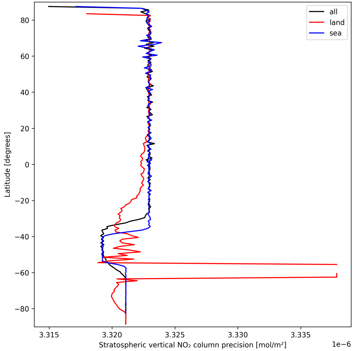
Figure 18: Zonal average of “Stratospheric vertical NO 2 column precision” for 2025-09-24 to 2025-09-25.
