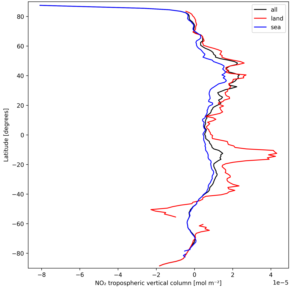
Figure 10: Zonal average of “NO 2 tropospheric vertical column” for 2025-09-24 to 2025-09-25.
