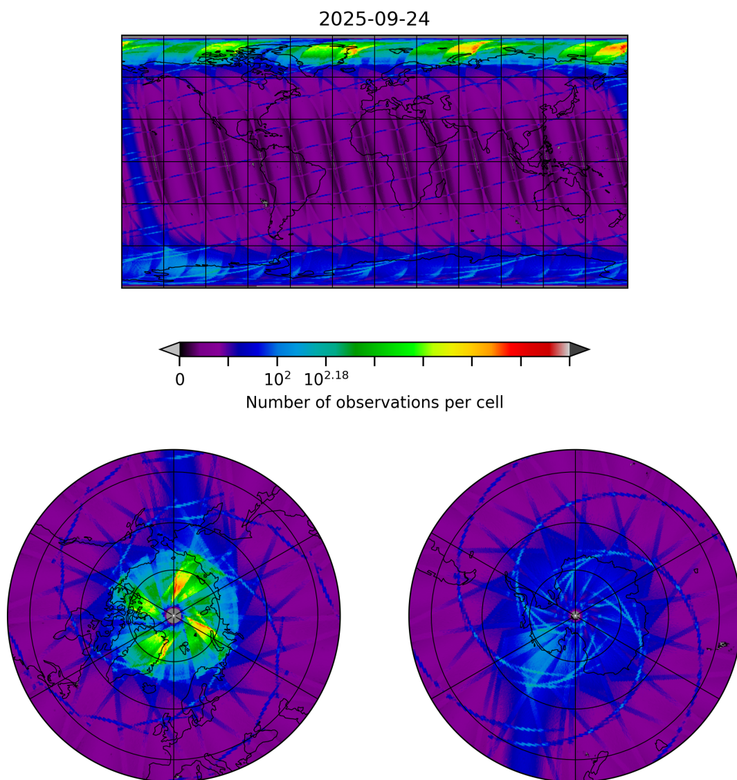
Figure 8: Map of the number of observations for 2025-09-24 to 2025-09-25
