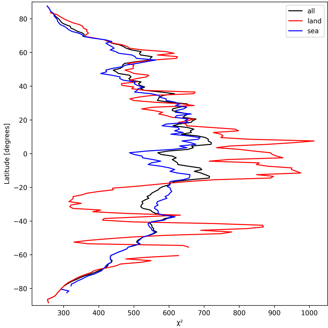
Figure 23: Zonal average of “ \chi^2 ” for 2025-09-24 to 2025-09-25.
