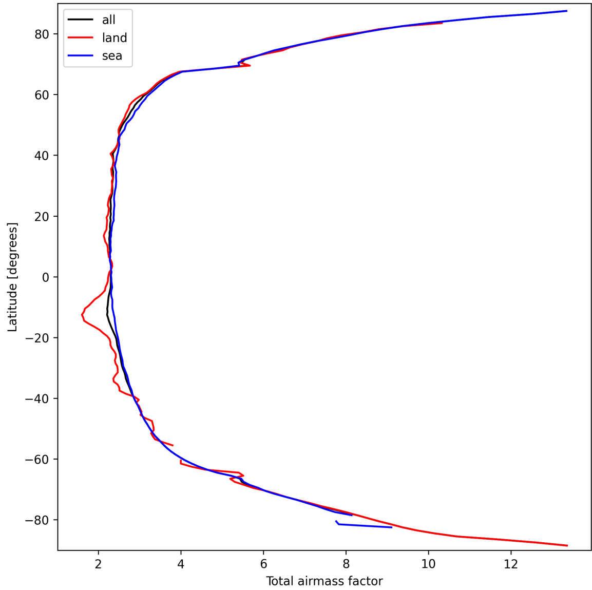
Figure 13: Zonal average of “Total airmass factor” for 2025-09-24 to 2025-09-25.
