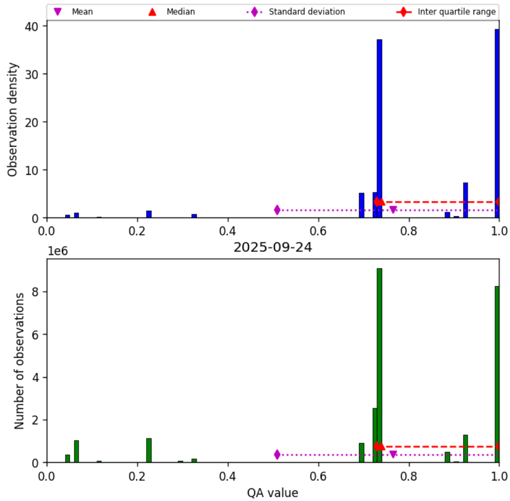
Figure 26: Histogram of “QA value” for 2025-09-24 to 2025-09-25
