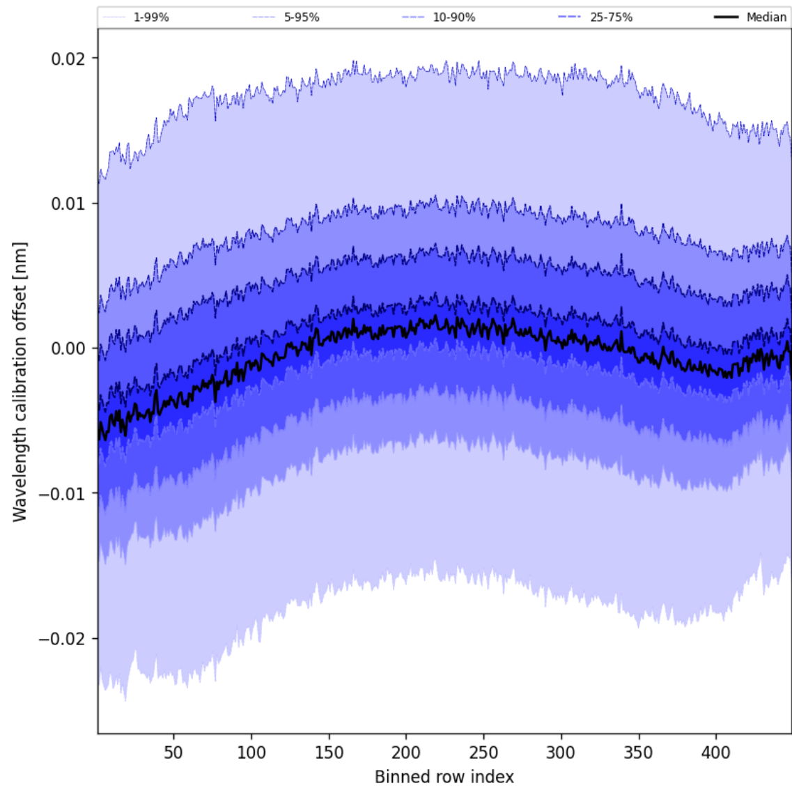
Figure 50: Along track statistics of “Wavelength calibration offset” for 2025-09-24 to 2025-09-25
