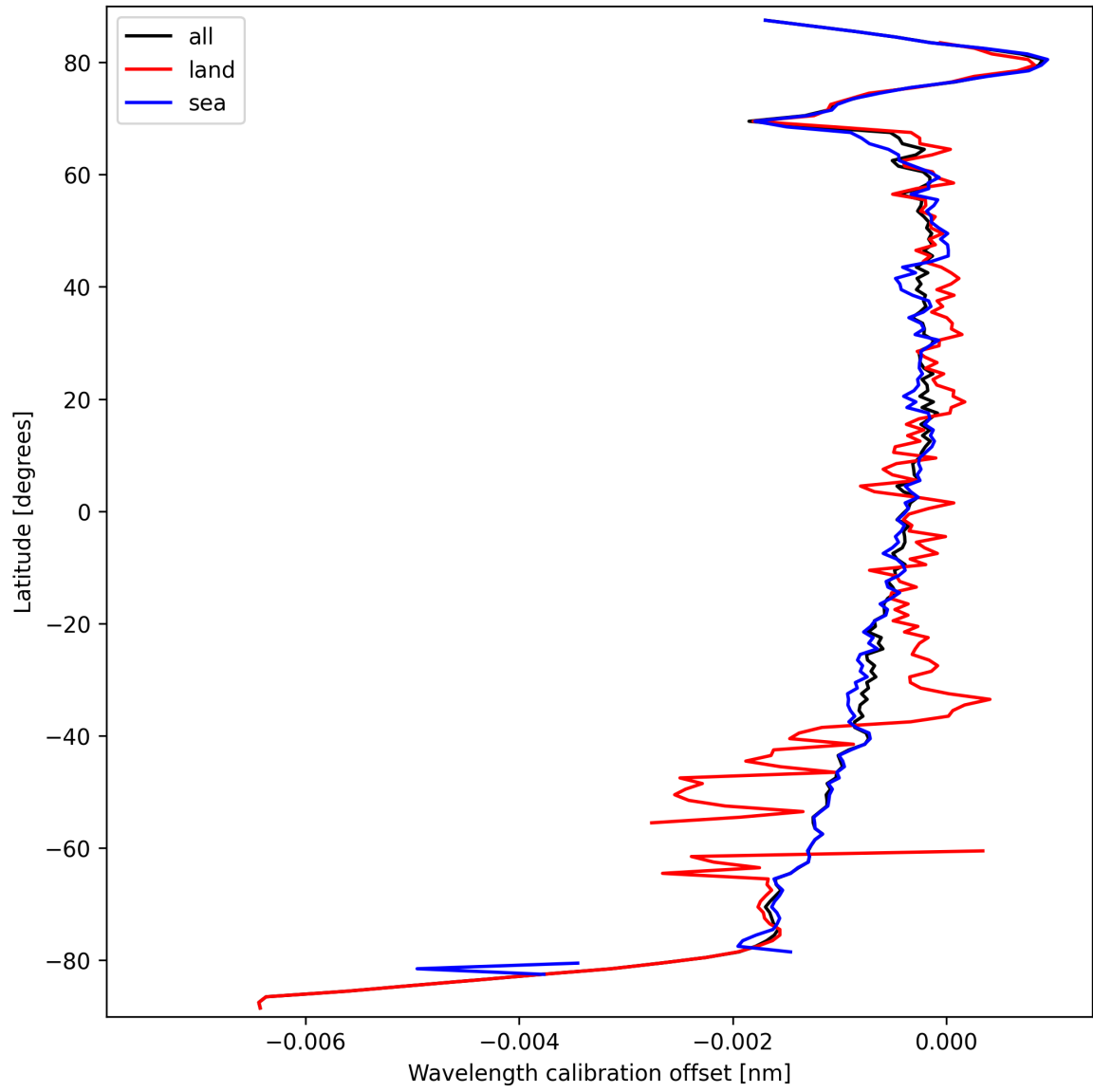
Figure 16: Zonal average of “Wavelength calibration offset” for 2025-09-24 to 2025-09-25.
