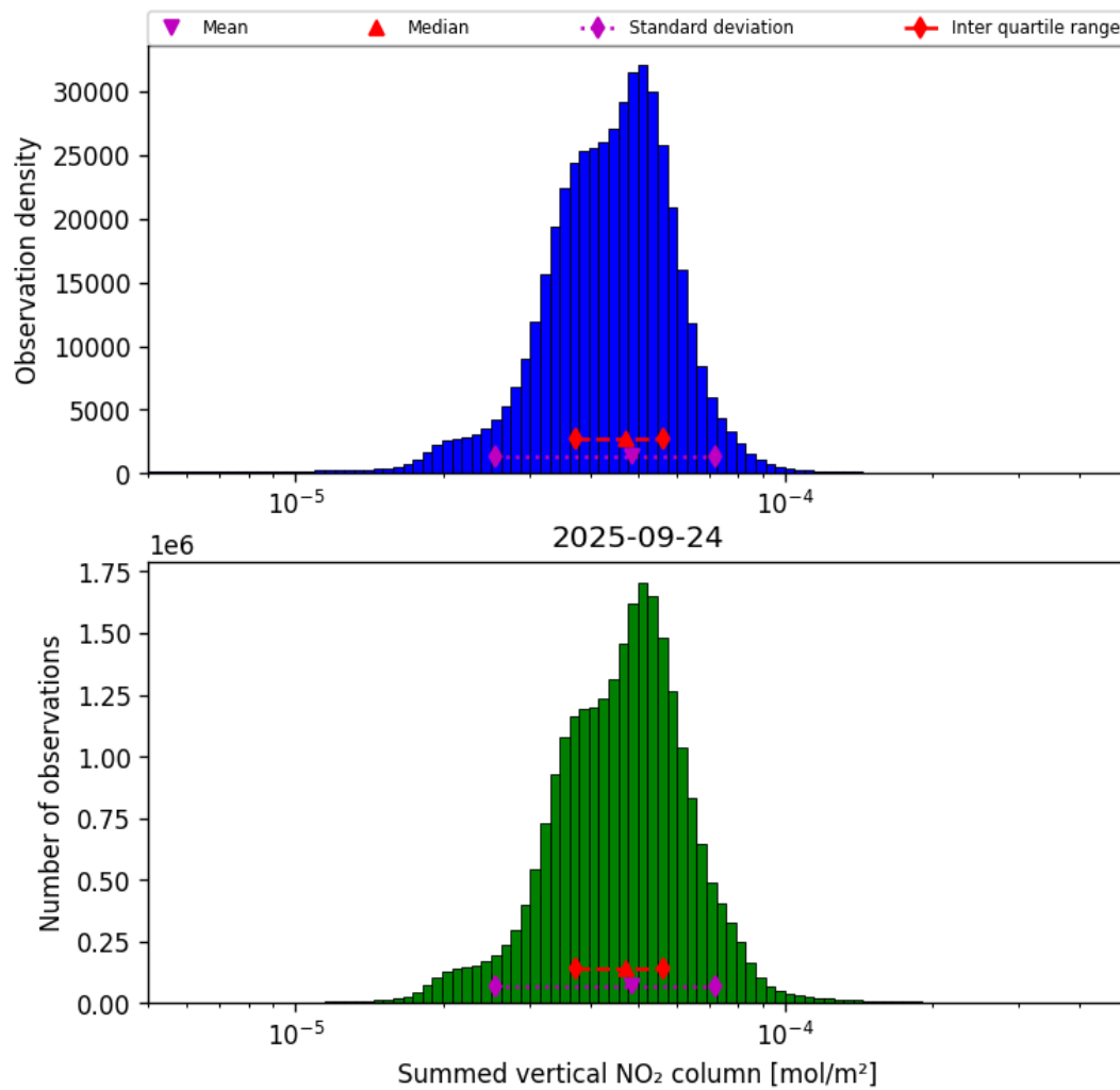
Figure 38: Histogram of "Summed vertical NO 2 column" for 2025-09-24 to 2025-09-25
