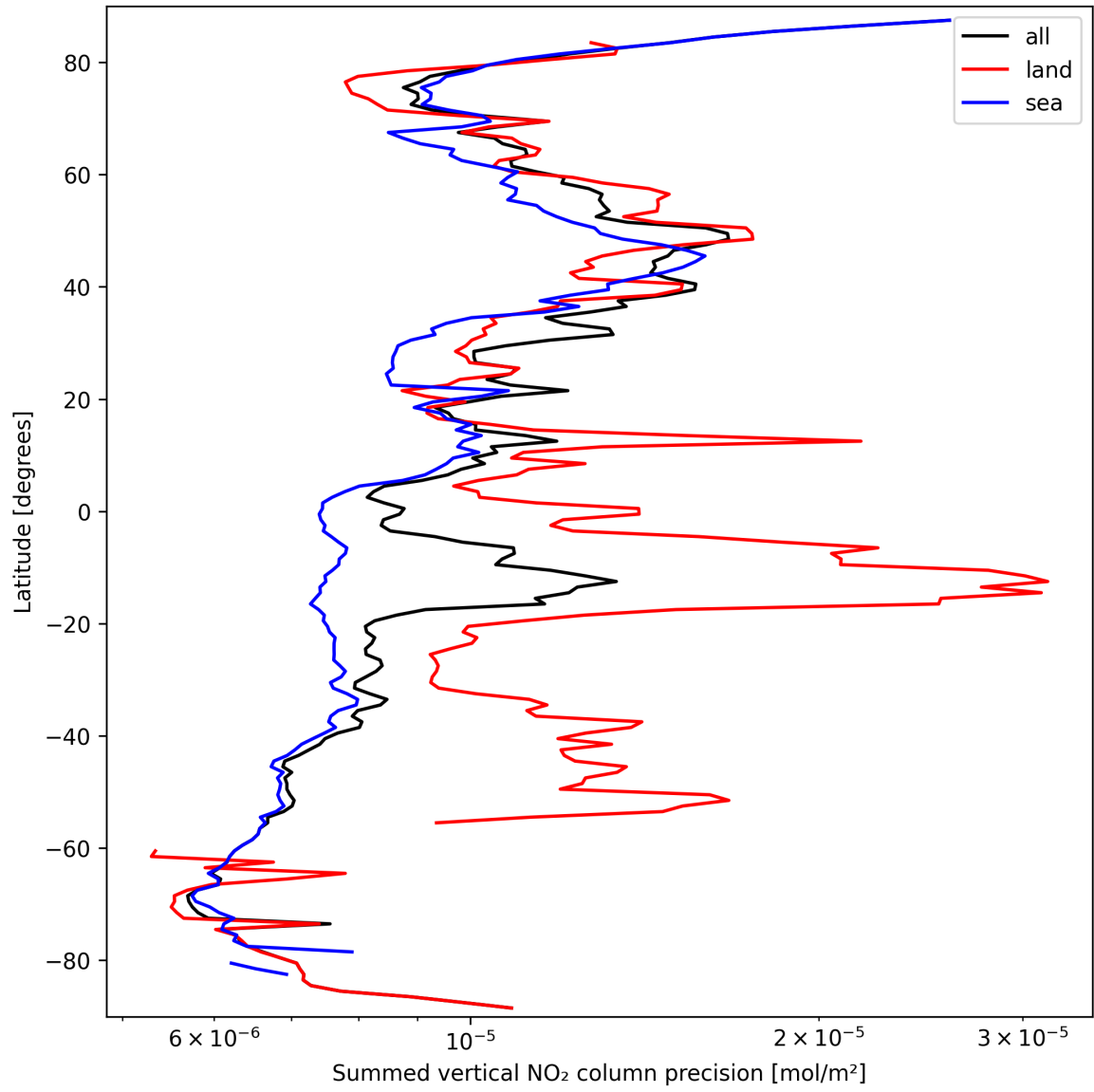
Figure 22: Zonal average of “Summed vertical NO 2 column precision” for 2025-09-24 to 2025-09-25.
