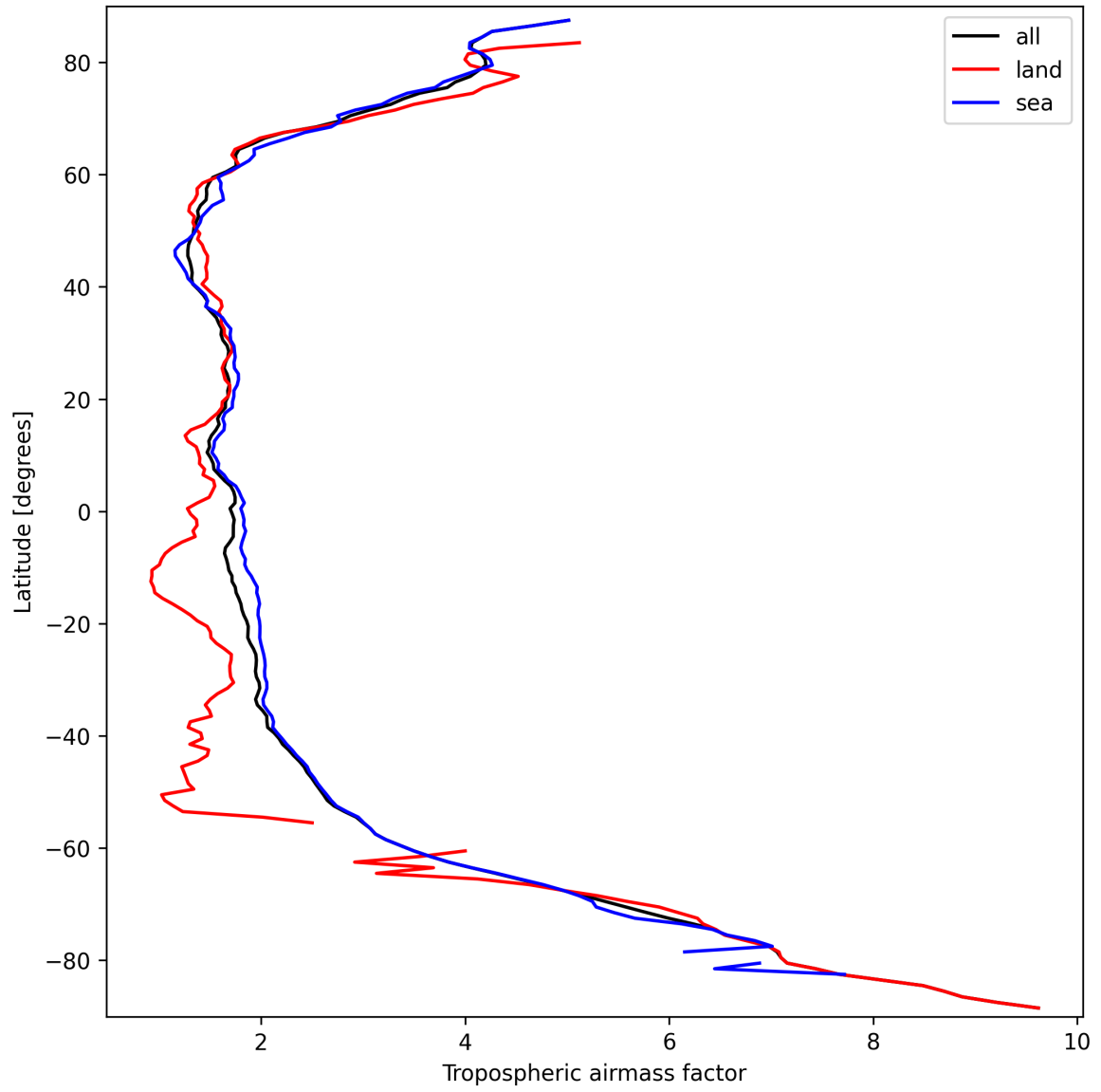
Figure 12: Zonal average of “Tropospheric airmass factor” for 2025-09-24 to 2025-09-25.
