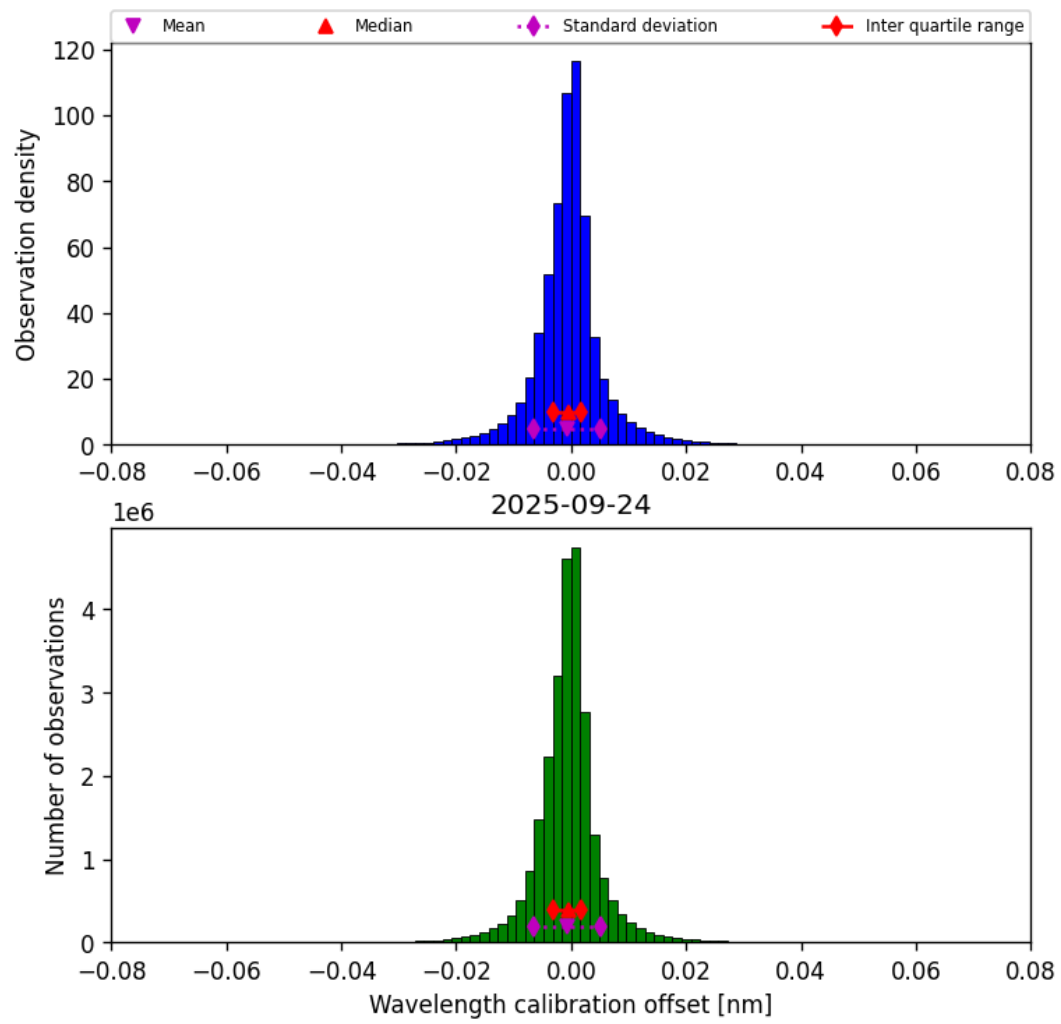
Figure 33: Histogram of “Wavelength calibration offset” for 2025-09-24 to 2025-09-25
