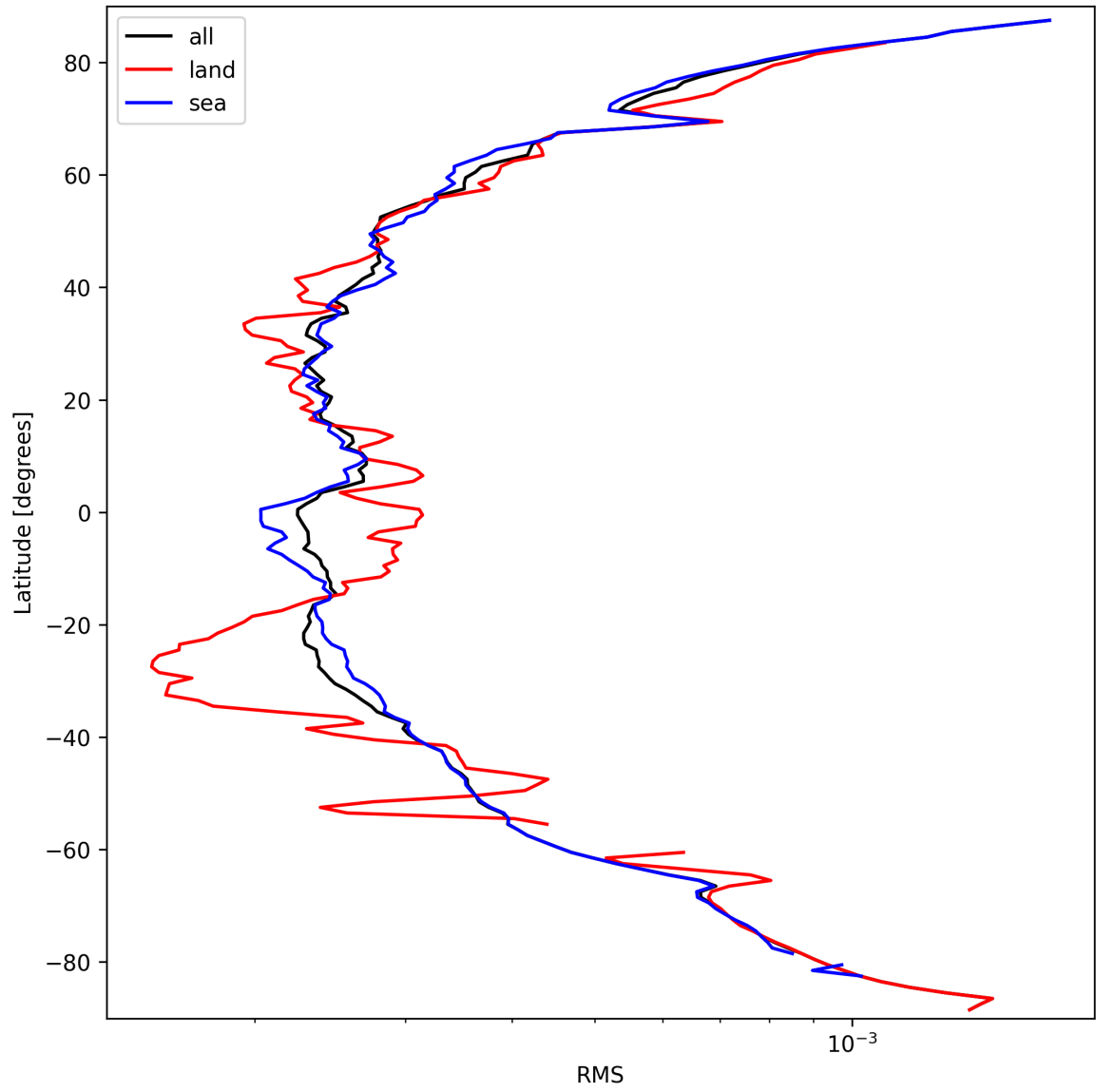
Figure 24: Zonal average of “RMS” for 2025-09-24 to 2025-09-25.
