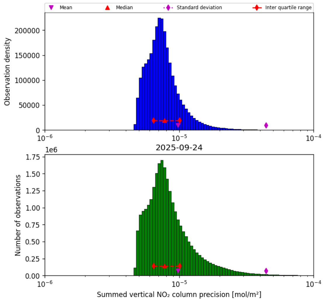
Figure 39: Histogram of “Summed vertical NO 2 column precision” for 2025-09-24 to 2025-09-25
