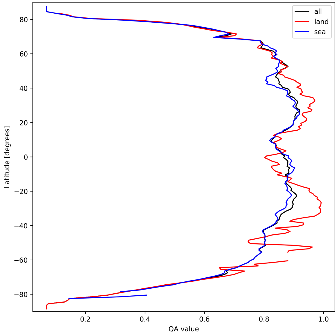
Figure 9: Zonal average of “QA value” for 2025-09-24 to 2025-09-25.
