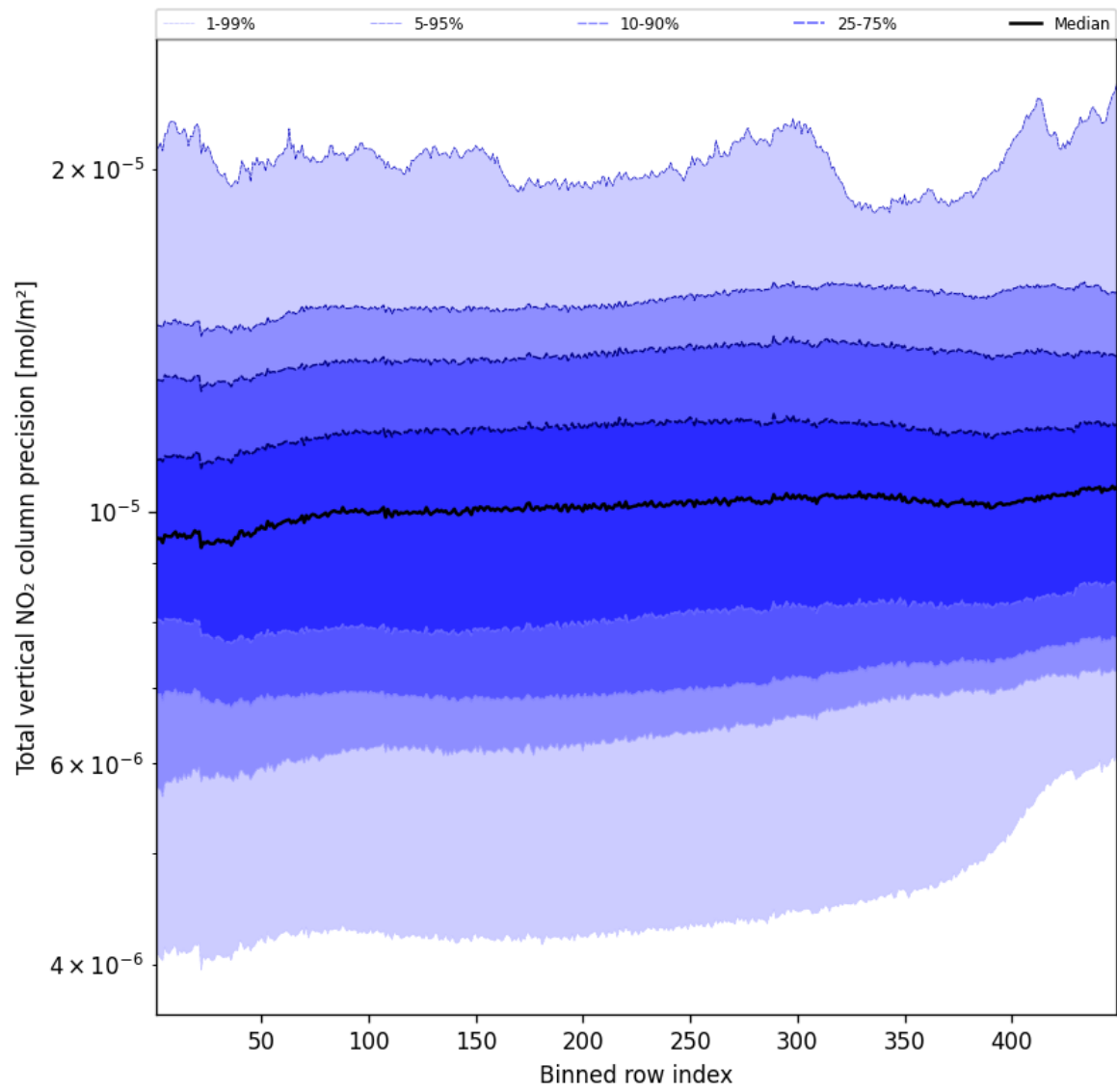
Figure 54: Along track statistics of "Total vertical NO 2 column precision" for 2025-09-24 to 2025-09-25
