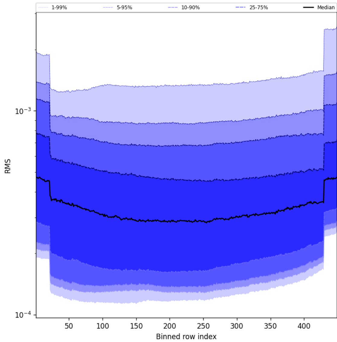
Figure 58: Along track statistics of “RMS” for 2025-09-24 to 2025-09-25
