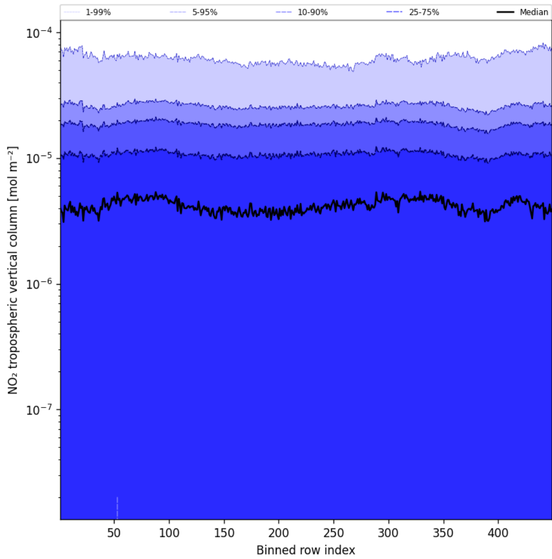
Figure 44: Along track statistics of “NO 2 tropospheric vertical column” for 2025-09-24 to 2025-09-25
