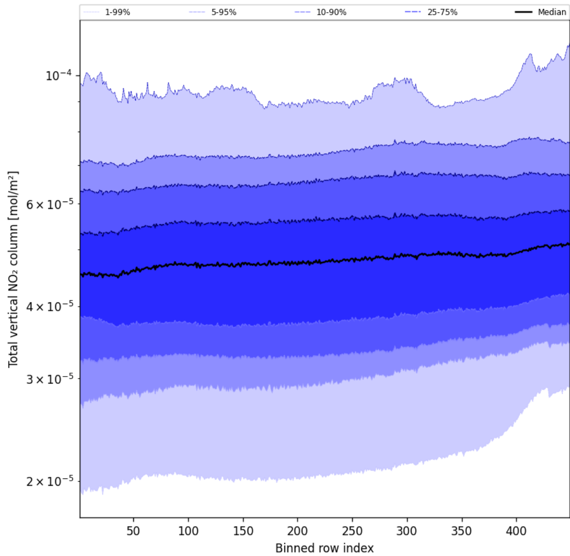
Figure 53: Along track statistics of “Total vertical NO 2 column” for 2025-09-24 to 2025-09-25
