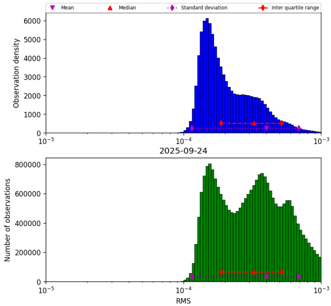
Figure 41: Histogram of “RMS” for 2025-09-24 to 2025-09-25
