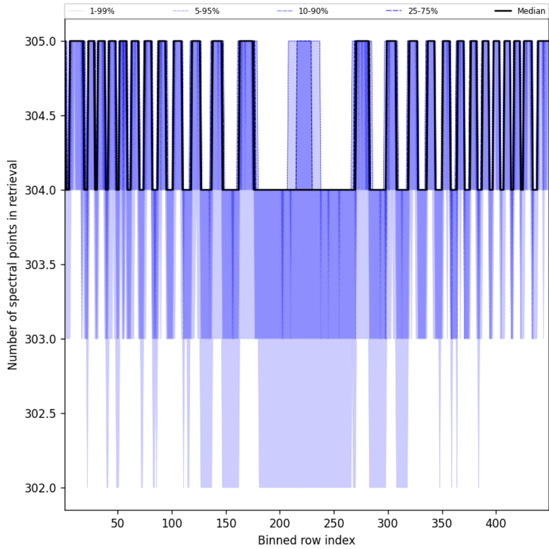
Figure 48: Along track statistics of “Number of spectral points in retrieval” for 2025-09-24 to 2025-09-25
