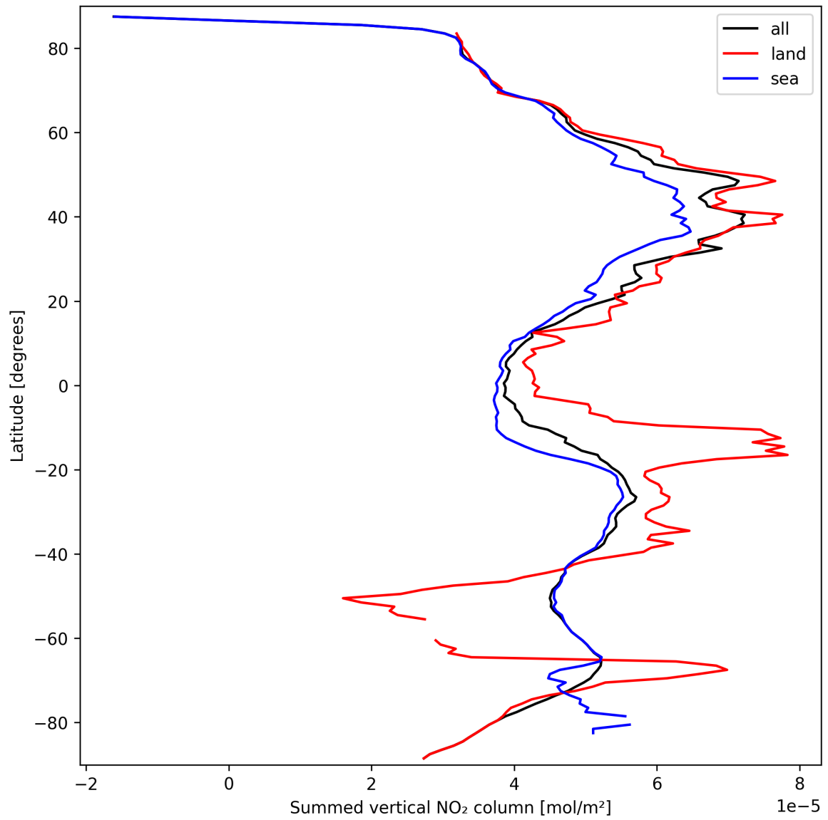
Figure 21: Zonal average of “Summed vertical NO 2 column” for 2025-09-24 to 2025-09-25.
