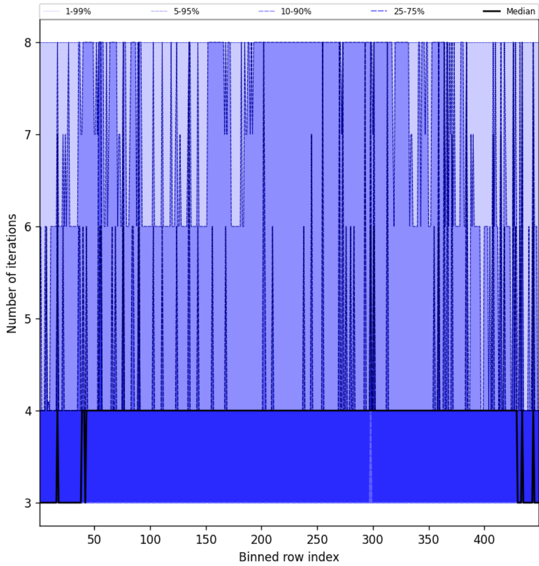
Figure 49: Along track statistics of “Number of iterations” for 2025-09-24 to 2025-09-25
