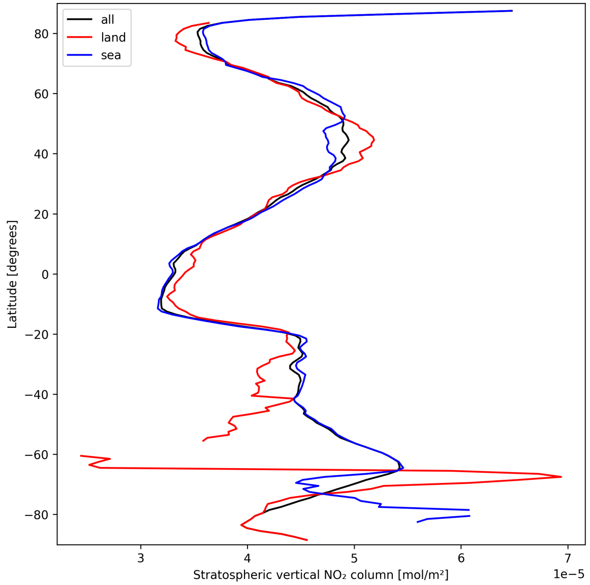
Figure 17: Zonal average of “Stratospheric vertical NO 2 column” for 2025-09-24 to 2025-09-25.
