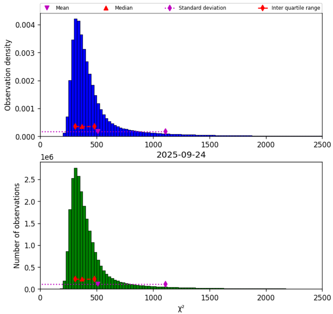
Figure 40: Histogram of “ \chi^2 ” for 2025-09-24 to 2025-09-25
