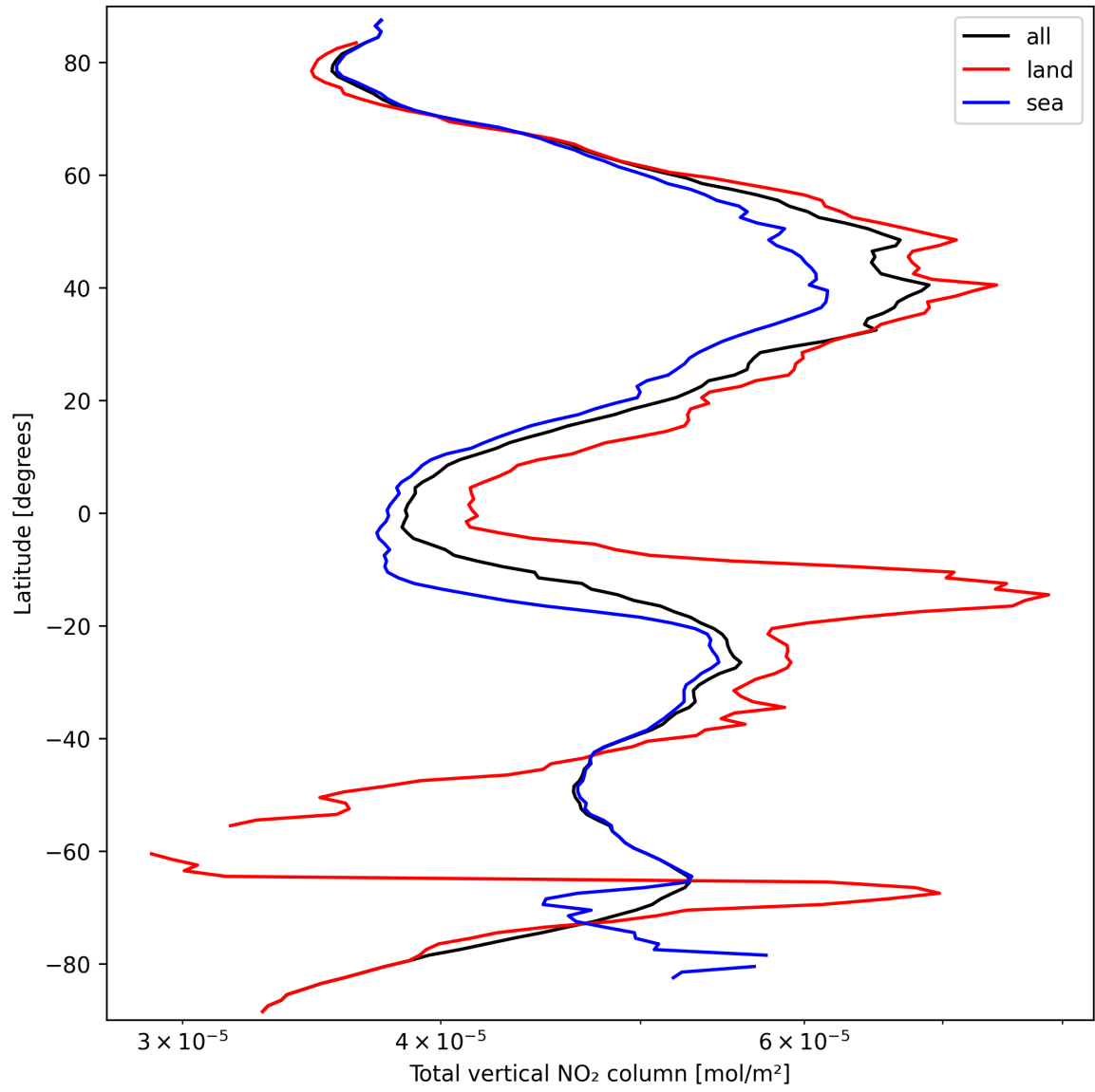
Figure 19: Zonal average of “Total vertical NO 2 column” for 2025-09-24 to 2025-09-25.
