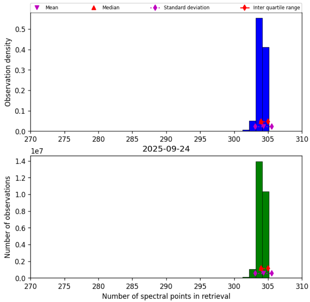
Figure 31: Histogram of “Number of spectral points in retrieval” for 2025-09-24 to 2025-09-25
