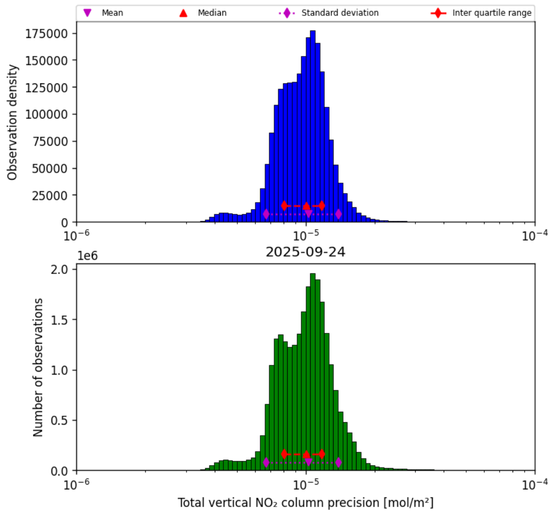
Figure 37: Histogram of “Total vertical NO 2 column precision” for 2025-09-24 to 2025-09-25
