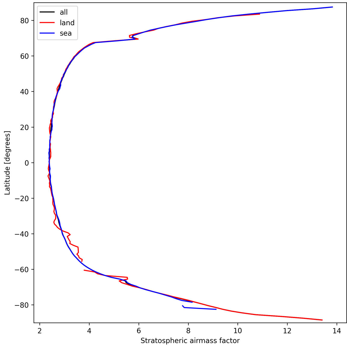
Figure 25: Zonal average of “Stratospheric air mass factor” for 2025-09-24 to 2025-09-25.
