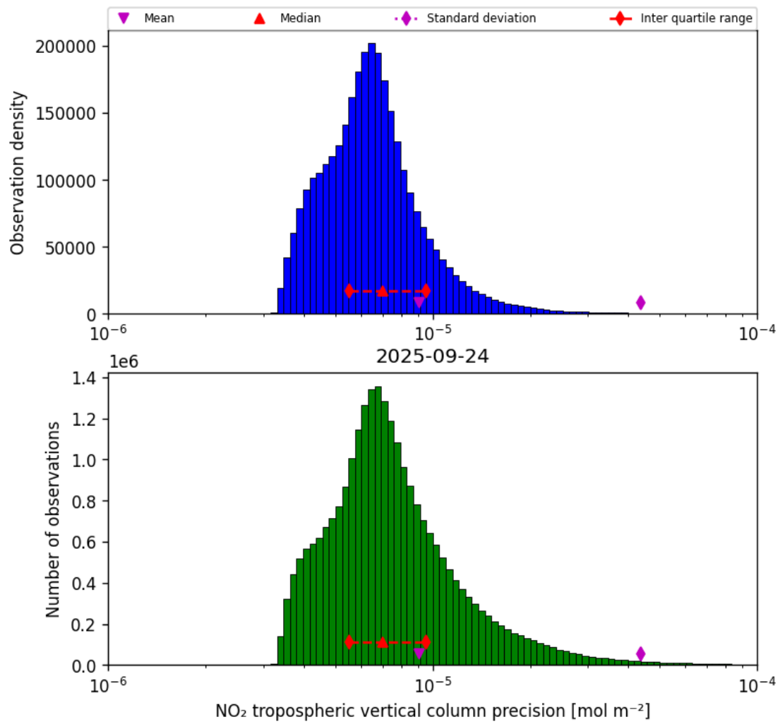
Figure 28: Histogram of “NO 2 tropospheric vertical column precision” for 2025-09-24 to 2025-09-25
