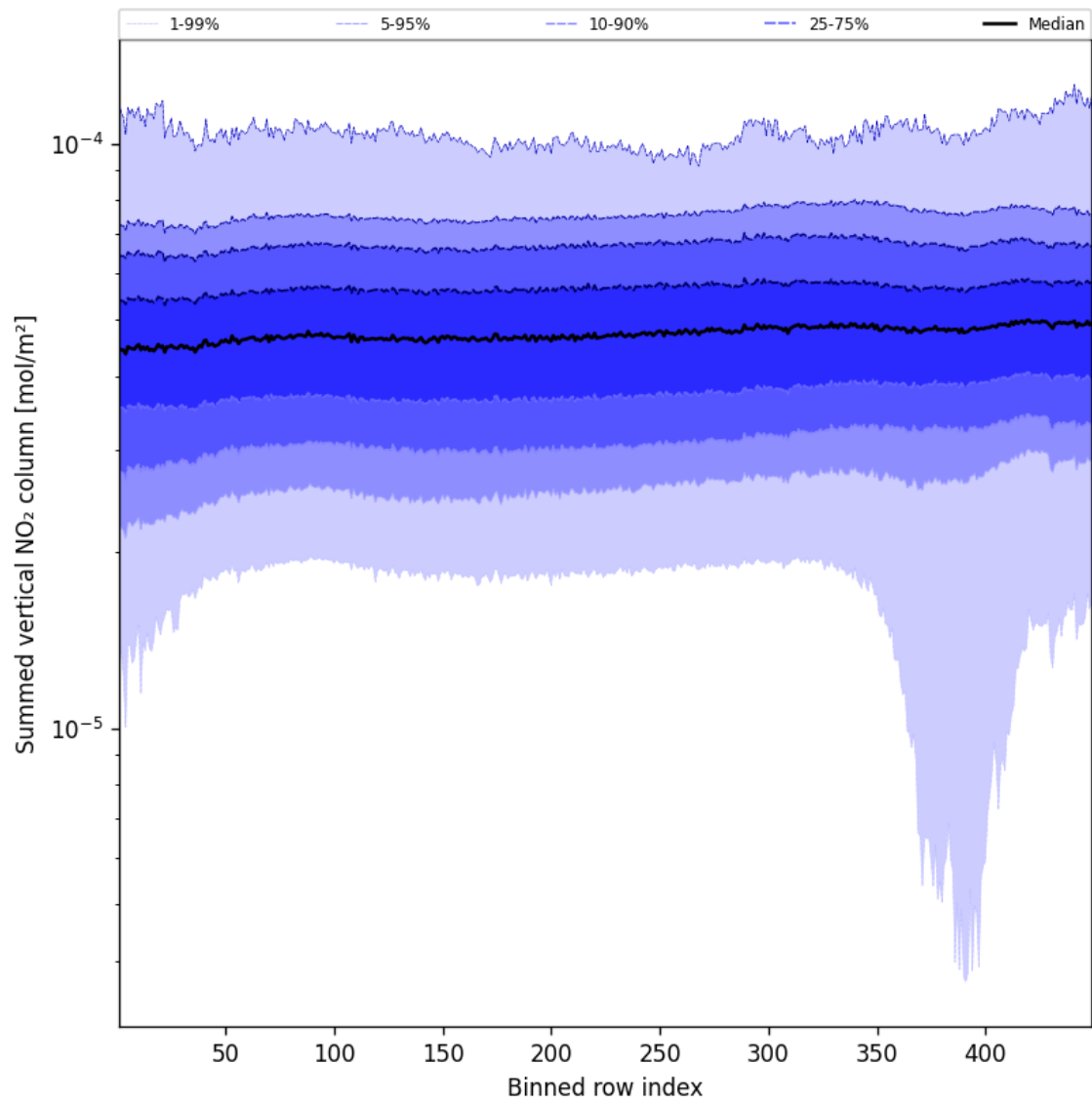
Figure 55: Along track statistics of “Summed vertical NO 2 column” for 2025-09-24 to 2025-09-25
