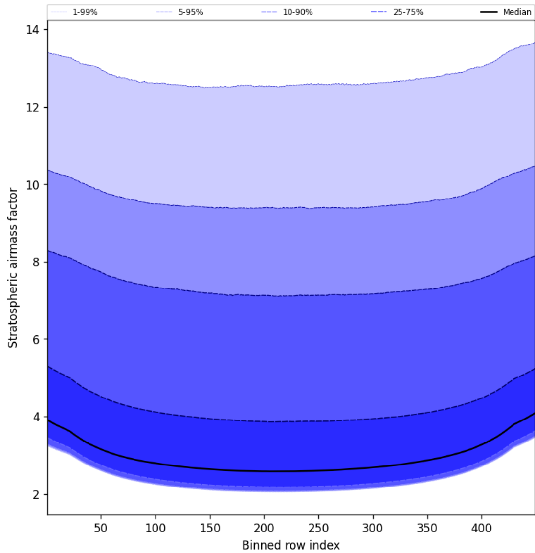
Figure 59: Along track statistics of “Stratospheric airmass factor” for 2025-09-26 to 2025-09-27
