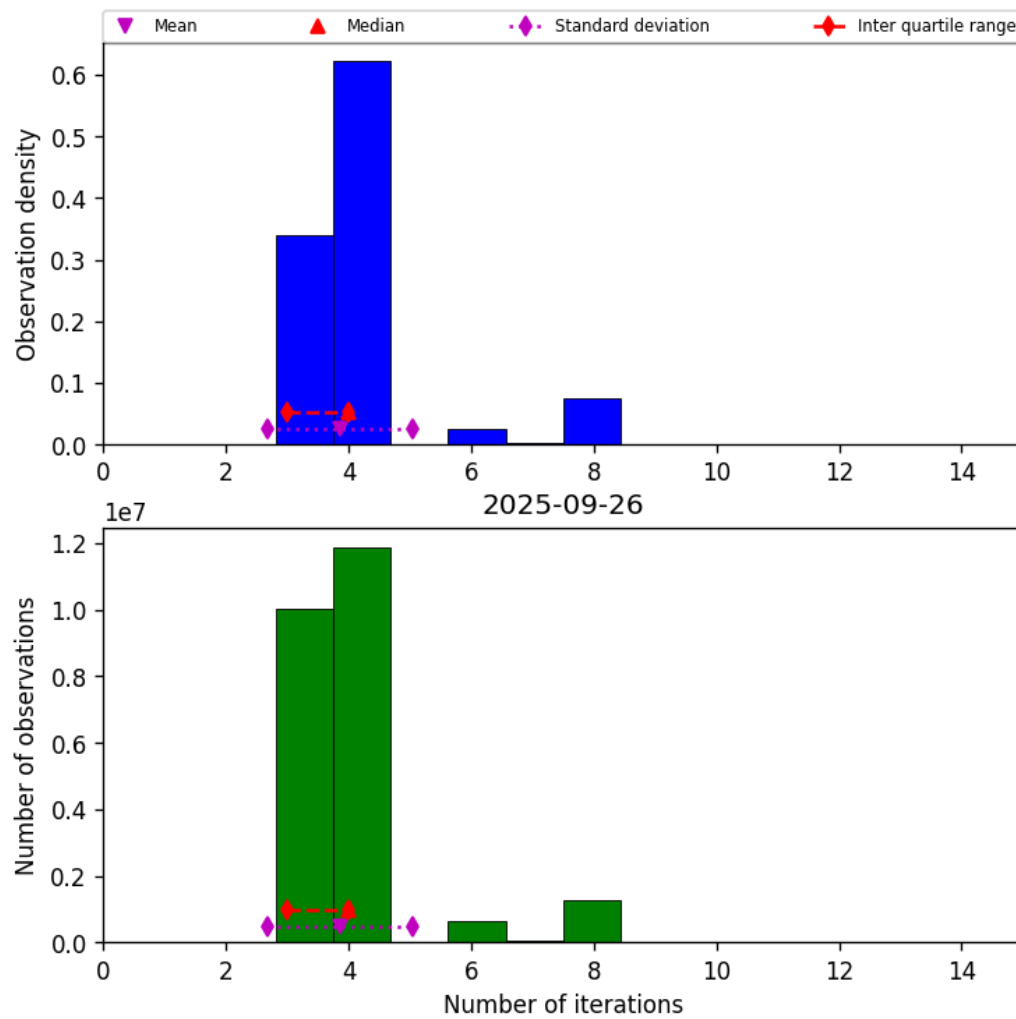
Figure 32: Histogram of “Number of iterations” for 2025-09-26 to 2025-09-27
