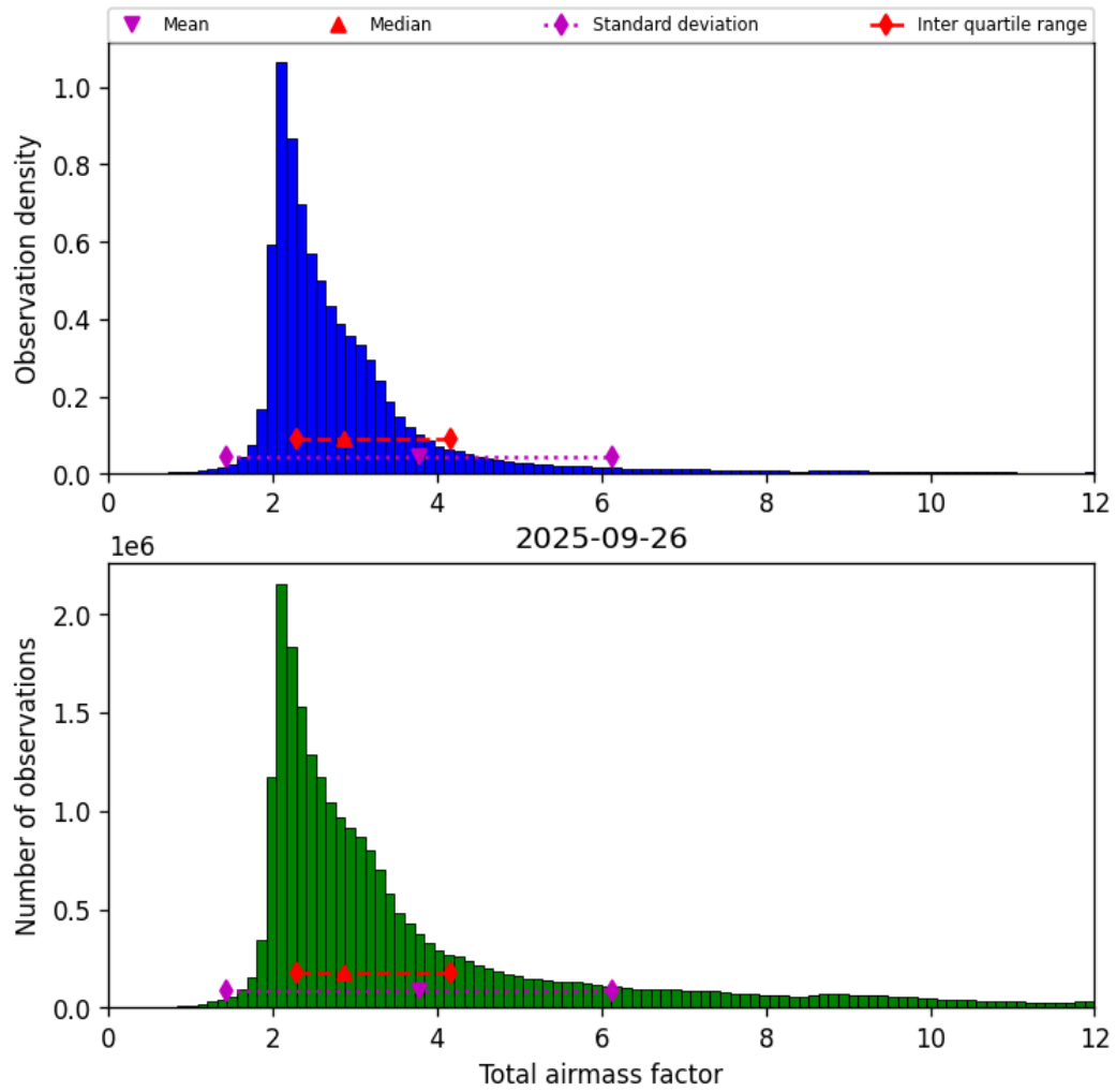
Figure 30: Histogram of “Total airmass factor” for 2025-09-26 to 2025-09-27
