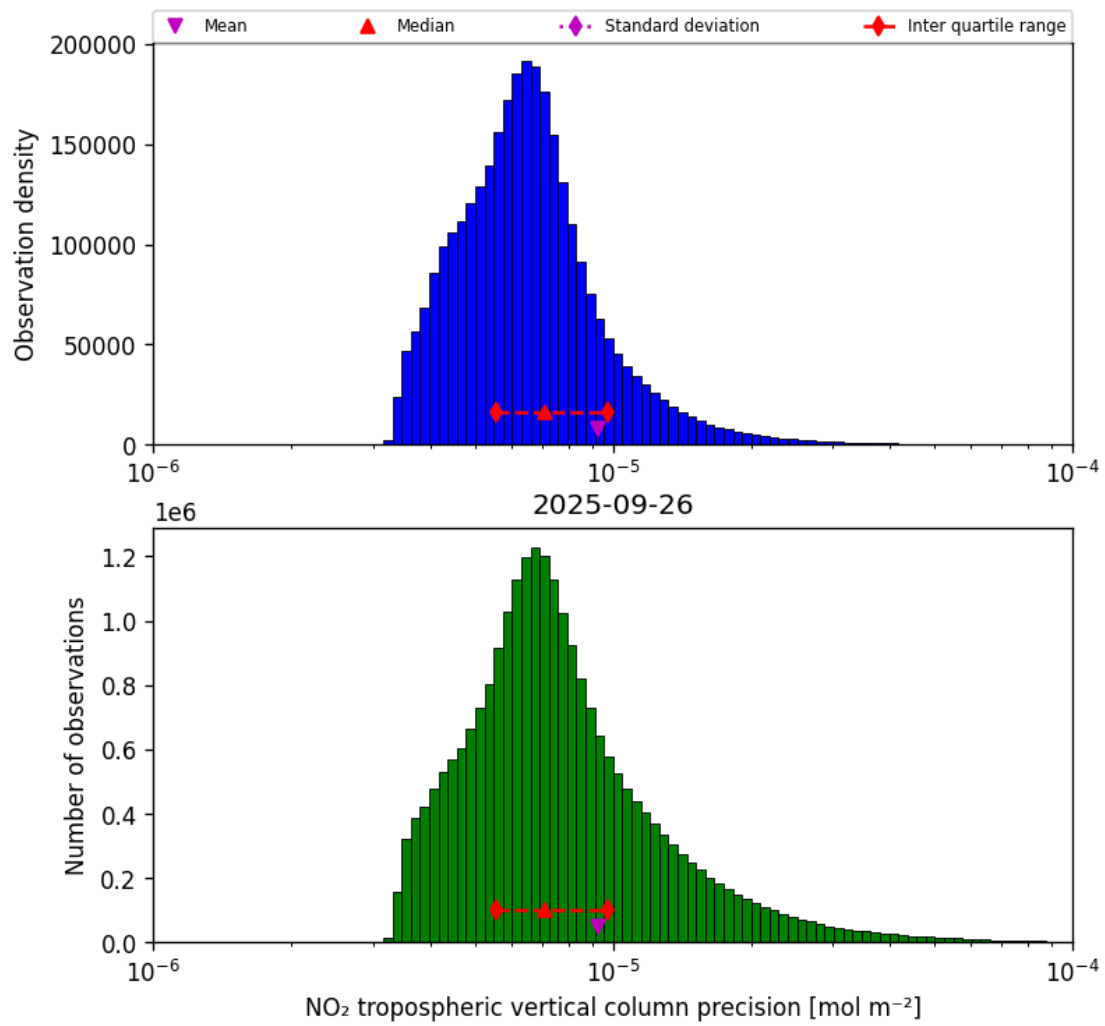
Figure 28: Histogram of “NO 2 tropospheric vertical column precision” for 2025-09-26 to 2025-09-27
