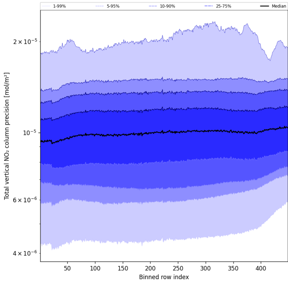
Figure 54: Along track statistics of “Total vertical NO 2 column precision” for 2025-09-26 to 2025-09-27
