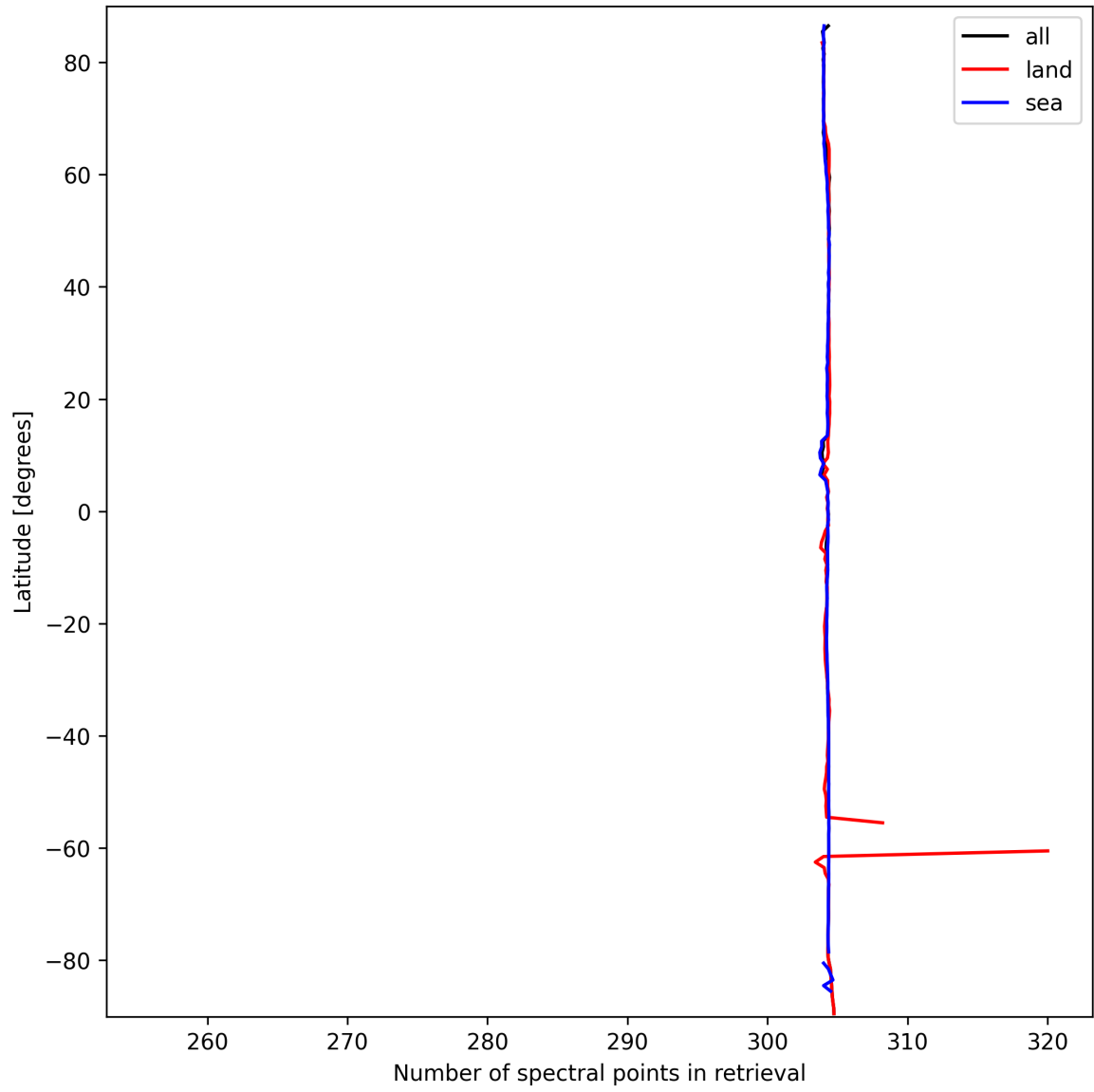
Figure 14: Zonal average of “Number of spectral points in retrieval” for 2025-09-26 to 2025-09-27.
