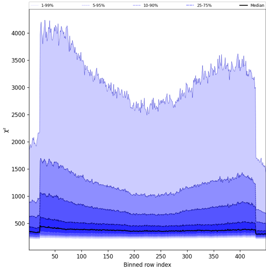
Figure 57: Along track statistics of “ \chi^2 ” for 2025-09-26 to 2025-09-27
