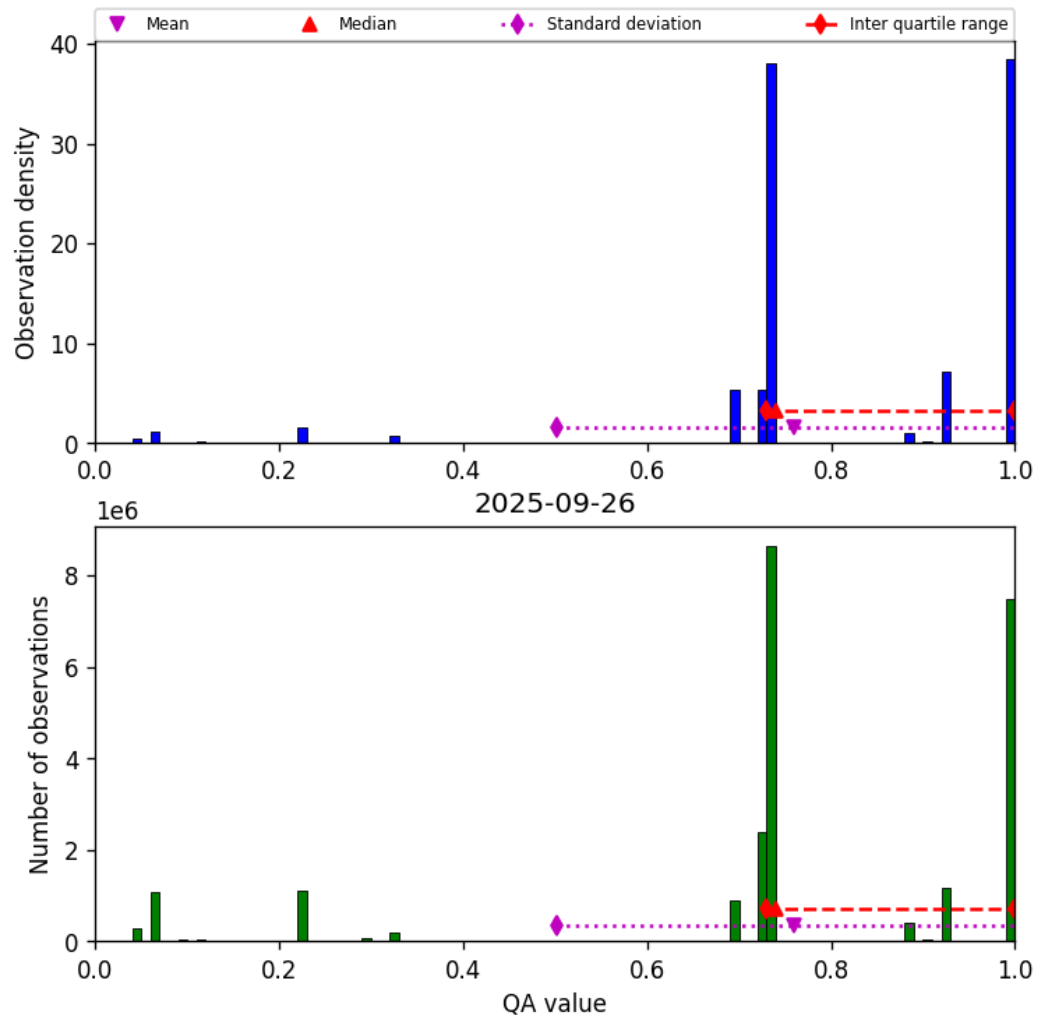
Figure 26: Histogram of “QA value” for 2025-09-26 to 2025-09-27
