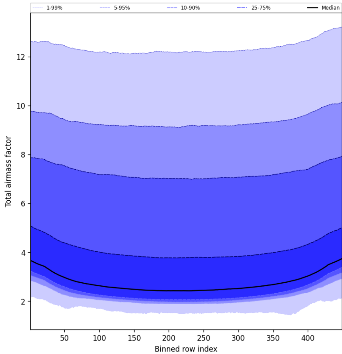
Figure 47: Along track statistics of “Total airmass factor” for 2025-09-26 to 2025-09-27
