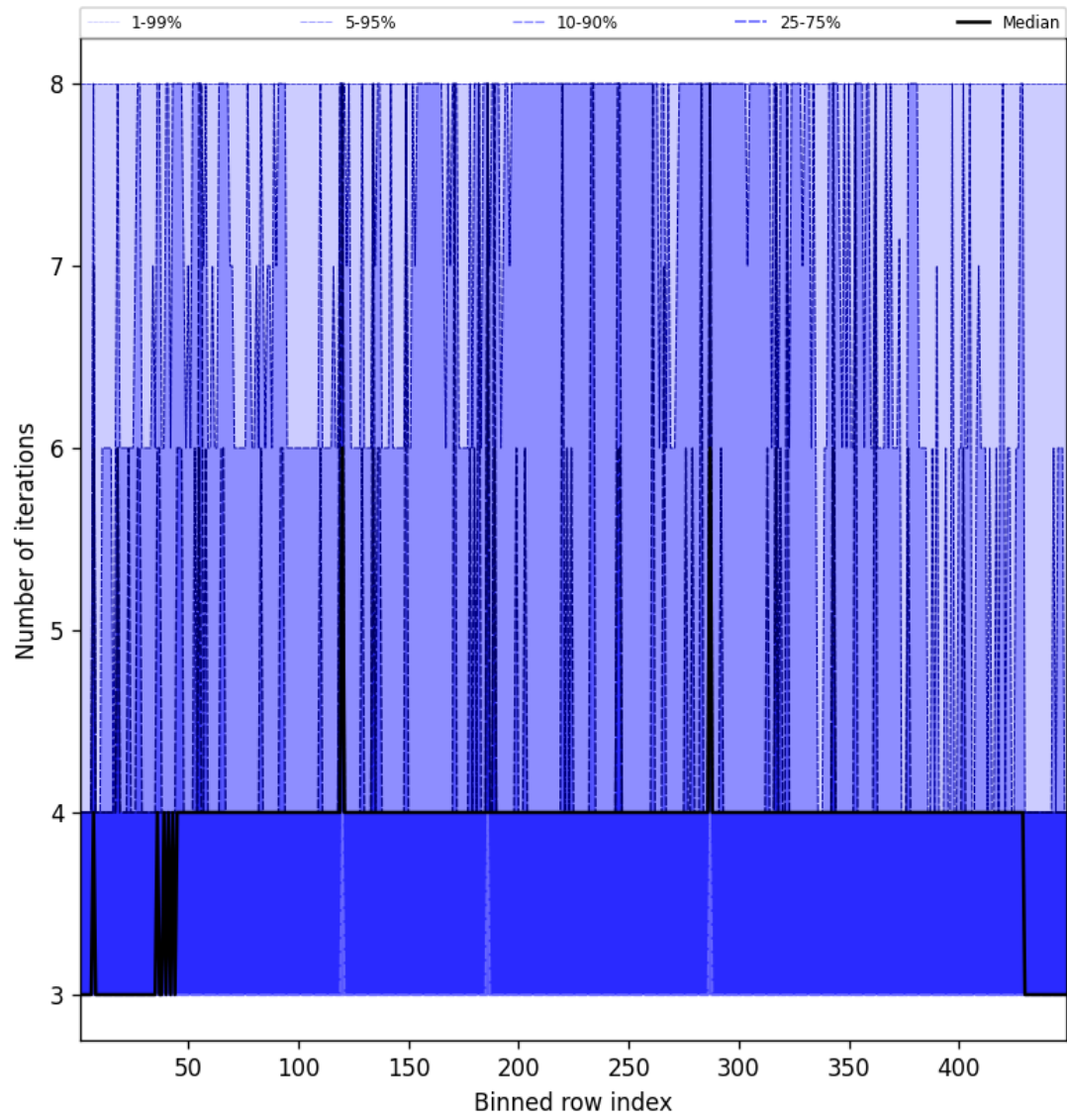
Figure 49: Along track statistics of “Number of iterations” for 2025-09-26 to 2025-09-27
