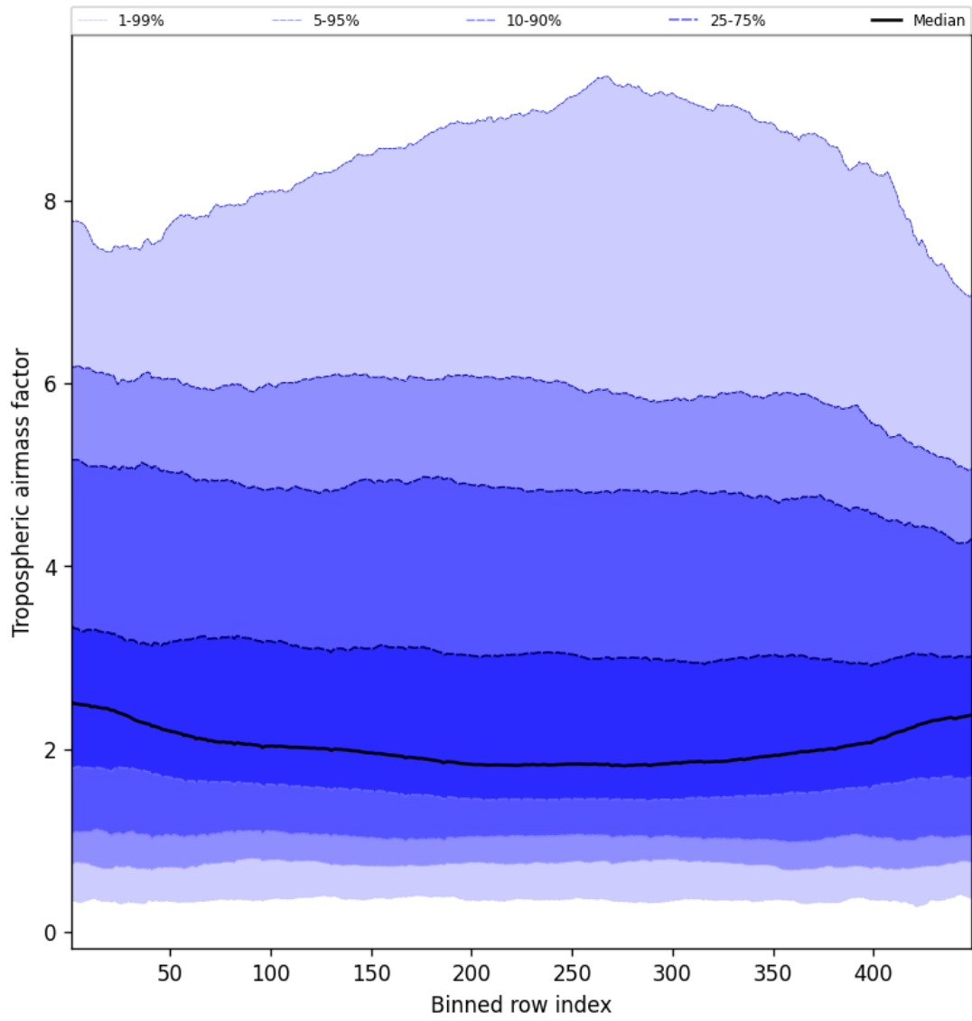
Figure 46: Along track statistics of “Tropospheric air mass factor” for 2025-09-26 to 2025-09-27
