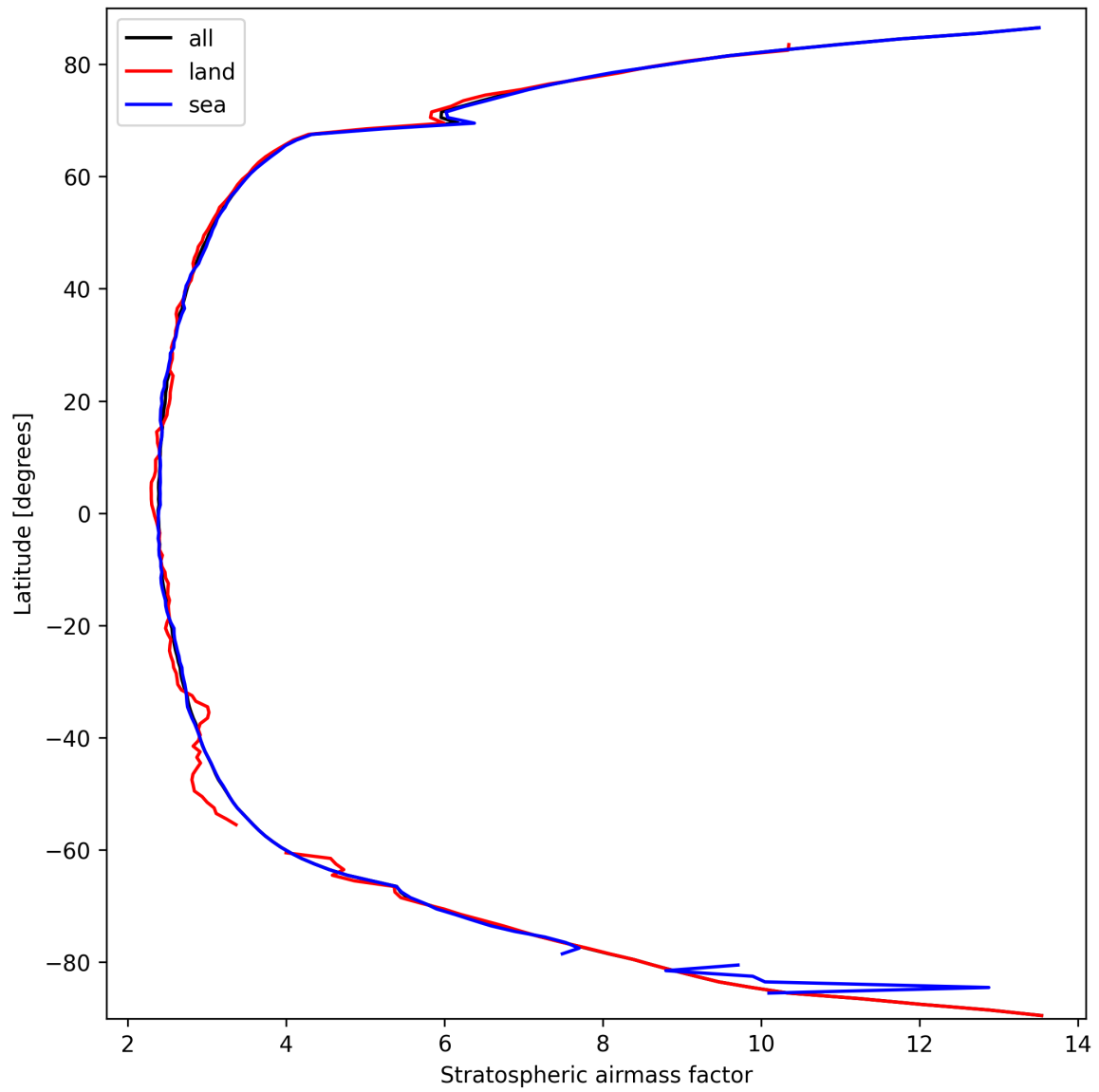
Figure 25: Zonal average of “Stratospheric airmass factor” for 2025-09-26 to 2025-09-27.
