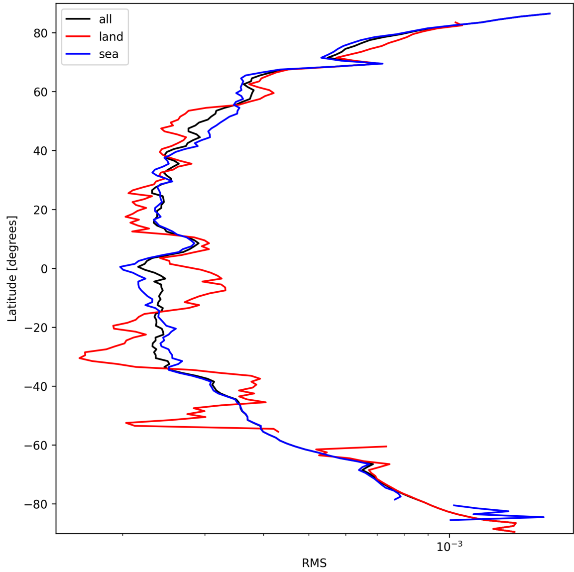
Figure 24: Zonal average of “RMS” for 2025-09-26 to 2025-09-27.
