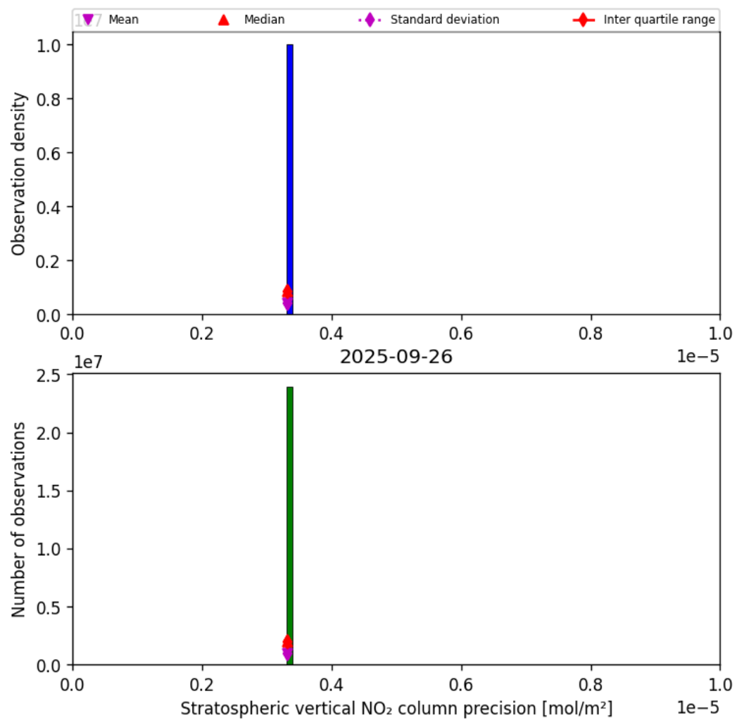
Figure 35: Histogram of “Stratospheric vertical NO 2 column precision” for 2025-09-26 to 2025-09-27
