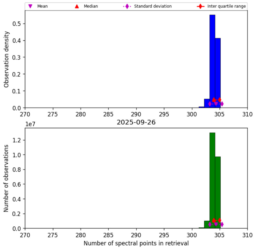
Figure 31: Histogram of “Number of spectral points in retrieval” for 2025-09-26 to 2025-09-27
