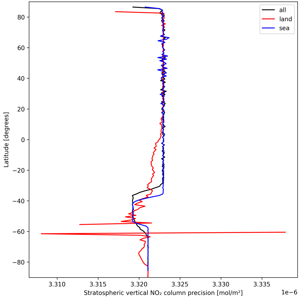
Figure 18: Zonal average of “Stratospheric vertical NO 2 column precision” for 2025-09-26 to 2025-09-27.
