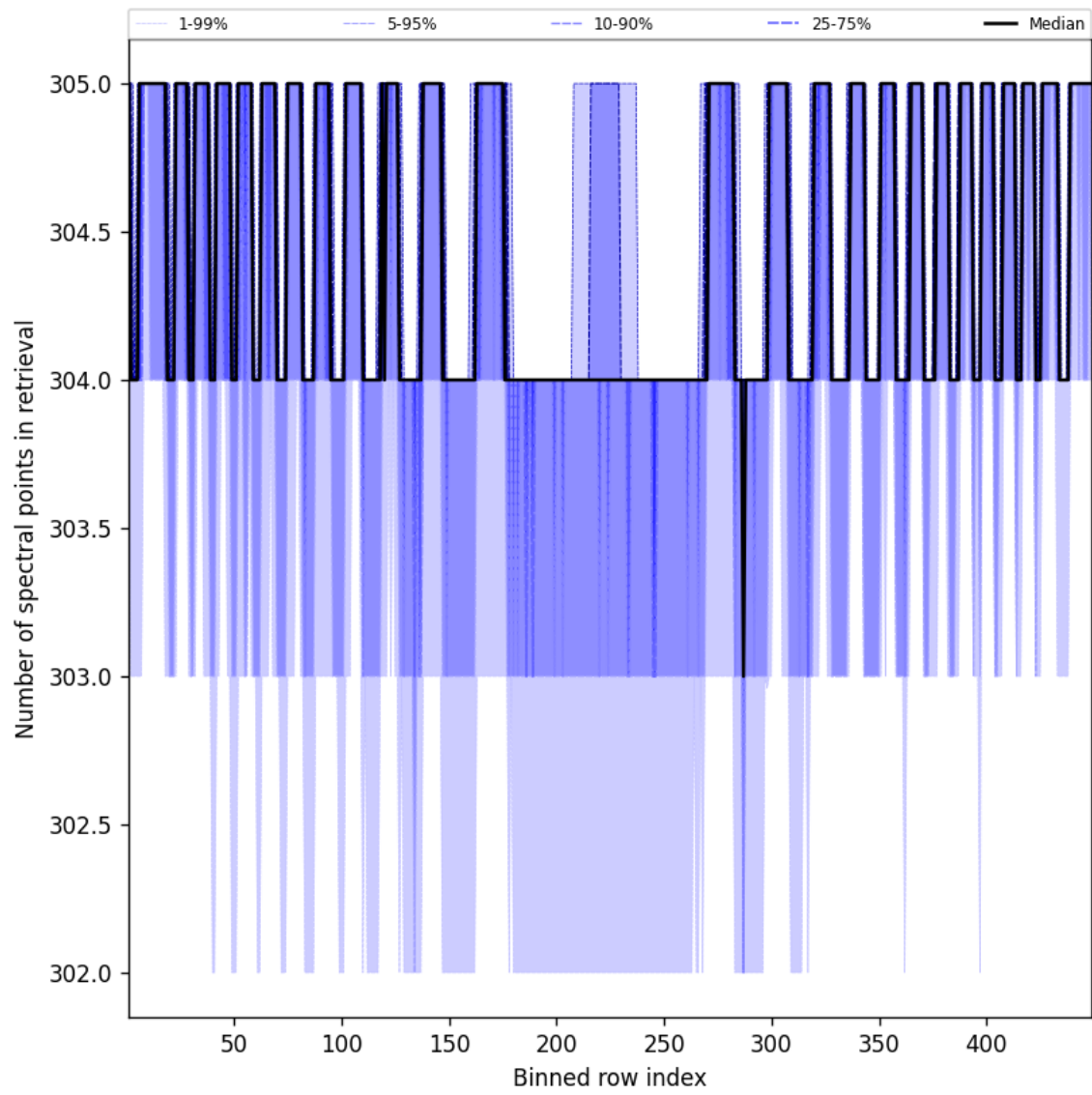
Figure 48: Along track statistics of “Number of spectral points in retrieval” for 2025-09-26 to 2025-09-27
