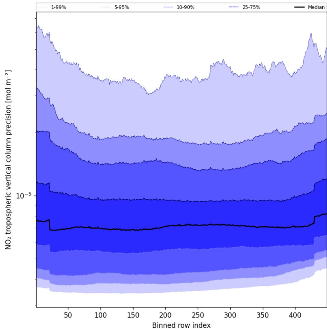
Figure 45: Along track statistics of “NO 2 tropospheric vertical column precision” for 2025-09-26 to 2025-09-27
