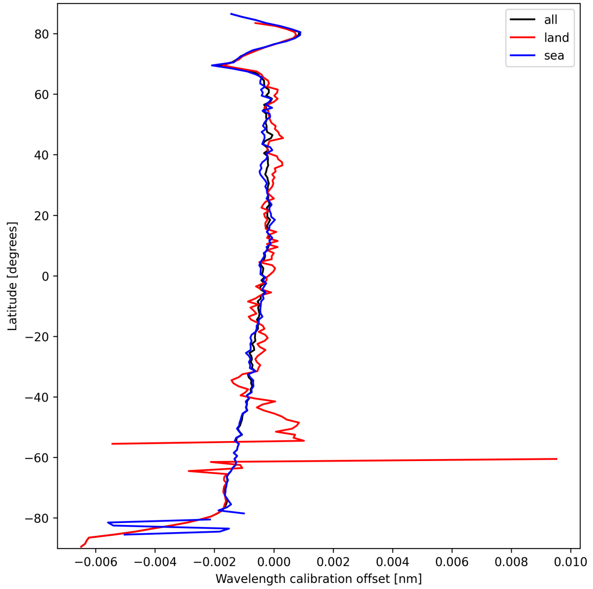
Figure 16: Zonal average of “Wavelength calibration offset” for 2025-09-26 to 2025-09-27.
