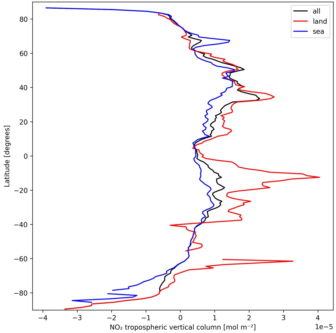
Figure 10: Zonal average of “NO 2 tropospheric vertical column” for 2025-09-26 to 2025-09-27.
