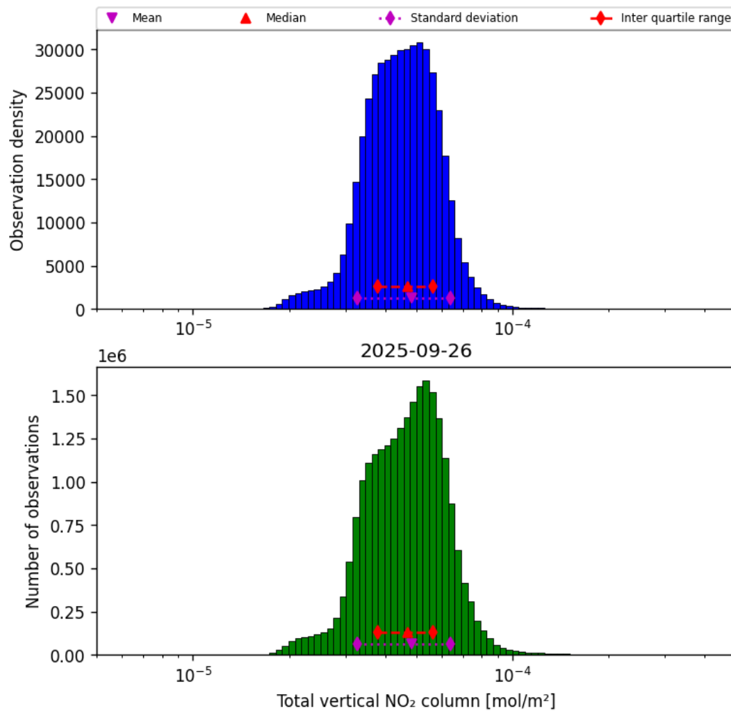
Figure 36: Histogram of “Total vertical NO 2 column” for 2025-09-26 to 2025-09-27
