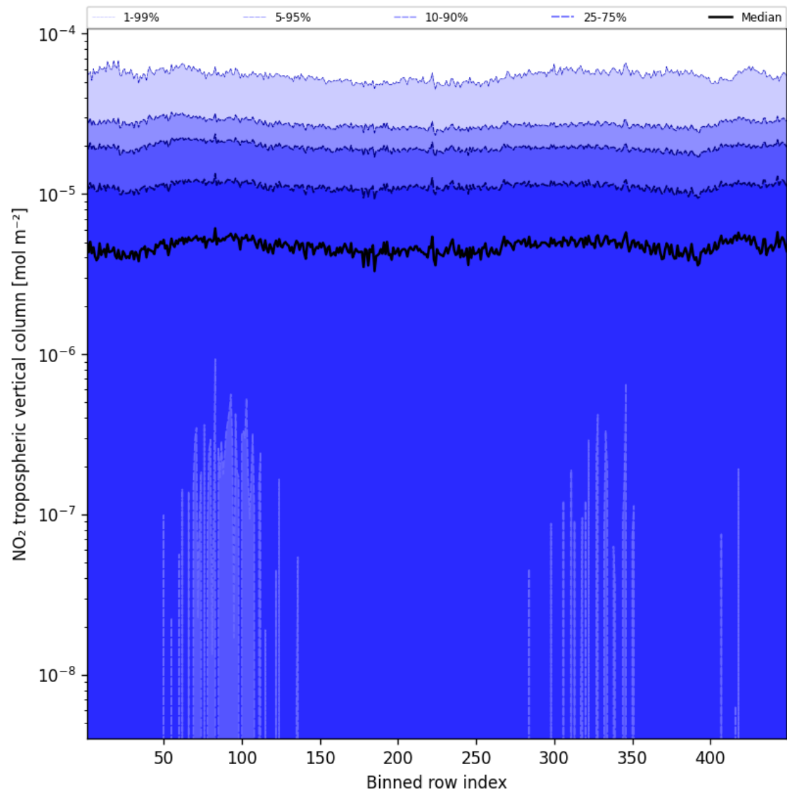
Figure 44: Along track statistics of “NO 2 tropospheric vertical column” for 2025-09-26 to 2025-09-27
