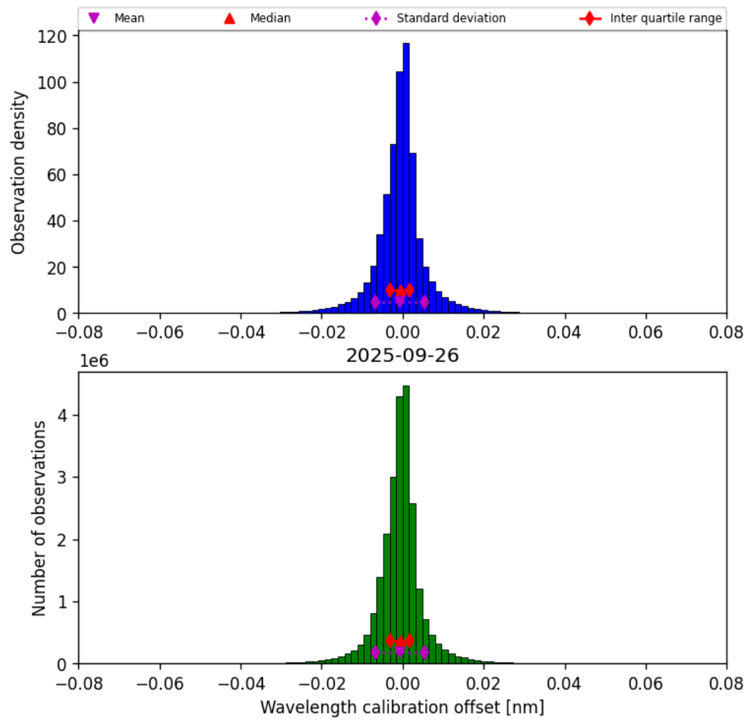
Figure 33: Histogram of “Wavelength calibration offset” for 2025-09-26 to 2025-09-27
