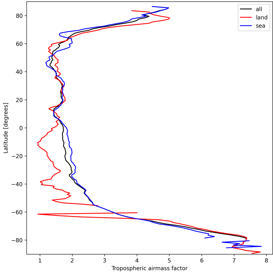
Figure 12: Zonal average of “Tropospheric airmass factor” for 2025-09-26 to 2025-09-27.
