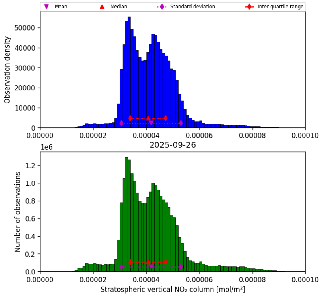
Figure 34: Histogram of “Stratospheric vertical NO 2 column” for 2025-09-26 to 2025-09-27
