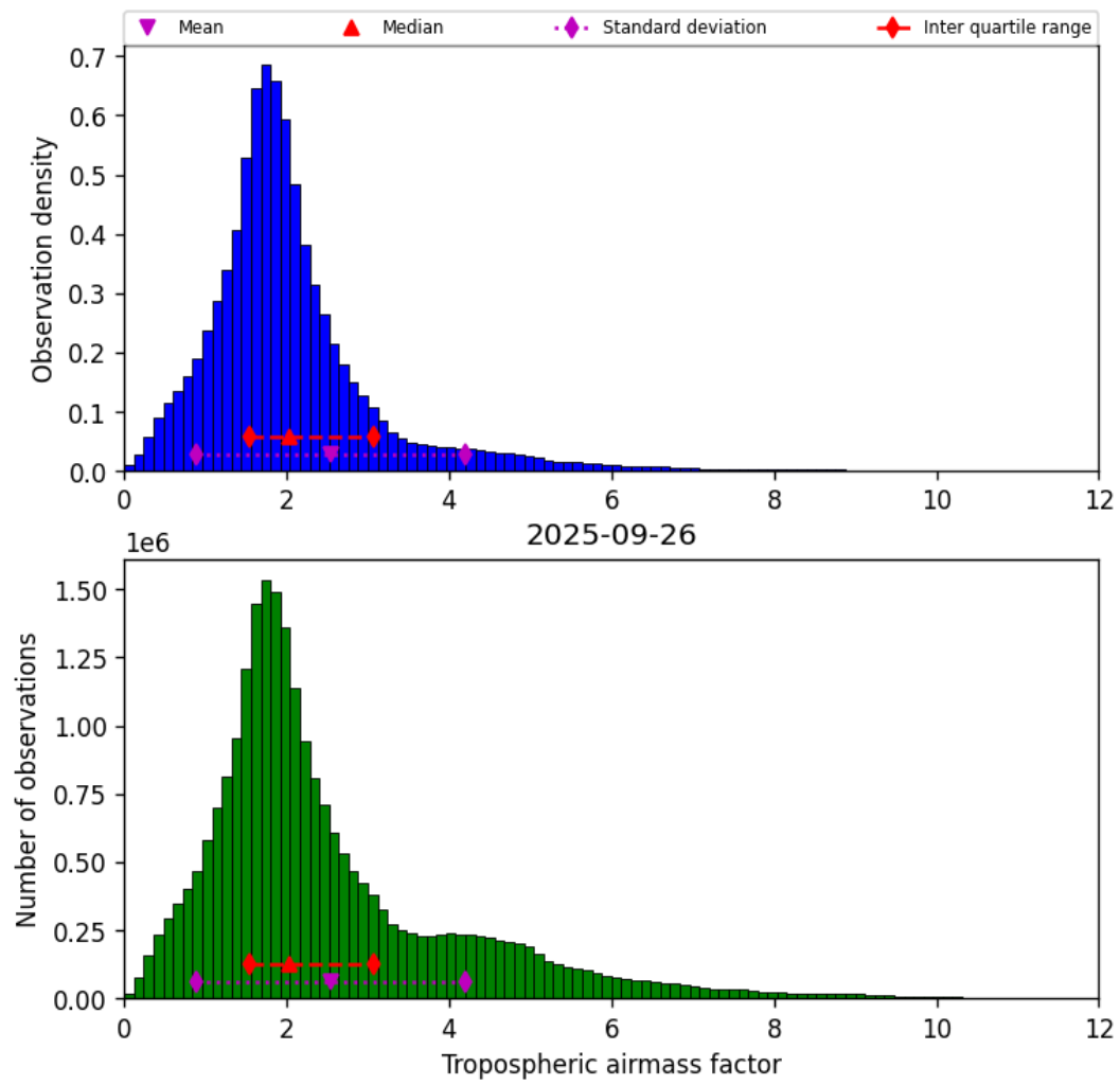
Figure 29: Histogram of “Tropospheric airmass factor” for 2025-09-26 to 2025-09-27
