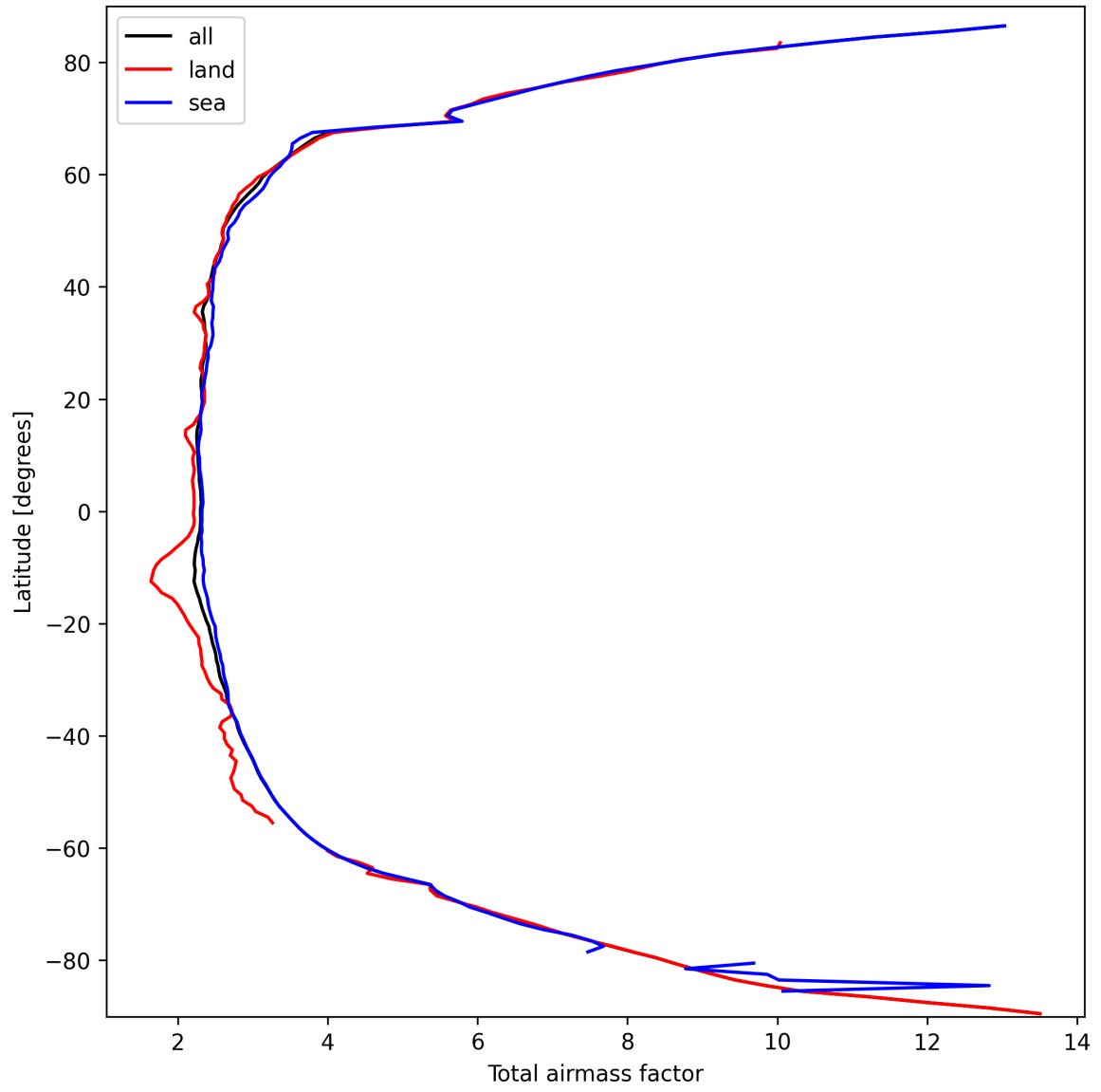
Figure 13: Zonal average of “Total airmass factor” for 2025-09-26 to 2025-09-27.
