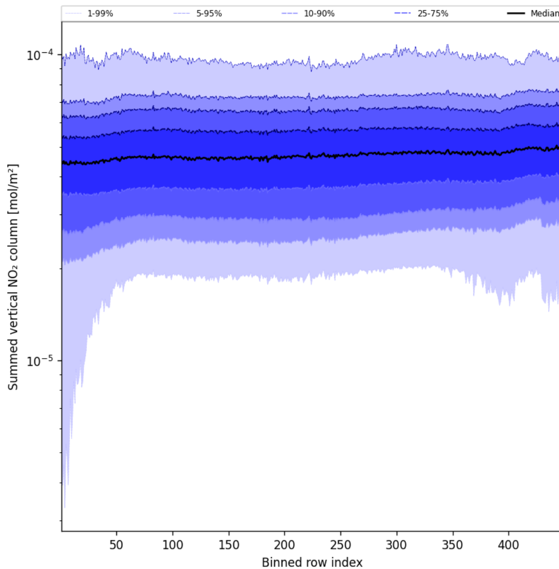
Figure 55: Along track statistics of “Summed vertical NO 2 column” for 2025-09-26 to 2025-09-27
