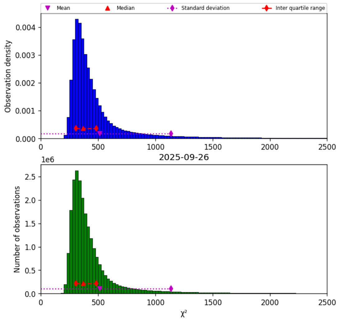
Figure 40: Histogram of “ \chi^2 ” for 2025-09-26 to 2025-09-27
