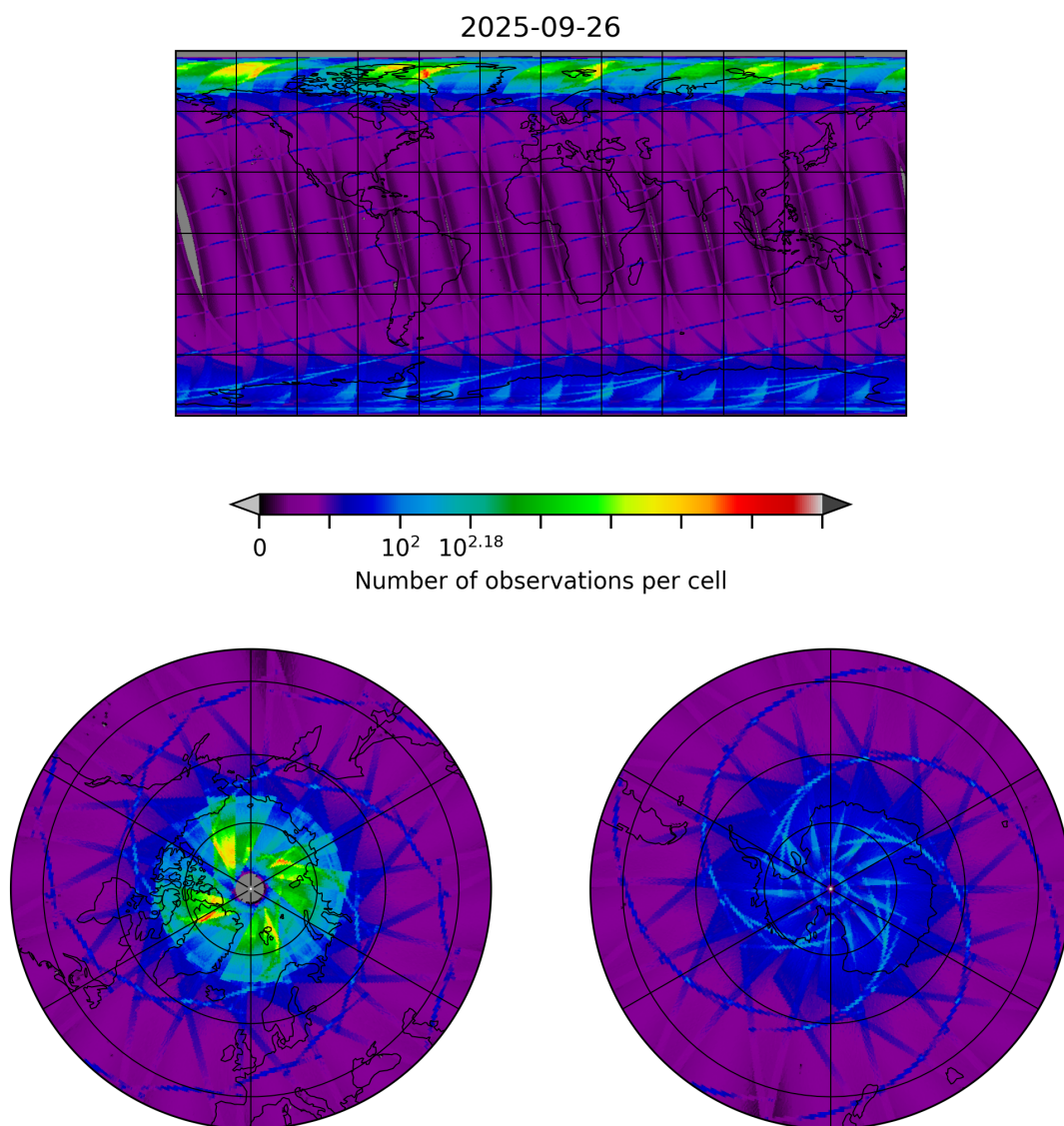
Figure 8: Map of the number of observations for 2025-09-26 to 2025-09-27
