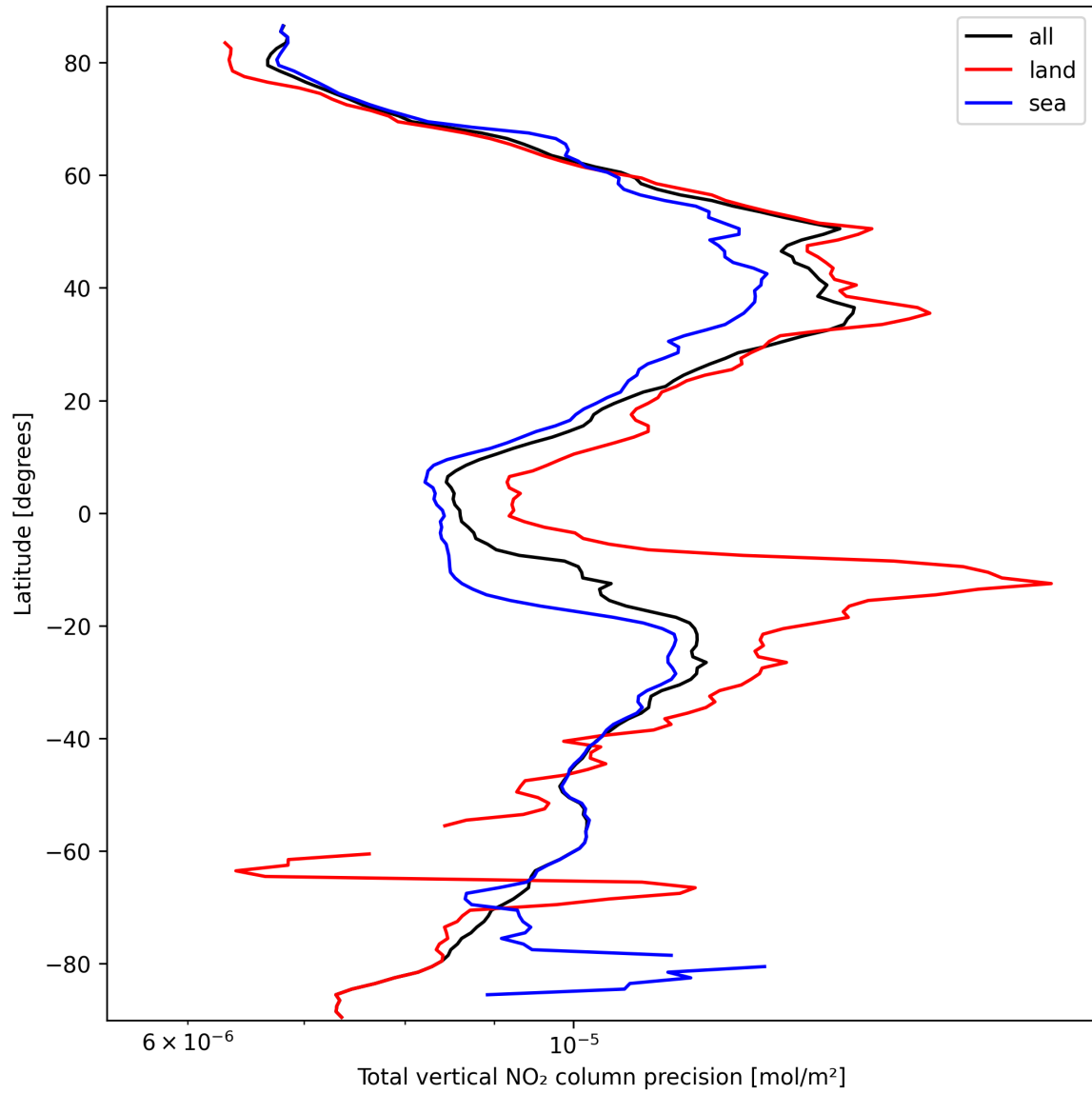
Figure 20: Zonal average of “Total vertical NO 2 column precision” for 2025-09-26 to 2025-09-27.
