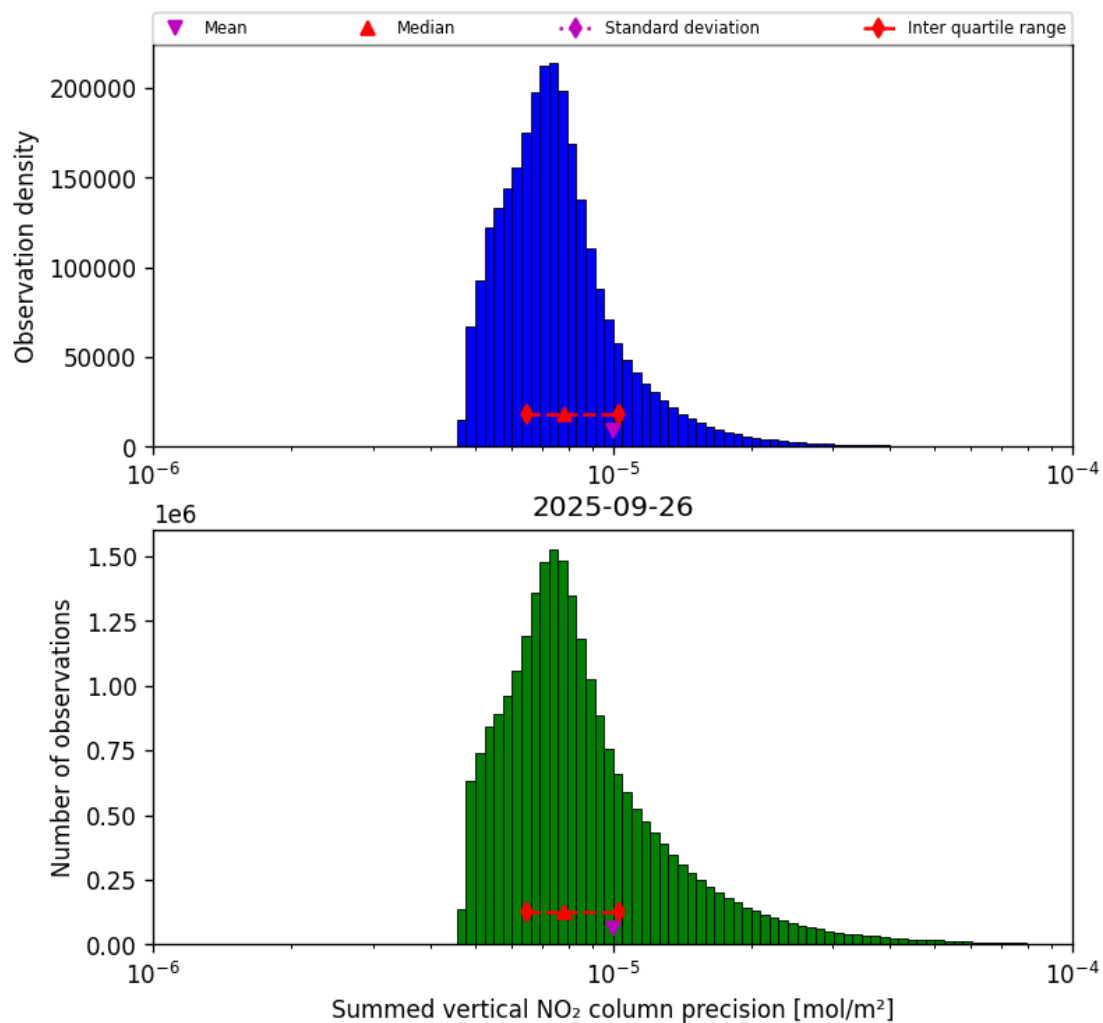
Figure 39: Histogram of "Summed vertical NO 2 column precision" for 2025-09-26 to 2025-09-27
