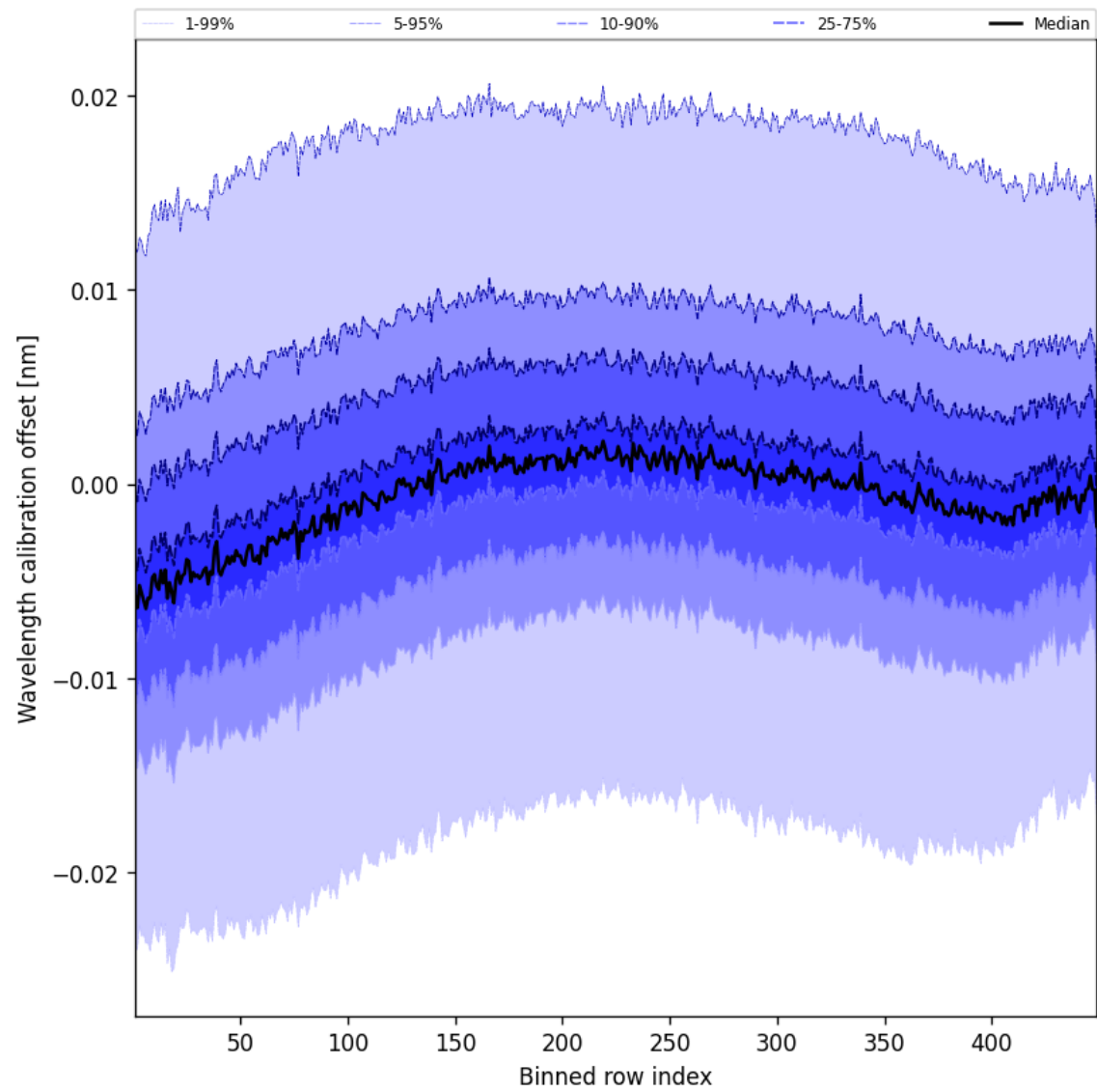
Figure 50: Along track statistics of “Wavelength calibration offset” for 2025-09-26 to 2025-09-27
