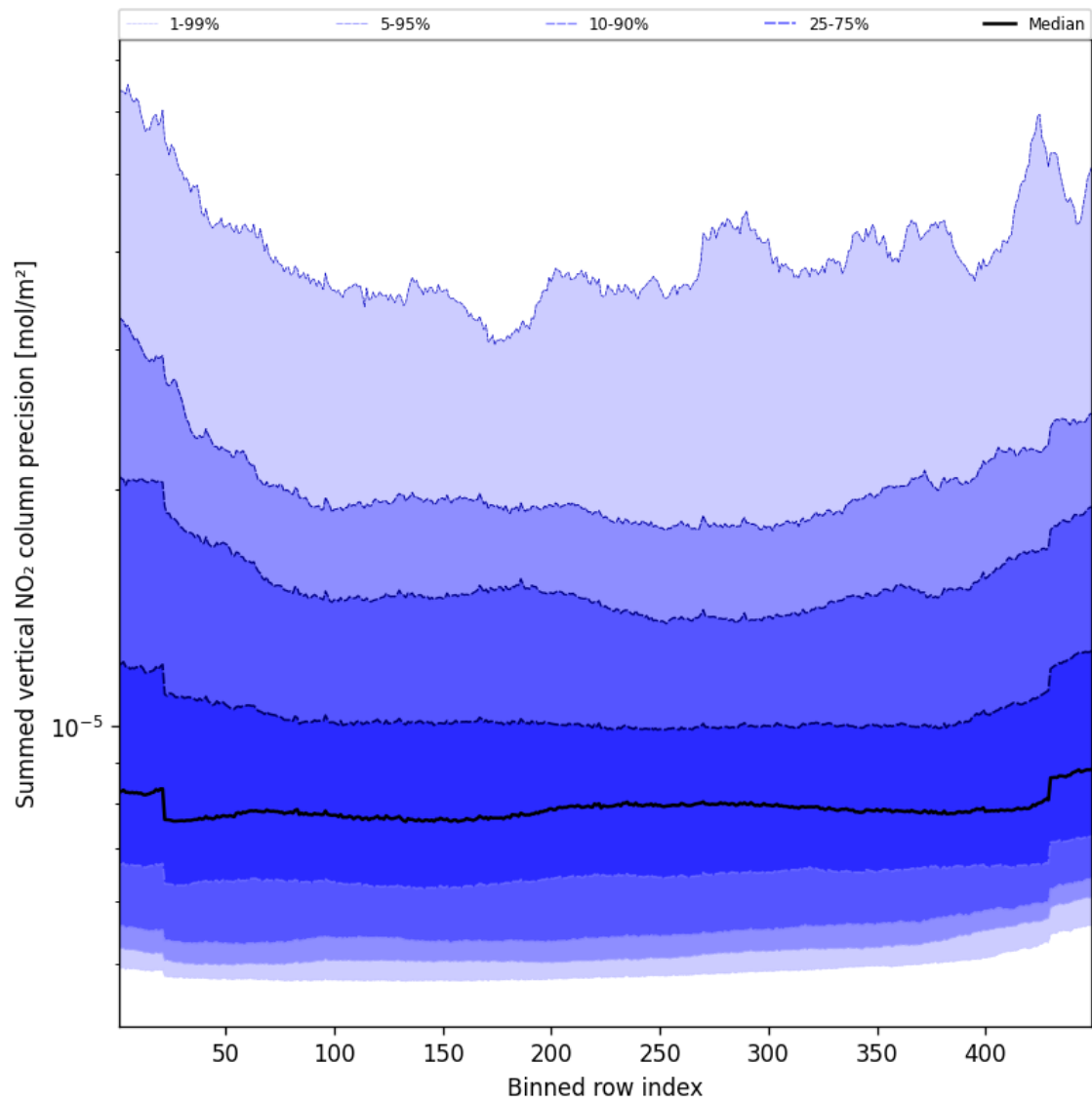
Figure 56: Along track statistics of “Summed vertical NO 2 column precision” for 2025-09-26 to 2025-09-27
