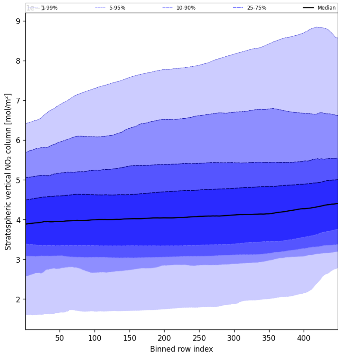
Figure 51: Along track statistics of “Stratospheric vertical NO 2 column” for 2025-09-26 to 2025-09-27
