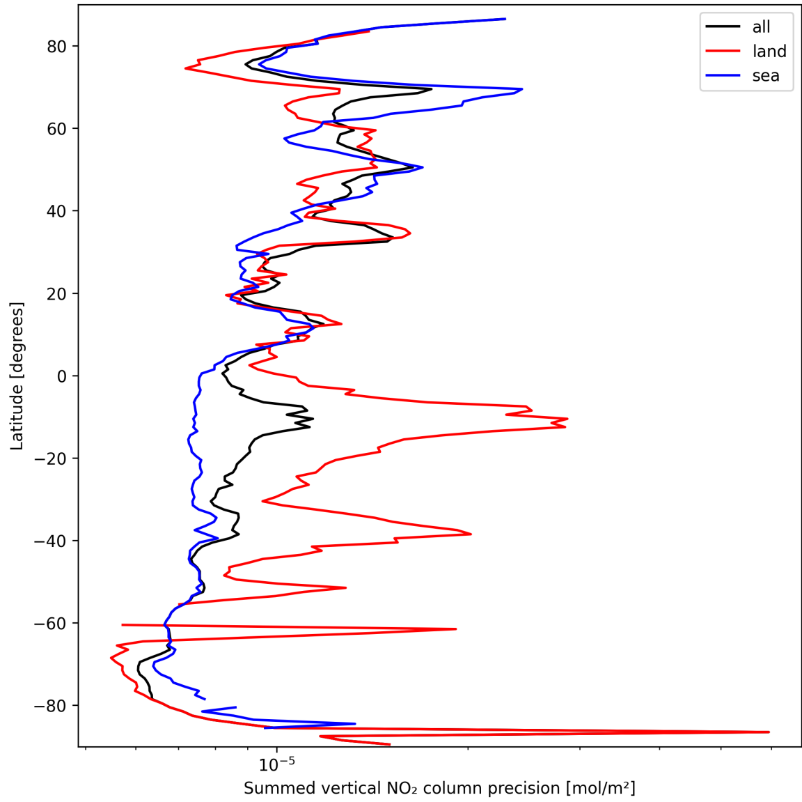
Figure 22: Zonal average of “Summed vertical NO 2 column precision” for 2025-09-26 to 2025-09-27.
