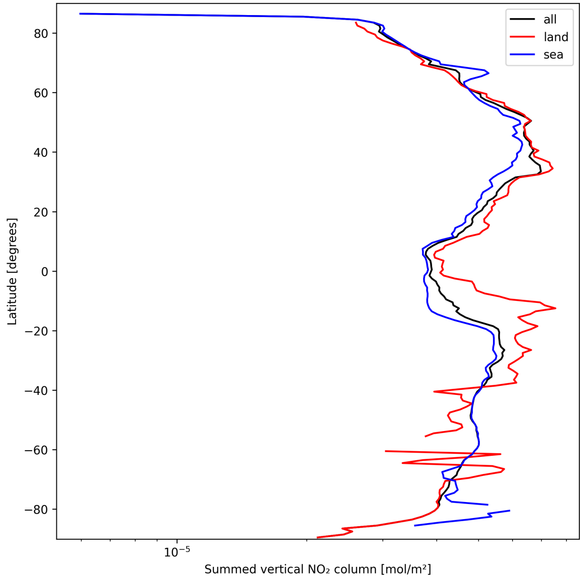
Figure 21: Zonal average of “Summed vertical NO 2 column” for 2025-09-26 to 2025-09-27.
