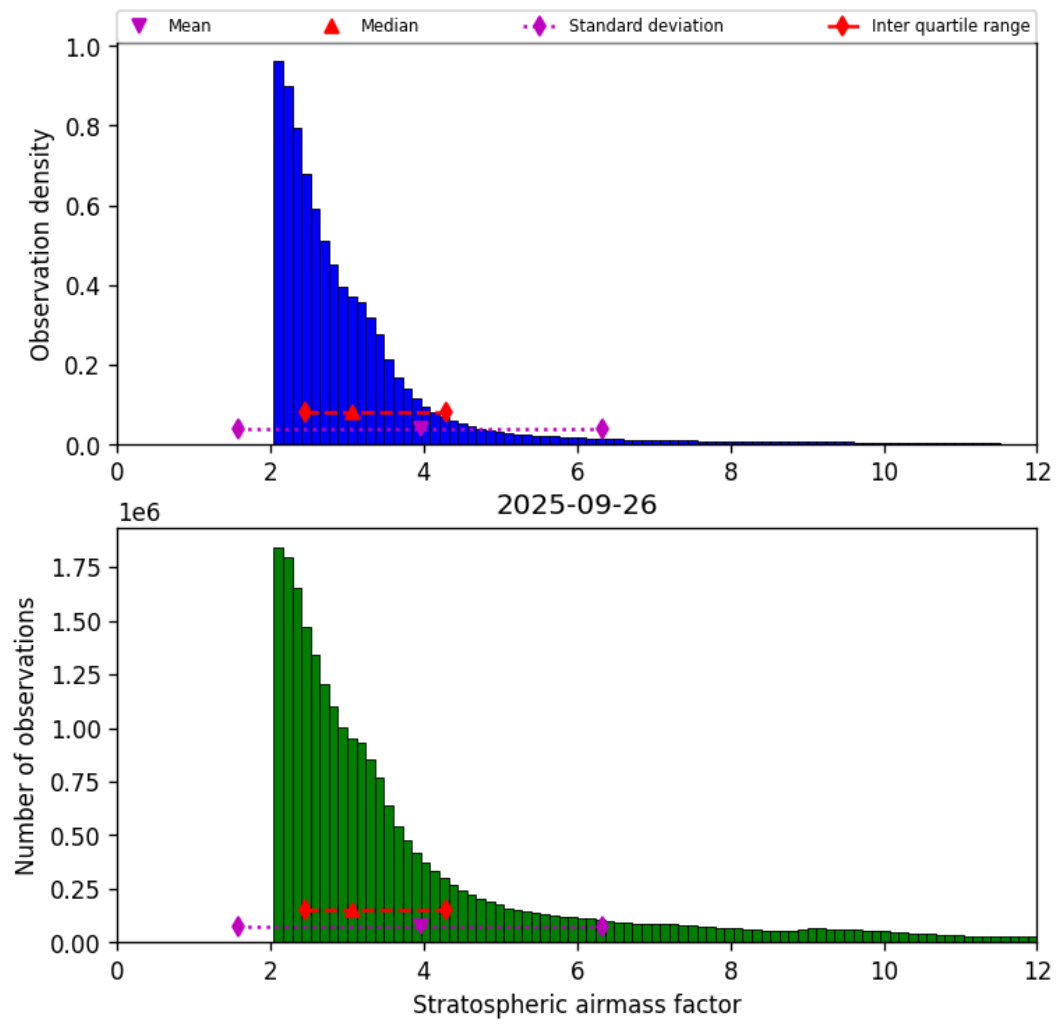
Figure 42: Histogram of “Stratospheric airmass factor” for 2025-09-26 to 2025-09-27
