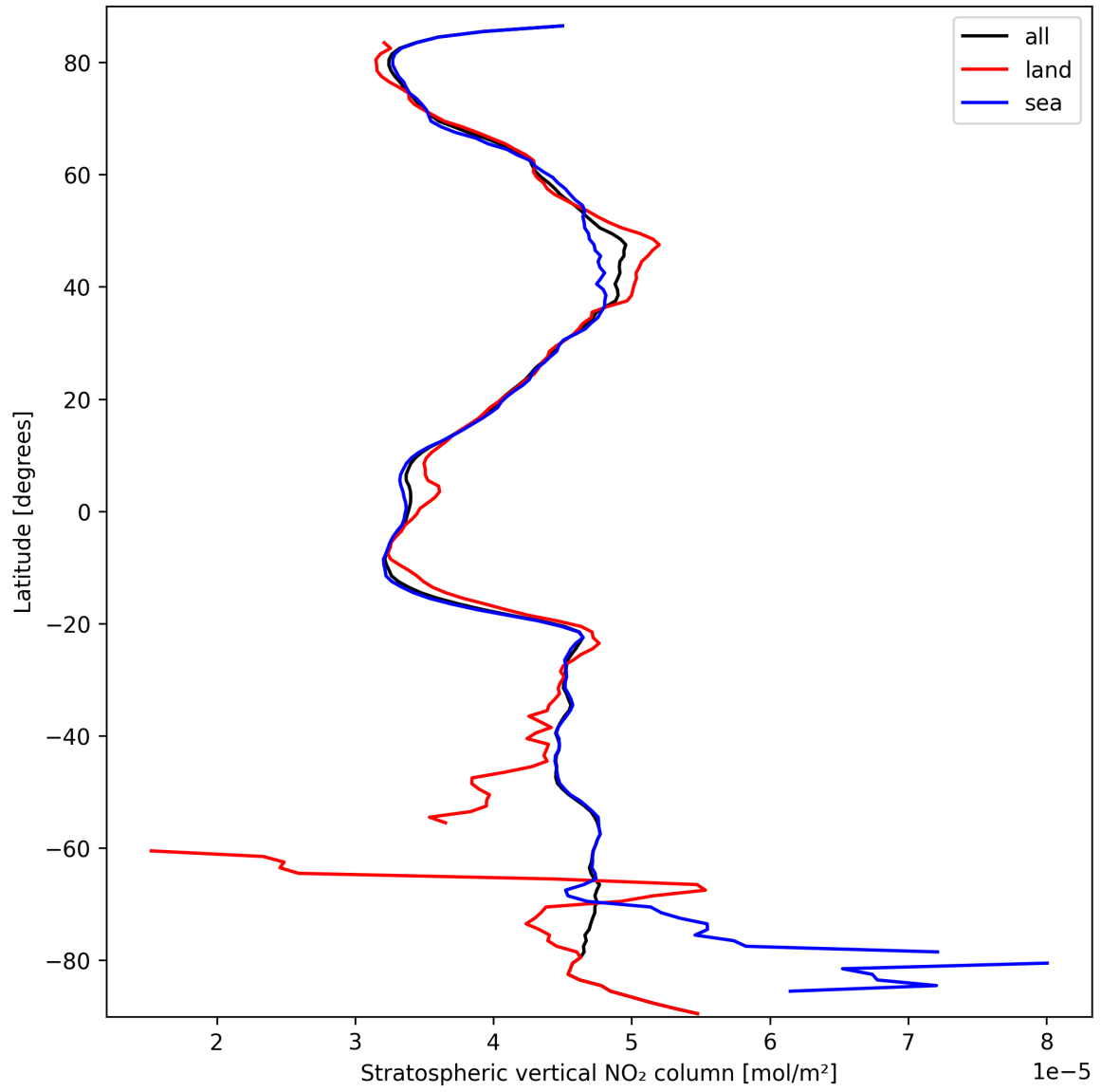
Figure 17: Zonal average of “Stratospheric vertical NO 2 column” for 2025-09-26 to 2025-09-27.
