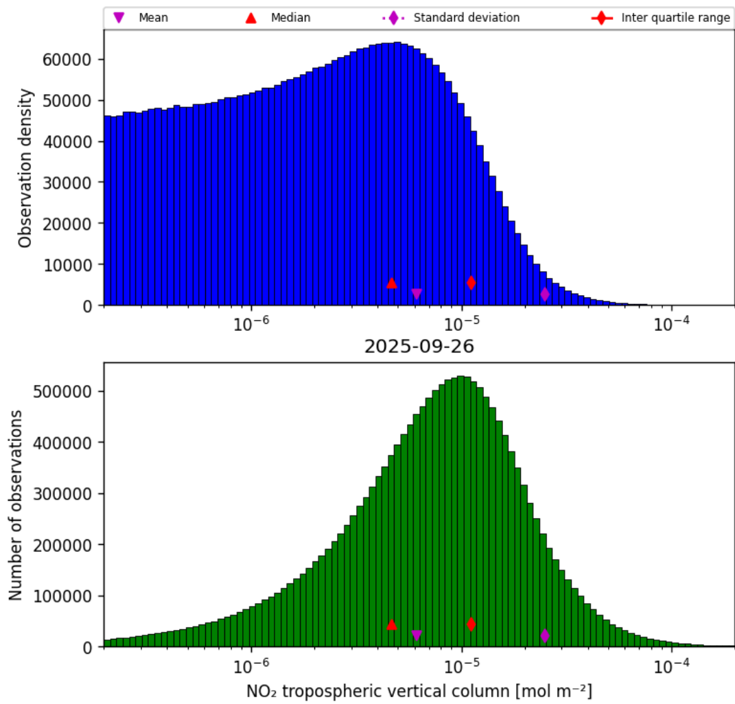
Figure 27: Histogram of “NO 2 tropospheric vertical column” for 2025-09-26 to 2025-09-27
