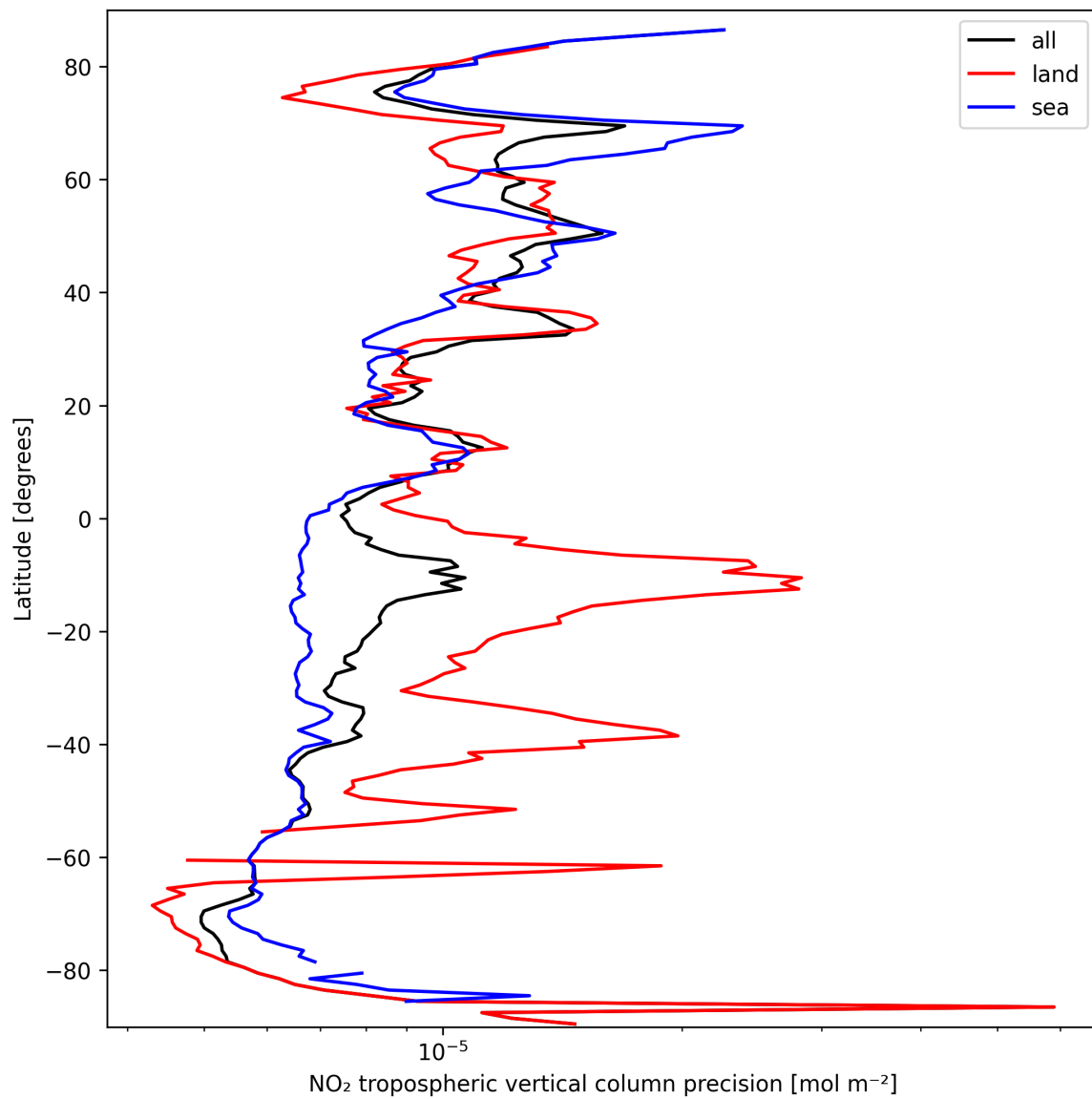
Figure 11: Zonal average of “NO 2 tropospheric vertical column precision” for 2025-09-26 to 2025-09-27.
