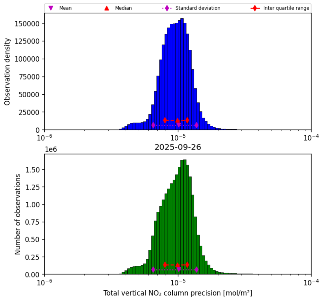
Figure 37: Histogram of “Total vertical NO 2 column precision” for 2025-09-26 to 2025-09-27
