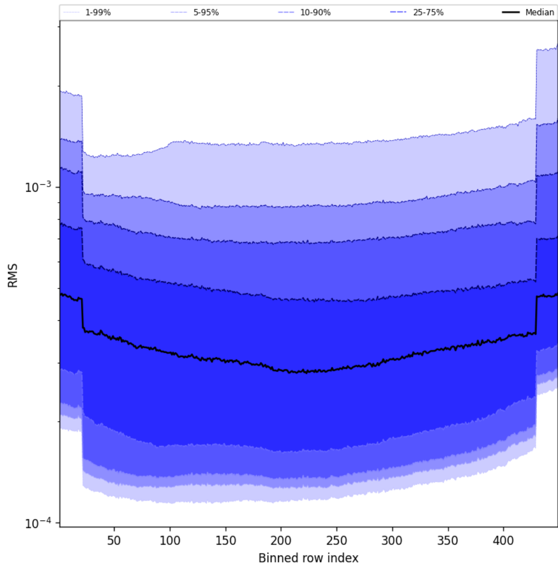
Figure 58: Along track statistics of “RMS” for 2025-09-26 to 2025-09-27
