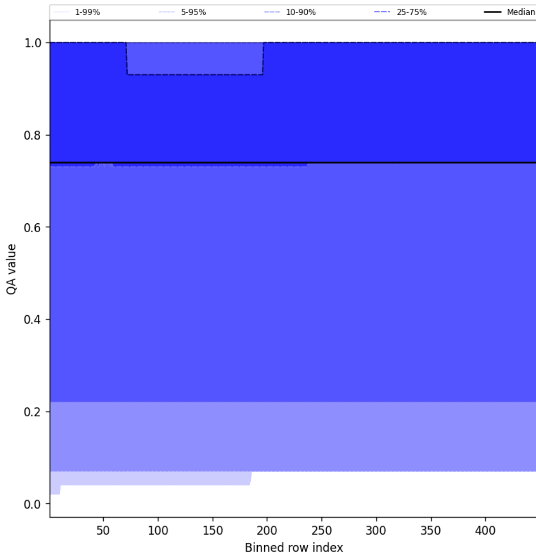
Figure 43: Along track statistics of “QA value” for 2025-09-26 to 2025-09-27
