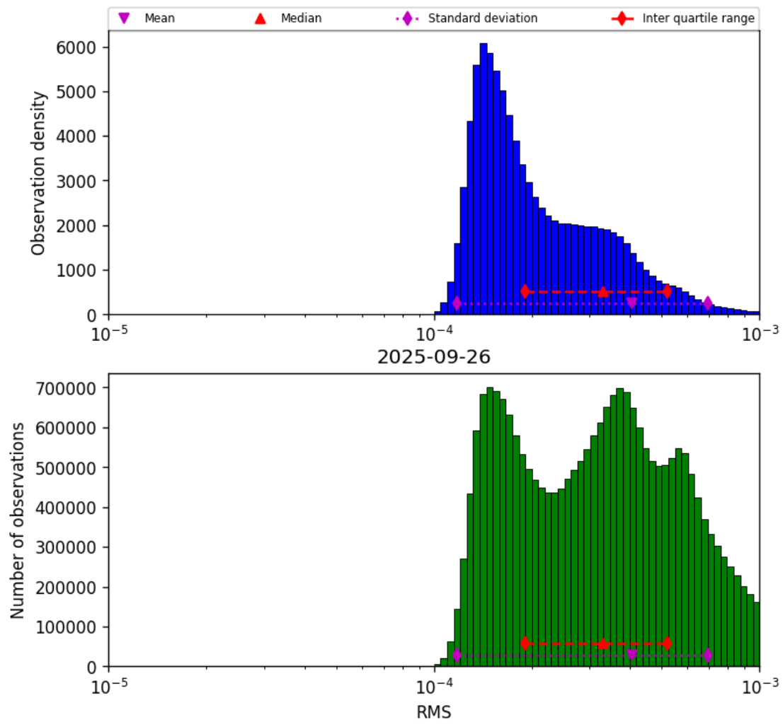
Figure 41: Histogram of “RMS” for 2025-09-26 to 2025-09-27
