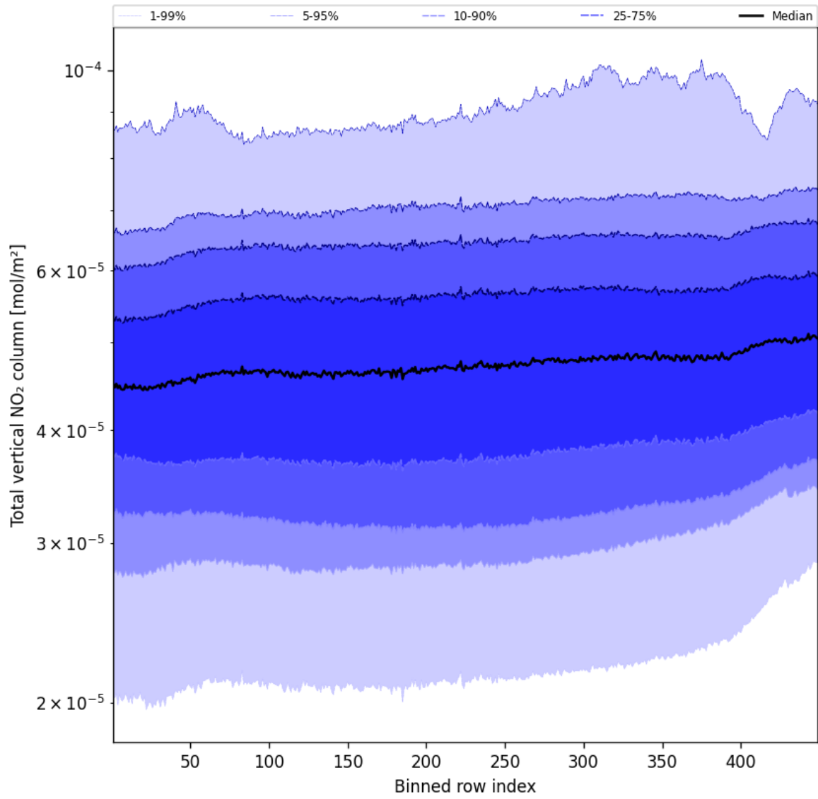
Figure 53: Along track statistics of “Total vertical NO 2 column” for 2025-09-26 to 2025-09-27
