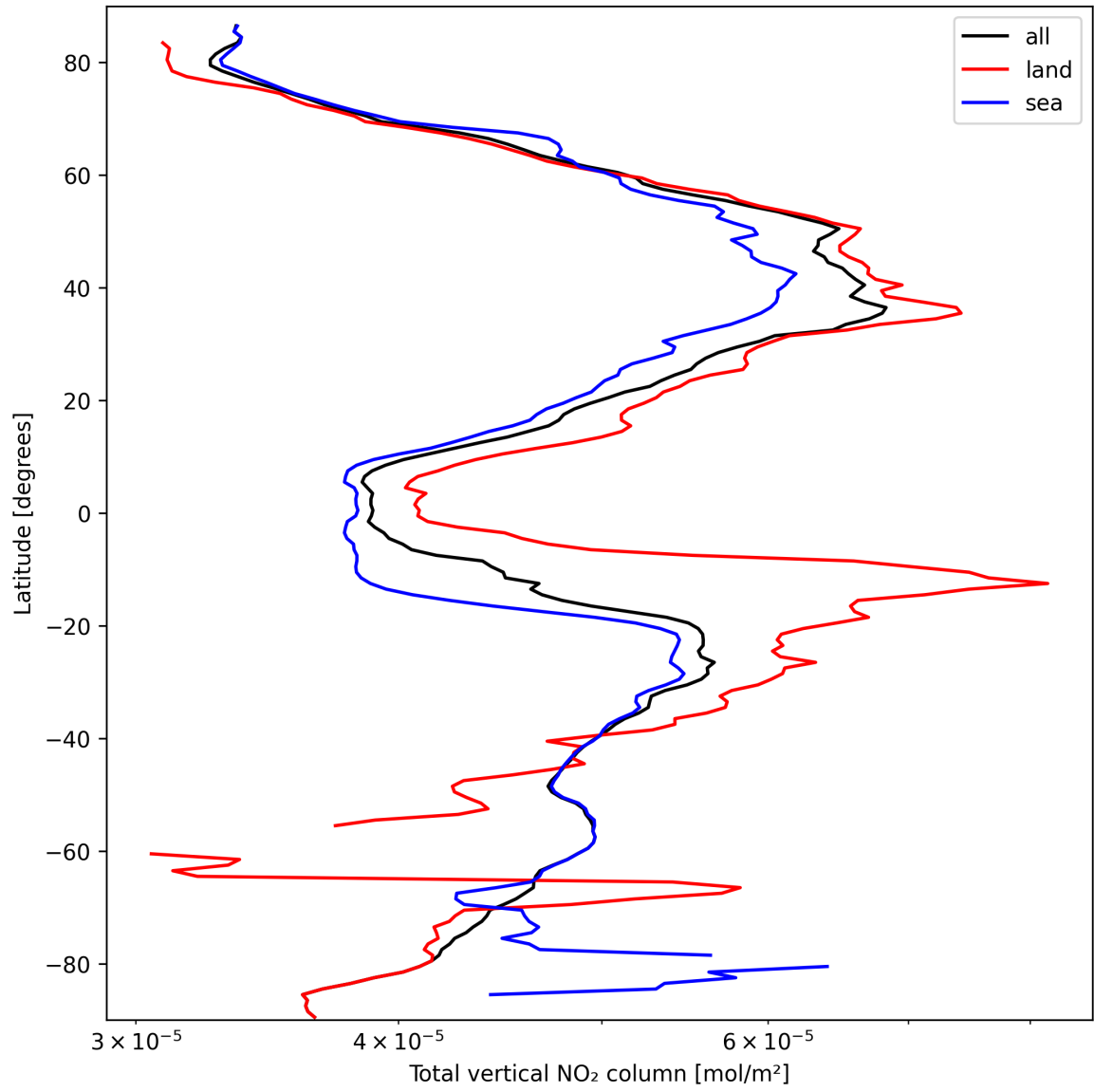
Figure 19: Zonal average of “Total vertical NO 2 column” for 2025-09-26 to 2025-09-27.
