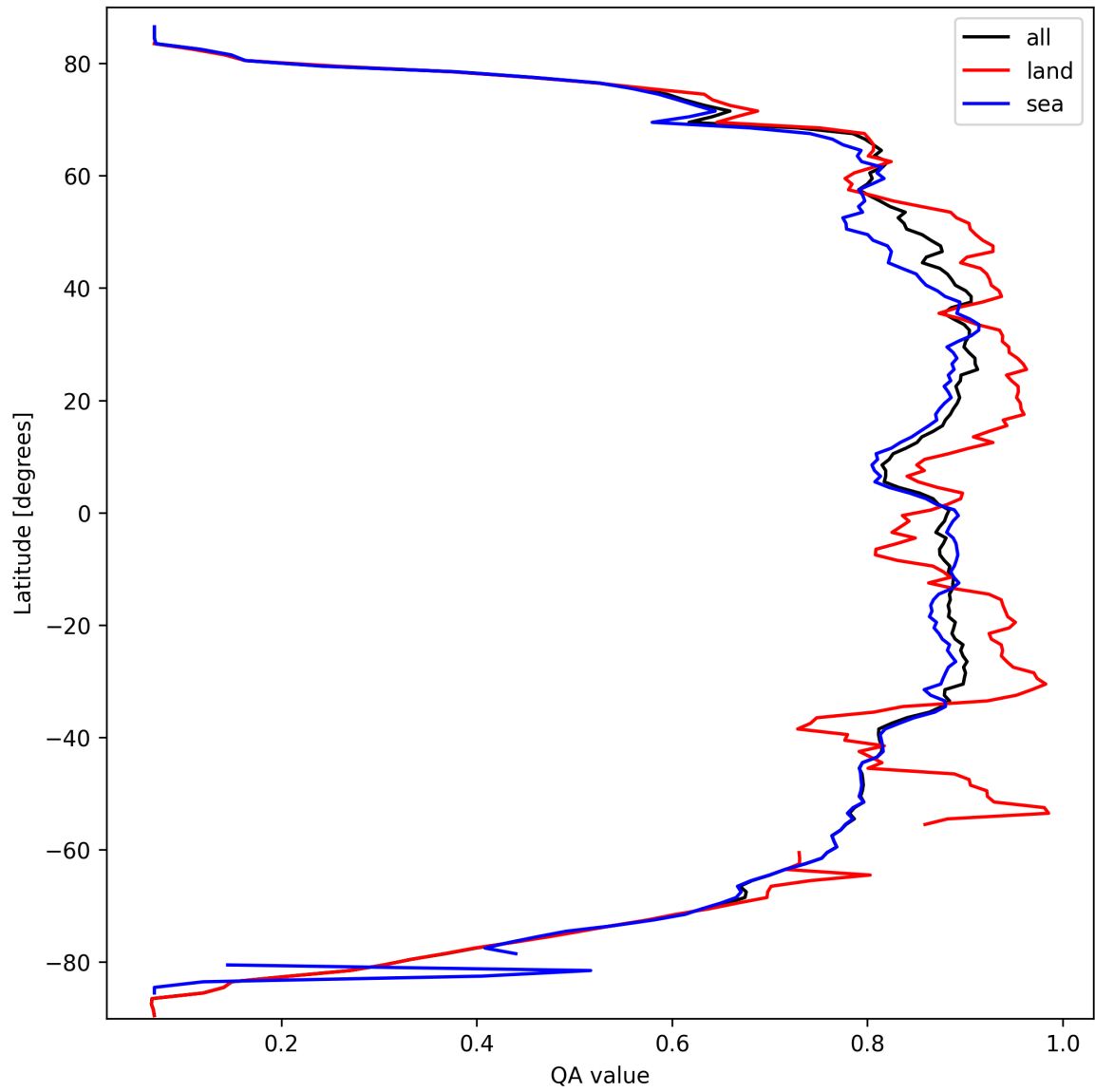
Figure 9: Zonal average of “QA value” for 2025-09-26 to 2025-09-27.
