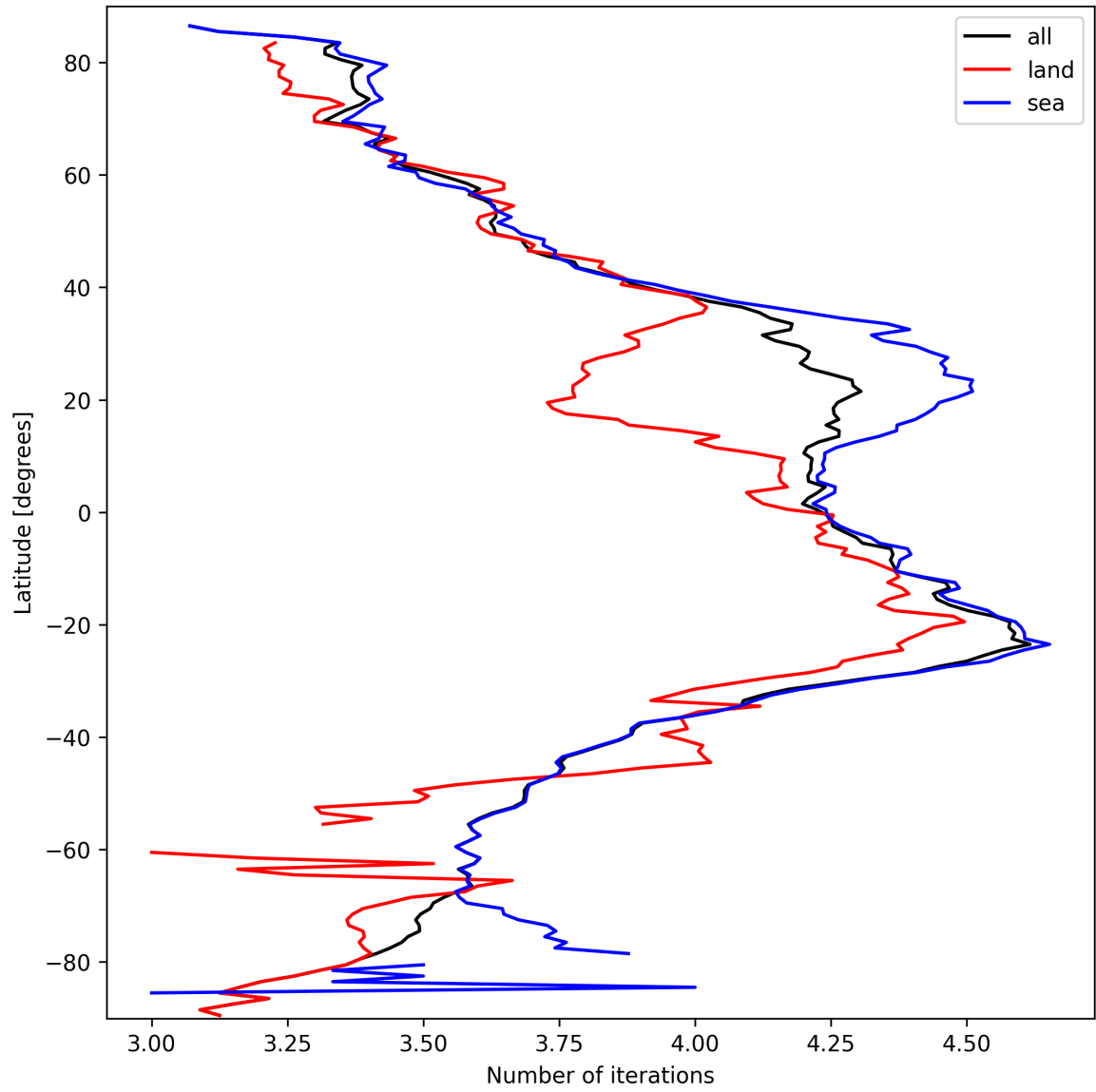
Figure 15: Zonal average of “Number of iterations” for 2025-09-26 to 2025-09-27.
