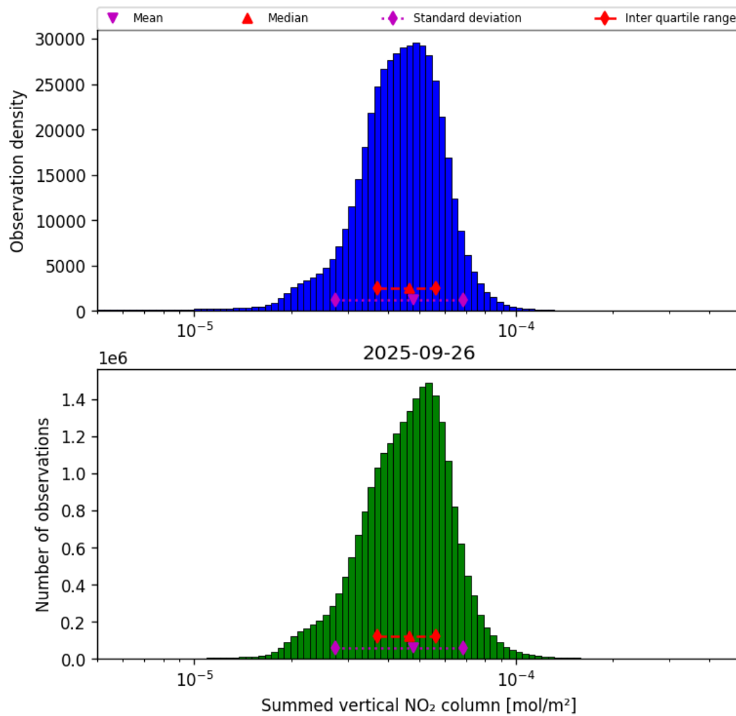
Figure 38: Histogram of "Summed vertical NO 2 column" for 2025-09-26 to 2025-09-27
