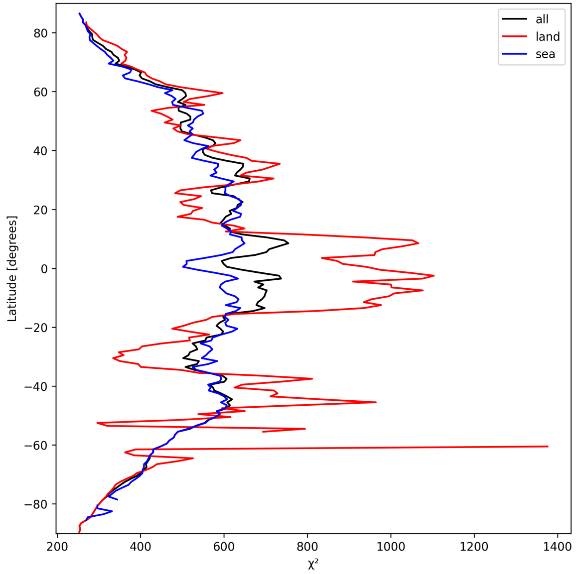
Figure 23: Zonal average of “ \chi^2 ” for 2025-09-26 to 2025-09-27.
