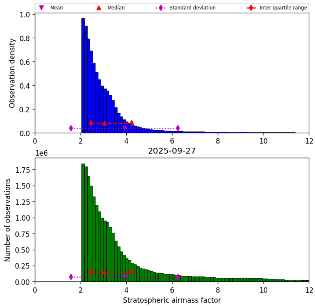
Figure 42: Histogram of “Stratospheric airmass factor” for 2025-09-27 to 2025-09-28
