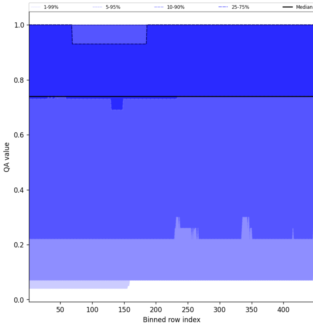
Figure 43: Along track statistics of “QA value” for 2025-09-27 to 2025-09-28
