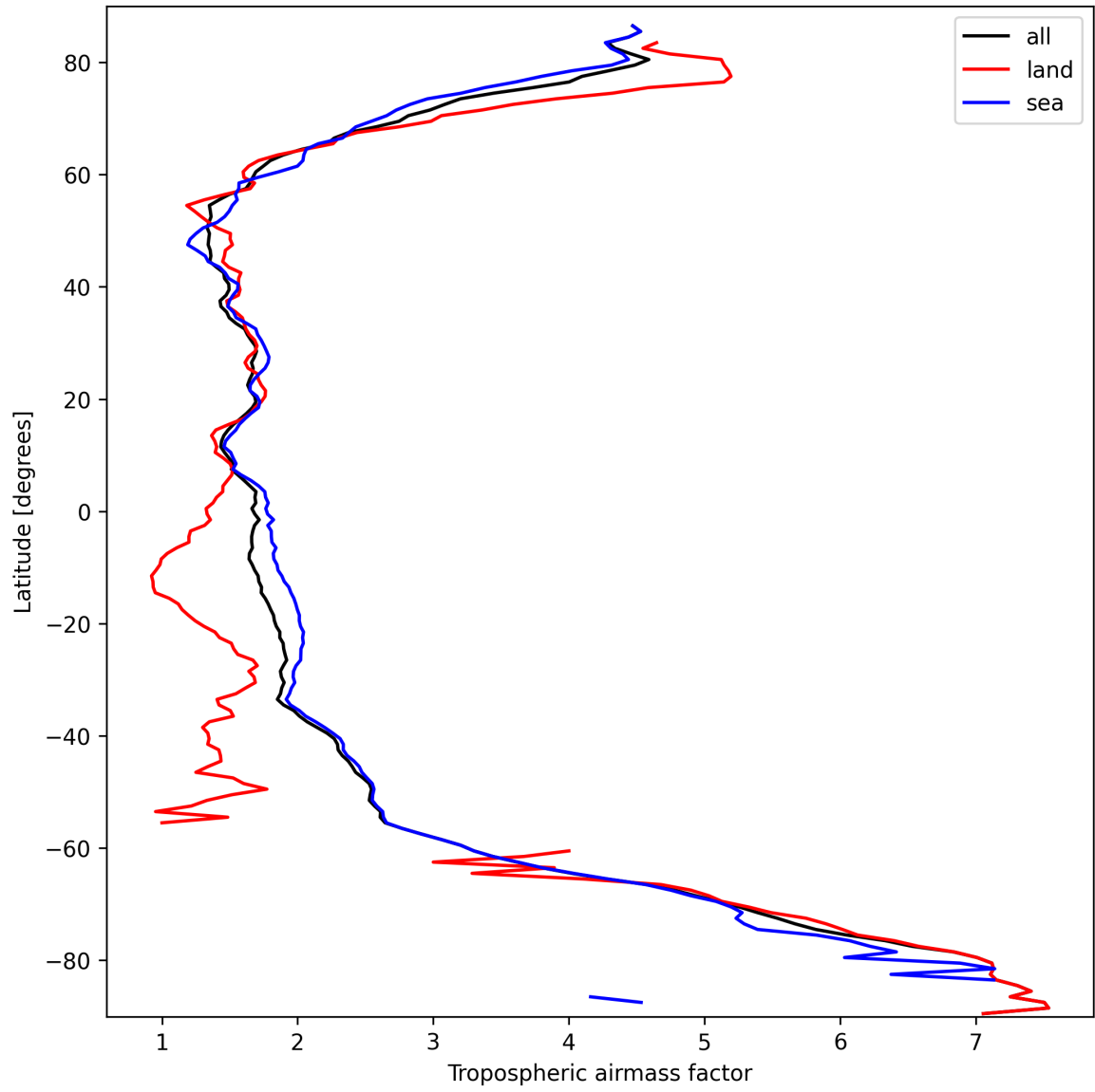
Figure 12: Zonal average of “Tropospheric airmass factor” for 2025-09-27 to 2025-09-28.
