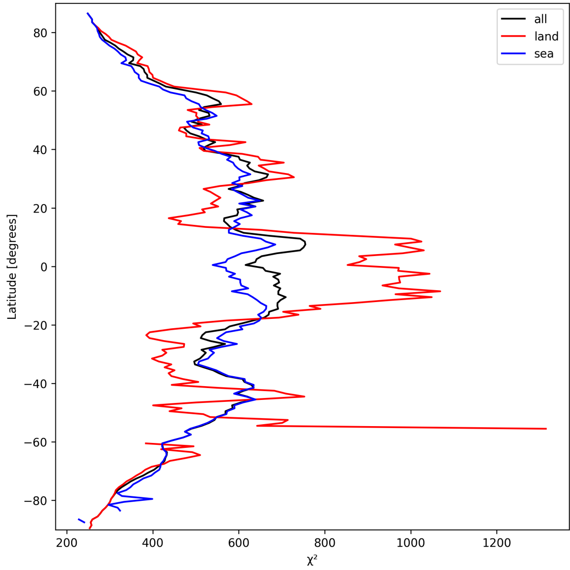
Figure 23: Zonal average of “ \chi^2 ” for 2025-09-27 to 2025-09-28.
