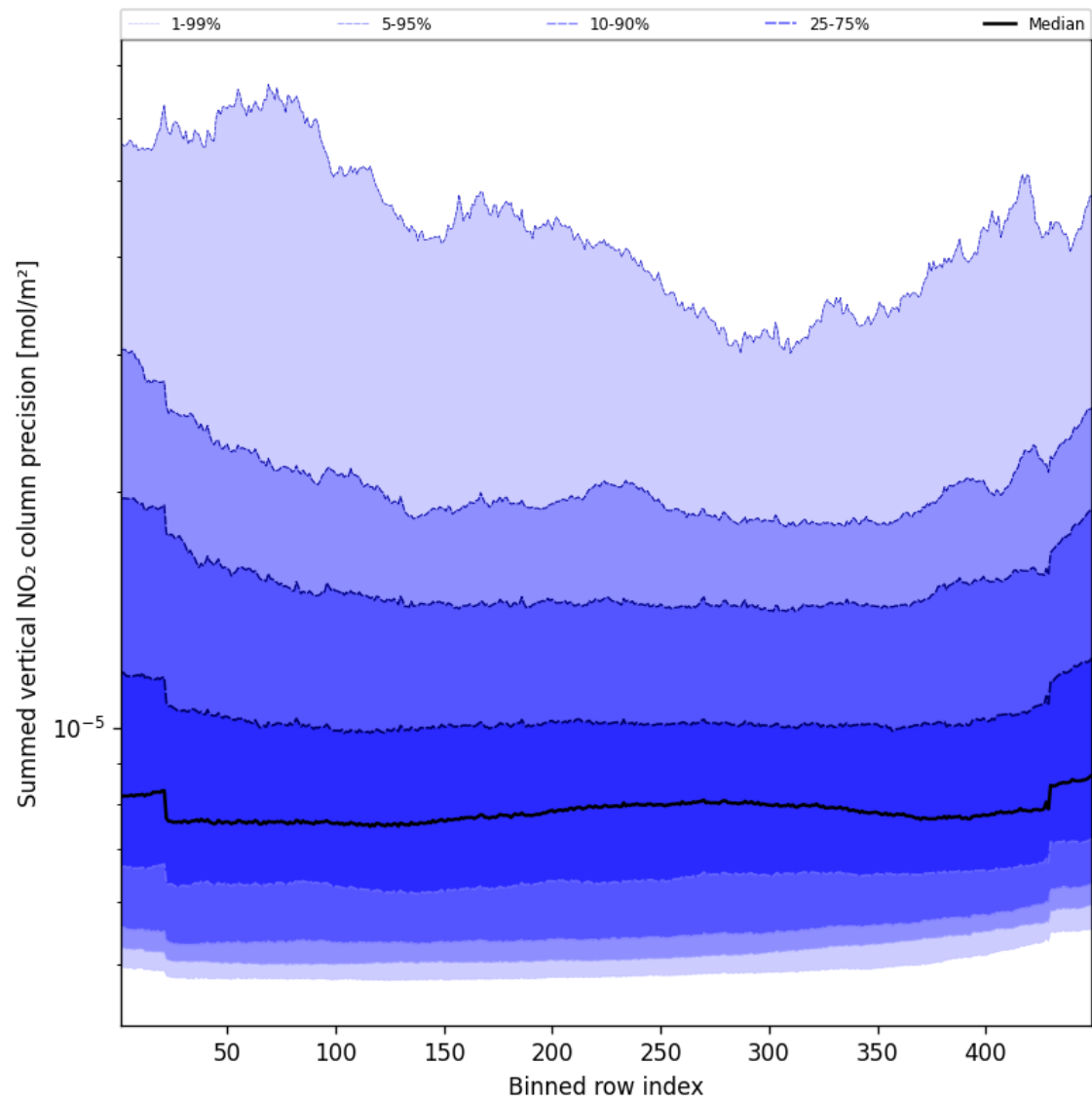
Figure 56: Along track statistics of “Summed vertical NO 2 column precision” for 2025-09-27 to 2025-09-28
