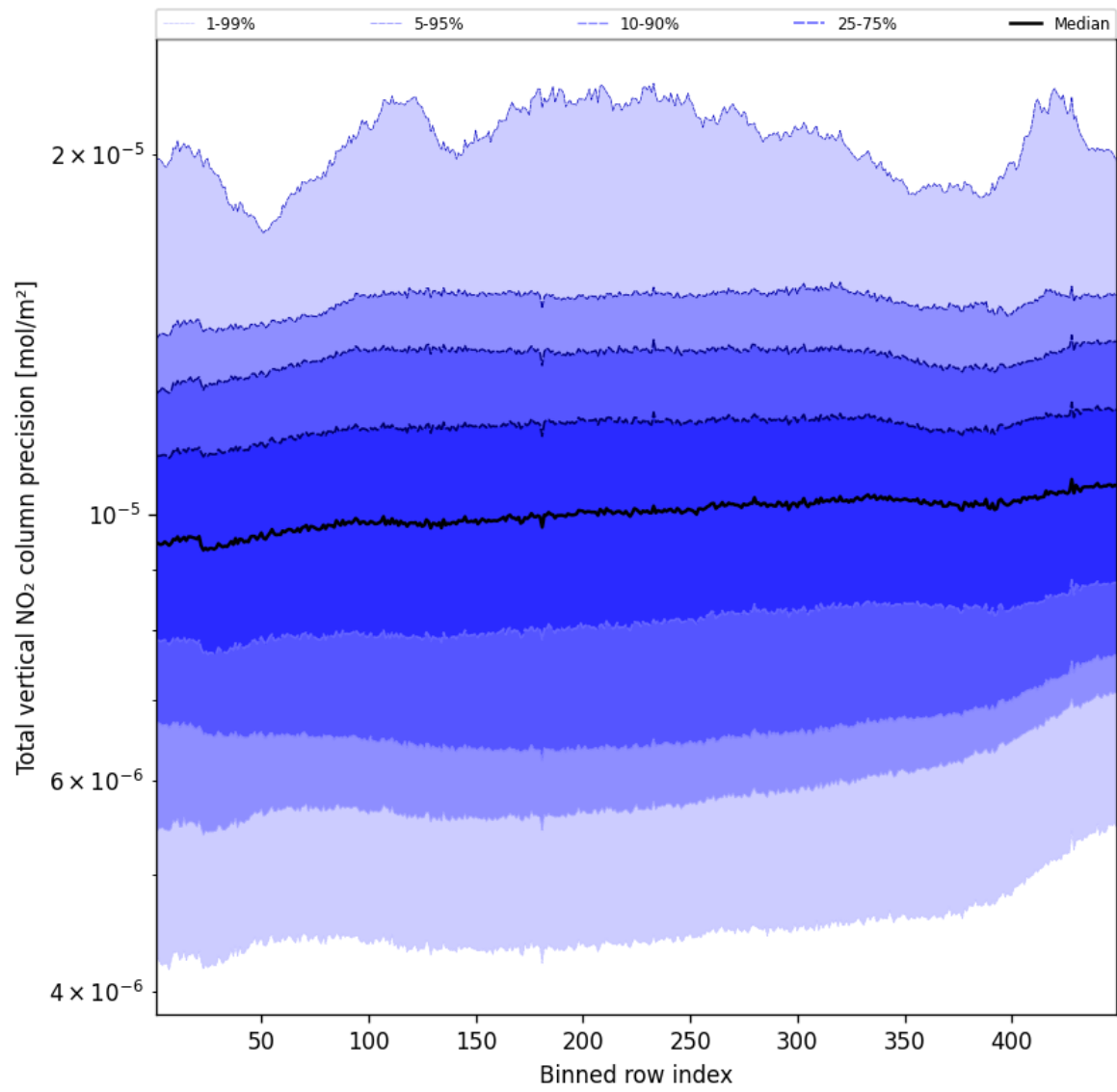
Figure 54: Along track statistics of “Total vertical NO 2 column precision” for 2025-09-27 to 2025-09-28
