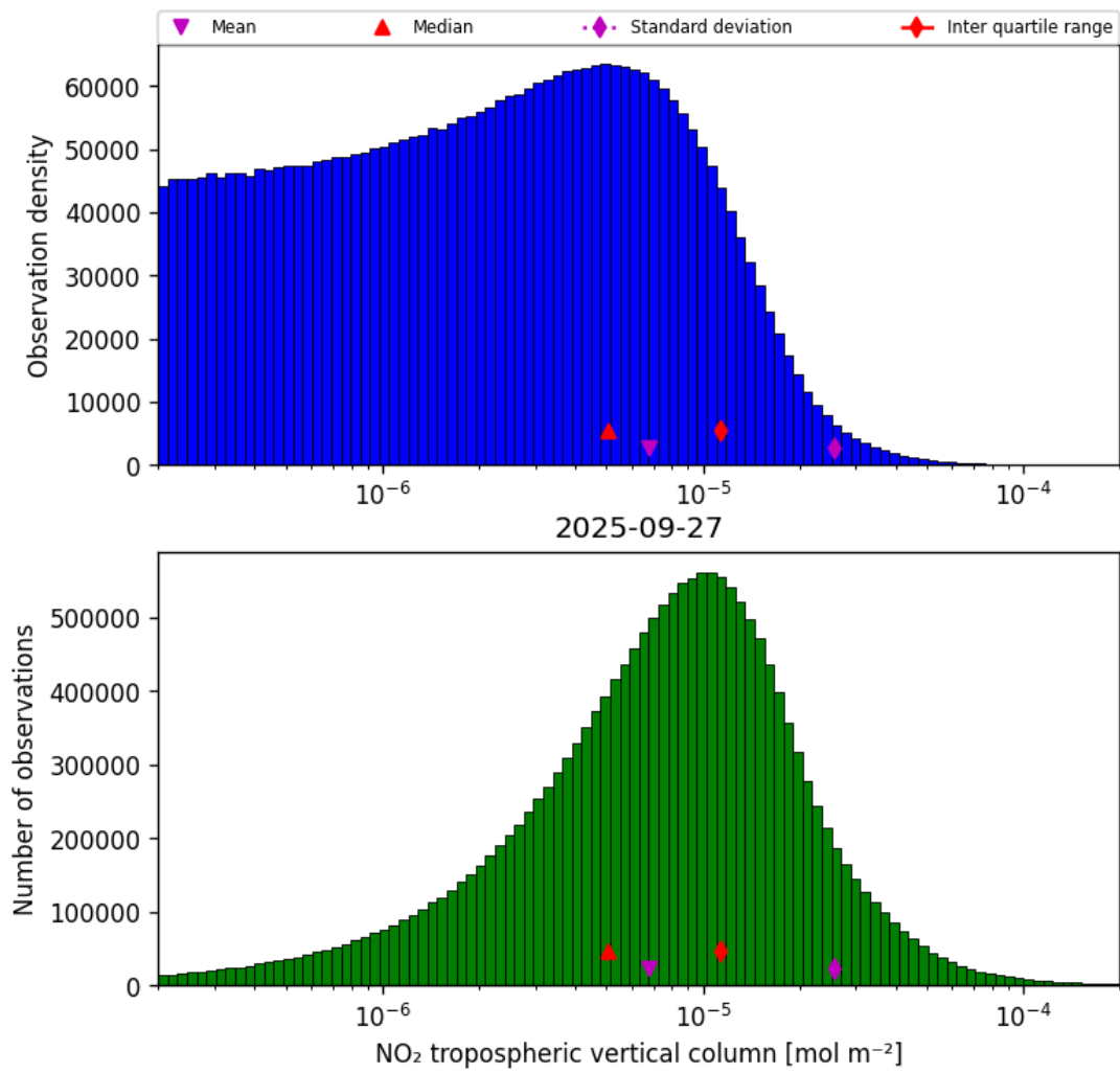
Figure 27: Histogram of “NO 2 tropospheric vertical column” for 2025-09-27 to 2025-09-28
