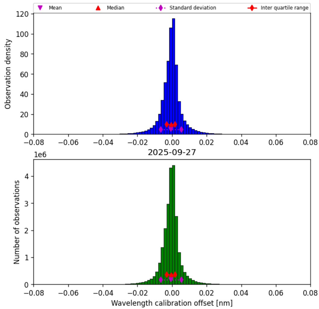
Figure 33: Histogram of “Wavelength calibration offset” for 2025-09-27 to 2025-09-28
