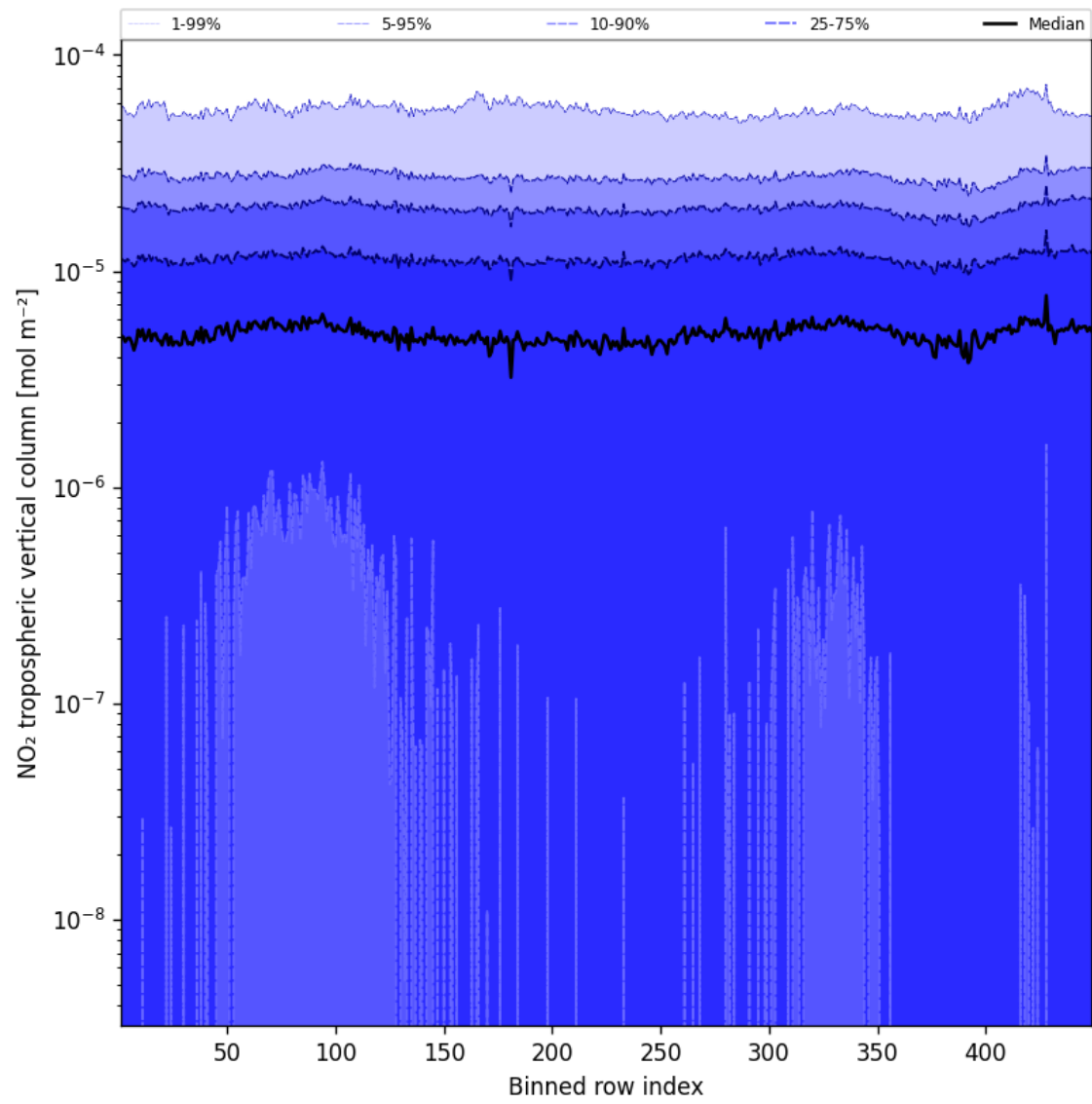
Figure 44: Along track statistics of “NO 2 tropospheric vertical column” for 2025-09-27 to 2025-09-28
