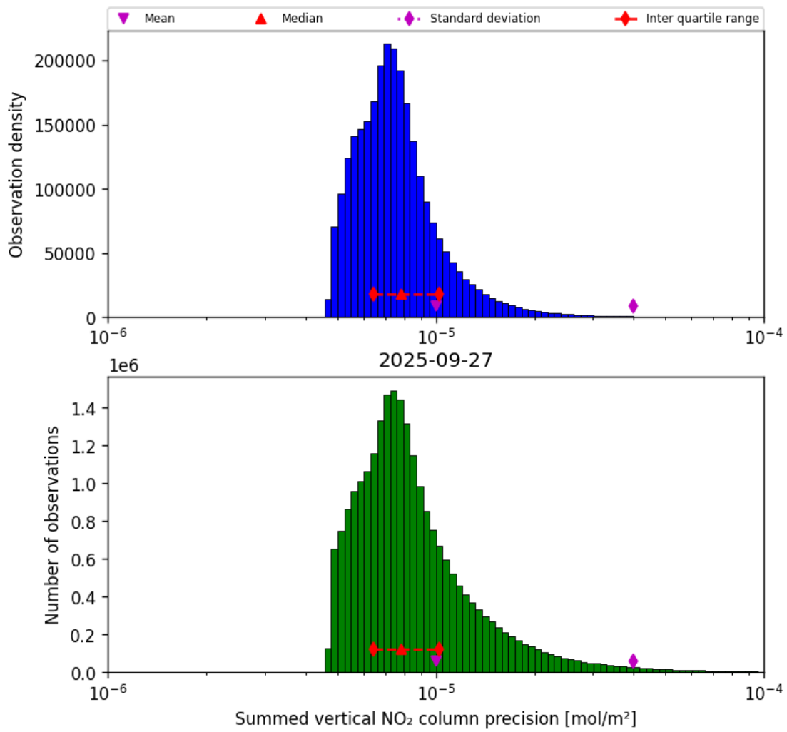
Figure 39: Histogram of “Summed vertical NO 2 column precision” for 2025-09-27 to 2025-09-28
