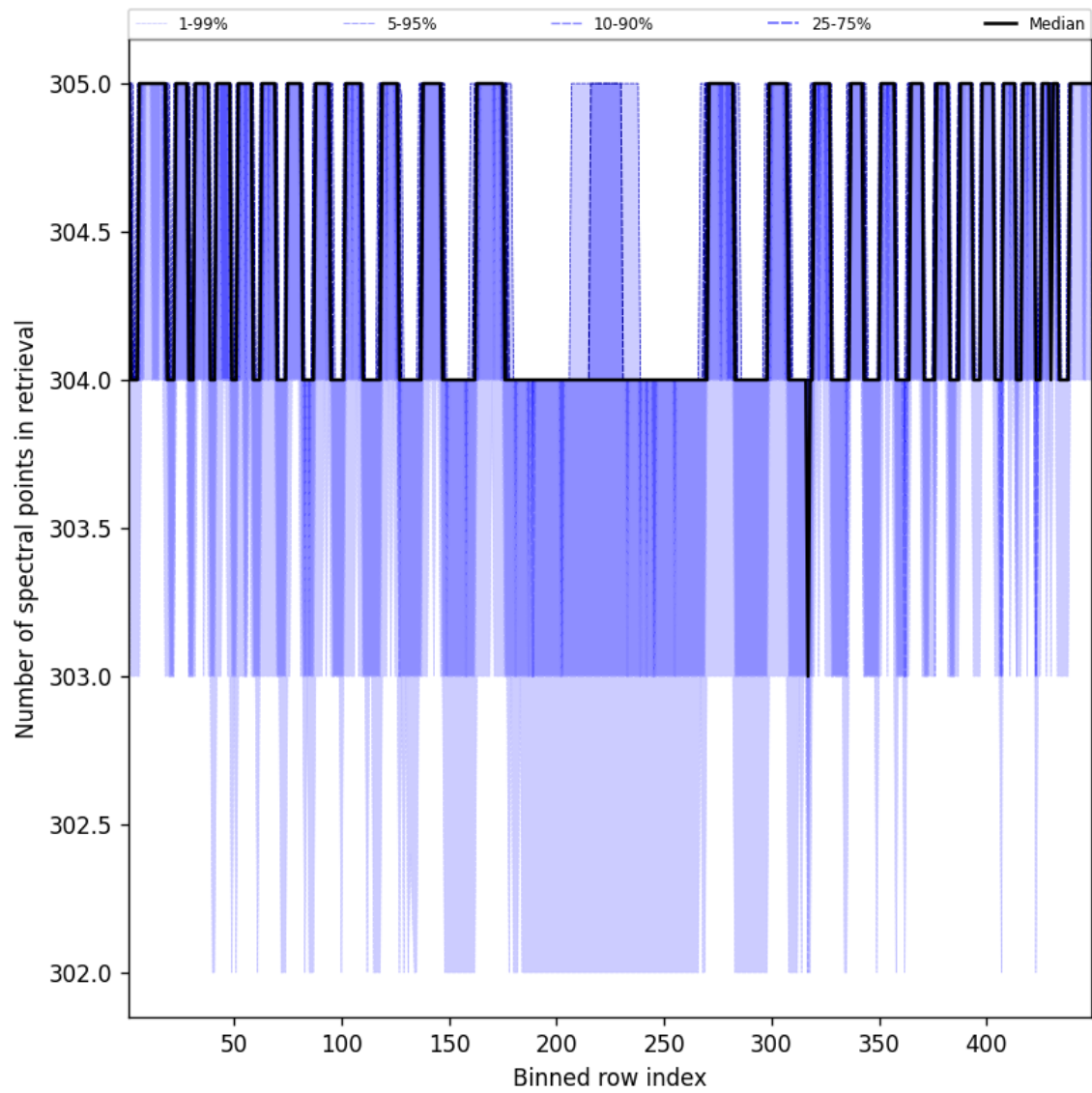
Figure 48: Along track statistics of “Number of spectral points in retrieval” for 2025-09-27 to 2025-09-28
