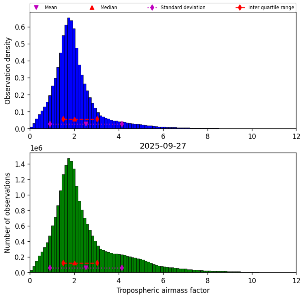
Figure 29: Histogram of “Tropospheric airmass factor” for 2025-09-27 to 2025-09-28
