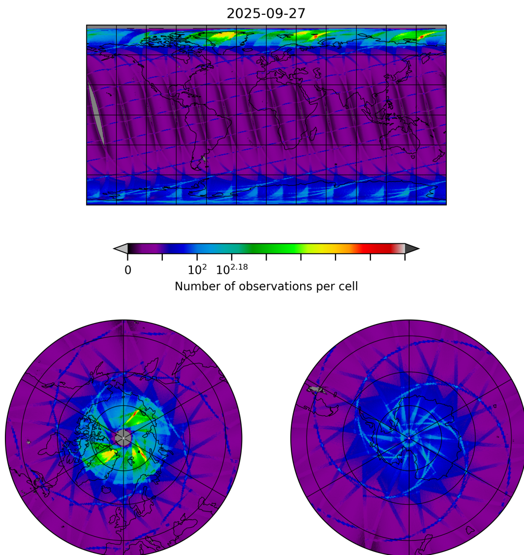
Figure 8: Map of the number of observations for 2025-09-27 to 2025-09-28
