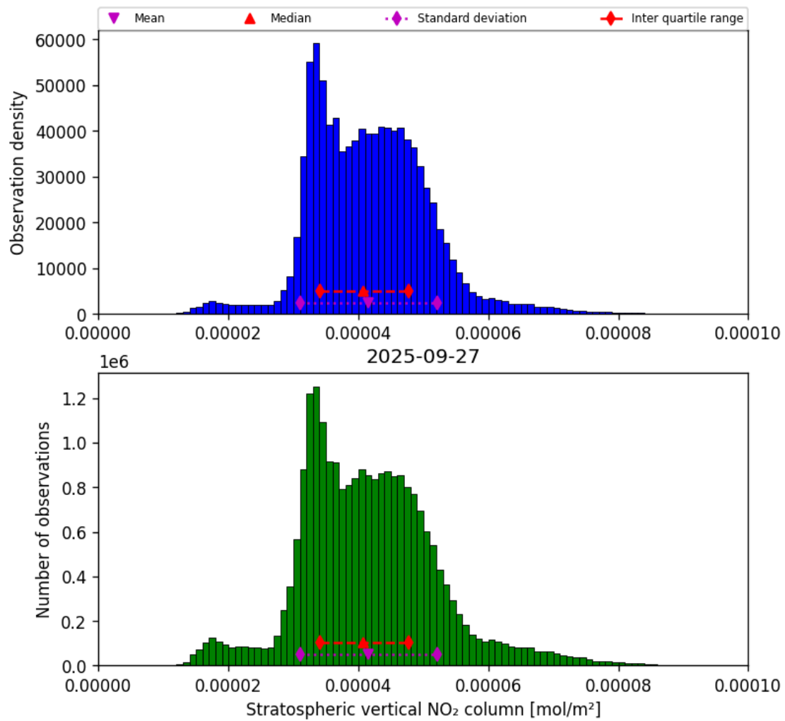
Figure 34: Histogram of “Stratospheric vertical NO 2 column” for 2025-09-27 to 2025-09-28
