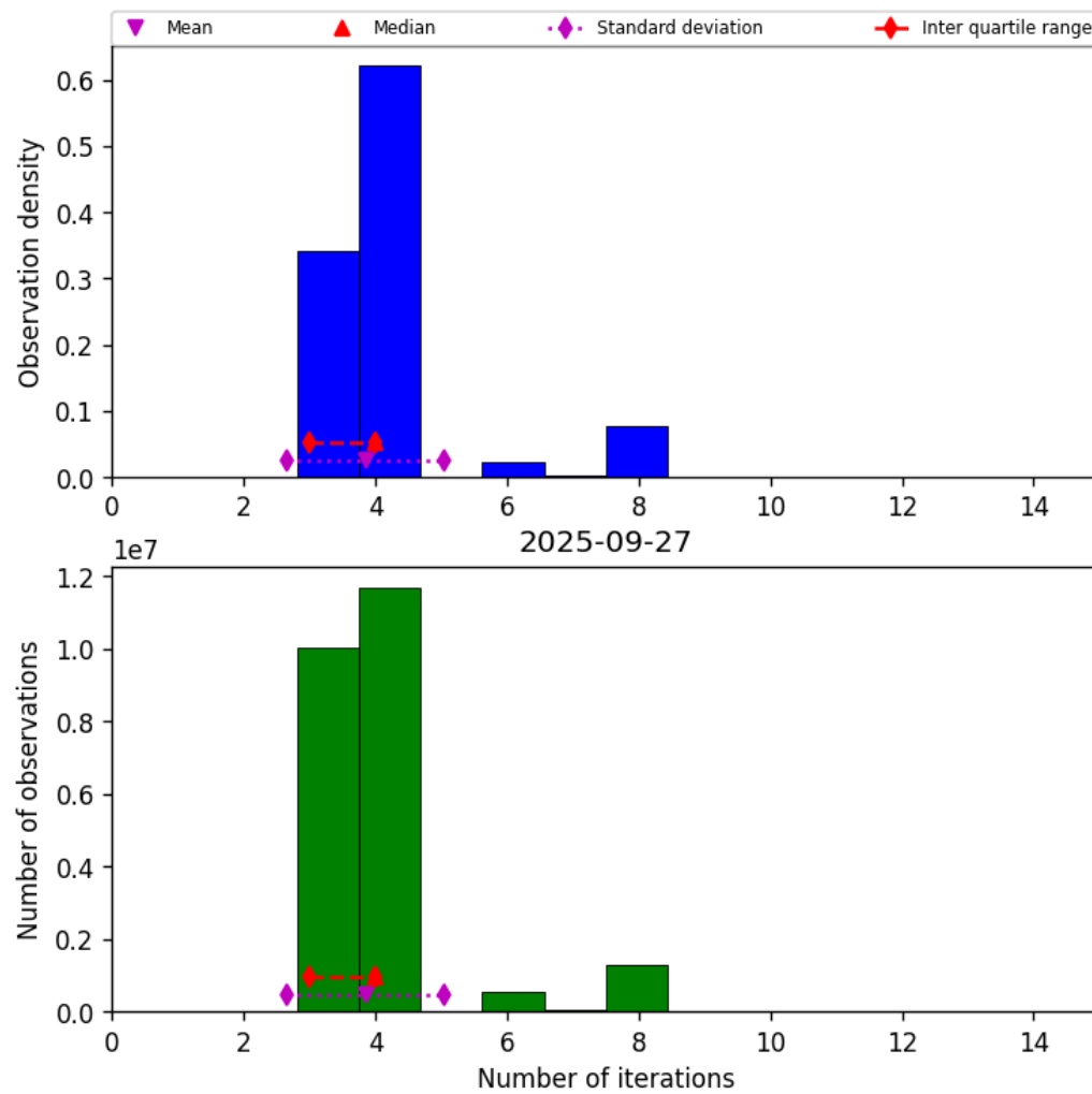
Figure 32: Histogram of “Number of iterations” for 2025-09-27 to 2025-09-28
