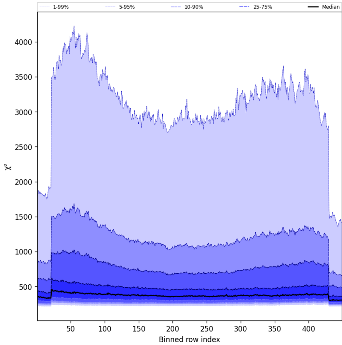
Figure 57: Along track statistics of “ \chi^2 ” for 2025-09-27 to 2025-09-28
