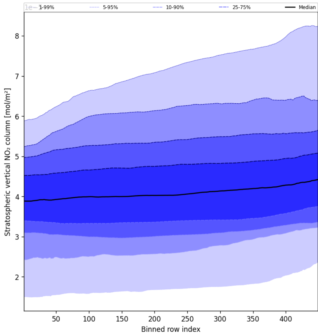
Figure 51: Along track statistics of “Stratospheric vertical NO 2 column” for 2025-09-27 to 2025-09-28
