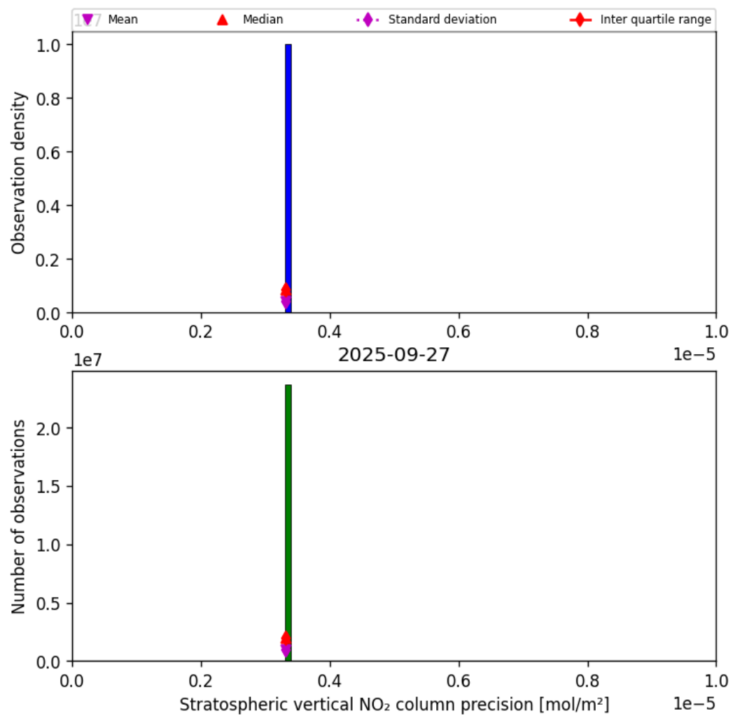
Figure 35: Histogram of “Stratospheric vertical NO 2 column precision” for 2025-09-27 to 2025-09-28
