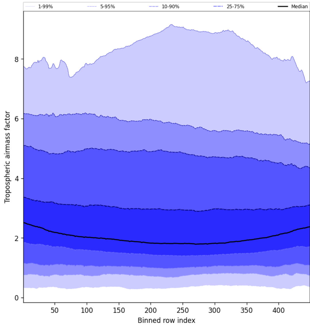
Figure 46: Along track statistics of “Tropospheric air mass factor” for 2025-09-27 to 2025-09-28
