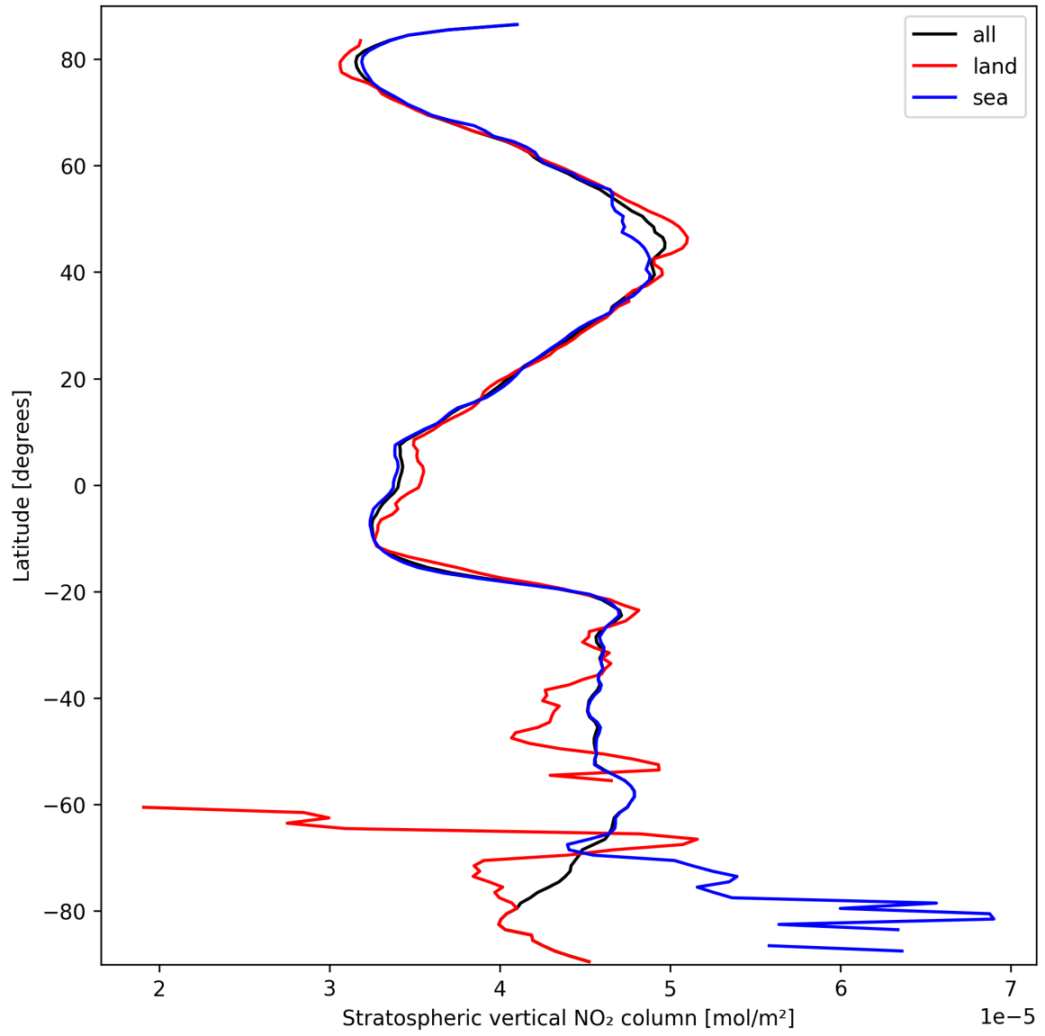
Figure 17: Zonal average of “Stratospheric vertical NO 2 column” for 2025-09-27 to 2025-09-28.
