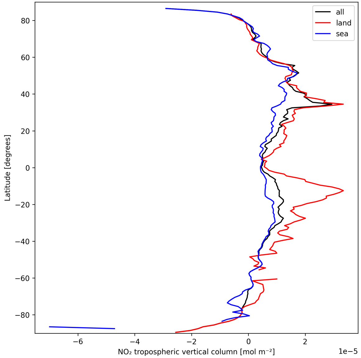
Figure 10: Zonal average of “NO 2 tropospheric vertical column” for 2025-09-27 to 2025-09-28.
