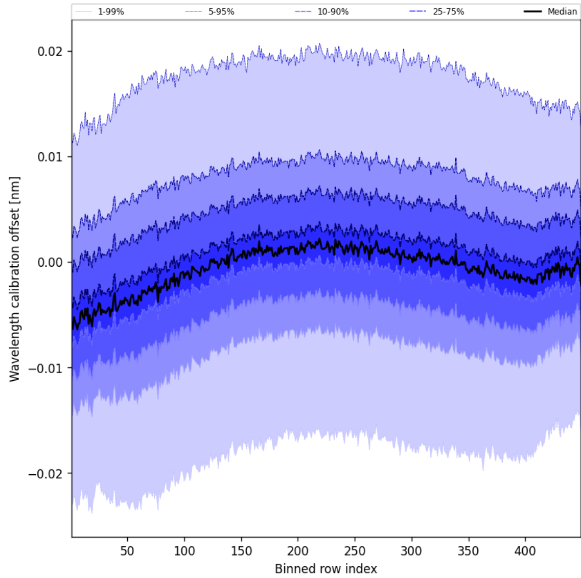
Figure 50: Along track statistics of “Wavelength calibration offset” for 2025-09-27 to 2025-09-28
