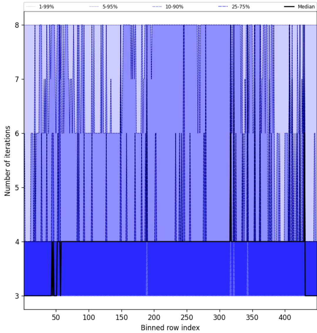
Figure 49: Along track statistics of “Number of iterations” for 2025-09-27 to 2025-09-28
