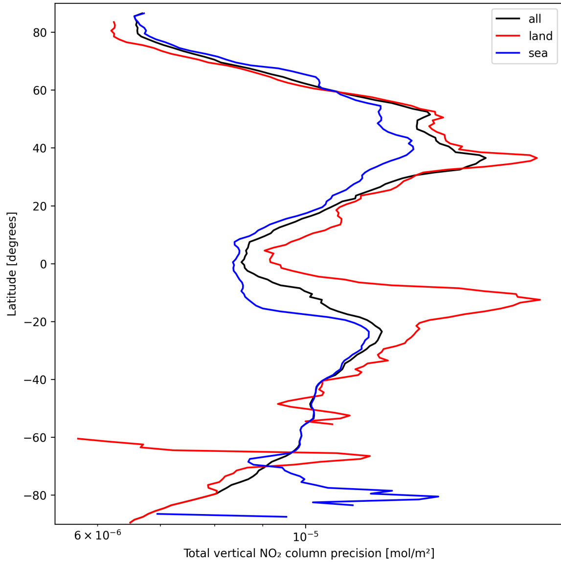
Figure 20: Zonal average of “Total vertical NO 2 column precision” for 2025-09-27 to 2025-09-28.
