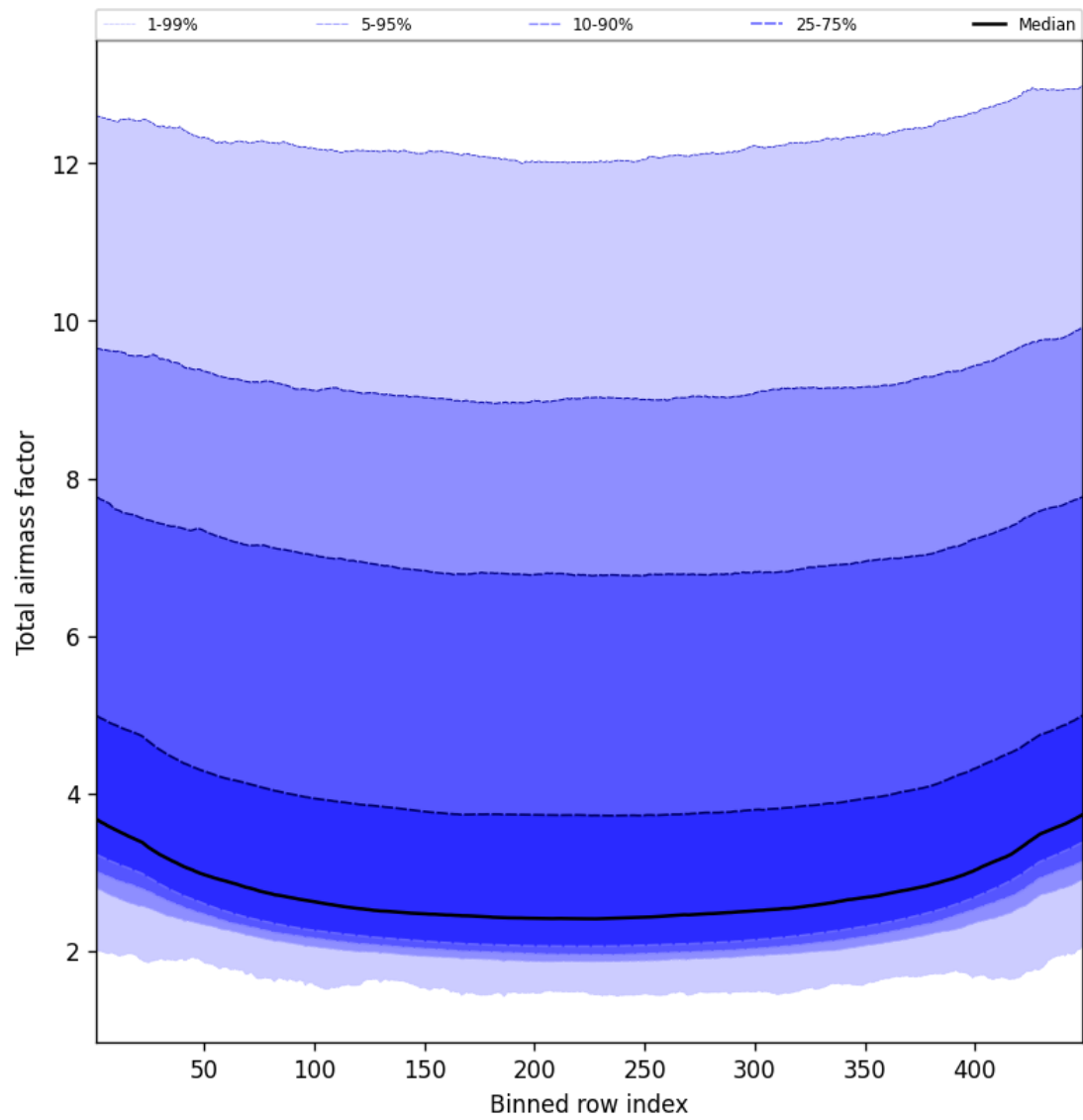
Figure 47: Along track statistics of “Total airmass factor” for 2025-09-27 to 2025-09-28
