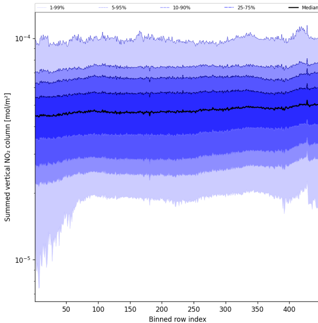
Figure 55: Along track statistics of “Summed vertical NO 2 column” for 2025-09-27 to 2025-09-28
