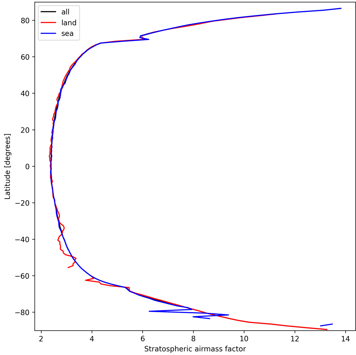
Figure 25: Zonal average of “Stratospheric air mass factor” for 2025-09-27 to 2025-09-28.
