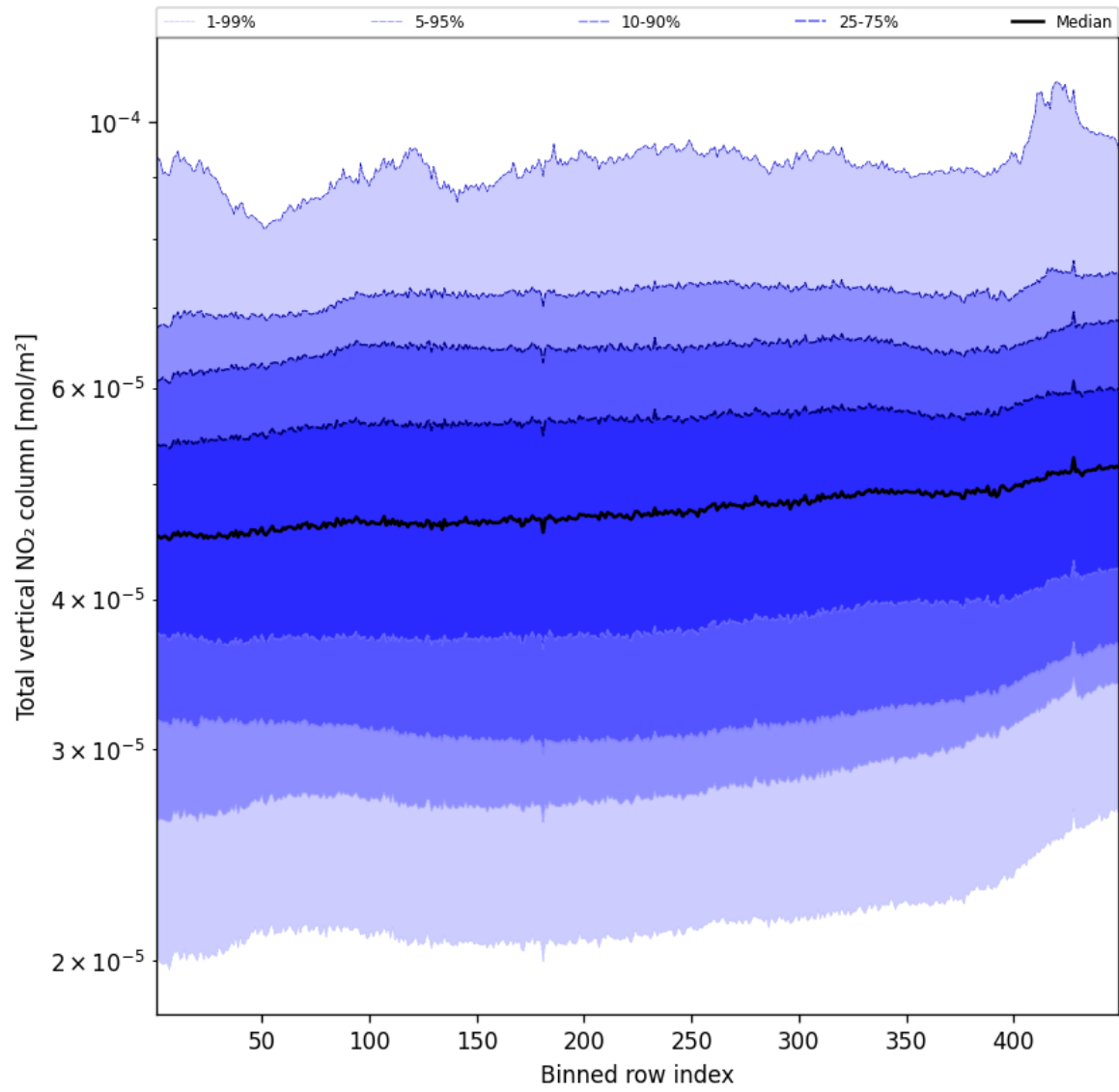
Figure 53: Along track statistics of “Total vertical NO 2 column” for 2025-09-27 to 2025-09-28
