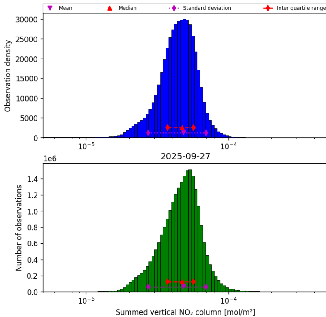
Figure 38: Histogram of “Summed vertical NO 2 column” for 2025-09-27 to 2025-09-28
