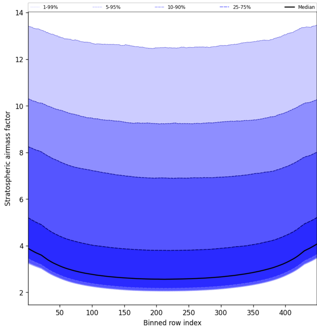
Figure 59: Along track statistics of “Stratospheric airmass factor” for 2025-09-27 to 2025-09-28
