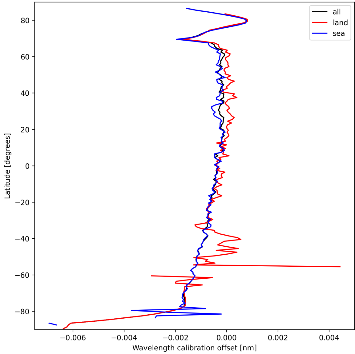
Figure 16: Zonal average of “Wavelength calibration offset” for 2025-09-27 to 2025-09-28.
