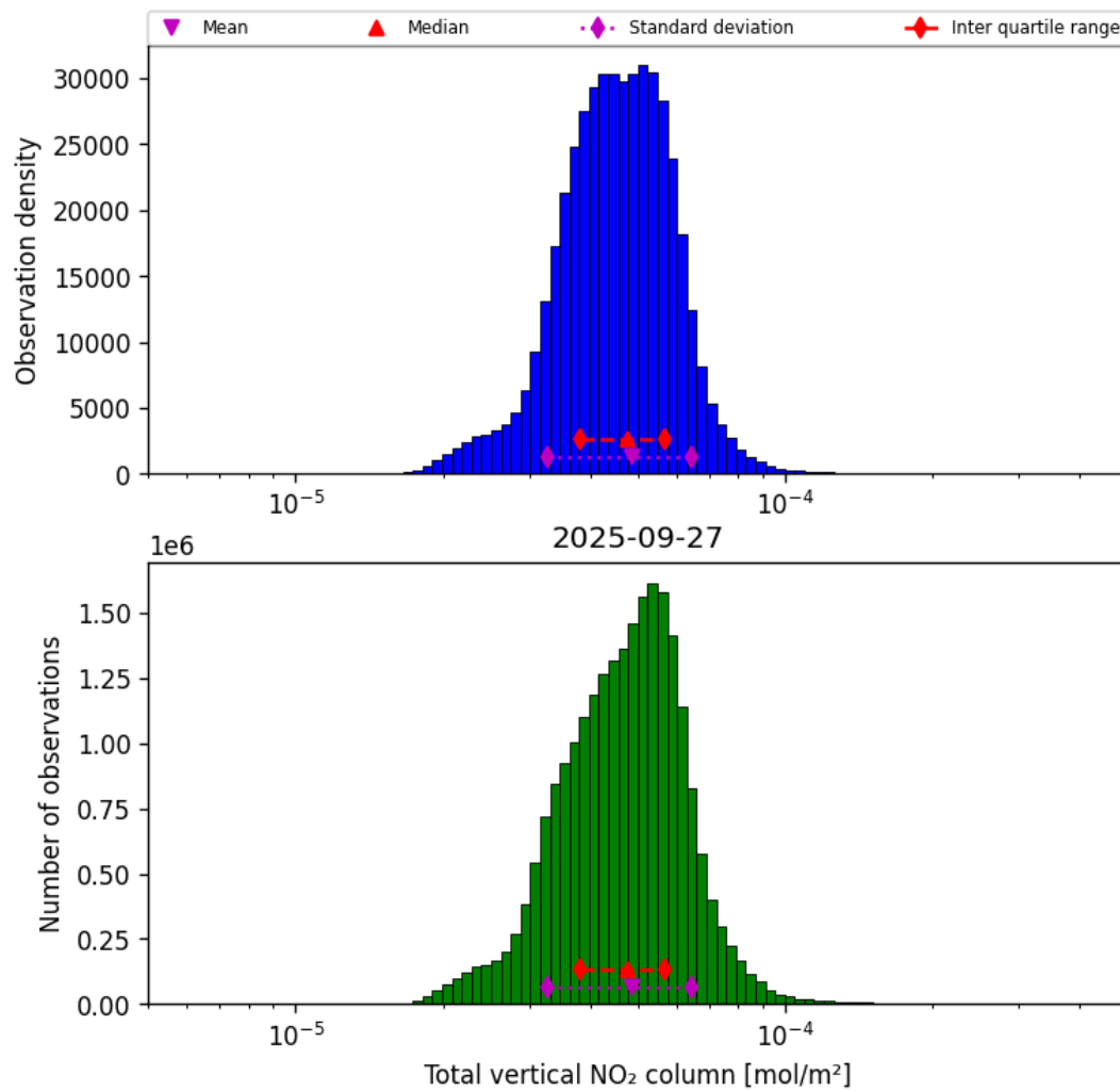
Figure 36: Histogram of “Total vertical NO 2 column” for 2025-09-27 to 2025-09-28
