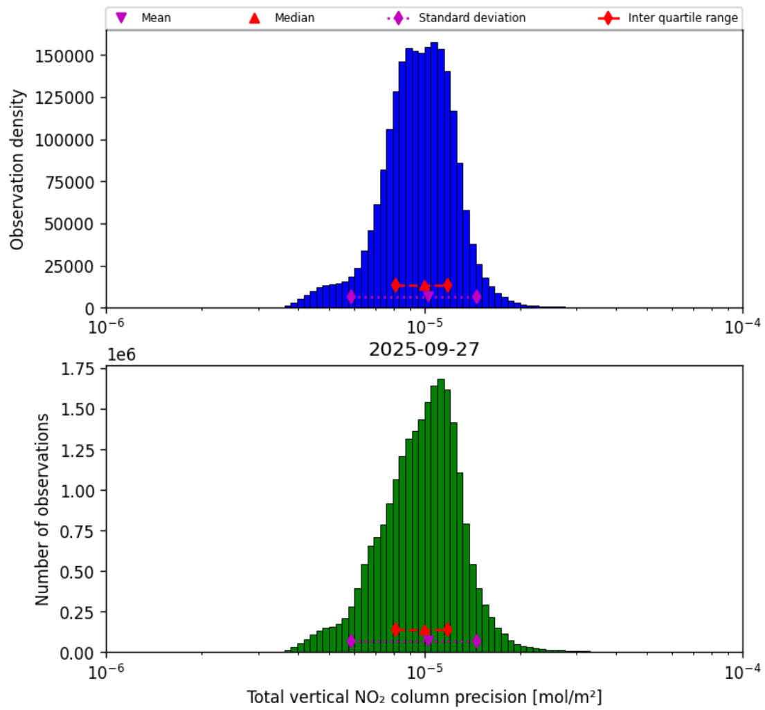
Figure 37: Histogram of “Total vertical NO 2 column precision” for 2025-09-27 to 2025-09-28
