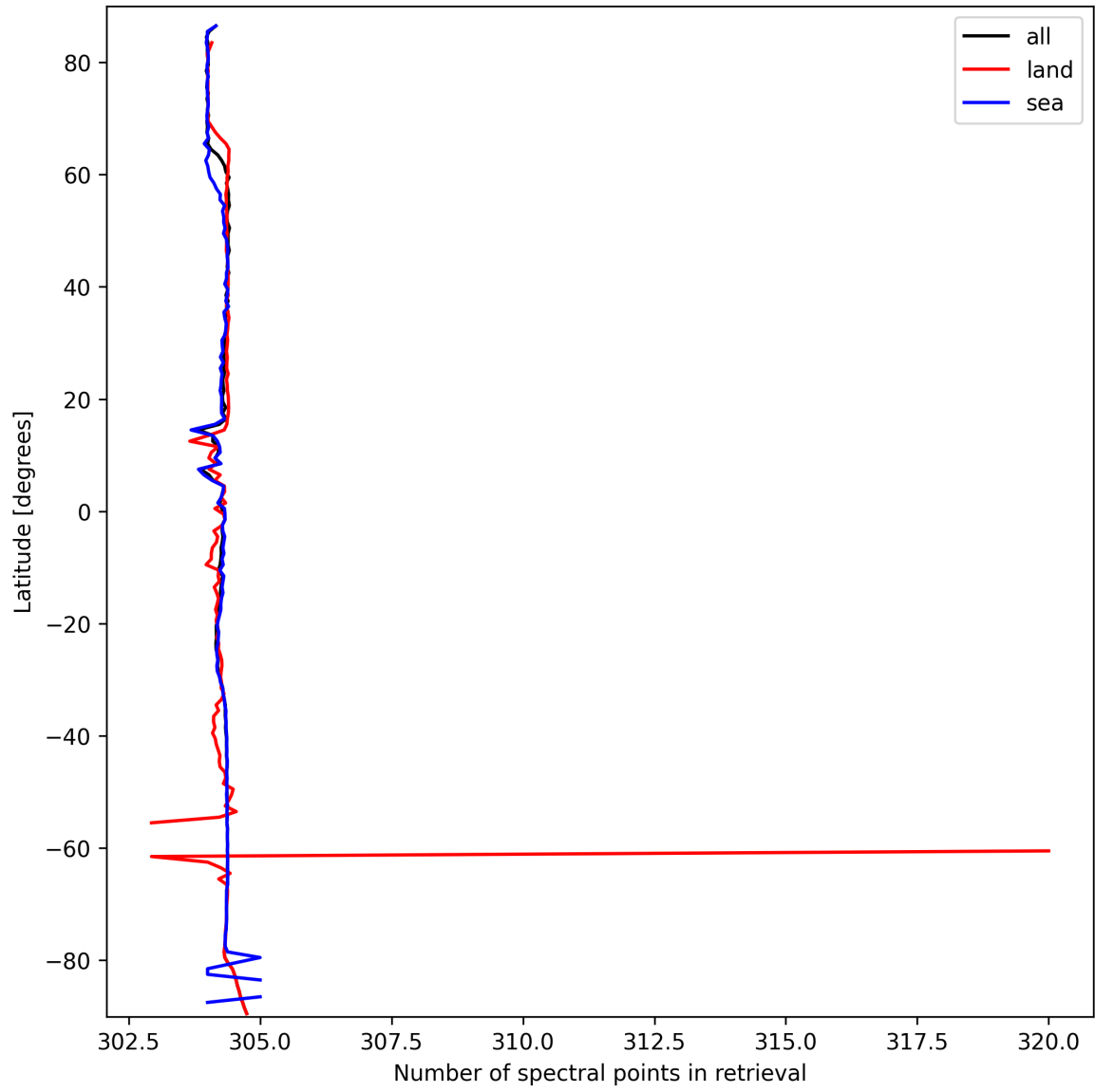
Figure 14: Zonal average of “Number of spectral points in retrieval” for 2025-09-27 to 2025-09-28.
