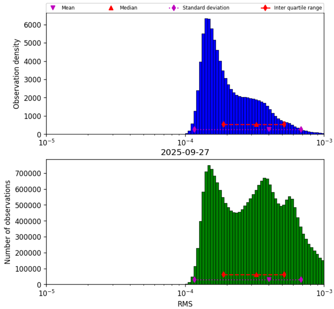
Figure 41: Histogram of “RMS” for 2025-09-27 to 2025-09-28
