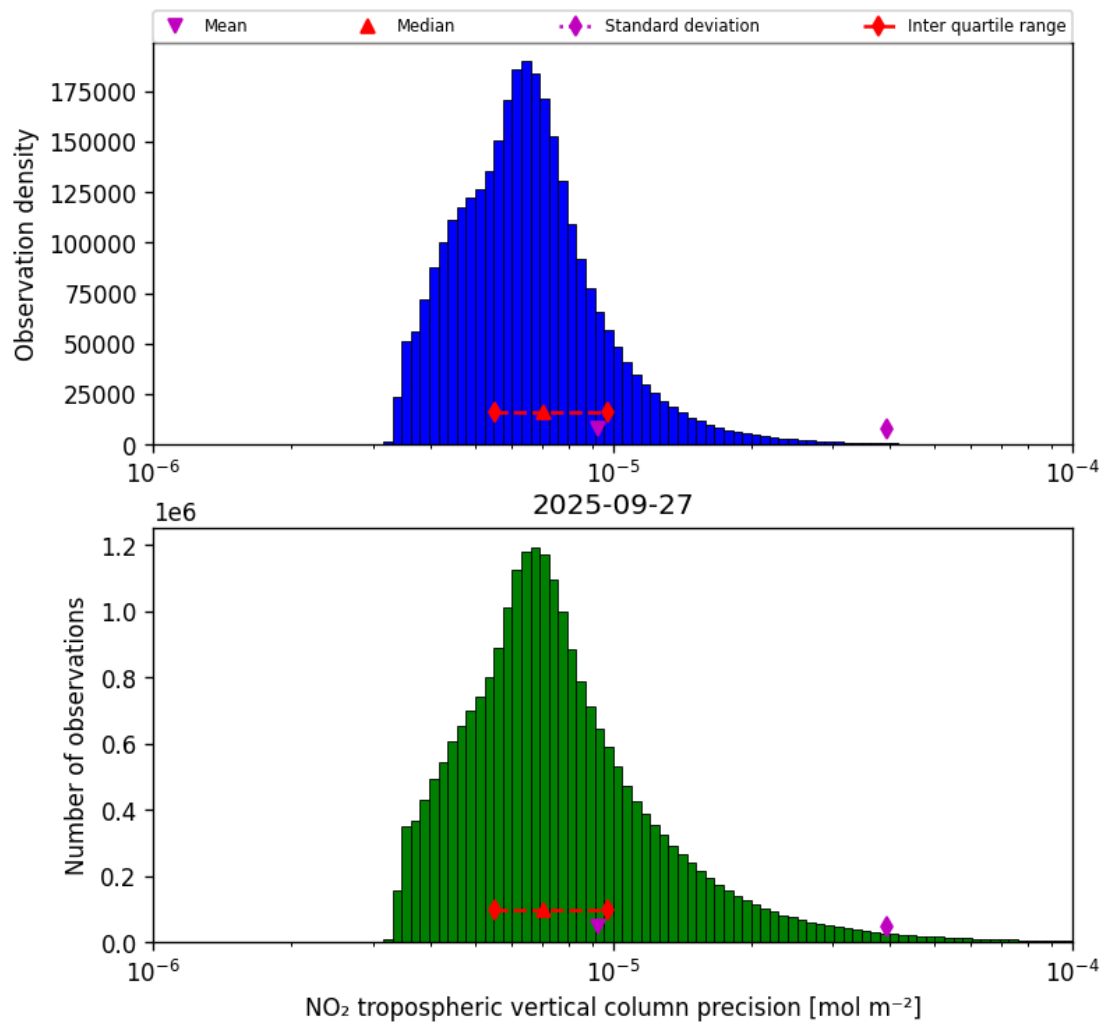
Figure 28: Histogram of “NO 2 tropospheric vertical column precision” for 2025-09-27 to 2025-09-28
