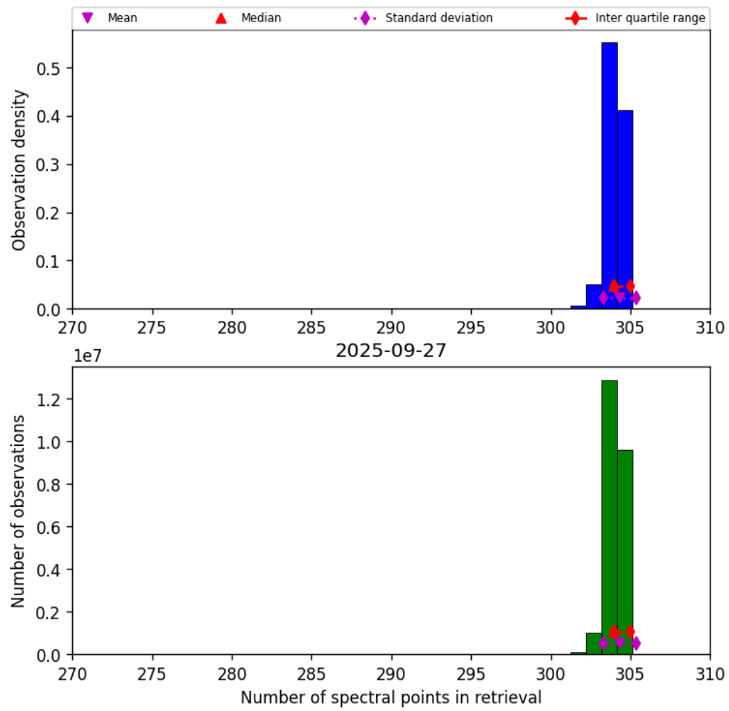
Figure 31: Histogram of “Number of spectral points in retrieval” for 2025-09-27 to 2025-09-28
