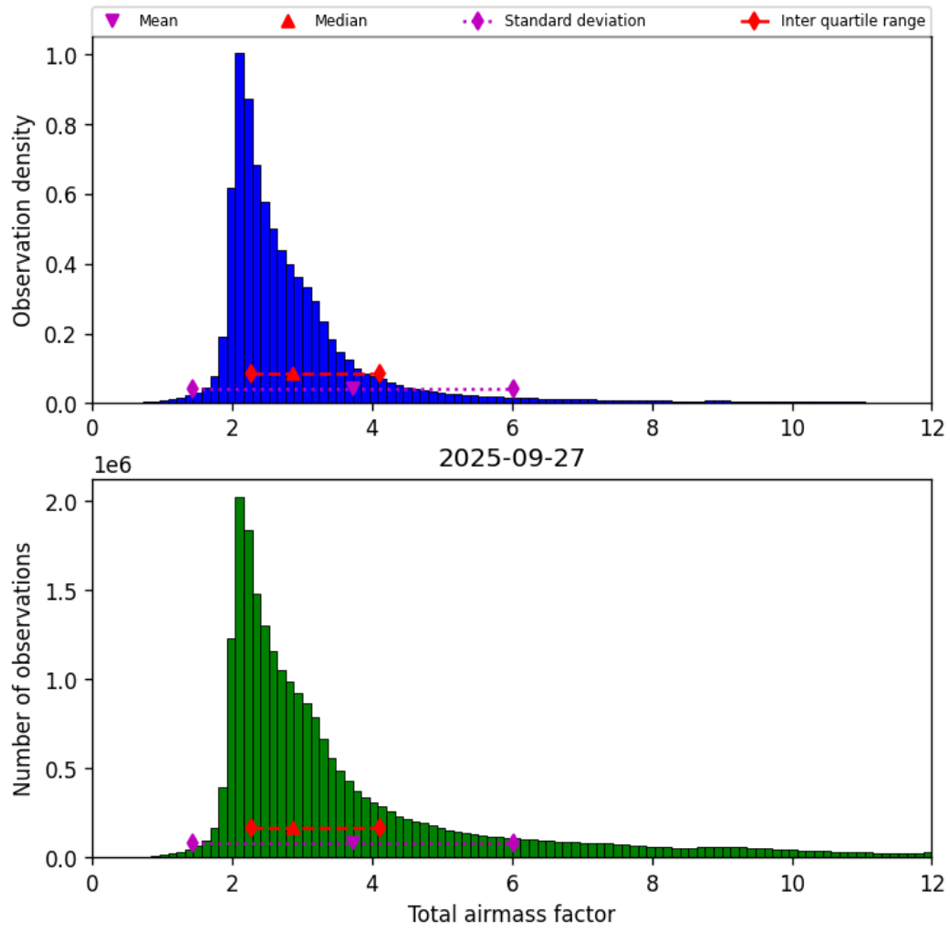
Figure 30: Histogram of “Total airmass factor” for 2025-09-27 to 2025-09-28
