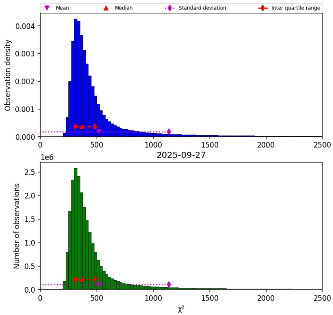
Figure 40: Histogram of “ \chi^2 ” for 2025-09-27 to 2025-09-28
