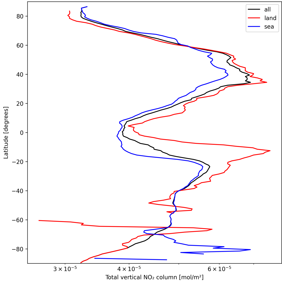
Figure 19: Zonal average of “Total vertical NO 2 column” for 2025-09-27 to 2025-09-28.
