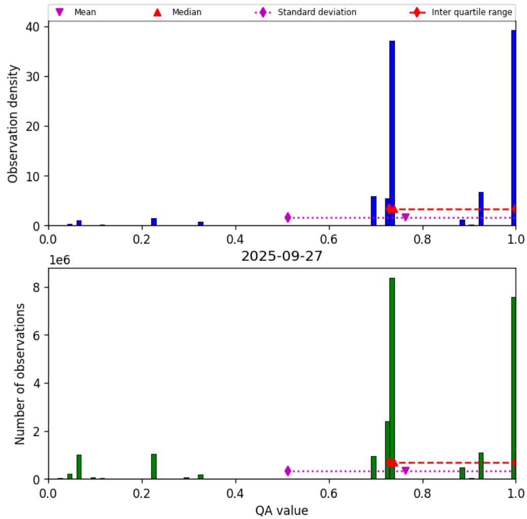
Figure 26: Histogram of “QA value” for 2025-09-27 to 2025-09-28
