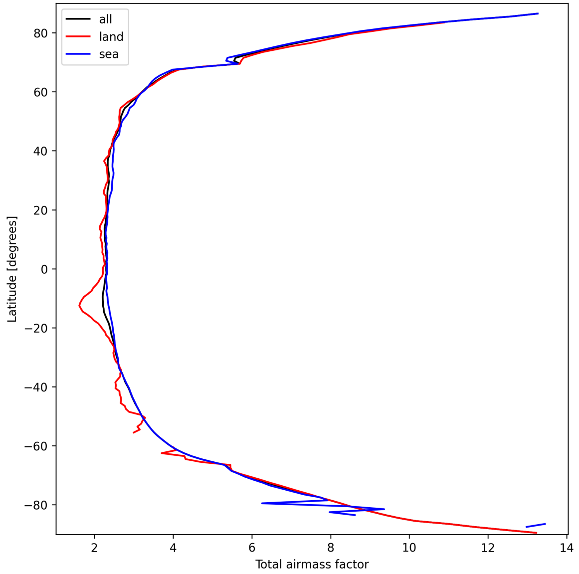
Figure 13: Zonal average of “Total airmass factor” for 2025-09-27 to 2025-09-28.
