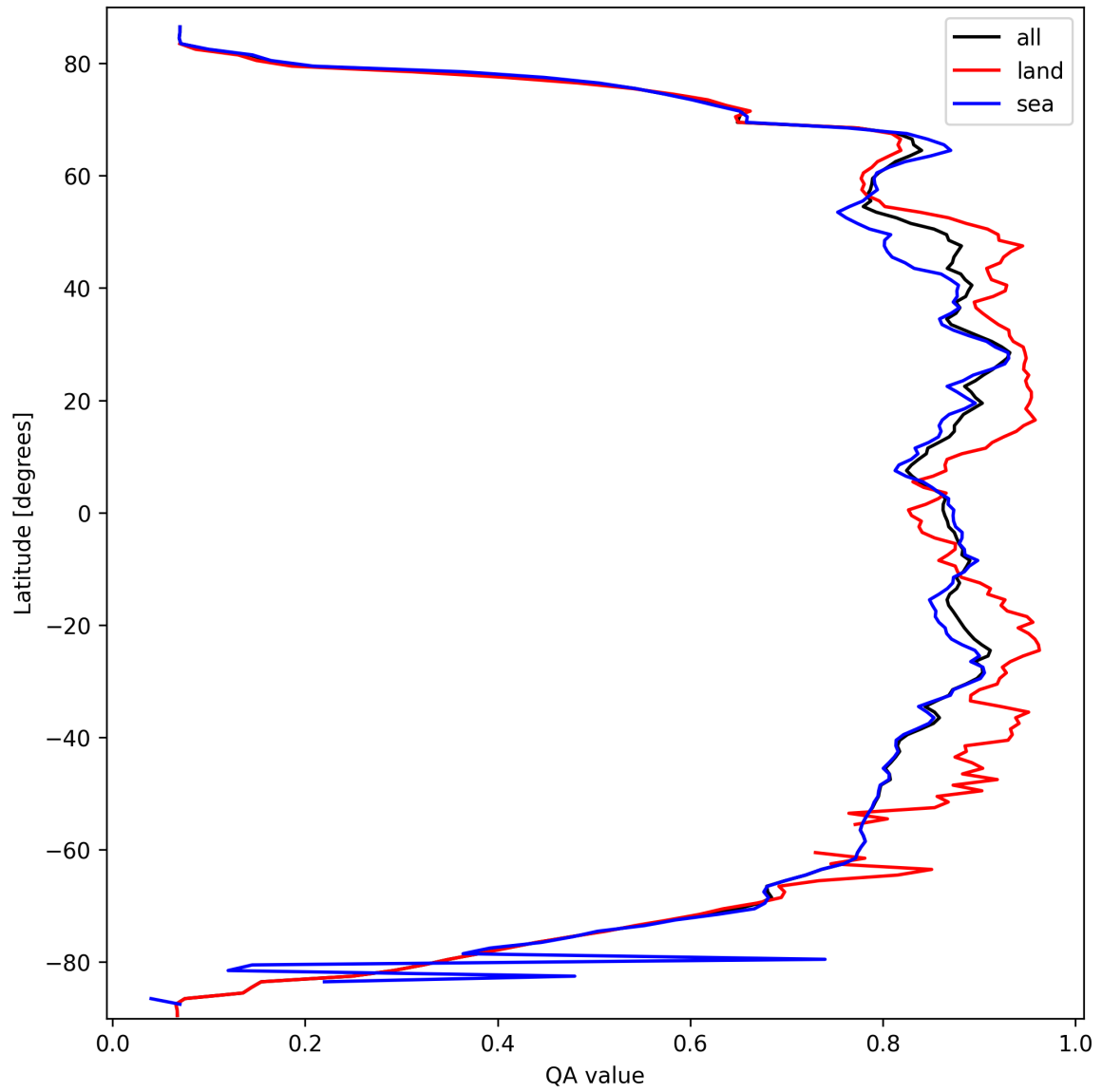
Figure 9: Zonal average of “QA value” for 2025-09-27 to 2025-09-28.
