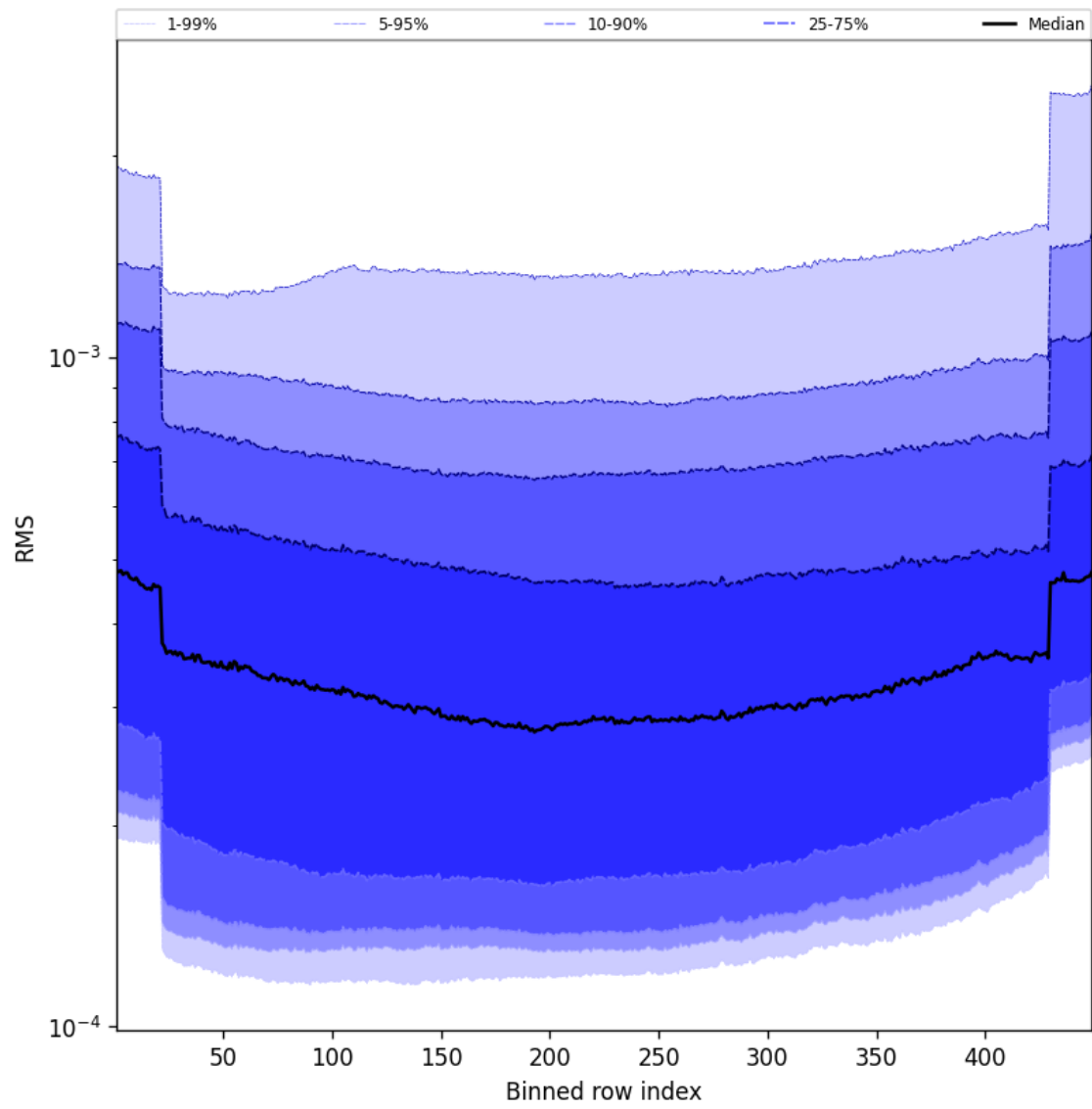
Figure 58: Along track statistics of “RMS” for 2025-09-27 to 2025-09-28
