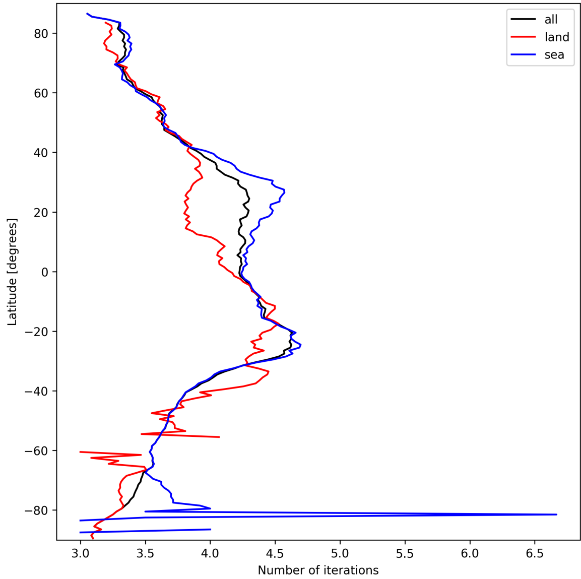
Figure 15: Zonal average of “Number of iterations” for 2025-09-27 to 2025-09-28.
