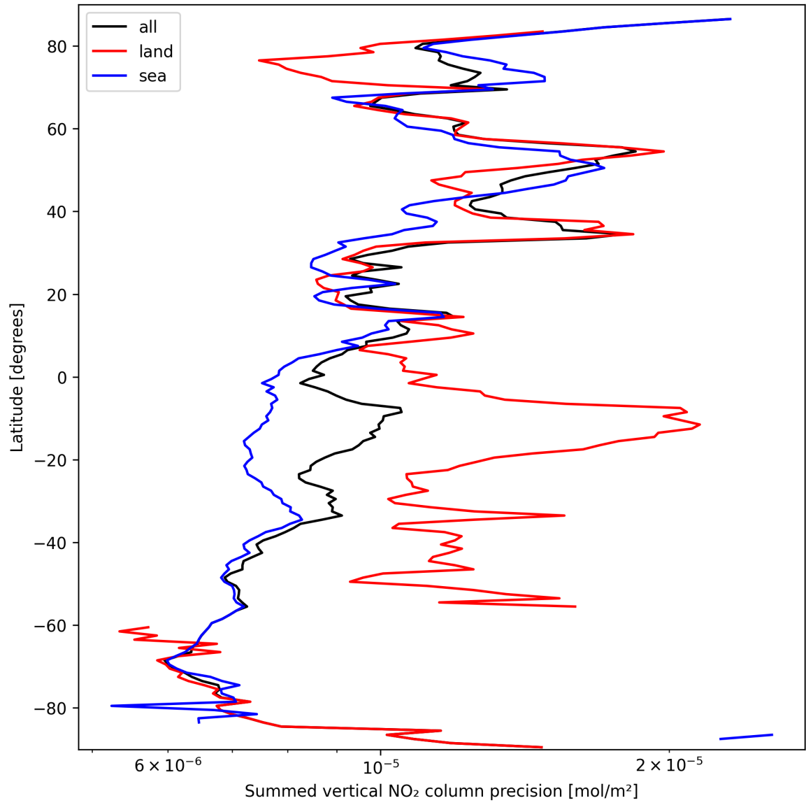
Figure 22: Zonal average of “Summed vertical NO 2 column precision” for 2025-09-27 to 2025-09-28.
