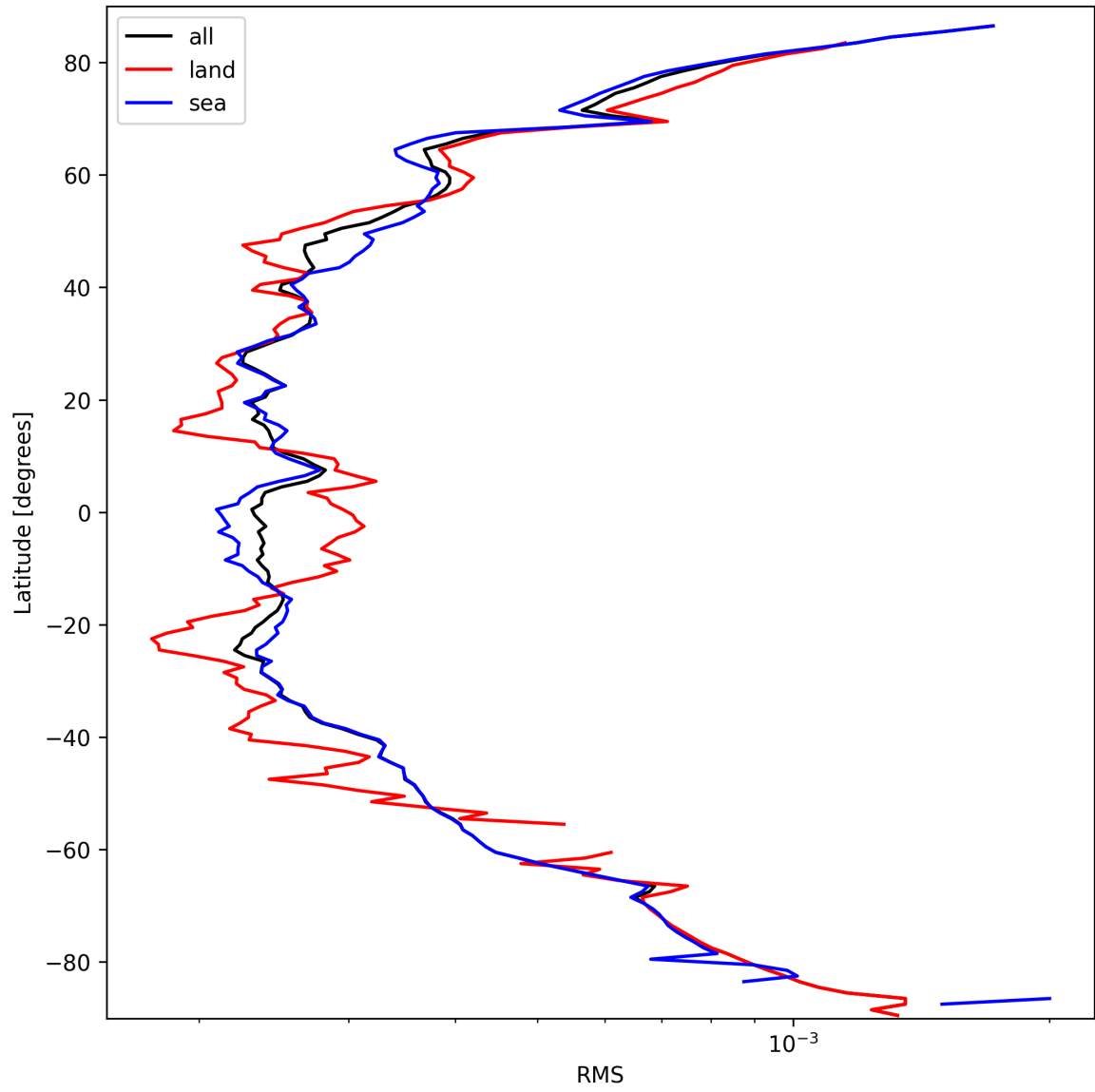
Figure 24: Zonal average of “RMS” for 2025-09-27 to 2025-09-28.
