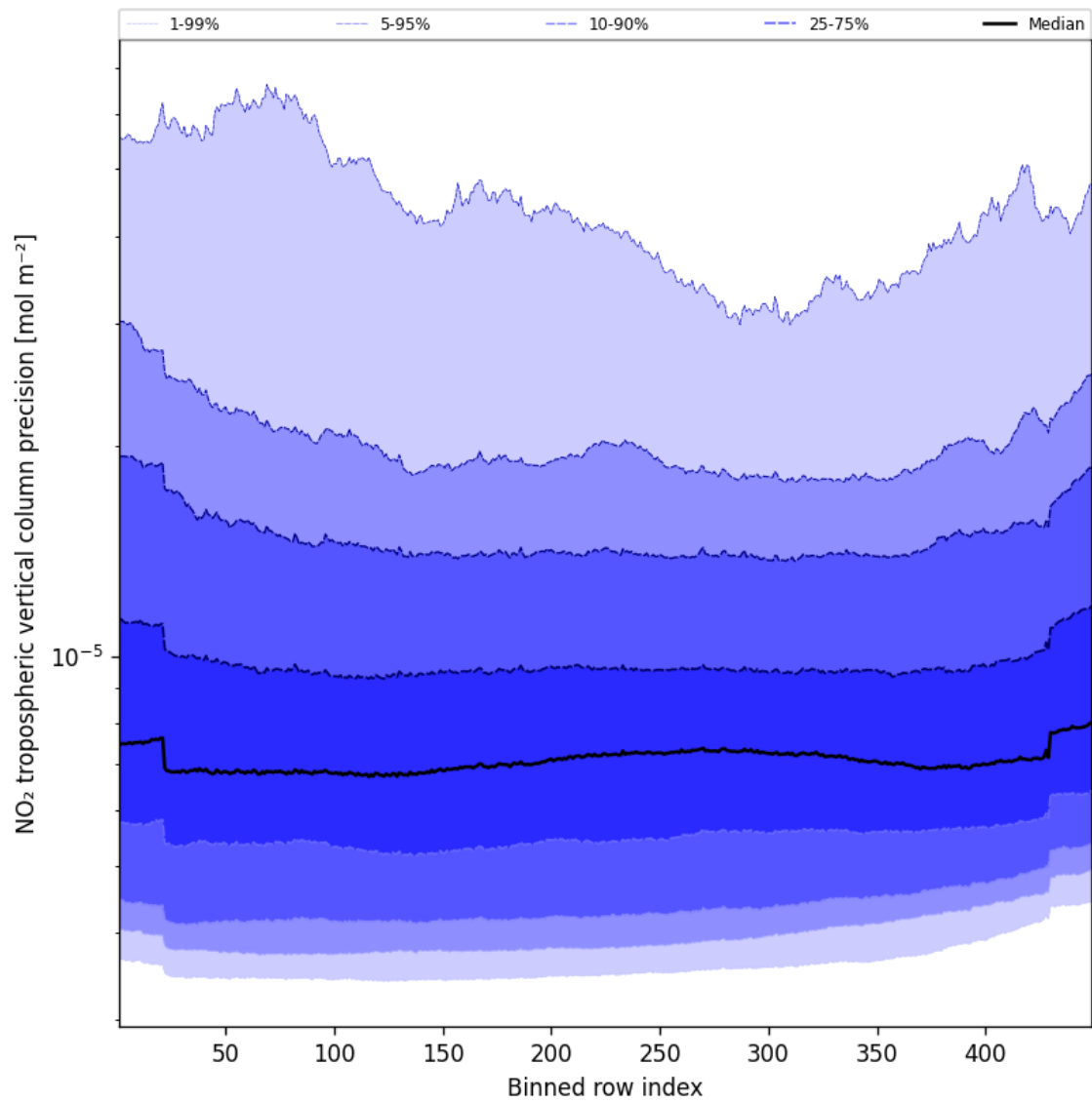
Figure 45: Along track statistics of “NO 2 tropospheric vertical column precision” for 2025-09-27 to 2025-09-28
