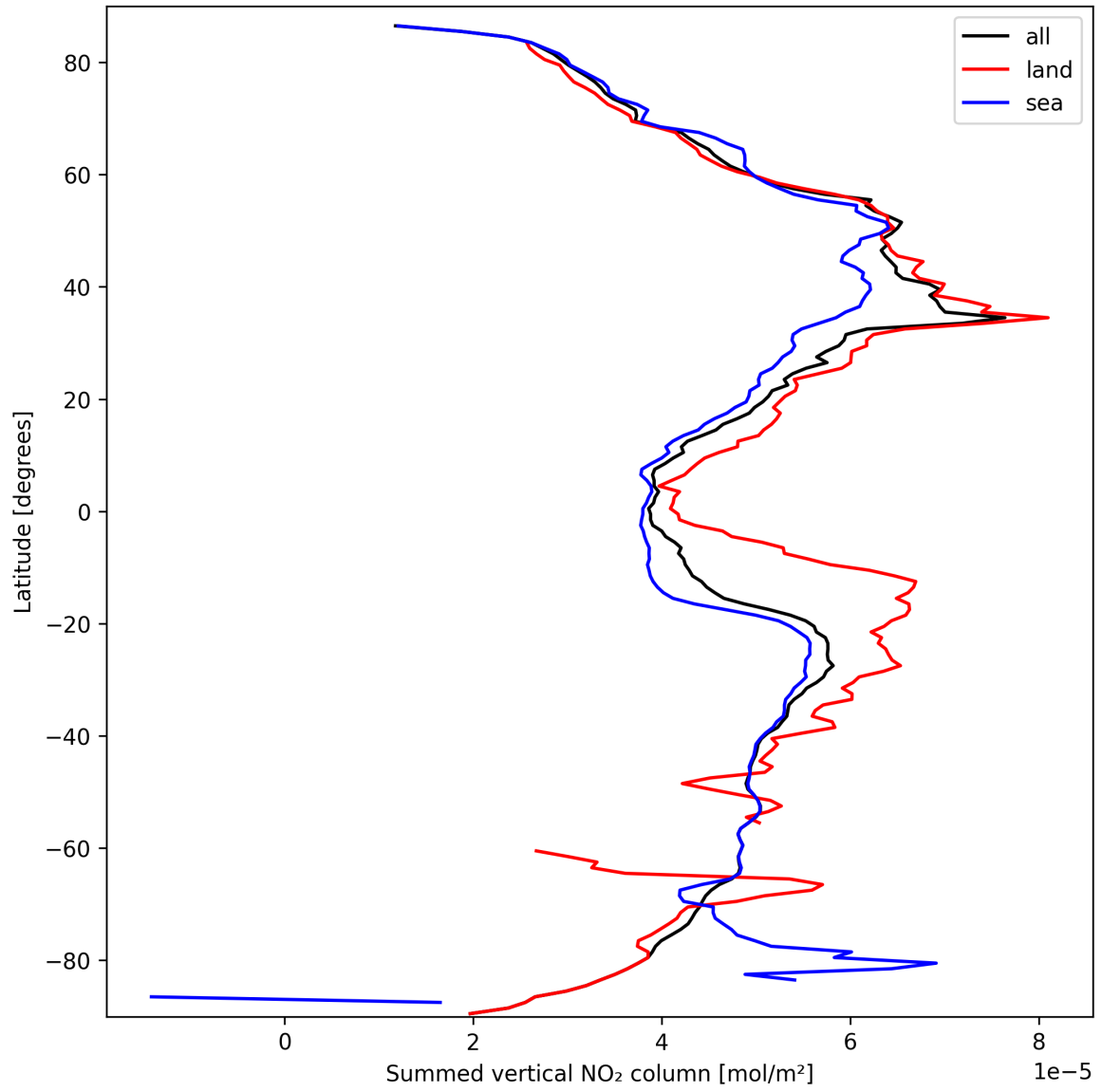
Figure 21: Zonal average of “Summed vertical NO 2 column” for 2025-09-27 to 2025-09-28.
