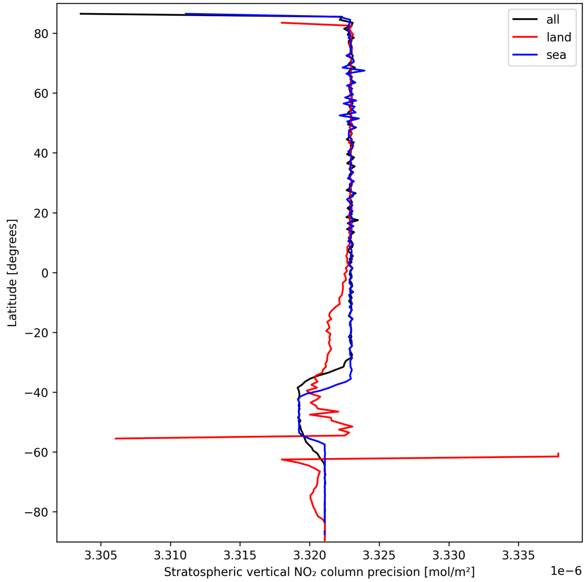
Figure 18: Zonal average of "Stratospheric vertical NO 2 column precision" for 2025-09-27 to 2025-09-28.
