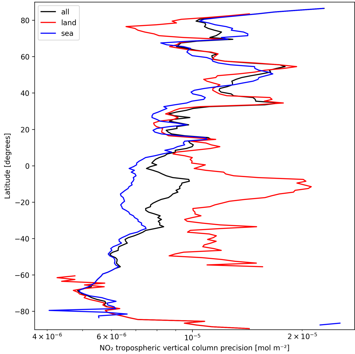
Figure 11: Zonal average of “NO 2 tropospheric vertical column precision” for 2025-09-27 to 2025-09-28.
