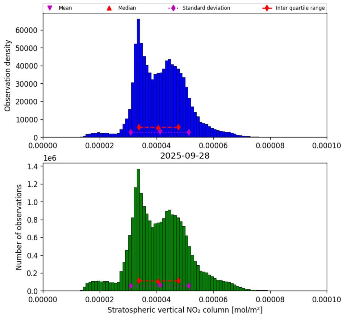
Figure 34: Histogram of “Stratospheric vertical NO 2 column” for 2025-09-28 to 2025-09-29
