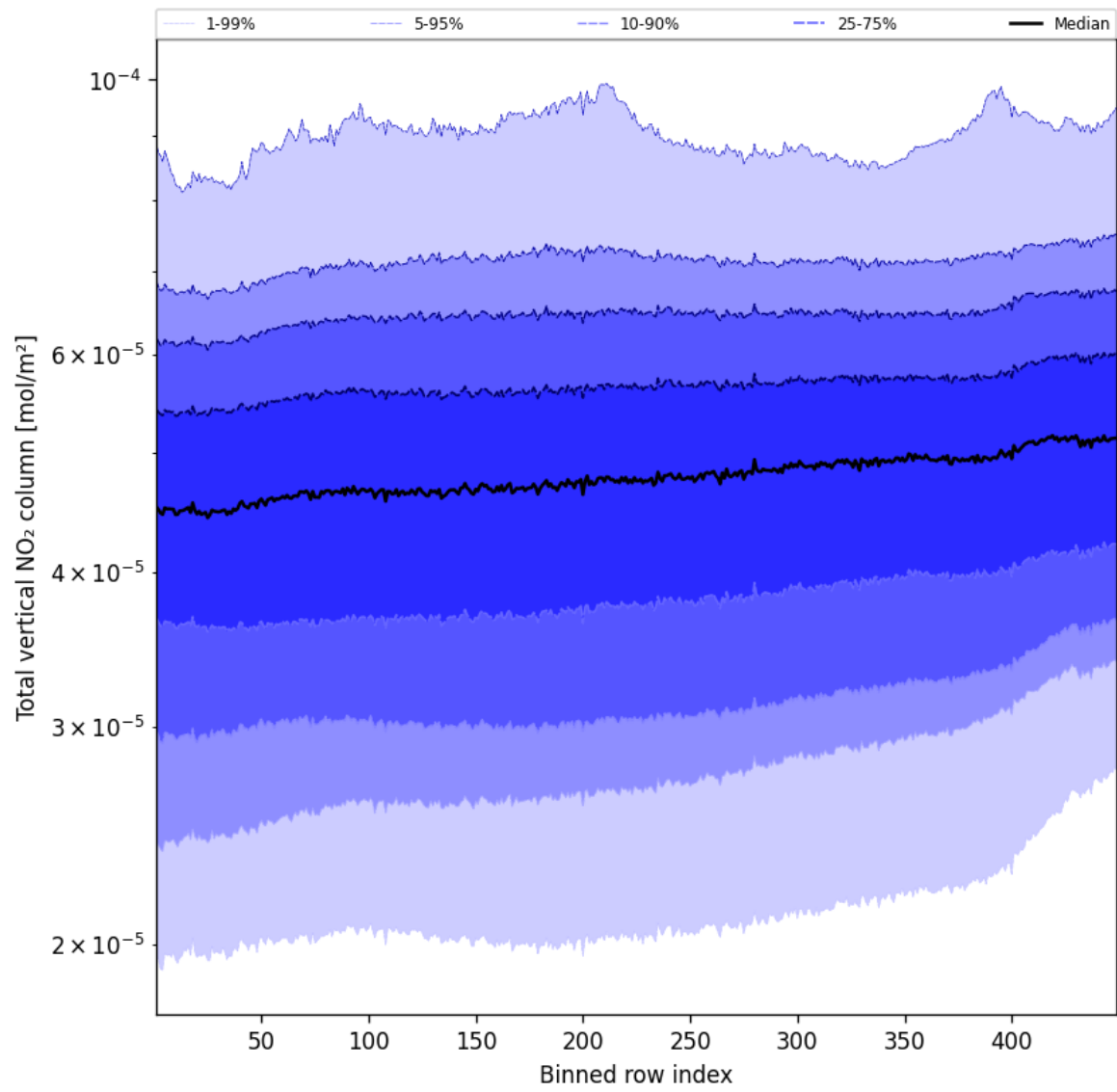
Figure 53: Along track statistics of “Total vertical NO 2 column” for 2025-09-28 to 2025-09-29
