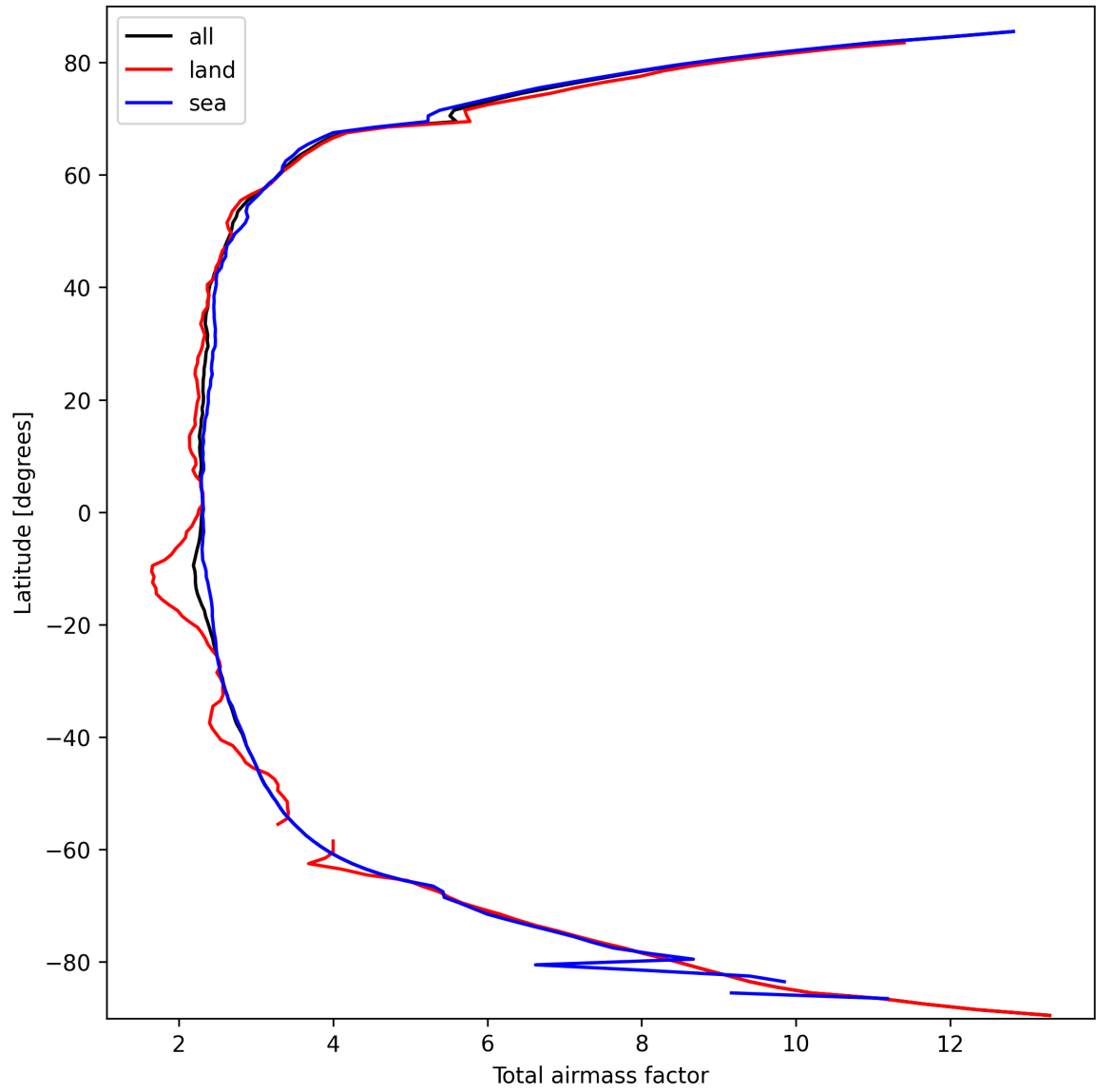
Figure 13: Zonal average of “Total airmass factor” for 2025-09-28 to 2025-09-29.
