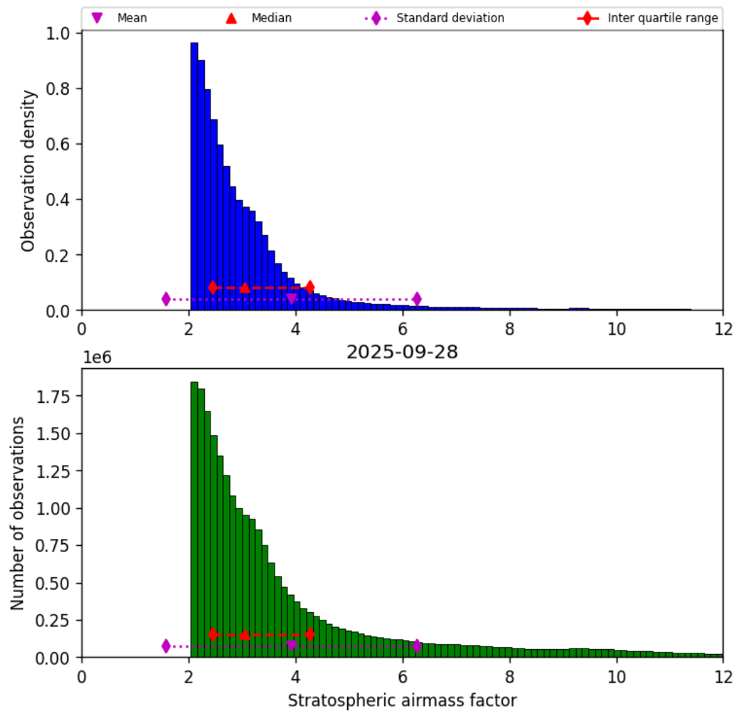
Figure 42: Histogram of “Stratospheric airmass factor” for 2025-09-28 to 2025-09-29
