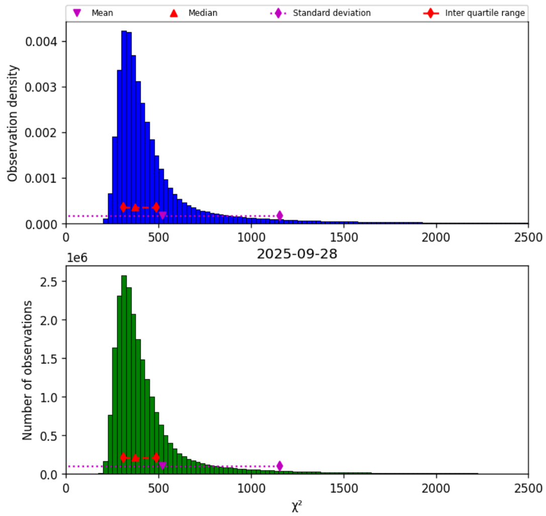
Figure 40: Histogram of “ \chi^2 ” for 2025-09-28 to 2025-09-29
