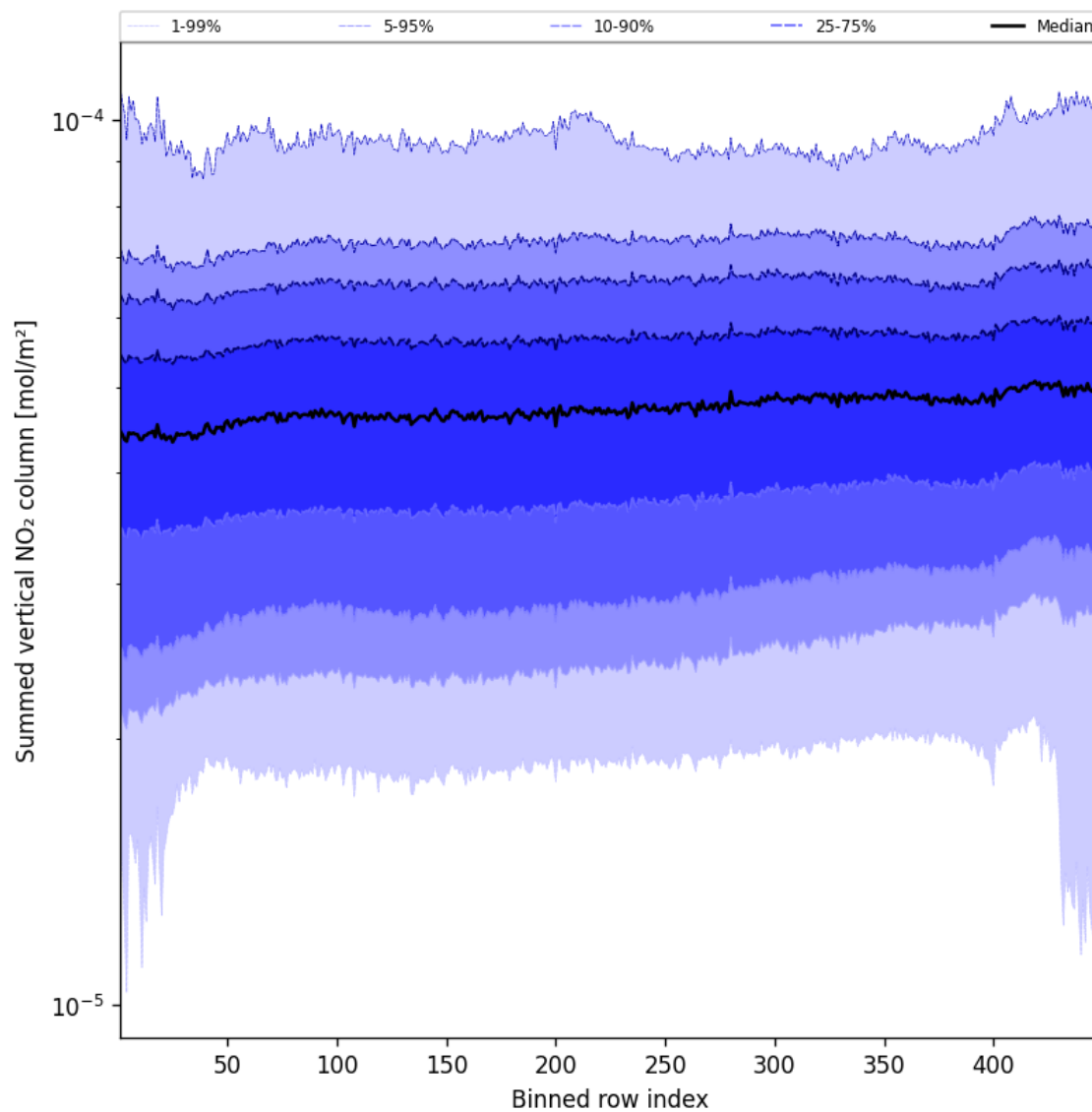
Figure 55: Along track statistics of “Summed vertical NO 2 column” for 2025-09-28 to 2025-09-29
