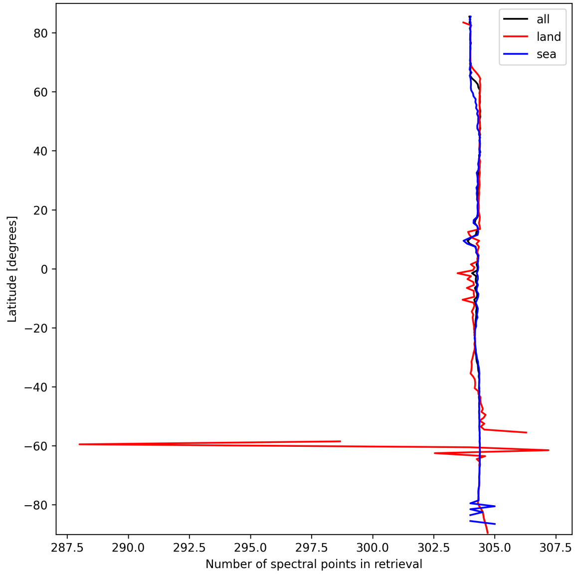
Figure 14: Zonal average of “Number of spectral points in retrieval” for 2025-09-28 to 2025-09-29.
