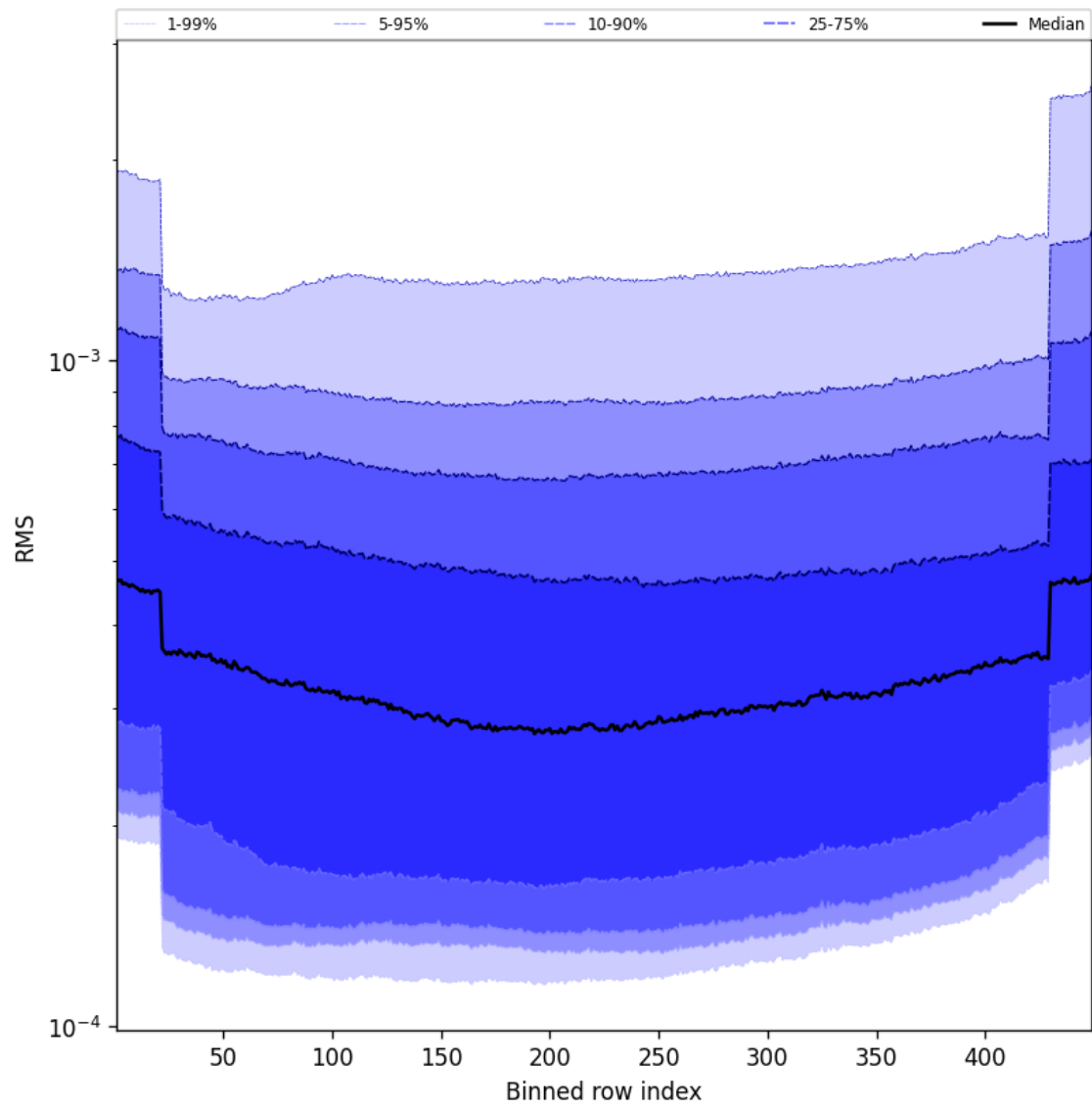
Figure 58: Along track statistics of “RMS” for 2025-09-28 to 2025-09-29
