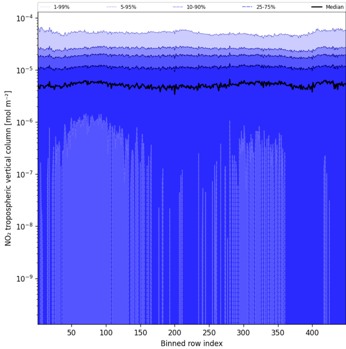
Figure 44: Along track statistics of “NO 2 tropospheric vertical column” for 2025-09-28 to 2025-09-29
