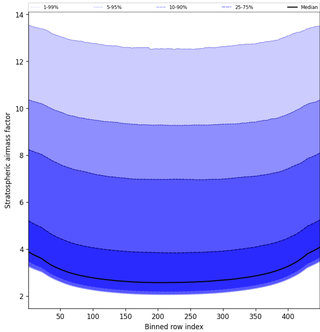
Figure 59: Along track statistics of “Stratospheric airmass factor” for 2025-09-28 to 2025-09-29
