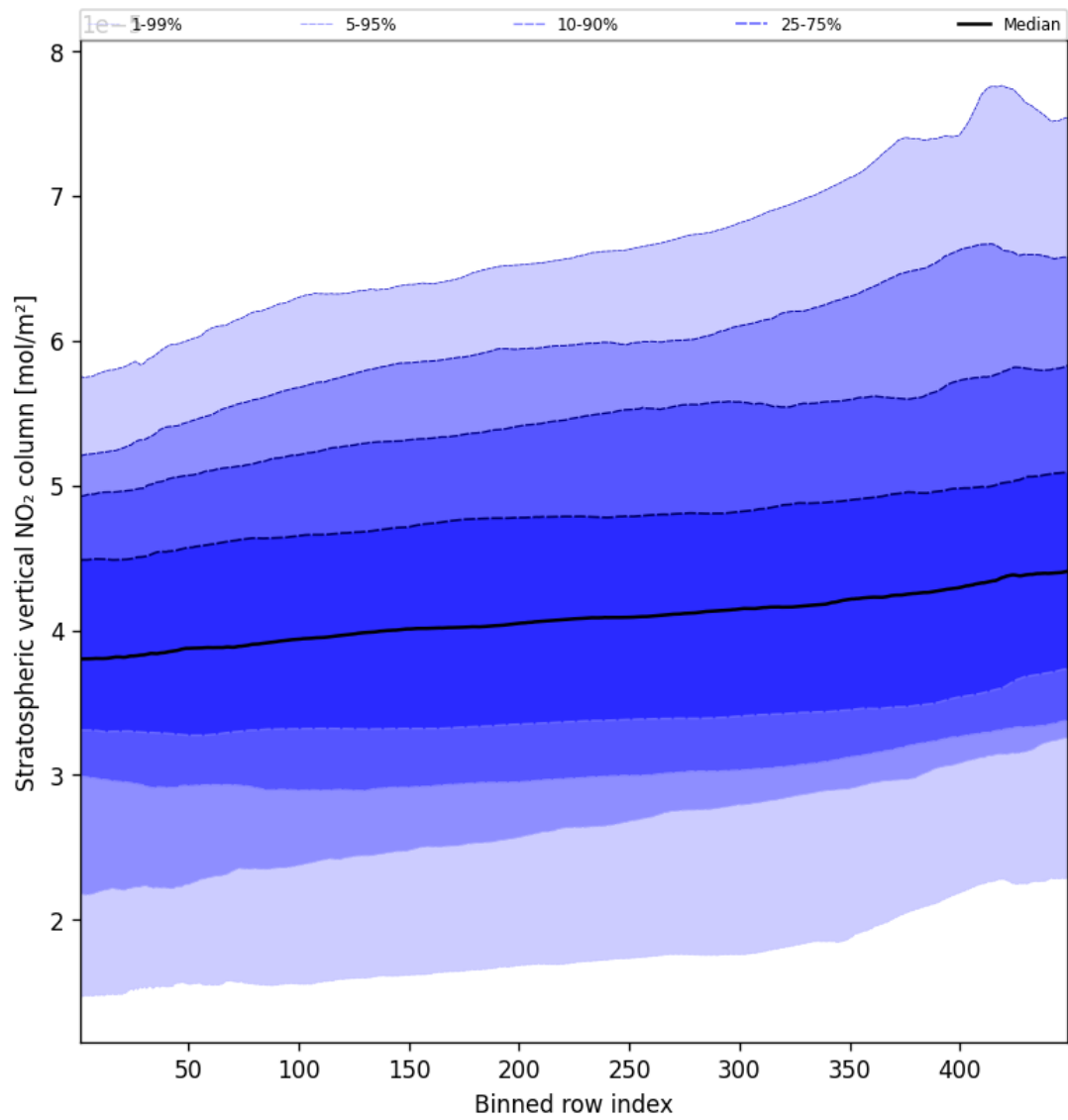
Figure 51: Along track statistics of “Stratospheric vertical NO 2 column” for 2025-09-28 to 2025-09-29
