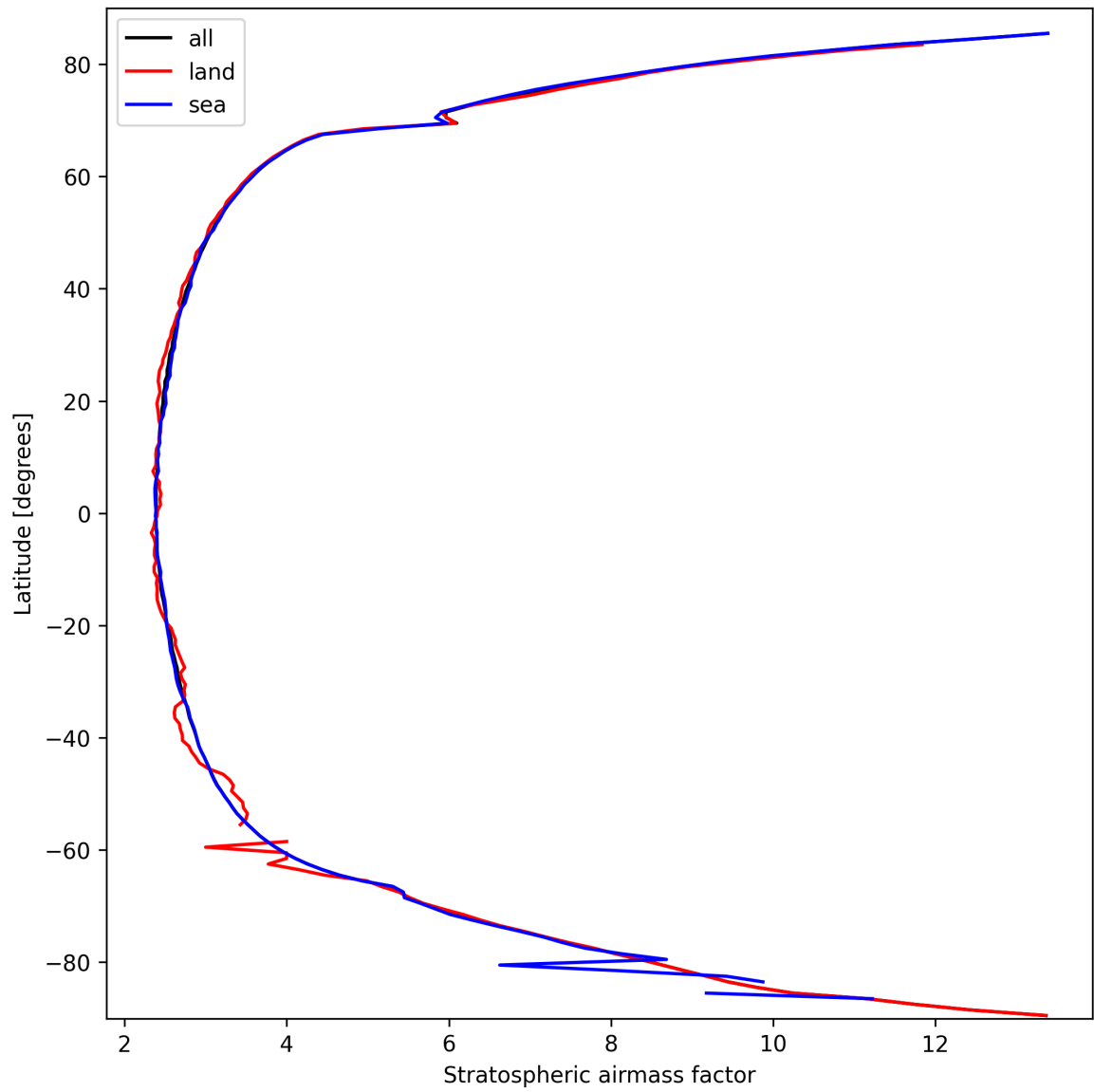
Figure 25: Zonal average of “Stratospheric airmass factor” for 2025-09-28 to 2025-09-29.
