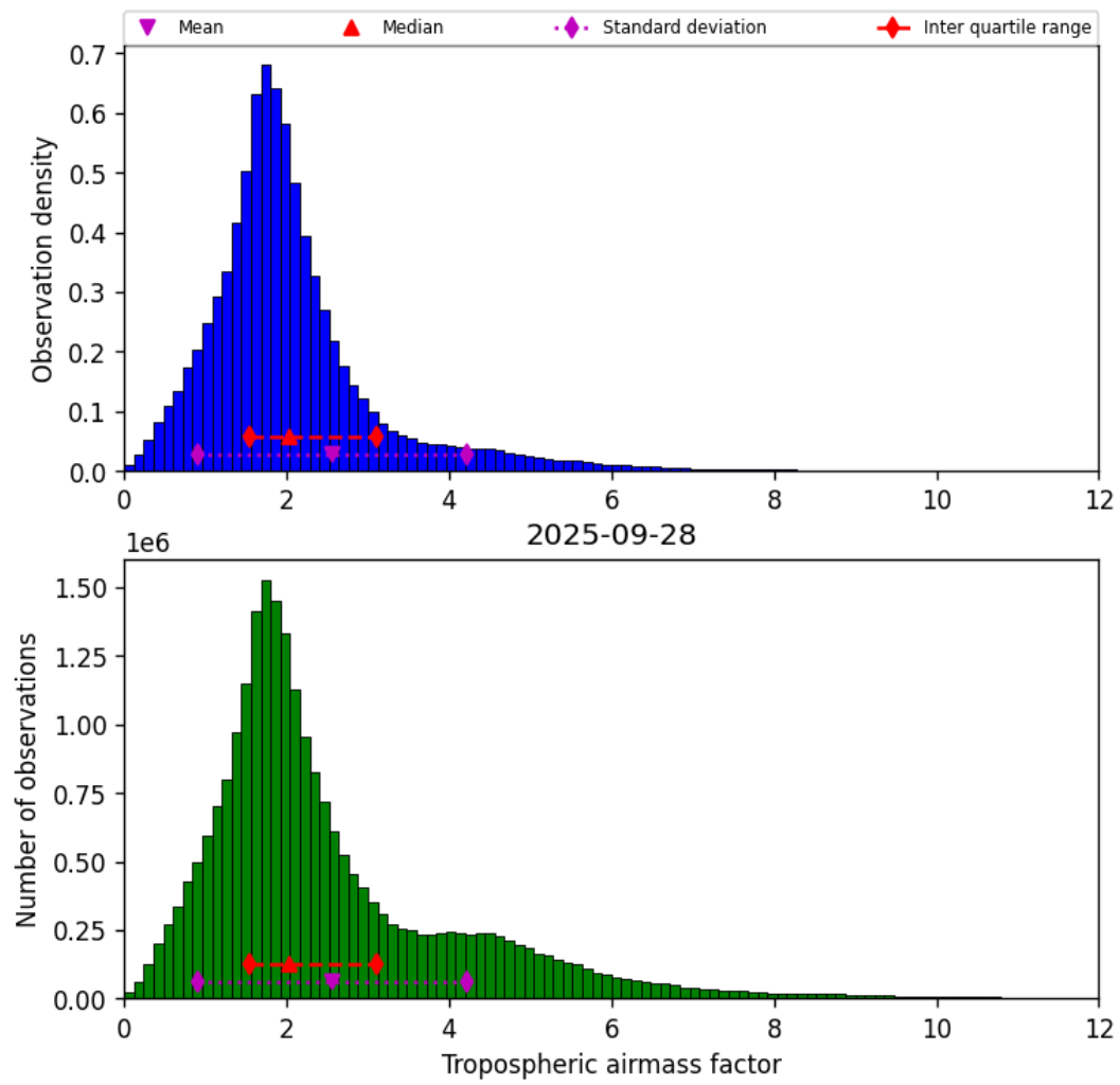
Figure 29: Histogram of “Tropospheric airmass factor” for 2025-09-28 to 2025-09-29
