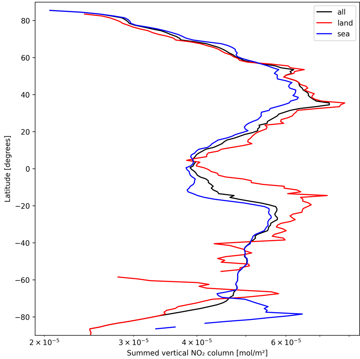
Figure 21: Zonal average of “Summed vertical NO 2 column” for 2025-09-28 to 2025-09-29.
