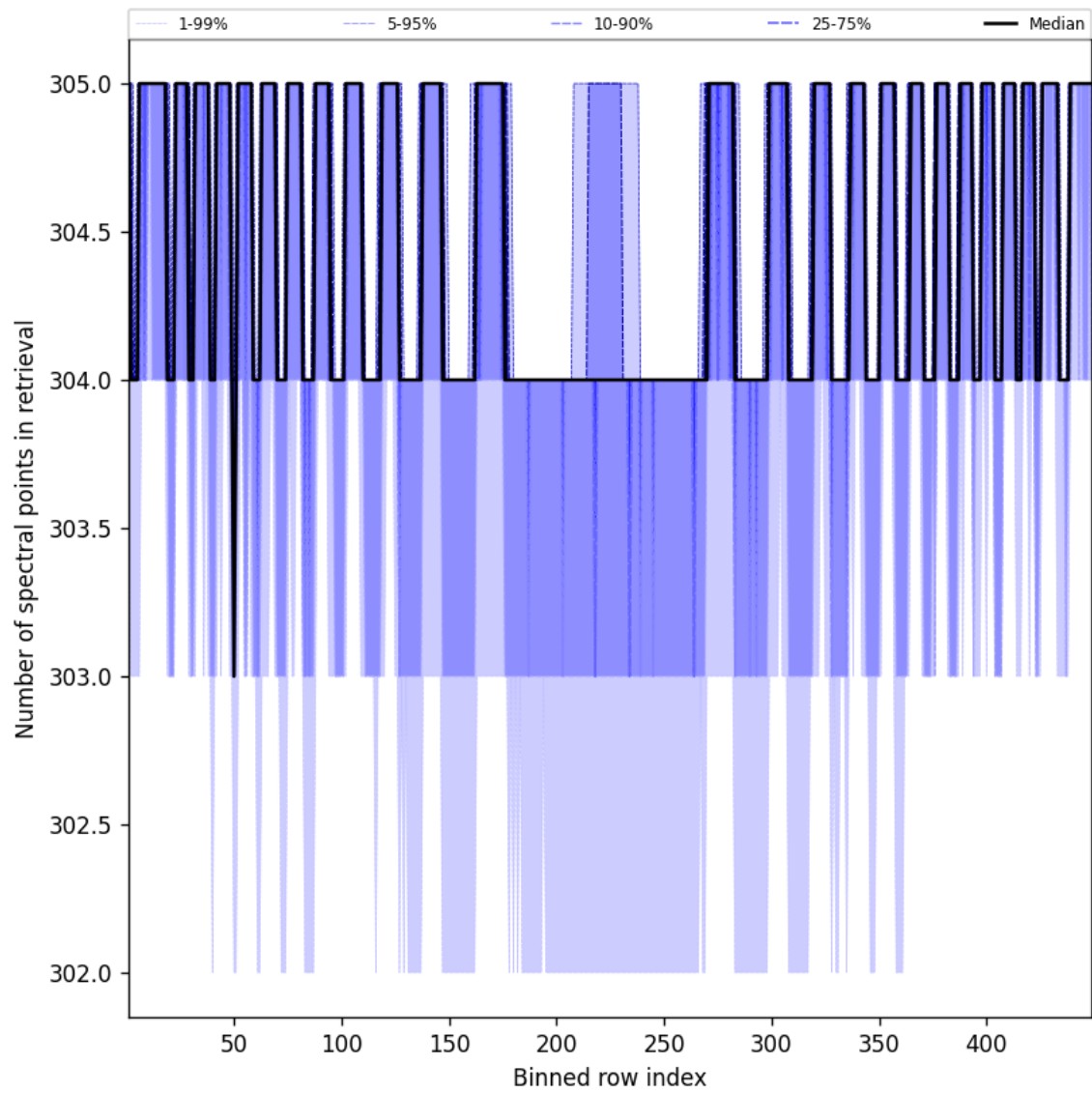
Figure 48: Along track statistics of “Number of spectral points in retrieval” for 2025-09-28 to 2025-09-29
