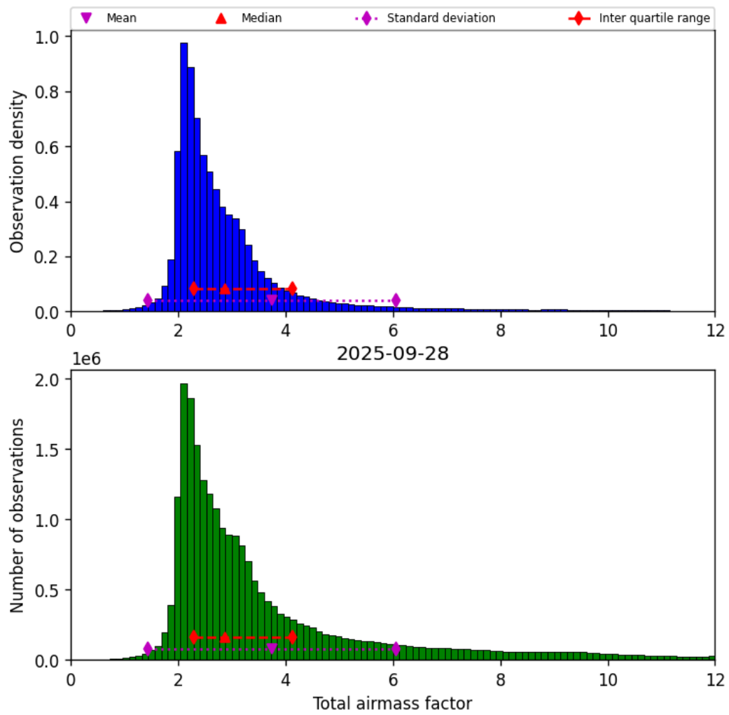
Figure 30: Histogram of “Total airmass factor” for 2025-09-28 to 2025-09-29
