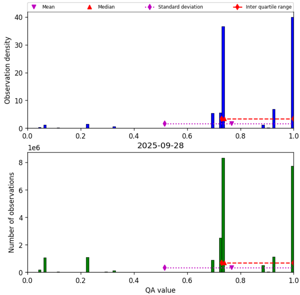
Figure 26: Histogram of “QA value” for 2025-09-28 to 2025-09-29
