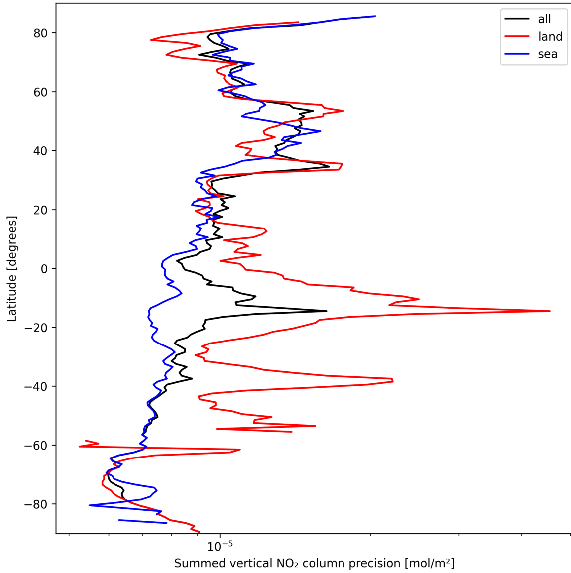
Figure 22: Zonal average of “Summed vertical NO 2 column precision” for 2025-09-28 to 2025-09-29.
