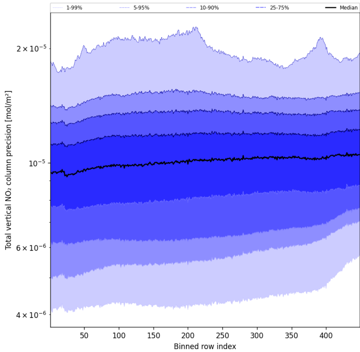
Figure 54: Along track statistics of “Total vertical NO 2 column precision” for 2025-09-28 to 2025-09-29
