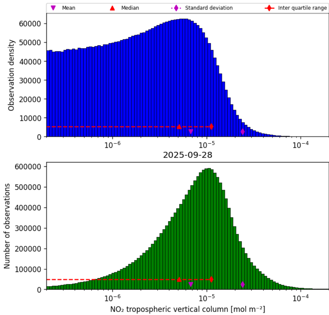
Figure 27: Histogram of “NO 2 tropospheric vertical column” for 2025-09-28 to 2025-09-29
