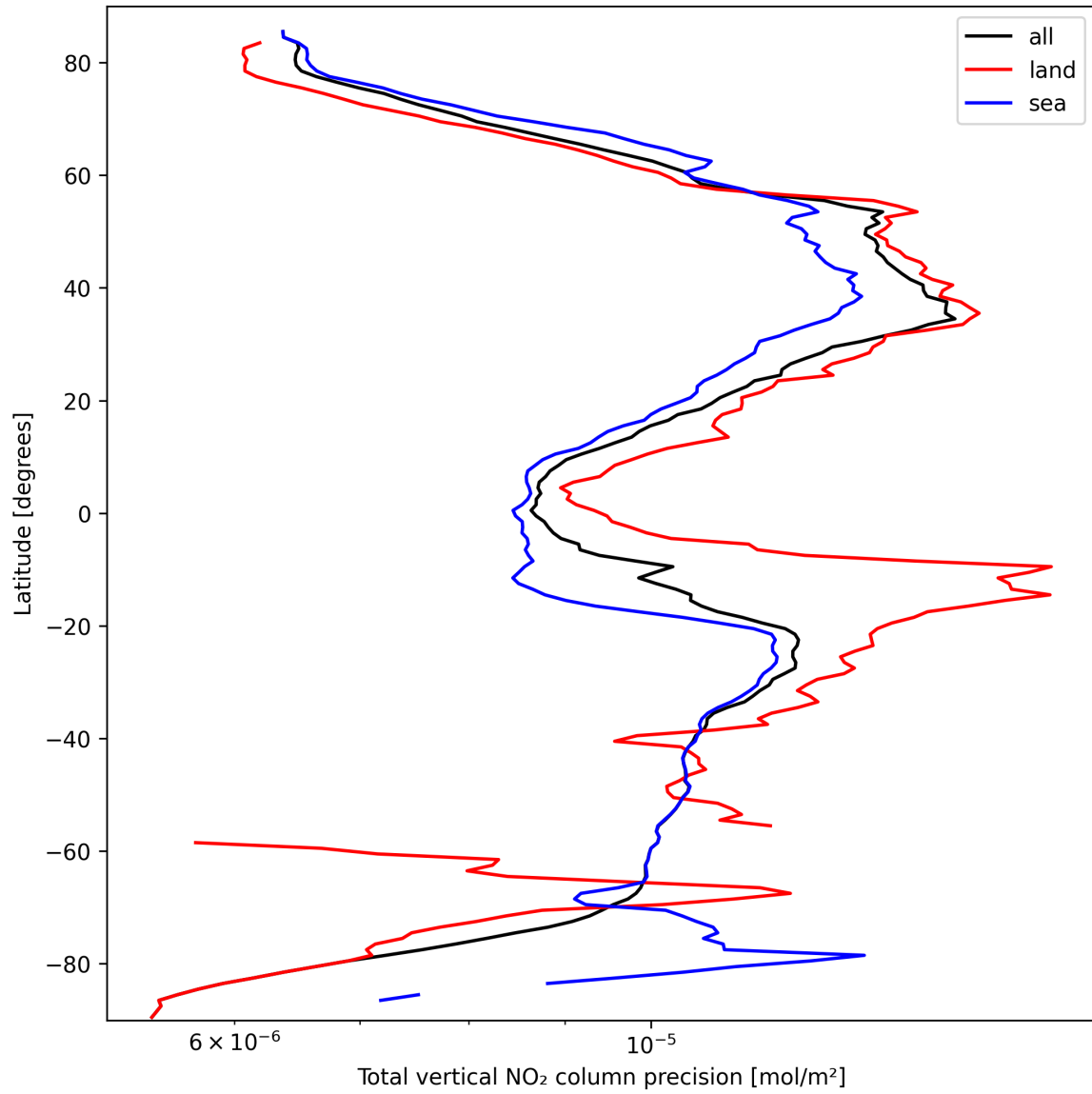
Figure 20: Zonal average of “Total vertical NO 2 column precision” for 2025-09-28 to 2025-09-29.
