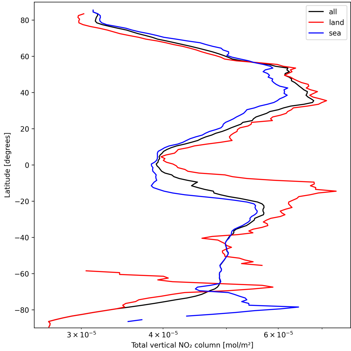
Figure 19: Zonal average of “Total vertical NO 2 column” for 2025-09-28 to 2025-09-29.
