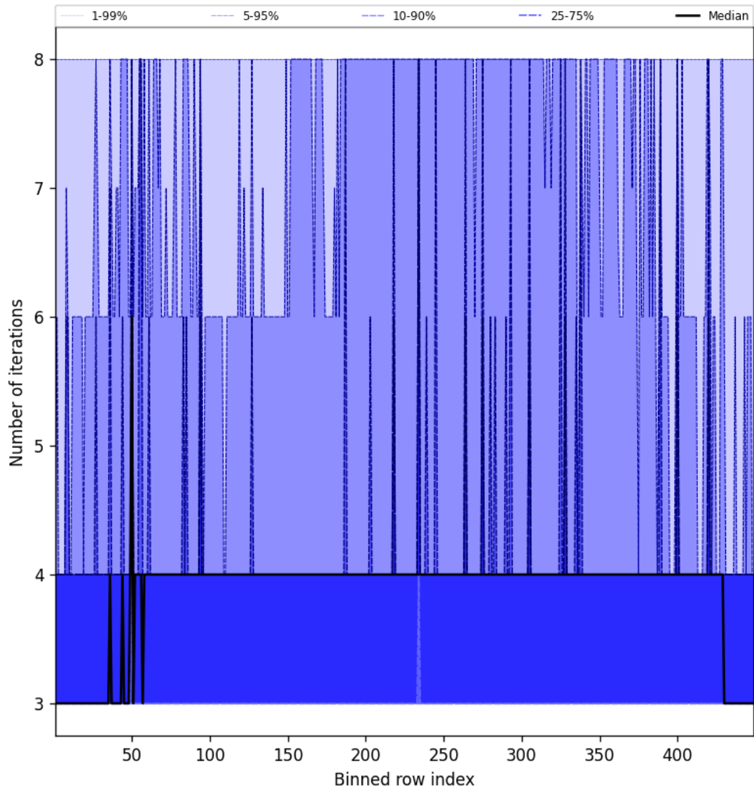
Figure 49: Along track statistics of “Number of iterations” for 2025-09-28 to 2025-09-29
