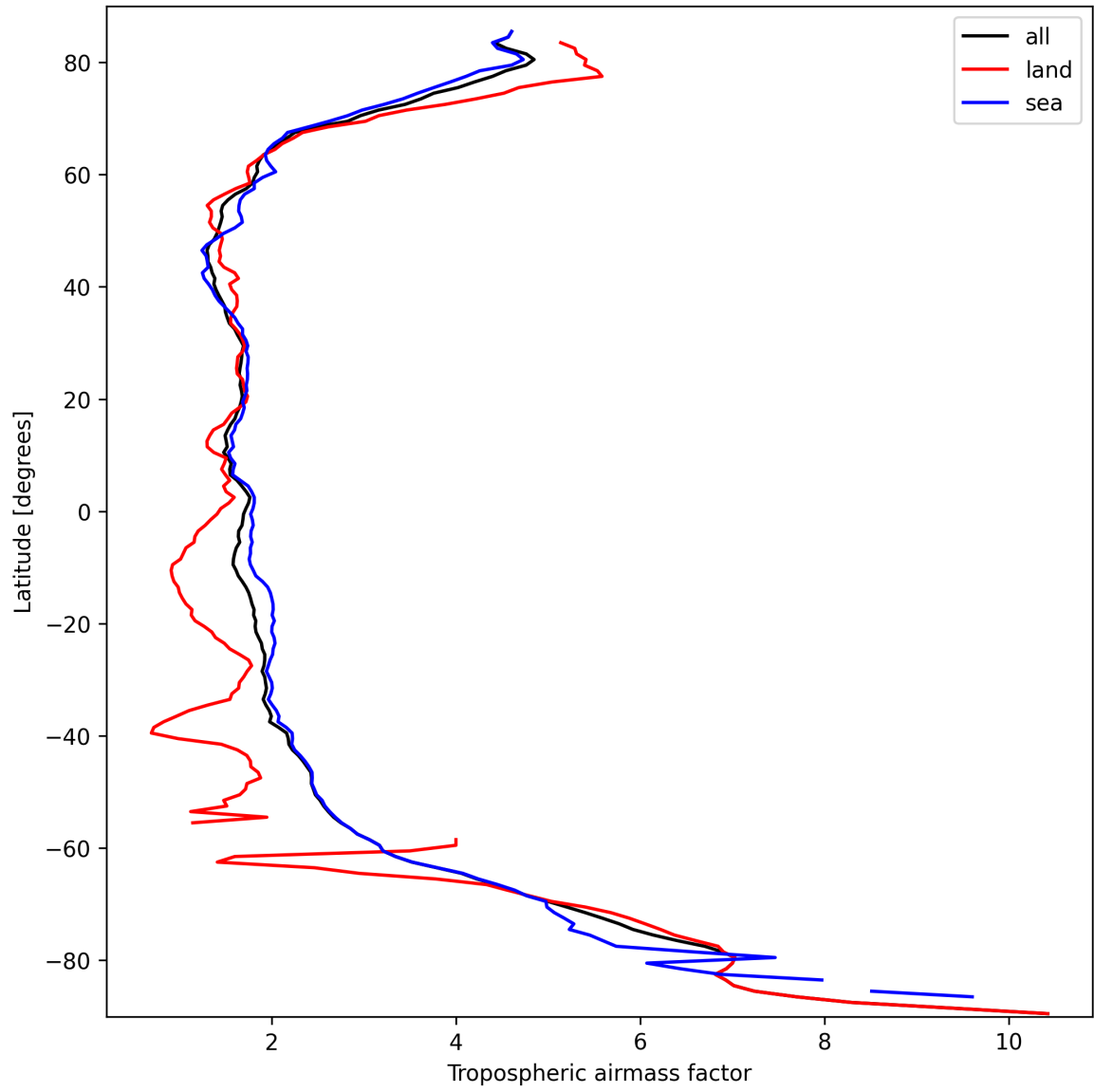
Figure 12: Zonal average of “Tropospheric air mass factor” for 2025-09-28 to 2025-09-29.
