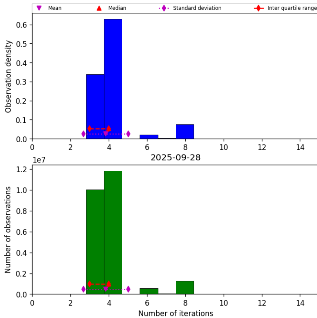
Figure 32: Histogram of “Number of iterations” for 2025-09-28 to 2025-09-29
