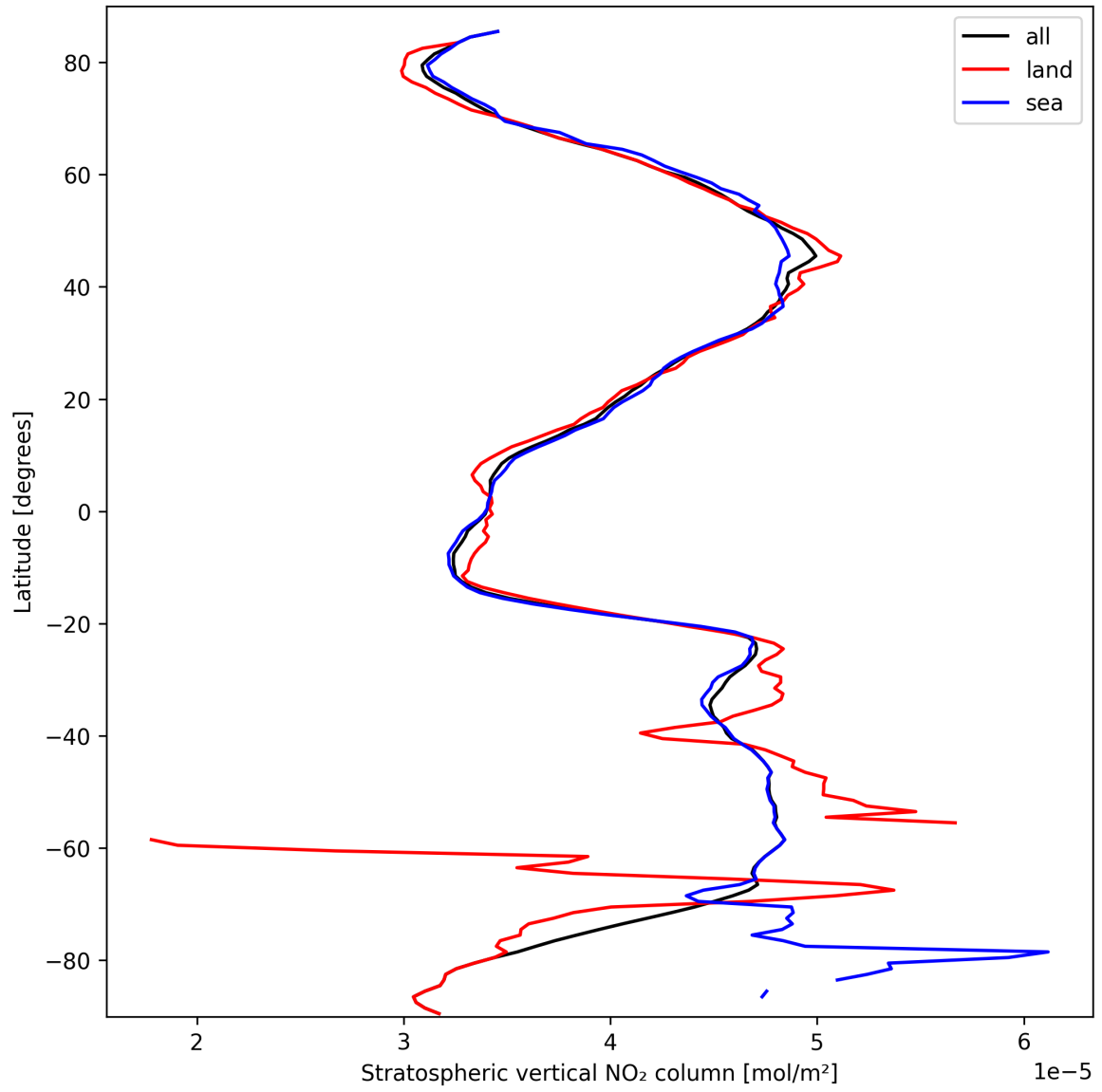
Figure 17: Zonal average of “Stratospheric vertical NO 2 column” for 2025-09-28 to 2025-09-29.
