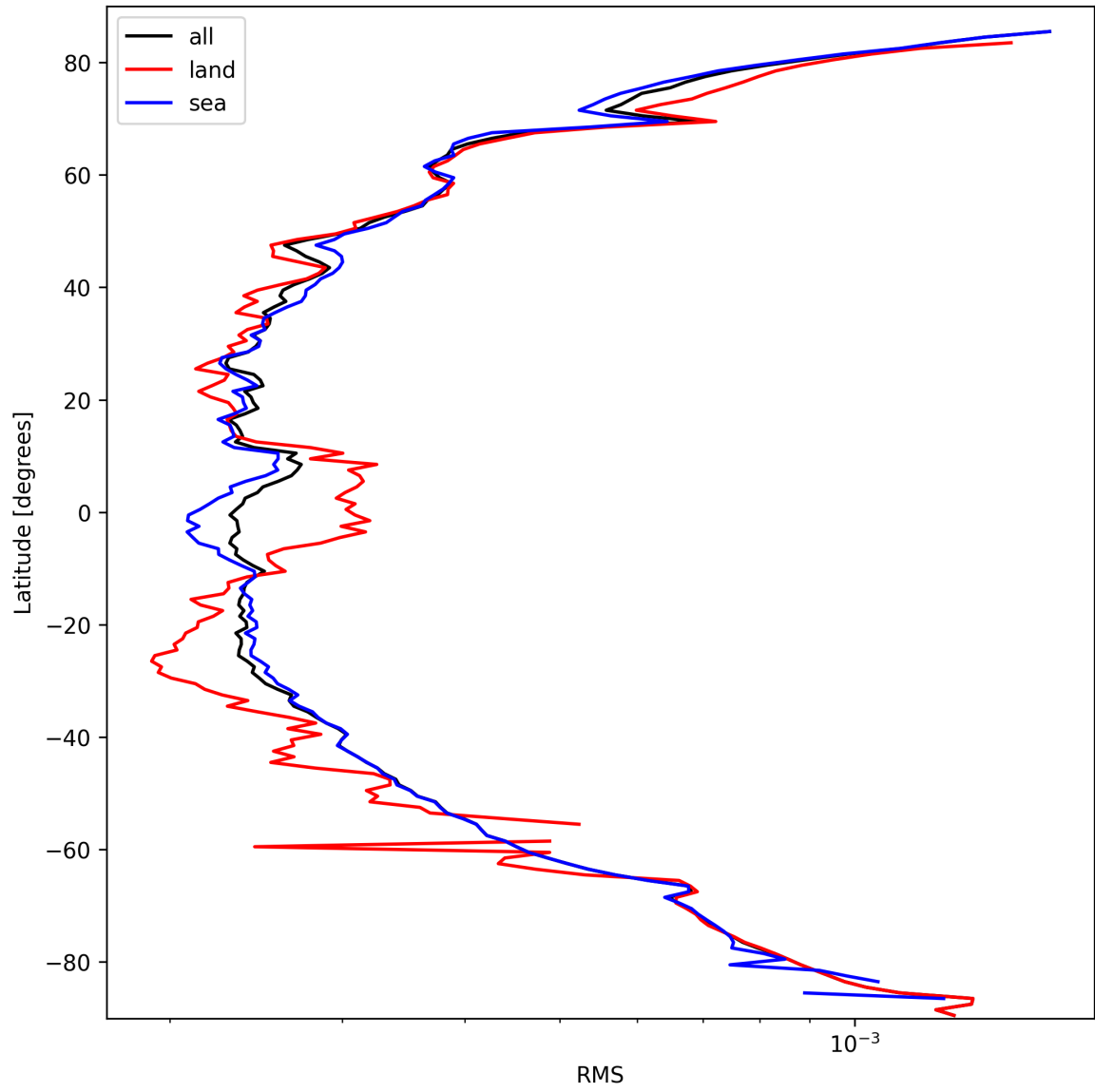
Figure 24: Zonal average of “RMS” for 2025-09-28 to 2025-09-29.
