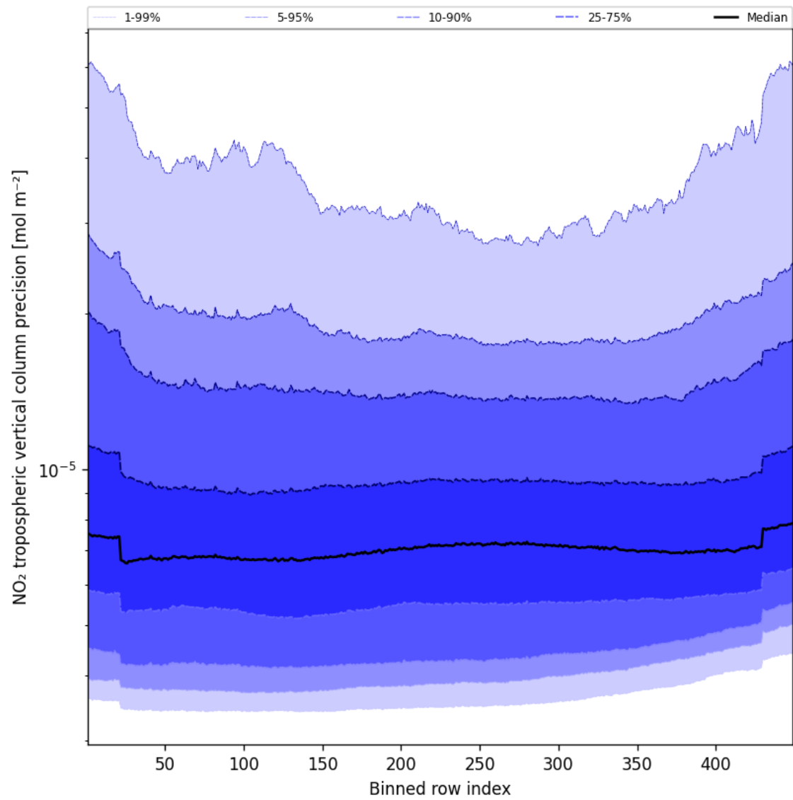
Figure 45: Along track statistics of “NO 2 tropospheric vertical column precision” for 2025-09-28 to 2025-09-29
