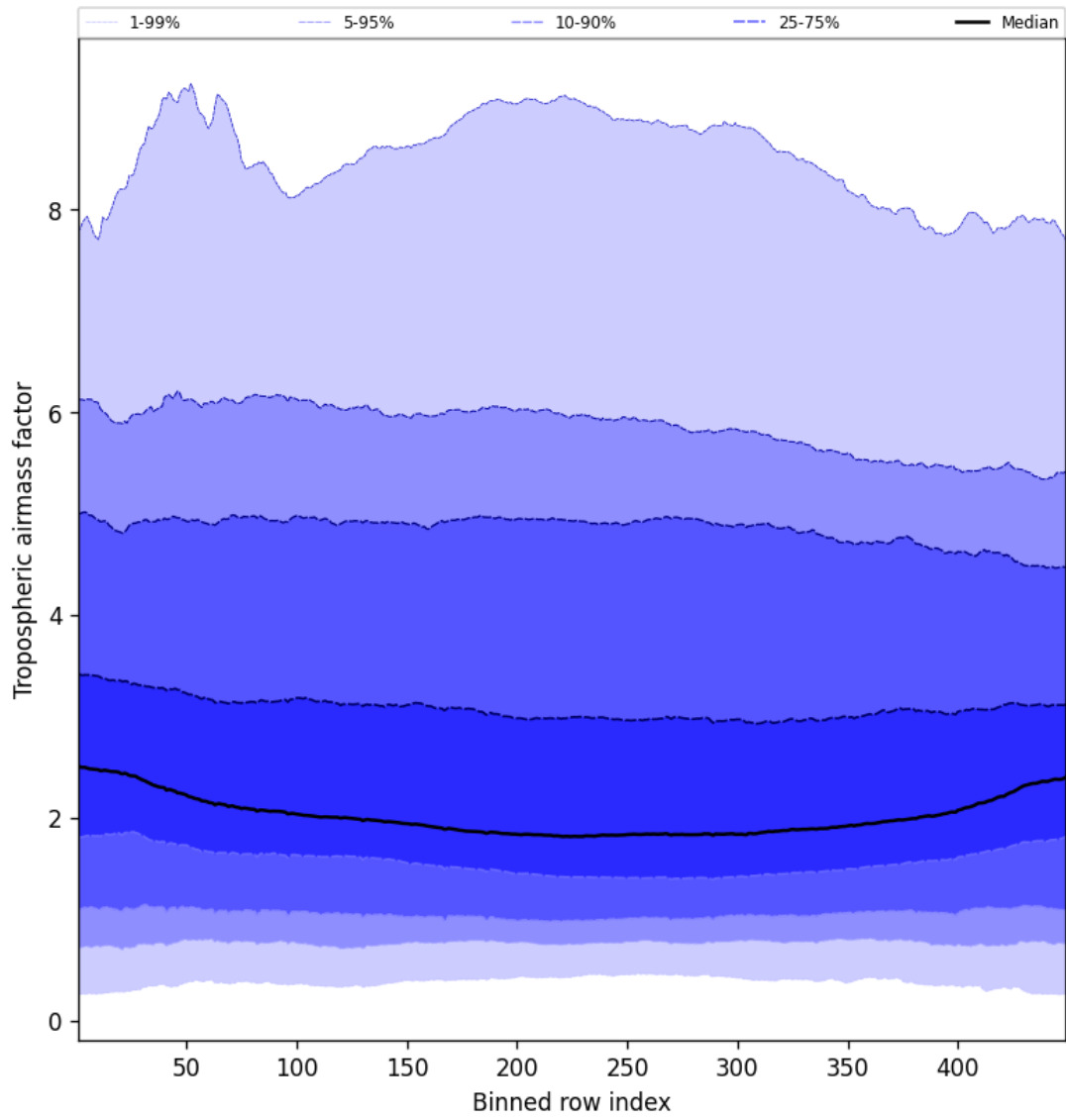
Figure 46: Along track statistics of “Tropospheric air mass factor” for 2025-09-28 to 2025-09-29
