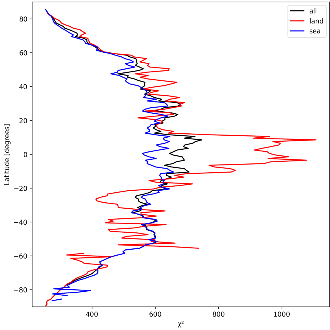
Figure 23: Zonal average of “ \chi^2 ” for 2025-09-28 to 2025-09-29.
