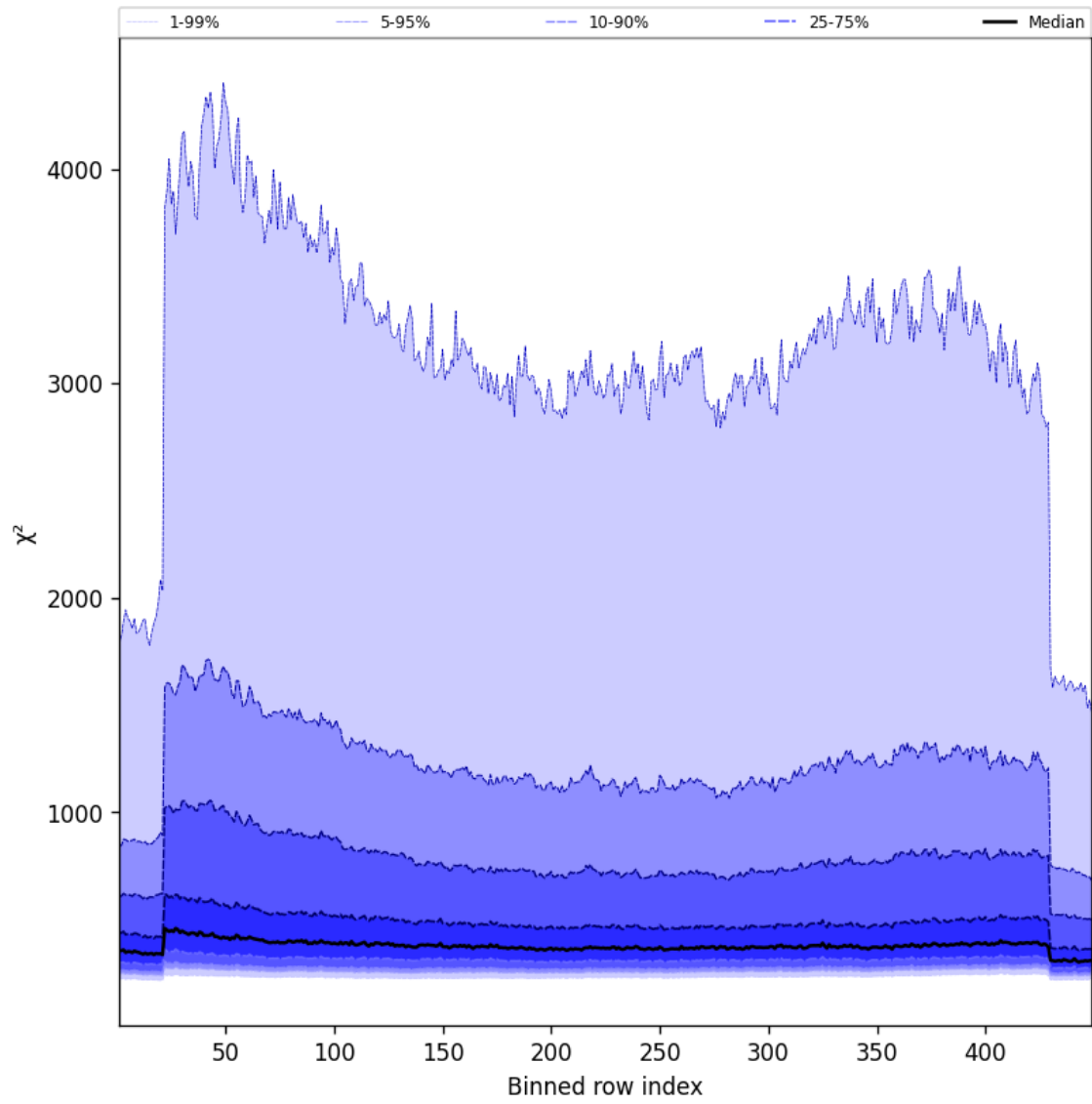
Figure 57: Along track statistics of “ \chi^2 ” for 2025-09-28 to 2025-09-29
