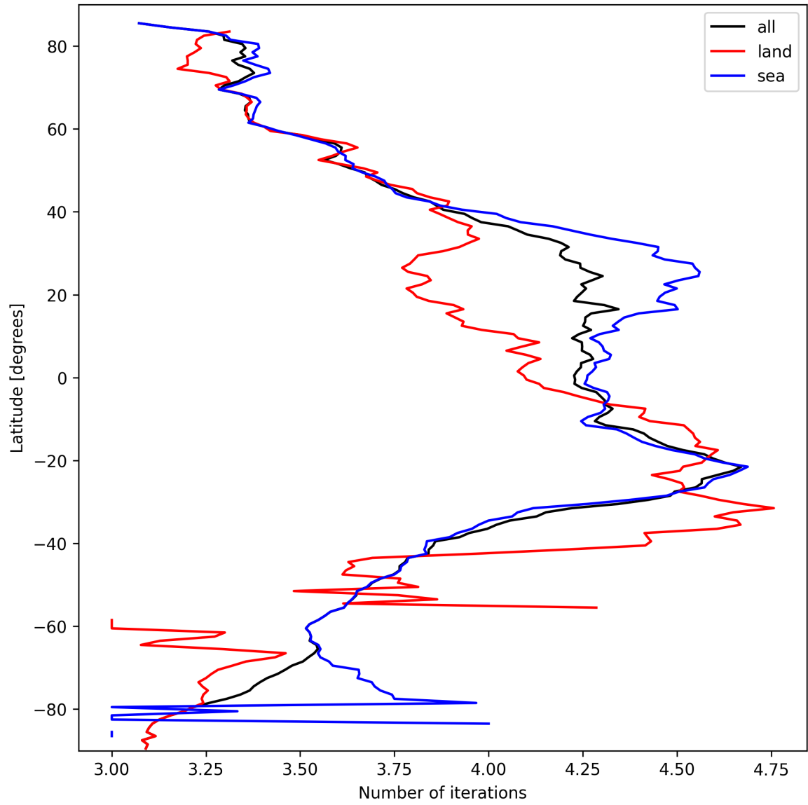
Figure 15: Zonal average of “Number of iterations” for 2025-09-28 to 2025-09-29.
