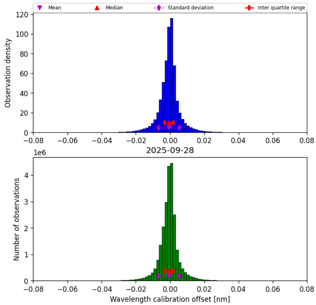
Figure 33: Histogram of “Wavelength calibration offset” for 2025-09-28 to 2025-09-29
