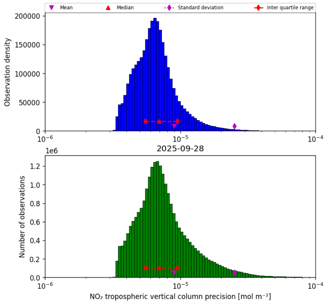
Figure 28: Histogram of “NO 2 tropospheric vertical column precision” for 2025-09-28 to 2025-09-29
