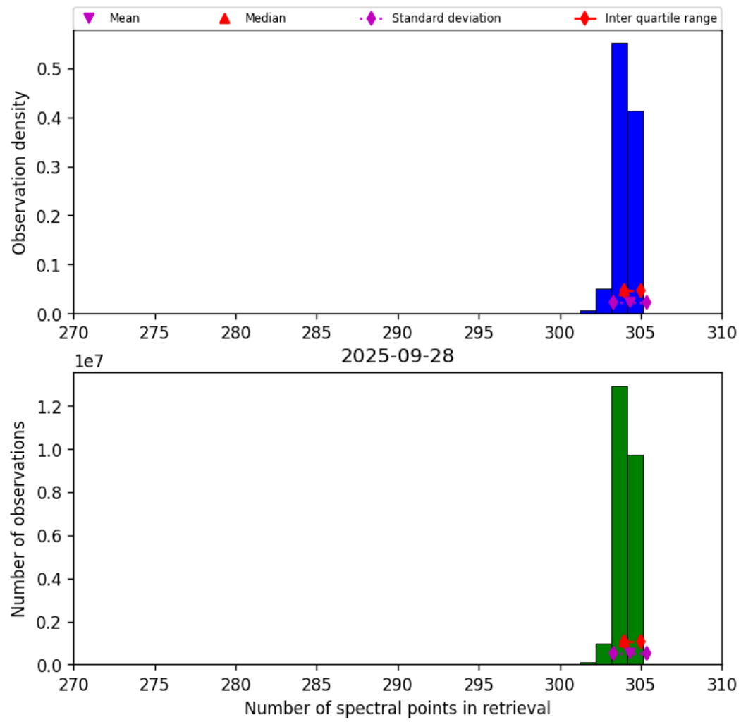
Figure 31: Histogram of “Number of spectral points in retrieval” for 2025-09-28 to 2025-09-29
