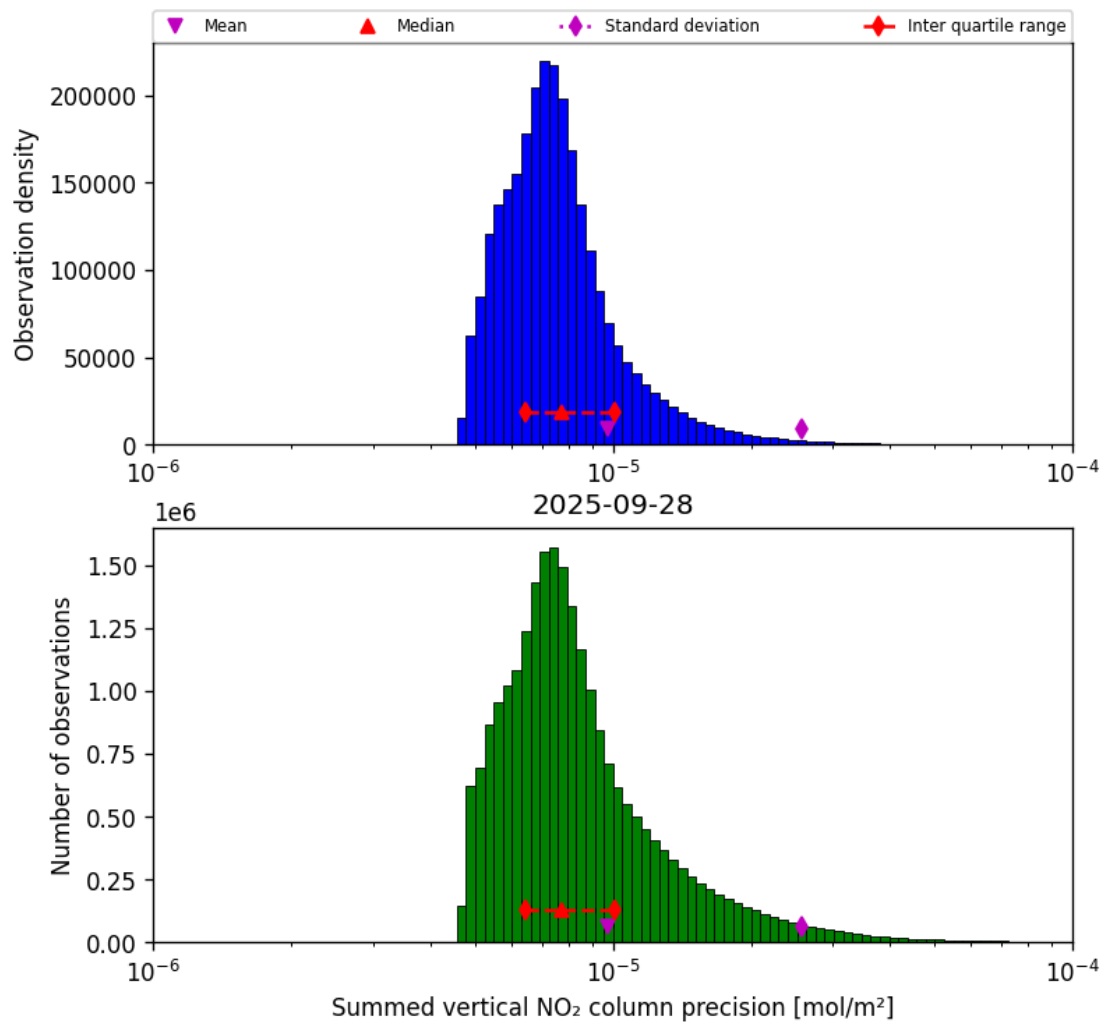
Figure 39: Histogram of “Summed vertical NO 2 column precision” for 2025-09-28 to 2025-09-29
