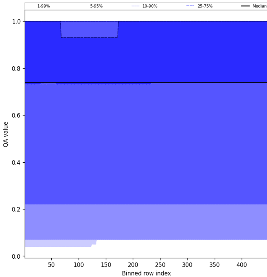
Figure 43: Along track statistics of “QA value” for 2025-09-28 to 2025-09-29
