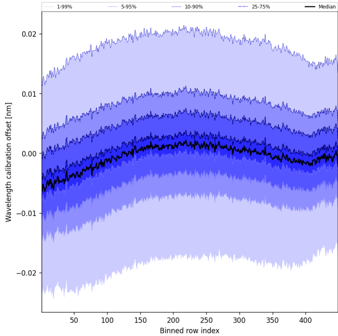
Figure 50: Along track statistics of “Wavelength calibration offset” for 2025-09-28 to 2025-09-29
