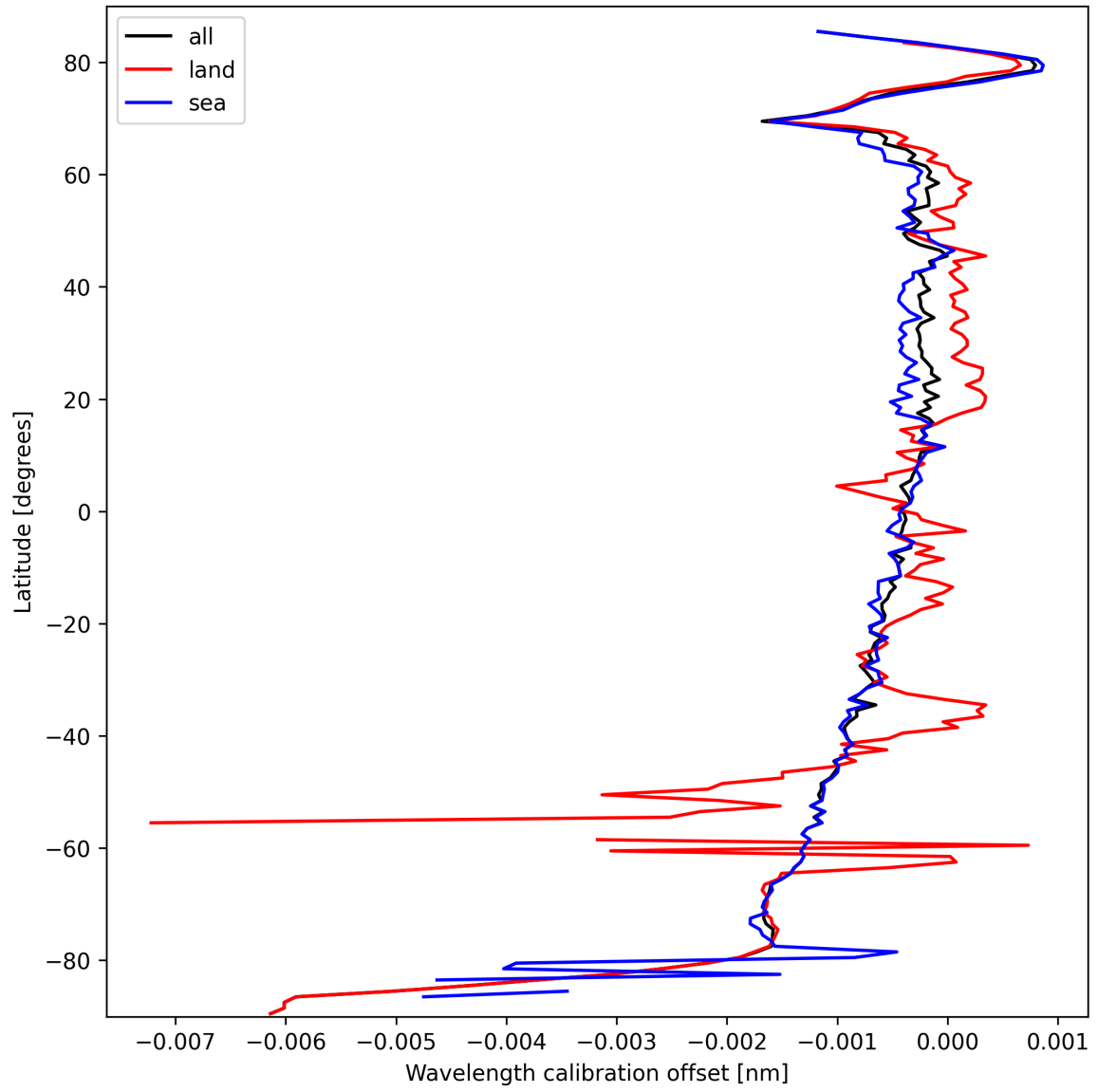
Figure 16: Zonal average of “Wavelength calibration offset” for 2025-09-28 to 2025-09-29.
