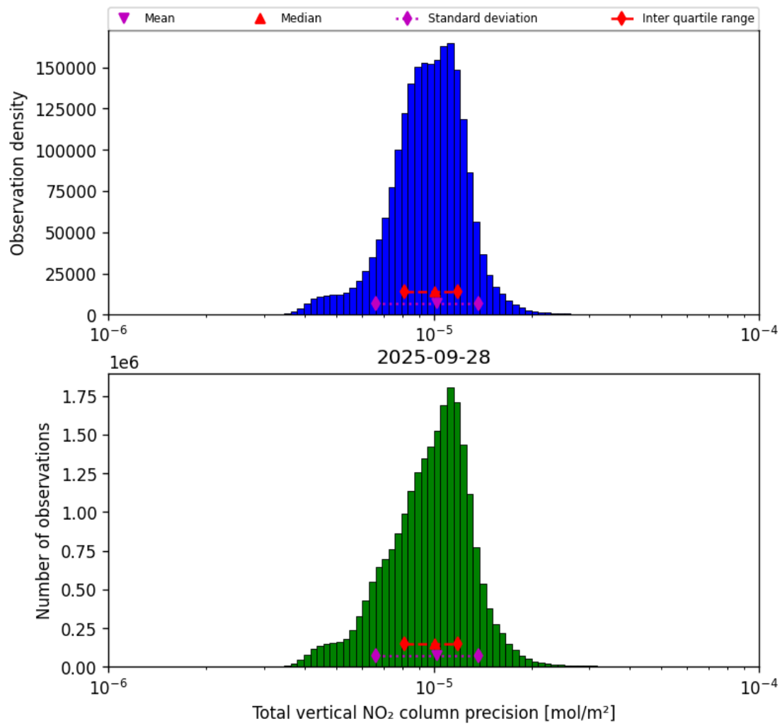
Figure 37: Histogram of “Total vertical NO 2 column precision” for 2025-09-28 to 2025-09-29
