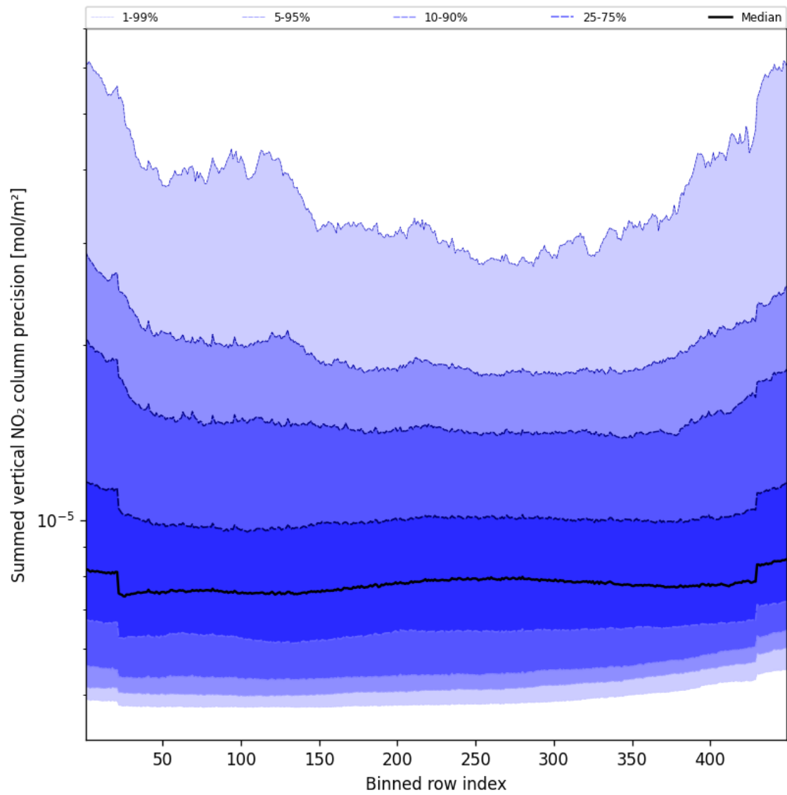
Figure 56: Along track statistics of “Summed vertical NO 2 column precision” for 2025-09-28 to 2025-09-29
