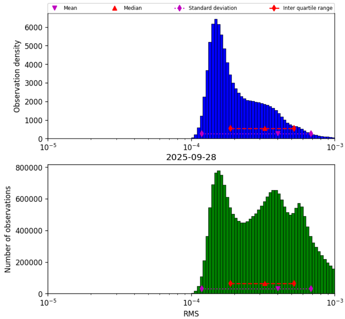
Figure 41: Histogram of “RMS” for 2025-09-28 to 2025-09-29
