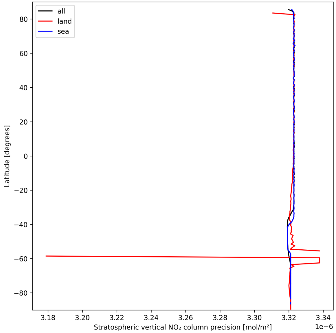
Figure 18: Zonal average of “Stratospheric vertical NO 2 column precision” for 2025-09-28 to 2025-09-29.
