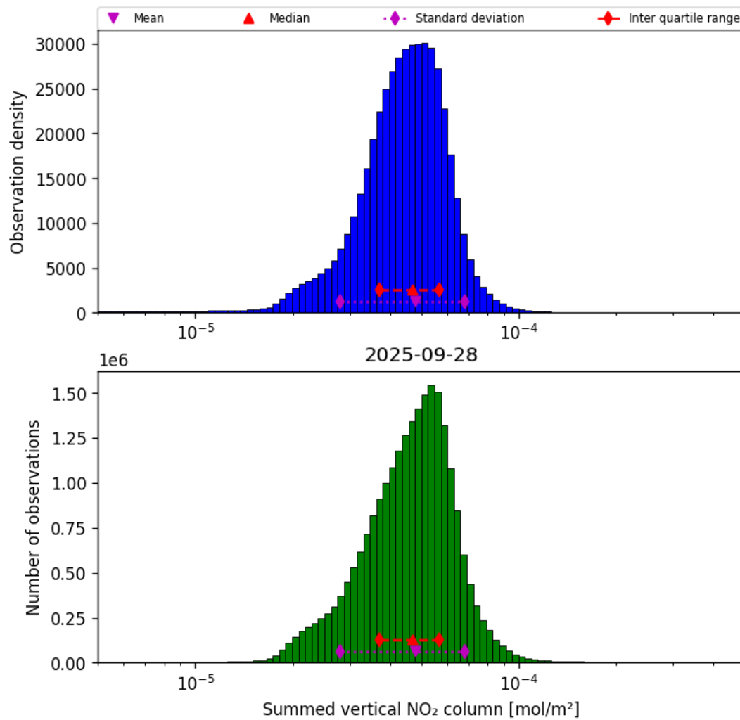
Figure 38: Histogram of “Summed vertical NO 2 column” for 2025-09-28 to 2025-09-29
