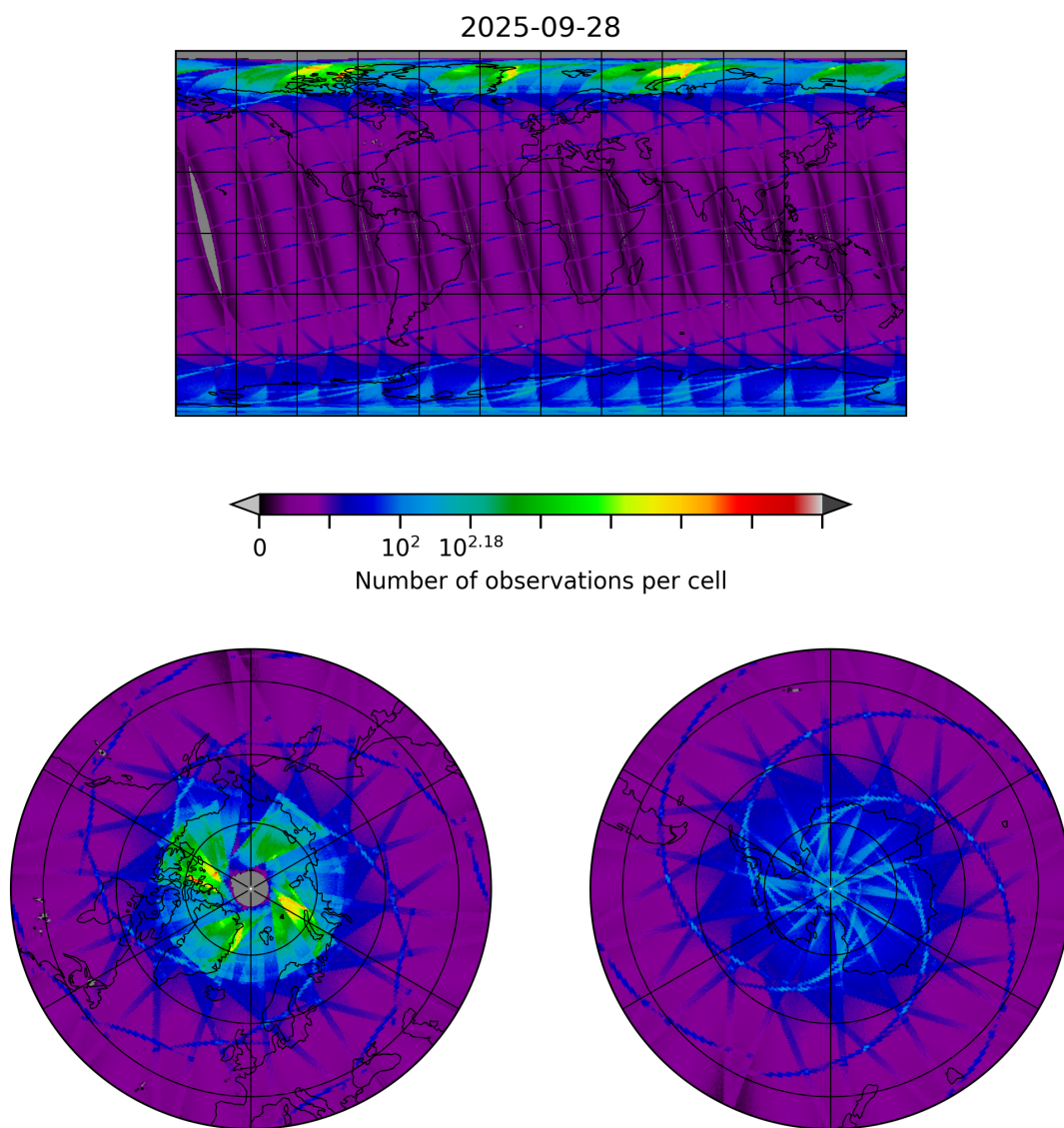
Figure 8: Map of the number of observations for 2025-09-28 to 2025-09-29
