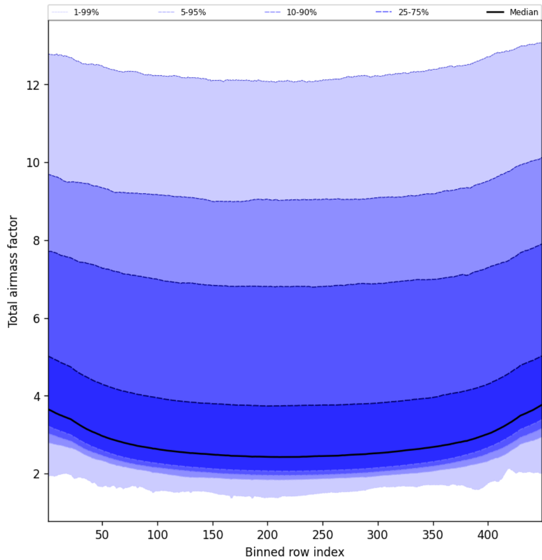
Figure 47: Along track statistics of “Total airmass factor” for 2025-09-28 to 2025-09-29
