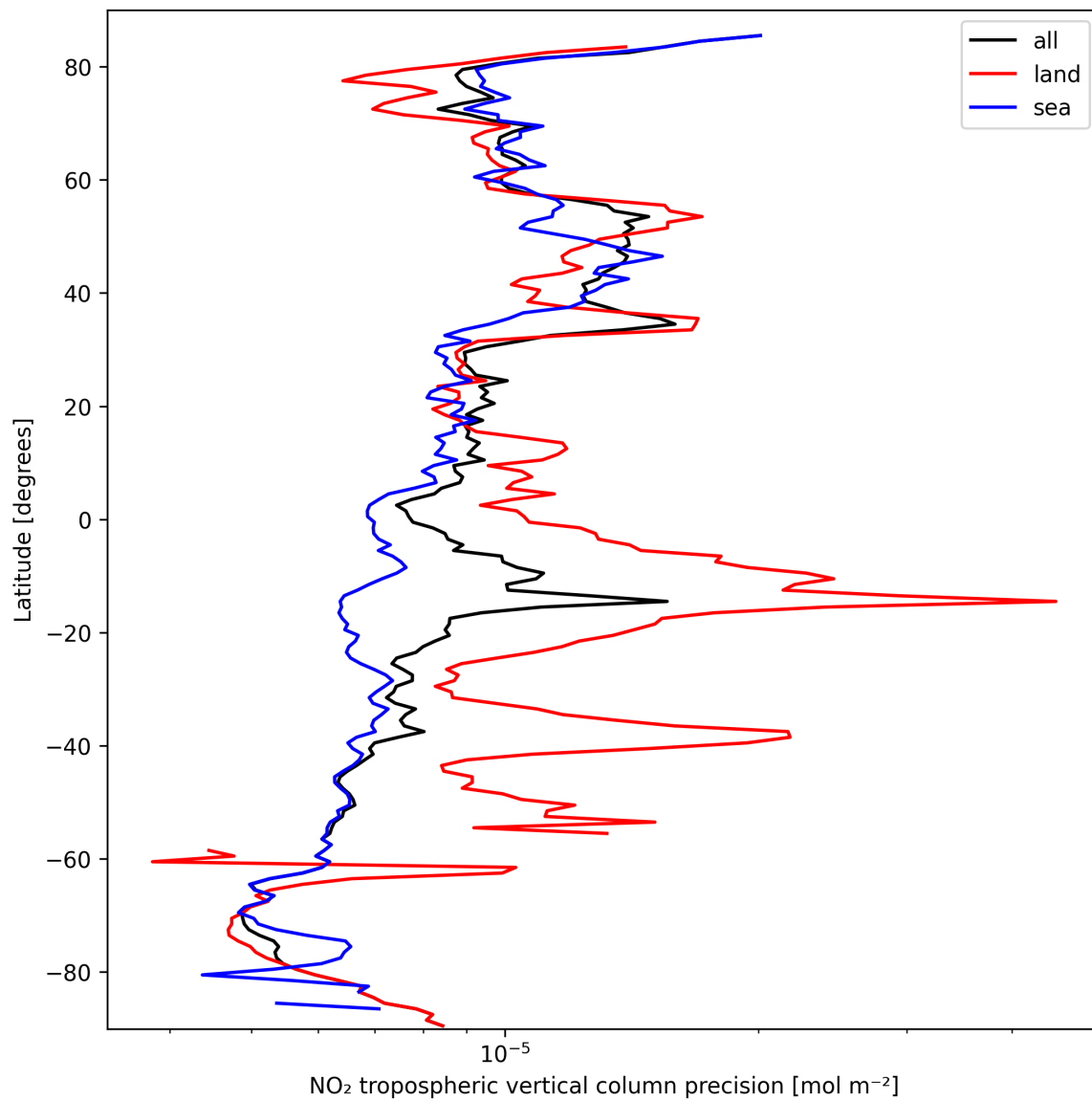
Figure 11: Zonal average of “NO 2 tropospheric vertical column precision” for 2025-09-28 to 2025-09-29.
