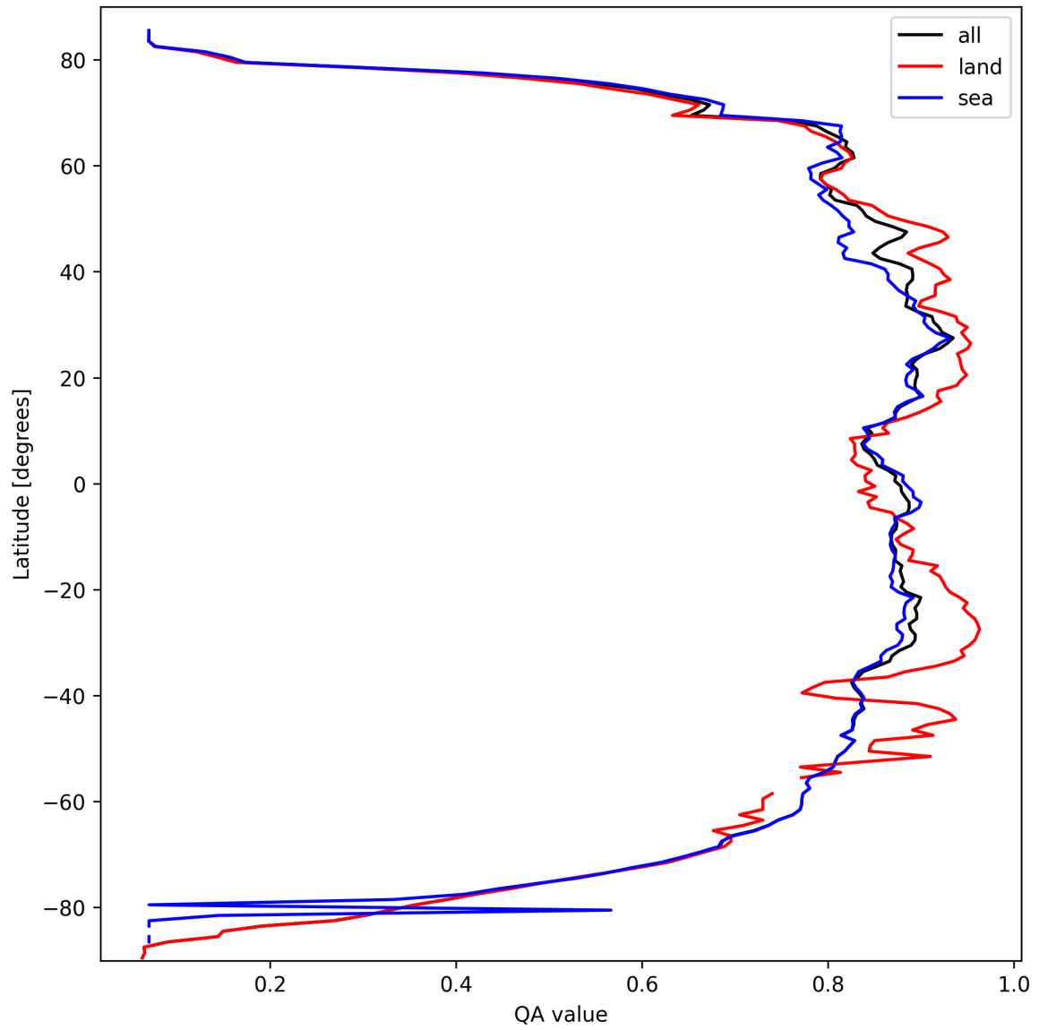
Figure 9: Zonal average of “QA value” for 2025-09-28 to 2025-09-29.
