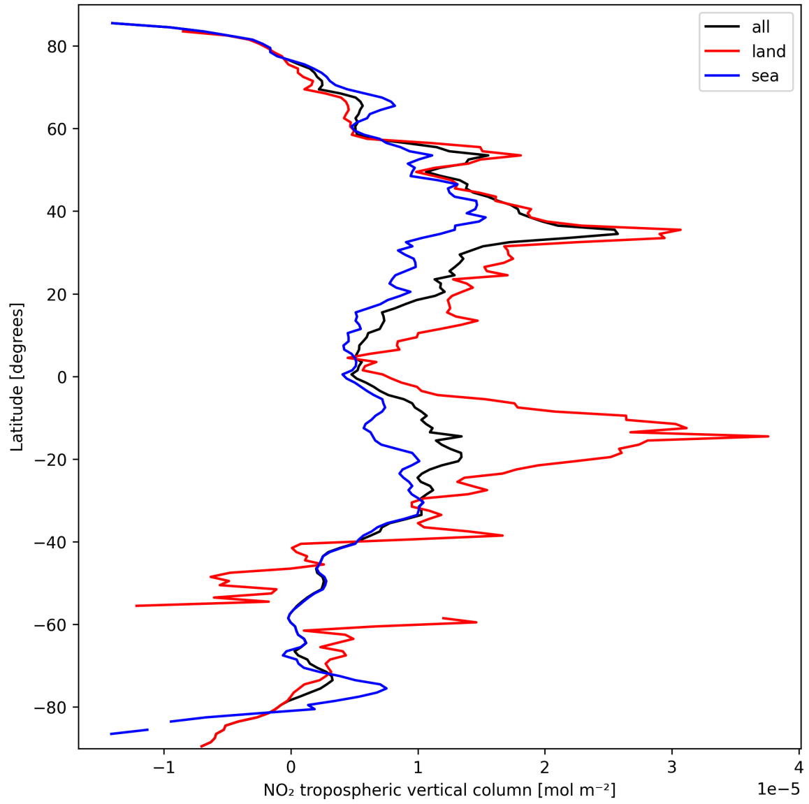
Figure 10: Zonal average of “NO 2 tropospheric vertical column” for 2025-09-28 to 2025-09-29.
