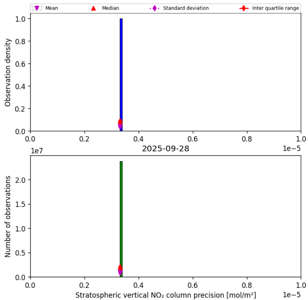
Figure 35: Histogram of “Stratospheric vertical NO 2 column precision” for 2025-09-28 to 2025-09-29
