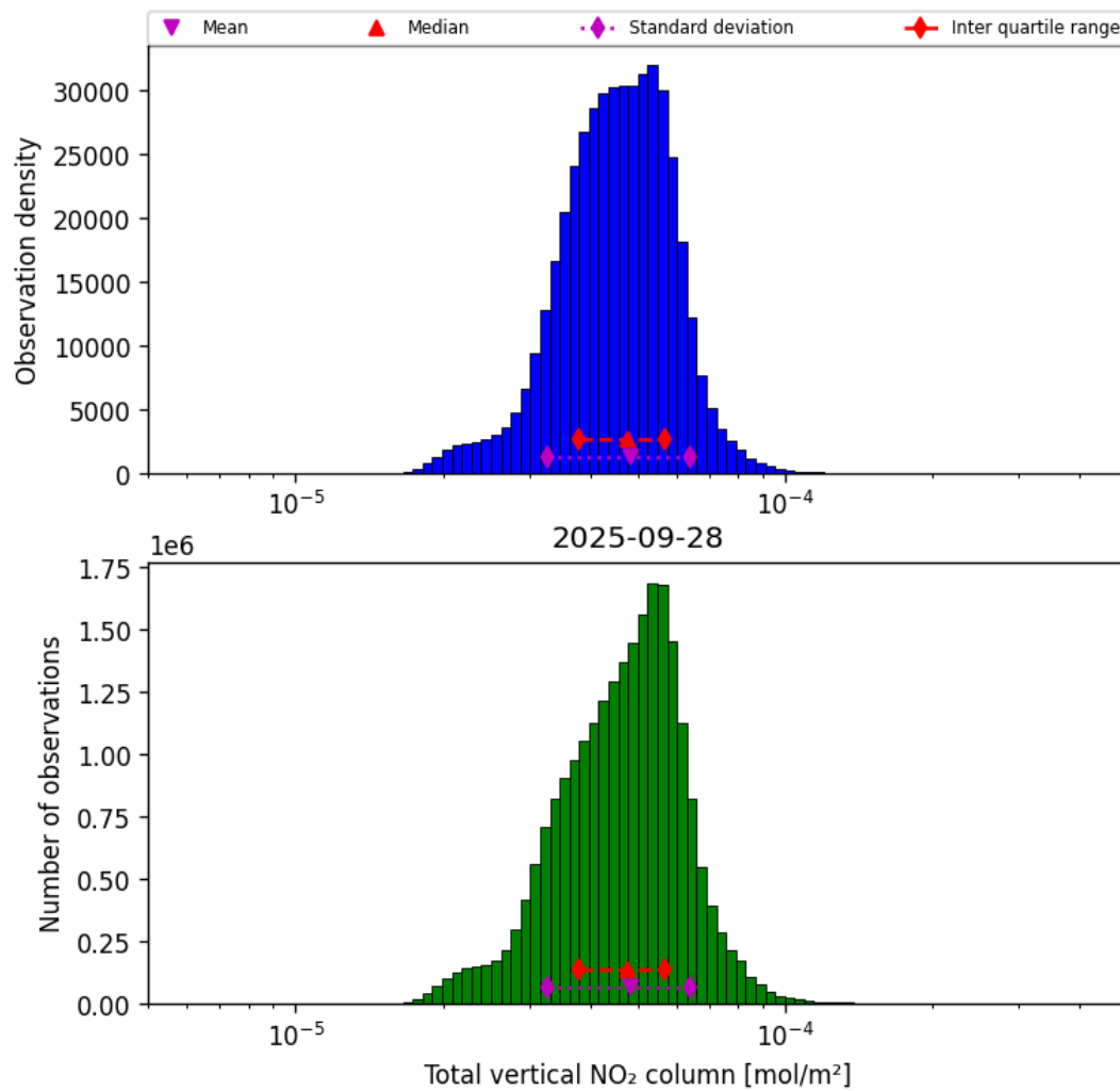
Figure 36: Histogram of "Total vertical NO 2 column" for 2025-09-28 to 2025-09-29
