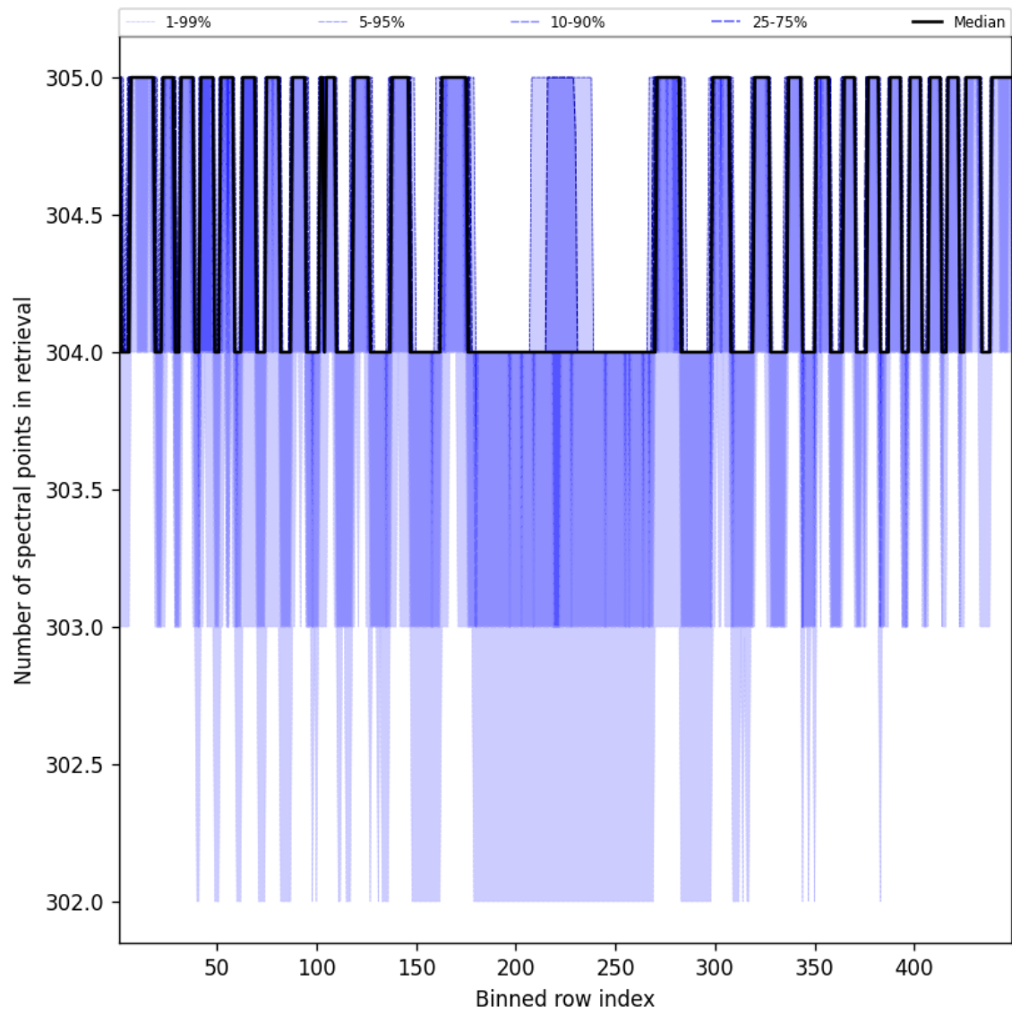
Figure 48: Along track statistics of “Number of spectral points in retrieval” for 2025-09-29 to 2025-09-29
