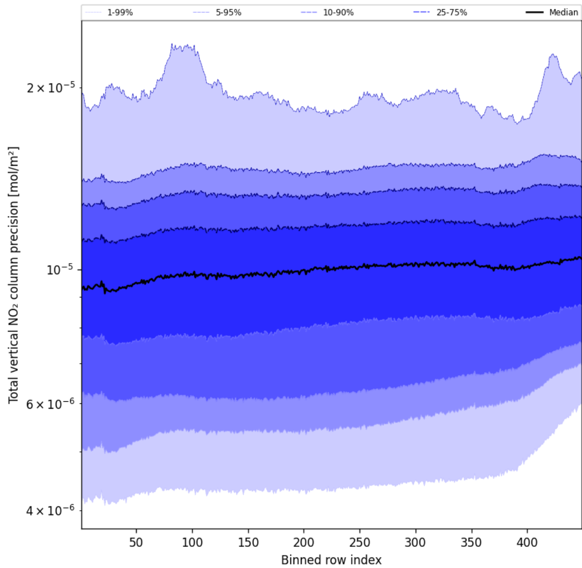
Figure 54: Along track statistics of “Total vertical NO 2 column precision” for 2025-09-29 to 2025-09-29
