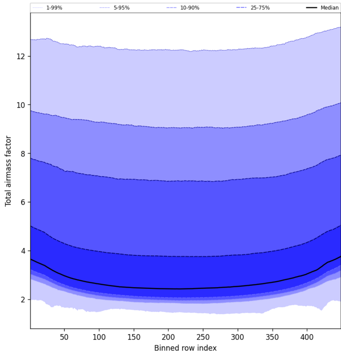
Figure 47: Along track statistics of “Total airmass factor” for 2025-09-29 to 2025-09-29
