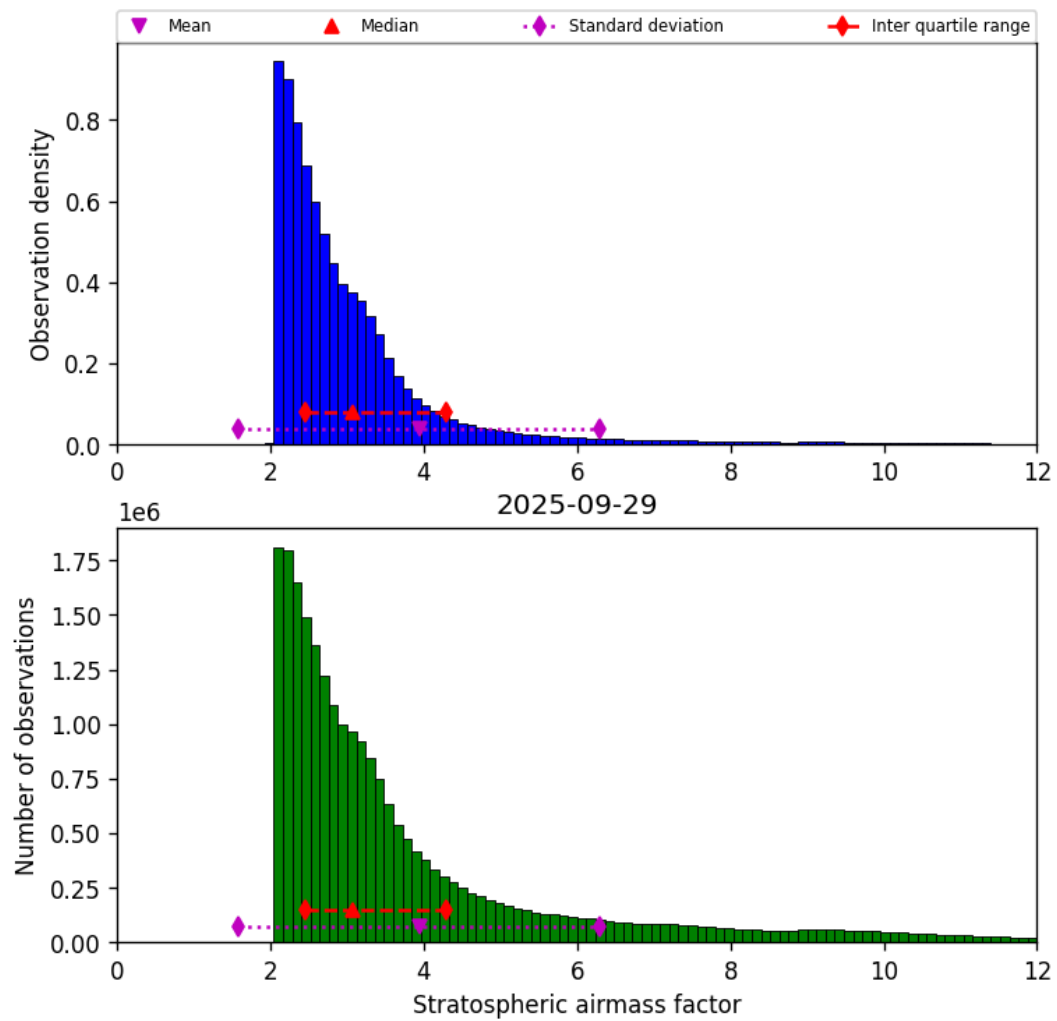
Figure 42: Histogram of “Stratospheric airmass factor” for 2025-09-29 to 2025-09-29
