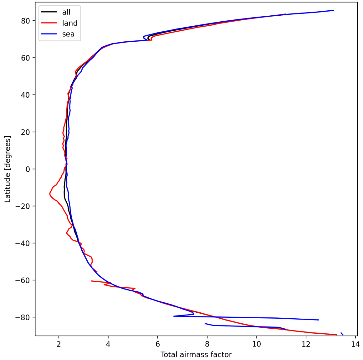
Figure 13: Zonal average of “Total airmass factor” for 2025-09-29 to 2025-09-29.
