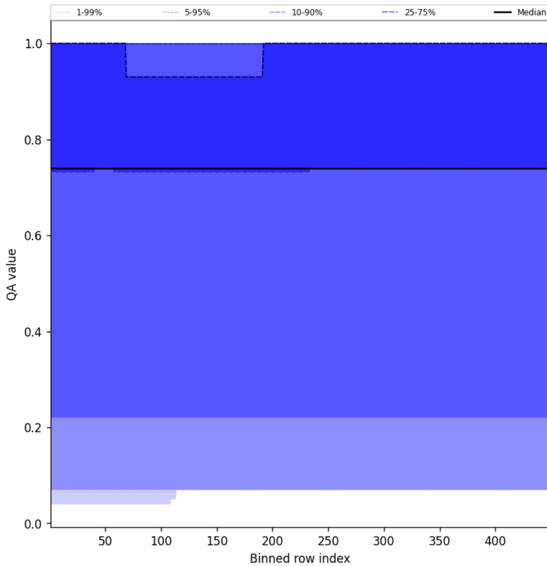
Figure 43: Along track statistics of "QA value" for 2025-09-29 to 2025-09-29
