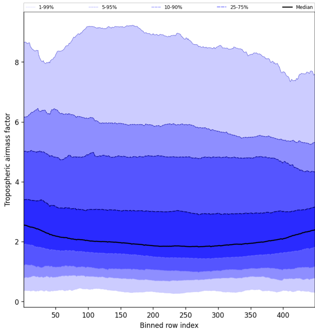
Figure 46: Along track statistics of “Tropospheric air mass factor” for 2025-09-29 to 2025-09-29
