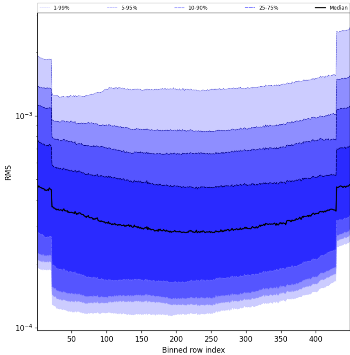
Figure 58: Along track statistics of “RMS” for 2025-09-29 to 2025-09-29
