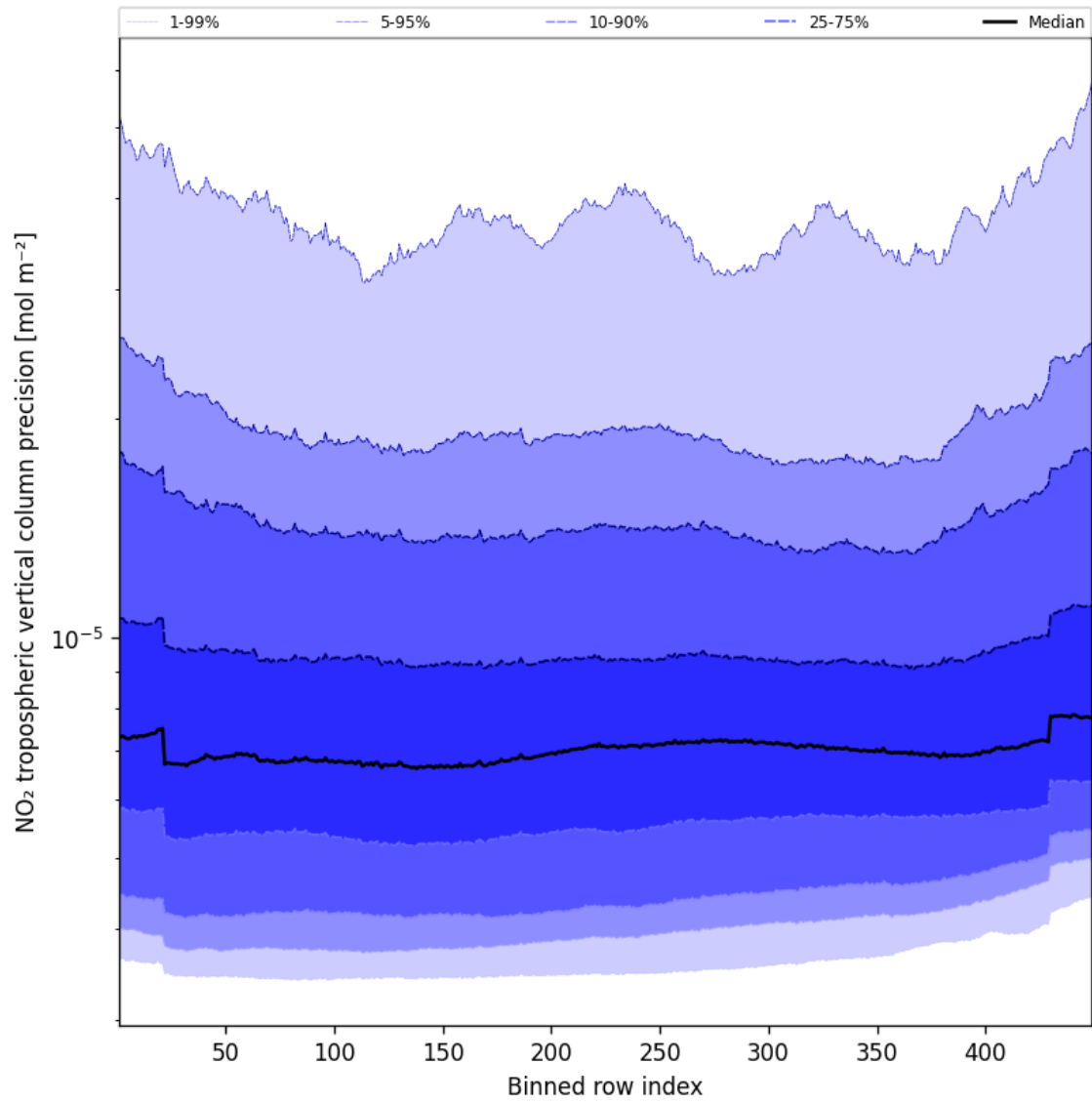
Figure 45: Along track statistics of “NO 2 tropospheric vertical column precision” for 2025-09-29 to 2025-09-29
