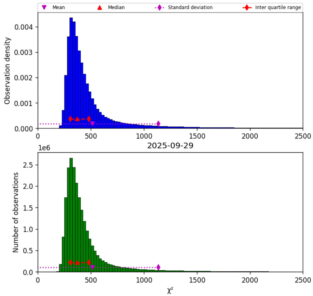
Figure 40: Histogram of " \chi^2 " for 2025-09-29 to 2025-09-29
