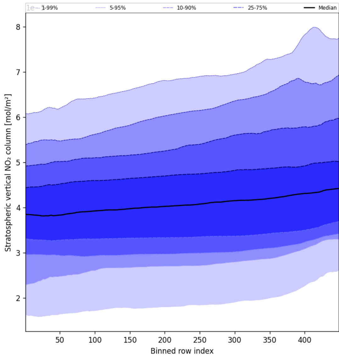
Figure 51: Along track statistics of “Stratospheric vertical NO 2 column” for 2025-09-29 to 2025-09-29
