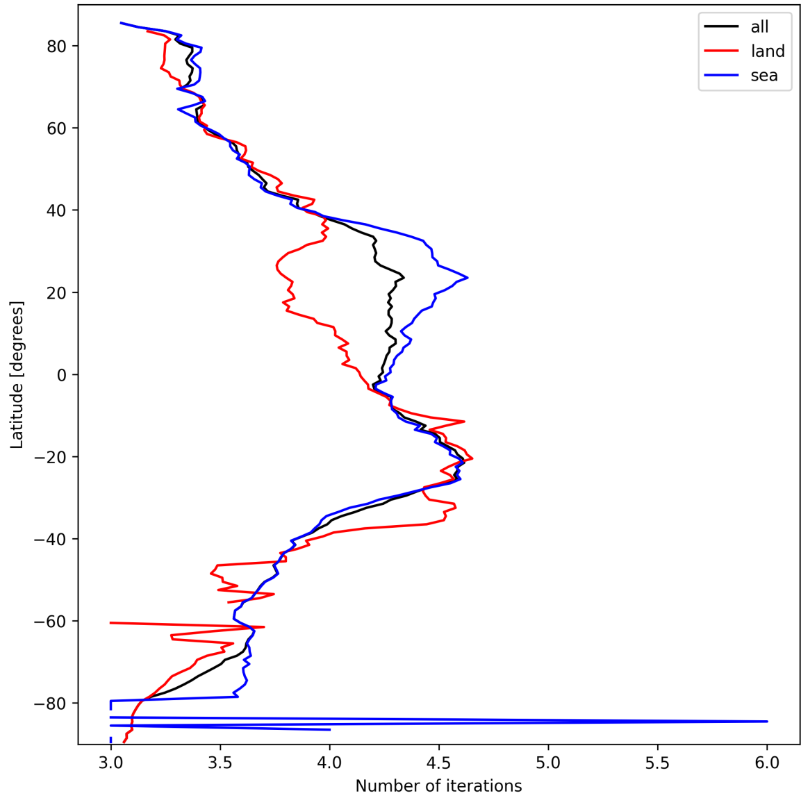
Figure 15: Zonal average of “Number of iterations” for 2025-09-29 to 2025-09-29.
