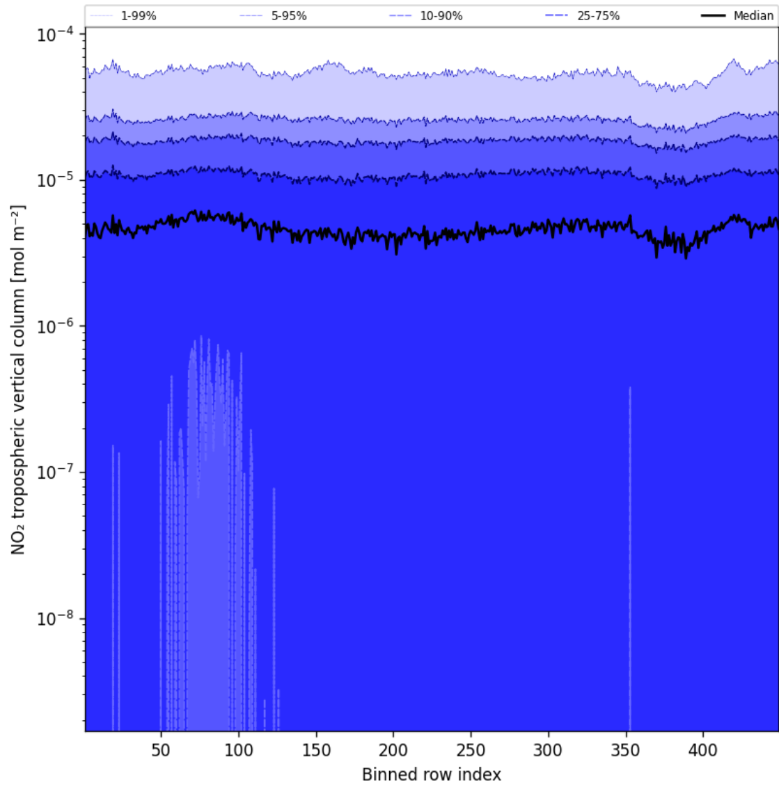
Figure 44: Along track statistics of “NO 2 tropospheric vertical column” for 2025-09-29 to 2025-09-29
