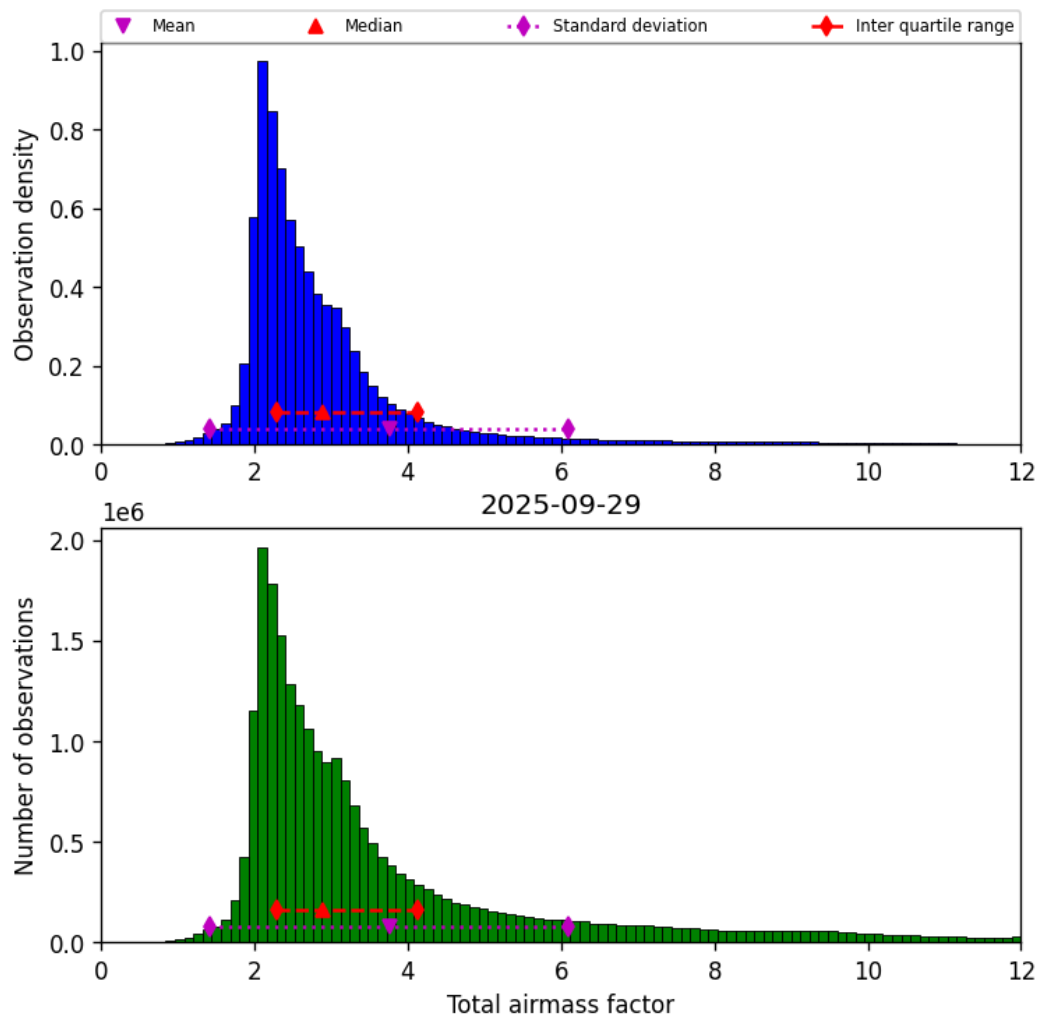
Figure 30: Histogram of “Total airmass factor” for 2025-09-29 to 2025-09-29
