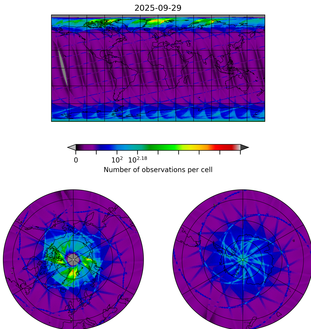
Figure 8: Map of the number of observations for 2025-09-29 to 2025-09-29
