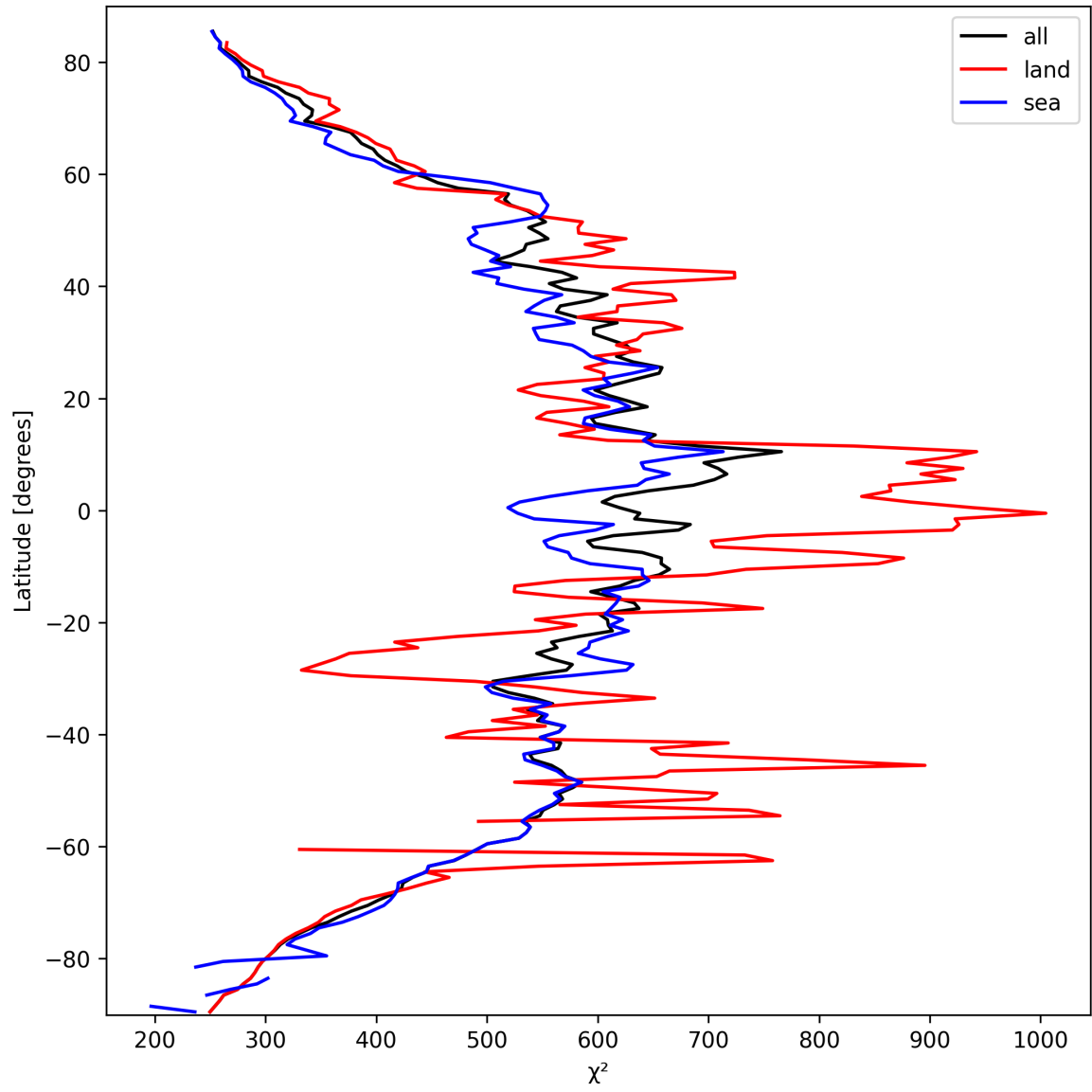
Figure 23: Zonal average of “ \chi^2 ” for 2025-09-29 to 2025-09-29.
