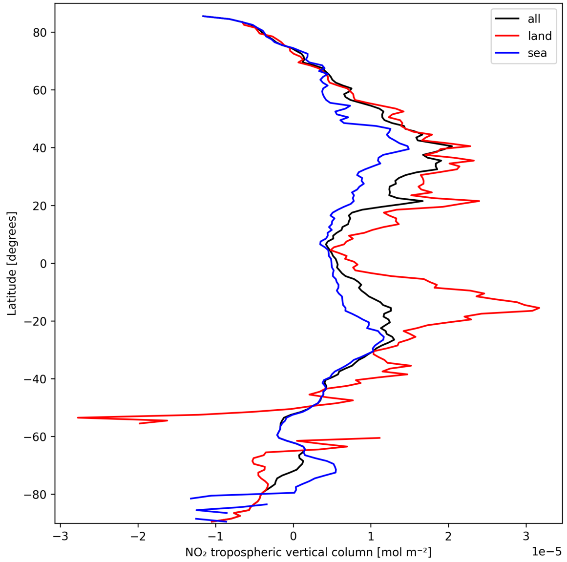
Figure 10: Zonal average of “NO 2 tropospheric vertical column” for 2025-09-29 to 2025-09-29.
