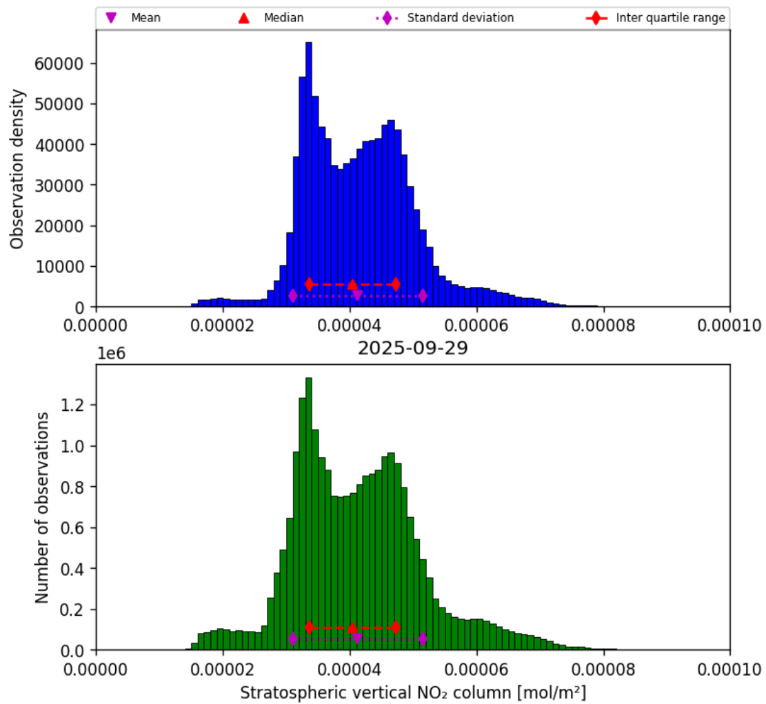
Figure 34: Histogram of “Stratospheric vertical NO 2 column” for 2025-09-29 to 2025-09-29
