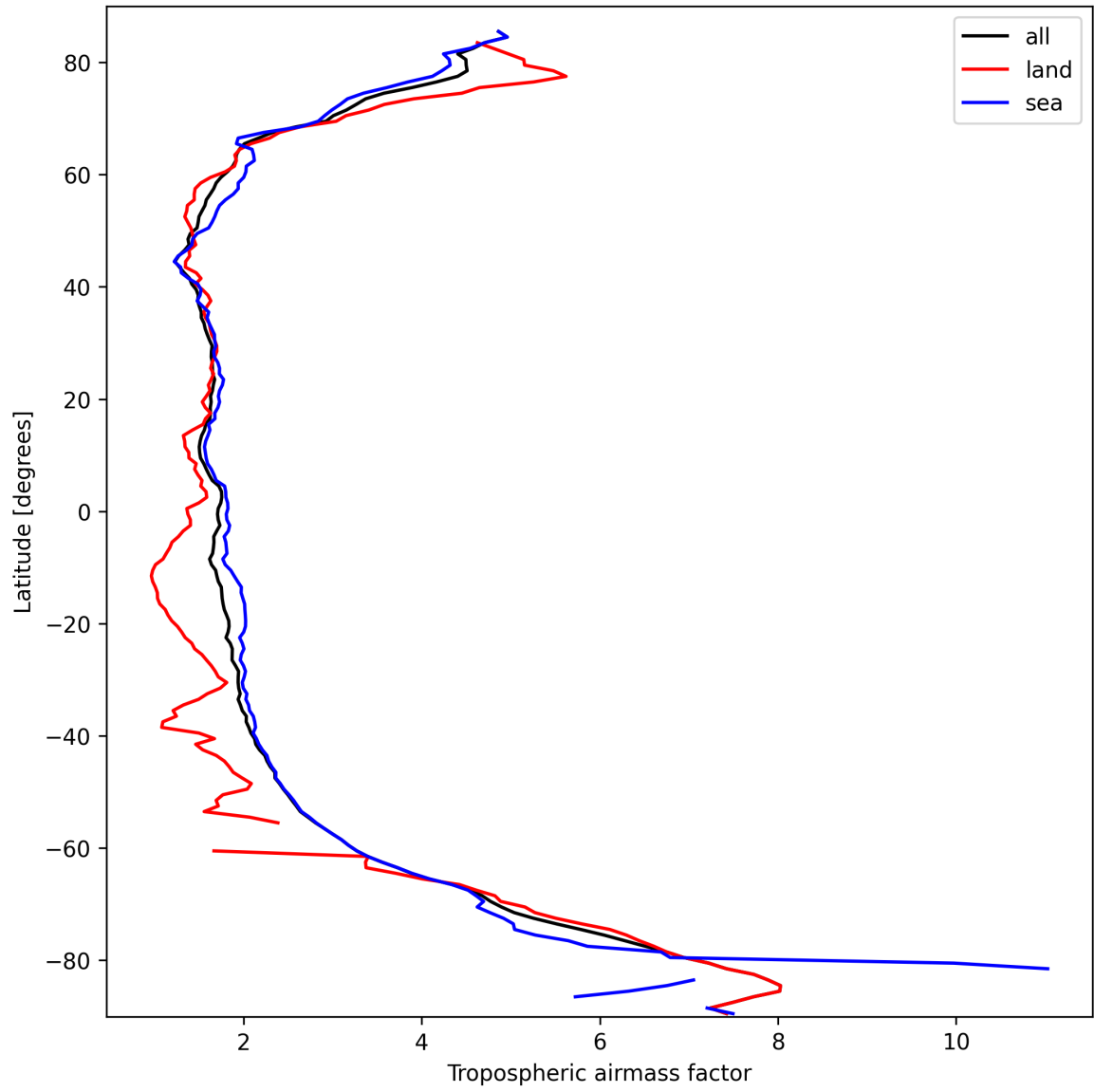
Figure 12: Zonal average of “Tropospheric air mass factor” for 2025-09-29 to 2025-09-29.
