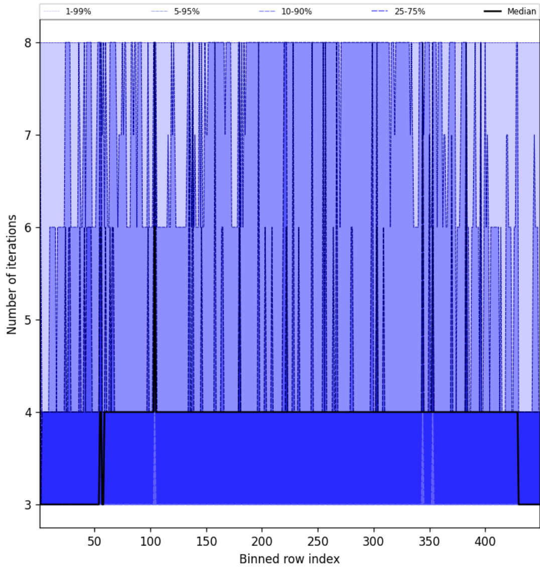
Figure 49: Along track statistics of “Number of iterations” for 2025-09-29 to 2025-09-29
