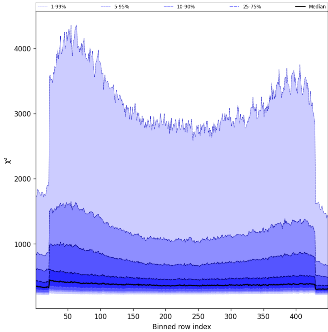
Figure 57: Along track statistics of “ \chi^2 ” for 2025-09-29 to 2025-09-29
