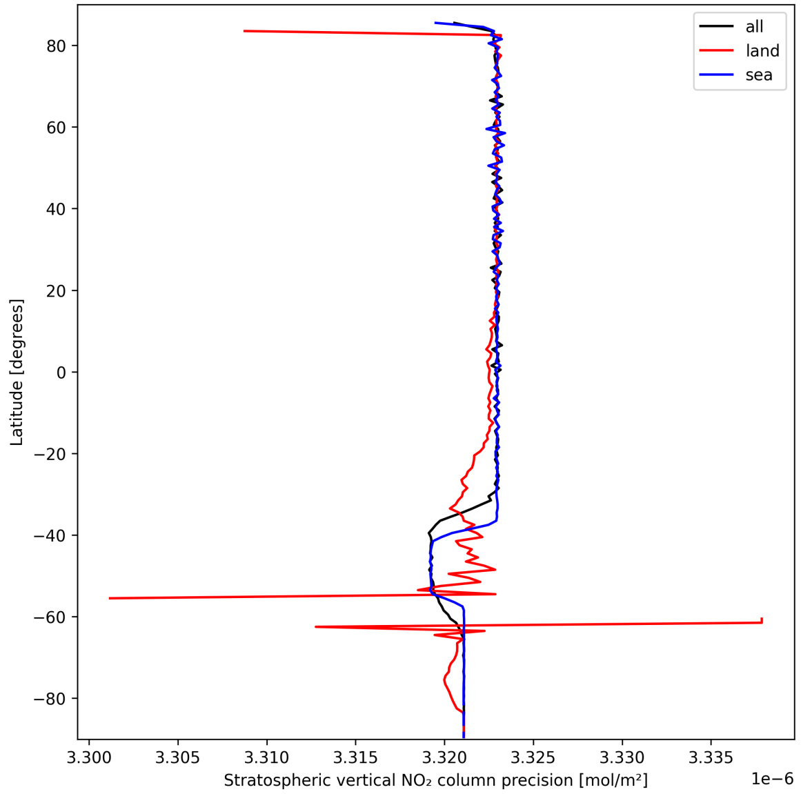
Figure 18: Zonal average of "Stratospheric vertical NO 2 column precision" for 2025-09-29 to 2025-09-29.
