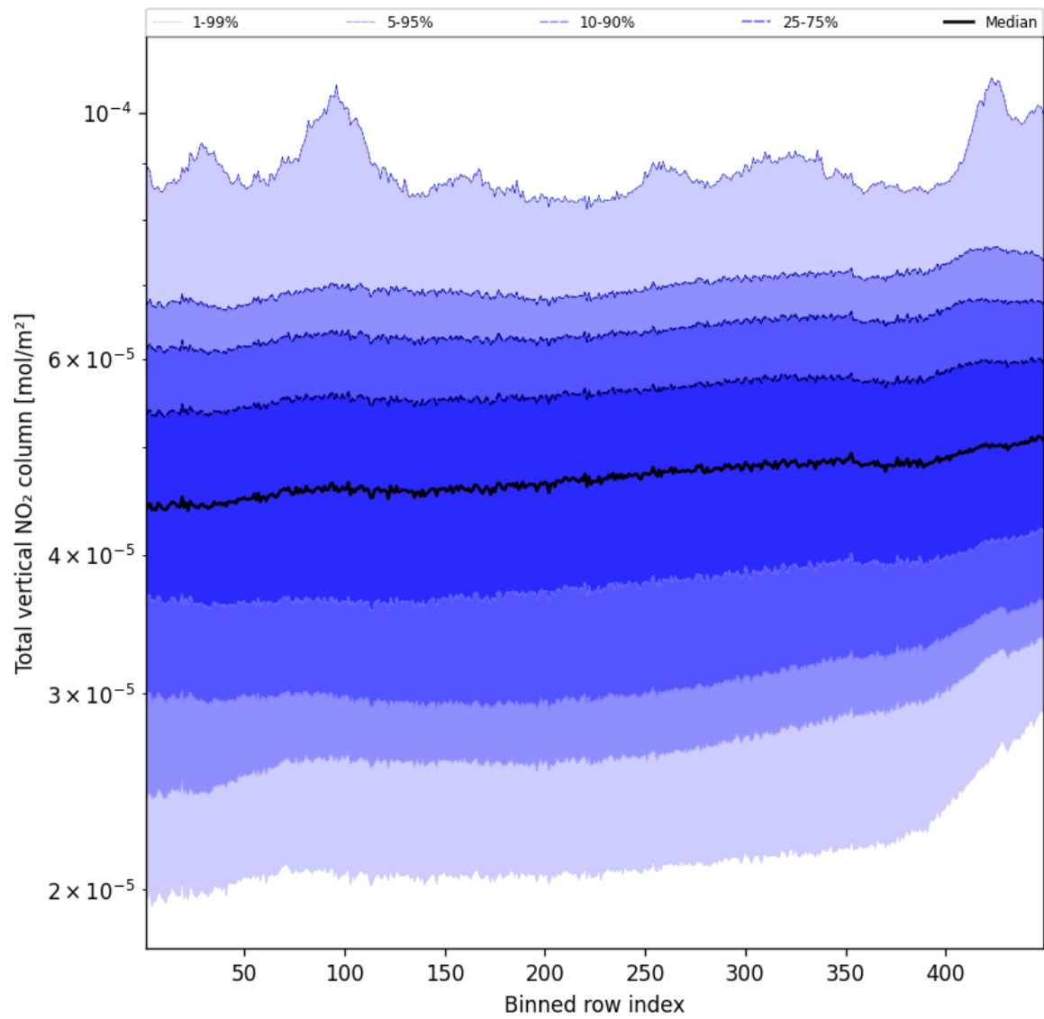
Figure 53: Along track statistics of “Total vertical NO 2 column” for 2025-09-29 to 2025-09-29
