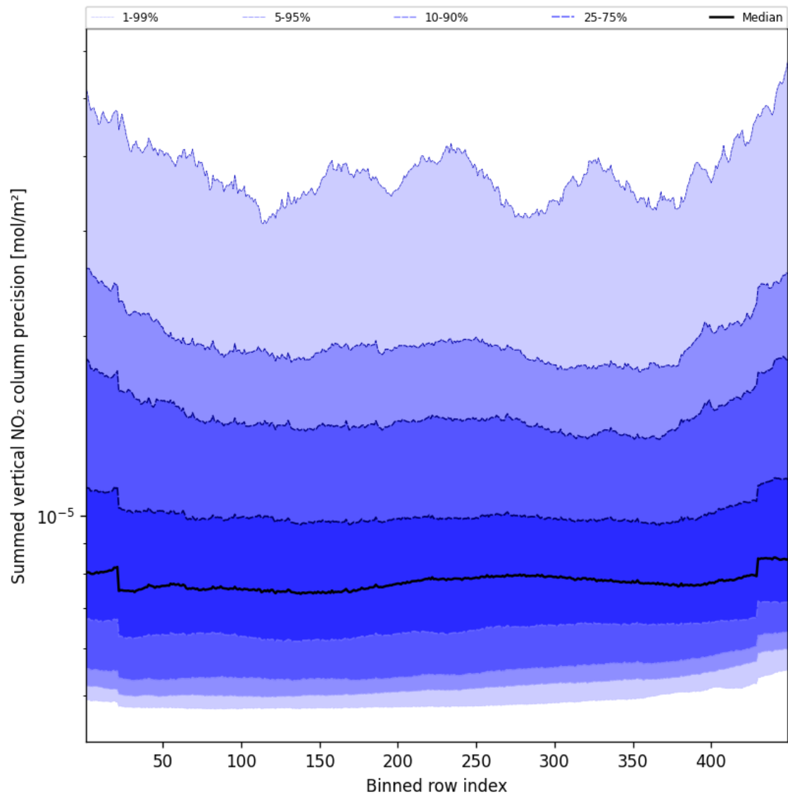
Figure 56: Along track statistics of “Summed vertical NO 2 column precision” for 2025-09-29 to 2025-09-29
