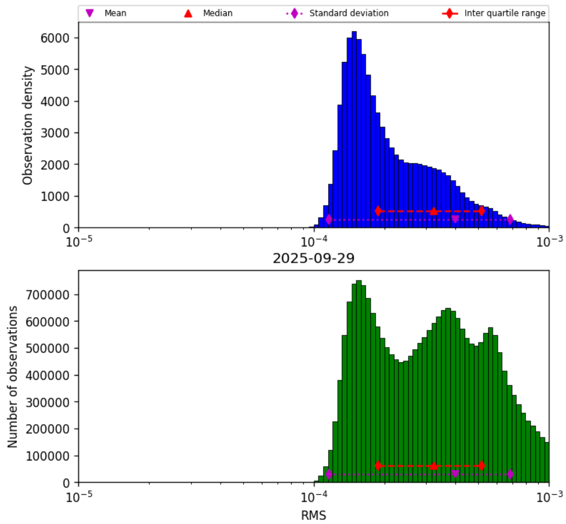
Figure 41: Histogram of “RMS” for 2025-09-29 to 2025-09-29
