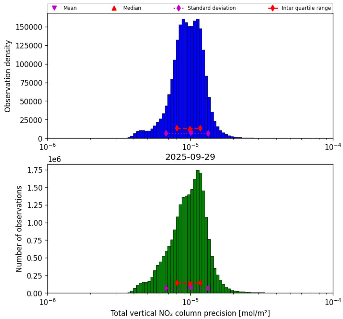
Figure 37: Histogram of "Total vertical NO 2 column precision" for 2025-09-29 to 2025-09-29
