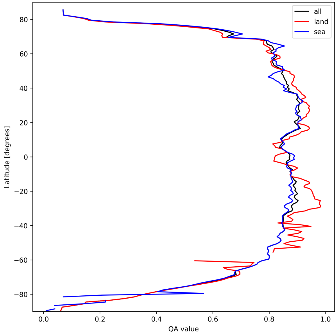
Figure 9: Zonal average of “QA value” for 2025-09-29 to 2025-09-29.
