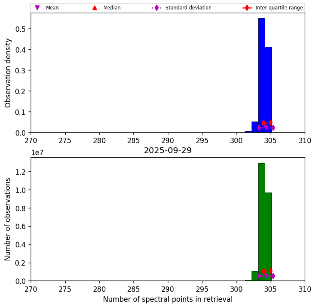
Figure 31: Histogram of “Number of spectral points in retrieval” for 2025-09-29 to 2025-09-29
