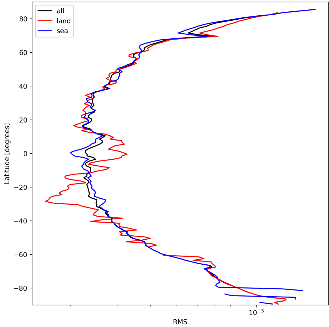
Figure 24: Zonal average of “RMS” for 2025-09-29 to 2025-09-29.
