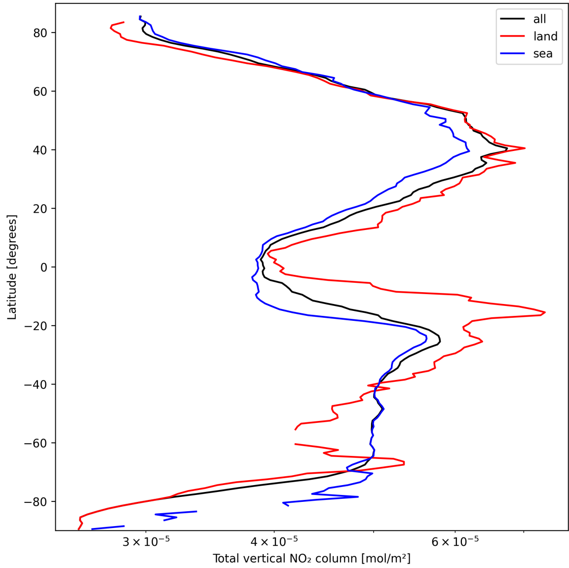
Figure 19: Zonal average of “Total vertical NO 2 column” for 2025-09-29 to 2025-09-29.
