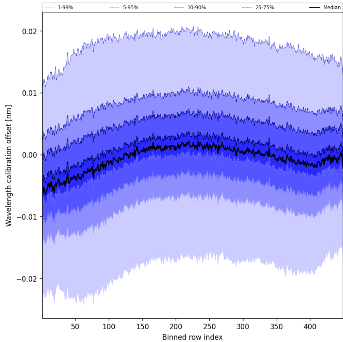
Figure 50: Along track statistics of “Wavelength calibration offset” for 2025-09-29 to 2025-09-29
