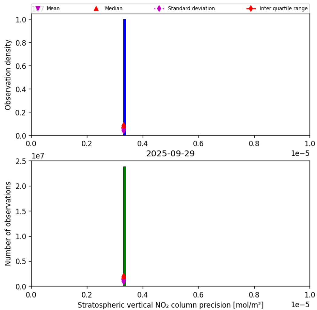
Figure 35: Histogram of “Stratospheric vertical NO 2 column precision” for 2025-09-29 to 2025-09-29
