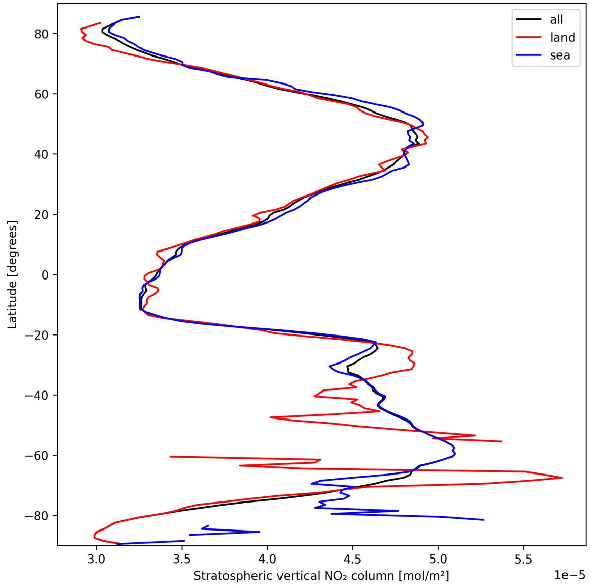
Figure 17: Zonal average of “Stratospheric vertical NO 2 column” for 2025-09-29 to 2025-09-29.
