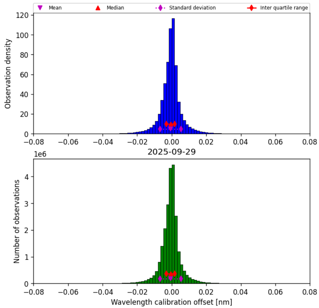
Figure 33: Histogram of “Wavelength calibration offset” for 2025-09-29 to 2025-09-29
