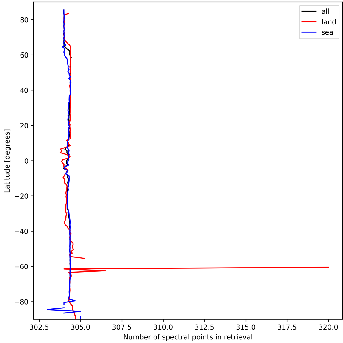
Figure 14: Zonal average of “Number of spectral points in retrieval” for 2025-09-29 to 2025-09-29.
