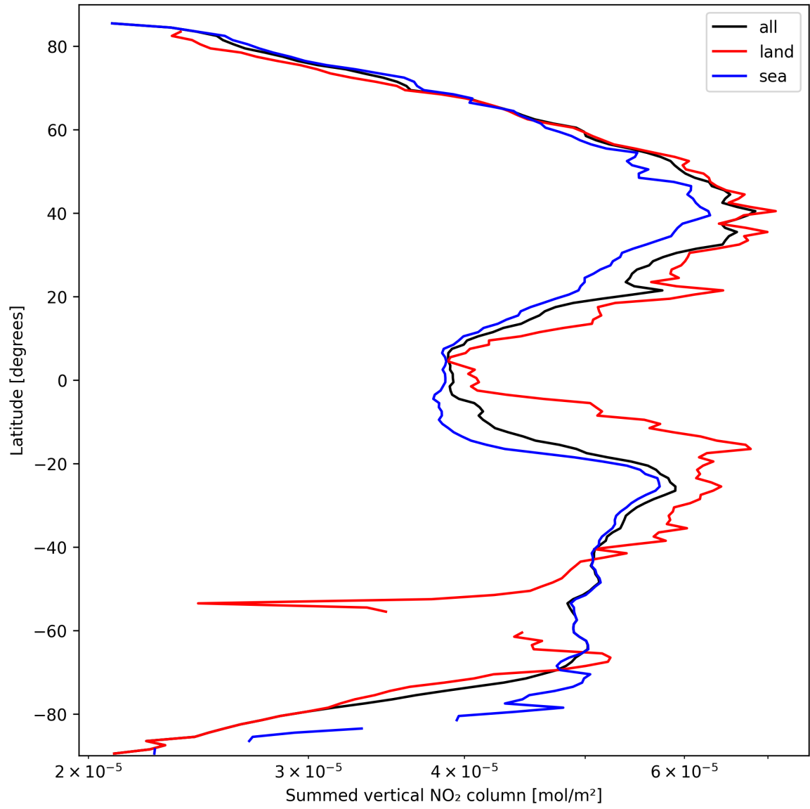
Figure 21: Zonal average of “Summed vertical NO 2 column” for 2025-09-29 to 2025-09-29.
