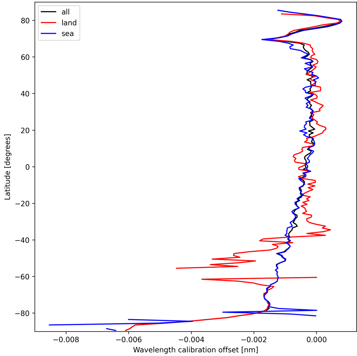
Figure 16: Zonal average of “Wavelength calibration offset” for 2025-09-29 to 2025-09-29.
