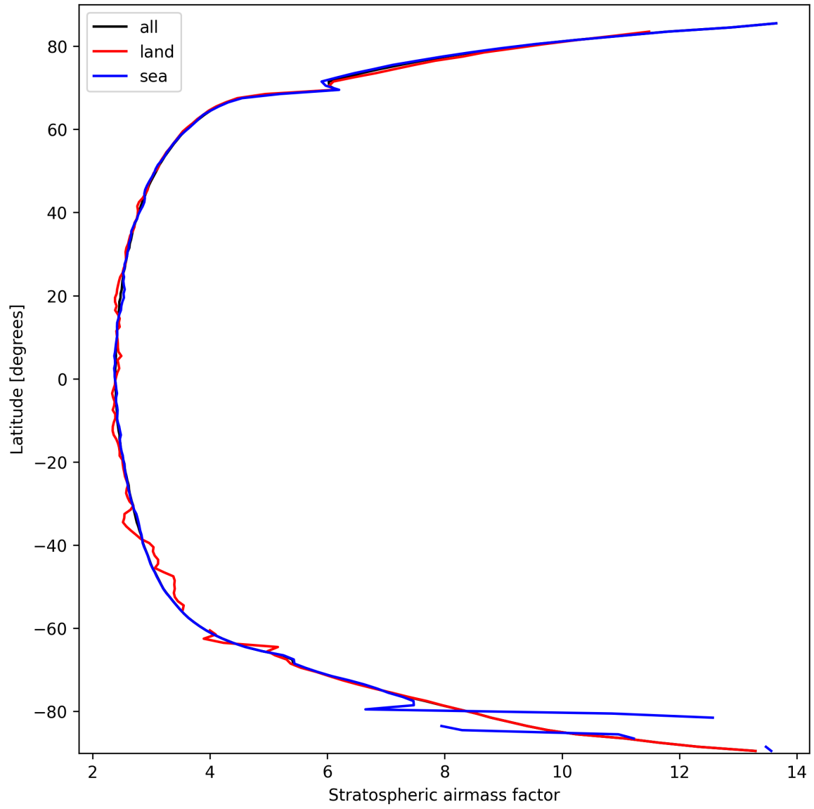
Figure 25: Zonal average of “Stratospheric air mass factor” for 2025-09-29 to 2025-09-29.
