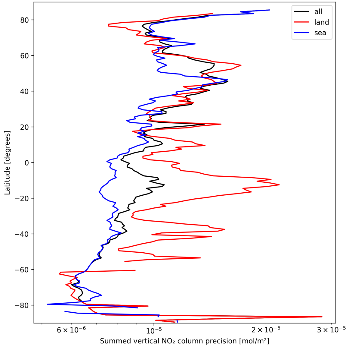
Figure 22: Zonal average of “Summed vertical NO 2 column precision” for 2025-09-29 to 2025-09-29.
