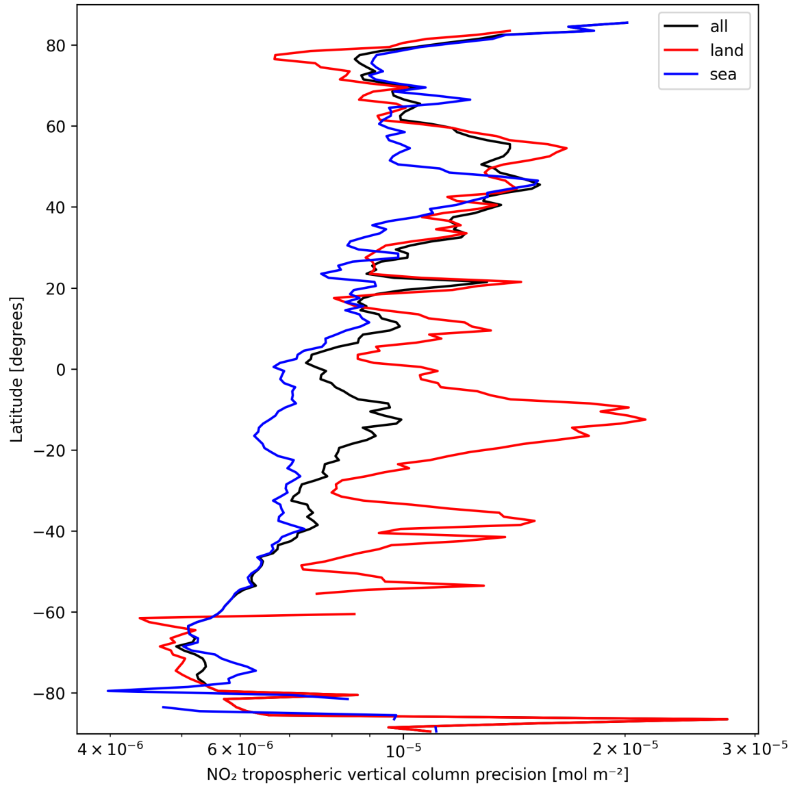
Figure 11: Zonal average of “NO 2 tropospheric vertical column precision” for 2025-09-29 to 2025-09-29.
