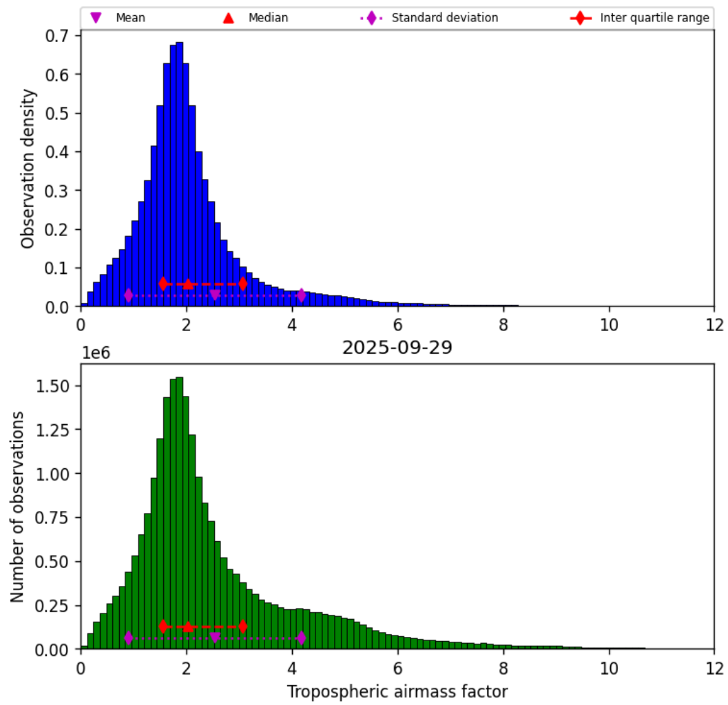
Figure 29: Histogram of “Tropospheric airmass factor” for 2025-09-29 to 2025-09-29
