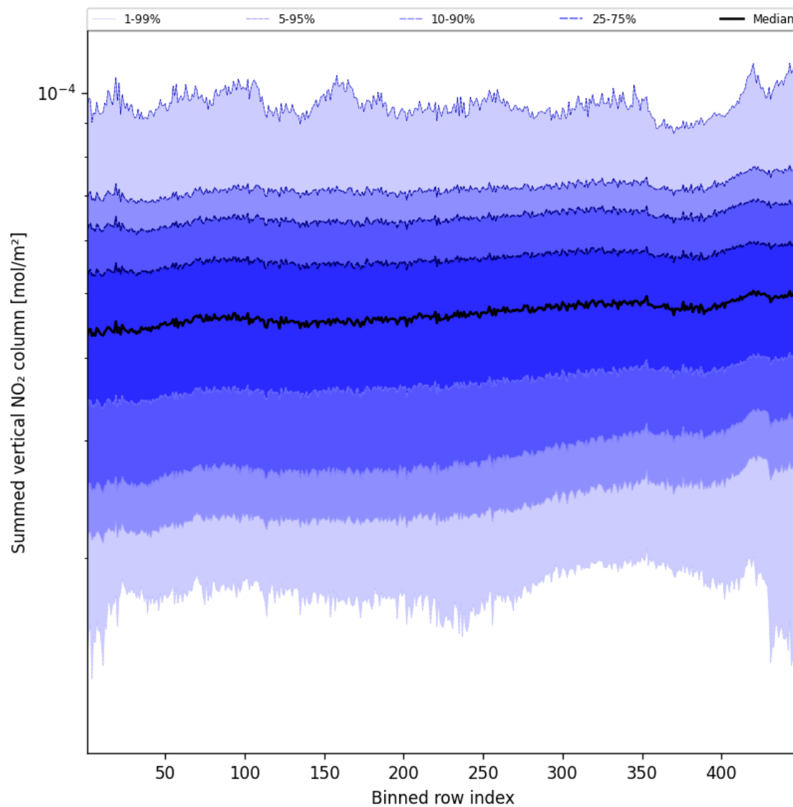
Figure 55: Along track statistics of “Summed vertical NO 2 column” for 2025-09-29 to 2025-09-29
