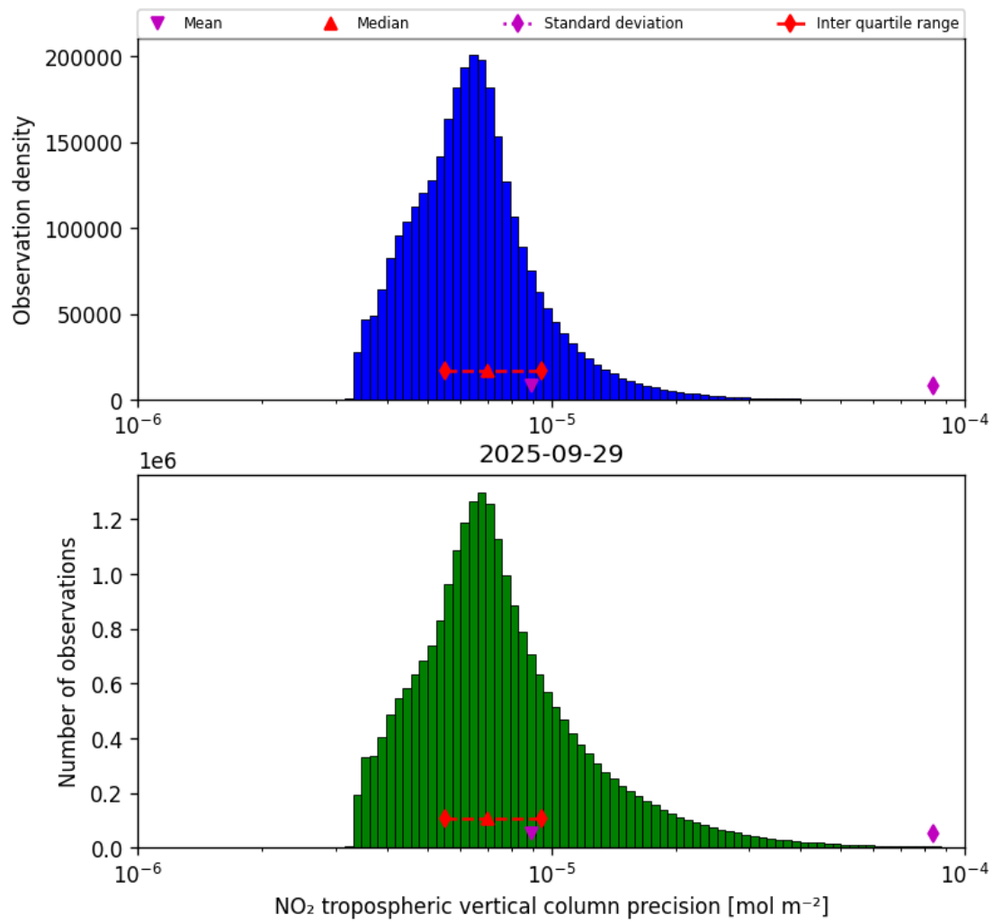
Figure 28: Histogram of “NO 2 tropospheric vertical column precision” for 2025-09-29 to 2025-09-29
