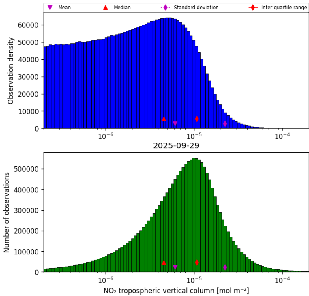
Figure 27: Histogram of “NO 2 tropospheric vertical column” for 2025-09-29 to 2025-09-29
