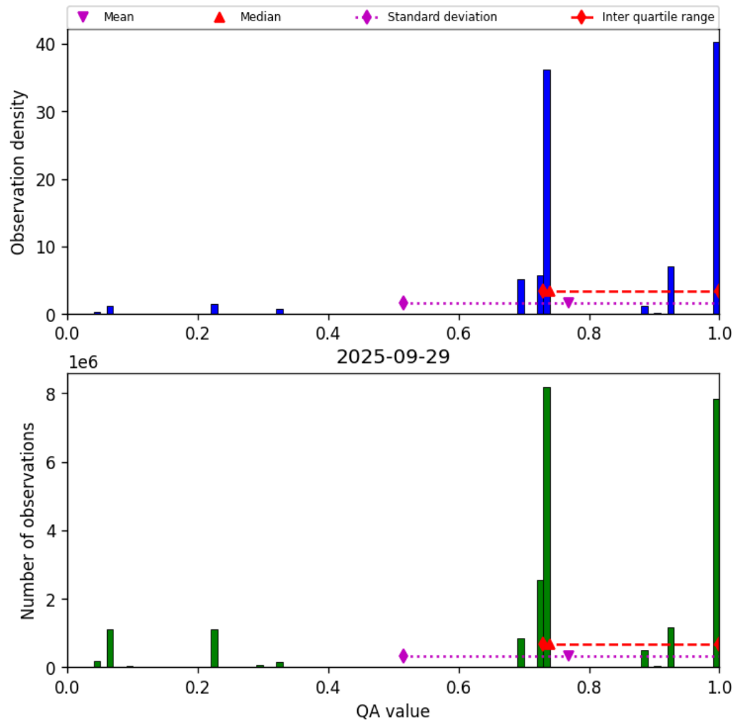
Figure 26: Histogram of “QA value” for 2025-09-29 to 2025-09-29
