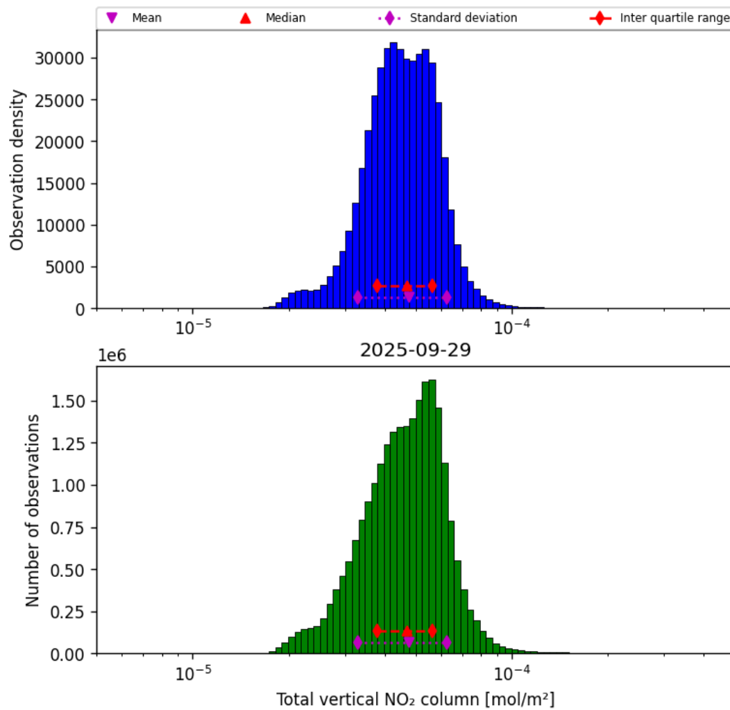
Figure 36: Histogram of “Total vertical NO 2 column” for 2025-09-29 to 2025-09-29
