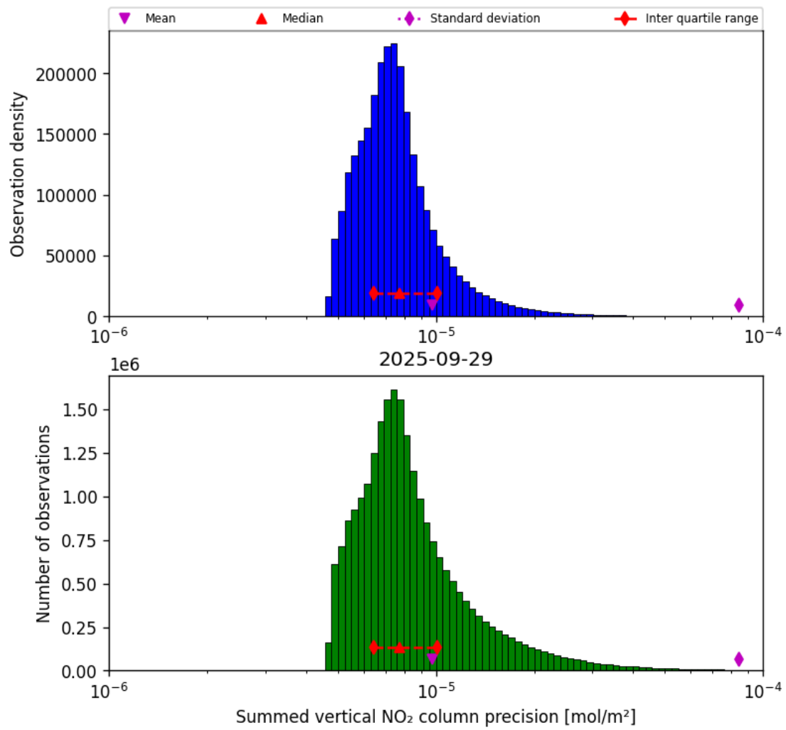
Figure 39: Histogram of "Summed vertical NO 2 column precision" for 2025-09-29 to 2025-09-29
