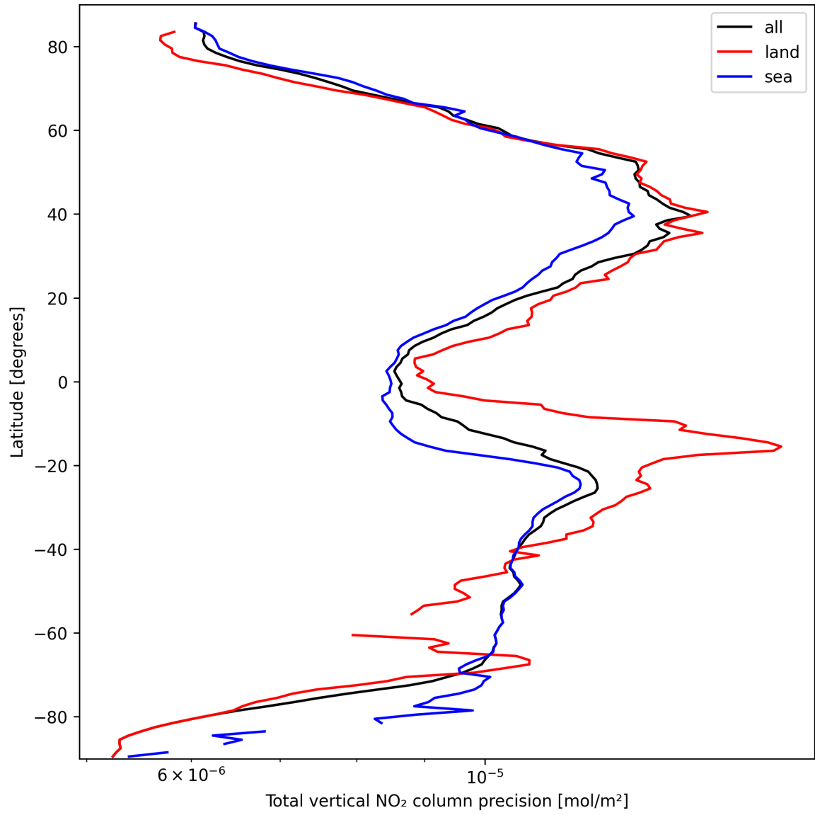
Figure 20: Zonal average of “Total vertical NO 2 column precision” for 2025-09-29 to 2025-09-29.
