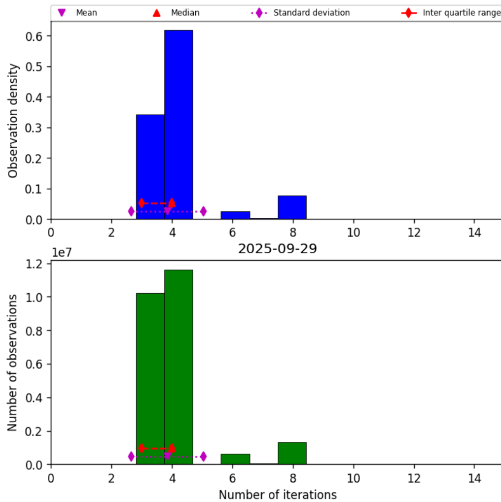
Figure 32: Histogram of “Number of iterations” for 2025-09-29 to 2025-09-29
