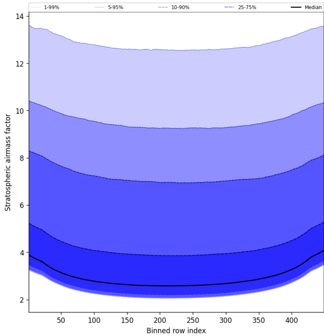
Figure 59: Along track statistics of “Stratospheric airmass factor” for 2025-09-29 to 2025-09-29
