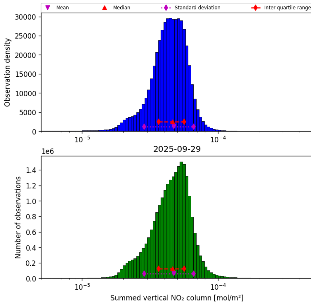
Figure 38: Histogram of "Summed vertical NO 2 column" for 2025-09-29 to 2025-09-29
