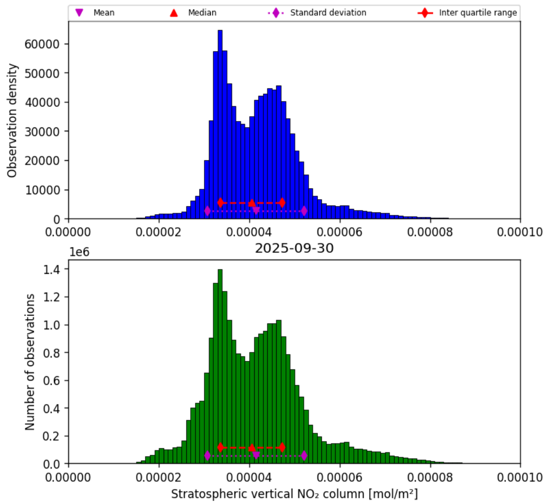
Figure 34: Histogram of “Stratospheric vertical NO 2 column” for 2025-09-30 to 2025-10-01
