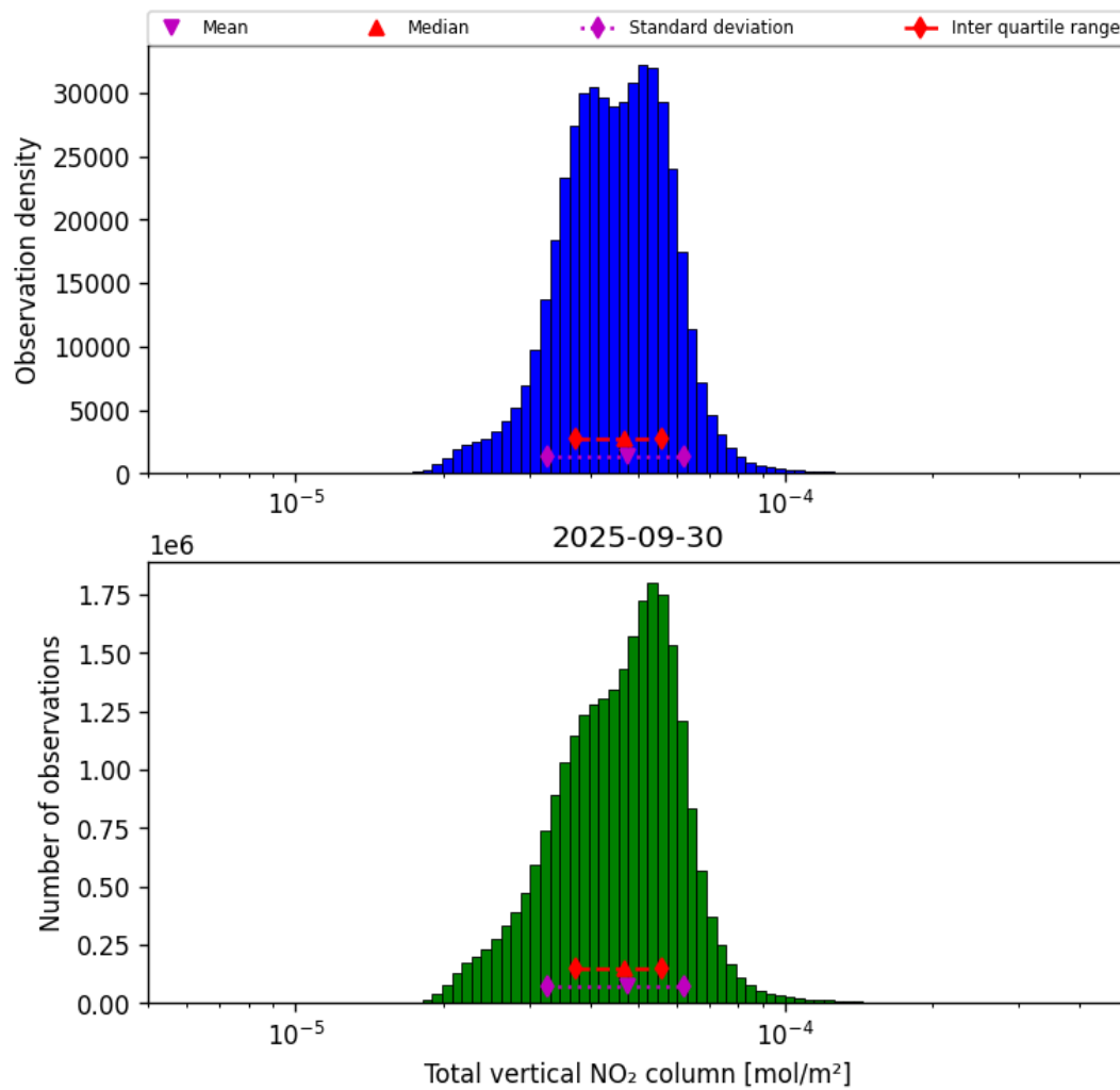
Figure 36: Histogram of “Total vertical NO 2 column” for 2025-09-30 to 2025-10-01
