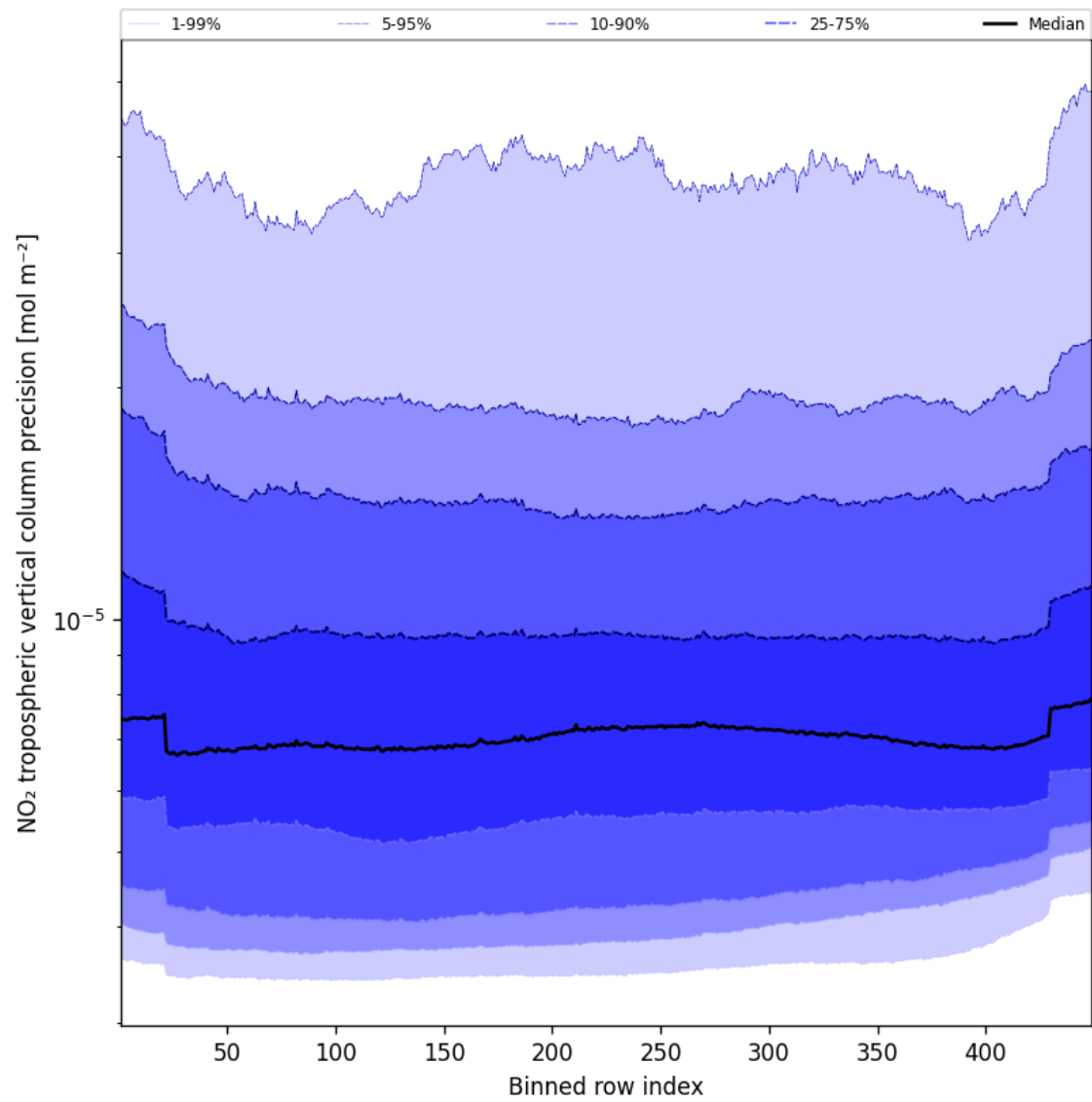
Figure 45: Along track statistics of “NO 2 tropospheric vertical column precision” for 2025-09-30 to 2025-10-01
