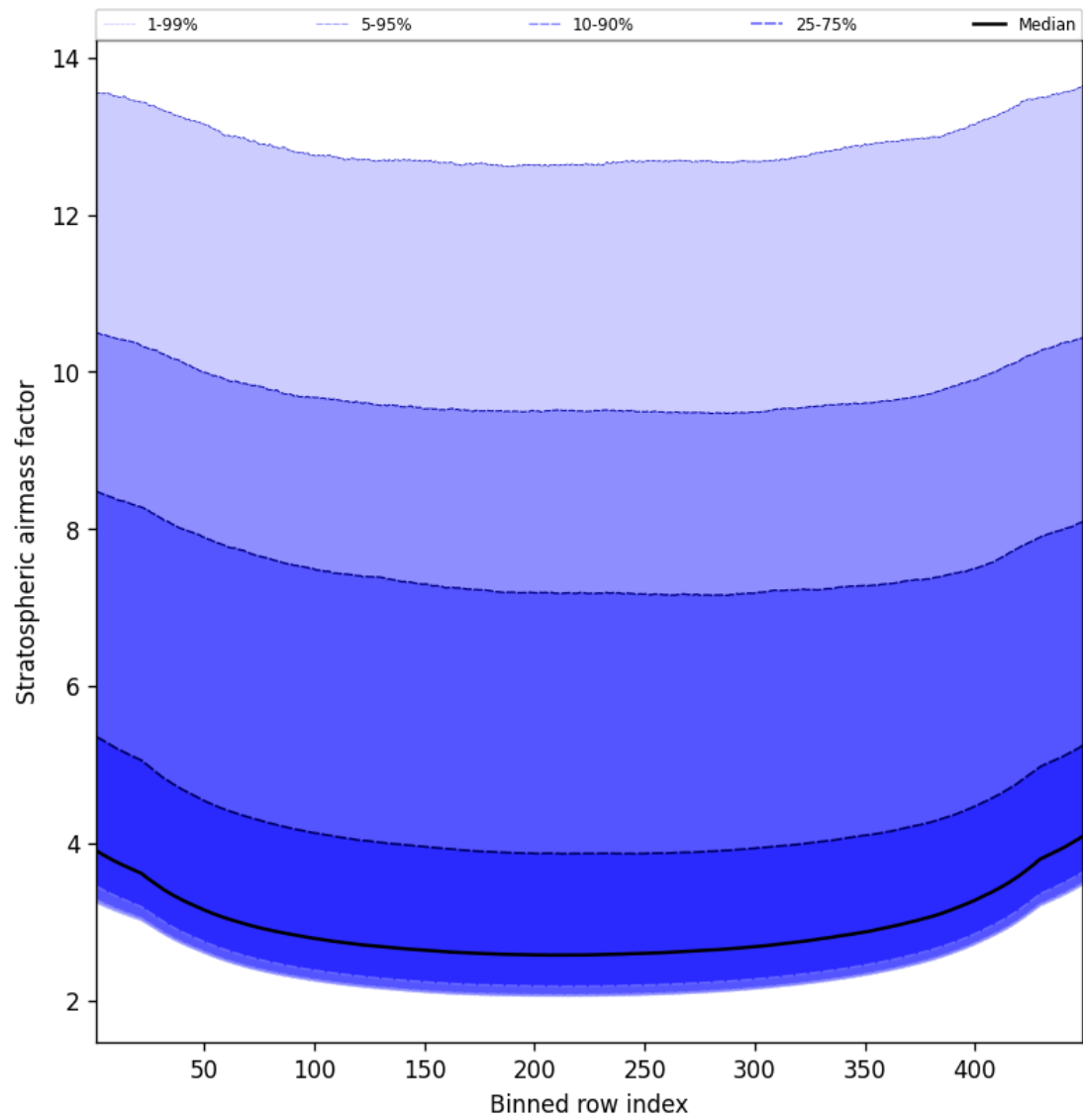
Figure 59: Along track statistics of “Stratospheric airmass factor” for 2025-09-30 to 2025-10-01
