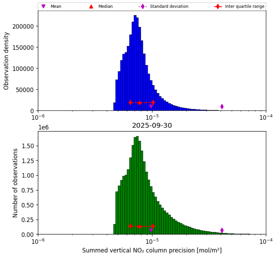
Figure 39: Histogram of "Summed vertical NO 2 column precision" for 2025-09-30 to 2025-10-01
