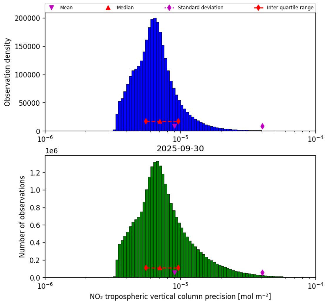
Figure 28: Histogram of “NO 2 tropospheric vertical column precision” for 2025-09-30 to 2025-10-01
