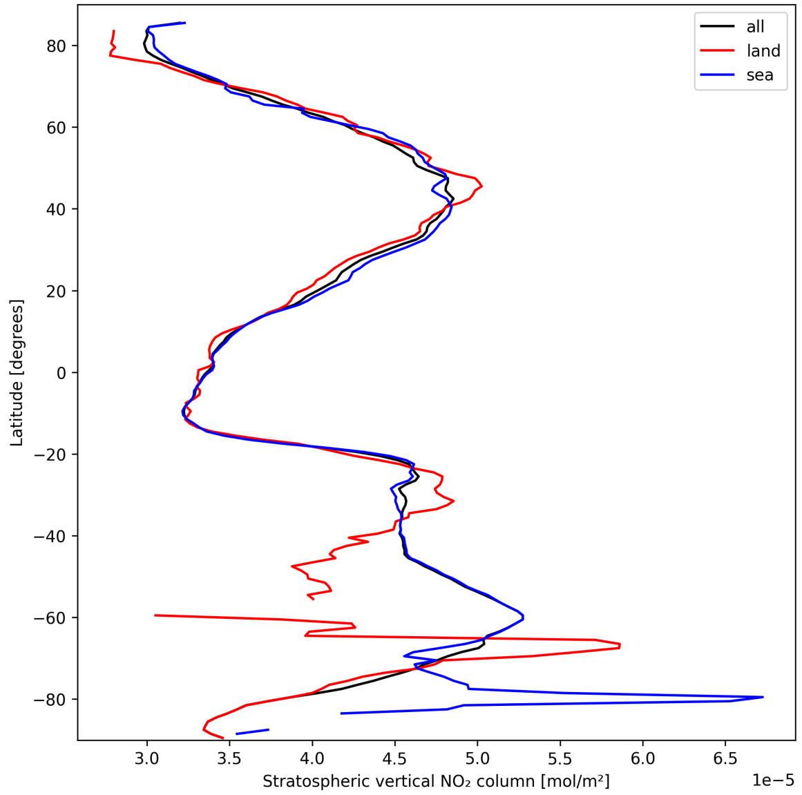
Figure 17: Zonal average of “Stratospheric vertical NO 2 column” for 2025-09-30 to 2025-10-01.
