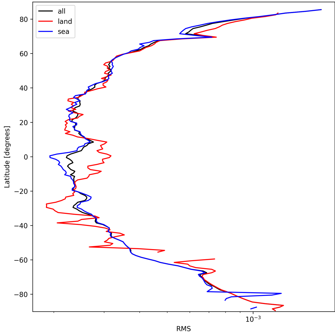
Figure 24: Zonal average of “RMS” for 2025-09-30 to 2025-10-01.
