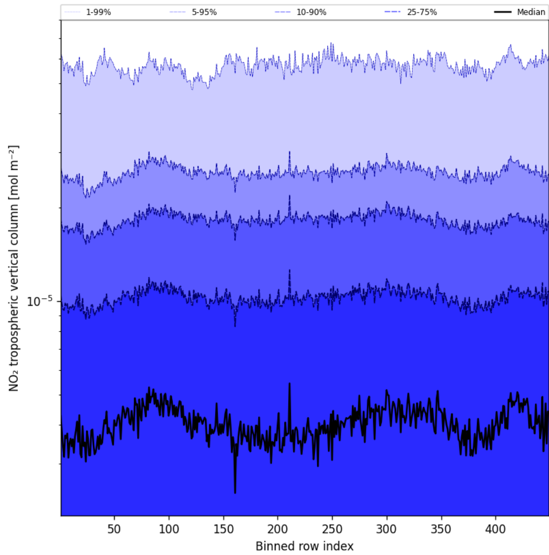
Figure 44: Along track statistics of “NO 2 tropospheric vertical column” for 2025-09-30 to 2025-10-01
