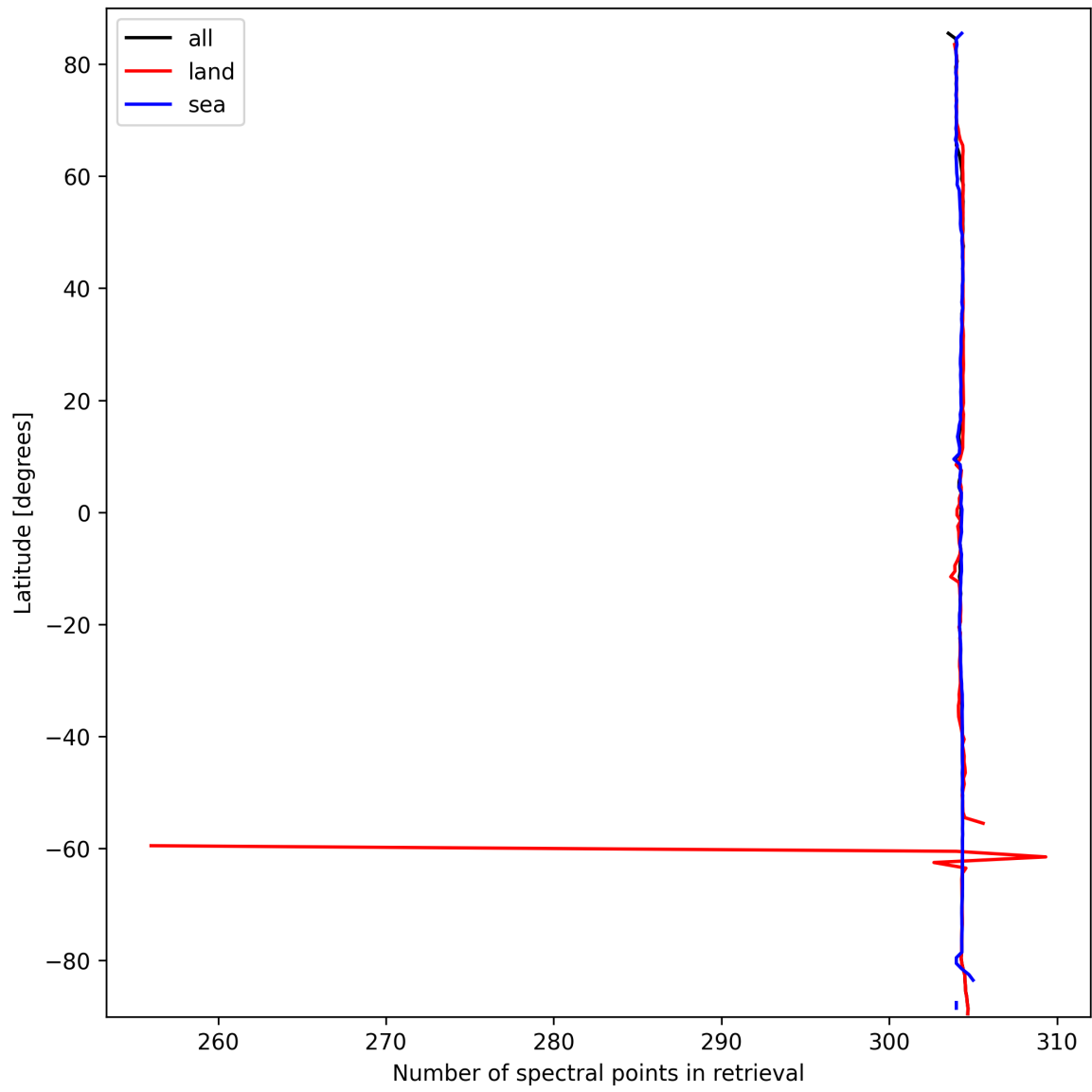
Figure 14: Zonal average of “Number of spectral points in retrieval” for 2025-09-30 to 2025-10-01.
