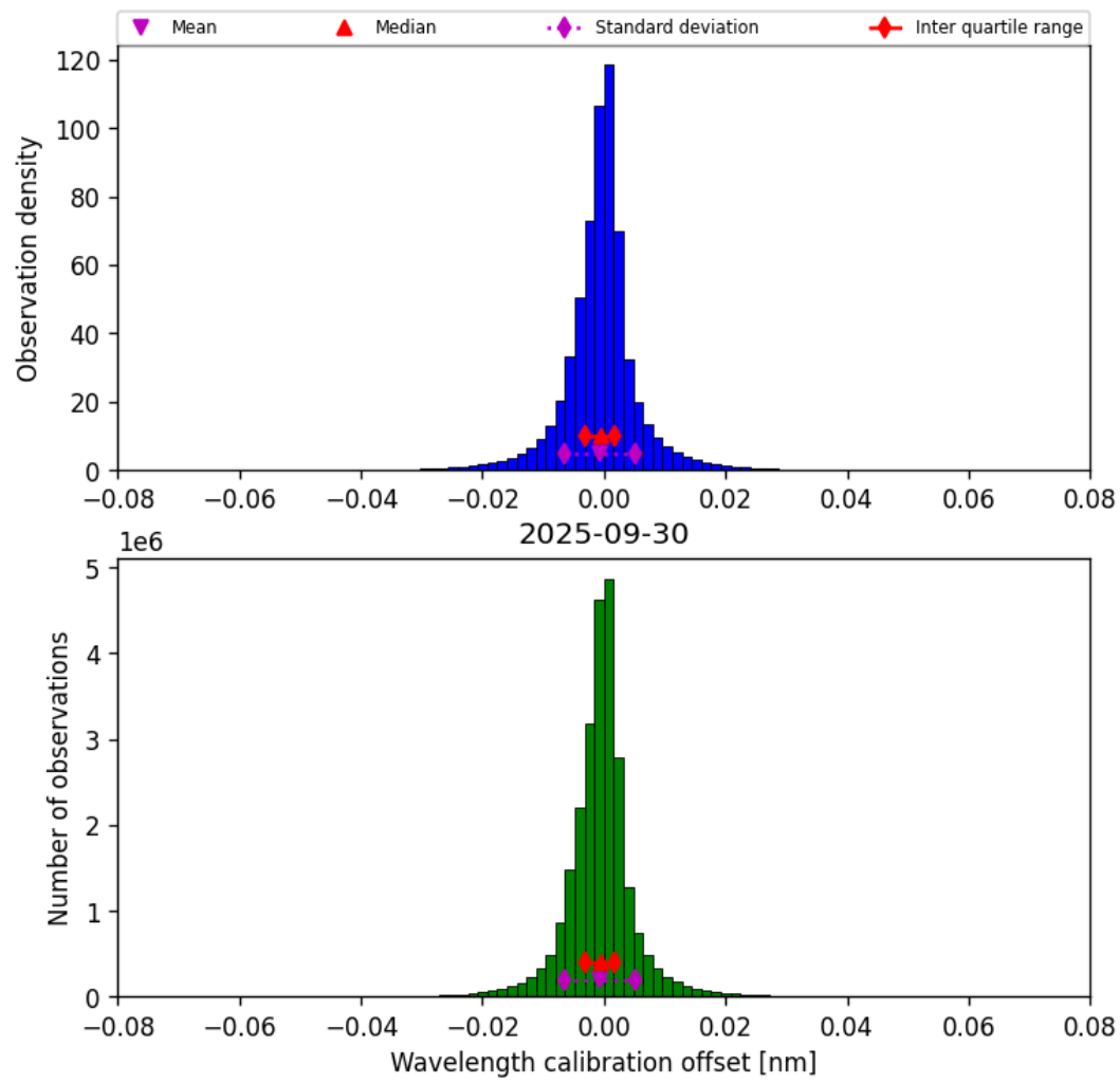
Figure 33: Histogram of “Wavelength calibration offset” for 2025-09-30 to 2025-10-01
