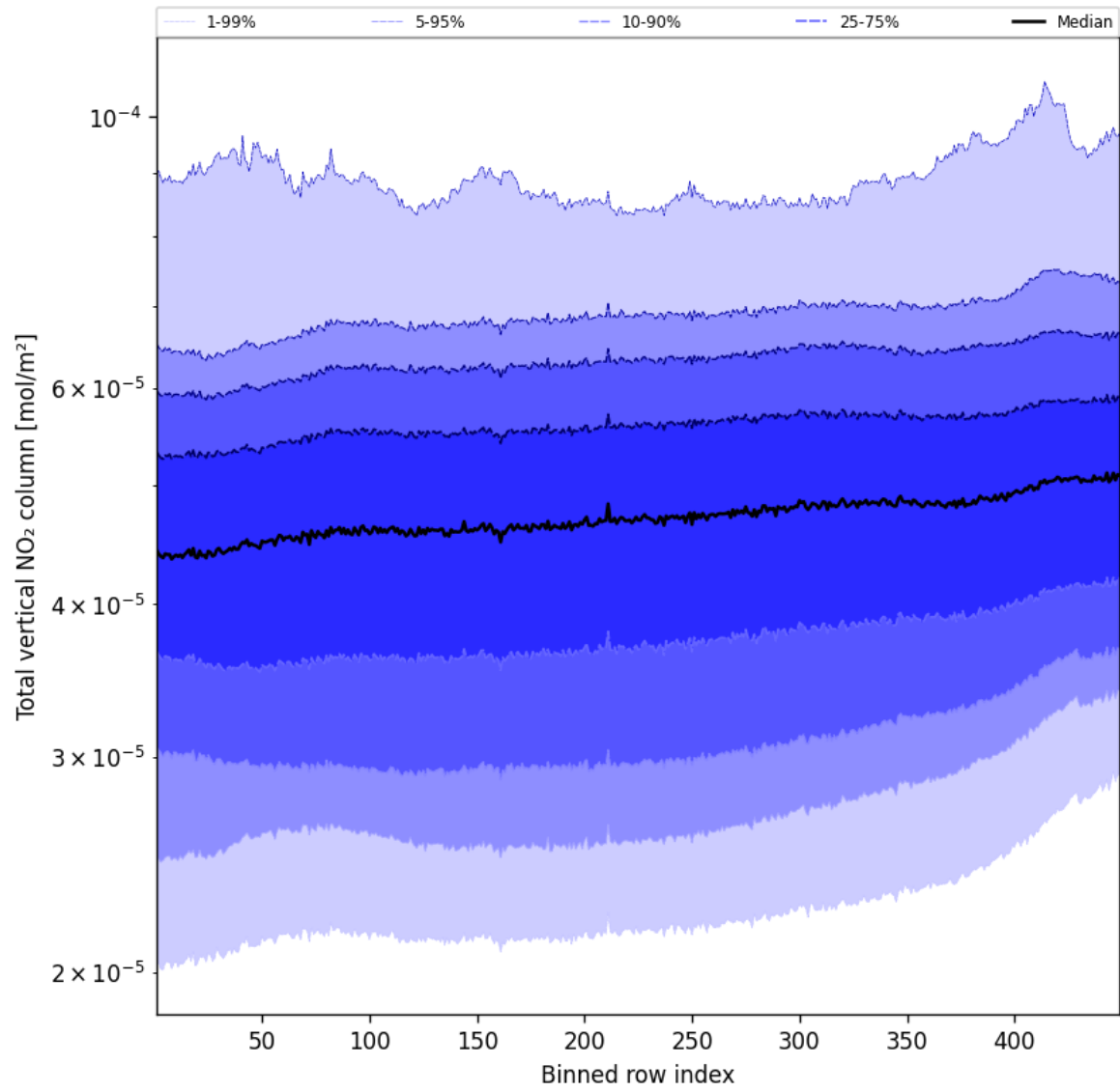
Figure 53: Along track statistics of “Total vertical NO 2 column” for 2025-09-30 to 2025-10-01
