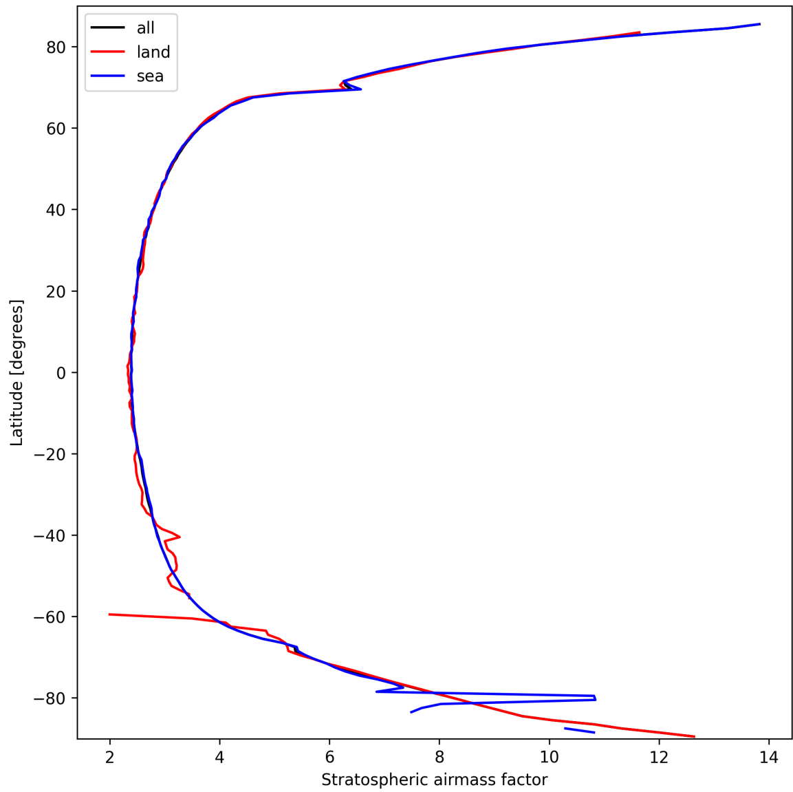
Figure 25: Zonal average of “Stratospheric air mass factor” for 2025-09-30 to 2025-10-01.
