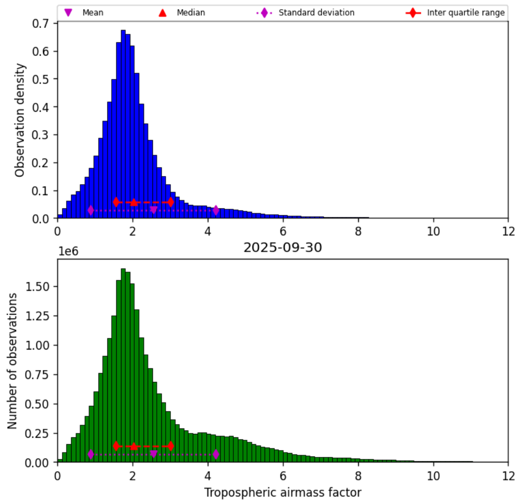
Figure 29: Histogram of “Tropospheric airmass factor” for 2025-09-30 to 2025-10-01
