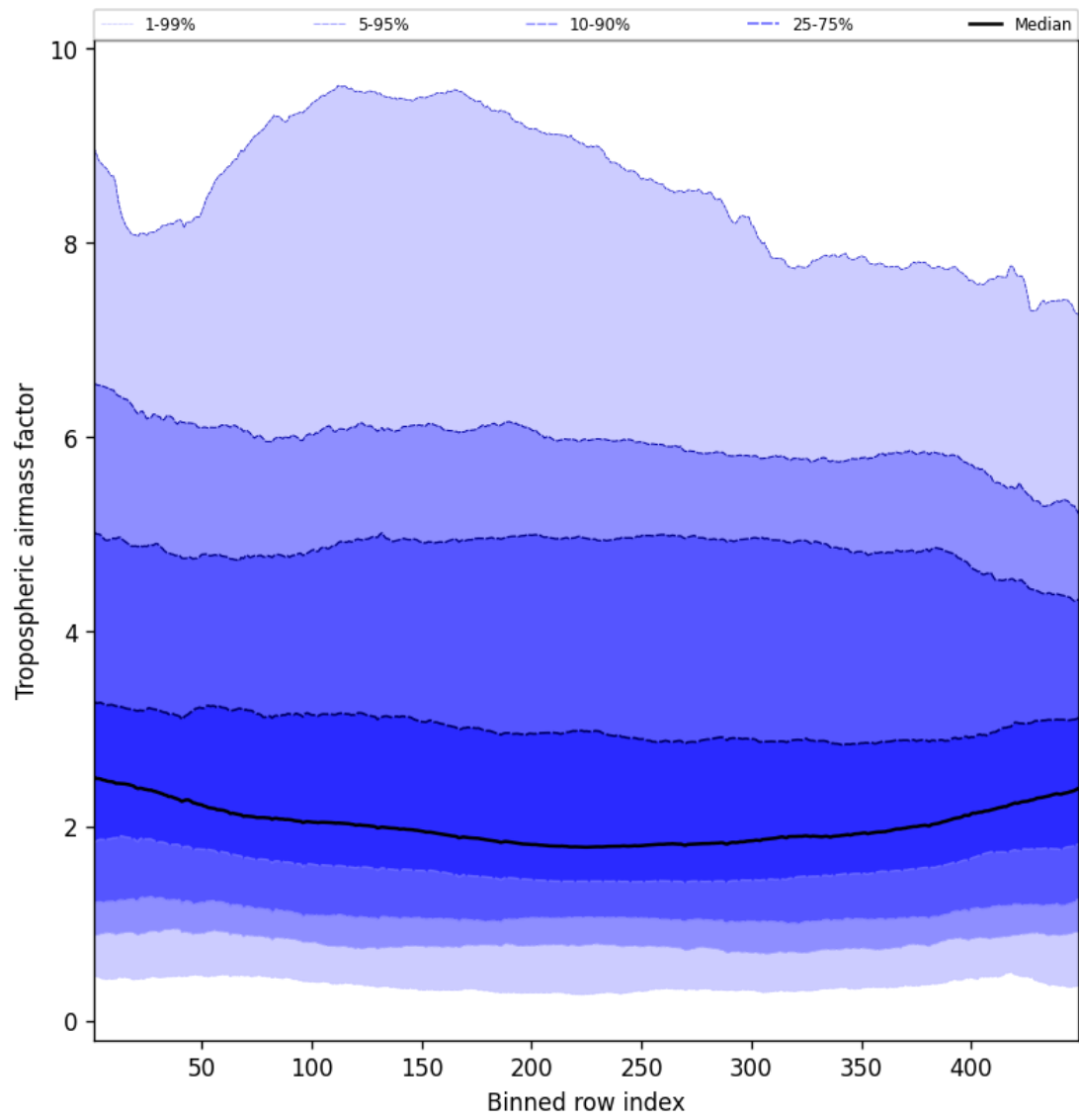
Figure 46: Along track statistics of “Tropospheric air mass factor” for 2025-09-30 to 2025-10-01
