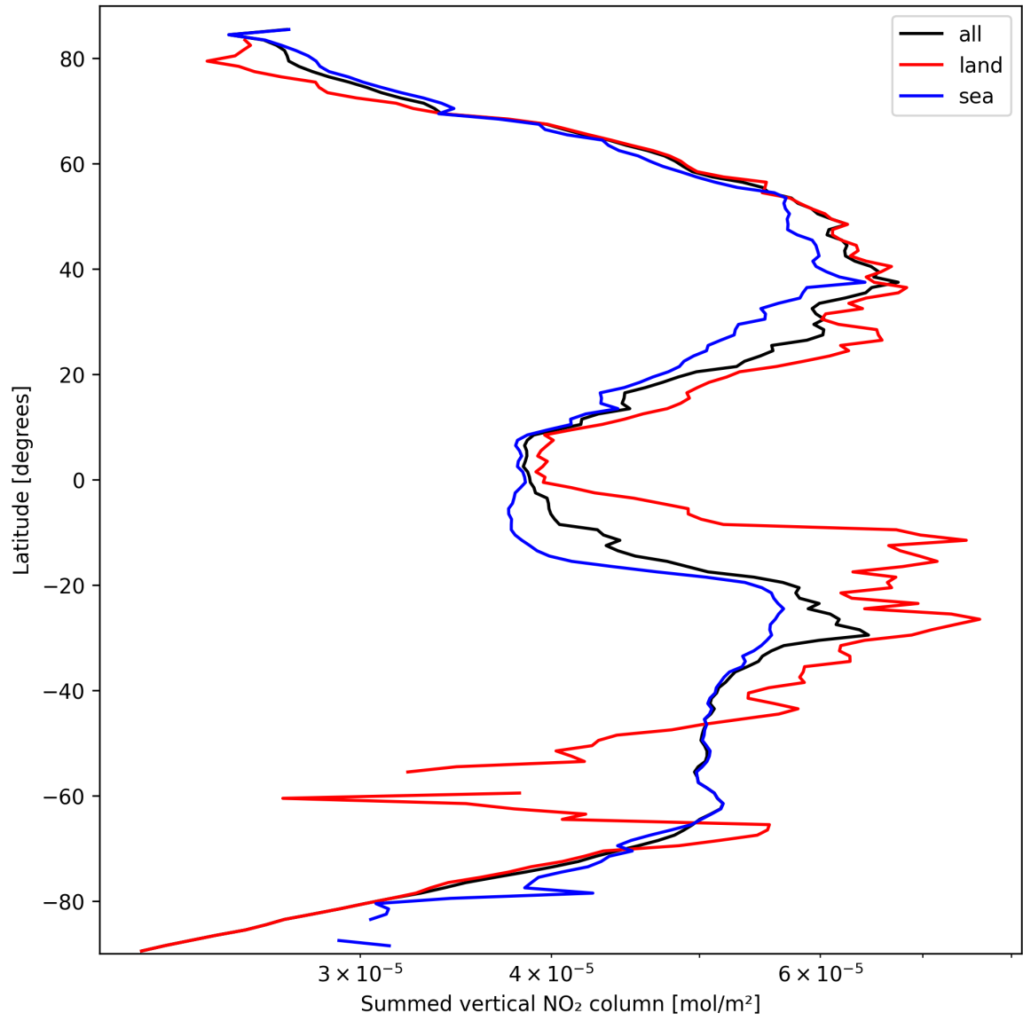
Figure 21: Zonal average of “Summed vertical NO 2 column” for 2025-09-30 to 2025-10-01.
