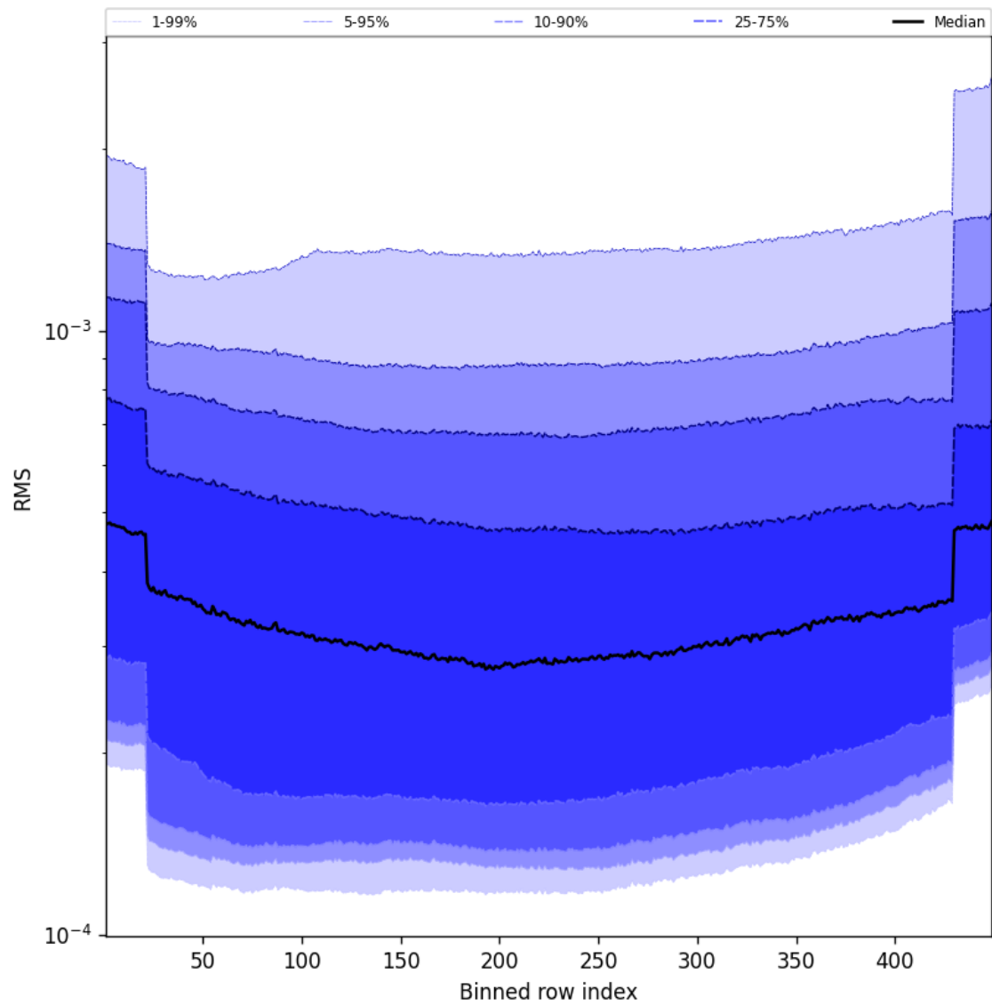
Figure 58: Along track statistics of “RMS” for 2025-09-30 to 2025-10-01
