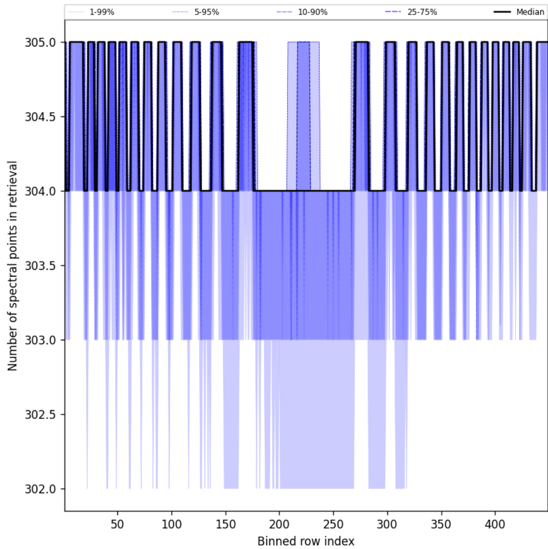
Figure 48: Along track statistics of “Number of spectral points in retrieval” for 2025-09-30 to 2025-10-01
