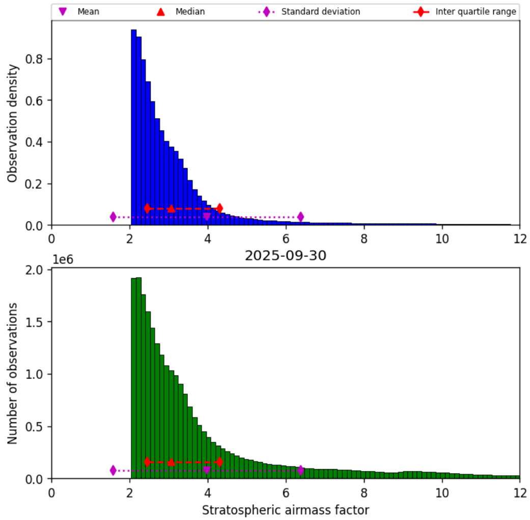
Figure 42: Histogram of “Stratospheric airmass factor” for 2025-09-30 to 2025-10-01
