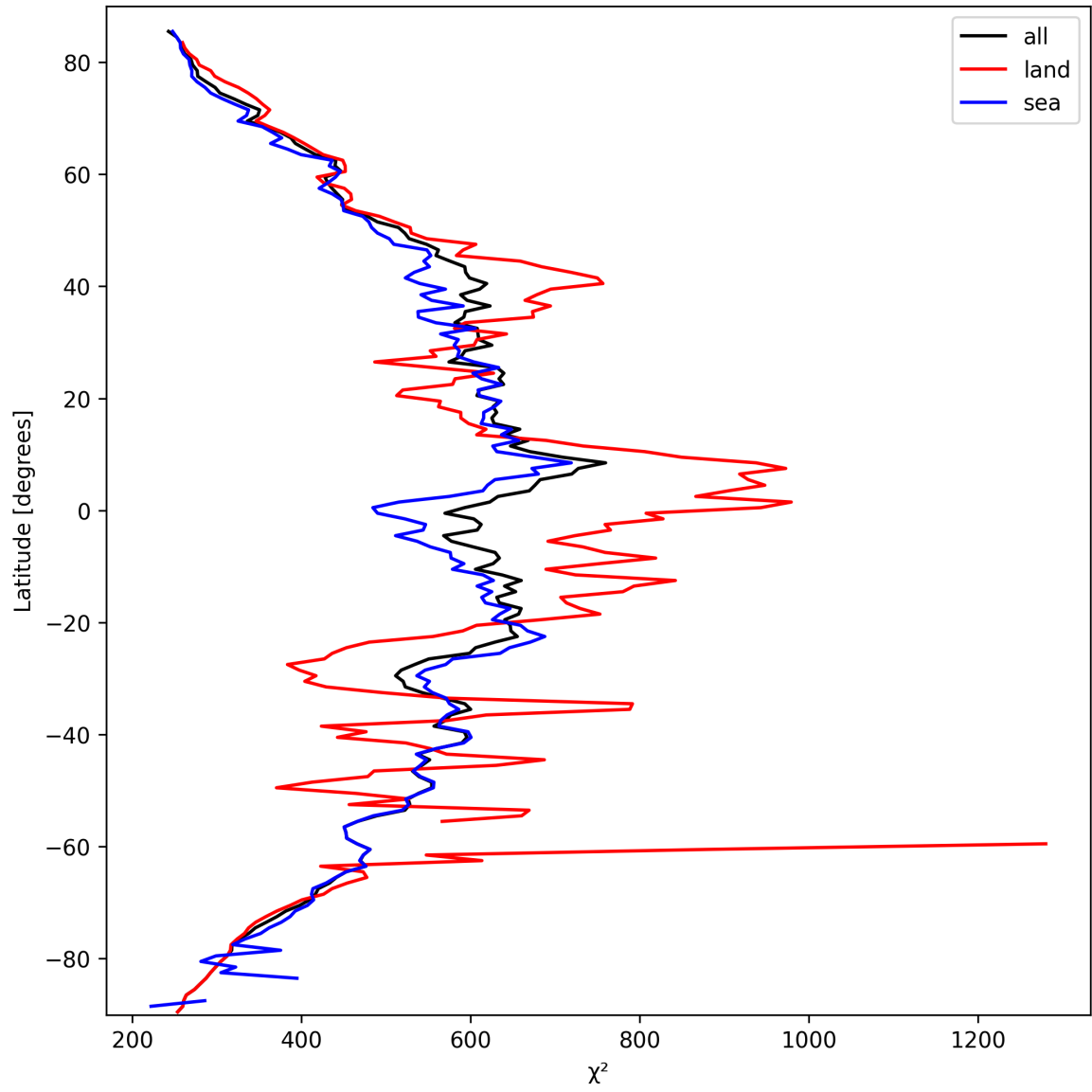
Figure 23: Zonal average of “ \chi^2 ” for 2025-09-30 to 2025-10-01.
