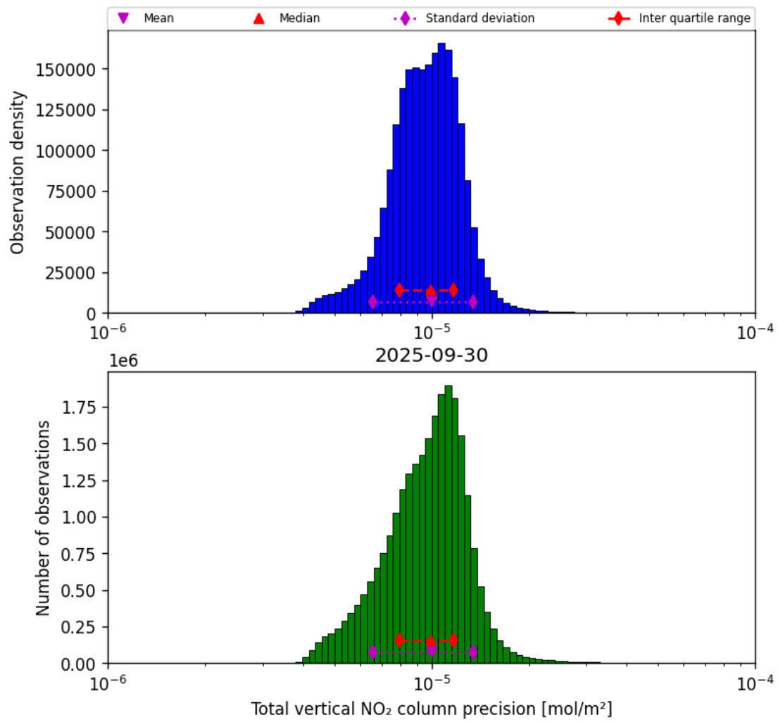
Figure 37: Histogram of "Total vertical NO 2 column precision" for 2025-09-30 to 2025-10-01
