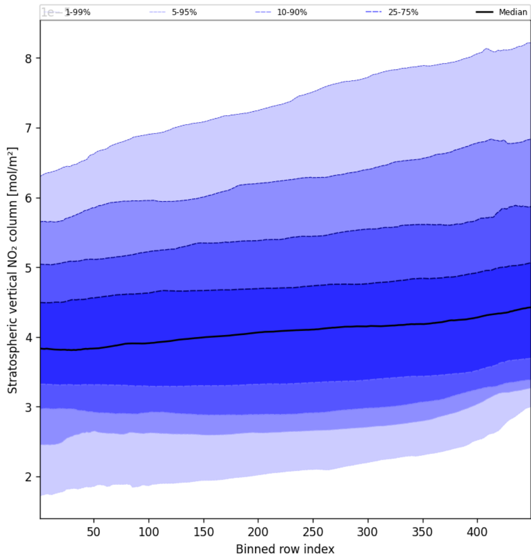
Figure 51: Along track statistics of “Stratospheric vertical NO 2 column” for 2025-09-30 to 2025-10-01
