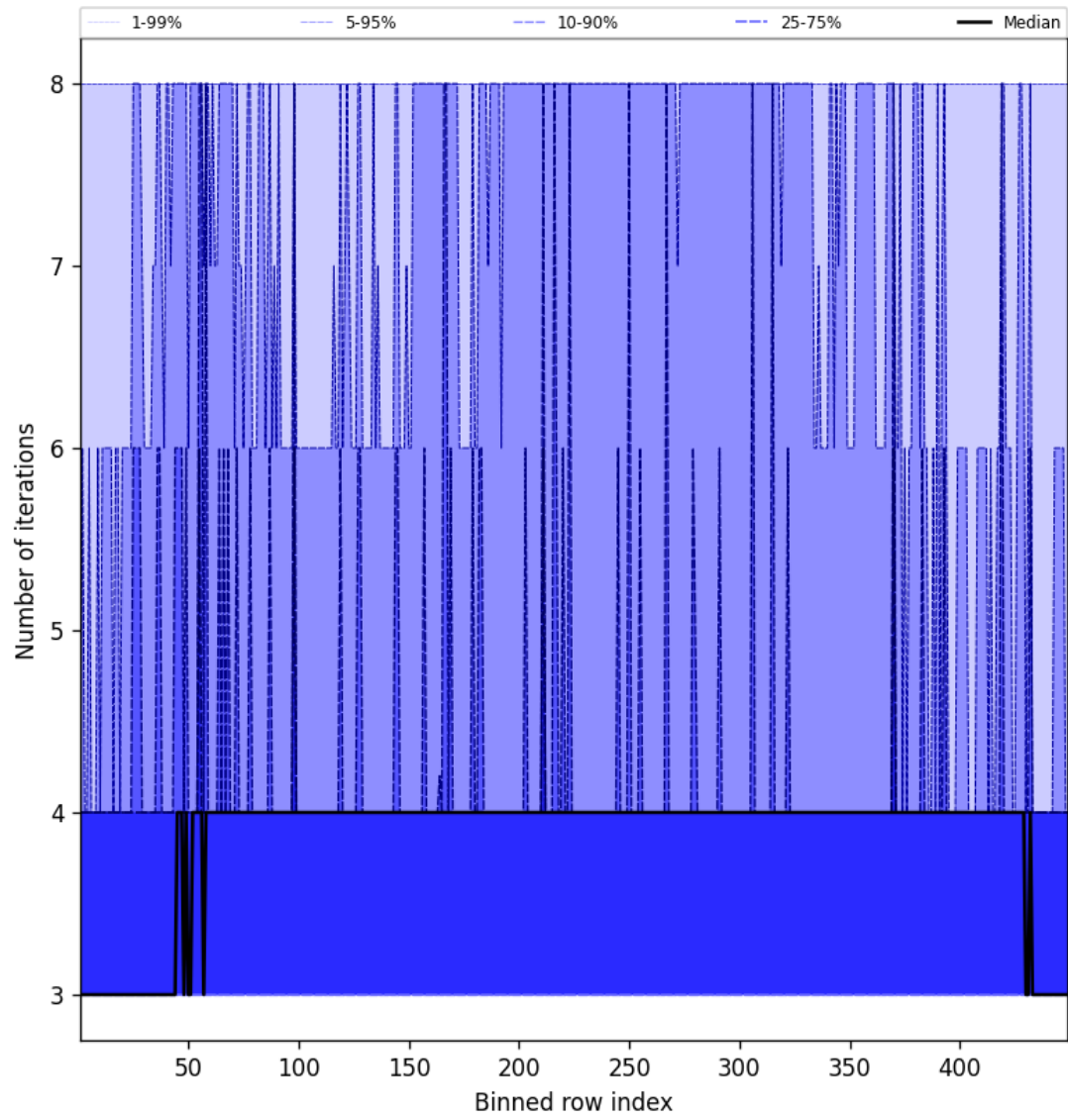
Figure 49: Along track statistics of “Number of iterations” for 2025-09-30 to 2025-10-01
