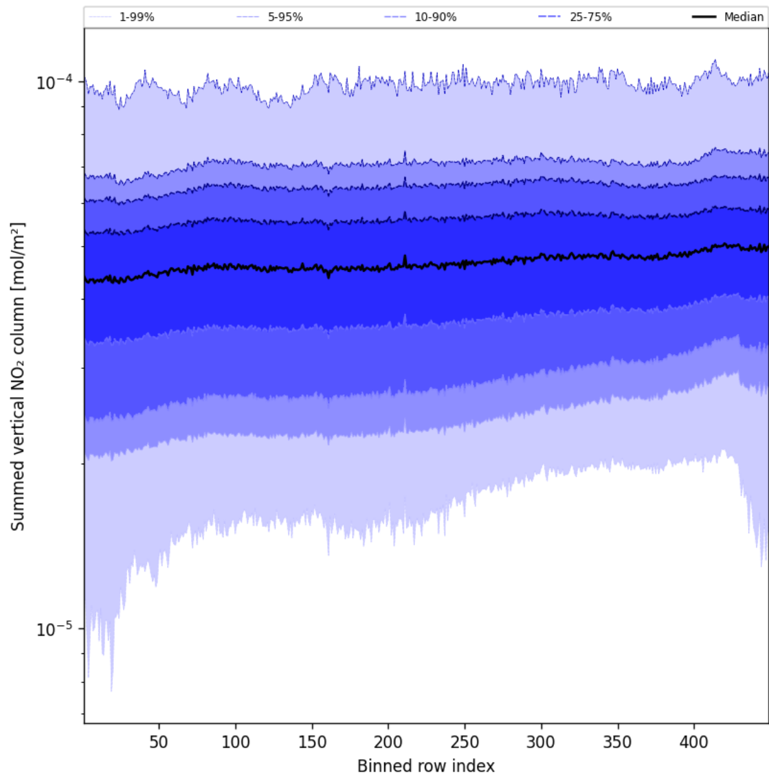
Figure 55: Along track statistics of “Summed vertical NO 2 column” for 2025-09-30 to 2025-10-01
