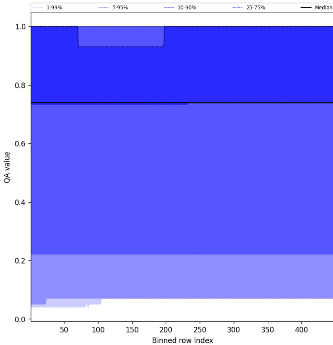
Figure 43: Along track statistics of “QA value” for 2025-09-30 to 2025-10-01
