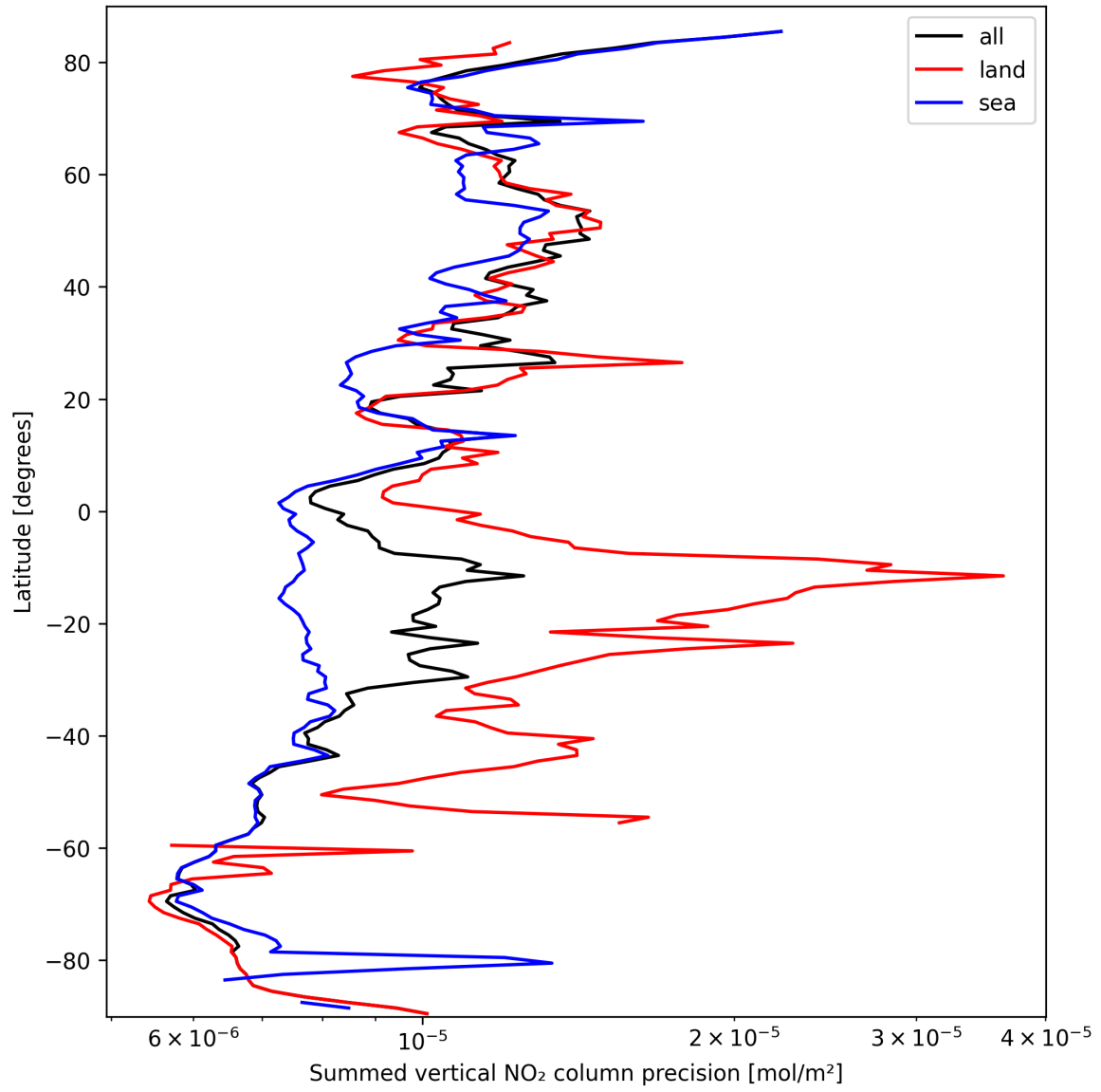
Figure 22: Zonal average of “Summed vertical NO 2 column precision” for 2025-09-30 to 2025-10-01.
