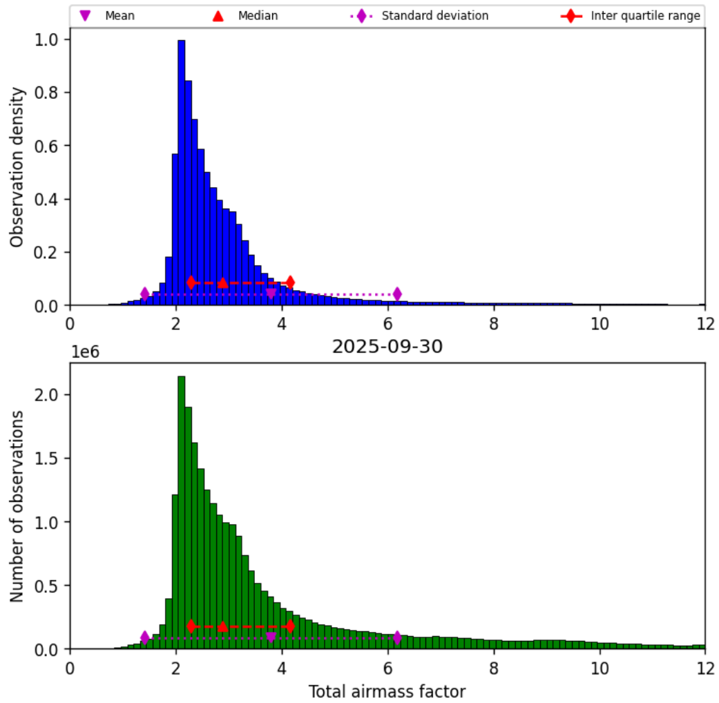
Figure 30: Histogram of “Total airmass factor” for 2025-09-30 to 2025-10-01
