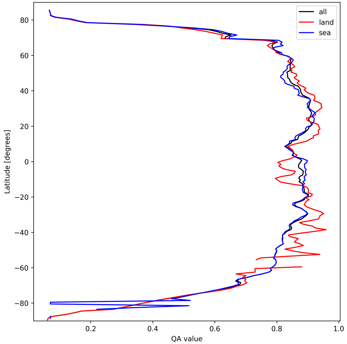
Figure 9: Zonal average of “QA value” for 2025-09-30 to 2025-10-01.
