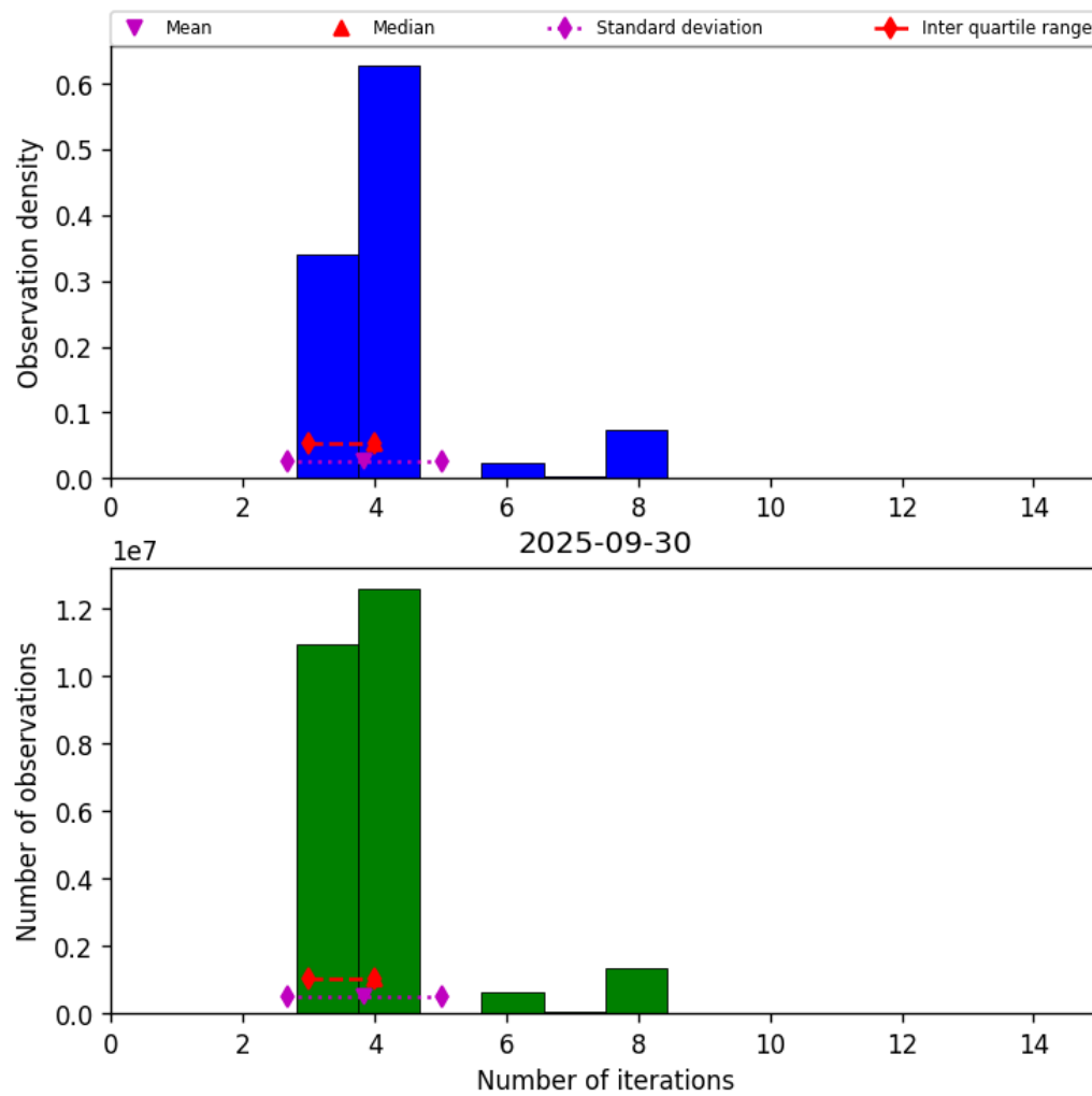
Figure 32: Histogram of “Number of iterations” for 2025-09-30 to 2025-10-01
