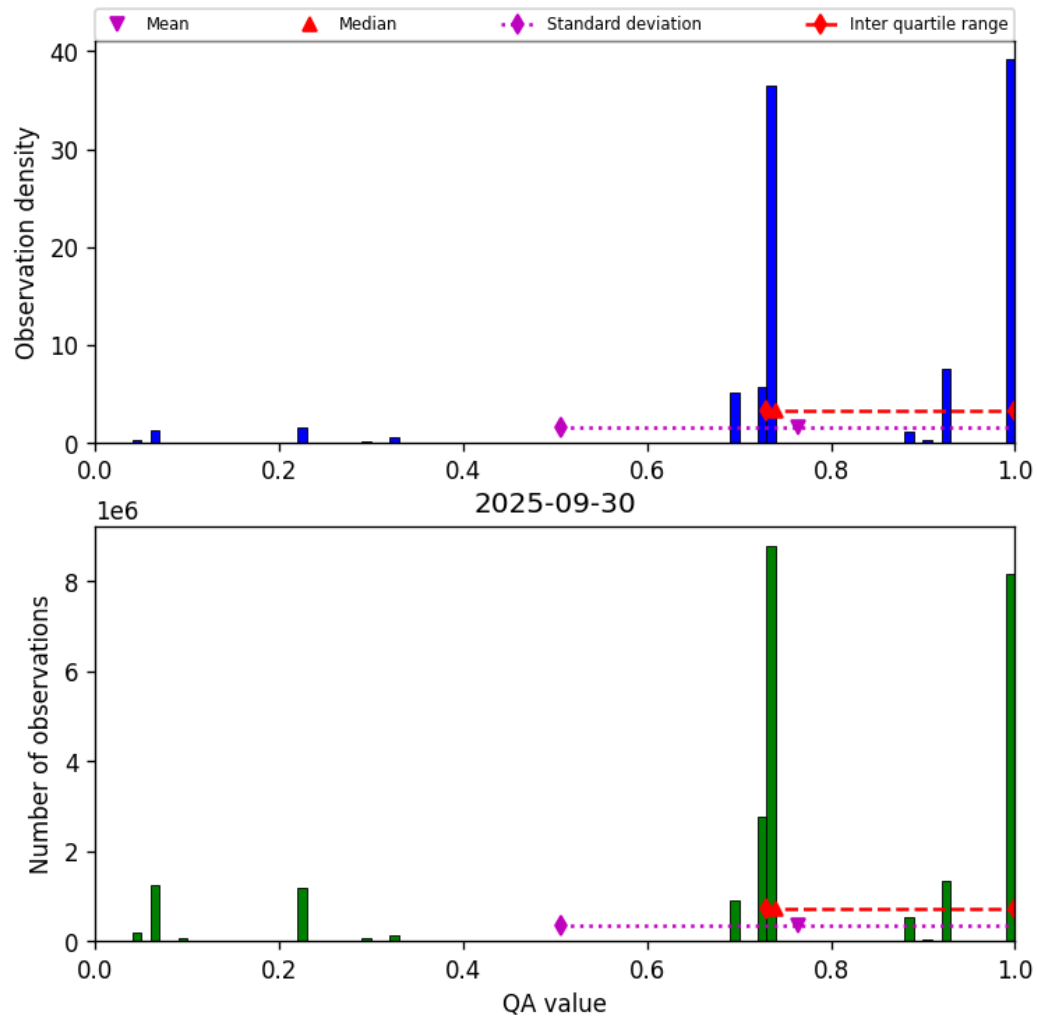
Figure 26: Histogram of “QA value” for 2025-09-30 to 2025-10-01
