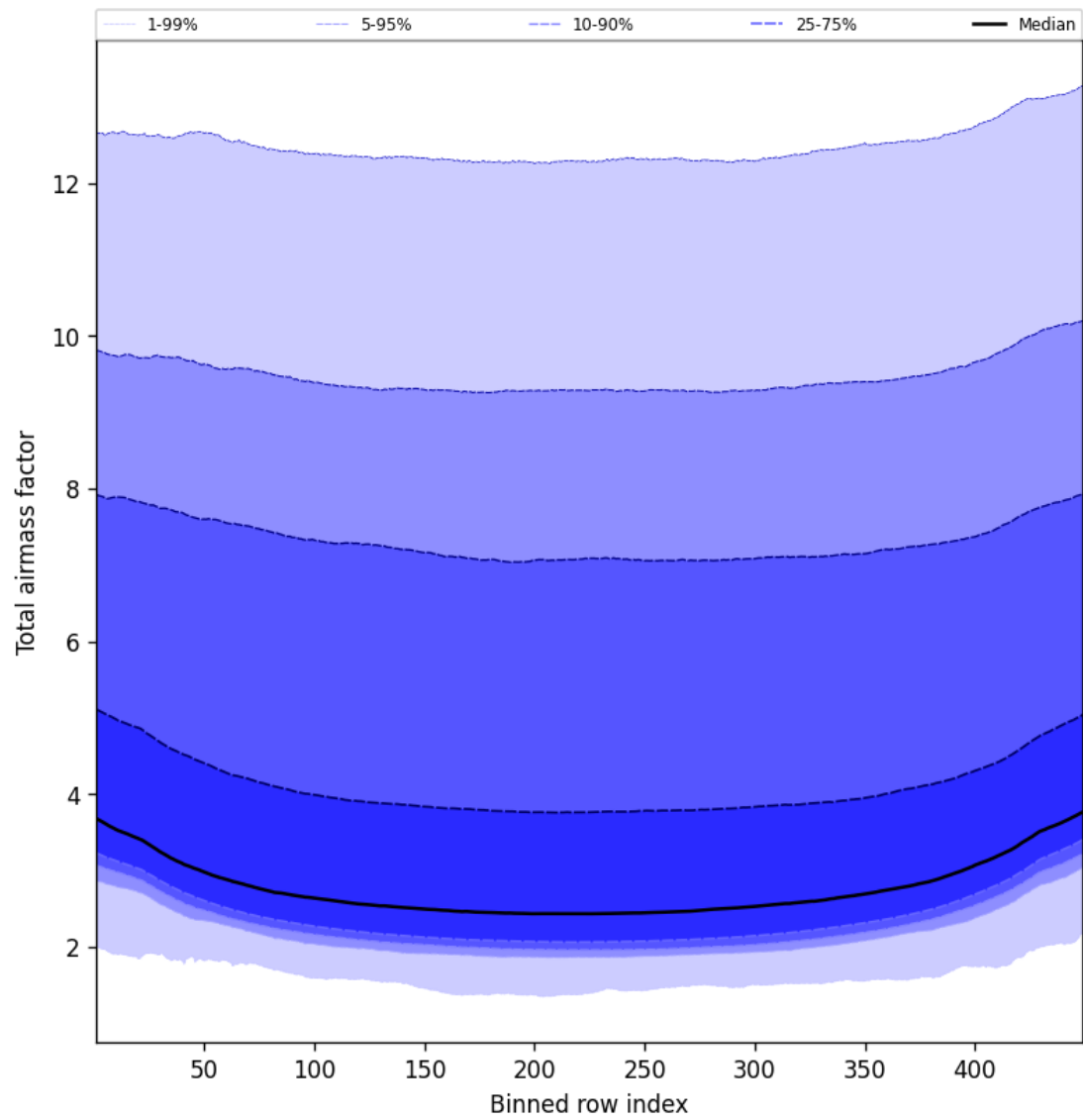
Figure 47: Along track statistics of “Total airmass factor” for 2025-09-30 to 2025-10-01
