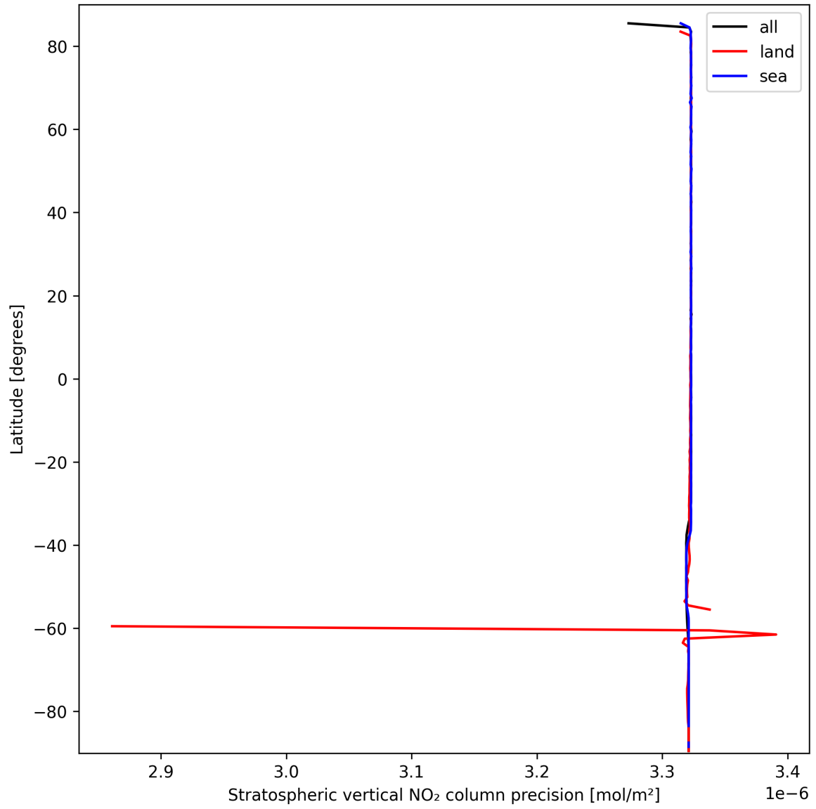
Figure 18: Zonal average of “Stratospheric vertical NO 2 column precision” for 2025-09-30 to 2025-10-01.
