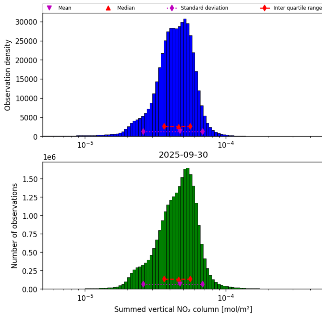
Figure 38: Histogram of “Summed vertical NO 2 column” for 2025-09-30 to 2025-10-01
