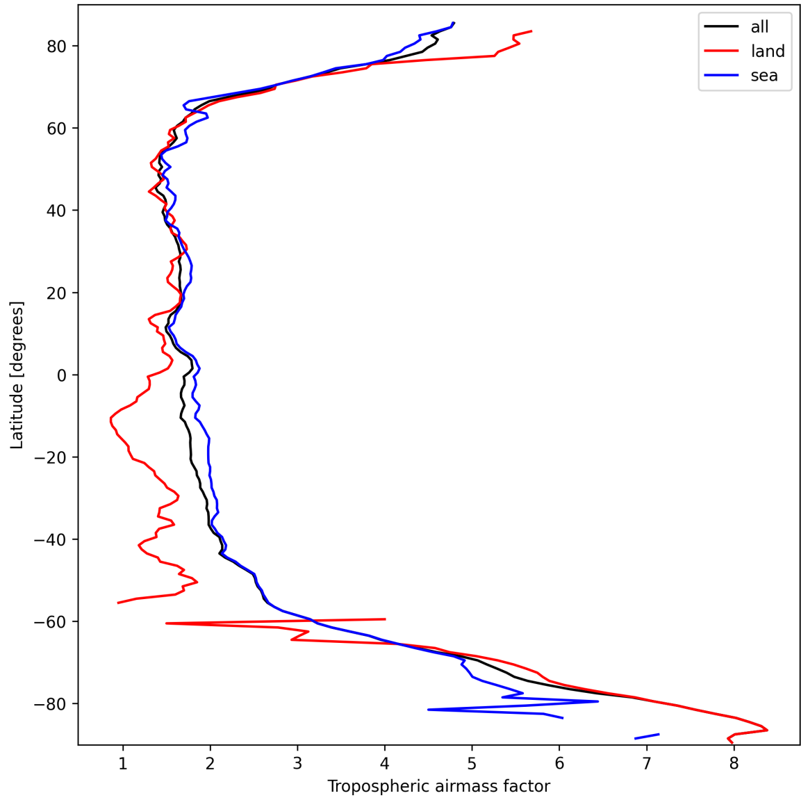
Figure 12: Zonal average of “Tropospheric airmass factor” for 2025-09-30 to 2025-10-01.
