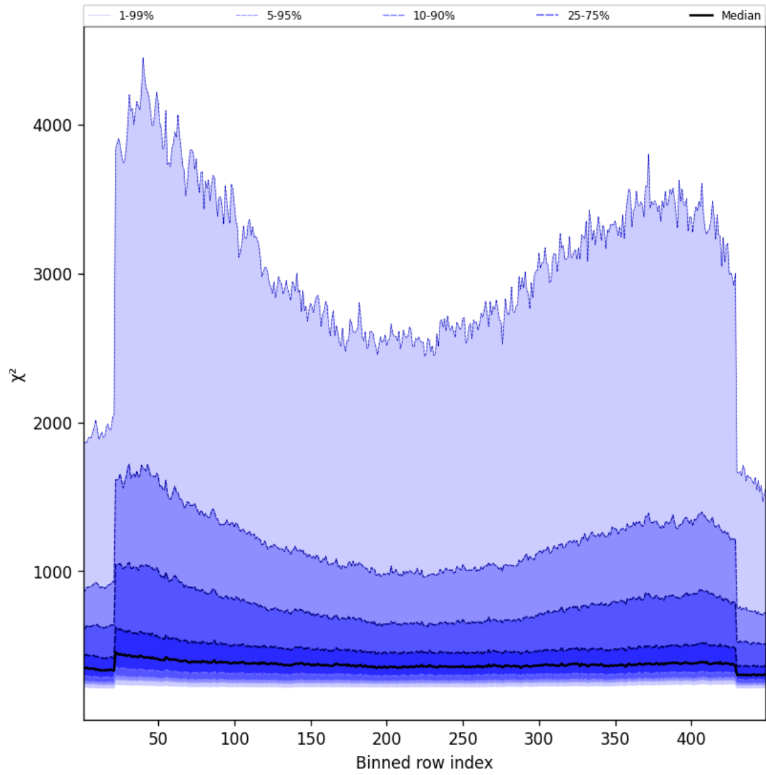
Figure 57: Along track statistics of “ \chi^2 ” for 2025-09-30 to 2025-10-01
