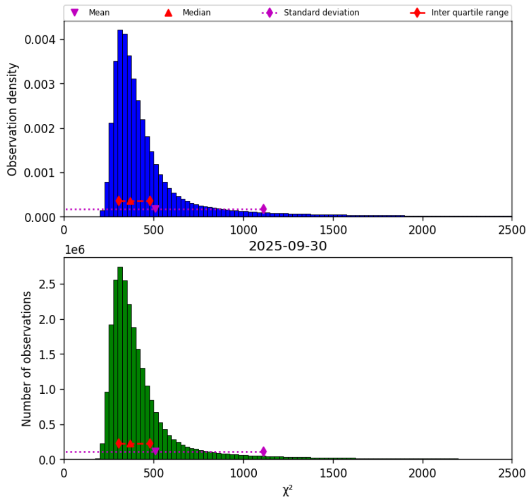
Figure 40: Histogram of “ \chi^2 ” for 2025-09-30 to 2025-10-01
