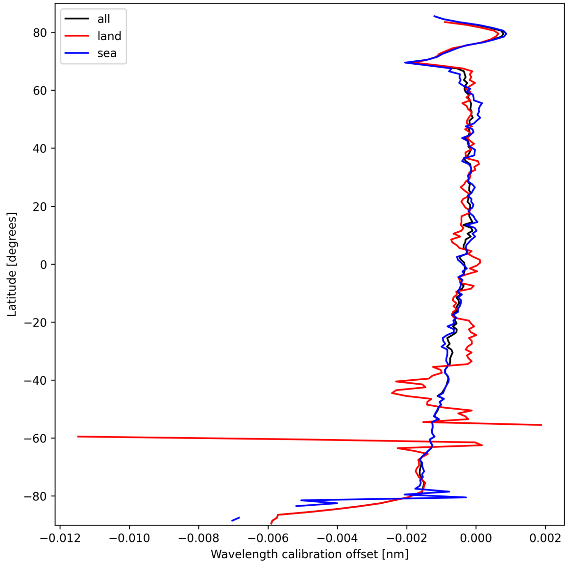
Figure 16: Zonal average of “Wavelength calibration offset” for 2025-09-30 to 2025-10-01.
