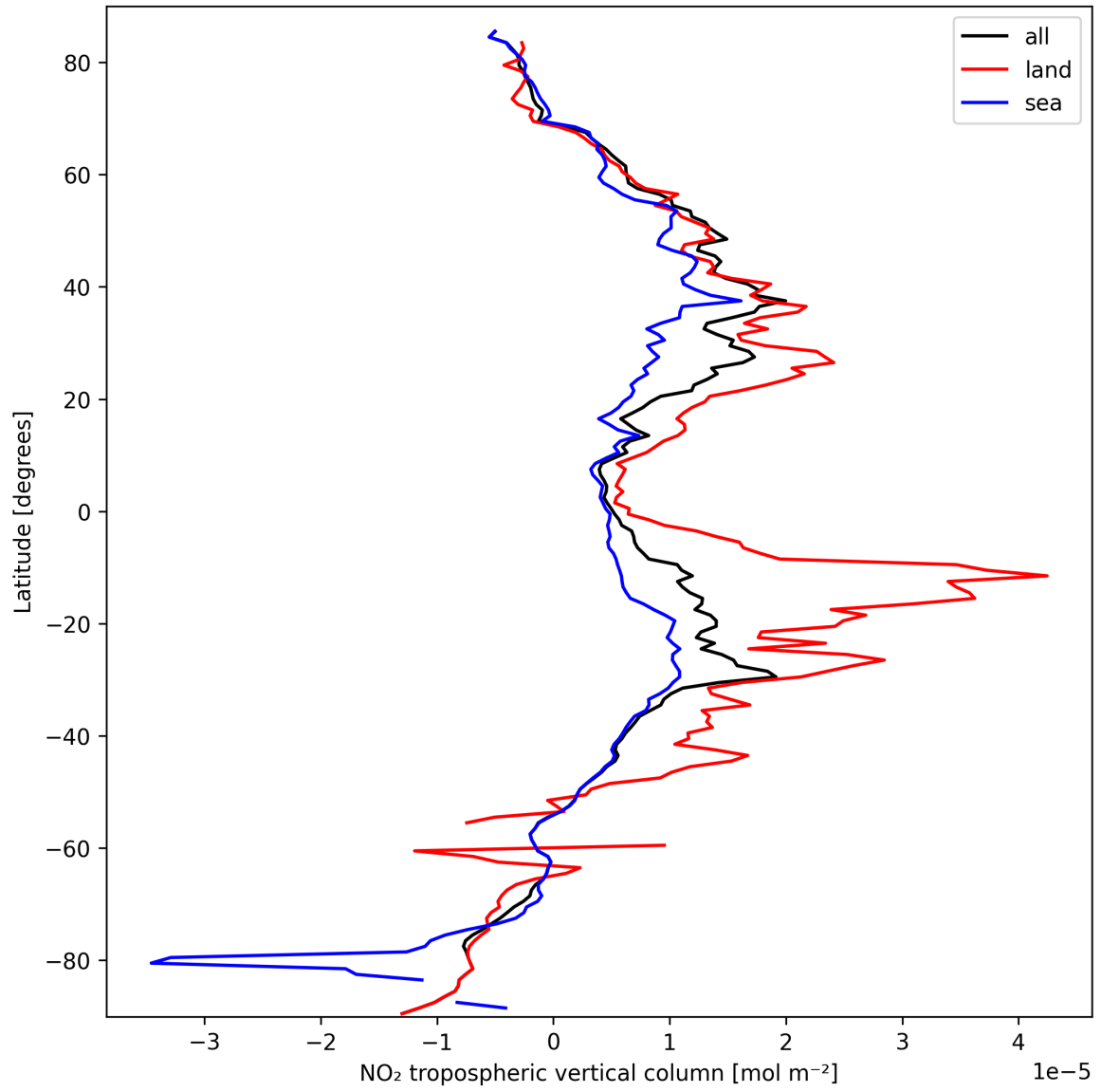
Figure 10: Zonal average of “NO 2 tropospheric vertical column” for 2025-09-30 to 2025-10-01.
