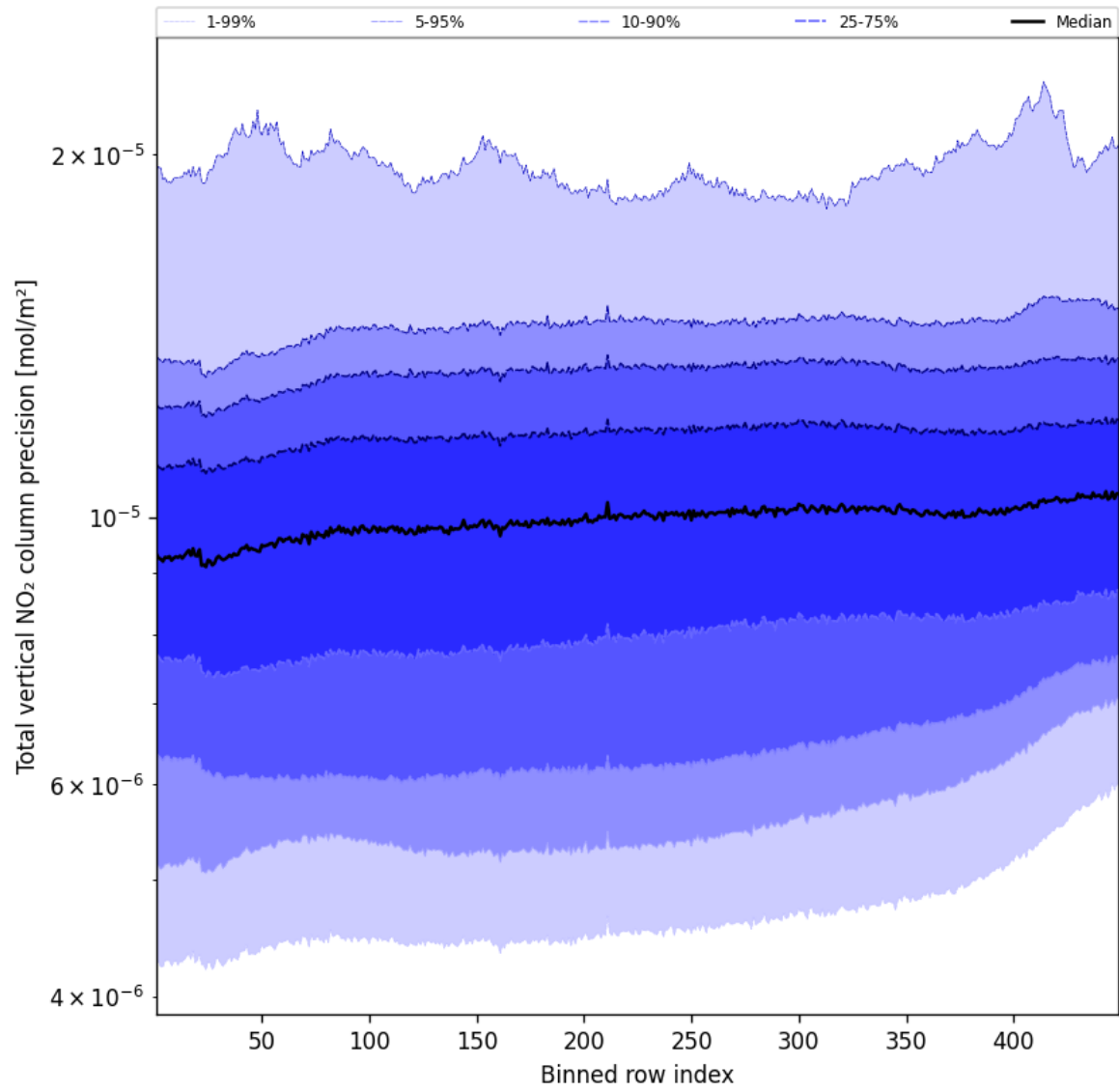
Figure 54: Along track statistics of “Total vertical NO 2 column precision” for 2025-09-30 to 2025-10-01
