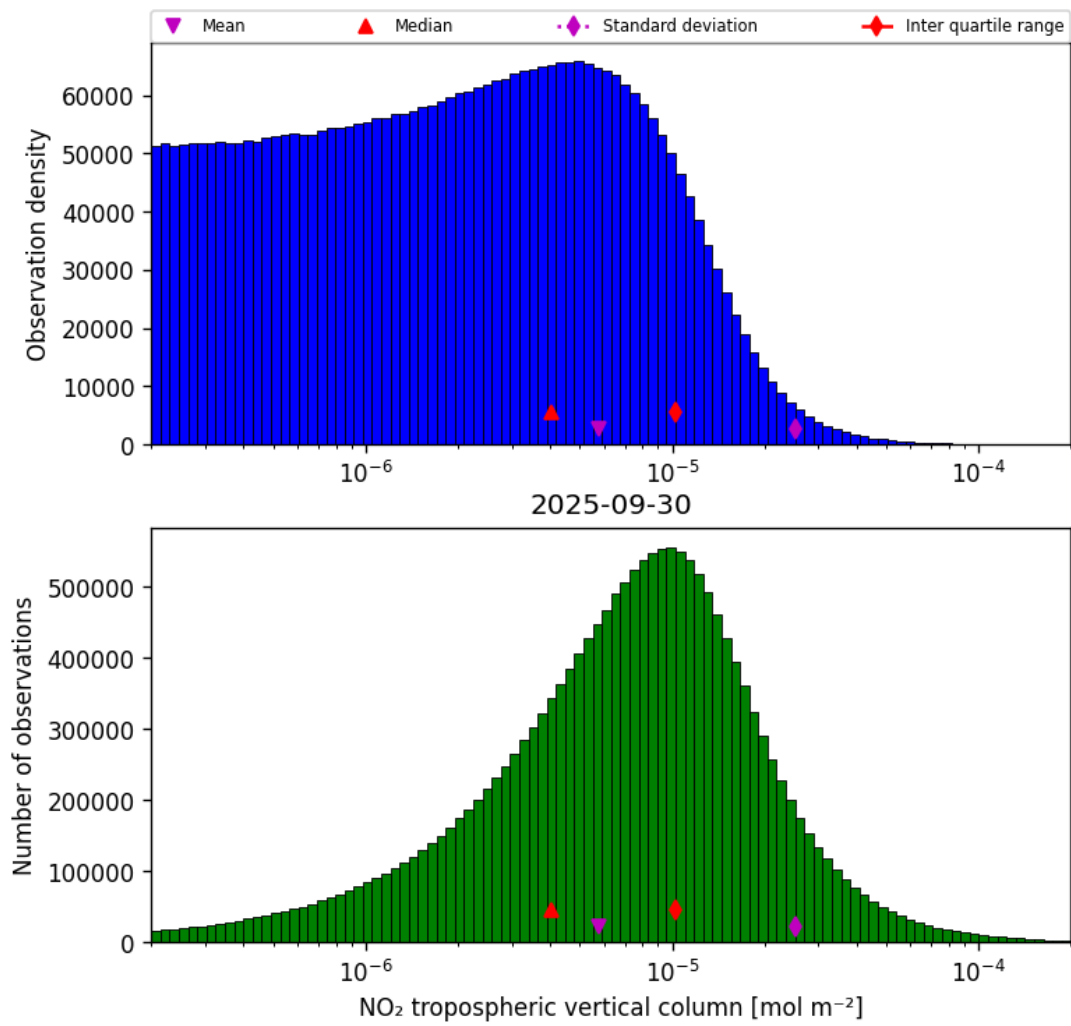
Figure 27: Histogram of “NO 2 tropospheric vertical column” for 2025-09-30 to 2025-10-01
