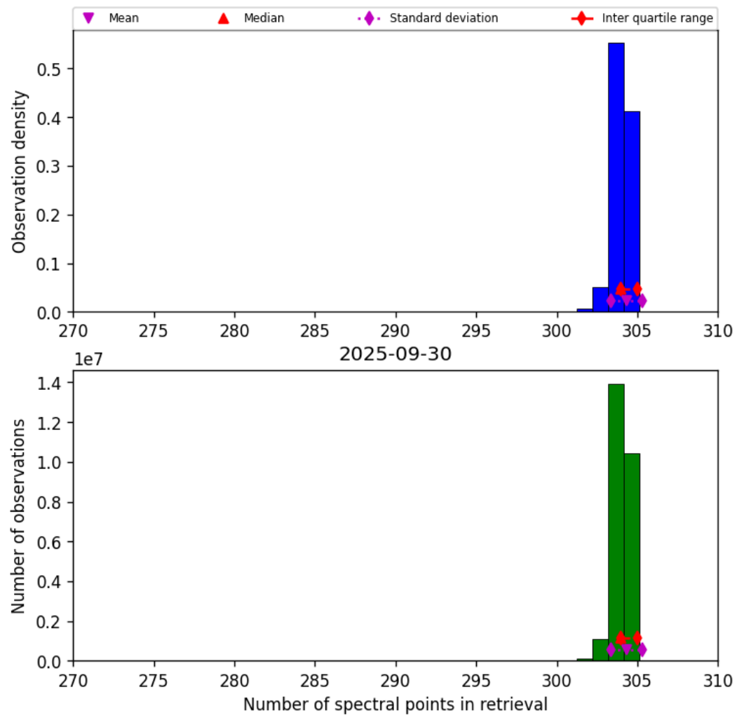
Figure 31: Histogram of “Number of spectral points in retrieval” for 2025-09-30 to 2025-10-01
