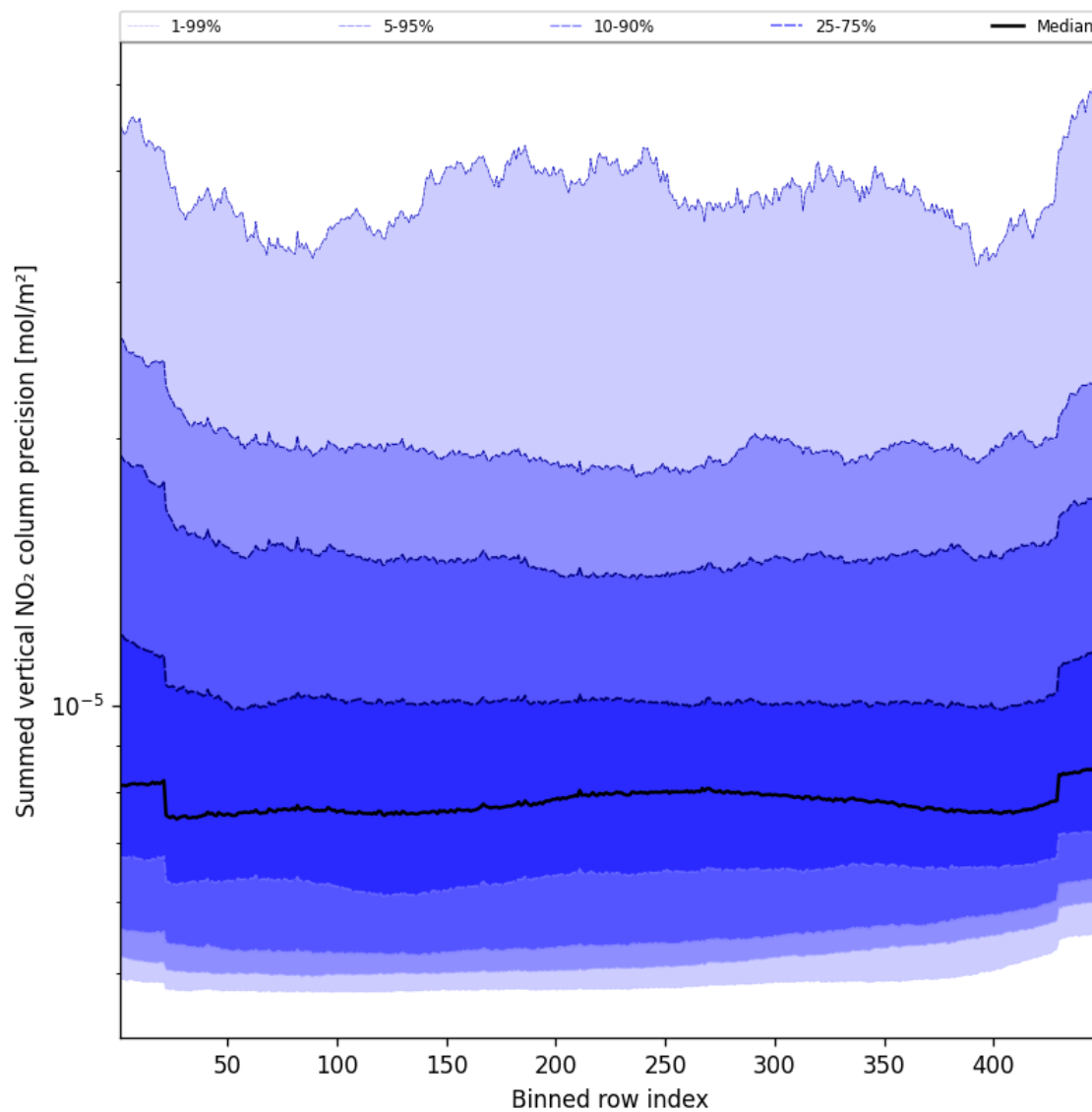
Figure 56: Along track statistics of “Summed vertical NO 2 column precision” for 2025-09-30 to 2025-10-01
