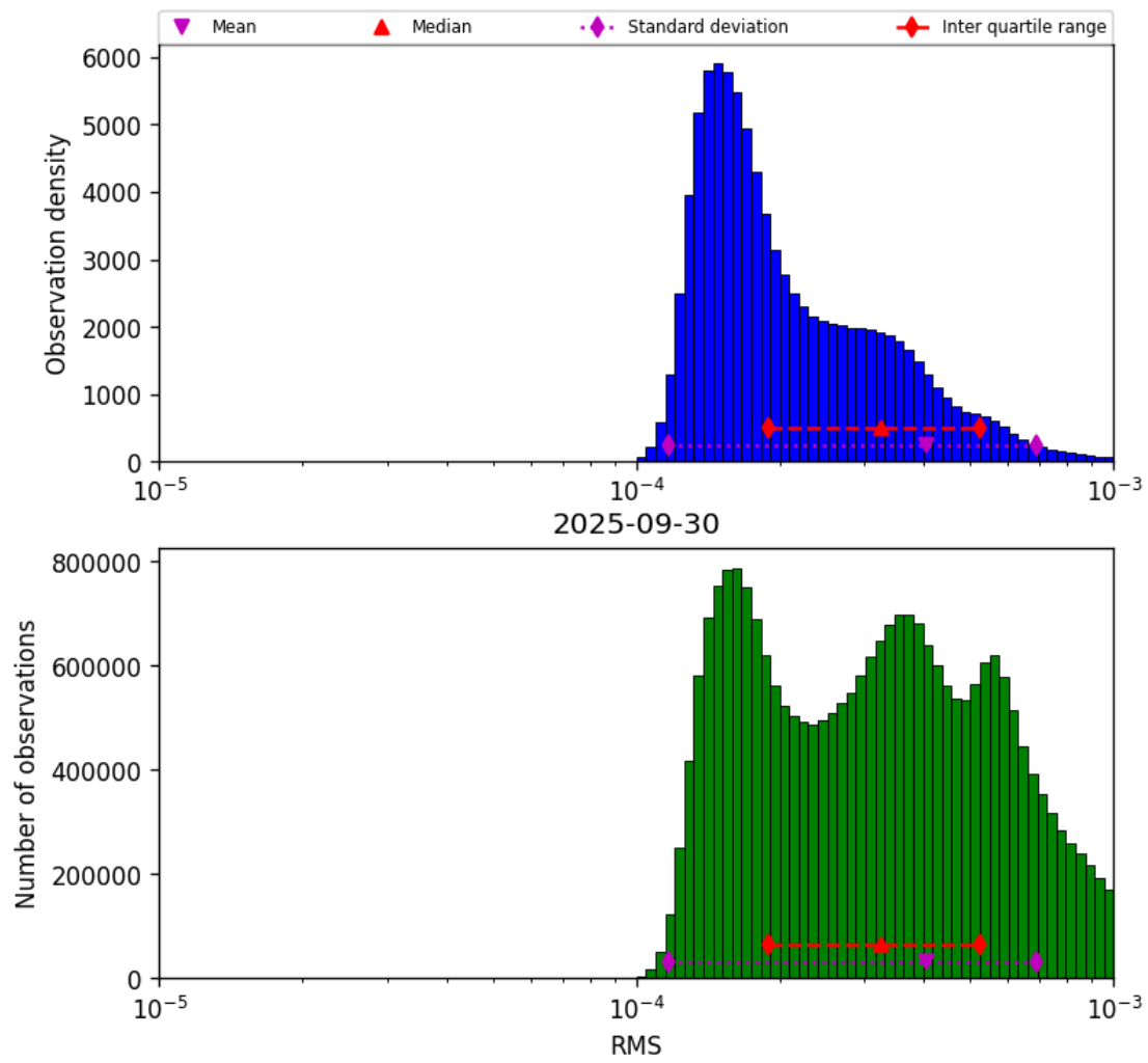
Figure 41: Histogram of “RMS” for 2025-09-30 to 2025-10-01
