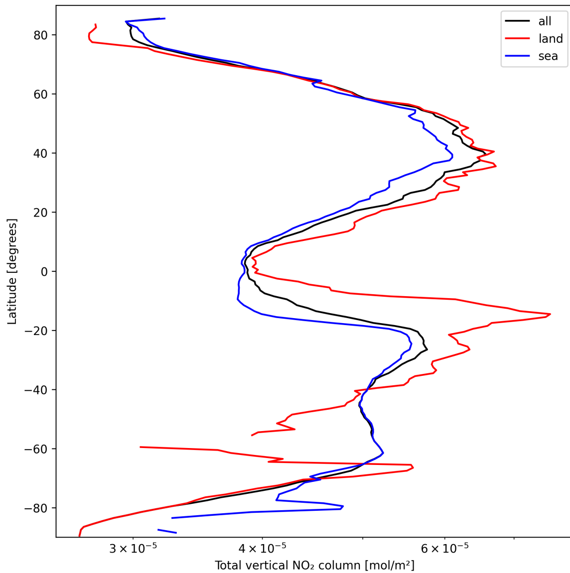
Figure 19: Zonal average of “Total vertical NO 2 column” for 2025-09-30 to 2025-10-01.
