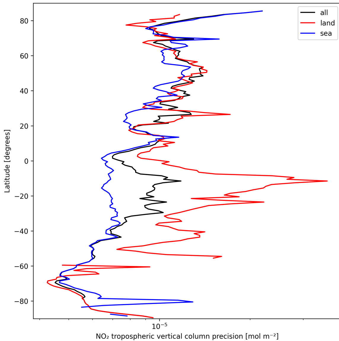
Figure 11: Zonal average of “NO 2 tropospheric vertical column precision” for 2025-09-30 to 2025-10-01.
