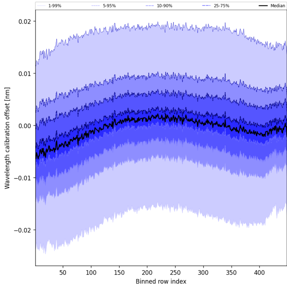
Figure 50: Along track statistics of “Wavelength calibration offset” for 2025-09-30 to 2025-10-01
