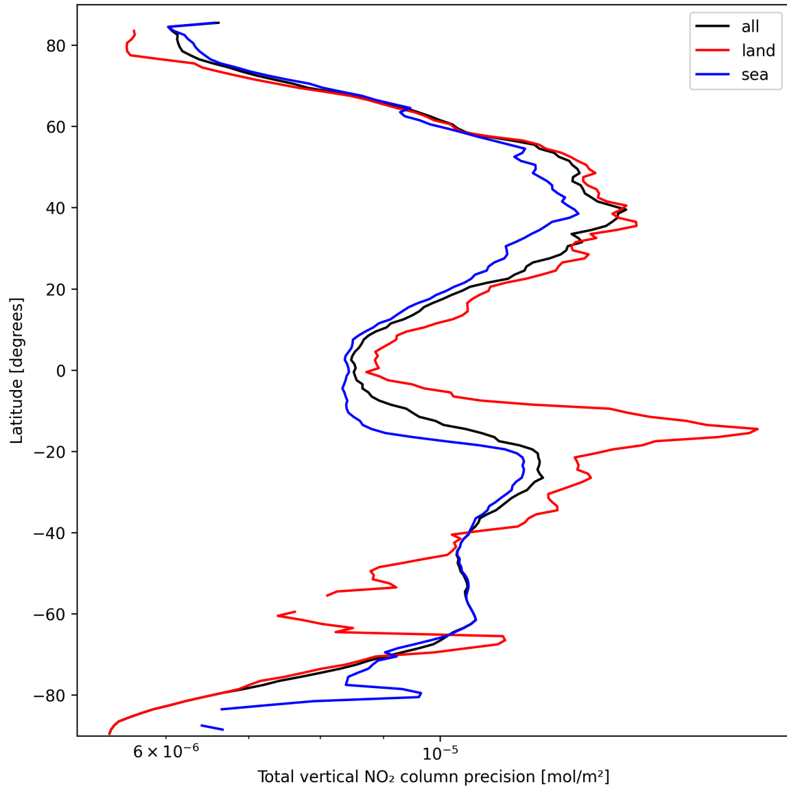
Figure 20: Zonal average of “Total vertical NO 2 column precision” for 2025-09-30 to 2025-10-01.
