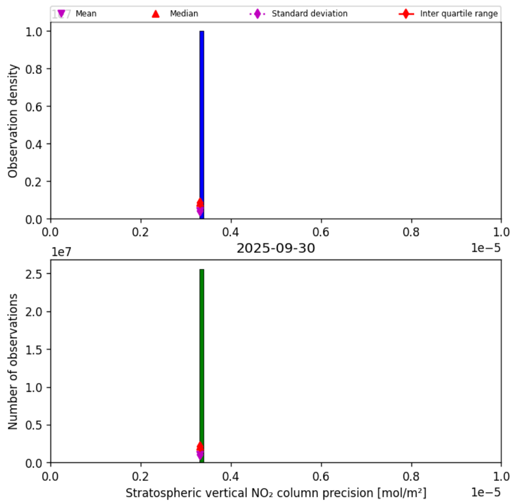
Figure 35: Histogram of “Stratospheric vertical NO 2 column precision” for 2025-09-30 to 2025-10-01
