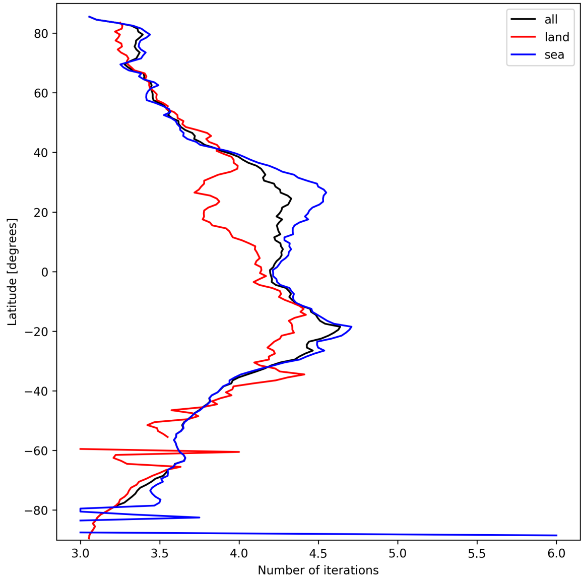
Figure 15: Zonal average of “Number of iterations” for 2025-09-30 to 2025-10-01.
