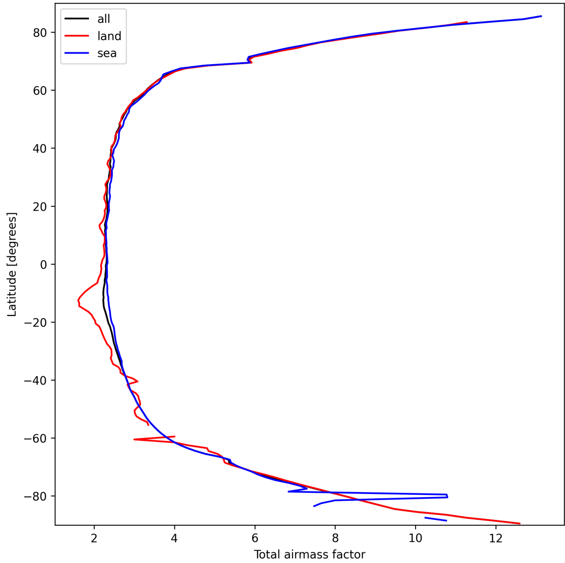
Figure 13: Zonal average of “Total airmass factor” for 2025-09-30 to 2025-10-01.
