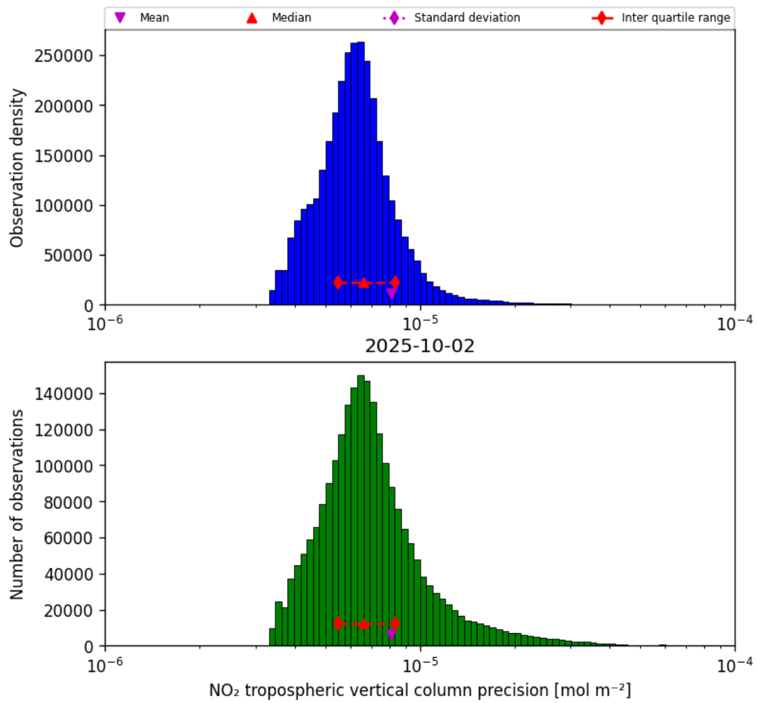
Figure 28: Histogram of “NO 2 tropospheric vertical column precision” for 2025-10-02 to 2025-10-03
