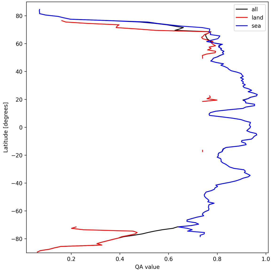
Figure 9: Zonal average of “QA value” for 2025-10-02 to 2025-10-03.
