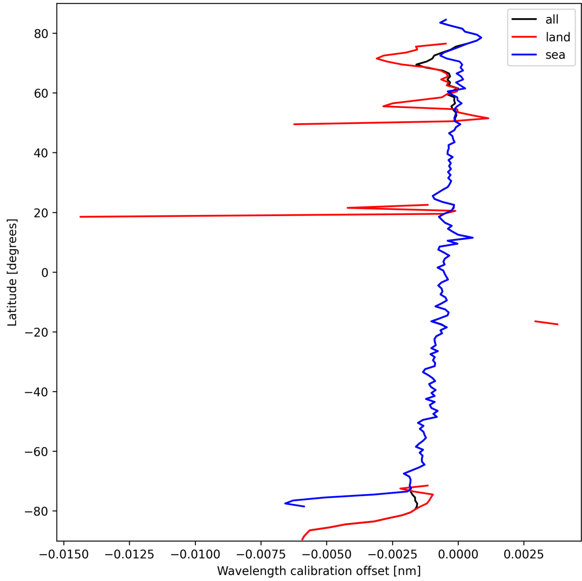
Figure 16: Zonal average of “Wavelength calibration offset” for 2025-10-02 to 2025-10-03.
