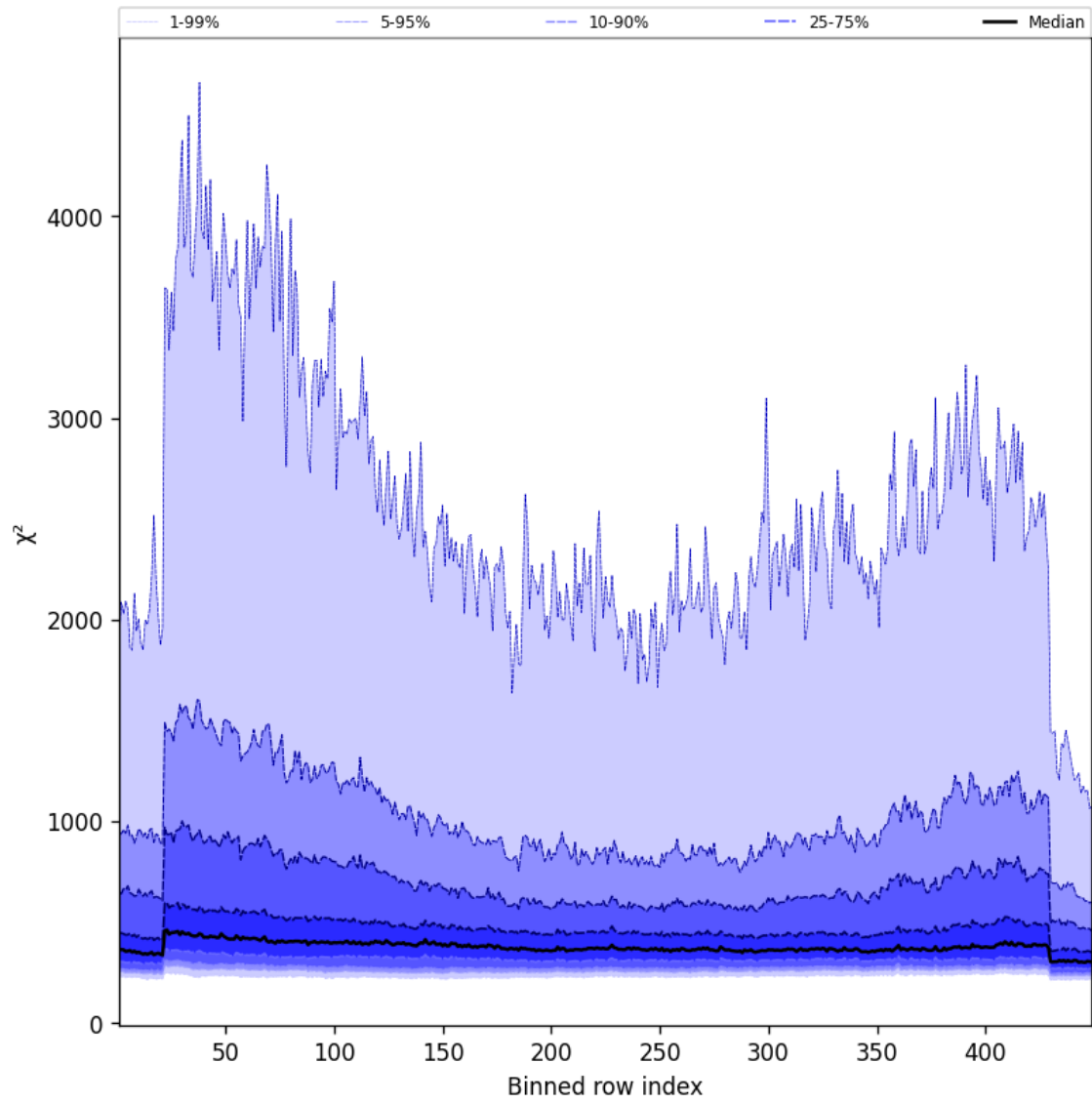
Figure 57: Along track statistics of “ \chi^2 ” for 2025-10-02 to 2025-10-03
