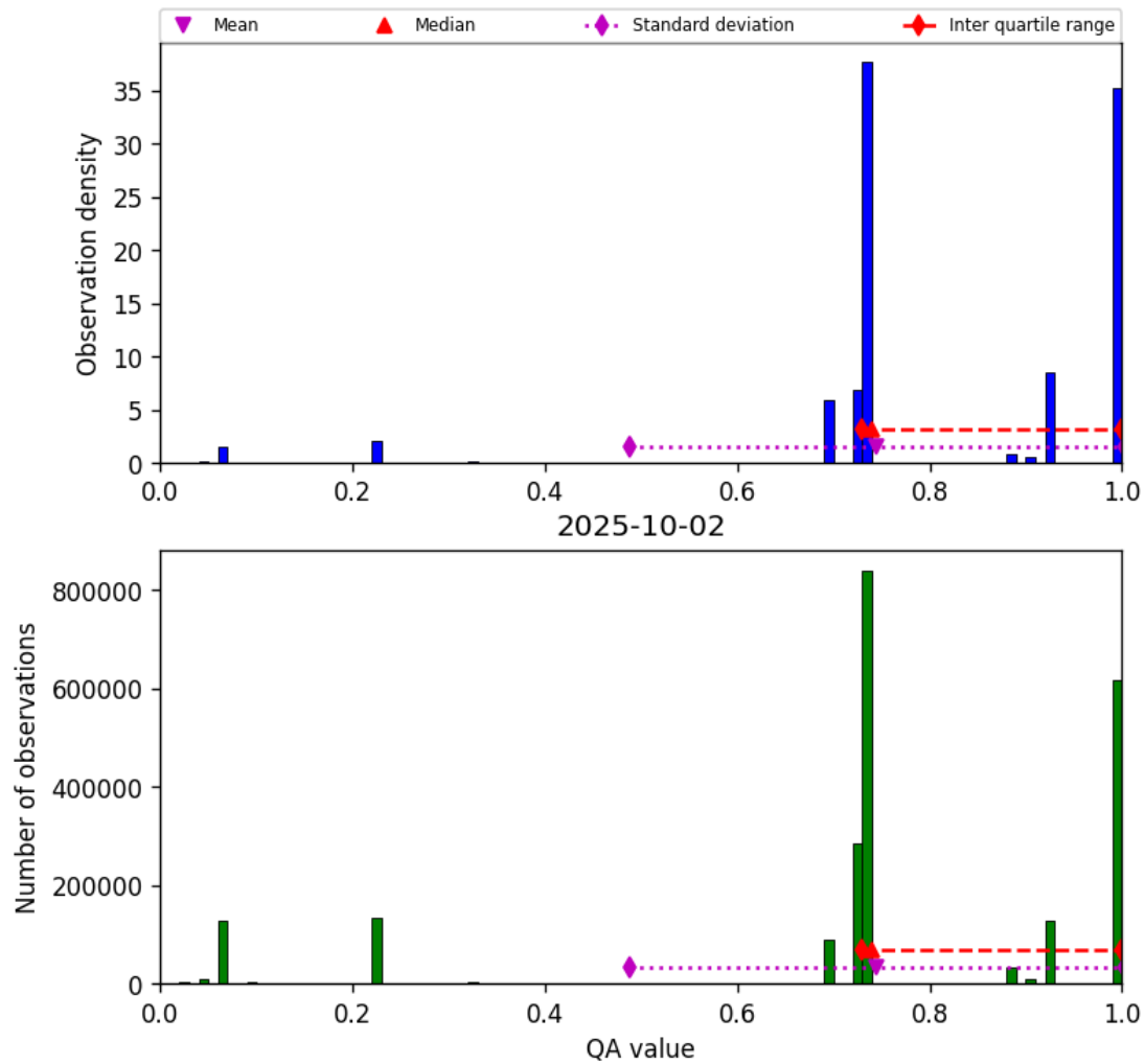
Figure 26: Histogram of “QA value” for 2025-10-02 to 2025-10-03
