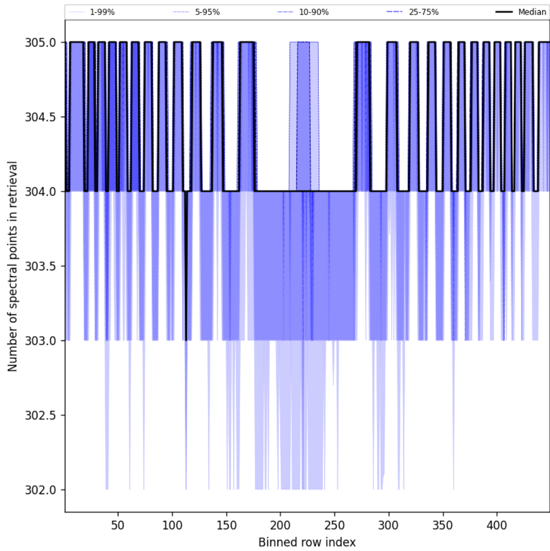
Figure 48: Along track statistics of “Number of spectral points in retrieval” for 2025-10-02 to 2025-10-03
