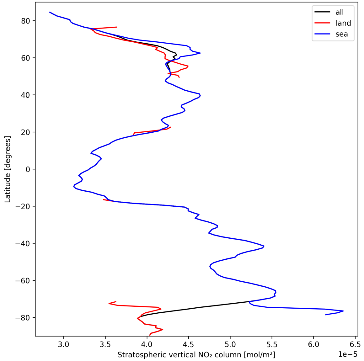
Figure 17: Zonal average of “Stratospheric vertical NO 2 column” for 2025-10-02 to 2025-10-03.
