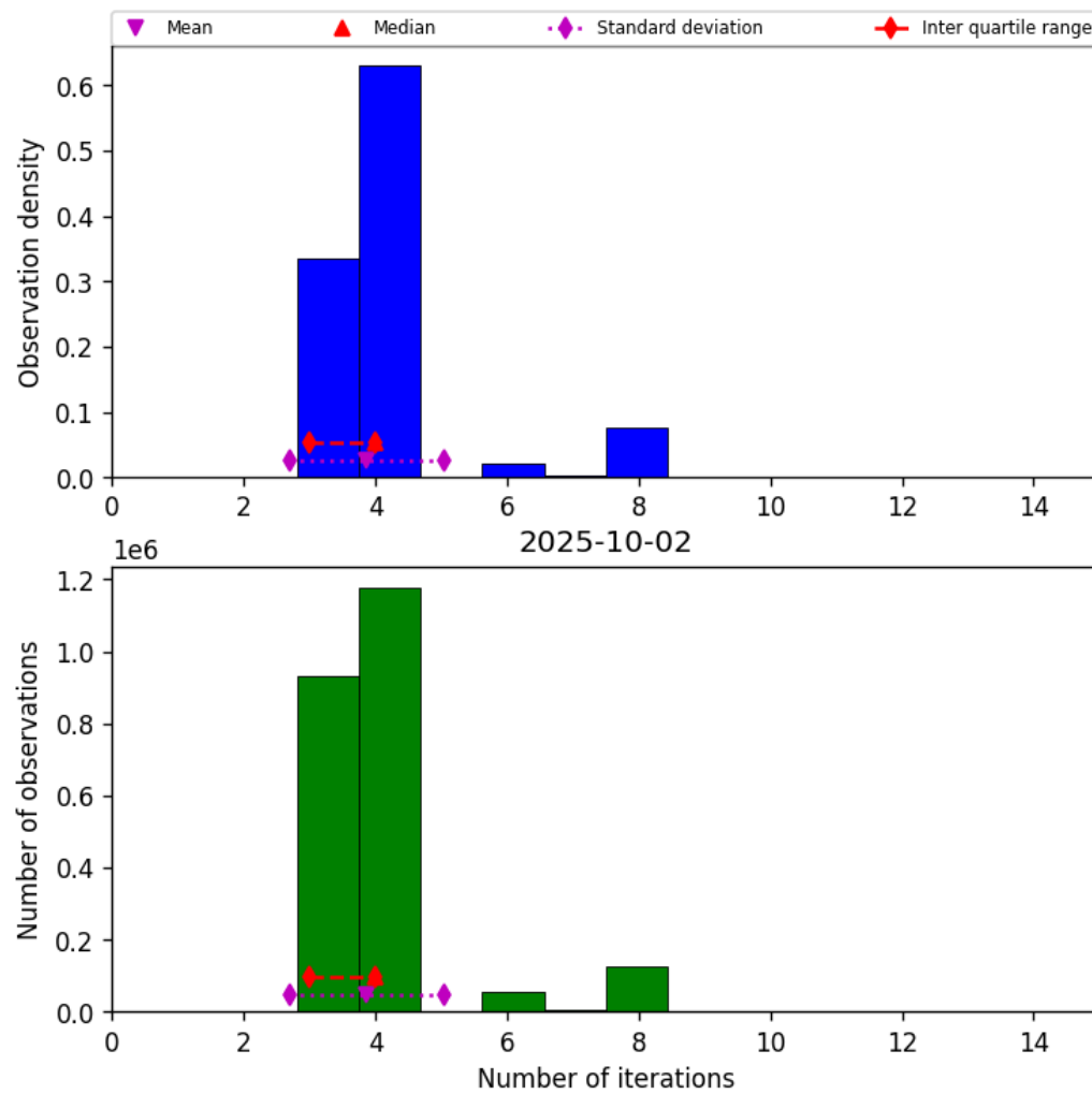
Figure 32: Histogram of “Number of iterations” for 2025-10-02 to 2025-10-03
