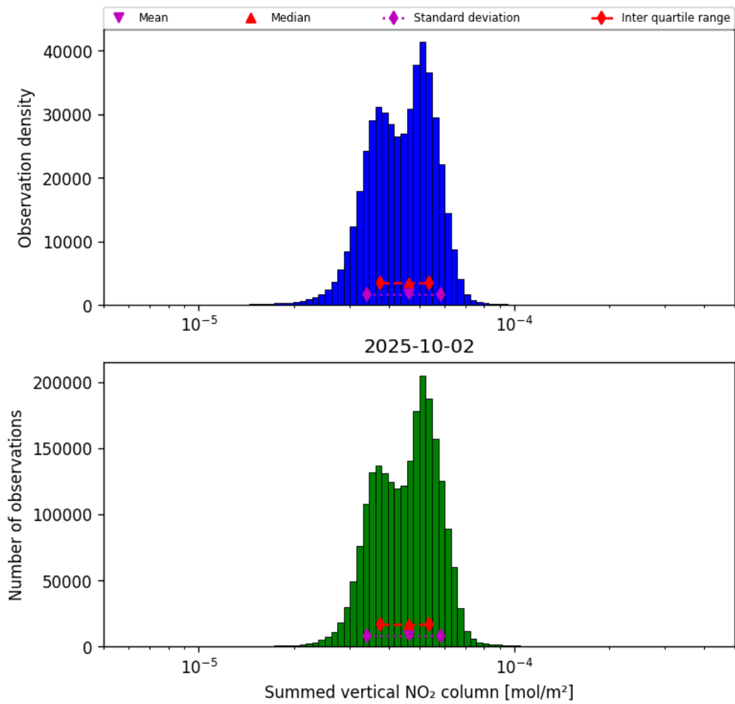
Figure 38: Histogram of “Summed vertical NO 2 column” for 2025-10-02 to 2025-10-03
