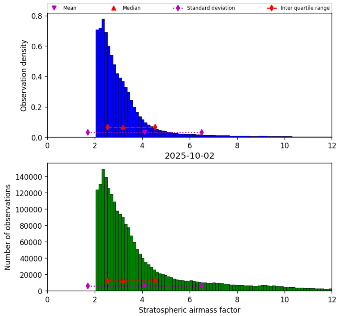
Figure 42: Histogram of “Stratospheric airmass factor” for 2025-10-02 to 2025-10-03
