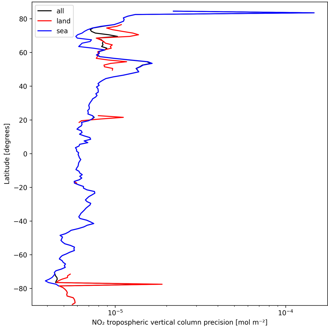
Figure 11: Zonal average of “NO 2 tropospheric vertical column precision” for 2025-10-02 to 2025-10-03.
