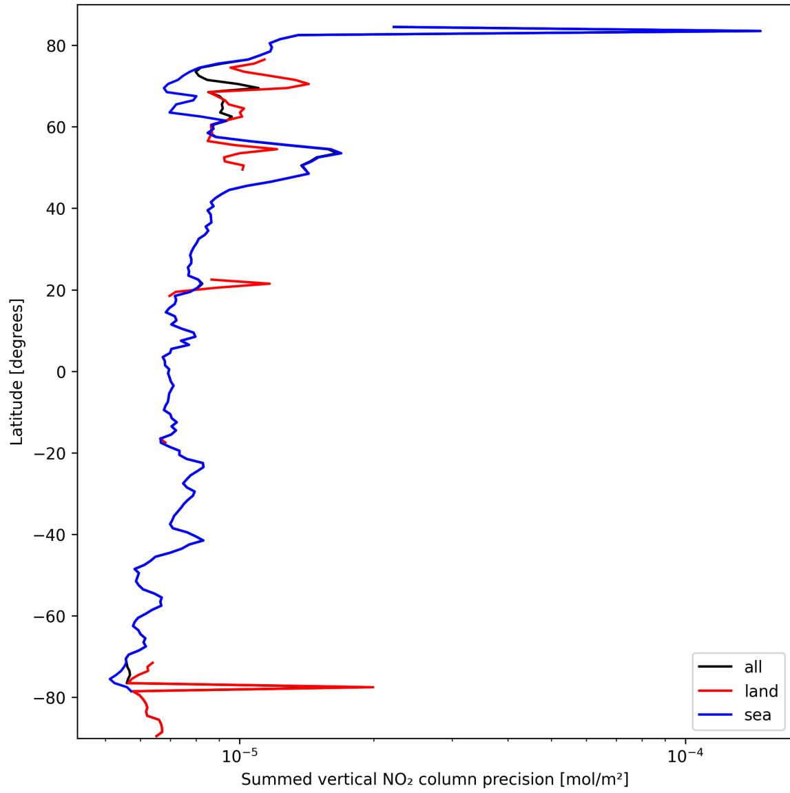
Figure 22: Zonal average of “Summed vertical NO 2 column precision” for 2025-10-02 to 2025-10-03.
