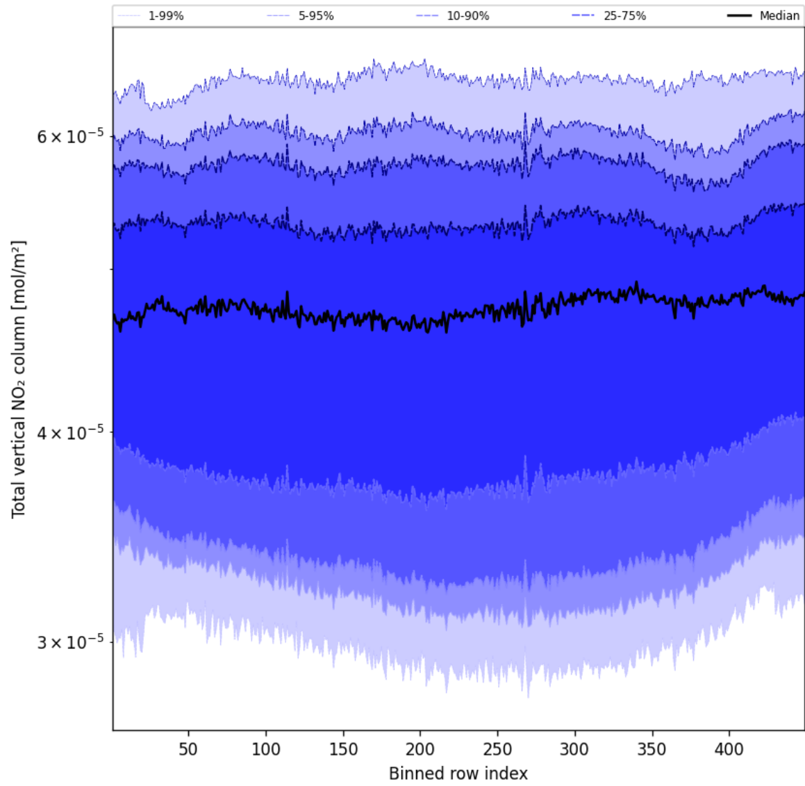
Figure 53: Along track statistics of “Total vertical NO 2 column” for 2025-10-02 to 2025-10-03
