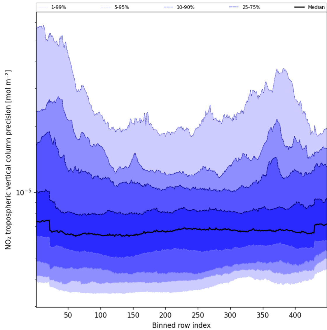
Figure 45: Along track statistics of “NO 2 tropospheric vertical column precision” for 2025-10-02 to 2025-10-03
