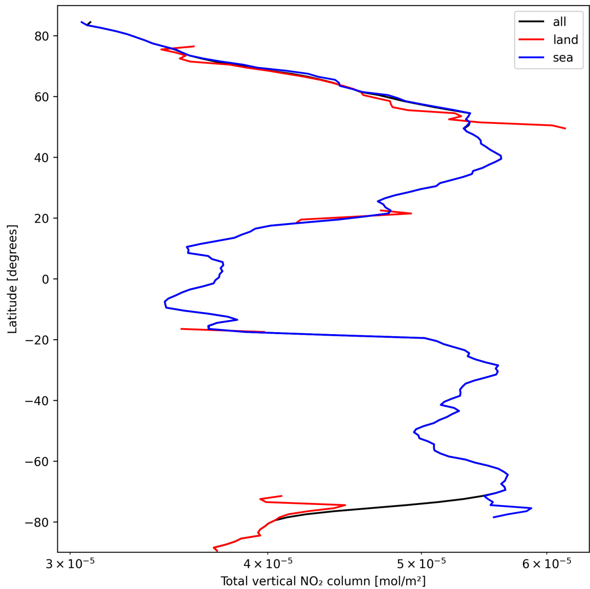
Figure 19: Zonal average of “Total vertical NO 2 column” for 2025-10-02 to 2025-10-03.
