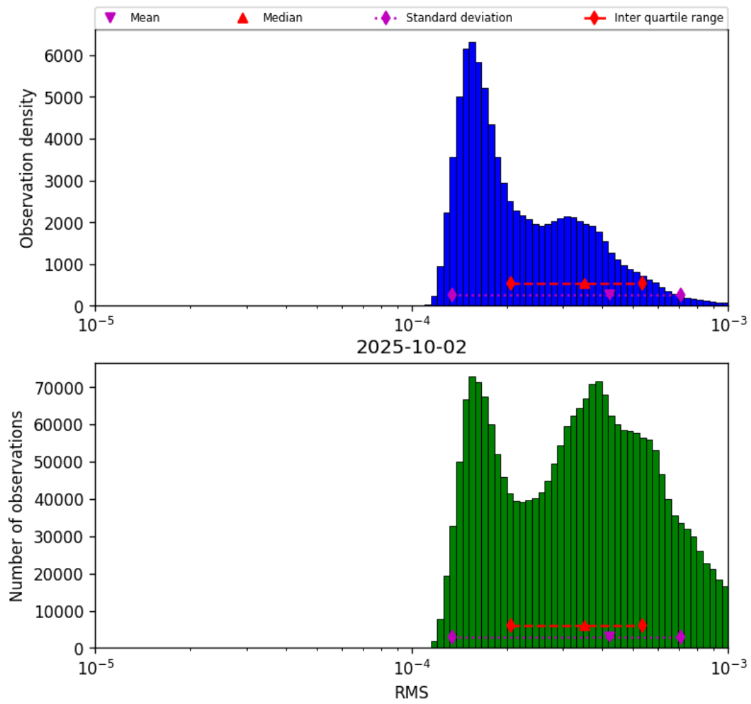
Figure 41: Histogram of “RMS” for 2025-10-02 to 2025-10-03
