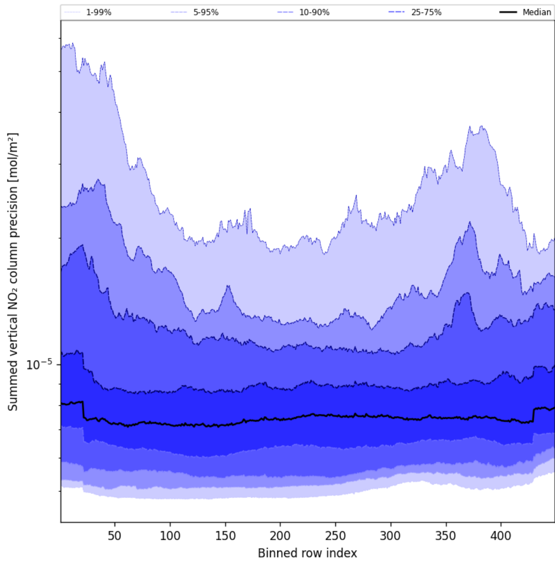
Figure 56: Along track statistics of “Summed vertical NO 2 column precision” for 2025-10-02 to 2025-10-03
