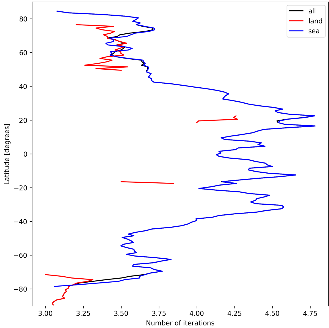
Figure 15: Zonal average of “Number of iterations” for 2025-10-02 to 2025-10-03.
