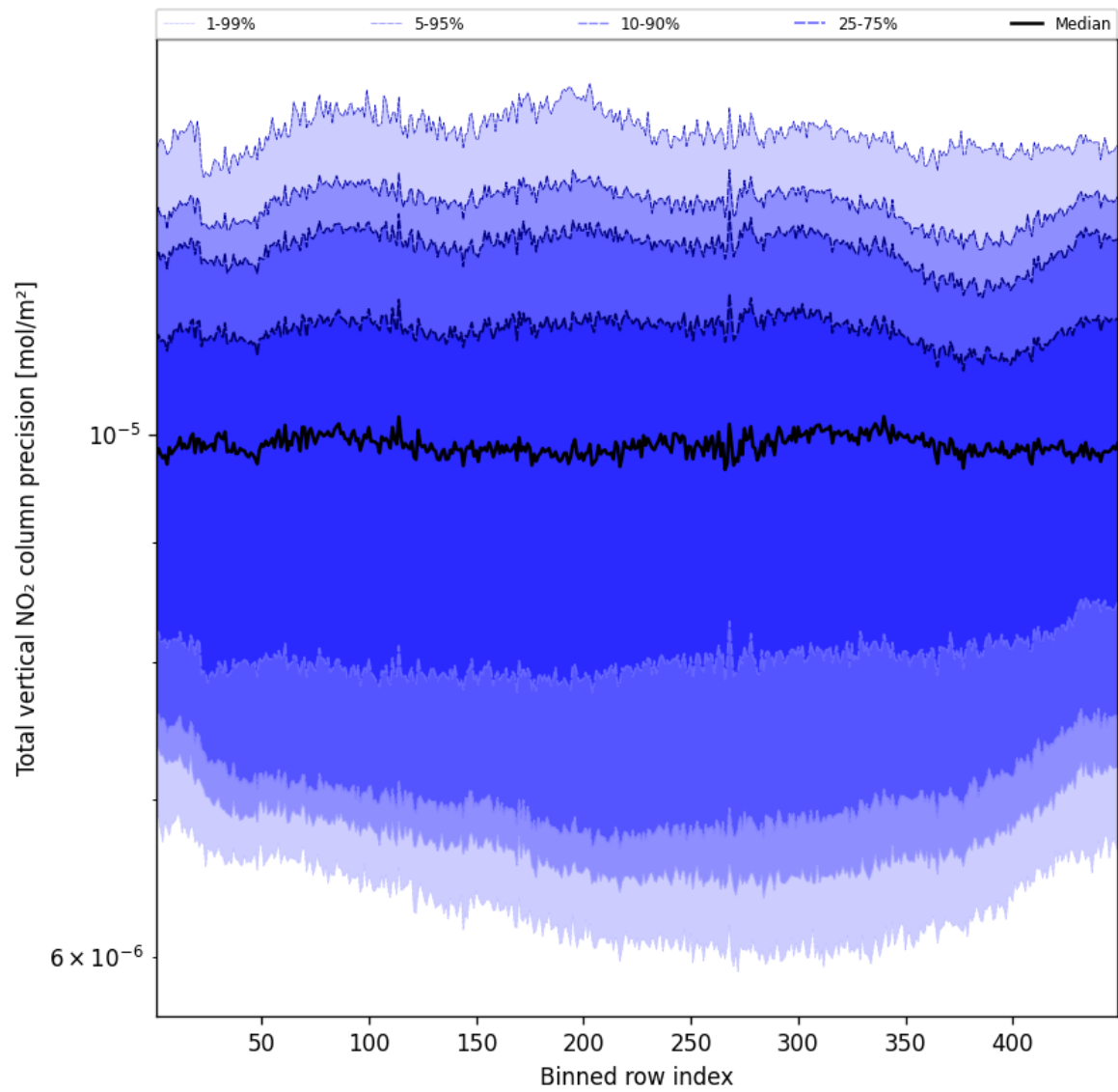
Figure 54: Along track statistics of “Total vertical NO 2 column precision” for 2025-10-02 to 2025-10-03
