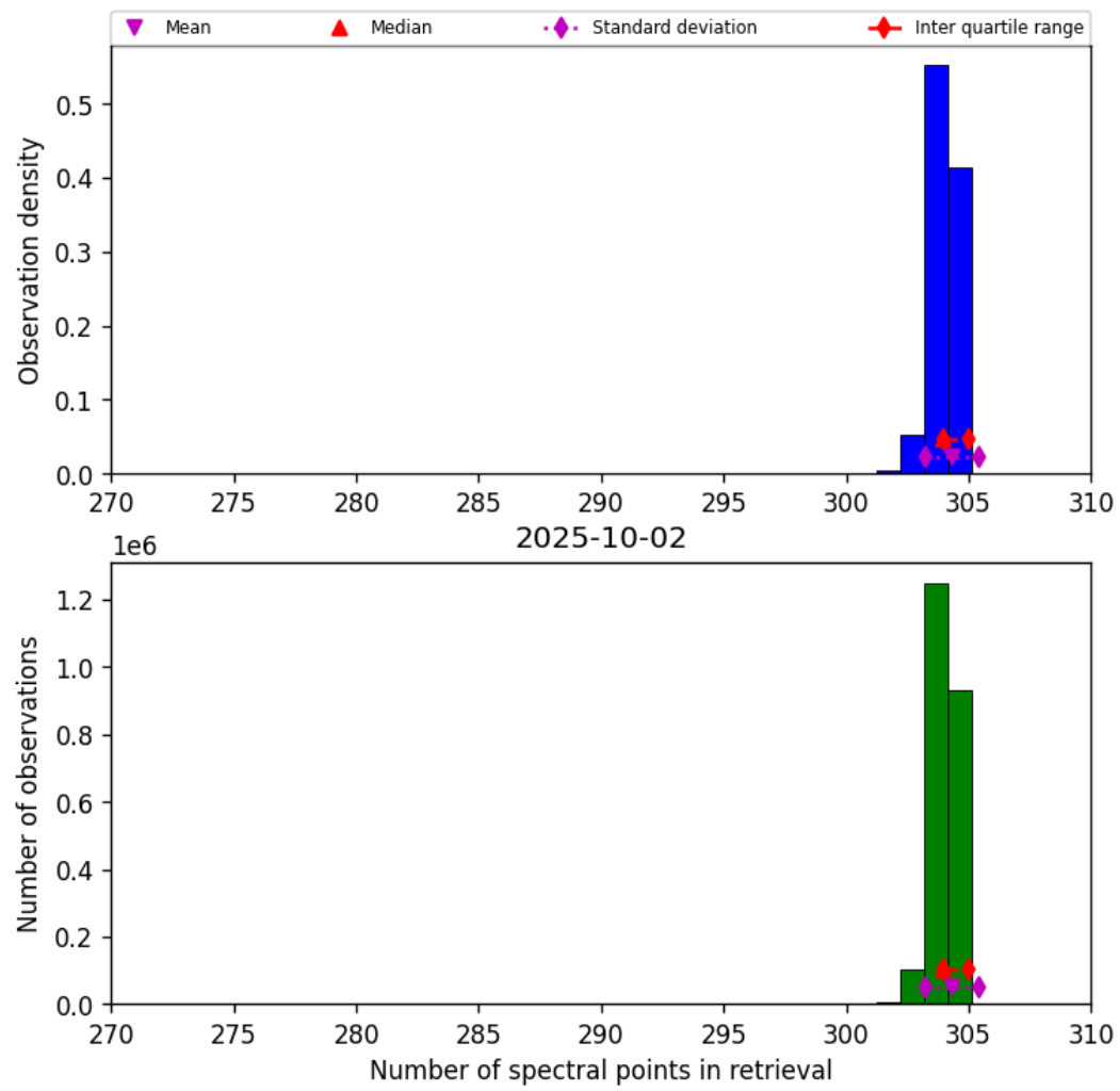
Figure 31: Histogram of “Number of spectral points in retrieval” for 2025-10-02 to 2025-10-03
