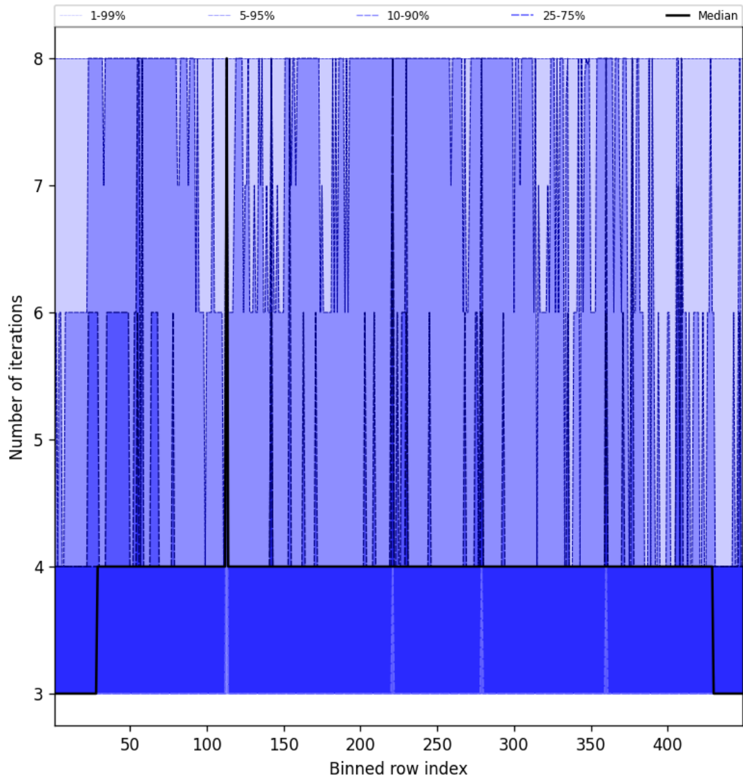
Figure 49: Along track statistics of “Number of iterations” for 2025-10-02 to 2025-10-03
