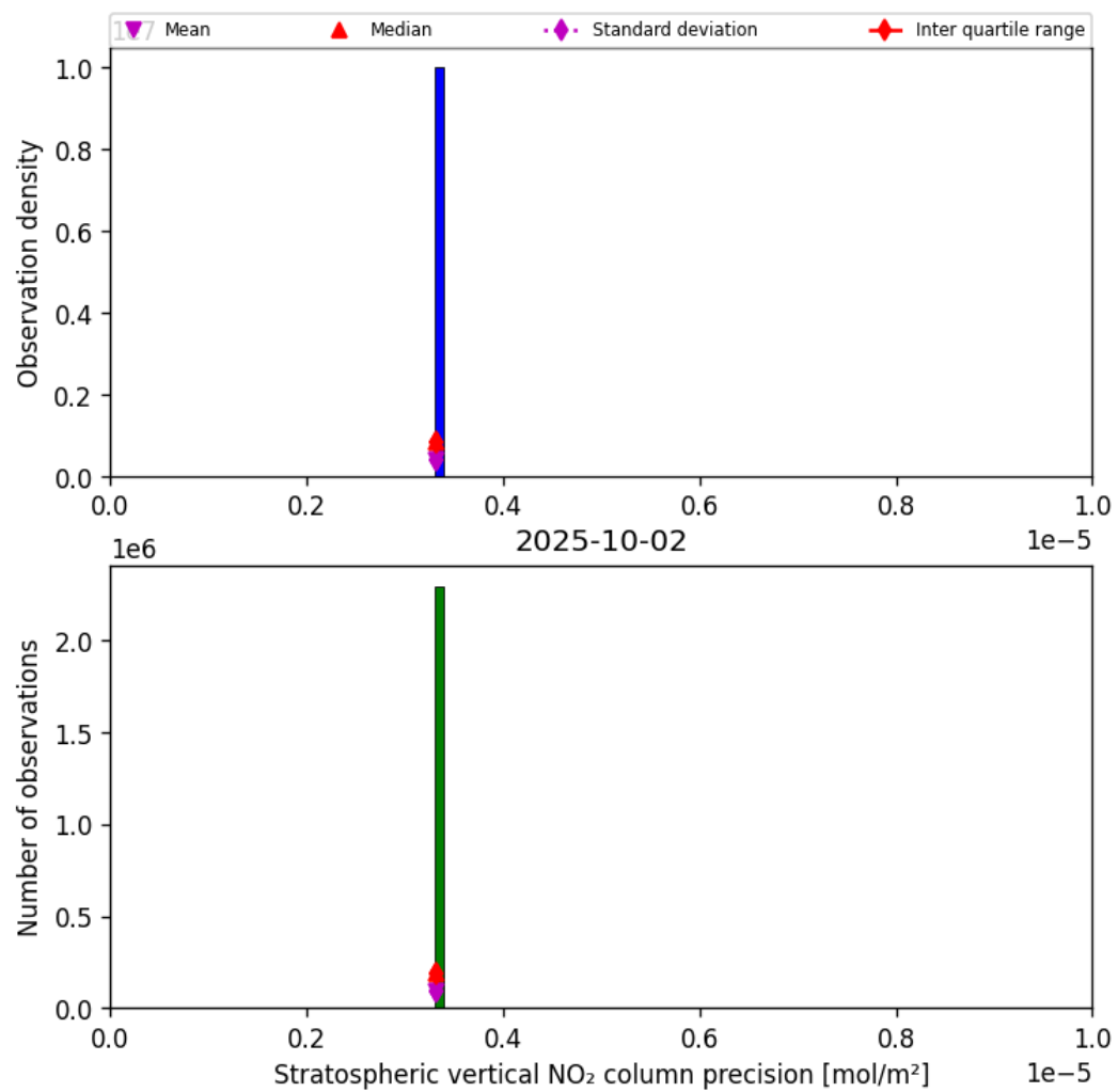
Figure 35: Histogram of “Stratospheric vertical NO 2 column precision” for 2025-10-02 to 2025-10-03
