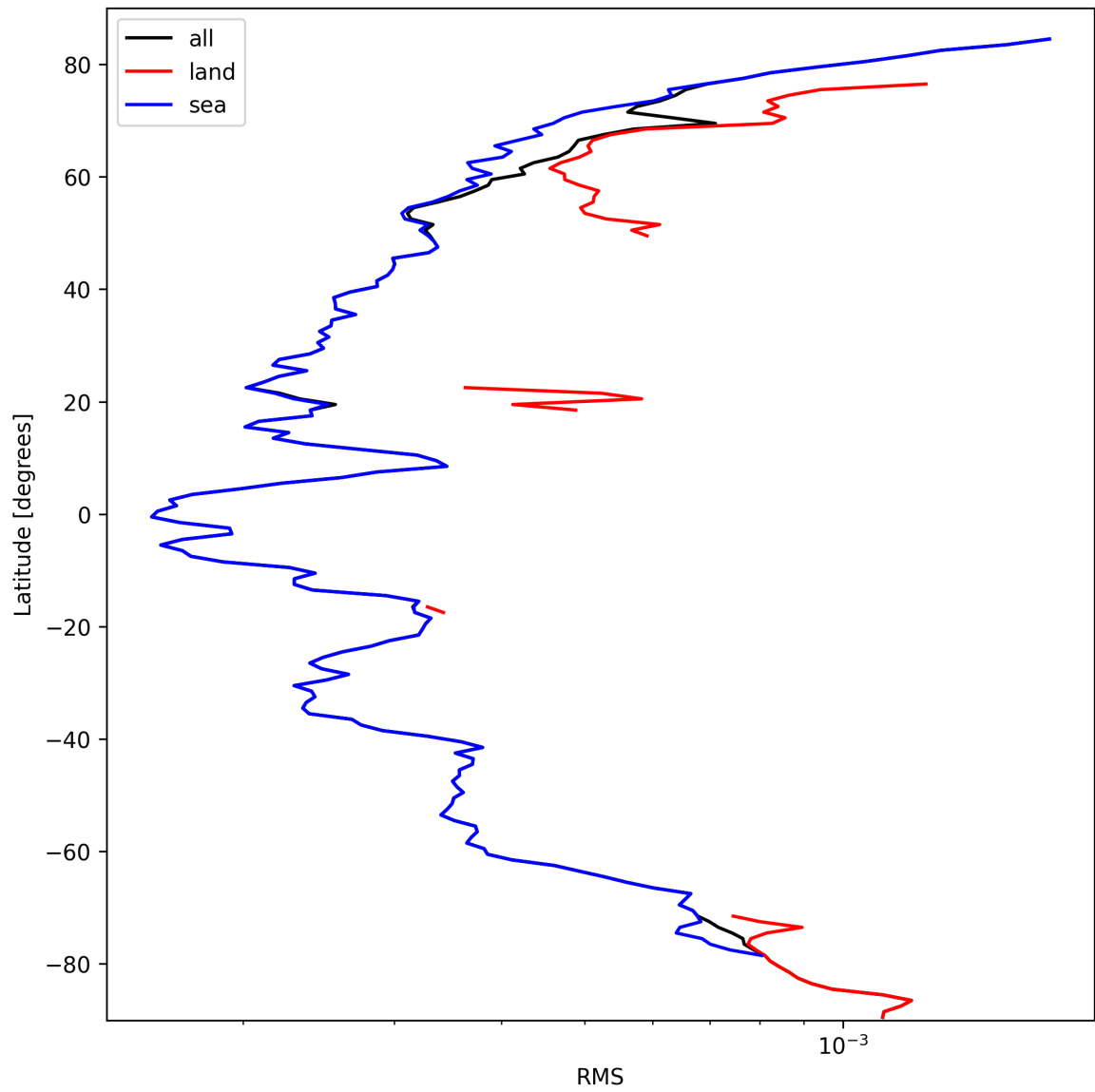
Figure 24: Zonal average of “RMS” for 2025-10-02 to 2025-10-03.
