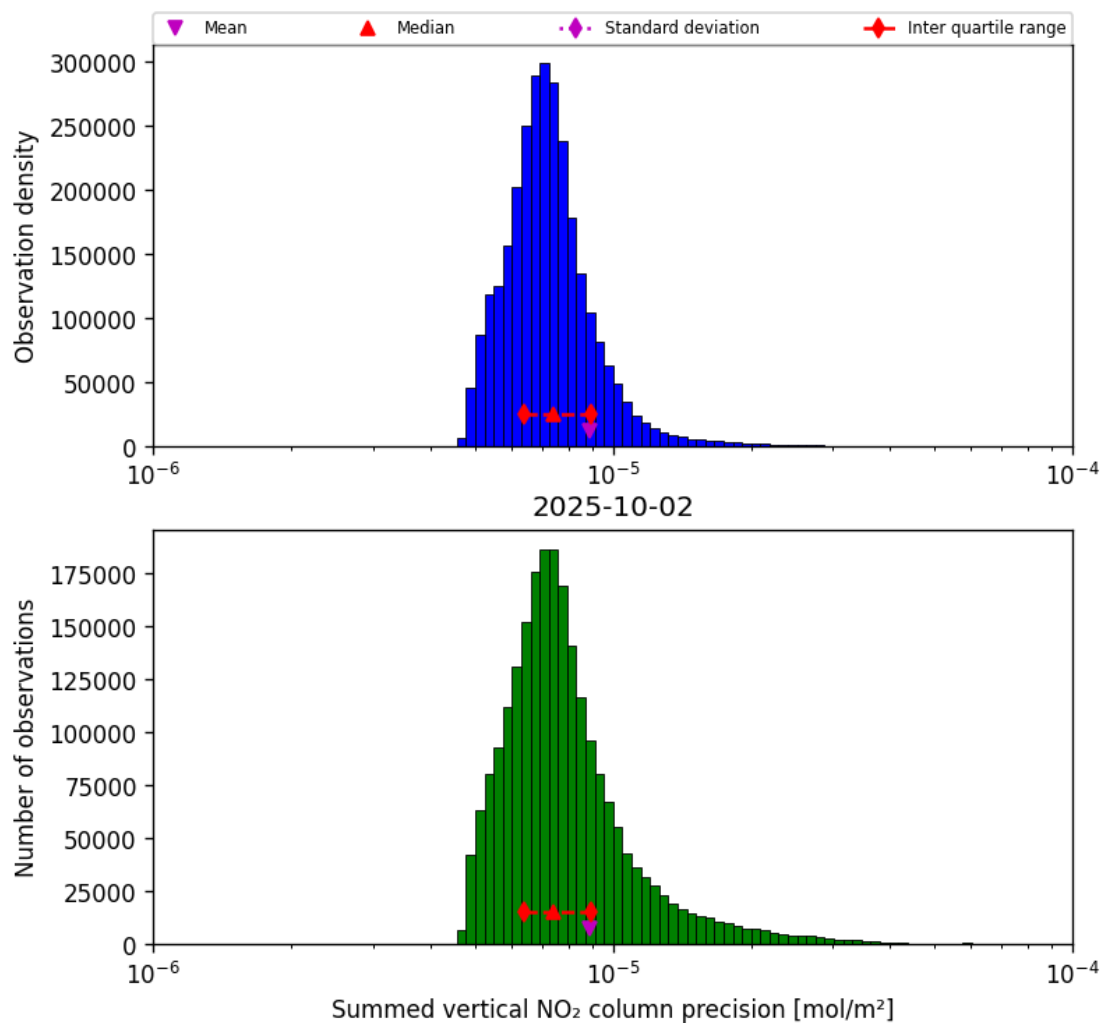
Figure 39: Histogram of “Summed vertical NO 2 column precision” for 2025-10-02 to 2025-10-03
