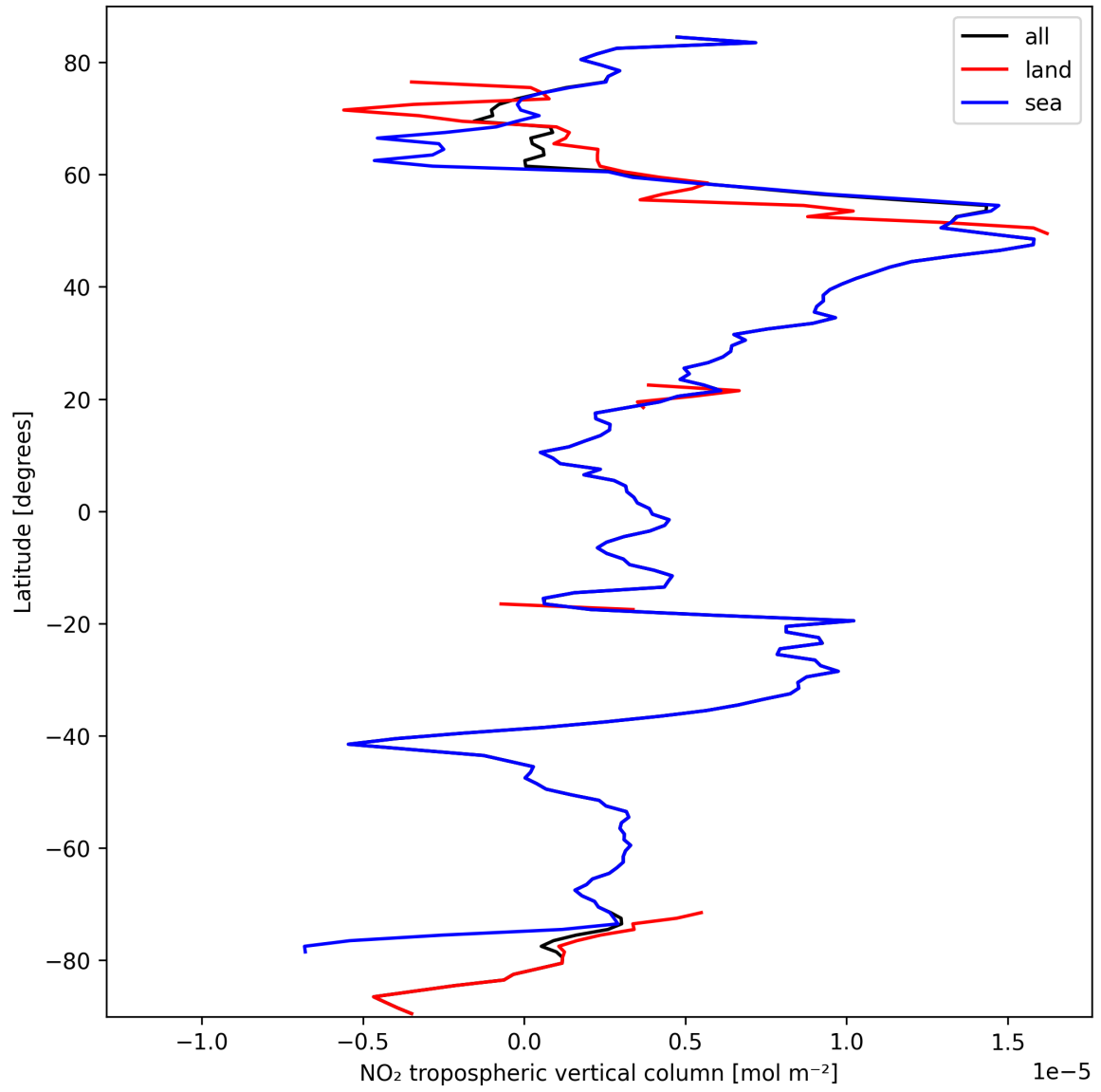
Figure 10: Zonal average of “NO 2 tropospheric vertical column” for 2025-10-02 to 2025-10-03.
