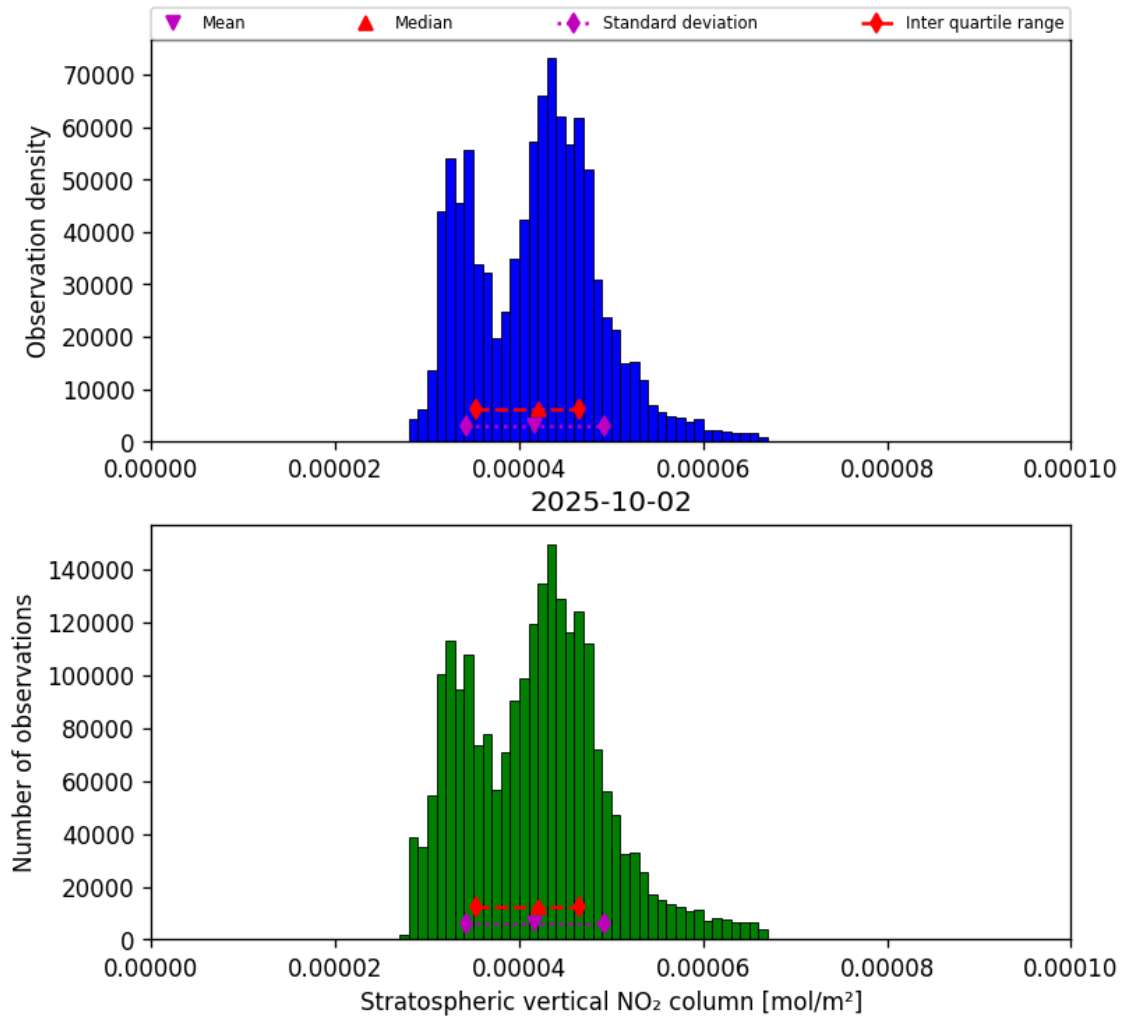
Figure 34: Histogram of “Stratospheric vertical NO 2 column” for 2025-10-02 to 2025-10-03
