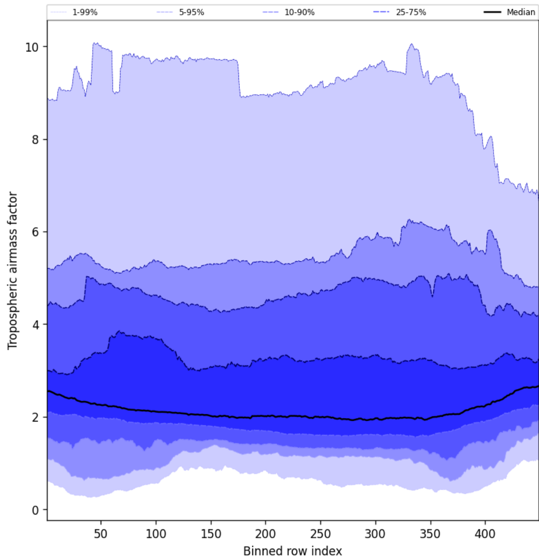
Figure 46: Along track statistics of “Tropospheric air mass factor” for 2025-10-02 to 2025-10-03
