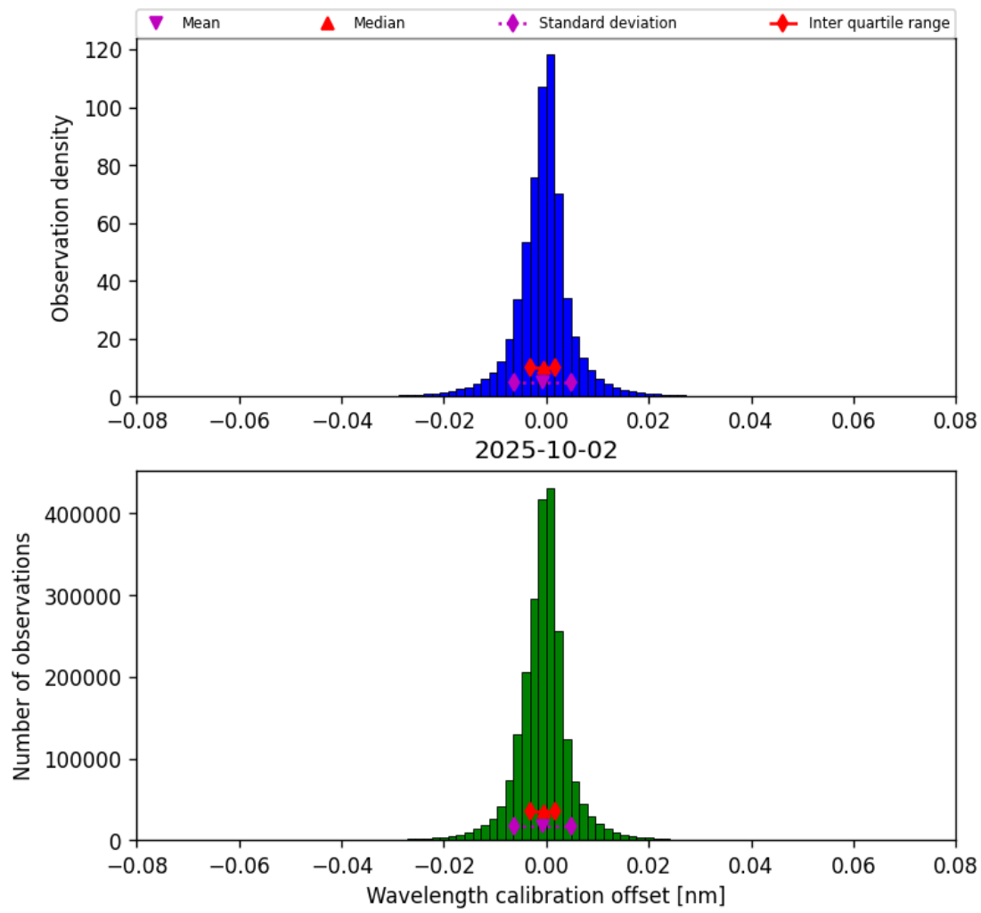
Figure 33: Histogram of “Wavelength calibration offset” for 2025-10-02 to 2025-10-03
