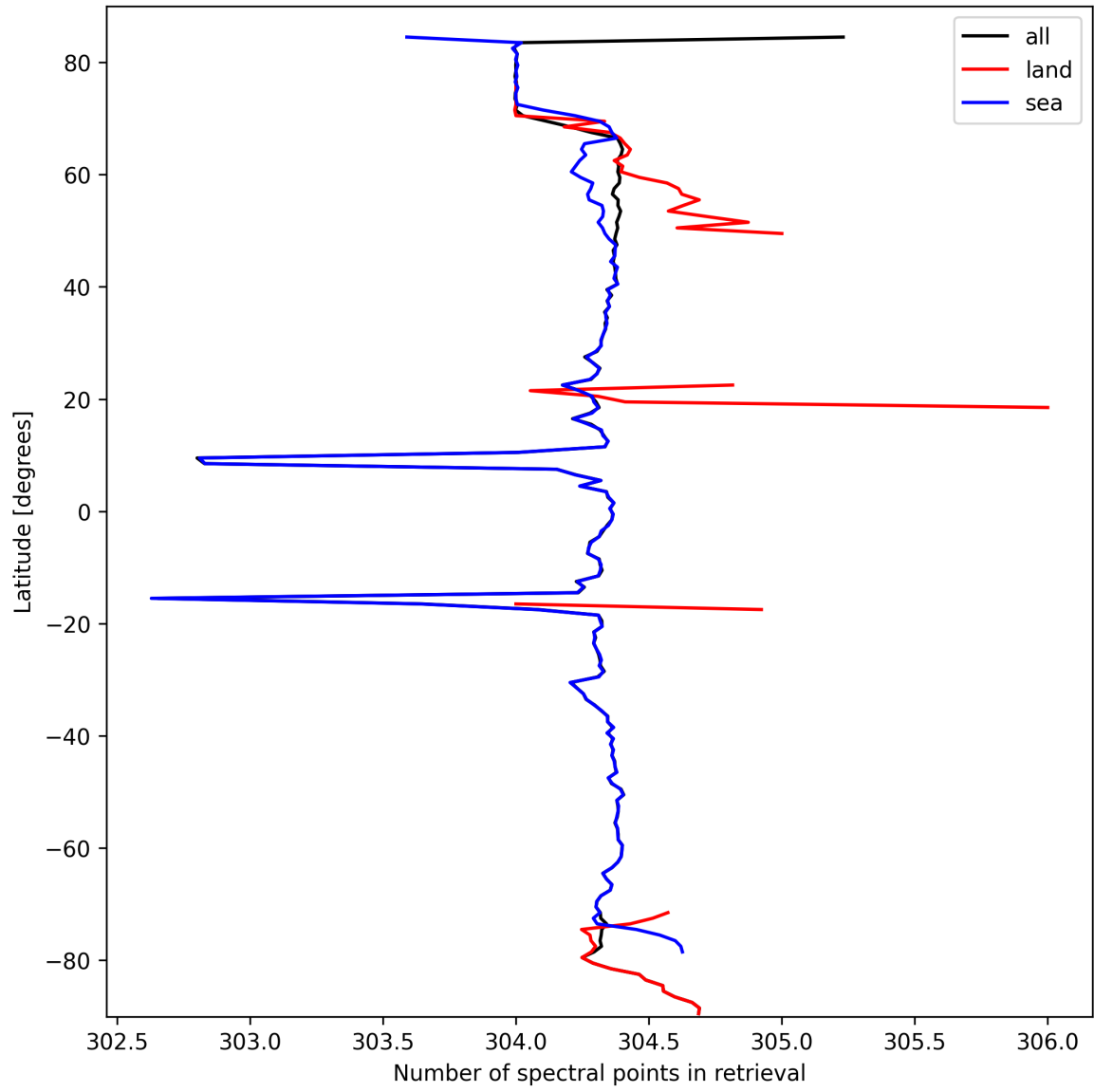
Figure 14: Zonal average of “Number of spectral points in retrieval” for 2025-10-02 to 2025-10-03.
