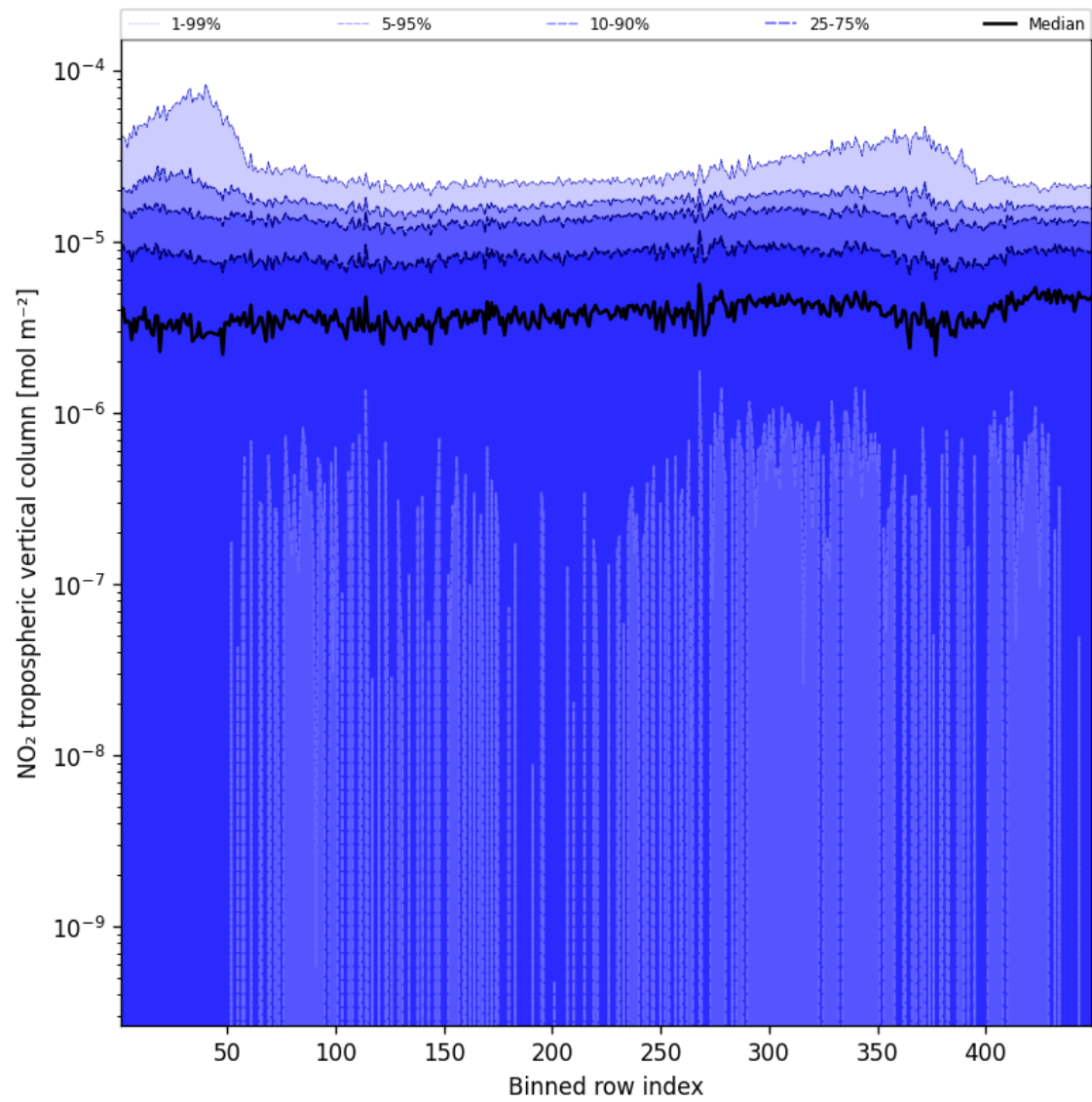
Figure 44: Along track statistics of “NO 2 tropospheric vertical column” for 2025-10-02 to 2025-10-03
