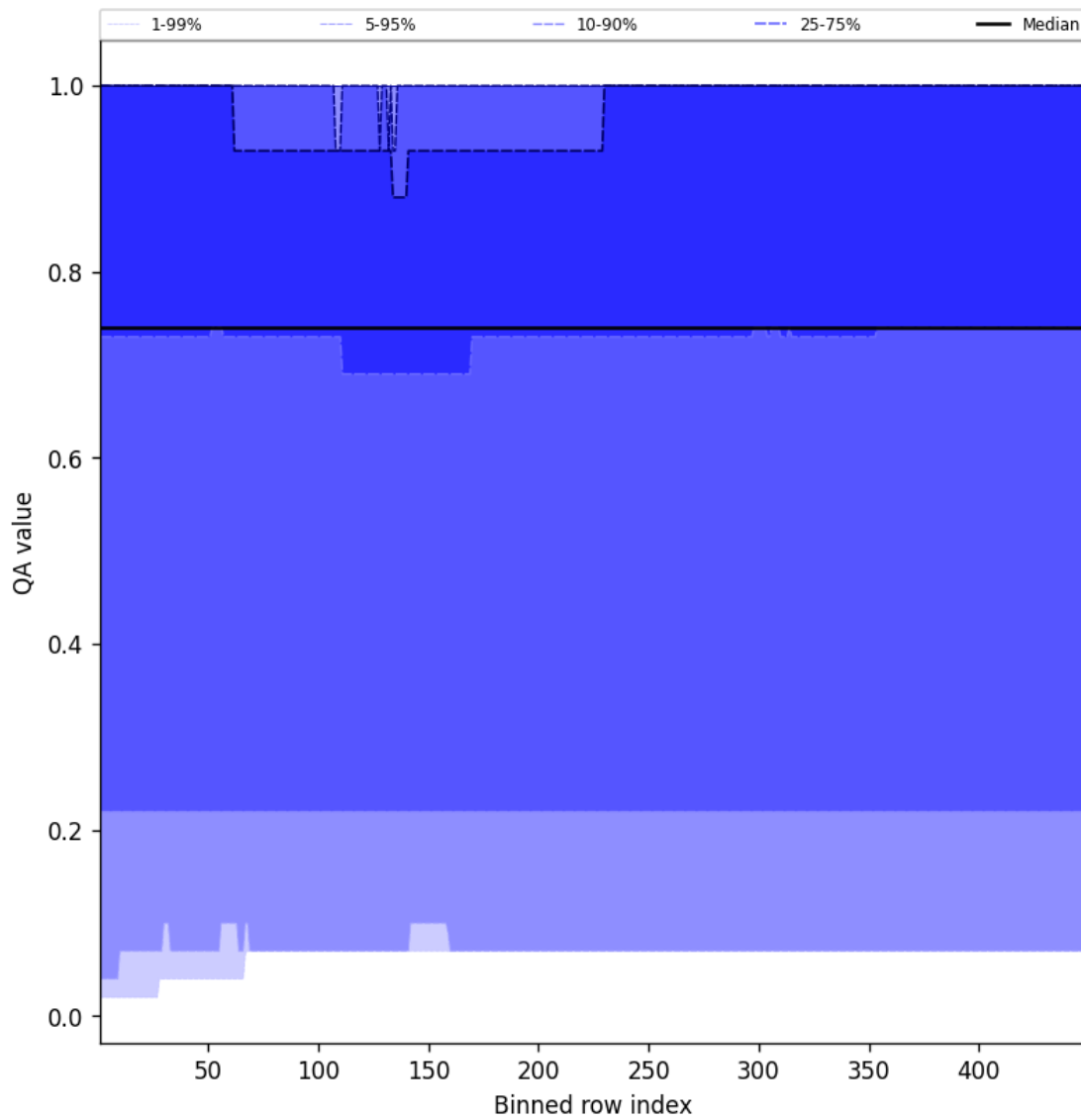
Figure 43: Along track statistics of “QA value” for 2025-10-02 to 2025-10-03
