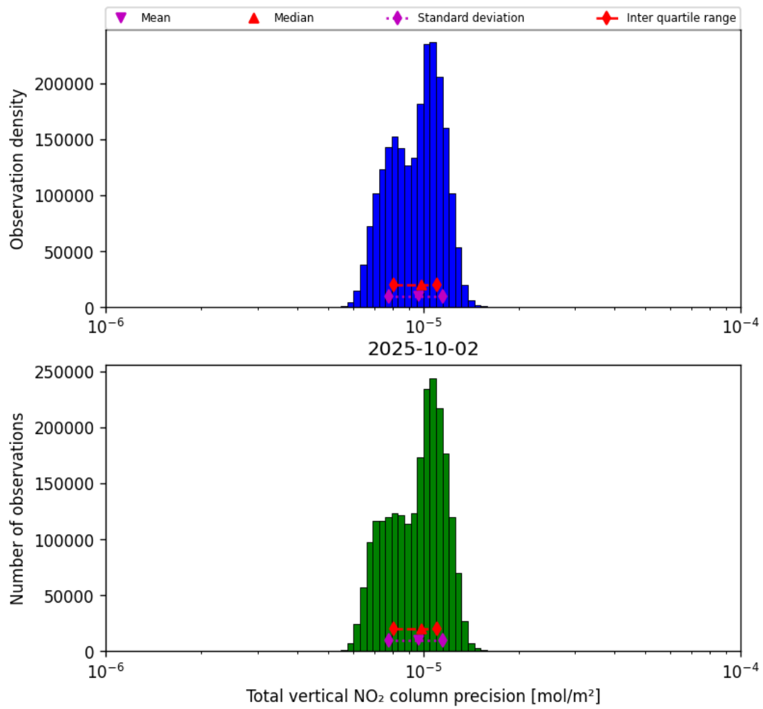
Figure 37: Histogram of “Total vertical NO 2 column precision” for 2025-10-02 to 2025-10-03
