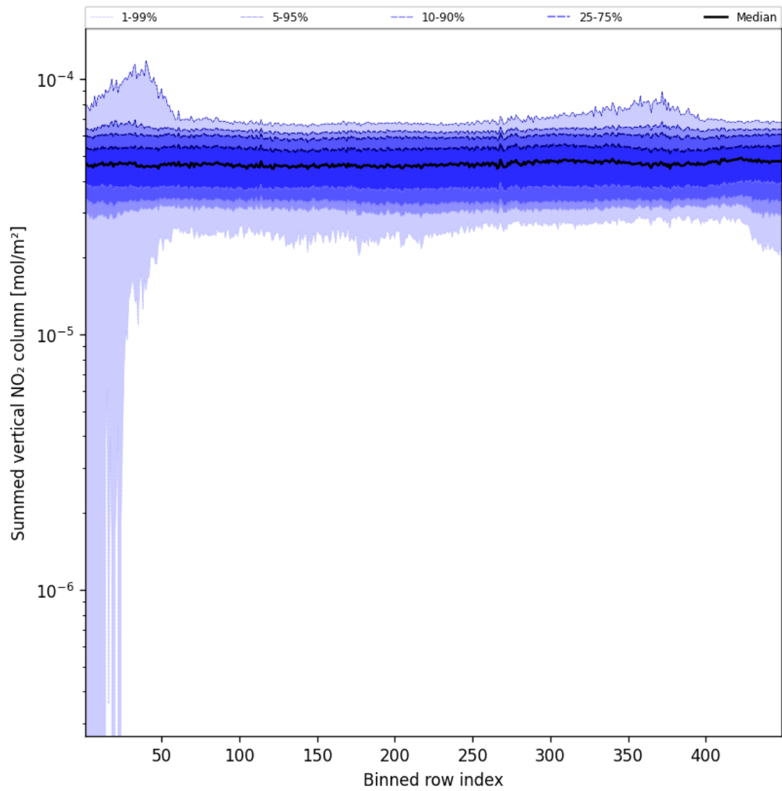
Figure 55: Along track statistics of “Summed vertical NO 2 column” for 2025-10-02 to 2025-10-03
