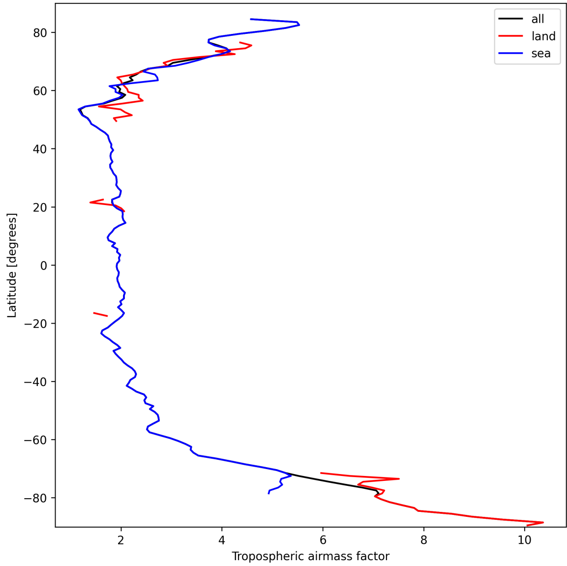
Figure 12: Zonal average of “Tropospheric air mass factor” for 2025-10-02 to 2025-10-03.
