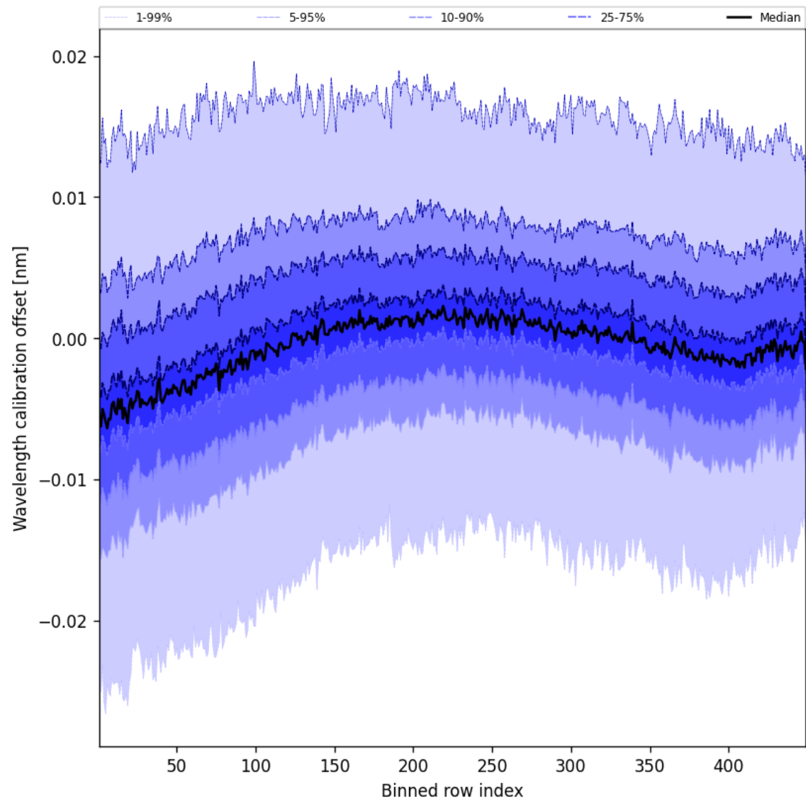
Figure 50: Along track statistics of “Wavelength calibration offset” for 2025-10-02 to 2025-10-03
