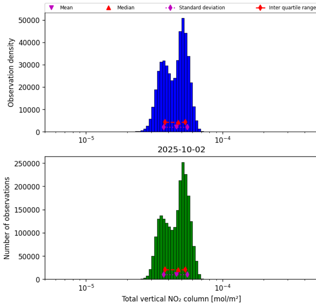
Figure 36: Histogram of “Total vertical NO 2 column” for 2025-10-02 to 2025-10-03
