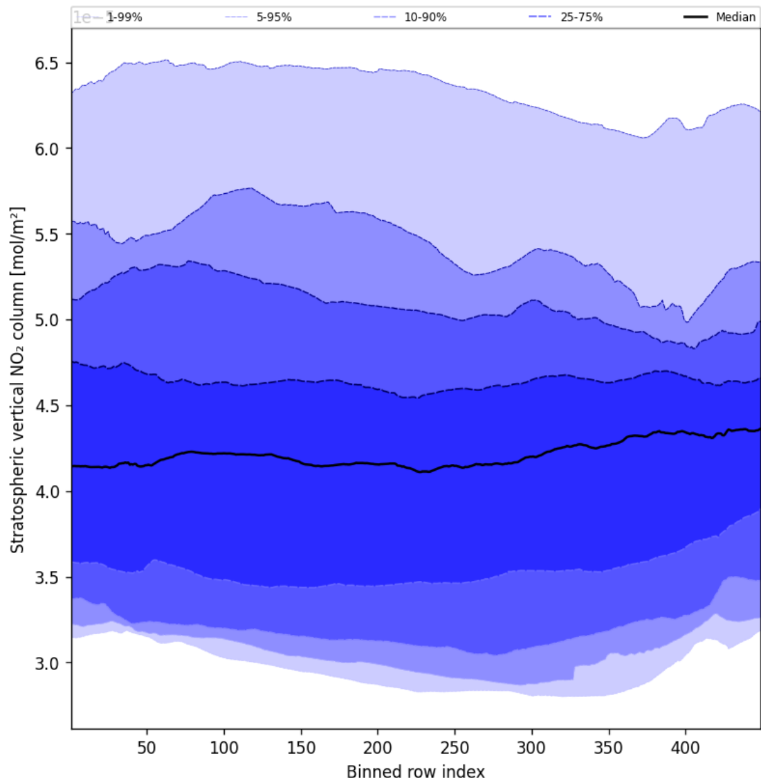
Figure 51: Along track statistics of “Stratospheric vertical NO 2 column” for 2025-10-02 to 2025-10-03
