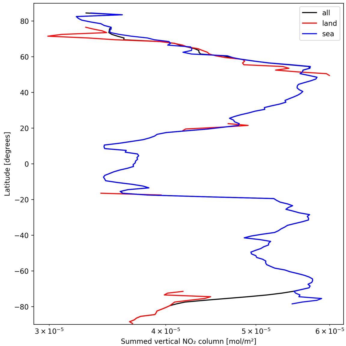
Figure 21: Zonal average of “Summed vertical NO 2 column” for 2025-10-02 to 2025-10-03.
