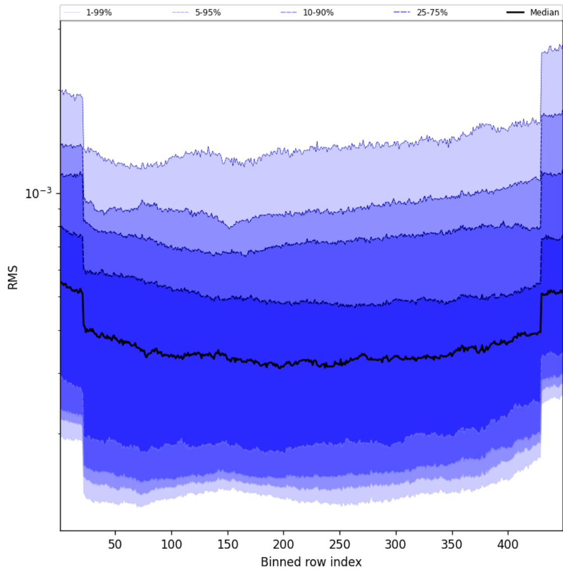
Figure 58: Along track statistics of “RMS” for 2025-10-02 to 2025-10-03
