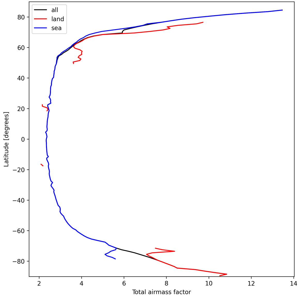
Figure 13: Zonal average of “Total airmass factor” for 2025-10-02 to 2025-10-03.
