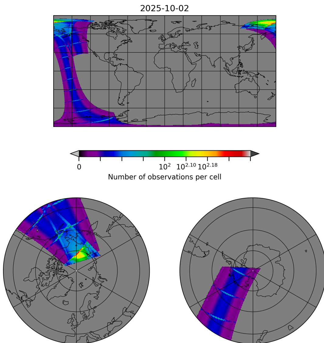
Figure 8: Map of the number of observations for 2025-10-02 to 2025-10-03
