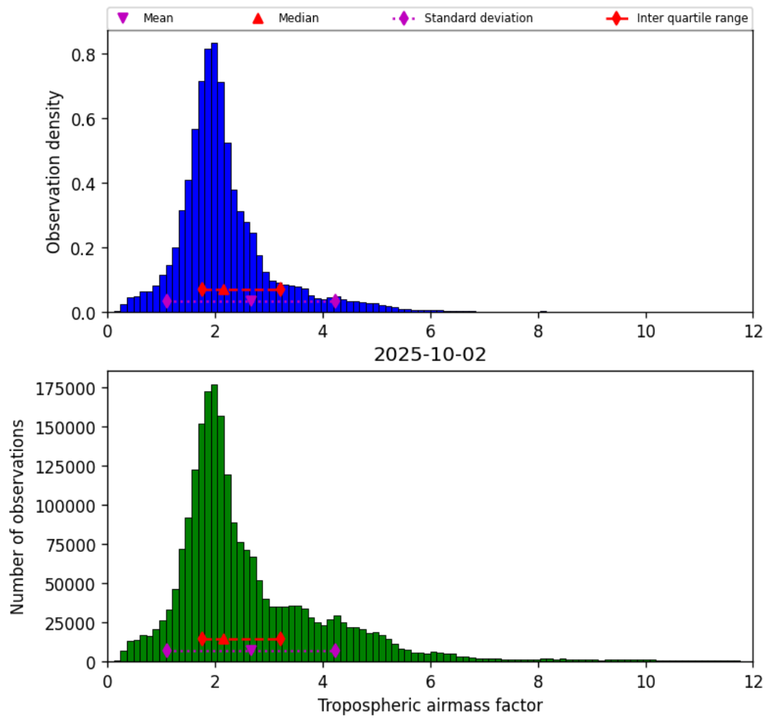
Figure 29: Histogram of “Tropospheric airmass factor” for 2025-10-02 to 2025-10-03
