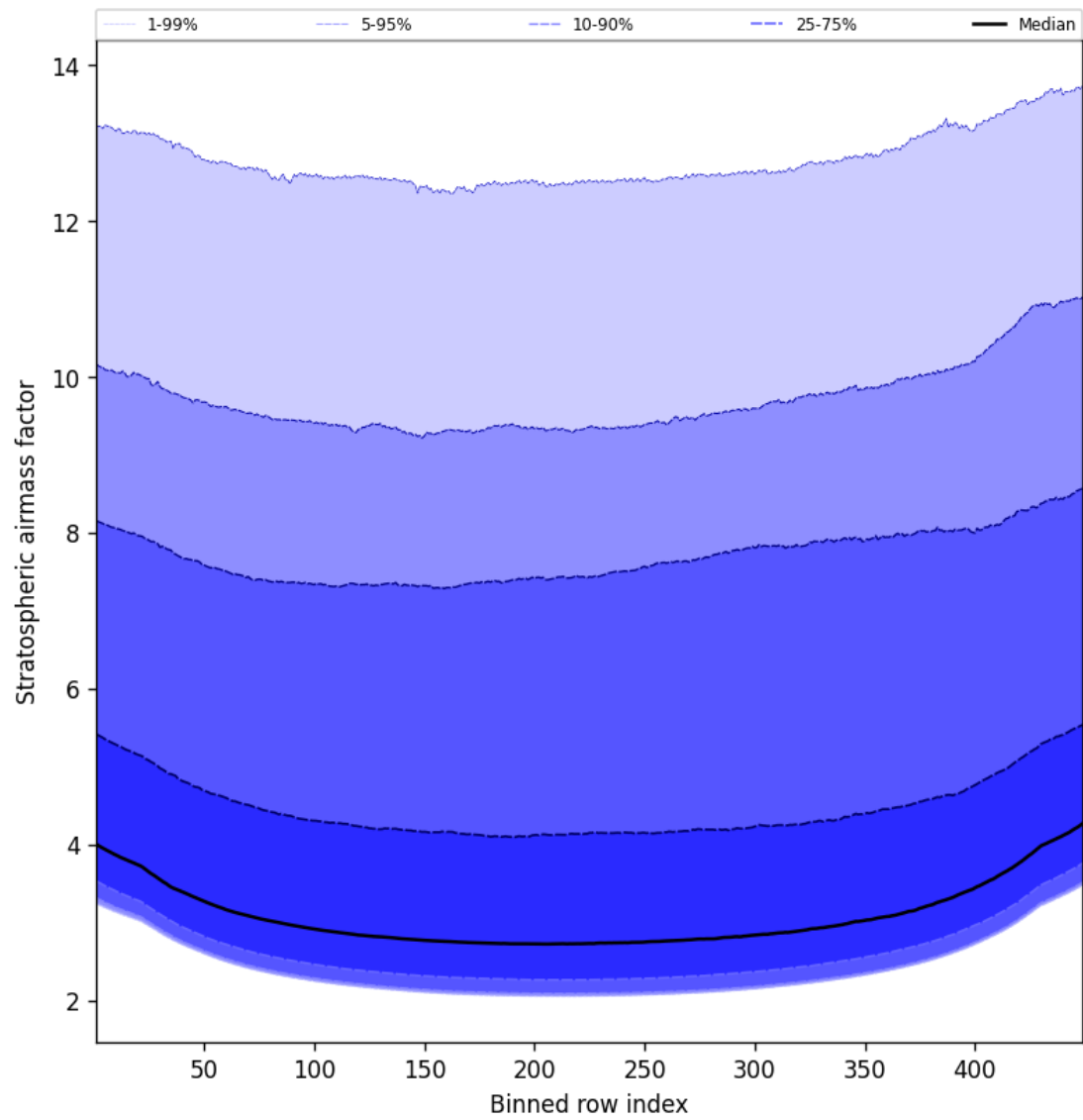
Figure 59: Along track statistics of “Stratospheric airmass factor” for 2025-10-02 to 2025-10-03
