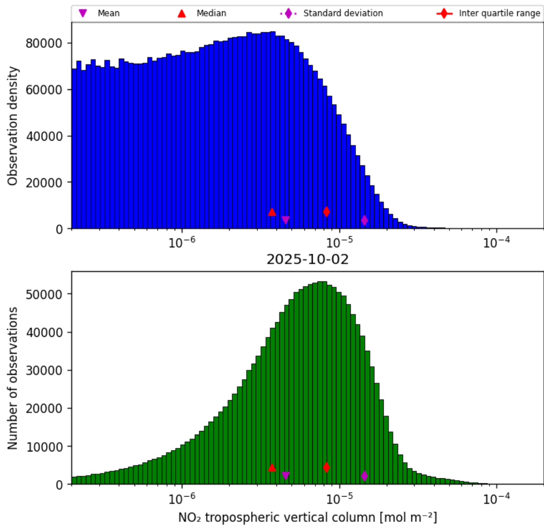
Figure 27: Histogram of “NO 2 tropospheric vertical column” for 2025-10-02 to 2025-10-03
