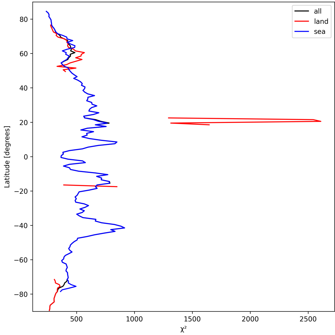
Figure 23: Zonal average of “ \chi^2 ” for 2025-10-02 to 2025-10-03.
