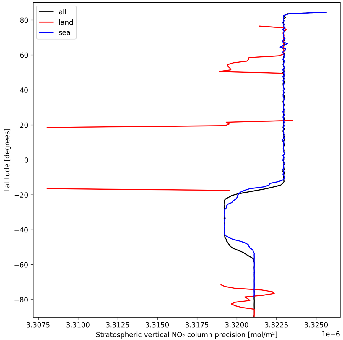
Figure 18: Zonal average of “Stratospheric vertical NO 2 column precision” for 2025-10-02 to 2025-10-03.
