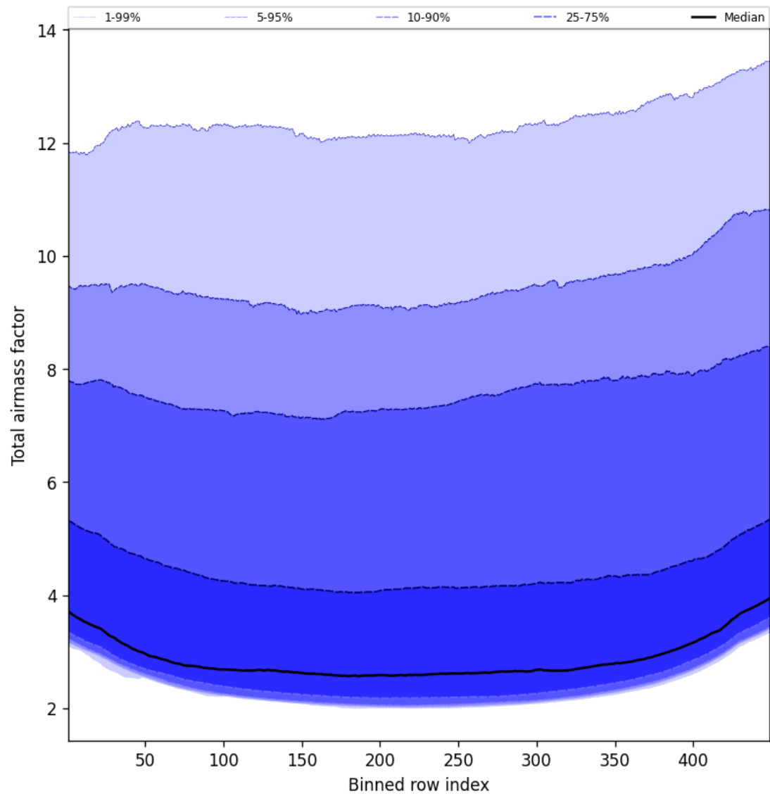
Figure 47: Along track statistics of “Total airmass factor” for 2025-10-02 to 2025-10-03
