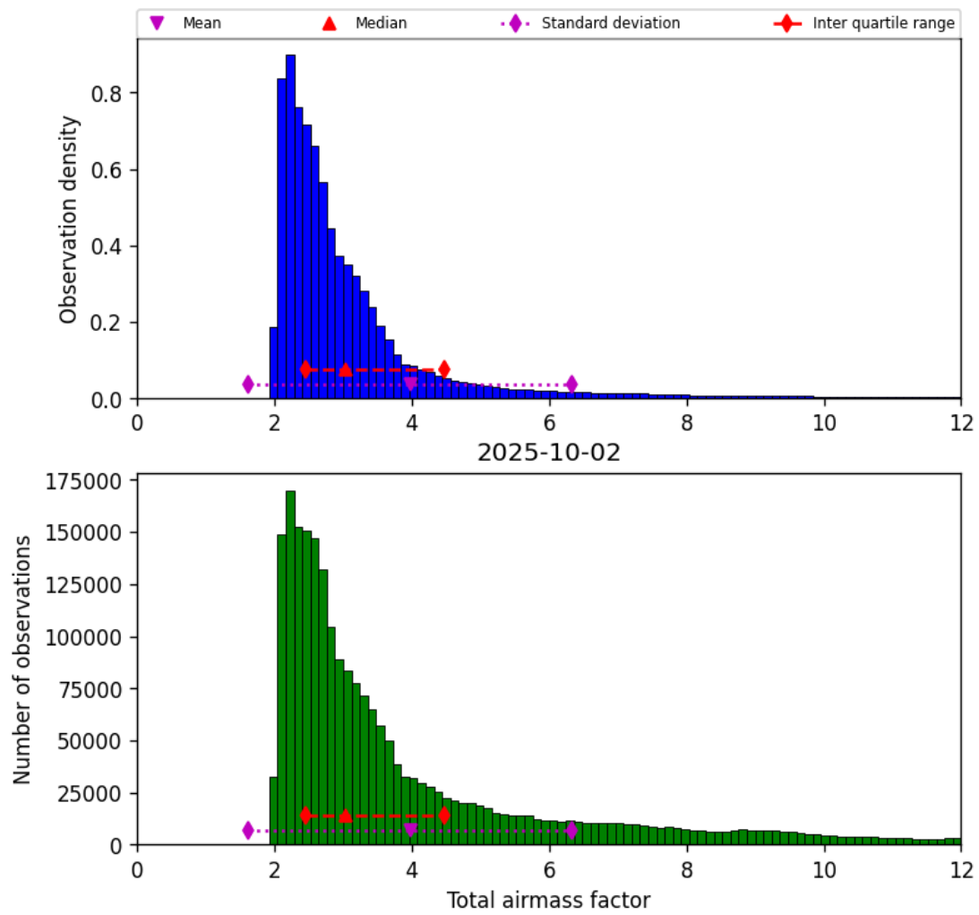
Figure 30: Histogram of “Total airmass factor” for 2025-10-02 to 2025-10-03
