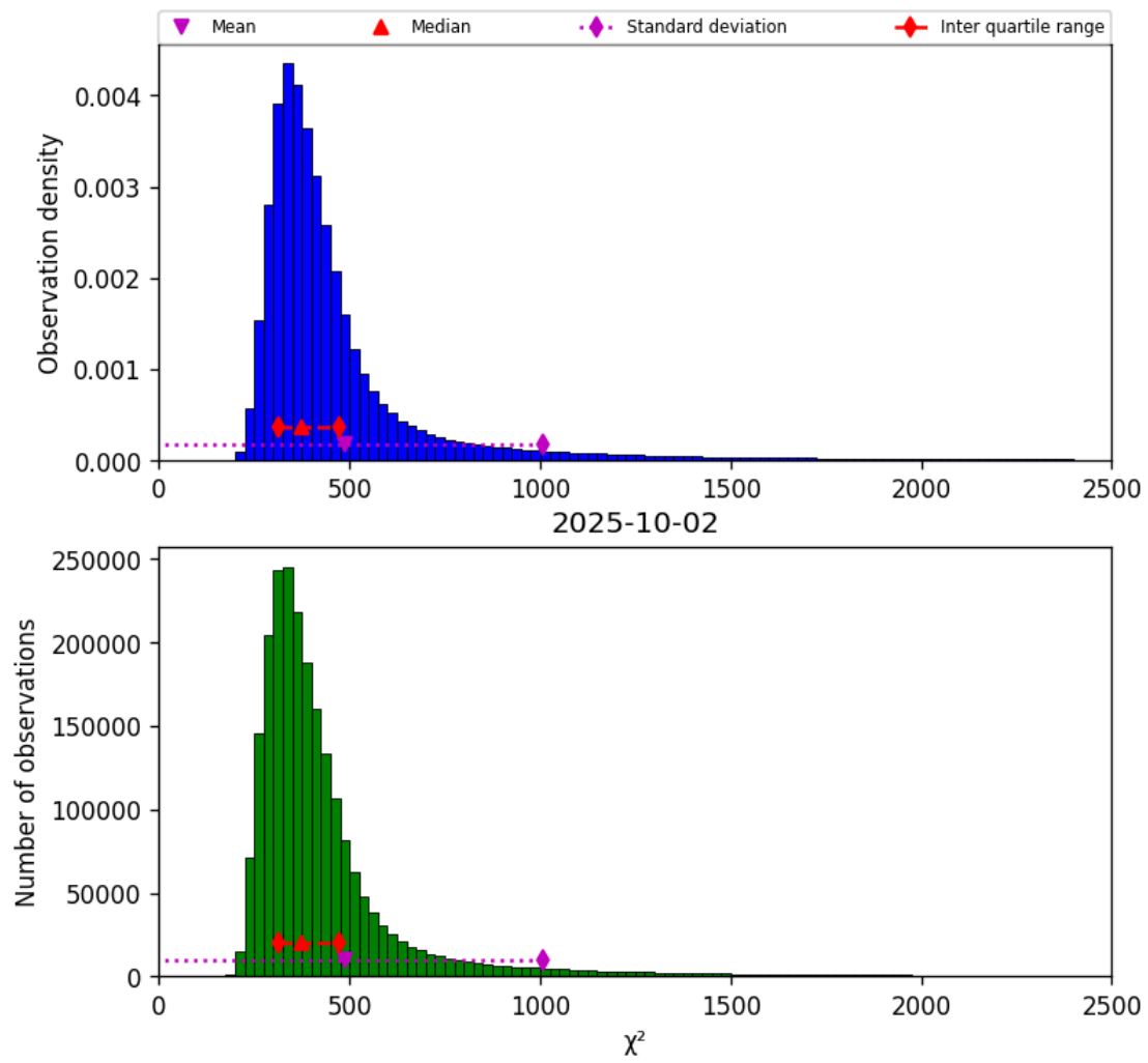
Figure 40: Histogram of " \chi^2 " for 2025-10-02 to 2025-10-03
