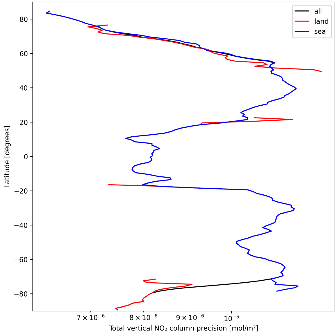
Figure 20: Zonal average of “Total vertical NO 2 column precision” for 2025-10-02 to 2025-10-03.
