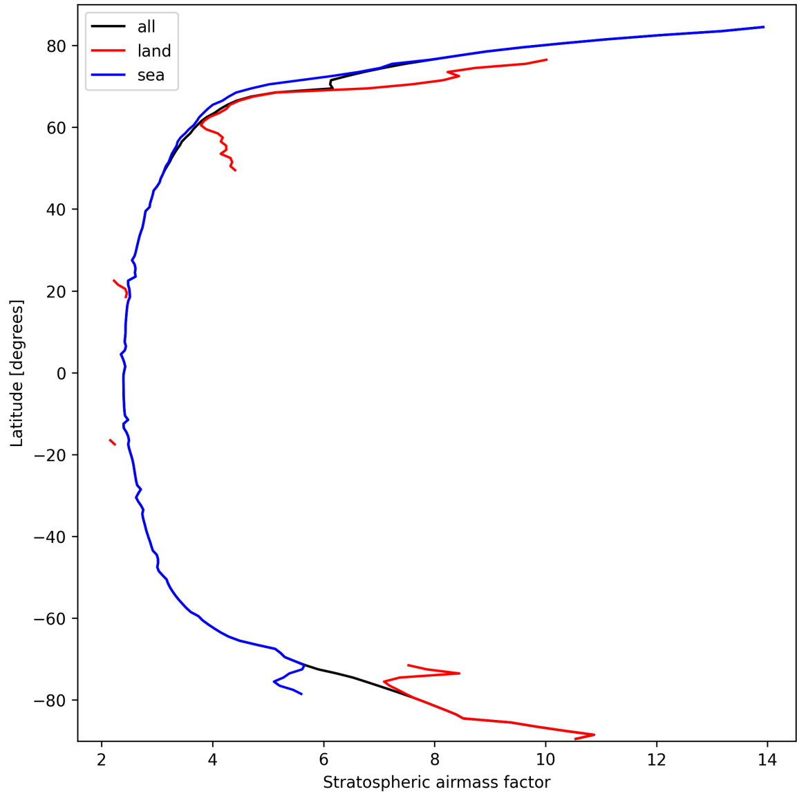
Figure 25: Zonal average of “Stratospheric air mass factor” for 2025-10-02 to 2025-10-03.
