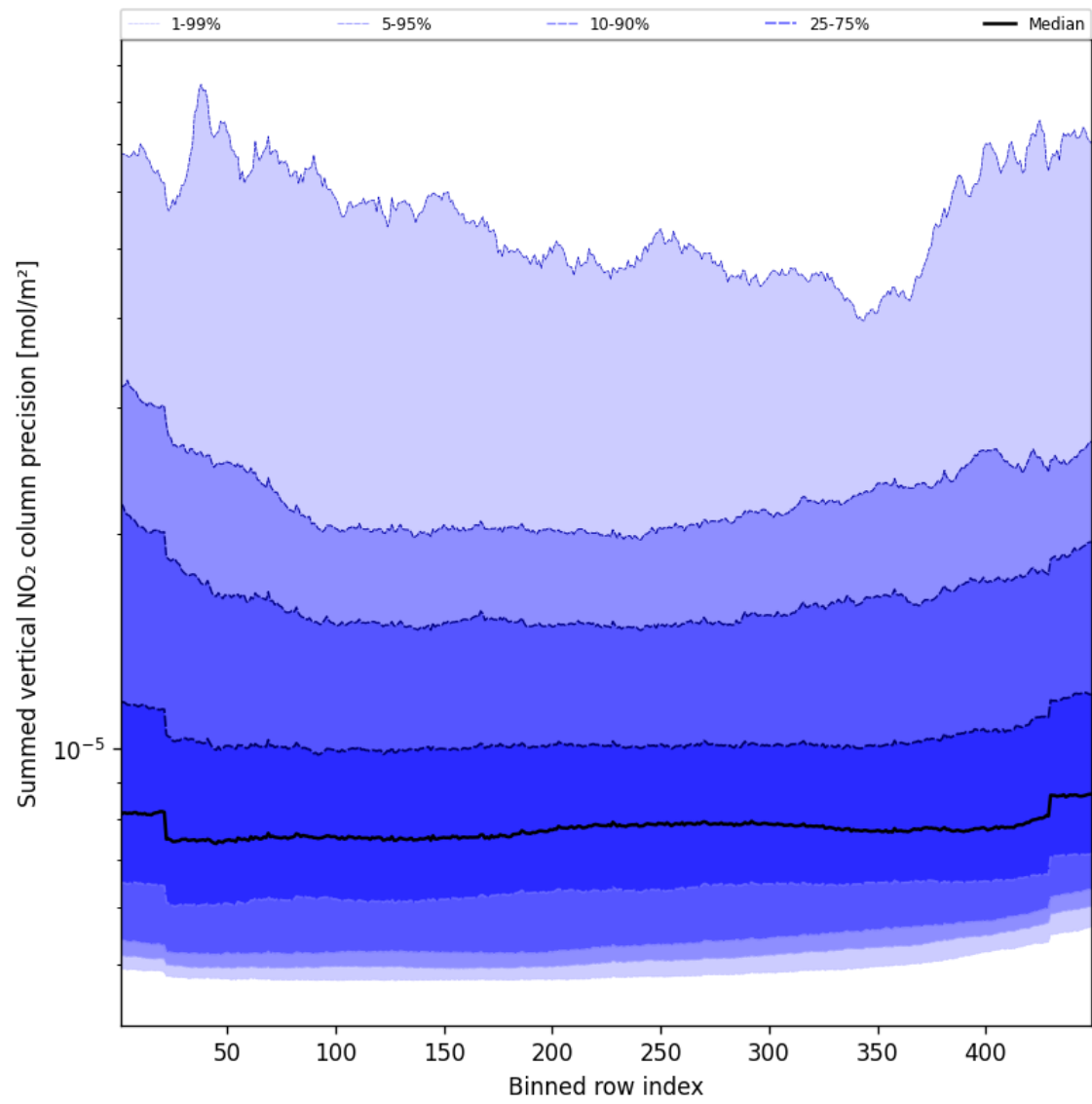
Figure 56: Along track statistics of “Summed vertical NO 2 column precision” for 2025-10-03 to 2025-10-04
