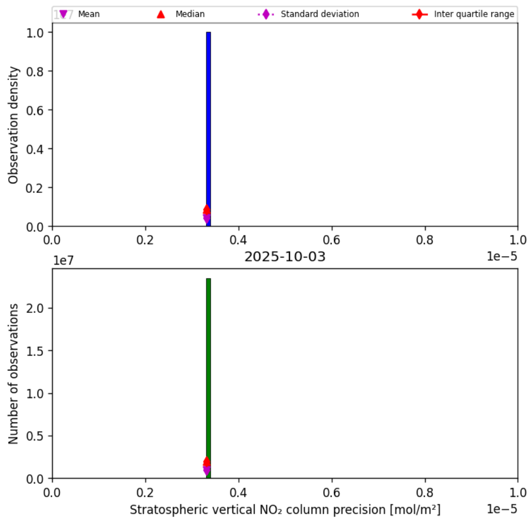
Figure 35: Histogram of “Stratospheric vertical NO 2 column precision” for 2025-10-03 to 2025-10-04
