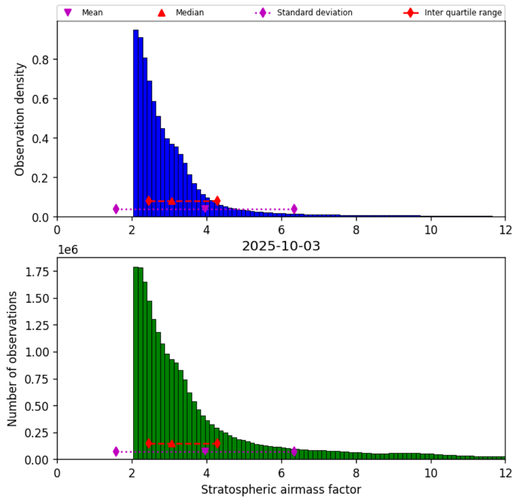
Figure 42: Histogram of “Stratospheric airmass factor” for 2025-10-03 to 2025-10-04
