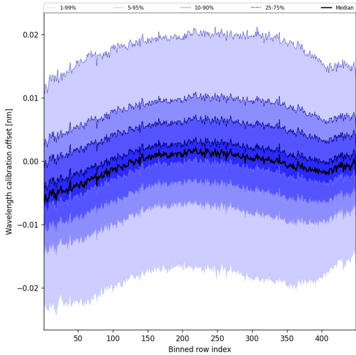
Figure 50: Along track statistics of “Wavelength calibration offset” for 2025-10-03 to 2025-10-04
