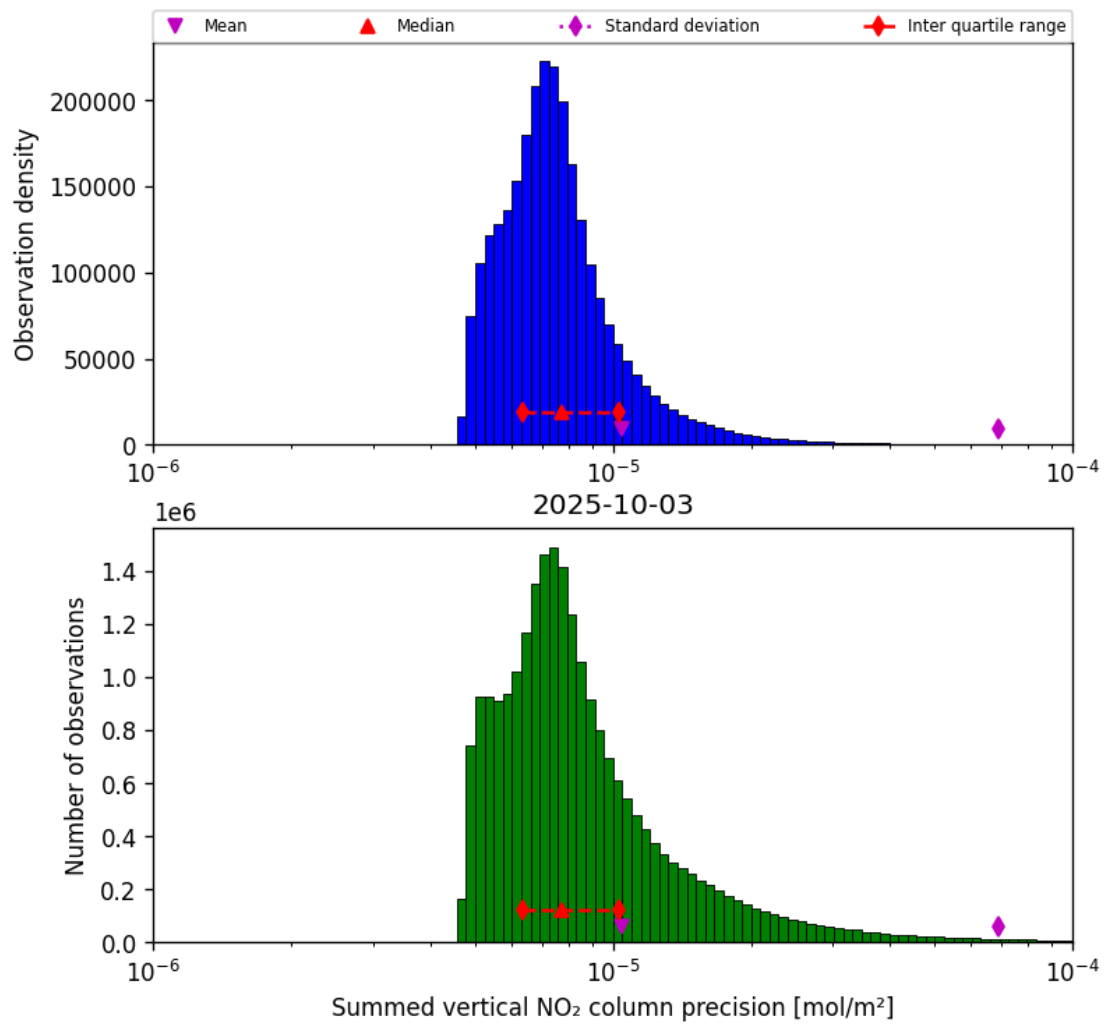
Figure 39: Histogram of "Summed vertical NO 2 column precision" for 2025-10-03 to 2025-10-04
