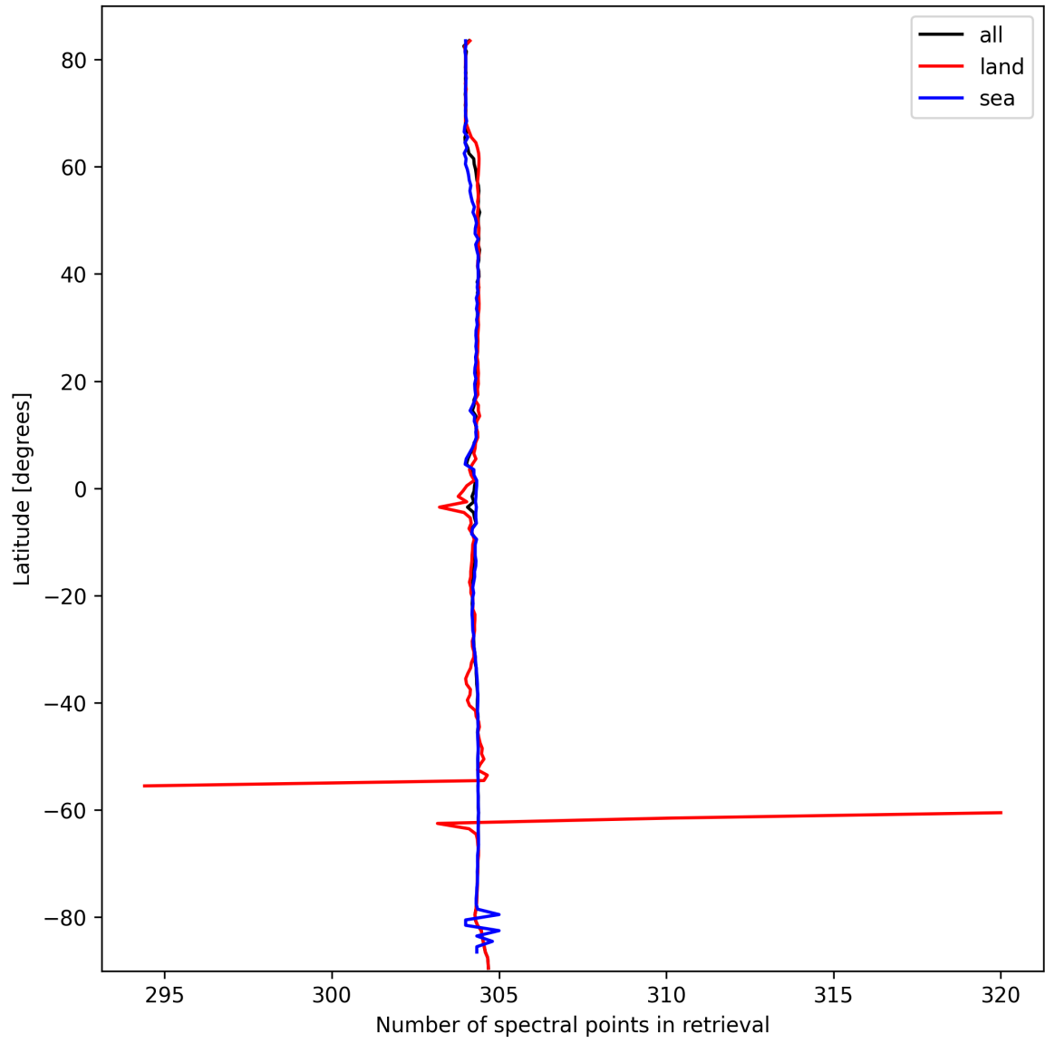
Figure 14: Zonal average of “Number of spectral points in retrieval” for 2025-10-03 to 2025-10-04.
