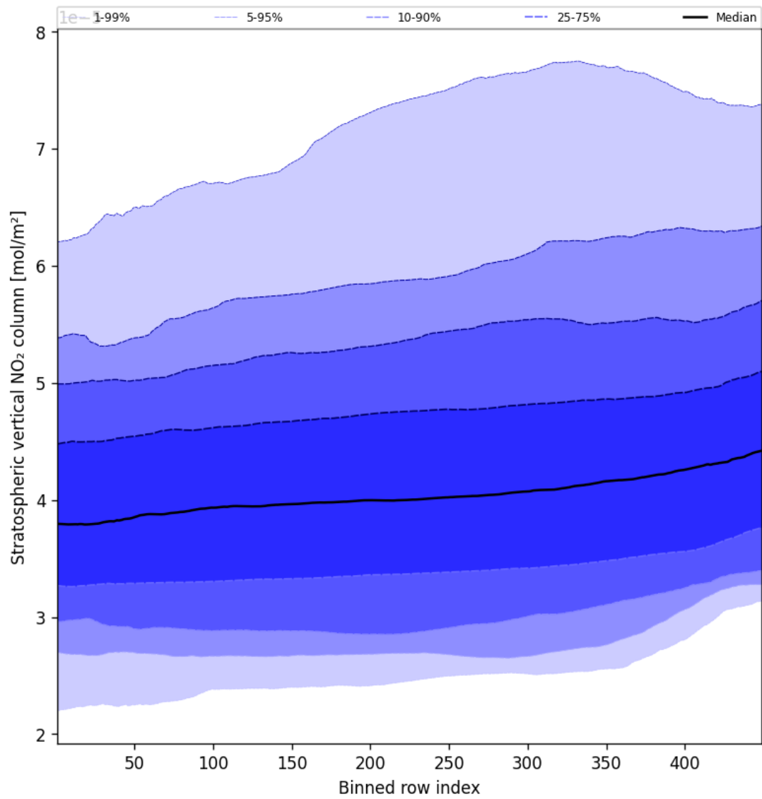
Figure 51: Along track statistics of “Stratospheric vertical NO 2 column” for 2025-10-03 to 2025-10-04
