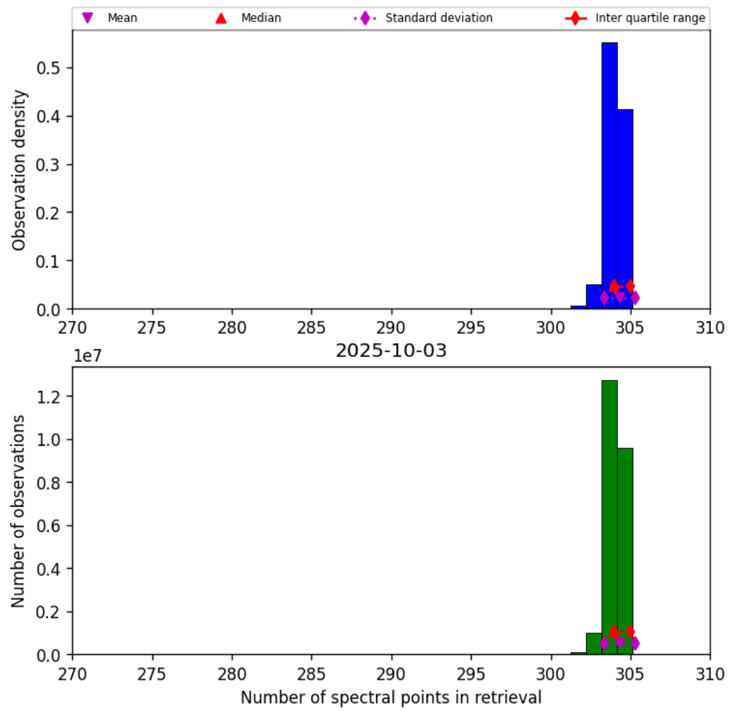
Figure 31: Histogram of “Number of spectral points in retrieval” for 2025-10-03 to 2025-10-04
