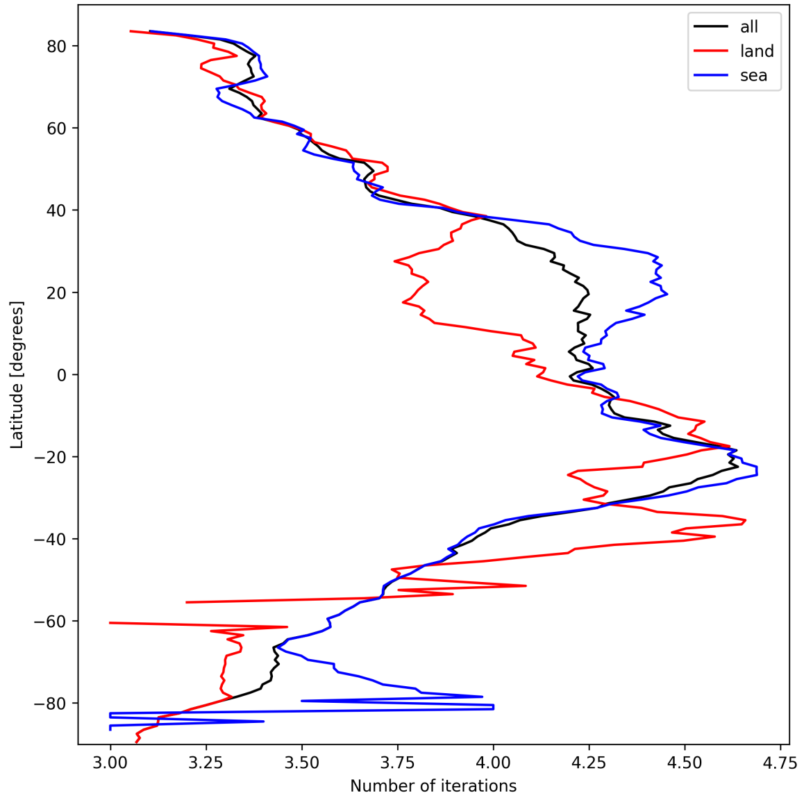
Figure 15: Zonal average of “Number of iterations” for 2025-10-03 to 2025-10-04.
