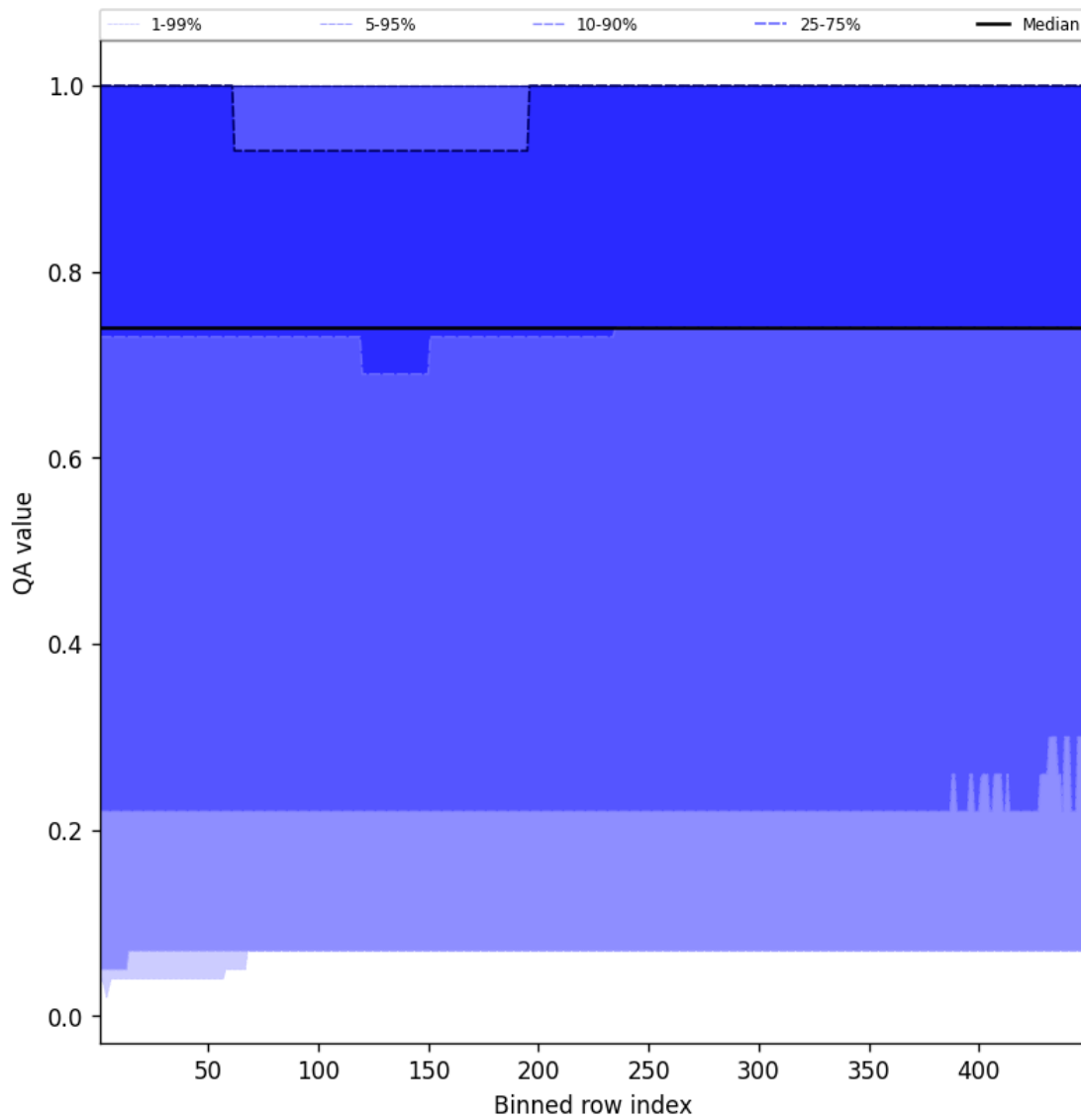
Figure 43: Along track statistics of "QA value" for 2025-10-03 to 2025-10-04
