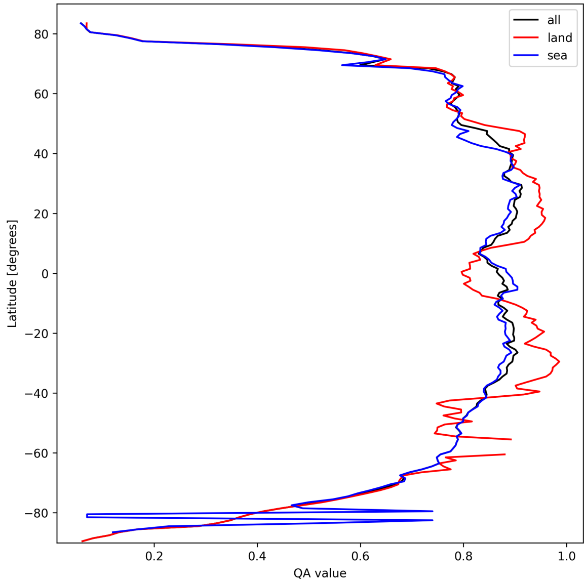
Figure 9: Zonal average of “QA value” for 2025-10-03 to 2025-10-04.
