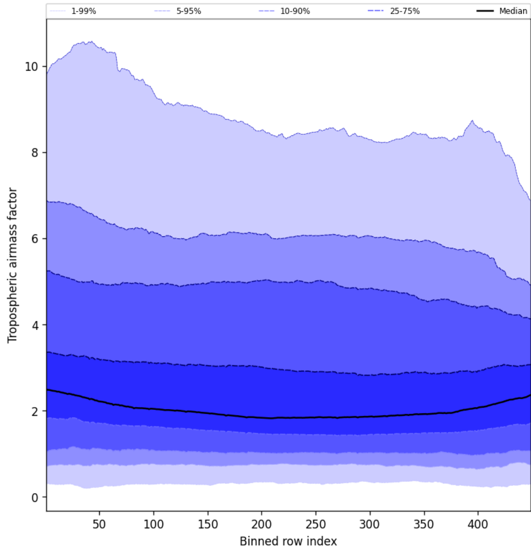
Figure 46: Along track statistics of “Tropospheric air mass factor” for 2025-10-03 to 2025-10-04
