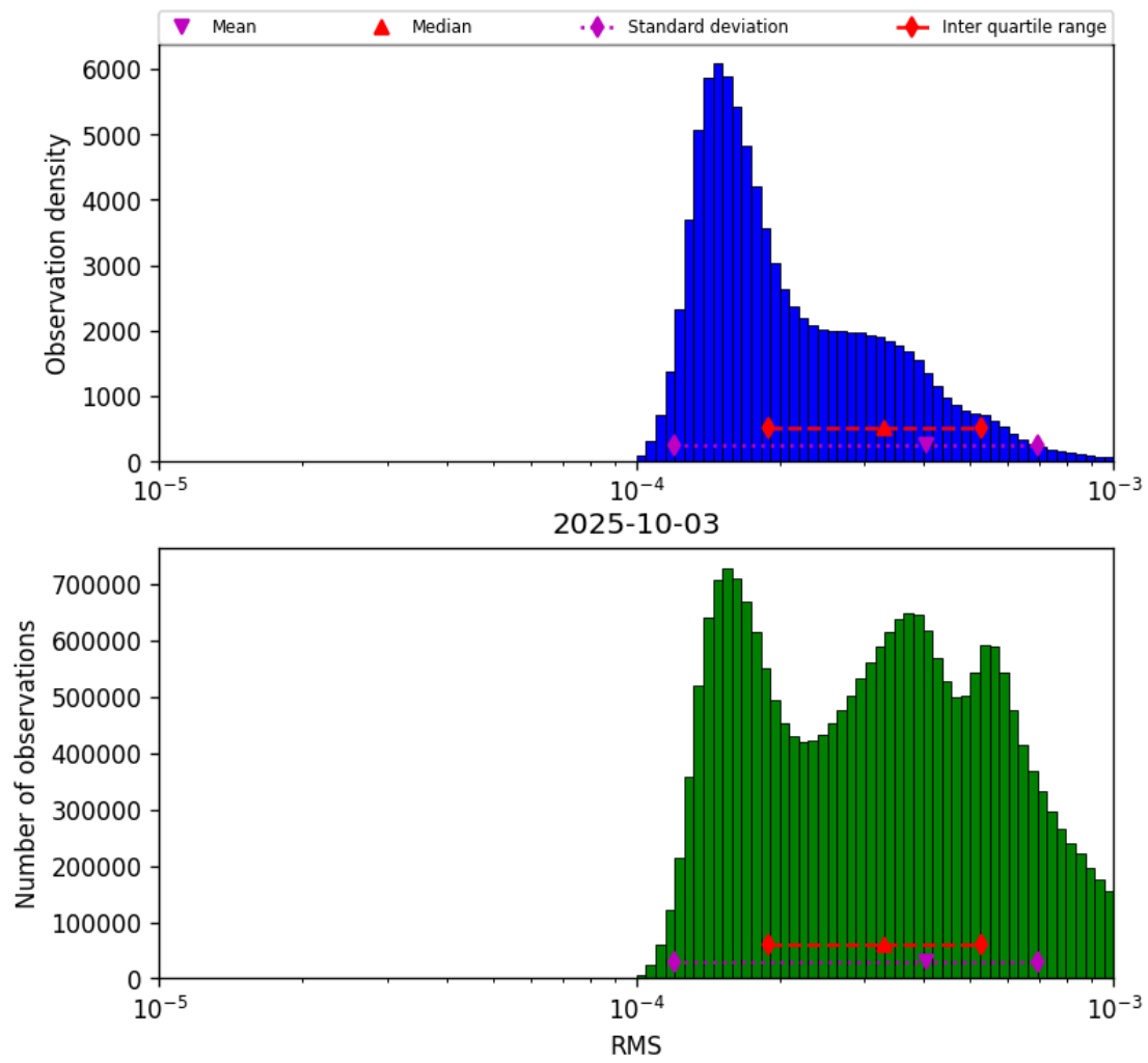
Figure 41: Histogram of “RMS” for 2025-10-03 to 2025-10-04
