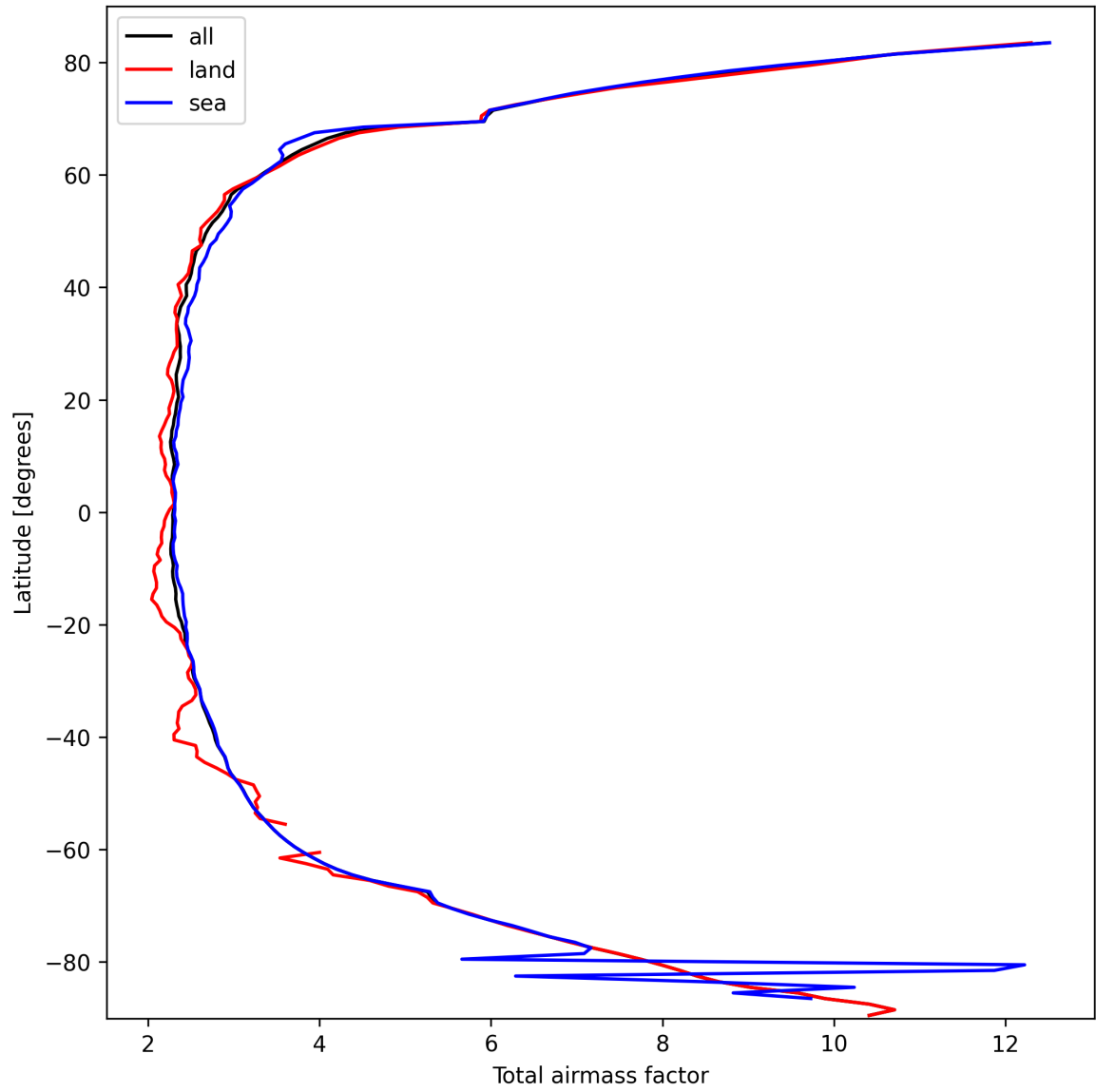
Figure 13: Zonal average of “Total airmass factor” for 2025-10-03 to 2025-10-04.
