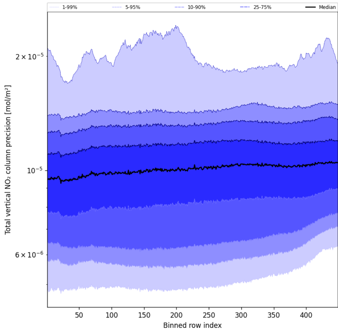
Figure 54: Along track statistics of “Total vertical NO 2 column precision” for 2025-10-03 to 2025-10-04
