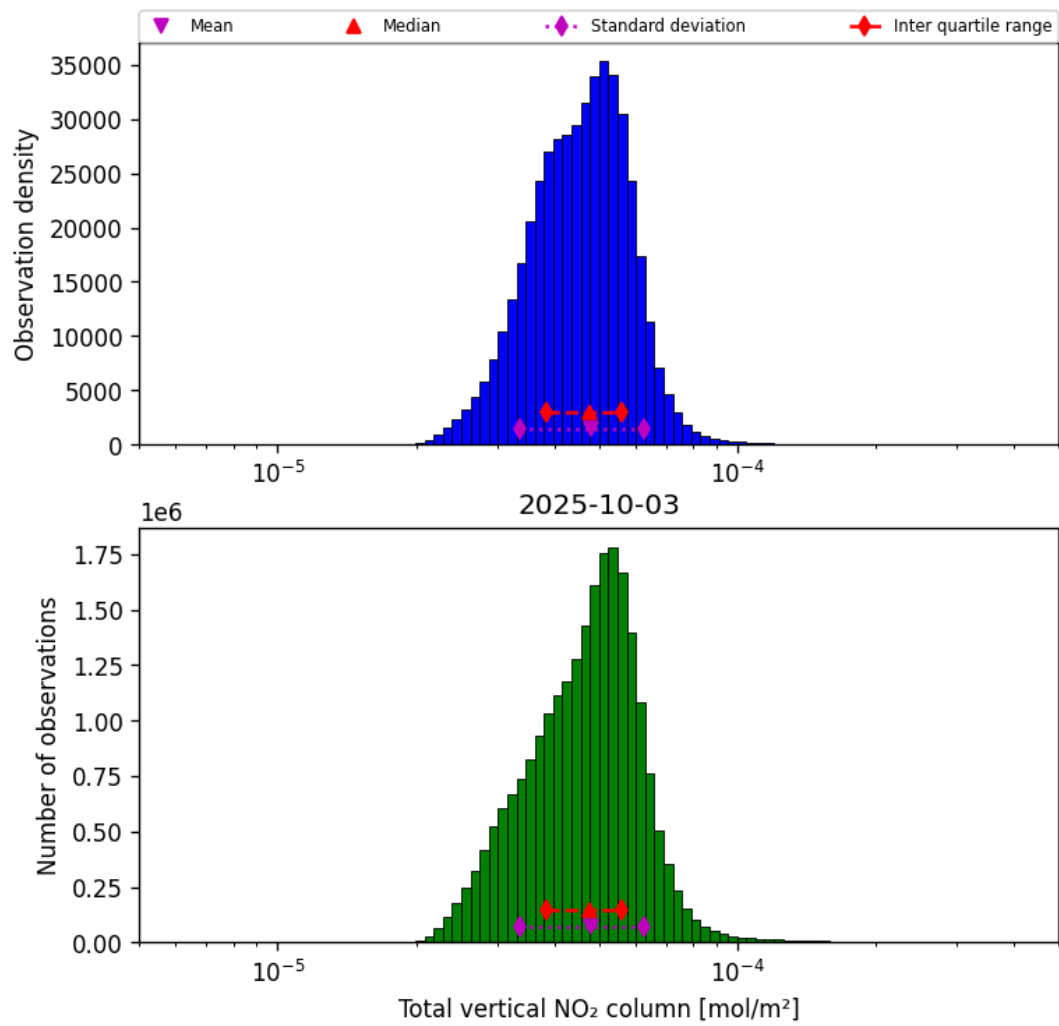
Figure 36: Histogram of “Total vertical NO 2 column” for 2025-10-03 to 2025-10-04
