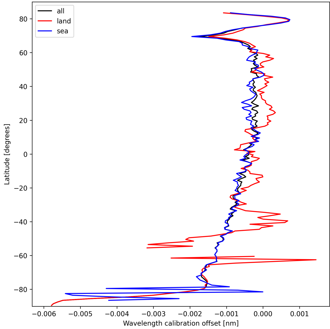
Figure 16: Zonal average of “Wavelength calibration offset” for 2025-10-03 to 2025-10-04.
