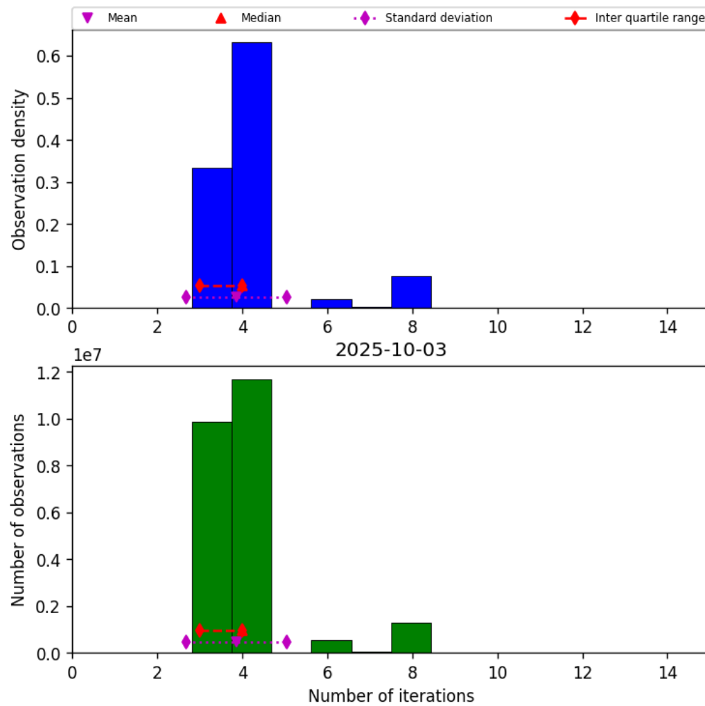
Figure 32: Histogram of “Number of iterations” for 2025-10-03 to 2025-10-04
