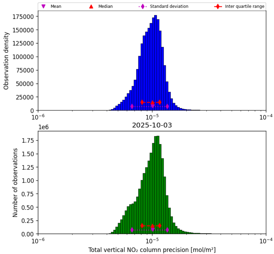
Figure 37: Histogram of "Total vertical NO 2 column precision" for 2025-10-03 to 2025-10-04
