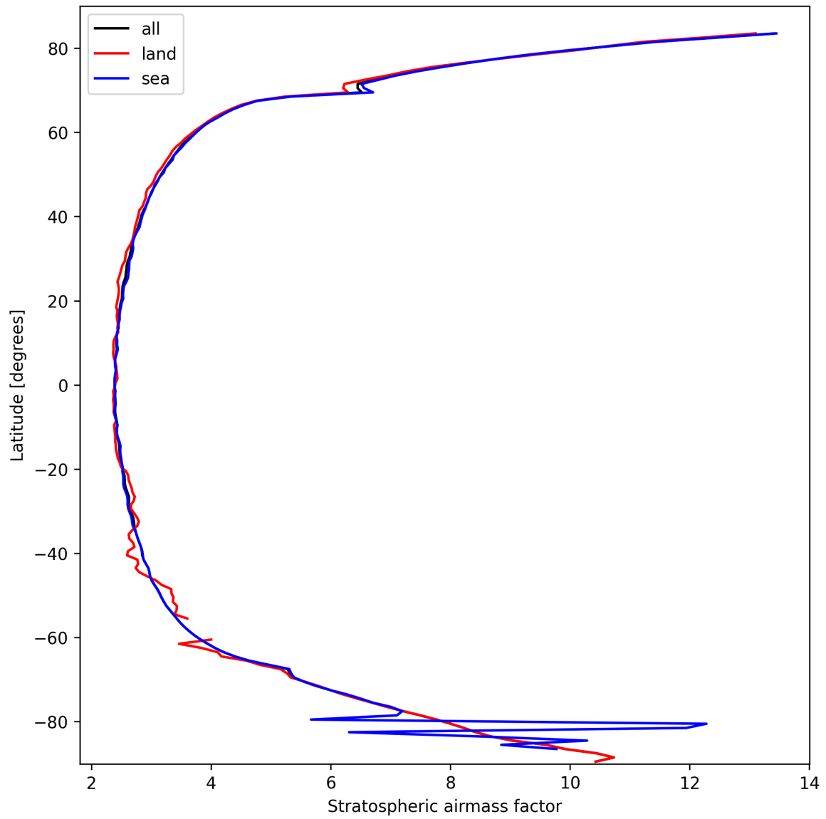
Figure 25: Zonal average of “Stratospheric airmass factor” for 2025-10-03 to 2025-10-04.
