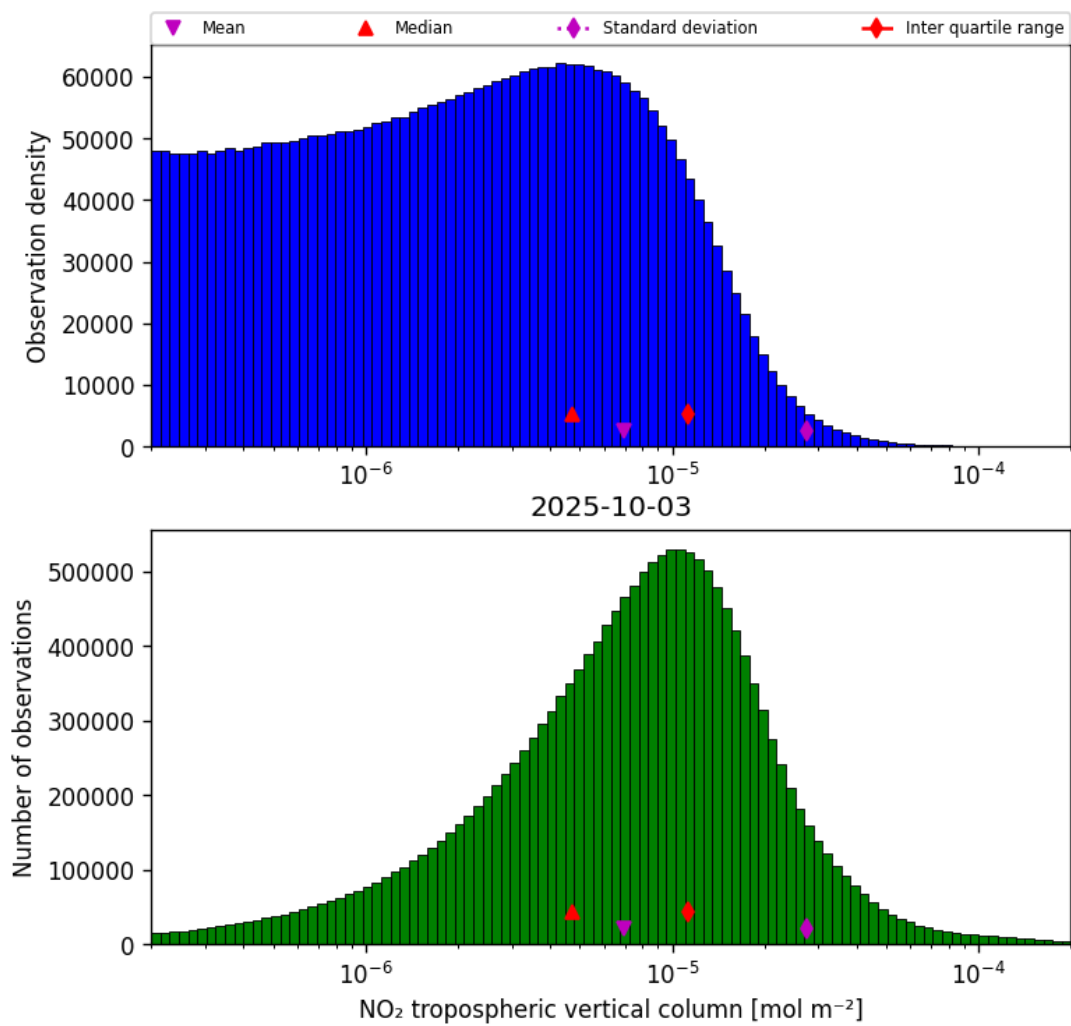
Figure 27: Histogram of “NO 2 tropospheric vertical column” for 2025-10-03 to 2025-10-04
