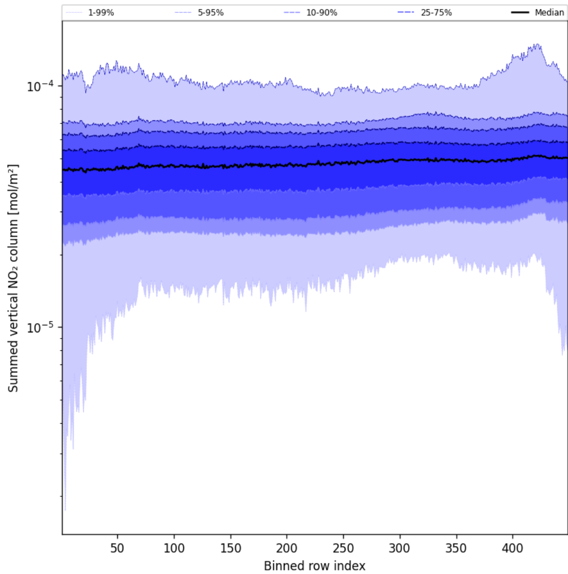
Figure 55: Along track statistics of “Summed vertical NO 2 column” for 2025-10-03 to 2025-10-04
