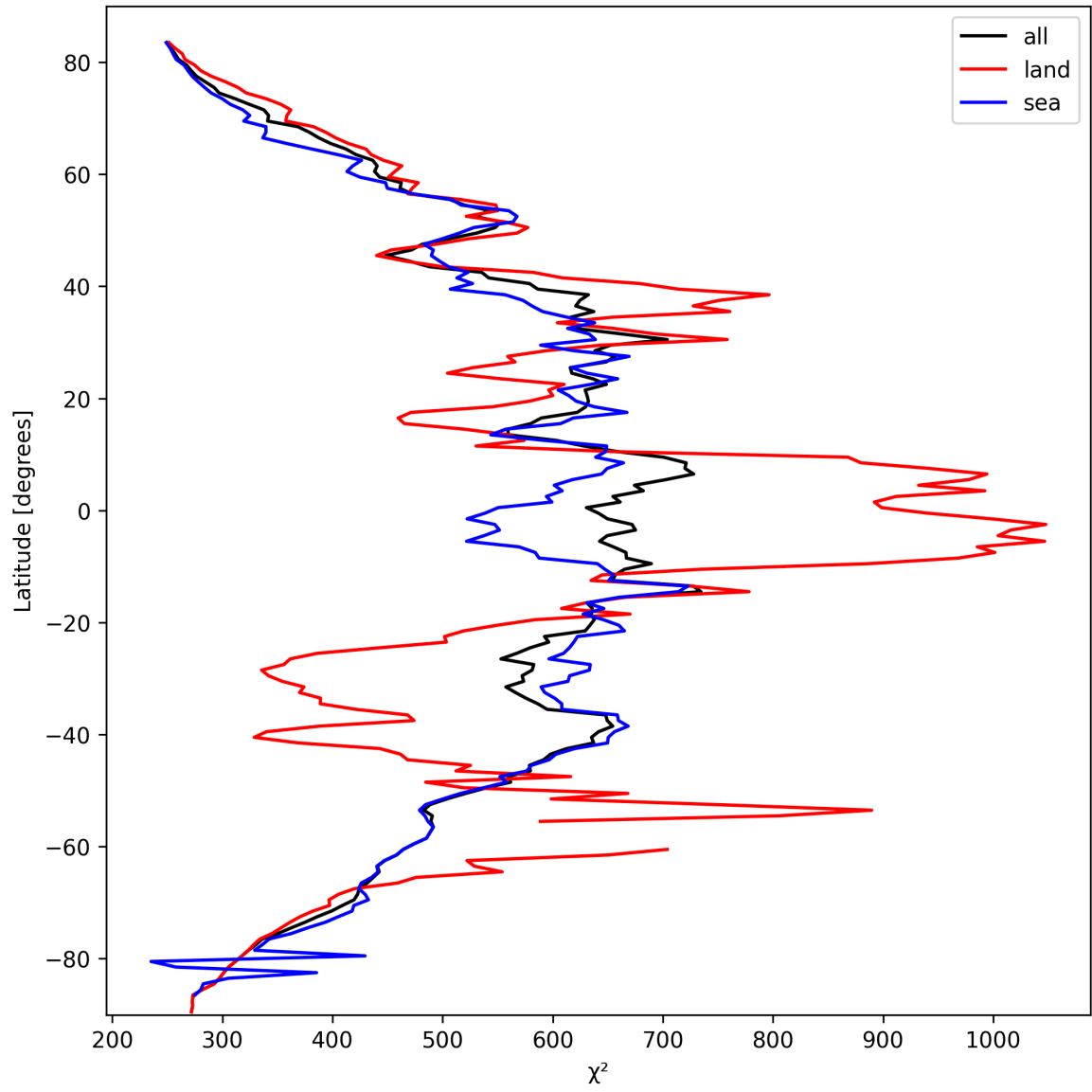
Figure 23: Zonal average of “ \chi^2 ” for 2025-10-03 to 2025-10-04.
