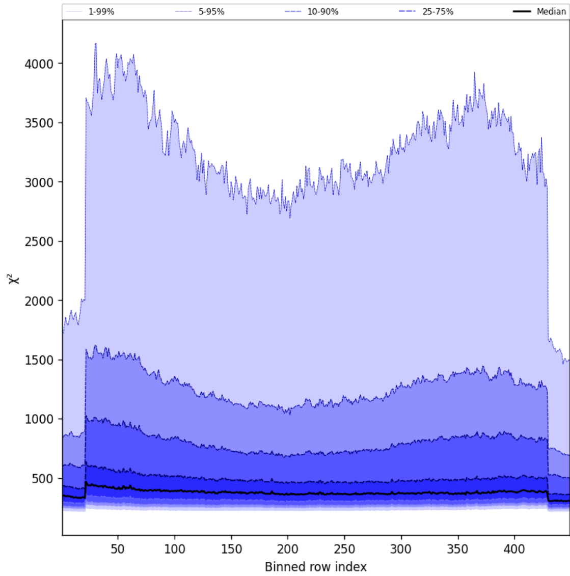
Figure 57: Along track statistics of “ \chi^2 ” for 2025-10-03 to 2025-10-04
