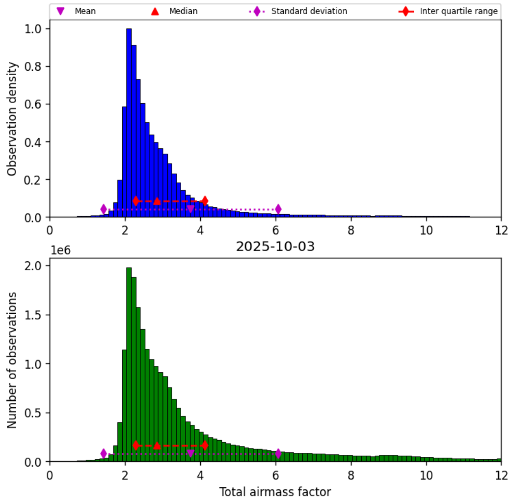
Figure 30: Histogram of “Total airmass factor” for 2025-10-03 to 2025-10-04
