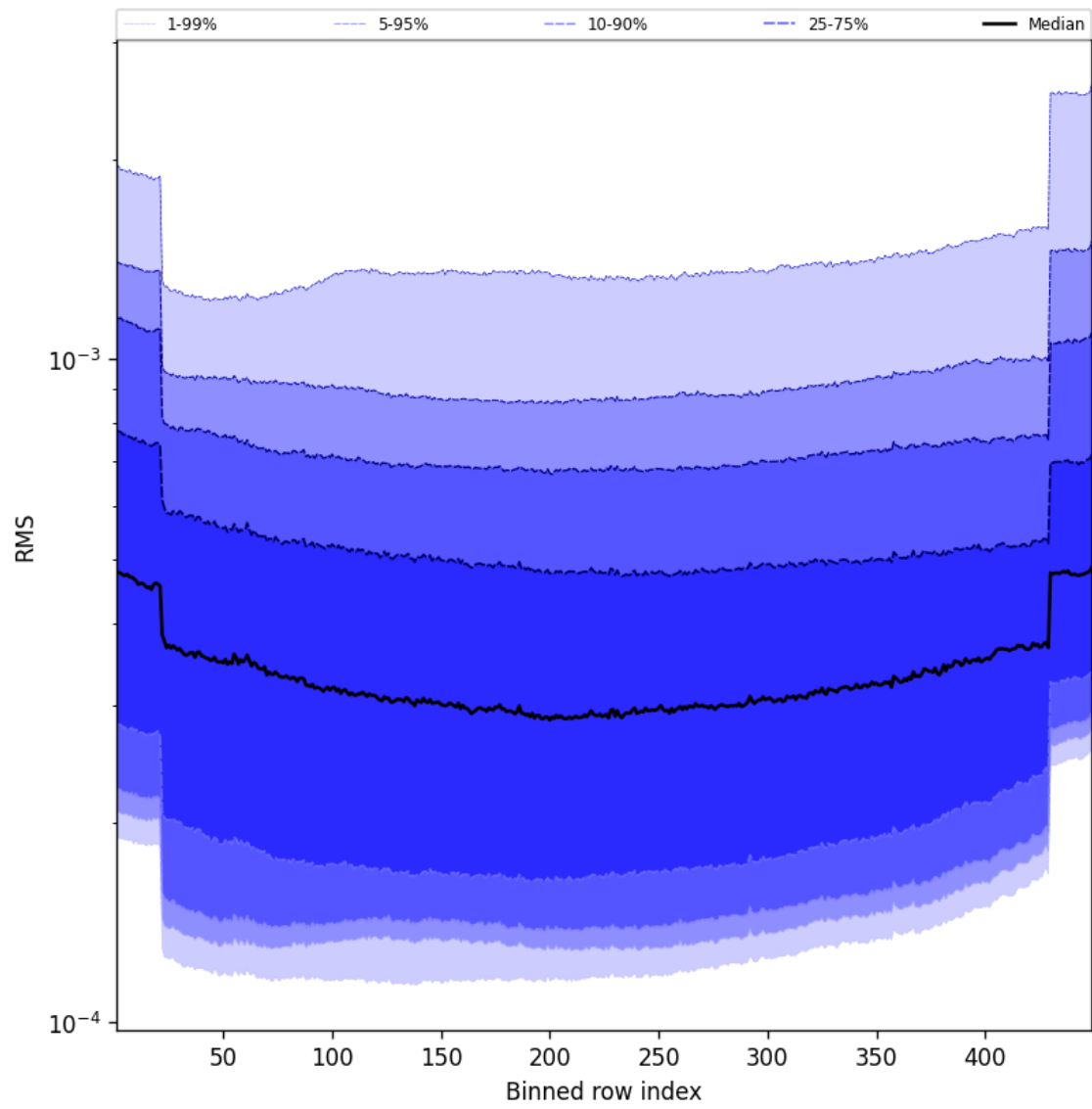
Figure 58: Along track statistics of “RMS” for 2025-10-03 to 2025-10-04
