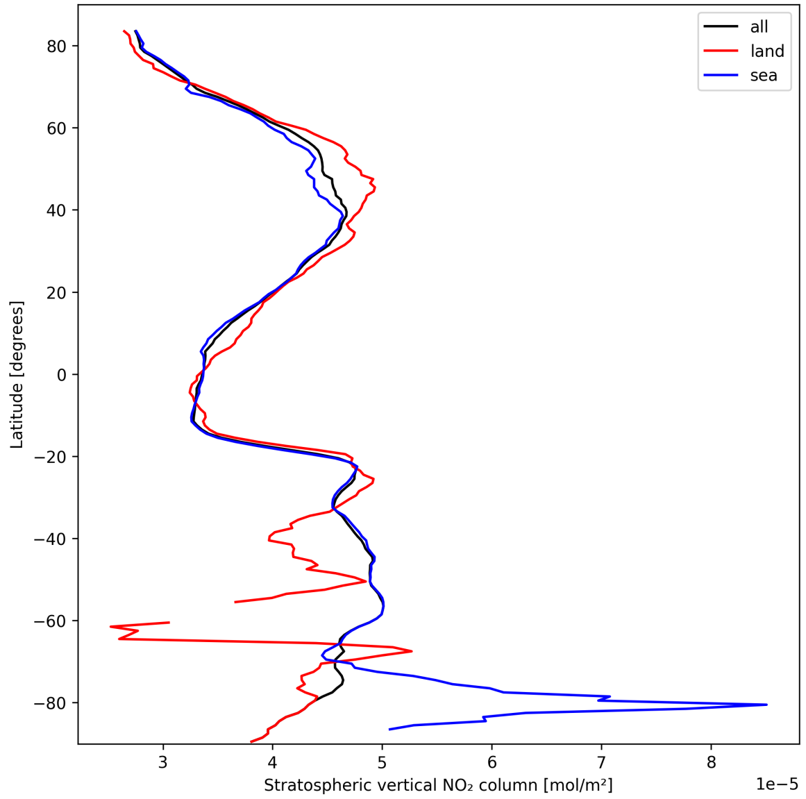
Figure 17: Zonal average of “Stratospheric vertical NO 2 column” for 2025-10-03 to 2025-10-04.
