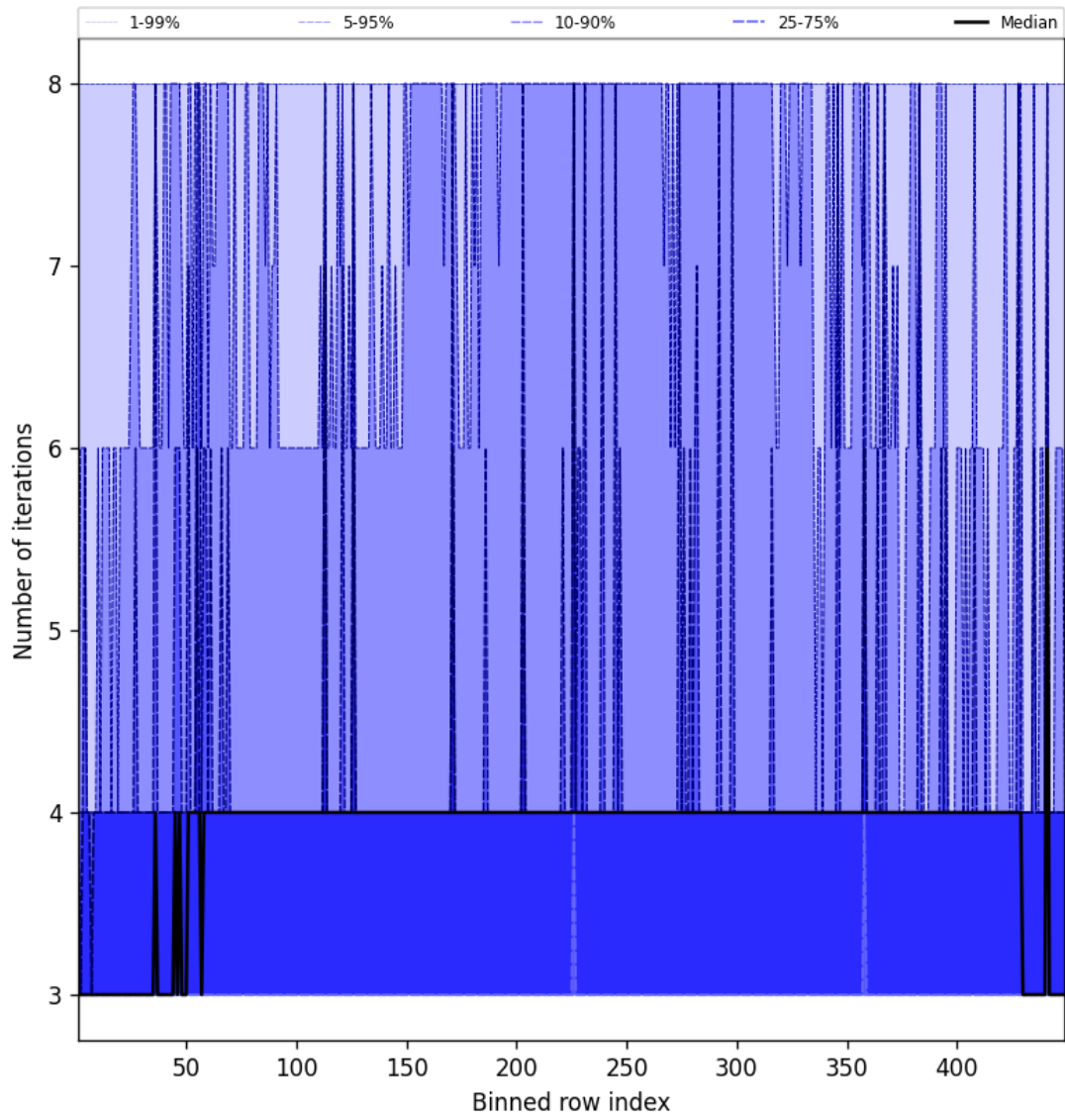
Figure 49: Along track statistics of “Number of iterations” for 2025-10-03 to 2025-10-04
