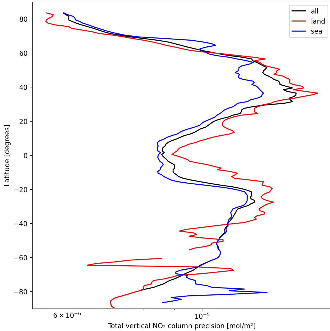
Figure 20: Zonal average of “Total vertical NO 2 column precision” for 2025-10-03 to 2025-10-04.
