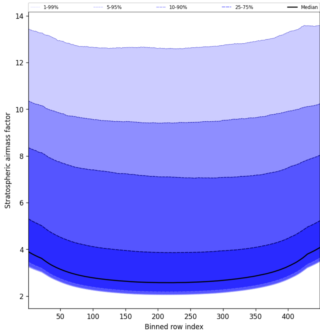
Figure 59: Along track statistics of “Stratospheric airmass factor” for 2025-10-03 to 2025-10-04
