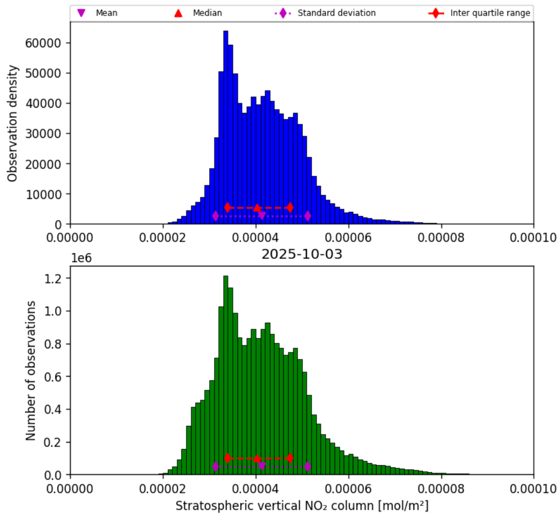
Figure 34: Histogram of “Stratospheric vertical NO 2 column” for 2025-10-03 to 2025-10-04
