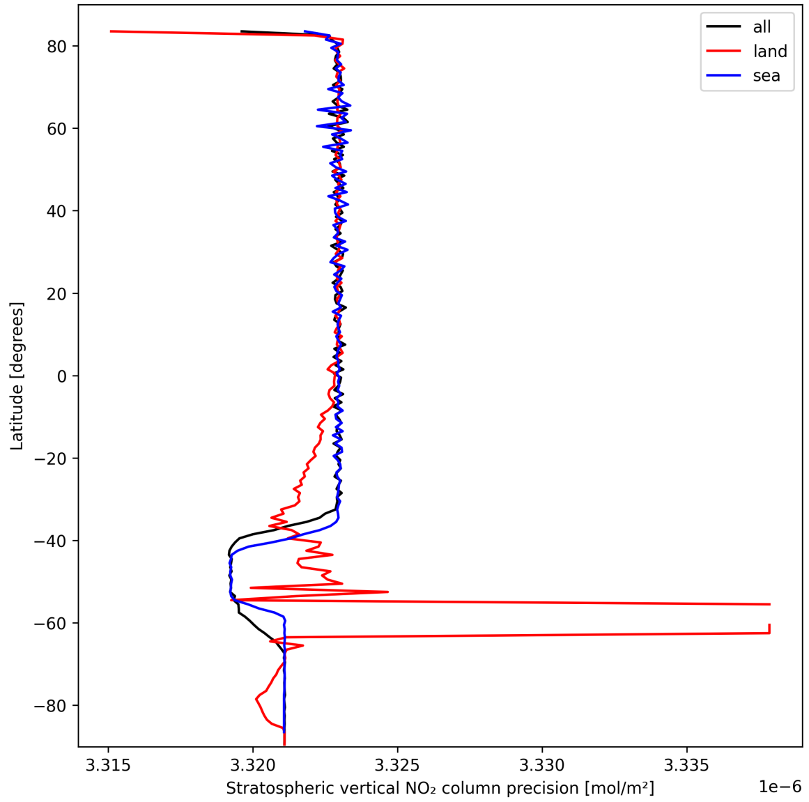
Figure 18: Zonal average of “Stratospheric vertical NO 2 column precision” for 2025-10-03 to 2025-10-04.
