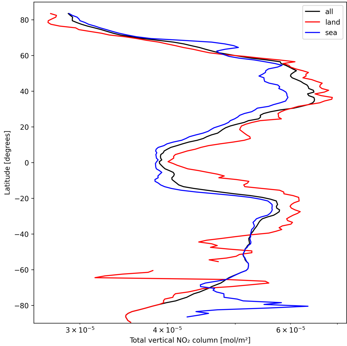
Figure 19: Zonal average of “Total vertical NO 2 column” for 2025-10-03 to 2025-10-04.
