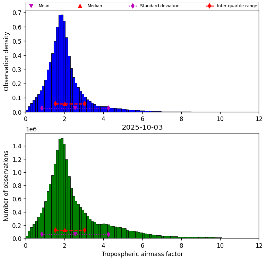
Figure 29: Histogram of “Tropospheric airmass factor” for 2025-10-03 to 2025-10-04
