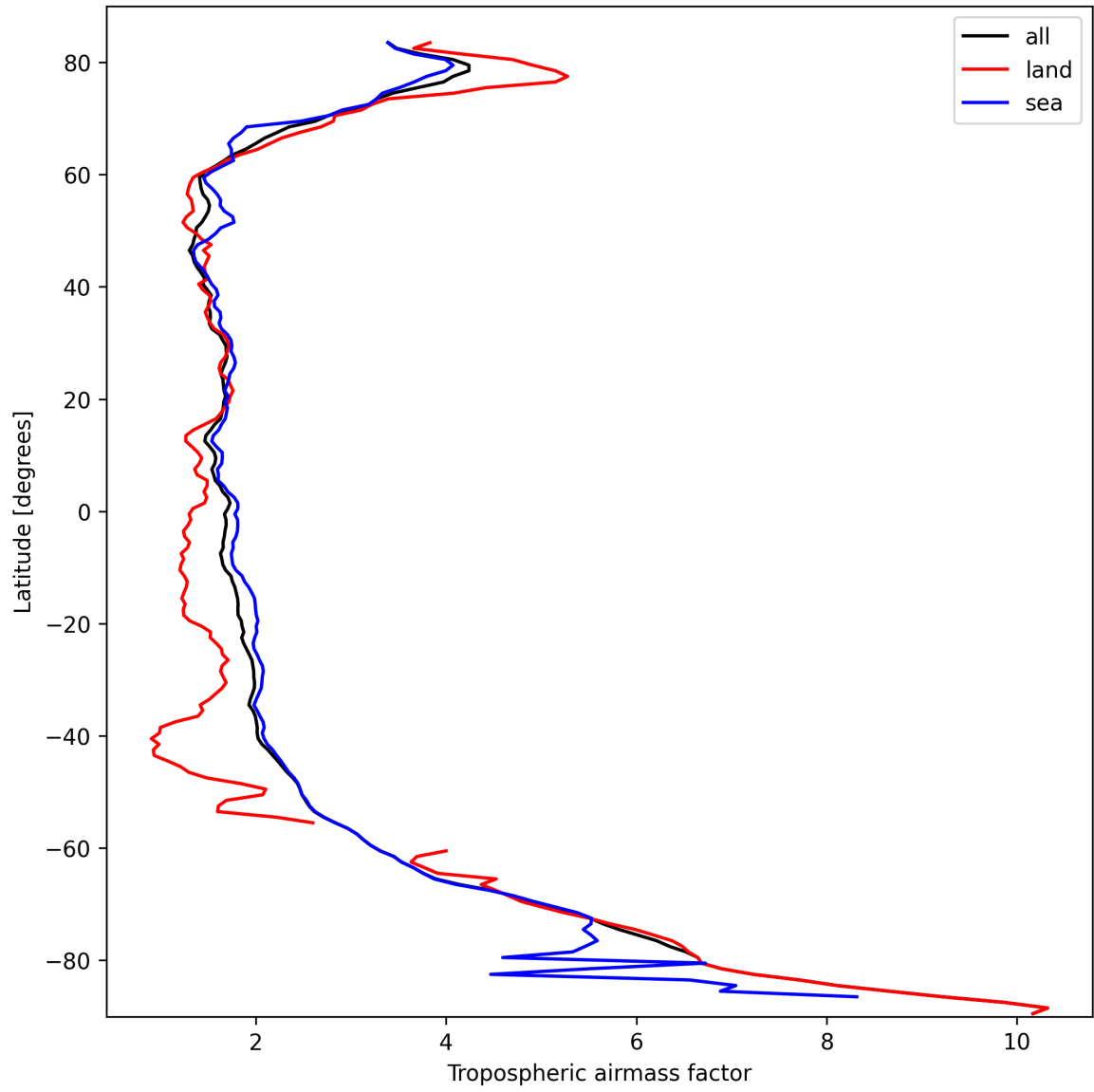
Figure 12: Zonal average of “Tropospheric airmass factor” for 2025-10-03 to 2025-10-04.
