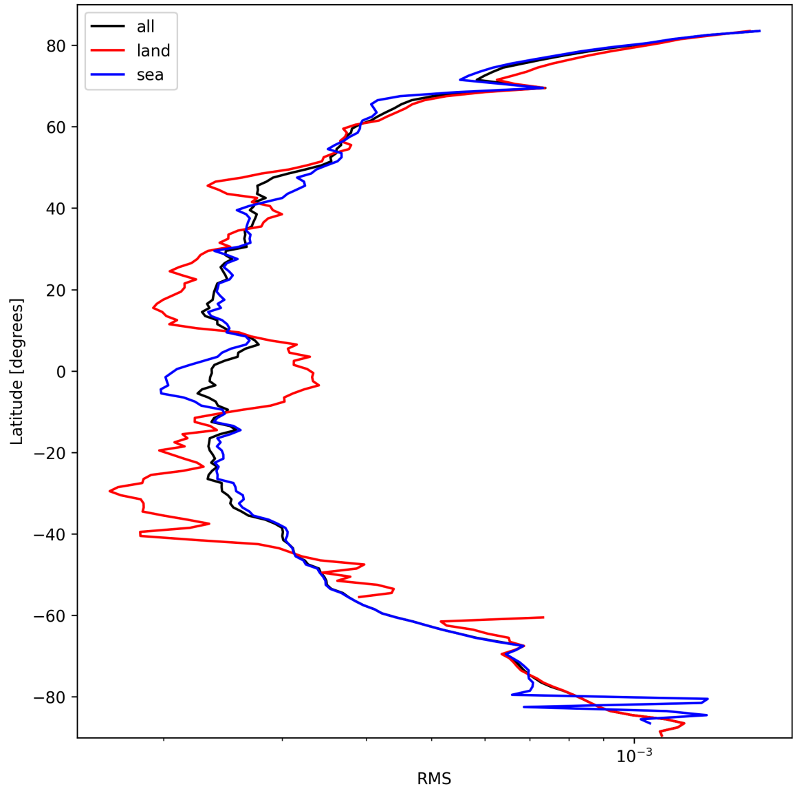
Figure 24: Zonal average of “RMS” for 2025-10-03 to 2025-10-04.
