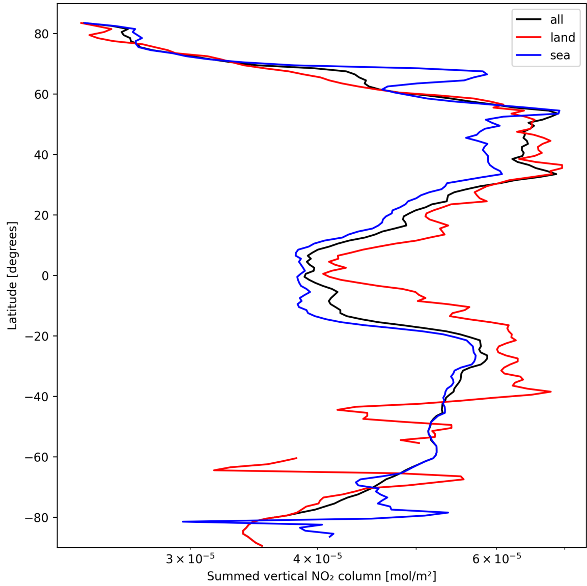
Figure 21: Zonal average of “Summed vertical NO 2 column” for 2025-10-03 to 2025-10-04.
