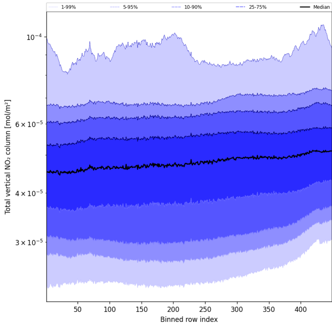
Figure 53: Along track statistics of “Total vertical NO 2 column” for 2025-10-03 to 2025-10-04
