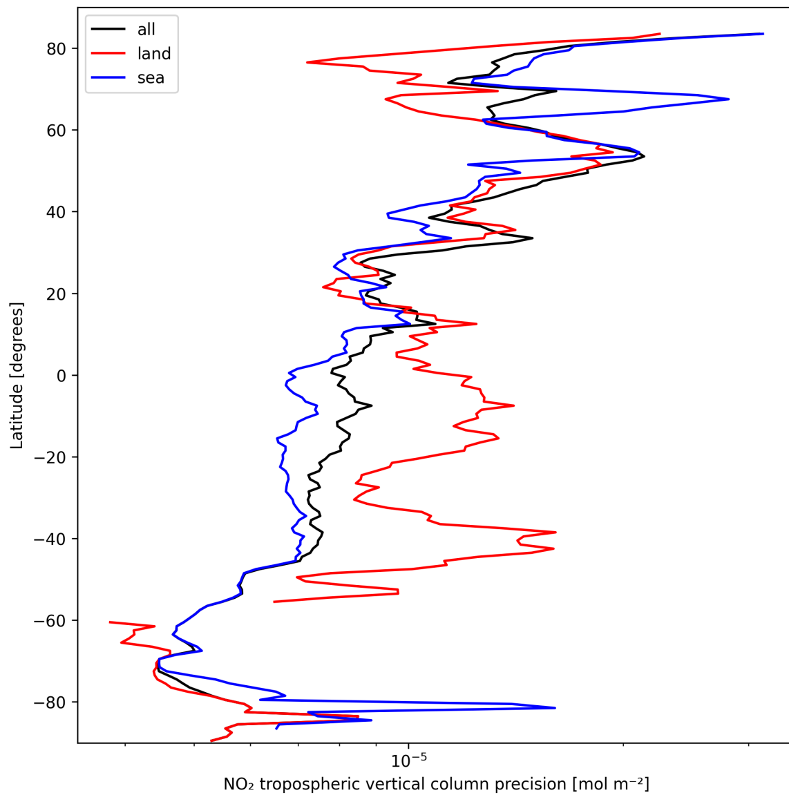
Figure 11: Zonal average of "NO 2 tropospheric vertical column precision" for 2025-10-03 to 2025-10-04.
