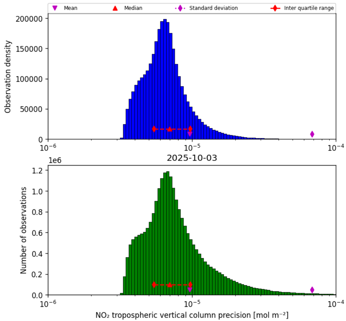
Figure 28: Histogram of “NO 2 tropospheric vertical column precision” for 2025-10-03 to 2025-10-04
