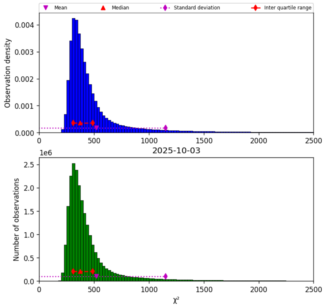
Figure 40: Histogram of “ \chi^2 ” for 2025-10-03 to 2025-10-04
