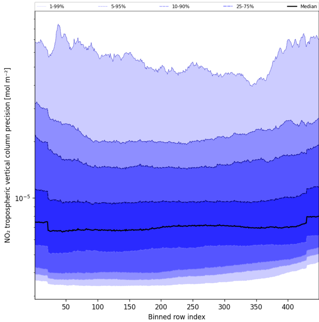
Figure 45: Along track statistics of “NO 2 tropospheric vertical column precision” for 2025-10-03 to 2025-10-04
