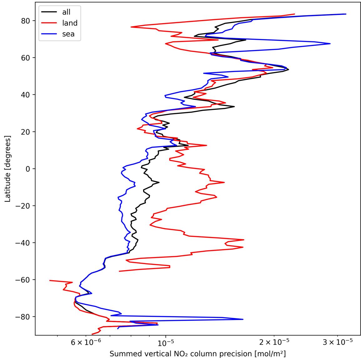
Figure 22: Zonal average of “Summed vertical NO 2 column precision” for 2025-10-03 to 2025-10-04.
