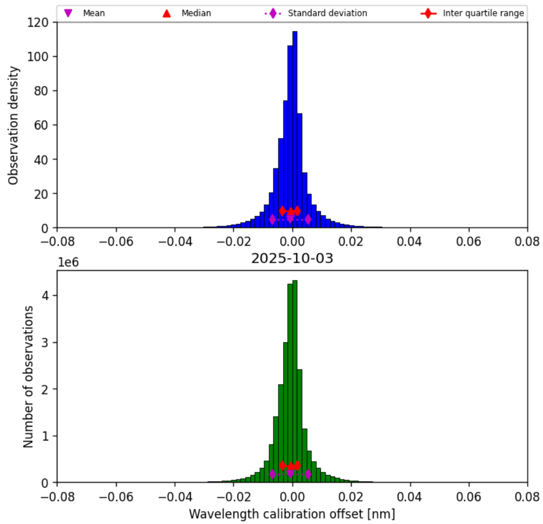
Figure 33: Histogram of “Wavelength calibration offset” for 2025-10-03 to 2025-10-04
