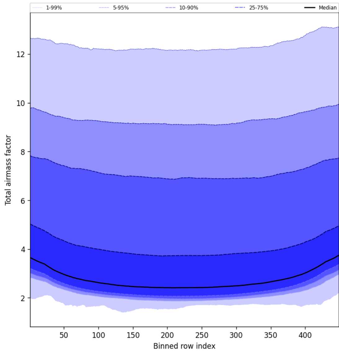
Figure 47: Along track statistics of “Total airmass factor” for 2025-10-03 to 2025-10-04
