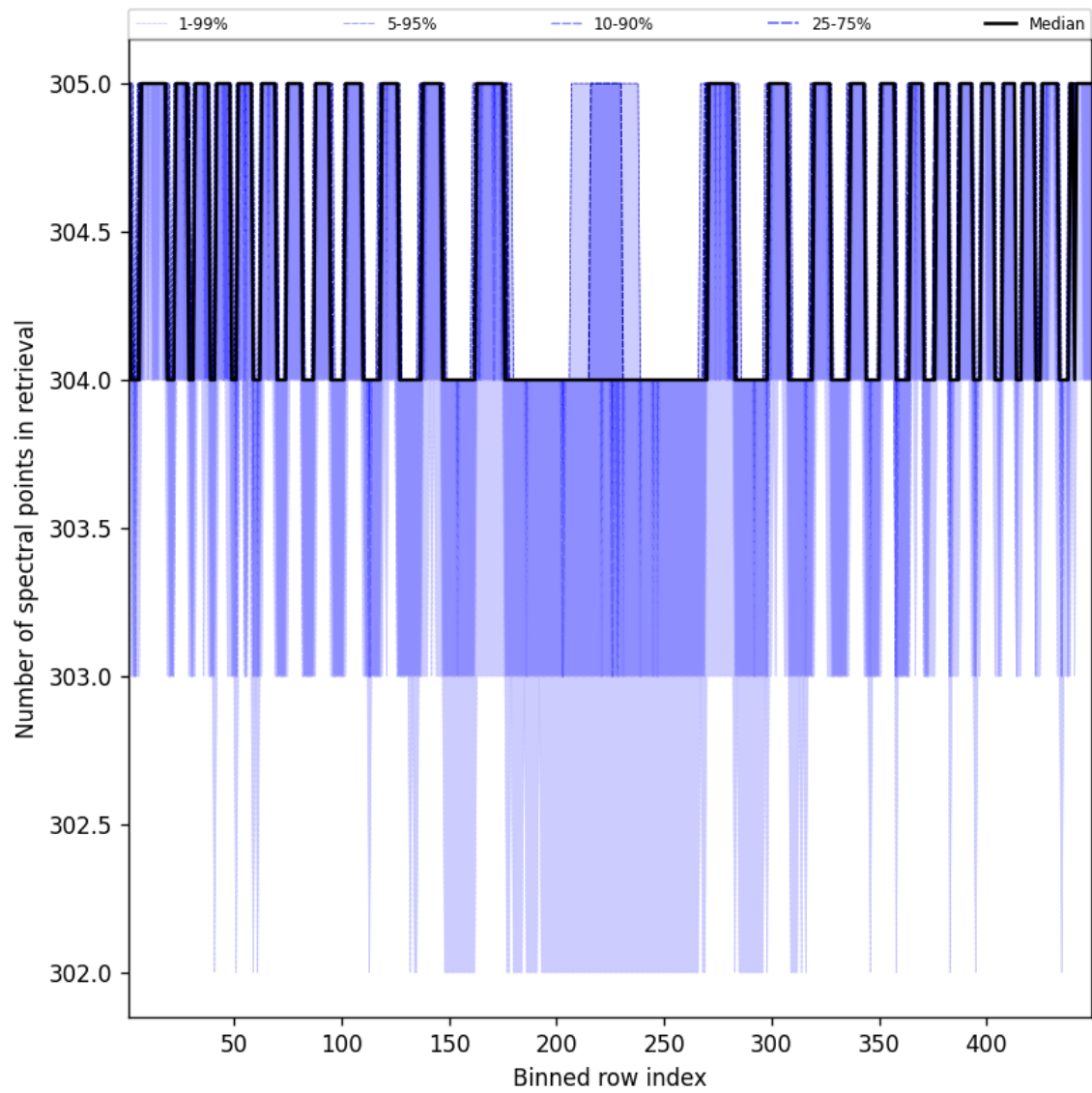
Figure 48: Along track statistics of “Number of spectral points in retrieval” for 2025-10-03 to 2025-10-04
