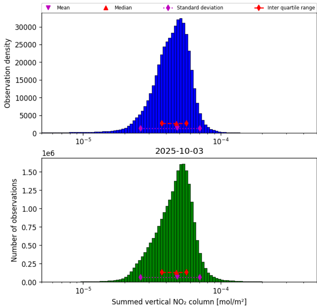
Figure 38: Histogram of “Summed vertical NO 2 column” for 2025-10-03 to 2025-10-04
