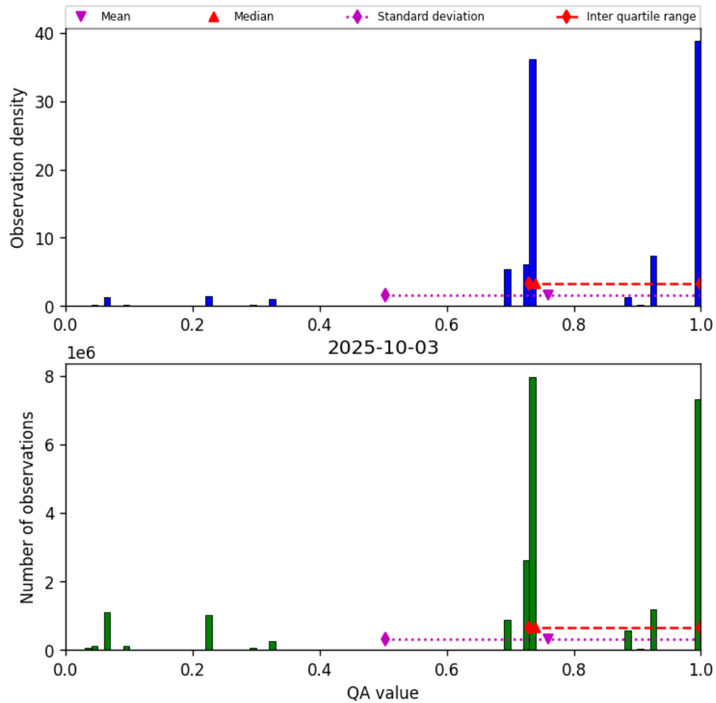
Figure 26: Histogram of “QA value” for 2025-10-03 to 2025-10-04
