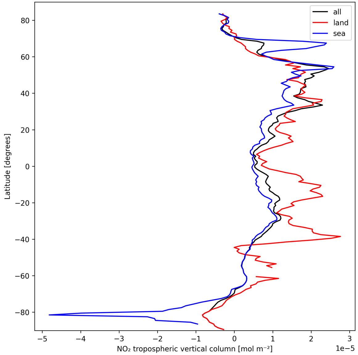
Figure 10: Zonal average of “NO 2 tropospheric vertical column” for 2025-10-03 to 2025-10-04.
