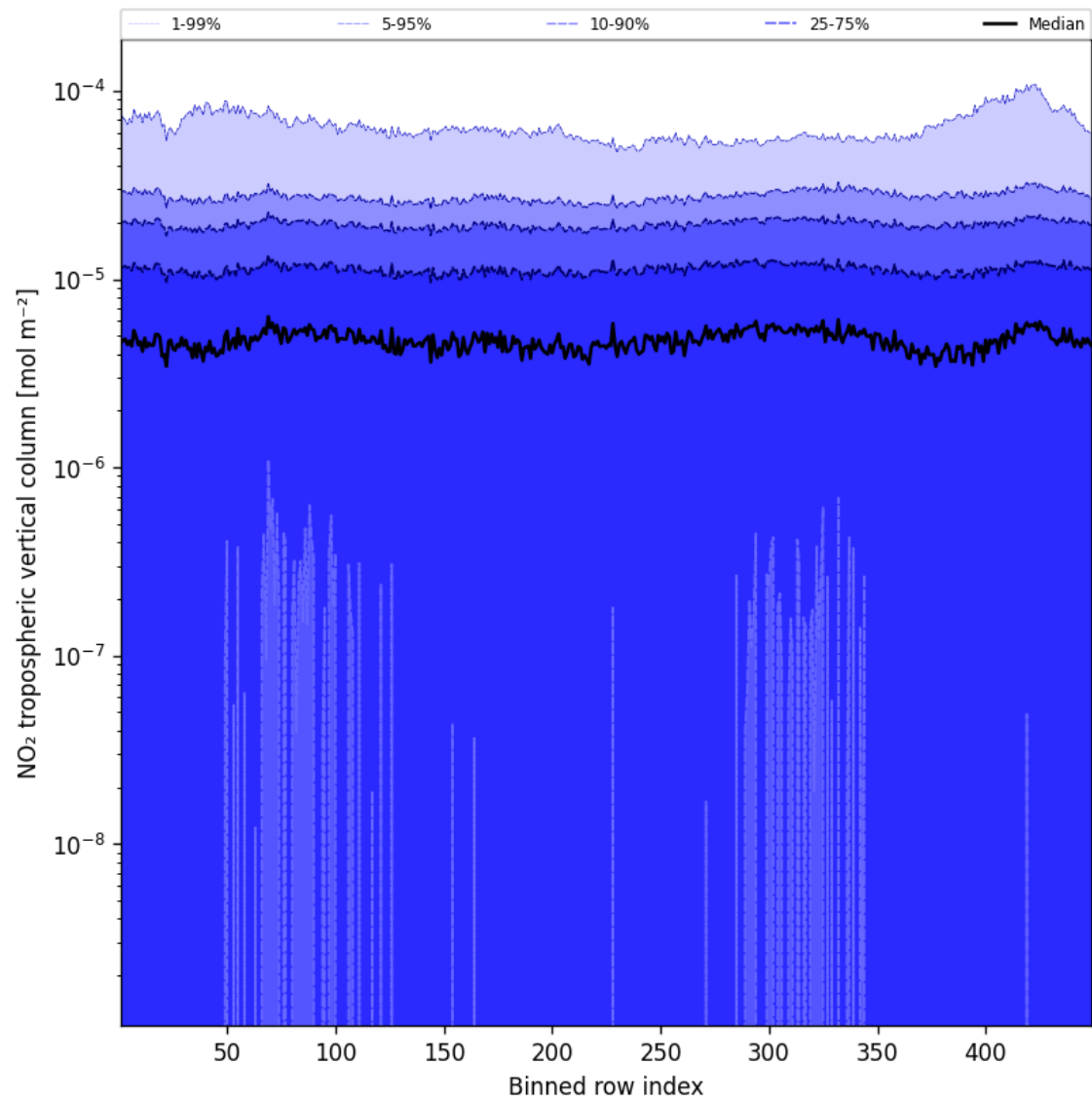
Figure 44: Along track statistics of “NO 2 tropospheric vertical column” for 2025-10-03 to 2025-10-04
