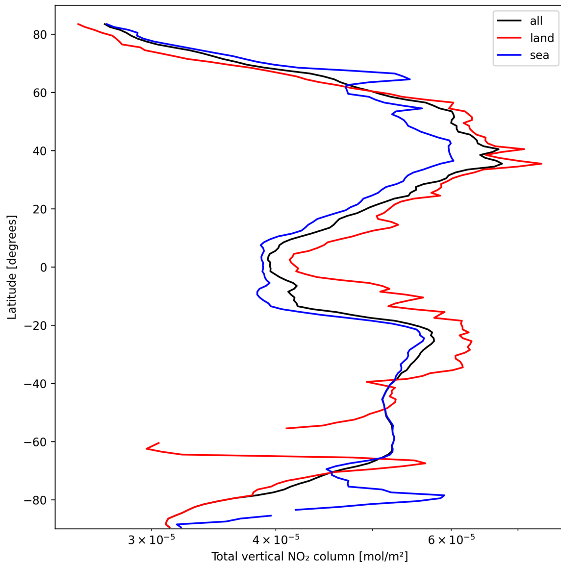
Figure 19: Zonal average of “Total vertical NO 2 column” for 2025-10-04 to 2025-10-04.
