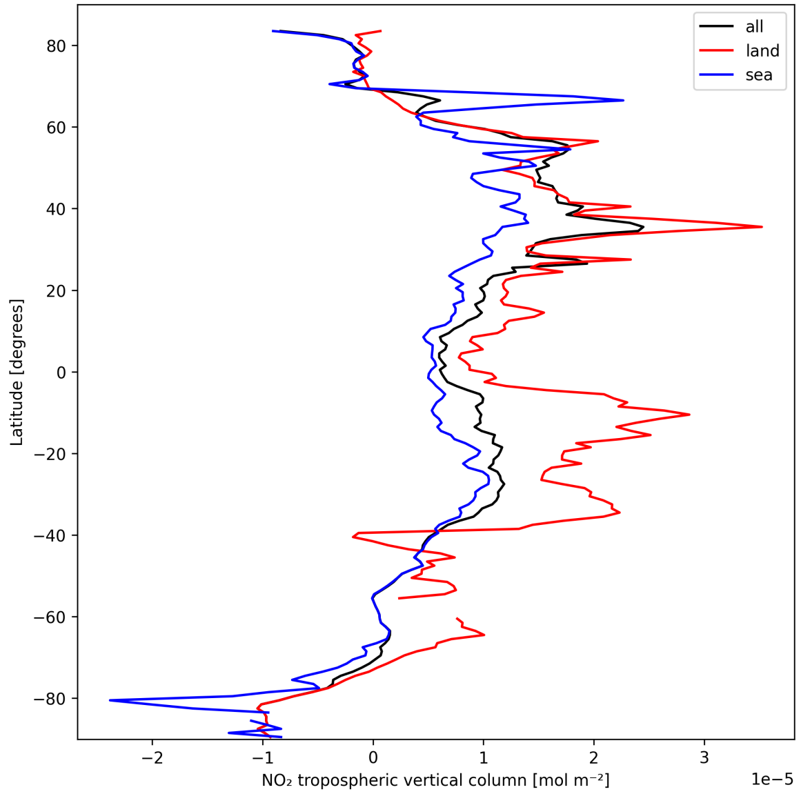
Figure 10: Zonal average of “NO 2 tropospheric vertical column” for 2025-10-04 to 2025-10-04.
