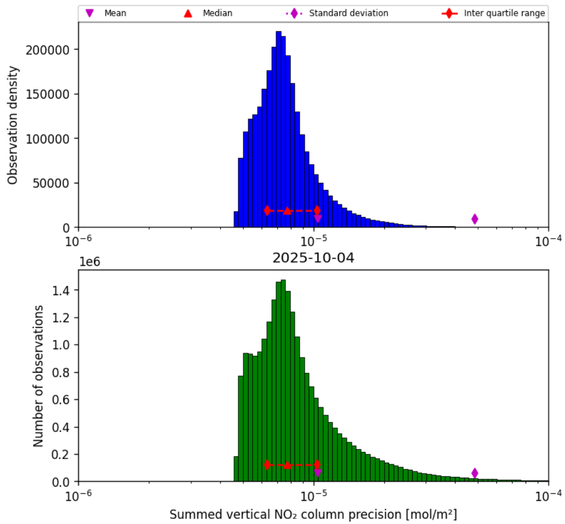
Figure 39: Histogram of "Summed vertical NO 2 column precision" for 2025-10-04 to 2025-10-04
