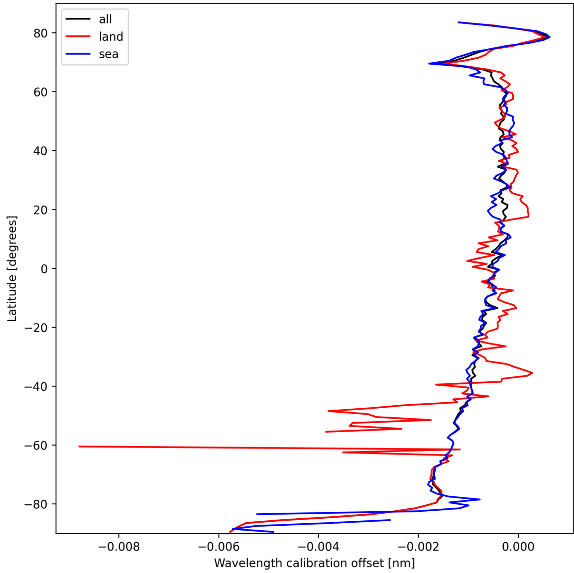
Figure 16: Zonal average of “Wavelength calibration offset” for 2025-10-04 to 2025-10-04.
