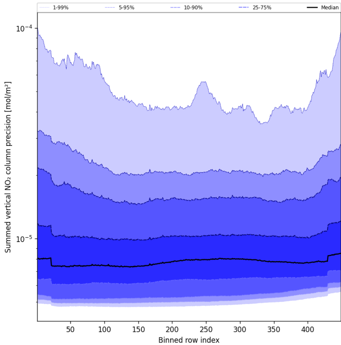
Figure 56: Along track statistics of “Summed vertical NO 2 column precision” for 2025-10-04 to 2025-10-04
