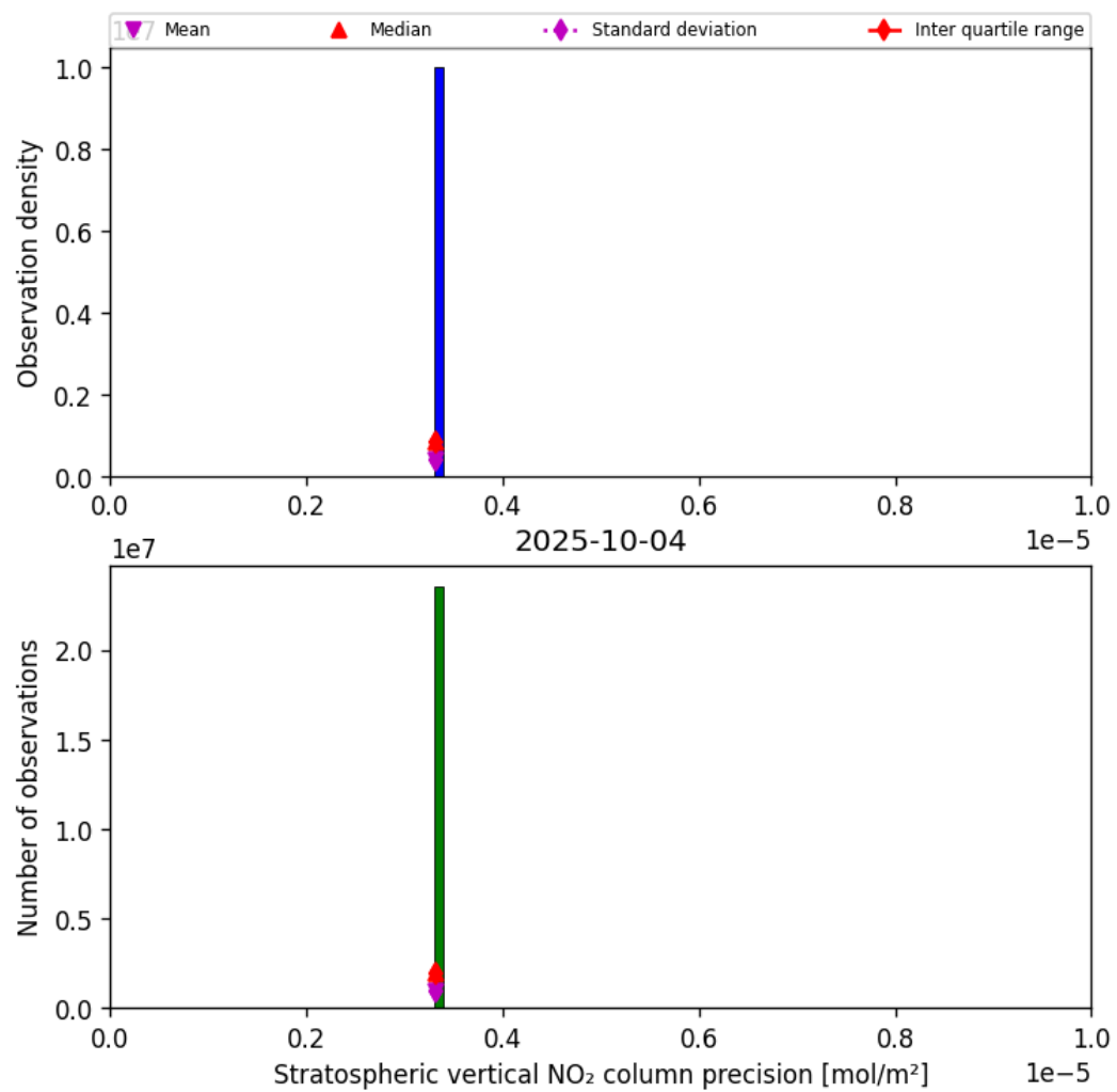
Figure 35: Histogram of “Stratospheric vertical NO 2 column precision” for 2025-10-04 to 2025-10-04
