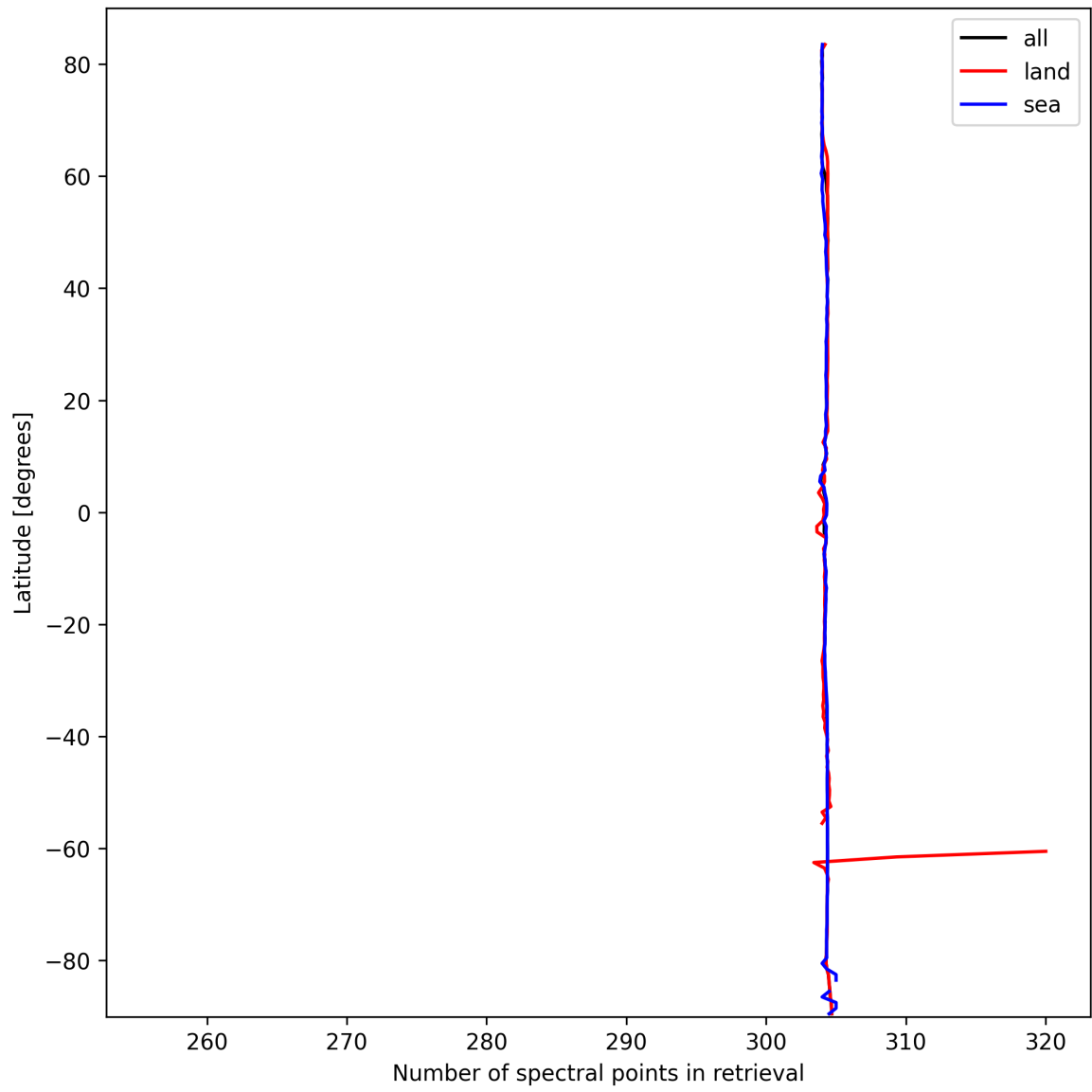
Figure 14: Zonal average of “Number of spectral points in retrieval” for 2025-10-04 to 2025-10-04.
