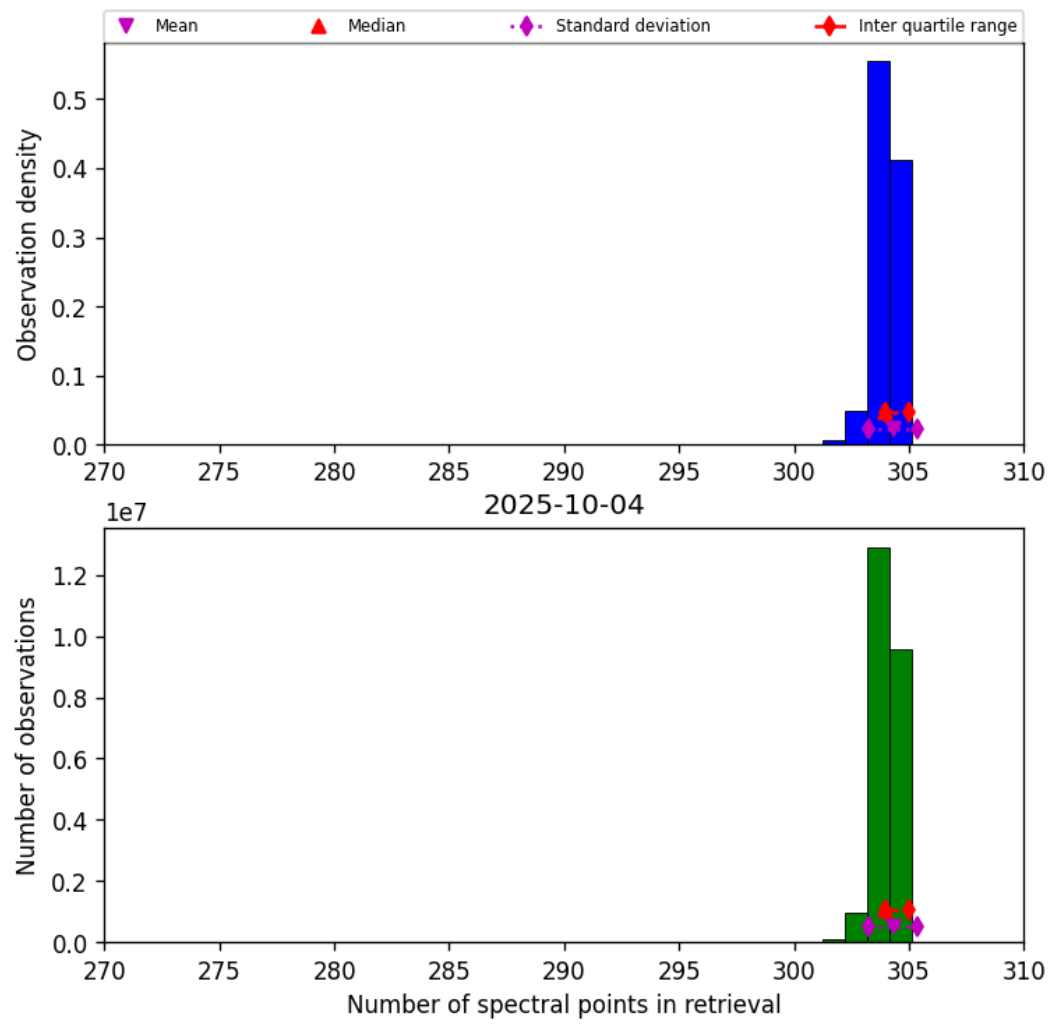
Figure 31: Histogram of “Number of spectral points in retrieval” for 2025-10-04 to 2025-10-04
