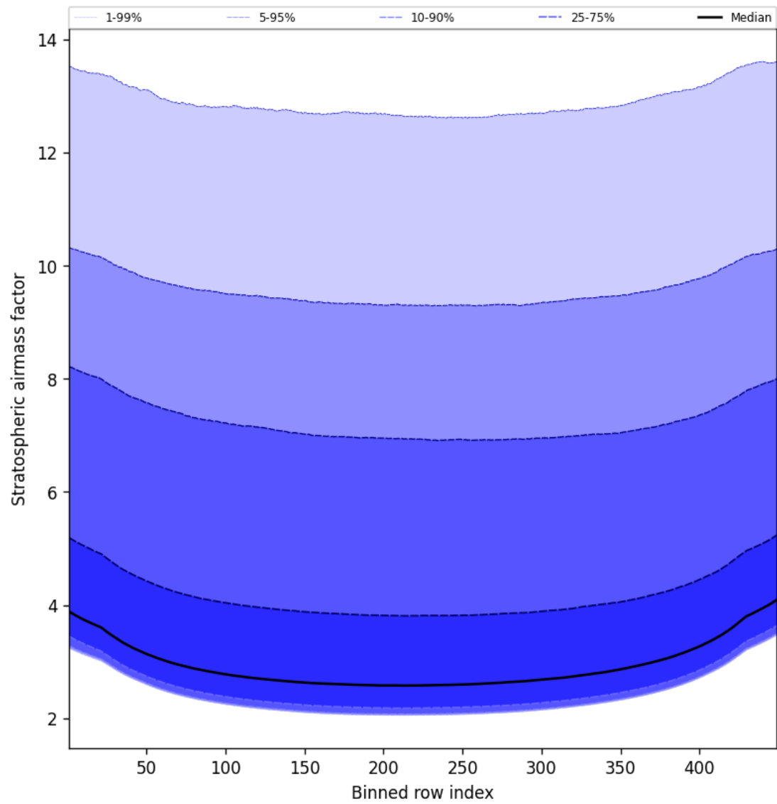
Figure 59: Along track statistics of “Stratospheric airmass factor” for 2025-10-04 to 2025-10-04
