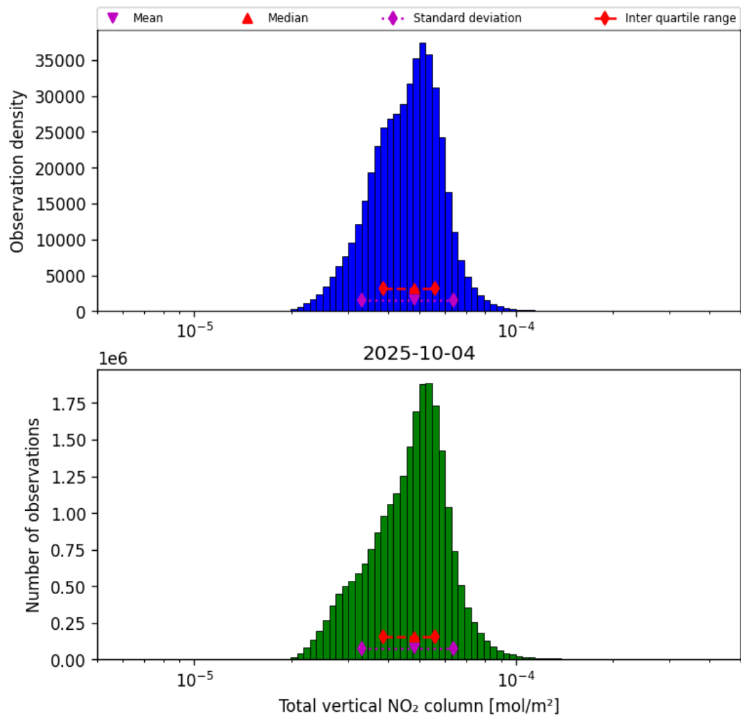
Figure 36: Histogram of “Total vertical NO 2 column” for 2025-10-04 to 2025-10-04
