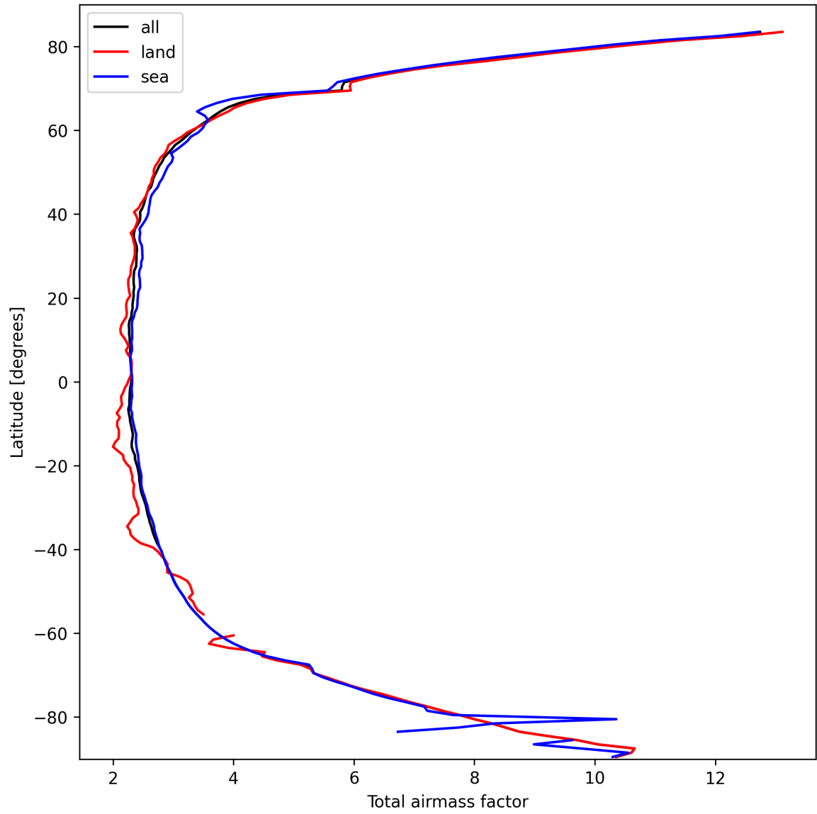
Figure 13: Zonal average of “Total airmass factor” for 2025-10-04 to 2025-10-04.
