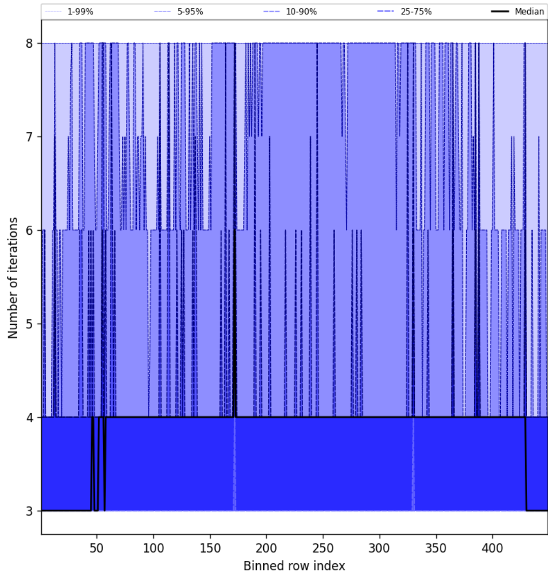
Figure 49: Along track statistics of “Number of iterations” for 2025-10-04 to 2025-10-04
