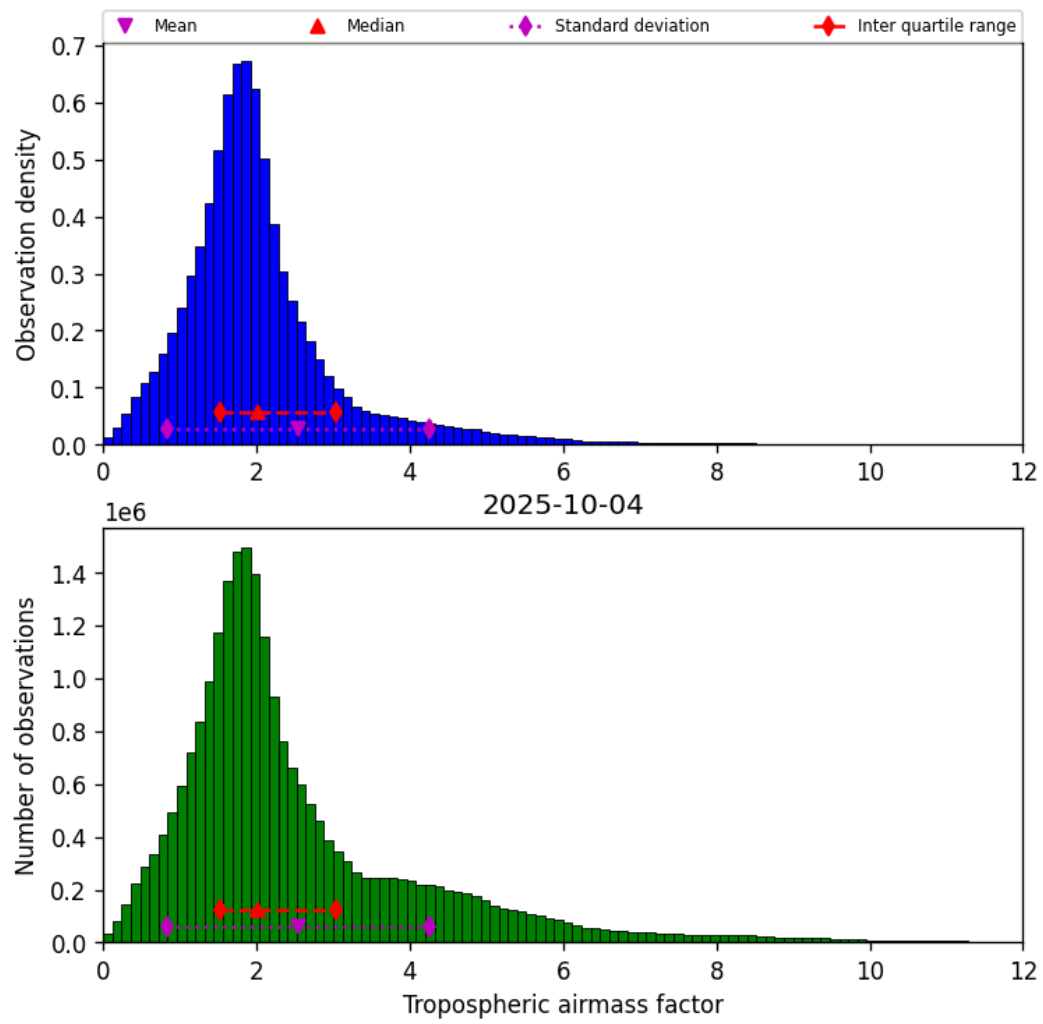
Figure 29: Histogram of “Tropospheric airmass factor” for 2025-10-04 to 2025-10-04
