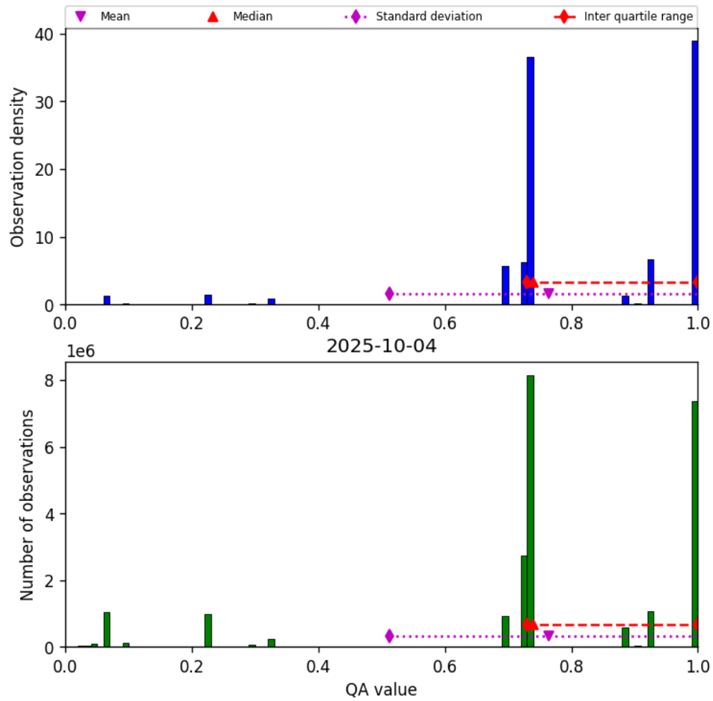
Figure 26: Histogram of “QA value” for 2025-10-04 to 2025-10-04
