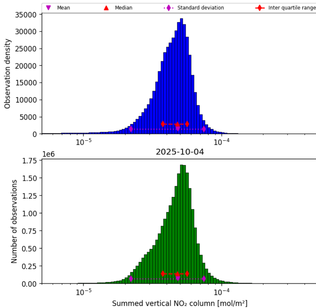
Figure 38: Histogram of “Summed vertical NO 2 column” for 2025-10-04 to 2025-10-04
