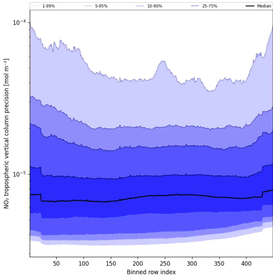
Figure 45: Along track statistics of “NO 2 tropospheric vertical column precision” for 2025-10-04 to 2025-10-04
