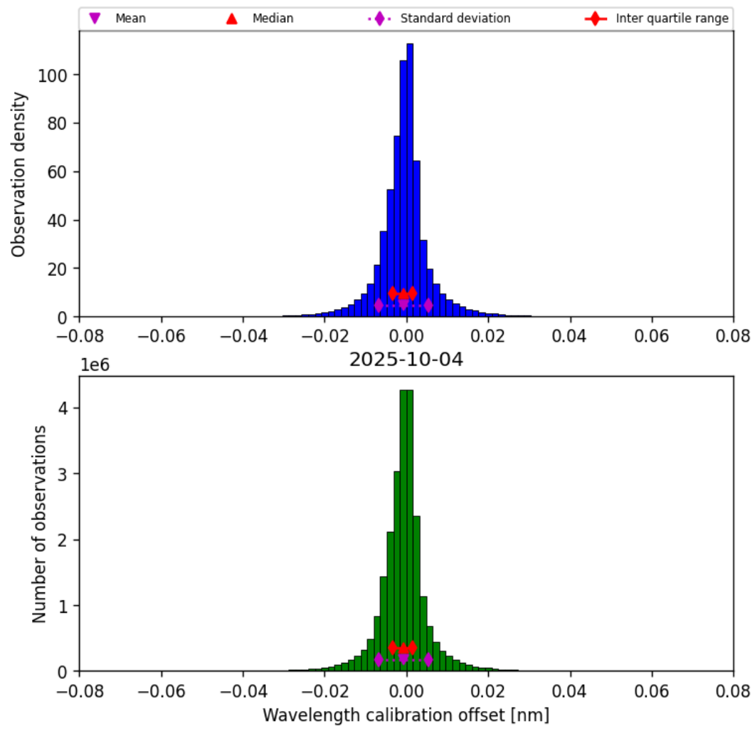
Figure 33: Histogram of “Wavelength calibration offset” for 2025-10-04 to 2025-10-04
