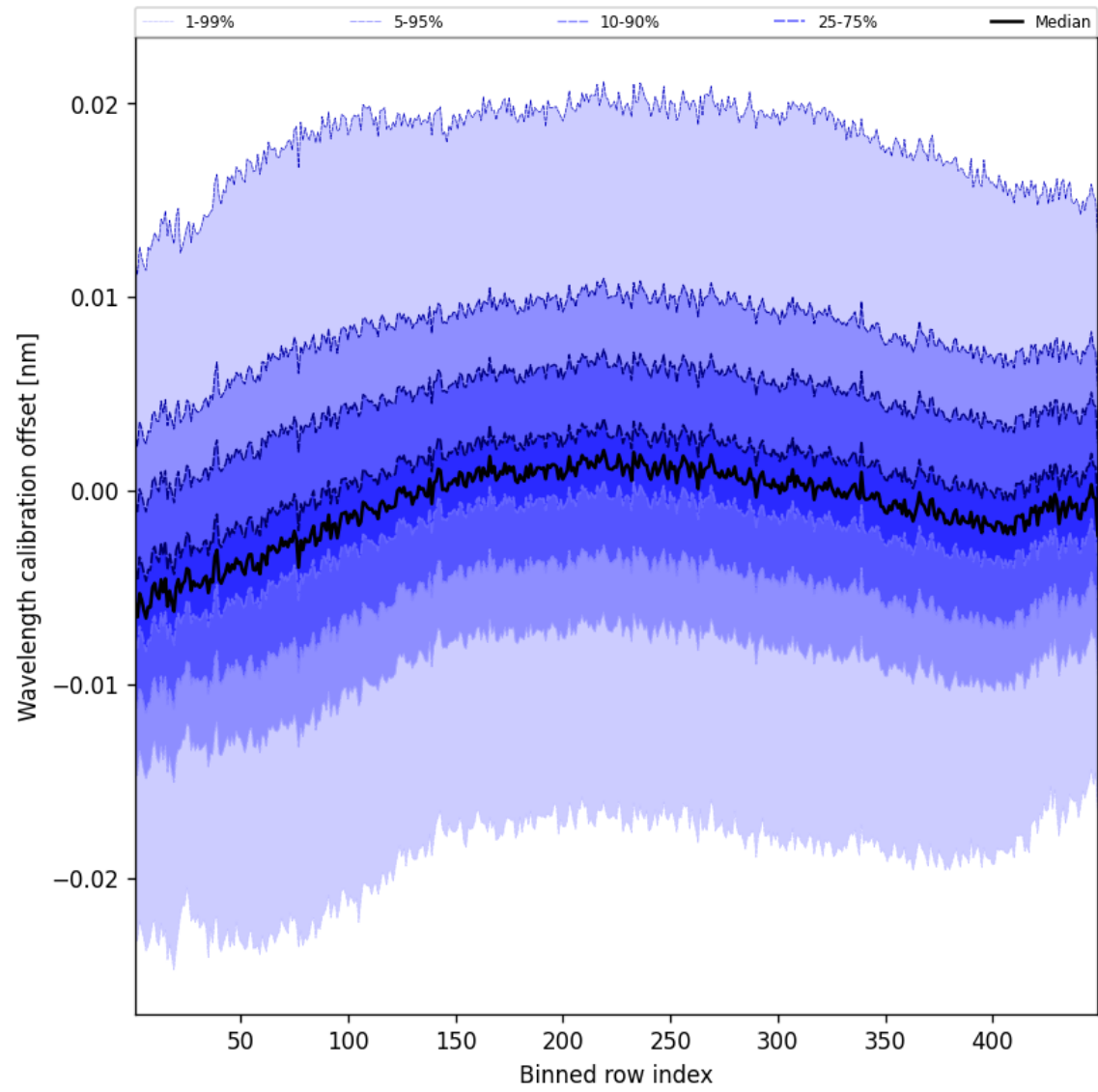
Figure 50: Along track statistics of “Wavelength calibration offset” for 2025-10-04 to 2025-10-04
