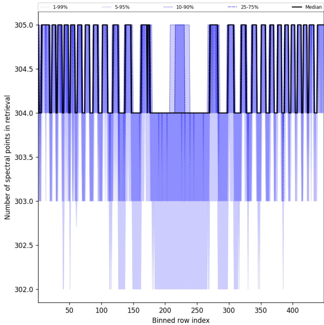
Figure 48: Along track statistics of “Number of spectral points in retrieval” for 2025-10-04 to 2025-10-04
