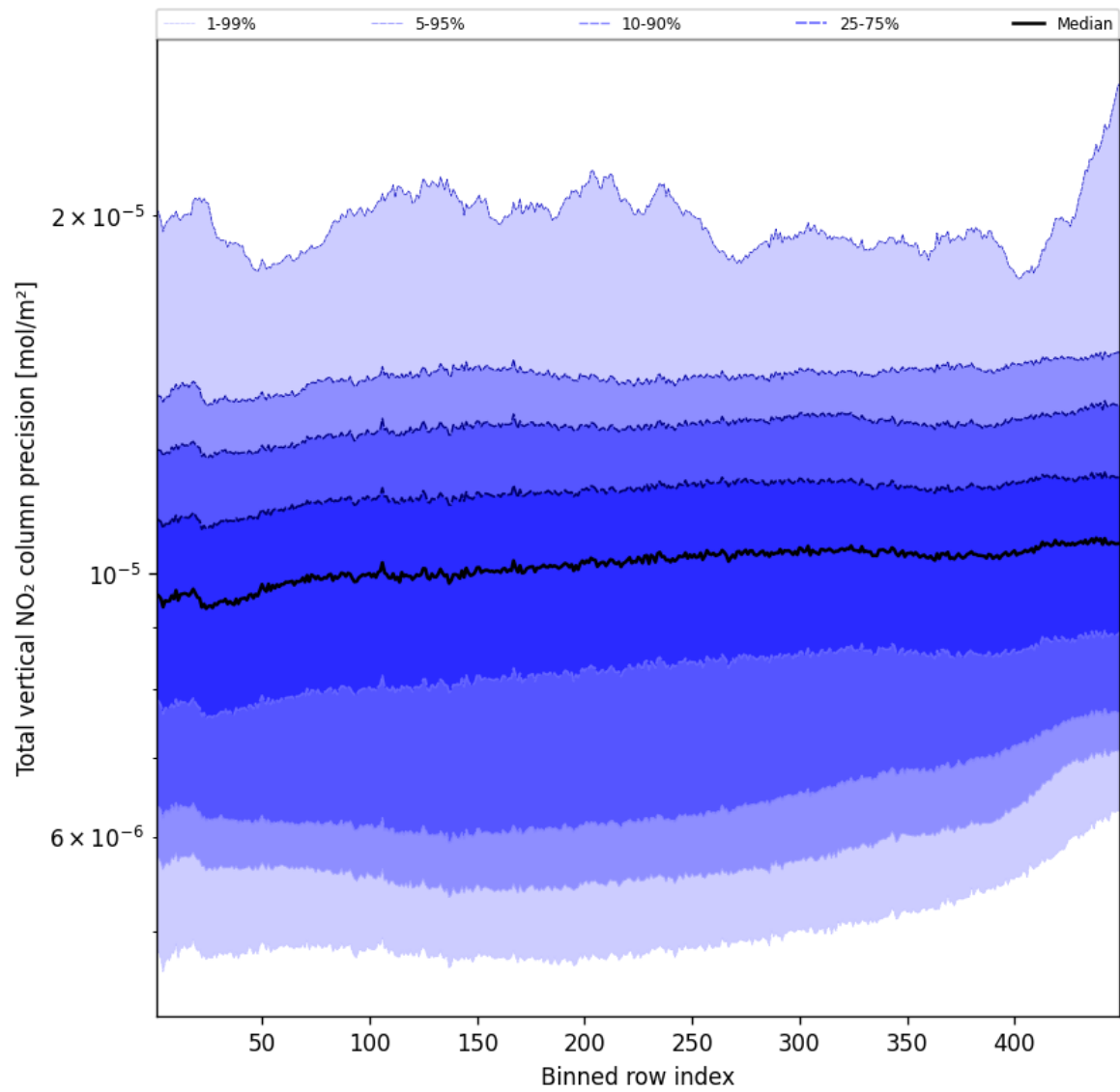
Figure 54: Along track statistics of “Total vertical NO 2 column precision” for 2025-10-04 to 2025-10-04
