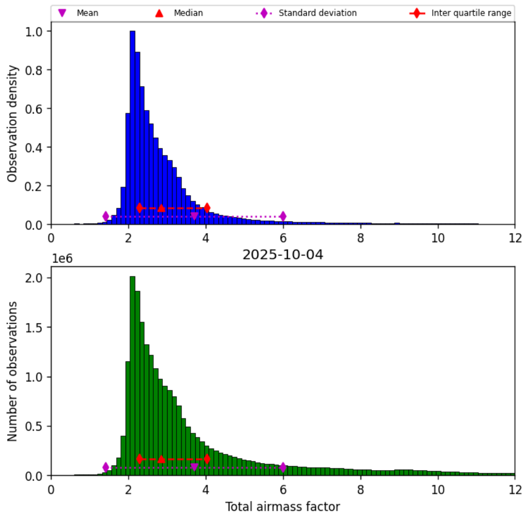
Figure 30: Histogram of “Total airmass factor” for 2025-10-04 to 2025-10-04
