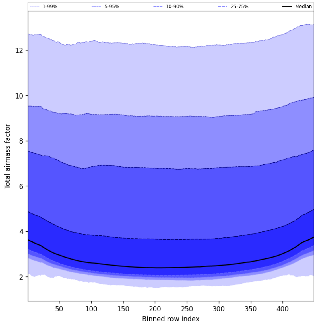
Figure 47: Along track statistics of “Total airmass factor” for 2025-10-04 to 2025-10-04
