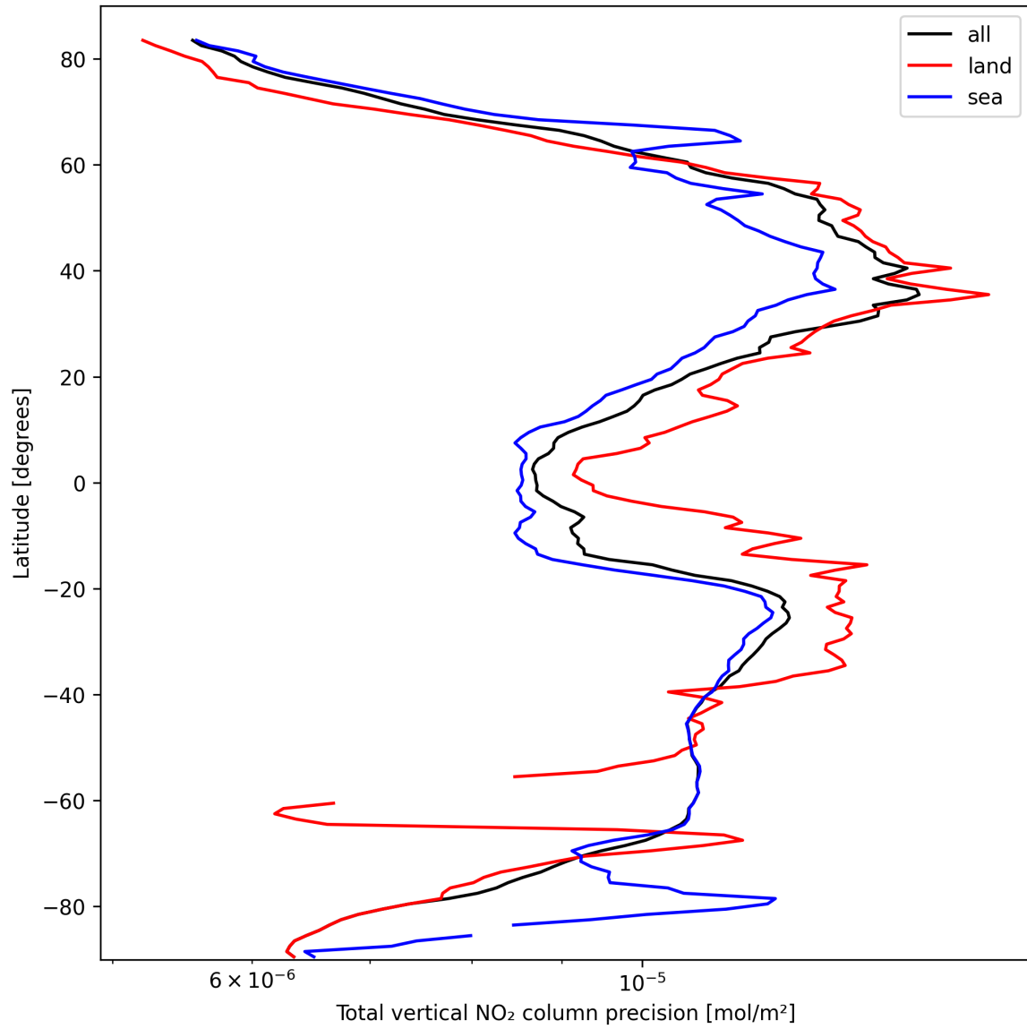
Figure 20: Zonal average of “Total vertical NO 2 column precision” for 2025-10-04 to 2025-10-04.
