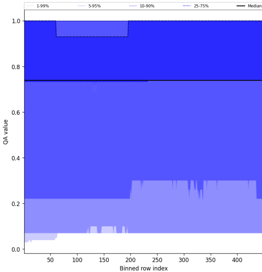
Figure 43: Along track statistics of "QA value" for 2025-10-04 to 2025-10-04
