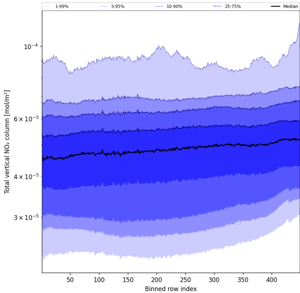
Figure 53: Along track statistics of “Total vertical NO 2 column” for 2025-10-04 to 2025-10-04
