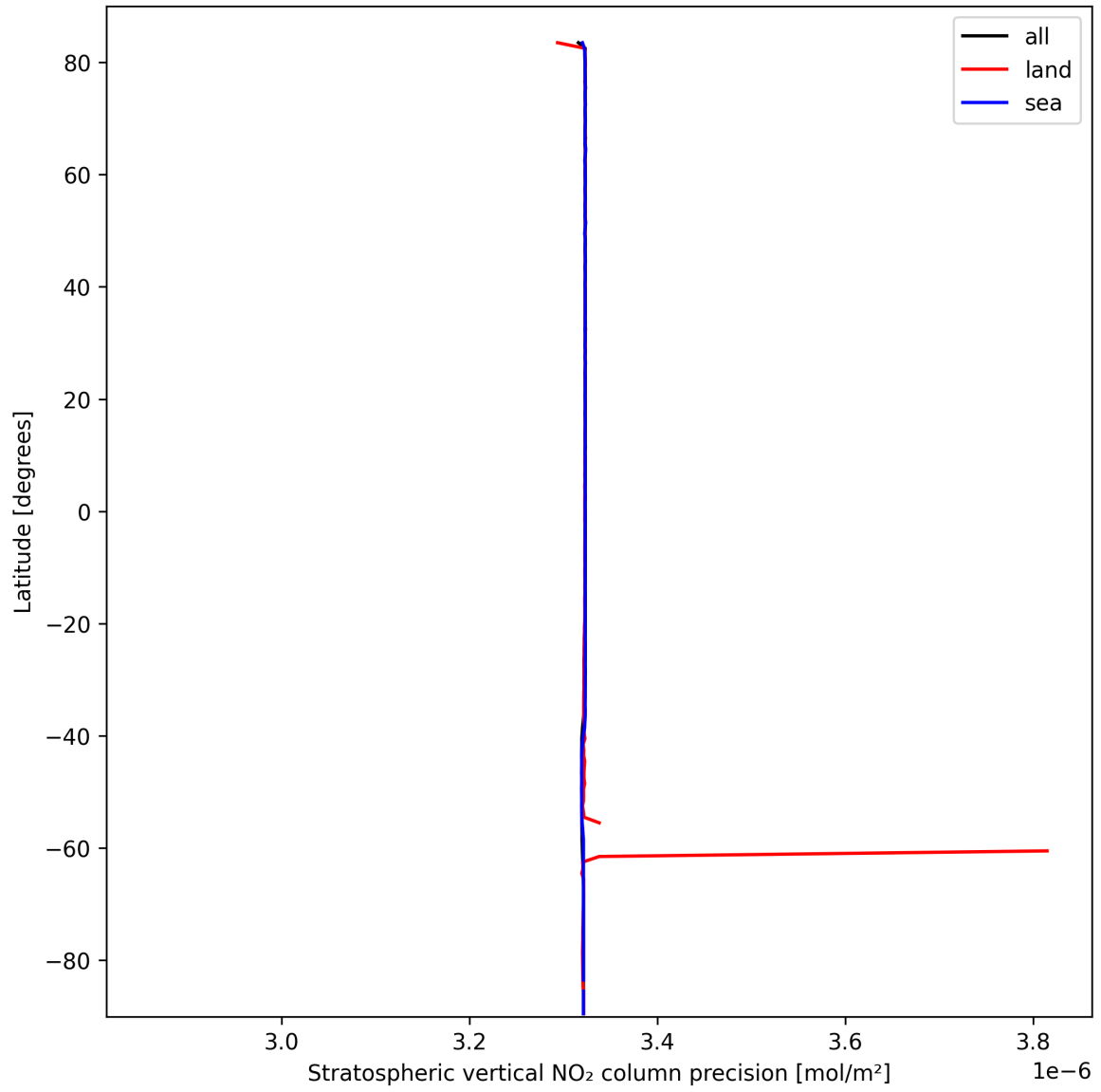
Figure 18: Zonal average of “Stratospheric vertical NO 2 column precision” for 2025-10-04 to 2025-10-04.
