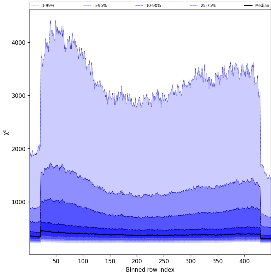
Figure 57: Along track statistics of “ \chi^2 ” for 2025-10-04 to 2025-10-04
