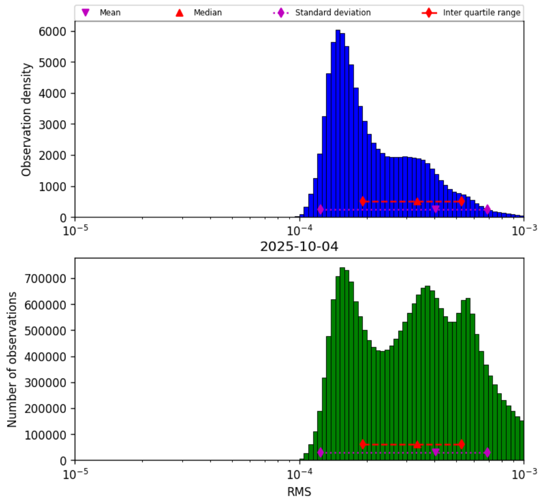
Figure 41: Histogram of “RMS” for 2025-10-04 to 2025-10-04
