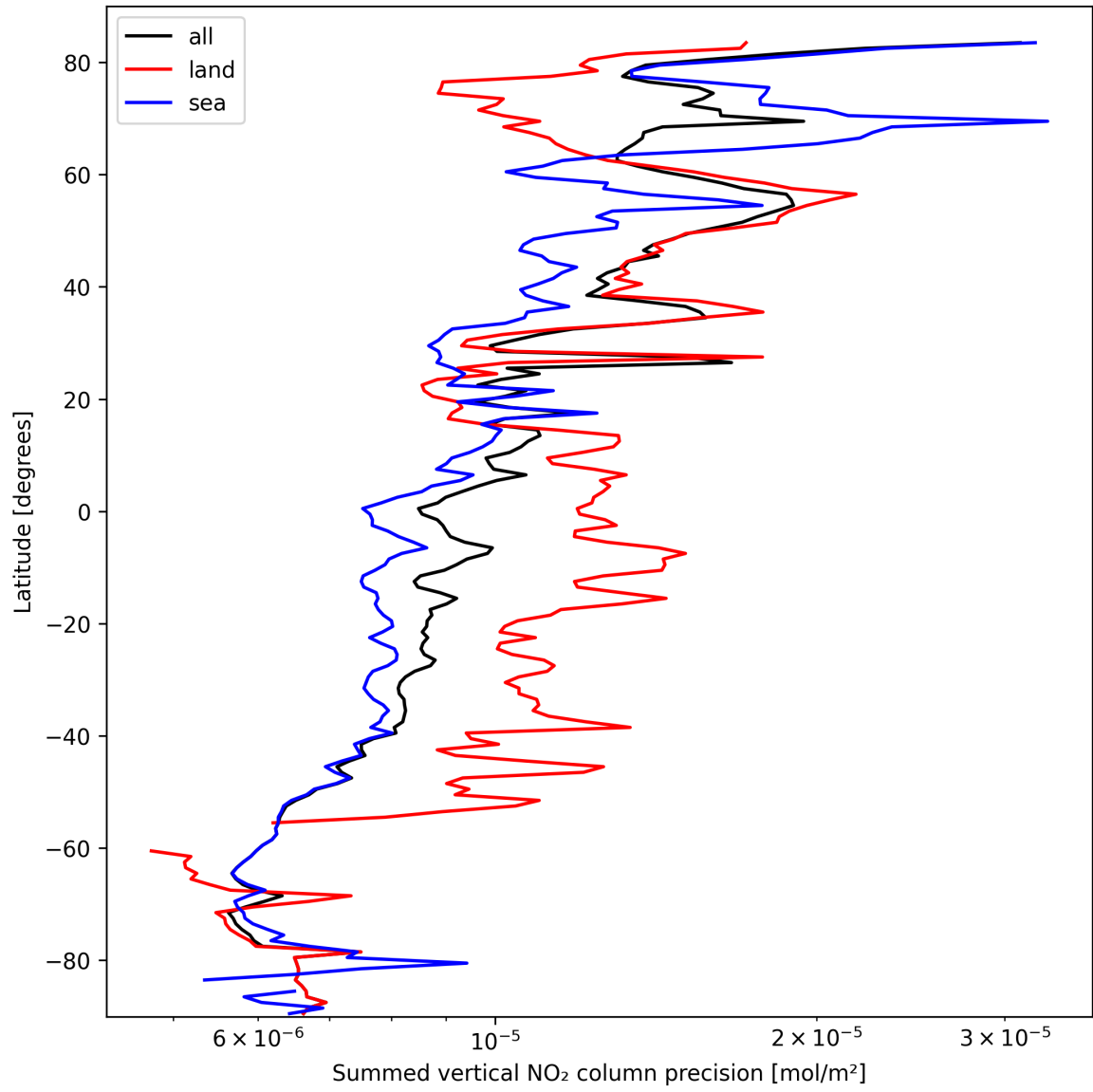
Figure 22: Zonal average of “Summed vertical NO 2 column precision” for 2025-10-04 to 2025-10-04.
