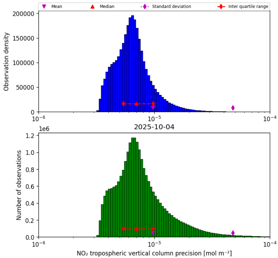
Figure 28: Histogram of “NO 2 tropospheric vertical column precision” for 2025-10-04 to 2025-10-04
