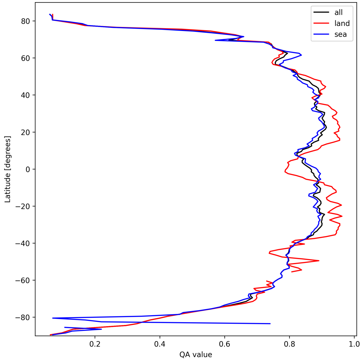
Figure 9: Zonal average of “QA value” for 2025-10-04 to 2025-10-04.
