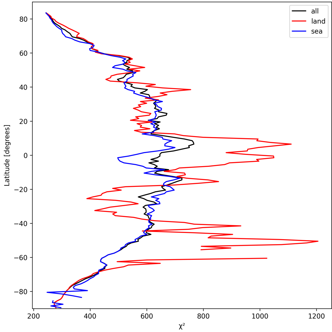
Figure 23: Zonal average of “ \chi^2 ” for 2025-10-04 to 2025-10-04.
