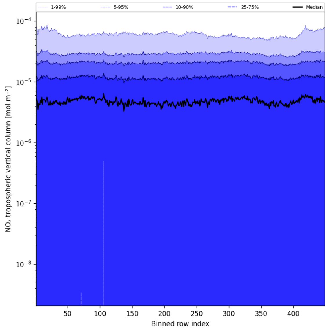
Figure 44: Along track statistics of “NO 2 tropospheric vertical column” for 2025-10-04 to 2025-10-04
