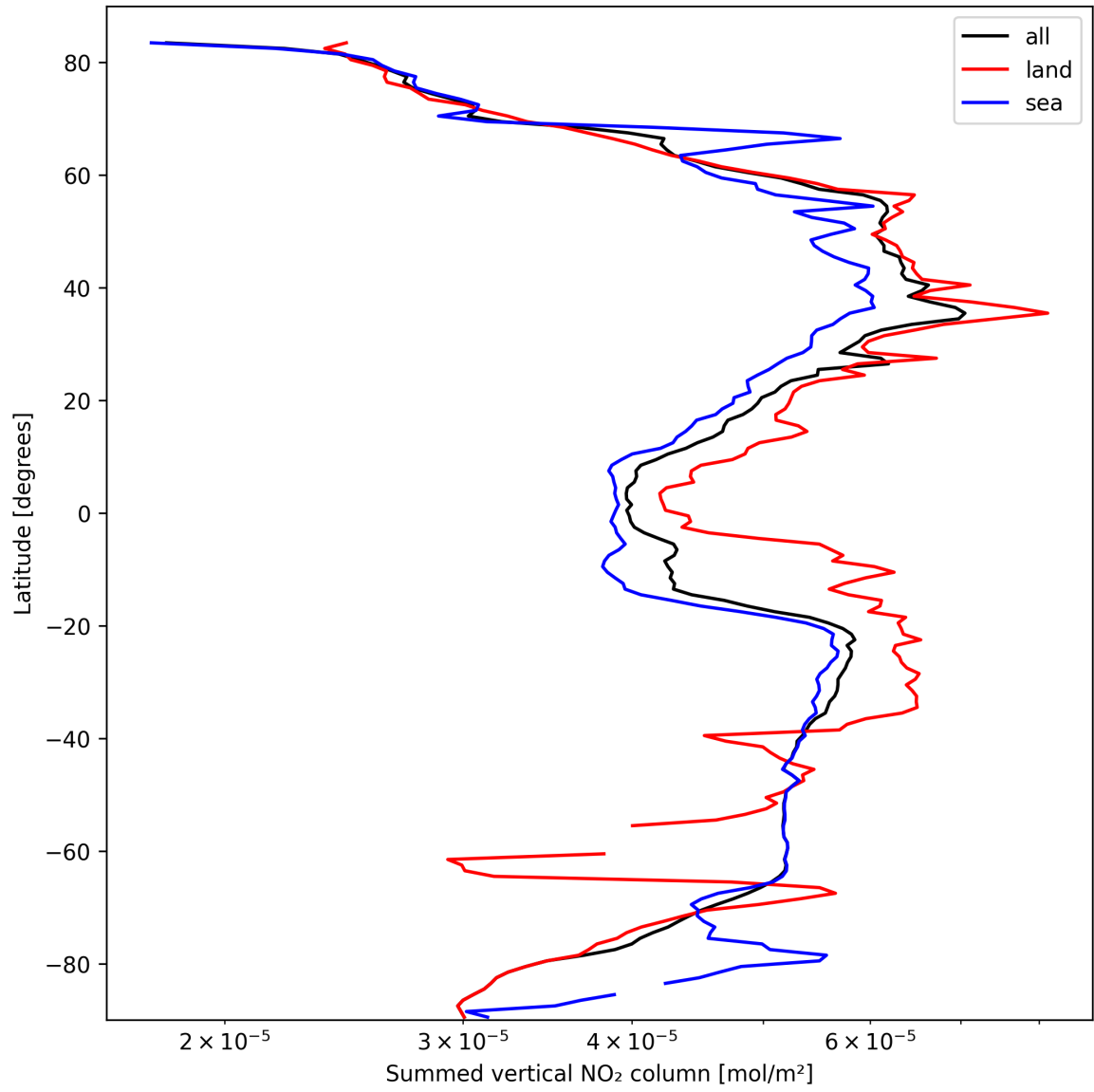
Figure 21: Zonal average of “Summed vertical NO 2 column” for 2025-10-04 to 2025-10-04.
