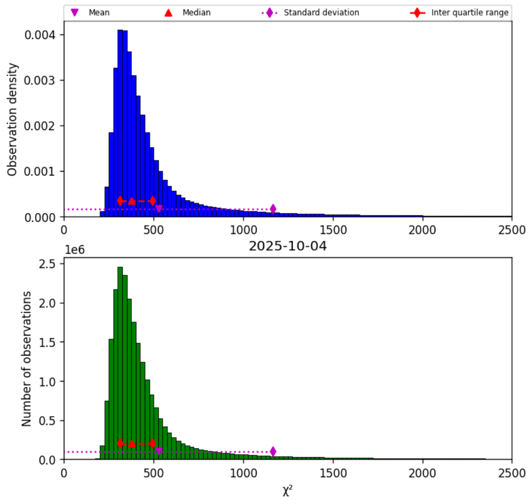
Figure 40: Histogram of “ \chi^2 ” for 2025-10-04 to 2025-10-04
