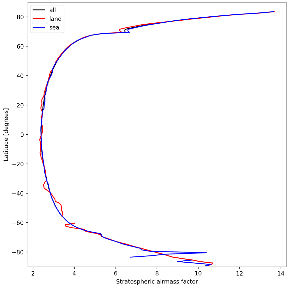
Figure 25: Zonal average of “Stratospheric airmass factor” for 2025-10-04 to 2025-10-04.
