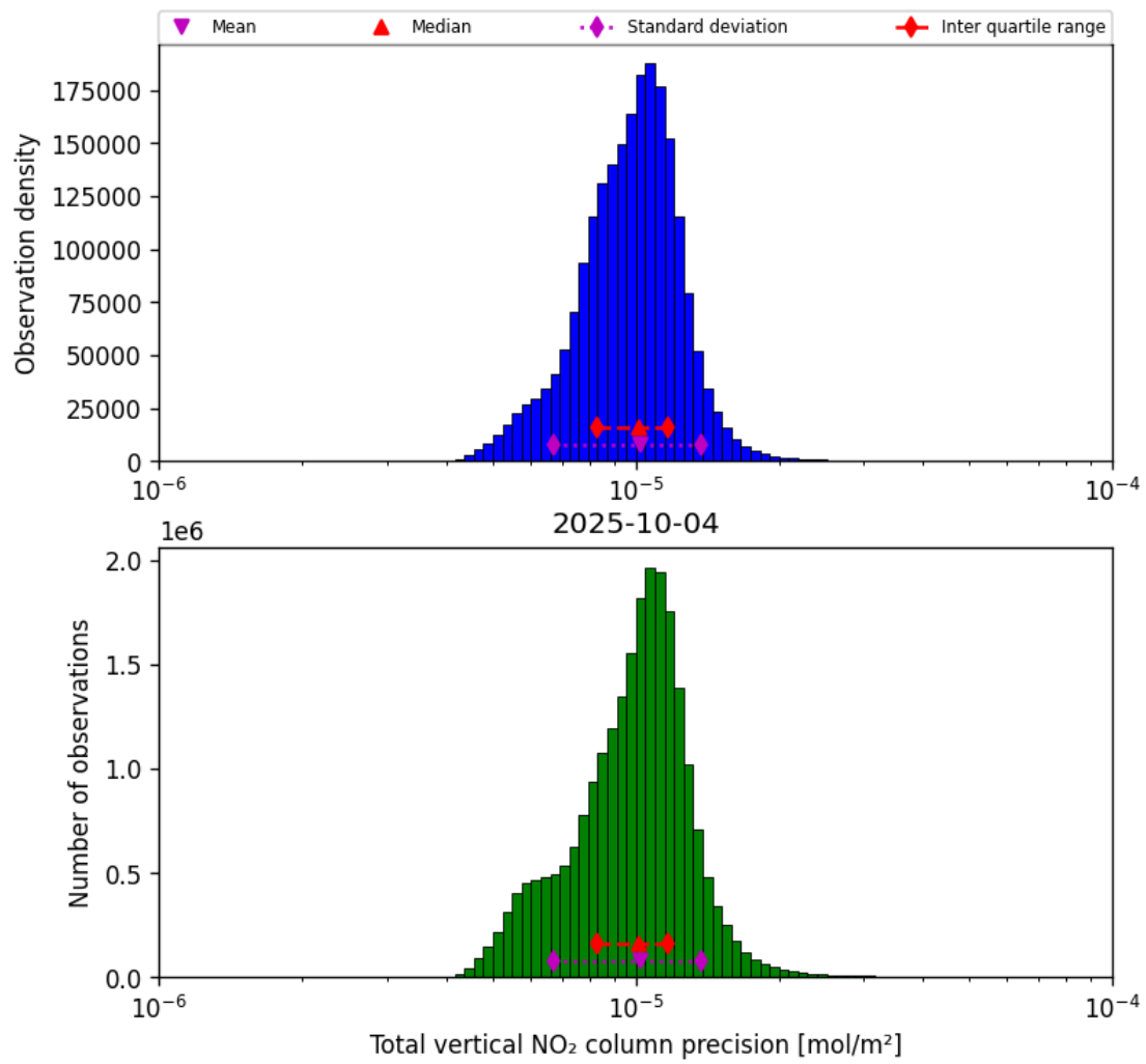
Figure 37: Histogram of “Total vertical NO 2 column precision” for 2025-10-04 to 2025-10-04
