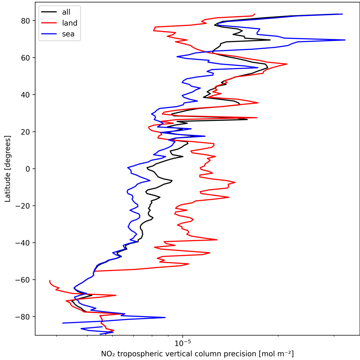
Figure 11: Zonal average of “NO 2 tropospheric vertical column precision” for 2025-10-04 to 2025-10-04.
