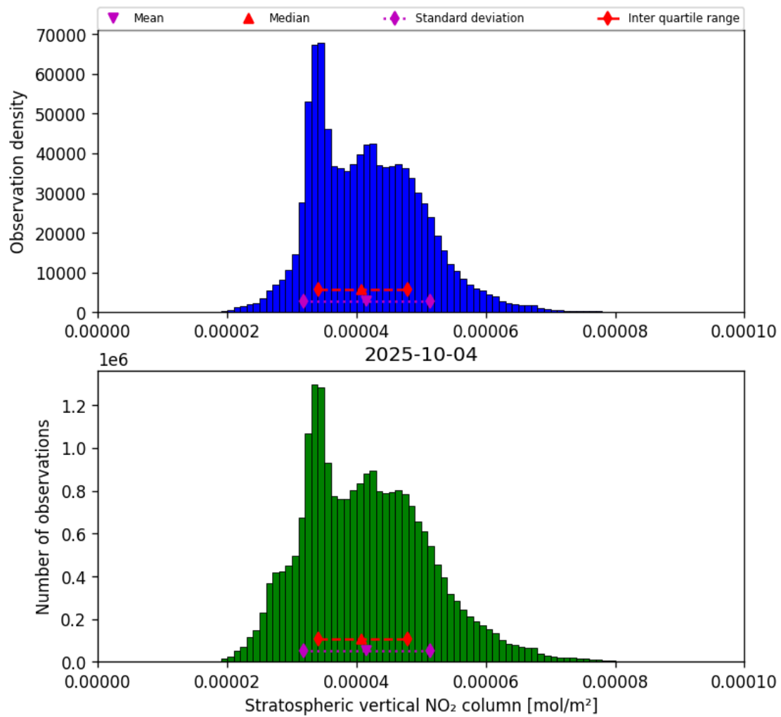
Figure 34: Histogram of “Stratospheric vertical NO 2 column” for 2025-10-04 to 2025-10-04
