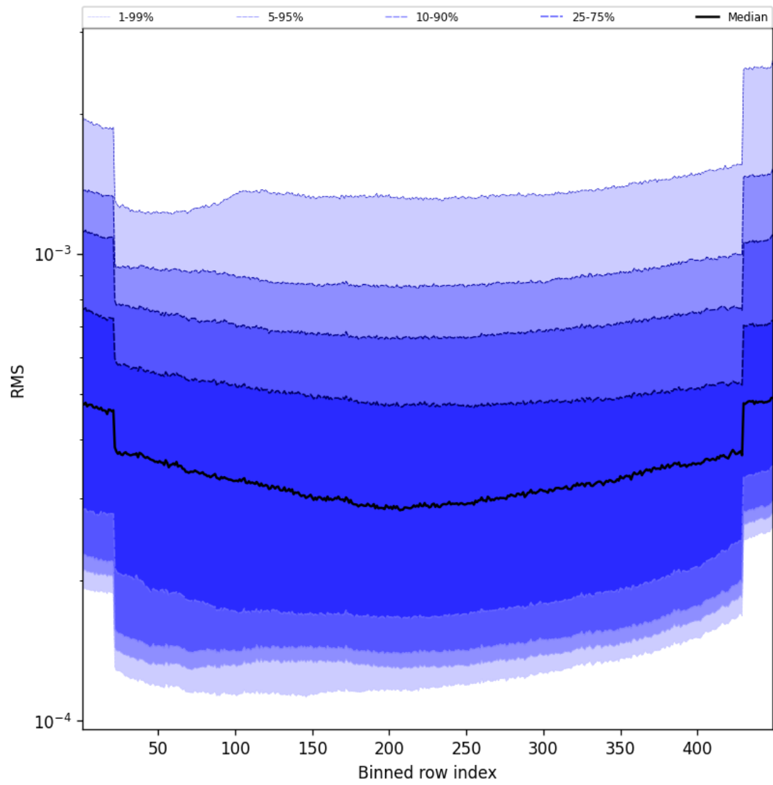
Figure 58: Along track statistics of “RMS” for 2025-10-04 to 2025-10-04
