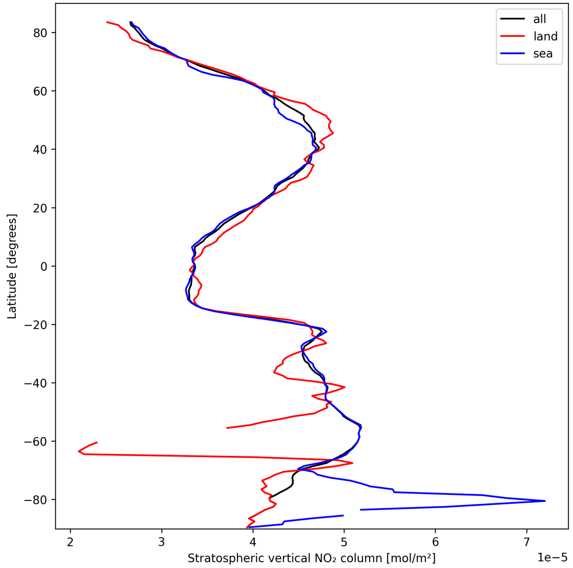
Figure 17: Zonal average of “Stratospheric vertical NO 2 column” for 2025-10-04 to 2025-10-04.
