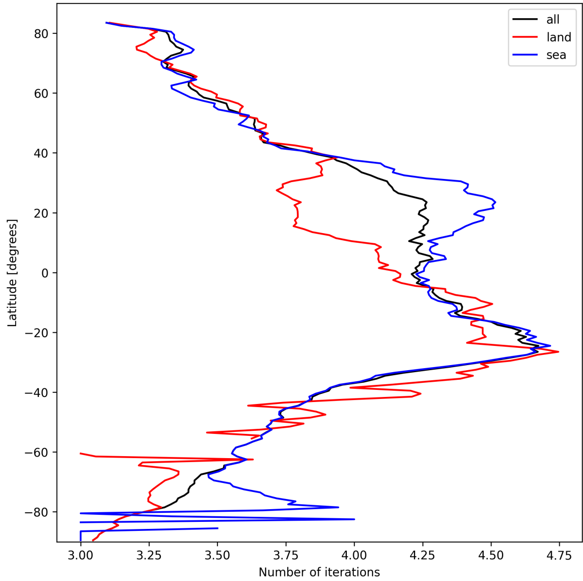
Figure 15: Zonal average of “Number of iterations” for 2025-10-04 to 2025-10-04.
