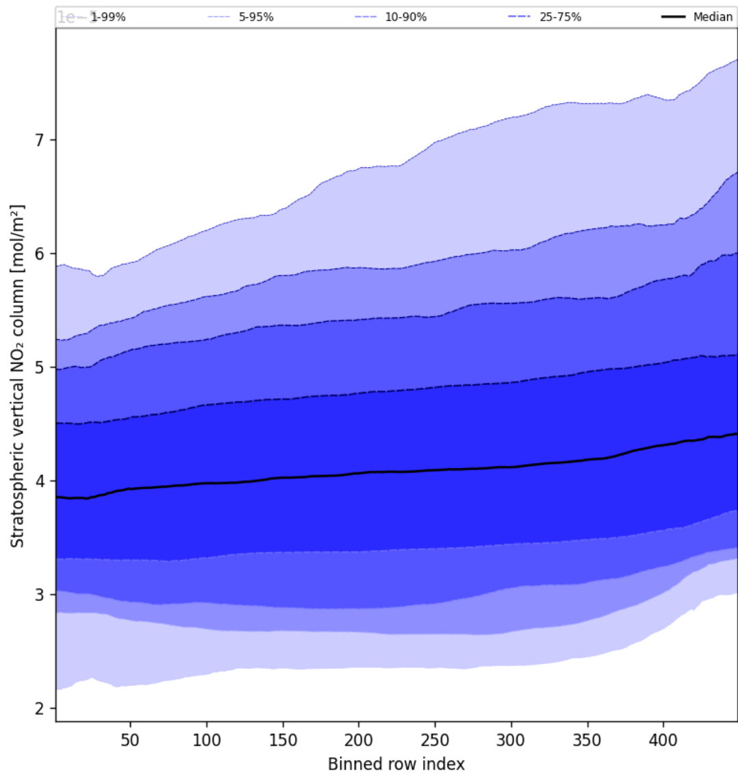
Figure 51: Along track statistics of “Stratospheric vertical NO 2 column” for 2025-10-04 to 2025-10-04
