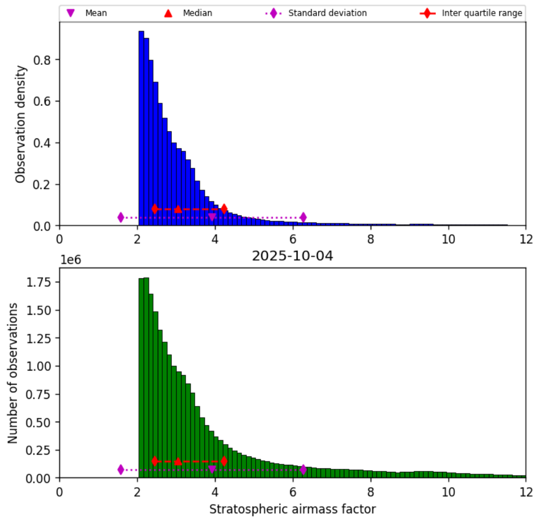
Figure 42: Histogram of “Stratospheric airmass factor” for 2025-10-04 to 2025-10-04
