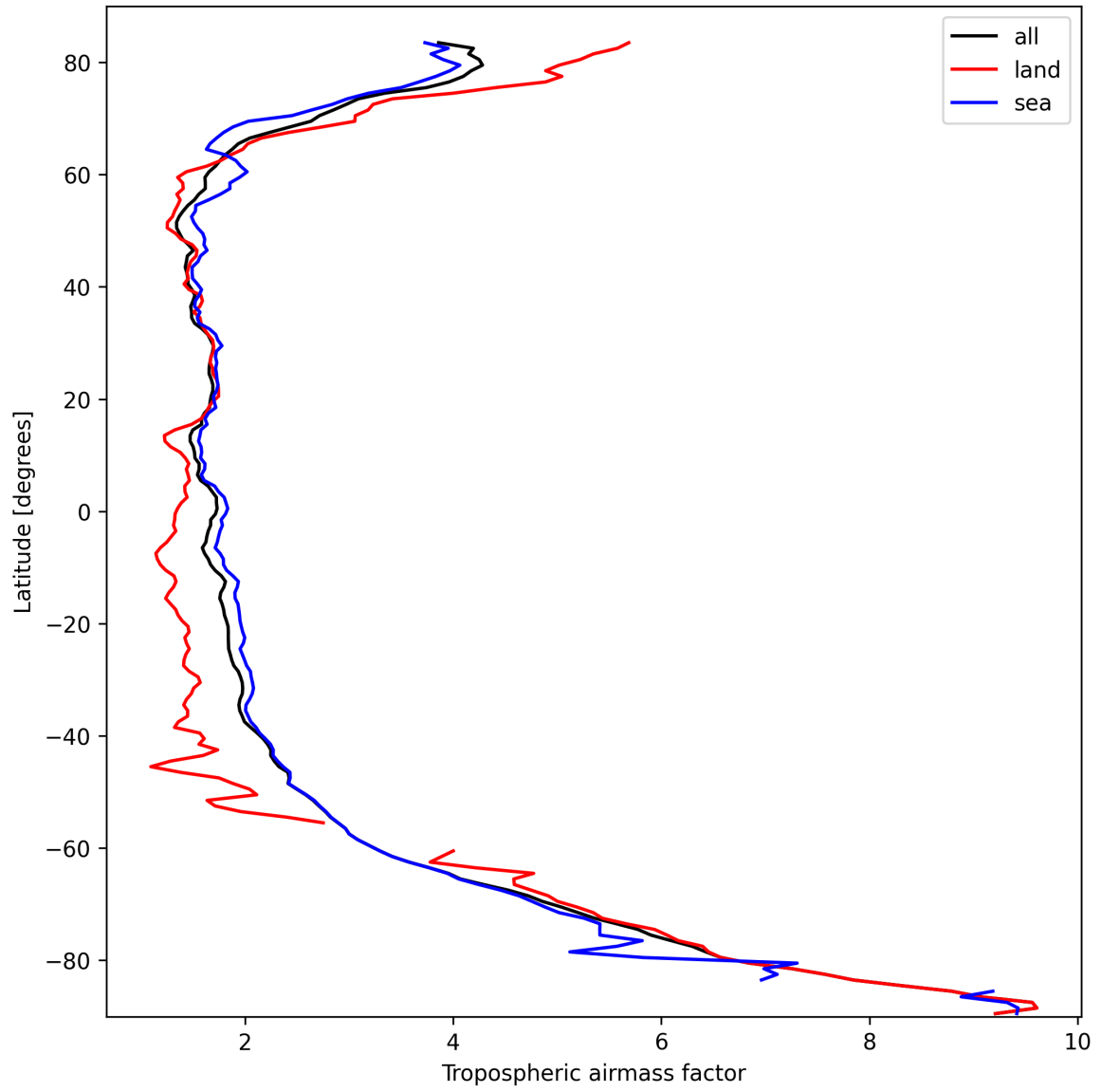
Figure 12: Zonal average of “Tropospheric airmass factor” for 2025-10-04 to 2025-10-04.
