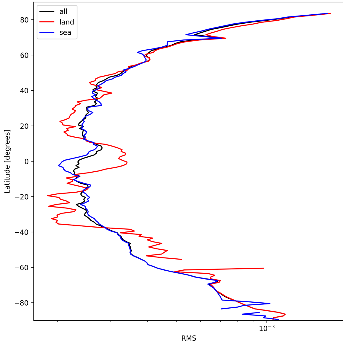
Figure 24: Zonal average of “RMS” for 2025-10-04 to 2025-10-04.
