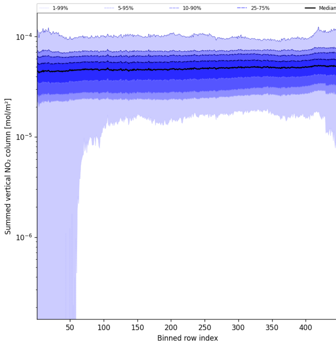
Figure 55: Along track statistics of “Summed vertical NO 2 column” for 2025-10-04 to 2025-10-04
