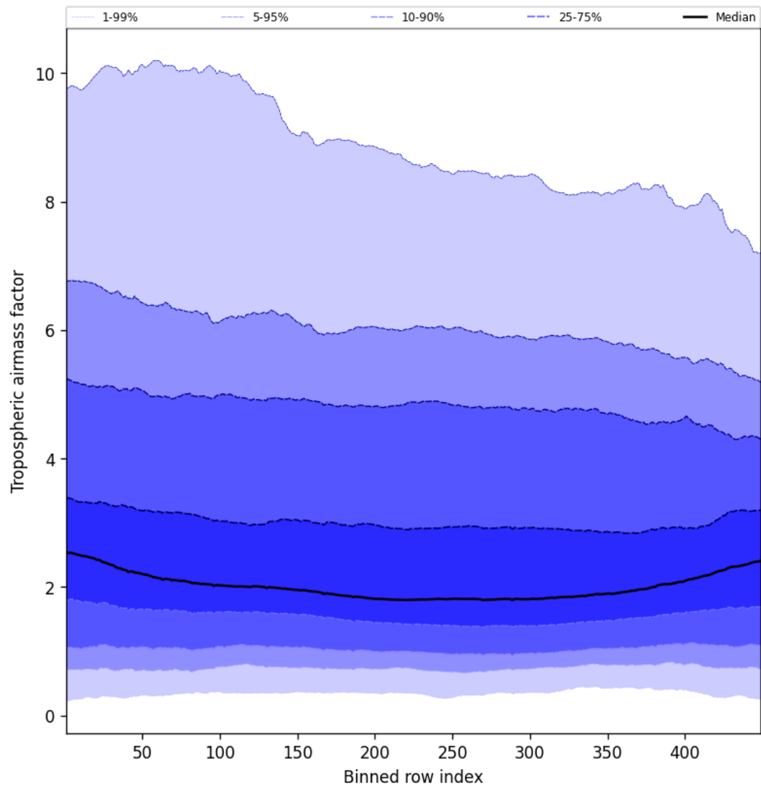
Figure 46: Along track statistics of “Tropospheric air mass factor” for 2025-10-04 to 2025-10-04
