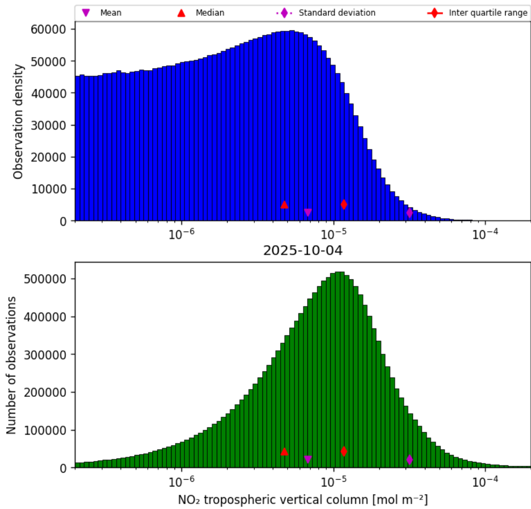
Figure 27: Histogram of “ \text{NO}_2 tropospheric vertical column” for 2025-10-04 to 2025-10-04
