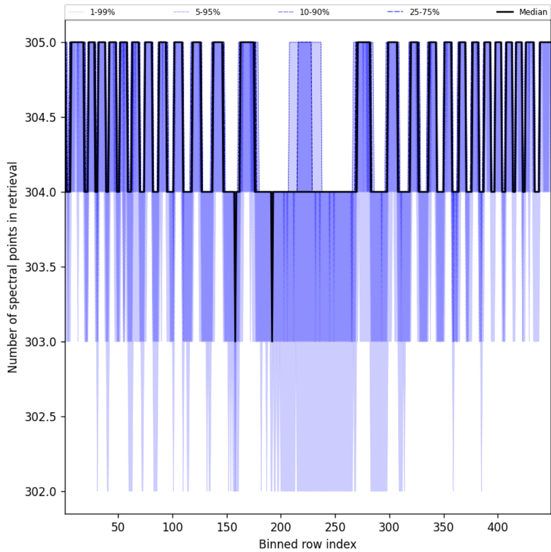
Figure 48: Along track statistics of “Number of spectral points in retrieval” for 2025-10-05 to 2025-10-06
