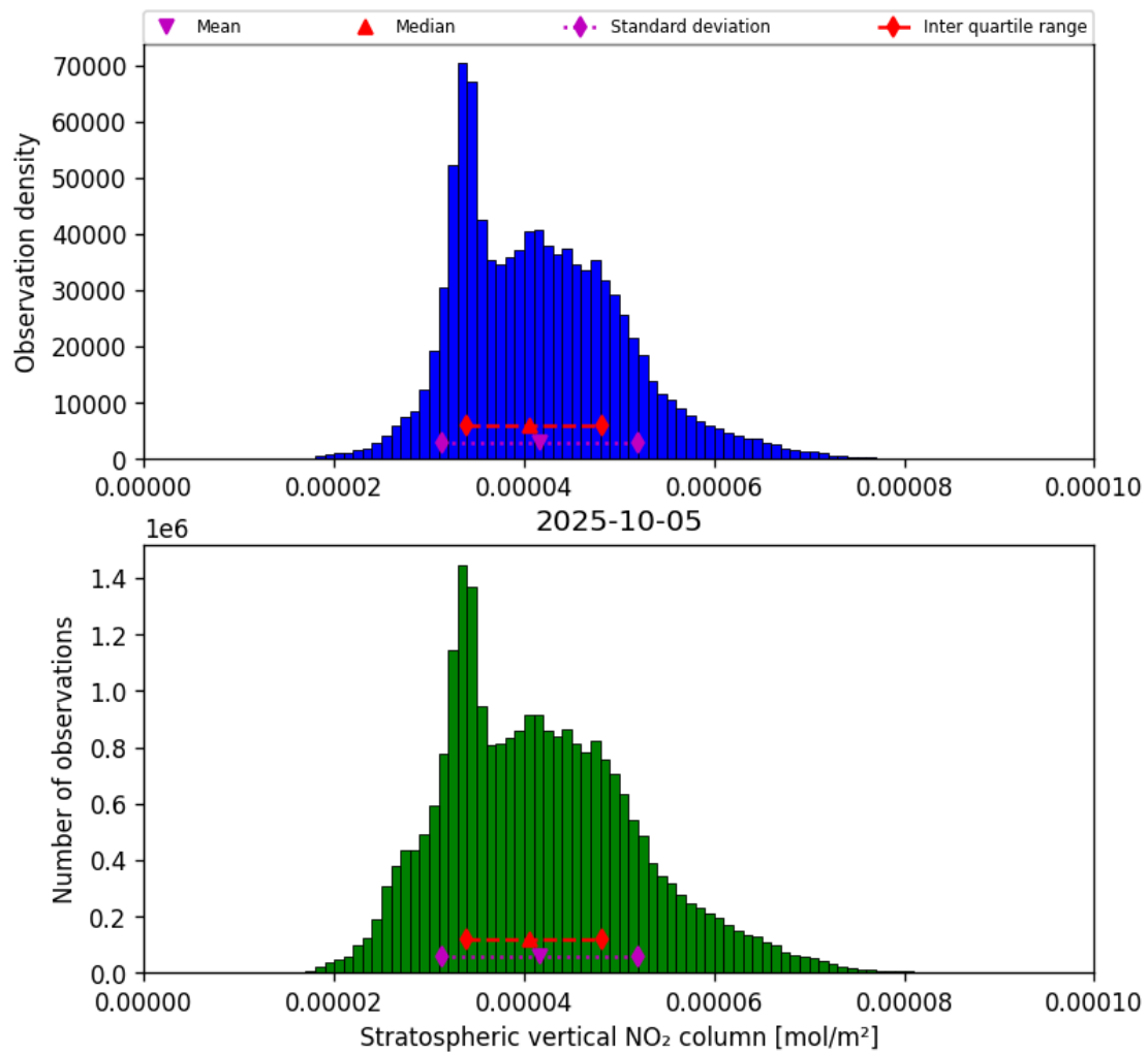
Figure 34: Histogram of “Stratospheric vertical NO 2 column” for 2025-10-05 to 2025-10-06
