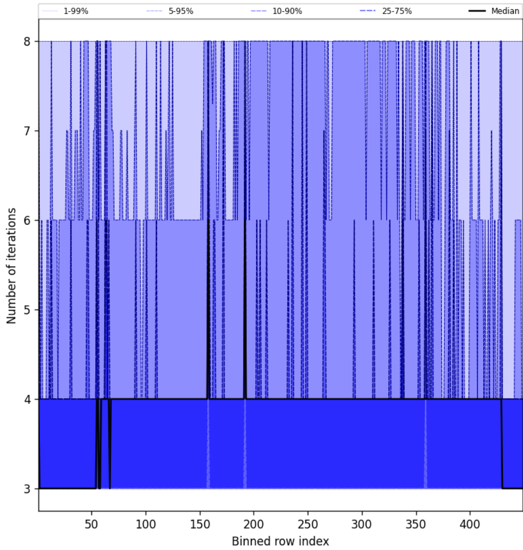
Figure 49: Along track statistics of “Number of iterations” for 2025-10-05 to 2025-10-06
