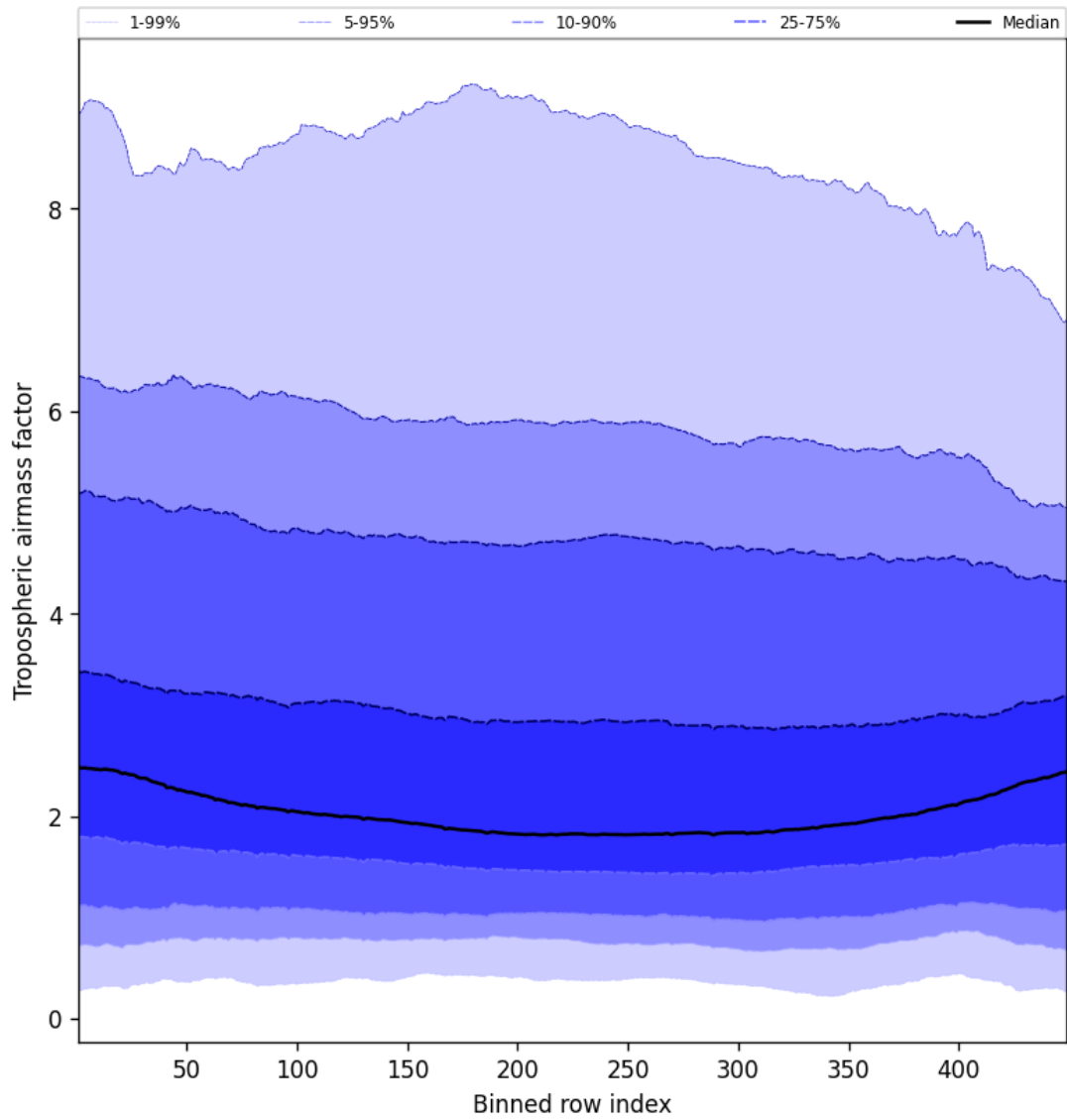
Figure 46: Along track statistics of “Tropospheric air mass factor” for 2025-10-05 to 2025-10-06
