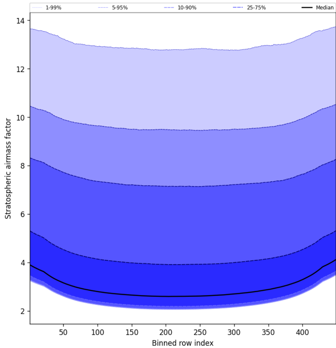
Figure 59: Along track statistics of “Stratospheric airmass factor” for 2025-10-05 to 2025-10-06
