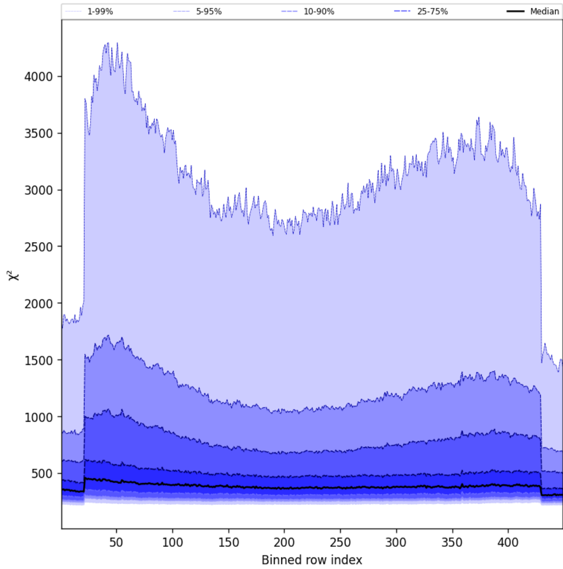
Figure 57: Along track statistics of “ \chi^2 ” for 2025-10-05 to 2025-10-06
