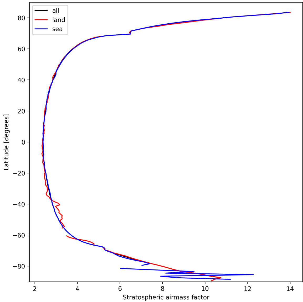
Figure 25: Zonal average of “Stratospheric air mass factor” for 2025-10-05 to 2025-10-06.
