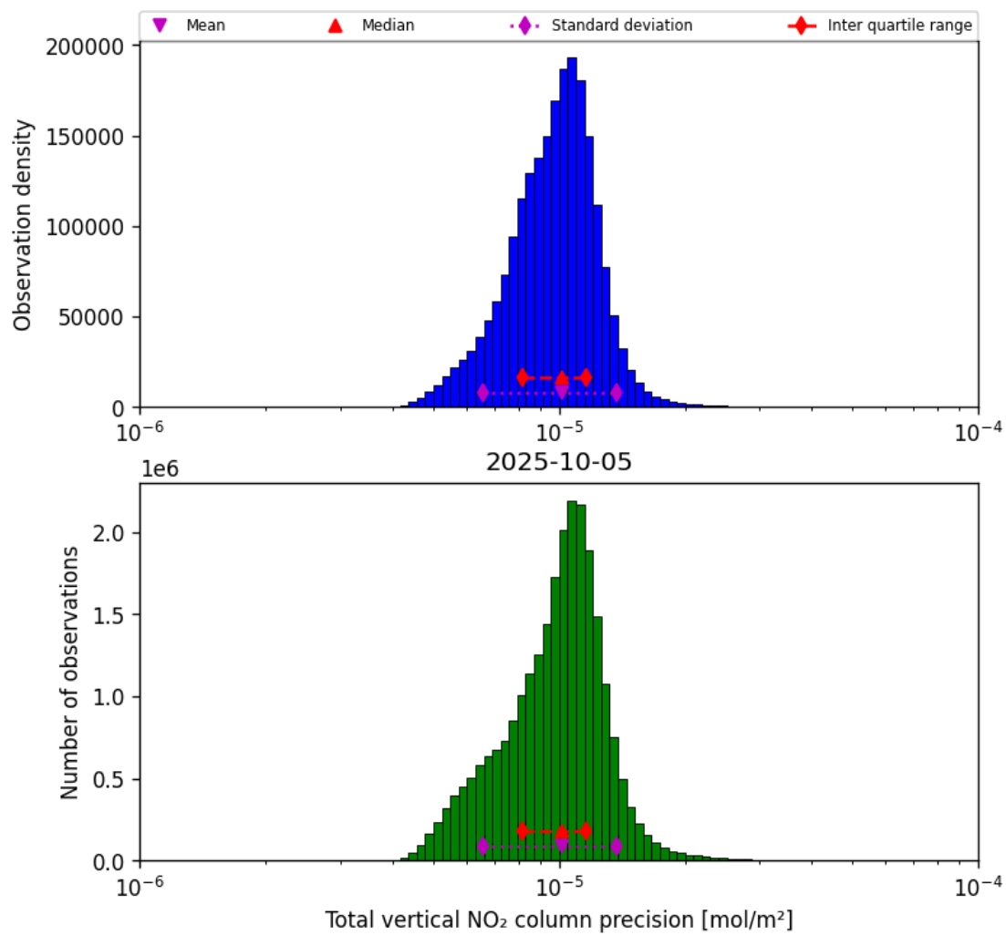
Figure 37: Histogram of "Total vertical NO 2 column precision" for 2025-10-05 to 2025-10-06
