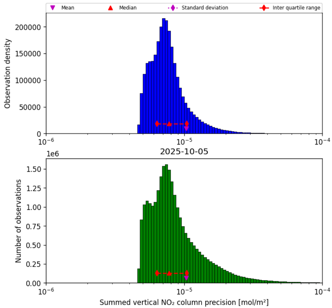
Figure 39: Histogram of “Summed vertical NO 2 column precision” for 2025-10-05 to 2025-10-06
