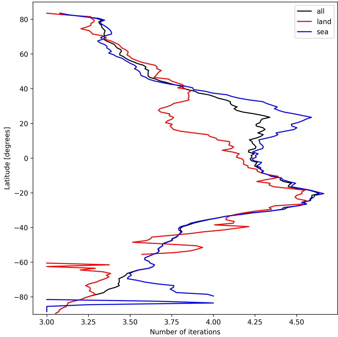
Figure 15: Zonal average of “Number of iterations” for 2025-10-05 to 2025-10-06.
