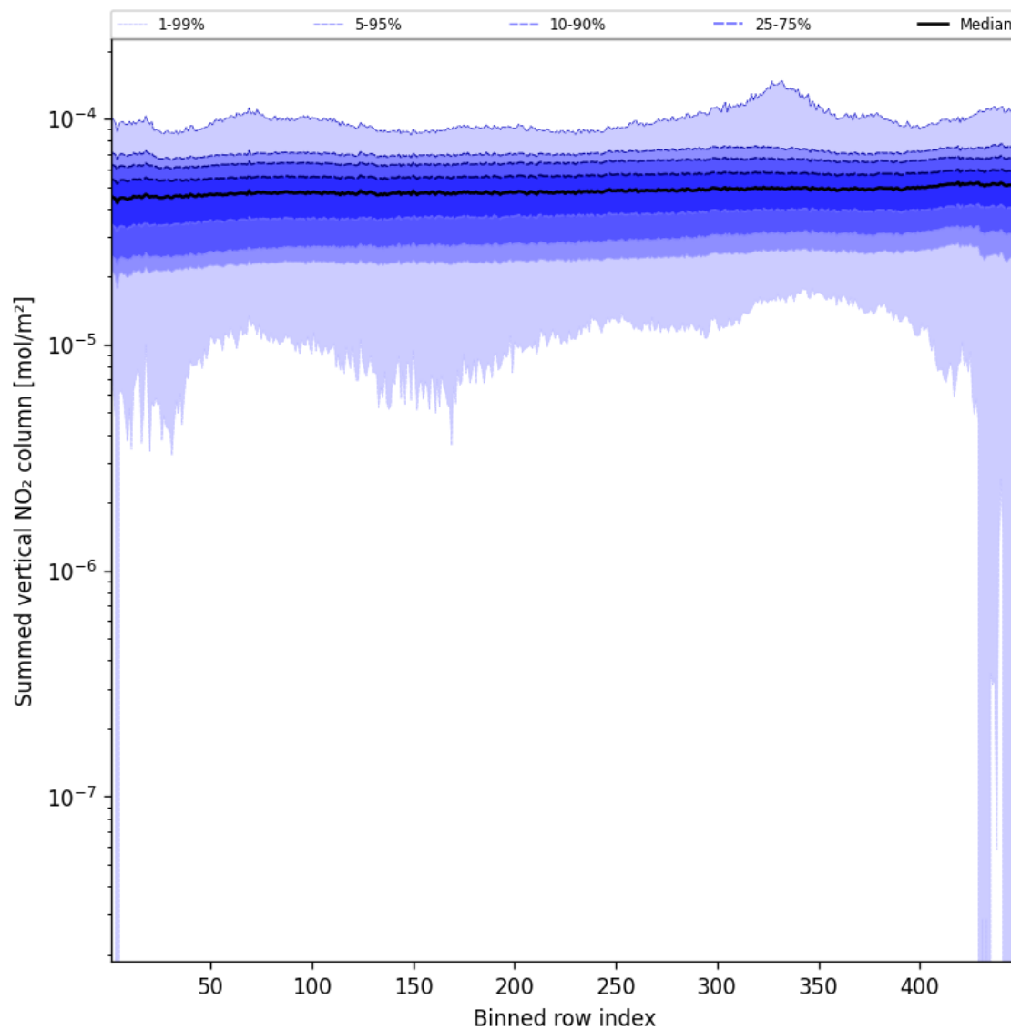
Figure 55: Along track statistics of “Summed vertical NO 2 column” for 2025-10-05 to 2025-10-06
