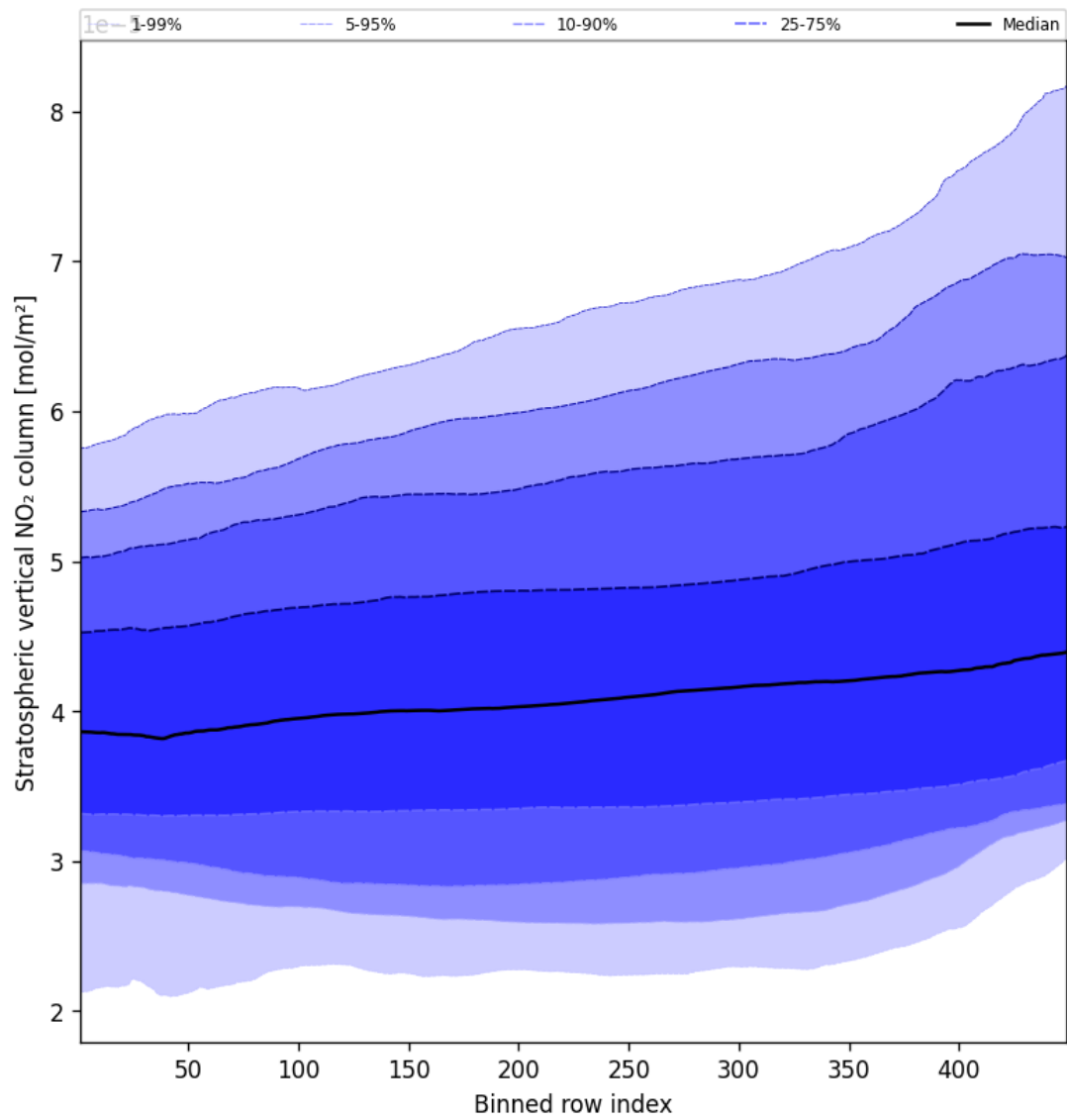
Figure 51: Along track statistics of “Stratospheric vertical NO 2 column” for 2025-10-05 to 2025-10-06
