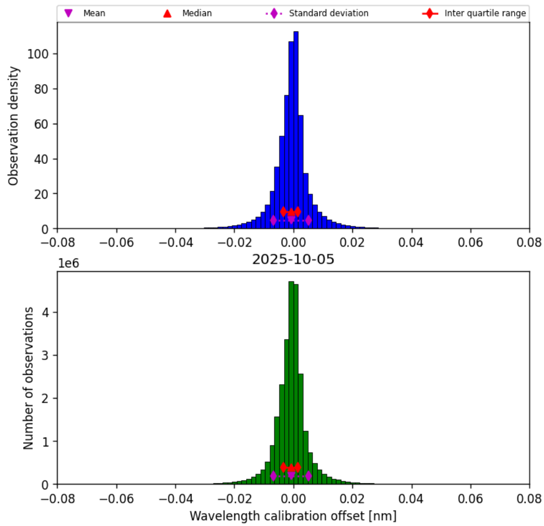
Figure 33: Histogram of “Wavelength calibration offset” for 2025-10-05 to 2025-10-06
