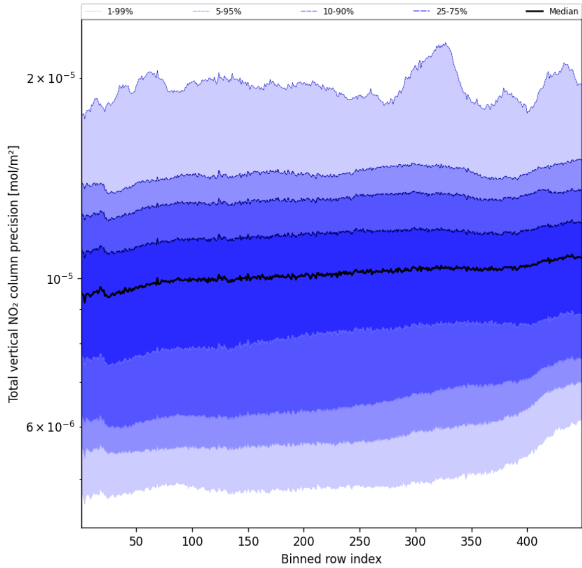
Figure 54: Along track statistics of “Total vertical NO 2 column precision” for 2025-10-05 to 2025-10-06
