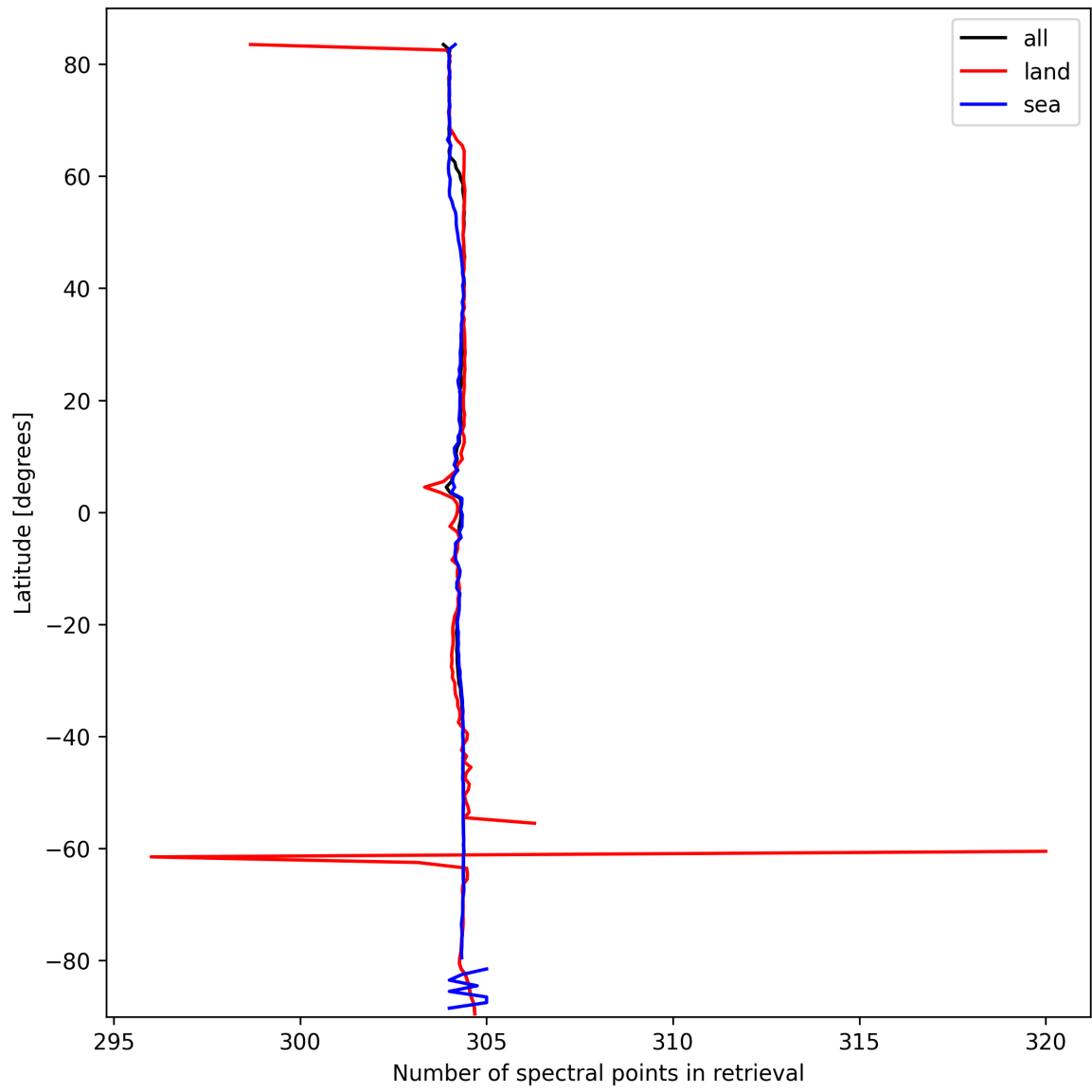
Figure 14: Zonal average of “Number of spectral points in retrieval” for 2025-10-05 to 2025-10-06.
