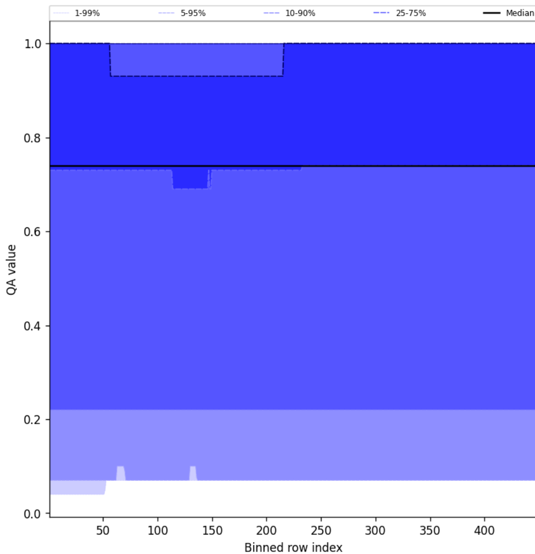
Figure 43: Along track statistics of “QA value” for 2025-10-05 to 2025-10-06
