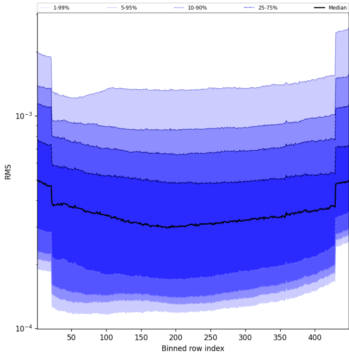
Figure 58: Along track statistics of “RMS” for 2025-10-05 to 2025-10-06
