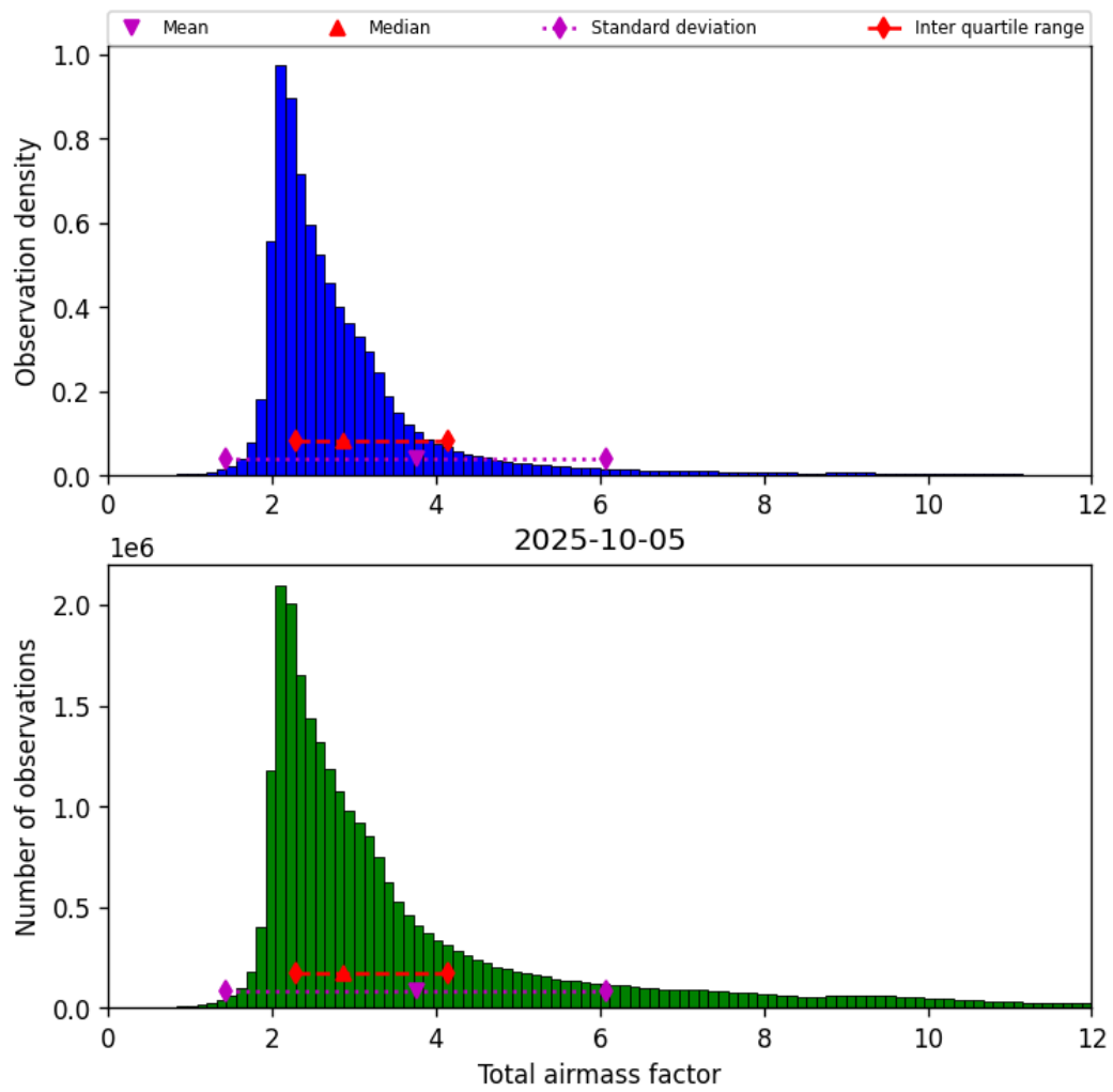
Figure 30: Histogram of “Total airmass factor” for 2025-10-05 to 2025-10-06
