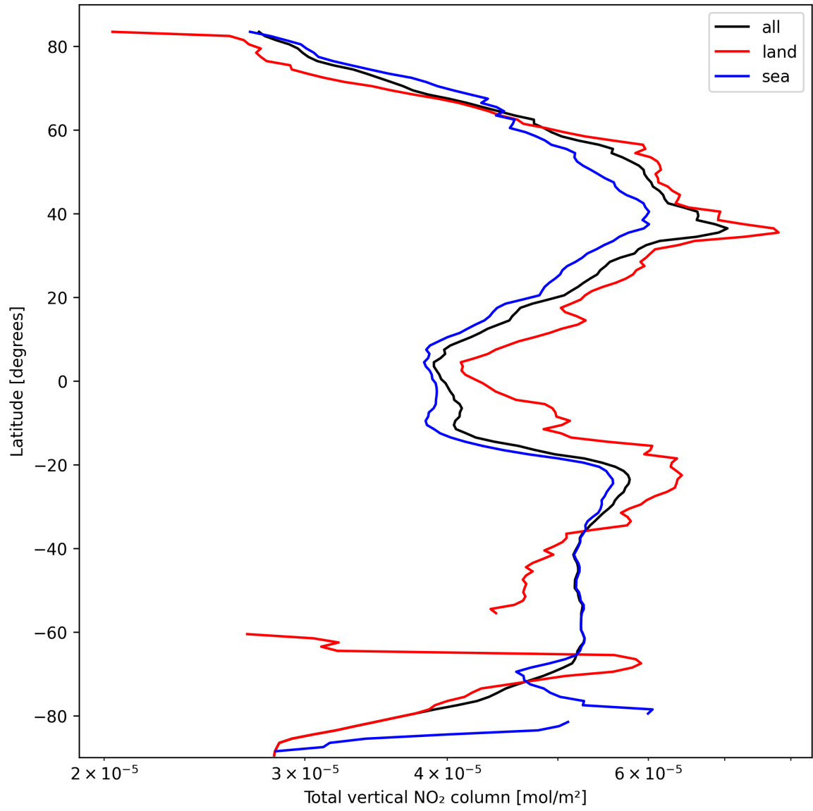
Figure 19: Zonal average of “Total vertical NO 2 column” for 2025-10-05 to 2025-10-06.
