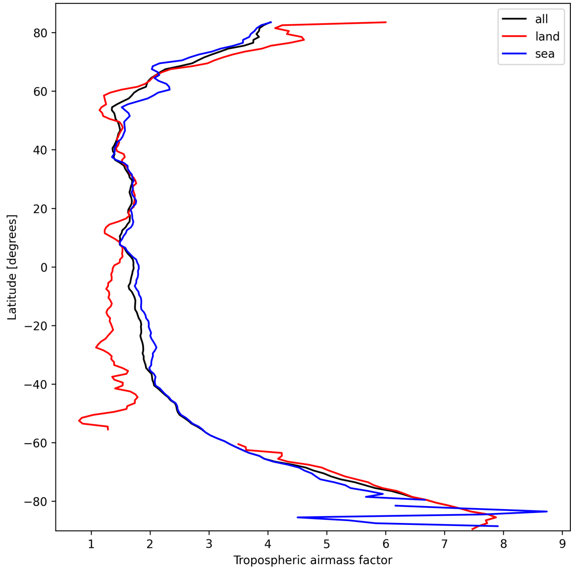
Figure 12: Zonal average of “Tropospheric airmass factor” for 2025-10-05 to 2025-10-06.
