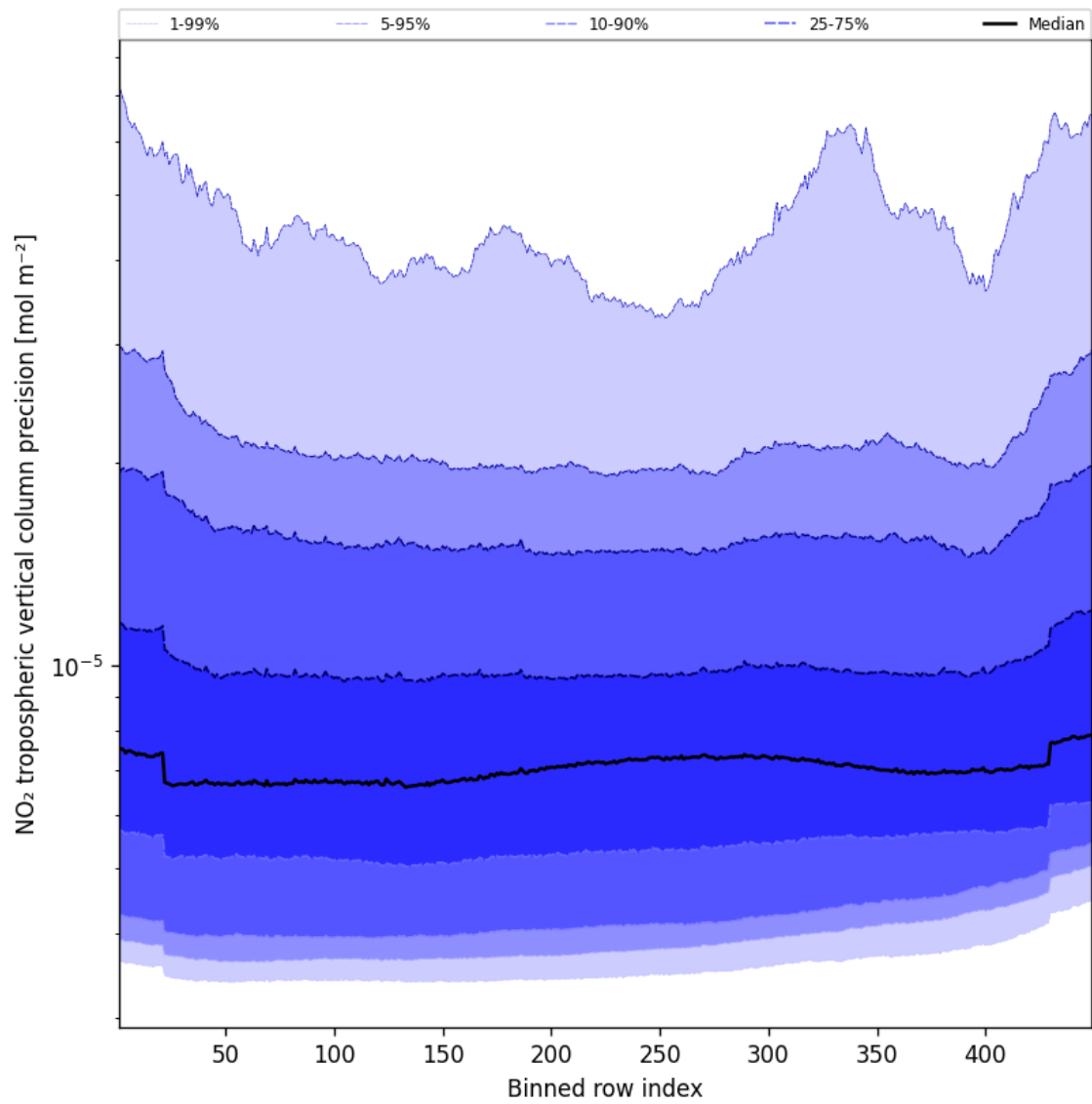
Figure 45: Along track statistics of “NO 2 tropospheric vertical column precision” for 2025-10-05 to 2025-10-06
