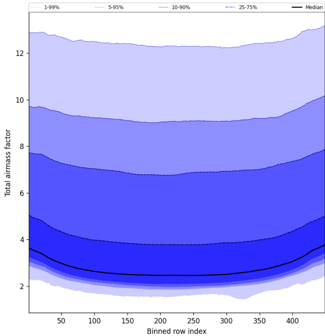
Figure 47: Along track statistics of “Total airmass factor” for 2025-10-05 to 2025-10-06
