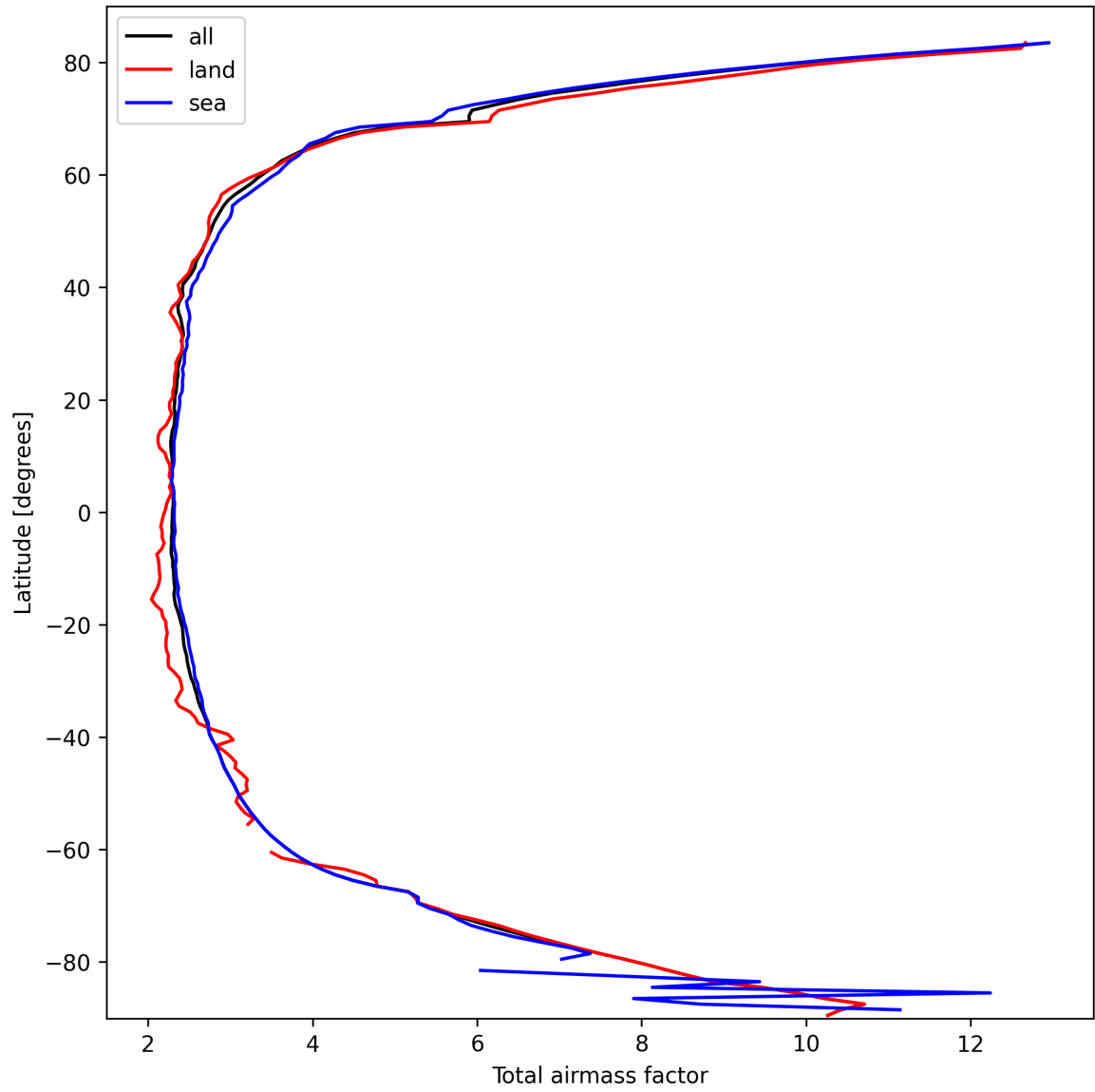
Figure 13: Zonal average of “Total airmass factor” for 2025-10-05 to 2025-10-06.
