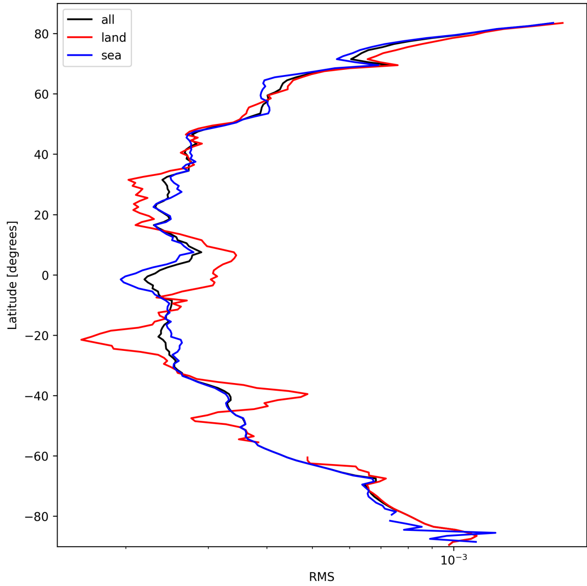
Figure 24: Zonal average of “RMS” for 2025-10-05 to 2025-10-06.
