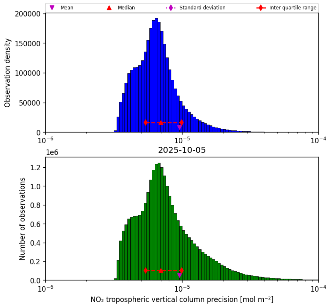
Figure 28: Histogram of “NO 2 tropospheric vertical column precision” for 2025-10-05 to 2025-10-06
