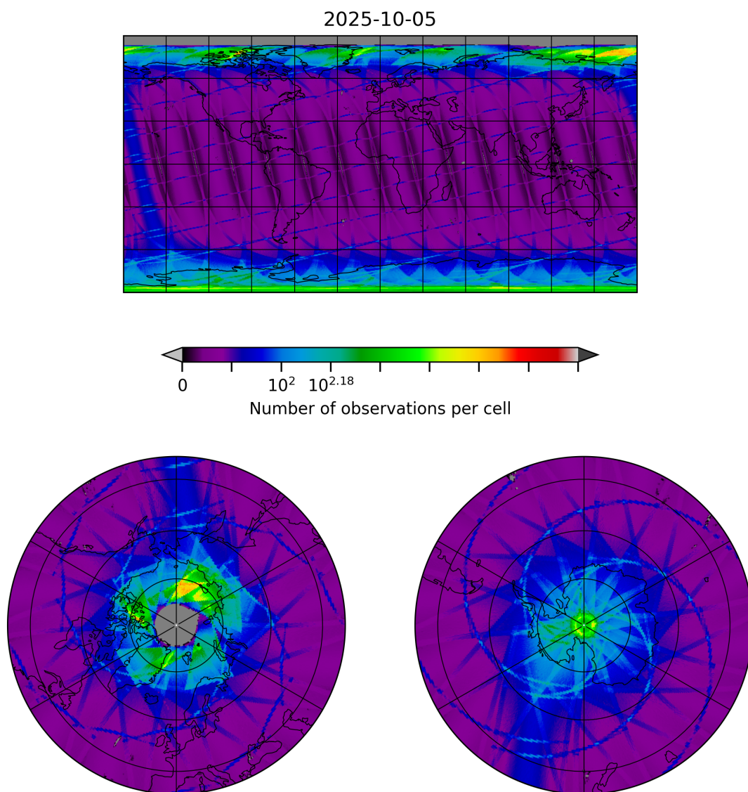
Figure 8: Map of the number of observations for 2025-10-05 to 2025-10-06
