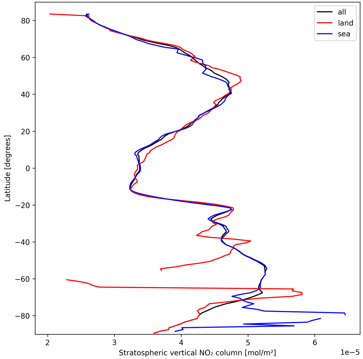
Figure 17: Zonal average of “Stratospheric vertical NO 2 column” for 2025-10-05 to 2025-10-06.
