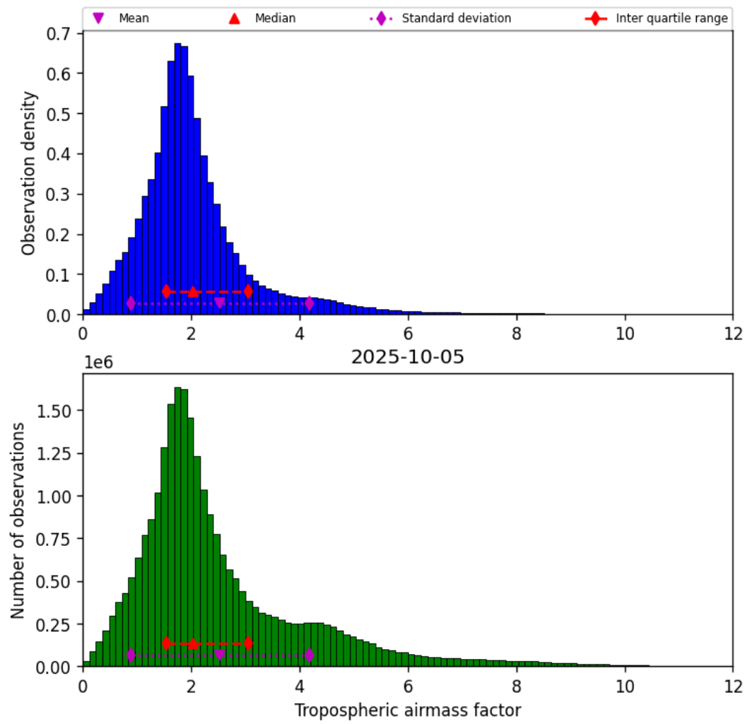
Figure 29: Histogram of “Tropospheric airmass factor” for 2025-10-05 to 2025-10-06
