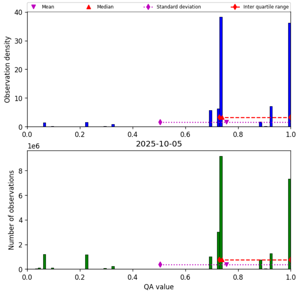
Figure 26: Histogram of “QA value” for 2025-10-05 to 2025-10-06
