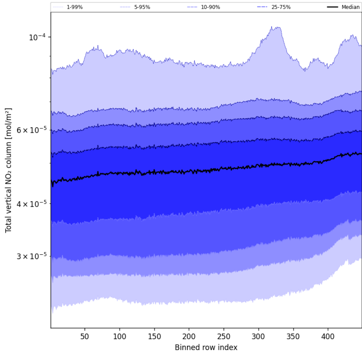
Figure 53: Along track statistics of “Total vertical NO 2 column” for 2025-10-05 to 2025-10-06
