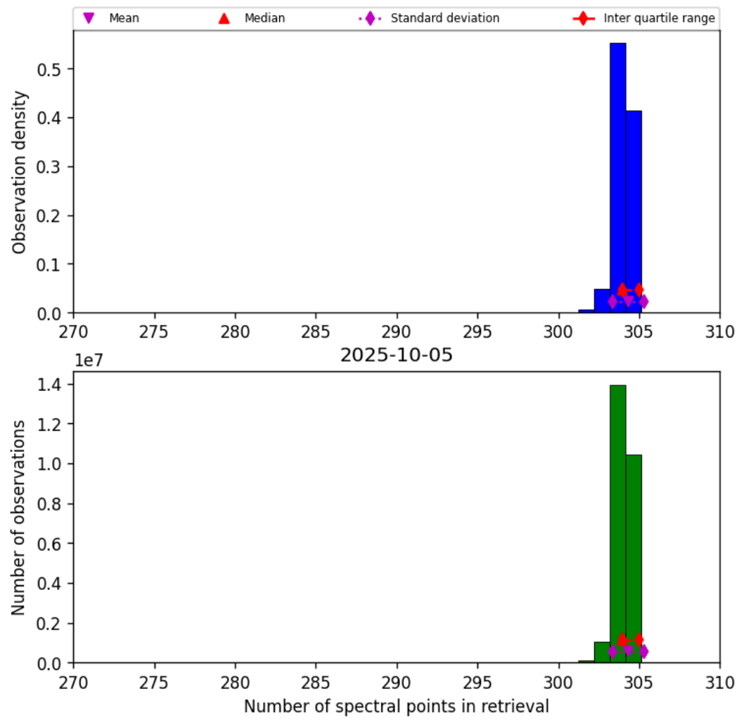
Figure 31: Histogram of “Number of spectral points in retrieval” for 2025-10-05 to 2025-10-06
