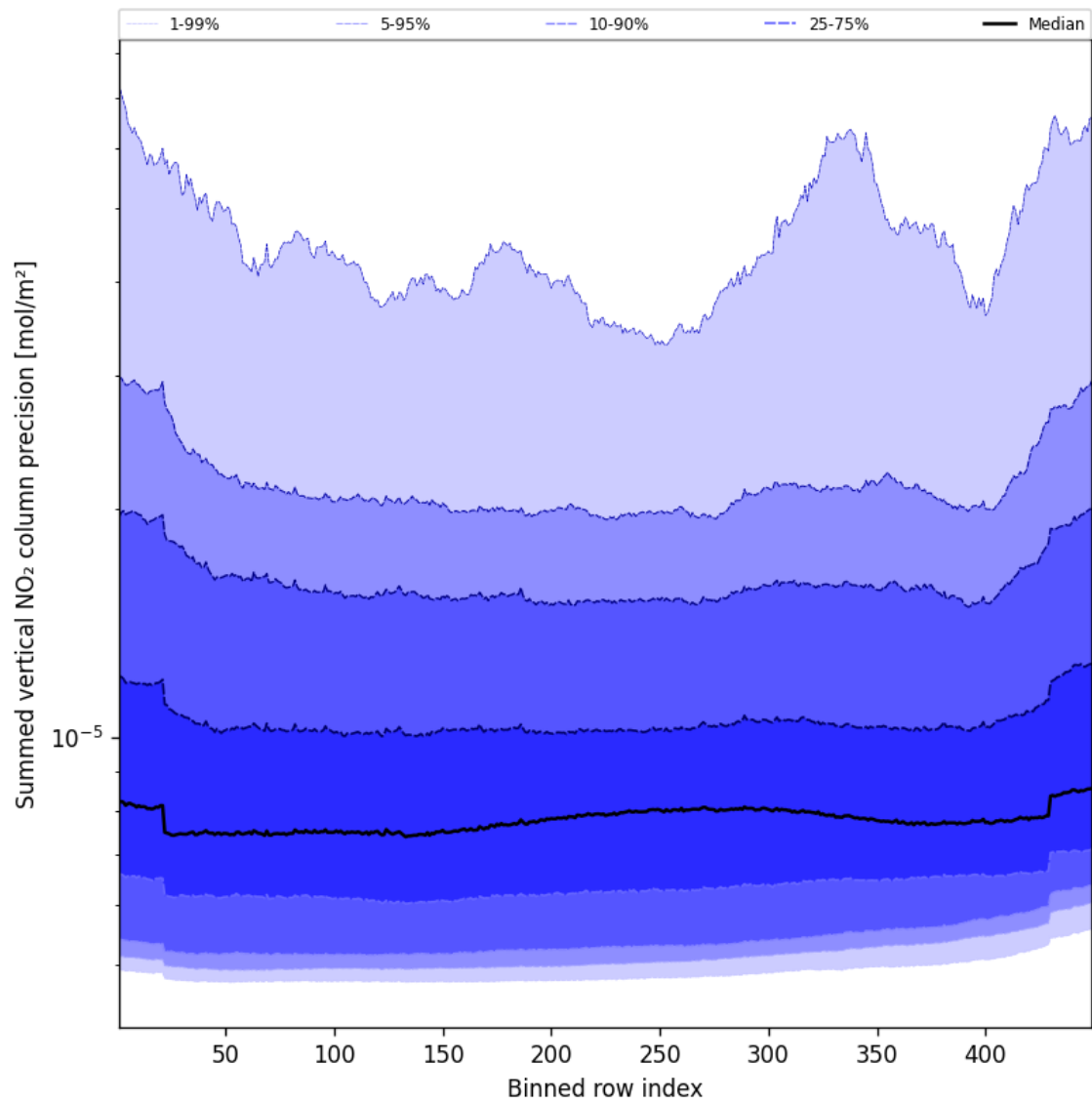
Figure 56: Along track statistics of “Summed vertical NO 2 column precision” for 2025-10-05 to 2025-10-06
