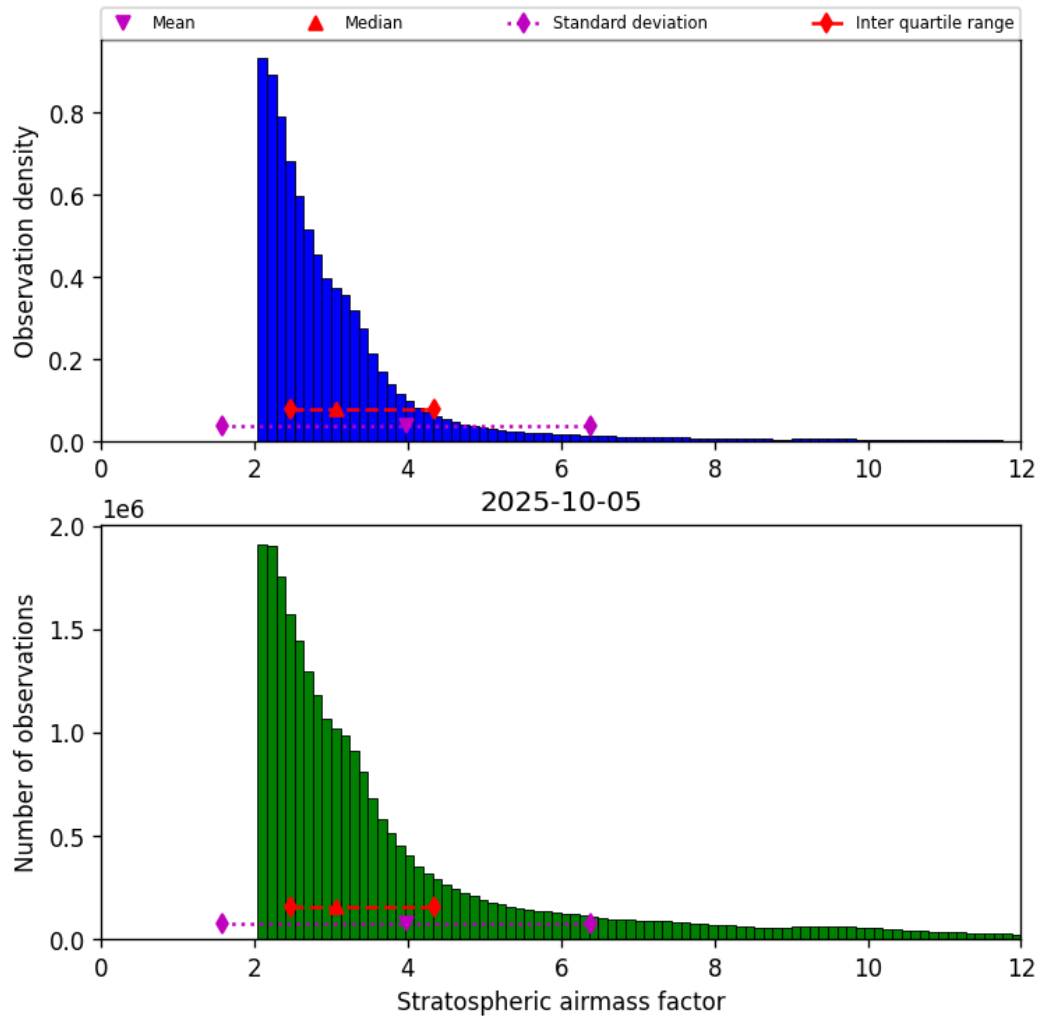
Figure 42: Histogram of “Stratospheric airmass factor” for 2025-10-05 to 2025-10-06
