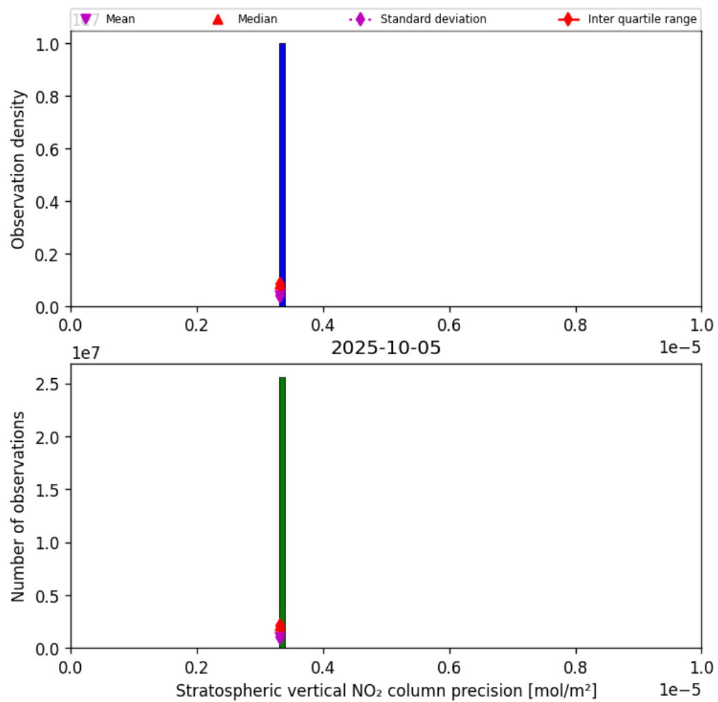
Figure 35: Histogram of “Stratospheric vertical NO 2 column precision” for 2025-10-05 to 2025-10-06
