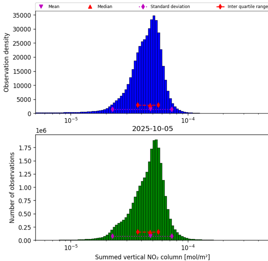
Figure 38: Histogram of "Summed vertical NO 2 column" for 2025-10-05 to 2025-10-06
