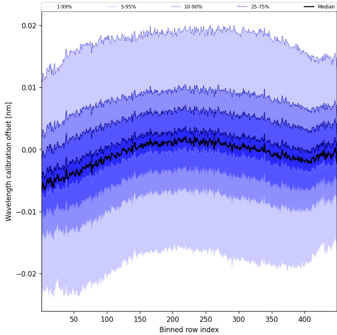
Figure 50: Along track statistics of “Wavelength calibration offset” for 2025-10-05 to 2025-10-06
