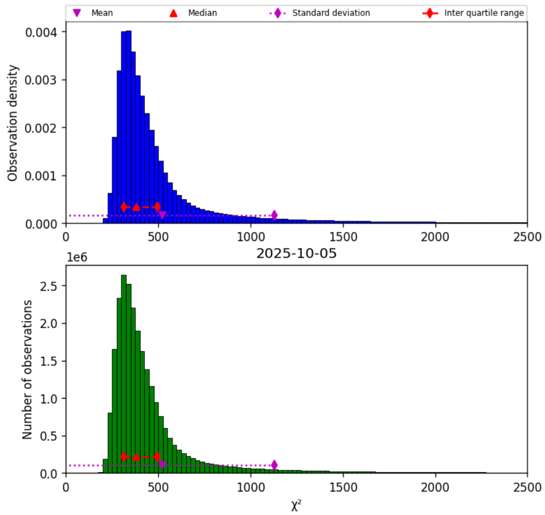
Figure 40: Histogram of “ \chi^2 ” for 2025-10-05 to 2025-10-06
