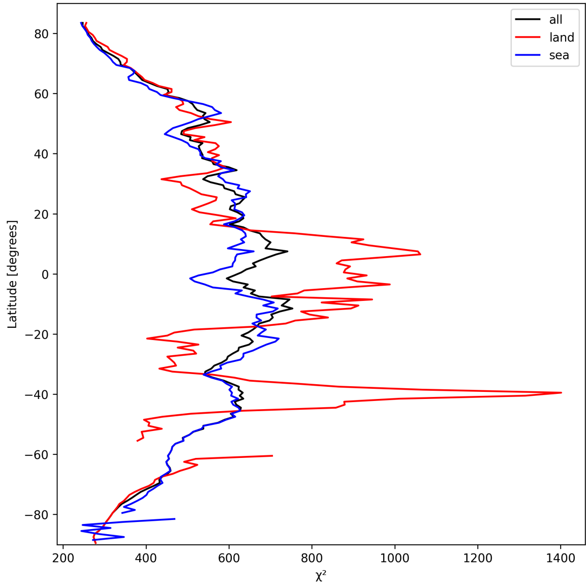
Figure 23: Zonal average of “ \chi^2 ” for 2025-10-05 to 2025-10-06.
