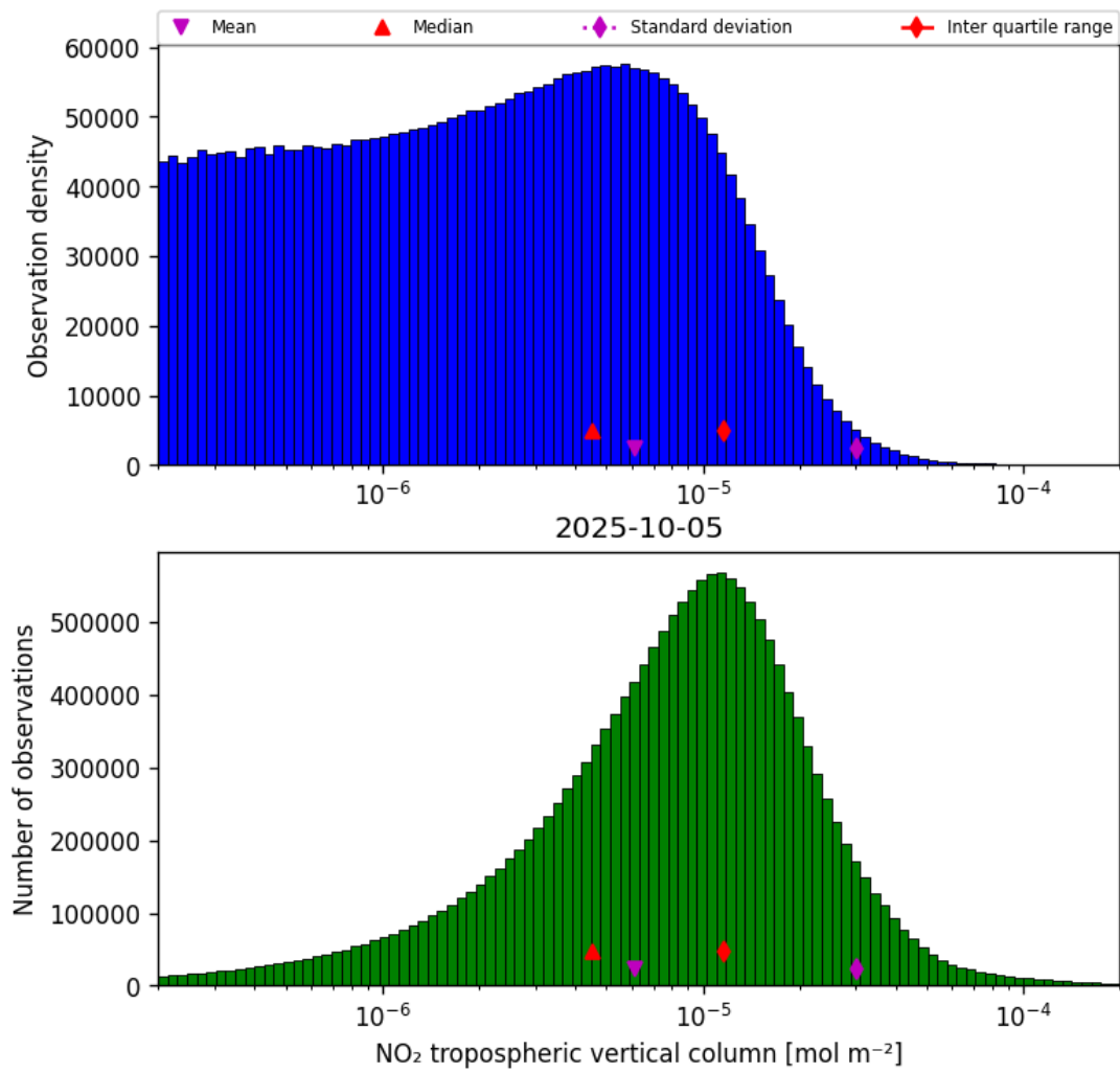
Figure 27: Histogram of “NO 2 tropospheric vertical column” for 2025-10-05 to 2025-10-06
