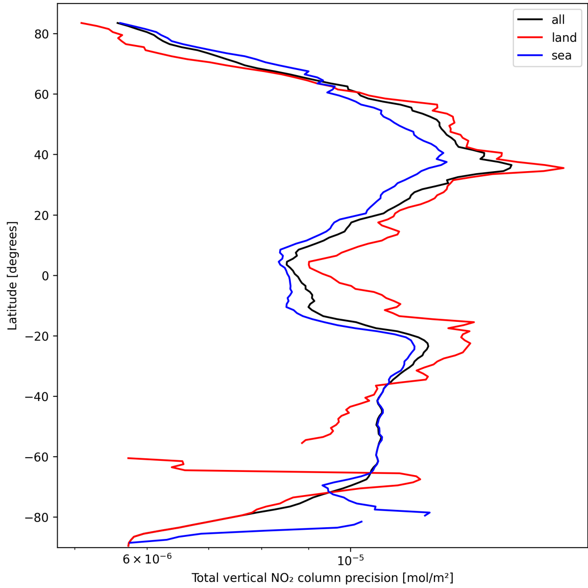
Figure 20: Zonal average of “Total vertical NO 2 column precision” for 2025-10-05 to 2025-10-06.
