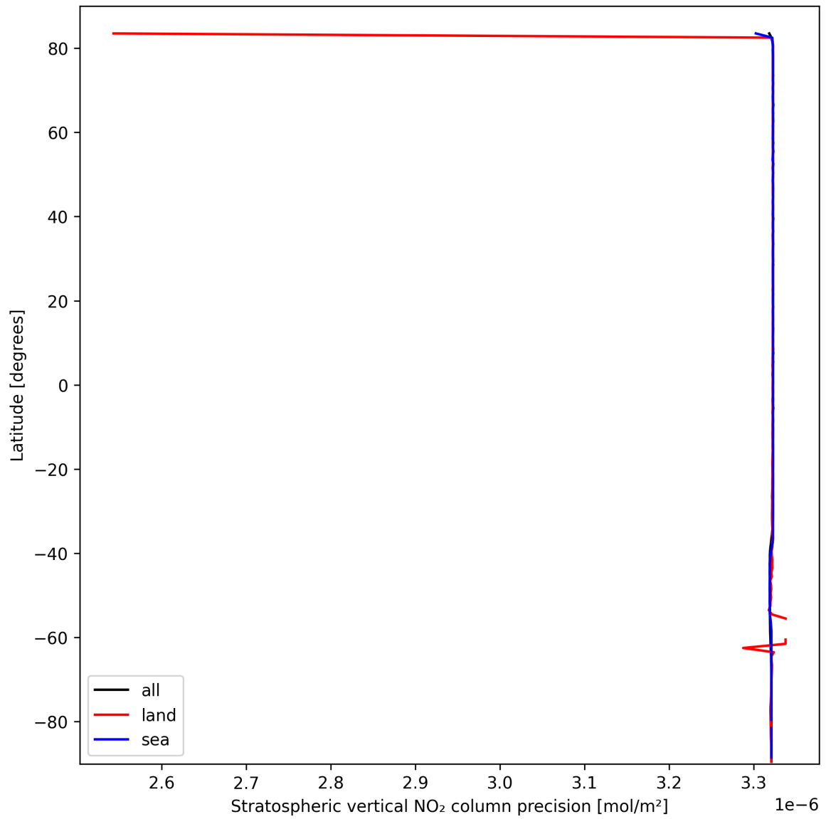
Figure 18: Zonal average of “Stratospheric vertical NO 2 column precision” for 2025-10-05 to 2025-10-06.
