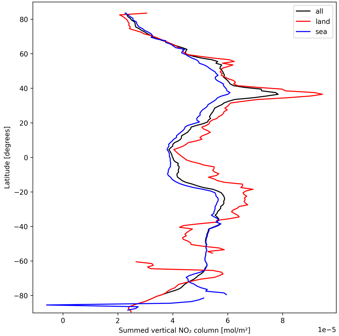
Figure 21: Zonal average of “Summed vertical NO 2 column” for 2025-10-05 to 2025-10-06.
