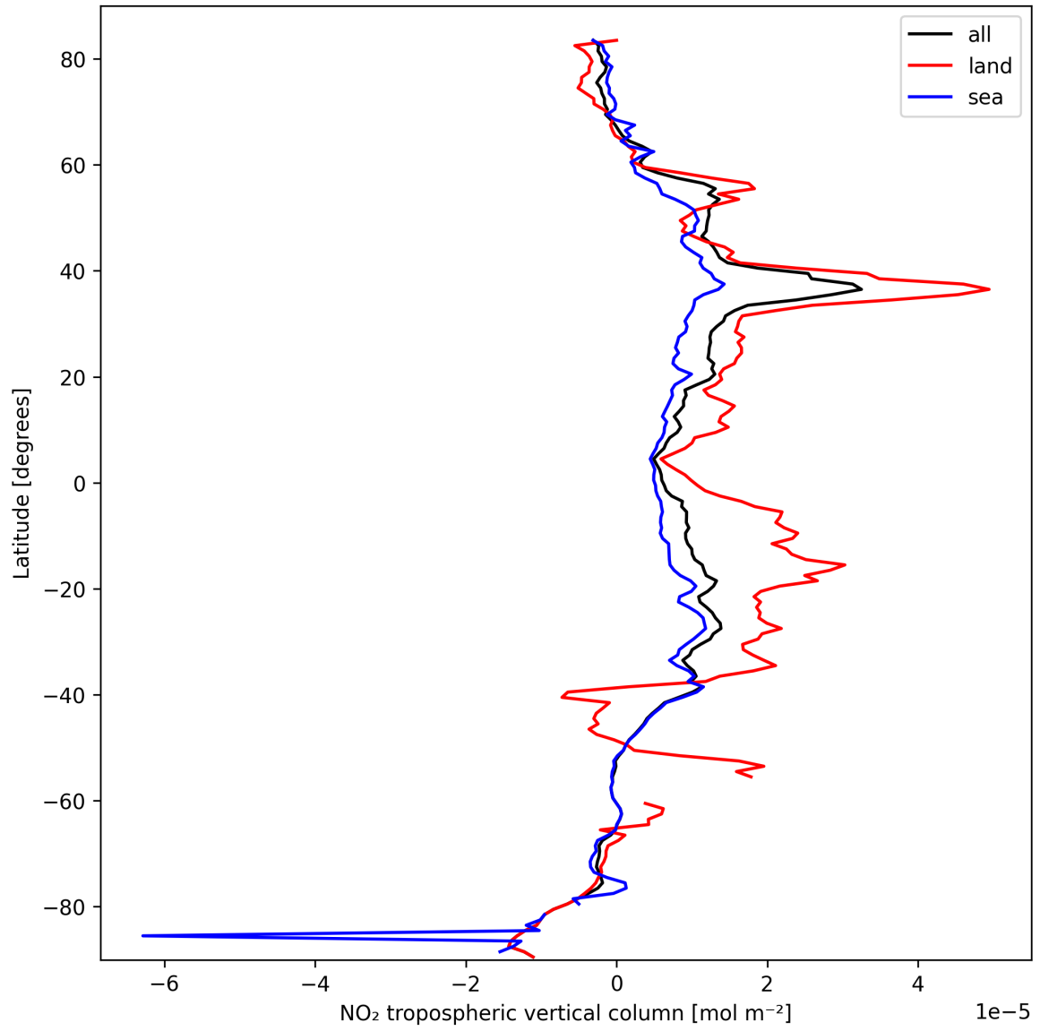
Figure 10: Zonal average of “NO 2 tropospheric vertical column” for 2025-10-05 to 2025-10-06.
