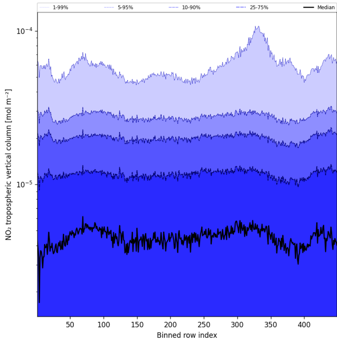
Figure 44: Along track statistics of “NO 2 tropospheric vertical column” for 2025-10-05 to 2025-10-06
