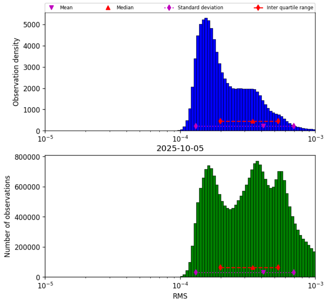
Figure 41: Histogram of “RMS” for 2025-10-05 to 2025-10-06
