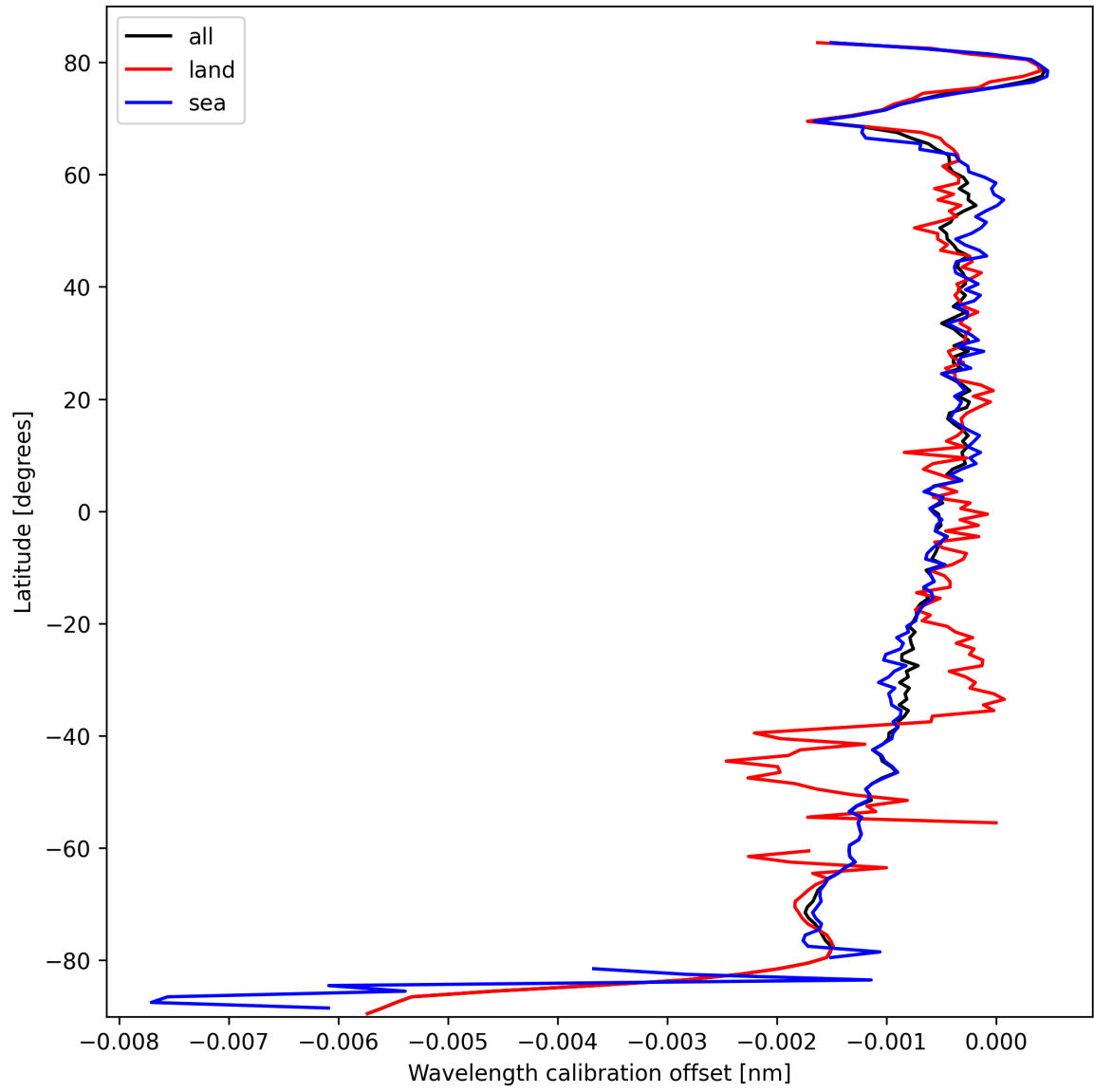
Figure 16: Zonal average of “Wavelength calibration offset” for 2025-10-05 to 2025-10-06.
