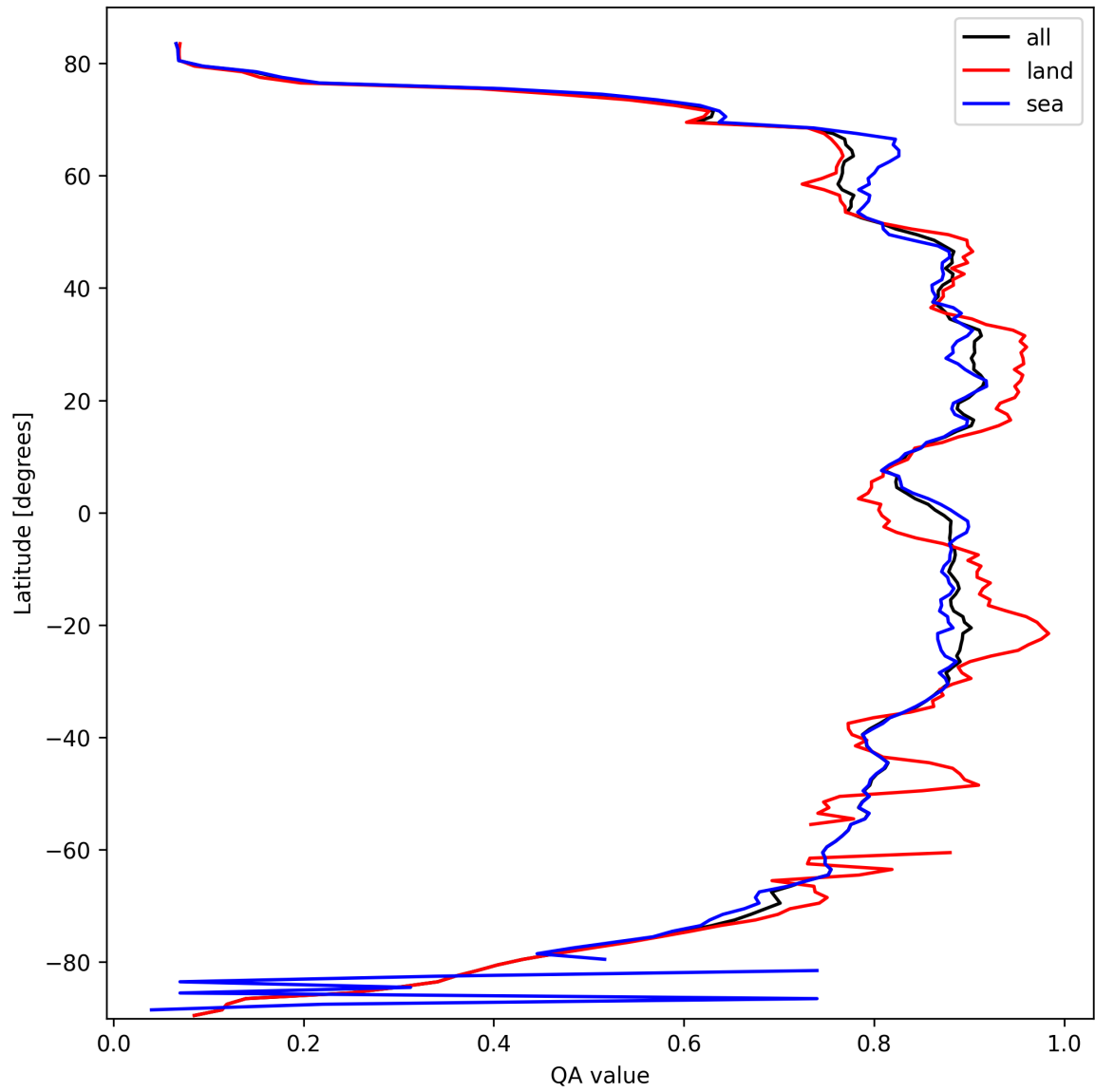
Figure 9: Zonal average of “QA value” for 2025-10-05 to 2025-10-06.
