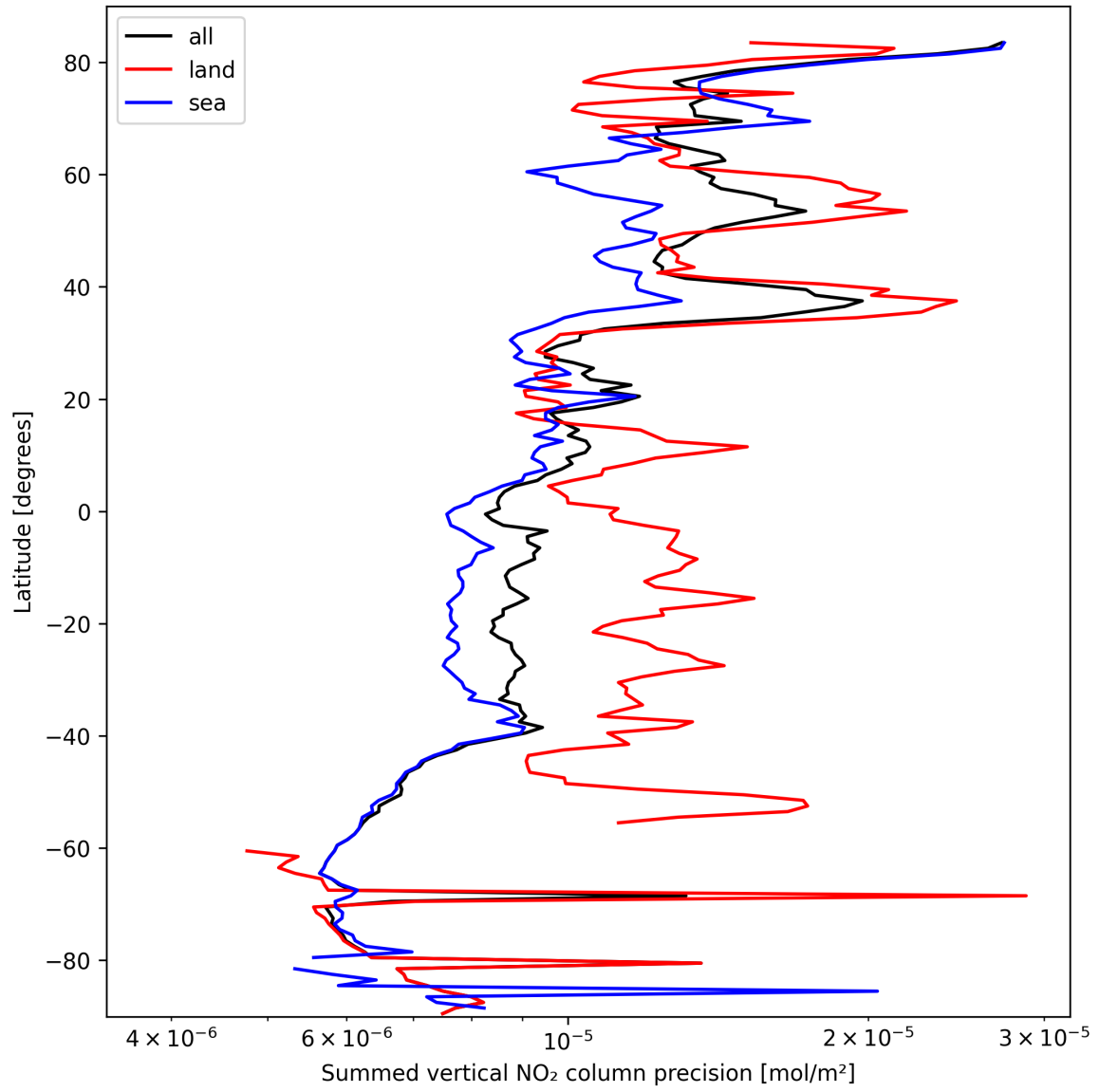
Figure 22: Zonal average of “Summed vertical NO 2 column precision” for 2025-10-05 to 2025-10-06.
