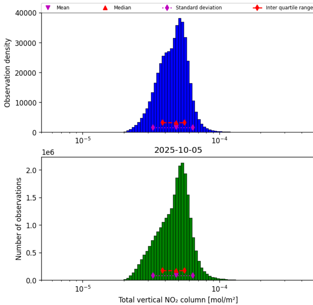
Figure 36: Histogram of “Total vertical NO 2 column” for 2025-10-05 to 2025-10-06
