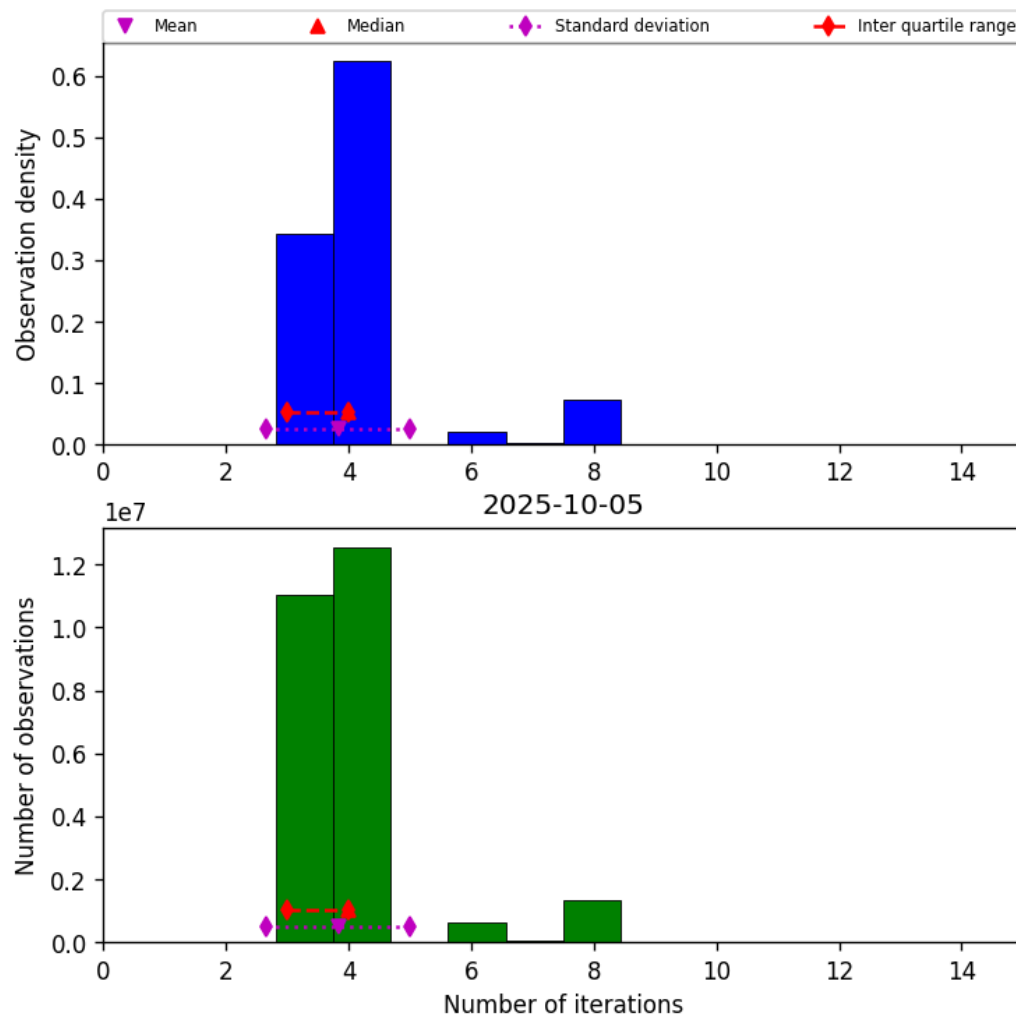
Figure 32: Histogram of “Number of iterations” for 2025-10-05 to 2025-10-06
