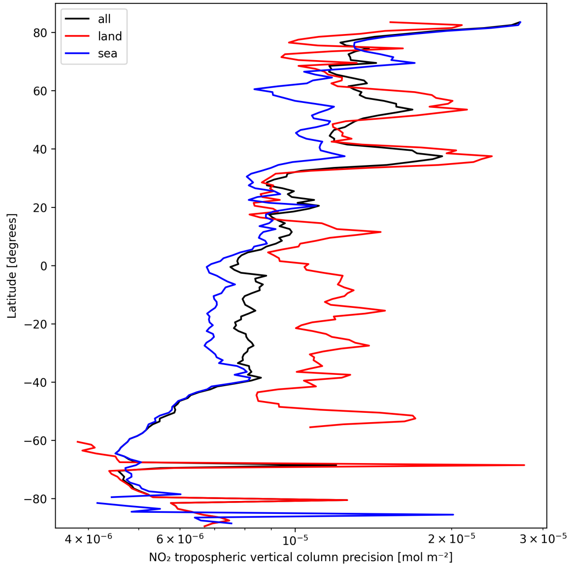
Figure 11: Zonal average of “NO 2 tropospheric vertical column precision” for 2025-10-05 to 2025-10-06.
