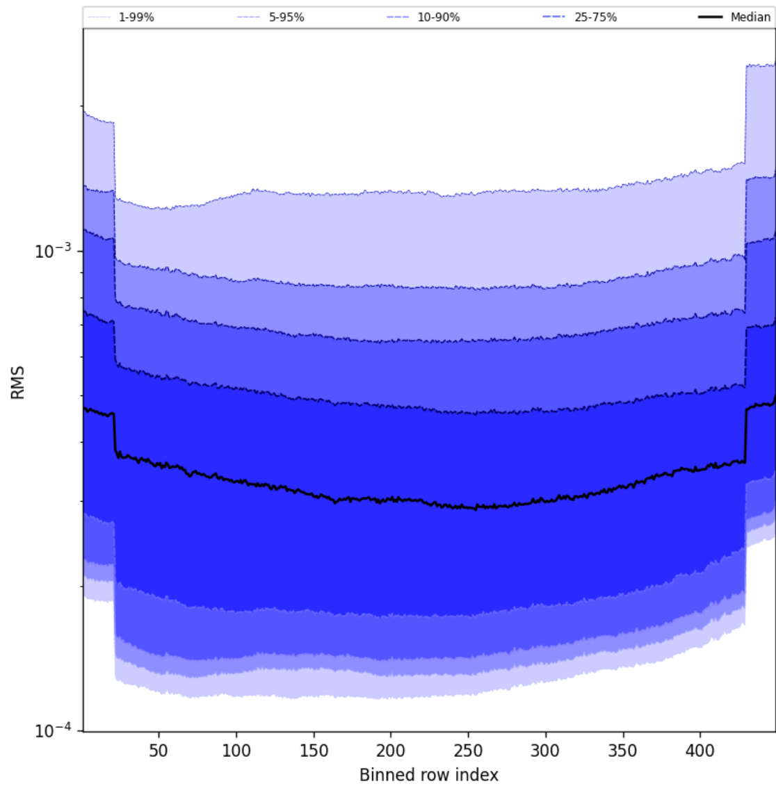
Figure 58: Along track statistics of “RMS” for 2025-10-06 to 2025-10-07
