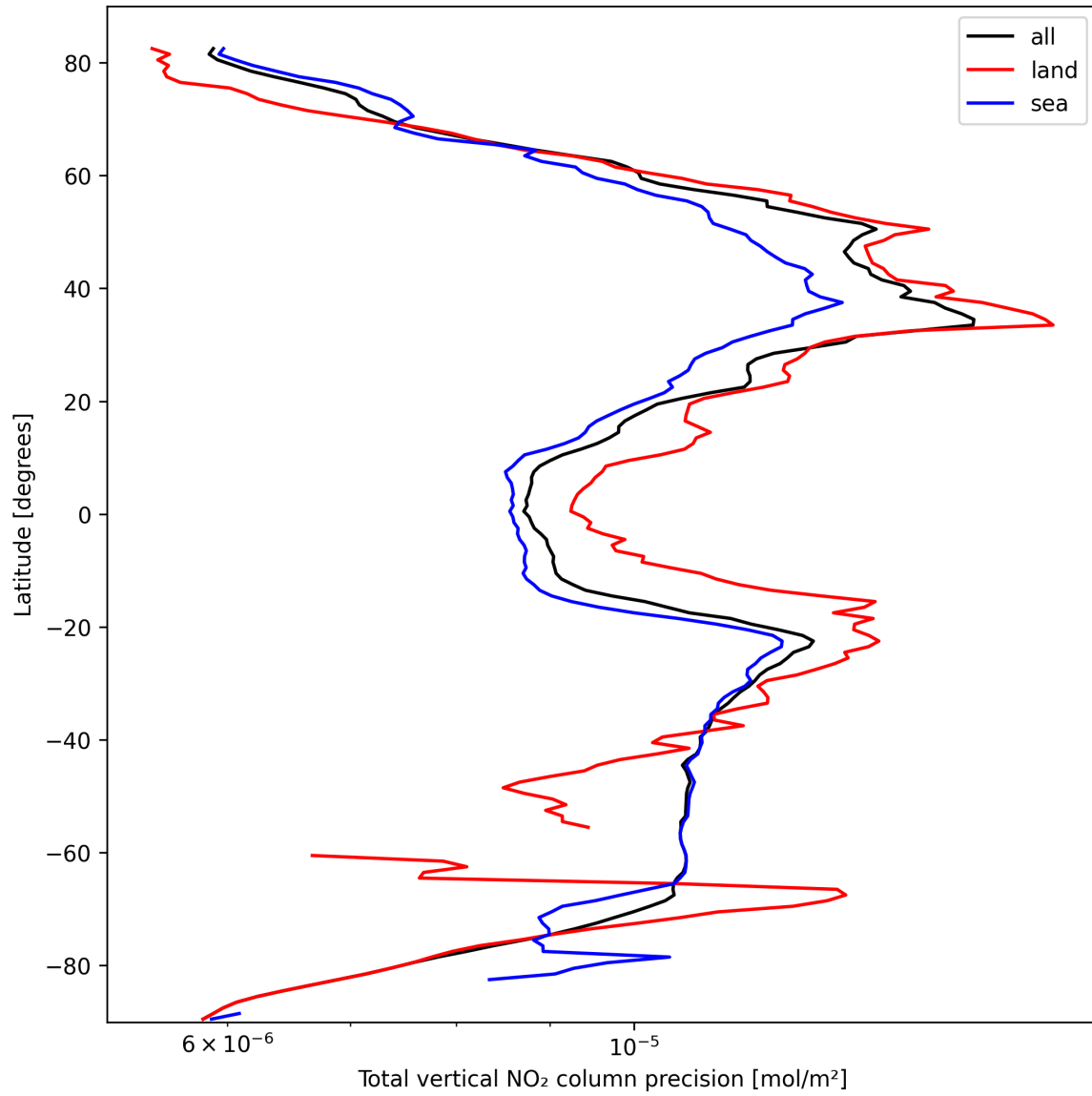
Figure 20: Zonal average of “Total vertical NO 2 column precision” for 2025-10-06 to 2025-10-07.
