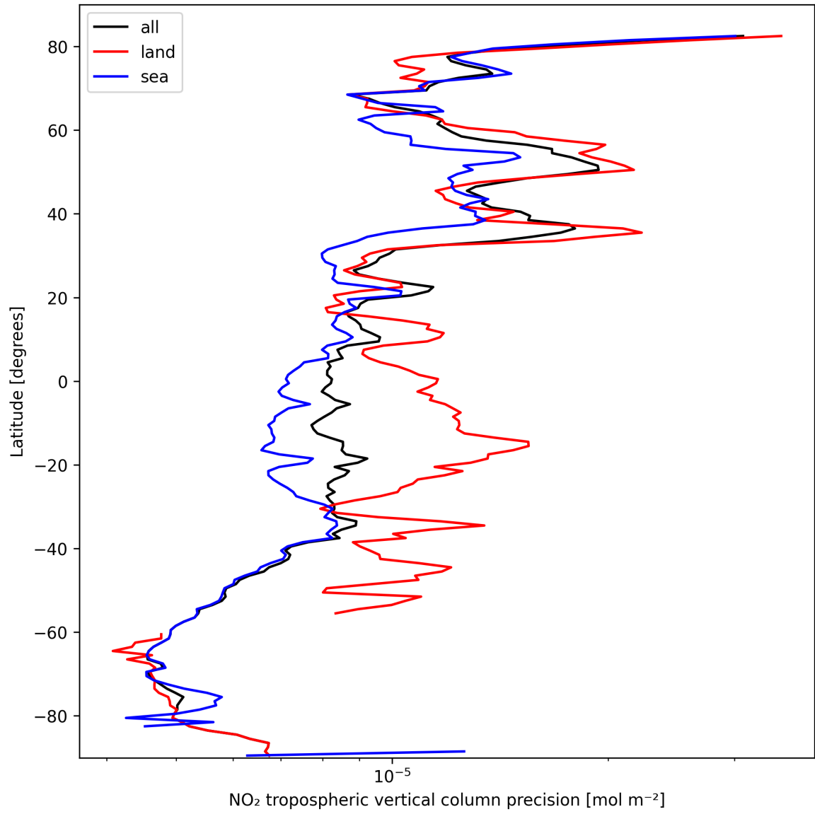
Figure 11: Zonal average of “NO 2 tropospheric vertical column precision” for 2025-10-06 to 2025-10-07.
