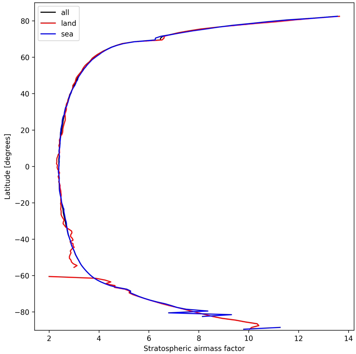
Figure 25: Zonal average of “Stratospheric airmass factor” for 2025-10-06 to 2025-10-07.
