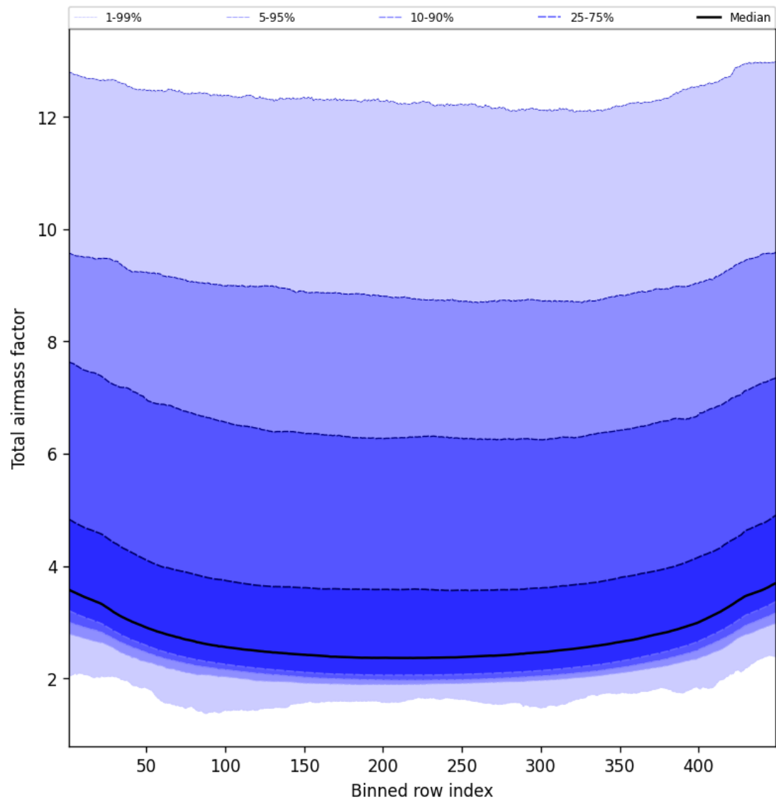
Figure 47: Along track statistics of “Total airmass factor” for 2025-10-06 to 2025-10-07
