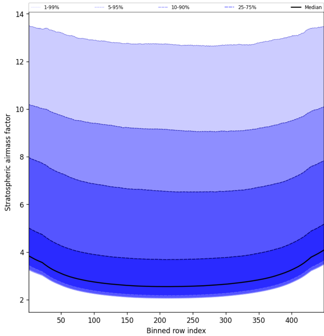
Figure 59: Along track statistics of “Stratospheric airmass factor” for 2025-10-06 to 2025-10-07
