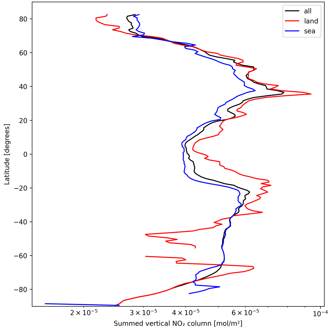
Figure 21: Zonal average of “Summed vertical NO 2 column” for 2025-10-06 to 2025-10-07.
