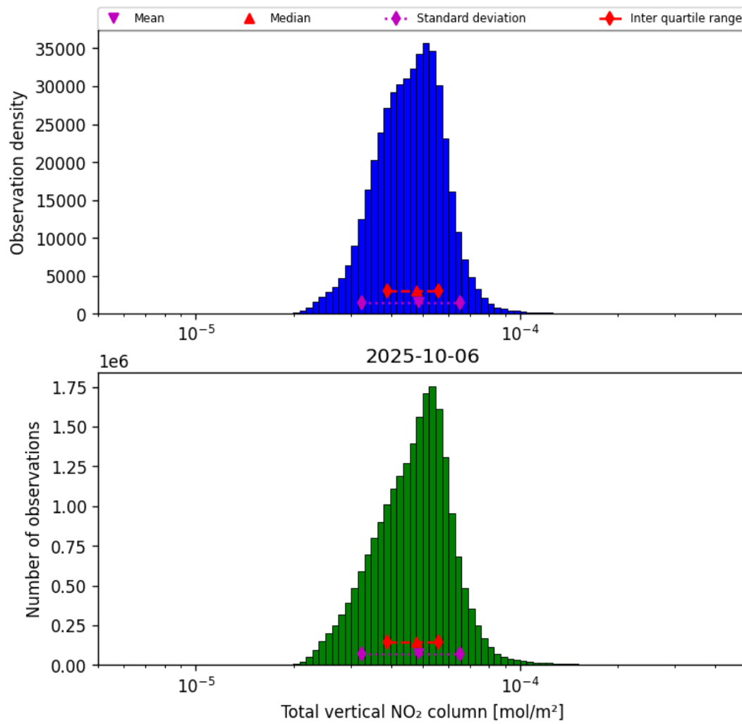
Figure 36: Histogram of “Total vertical NO 2 column” for 2025-10-06 to 2025-10-07
