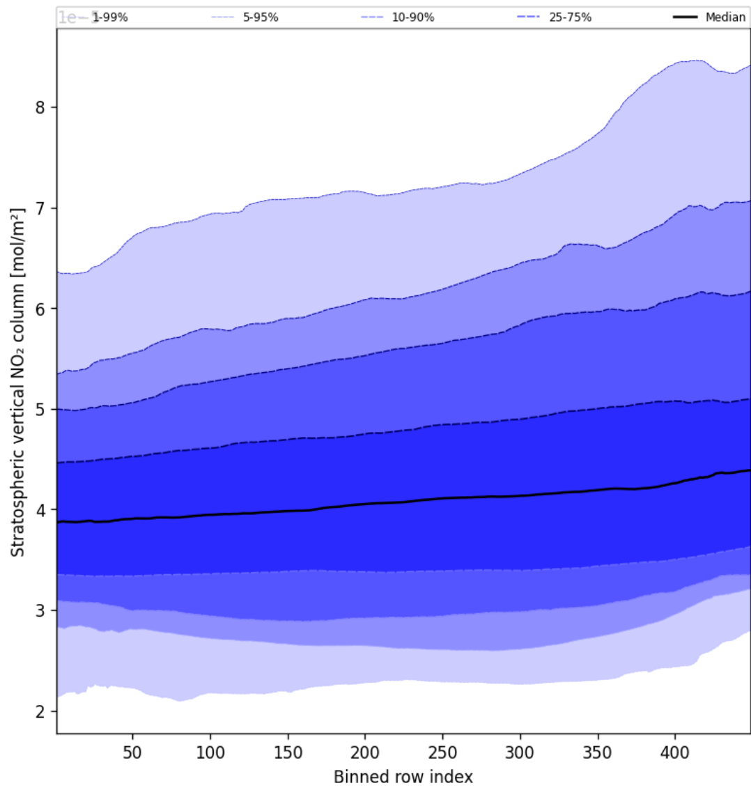
Figure 51: Along track statistics of “Stratospheric vertical NO 2 column” for 2025-10-06 to 2025-10-07
