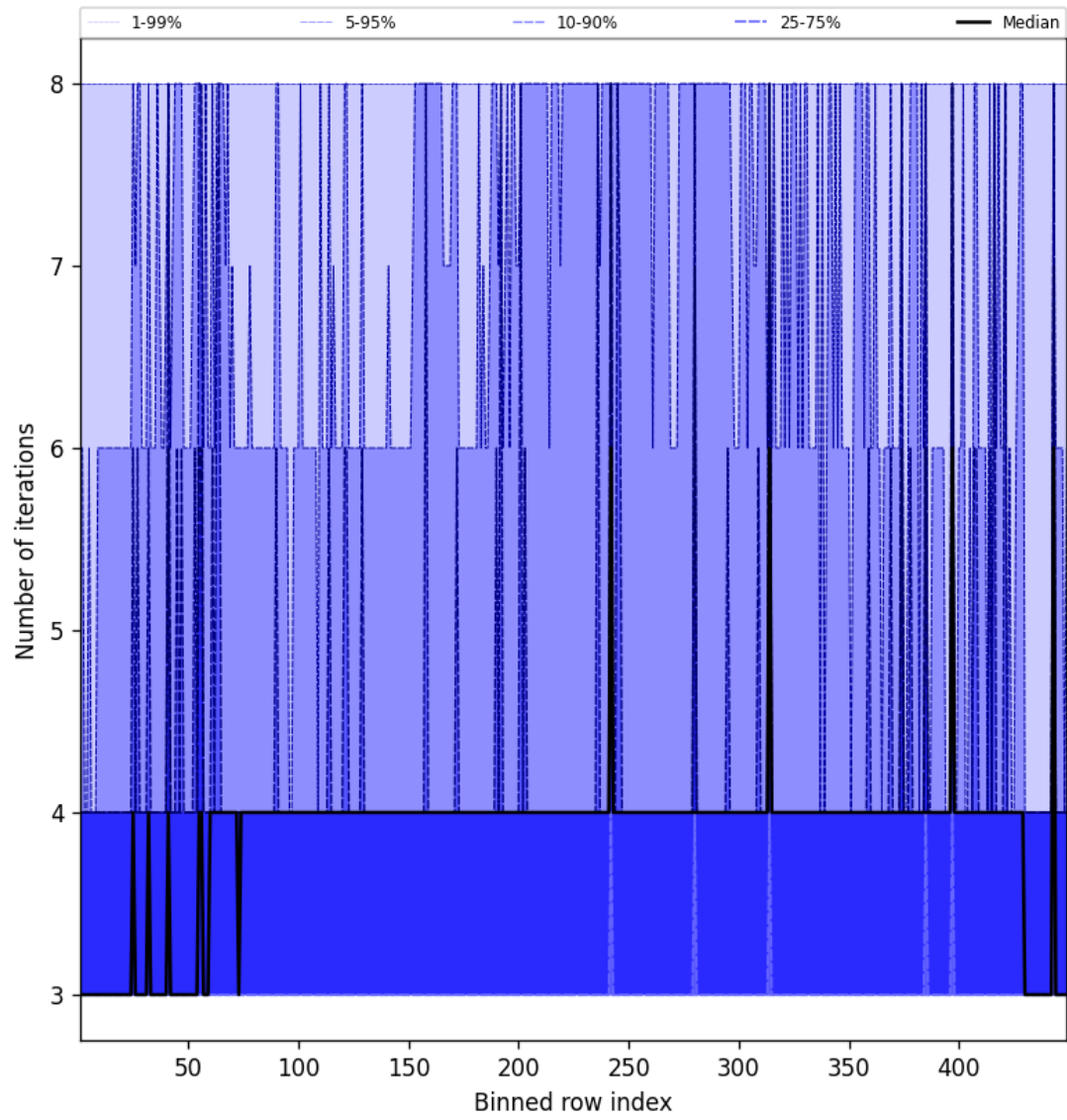
Figure 49: Along track statistics of “Number of iterations” for 2025-10-06 to 2025-10-07
