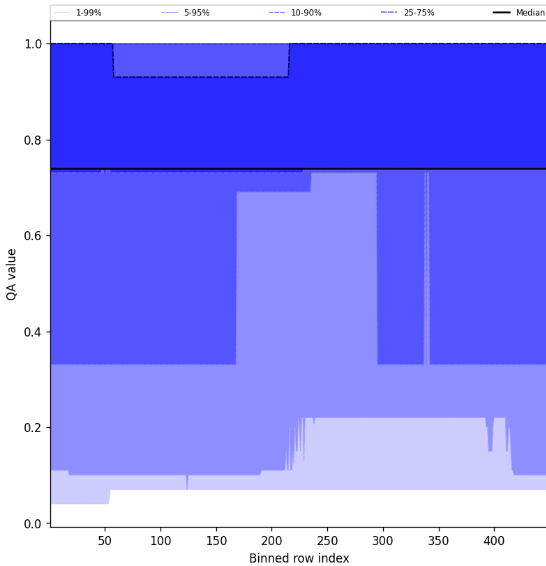
Figure 43: Along track statistics of “QA value” for 2025-10-06 to 2025-10-07
