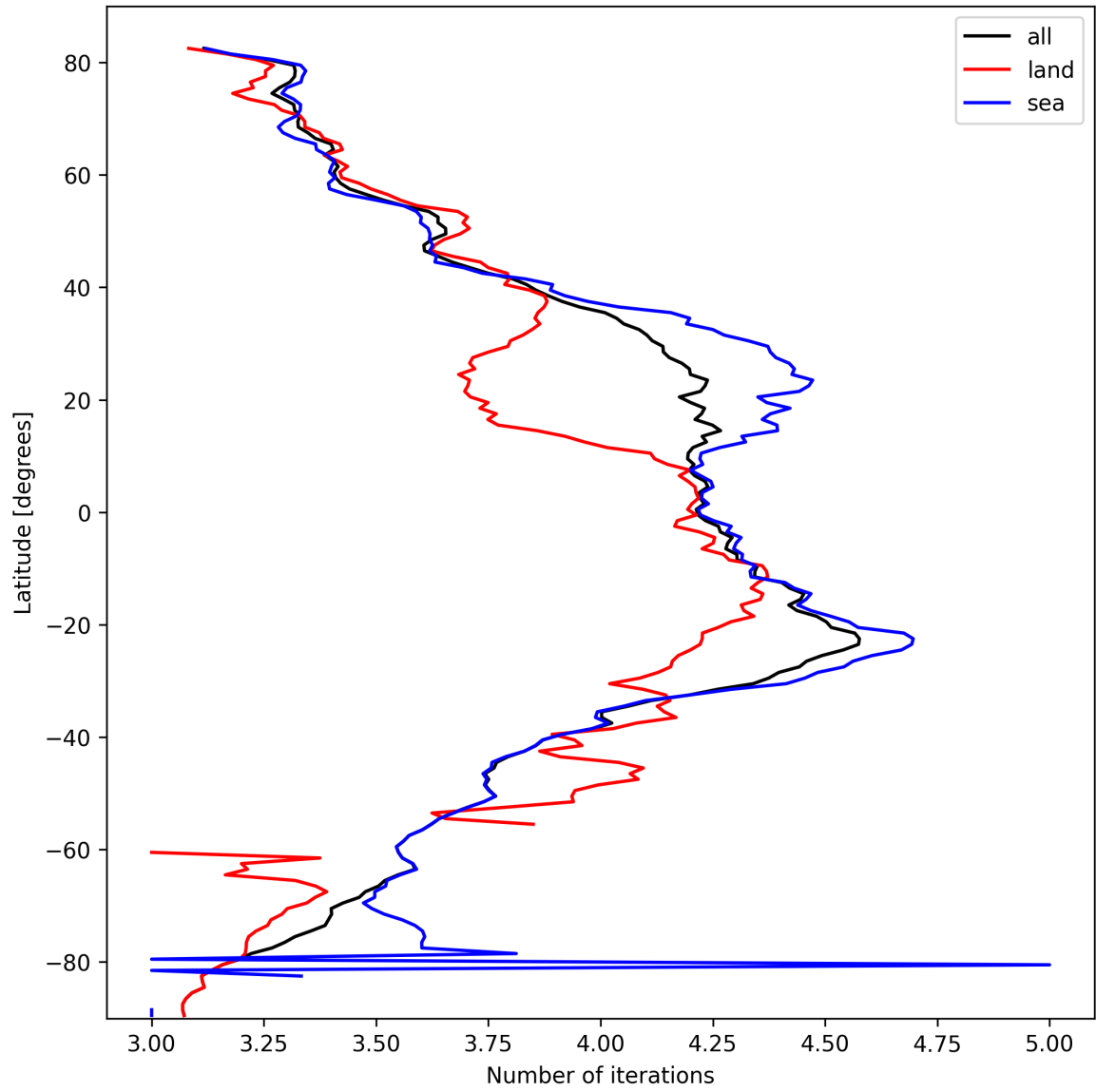
Figure 15: Zonal average of “Number of iterations” for 2025-10-06 to 2025-10-07.
