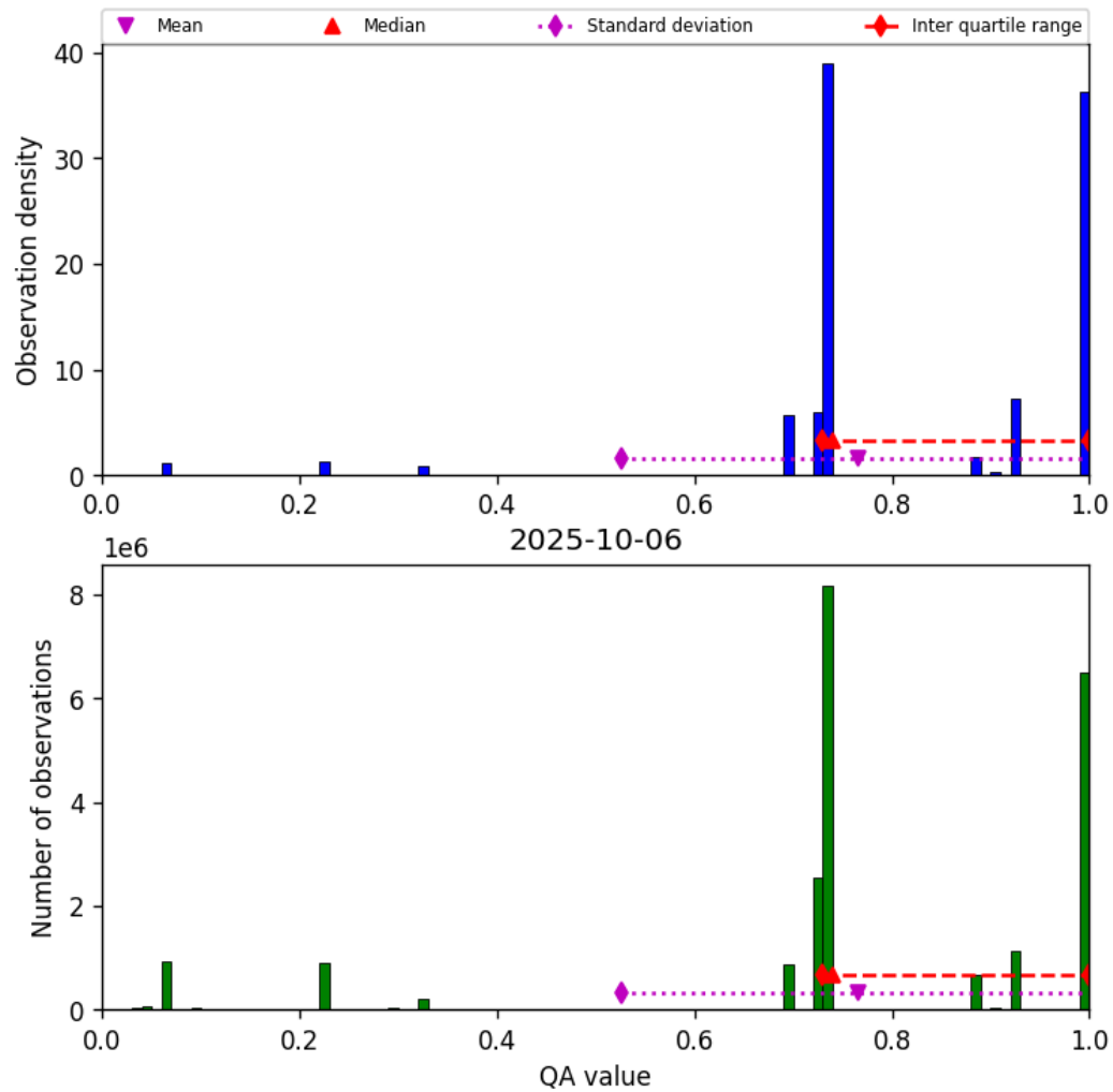
Figure 26: Histogram of “QA value” for 2025-10-06 to 2025-10-07
