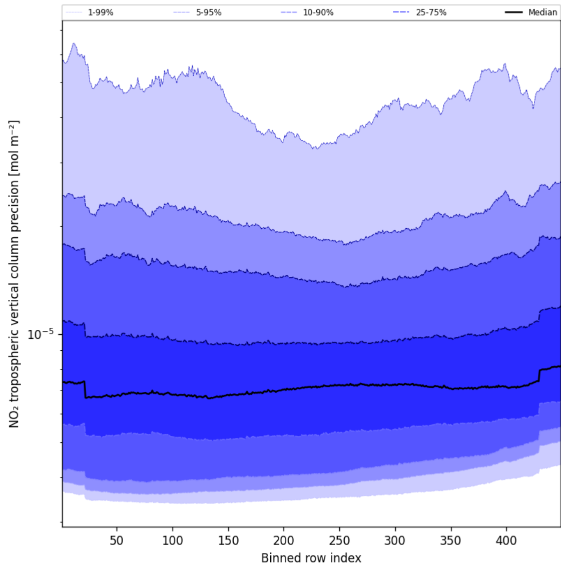
Figure 45: Along track statistics of “NO 2 tropospheric vertical column precision” for 2025-10-06 to 2025-10-07
