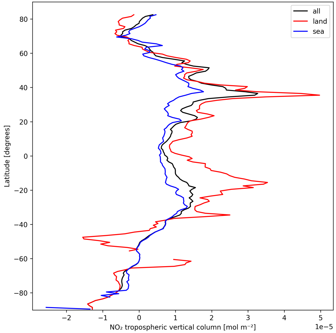
Figure 10: Zonal average of “NO 2 tropospheric vertical column” for 2025-10-06 to 2025-10-07.
