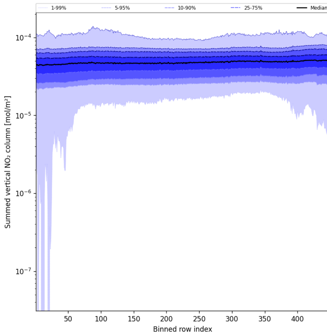
Figure 55: Along track statistics of “Summed vertical NO 2 column” for 2025-10-06 to 2025-10-07
