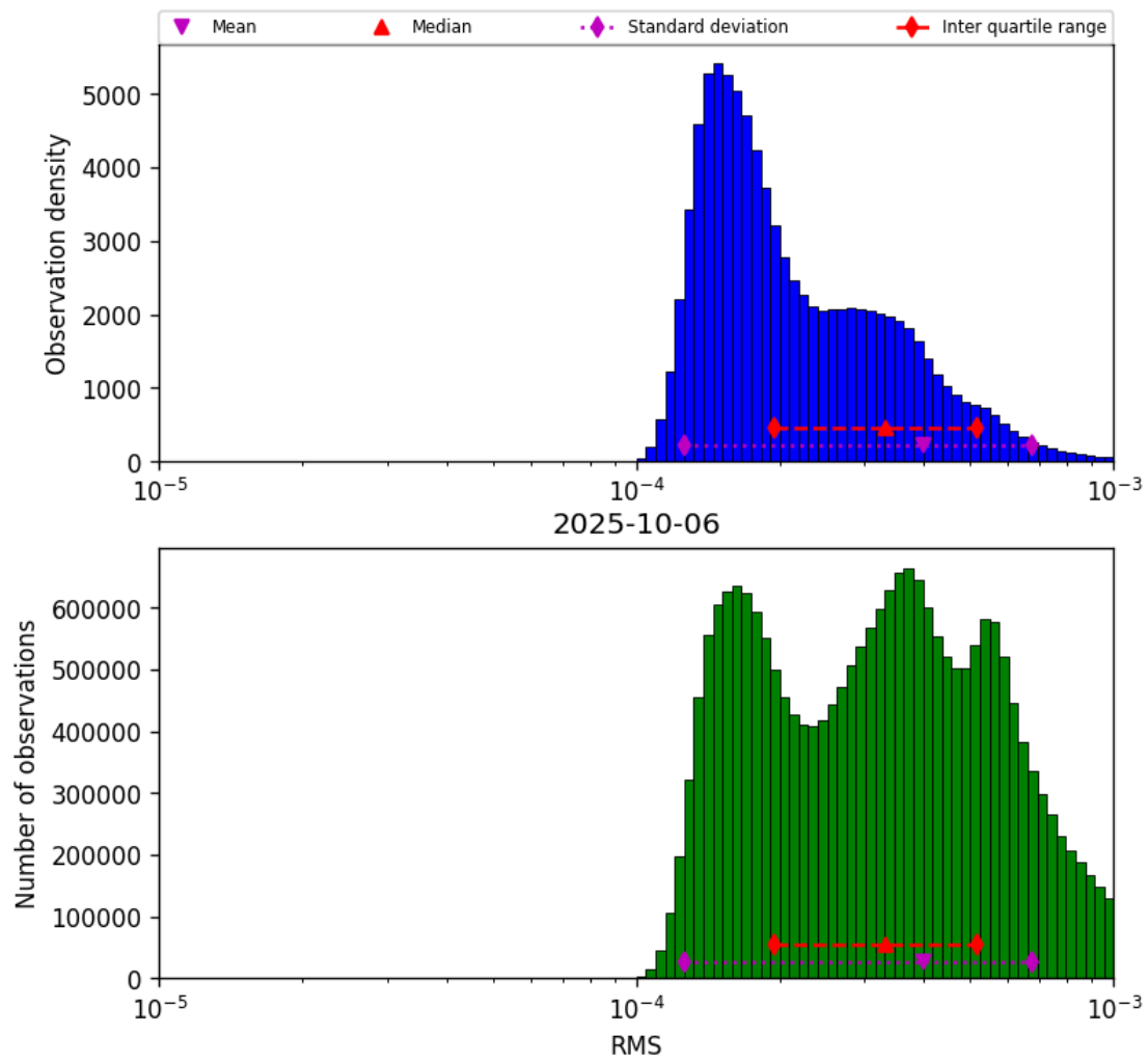
Figure 41: Histogram of “RMS” for 2025-10-06 to 2025-10-07
