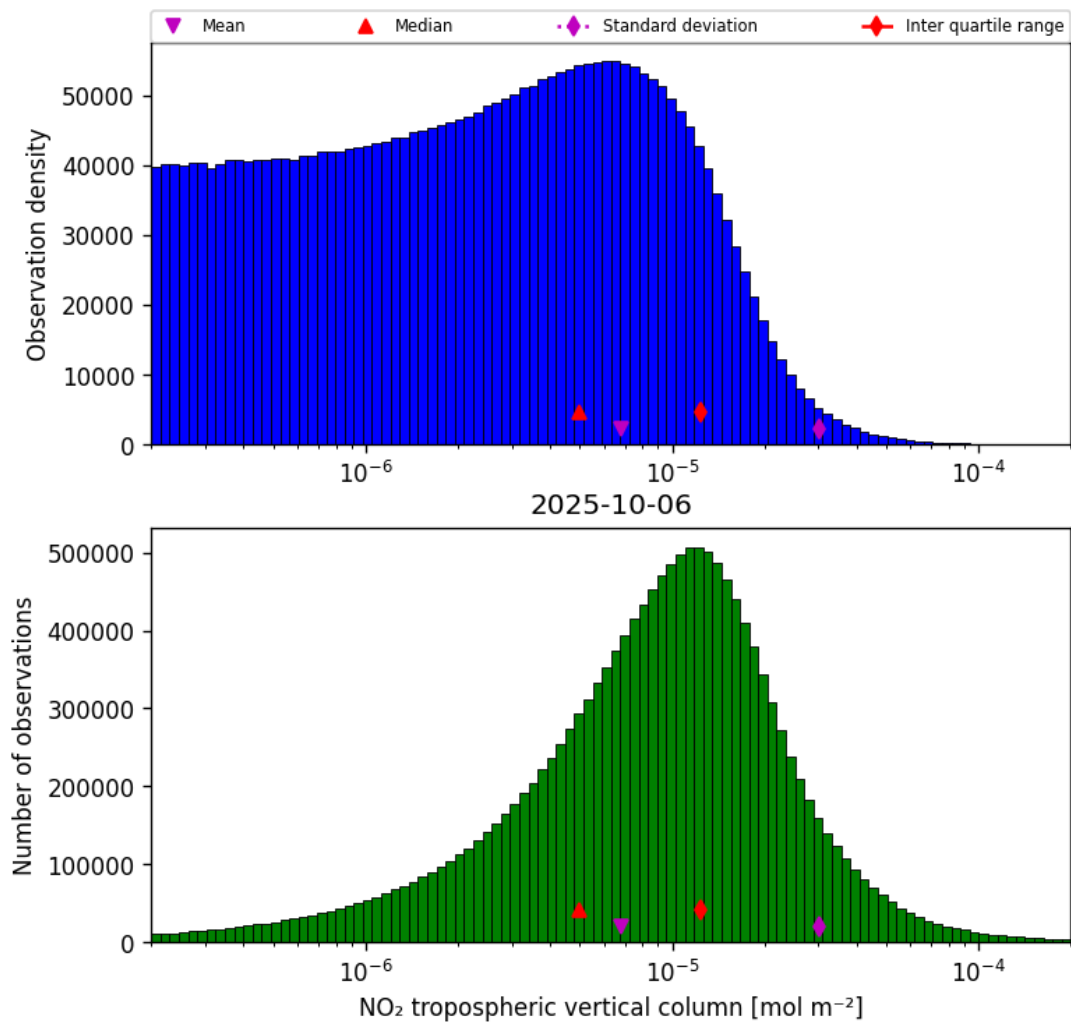
Figure 27: Histogram of “NO 2 tropospheric vertical column” for 2025-10-06 to 2025-10-07
