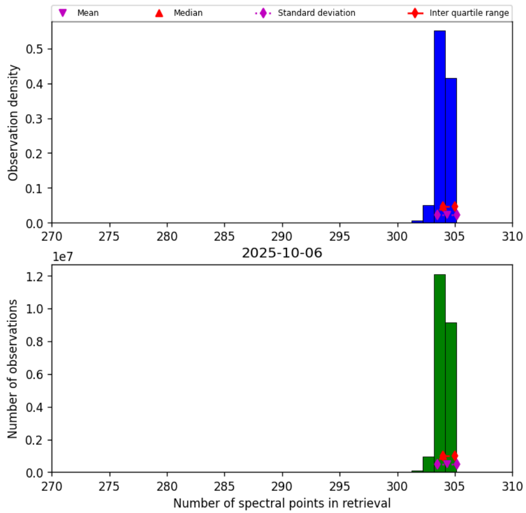
Figure 31: Histogram of “Number of spectral points in retrieval” for 2025-10-06 to 2025-10-07
