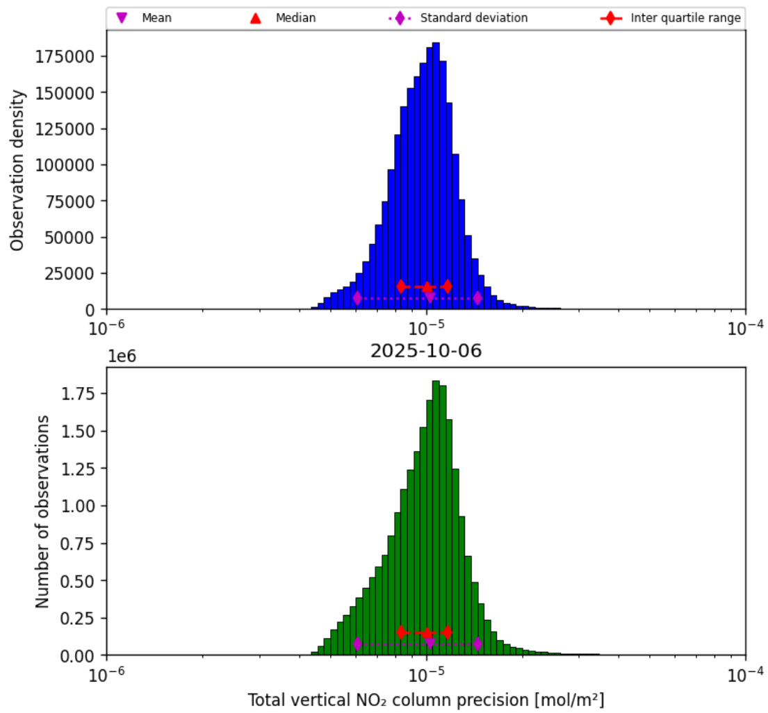
Figure 37: Histogram of “Total vertical NO 2 column precision” for 2025-10-06 to 2025-10-07
