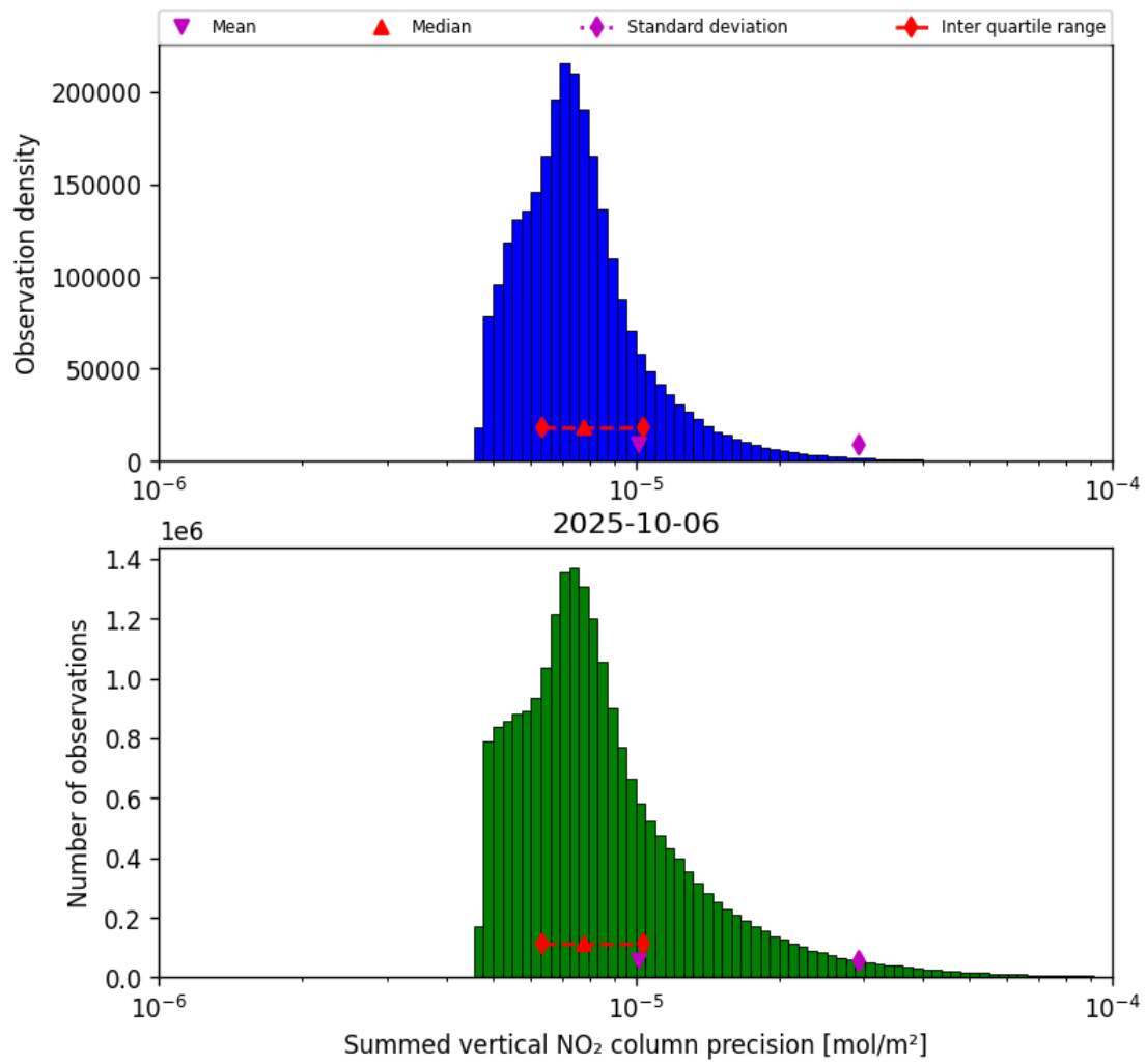
Figure 39: Histogram of "Summed vertical NO 2 column precision" for 2025-10-06 to 2025-10-07
