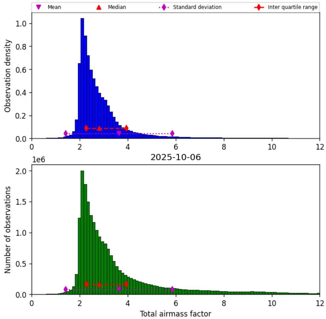
Figure 30: Histogram of “Total airmass factor” for 2025-10-06 to 2025-10-07
