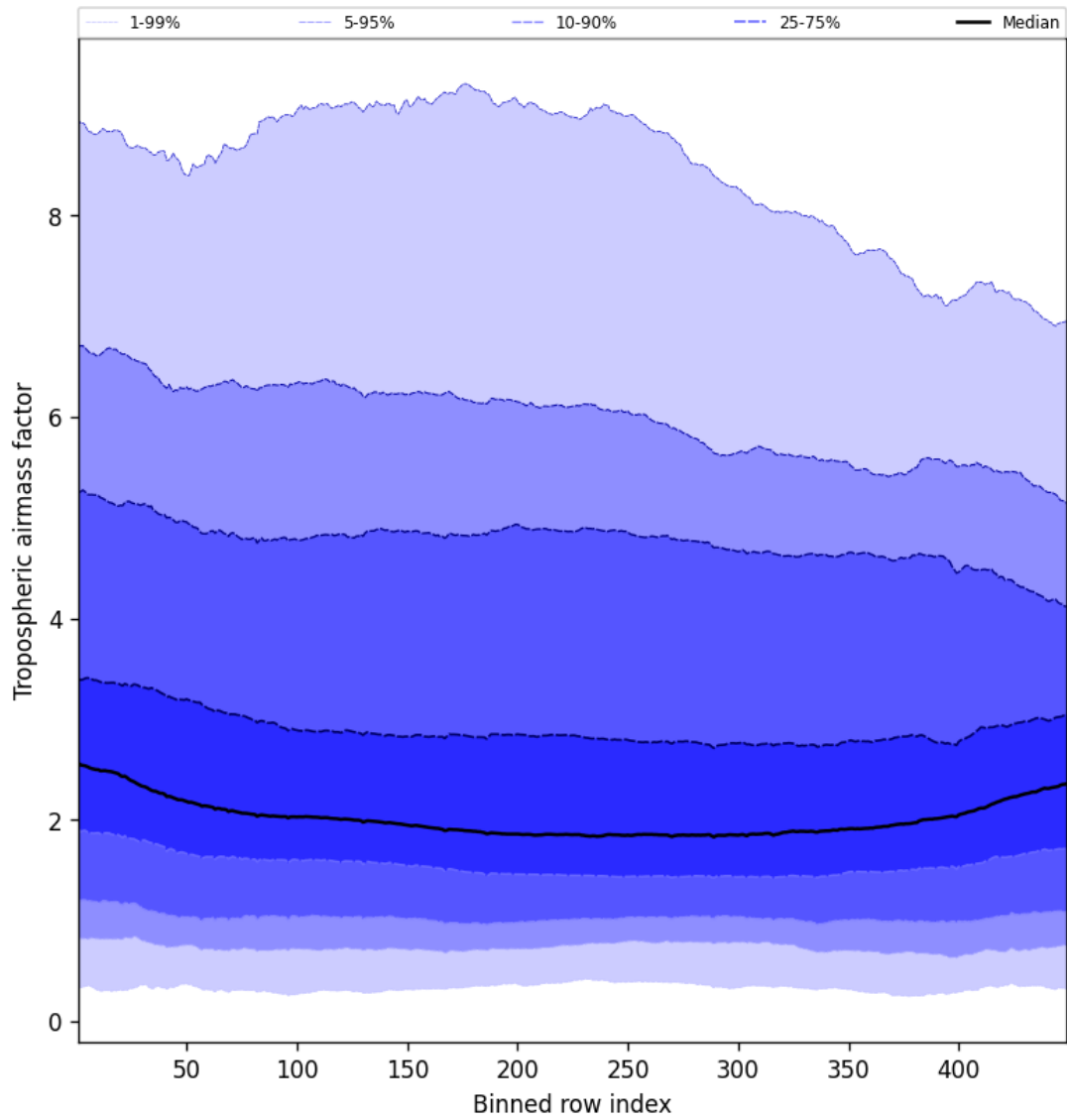
Figure 46: Along track statistics of “Tropospheric air mass factor” for 2025-10-06 to 2025-10-07
