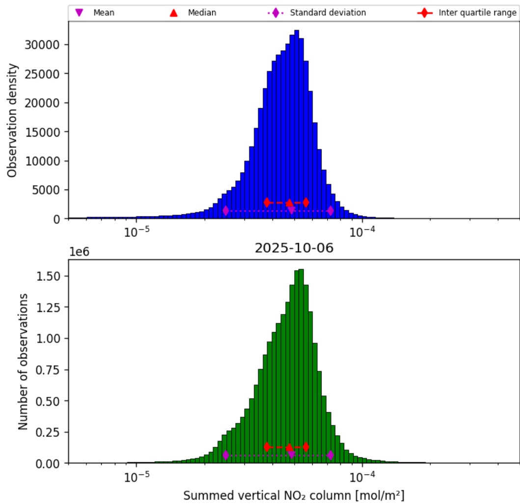
Figure 38: Histogram of “Summed vertical NO 2 column” for 2025-10-06 to 2025-10-07
