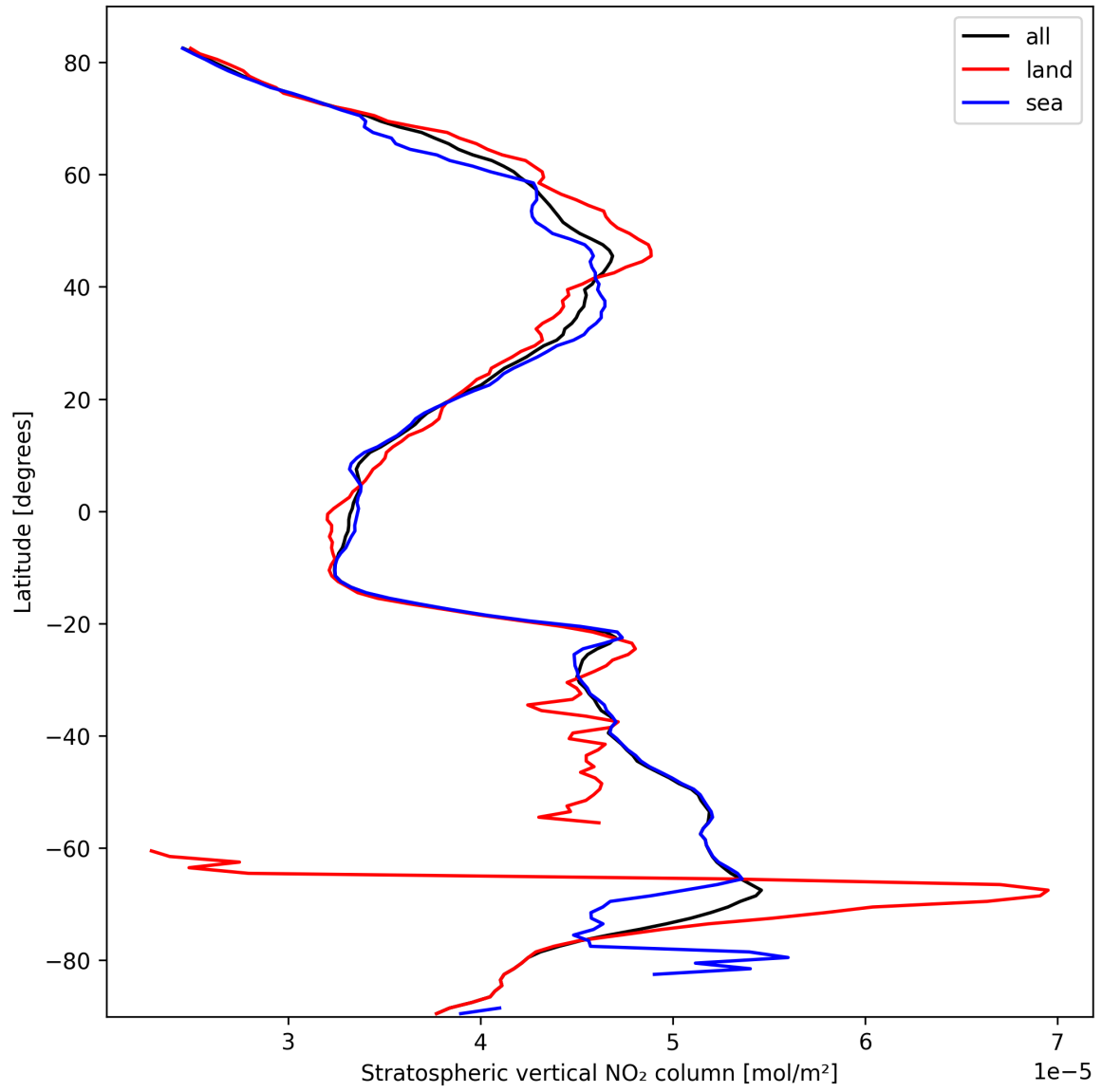
Figure 17: Zonal average of “Stratospheric vertical NO 2 column” for 2025-10-06 to 2025-10-07.
