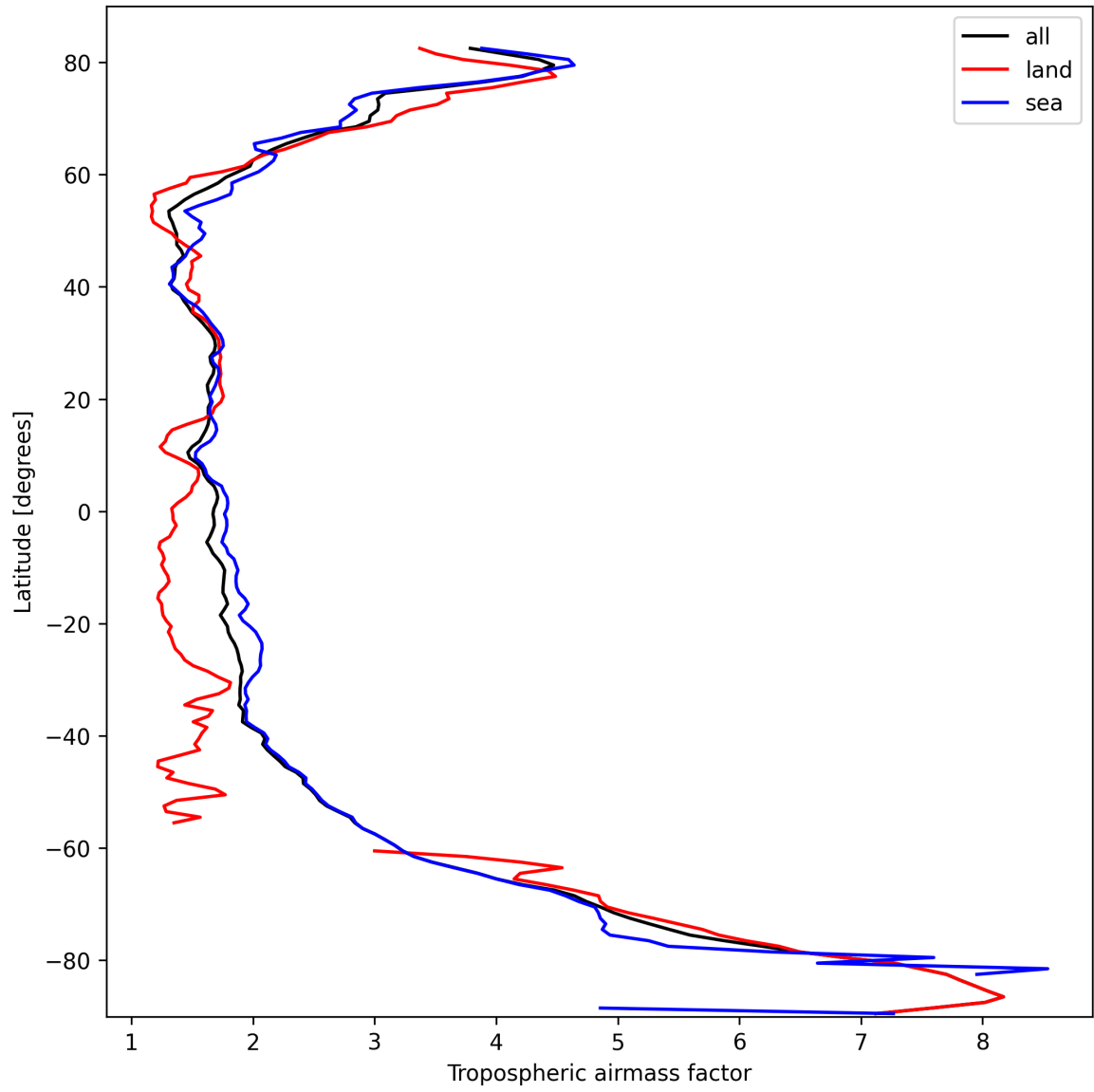
Figure 12: Zonal average of “Tropospheric airmass factor” for 2025-10-06 to 2025-10-07.
