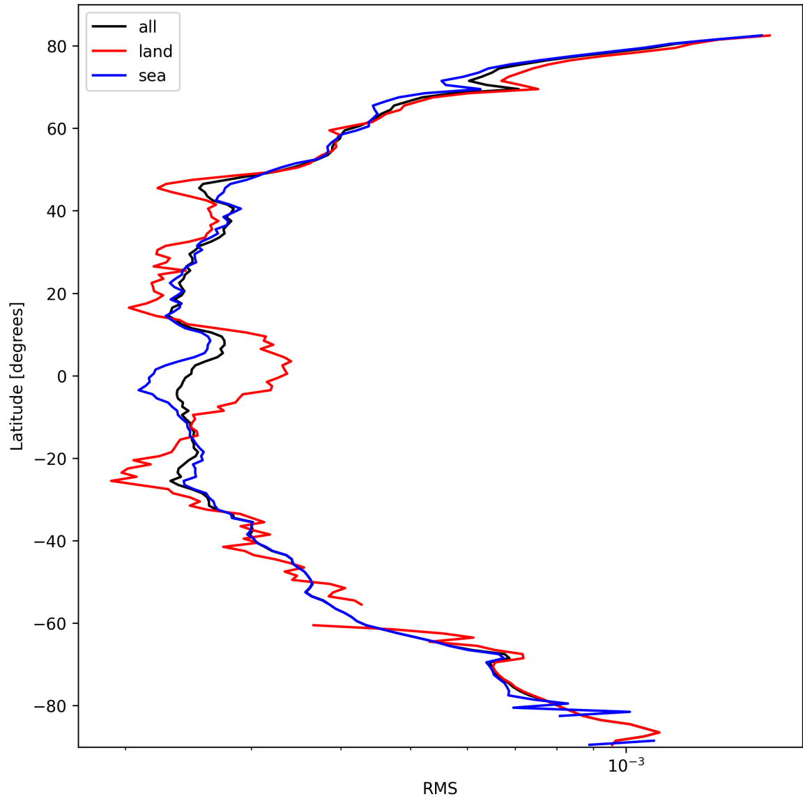
Figure 24: Zonal average of “RMS” for 2025-10-06 to 2025-10-07.
