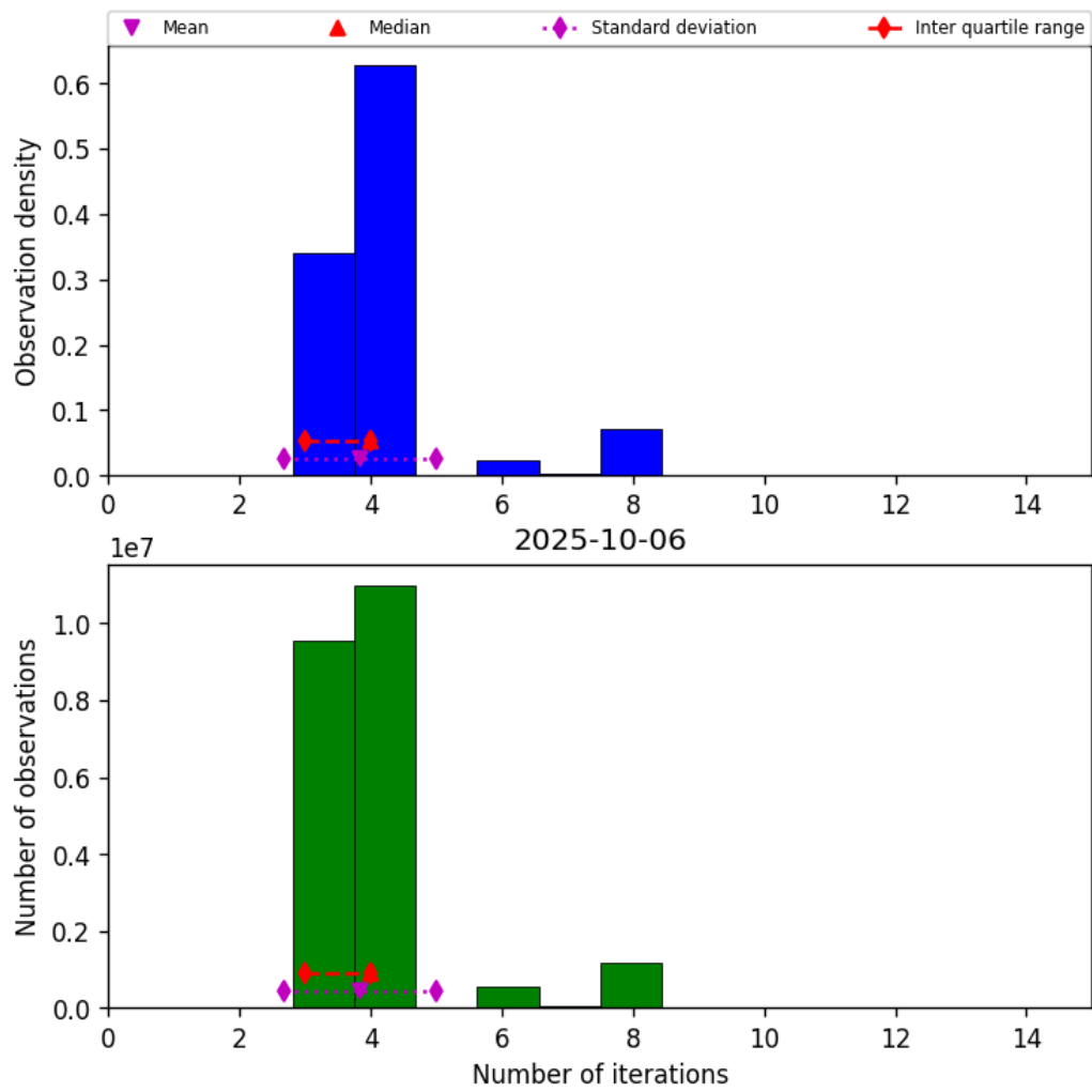
Figure 32: Histogram of “Number of iterations” for 2025-10-06 to 2025-10-07
