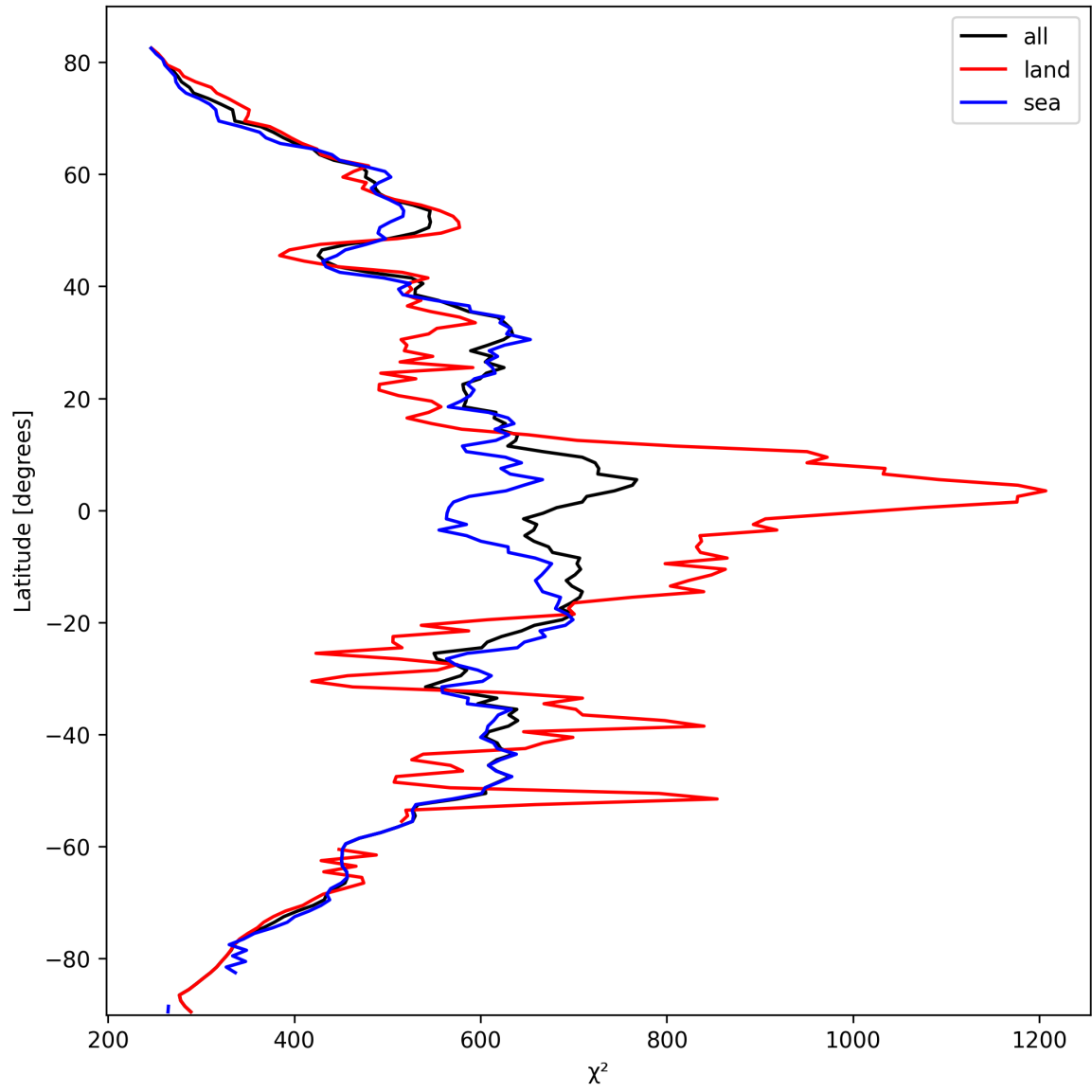
Figure 23: Zonal average of “ \chi^2 ” for 2025-10-06 to 2025-10-07.
