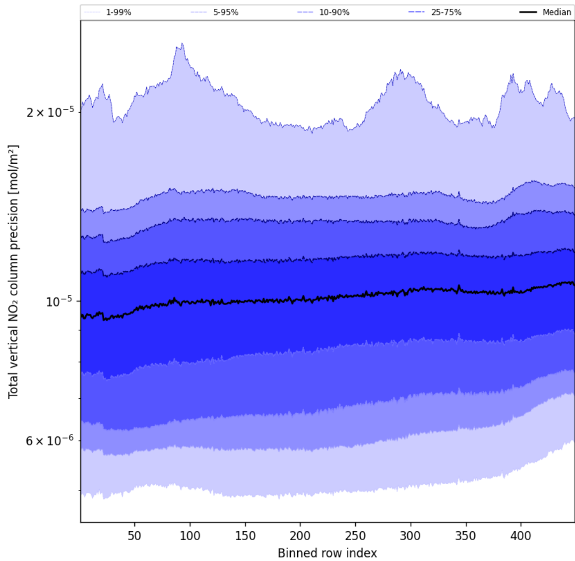
Figure 54: Along track statistics of "Total vertical NO 2 column precision" for 2025-10-06 to 2025-10-07
