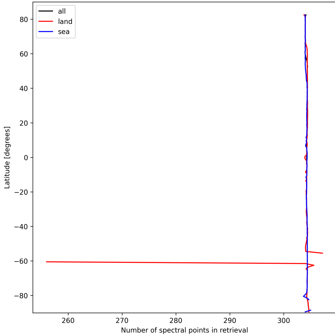
Figure 14: Zonal average of “Number of spectral points in retrieval” for 2025-10-06 to 2025-10-07.
