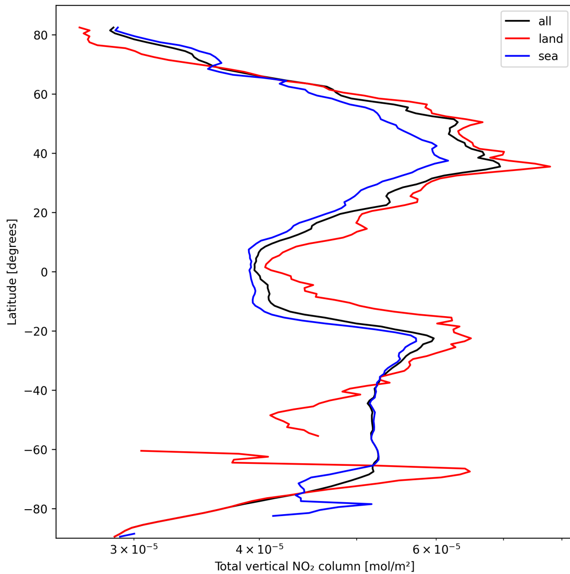
Figure 19: Zonal average of “Total vertical NO 2 column” for 2025-10-06 to 2025-10-07.
