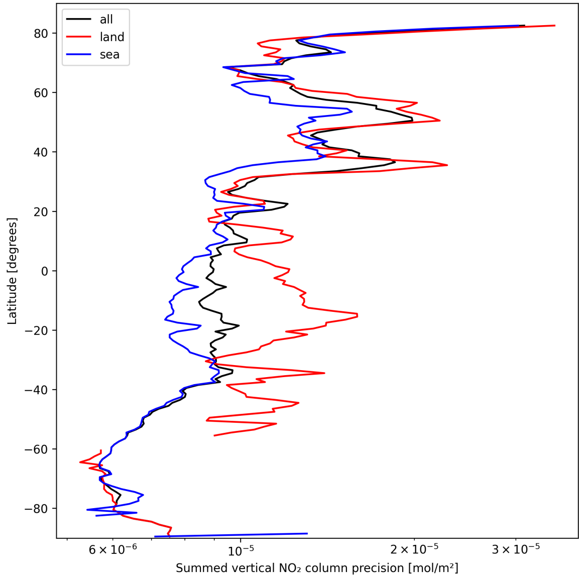
Figure 22: Zonal average of “Summed vertical NO 2 column precision” for 2025-10-06 to 2025-10-07.
