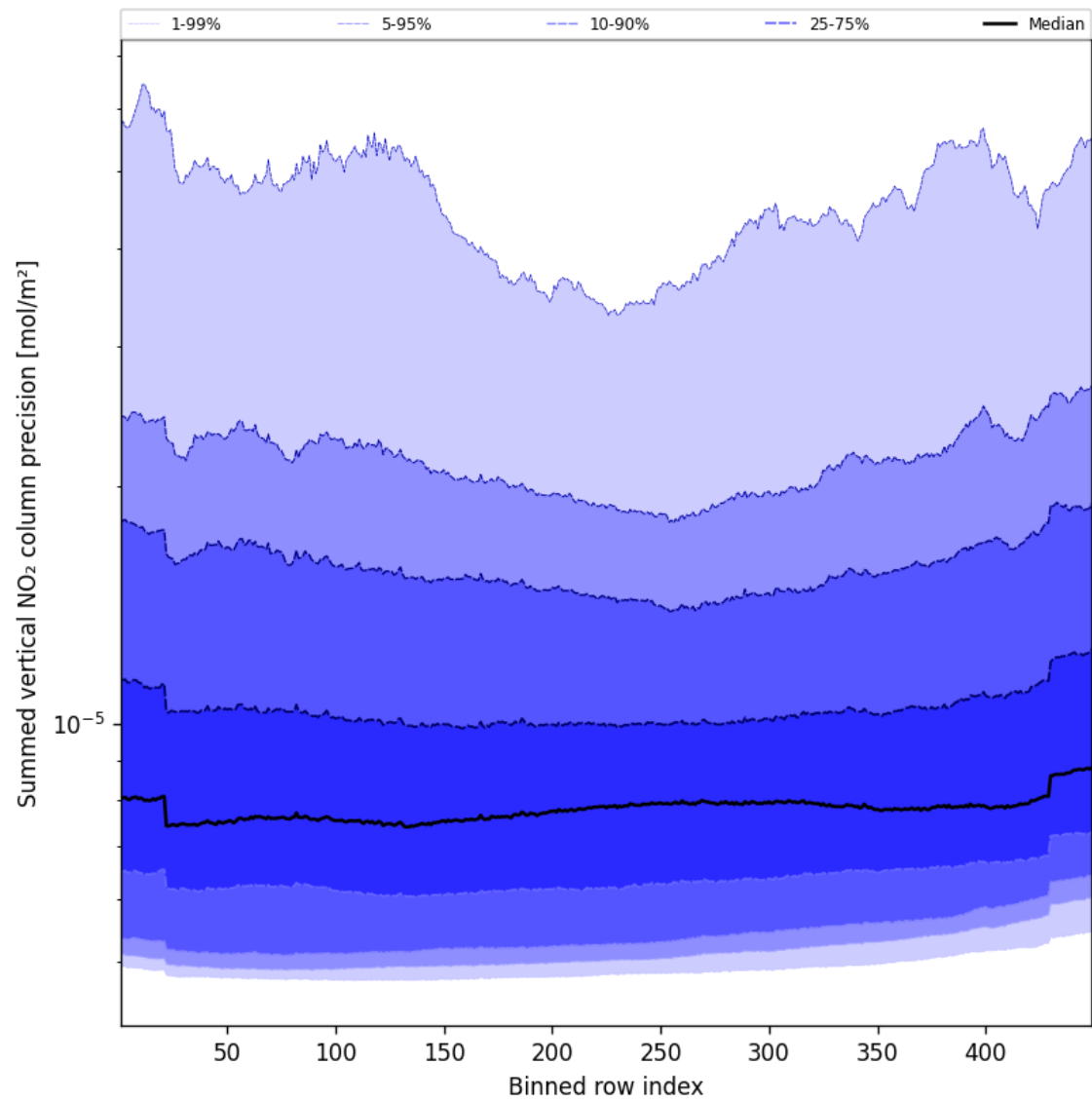
Figure 56: Along track statistics of “Summed vertical NO 2 column precision” for 2025-10-06 to 2025-10-07
