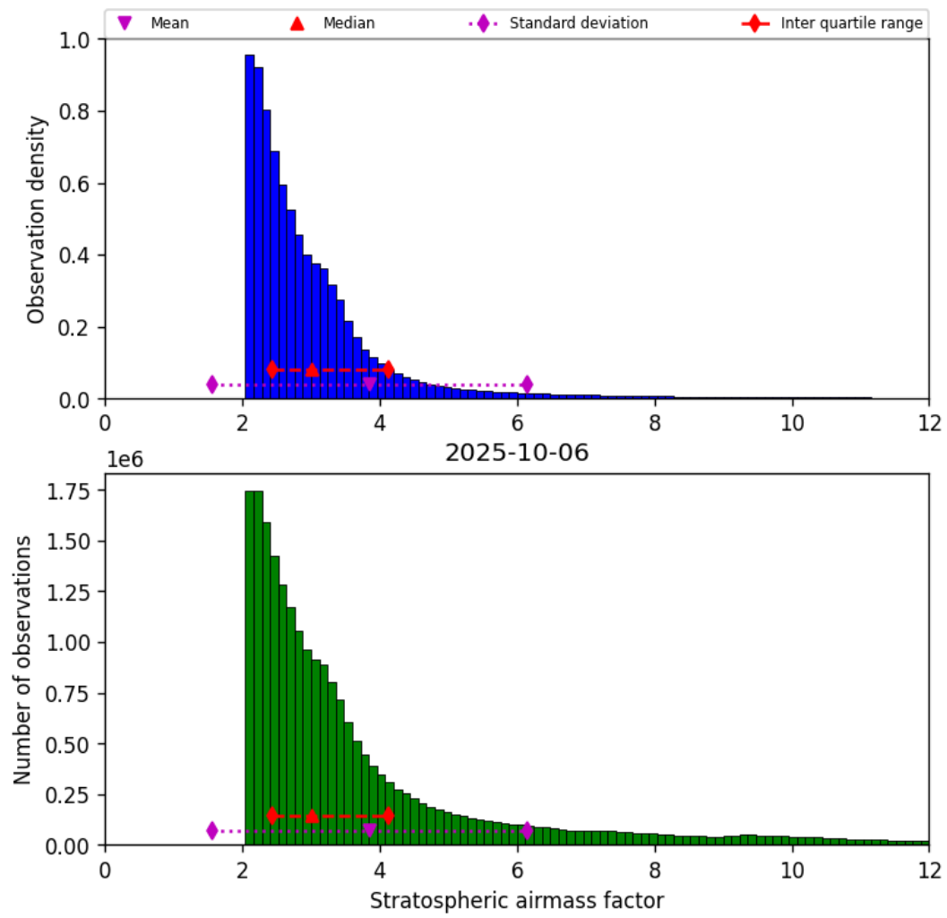
Figure 42: Histogram of “Stratospheric airmass factor” for 2025-10-06 to 2025-10-07
