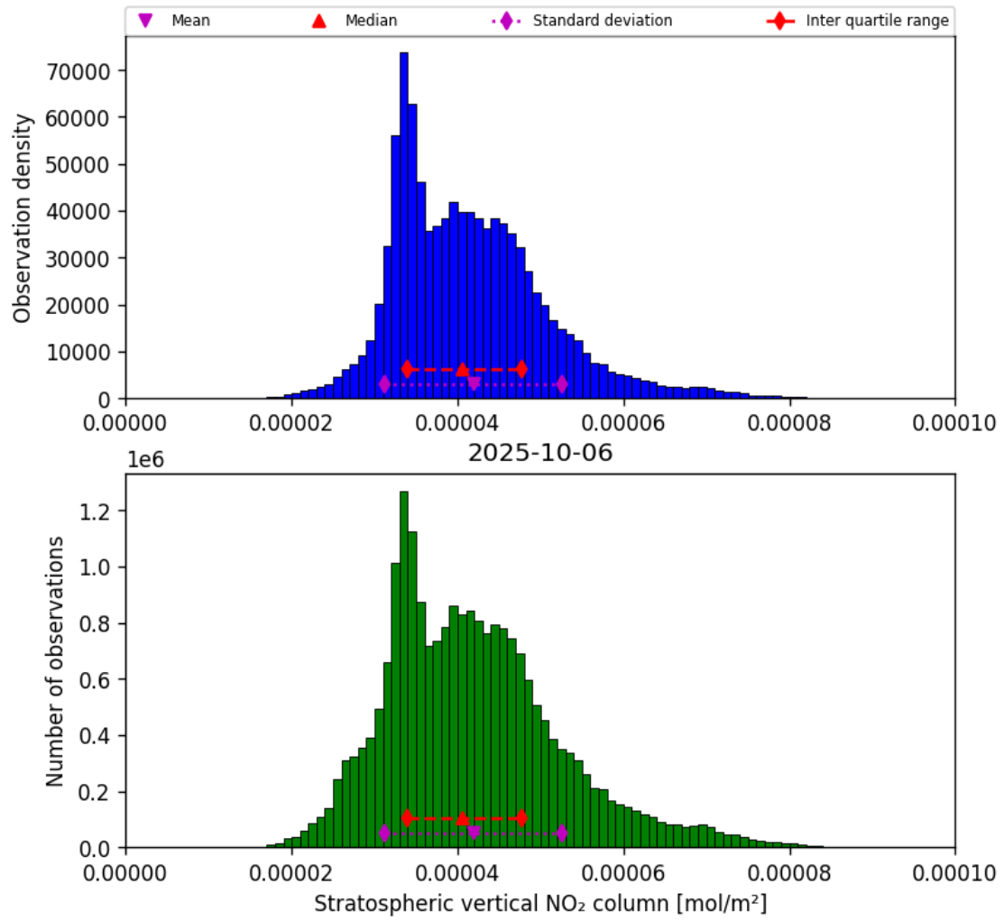
Figure 34: Histogram of “Stratospheric vertical NO 2 column” for 2025-10-06 to 2025-10-07
