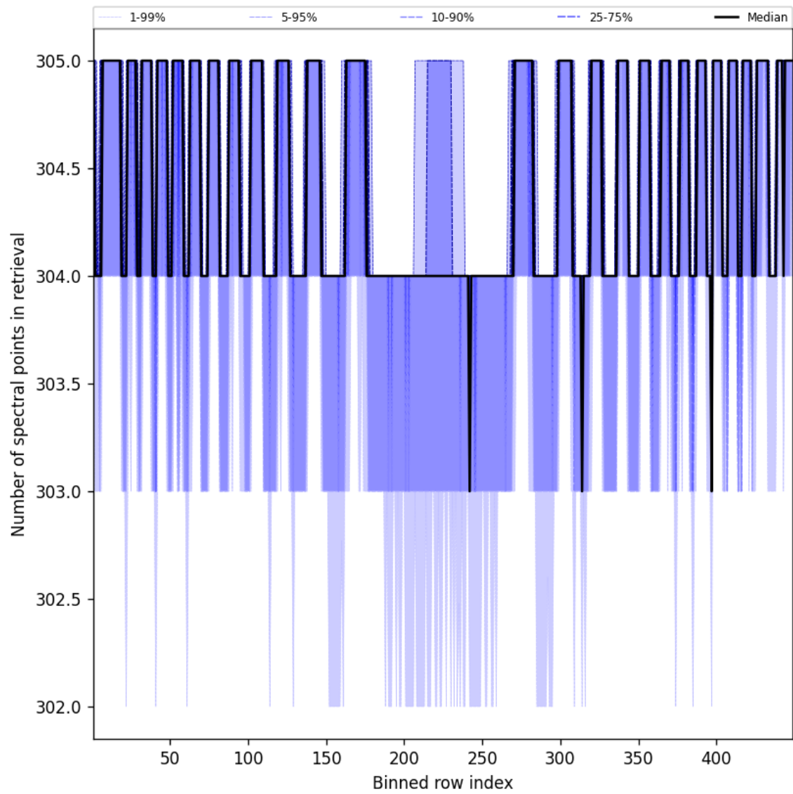
Figure 48: Along track statistics of “Number of spectral points in retrieval” for 2025-10-06 to 2025-10-07
