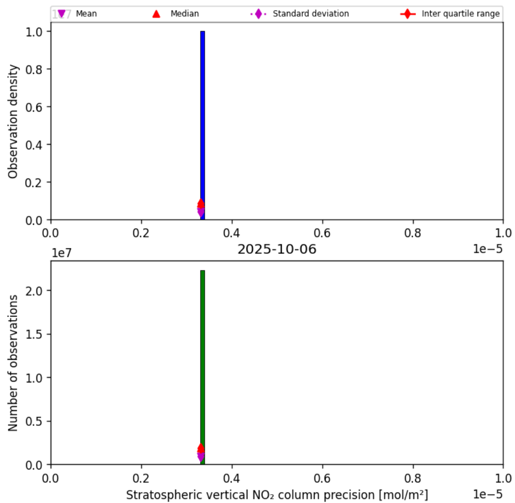
Figure 35: Histogram of “Stratospheric vertical NO 2 column precision” for 2025-10-06 to 2025-10-07
