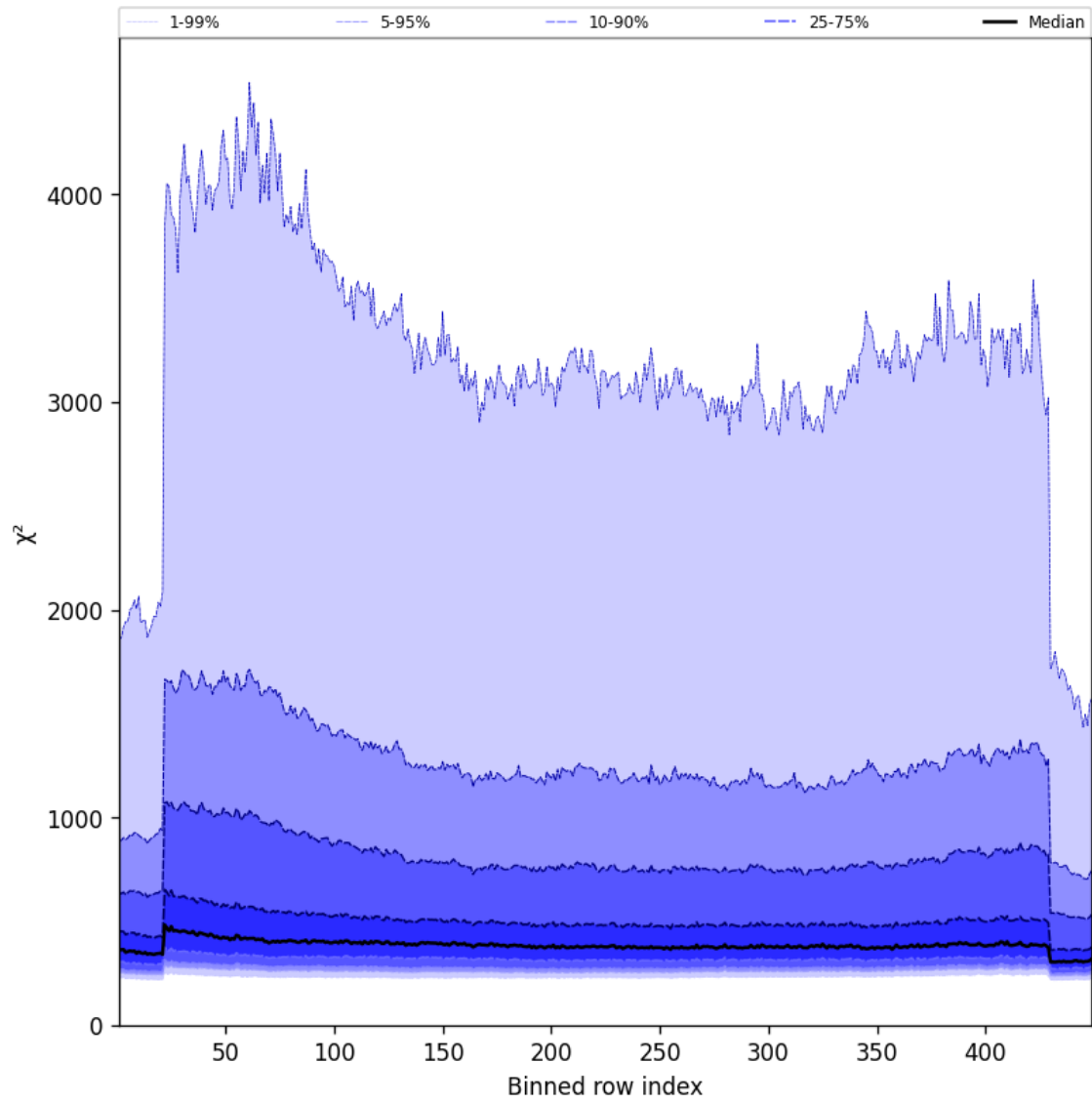
Figure 57: Along track statistics of “ \chi^2 ” for 2025-10-06 to 2025-10-07
