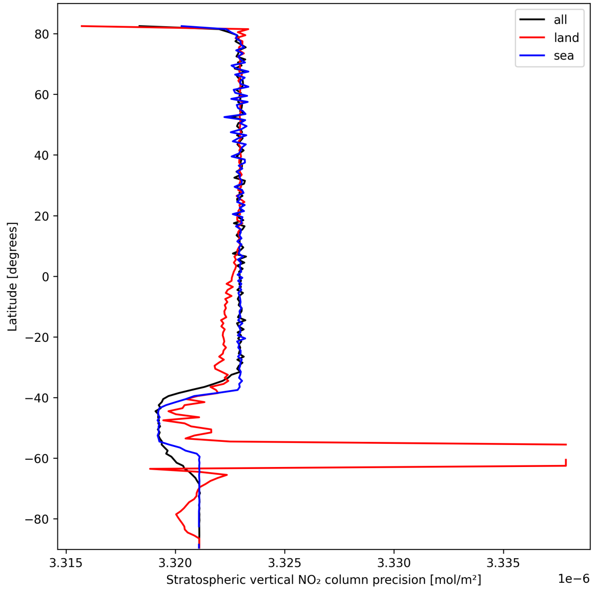
Figure 18: Zonal average of “Stratospheric vertical NO 2 column precision” for 2025-10-06 to 2025-10-07.
