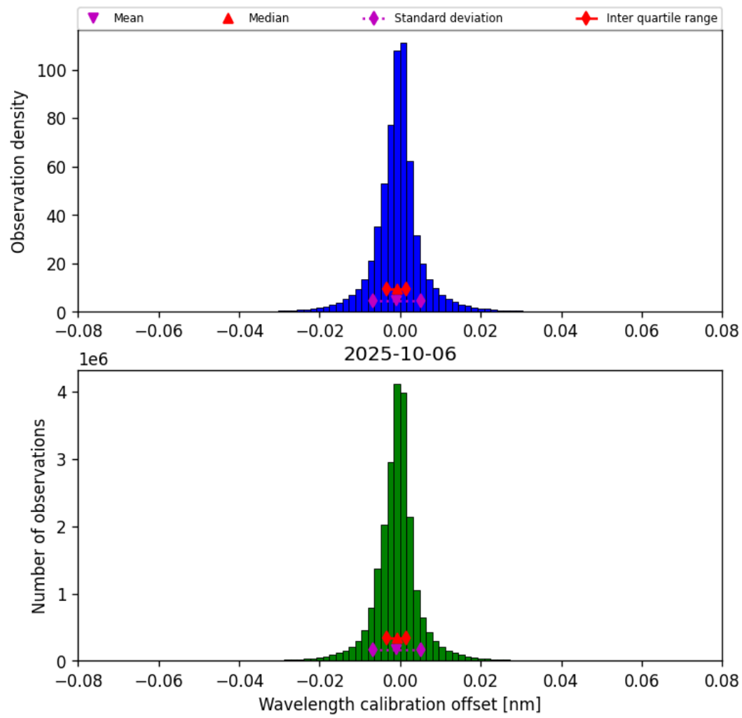
Figure 33: Histogram of “Wavelength calibration offset” for 2025-10-06 to 2025-10-07
