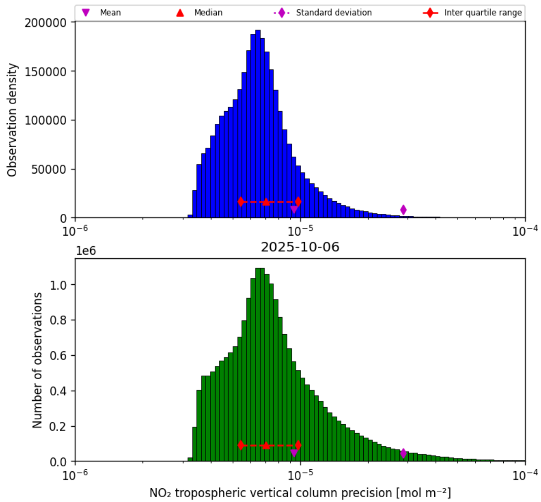
Figure 28: Histogram of “NO 2 tropospheric vertical column precision” for 2025-10-06 to 2025-10-07
