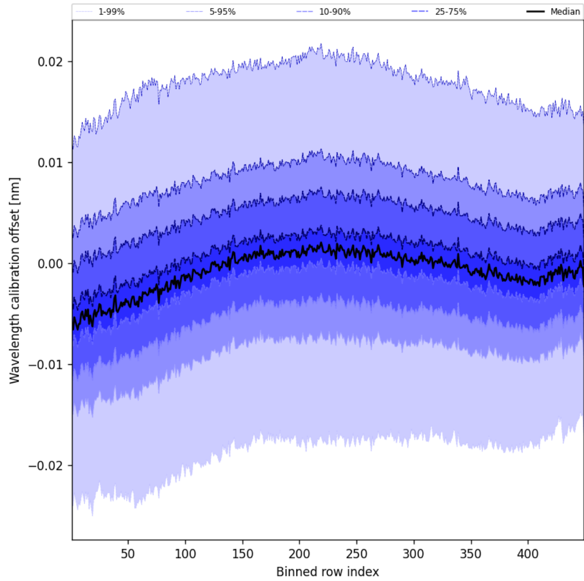
Figure 50: Along track statistics of “Wavelength calibration offset” for 2025-10-06 to 2025-10-07
