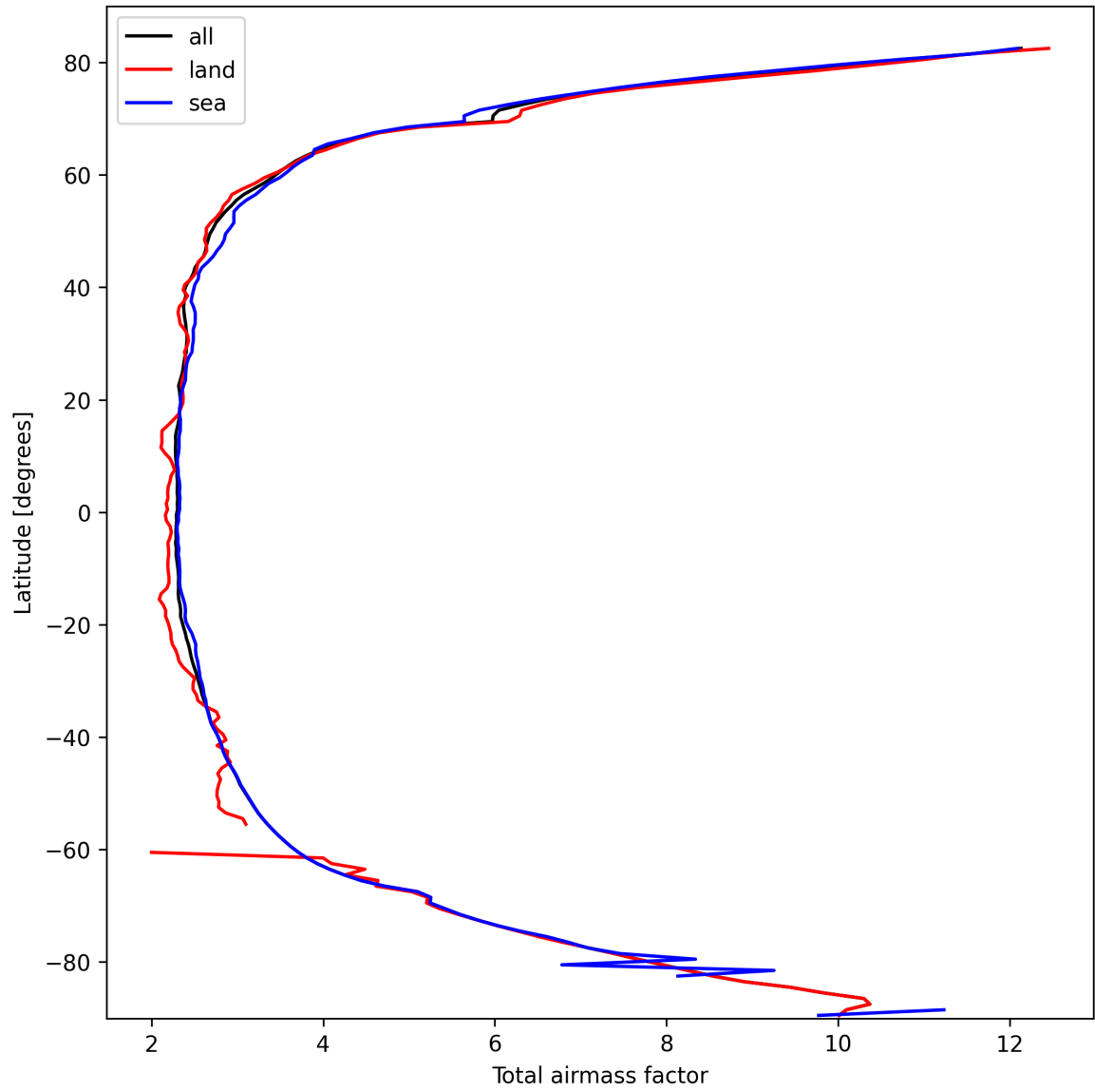
Figure 13: Zonal average of “Total airmass factor” for 2025-10-06 to 2025-10-07.
