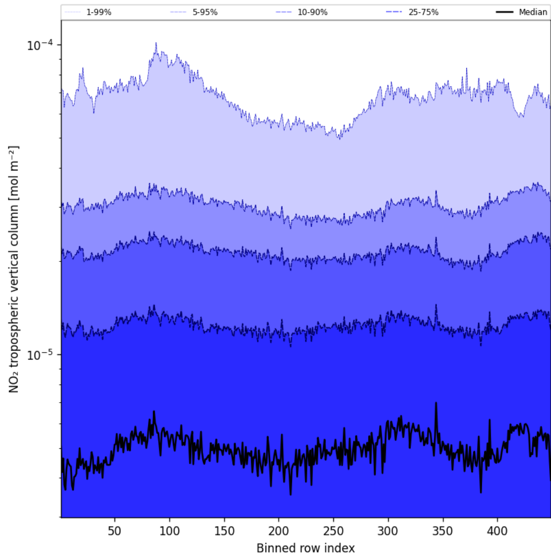
Figure 44: Along track statistics of “NO 2 tropospheric vertical column” for 2025-10-06 to 2025-10-07
