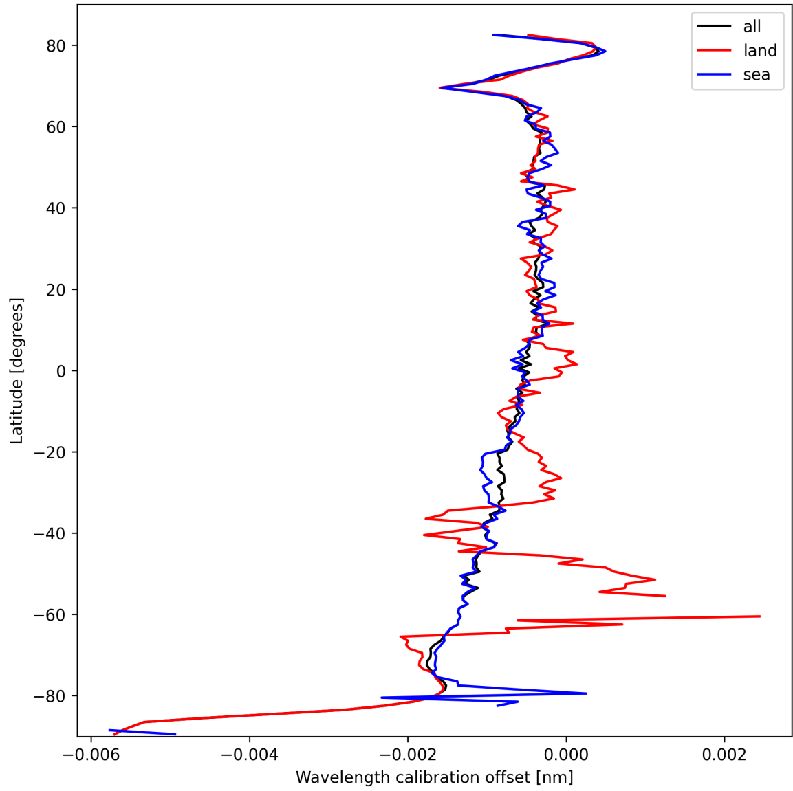
Figure 16: Zonal average of “Wavelength calibration offset” for 2025-10-06 to 2025-10-07.
