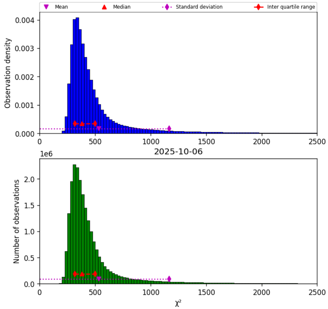
Figure 40: Histogram of “ \chi^2 ” for 2025-10-06 to 2025-10-07
