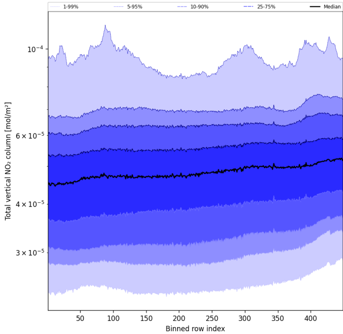
Figure 53: Along track statistics of “Total vertical NO 2 column” for 2025-10-06 to 2025-10-07
