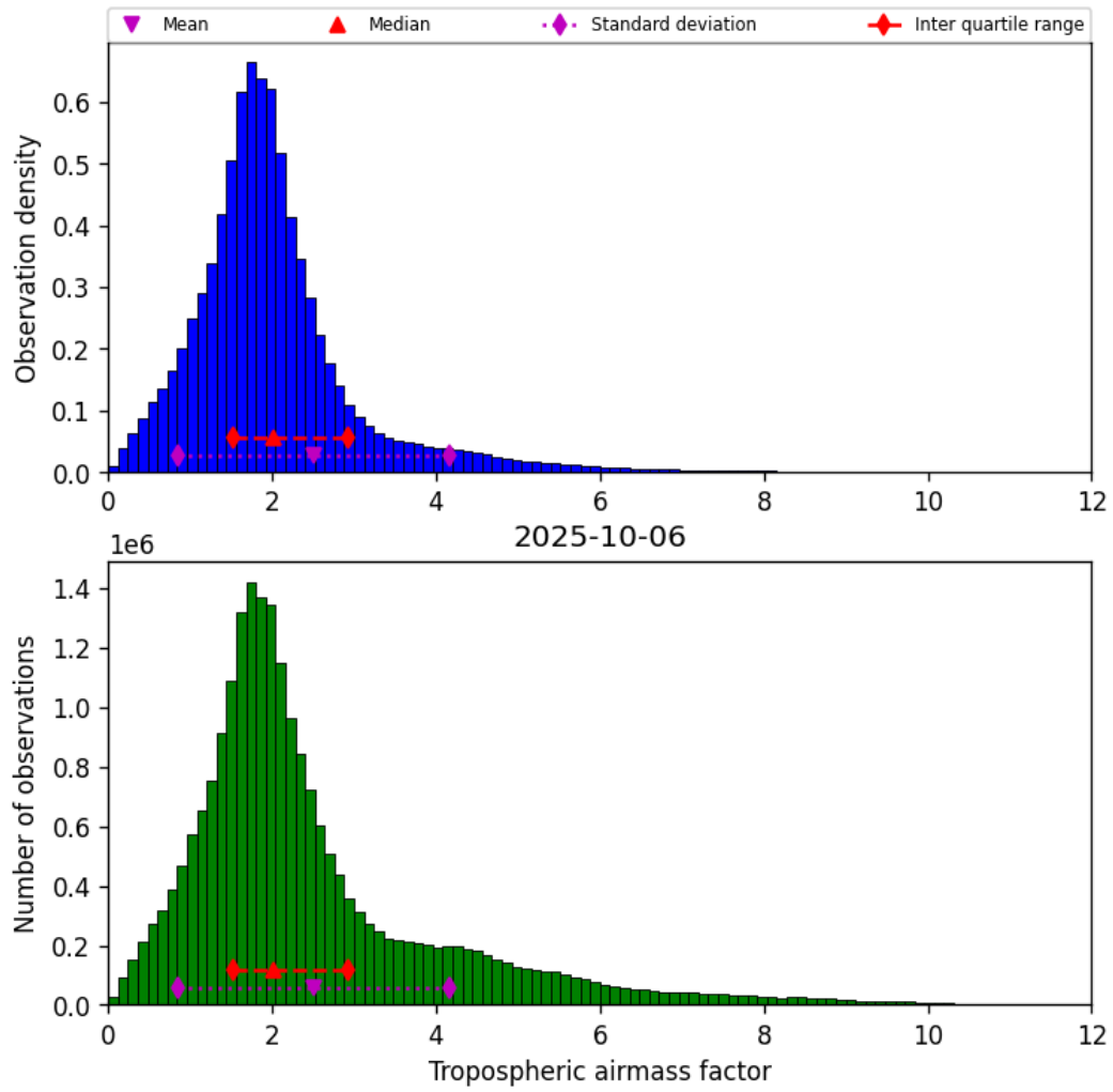
Figure 29: Histogram of “Tropospheric airmass factor” for 2025-10-06 to 2025-10-07
