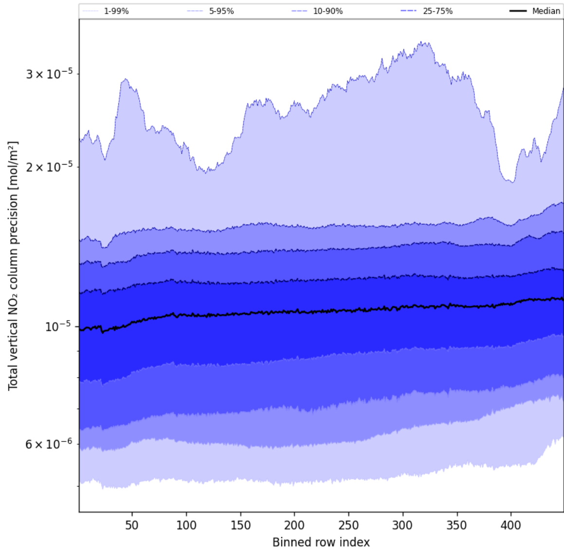
Figure 54: Along track statistics of “Total vertical NO 2 column precision” for 2025-10-07 to 2025-10-07
