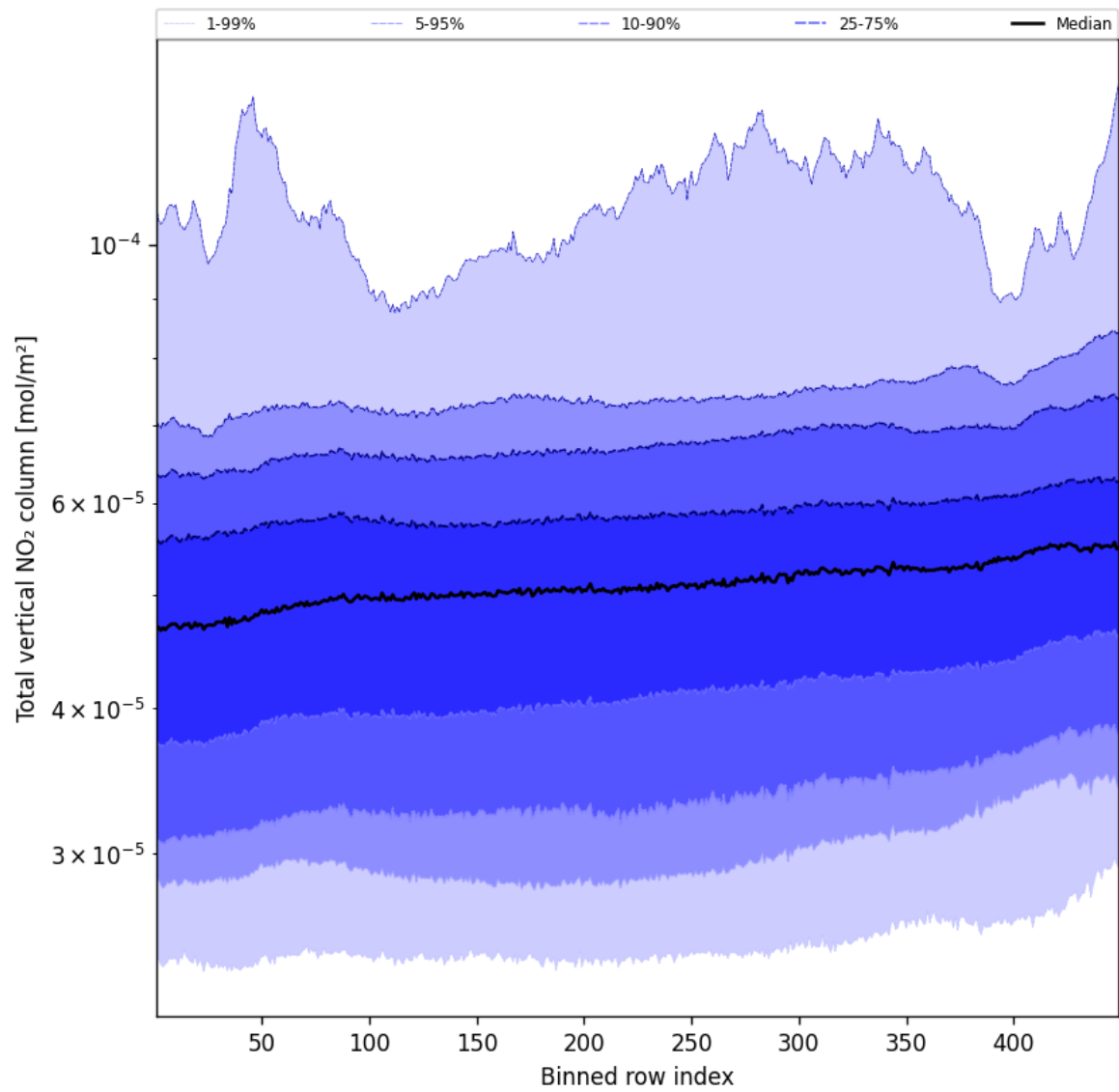
Figure 53: Along track statistics of “Total vertical NO 2 column” for 2025-10-07 to 2025-10-07
