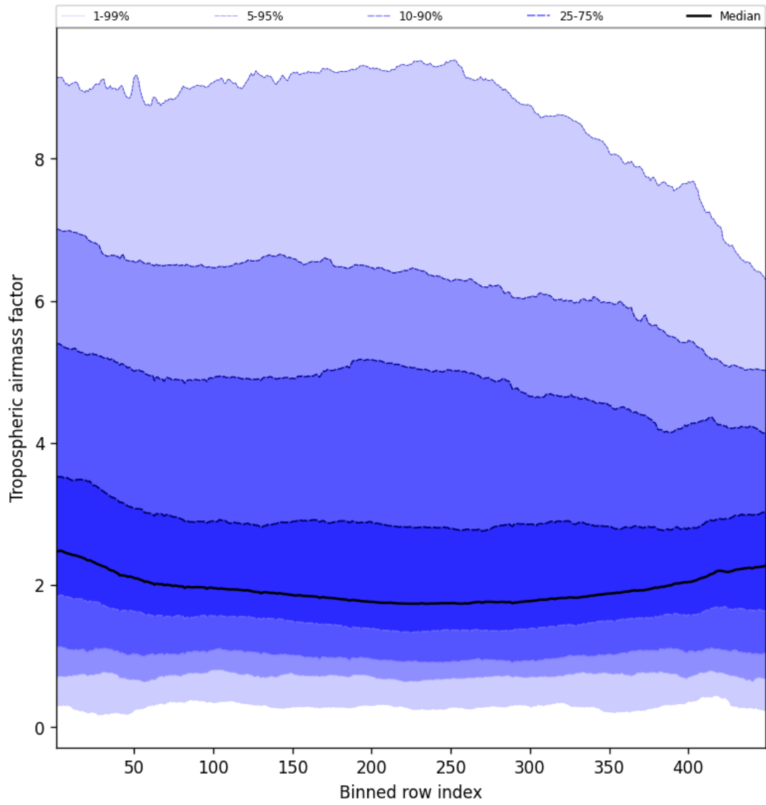
Figure 46: Along track statistics of “Tropospheric air mass factor” for 2025-10-07 to 2025-10-07
