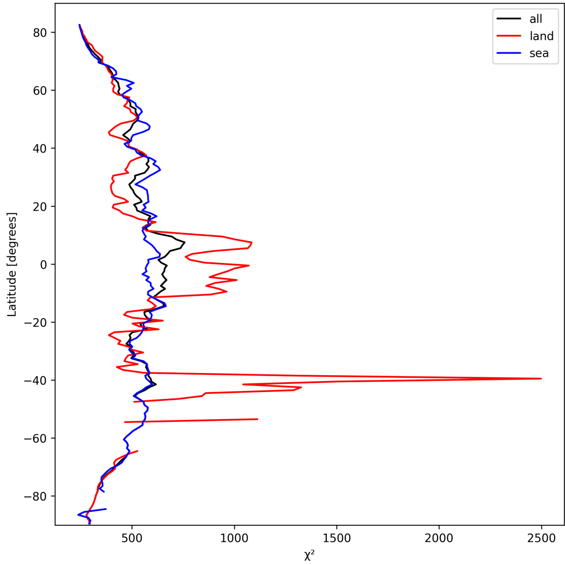
Figure 23: Zonal average of “ \chi^2 ” for 2025-10-07 to 2025-10-07.
