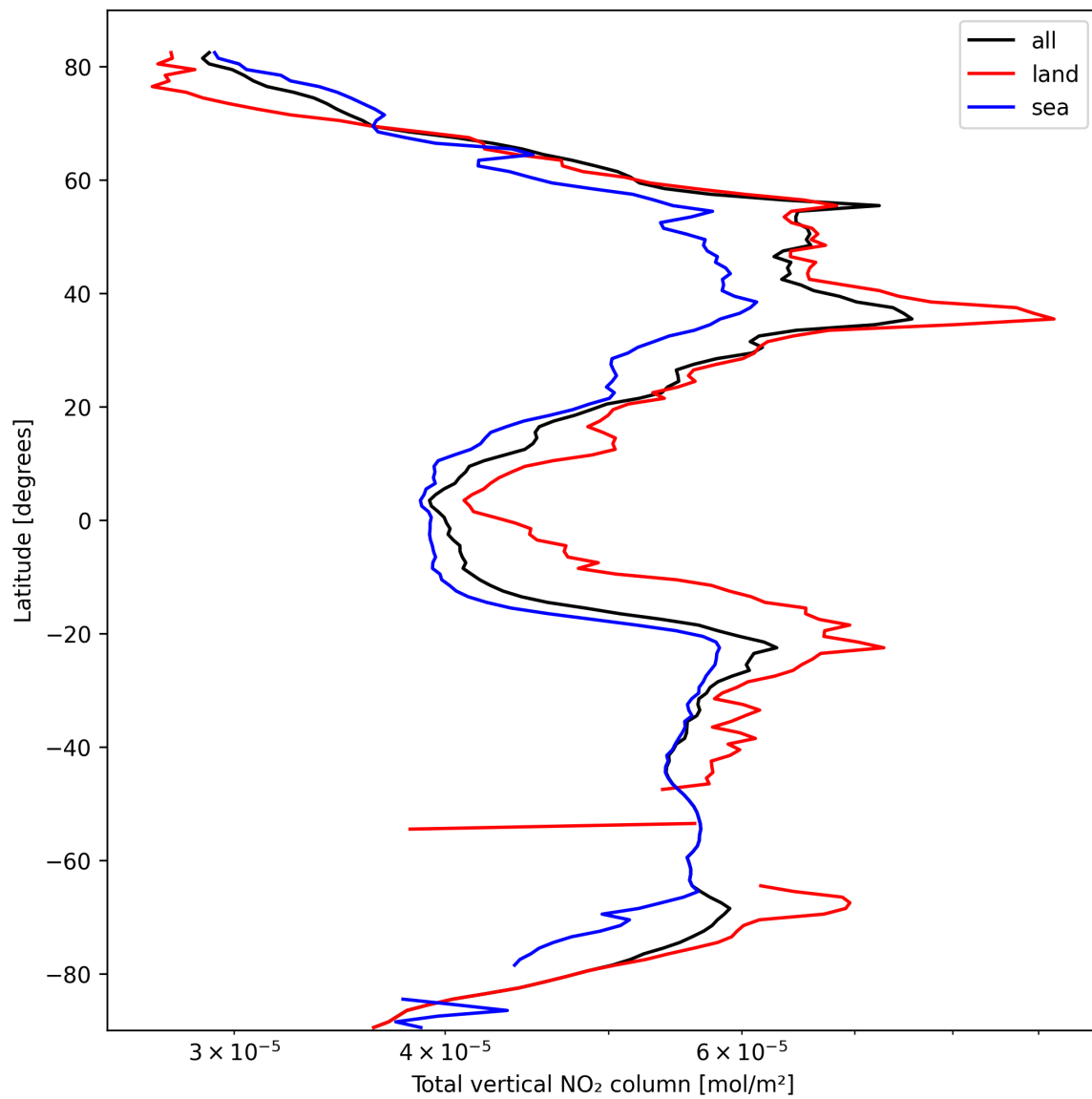
Figure 19: Zonal average of “Total vertical NO 2 column” for 2025-10-07 to 2025-10-07.
