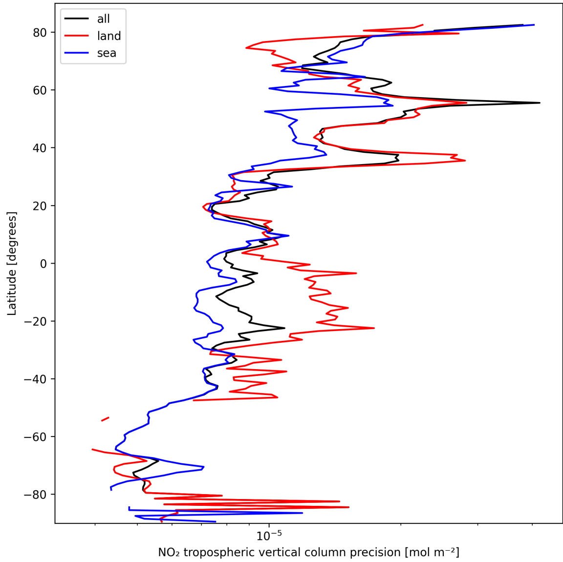
Figure 11: Zonal average of “NO 2 tropospheric vertical column precision” for 2025-10-07 to 2025-10-07.
