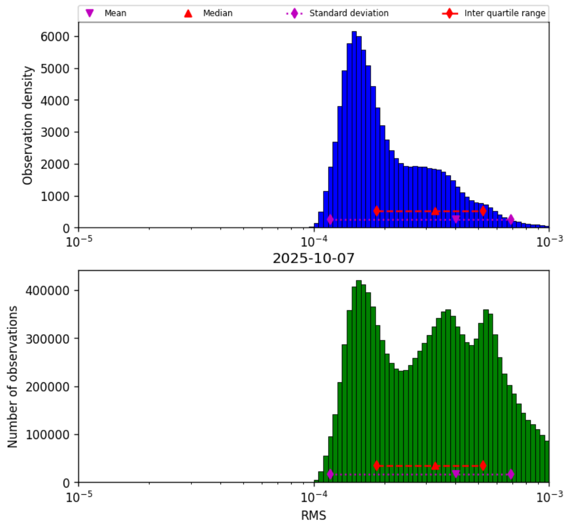
Figure 41: Histogram of “RMS” for 2025-10-07 to 2025-10-07
