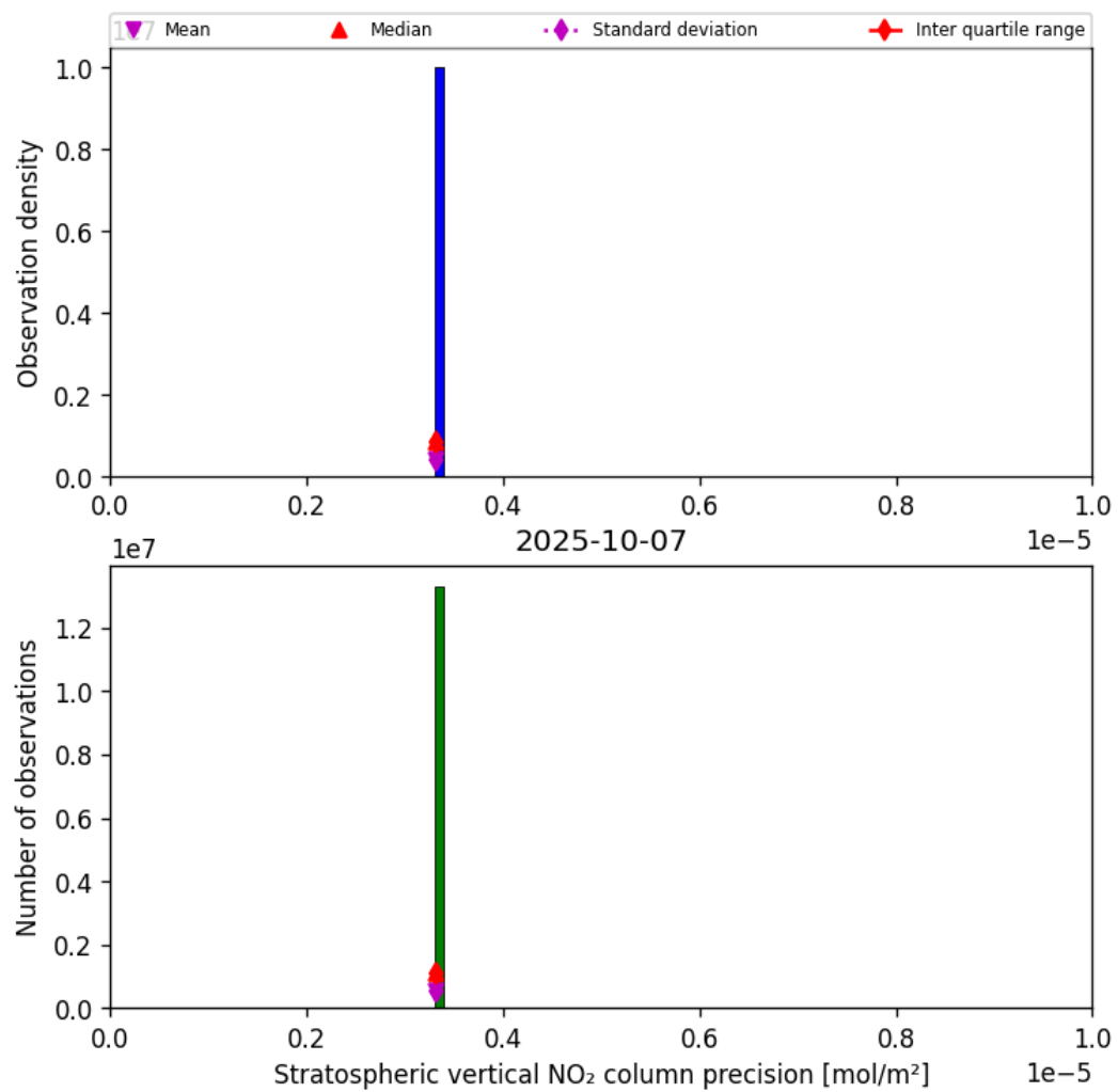
Figure 35: Histogram of “Stratospheric vertical NO 2 column precision” for 2025-10-07 to 2025-10-07
