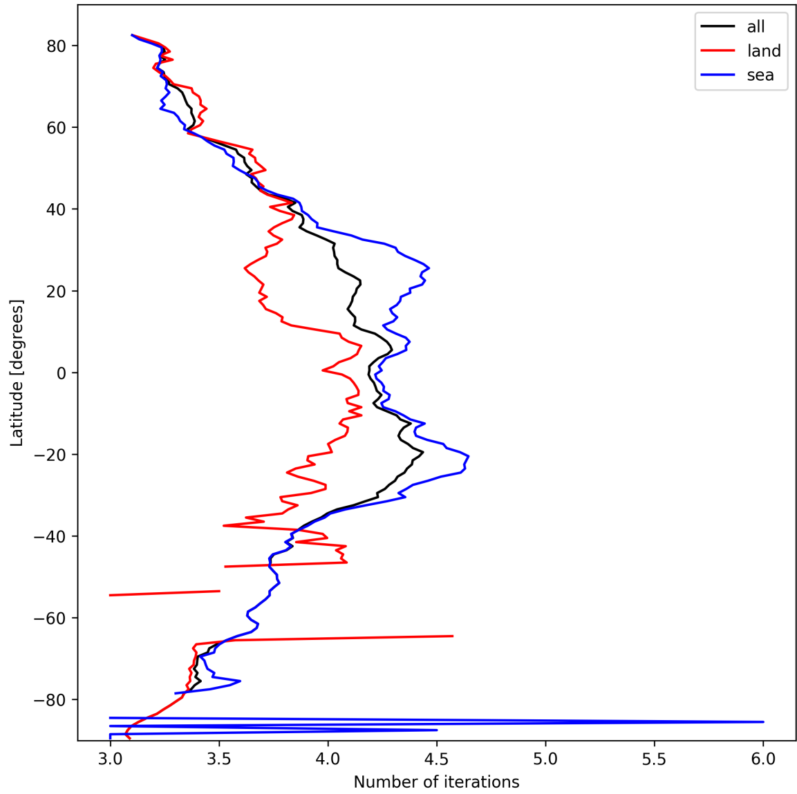
Figure 15: Zonal average of “Number of iterations” for 2025-10-07 to 2025-10-07.
