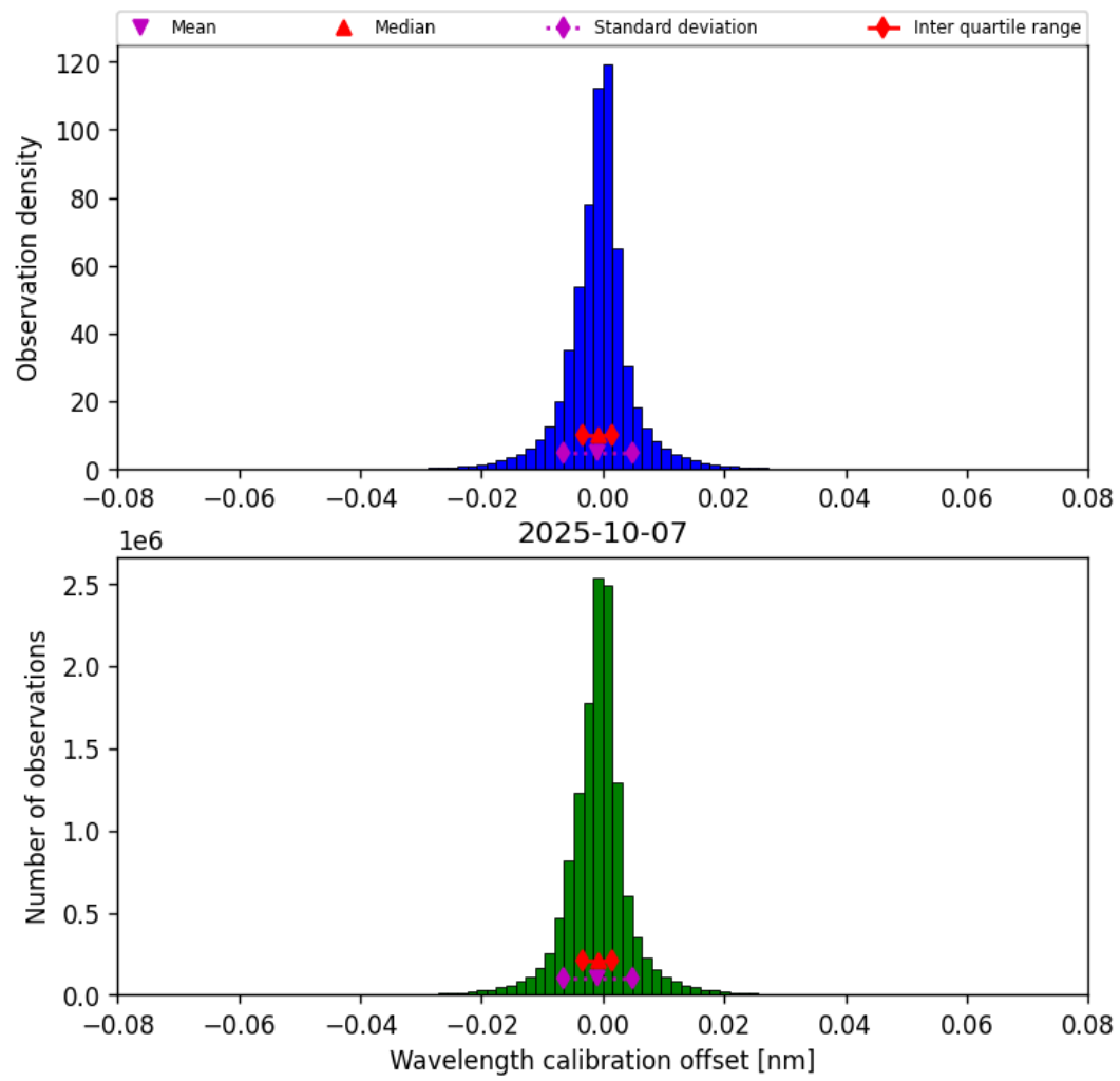
Figure 33: Histogram of “Wavelength calibration offset” for 2025-10-07 to 2025-10-07
