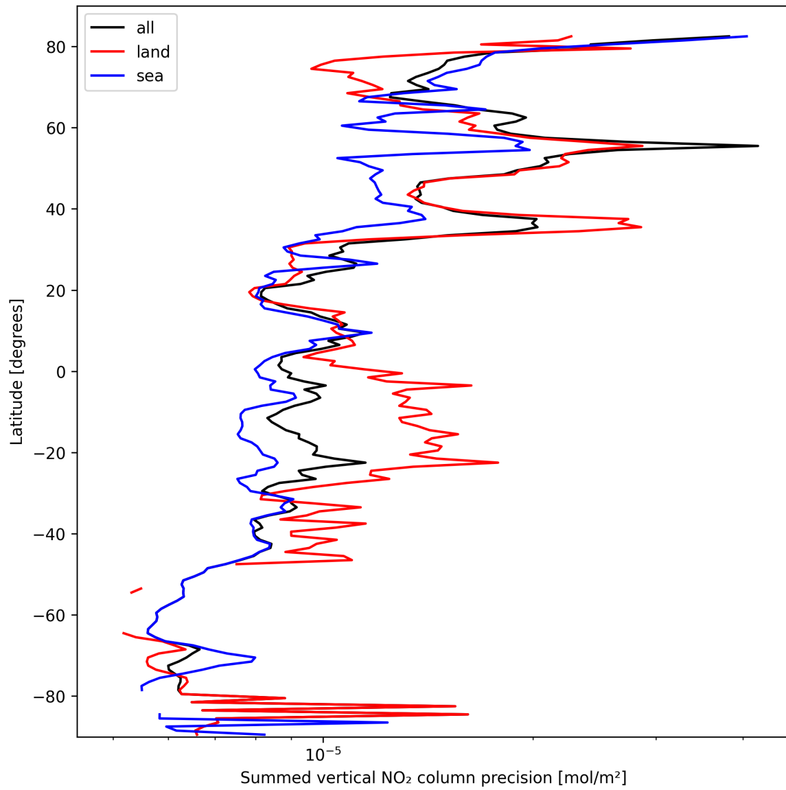
Figure 22: Zonal average of “Summed vertical NO 2 column precision” for 2025-10-07 to 2025-10-07.
