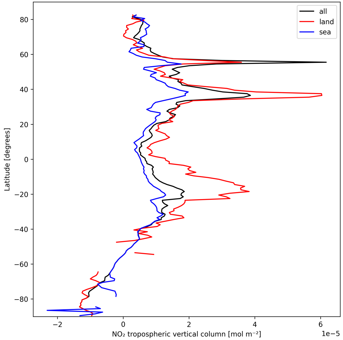
Figure 10: Zonal average of “NO 2 tropospheric vertical column” for 2025-10-07 to 2025-10-07.
