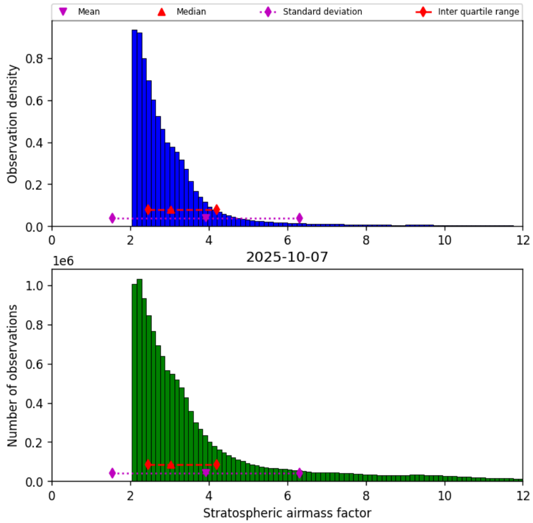
Figure 42: Histogram of “Stratospheric airmass factor” for 2025-10-07 to 2025-10-07
