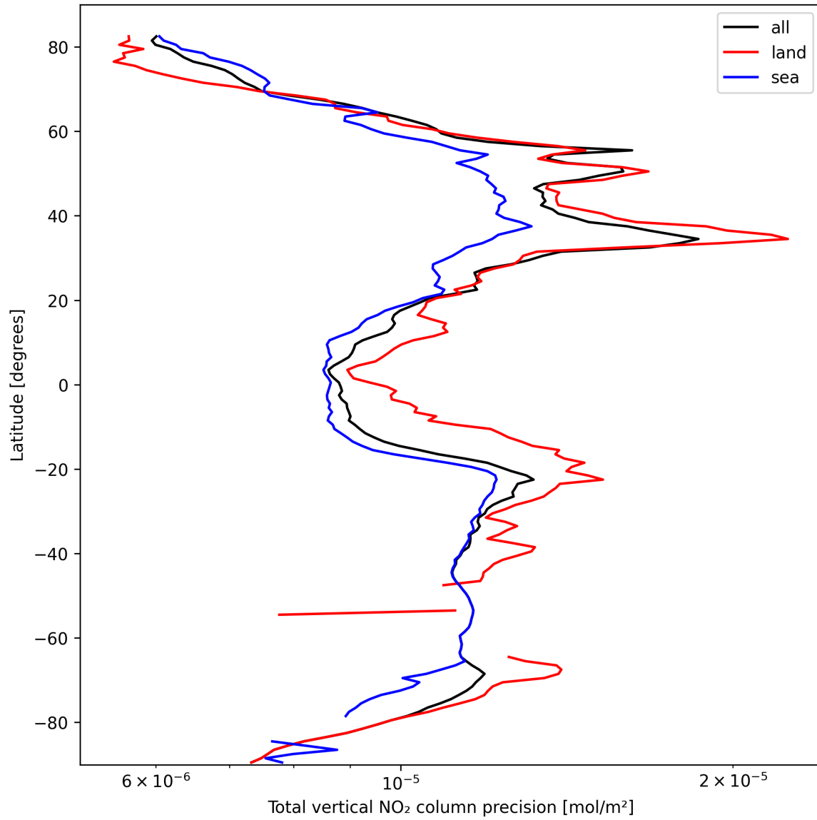
Figure 20: Zonal average of “Total vertical NO 2 column precision” for 2025-10-07 to 2025-10-07.
