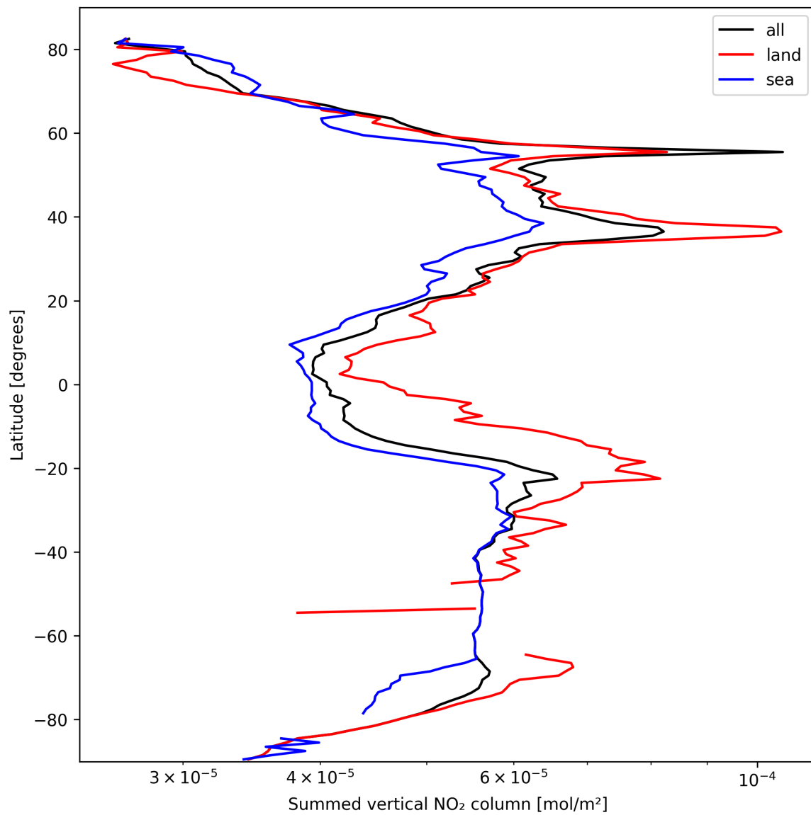
Figure 21: Zonal average of “Summed vertical NO 2 column” for 2025-10-07 to 2025-10-07.
