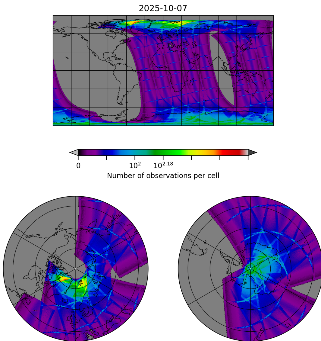
Figure 8: Map of the number of observations for 2025-10-07 to 2025-10-07
