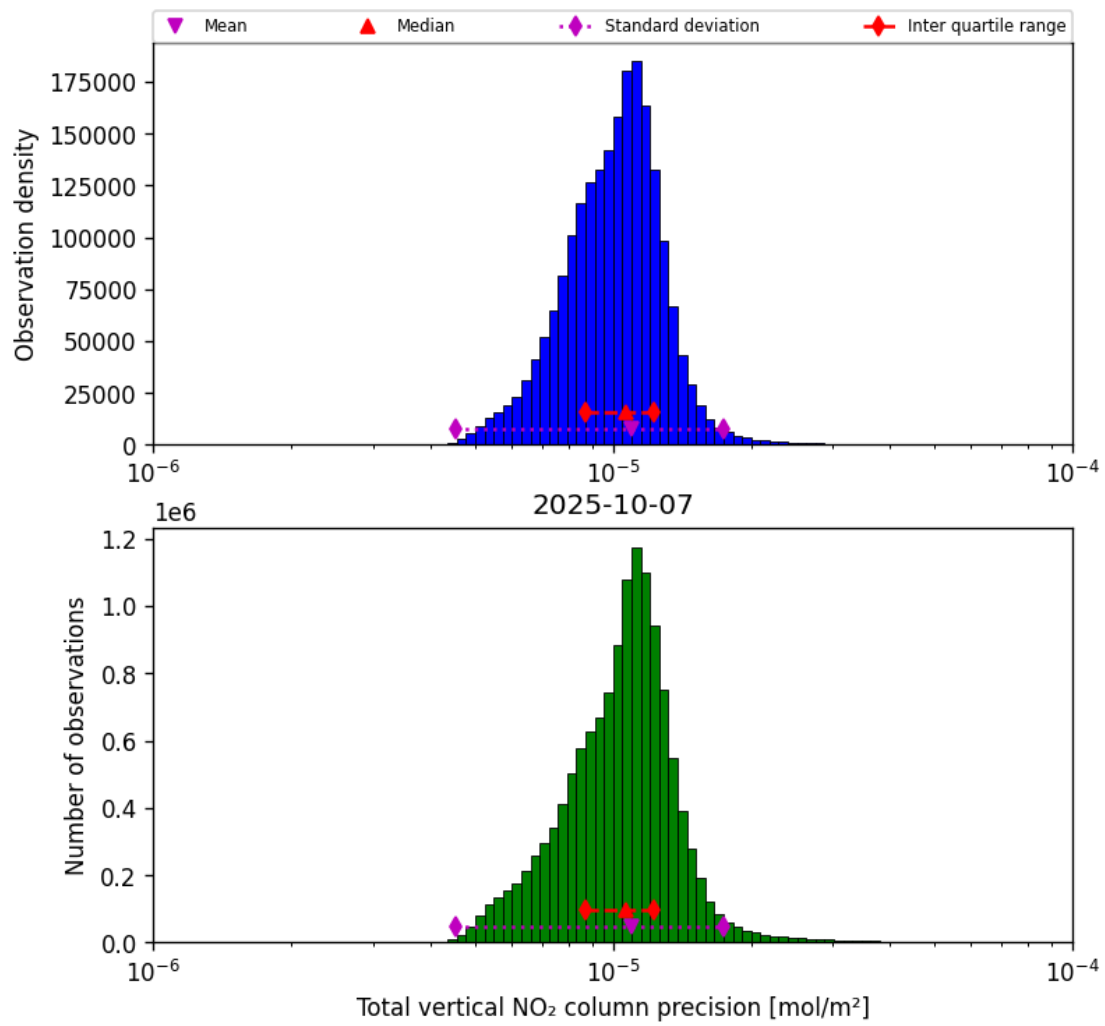
Figure 37: Histogram of "Total vertical NO 2 column precision" for 2025-10-07 to 2025-10-07
