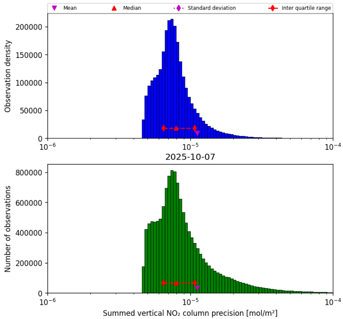
Figure 39: Histogram of “Summed vertical NO 2 column precision” for 2025-10-07 to 2025-10-07
