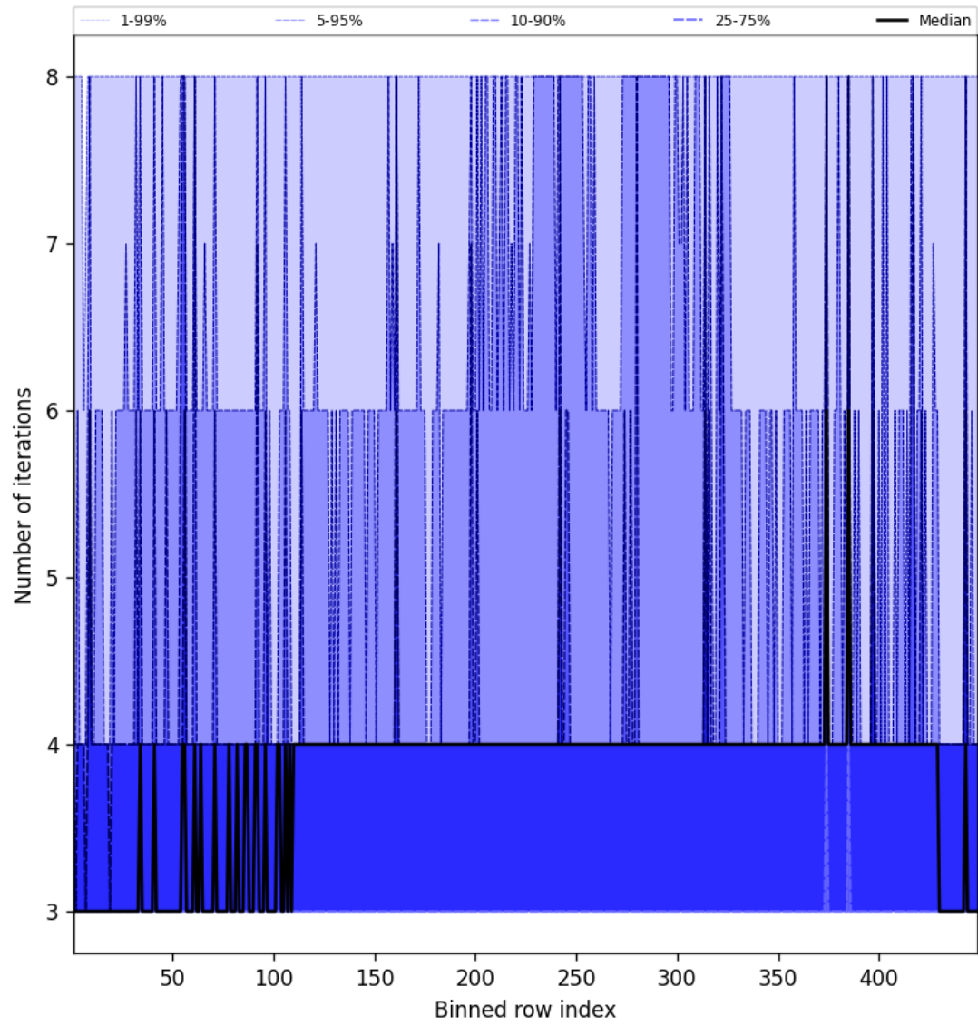
Figure 49: Along track statistics of “Number of iterations” for 2025-10-07 to 2025-10-07
