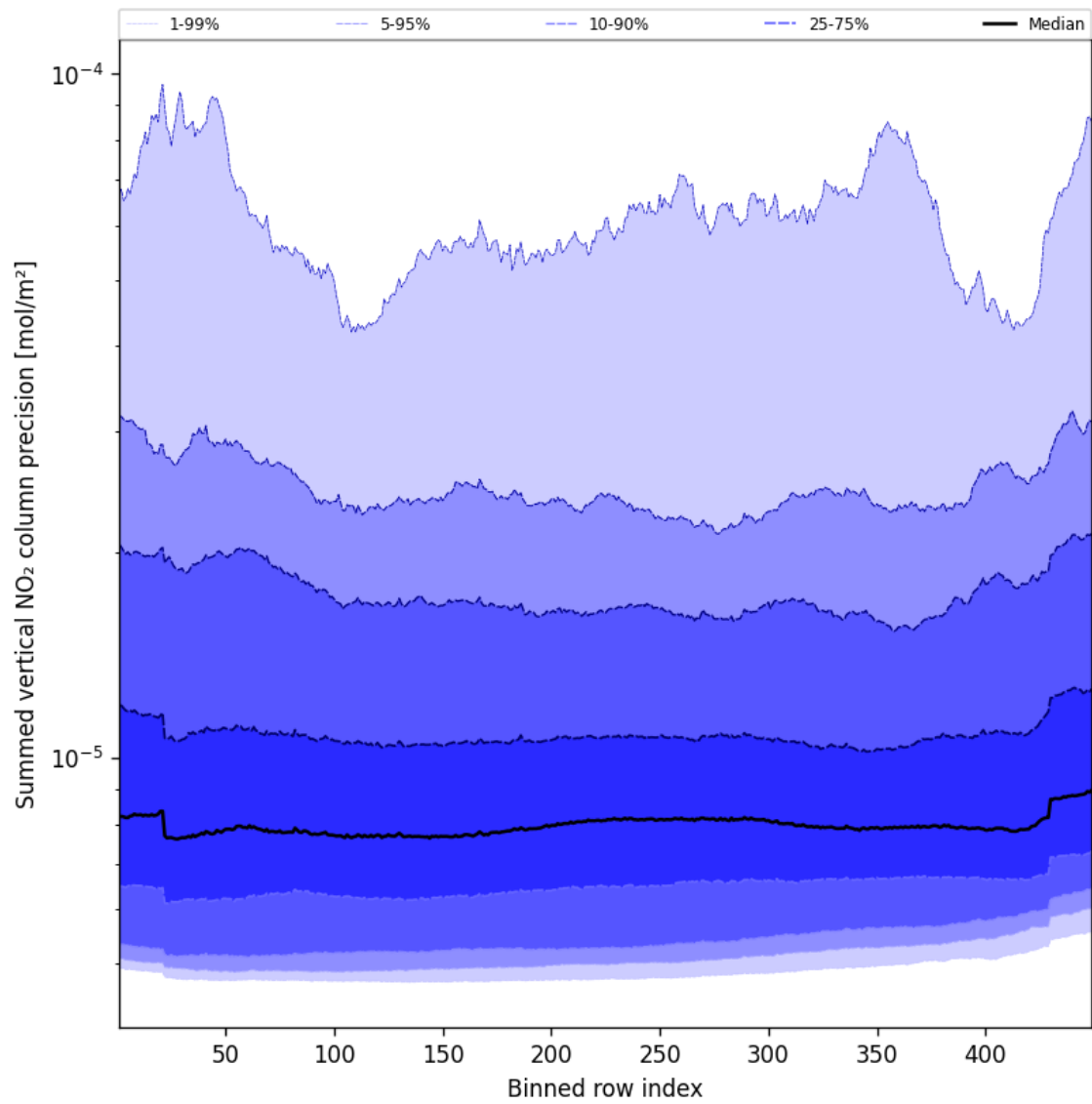
Figure 56: Along track statistics of “Summed vertical NO 2 column precision” for 2025-10-07 to 2025-10-07
