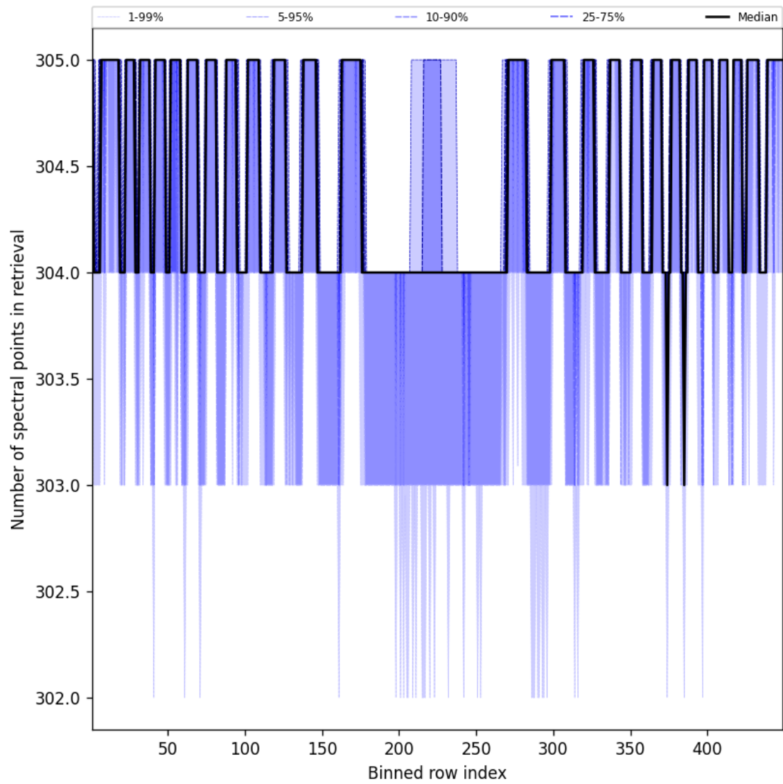
Figure 48: Along track statistics of “Number of spectral points in retrieval” for 2025-10-07 to 2025-10-07
