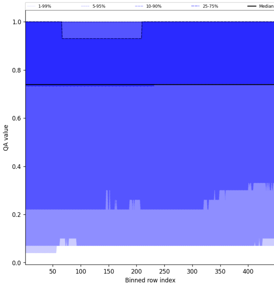
Figure 43: Along track statistics of “QA value” for 2025-10-07 to 2025-10-07
