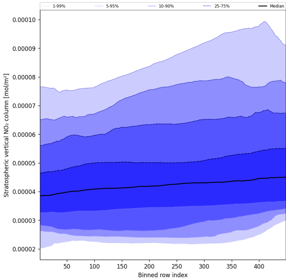
Figure 51: Along track statistics of “Stratospheric vertical NO 2 column” for 2025-10-07 to 2025-10-07
