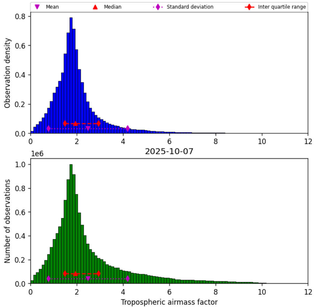
Figure 29: Histogram of “Tropospheric airmass factor” for 2025-10-07 to 2025-10-07
