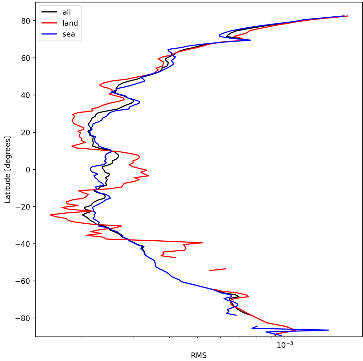
Figure 24: Zonal average of “RMS” for 2025-10-07 to 2025-10-07.
