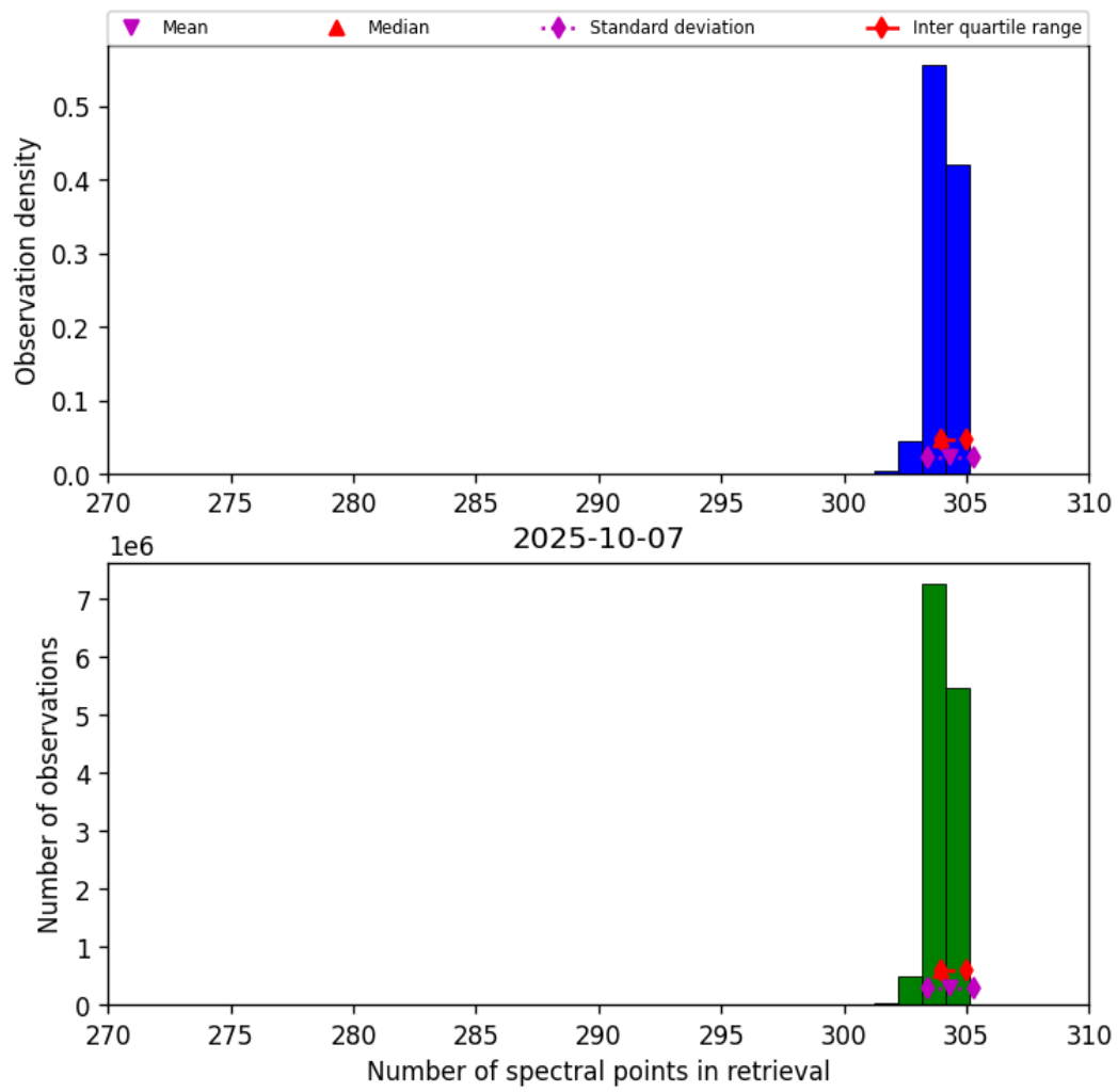
Figure 31: Histogram of “Number of spectral points in retrieval” for 2025-10-07 to 2025-10-07
