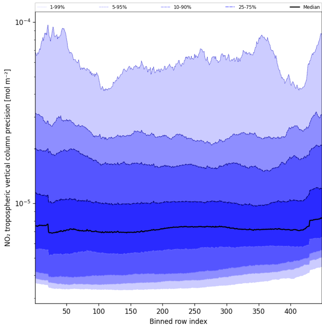
Figure 45: Along track statistics of “NO 2 tropospheric vertical column precision” for 2025-10-07 to 2025-10-07
