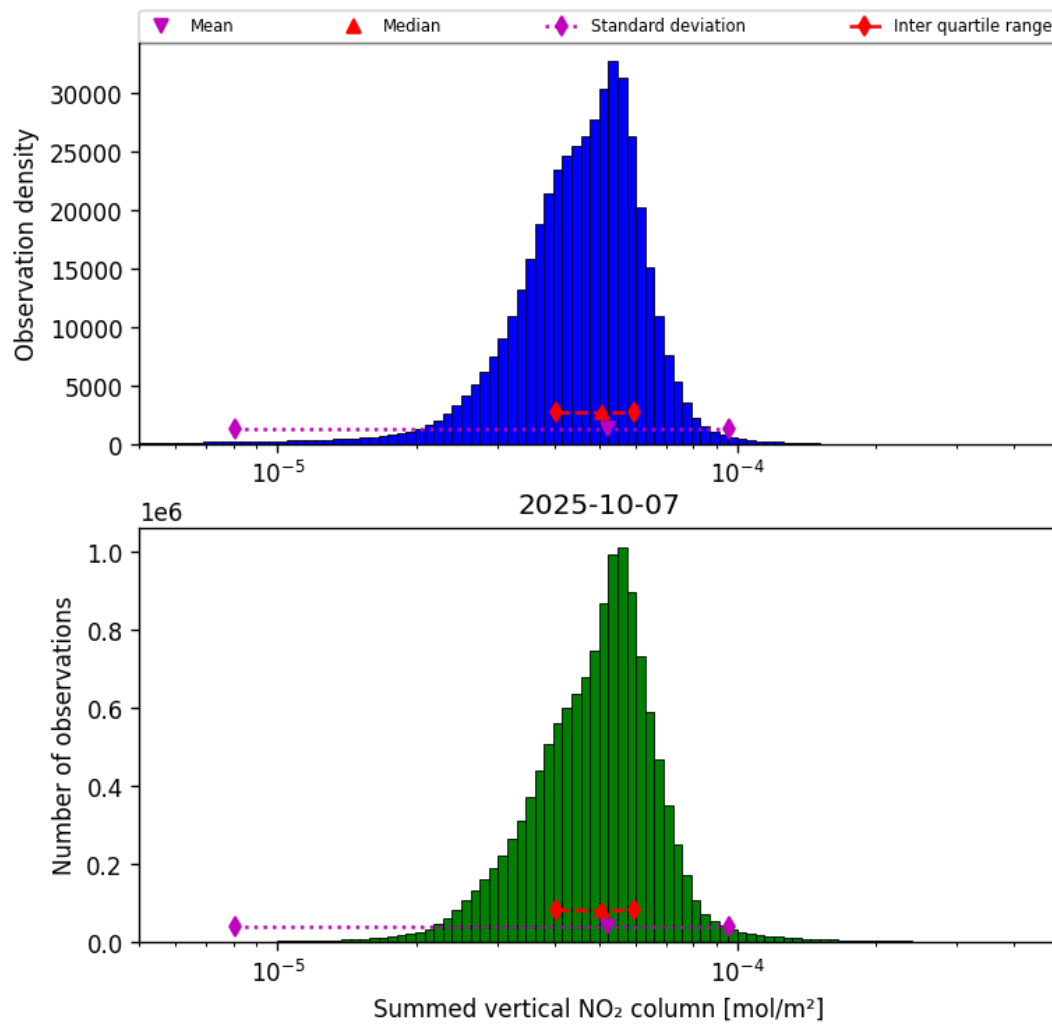
Figure 38: Histogram of “Summed vertical NO 2 column” for 2025-10-07 to 2025-10-07
