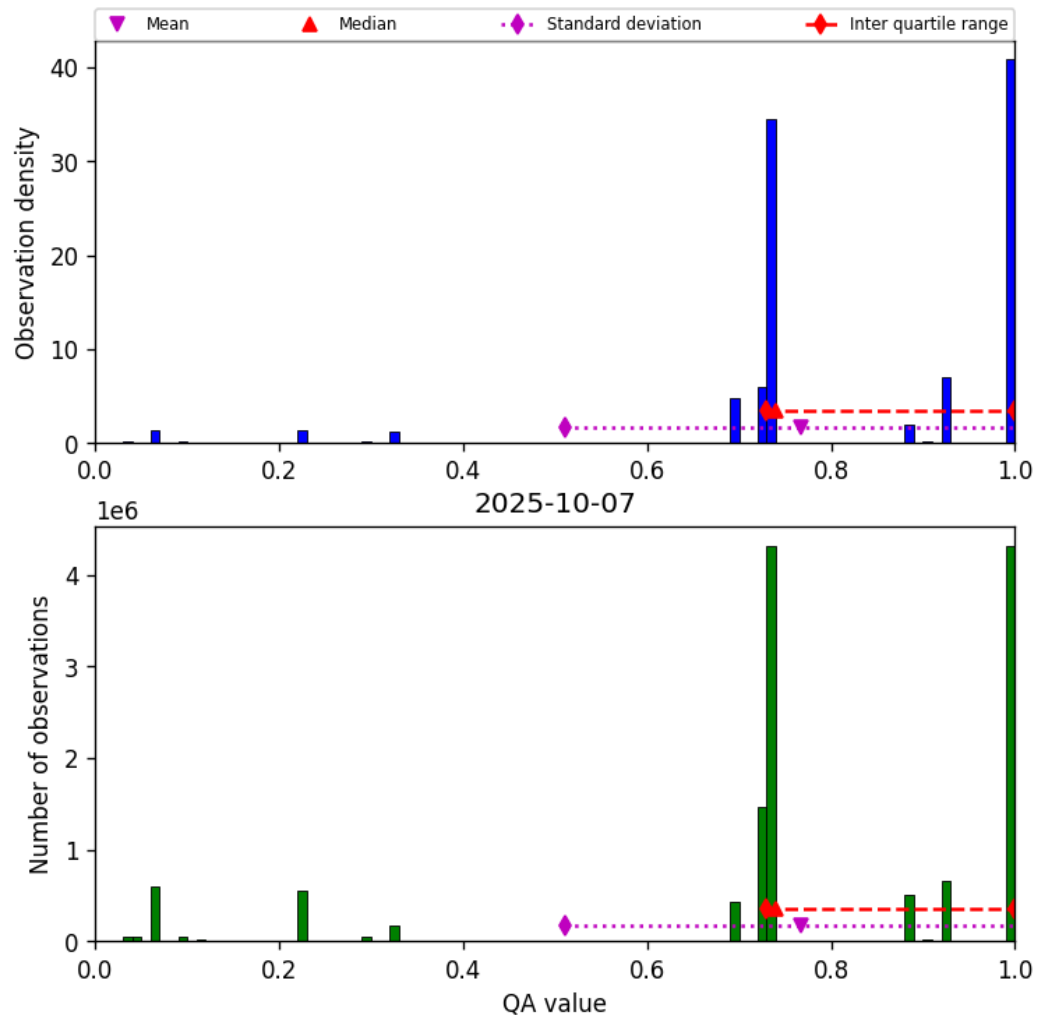
Figure 26: Histogram of “QA value” for 2025-10-07 to 2025-10-07
