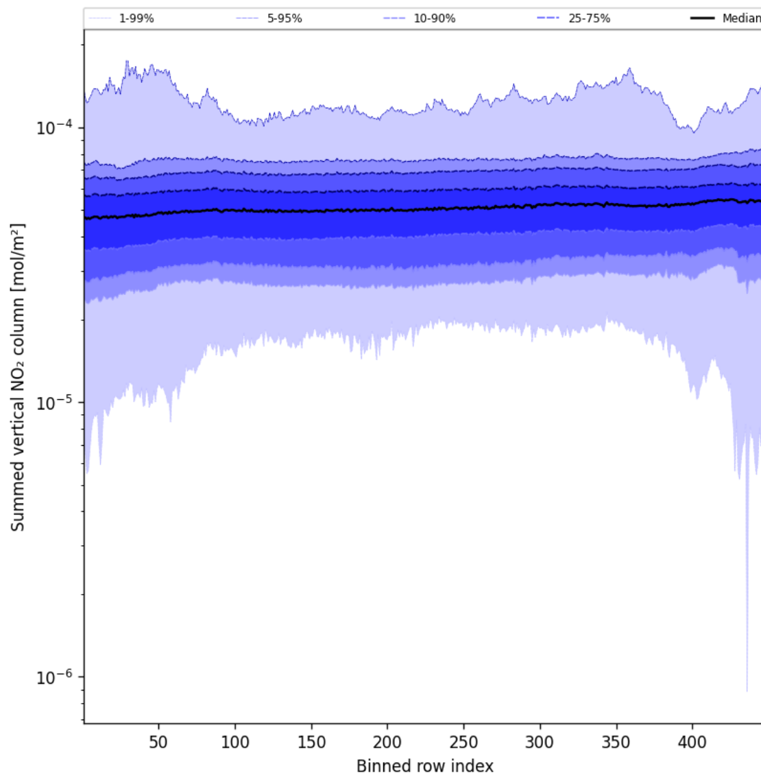
Figure 55: Along track statistics of “Summed vertical NO 2 column” for 2025-10-07 to 2025-10-07
