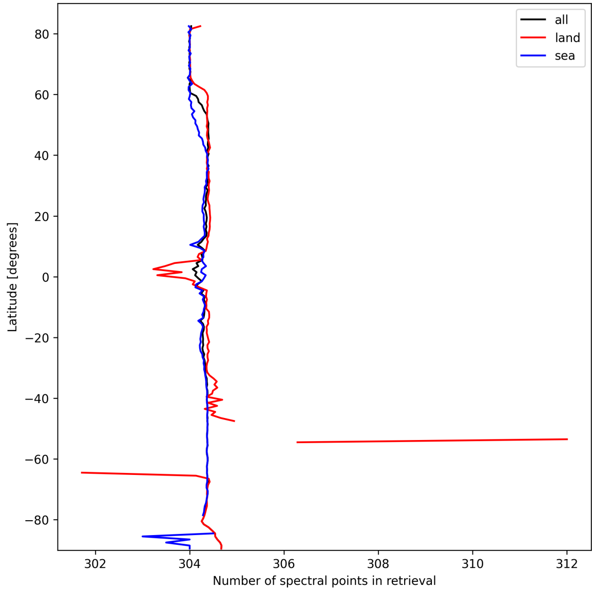
Figure 14: Zonal average of “Number of spectral points in retrieval” for 2025-10-07 to 2025-10-07.
