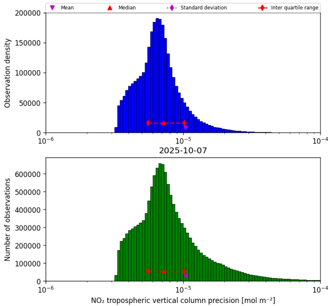
Figure 28: Histogram of “NO 2 tropospheric vertical column precision” for 2025-10-07 to 2025-10-07
