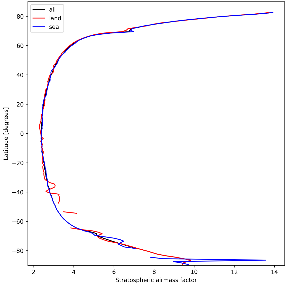
Figure 25: Zonal average of “Stratospheric air mass factor” for 2025-10-07 to 2025-10-07.
