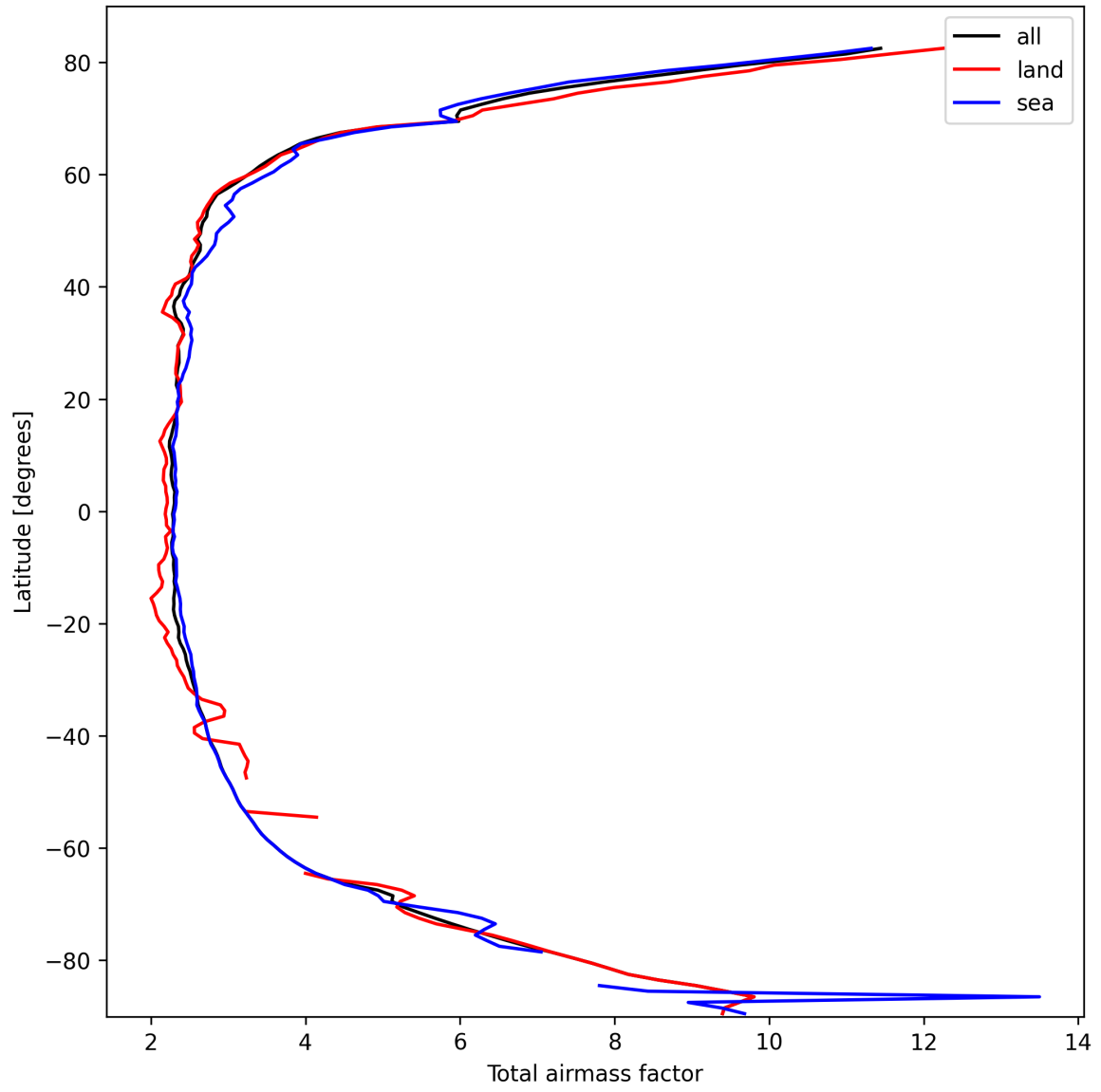
Figure 13: Zonal average of “Total airmass factor” for 2025-10-07 to 2025-10-07.
