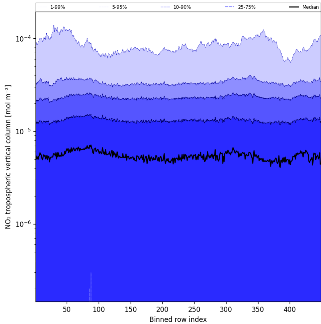
Figure 44: Along track statistics of “NO 2 tropospheric vertical column” for 2025-10-07 to 2025-10-07
