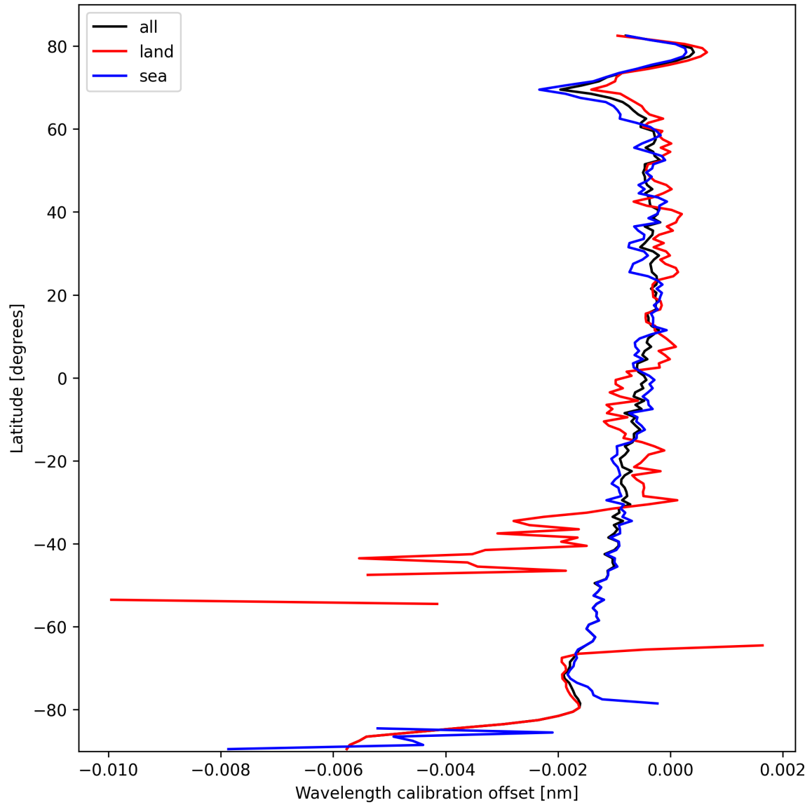
Figure 16: Zonal average of “Wavelength calibration offset” for 2025-10-07 to 2025-10-07.
