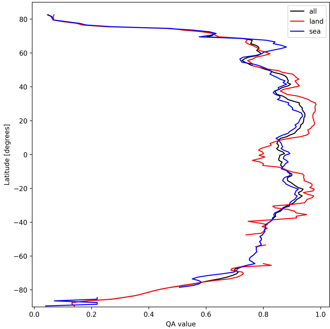
Figure 9: Zonal average of “QA value” for 2025-10-07 to 2025-10-07.
