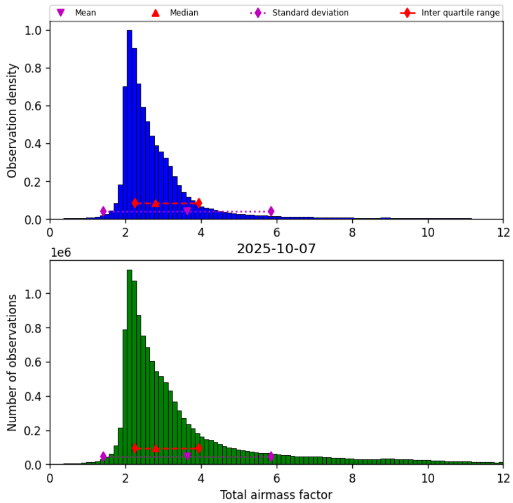
Figure 30: Histogram of “Total airmass factor” for 2025-10-07 to 2025-10-07
