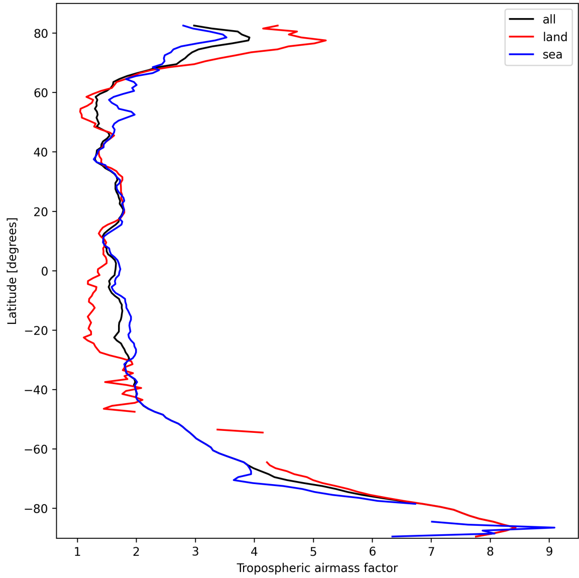
Figure 12: Zonal average of “Tropospheric airmass factor” for 2025-10-07 to 2025-10-07.
