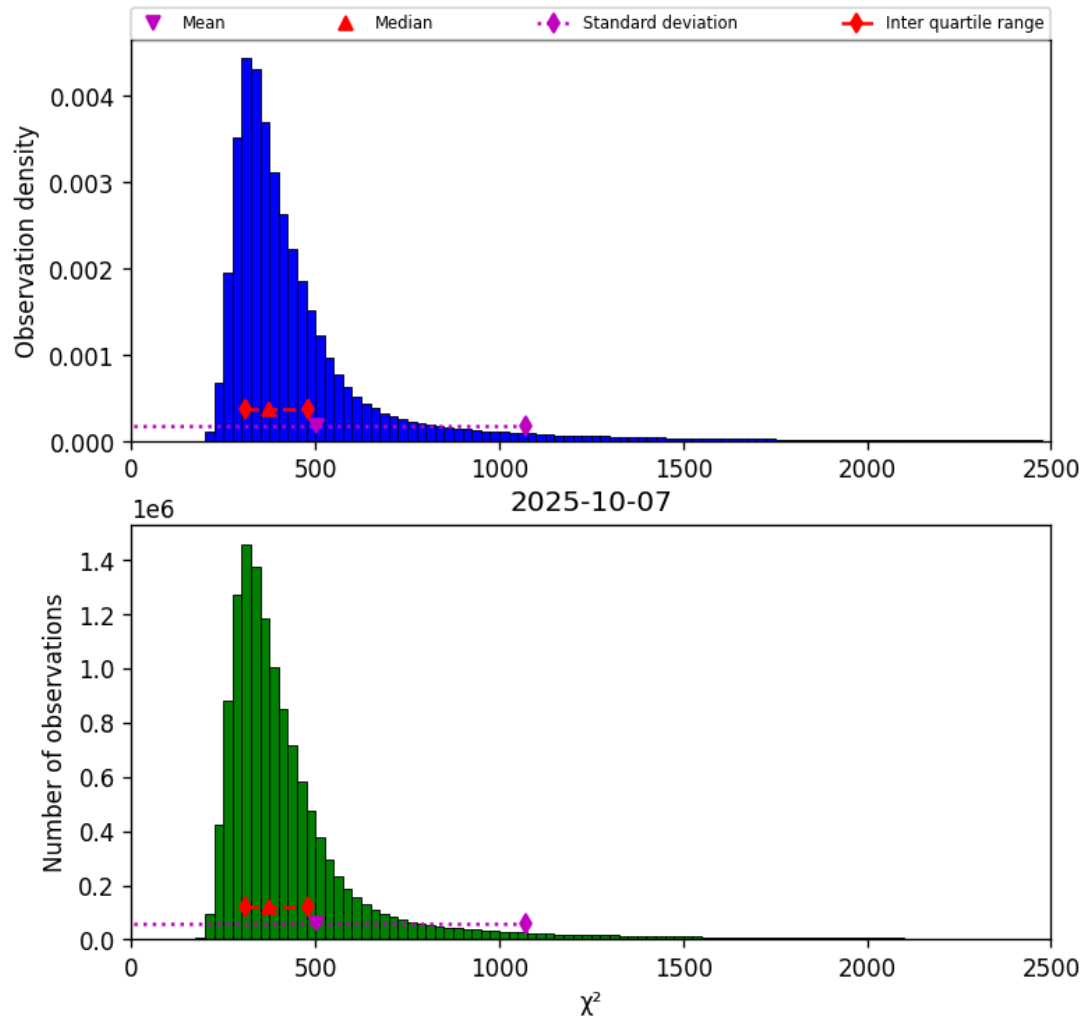
Figure 40: Histogram of “ \chi^2 ” for 2025-10-07 to 2025-10-07
