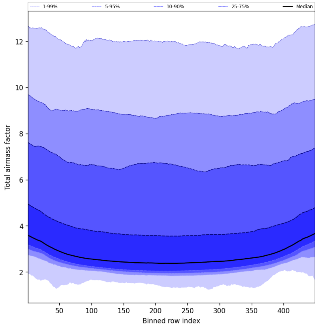
Figure 47: Along track statistics of “Total airmass factor” for 2025-10-07 to 2025-10-07
