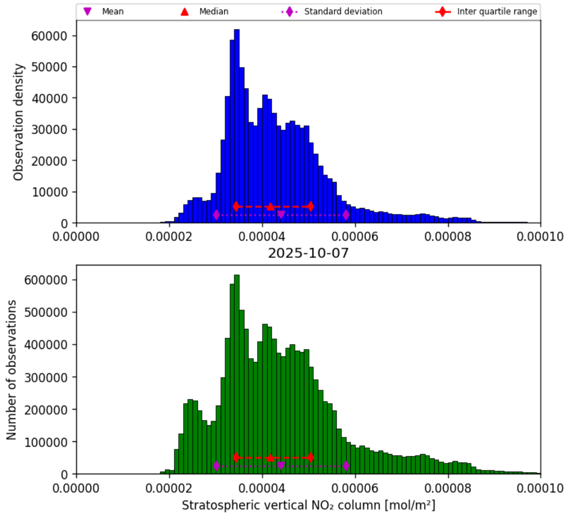
Figure 34: Histogram of “Stratospheric vertical NO 2 column” for 2025-10-07 to 2025-10-07
