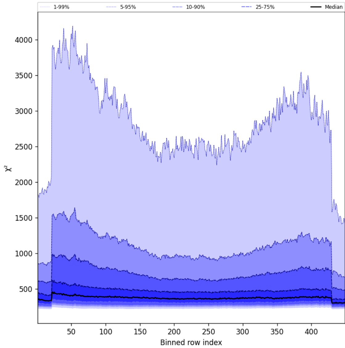
Figure 57: Along track statistics of “ \chi^2 ” for 2025-10-07 to 2025-10-07
