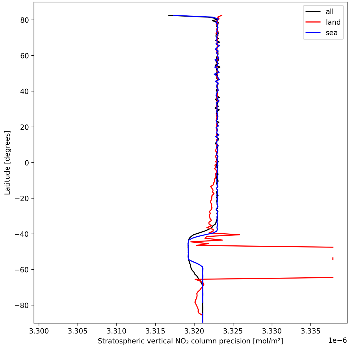
Figure 18: Zonal average of “Stratospheric vertical NO 2 column precision” for 2025-10-07 to 2025-10-07.
