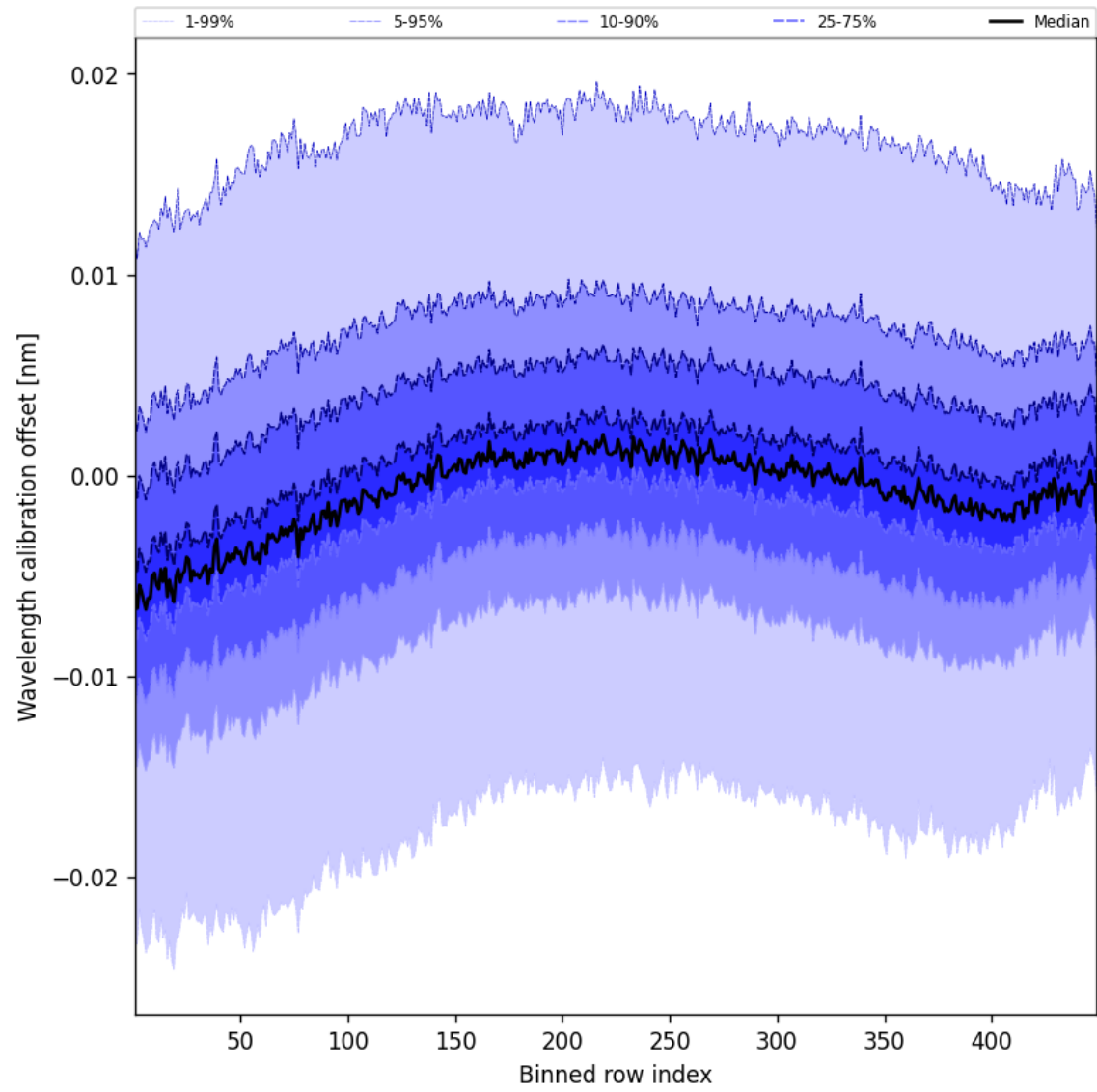
Figure 50: Along track statistics of “Wavelength calibration offset” for 2025-10-07 to 2025-10-07
