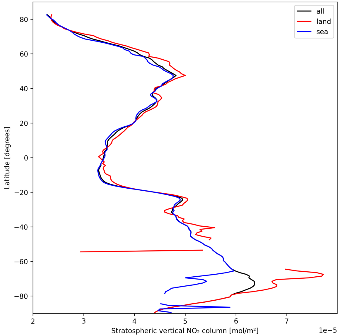
Figure 17: Zonal average of “Stratospheric vertical NO 2 column” for 2025-10-07 to 2025-10-07.
