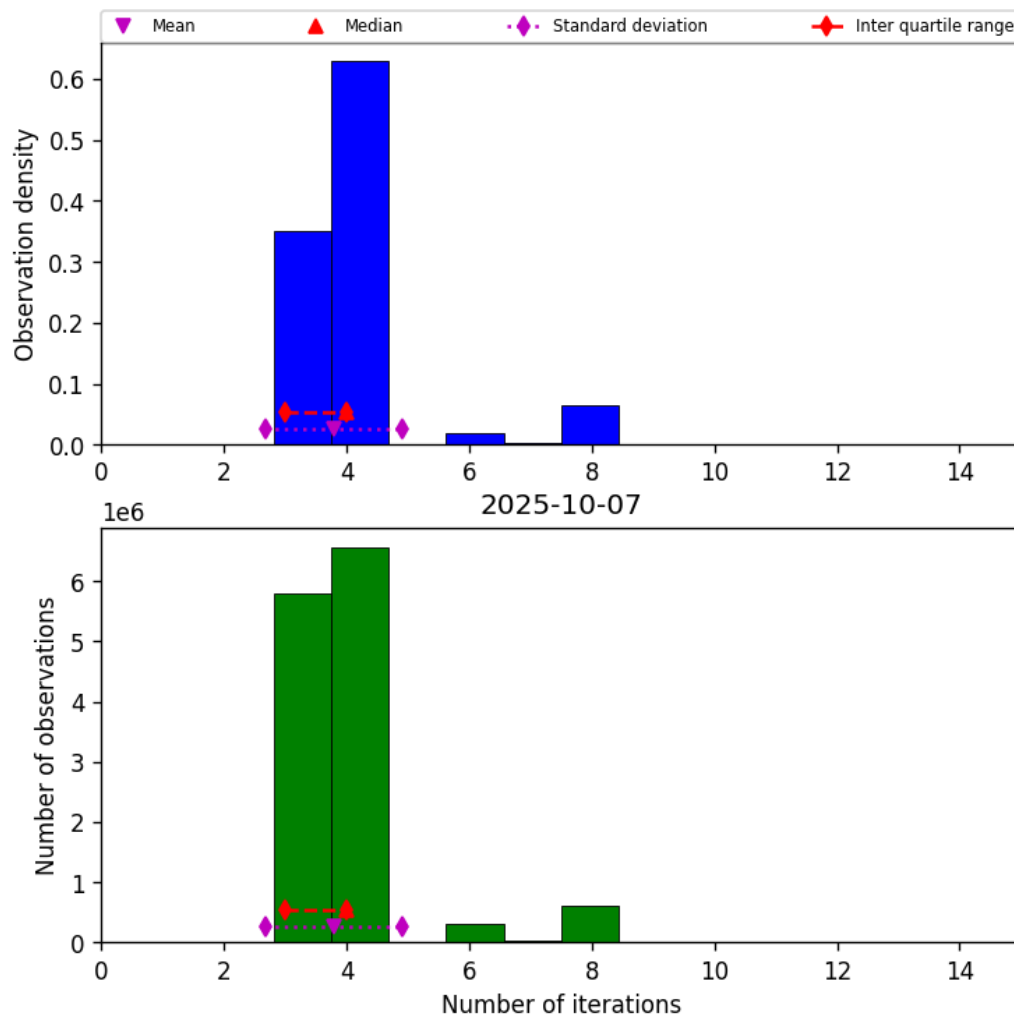
Figure 32: Histogram of “Number of iterations” for 2025-10-07 to 2025-10-07
