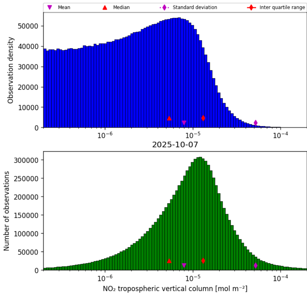
Figure 27: Histogram of “NO 2 tropospheric vertical column” for 2025-10-07 to 2025-10-07
