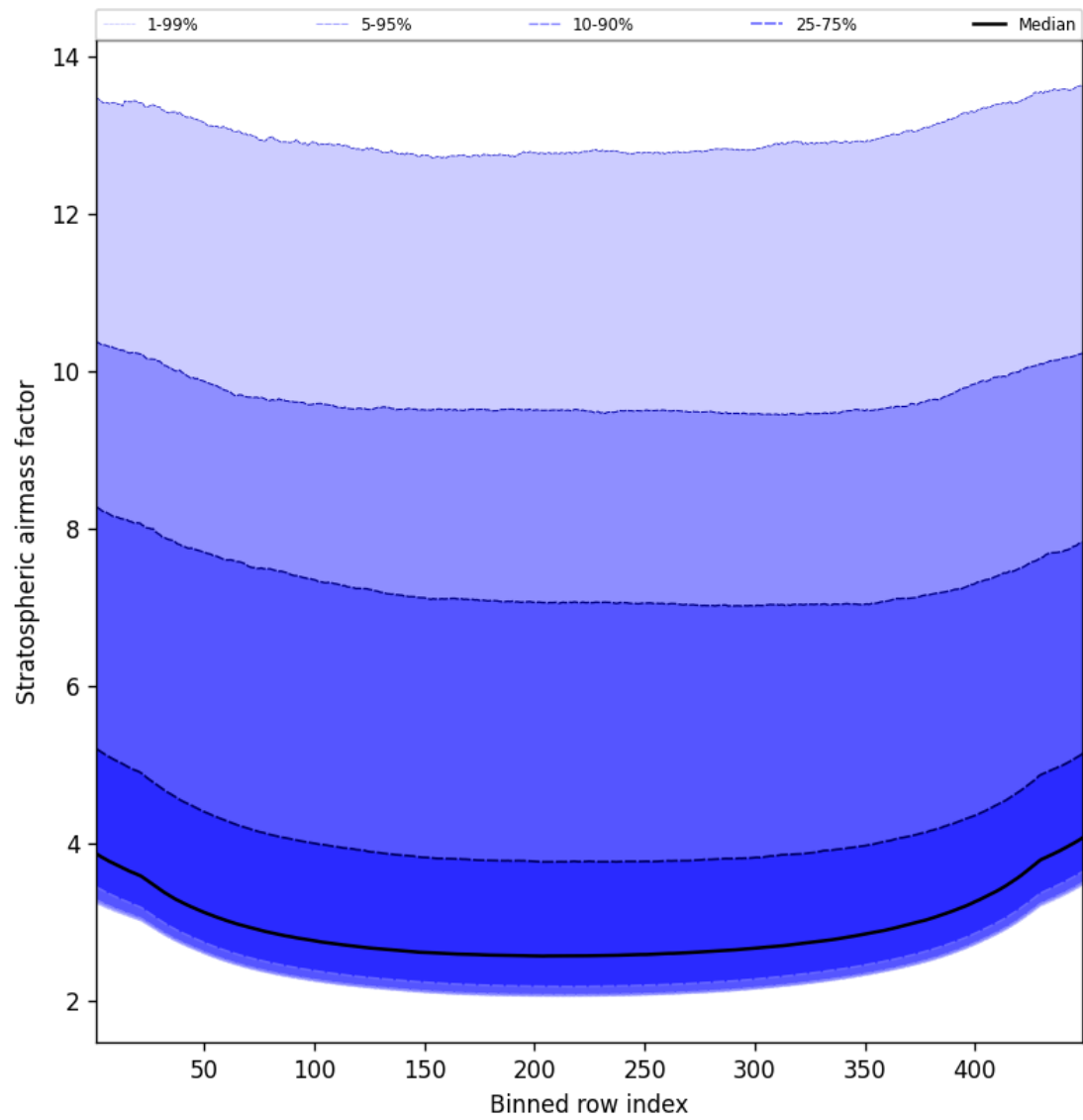
Figure 59: Along track statistics of “Stratospheric airmass factor” for 2025-10-07 to 2025-10-07
