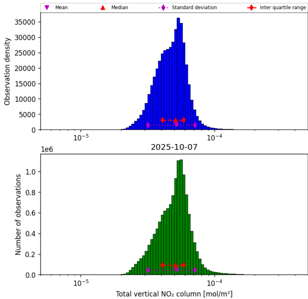
Figure 36: Histogram of "Total vertical NO 2 column" for 2025-10-07 to 2025-10-07
