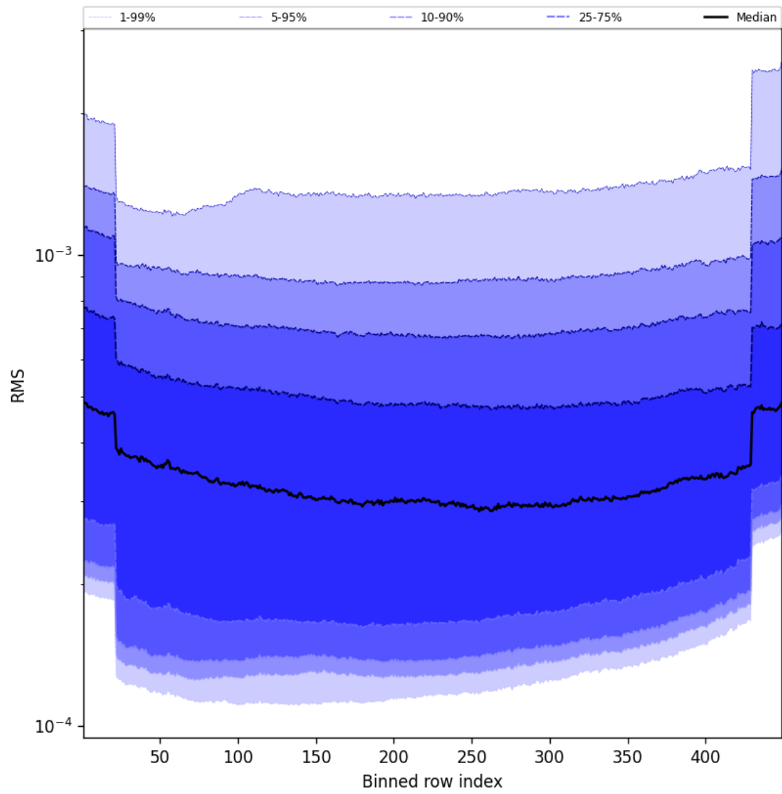
Figure 58: Along track statistics of “RMS” for 2025-10-07 to 2025-10-07
