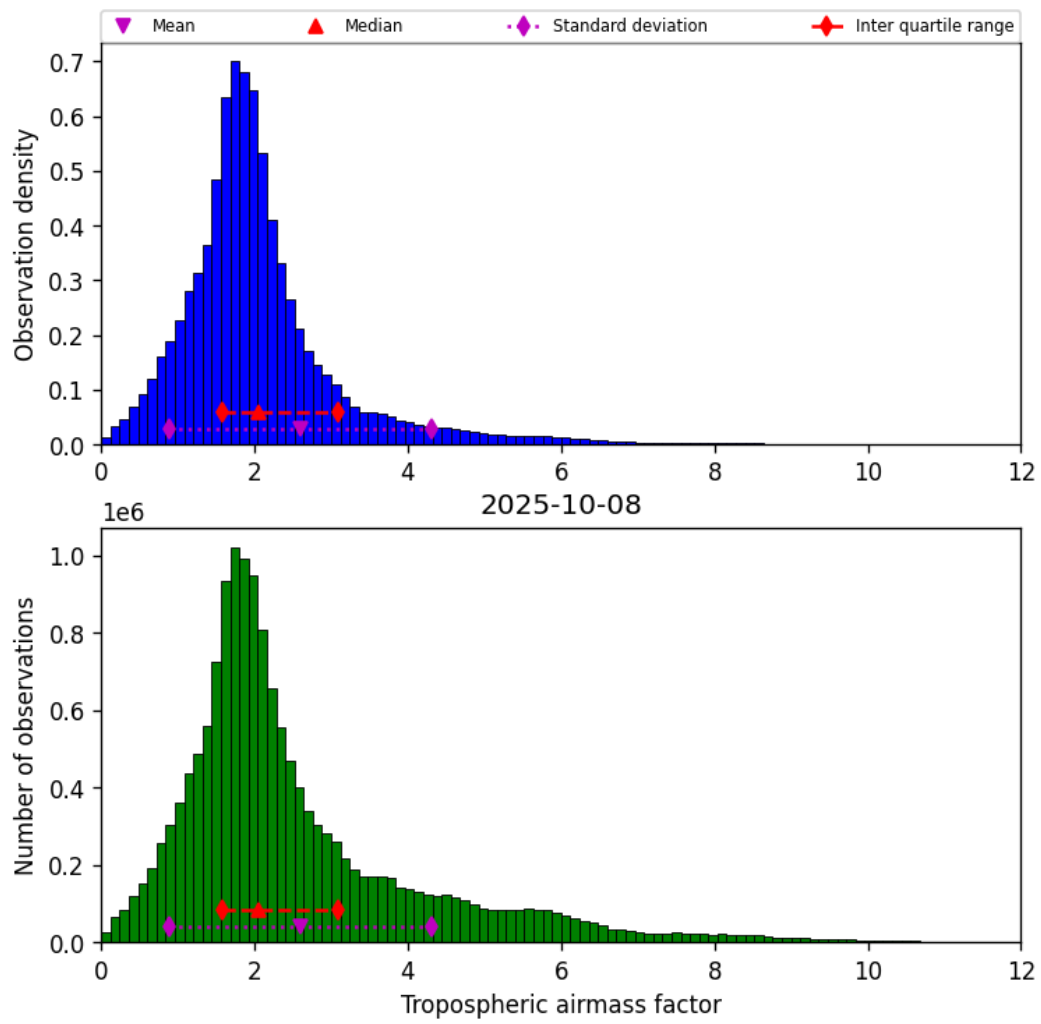
Figure 29: Histogram of “Tropospheric airmass factor” for 2025-10-08 to 2025-10-09
