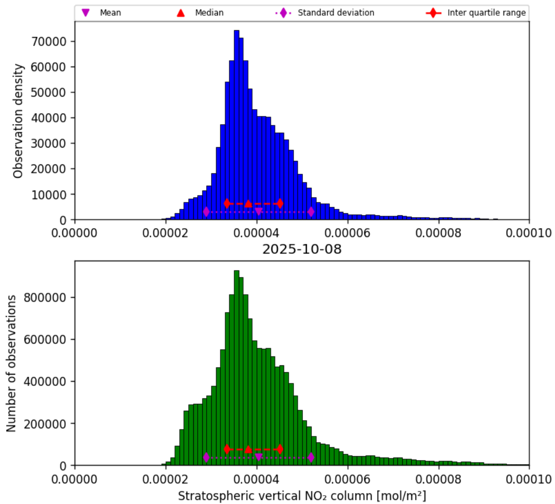
Figure 34: Histogram of “Stratospheric vertical NO 2 column” for 2025-10-08 to 2025-10-09
