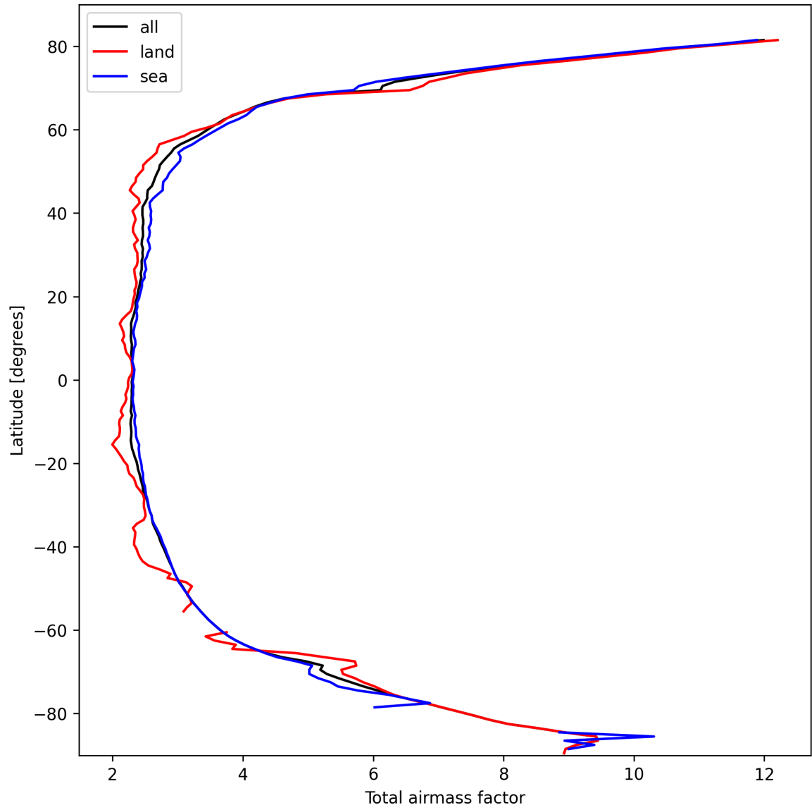
Figure 13: Zonal average of “Total airmass factor” for 2025-10-08 to 2025-10-09.
