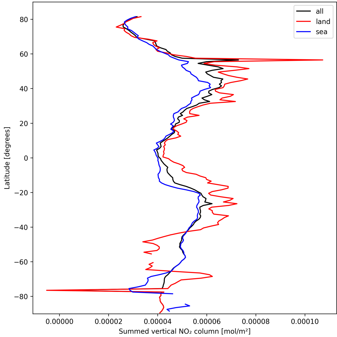
Figure 21: Zonal average of “Summed vertical NO 2 column” for 2025-10-08 to 2025-10-09.
