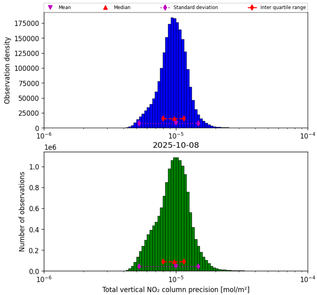
Figure 37: Histogram of “Total vertical NO 2 column precision” for 2025-10-08 to 2025-10-09
