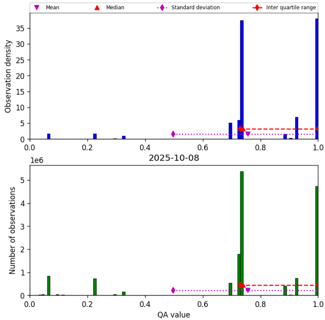
Figure 26: Histogram of “QA value” for 2025-10-08 to 2025-10-09
