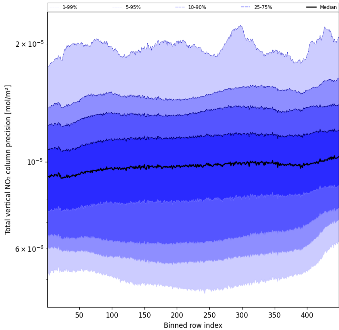
Figure 54: Along track statistics of “Total vertical NO 2 column precision” for 2025-10-08 to 2025-10-09
