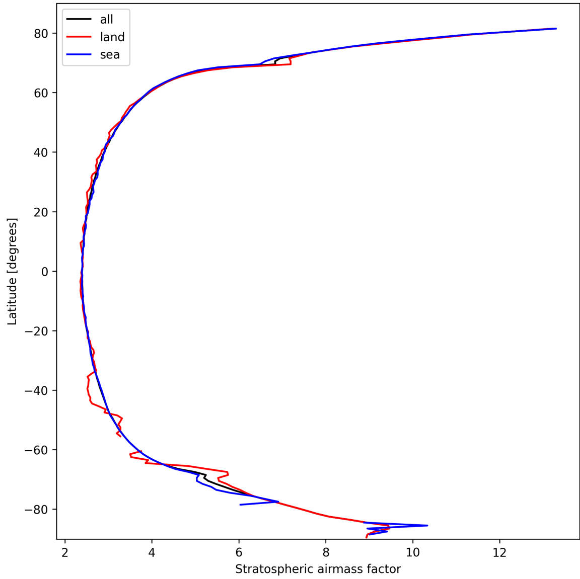
Figure 25: Zonal average of “Stratospheric air mass factor” for 2025-10-08 to 2025-10-09.
