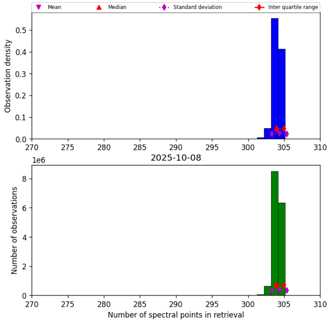
Figure 31: Histogram of “Number of spectral points in retrieval” for 2025-10-08 to 2025-10-09
