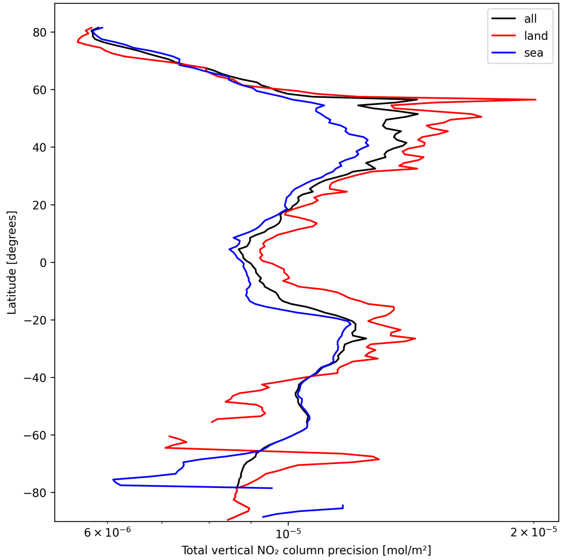
Figure 20: Zonal average of “Total vertical NO 2 column precision” for 2025-10-08 to 2025-10-09.
