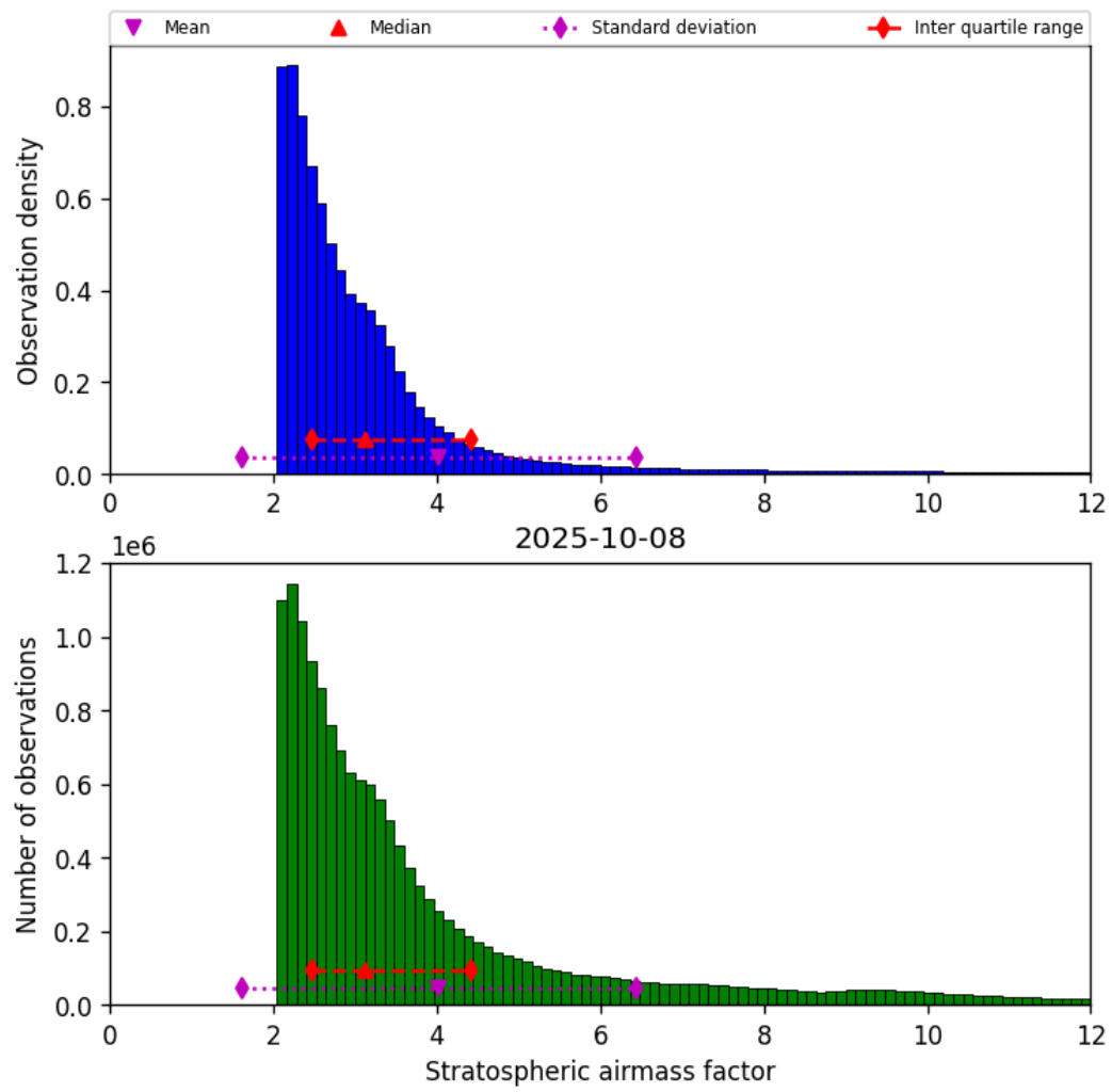
Figure 42: Histogram of “Stratospheric airmass factor” for 2025-10-08 to 2025-10-09
