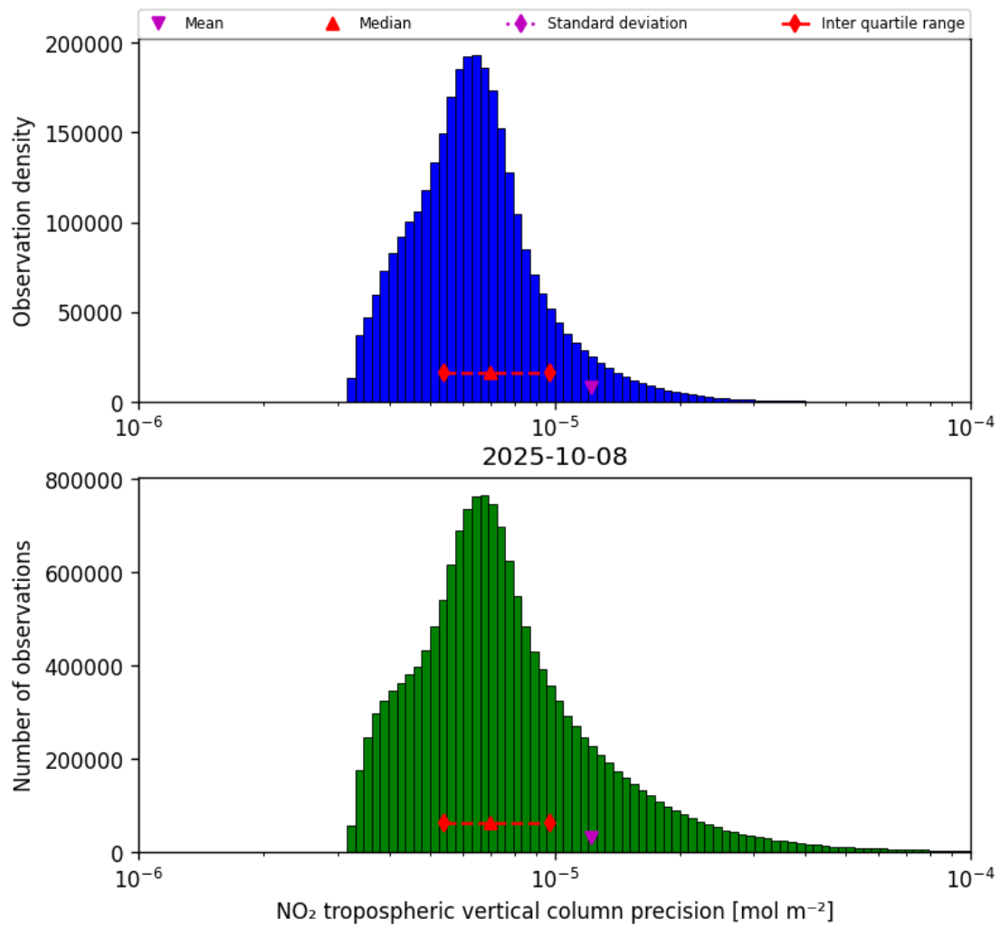
Figure 28: Histogram of “NO 2 tropospheric vertical column precision” for 2025-10-08 to 2025-10-09
