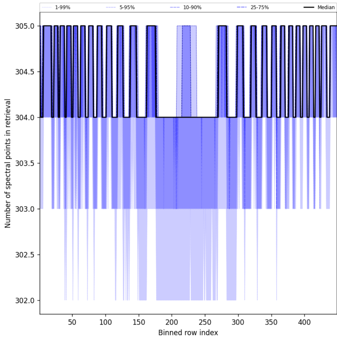
Figure 48: Along track statistics of “Number of spectral points in retrieval” for 2025-10-08 to 2025-10-09
