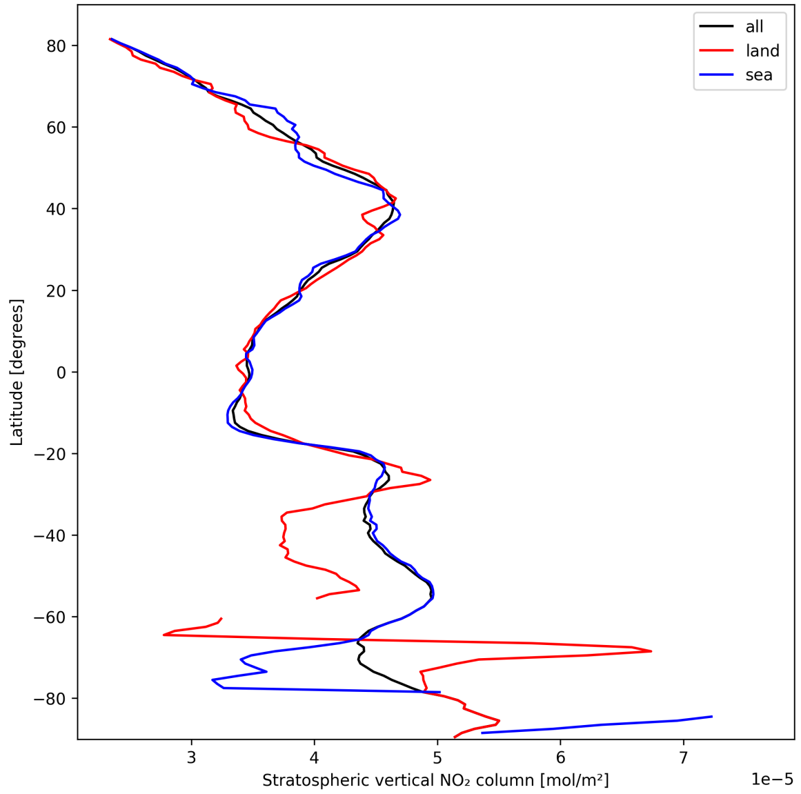
Figure 17: Zonal average of “Stratospheric vertical NO 2 column” for 2025-10-08 to 2025-10-09.
