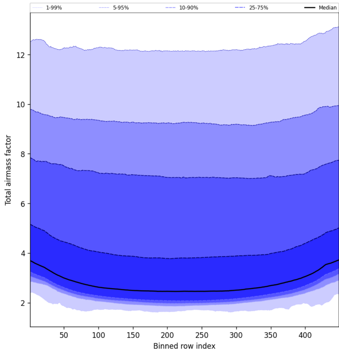
Figure 47: Along track statistics of “Total airmass factor” for 2025-10-08 to 2025-10-09
