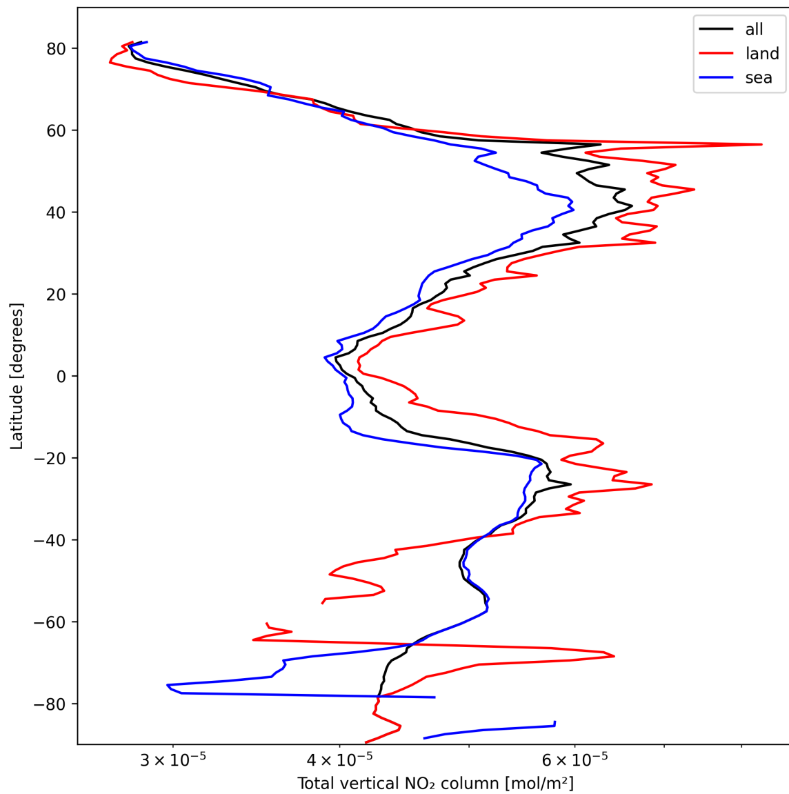
Figure 19: Zonal average of “Total vertical NO 2 column” for 2025-10-08 to 2025-10-09.
