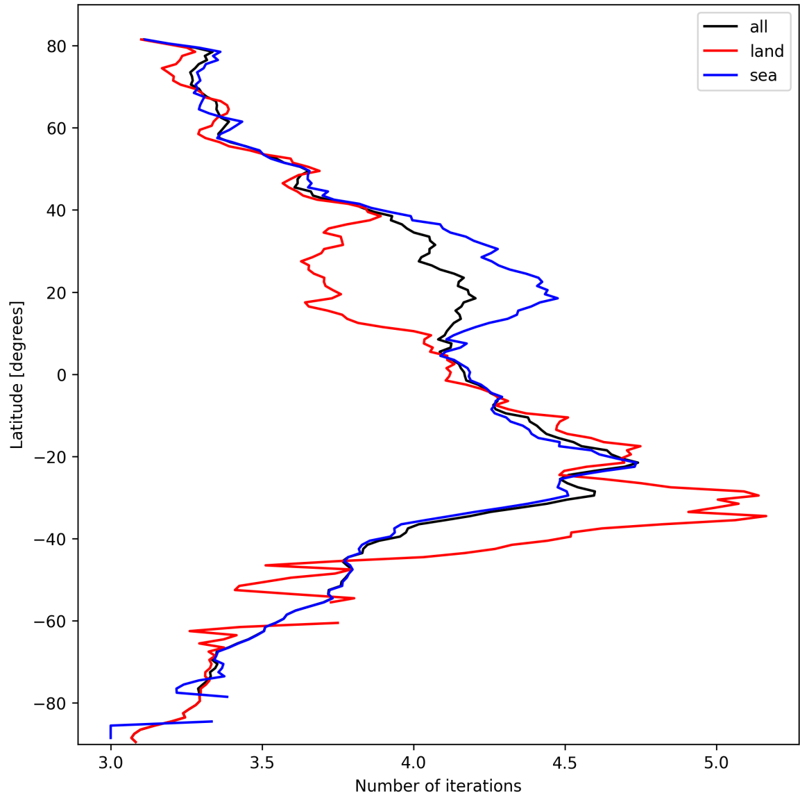
Figure 15: Zonal average of “Number of iterations” for 2025-10-08 to 2025-10-09.
