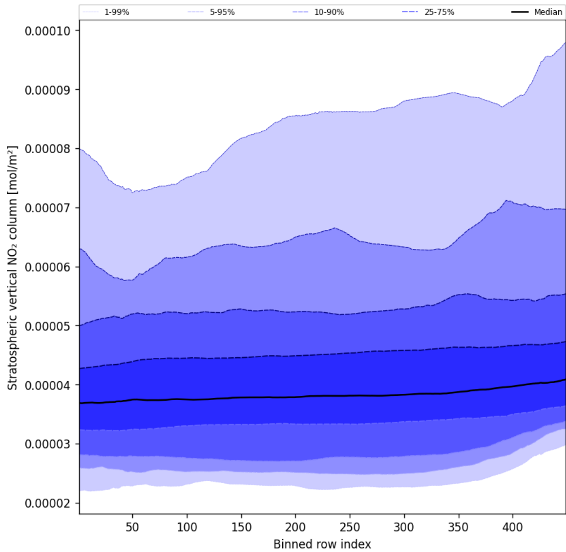
Figure 51: Along track statistics of “Stratospheric vertical NO 2 column” for 2025-10-08 to 2025-10-09
