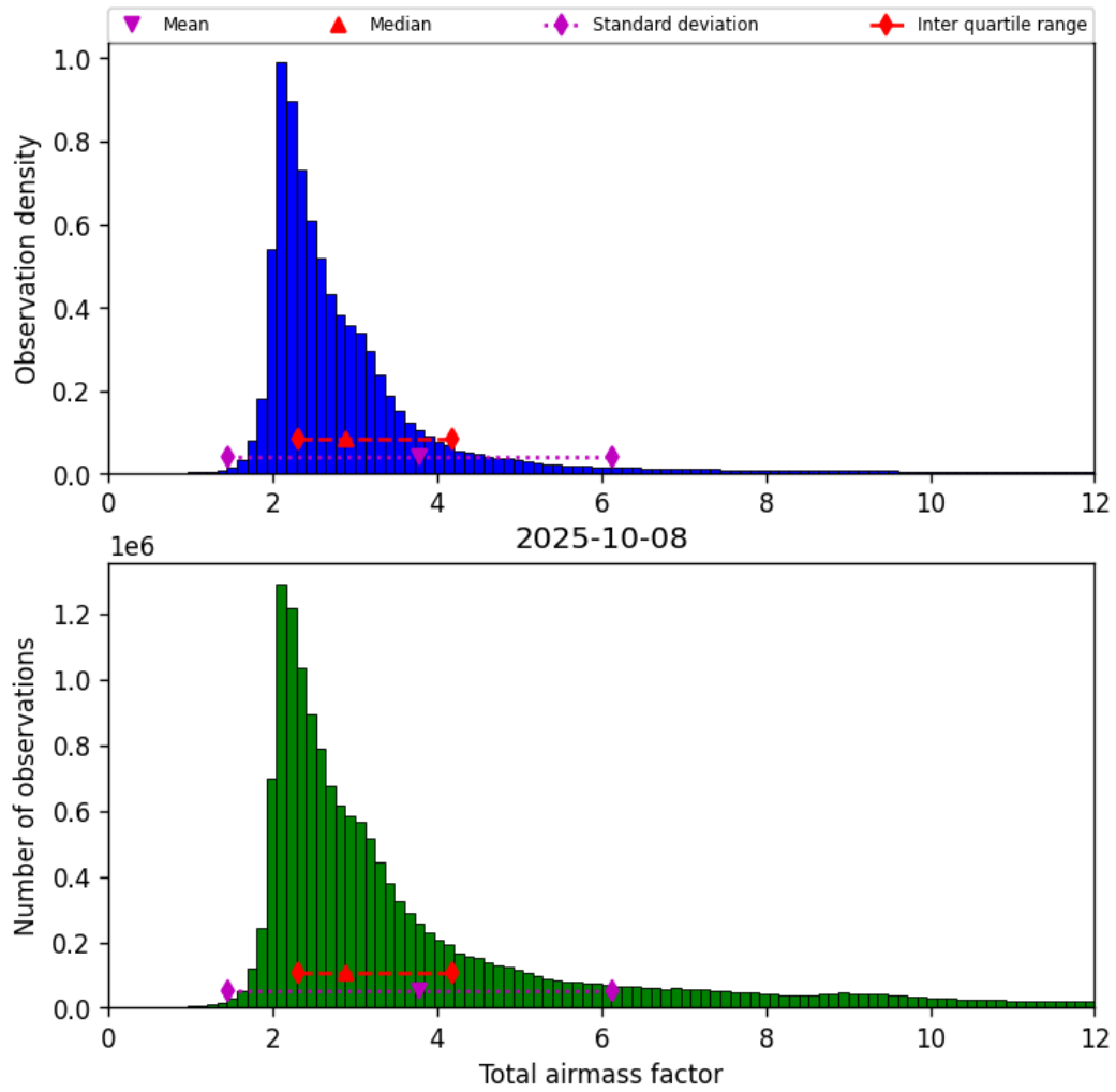
Figure 30: Histogram of “Total airmass factor” for 2025-10-08 to 2025-10-09
