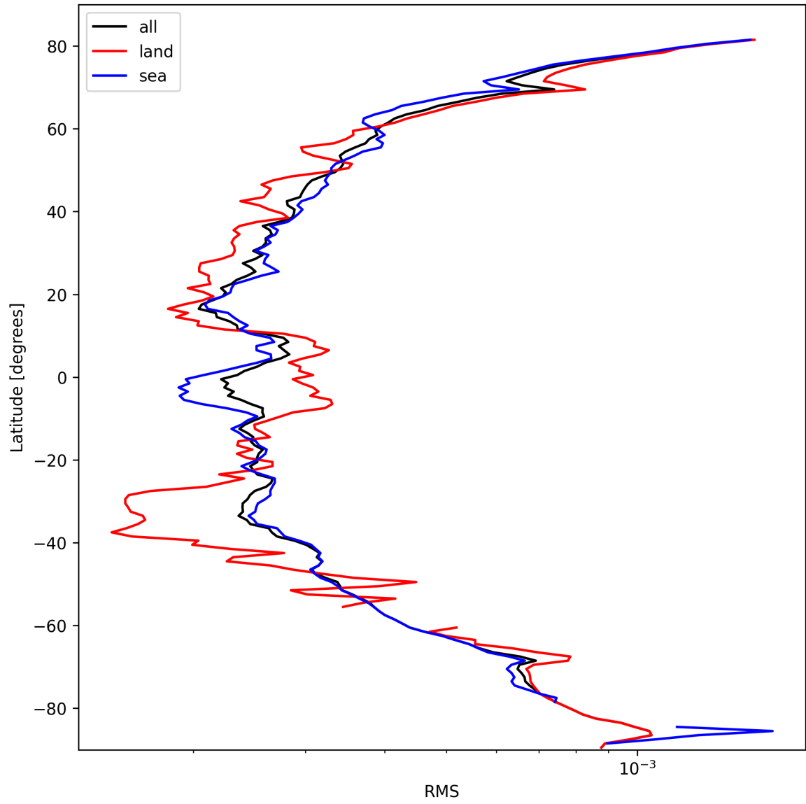
Figure 24: Zonal average of “RMS” for 2025-10-08 to 2025-10-09.
