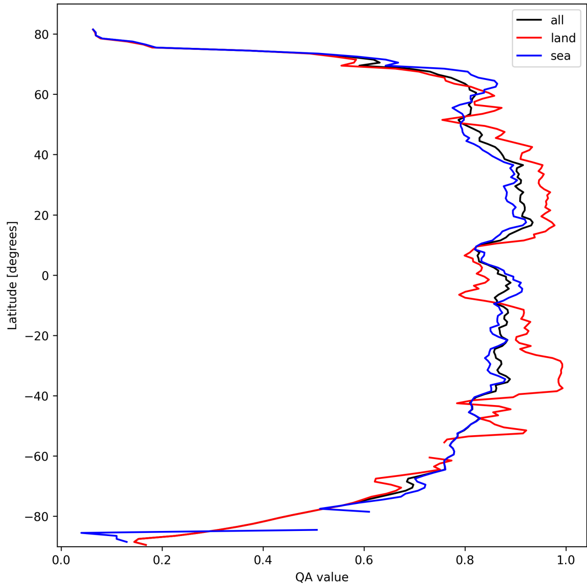
Figure 9: Zonal average of “QA value” for 2025-10-08 to 2025-10-09.
