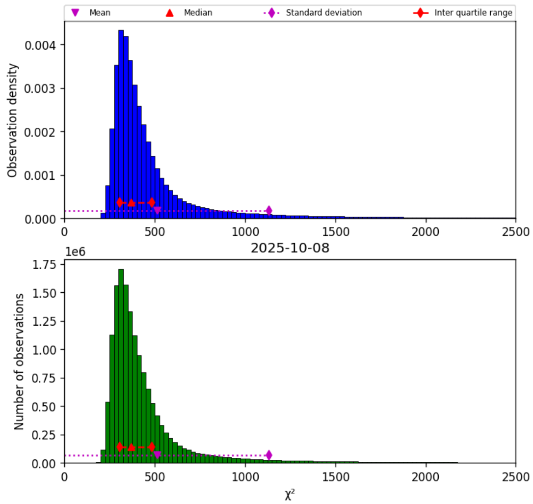
Figure 40: Histogram of “ \chi^2 ” for 2025-10-08 to 2025-10-09
