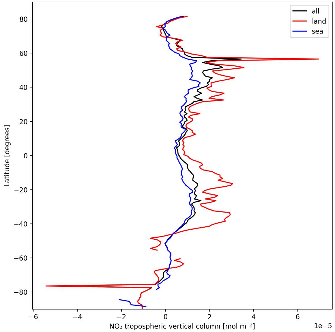
Figure 10: Zonal average of “NO 2 tropospheric vertical column” for 2025-10-08 to 2025-10-09.
