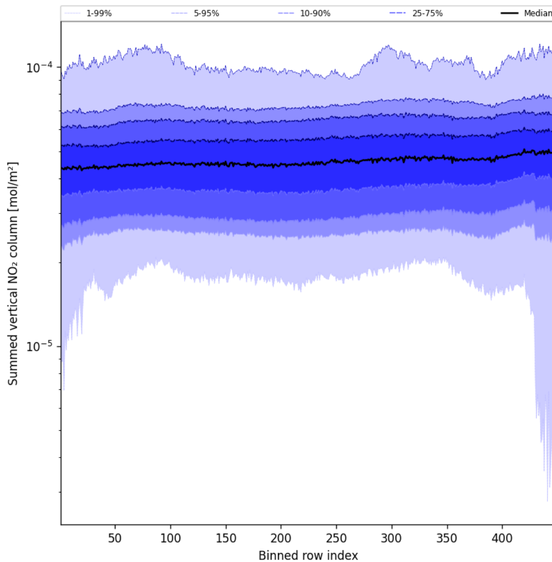
Figure 55: Along track statistics of “Summed vertical NO 2 column” for 2025-10-08 to 2025-10-09
