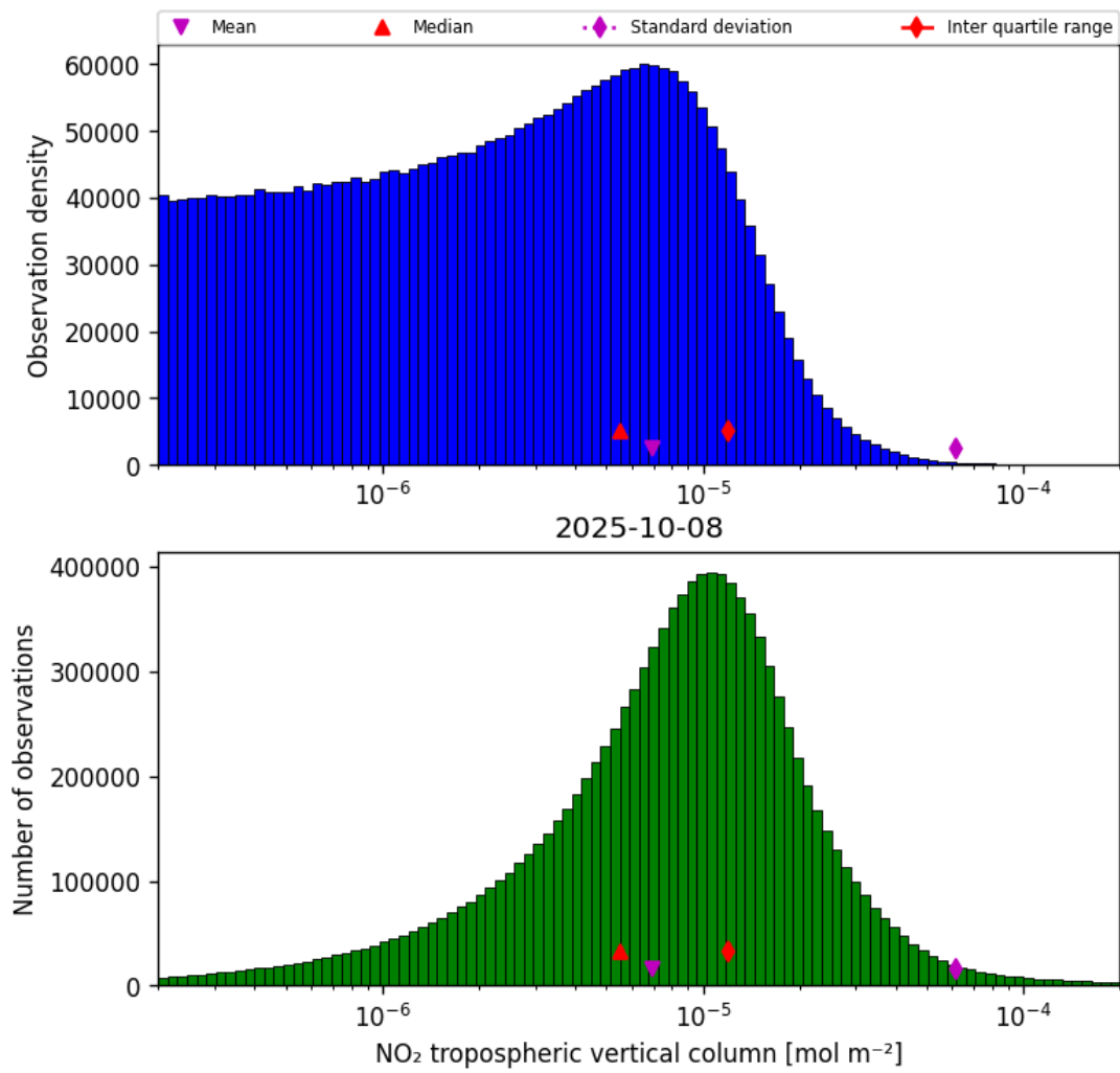
Figure 27: Histogram of “NO 2 tropospheric vertical column” for 2025-10-08 to 2025-10-09
