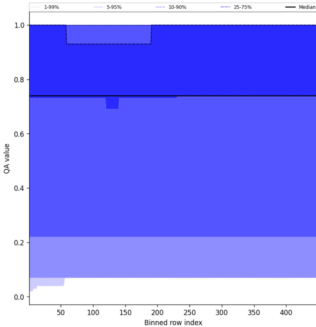
Figure 43: Along track statistics of "QA value" for 2025-10-08 to 2025-10-09
