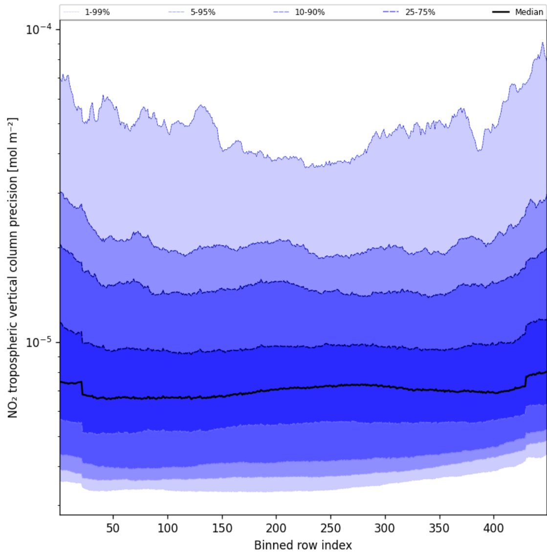
Figure 45: Along track statistics of “NO 2 tropospheric vertical column precision” for 2025-10-08 to 2025-10-09
