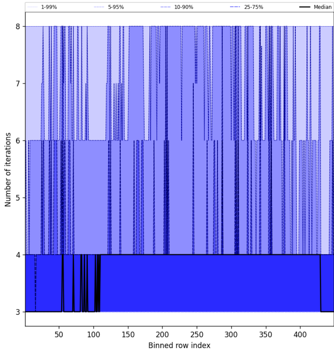
Figure 49: Along track statistics of “Number of iterations” for 2025-10-08 to 2025-10-09
