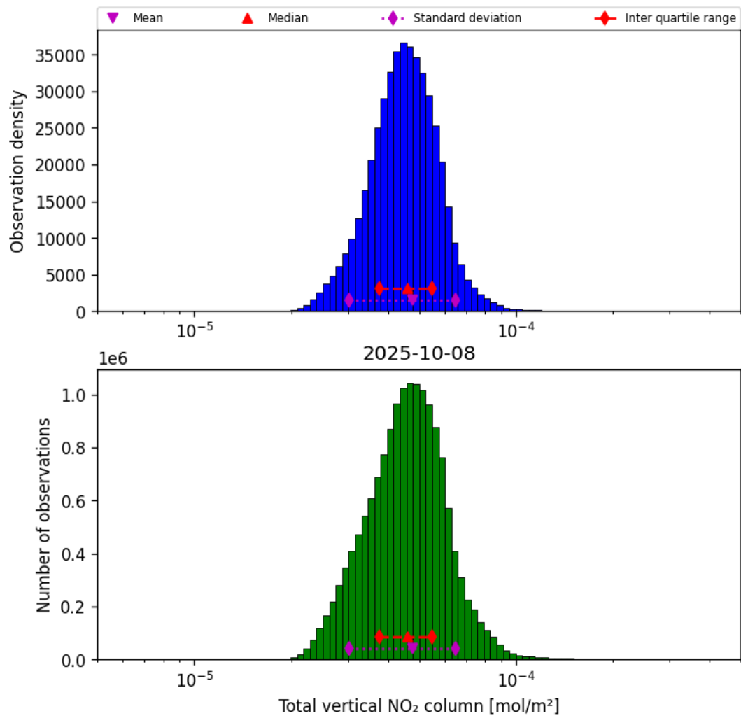
Figure 36: Histogram of “Total vertical NO 2 column” for 2025-10-08 to 2025-10-09
