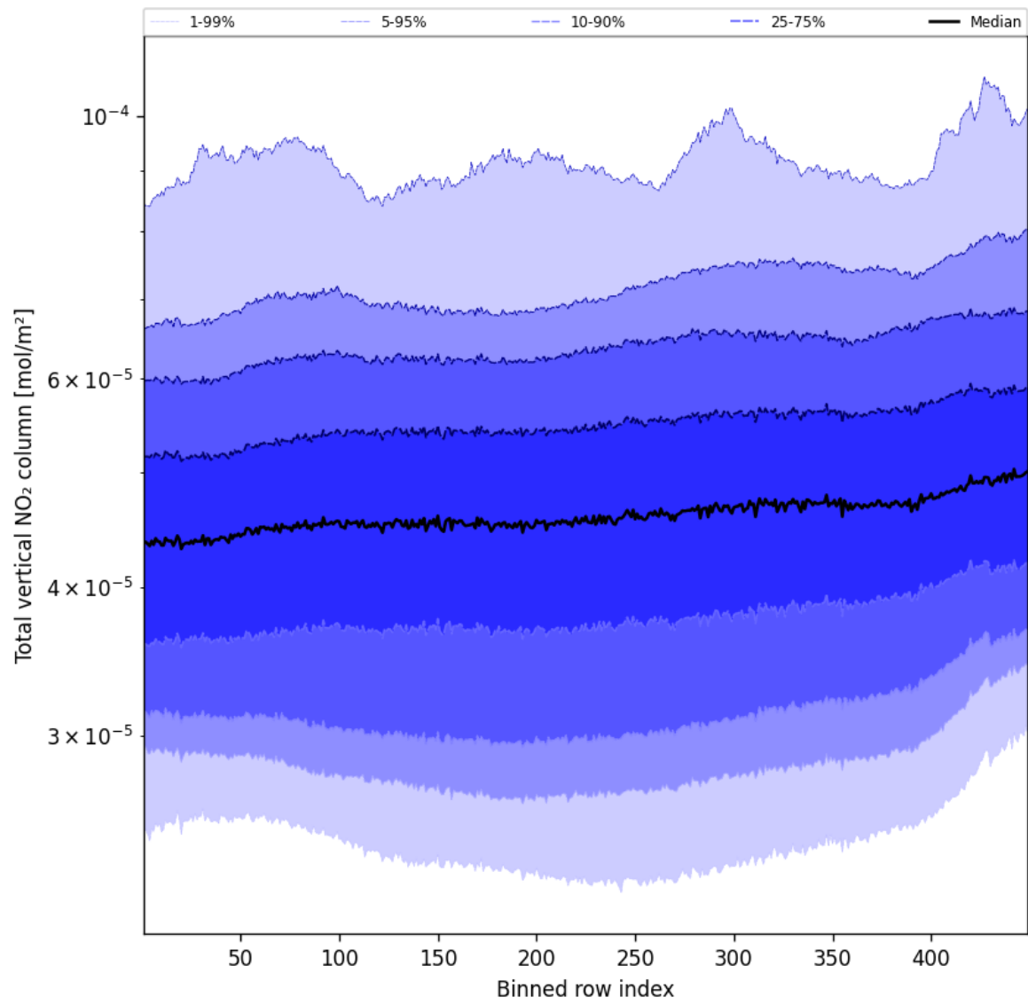
Figure 53: Along track statistics of “Total vertical NO 2 column” for 2025-10-08 to 2025-10-09
