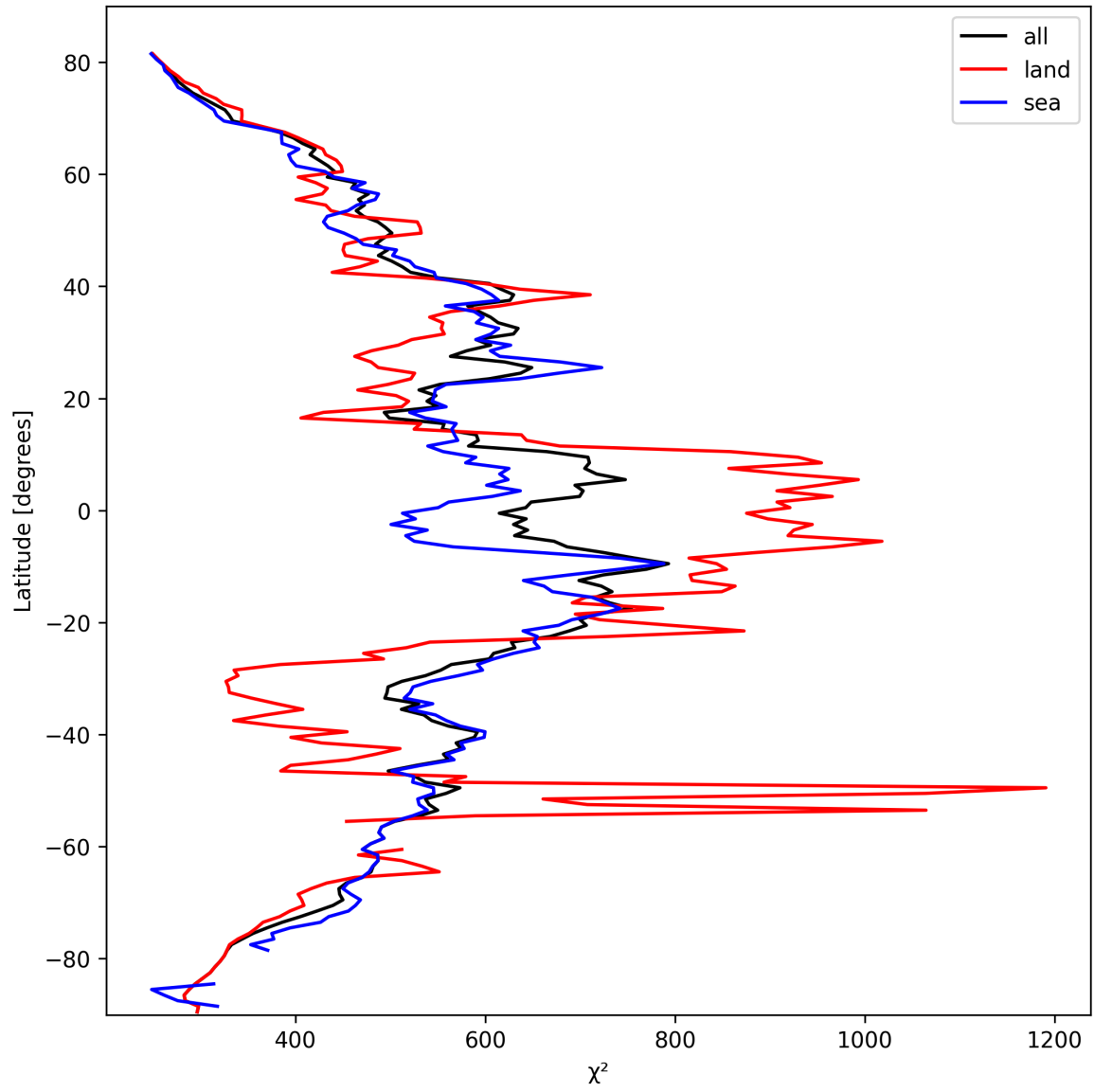
Figure 23: Zonal average of “ \chi^2 ” for 2025-10-08 to 2025-10-09.
