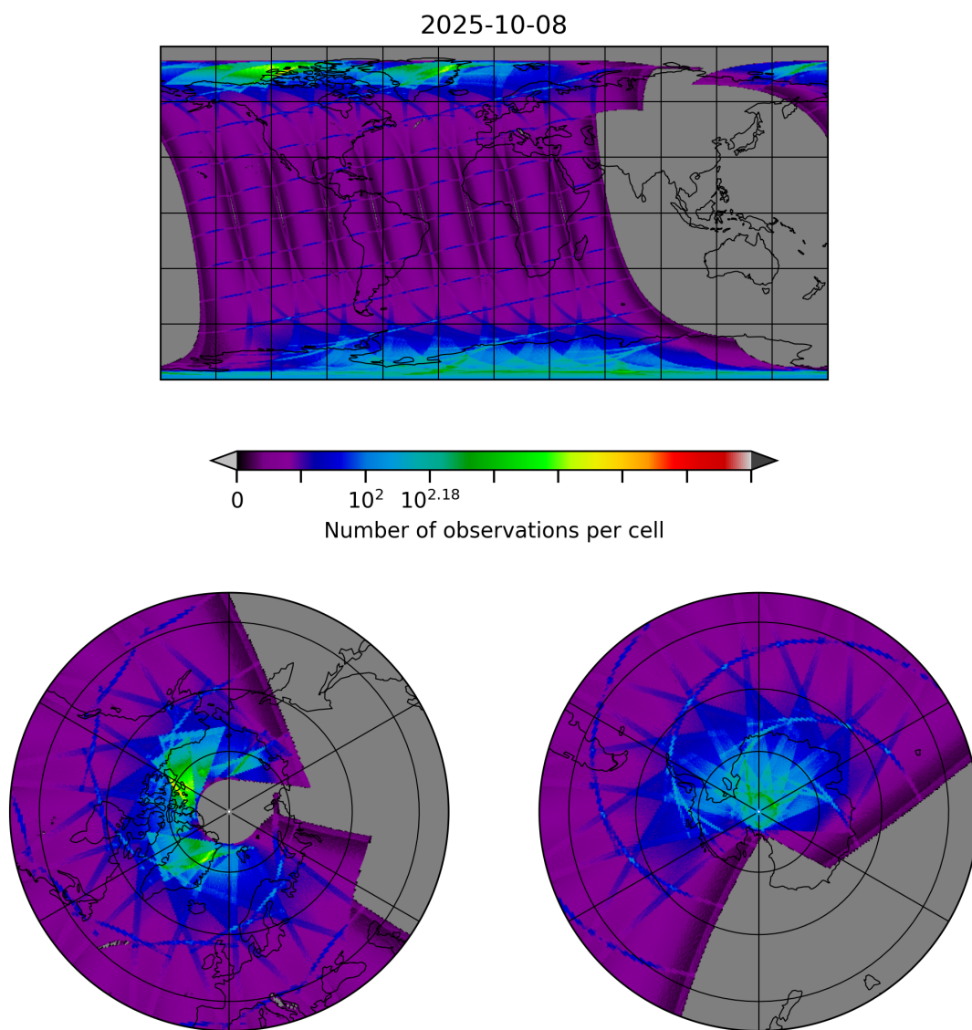
Figure 8: Map of the number of observations for 2025-10-08 to 2025-10-09
