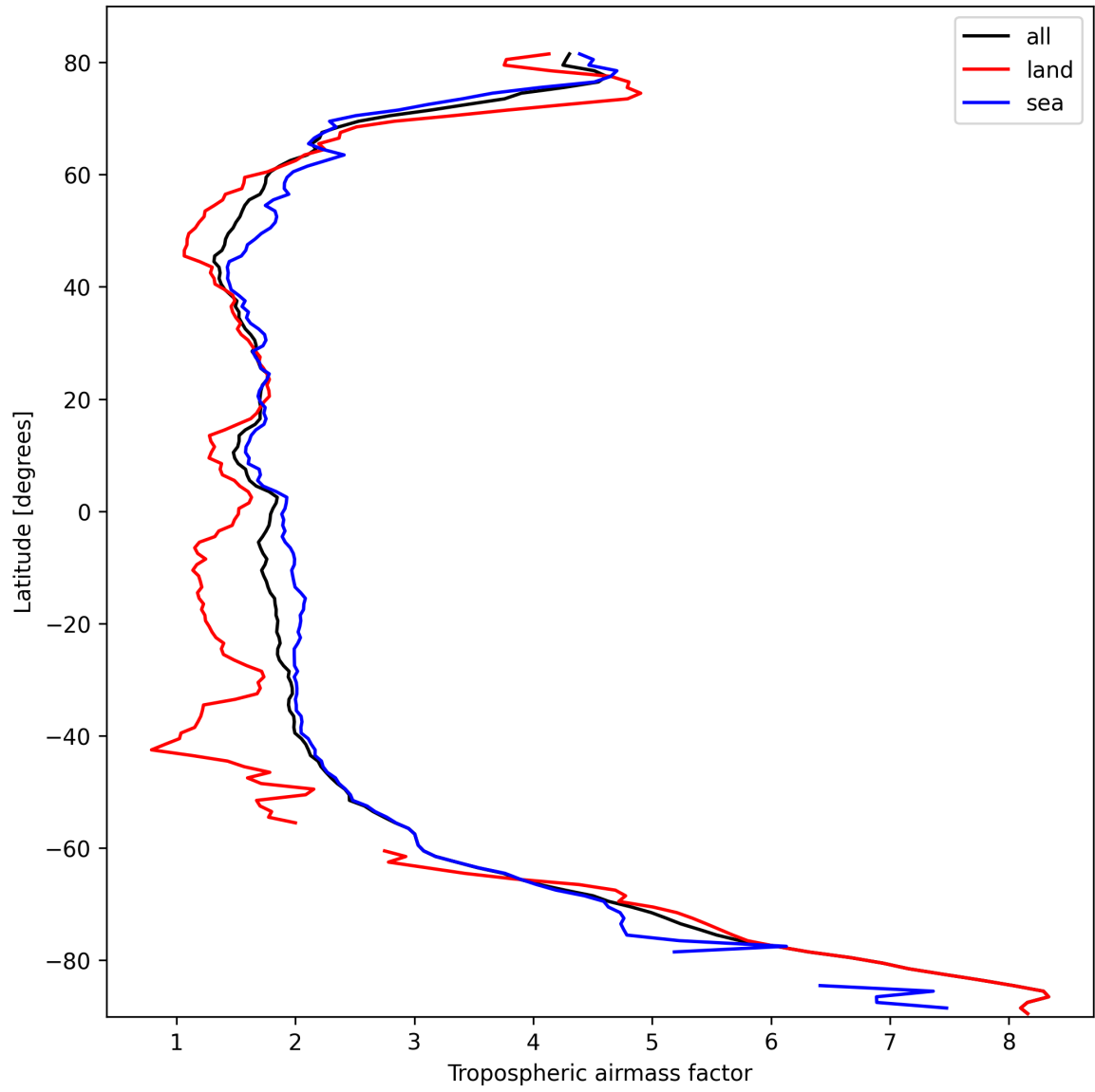
Figure 12: Zonal average of “Tropospheric airmass factor” for 2025-10-08 to 2025-10-09.
