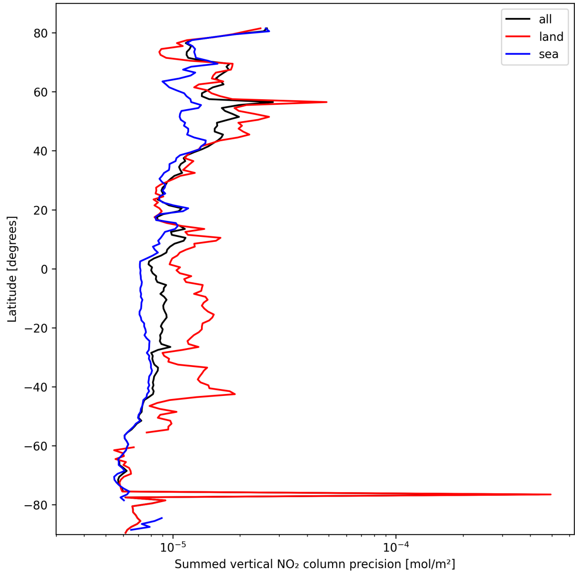
Figure 22: Zonal average of “Summed vertical NO 2 column precision” for 2025-10-08 to 2025-10-09.
