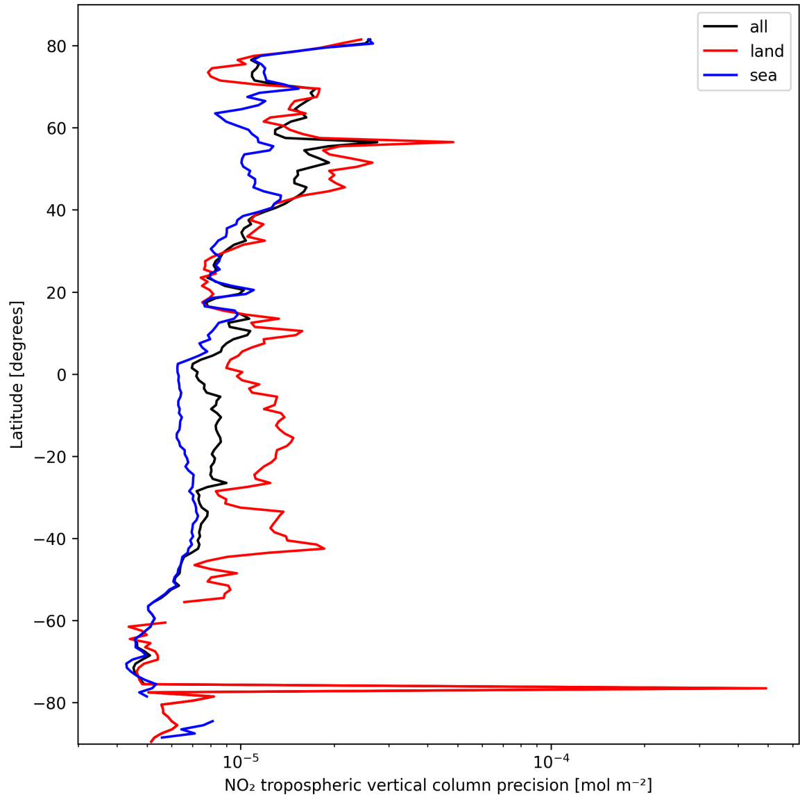
Figure 11: Zonal average of “NO 2 tropospheric vertical column precision” for 2025-10-08 to 2025-10-09.
