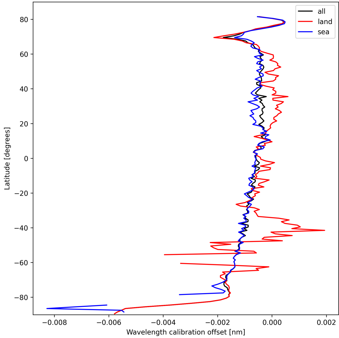
Figure 16: Zonal average of “Wavelength calibration offset” for 2025-10-08 to 2025-10-09.
