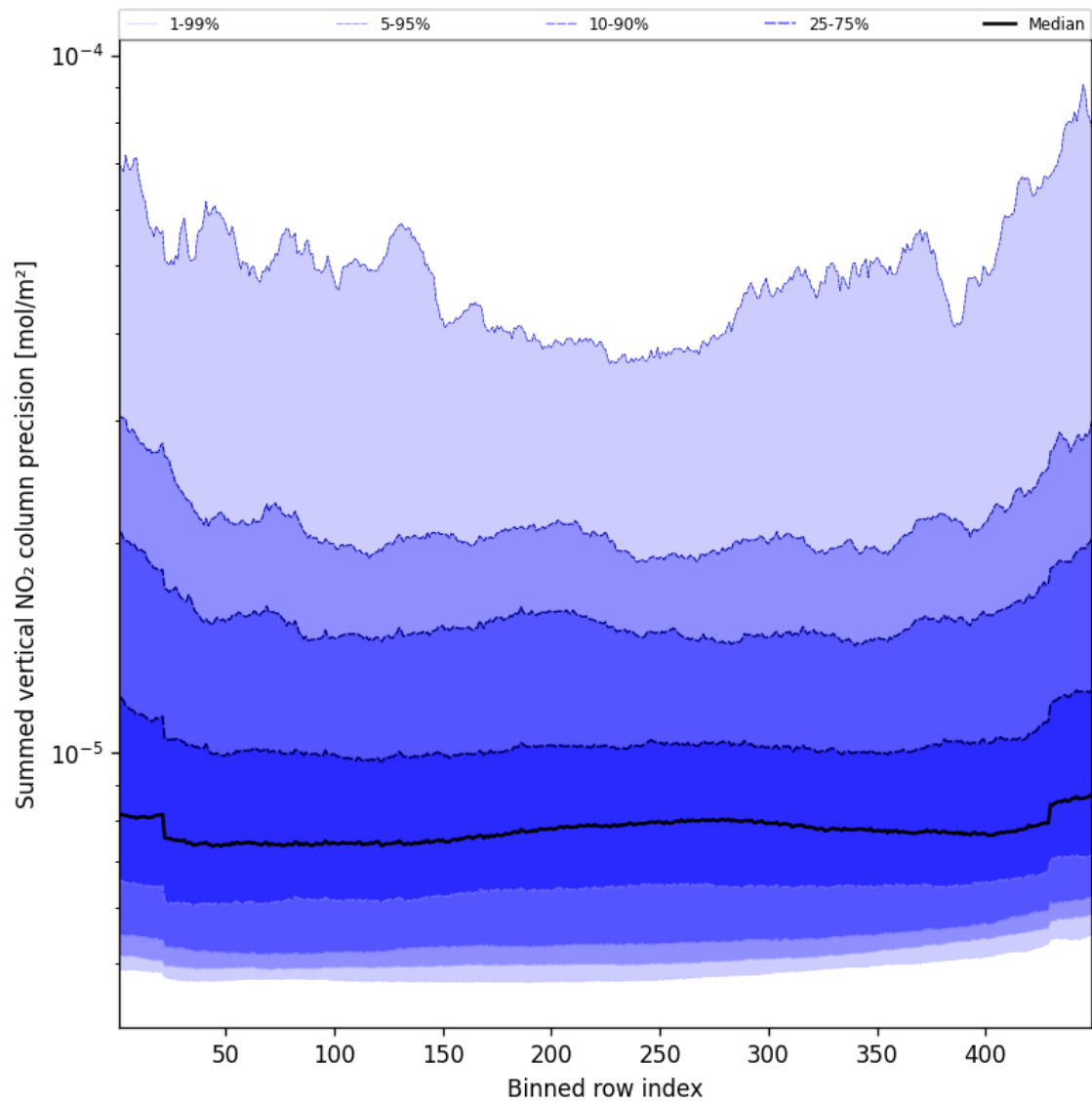
Figure 56: Along track statistics of “Summed vertical NO 2 column precision” for 2025-10-08 to 2025-10-09
