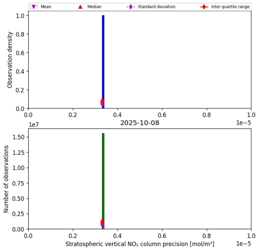
Figure 35: Histogram of “Stratospheric vertical NO 2 column precision” for 2025-10-08 to 2025-10-09
