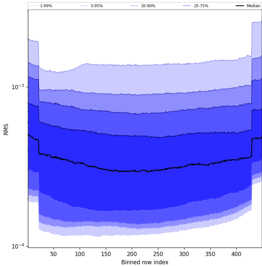
Figure 58: Along track statistics of “RMS” for 2025-10-08 to 2025-10-09
