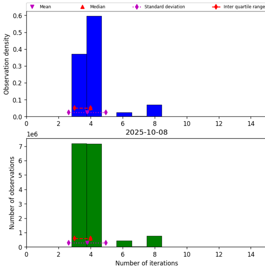
Figure 32: Histogram of “Number of iterations” for 2025-10-08 to 2025-10-09
