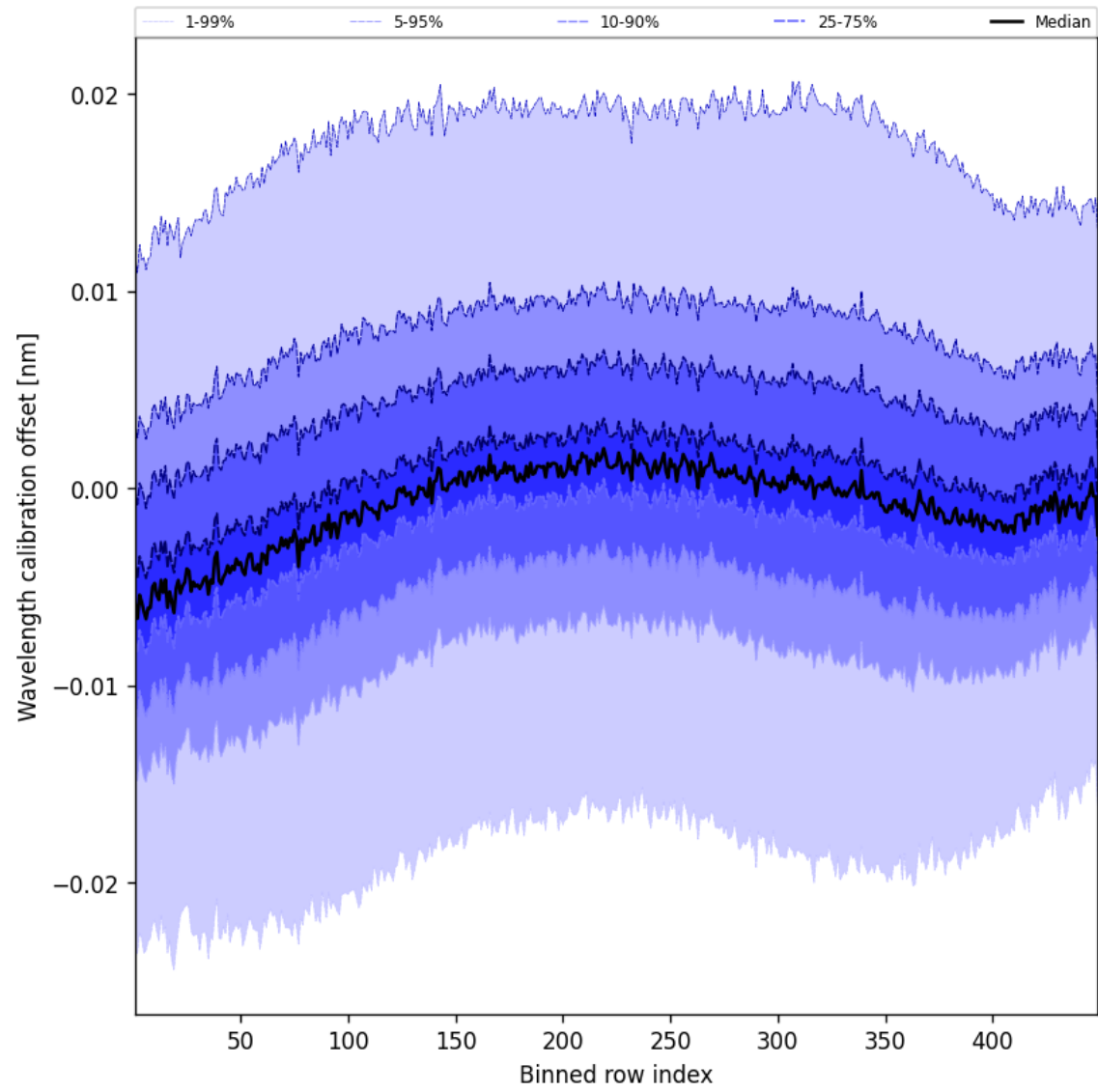
Figure 50: Along track statistics of “Wavelength calibration offset” for 2025-10-08 to 2025-10-09
