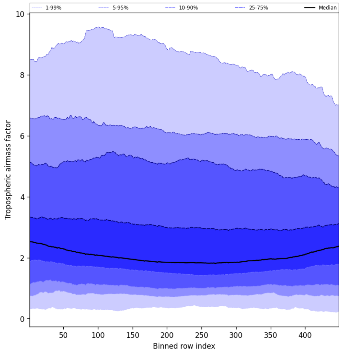
Figure 46: Along track statistics of “Tropospheric airmass factor” for 2025-10-08 to 2025-10-09
