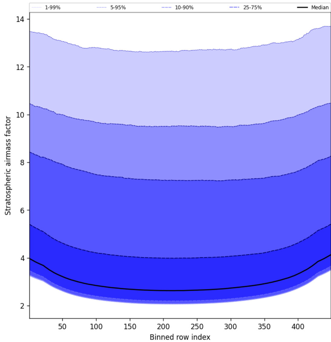
Figure 59: Along track statistics of “Stratospheric airmass factor” for 2025-10-08 to 2025-10-09
