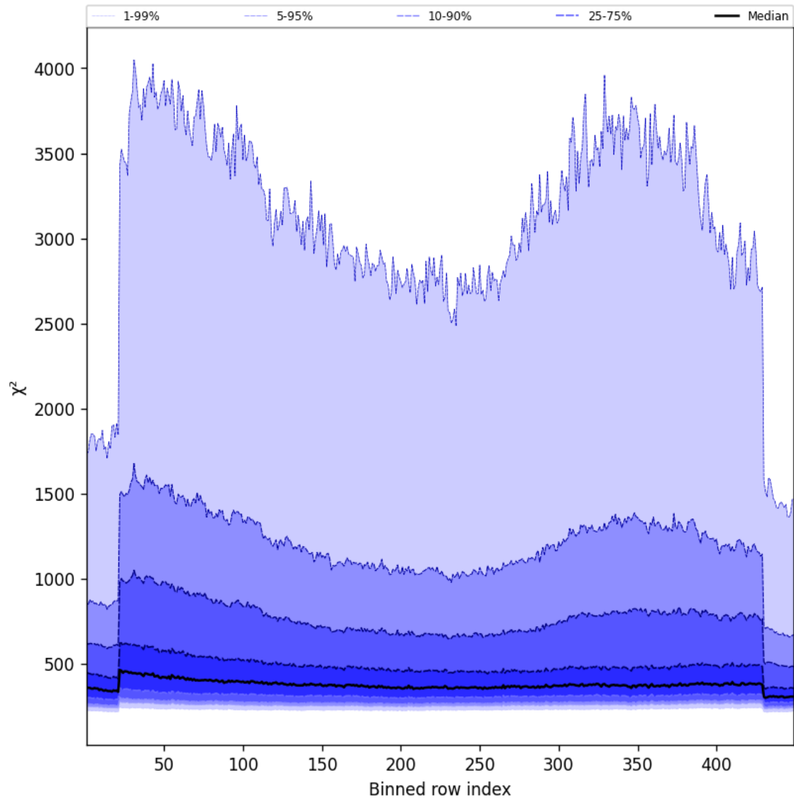
Figure 57: Along track statistics of “ \chi^2 ” for 2025-10-08 to 2025-10-09
