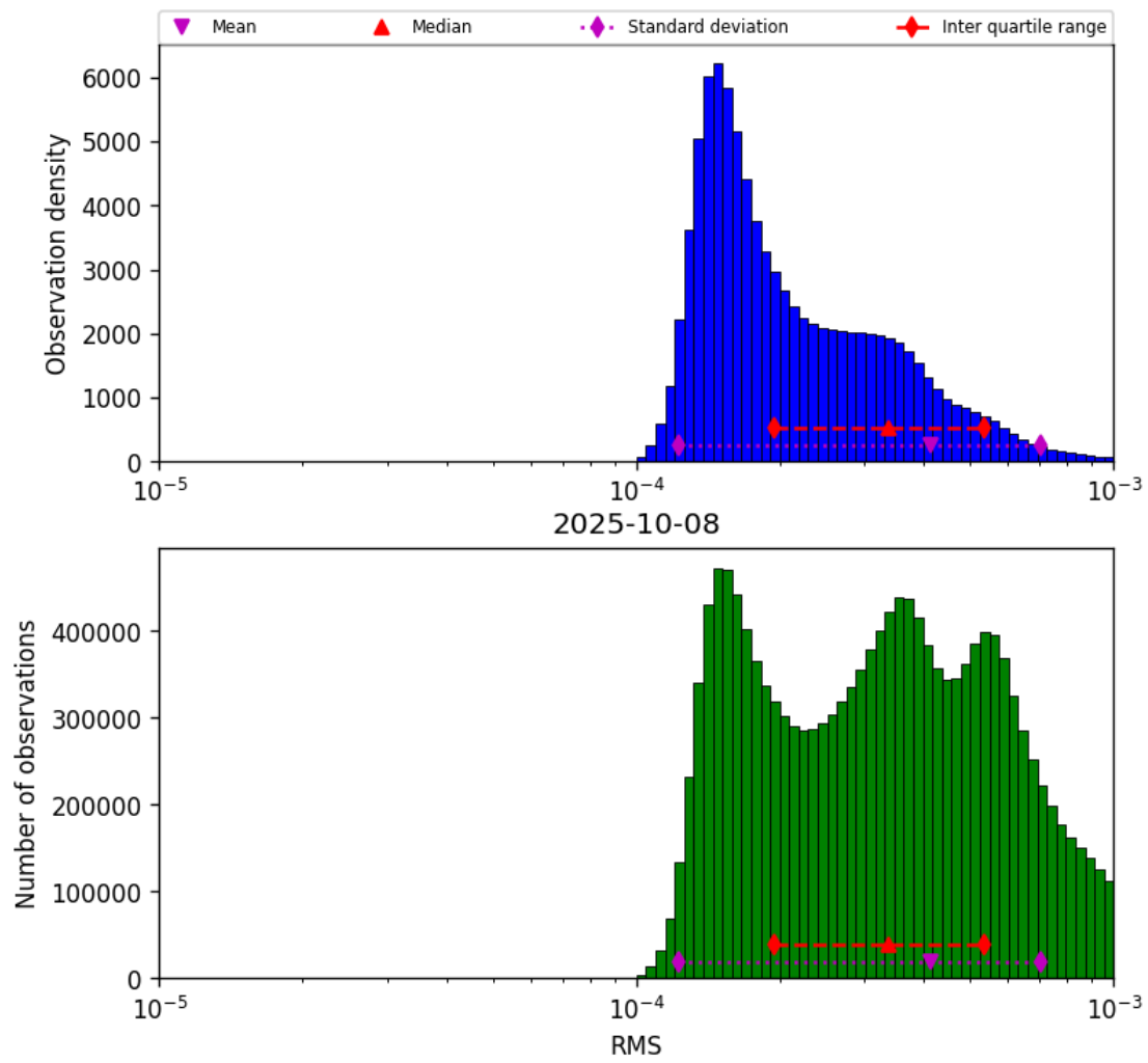
Figure 41: Histogram of “RMS” for 2025-10-08 to 2025-10-09
