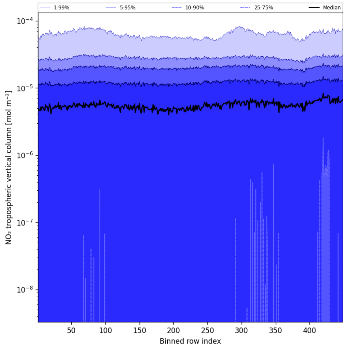
Figure 44: Along track statistics of “NO 2 tropospheric vertical column” for 2025-10-08 to 2025-10-09
