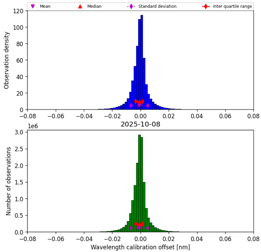
Figure 33: Histogram of “Wavelength calibration offset” for 2025-10-08 to 2025-10-09
