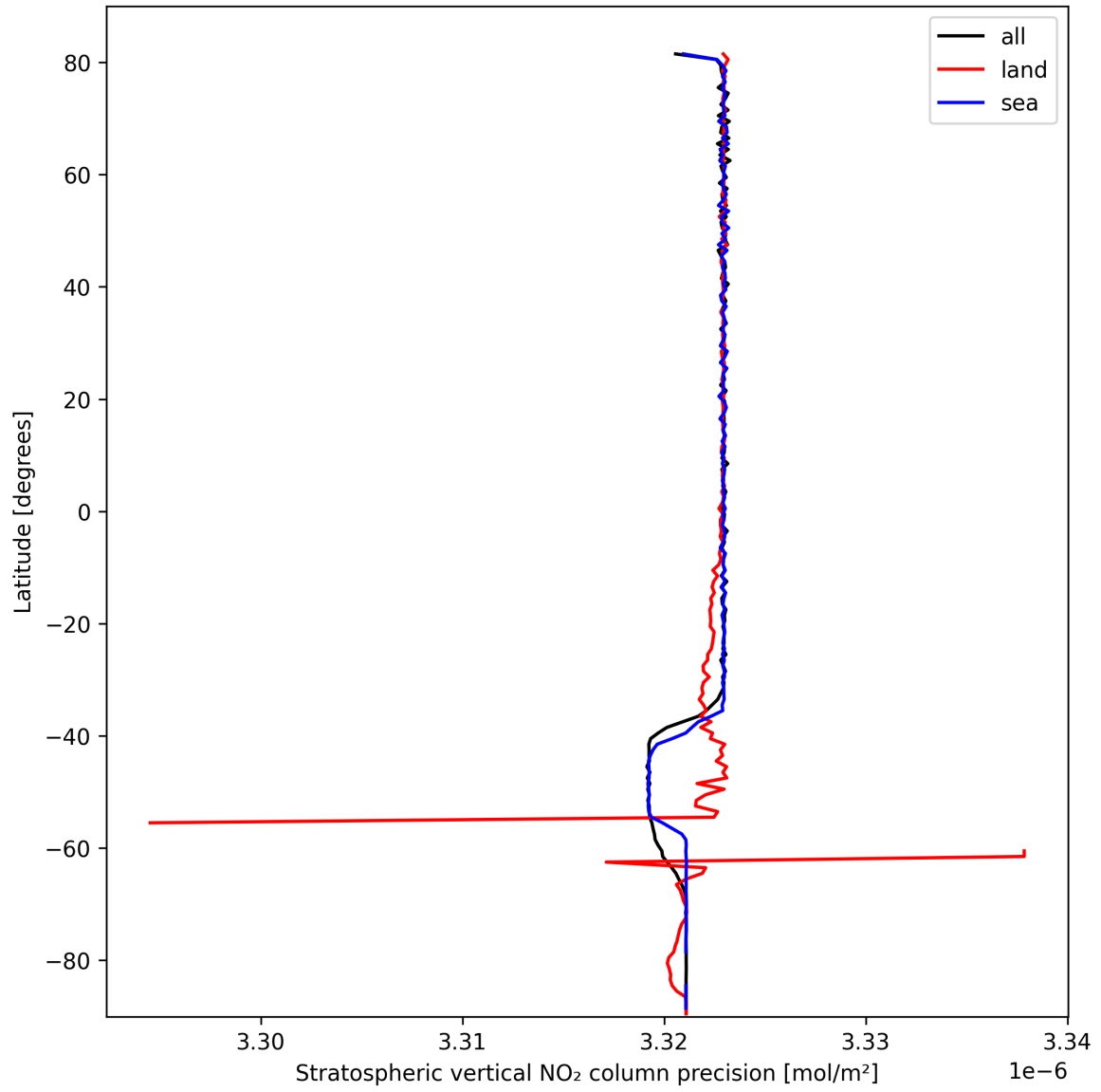
Figure 18: Zonal average of “Stratospheric vertical NO 2 column precision” for 2025-10-08 to 2025-10-09.
