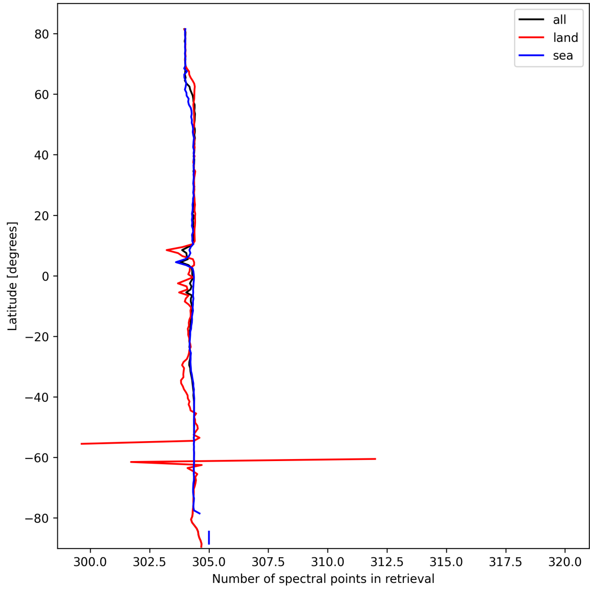
Figure 14: Zonal average of “Number of spectral points in retrieval” for 2025-10-08 to 2025-10-09.
