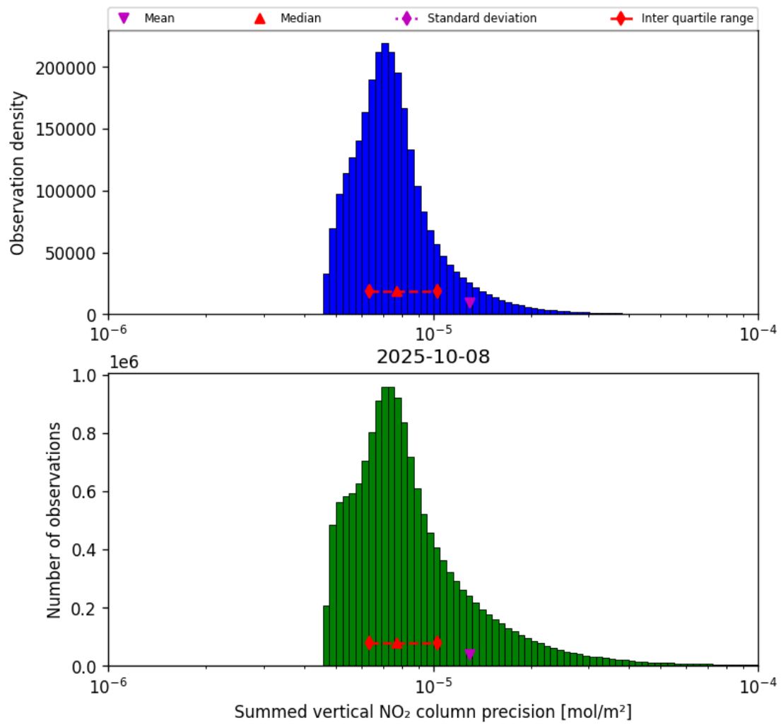
Figure 39: Histogram of "Summed vertical NO 2 column precision" for 2025-10-08 to 2025-10-09
