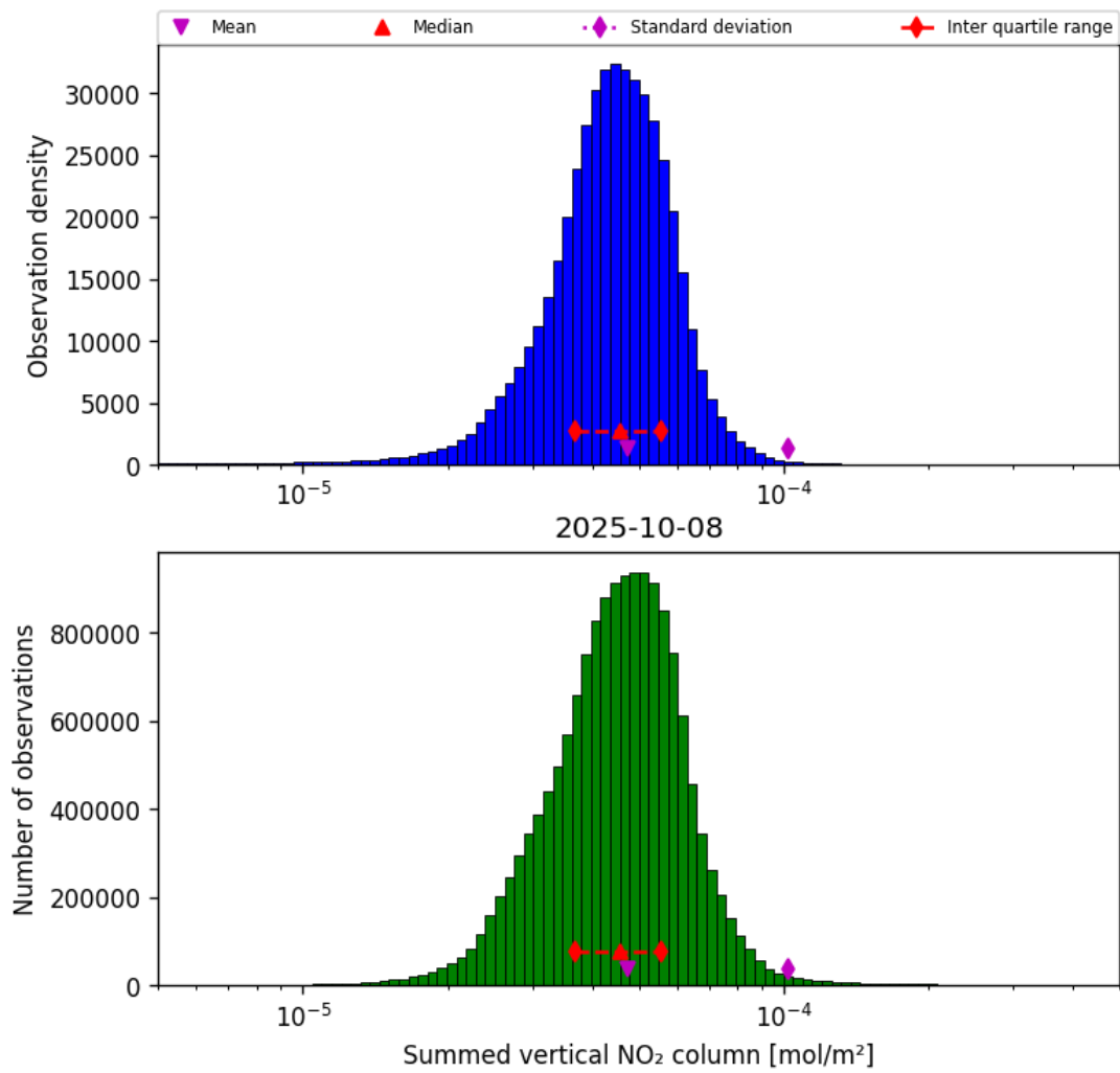
Figure 38: Histogram of “Summed vertical NO 2 column” for 2025-10-08 to 2025-10-09
