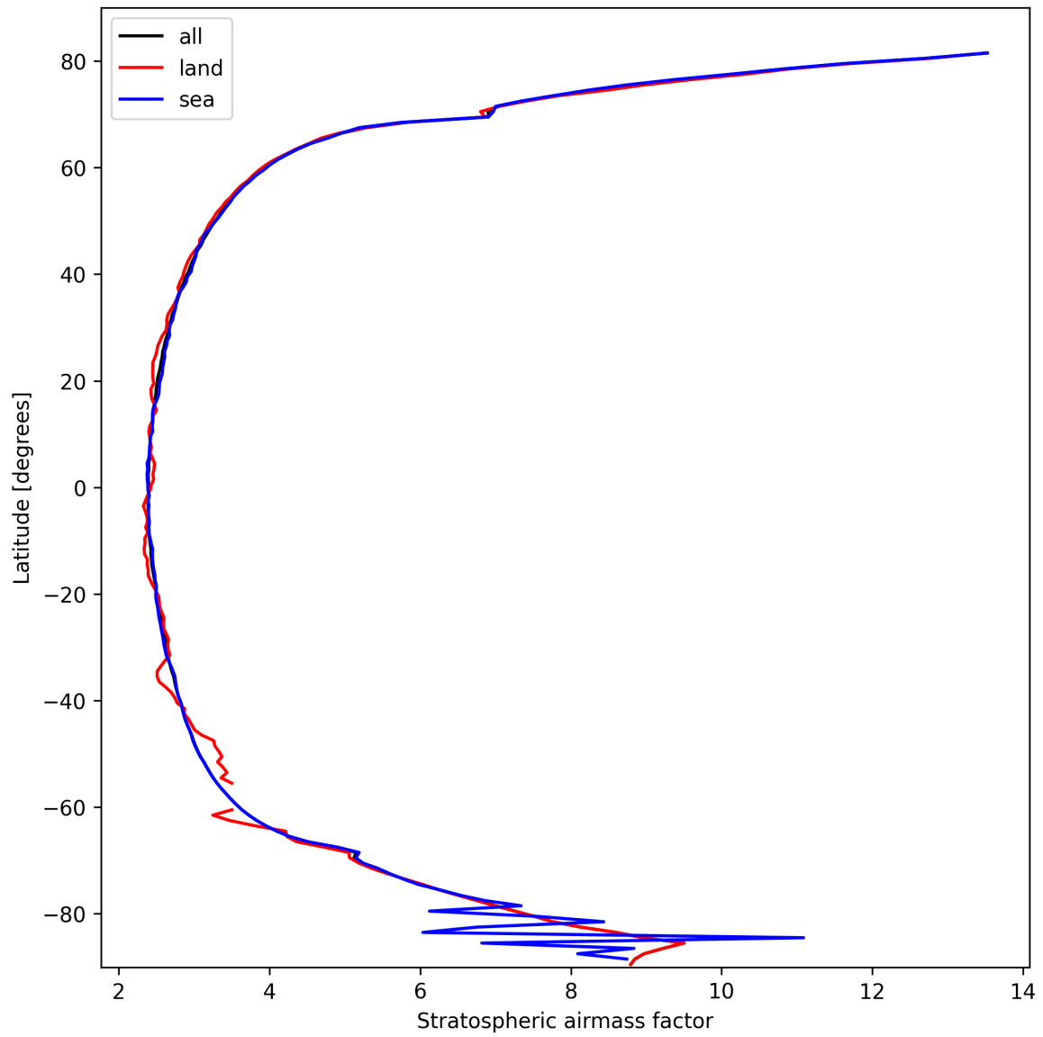
Figure 25: Zonal average of “Stratospheric airmass factor” for 2025-10-09 to 2025-10-09.
