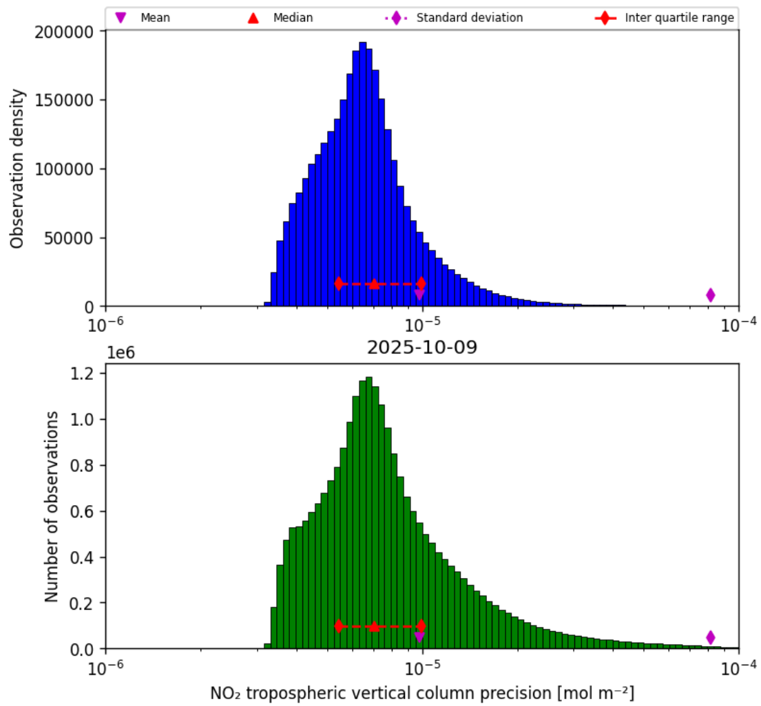
Figure 28: Histogram of "NO 2 tropospheric vertical column precision" for 2025-10-09 to 2025-10-09
