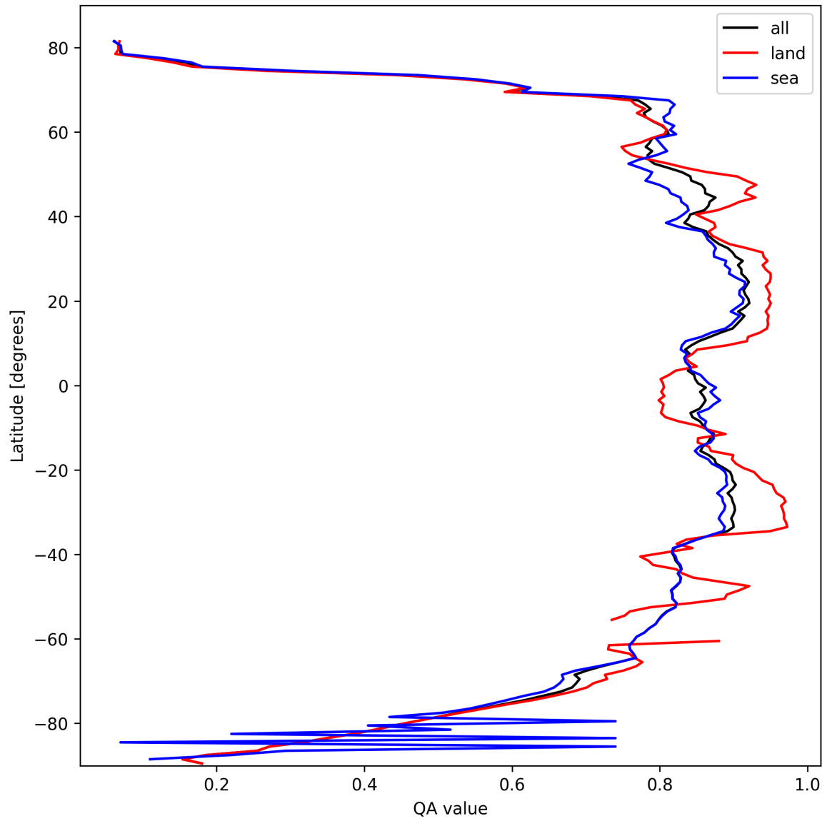
Figure 9: Zonal average of “QA value” for 2025-10-09 to 2025-10-09.
