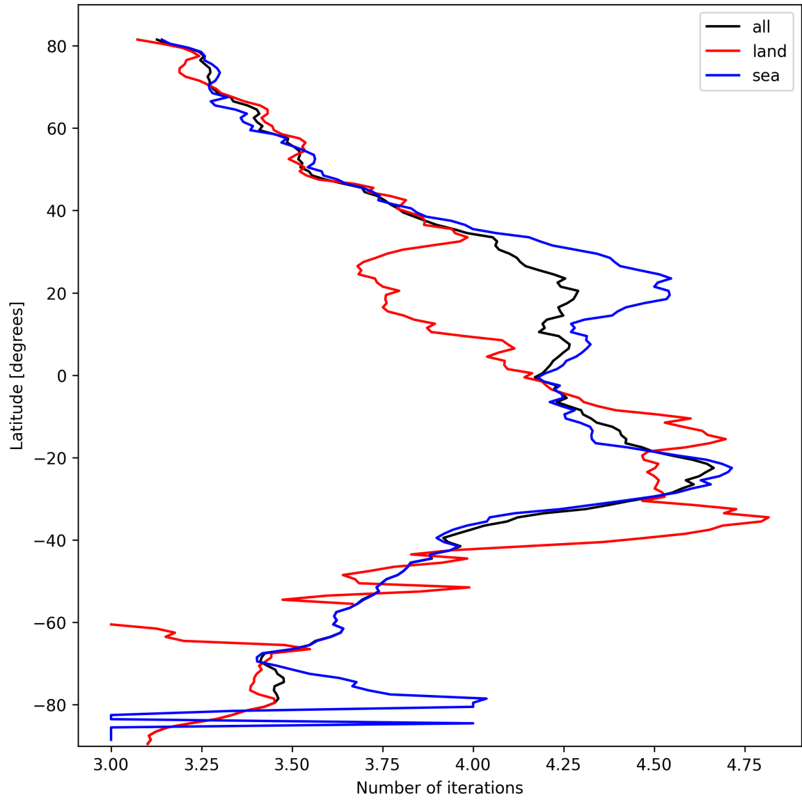
Figure 15: Zonal average of “Number of iterations” for 2025-10-09 to 2025-10-09.
