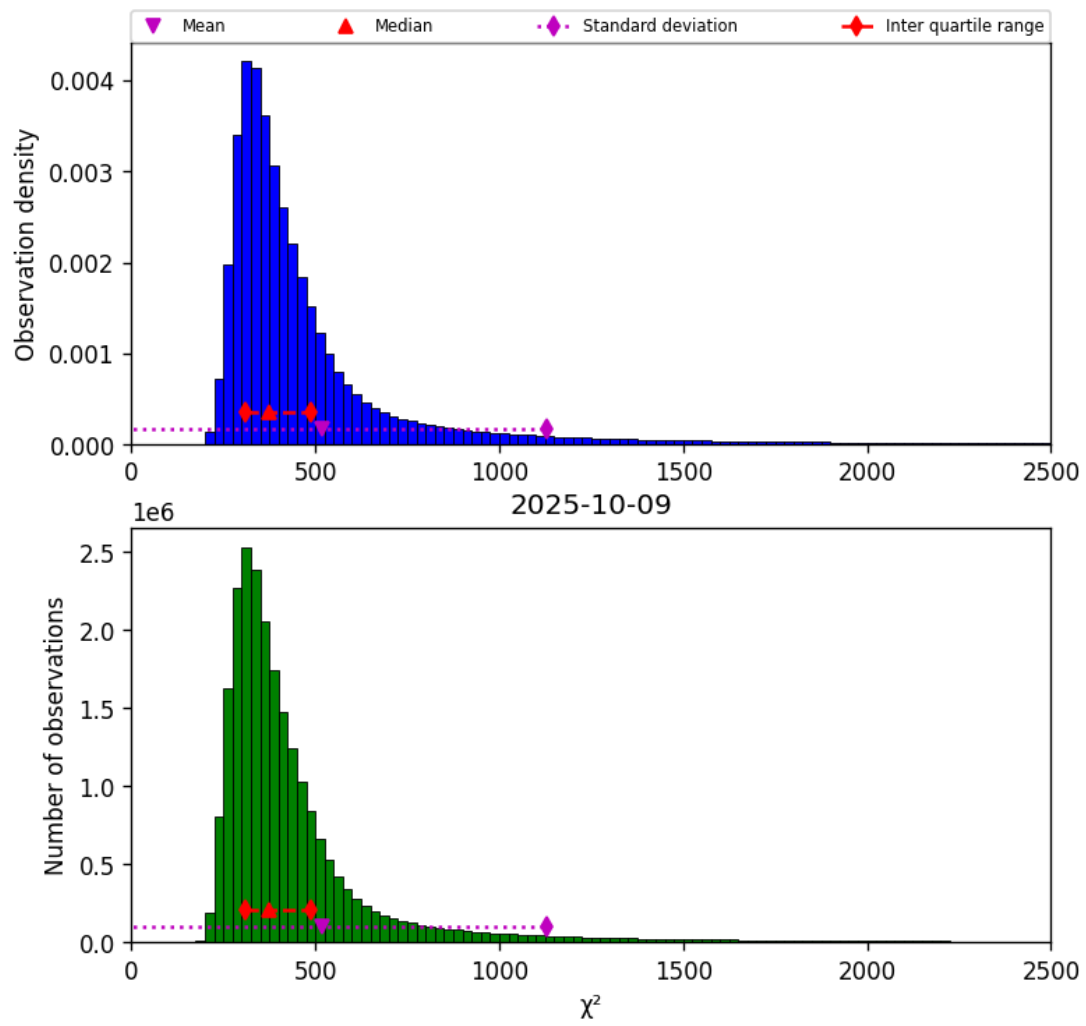
Figure 40: Histogram of “ \chi^2 ” for 2025-10-09 to 2025-10-09
