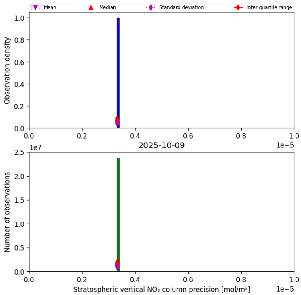
Figure 35: Histogram of “Stratospheric vertical NO 2 column precision” for 2025-10-09 to 2025-10-09
