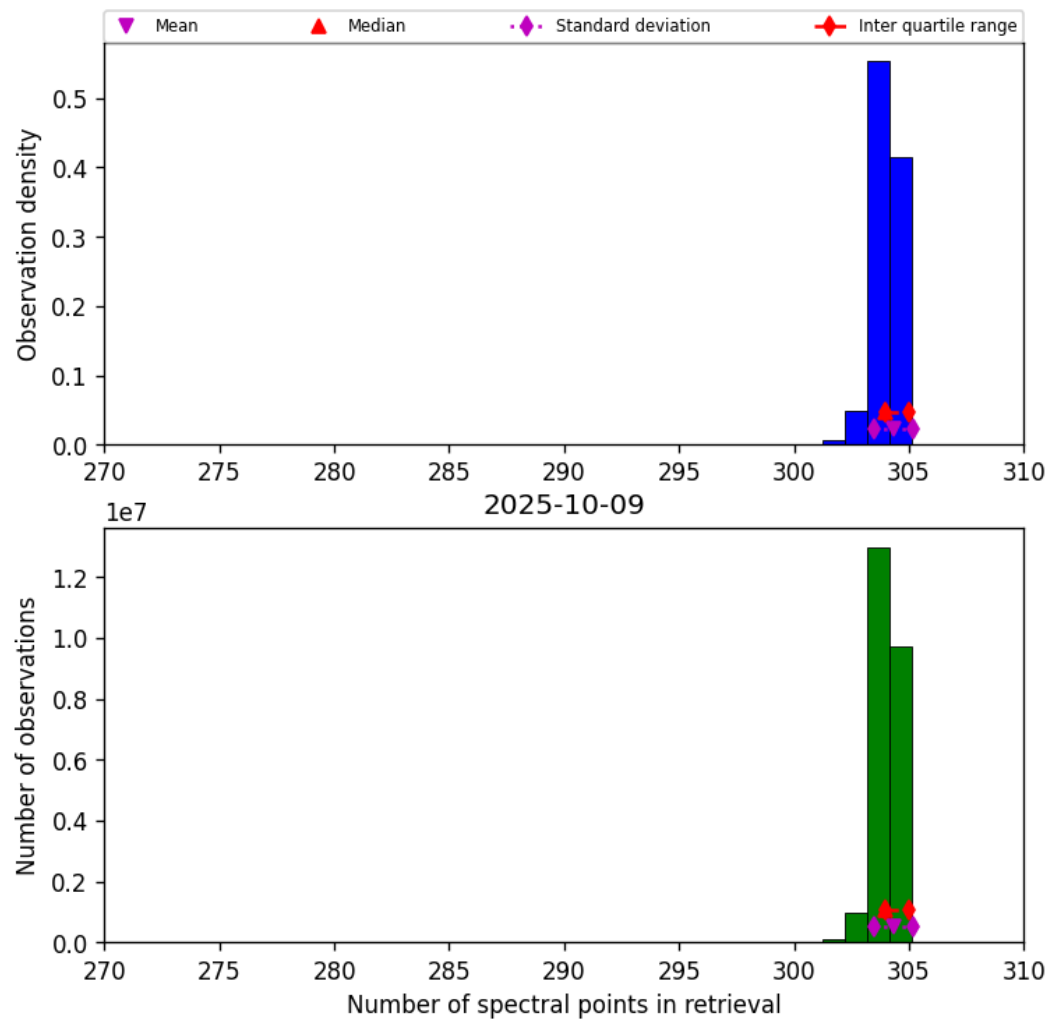
Figure 31: Histogram of “Number of spectral points in retrieval” for 2025-10-09 to 2025-10-09
