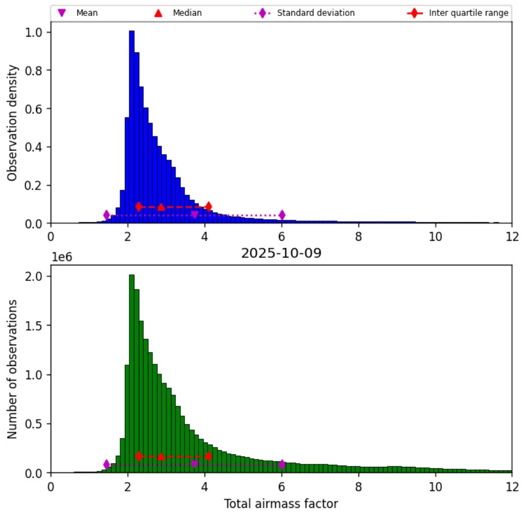
Figure 30: Histogram of “Total airmass factor” for 2025-10-09 to 2025-10-09
