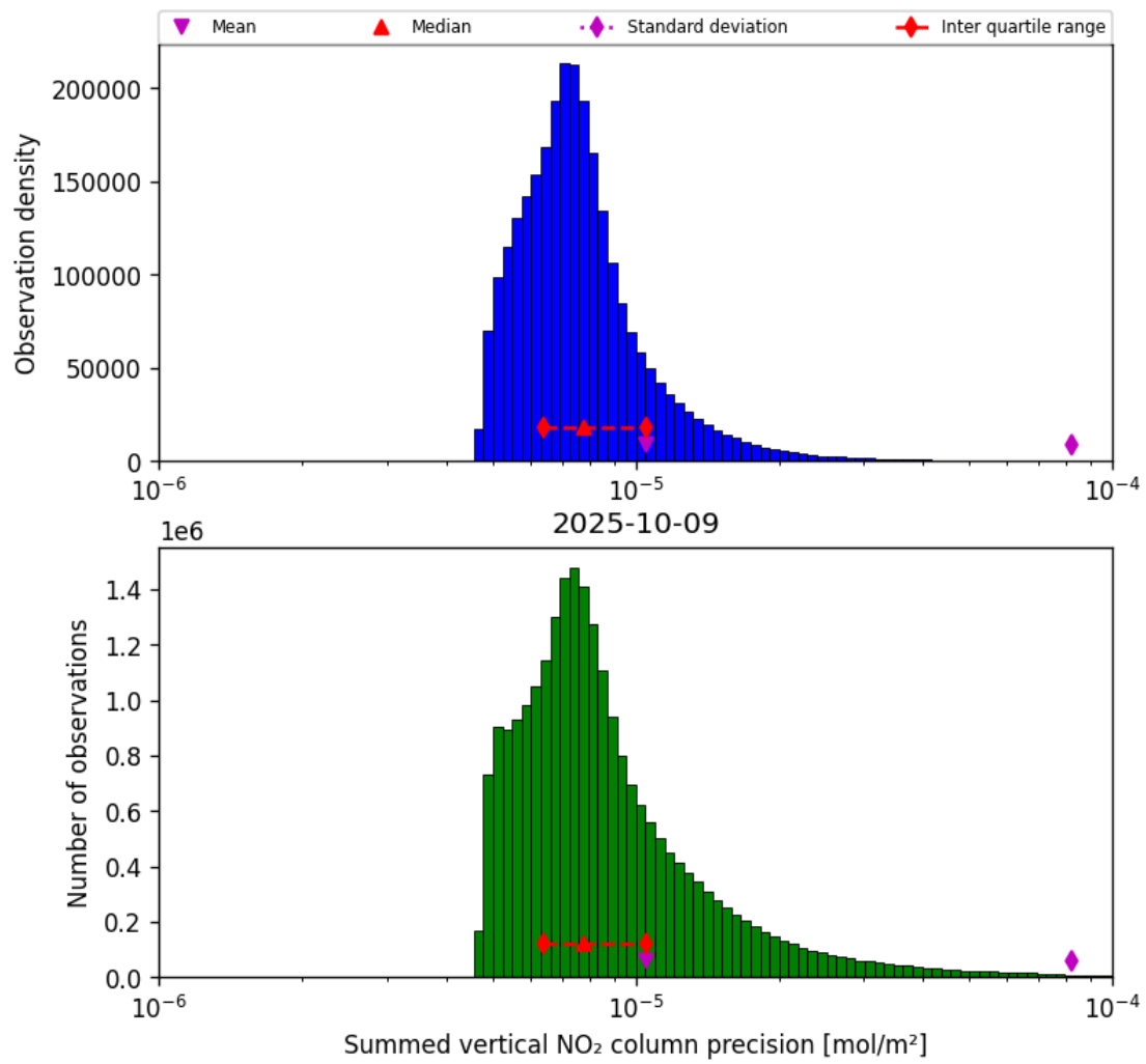
Figure 39: Histogram of "Summed vertical NO 2 column precision" for 2025-10-09 to 2025-10-09
