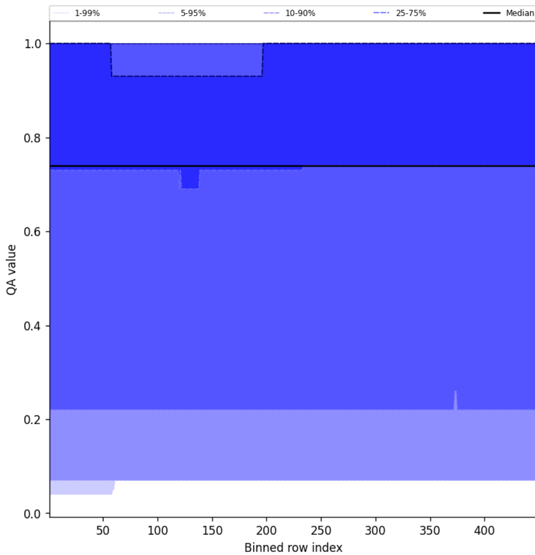
Figure 43: Along track statistics of “QA value” for 2025-10-09 to 2025-10-09
