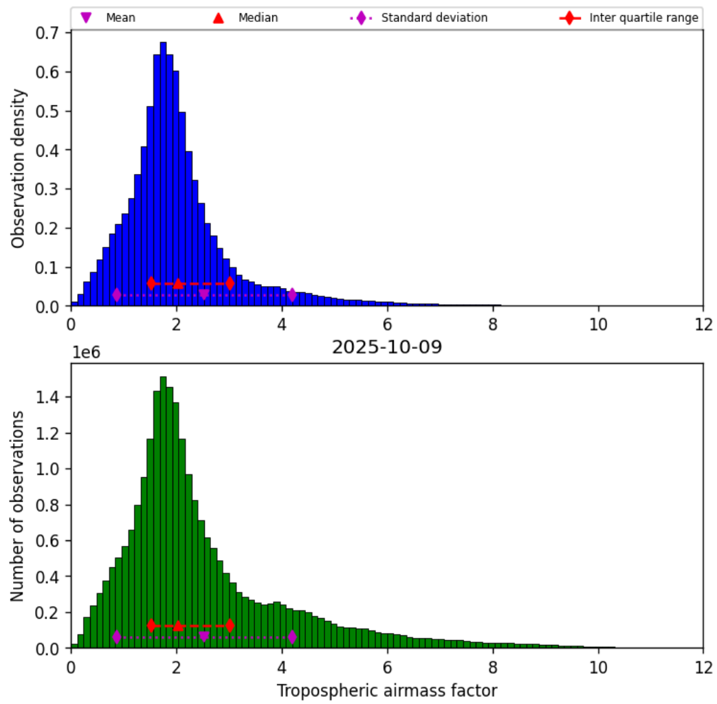
Figure 29: Histogram of “Tropospheric airmass factor” for 2025-10-09 to 2025-10-09
