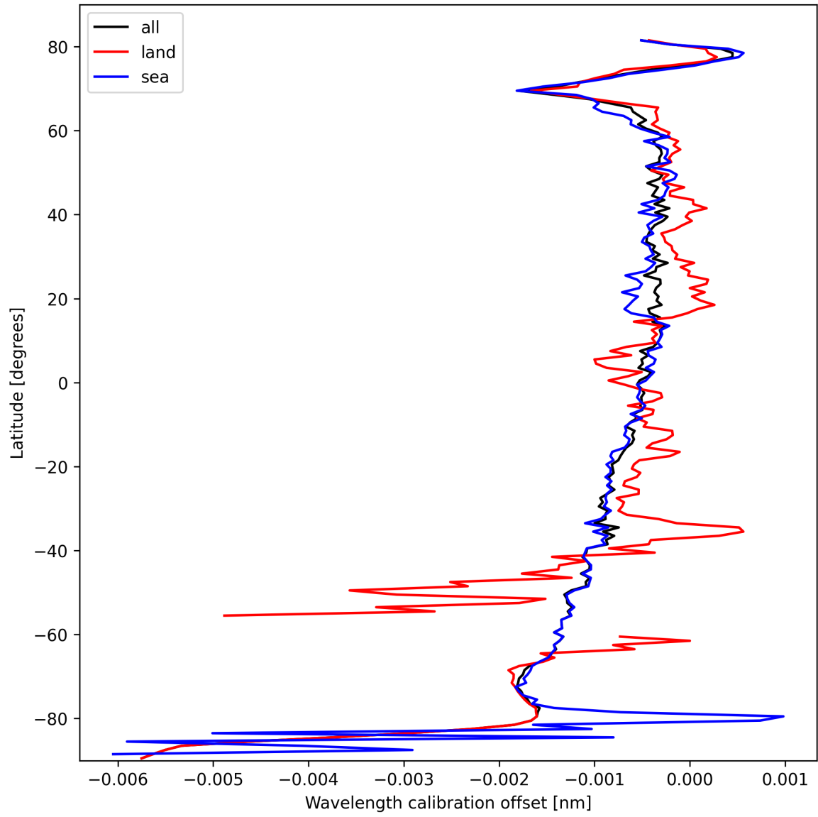
Figure 16: Zonal average of “Wavelength calibration offset” for 2025-10-09 to 2025-10-09.
