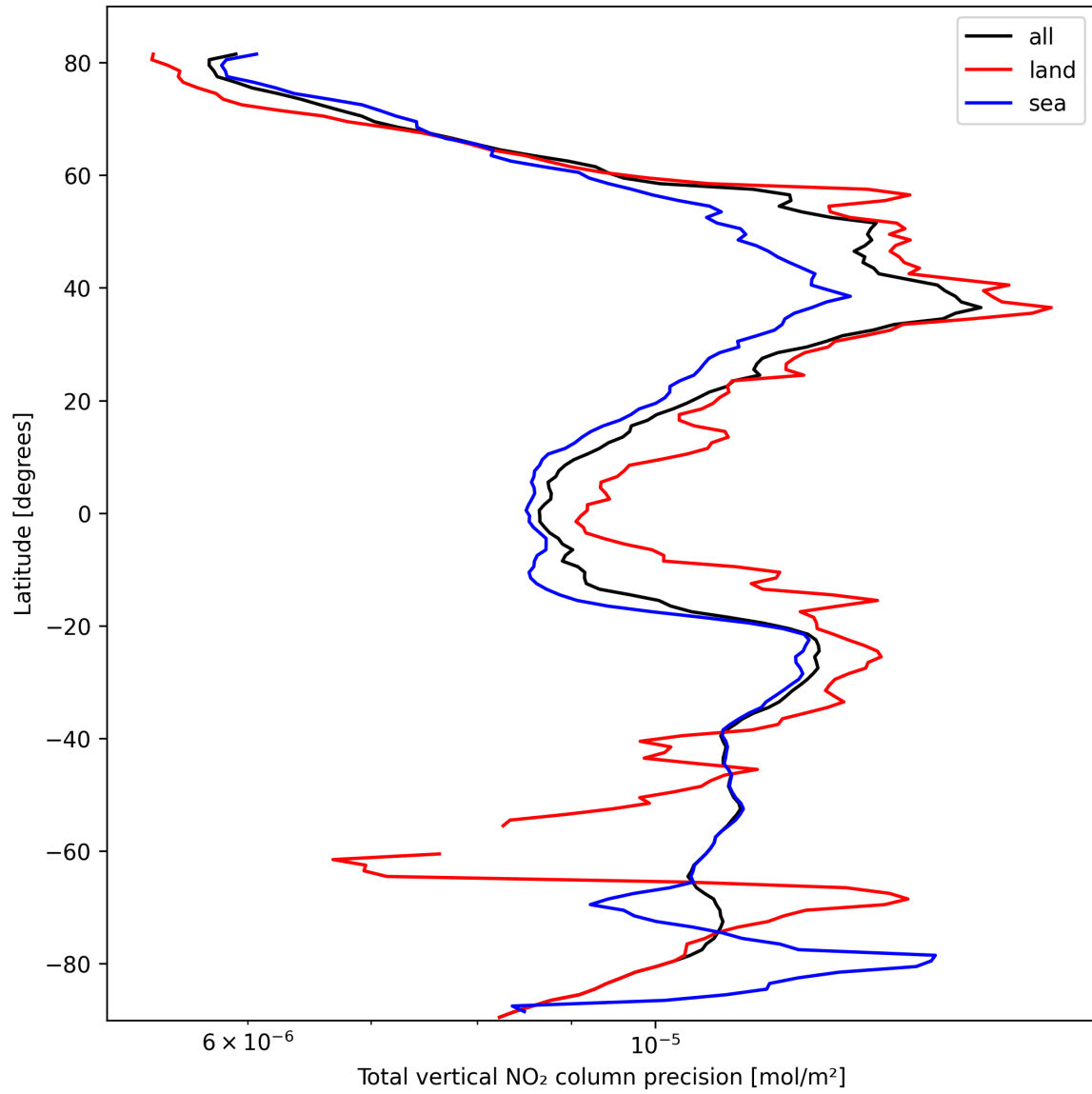
Figure 20: Zonal average of “Total vertical NO 2 column precision” for 2025-10-09 to 2025-10-09.
