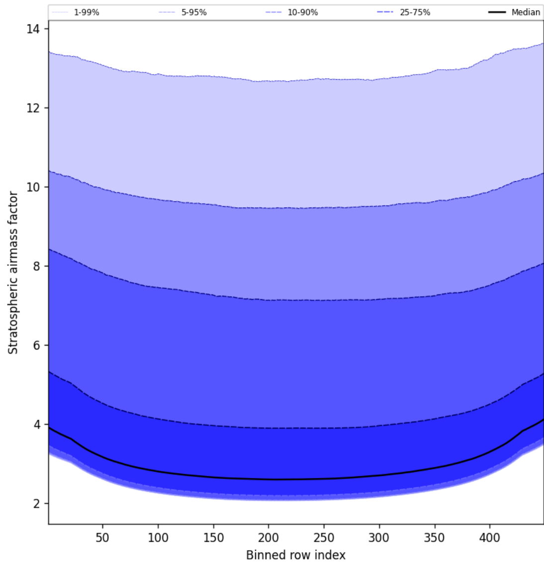
Figure 59: Along track statistics of “Stratospheric airmass factor” for 2025-10-09 to 2025-10-09
