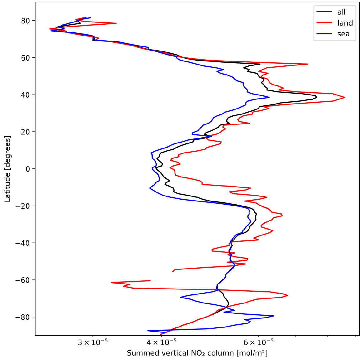
Figure 21: Zonal average of “Summed vertical NO 2 column” for 2025-10-09 to 2025-10-09.
