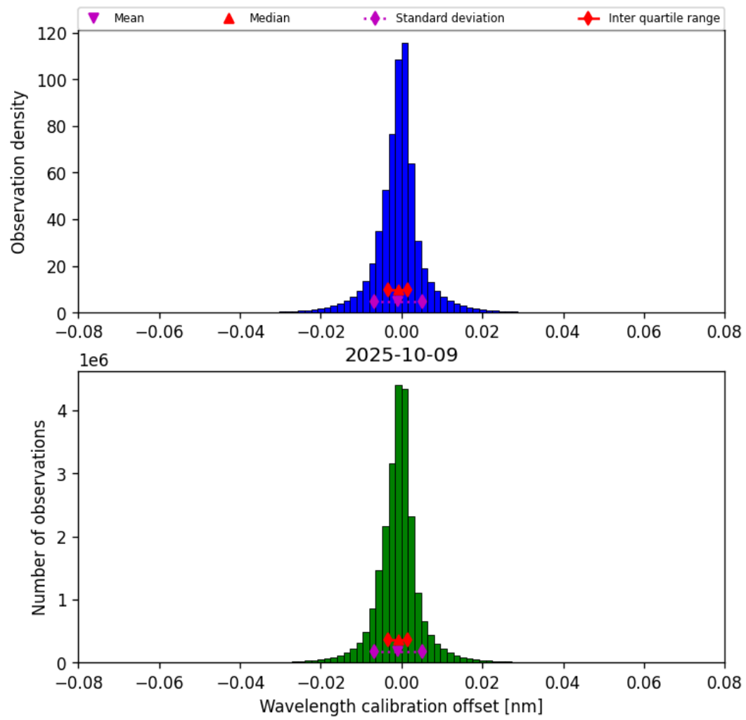
Figure 33: Histogram of “Wavelength calibration offset” for 2025-10-09 to 2025-10-09
