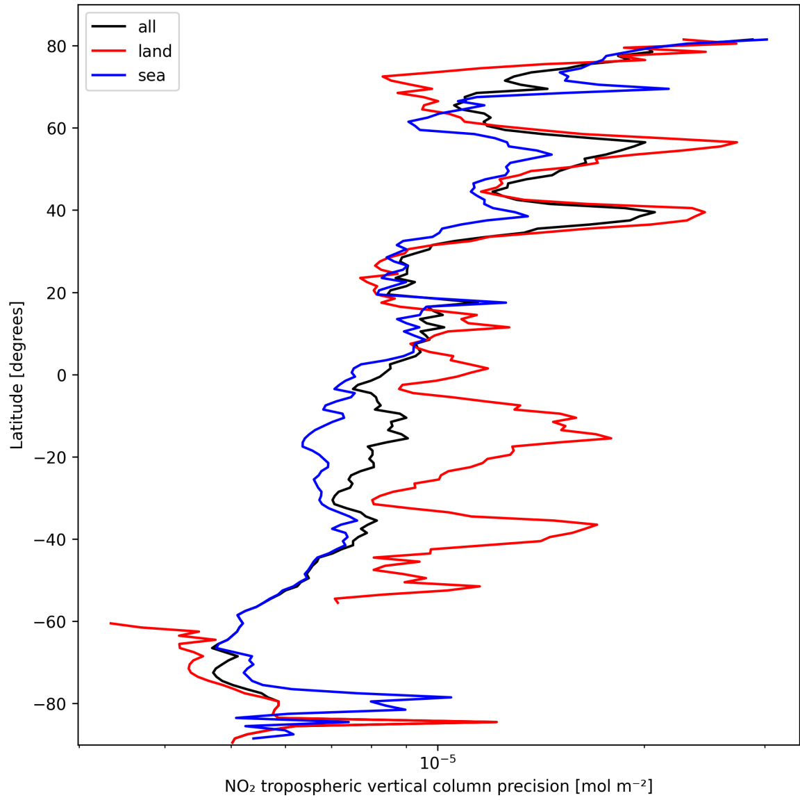
Figure 11: Zonal average of “NO 2 tropospheric vertical column precision” for 2025-10-09 to 2025-10-09.
