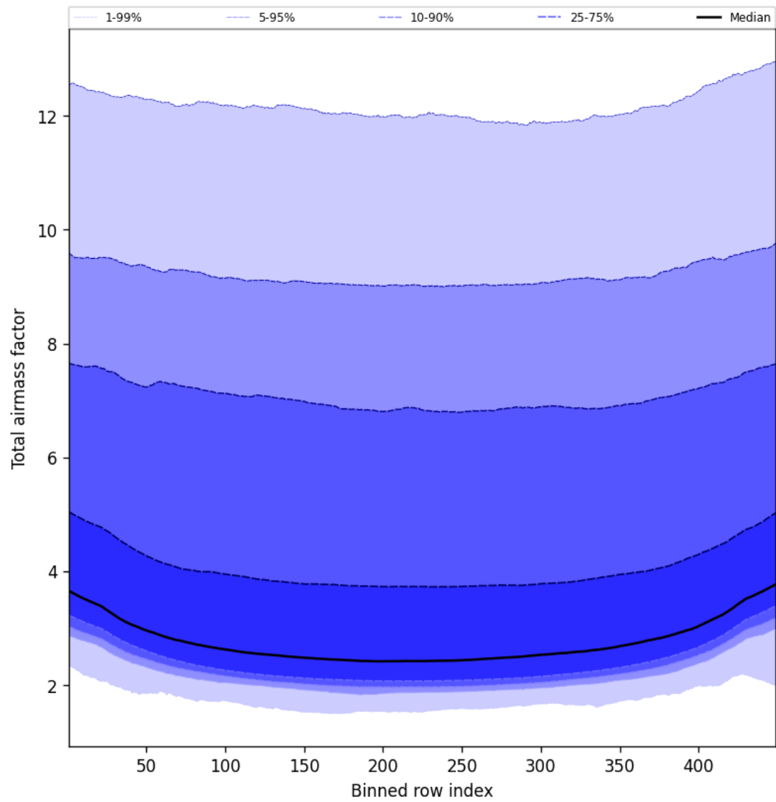
Figure 47: Along track statistics of “Total airmass factor” for 2025-10-09 to 2025-10-09
