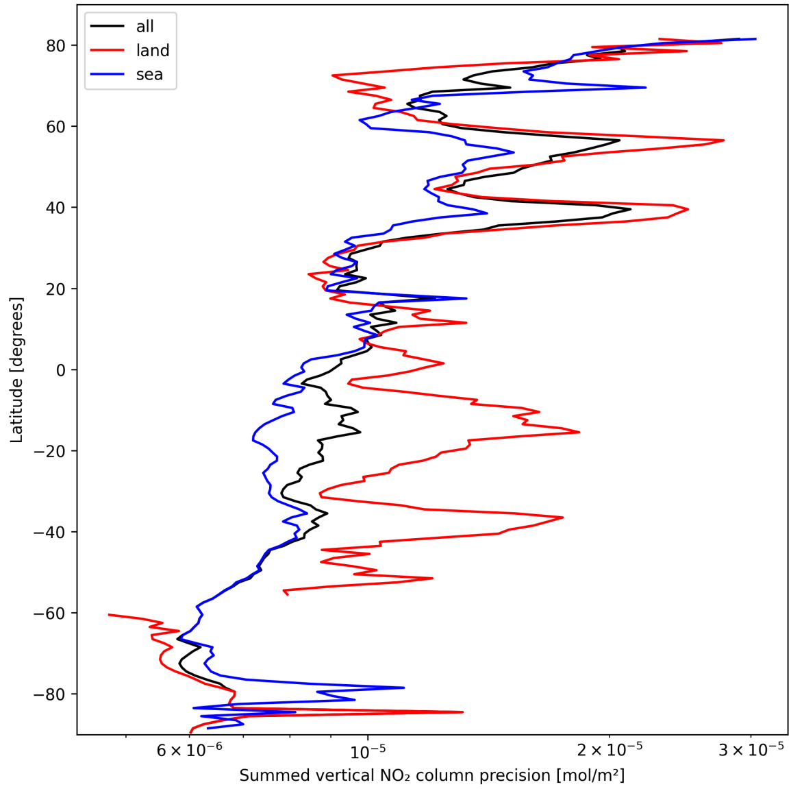
Figure 22: Zonal average of “Summed vertical NO 2 column precision” for 2025-10-09 to 2025-10-09.
