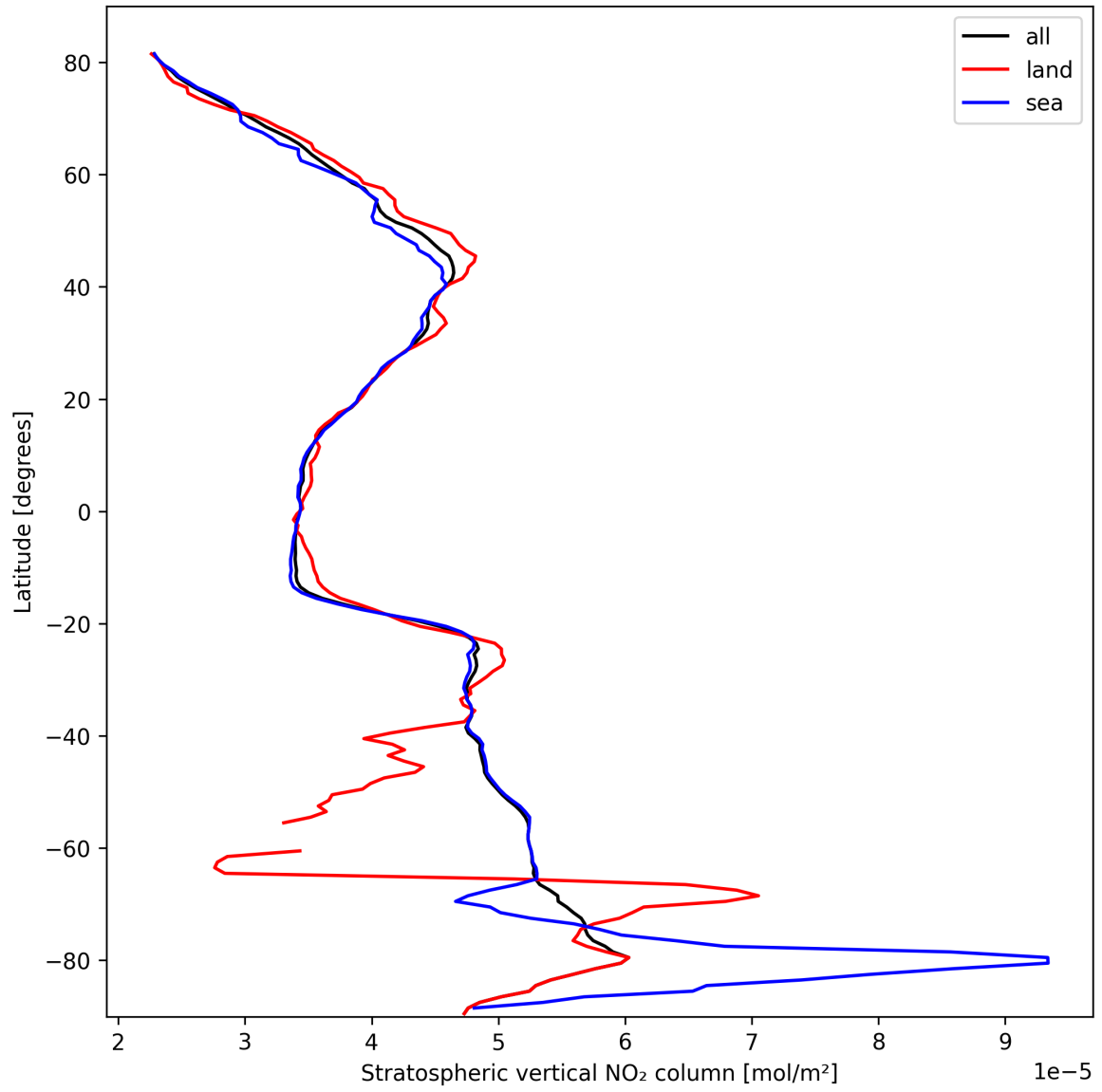
Figure 17: Zonal average of “Stratospheric vertical NO 2 column” for 2025-10-09 to 2025-10-09.
