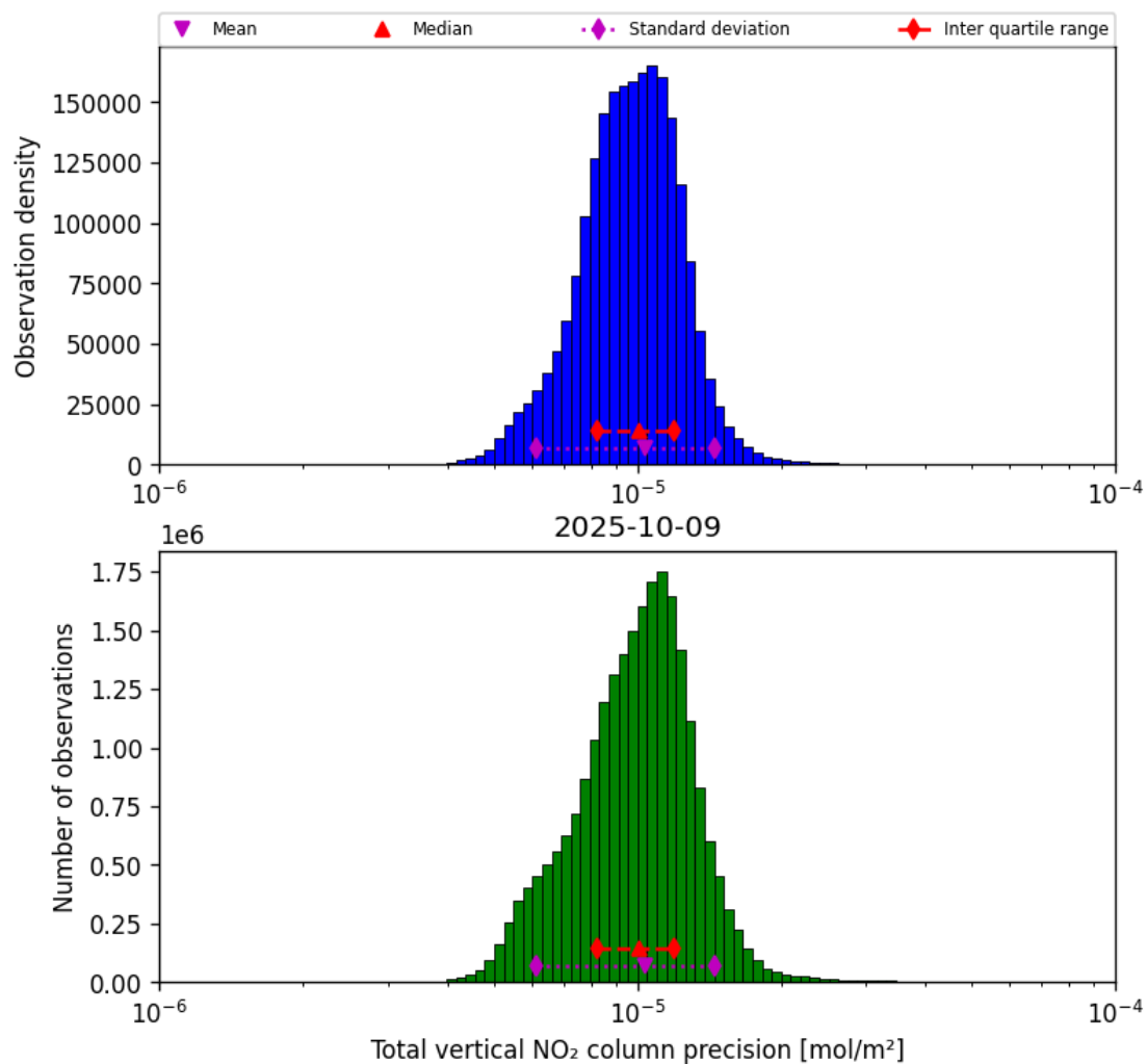
Figure 37: Histogram of "Total vertical NO 2 column precision" for 2025-10-09 to 2025-10-09
