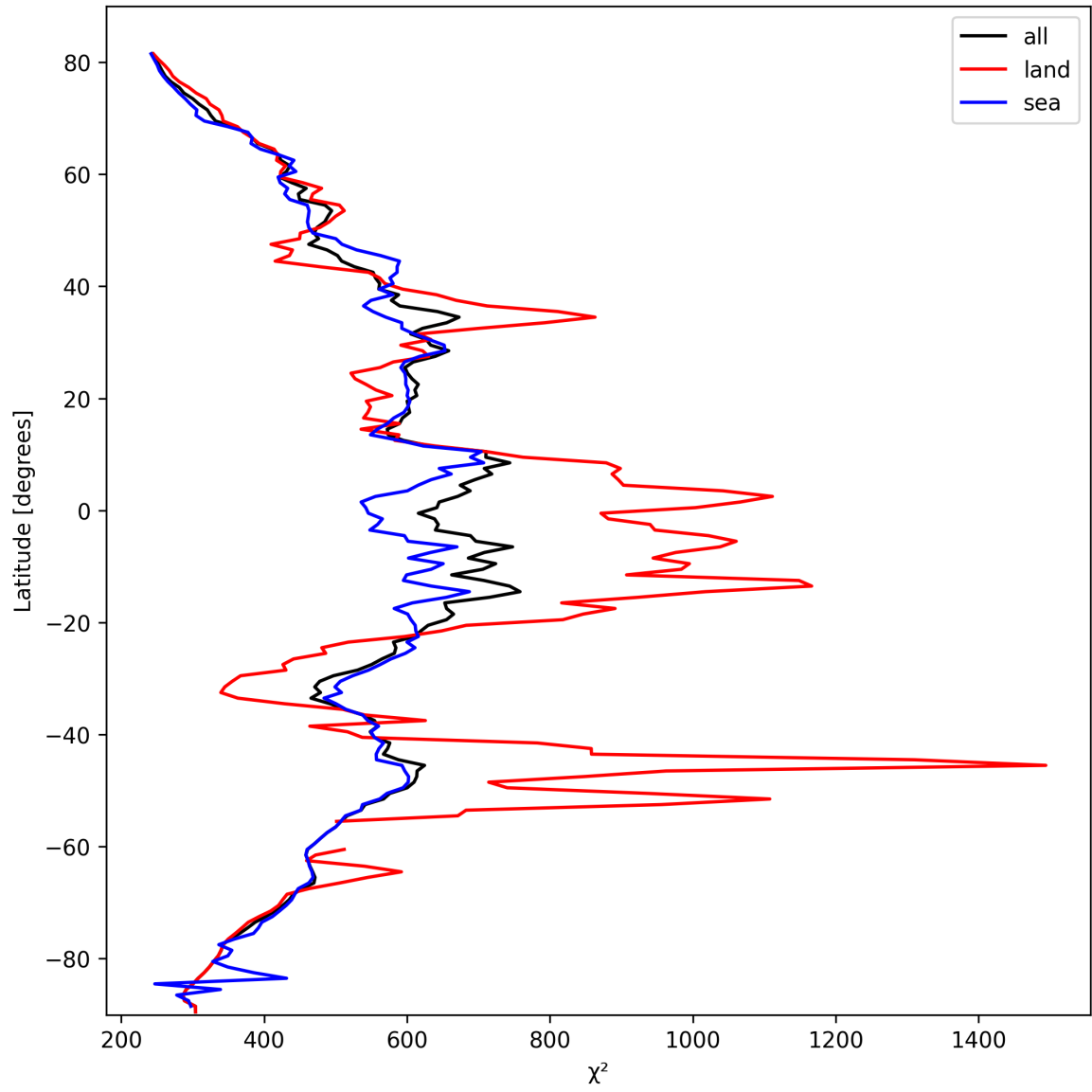
Figure 23: Zonal average of “ \chi^2 ” for 2025-10-09 to 2025-10-09.
