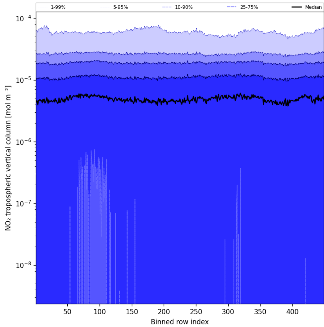
Figure 44: Along track statistics of “NO 2 tropospheric vertical column” for 2025-10-09 to 2025-10-09
