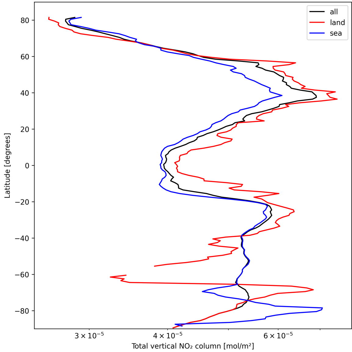
Figure 19: Zonal average of “Total vertical NO 2 column” for 2025-10-09 to 2025-10-09.
