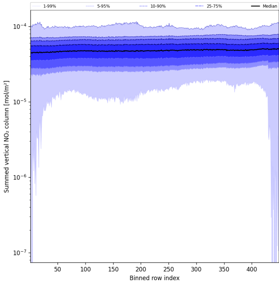
Figure 55: Along track statistics of “Summed vertical NO 2 column” for 2025-10-09 to 2025-10-09
