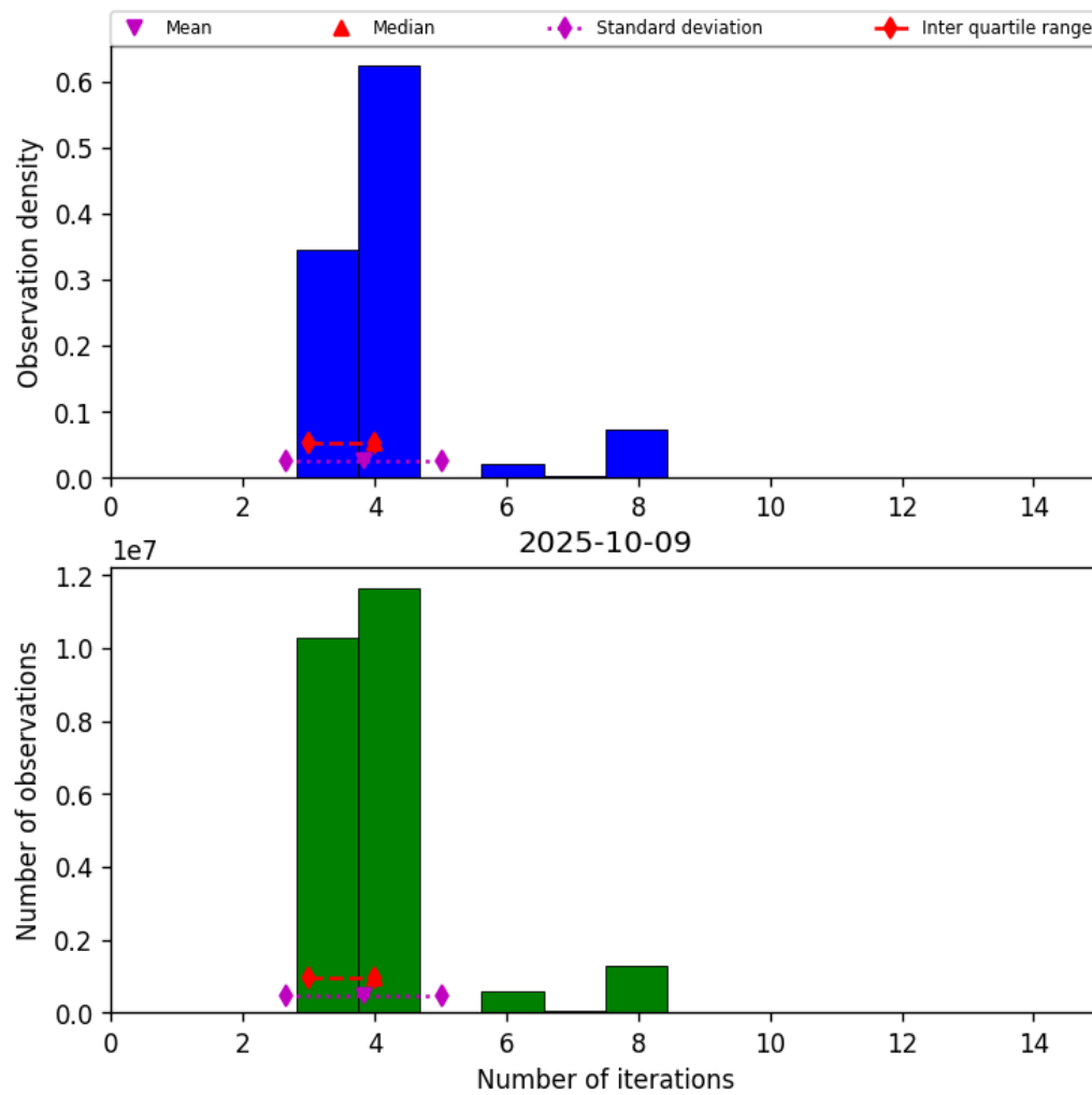
Figure 32: Histogram of “Number of iterations” for 2025-10-09 to 2025-10-09
