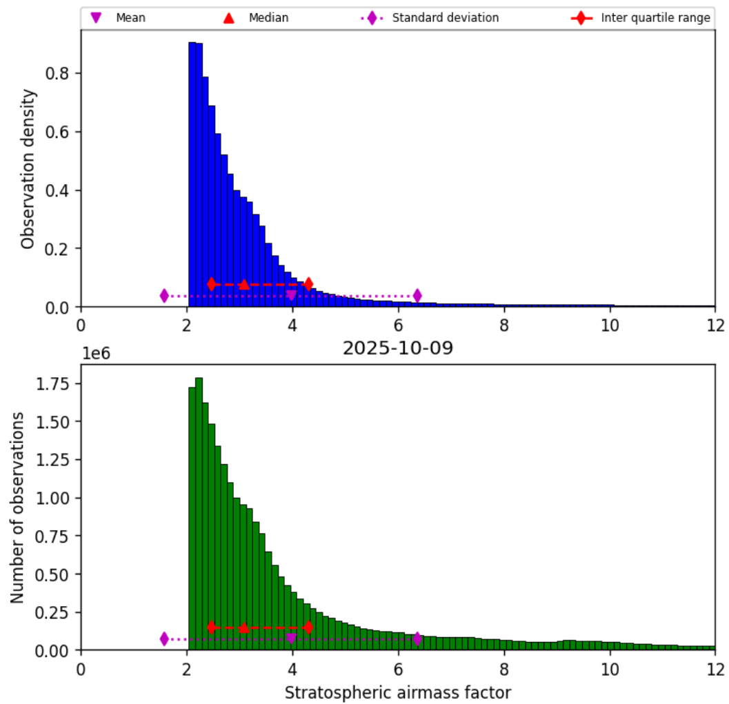
Figure 42: Histogram of “Stratospheric airmass factor” for 2025-10-09 to 2025-10-09
