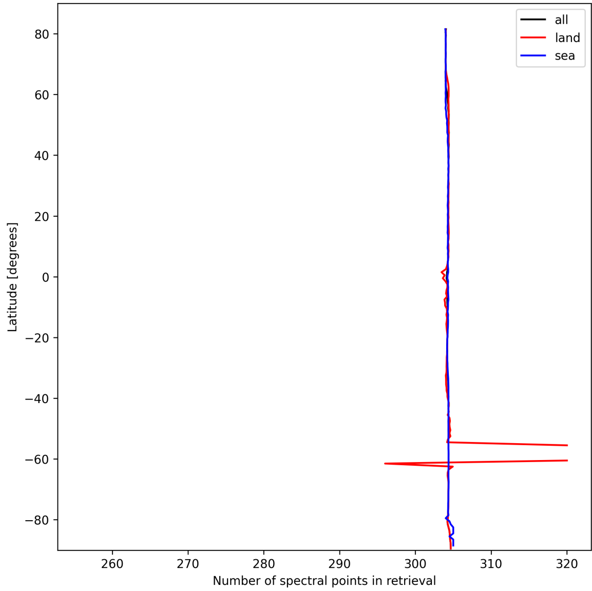
Figure 14: Zonal average of “Number of spectral points in retrieval” for 2025-10-09 to 2025-10-09.
