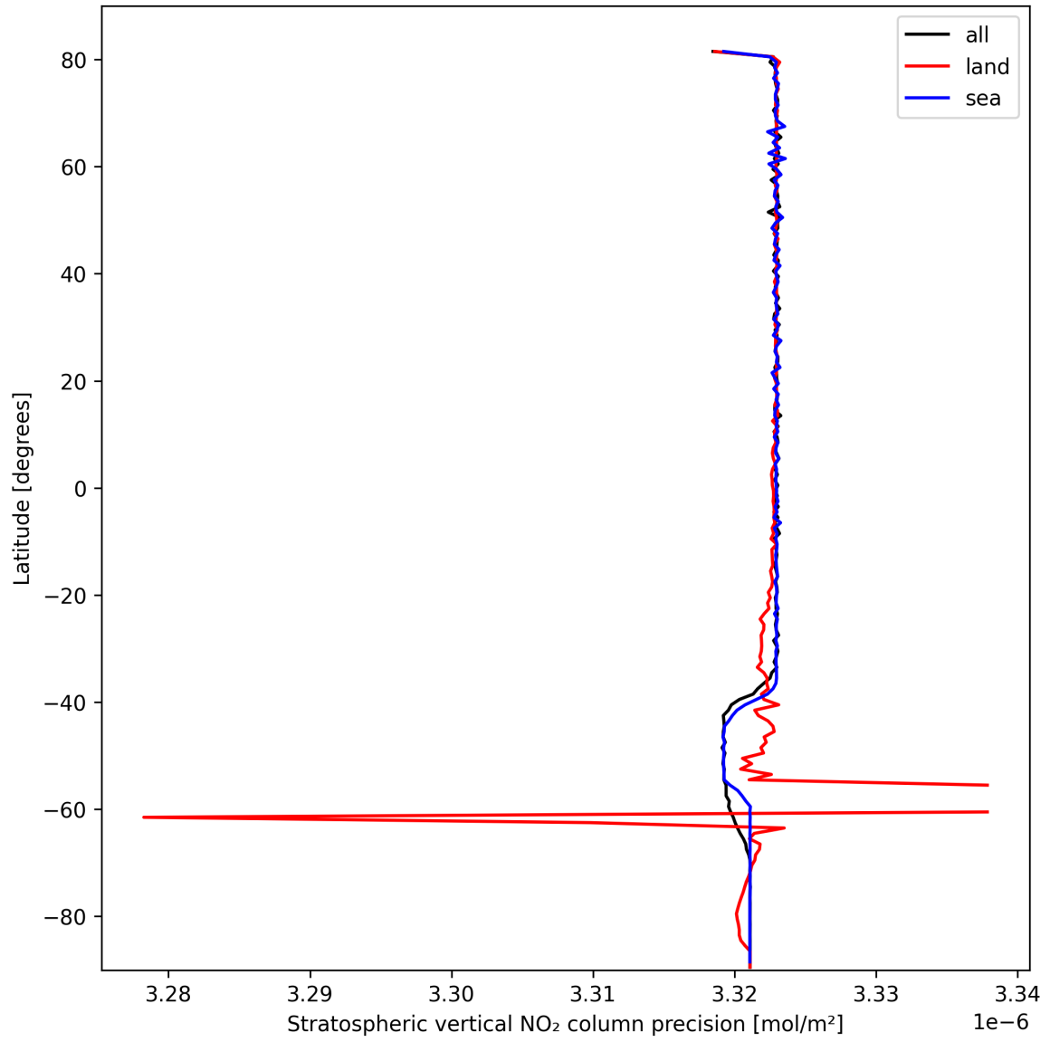
Figure 18: Zonal average of “Stratospheric vertical NO 2 column precision” for 2025-10-09 to 2025-10-09.
