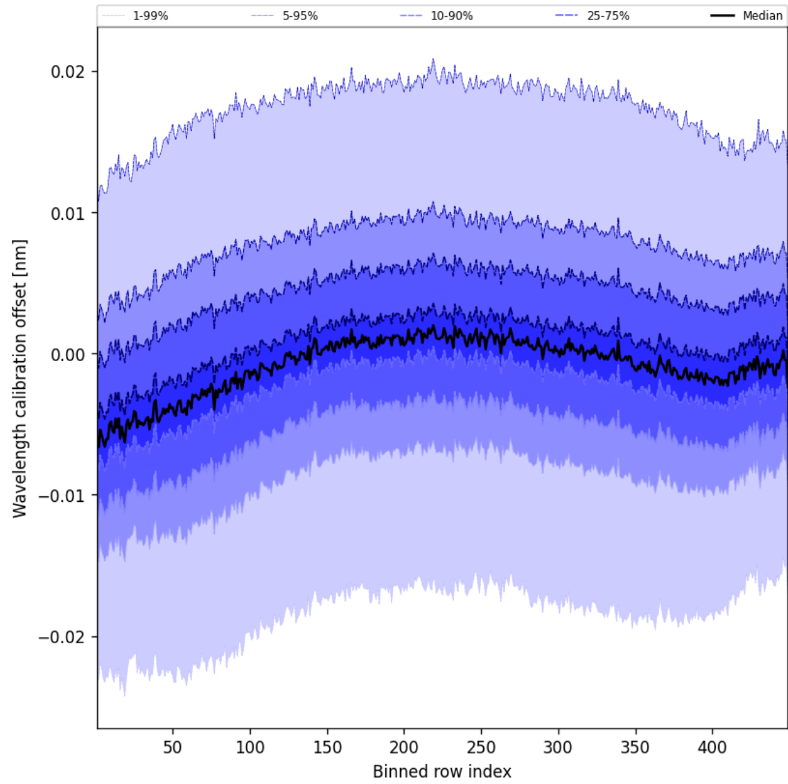
Figure 50: Along track statistics of “Wavelength calibration offset” for 2025-10-09 to 2025-10-09
