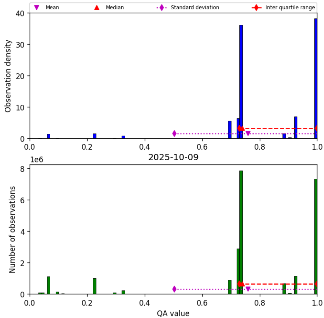
Figure 26: Histogram of “QA value” for 2025-10-09 to 2025-10-09
