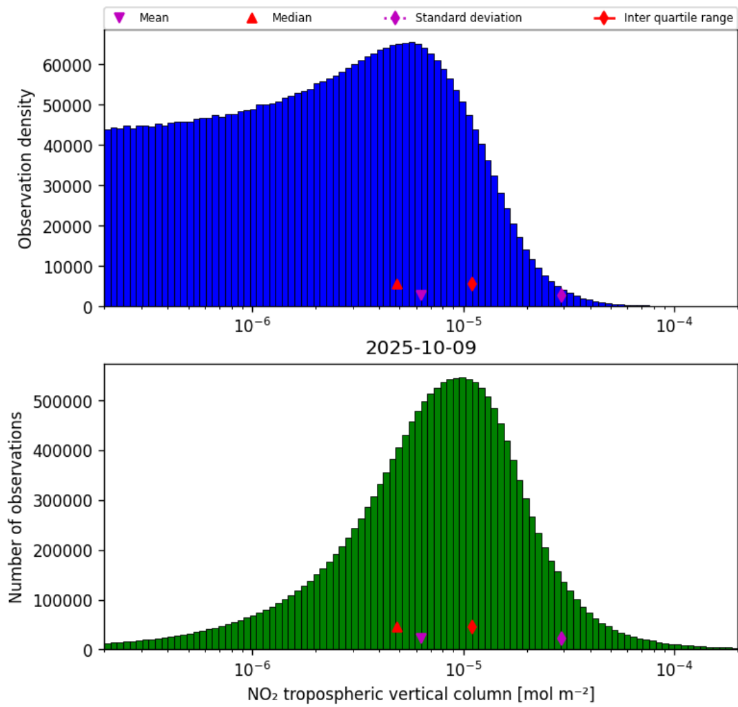
Figure 27: Histogram of “ \text{NO}_2 tropospheric vertical column” for 2025-10-09 to 2025-10-09
