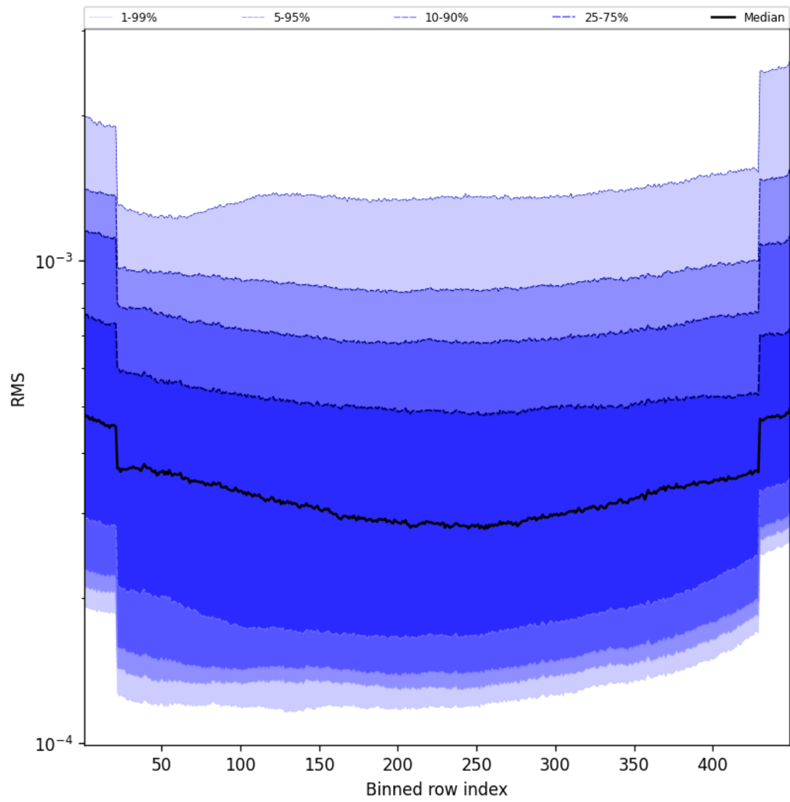
Figure 58: Along track statistics of “RMS” for 2025-10-09 to 2025-10-09
