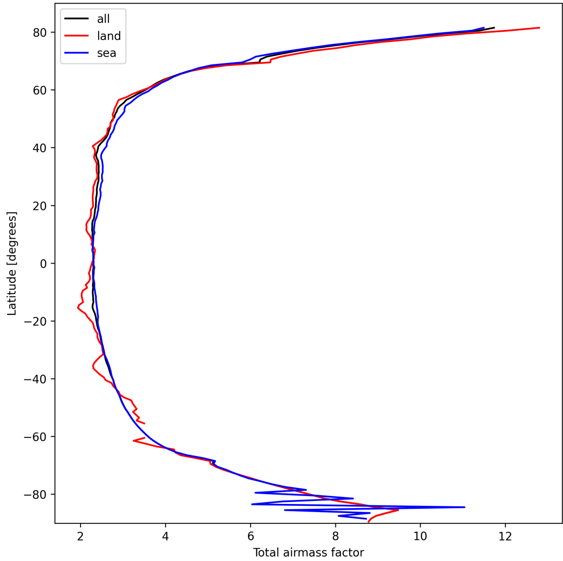
Figure 13: Zonal average of “Total airmass factor” for 2025-10-09 to 2025-10-09.
