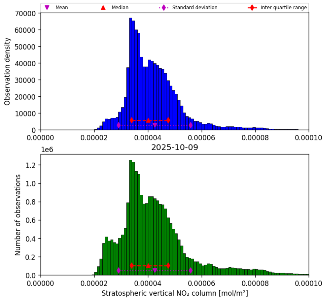
Figure 34: Histogram of “Stratospheric vertical NO 2 column” for 2025-10-09 to 2025-10-09
