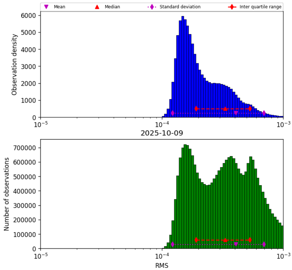
Figure 41: Histogram of “RMS” for 2025-10-09 to 2025-10-09
