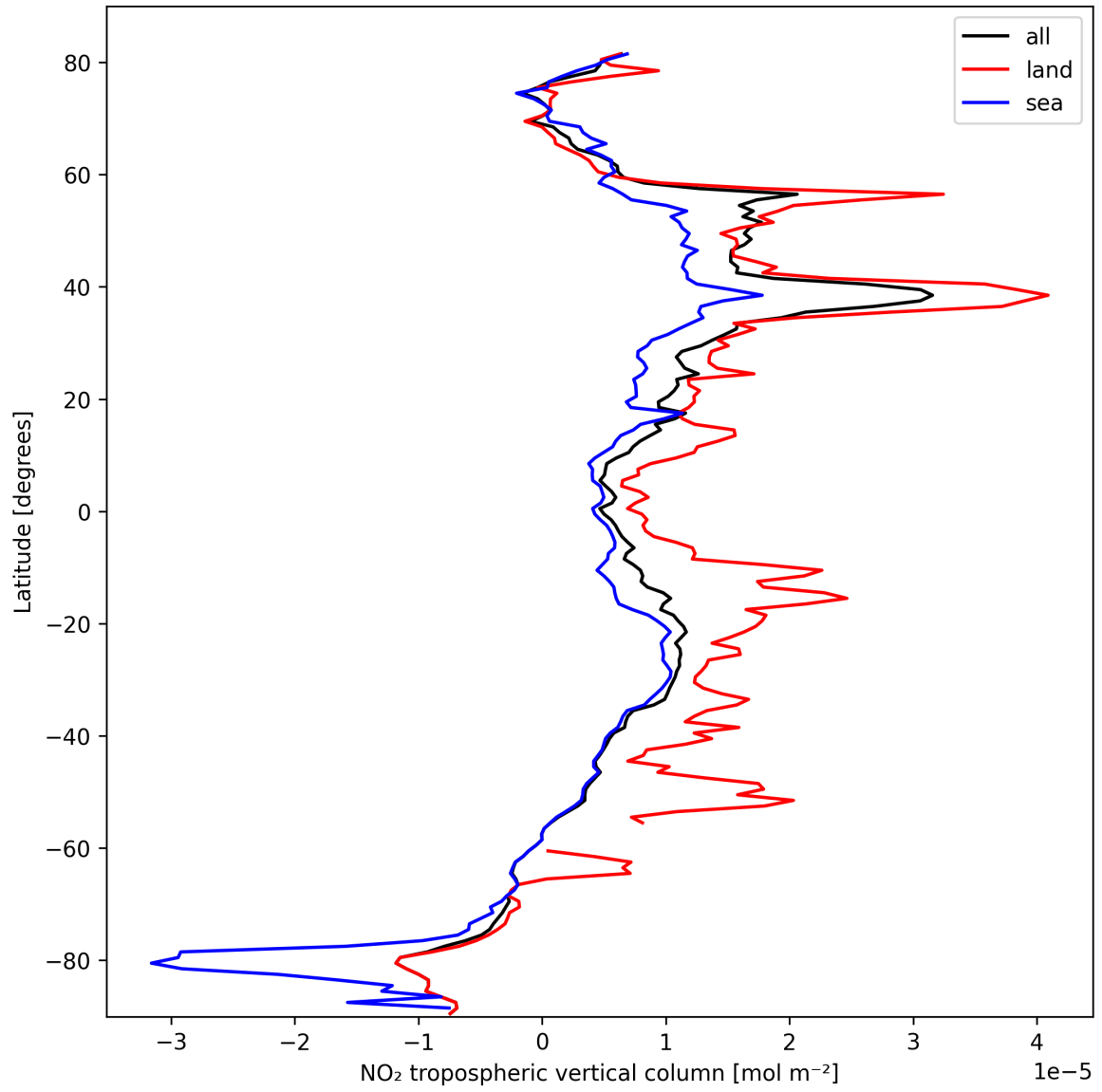
Figure 10: Zonal average of “NO 2 tropospheric vertical column” for 2025-10-09 to 2025-10-09.
