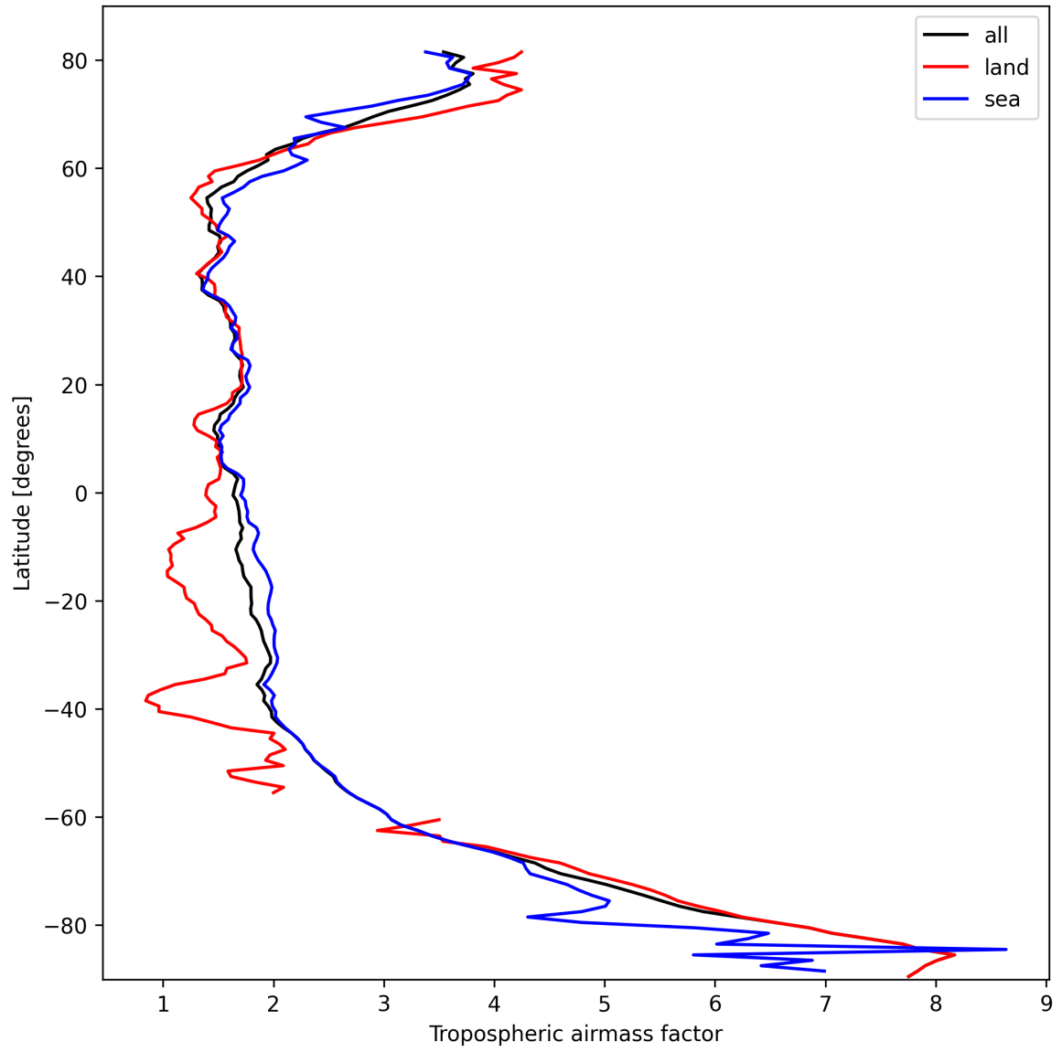
Figure 12: Zonal average of “Tropospheric airmass factor” for 2025-10-09 to 2025-10-09.
