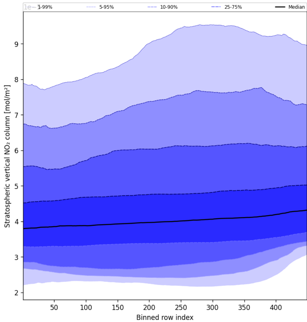
Figure 51: Along track statistics of “Stratospheric vertical NO 2 column” for 2025-10-09 to 2025-10-09
