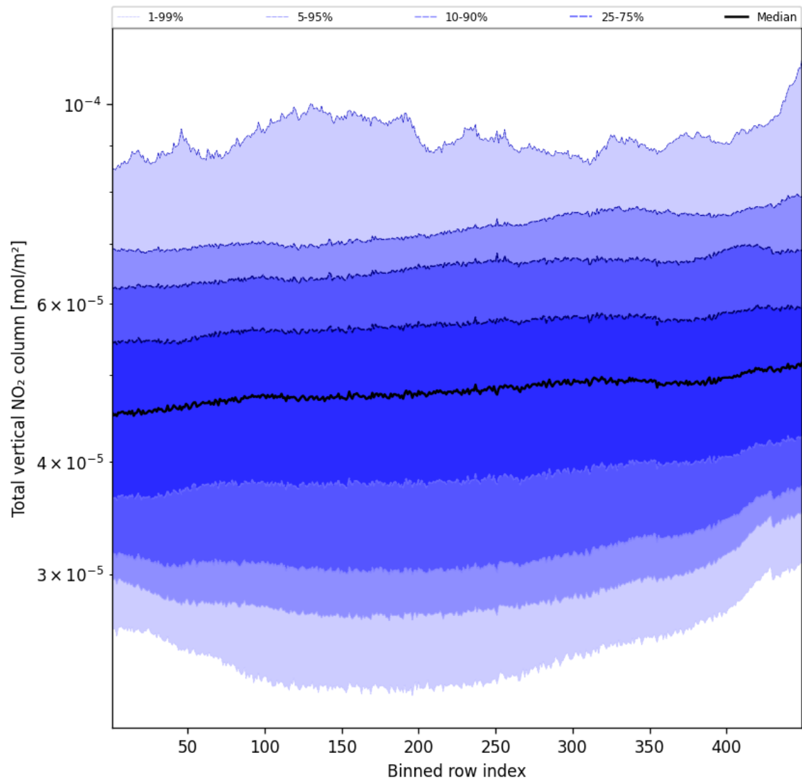
Figure 53: Along track statistics of “Total vertical NO 2 column” for 2025-10-09 to 2025-10-09
