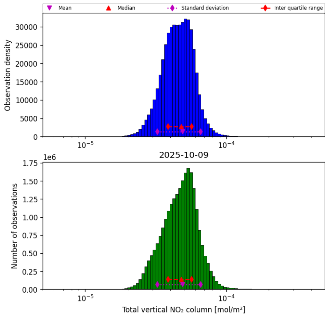
Figure 36: Histogram of “Total vertical NO 2 column” for 2025-10-09 to 2025-10-09
