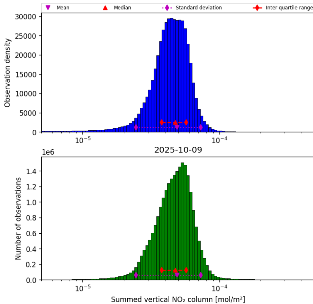
Figure 38: Histogram of “Summed vertical NO 2 column” for 2025-10-09 to 2025-10-09
