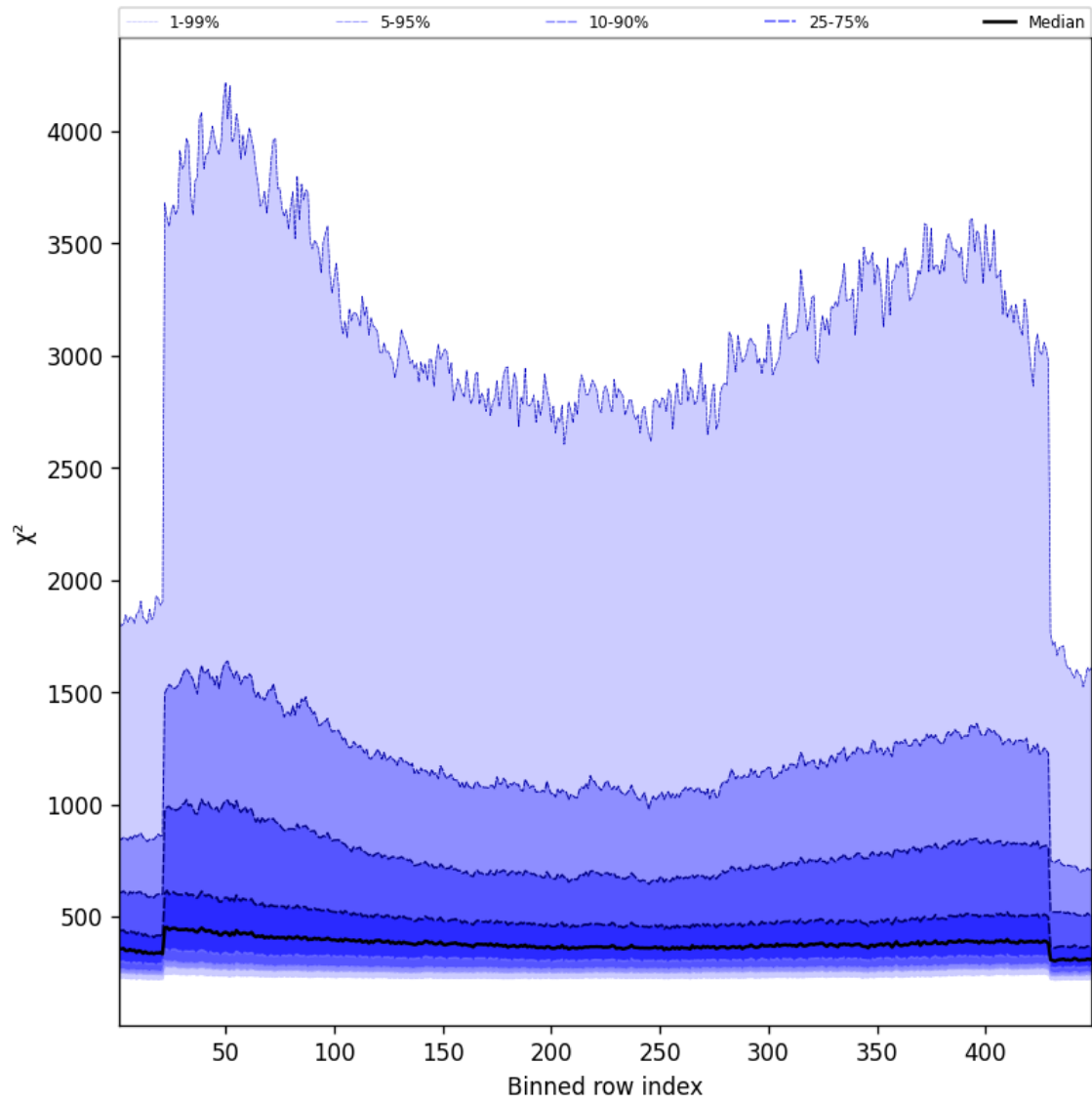
Figure 57: Along track statistics of “ \chi^2 ” for 2025-10-09 to 2025-10-09
