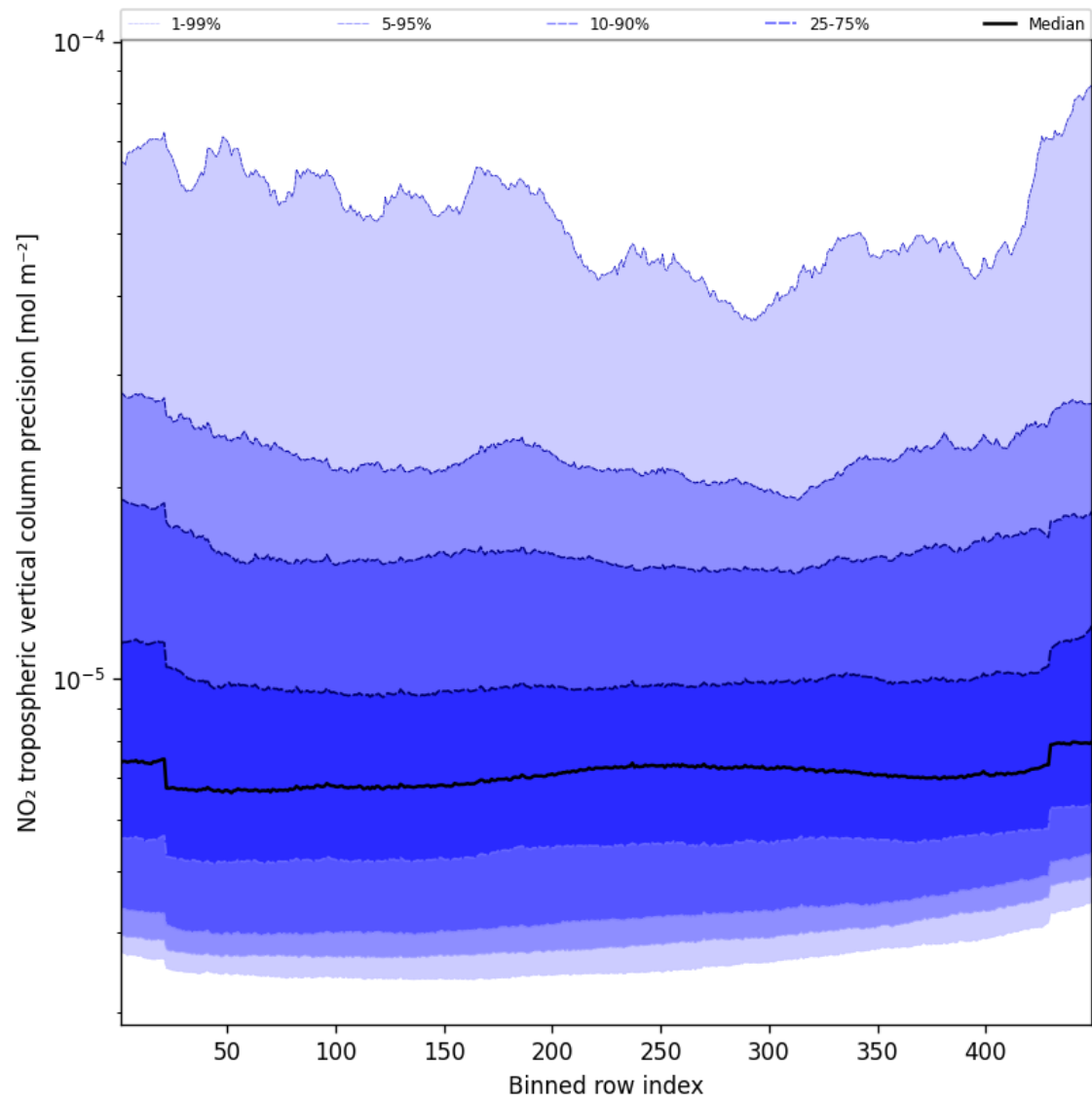
Figure 45: Along track statistics of “NO 2 tropospheric vertical column precision” for 2025-10-09 to 2025-10-09
