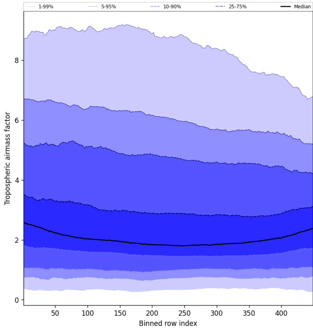
Figure 46: Along track statistics of “Tropospheric airmass factor” for 2025-10-09 to 2025-10-09
