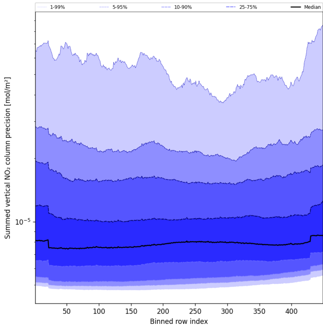
Figure 56: Along track statistics of “Summed vertical NO 2 column precision” for 2025-10-09 to 2025-10-09
