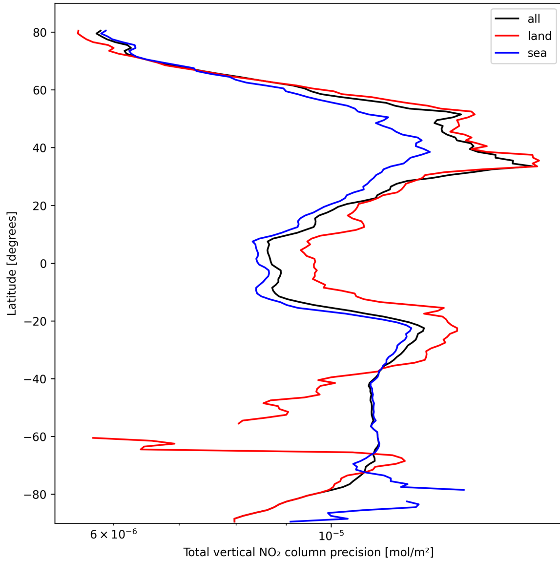
Figure 20: Zonal average of “Total vertical NO 2 column precision” for 2025-10-11 to 2025-10-12.
