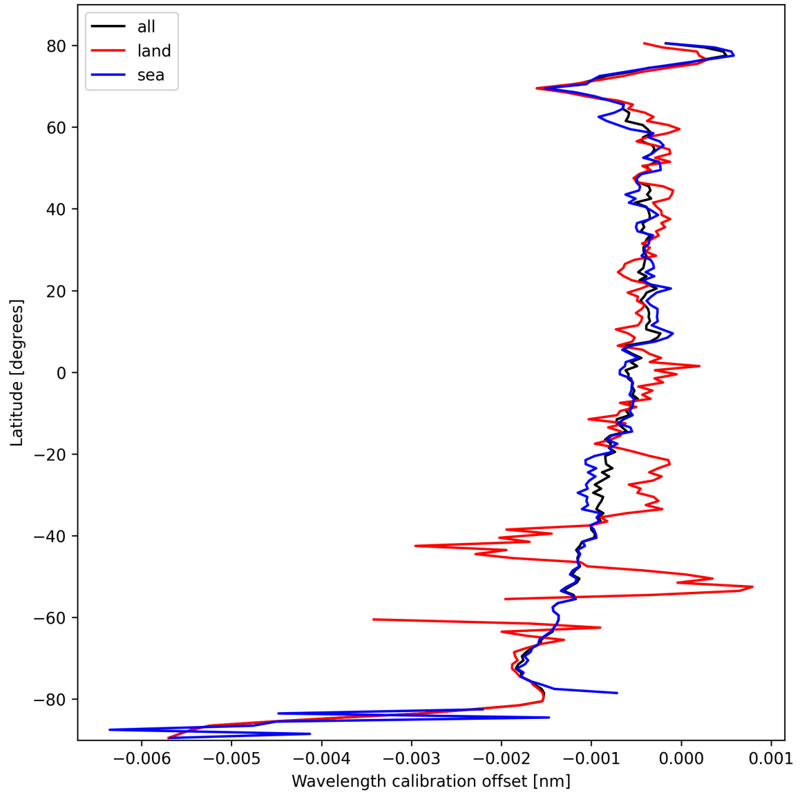
Figure 16: Zonal average of “Wavelength calibration offset” for 2025-10-11 to 2025-10-12.
