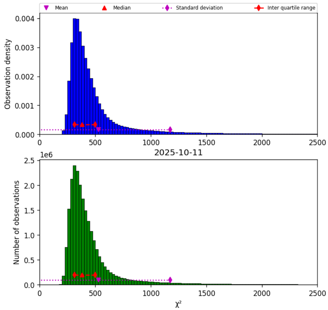
Figure 40: Histogram of “ \chi^2 ” for 2025-10-11 to 2025-10-12
