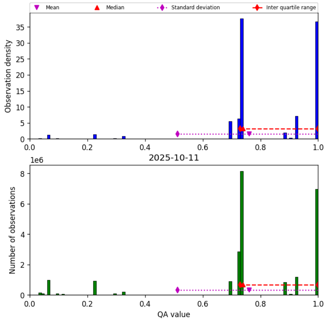
Figure 26: Histogram of “QA value” for 2025-10-11 to 2025-10-12
