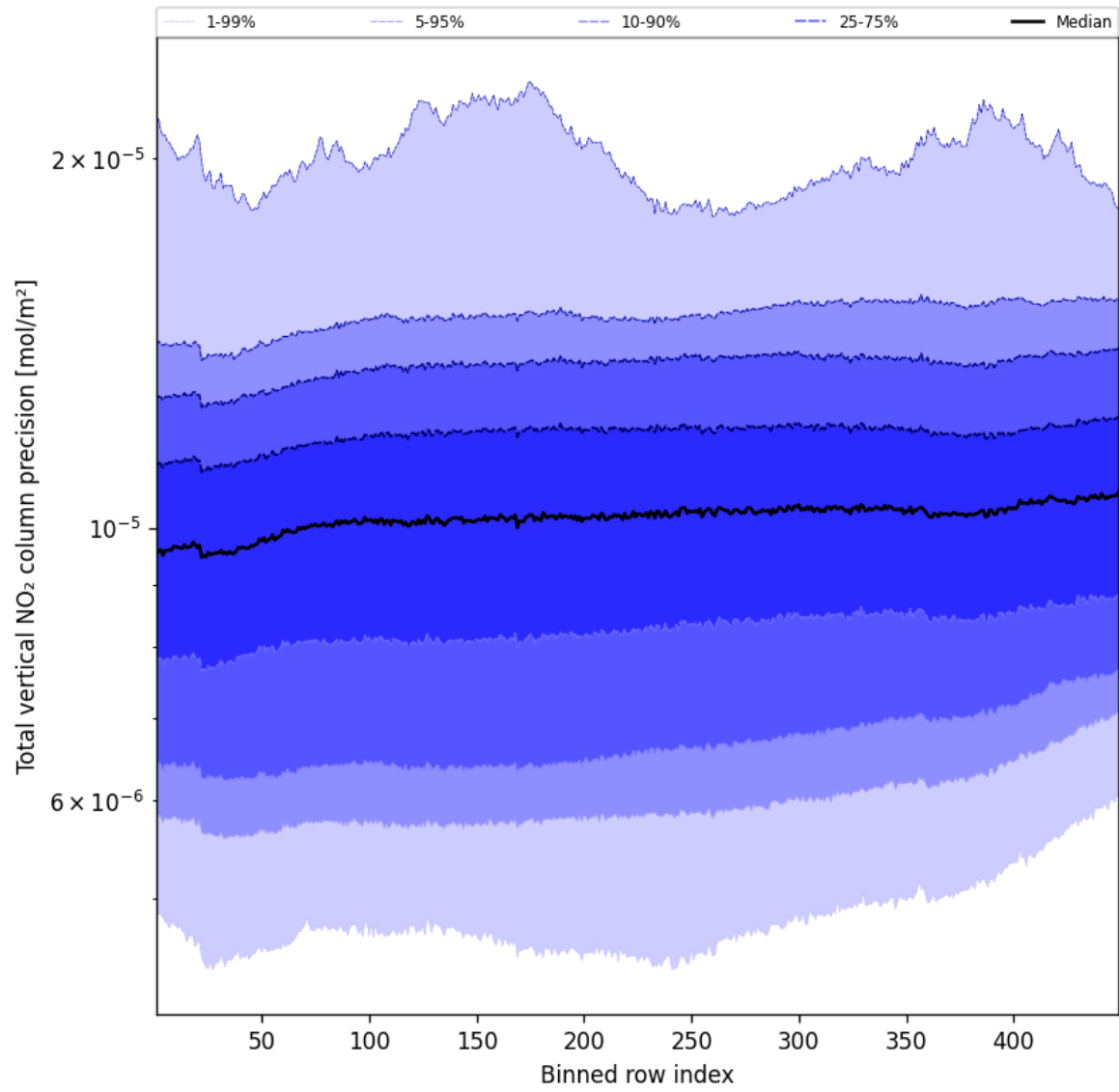
Figure 54: Along track statistics of “Total vertical NO 2 column precision” for 2025-10-11 to 2025-10-12
