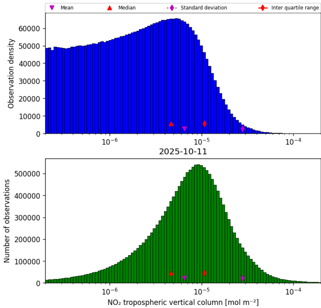
Figure 27: Histogram of “NO 2 tropospheric vertical column” for 2025-10-11 to 2025-10-12
