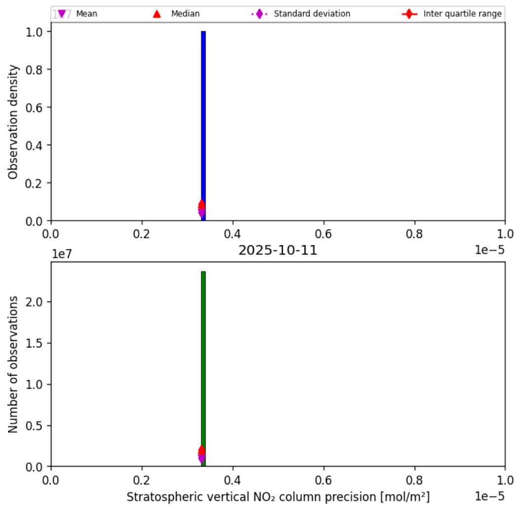
Figure 35: Histogram of “Stratospheric vertical NO 2 column precision” for 2025-10-11 to 2025-10-12
