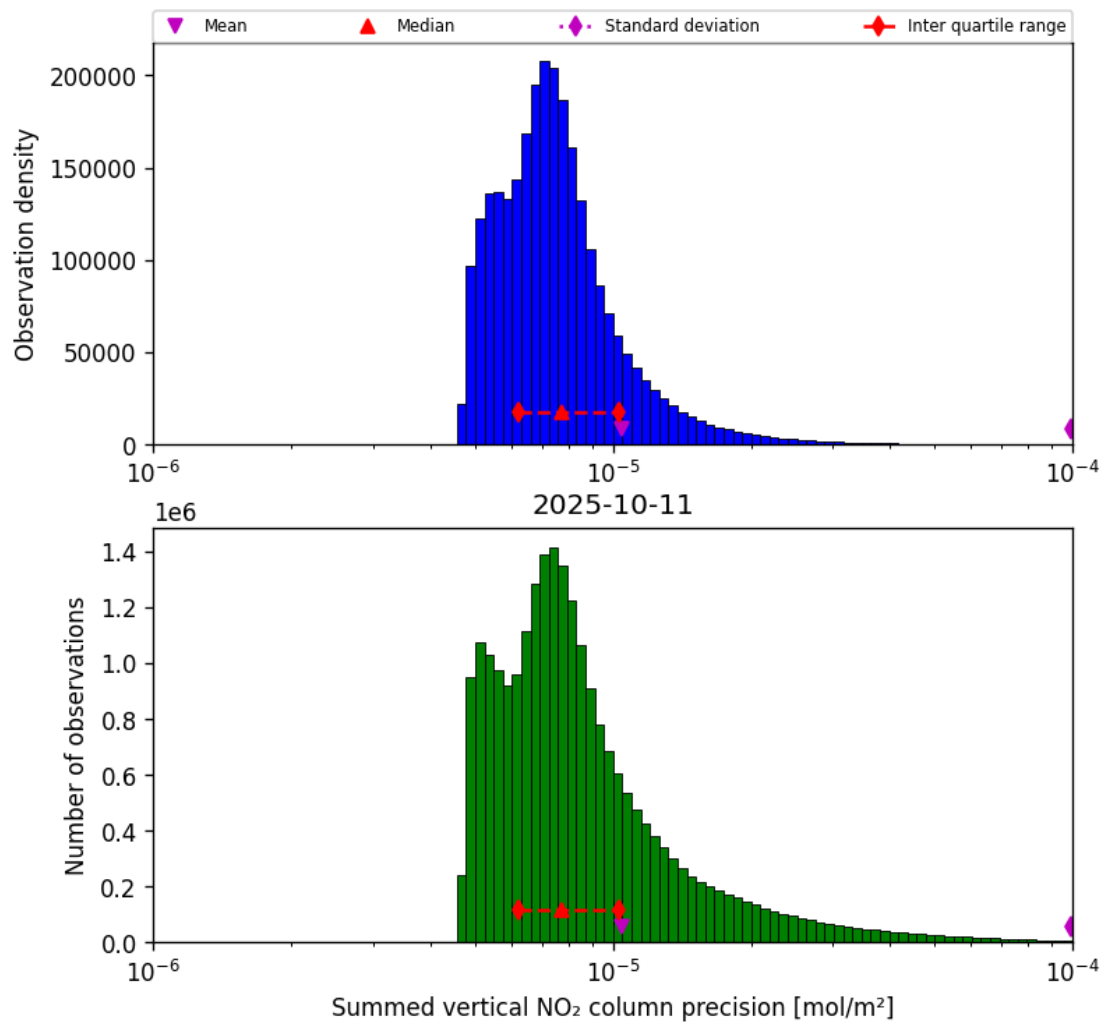
Figure 39: Histogram of “Summed vertical NO 2 column precision” for 2025-10-11 to 2025-10-12
