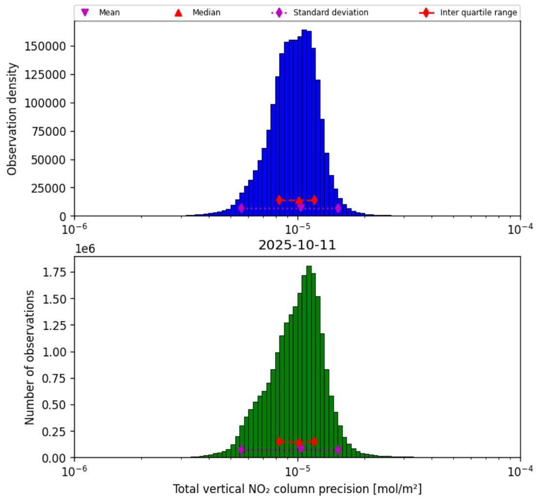
Figure 37: Histogram of “Total vertical NO 2 column precision” for 2025-10-11 to 2025-10-12
