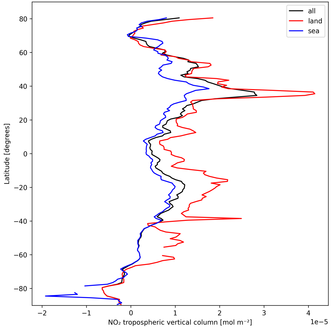
Figure 10: Zonal average of “NO 2 tropospheric vertical column” for 2025-10-11 to 2025-10-12.
