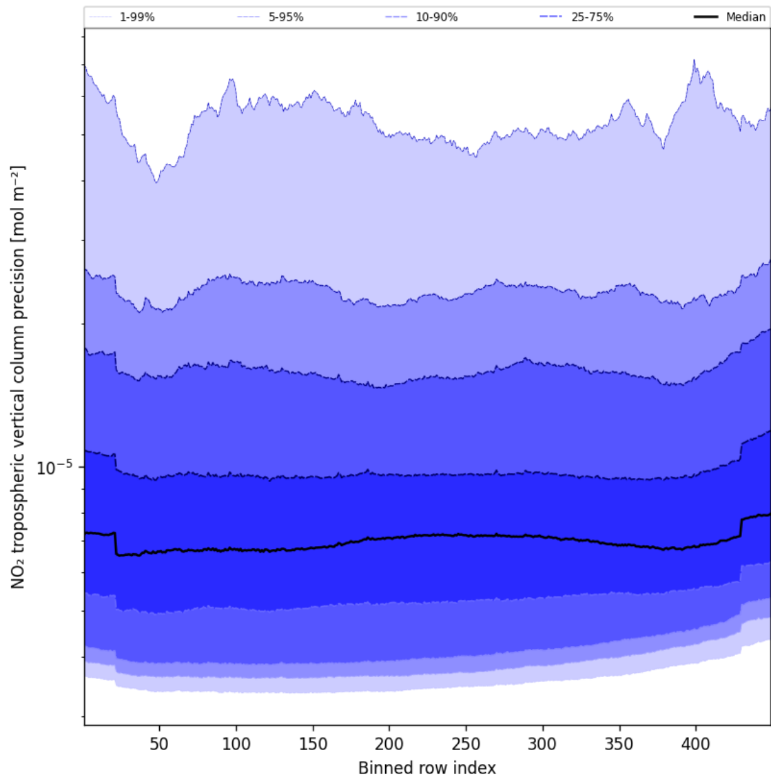
Figure 45: Along track statistics of “NO 2 tropospheric vertical column precision” for 2025-10-11 to 2025-10-12
