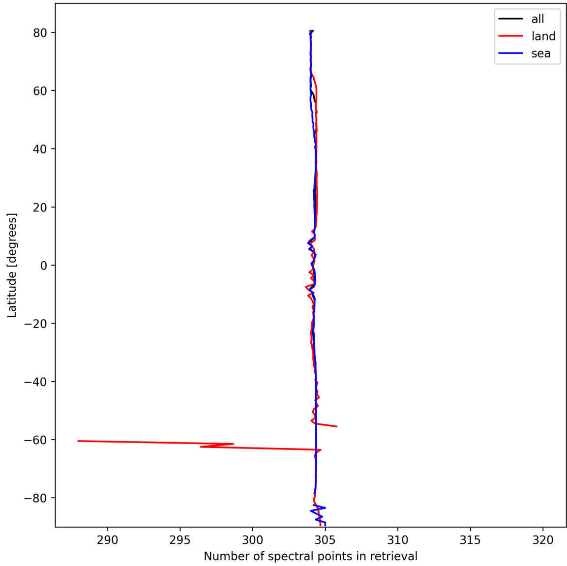
Figure 14: Zonal average of “Number of spectral points in retrieval” for 2025-10-11 to 2025-10-12.
