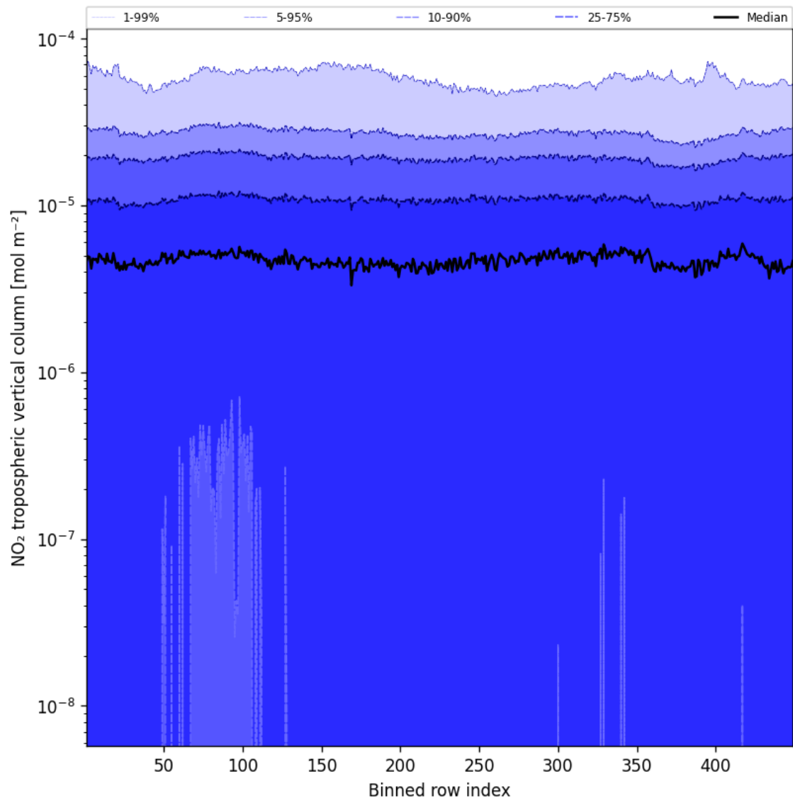
Figure 44: Along track statistics of “NO 2 tropospheric vertical column” for 2025-10-11 to 2025-10-12
