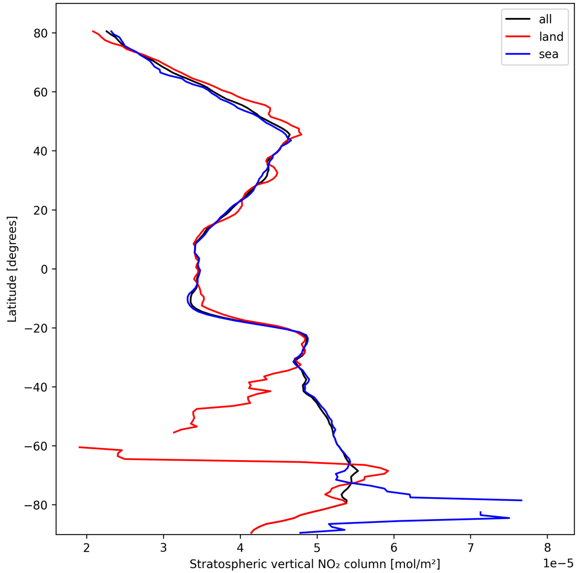
Figure 17: Zonal average of “Stratospheric vertical NO 2 column” for 2025-10-11 to 2025-10-12.
