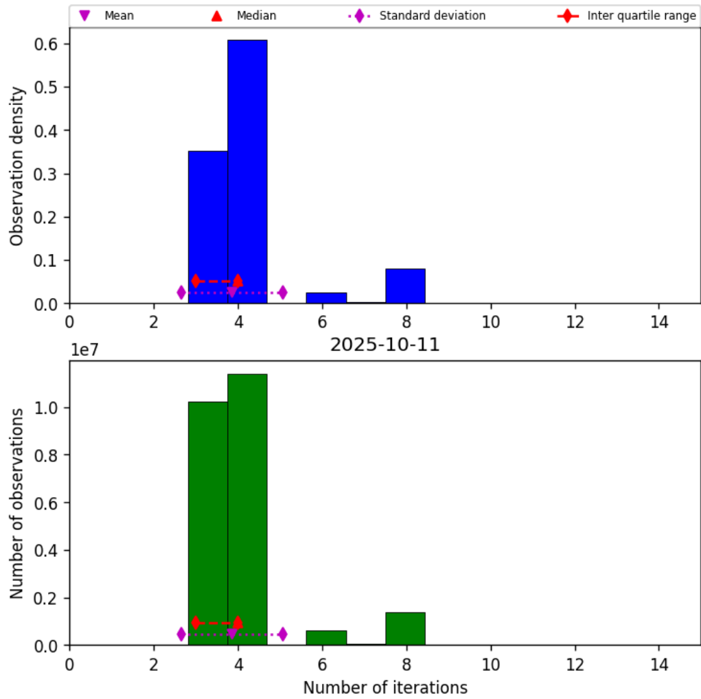
Figure 32: Histogram of “Number of iterations” for 2025-10-11 to 2025-10-12
