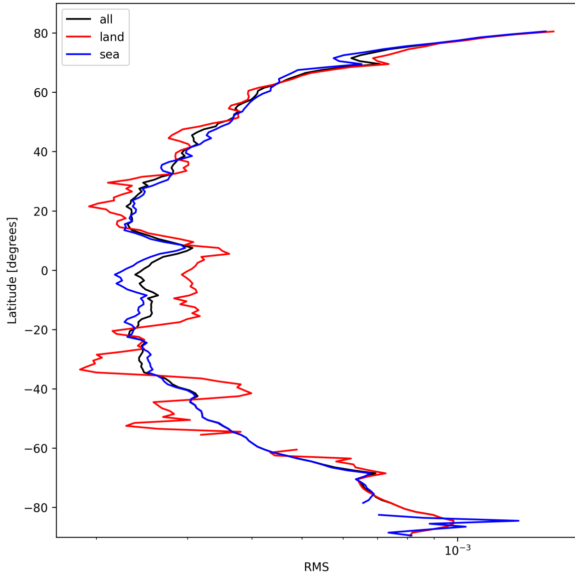
Figure 24: Zonal average of “RMS” for 2025-10-11 to 2025-10-12.
