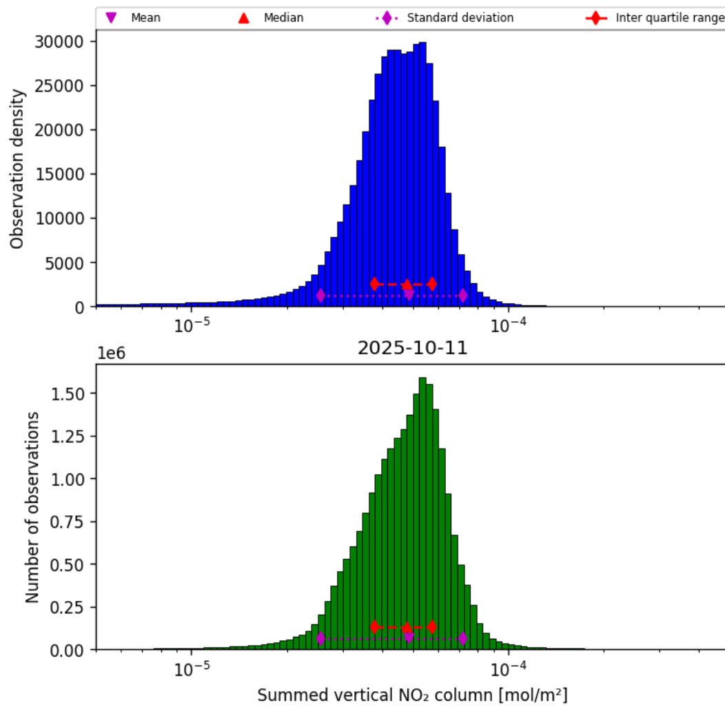
Figure 38: Histogram of “Summed vertical NO 2 column” for 2025-10-11 to 2025-10-12
