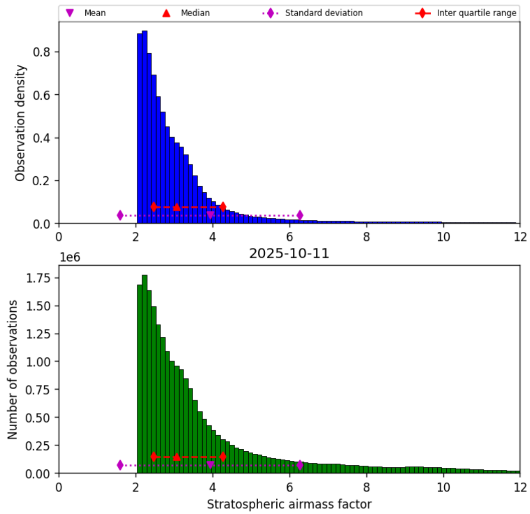
Figure 42: Histogram of “Stratospheric airmass factor” for 2025-10-11 to 2025-10-12
