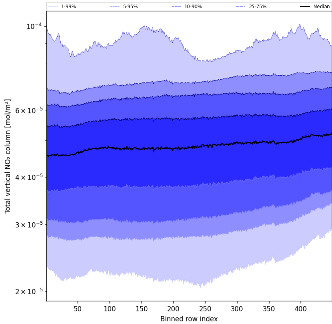
Figure 53: Along track statistics of “Total vertical NO 2 column” for 2025-10-11 to 2025-10-12
