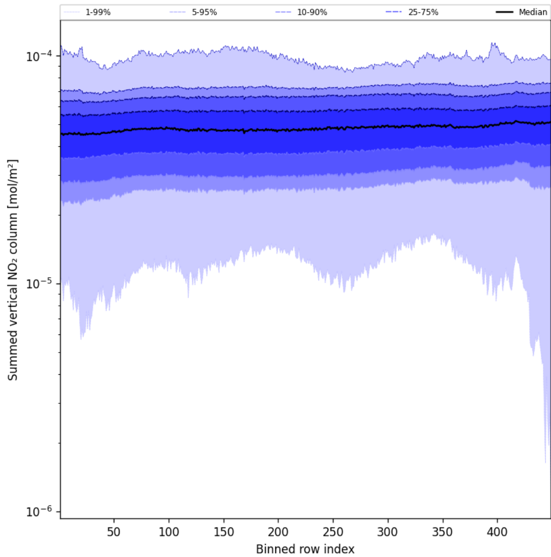
Figure 55: Along track statistics of “Summed vertical NO 2 column” for 2025-10-11 to 2025-10-12
