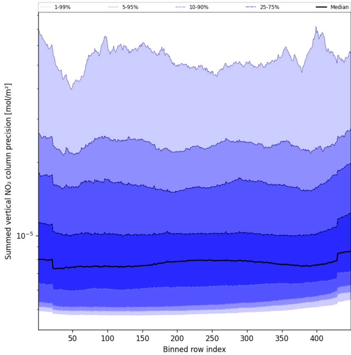
Figure 56: Along track statistics of “Summed vertical NO 2 column precision” for 2025-10-11 to 2025-10-12
