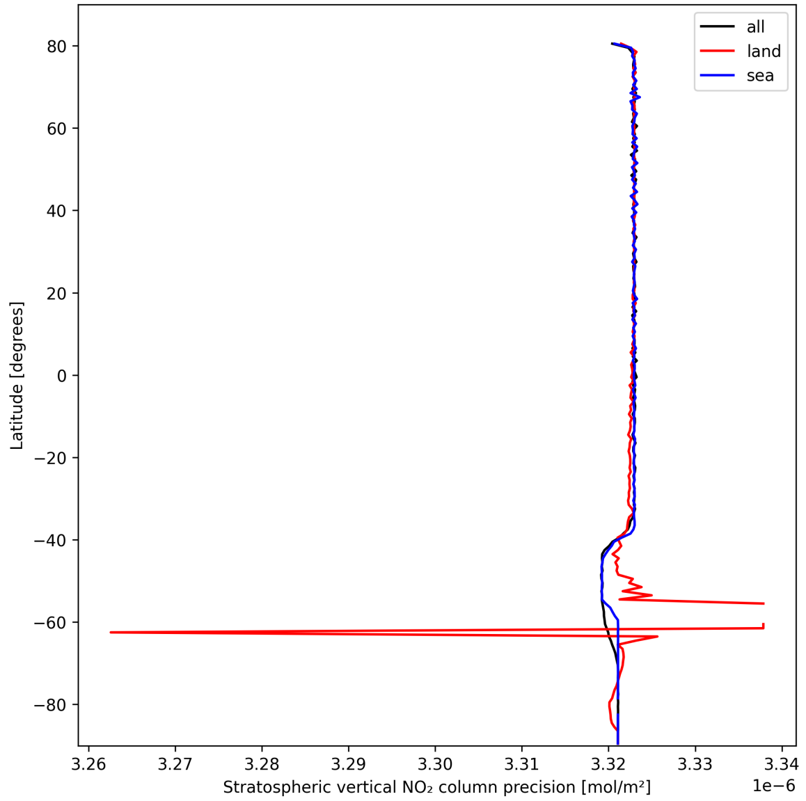
Figure 18: Zonal average of “Stratospheric vertical NO 2 column precision” for 2025-10-11 to 2025-10-12.
