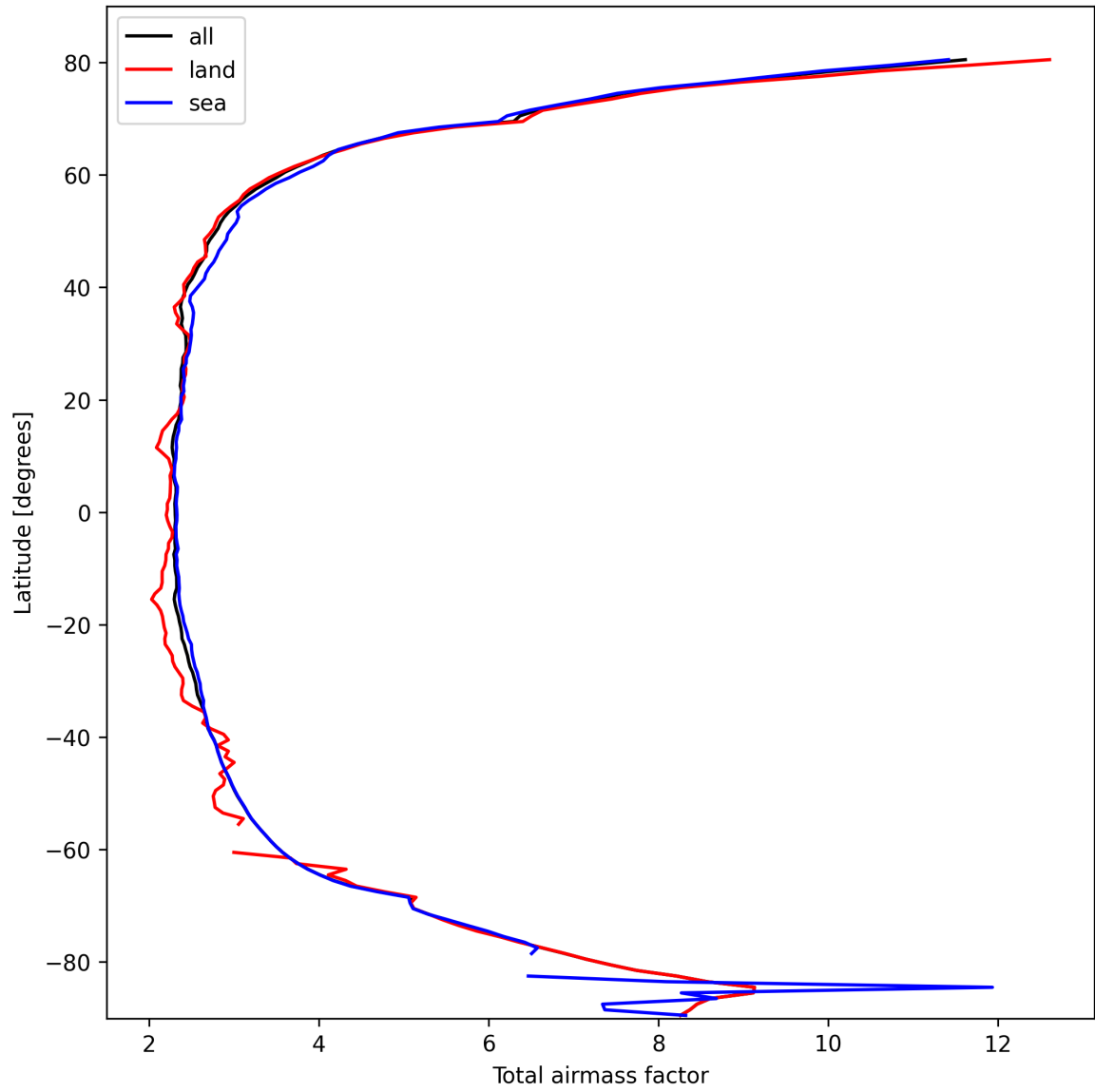
Figure 13: Zonal average of “Total airmass factor” for 2025-10-11 to 2025-10-12.
