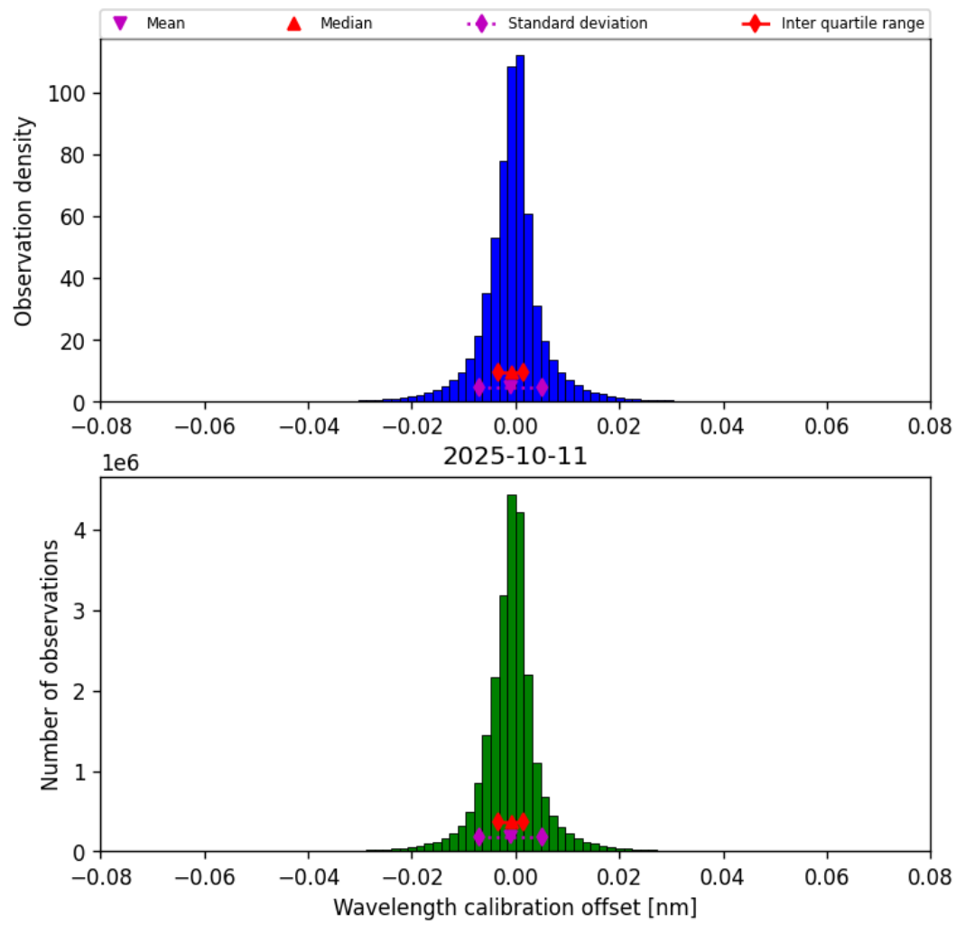
Figure 33: Histogram of “Wavelength calibration offset” for 2025-10-11 to 2025-10-12
