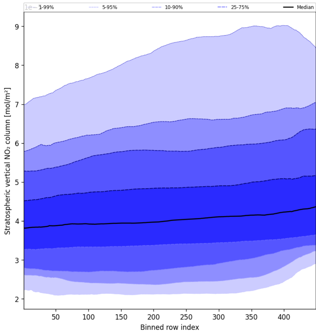
Figure 51: Along track statistics of “Stratospheric vertical NO 2 column” for 2025-10-11 to 2025-10-12
