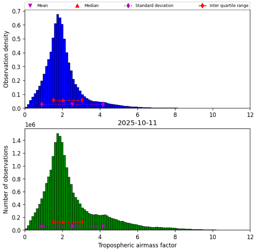
Figure 29: Histogram of “Tropospheric airmass factor” for 2025-10-11 to 2025-10-12
