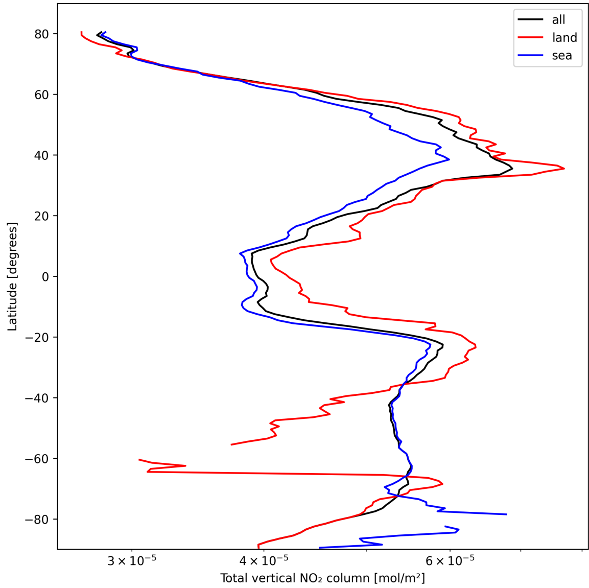
Figure 19: Zonal average of “Total vertical NO 2 column” for 2025-10-11 to 2025-10-12.
