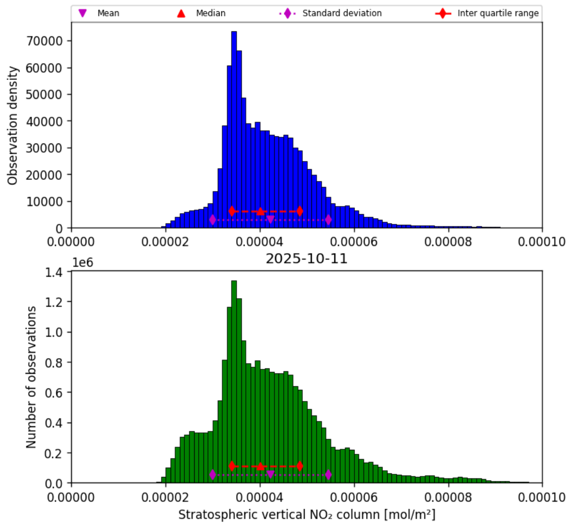
Figure 34: Histogram of “Stratospheric vertical NO 2 column” for 2025-10-11 to 2025-10-12
