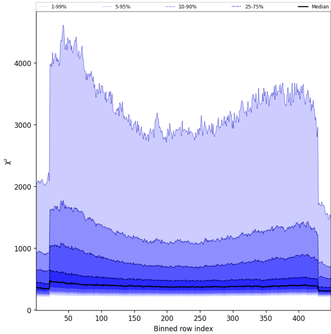
Figure 57: Along track statistics of “ \chi^2 ” for 2025-10-11 to 2025-10-12
