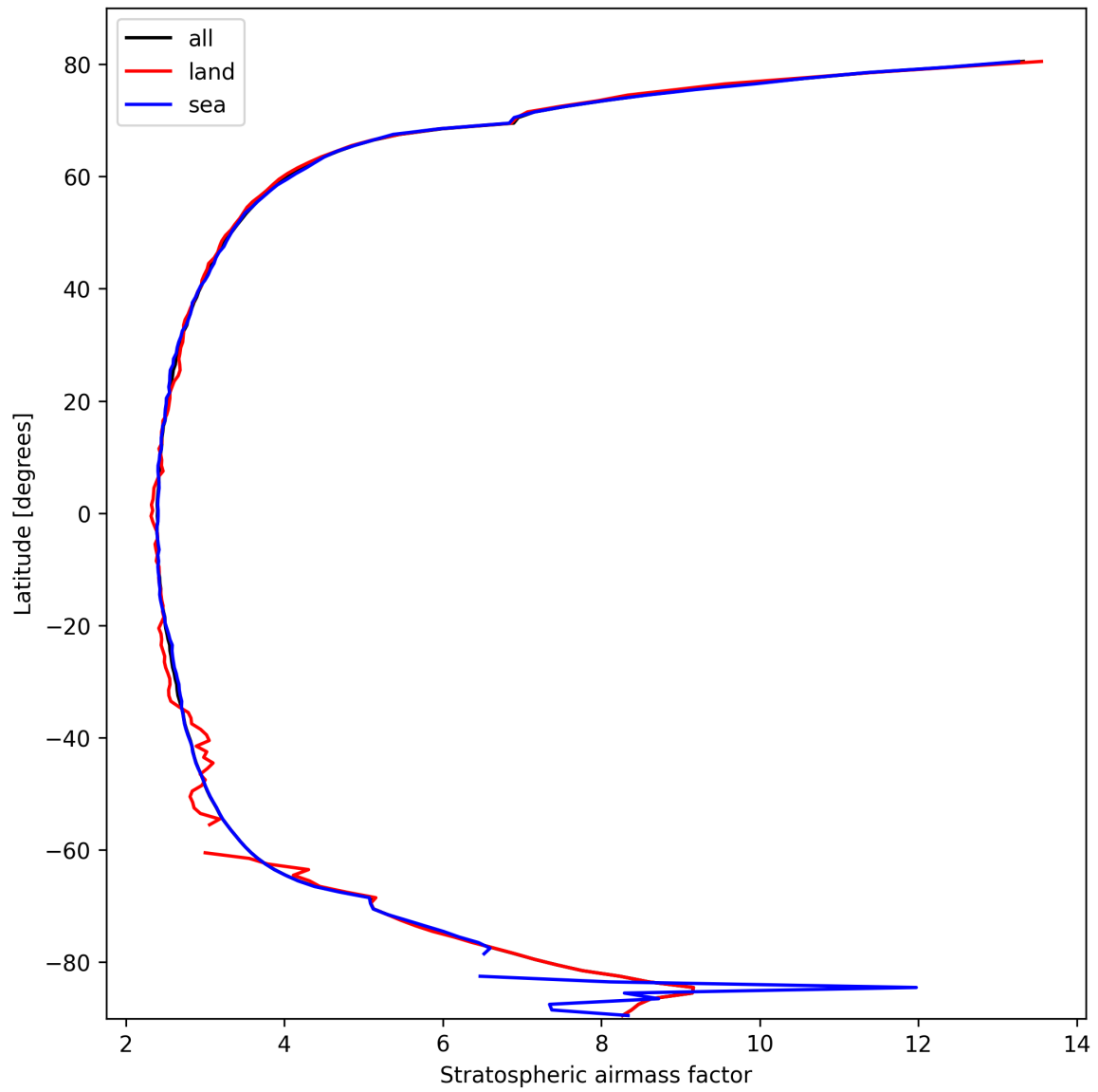
Figure 25: Zonal average of “Stratospheric airmass factor” for 2025-10-11 to 2025-10-12.
