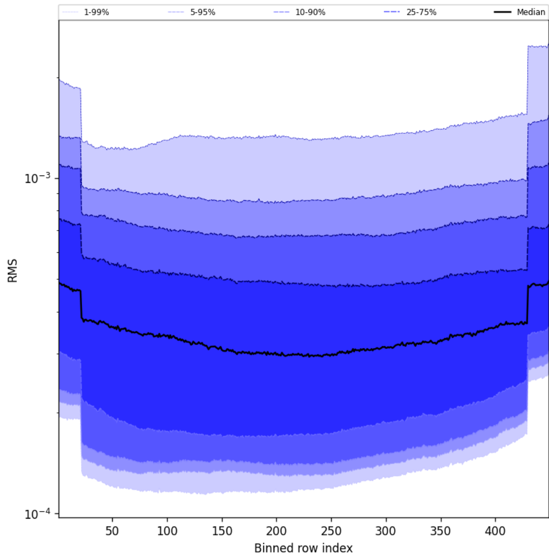
Figure 58: Along track statistics of “RMS” for 2025-10-11 to 2025-10-12
