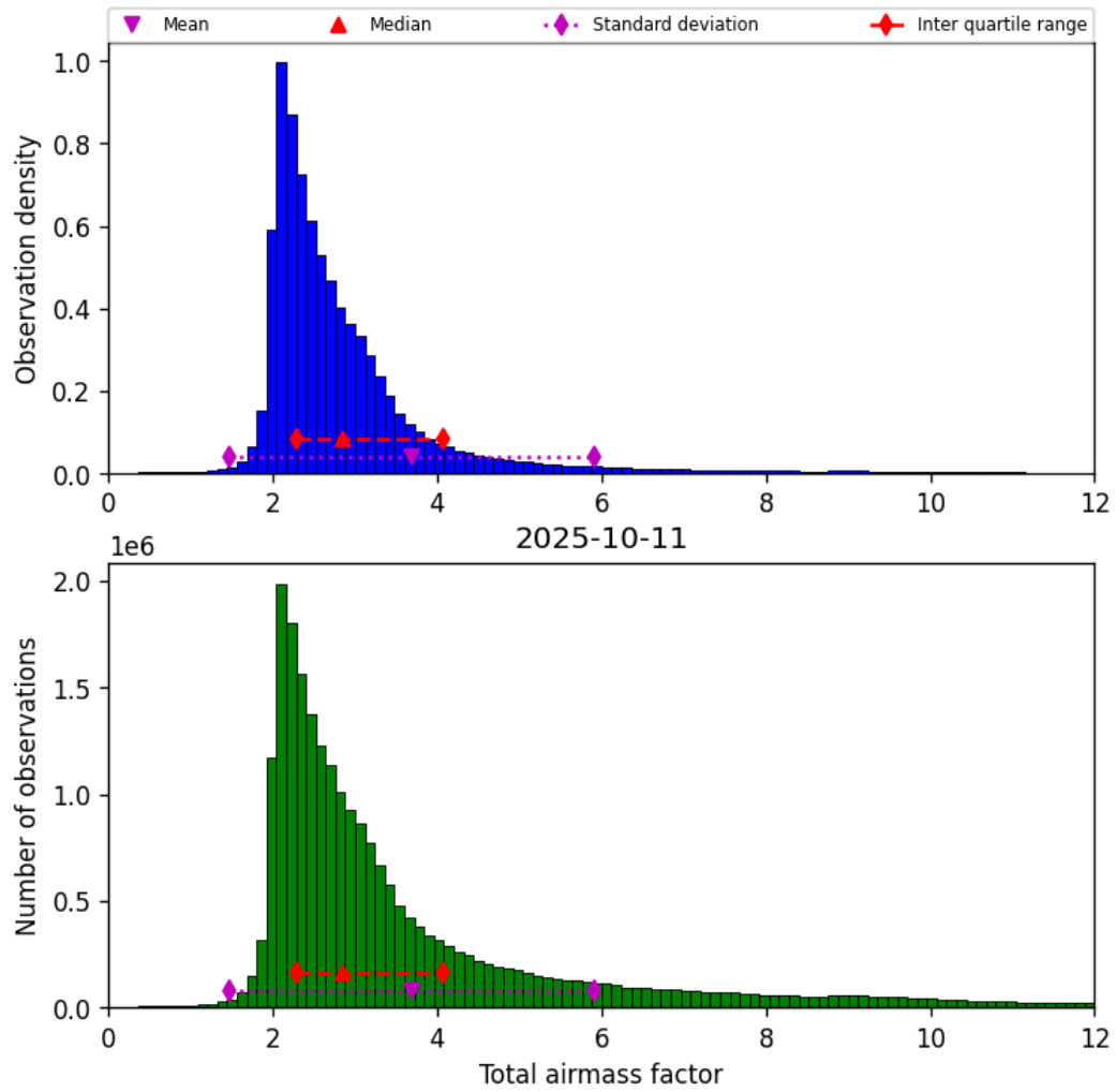
Figure 30: Histogram of “Total airmass factor” for 2025-10-11 to 2025-10-12
