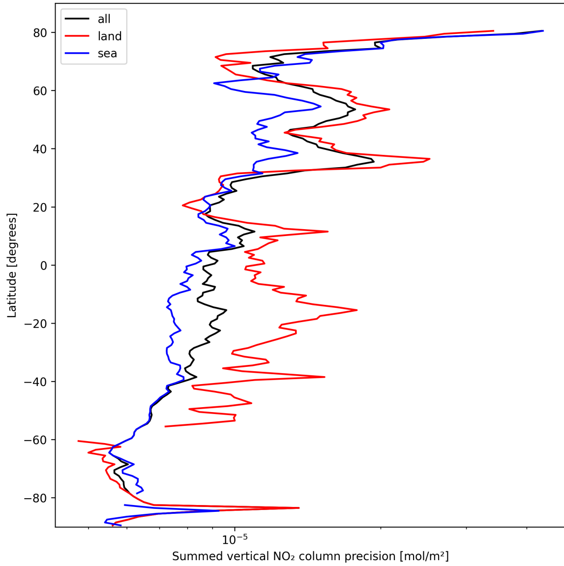
Figure 22: Zonal average of “Summed vertical NO 2 column precision” for 2025-10-11 to 2025-10-12.
