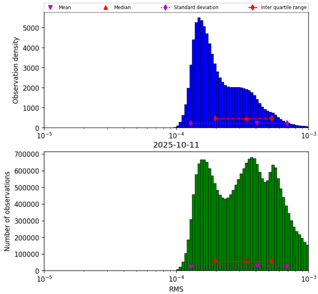
Figure 41: Histogram of “RMS” for 2025-10-11 to 2025-10-12
