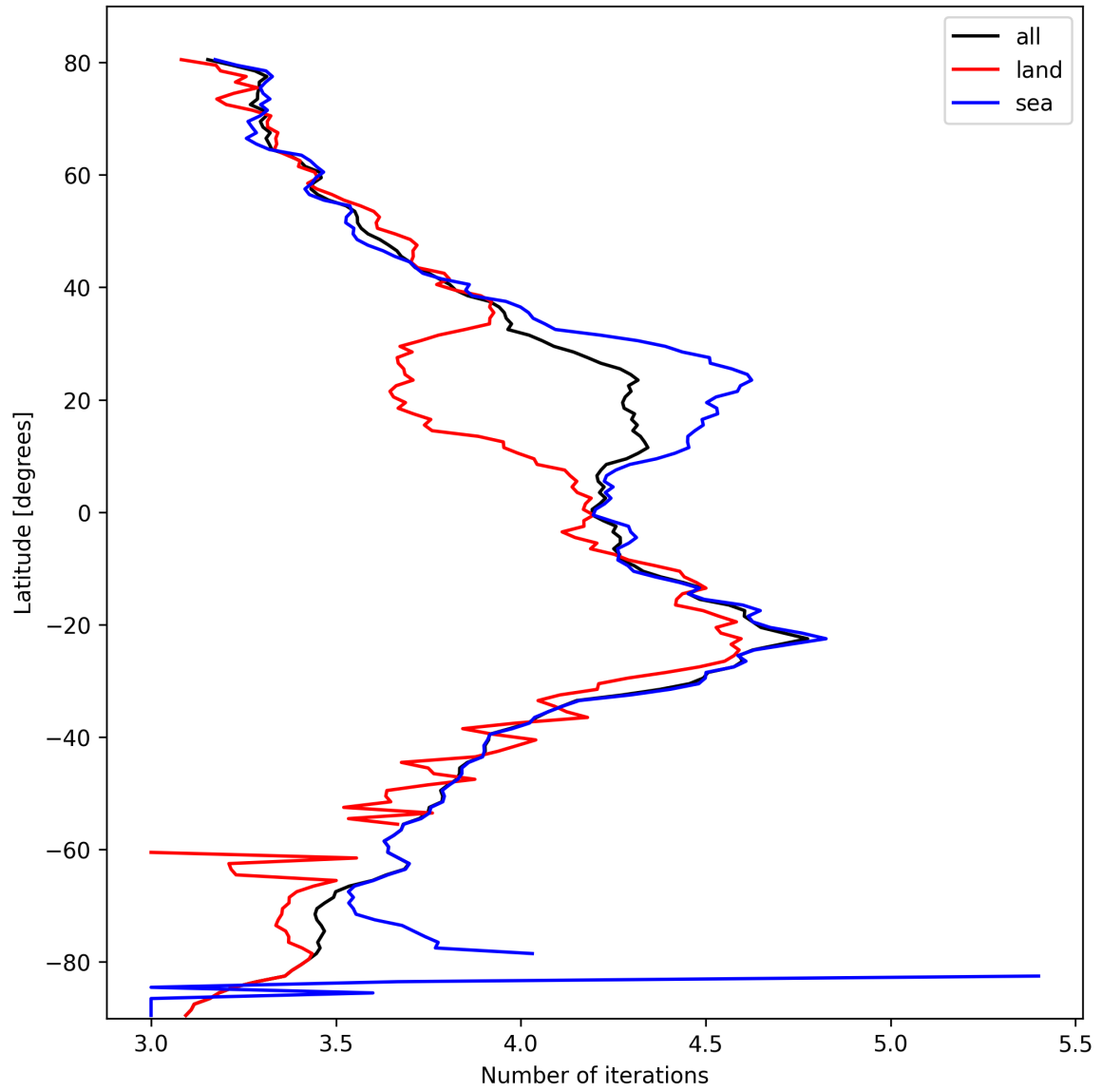
Figure 15: Zonal average of “Number of iterations” for 2025-10-11 to 2025-10-12.
