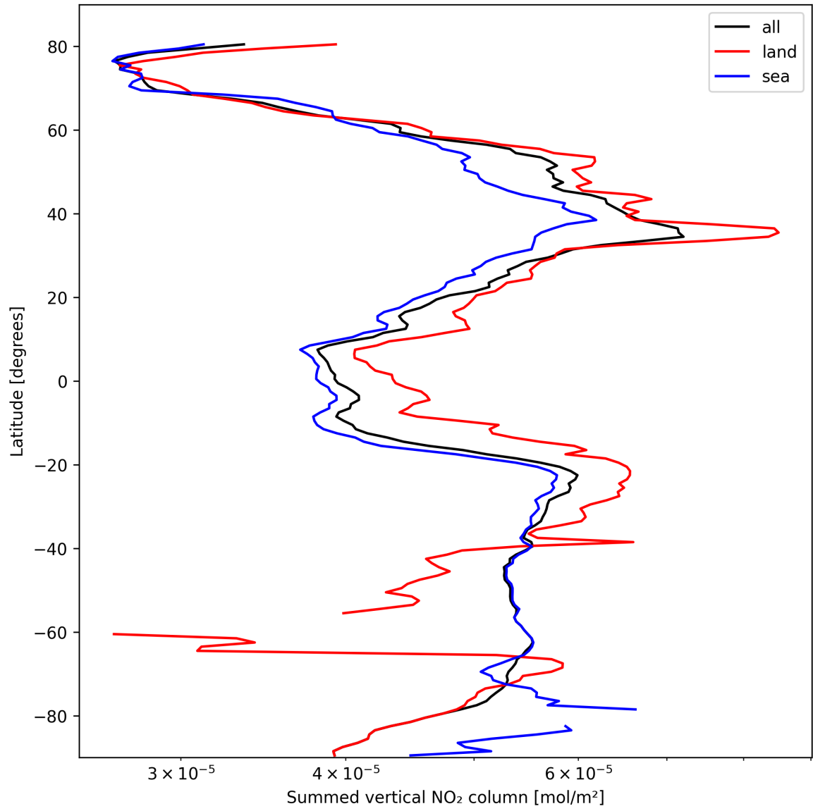
Figure 21: Zonal average of “Summed vertical NO 2 column” for 2025-10-11 to 2025-10-12.
