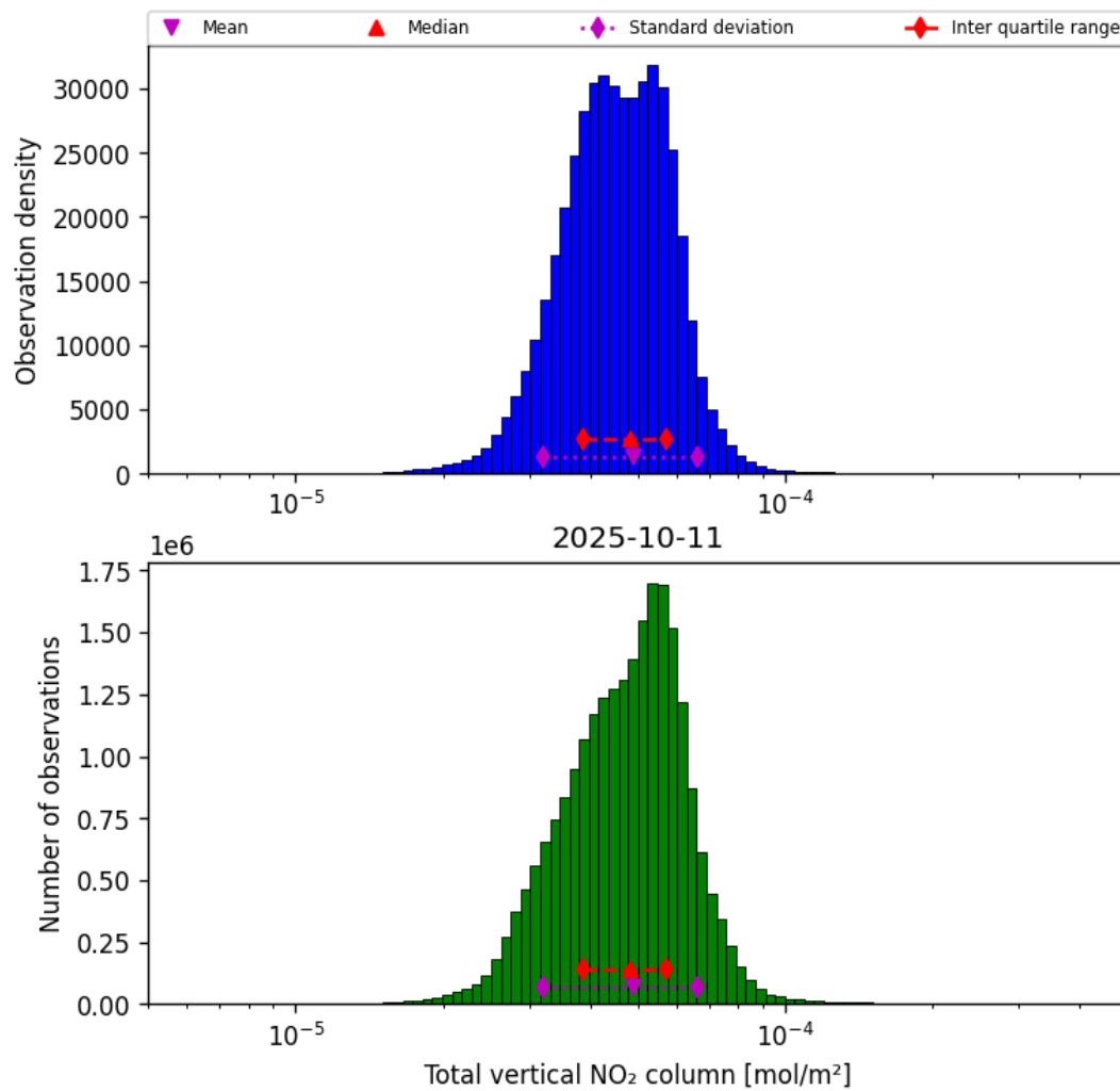
Figure 36: Histogram of “Total vertical NO 2 column” for 2025-10-11 to 2025-10-12
