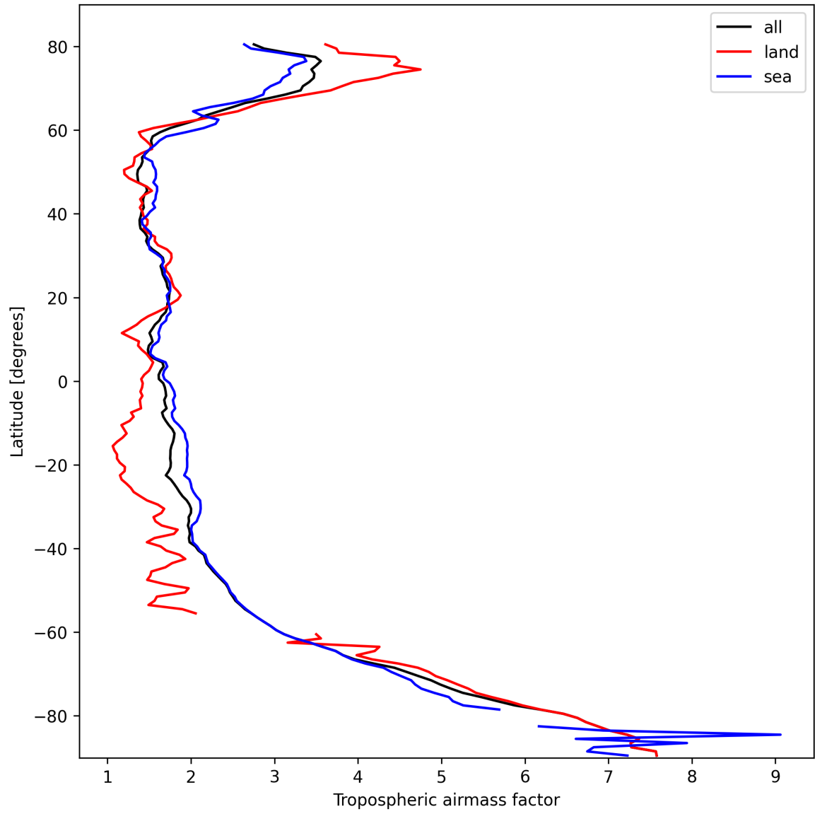
Figure 12: Zonal average of “Tropospheric airmass factor” for 2025-10-11 to 2025-10-12.
