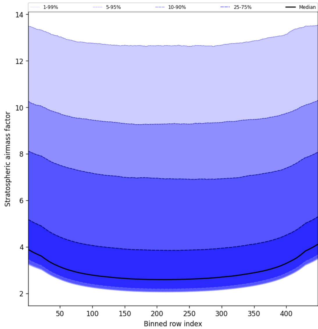
Figure 59: Along track statistics of “Stratospheric airmass factor” for 2025-10-11 to 2025-10-12
