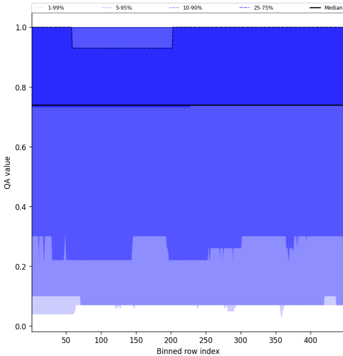
Figure 43: Along track statistics of “QA value” for 2025-10-11 to 2025-10-12
