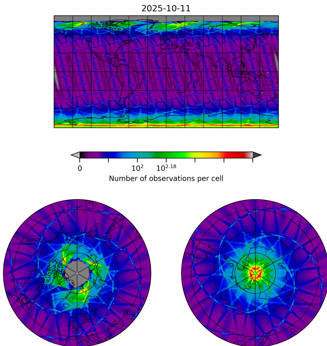
Figure 8: Map of the number of observations for 2025-10-11 to 2025-10-12
