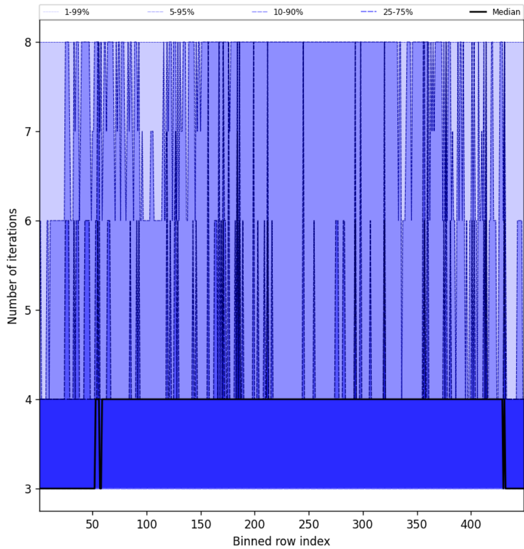
Figure 49: Along track statistics of “Number of iterations” for 2025-10-11 to 2025-10-12
