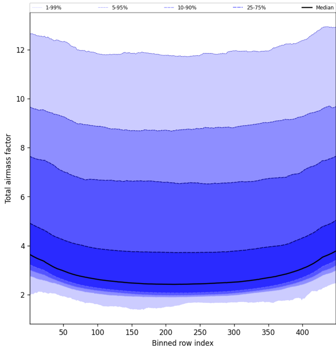
Figure 47: Along track statistics of “Total airmass factor” for 2025-10-11 to 2025-10-12
