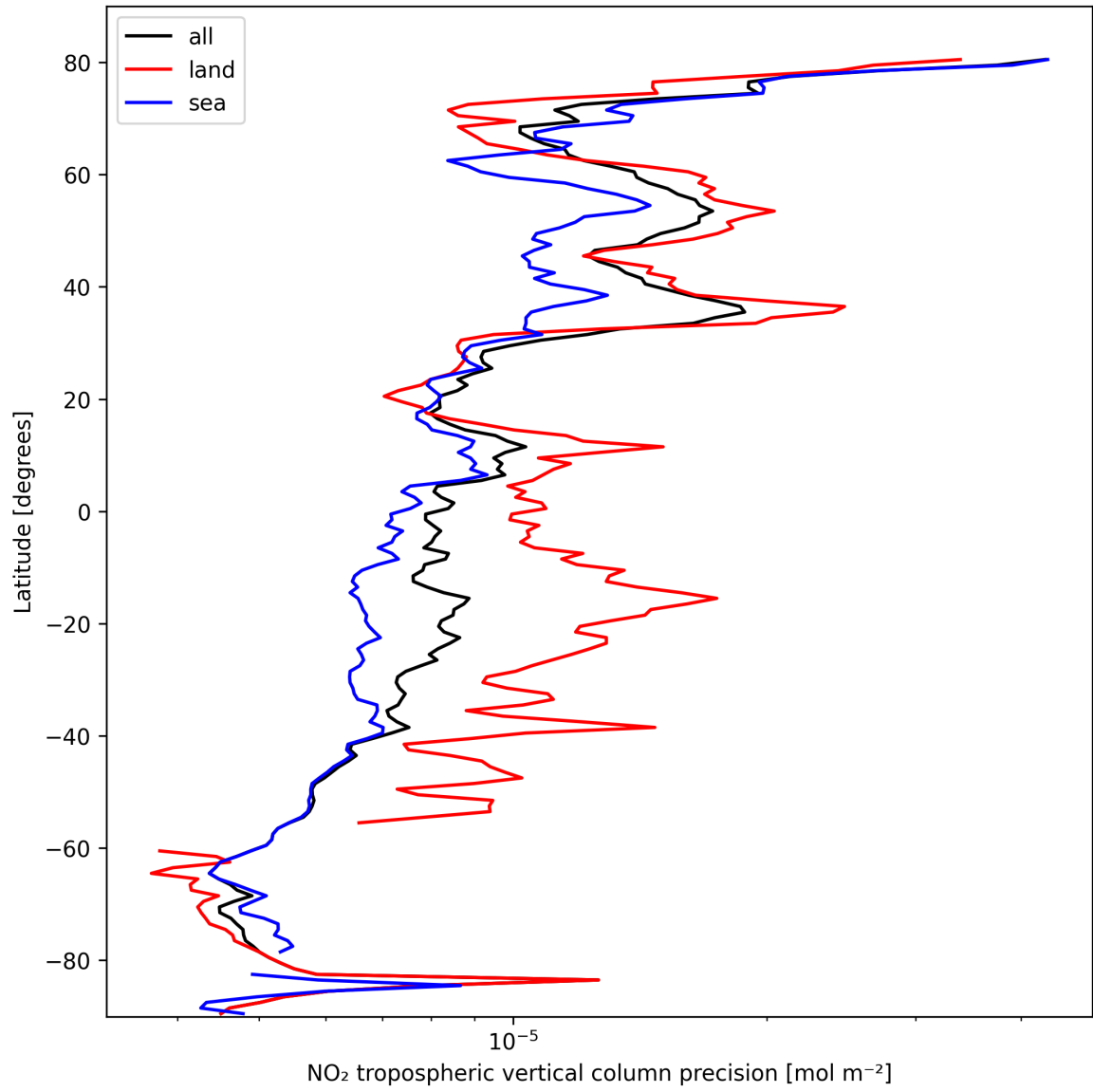
Figure 11: Zonal average of “NO 2 tropospheric vertical column precision” for 2025-10-11 to 2025-10-12.
