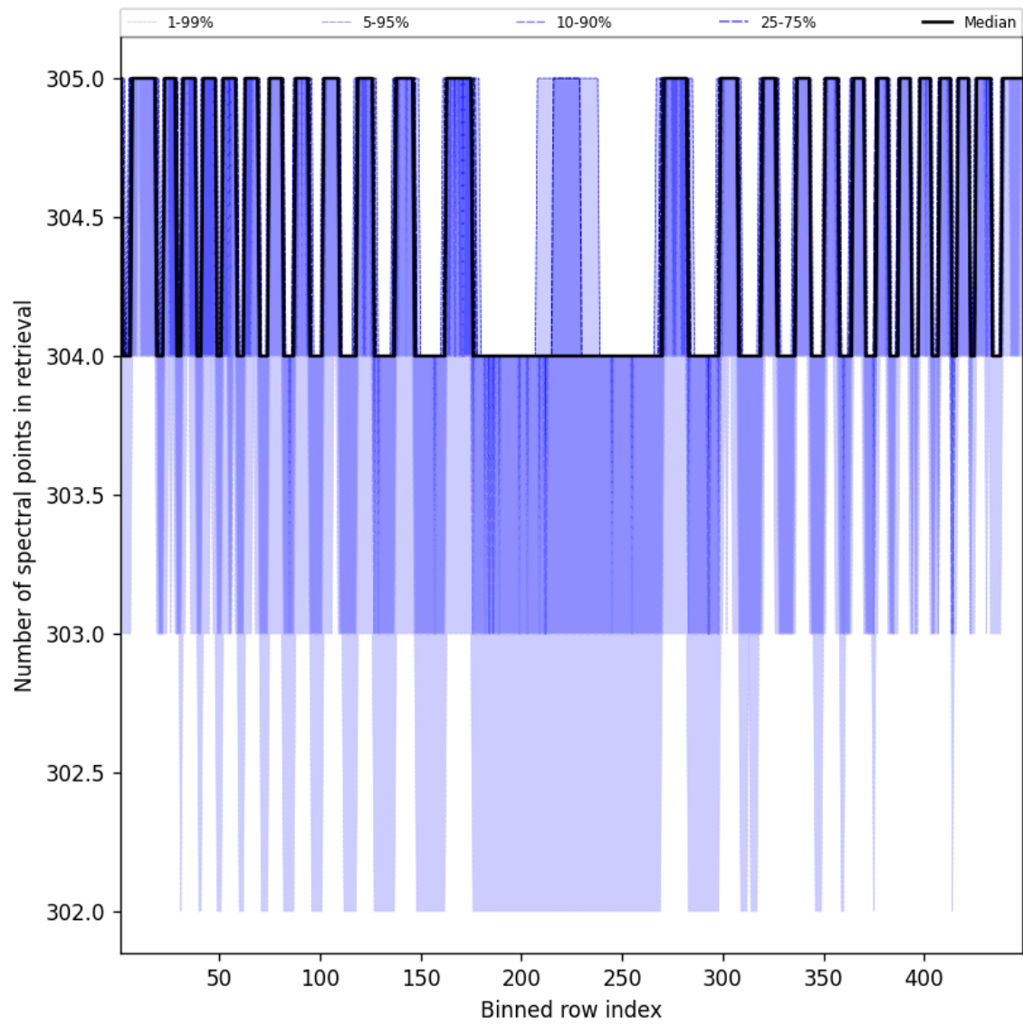
Figure 48: Along track statistics of “Number of spectral points in retrieval” for 2025-10-11 to 2025-10-12
