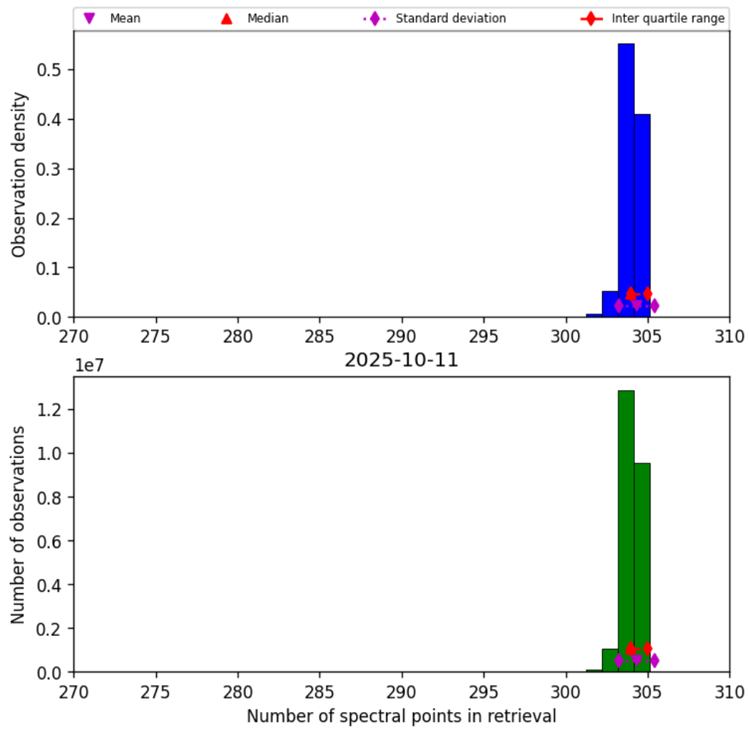
Figure 31: Histogram of “Number of spectral points in retrieval” for 2025-10-11 to 2025-10-12
