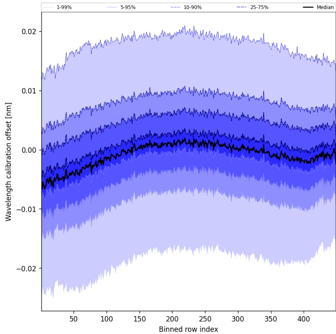
Figure 50: Along track statistics of “Wavelength calibration offset” for 2025-10-11 to 2025-10-12
