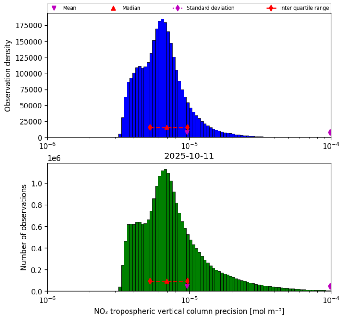
Figure 28: Histogram of “NO 2 tropospheric vertical column precision” for 2025-10-11 to 2025-10-12
