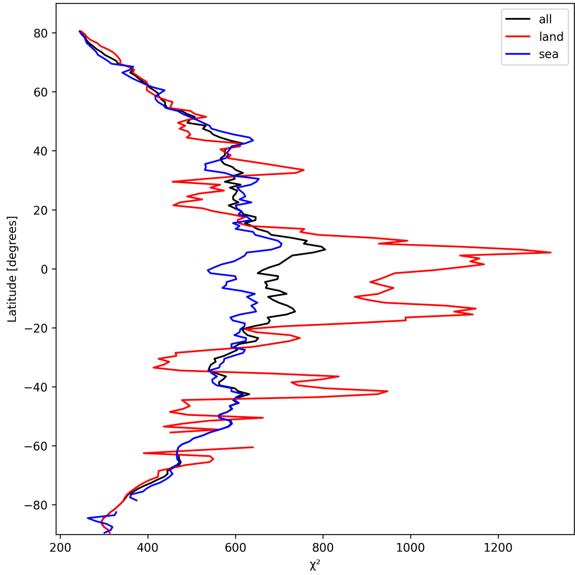
Figure 23: Zonal average of “ \chi^2 ” for 2025-10-11 to 2025-10-12.
