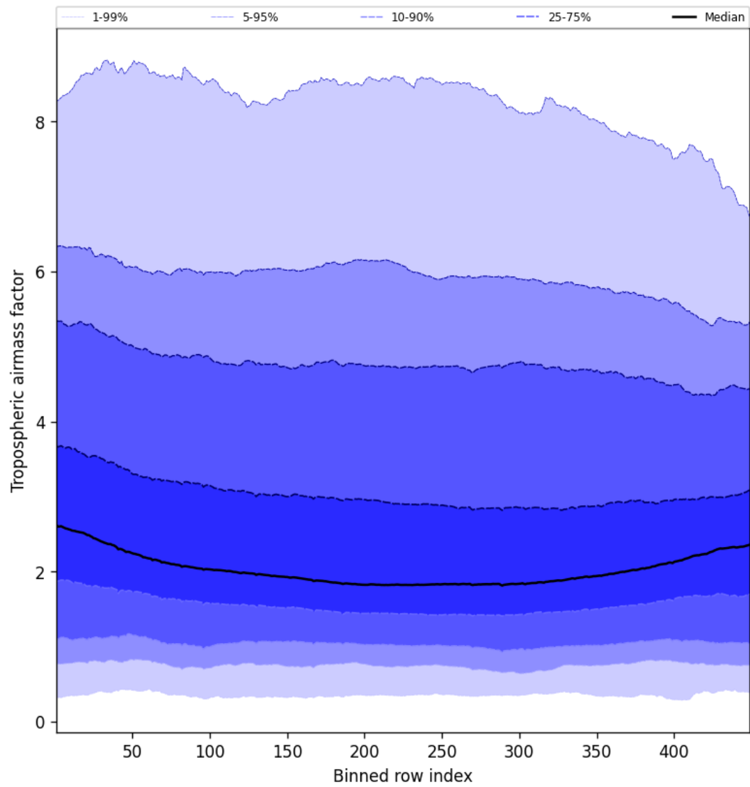
Figure 46: Along track statistics of “Tropospheric airmass factor” for 2025-10-11 to 2025-10-12
