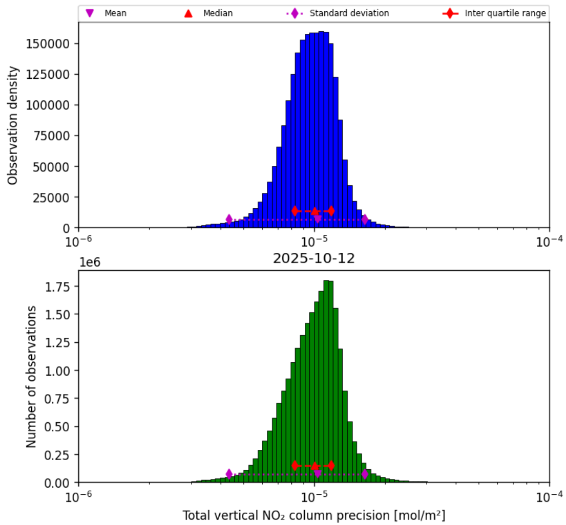
Figure 37: Histogram of “Total vertical NO 2 column precision” for 2025-10-12 to 2025-10-13
