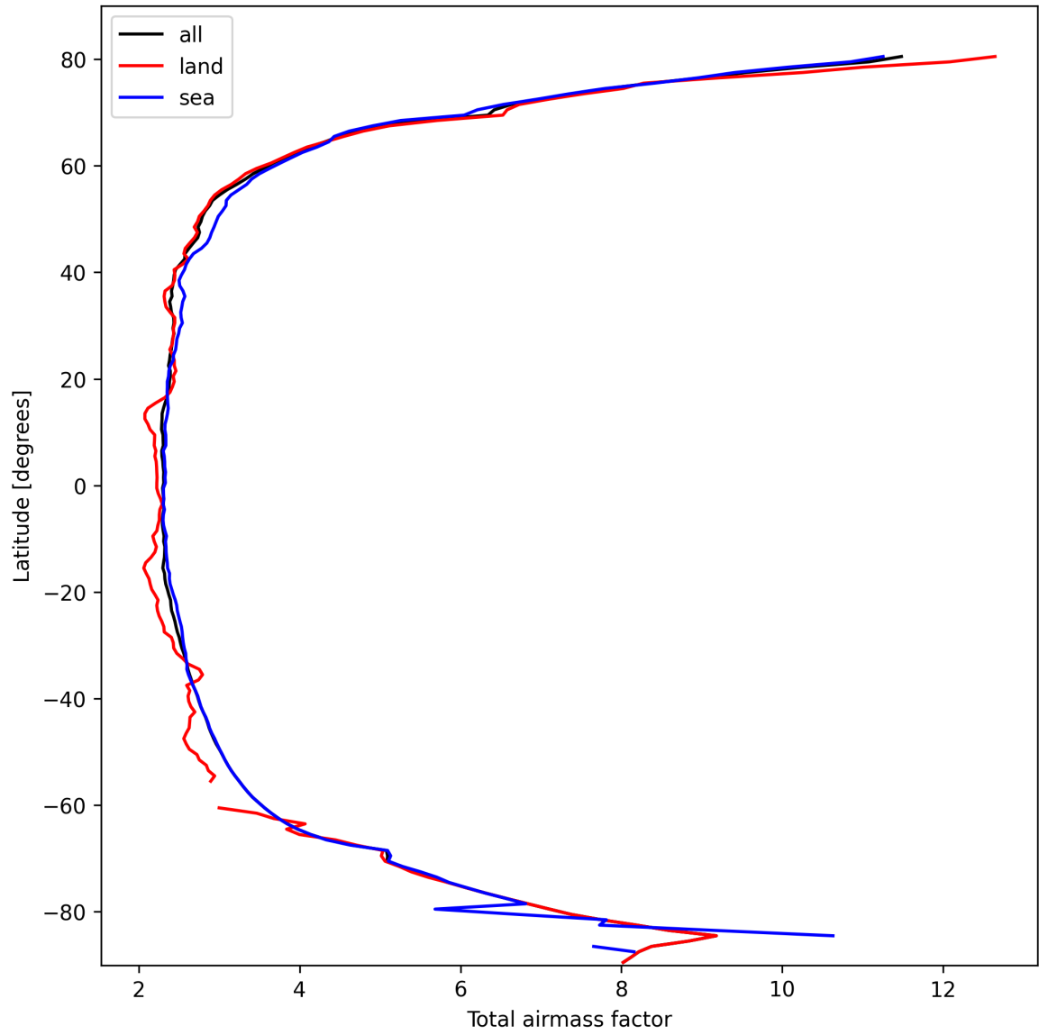
Figure 13: Zonal average of “Total airmass factor” for 2025-10-12 to 2025-10-13.
