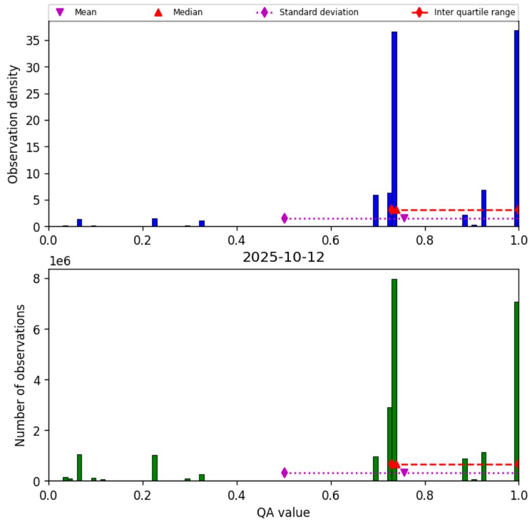
Figure 26: Histogram of “QA value” for 2025-10-12 to 2025-10-13
