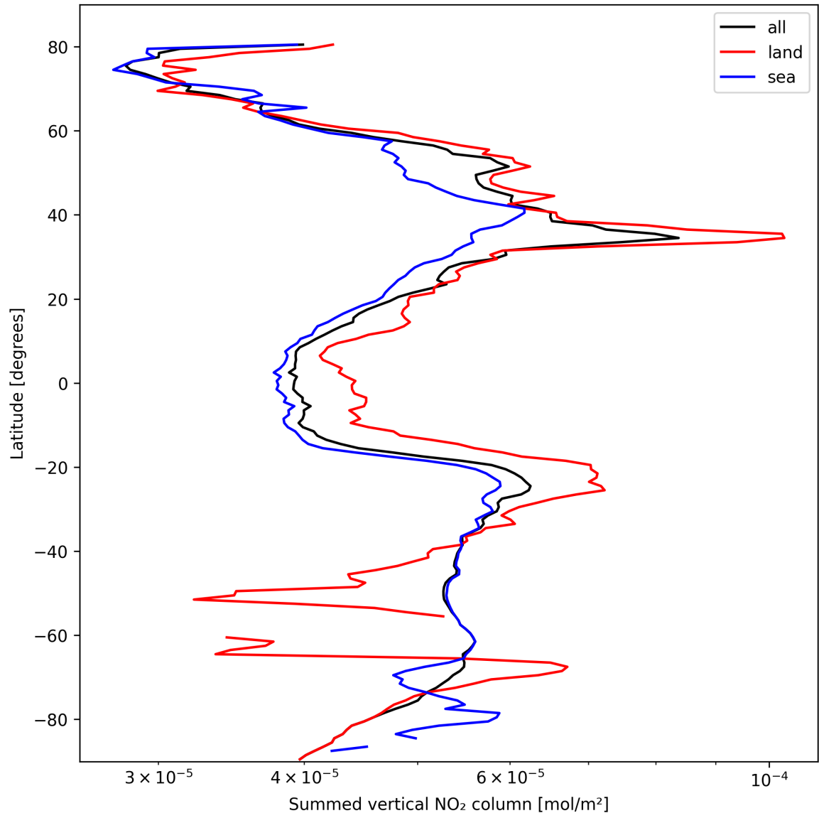
Figure 21: Zonal average of “Summed vertical NO 2 column” for 2025-10-12 to 2025-10-13.
