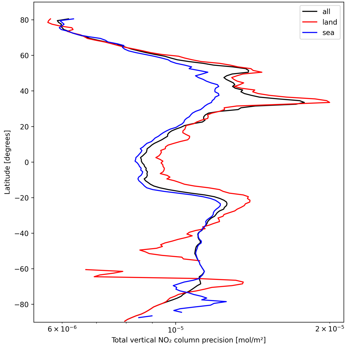
Figure 20: Zonal average of "Total vertical NO 2 column precision" for 2025-10-12 to 2025-10-13.
