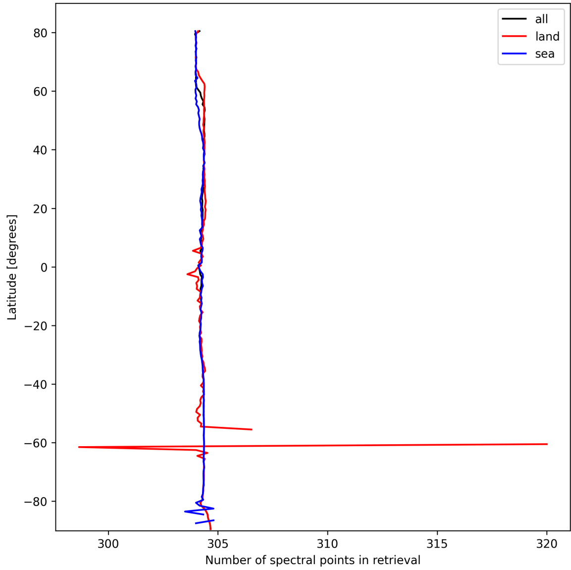
Figure 14: Zonal average of “Number of spectral points in retrieval” for 2025-10-12 to 2025-10-13.
