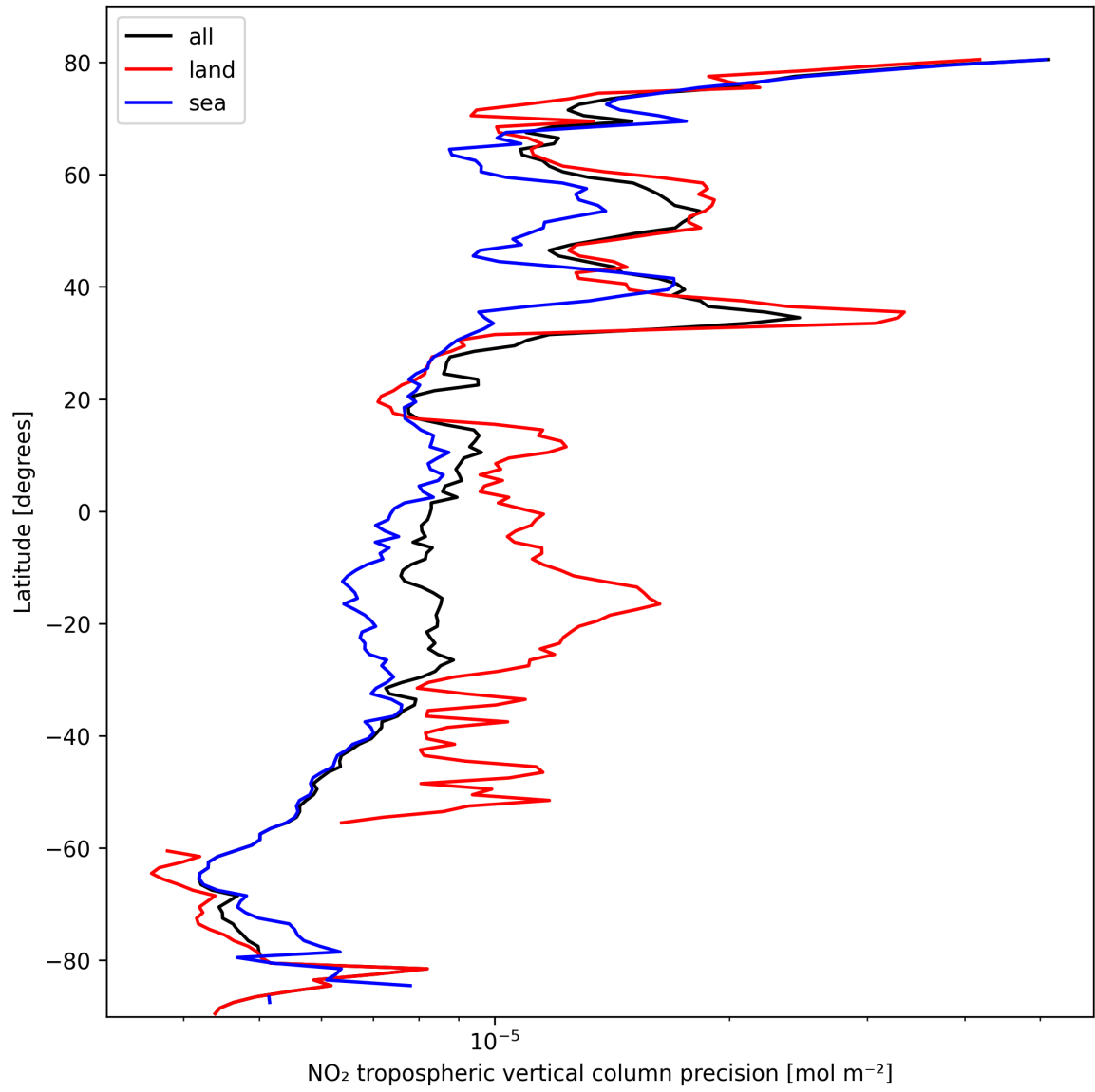
Figure 11: Zonal average of “NO 2 tropospheric vertical column precision” for 2025-10-12 to 2025-10-13.
