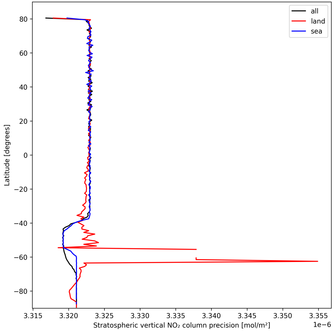
Figure 18: Zonal average of “Stratospheric vertical NO 2 column precision” for 2025-10-12 to 2025-10-13.
