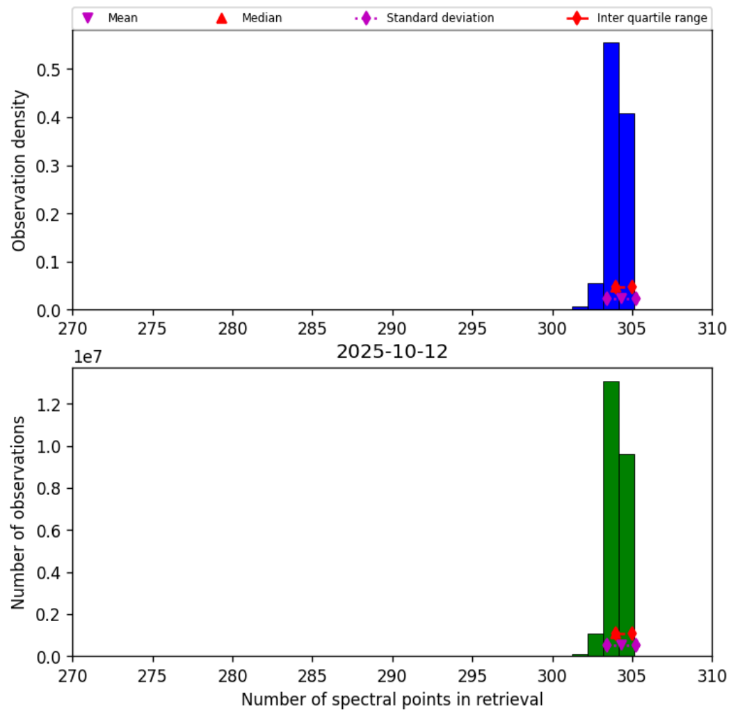
Figure 31: Histogram of “Number of spectral points in retrieval” for 2025-10-12 to 2025-10-13
