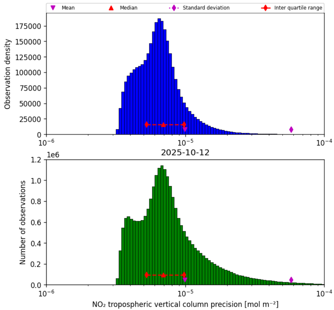
Figure 28: Histogram of “NO 2 tropospheric vertical column precision” for 2025-10-12 to 2025-10-13
