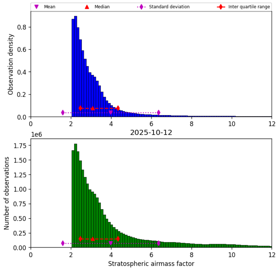
Figure 42: Histogram of “Stratospheric airmass factor” for 2025-10-12 to 2025-10-13
