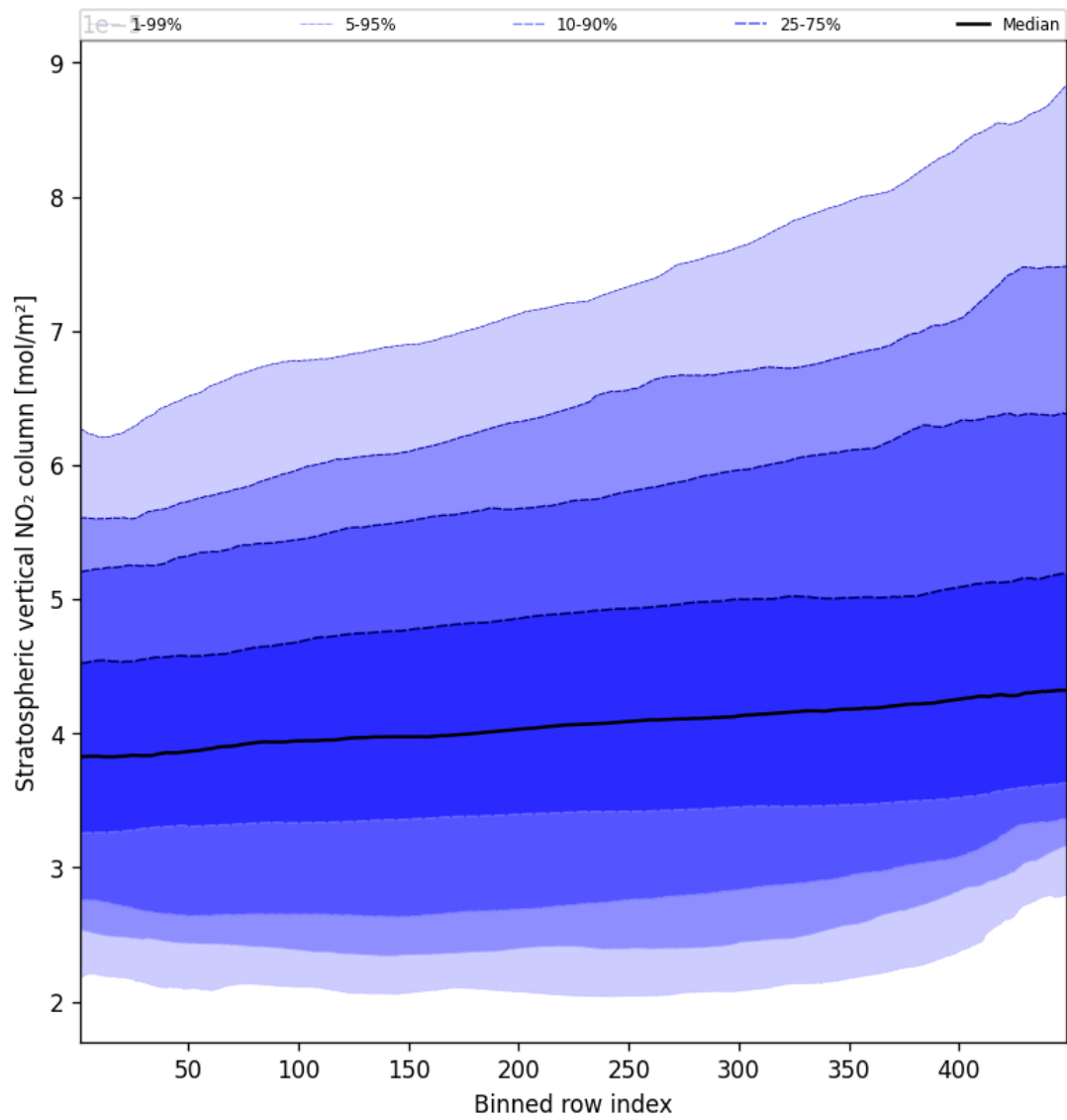
Figure 51: Along track statistics of “Stratospheric vertical NO 2 column” for 2025-10-12 to 2025-10-13
