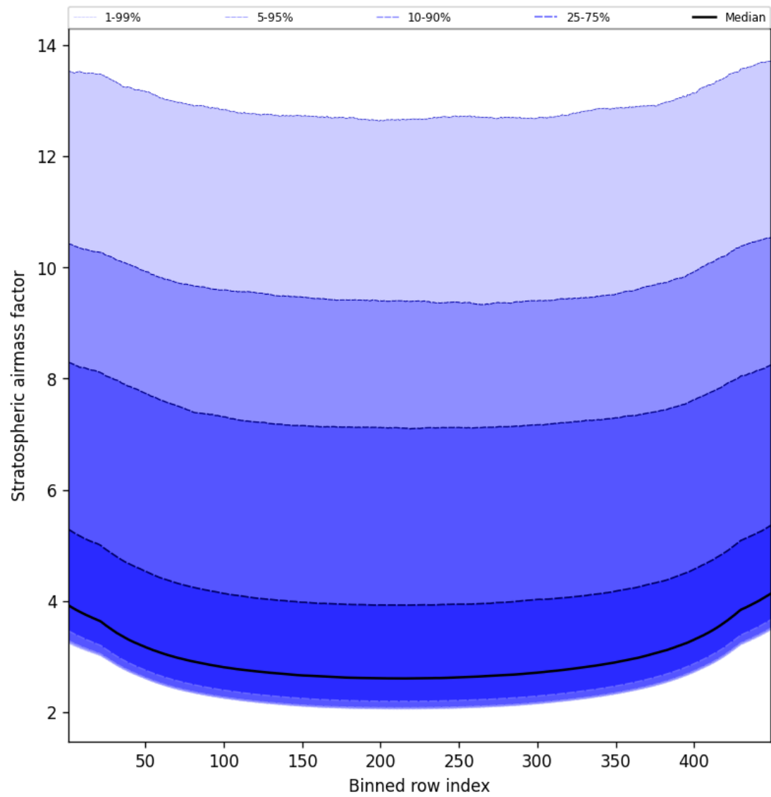
Figure 59: Along track statistics of “Stratospheric airmass factor” for 2025-10-12 to 2025-10-13
