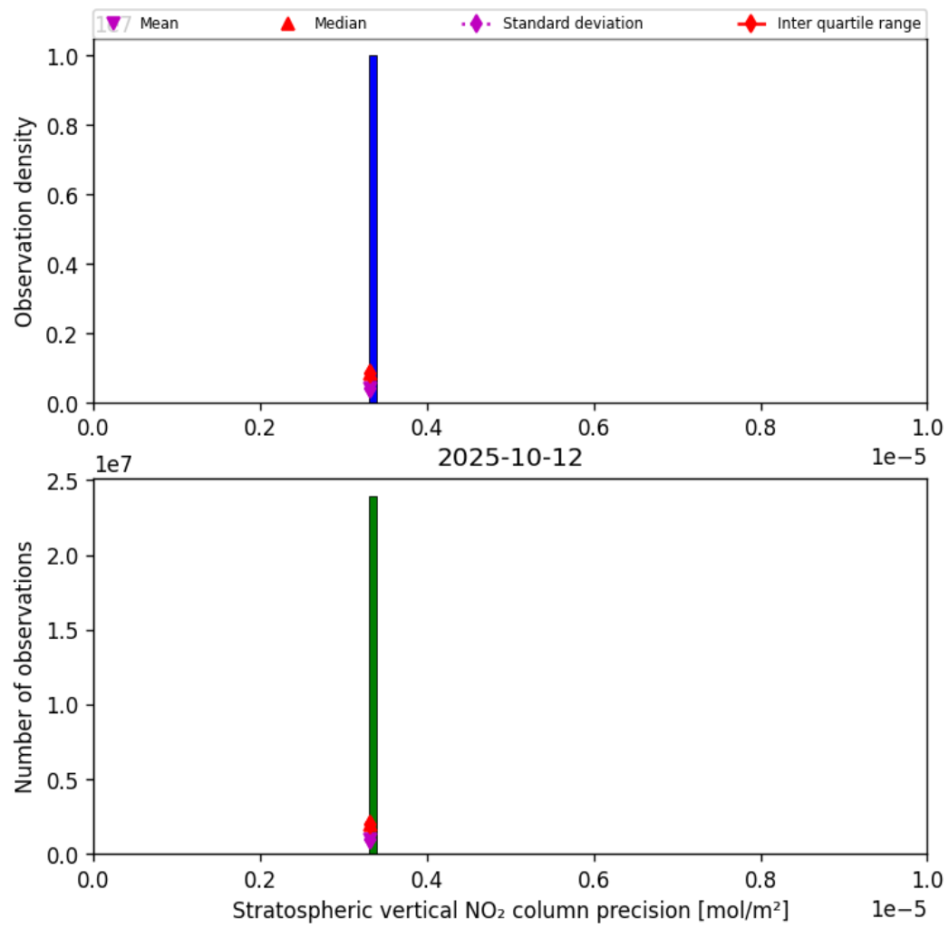
Figure 35: Histogram of “Stratospheric vertical NO 2 column precision” for 2025-10-12 to 2025-10-13
