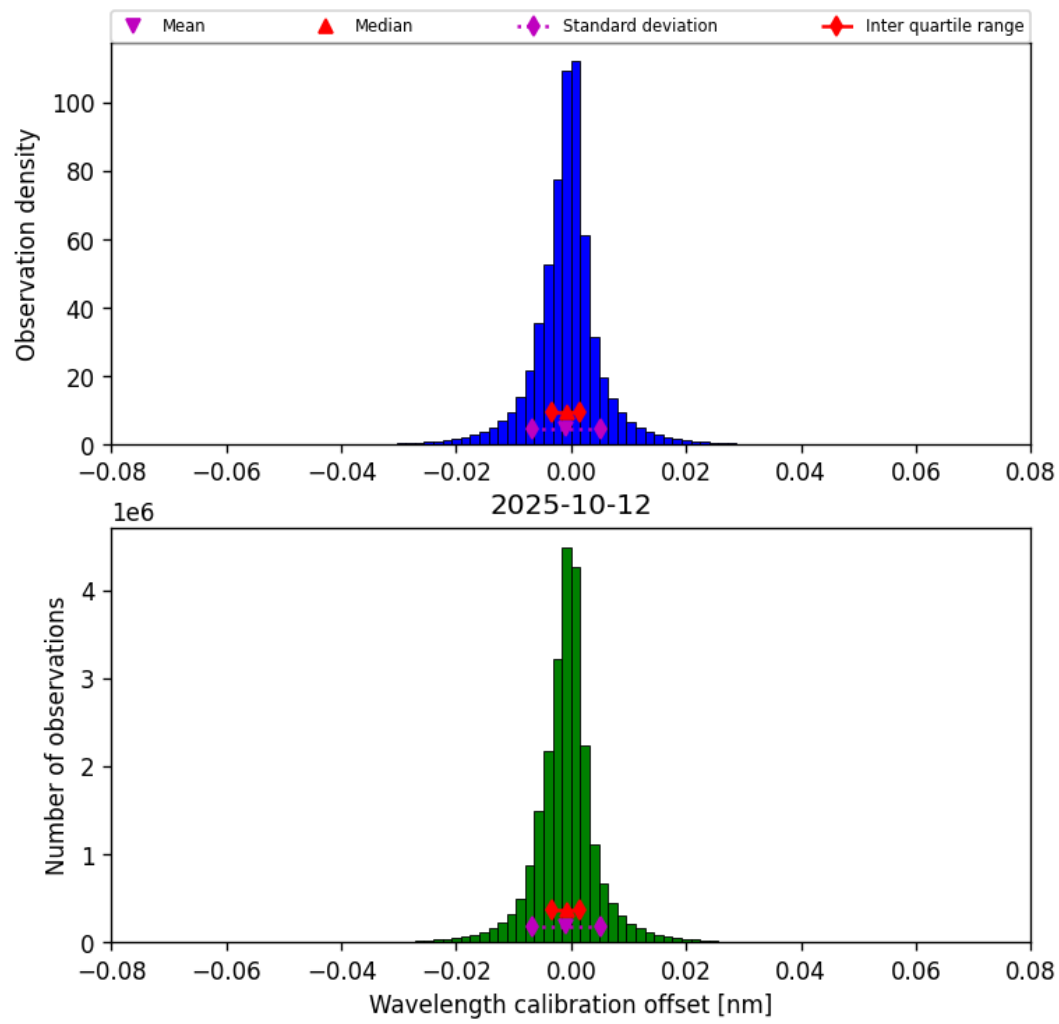
Figure 33: Histogram of “Wavelength calibration offset” for 2025-10-12 to 2025-10-13
