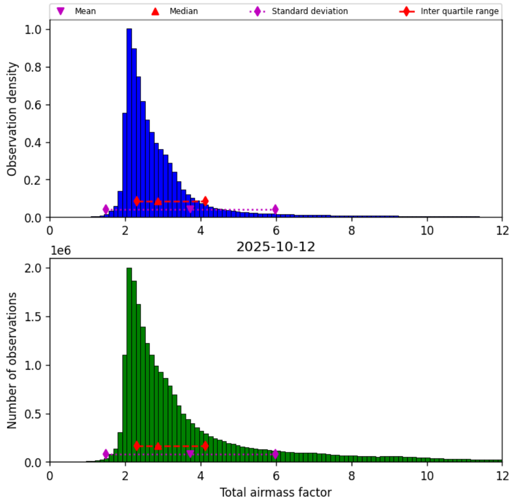
Figure 30: Histogram of “Total airmass factor” for 2025-10-12 to 2025-10-13
