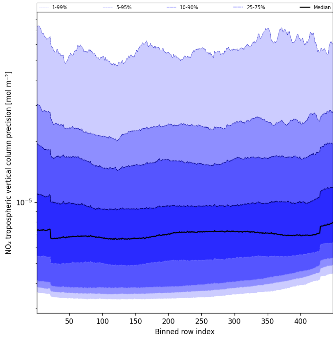
Figure 45: Along track statistics of “NO 2 tropospheric vertical column precision” for 2025-10-12 to 2025-10-13
