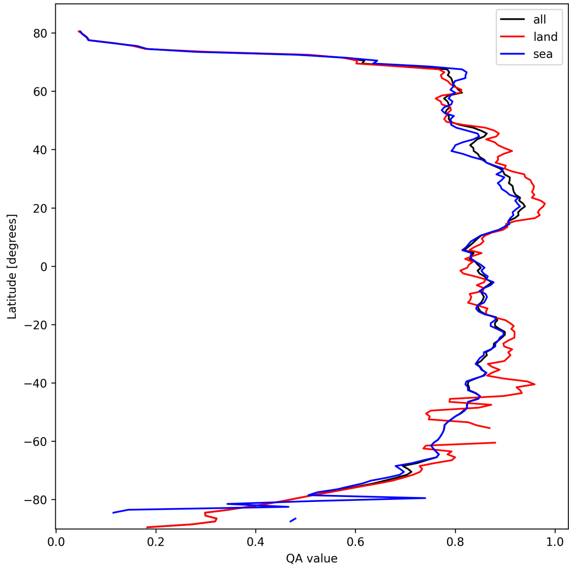
Figure 9: Zonal average of “QA value” for 2025-10-12 to 2025-10-13.
