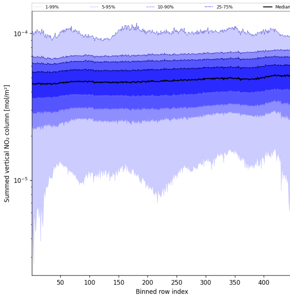
Figure 55: Along track statistics of “Summed vertical NO 2 column” for 2025-10-12 to 2025-10-13
