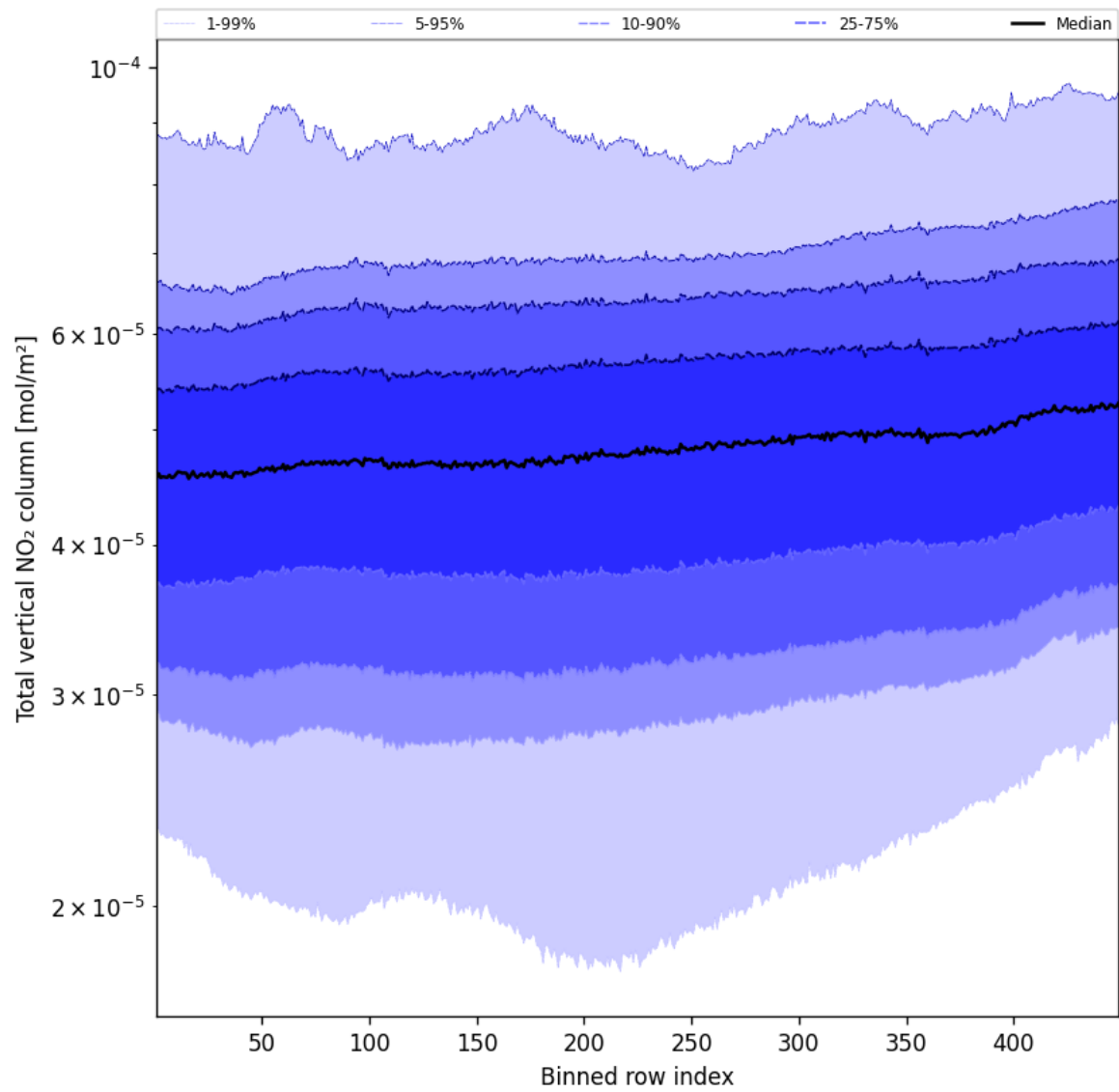
Figure 53: Along track statistics of “Total vertical NO 2 column” for 2025-10-12 to 2025-10-13
