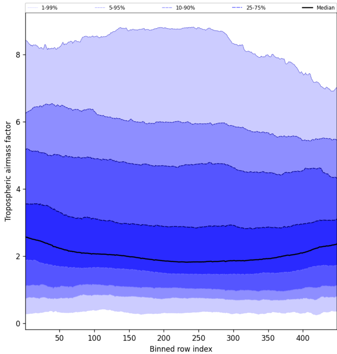
Figure 46: Along track statistics of “Tropospheric airmass factor” for 2025-10-12 to 2025-10-13
