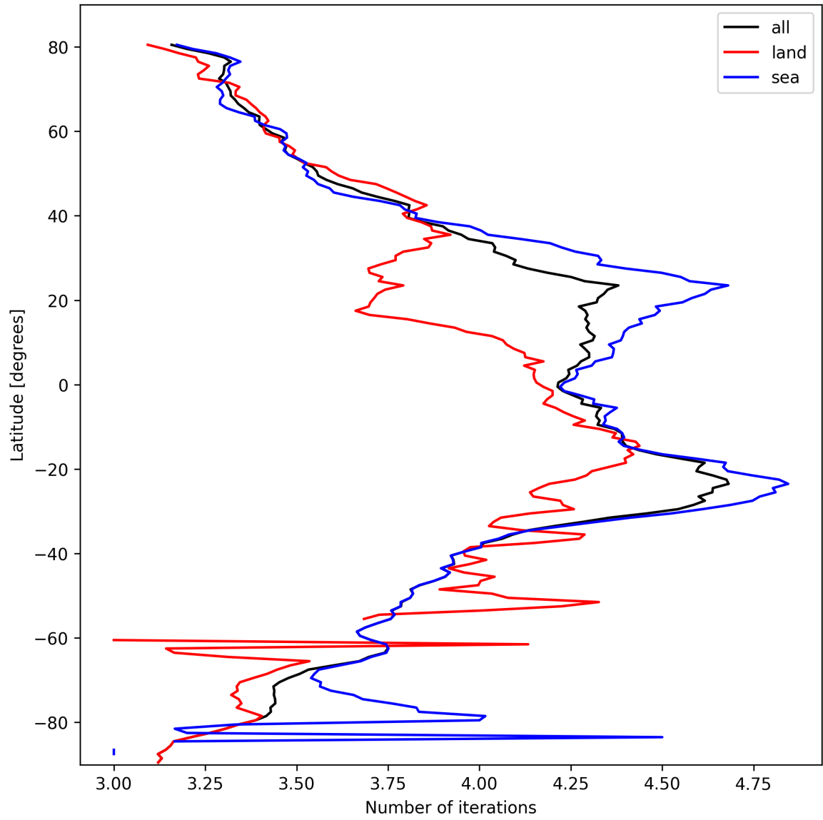
Figure 15: Zonal average of “Number of iterations” for 2025-10-12 to 2025-10-13.
