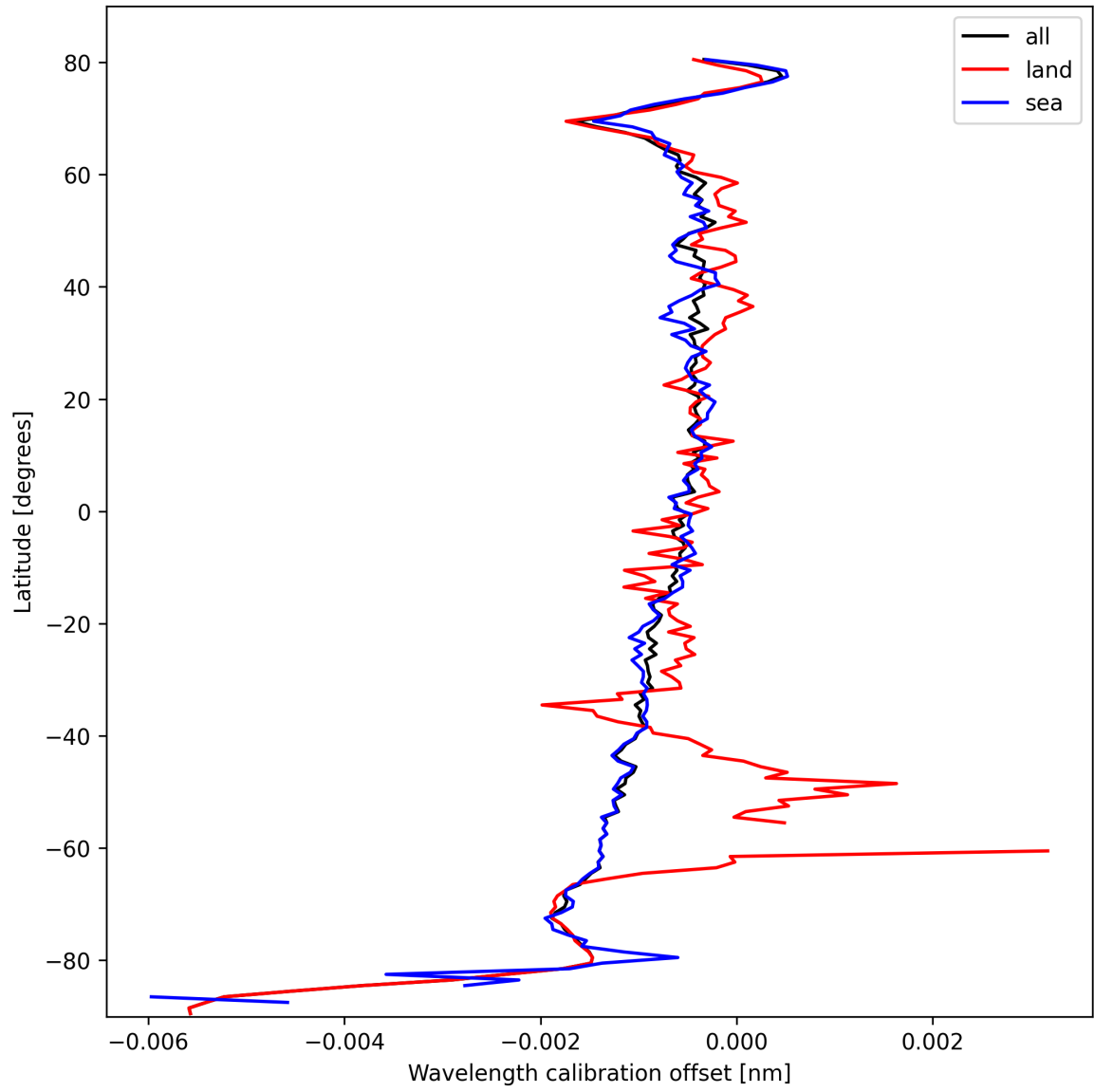
Figure 16: Zonal average of “Wavelength calibration offset” for 2025-10-12 to 2025-10-13.
