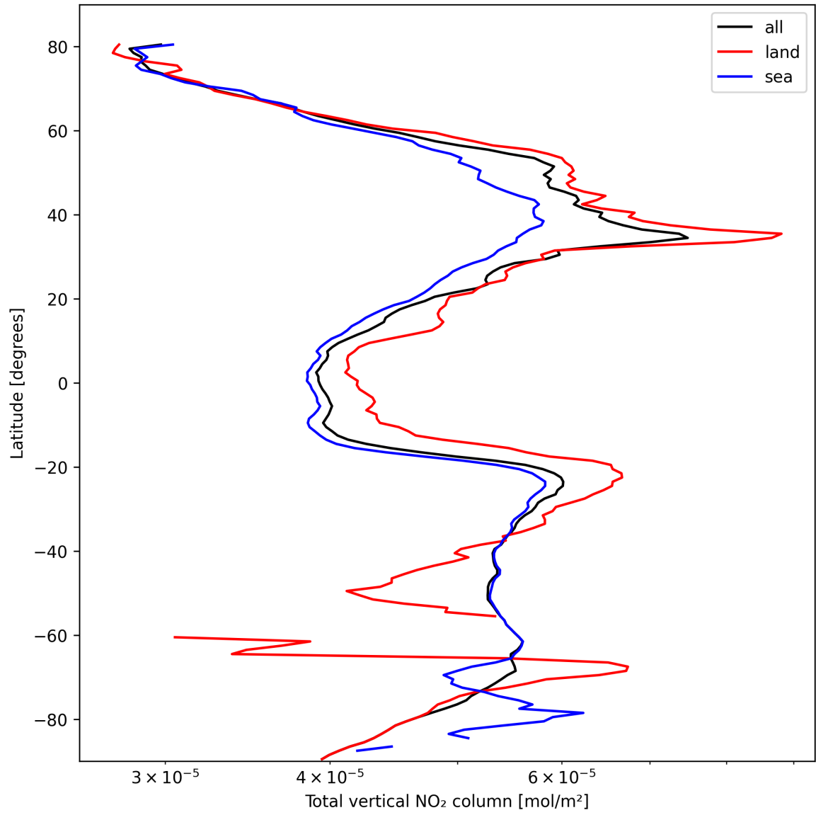
Figure 19: Zonal average of “Total vertical NO 2 column” for 2025-10-12 to 2025-10-13.
