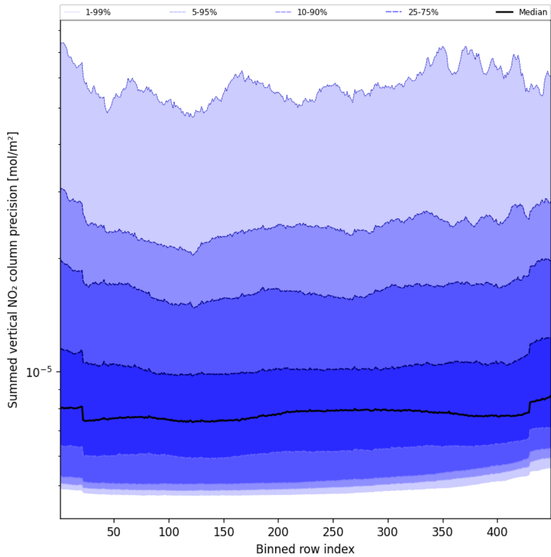
Figure 56: Along track statistics of “Summed vertical NO 2 column precision” for 2025-10-12 to 2025-10-13
