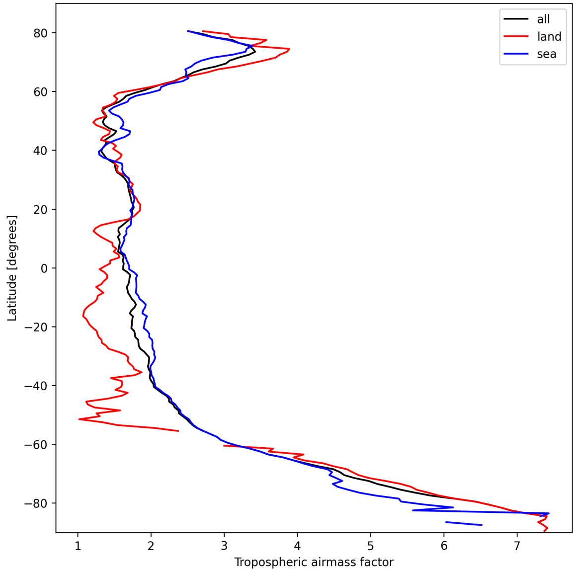
Figure 12: Zonal average of “Tropospheric airmass factor” for 2025-10-12 to 2025-10-13.
