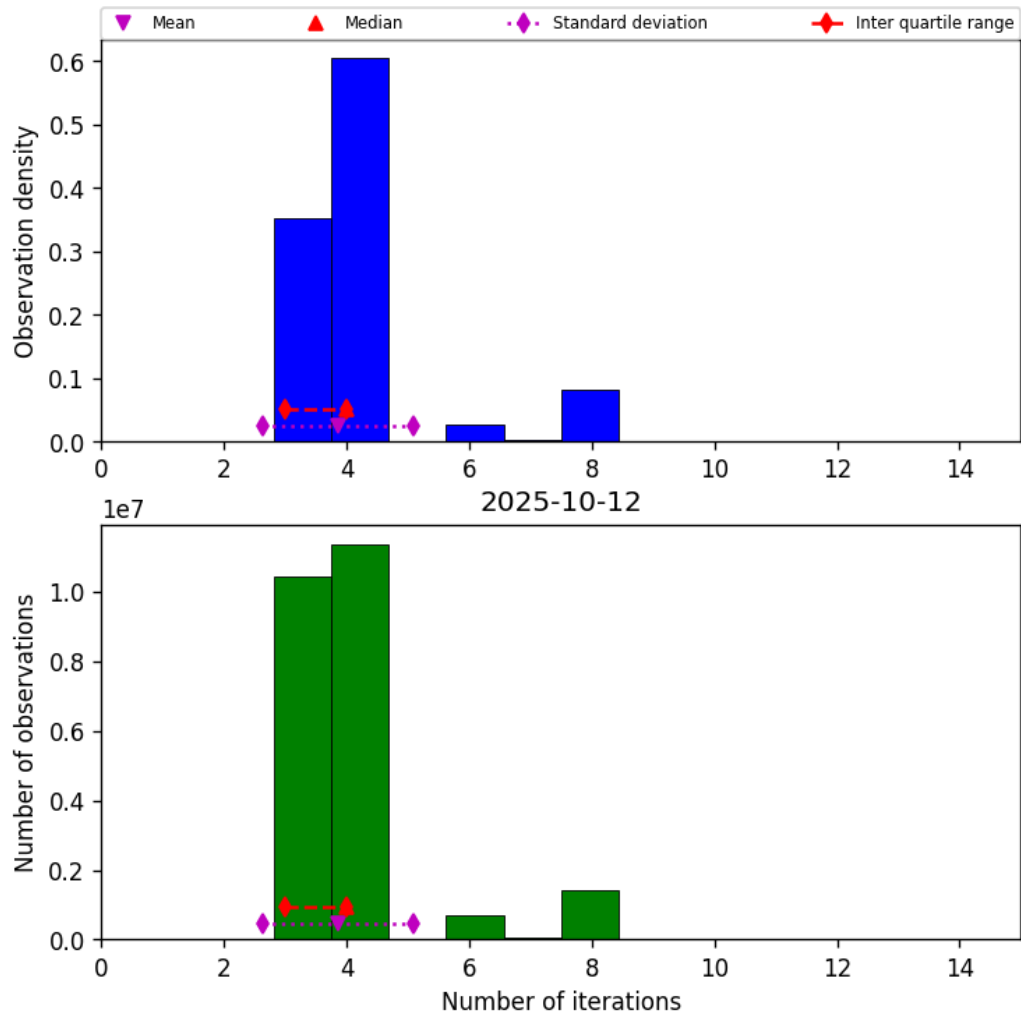
Figure 32: Histogram of “Number of iterations” for 2025-10-12 to 2025-10-13
