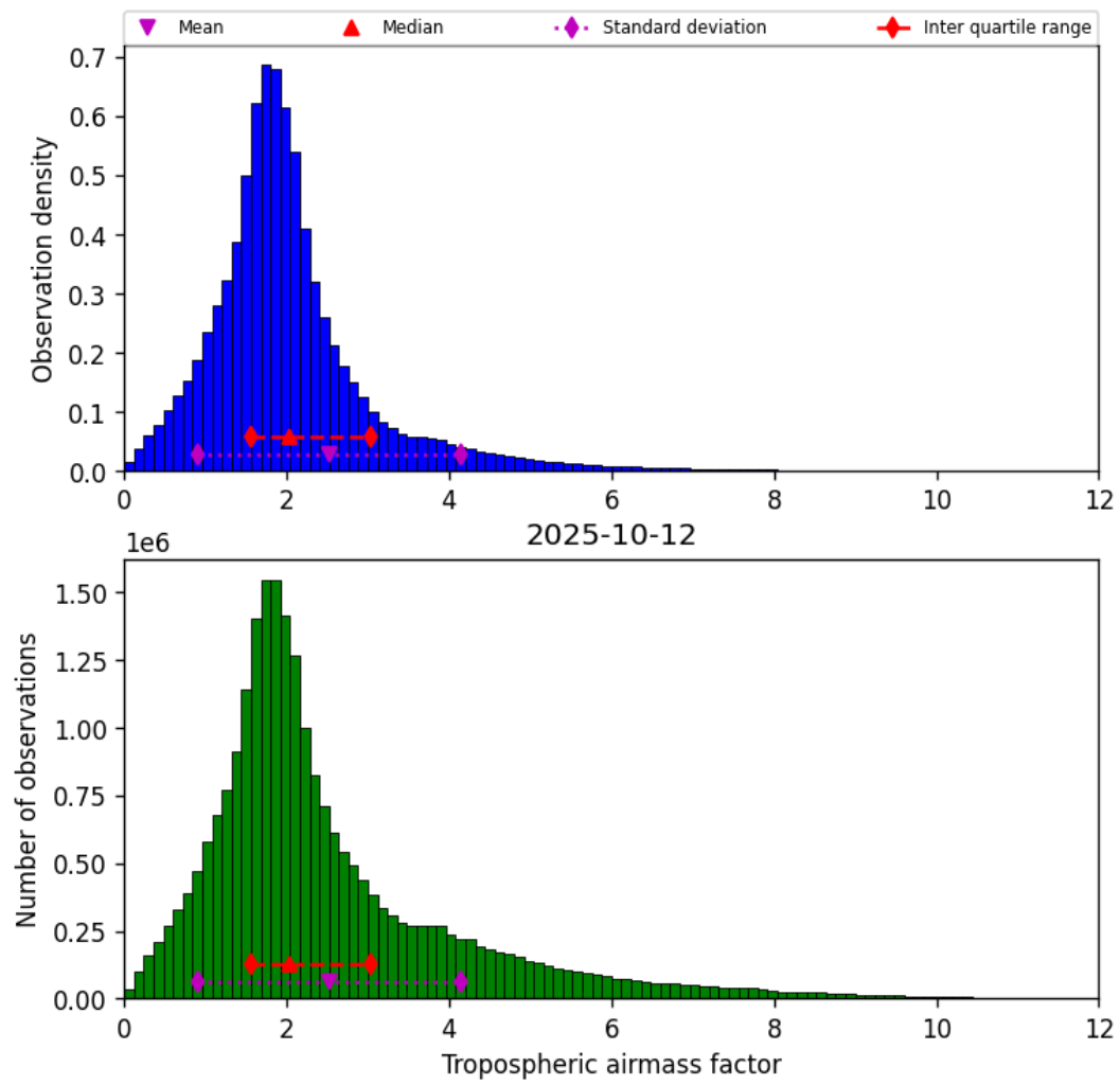
Figure 29: Histogram of “Tropospheric airmass factor” for 2025-10-12 to 2025-10-13
