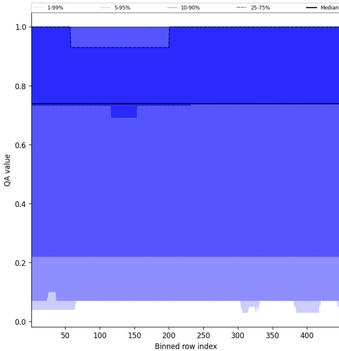
Figure 43: Along track statistics of “QA value” for 2025-10-12 to 2025-10-13
