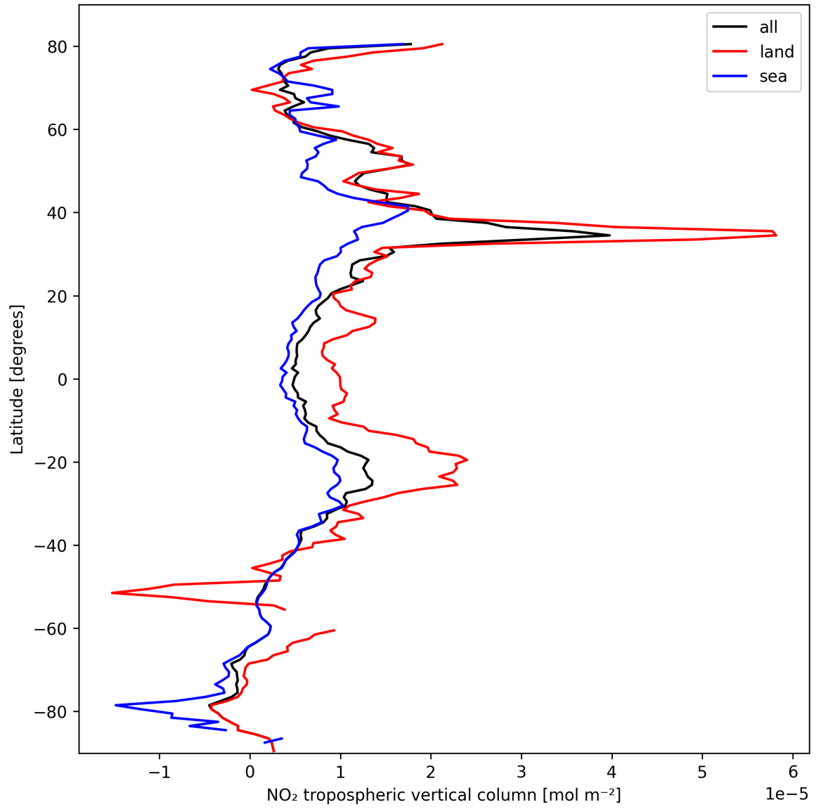
Figure 10: Zonal average of “NO 2 tropospheric vertical column” for 2025-10-12 to 2025-10-13.
