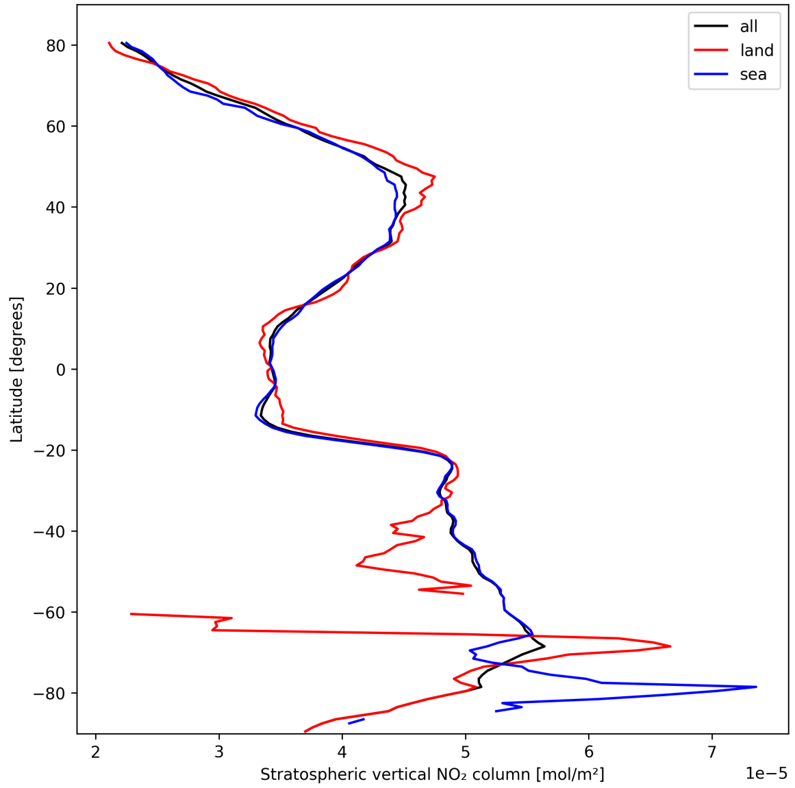
Figure 17: Zonal average of “Stratospheric vertical NO 2 column” for 2025-10-12 to 2025-10-13.
