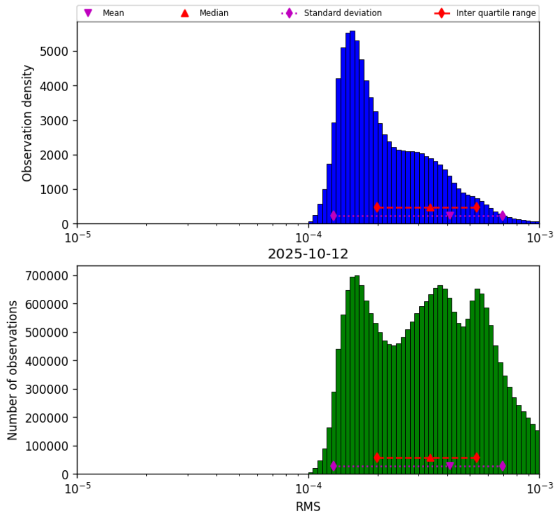
Figure 41: Histogram of “RMS” for 2025-10-12 to 2025-10-13
