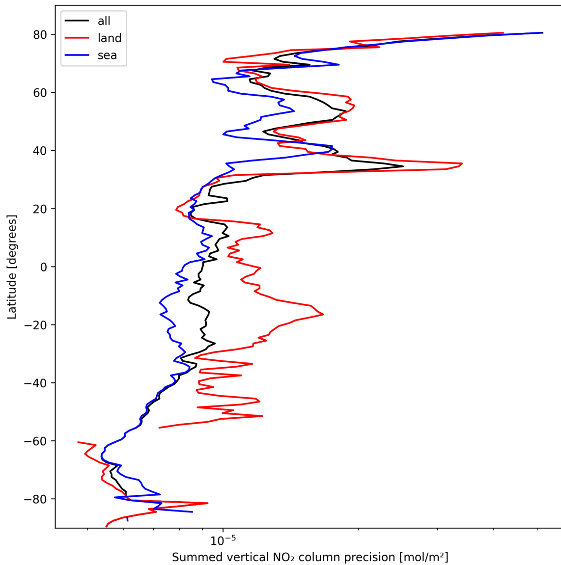
Figure 22: Zonal average of “Summed vertical NO 2 column precision” for 2025-10-12 to 2025-10-13.
