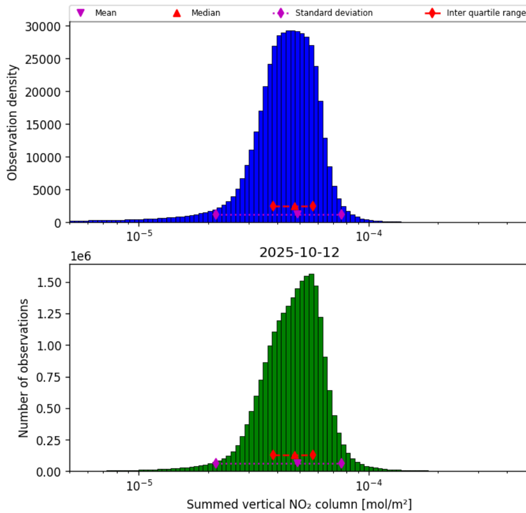
Figure 38: Histogram of “Summed vertical NO 2 column” for 2025-10-12 to 2025-10-13
