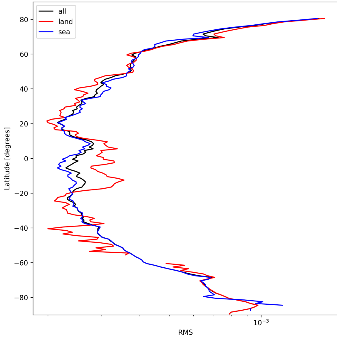
Figure 24: Zonal average of “RMS” for 2025-10-12 to 2025-10-13.
