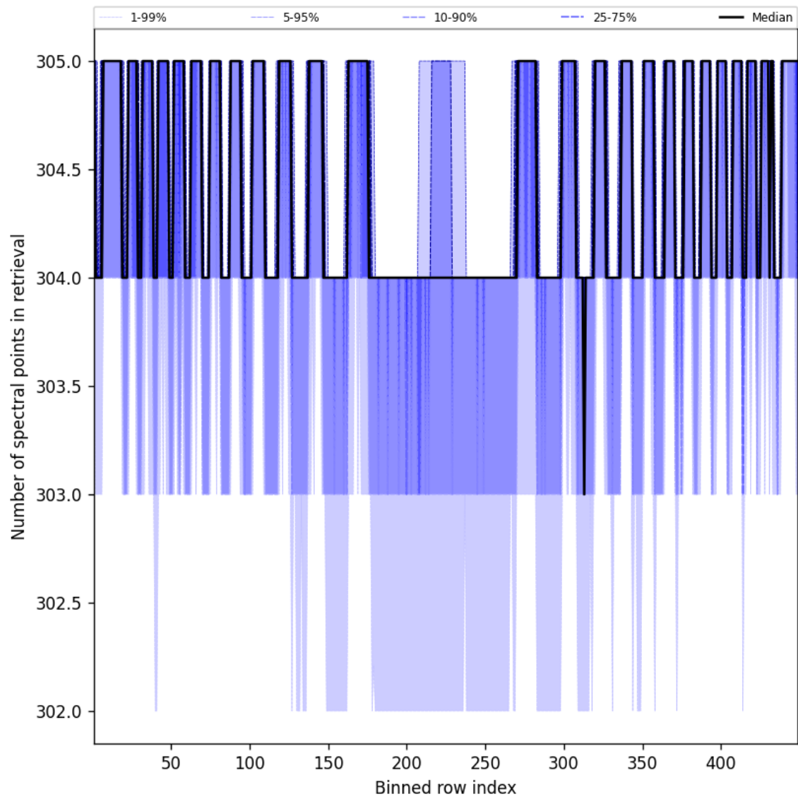
Figure 48: Along track statistics of “Number of spectral points in retrieval” for 2025-10-12 to 2025-10-13
