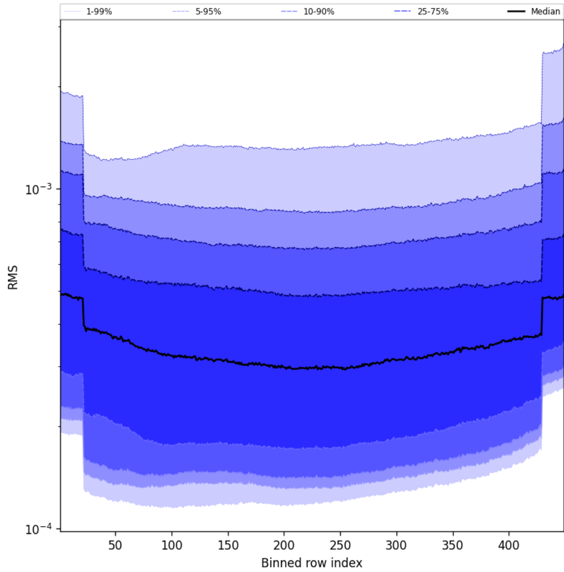
Figure 58: Along track statistics of “RMS” for 2025-10-12 to 2025-10-13
