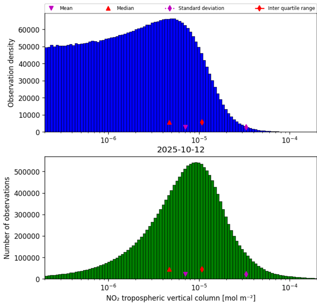
Figure 27: Histogram of “NO 2 tropospheric vertical column” for 2025-10-12 to 2025-10-13
