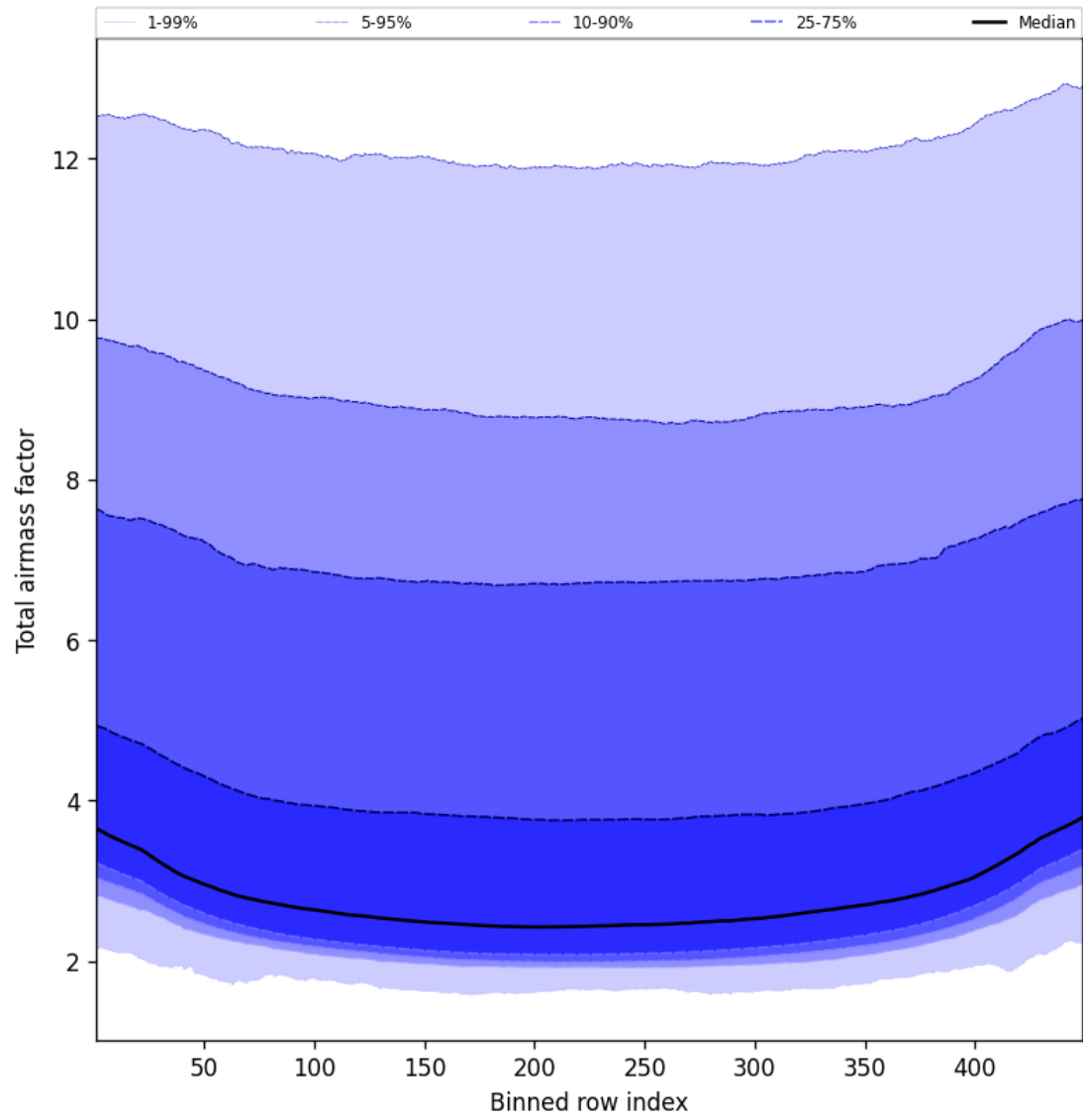
Figure 47: Along track statistics of “Total airmass factor” for 2025-10-12 to 2025-10-13
