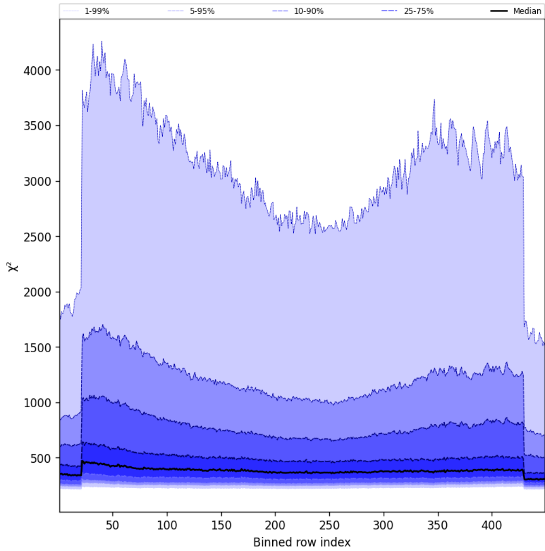
Figure 57: Along track statistics of “ \chi^2 ” for 2025-10-12 to 2025-10-13
