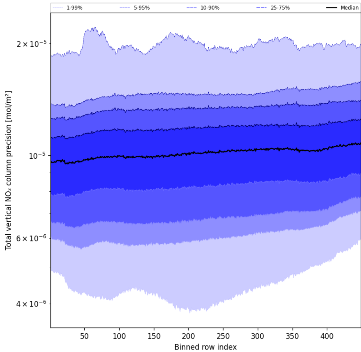
Figure 54: Along track statistics of “Total vertical NO 2 column precision” for 2025-10-12 to 2025-10-13
