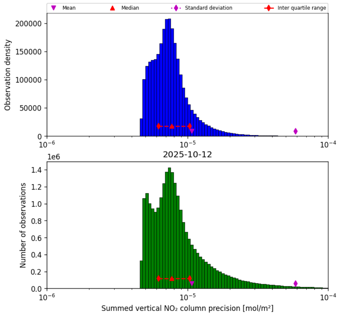
Figure 39: Histogram of “Summed vertical NO 2 column precision” for 2025-10-12 to 2025-10-13
