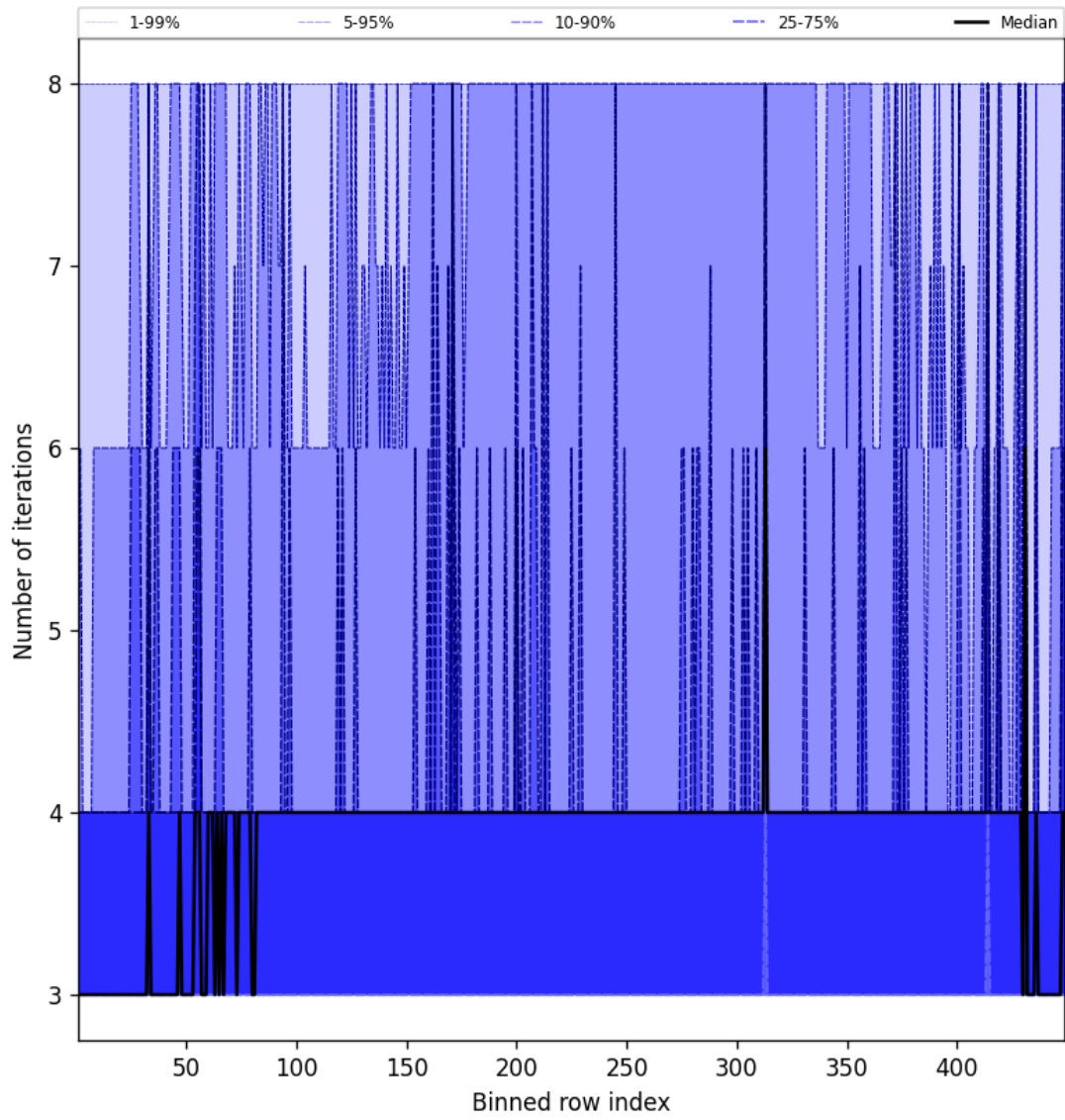
Figure 49: Along track statistics of “Number of iterations” for 2025-10-12 to 2025-10-13
