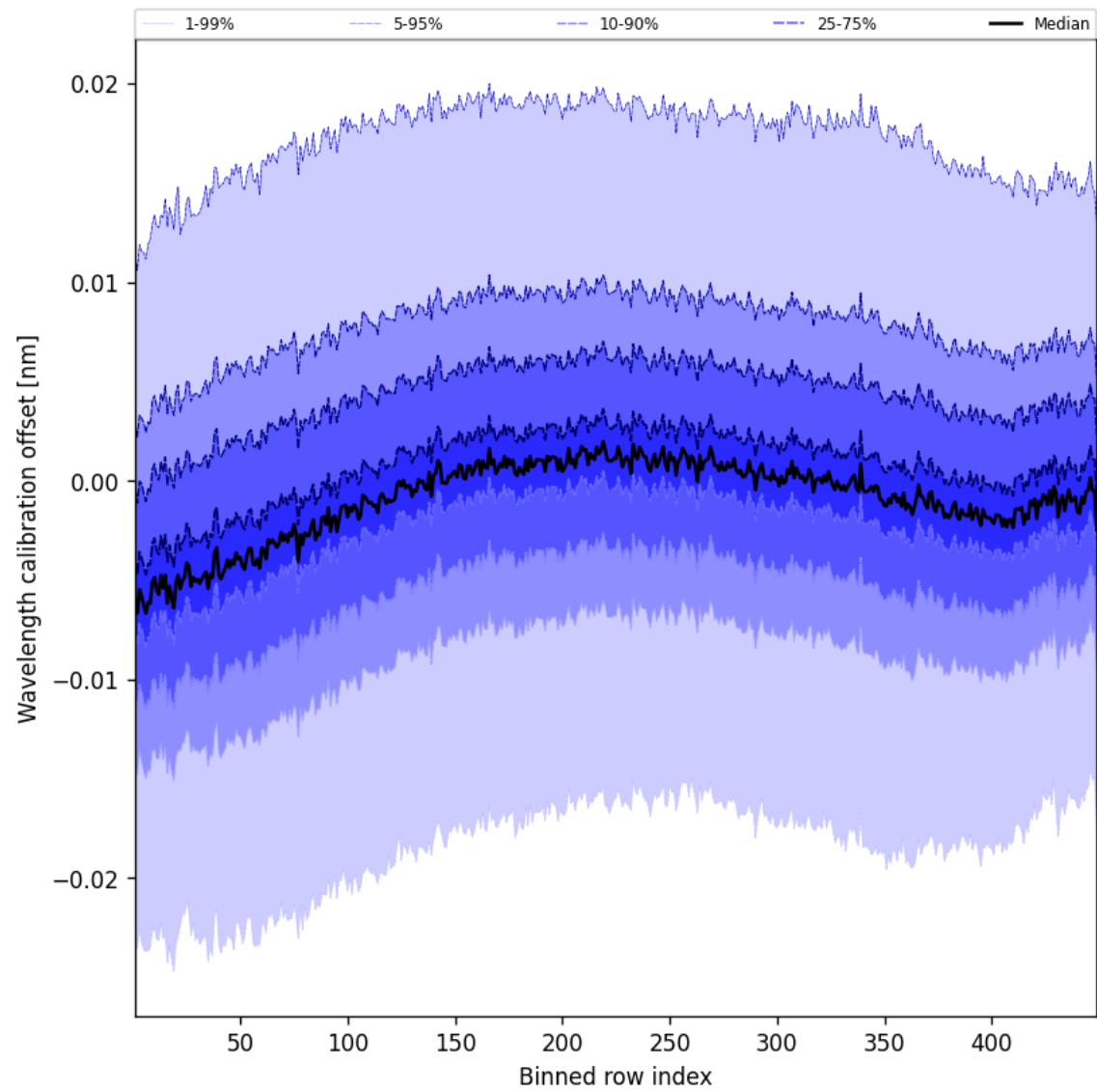
Figure 50: Along track statistics of “Wavelength calibration offset” for 2025-10-12 to 2025-10-13
