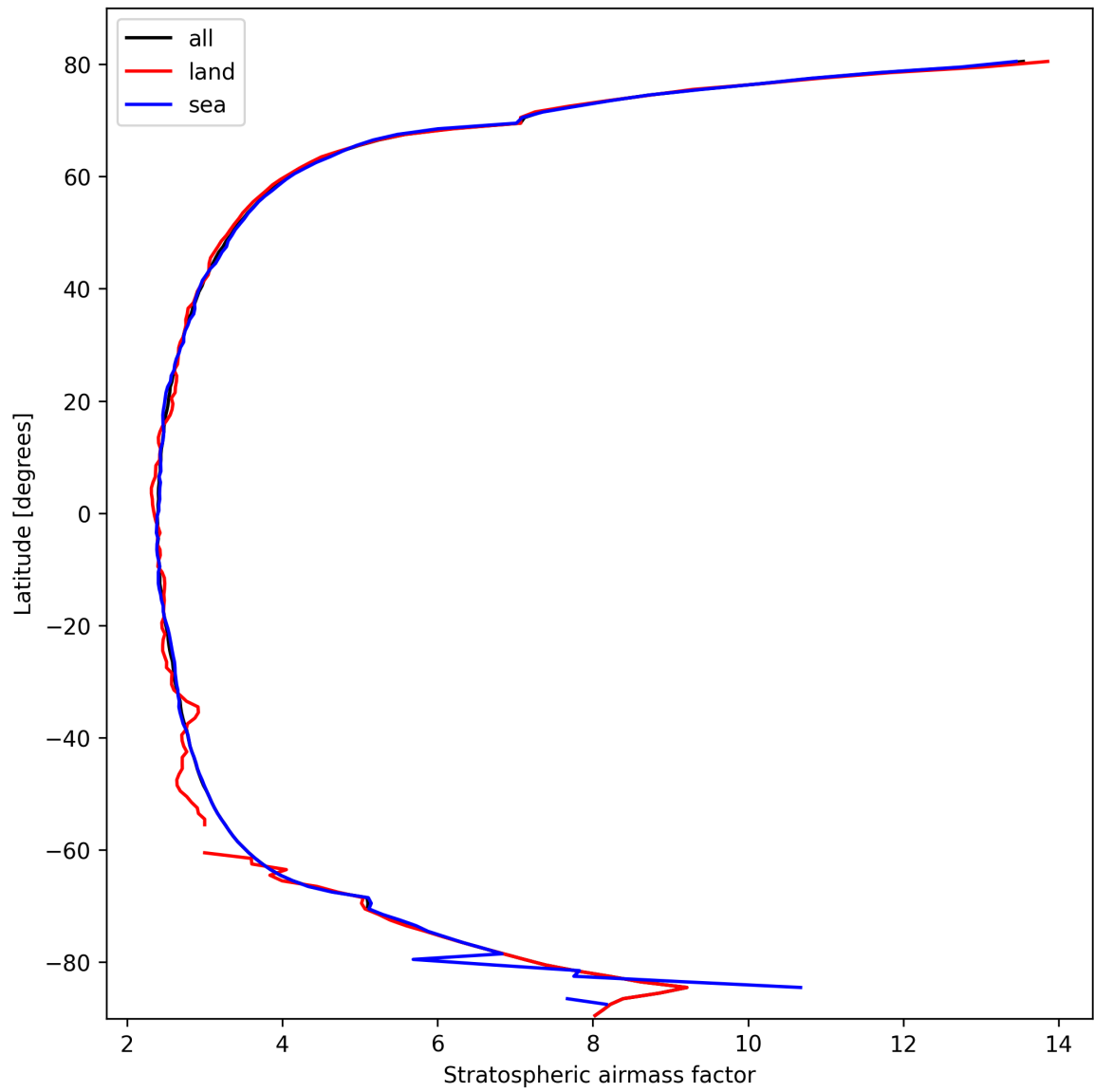
Figure 25: Zonal average of “Stratospheric air mass factor” for 2025-10-12 to 2025-10-13.
