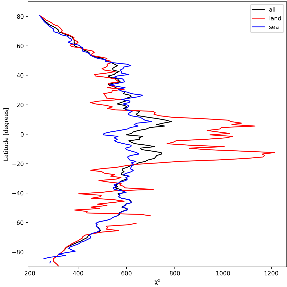
Figure 23: Zonal average of “ \chi^2 ” for 2025-10-12 to 2025-10-13.
