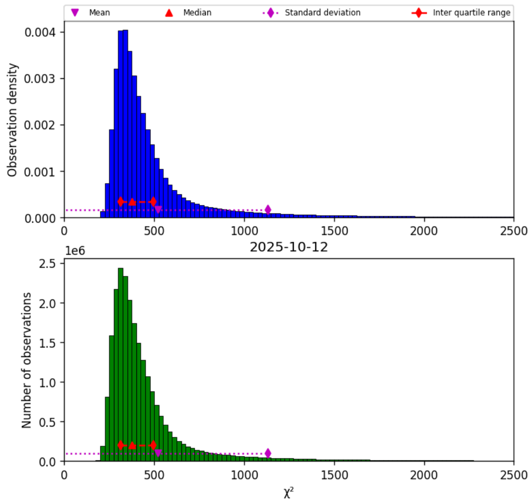
Figure 40: Histogram of " \chi^2 " for 2025-10-12 to 2025-10-13
