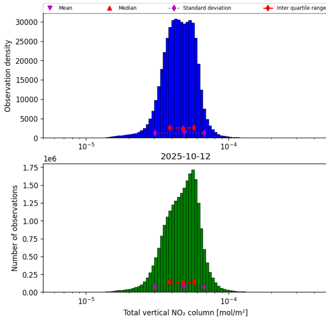
Figure 36: Histogram of "Total vertical NO 2 column" for 2025-10-12 to 2025-10-13
