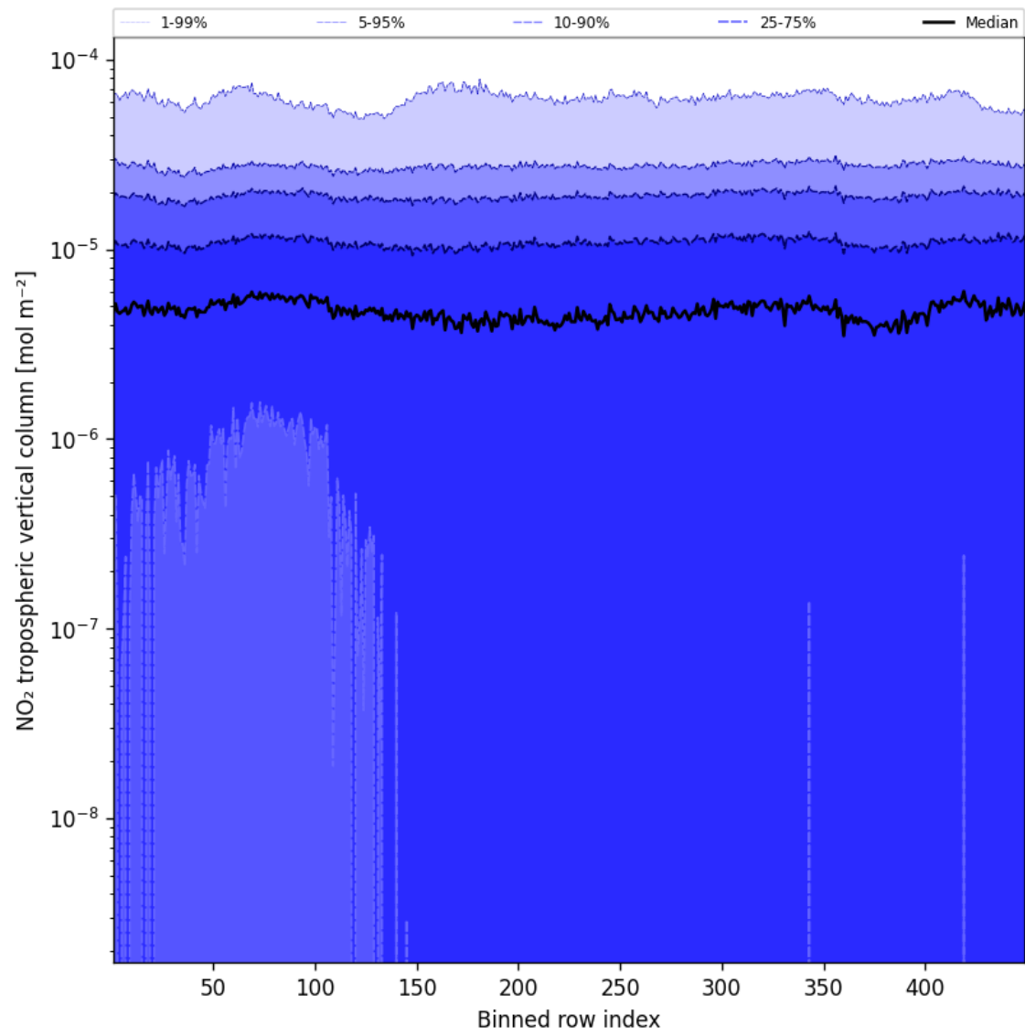
Figure 44: Along track statistics of “NO 2 tropospheric vertical column” for 2025-10-12 to 2025-10-13
