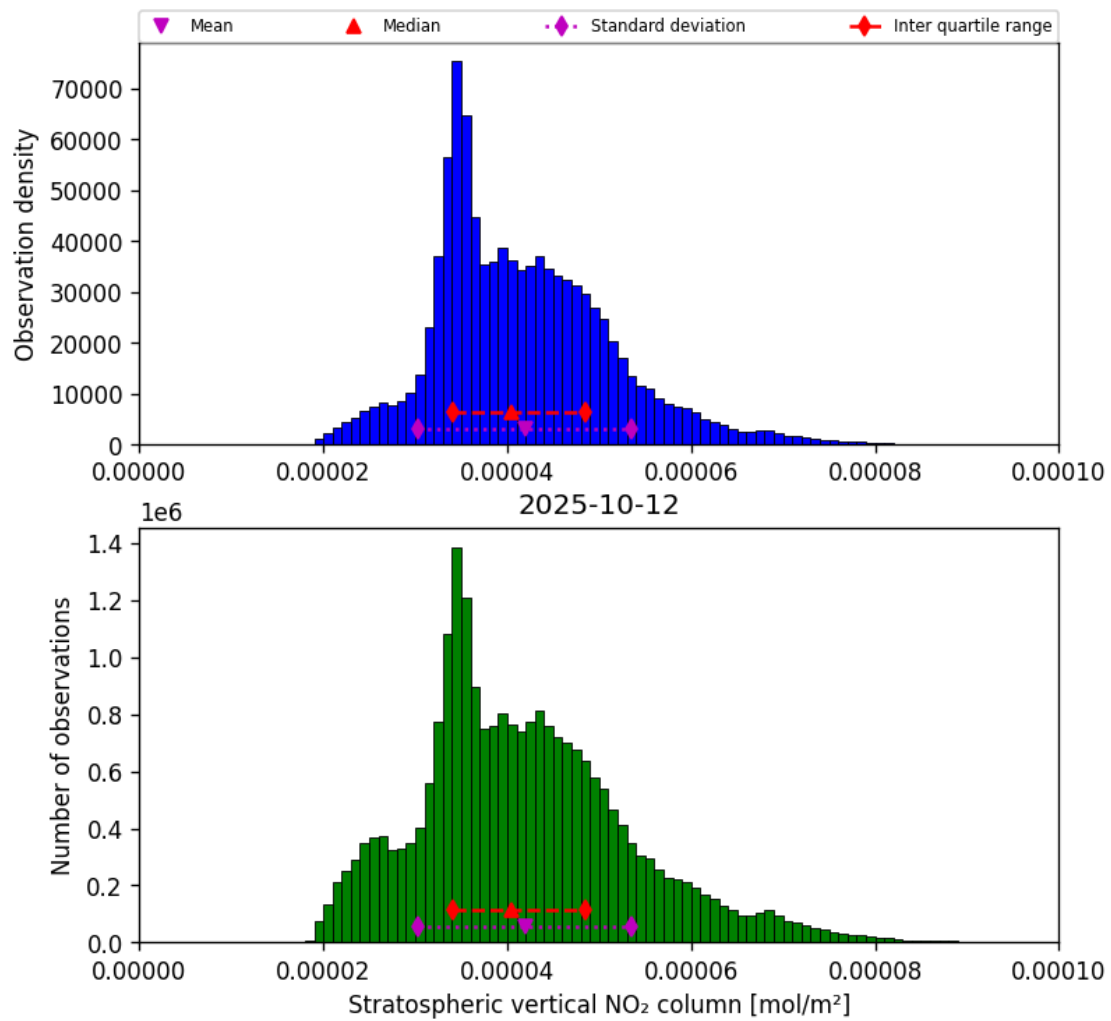
Figure 34: Histogram of “Stratospheric vertical NO 2 column” for 2025-10-12 to 2025-10-13
