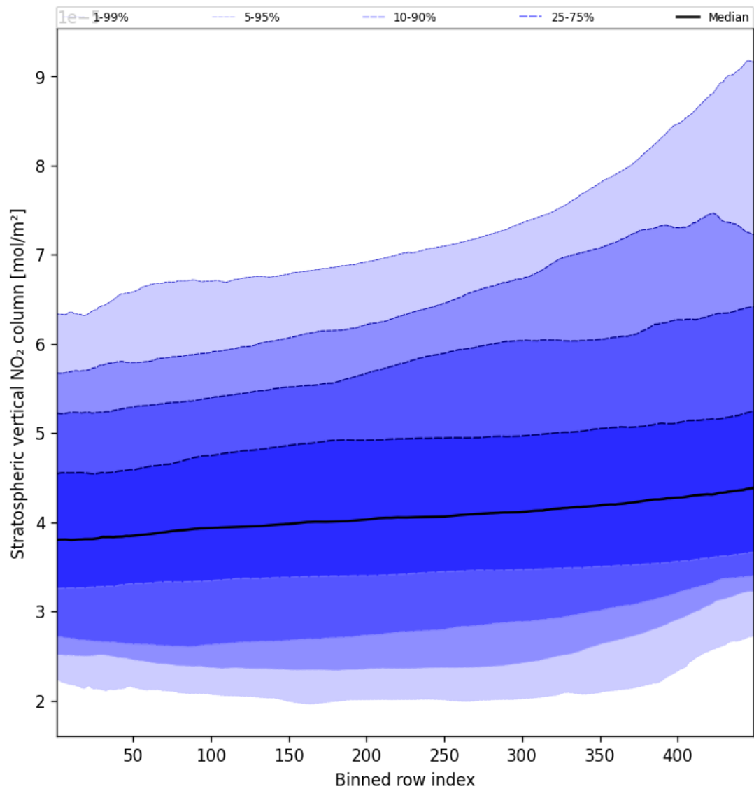
Figure 51: Along track statistics of “Stratospheric vertical NO 2 column” for 2025-10-13 to 2025-10-14
