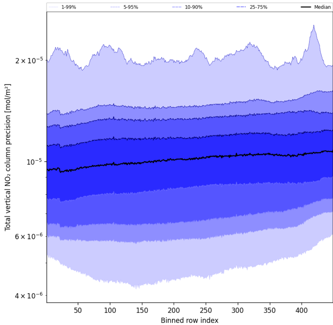
Figure 54: Along track statistics of “Total vertical NO 2 column precision” for 2025-10-13 to 2025-10-14
