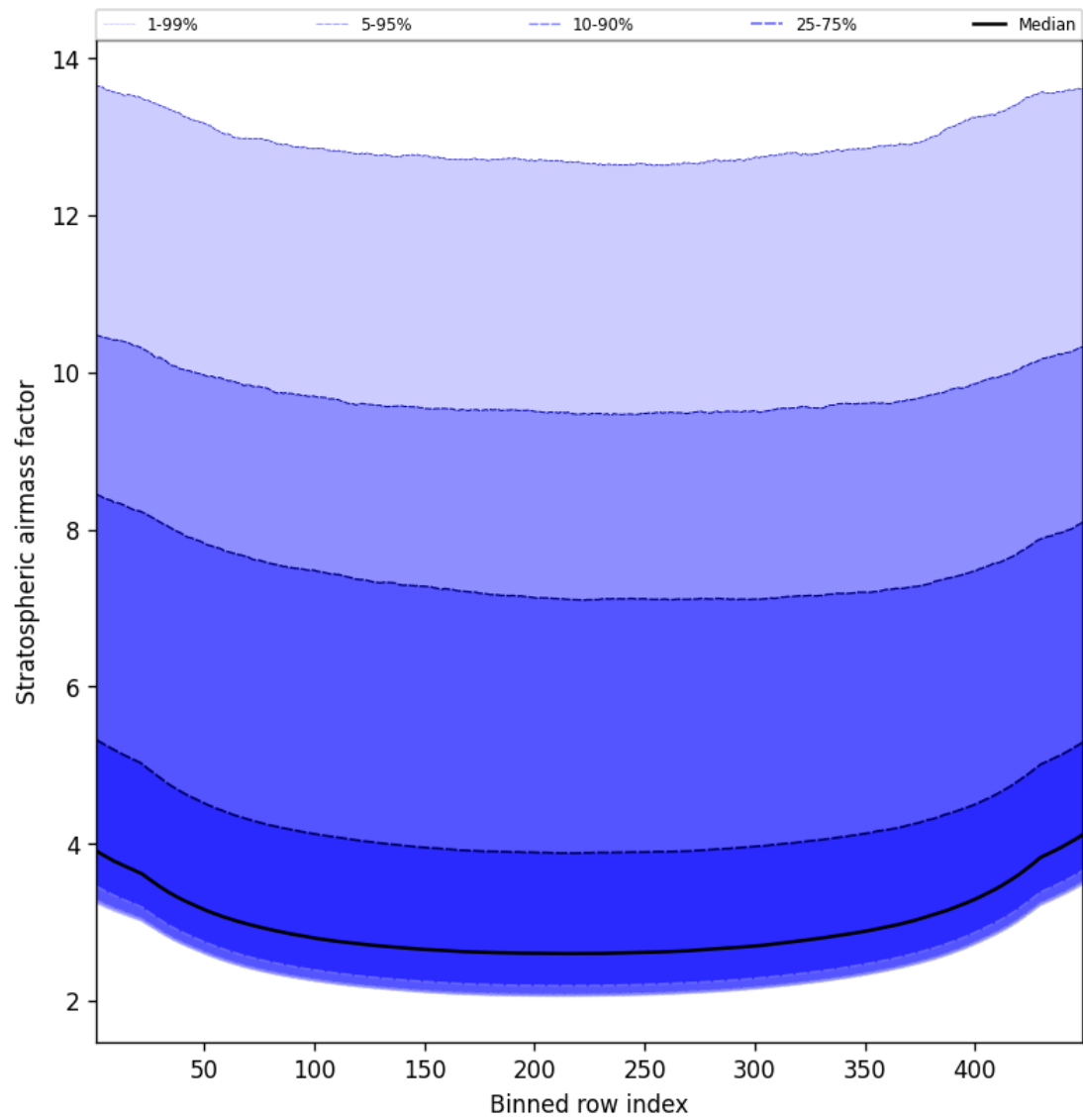
Figure 59: Along track statistics of “Stratospheric airmass factor” for 2025-10-13 to 2025-10-14
