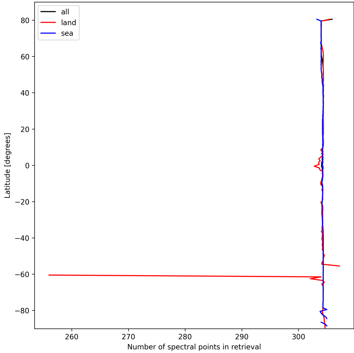
Figure 14: Zonal average of “Number of spectral points in retrieval” for 2025-10-13 to 2025-10-14.
