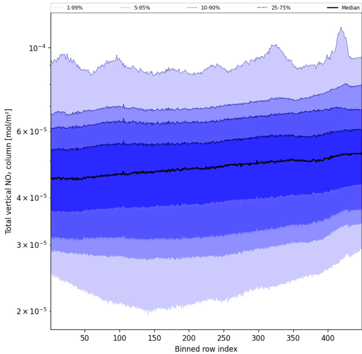
Figure 53: Along track statistics of “Total vertical NO 2 column” for 2025-10-13 to 2025-10-14
