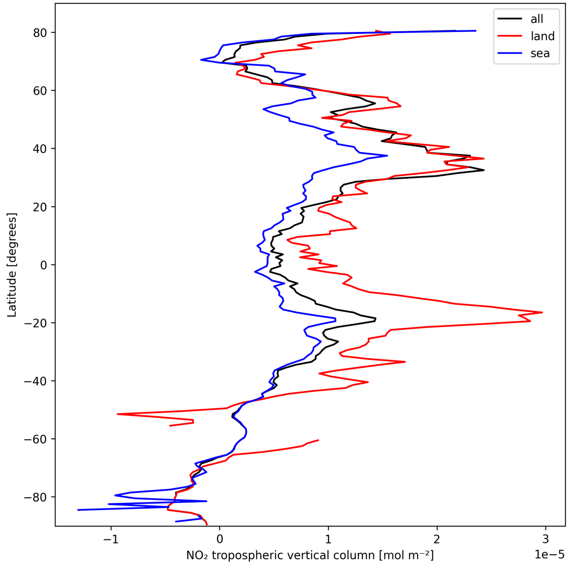
Figure 10: Zonal average of “NO 2 tropospheric vertical column” for 2025-10-13 to 2025-10-14.
