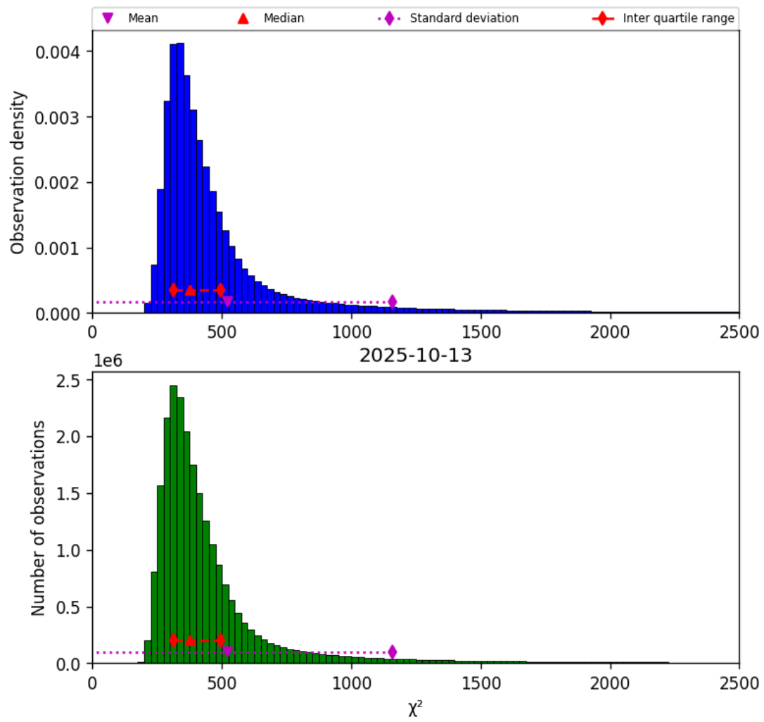
Figure 40: Histogram of " \chi^2 " for 2025-10-13 to 2025-10-14
