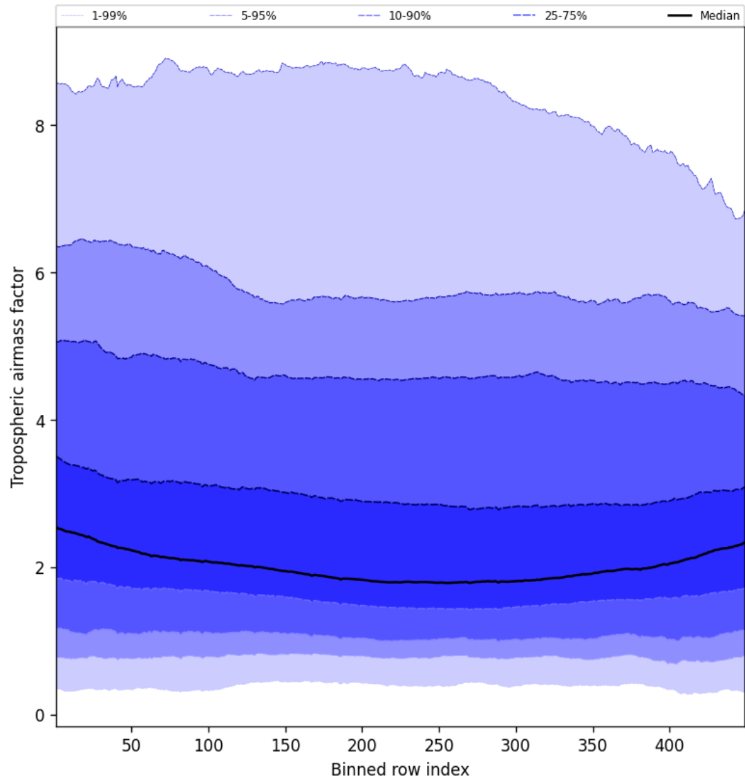
Figure 46: Along track statistics of “Tropospheric air mass factor” for 2025-10-13 to 2025-10-14
