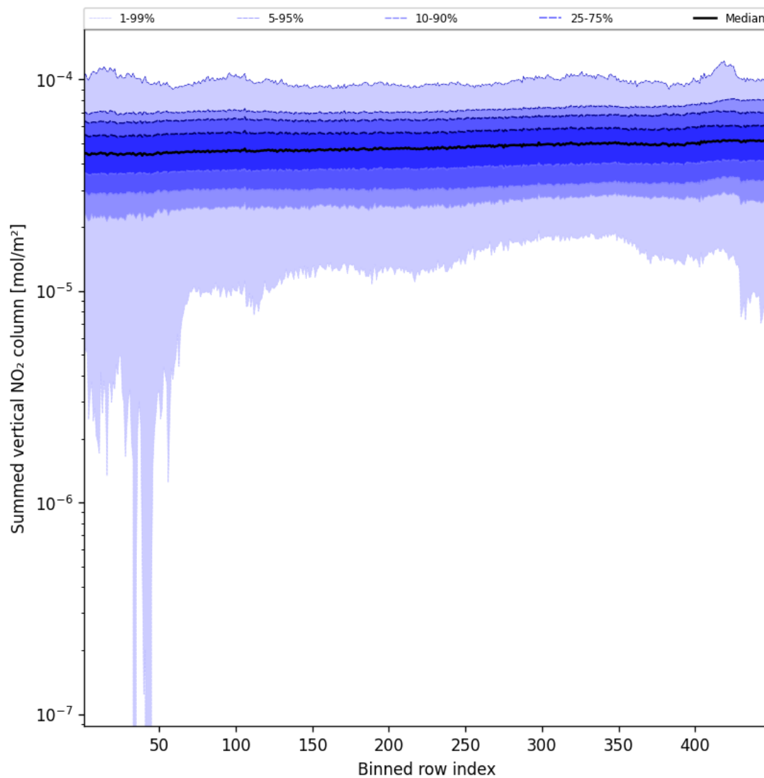
Figure 55: Along track statistics of “Summed vertical NO 2 column” for 2025-10-13 to 2025-10-14
