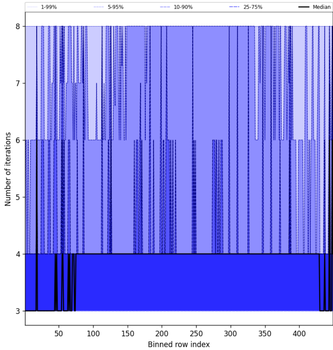
Figure 49: Along track statistics of “Number of iterations” for 2025-10-13 to 2025-10-14
