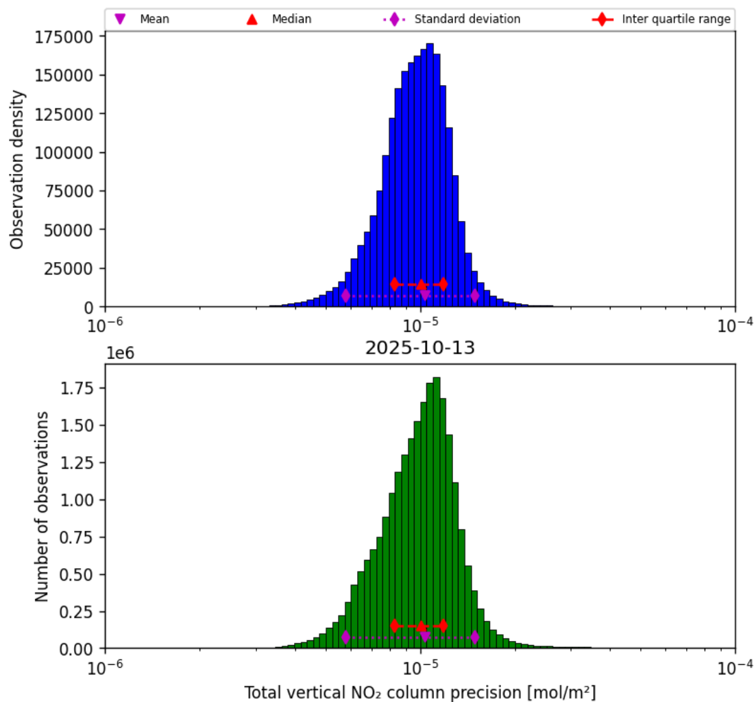
Figure 37: Histogram of “Total vertical NO 2 column precision” for 2025-10-13 to 2025-10-14
