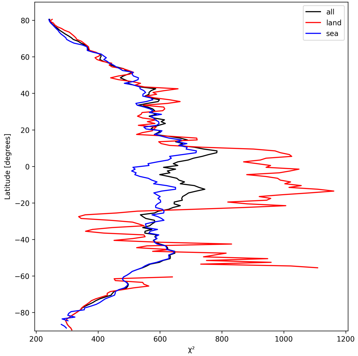
Figure 23: Zonal average of “ \chi^2 ” for 2025-10-13 to 2025-10-14.
