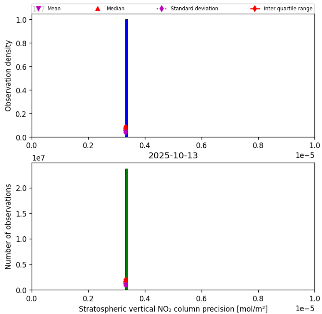
Figure 35: Histogram of “Stratospheric vertical NO 2 column precision” for 2025-10-13 to 2025-10-14
