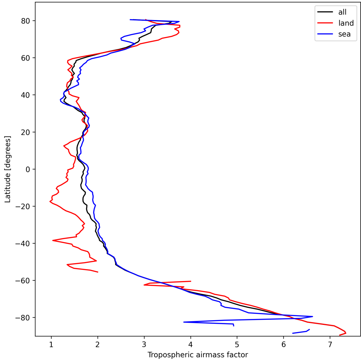
Figure 12: Zonal average of “Tropospheric airmass factor” for 2025-10-13 to 2025-10-14.
