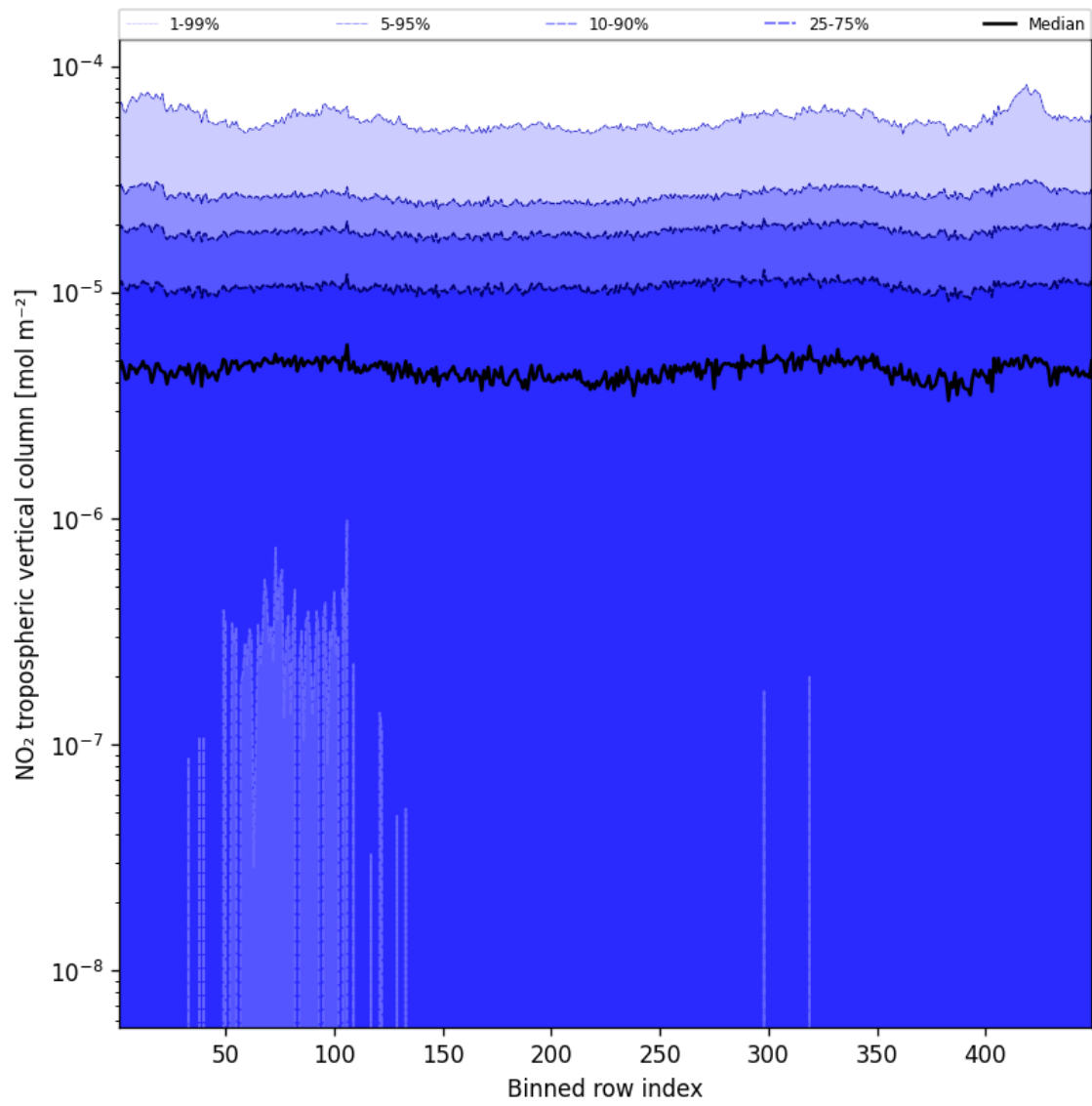
Figure 44: Along track statistics of “NO 2 tropospheric vertical column” for 2025-10-13 to 2025-10-14
