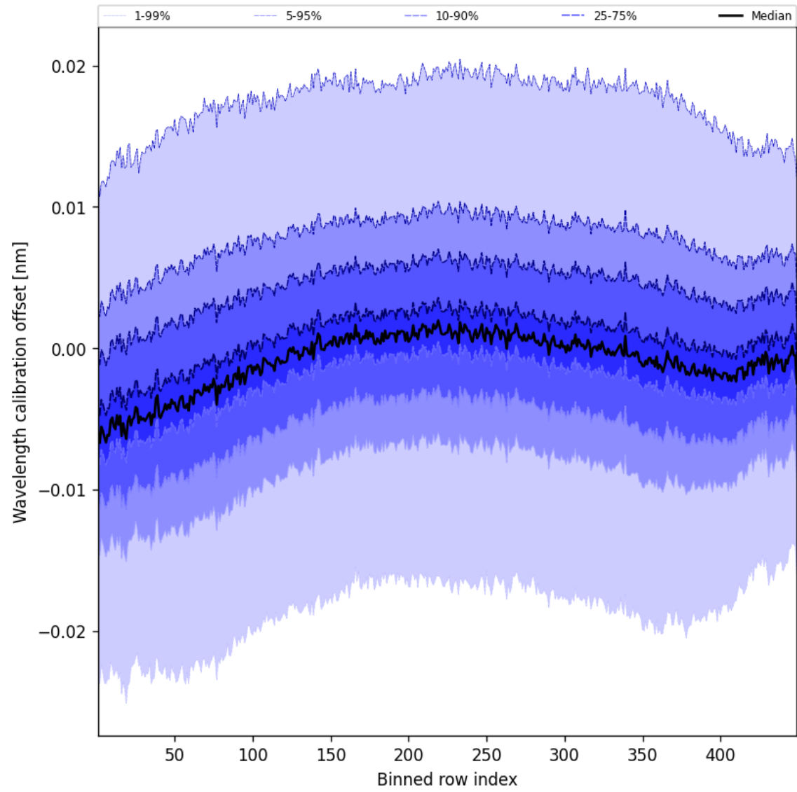
Figure 50: Along track statistics of “Wavelength calibration offset” for 2025-10-13 to 2025-10-14
