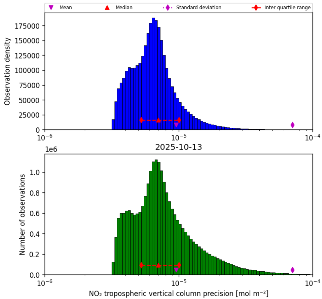
Figure 28: Histogram of “NO 2 tropospheric vertical column precision” for 2025-10-13 to 2025-10-14
