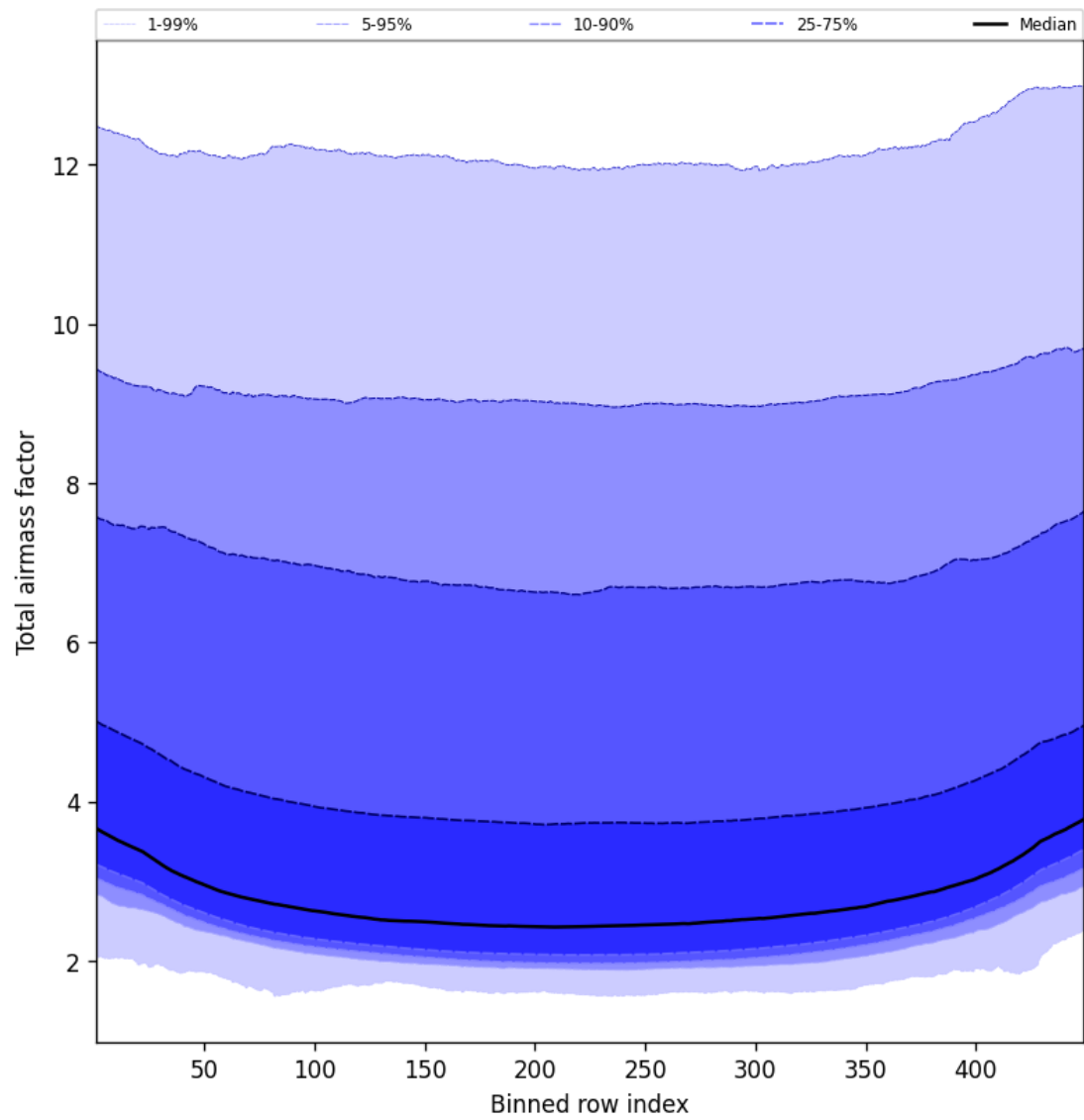
Figure 47: Along track statistics of “Total airmass factor” for 2025-10-13 to 2025-10-14
