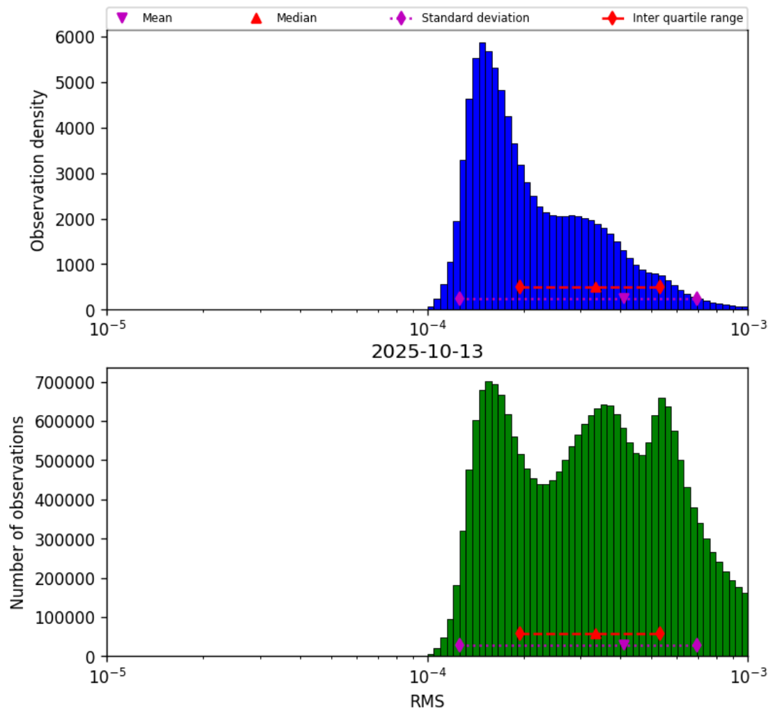
Figure 41: Histogram of “RMS” for 2025-10-13 to 2025-10-14
