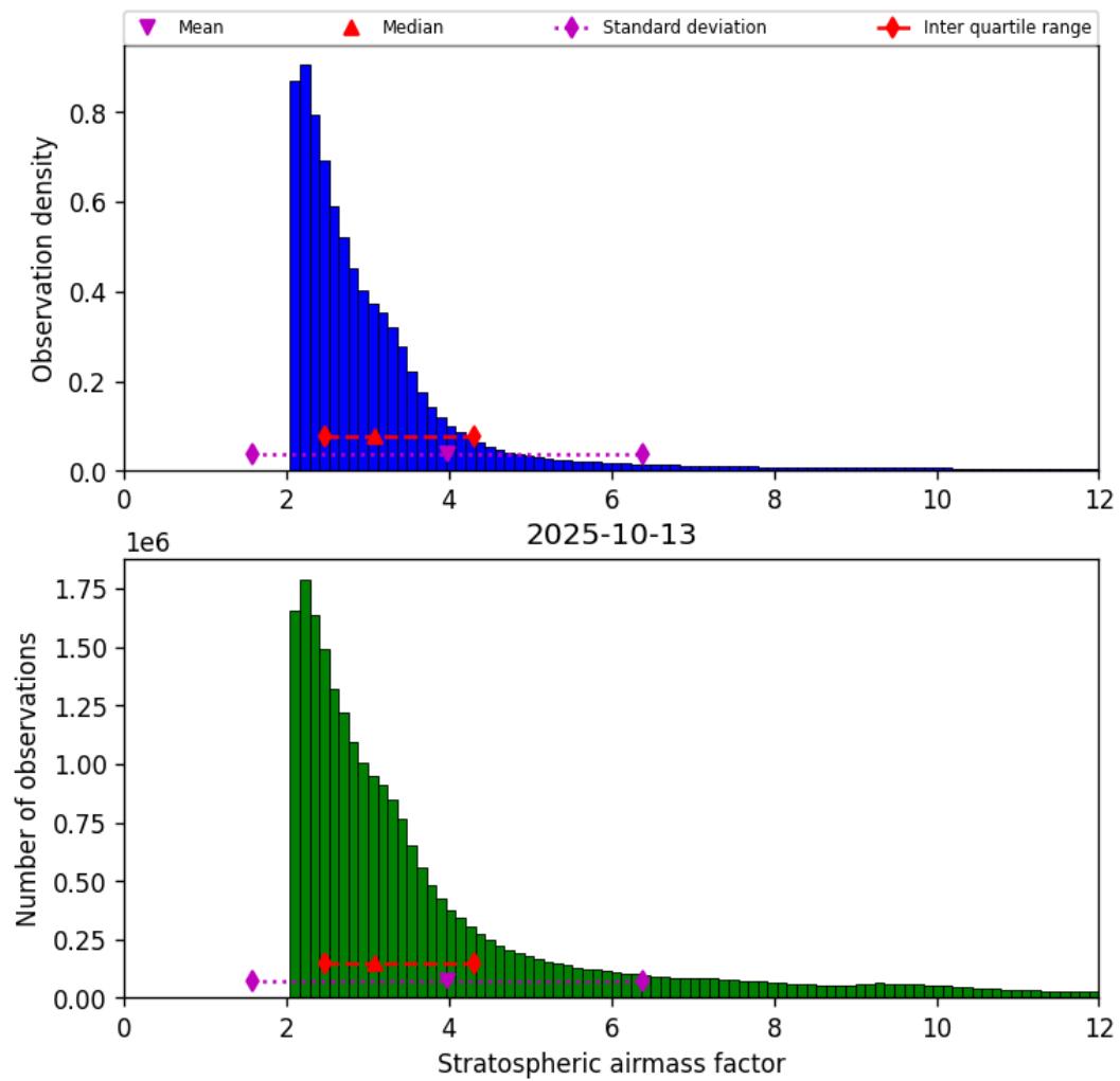
Figure 42: Histogram of “Stratospheric airmass factor” for 2025-10-13 to 2025-10-14
