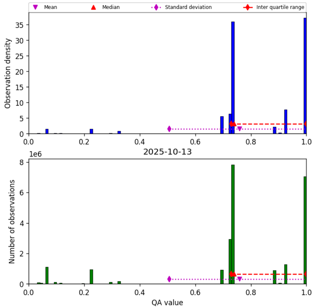
Figure 26: Histogram of “QA value” for 2025-10-13 to 2025-10-14
