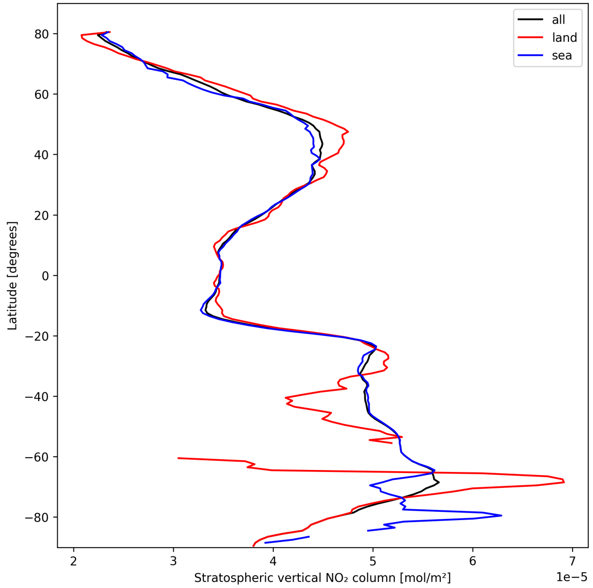
Figure 17: Zonal average of “Stratospheric vertical NO 2 column” for 2025-10-13 to 2025-10-14.
