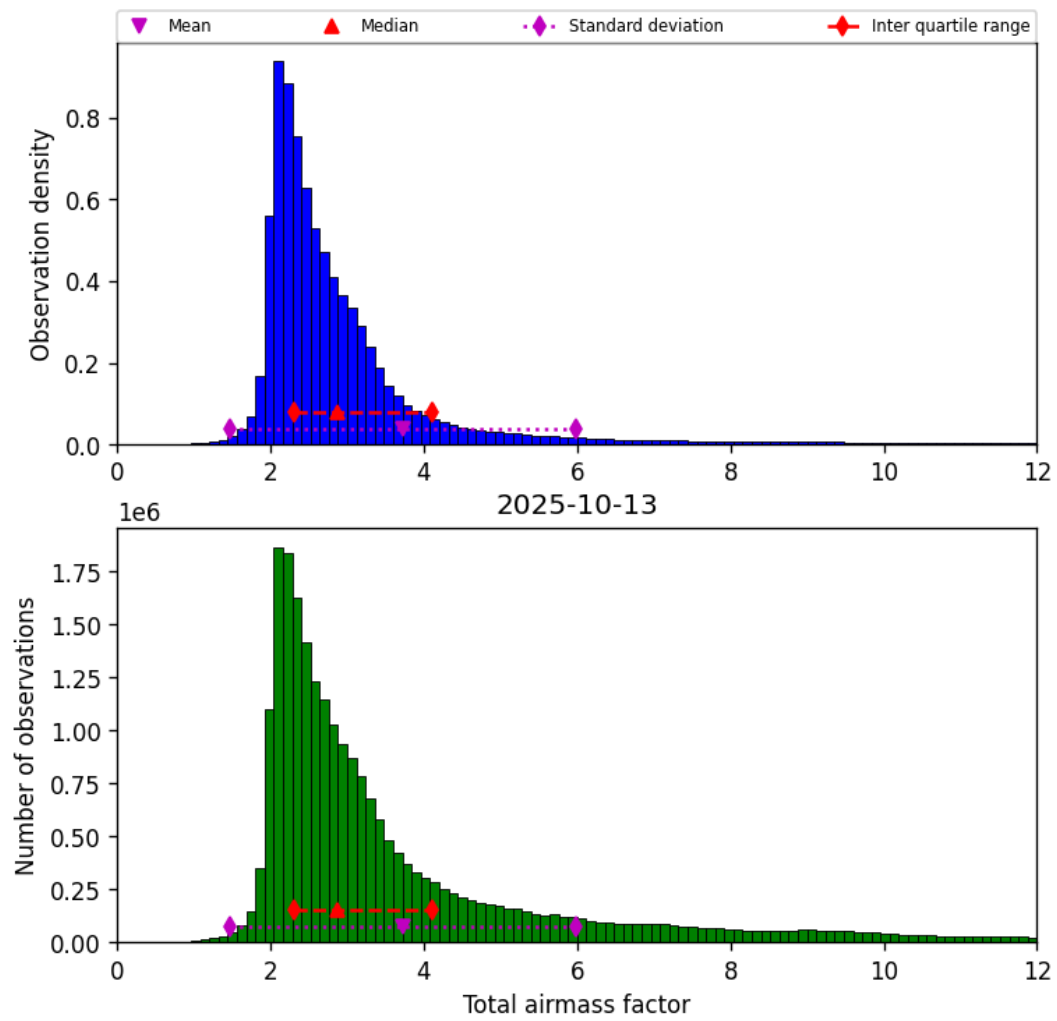
Figure 30: Histogram of “Total airmass factor” for 2025-10-13 to 2025-10-14
