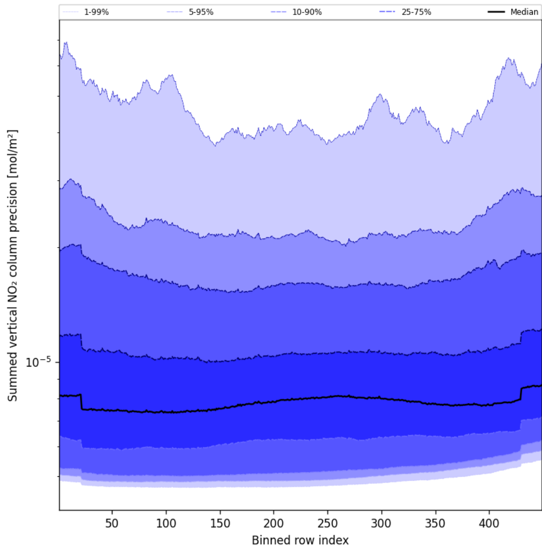
Figure 56: Along track statistics of “Summed vertical NO 2 column precision” for 2025-10-13 to 2025-10-14
