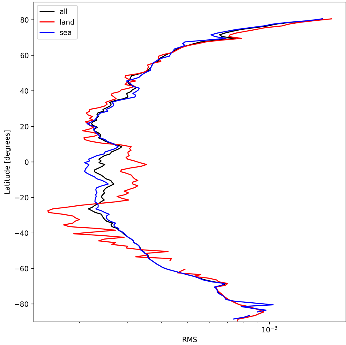
Figure 24: Zonal average of “RMS” for 2025-10-13 to 2025-10-14.
