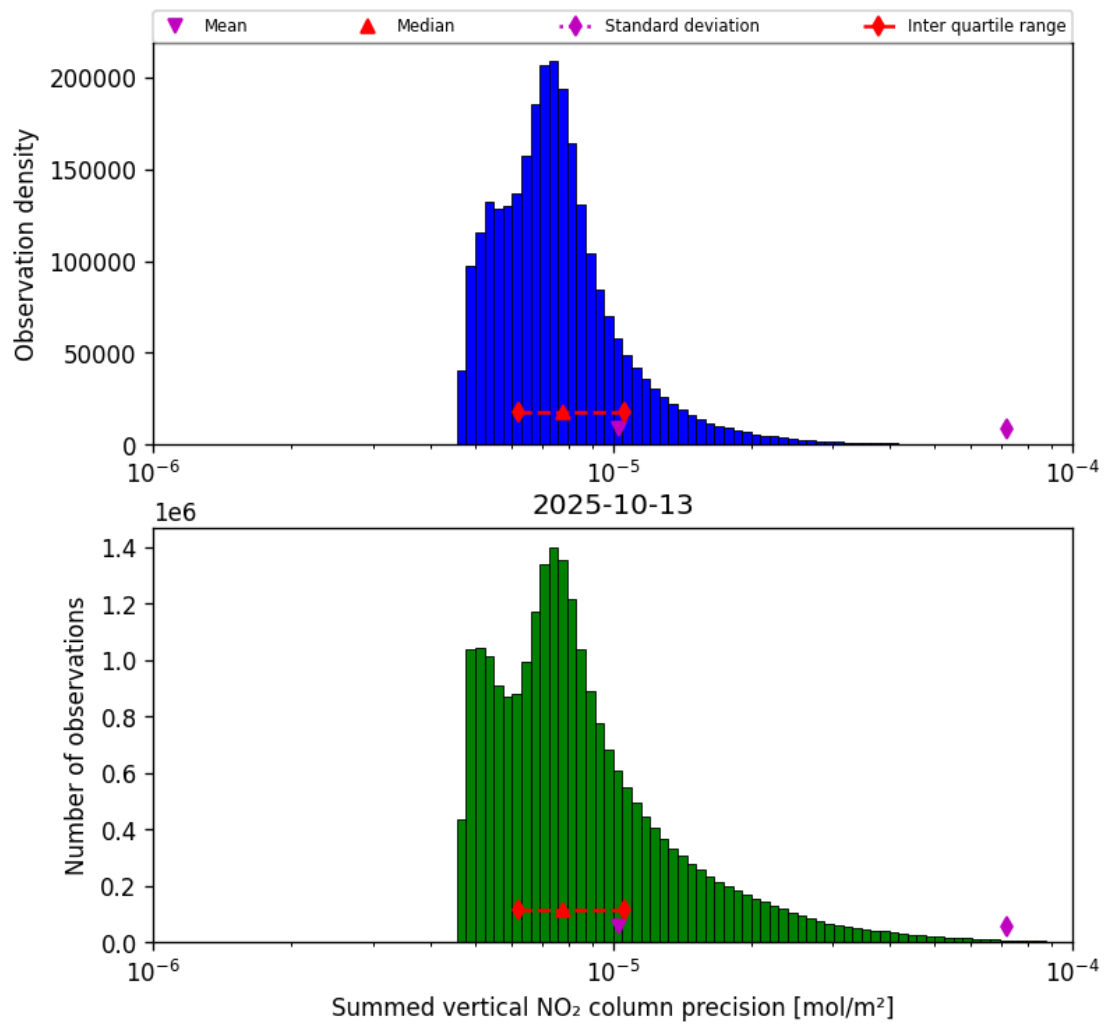
Figure 39: Histogram of “Summed vertical NO 2 column precision” for 2025-10-13 to 2025-10-14
