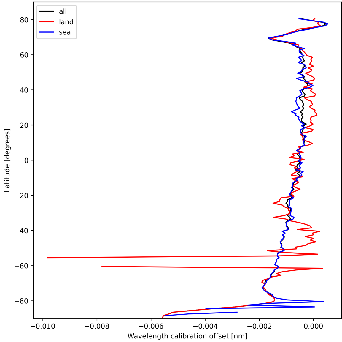
Figure 16: Zonal average of “Wavelength calibration offset” for 2025-10-13 to 2025-10-14.
