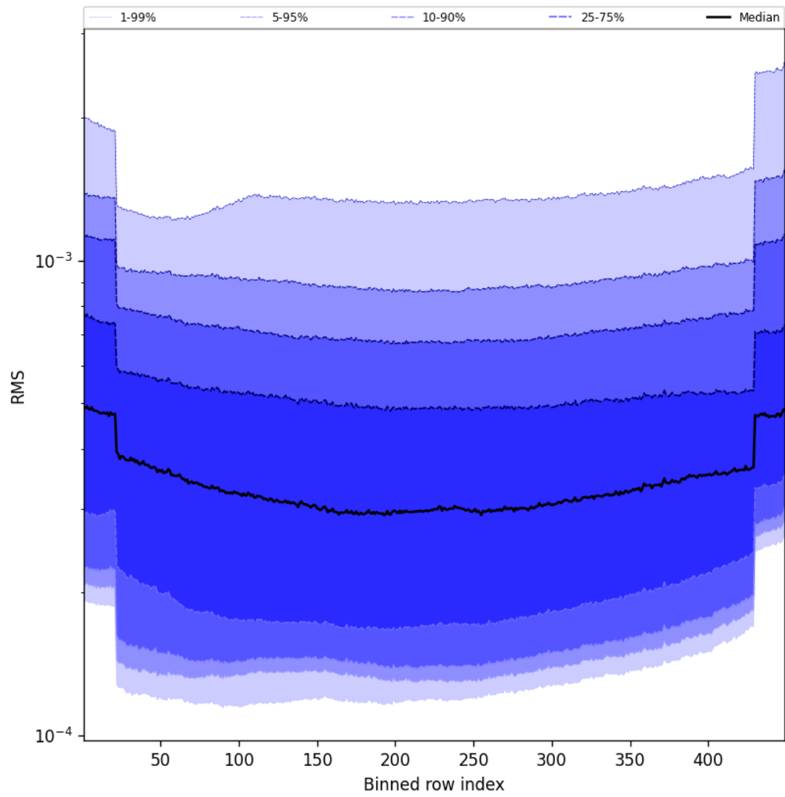
Figure 58: Along track statistics of “RMS” for 2025-10-13 to 2025-10-14
