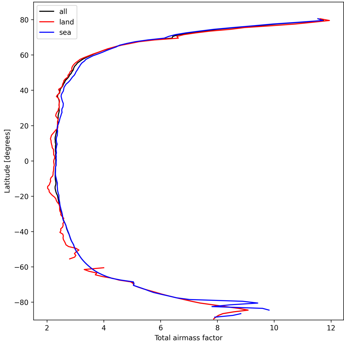
Figure 13: Zonal average of “Total airmass factor” for 2025-10-13 to 2025-10-14.
