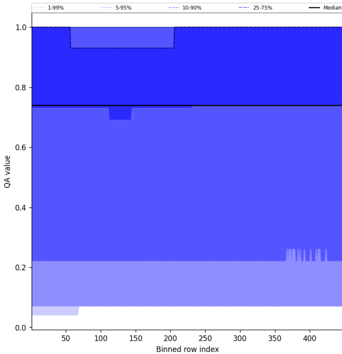
Figure 43: Along track statistics of “QA value” for 2025-10-13 to 2025-10-14
