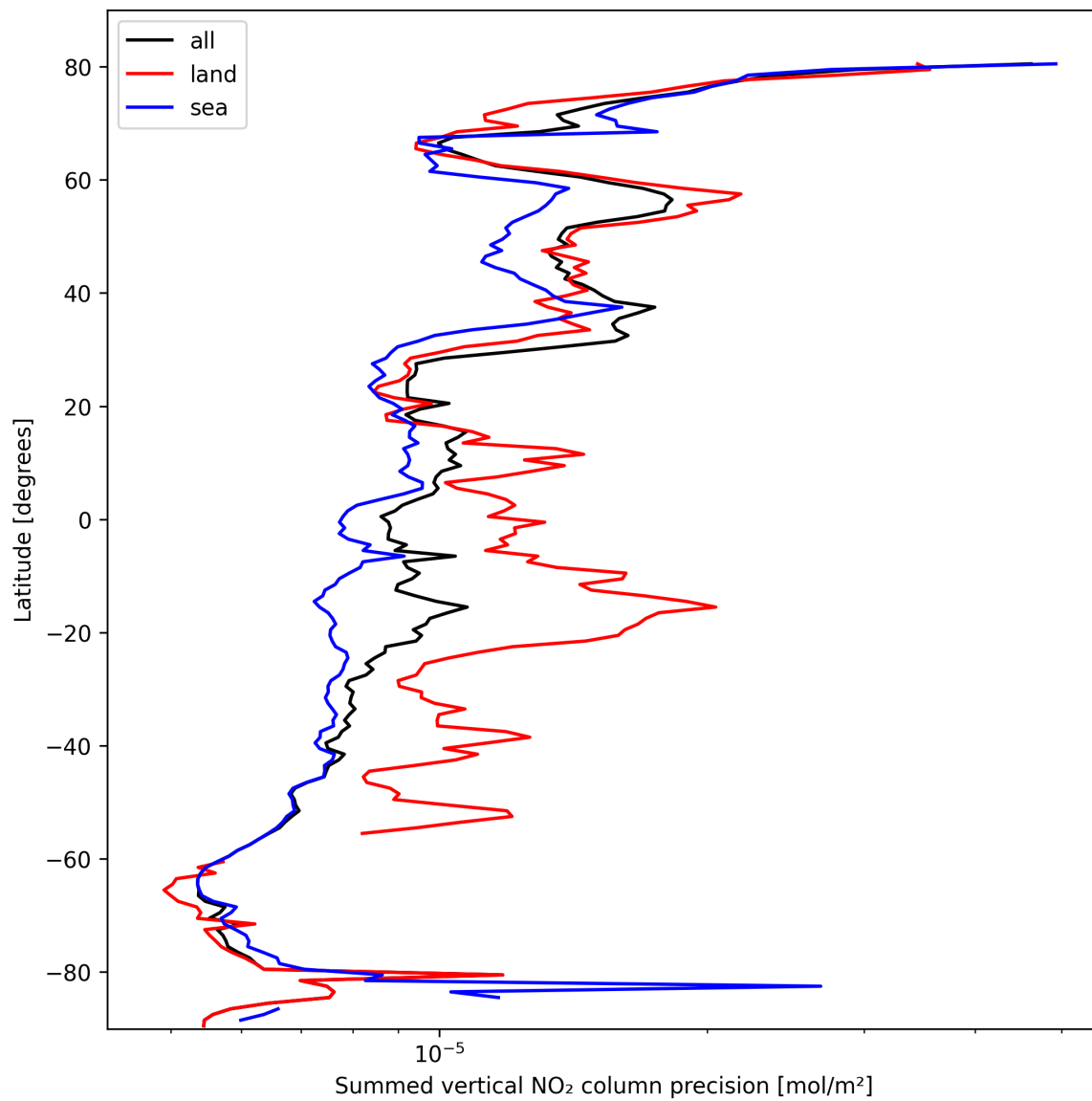
Figure 22: Zonal average of “Summed vertical NO 2 column precision” for 2025-10-13 to 2025-10-14.
