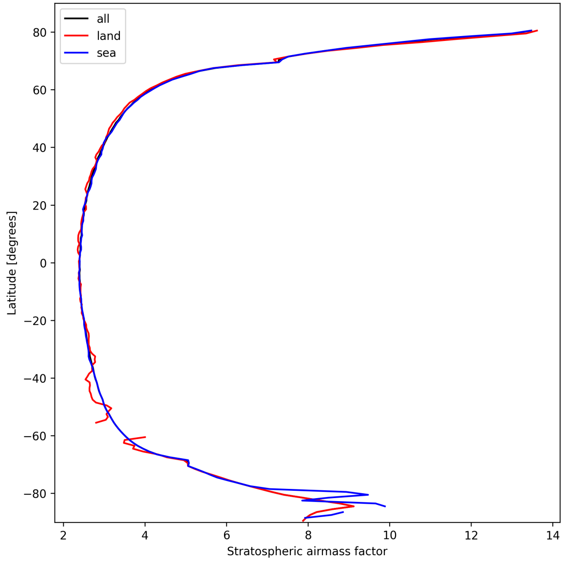
Figure 25: Zonal average of “Stratospheric airmass factor” for 2025-10-13 to 2025-10-14.
