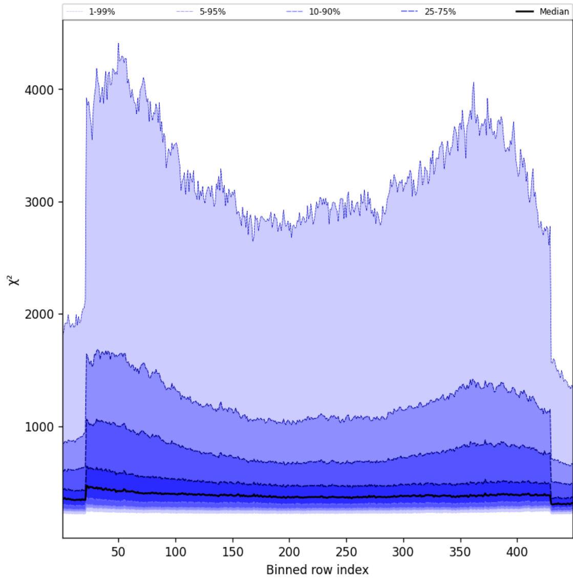
Figure 57: Along track statistics of “ \chi^2 ” for 2025-10-13 to 2025-10-14
