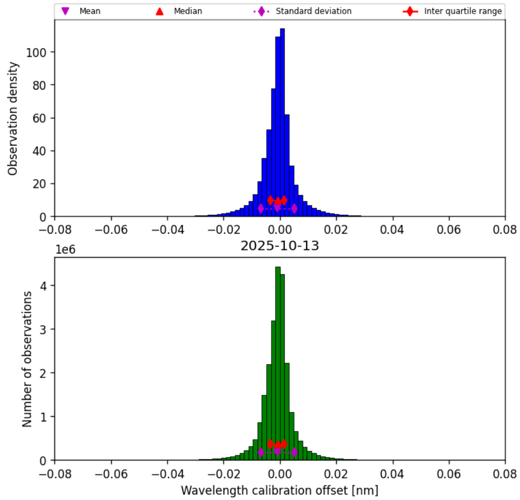
Figure 33: Histogram of “Wavelength calibration offset” for 2025-10-13 to 2025-10-14
