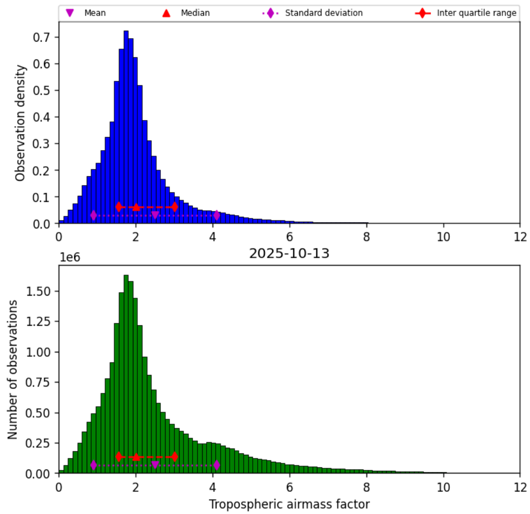
Figure 29: Histogram of “Tropospheric airmass factor” for 2025-10-13 to 2025-10-14
