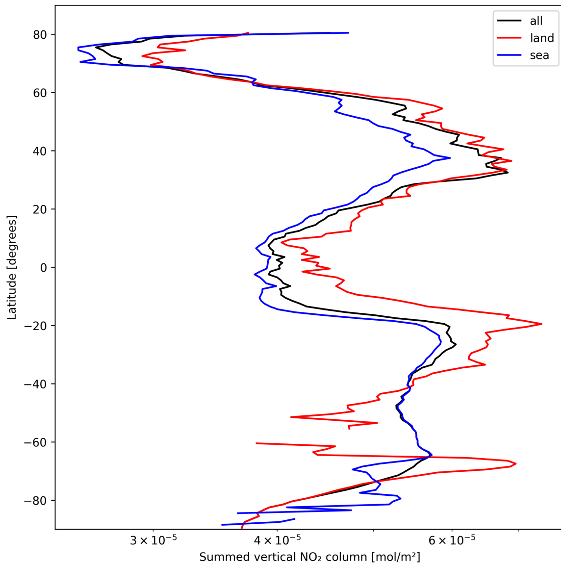
Figure 21: Zonal average of “Summed vertical NO 2 column” for 2025-10-13 to 2025-10-14.
