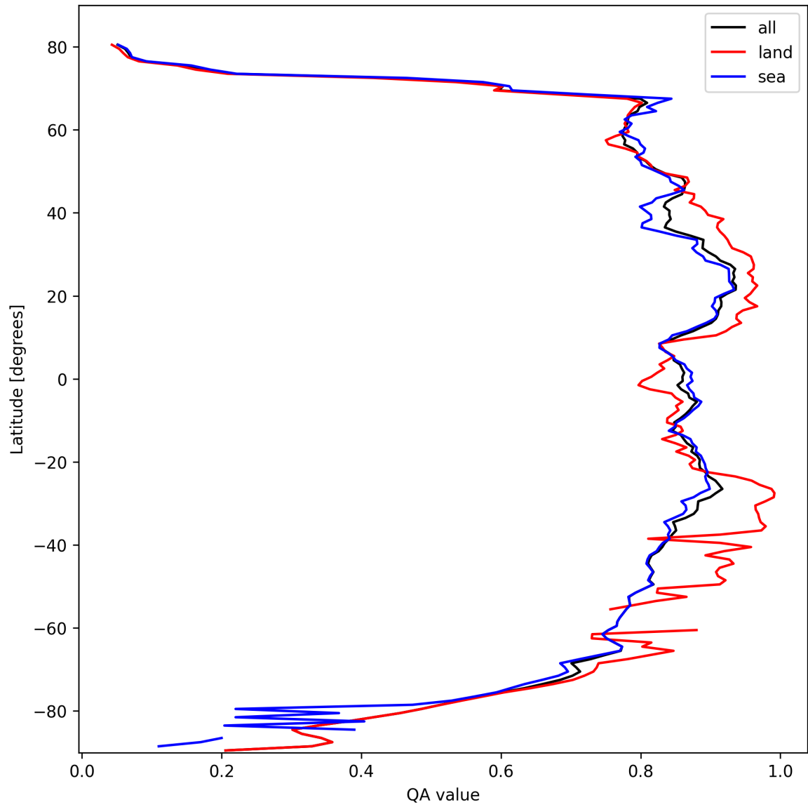
Figure 9: Zonal average of “QA value” for 2025-10-13 to 2025-10-14.
