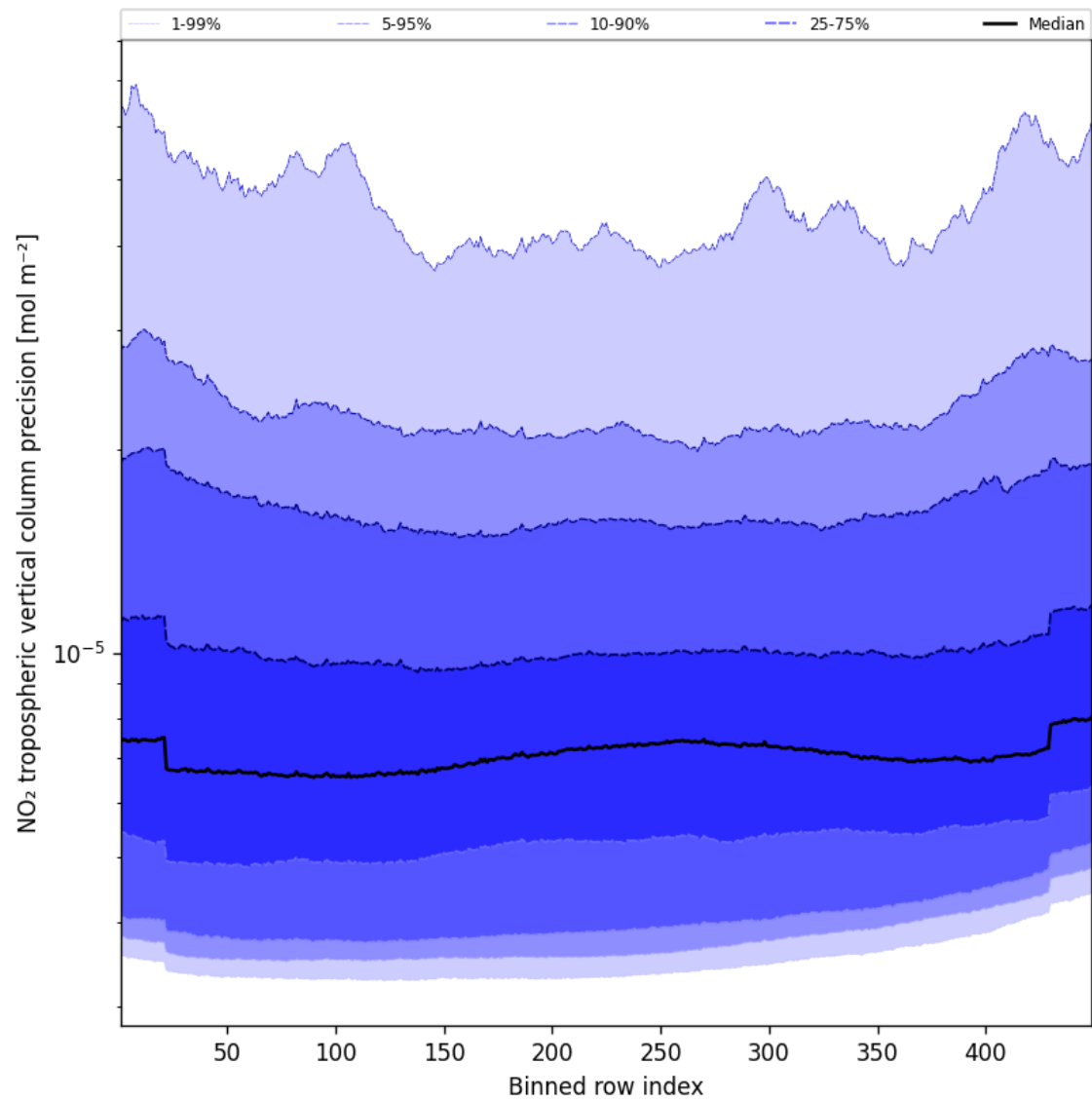
Figure 45: Along track statistics of “NO 2 tropospheric vertical column precision” for 2025-10-13 to 2025-10-14
