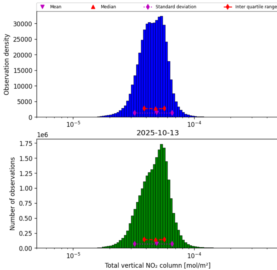
Figure 36: Histogram of “Total vertical NO 2 column” for 2025-10-13 to 2025-10-14
