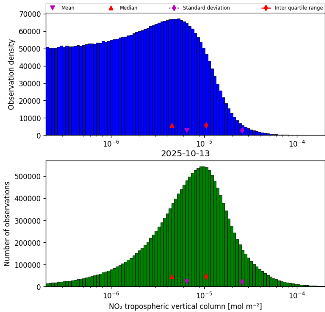
Figure 27: Histogram of “NO 2 tropospheric vertical column” for 2025-10-13 to 2025-10-14
