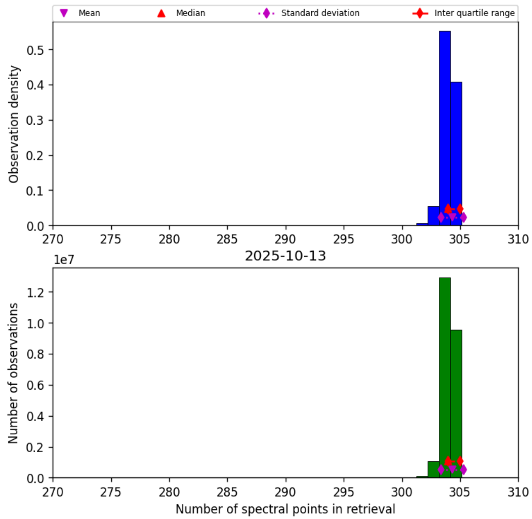
Figure 31: Histogram of “Number of spectral points in retrieval” for 2025-10-13 to 2025-10-14
