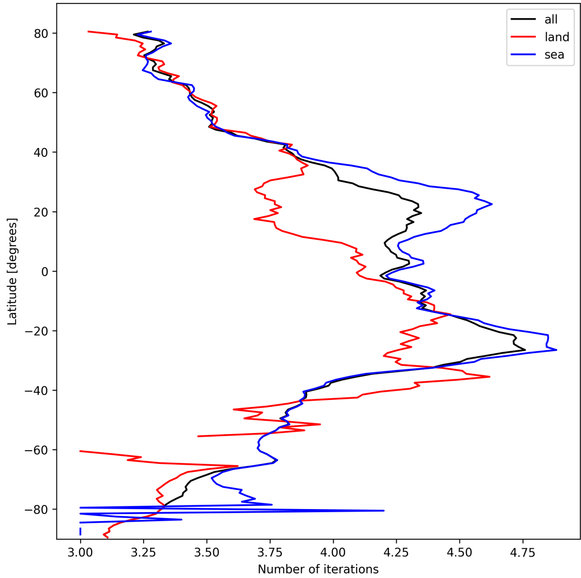
Figure 15: Zonal average of “Number of iterations” for 2025-10-13 to 2025-10-14.
