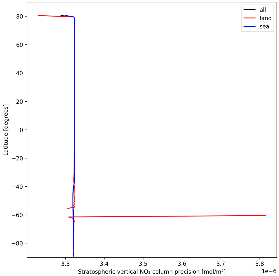
Figure 18: Zonal average of “Stratospheric vertical NO 2 column precision” for 2025-10-13 to 2025-10-14.
