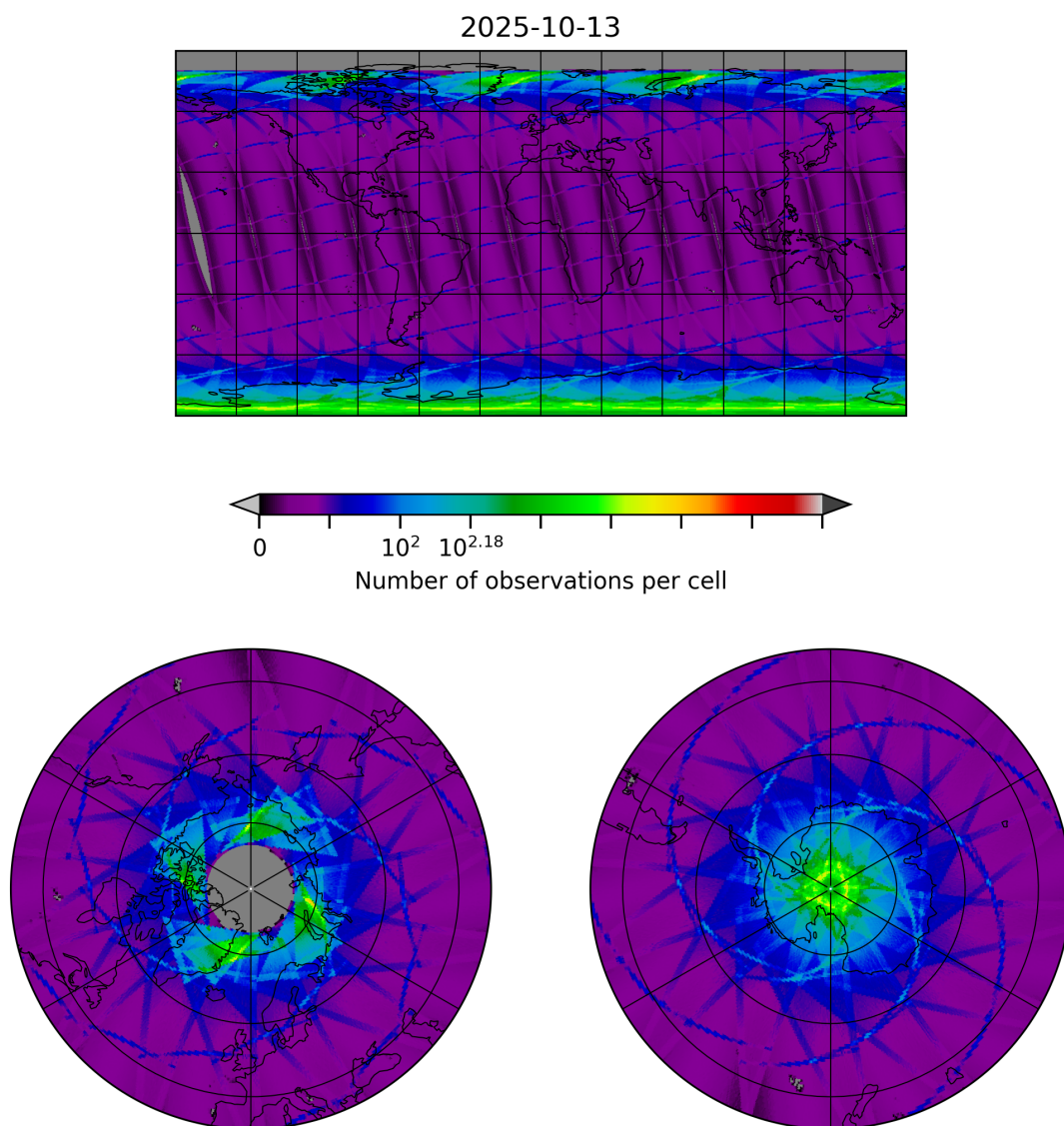
Figure 8: Map of the number of observations for 2025-10-13 to 2025-10-14
