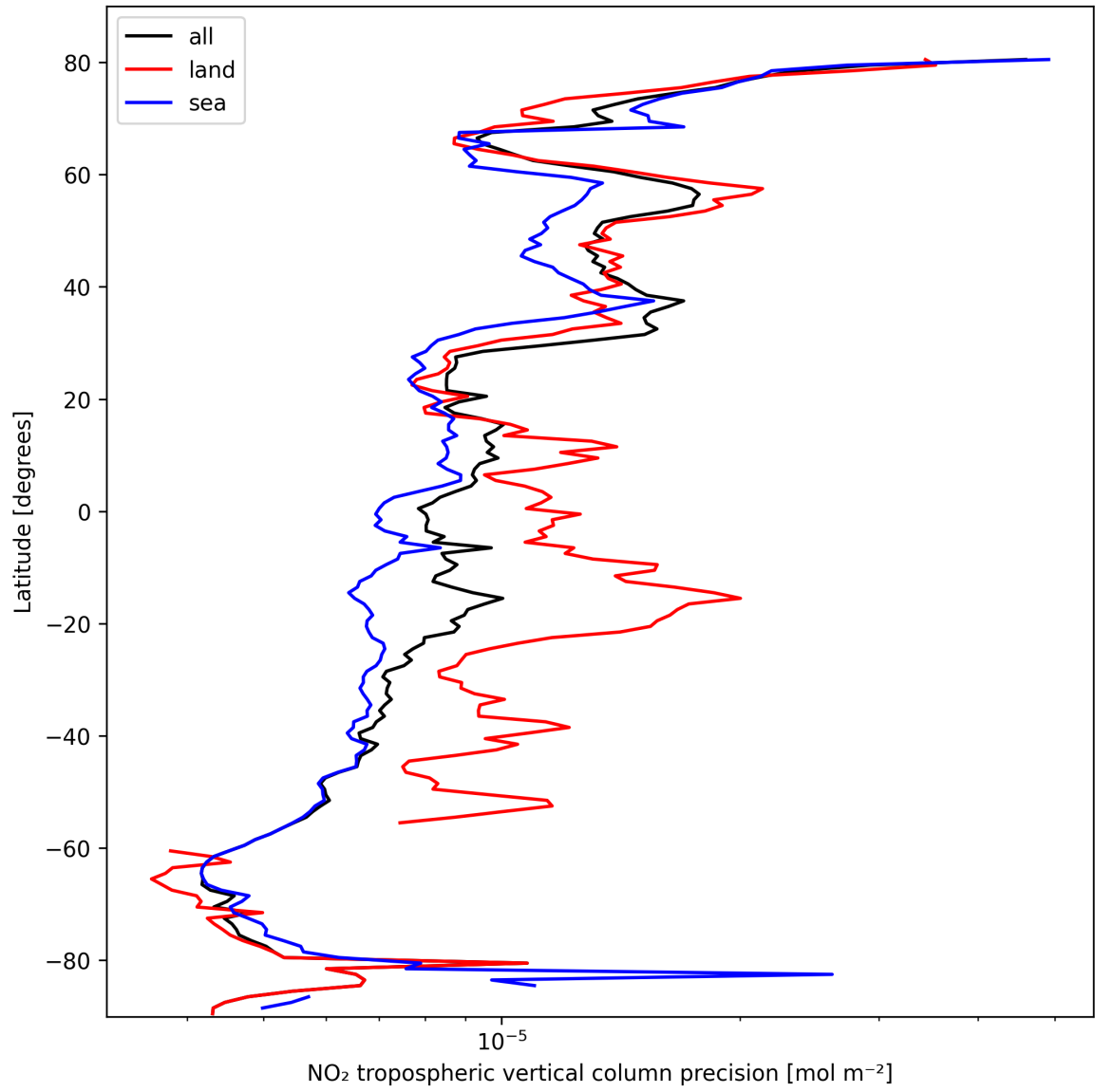
Figure 11: Zonal average of “NO 2 tropospheric vertical column precision” for 2025-10-13 to 2025-10-14.
