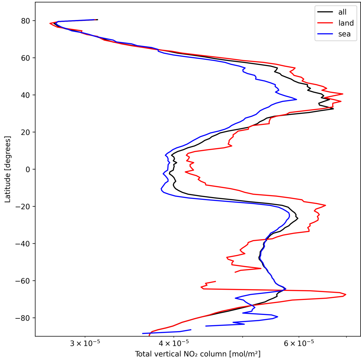
Figure 19: Zonal average of “Total vertical NO 2 column” for 2025-10-13 to 2025-10-14.
