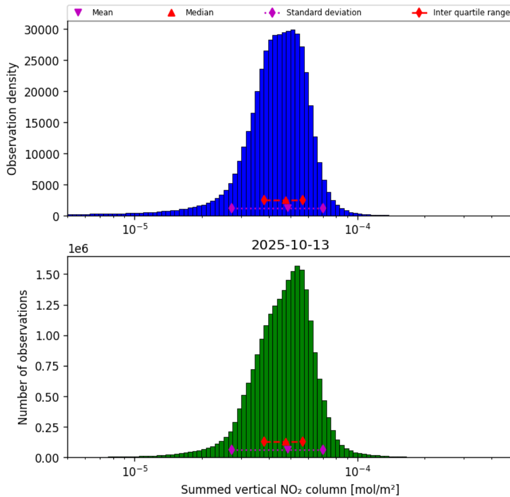
Figure 38: Histogram of “Summed vertical NO 2 column” for 2025-10-13 to 2025-10-14
