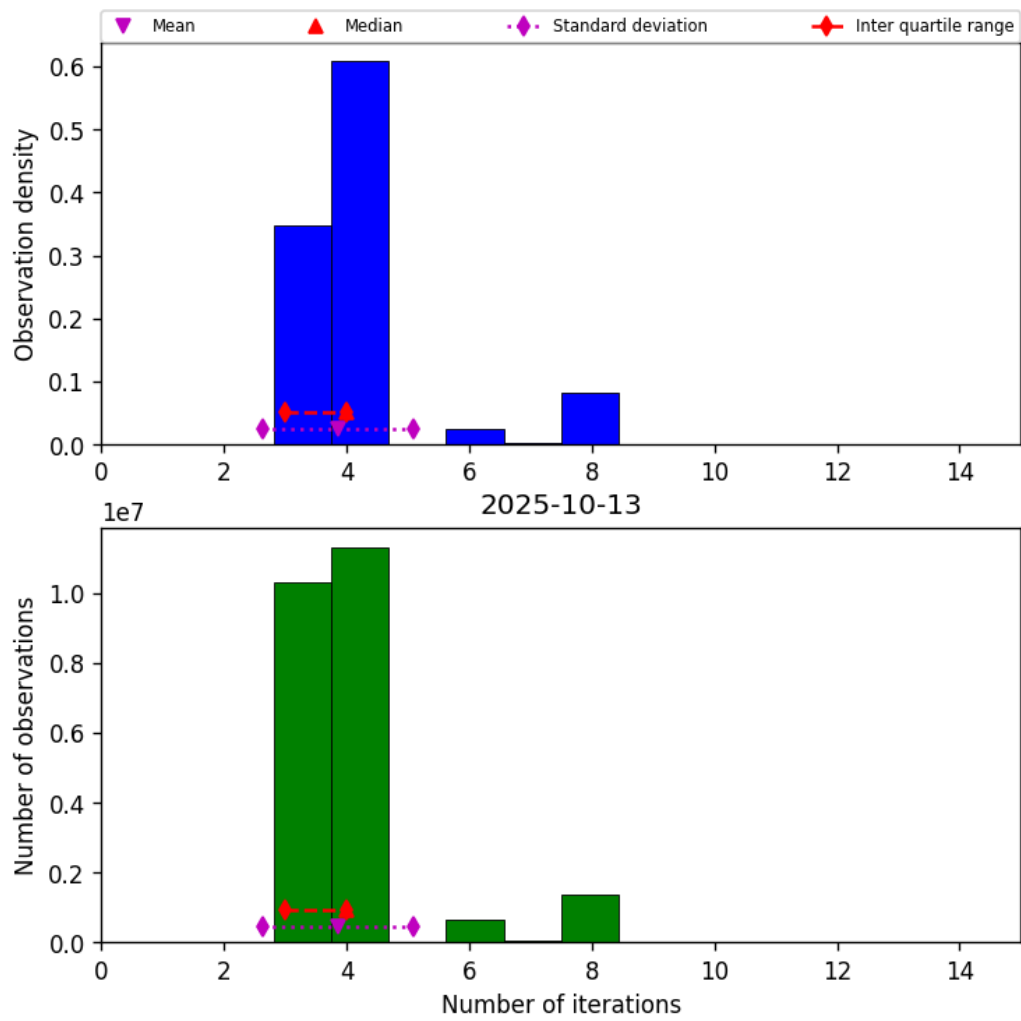
Figure 32: Histogram of “Number of iterations” for 2025-10-13 to 2025-10-14
