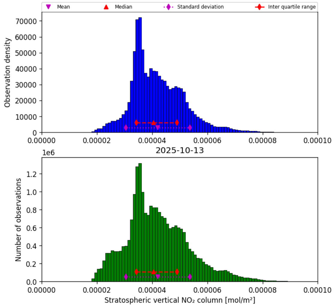
Figure 34: Histogram of “Stratospheric vertical NO 2 column” for 2025-10-13 to 2025-10-14
