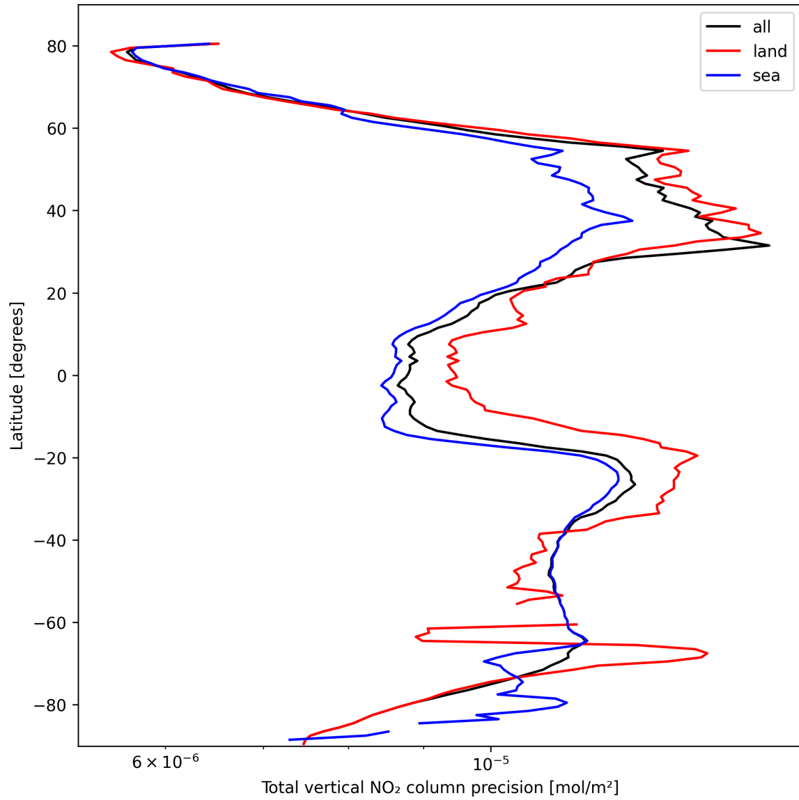
Figure 20: Zonal average of “Total vertical NO 2 column precision” for 2025-10-13 to 2025-10-14.
