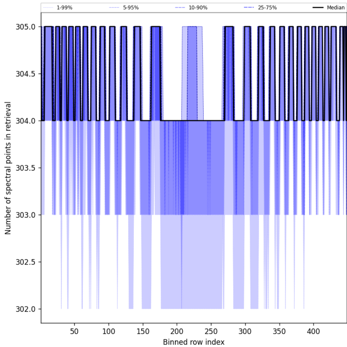
Figure 48: Along track statistics of “Number of spectral points in retrieval” for 2025-10-13 to 2025-10-14
