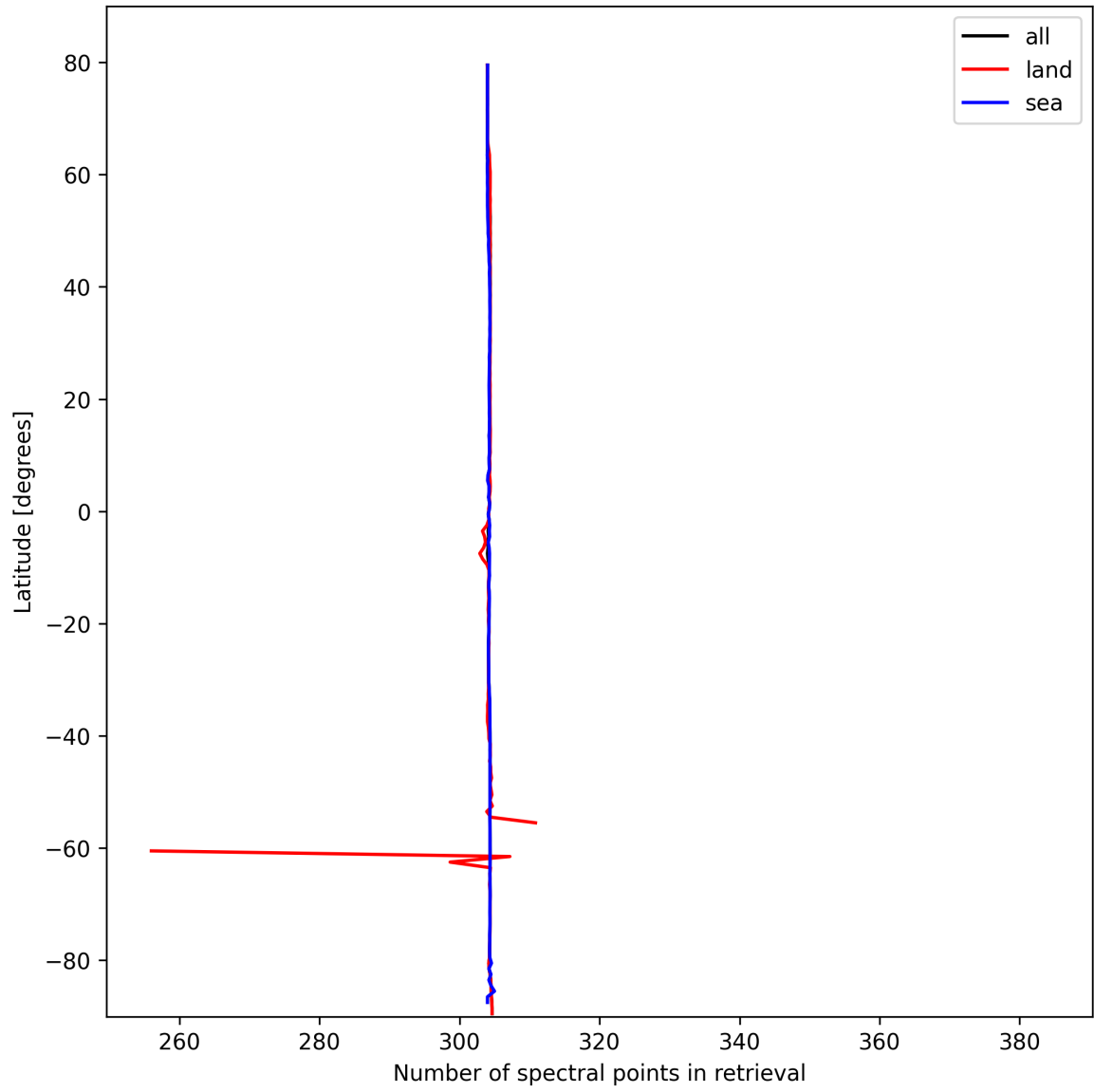
Figure 14: Zonal average of “Number of spectral points in retrieval” for 2025-10-14 to 2025-10-15.
