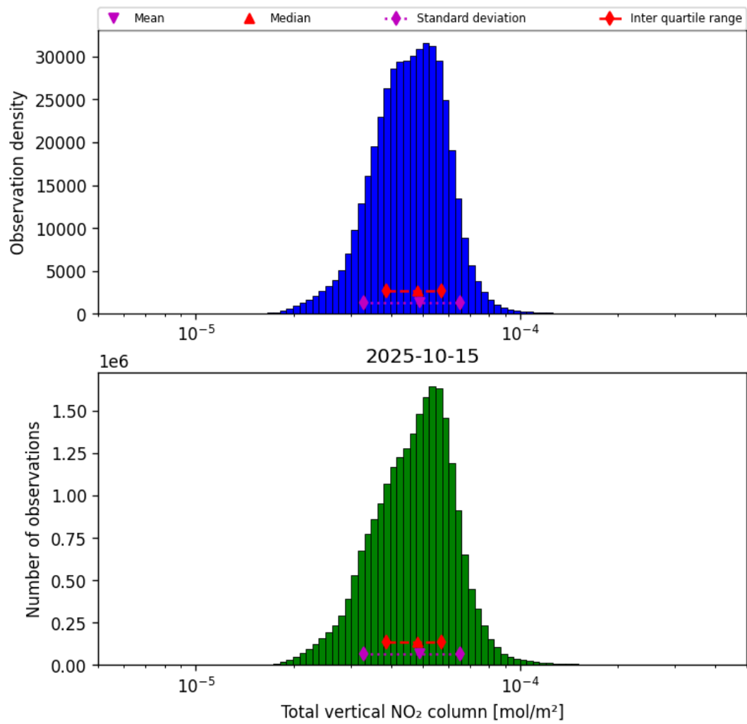
Figure 36: Histogram of “Total vertical NO 2 column” for 2025-10-15 to 2025-10-15
