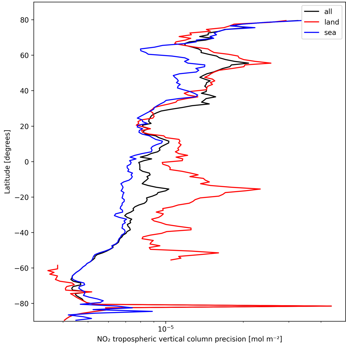
Figure 11: Zonal average of “NO 2 tropospheric vertical column precision” for 2025-10-15 to 2025-10-15.
