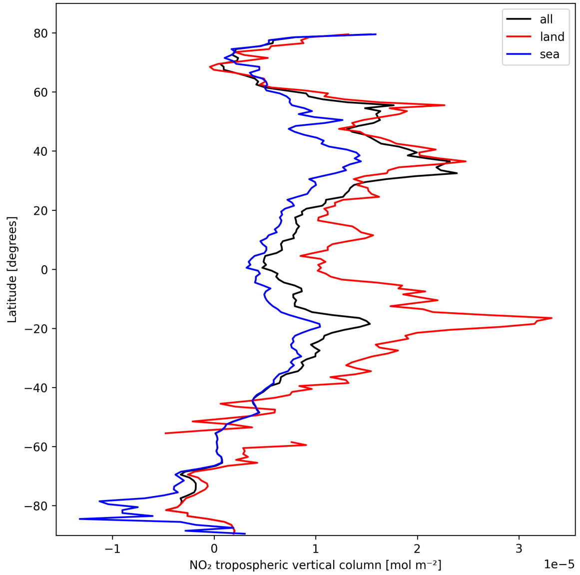
Figure 10: Zonal average of “NO 2 tropospheric vertical column” for 2025-10-15 to 2025-10-15.
