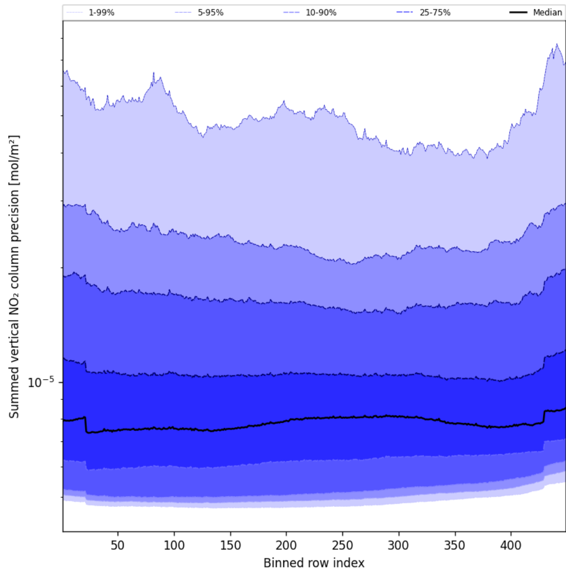
Figure 56: Along track statistics of “Summed vertical NO 2 column precision” for 2025-10-15 to 2025-10-15
