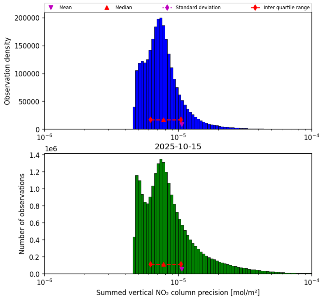
Figure 39: Histogram of "Summed vertical NO 2 column precision" for 2025-10-15 to 2025-10-15
