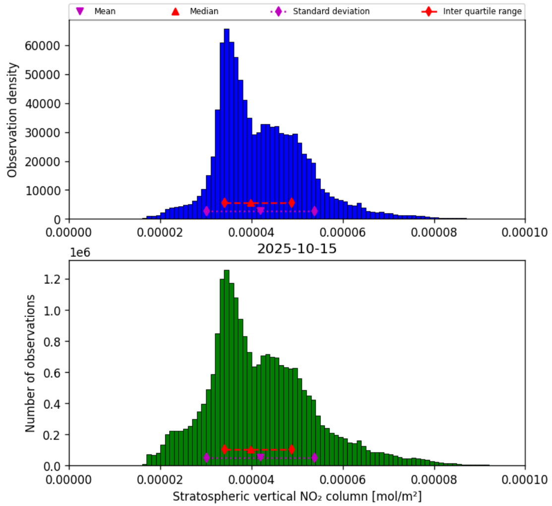
Figure 34: Histogram of “Stratospheric vertical NO 2 column” for 2025-10-15 to 2025-10-15
