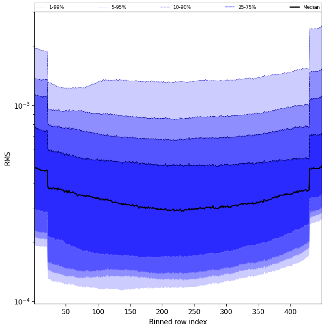
Figure 58: Along track statistics of “RMS” for 2025-10-15 to 2025-10-15
