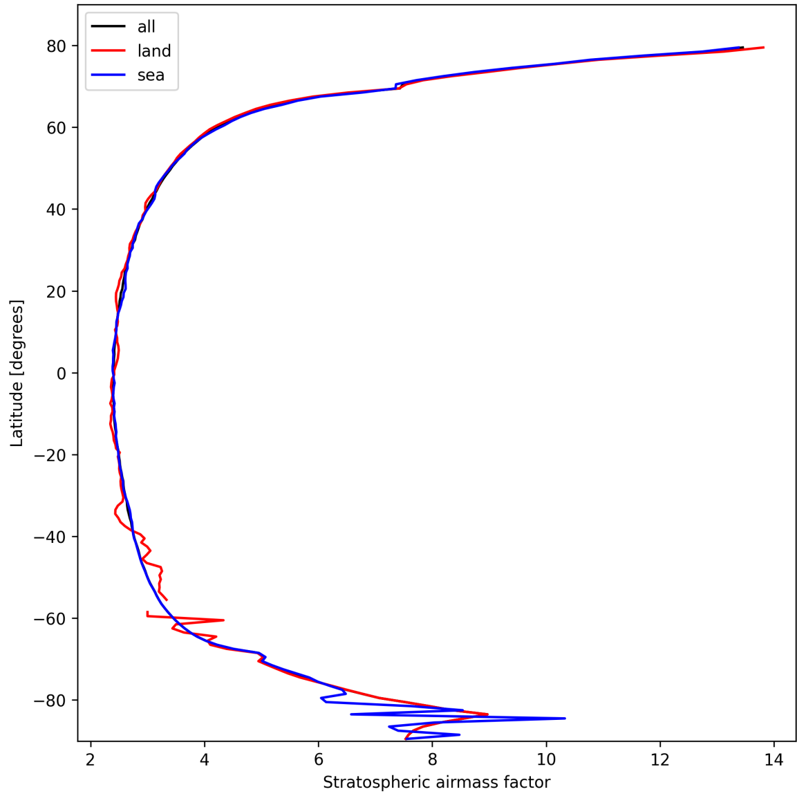
Figure 25: Zonal average of “Stratospheric air mass factor” for 2025-10-15 to 2025-10-15.
