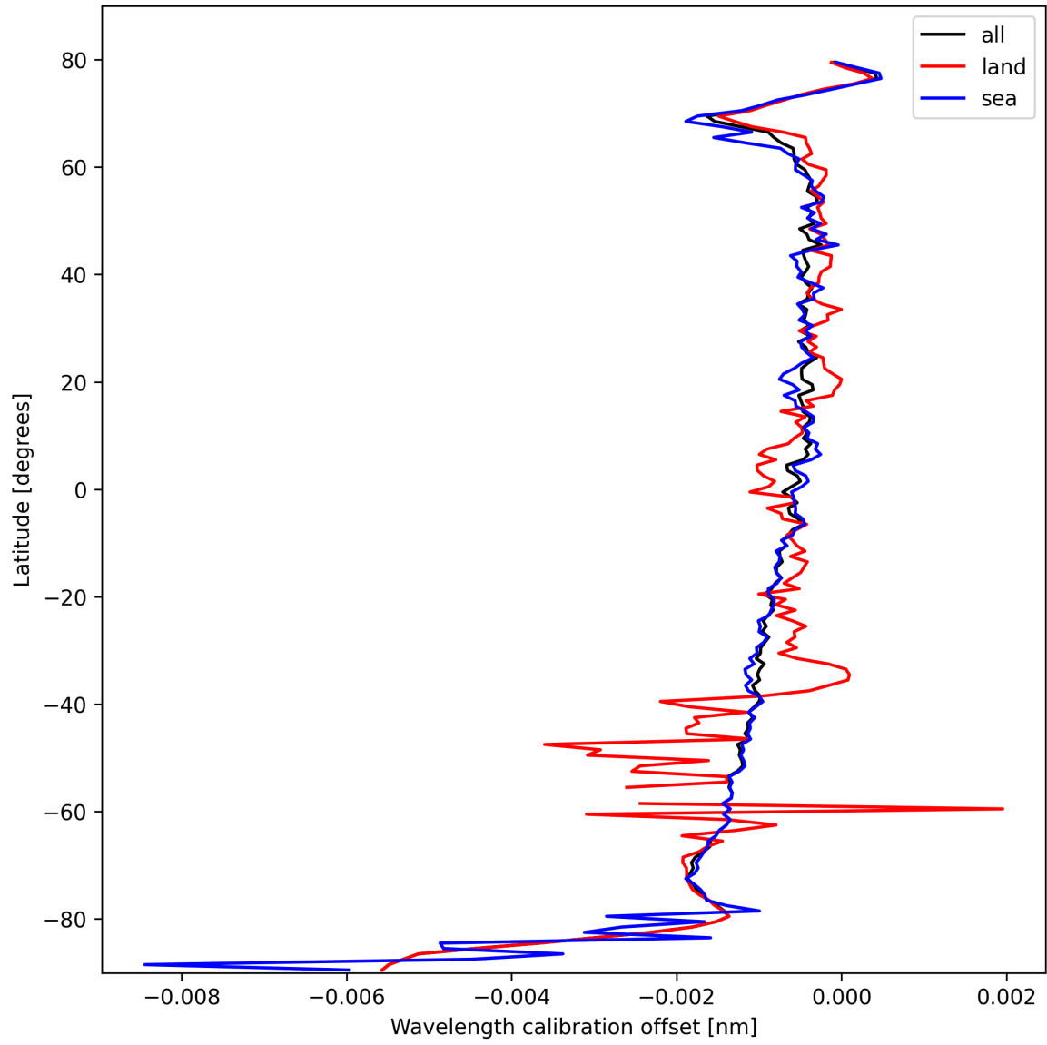
Figure 16: Zonal average of “Wavelength calibration offset” for 2025-10-15 to 2025-10-15.
