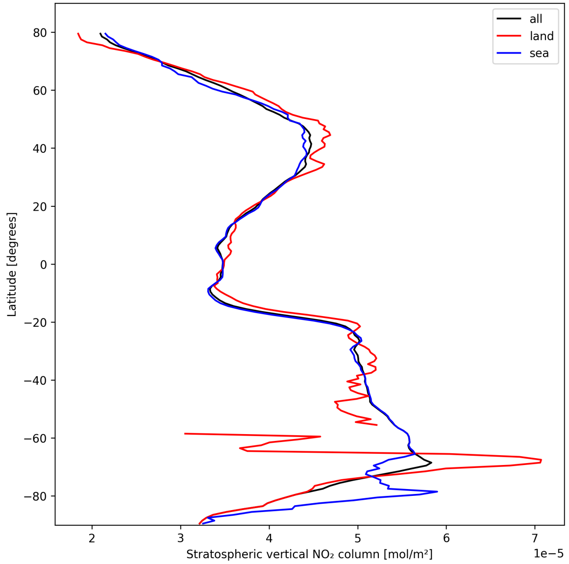
Figure 17: Zonal average of “Stratospheric vertical NO 2 column” for 2025-10-15 to 2025-10-15.
