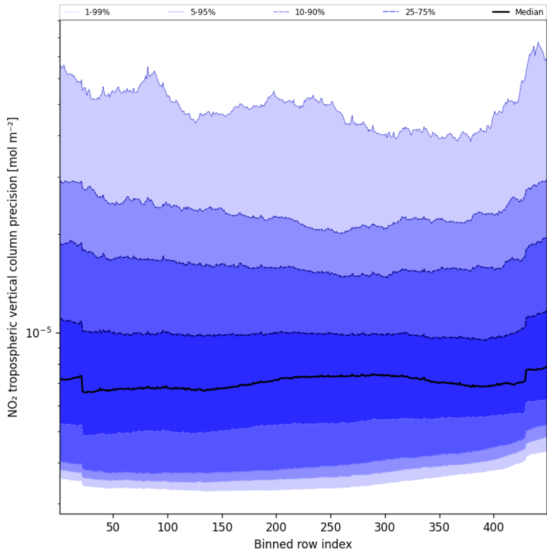
Figure 45: Along track statistics of “NO 2 tropospheric vertical column precision” for 2025-10-15 to 2025-10-15
