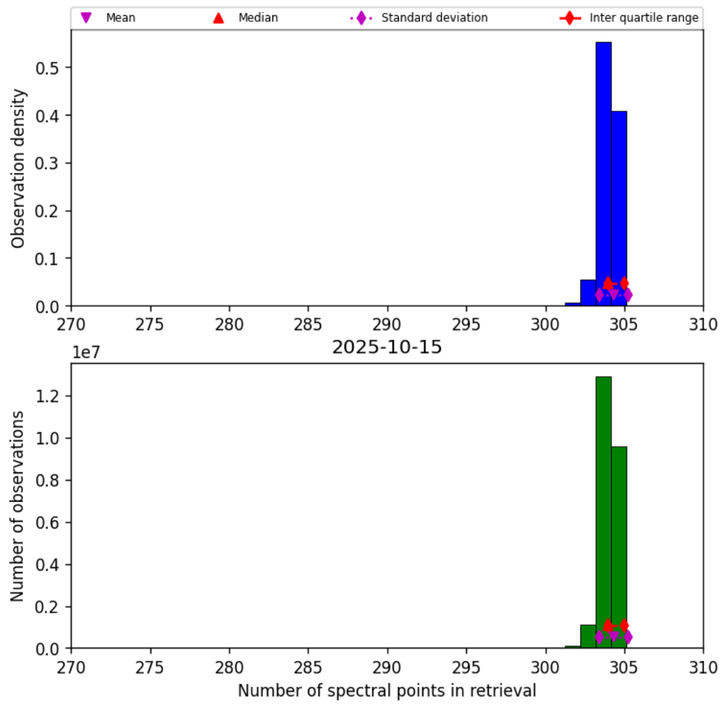
Figure 31: Histogram of “Number of spectral points in retrieval” for 2025-10-15 to 2025-10-15
