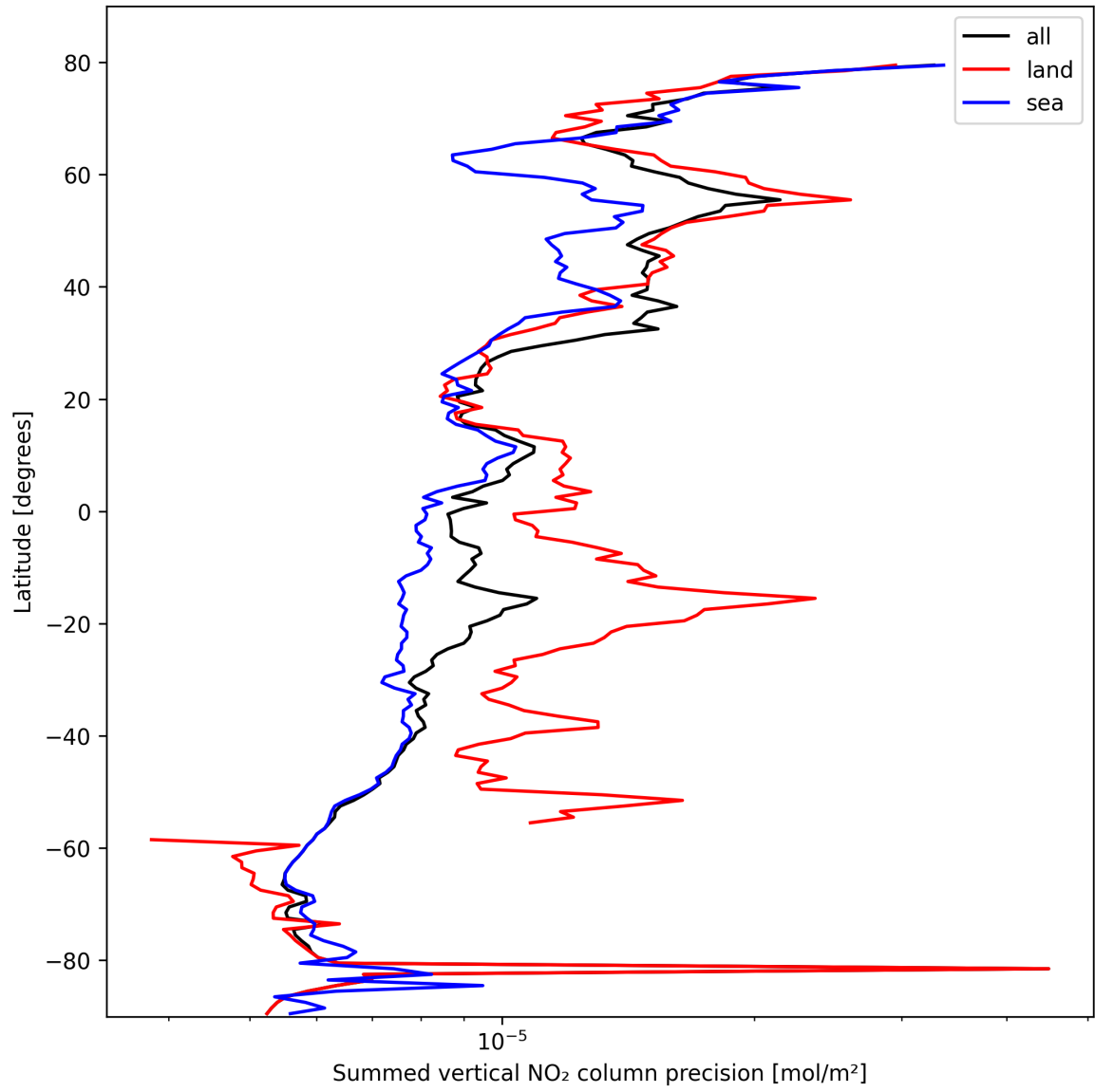
Figure 22: Zonal average of “Summed vertical NO 2 column precision” for 2025-10-15 to 2025-10-15.
