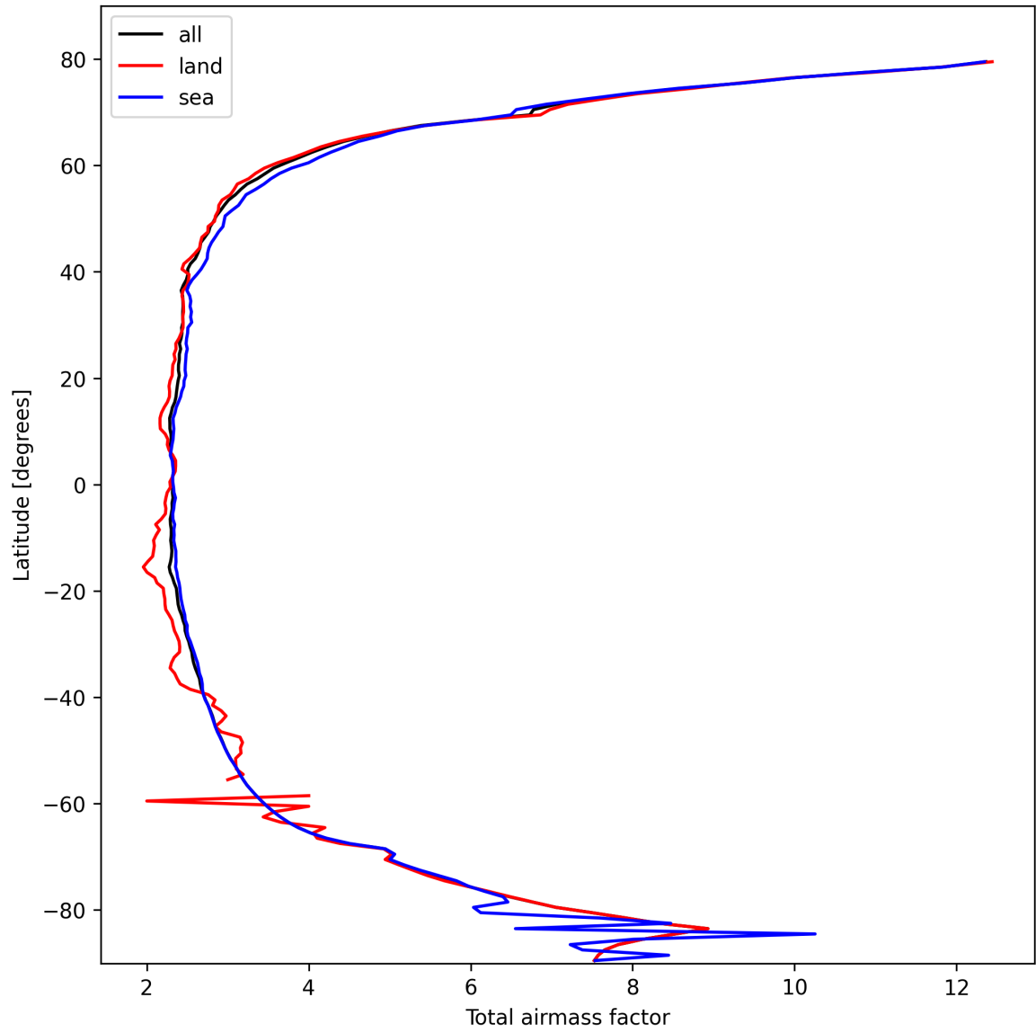
Figure 13: Zonal average of “Total airmass factor” for 2025-10-15 to 2025-10-15.
