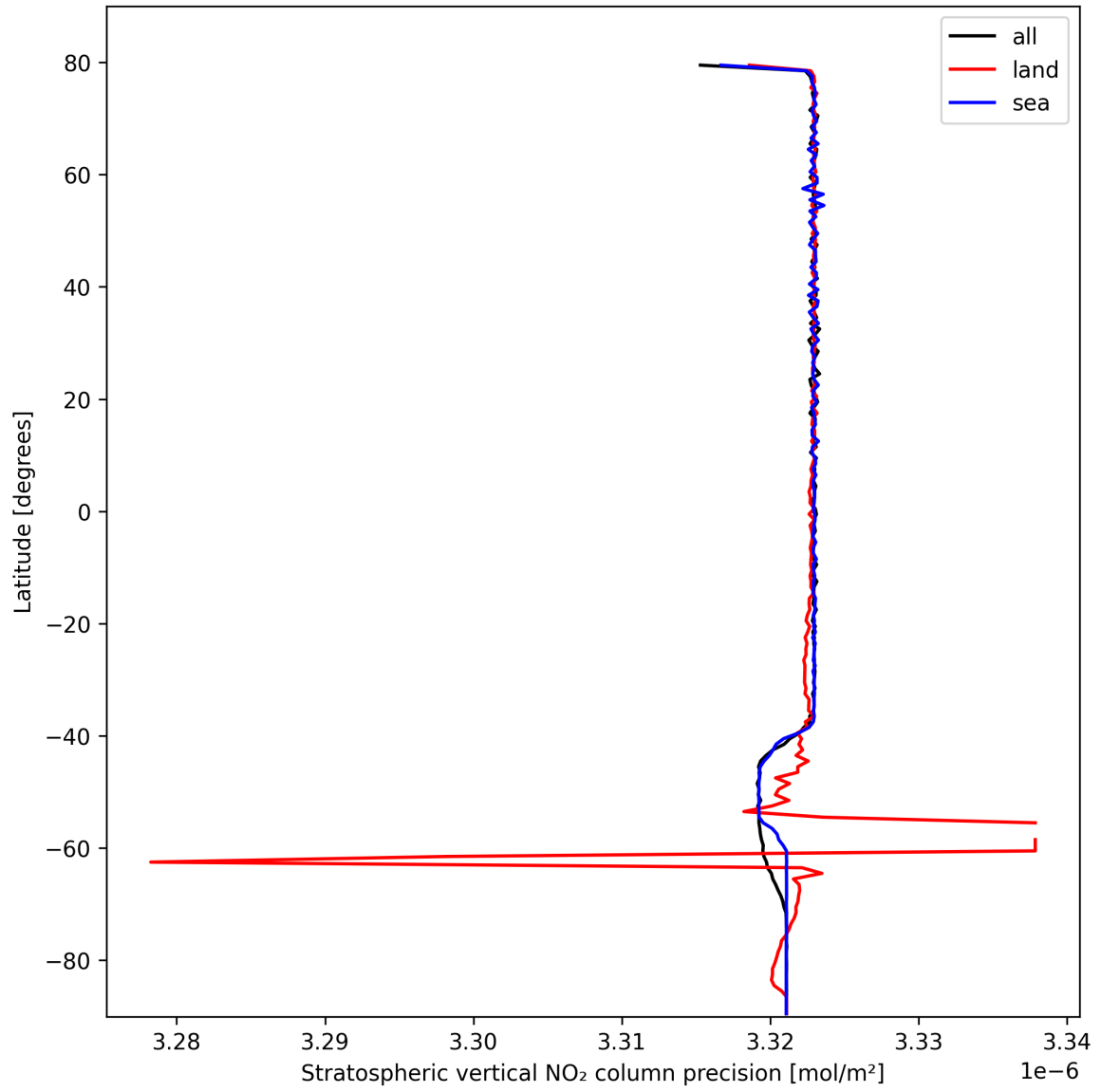
Figure 18: Zonal average of “Stratospheric vertical NO 2 column precision” for 2025-10-15 to 2025-10-15.
