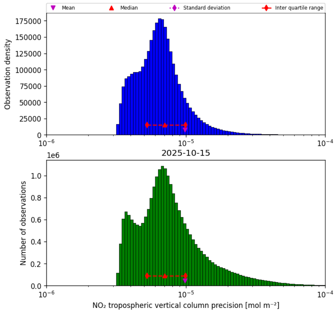
Figure 28: Histogram of “NO 2 tropospheric vertical column precision” for 2025-10-15 to 2025-10-15
