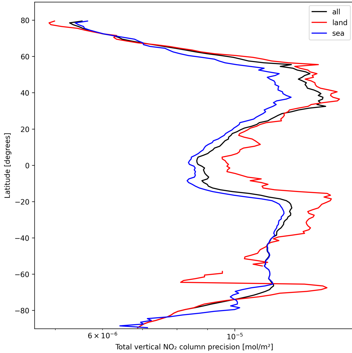
Figure 20: Zonal average of “Total vertical NO 2 column precision” for 2025-10-15 to 2025-10-15.
