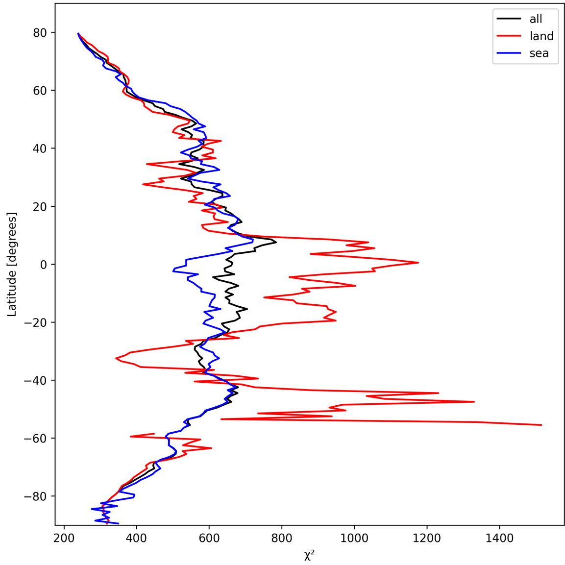
Figure 23: Zonal average of “ \chi^2 ” for 2025-10-15 to 2025-10-15.
