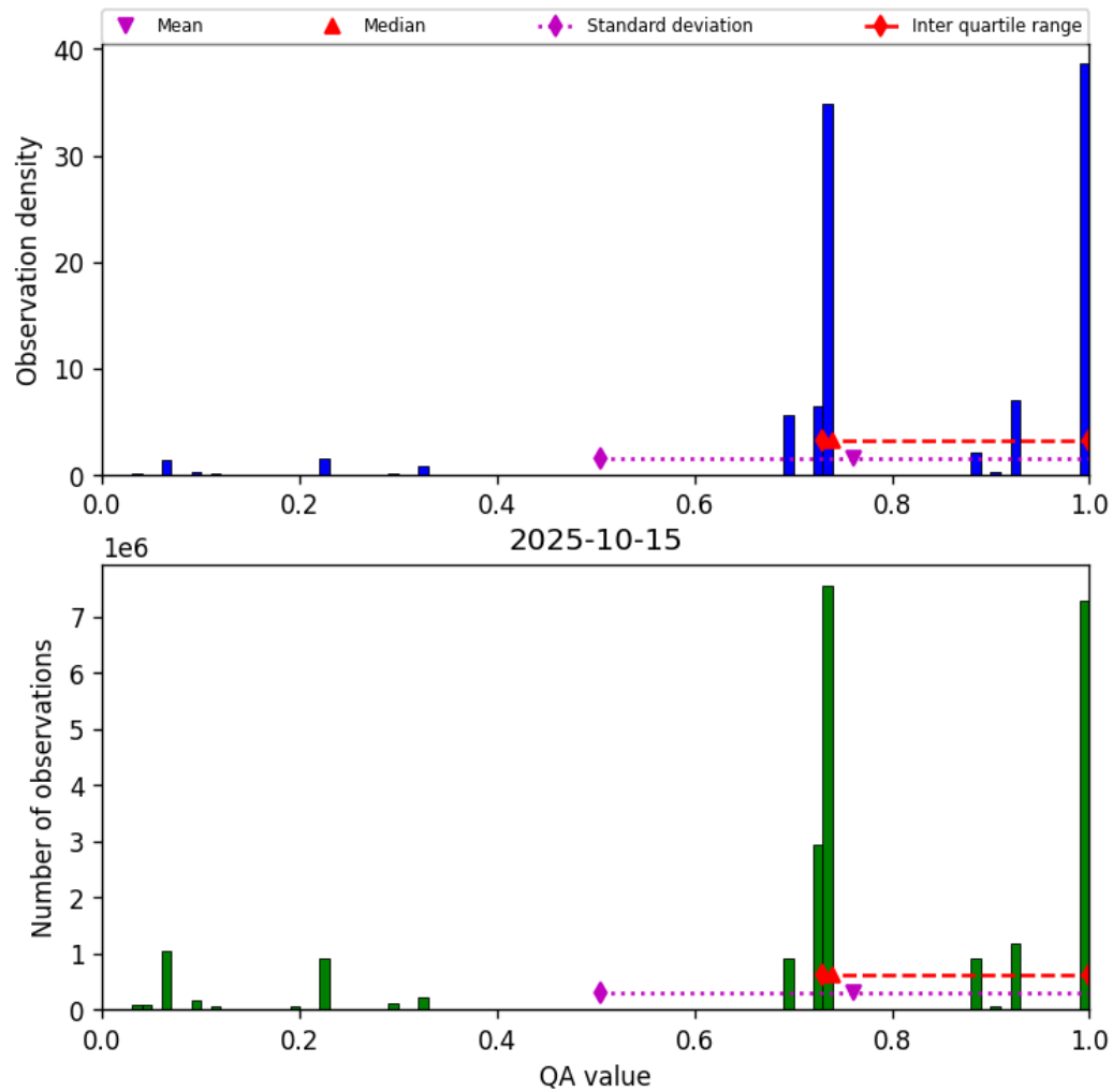
Figure 26: Histogram of “QA value” for 2025-10-15 to 2025-10-15
