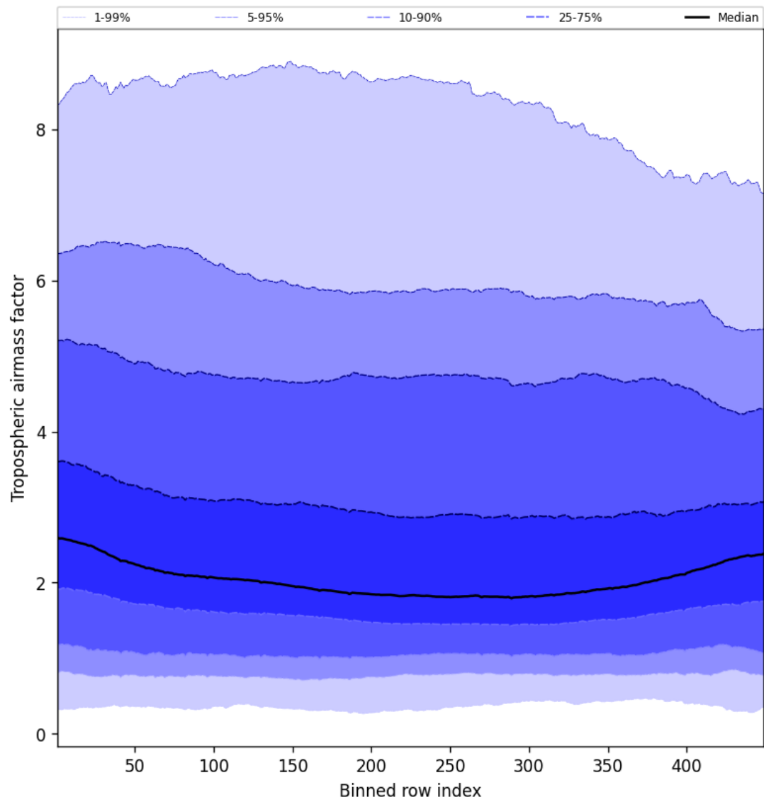
Figure 46: Along track statistics of “Tropospheric airmass factor” for 2025-10-15 to 2025-10-15
