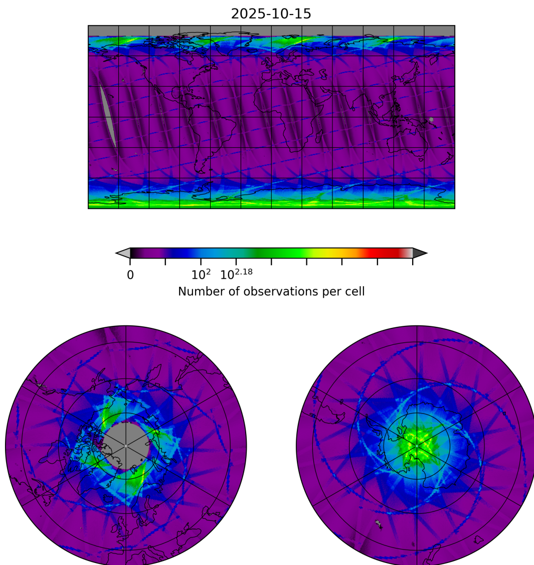
Figure 8: Map of the number of observations for 2025-10-15 to 2025-10-15
