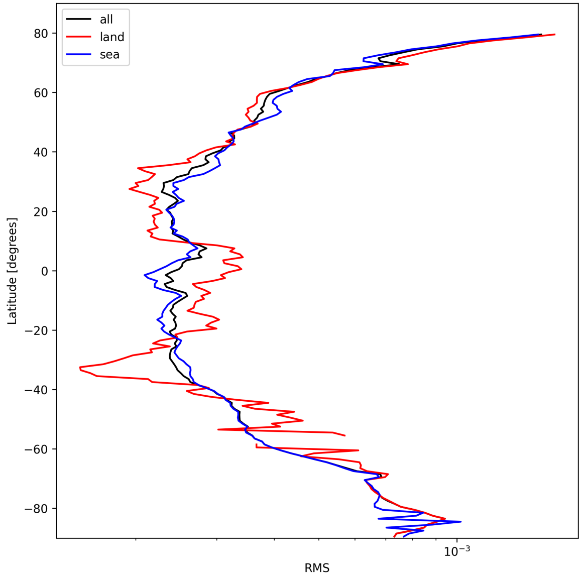
Figure 24: Zonal average of “RMS” for 2025-10-15 to 2025-10-15.
