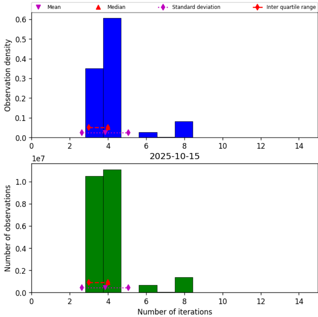
Figure 32: Histogram of “Number of iterations” for 2025-10-15 to 2025-10-15
