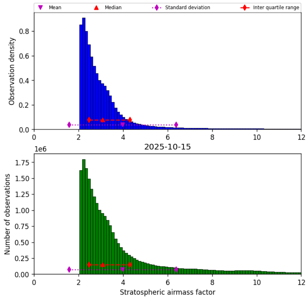
Figure 42: Histogram of “Stratospheric airmass factor” for 2025-10-15 to 2025-10-15
