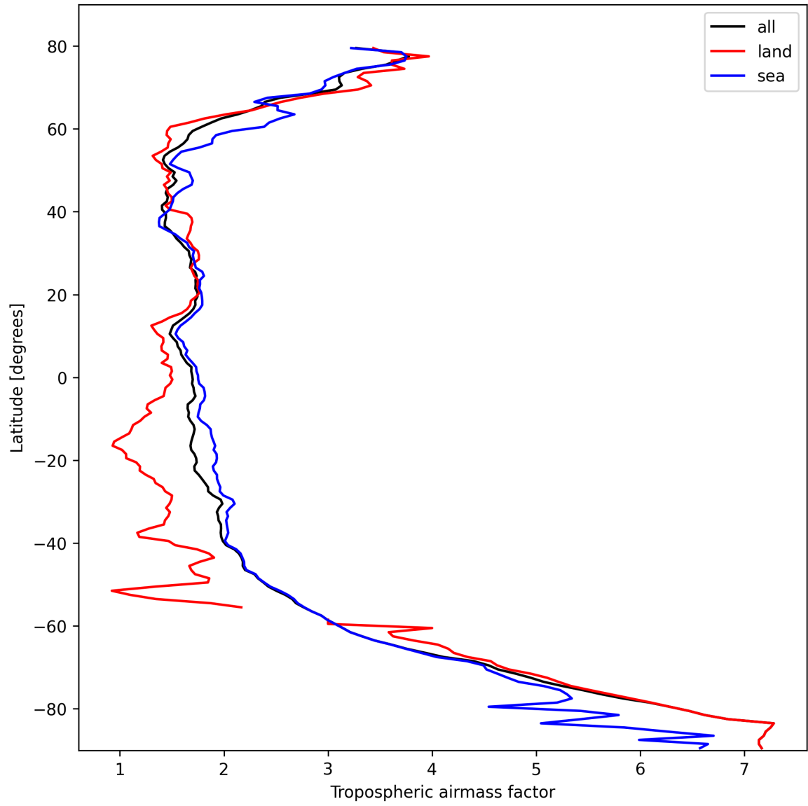
Figure 12: Zonal average of “Tropospheric airmass factor” for 2025-10-15 to 2025-10-15.
