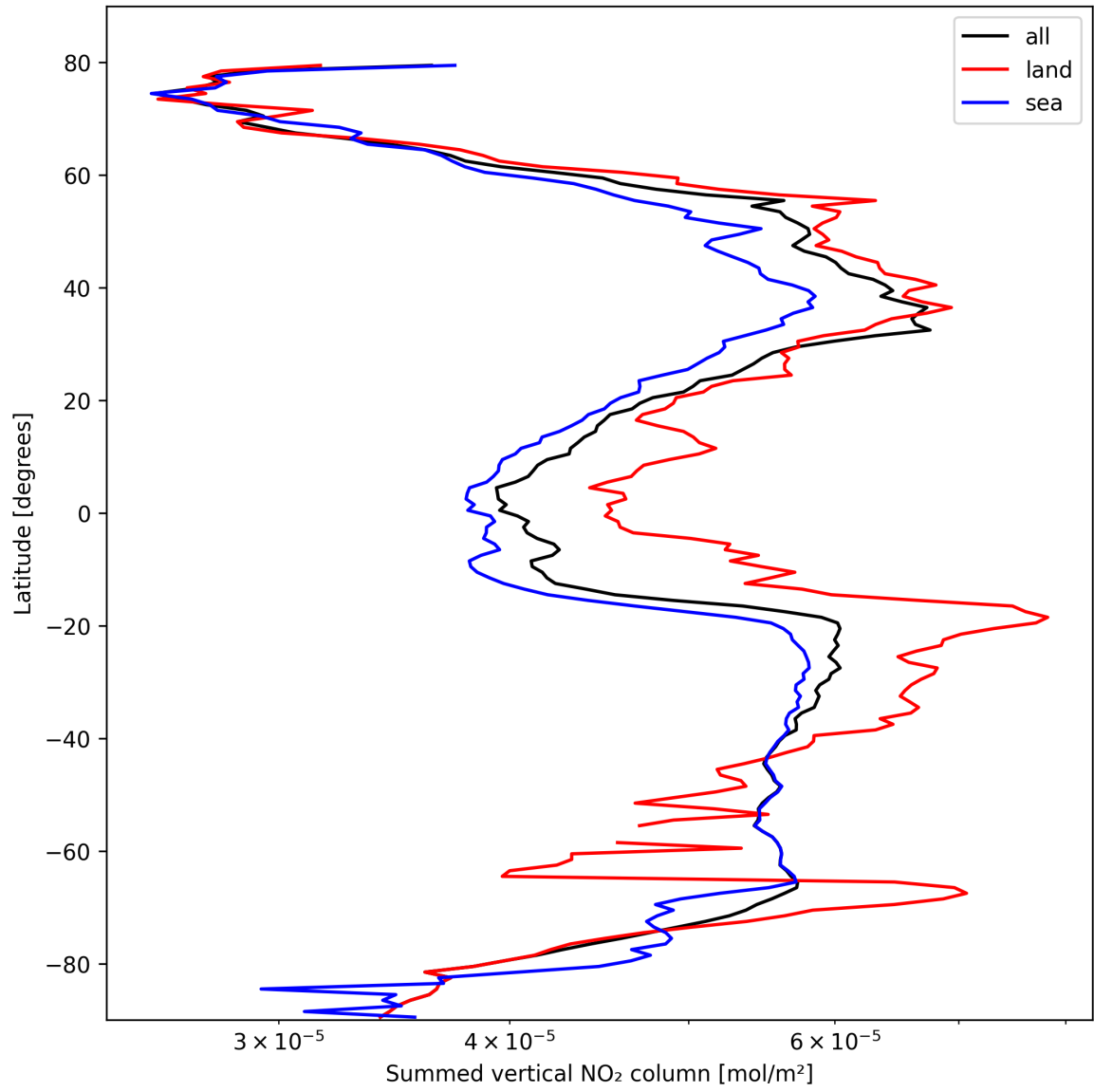
Figure 21: Zonal average of “Summed vertical NO 2 column” for 2025-10-15 to 2025-10-15.
