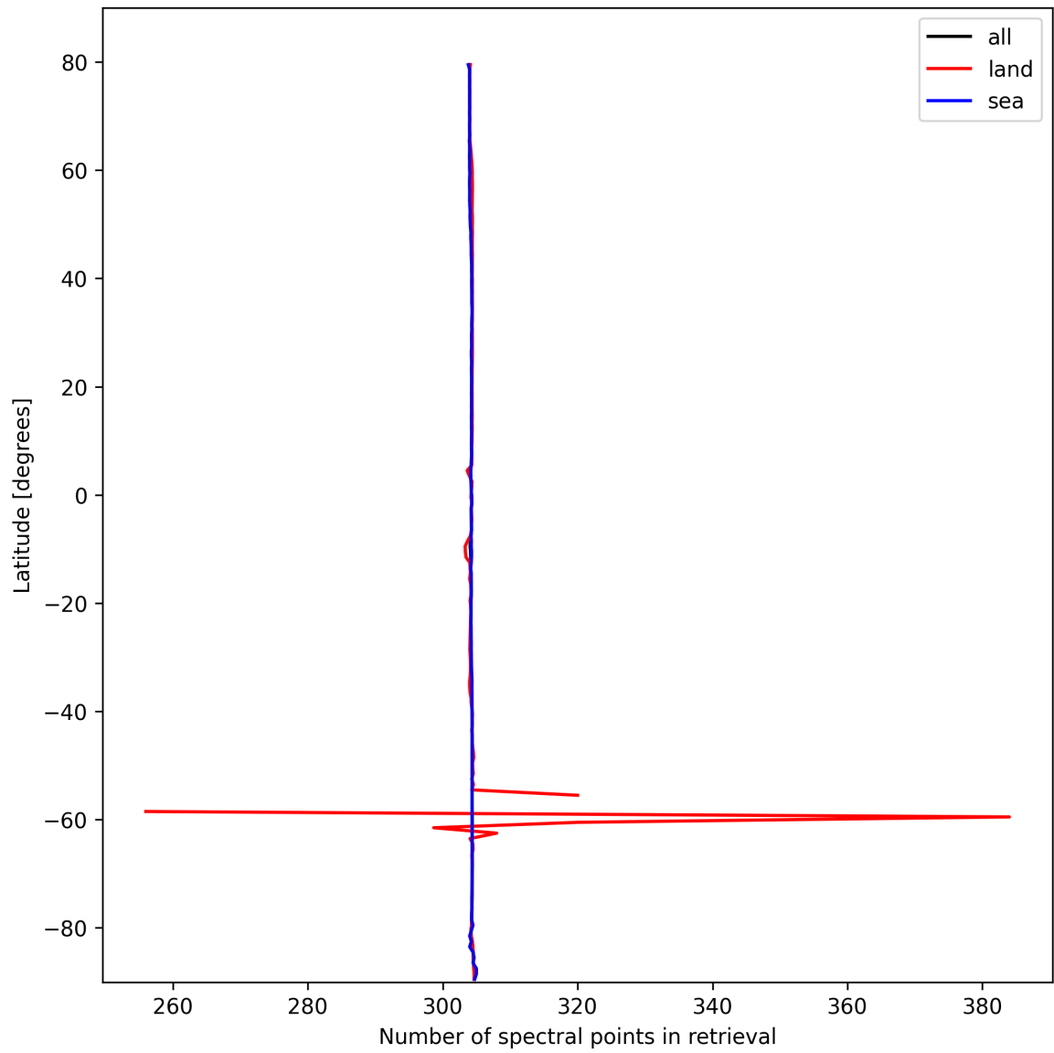
Figure 14: Zonal average of “Number of spectral points in retrieval” for 2025-10-15 to 2025-10-15.
