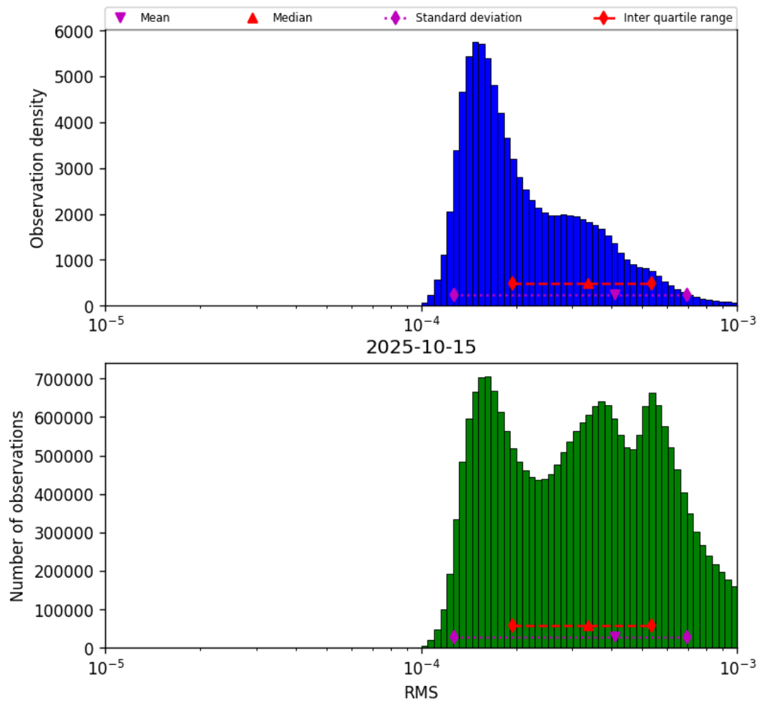
Figure 41: Histogram of “RMS” for 2025-10-15 to 2025-10-15
