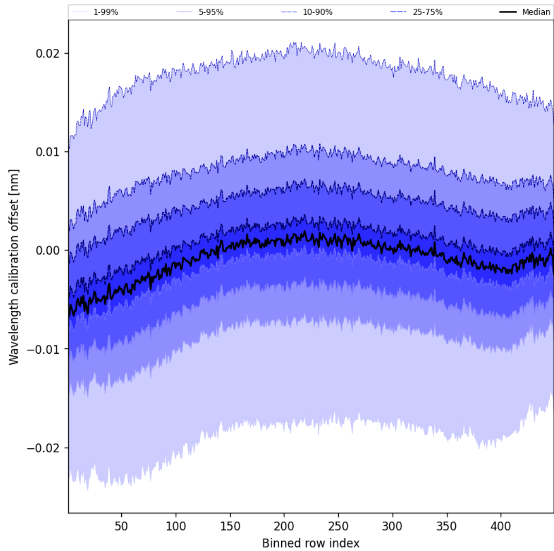
Figure 50: Along track statistics of “Wavelength calibration offset” for 2025-10-15 to 2025-10-15
