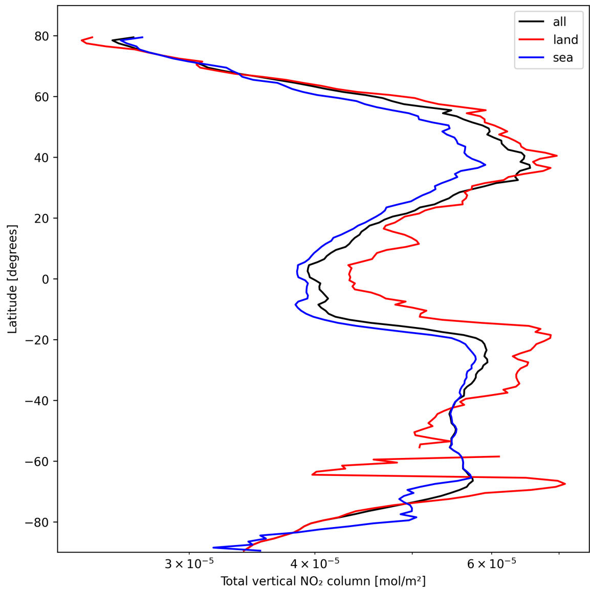
Figure 19: Zonal average of “Total vertical NO 2 column” for 2025-10-15 to 2025-10-15.
