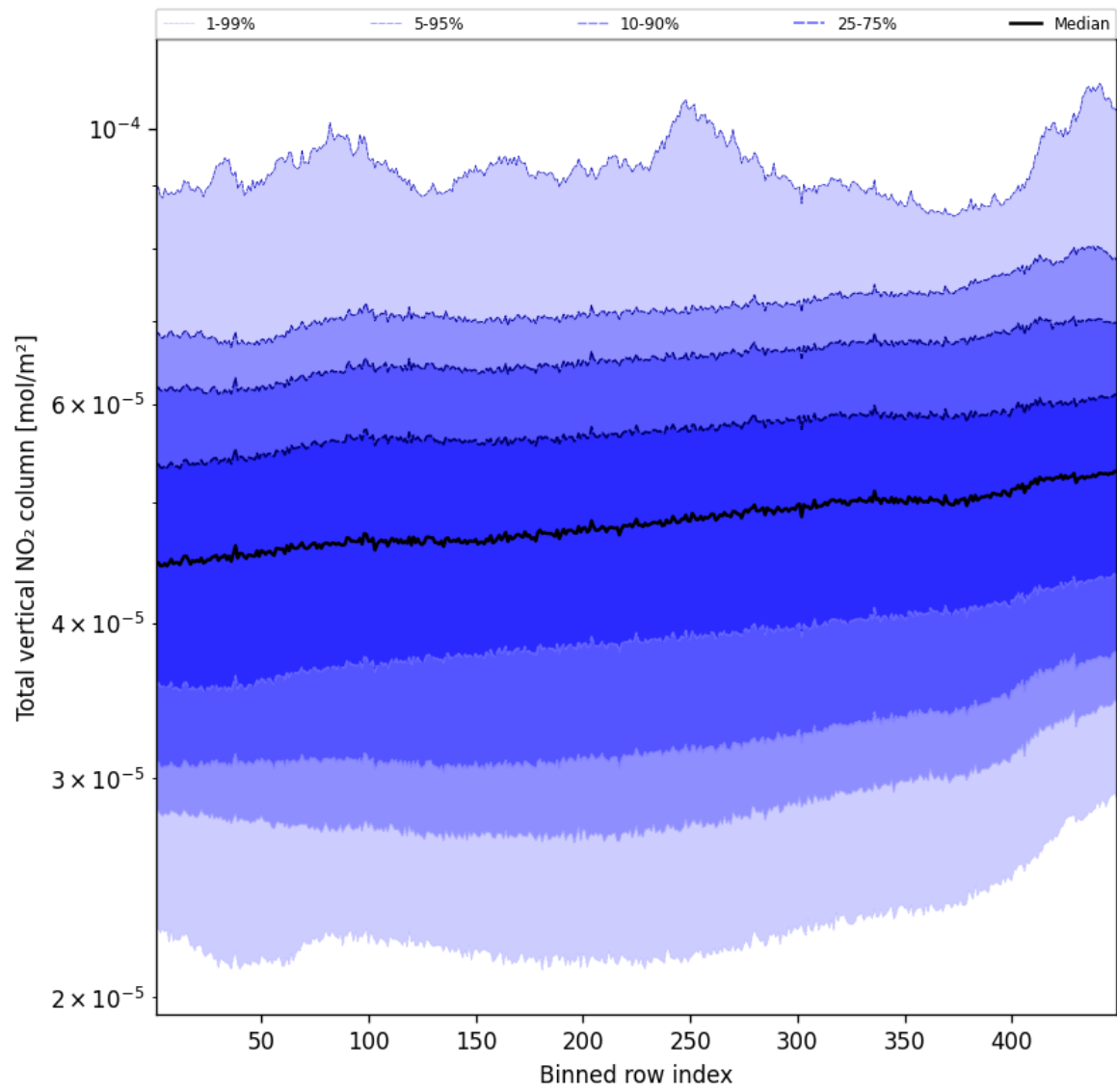
Figure 53: Along track statistics of “Total vertical NO 2 column” for 2025-10-15 to 2025-10-15
