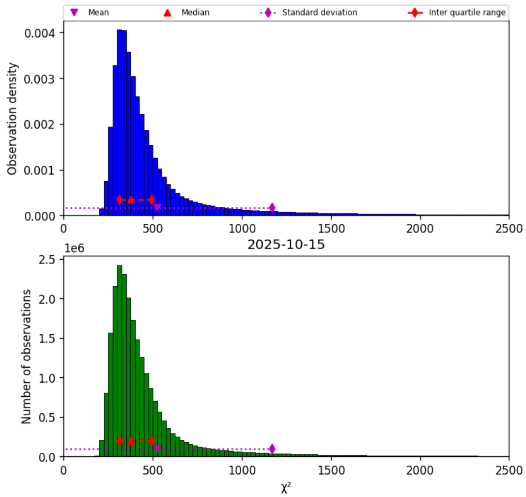
Figure 40: Histogram of “ \chi^2 ” for 2025-10-15 to 2025-10-15
