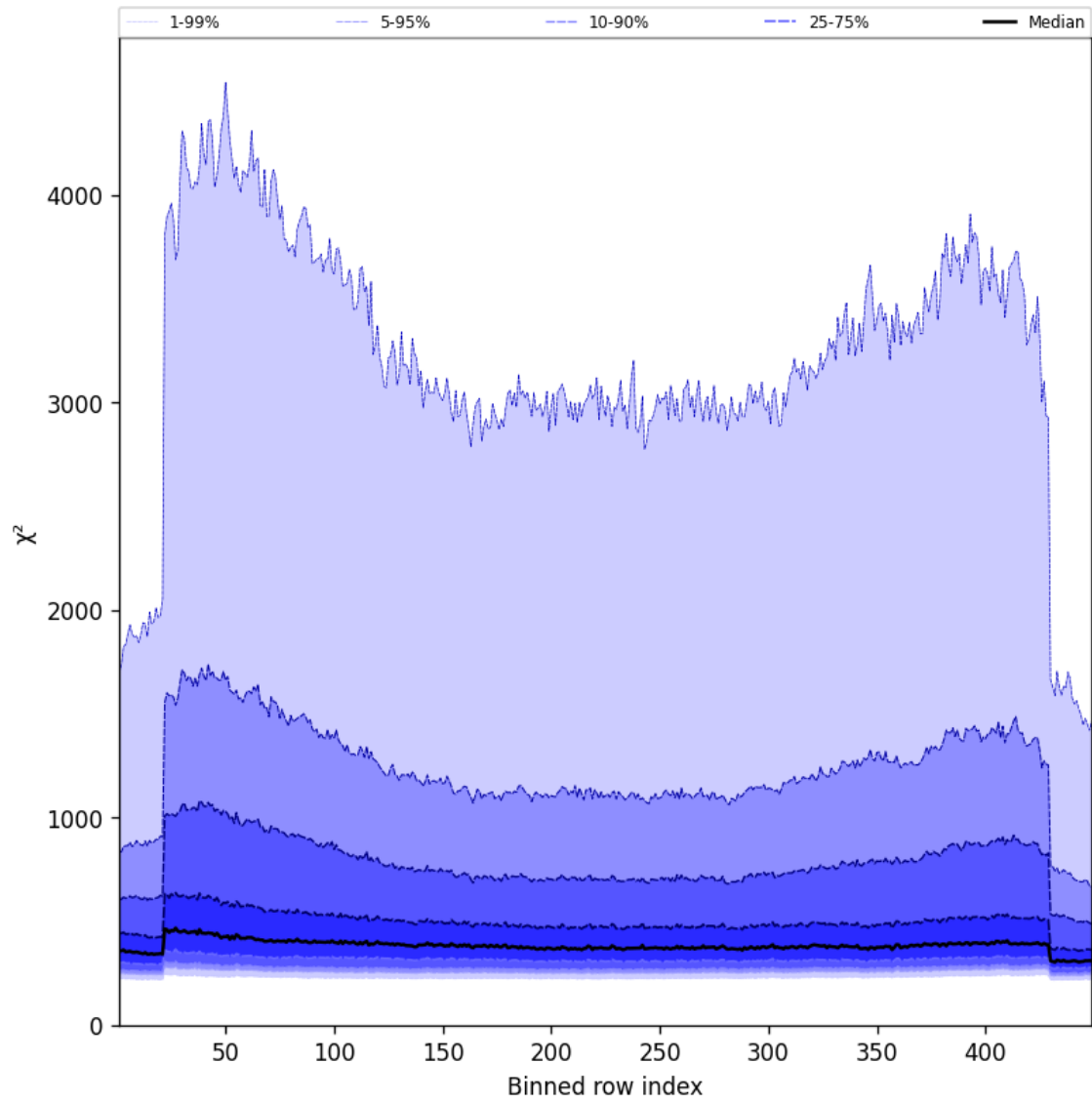
Figure 57: Along track statistics of “ \chi^2 ” for 2025-10-15 to 2025-10-15
