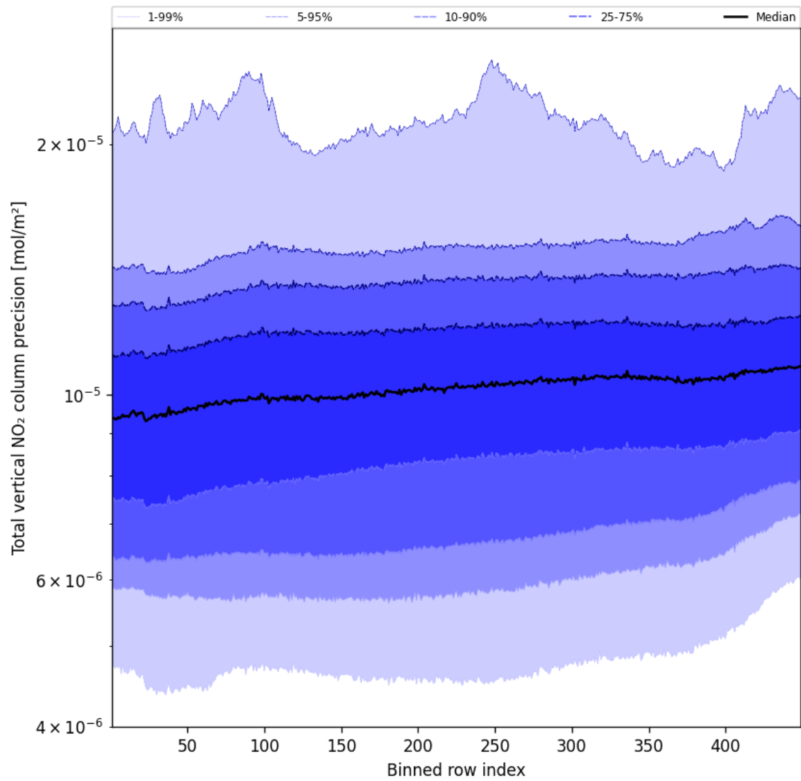
Figure 54: Along track statistics of “Total vertical NO 2 column precision” for 2025-10-15 to 2025-10-15
