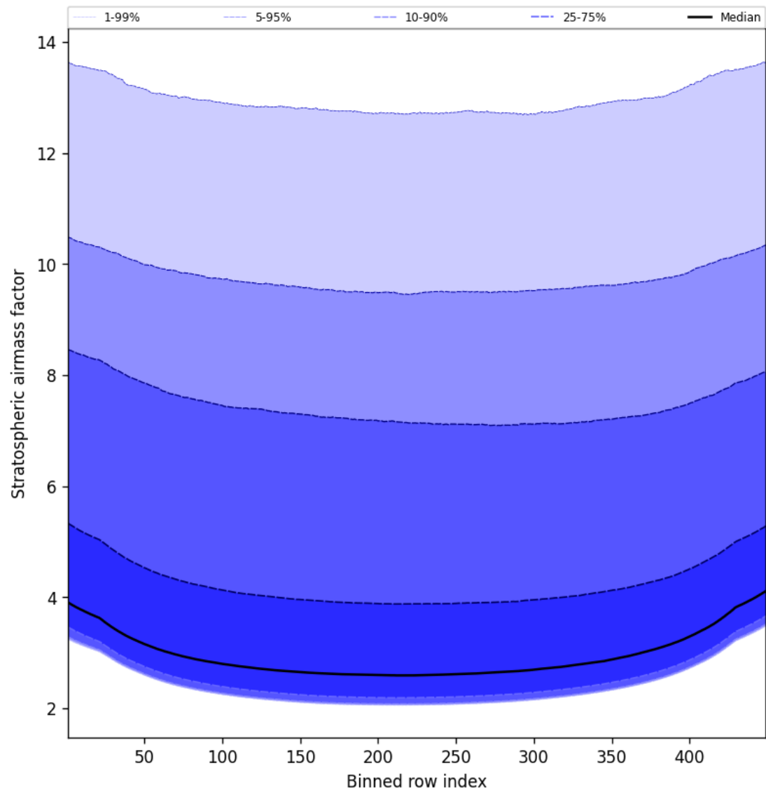
Figure 59: Along track statistics of “Stratospheric air mass factor” for 2025-10-15 to 2025-10-15
