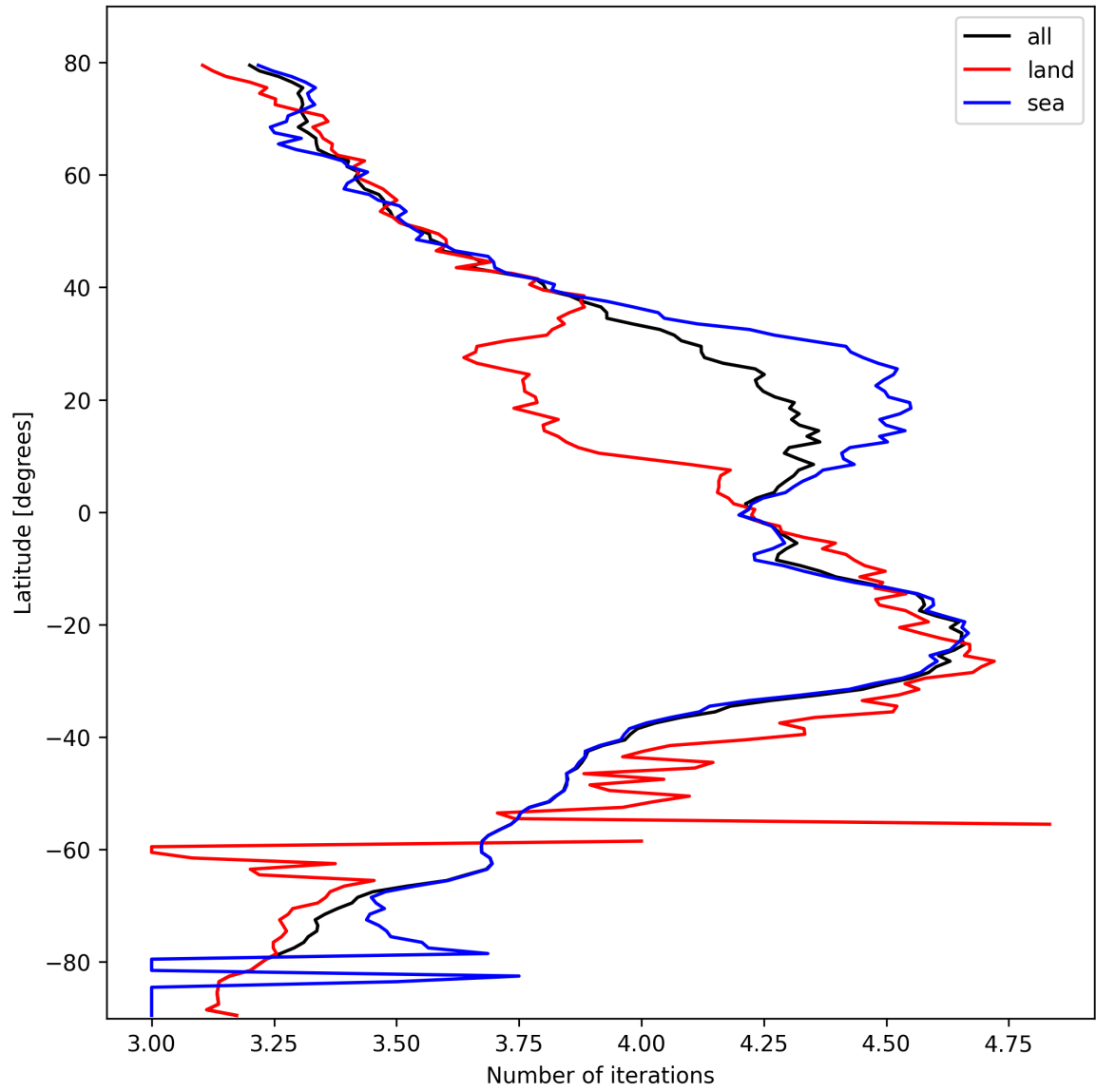
Figure 15: Zonal average of “Number of iterations” for 2025-10-15 to 2025-10-15.
