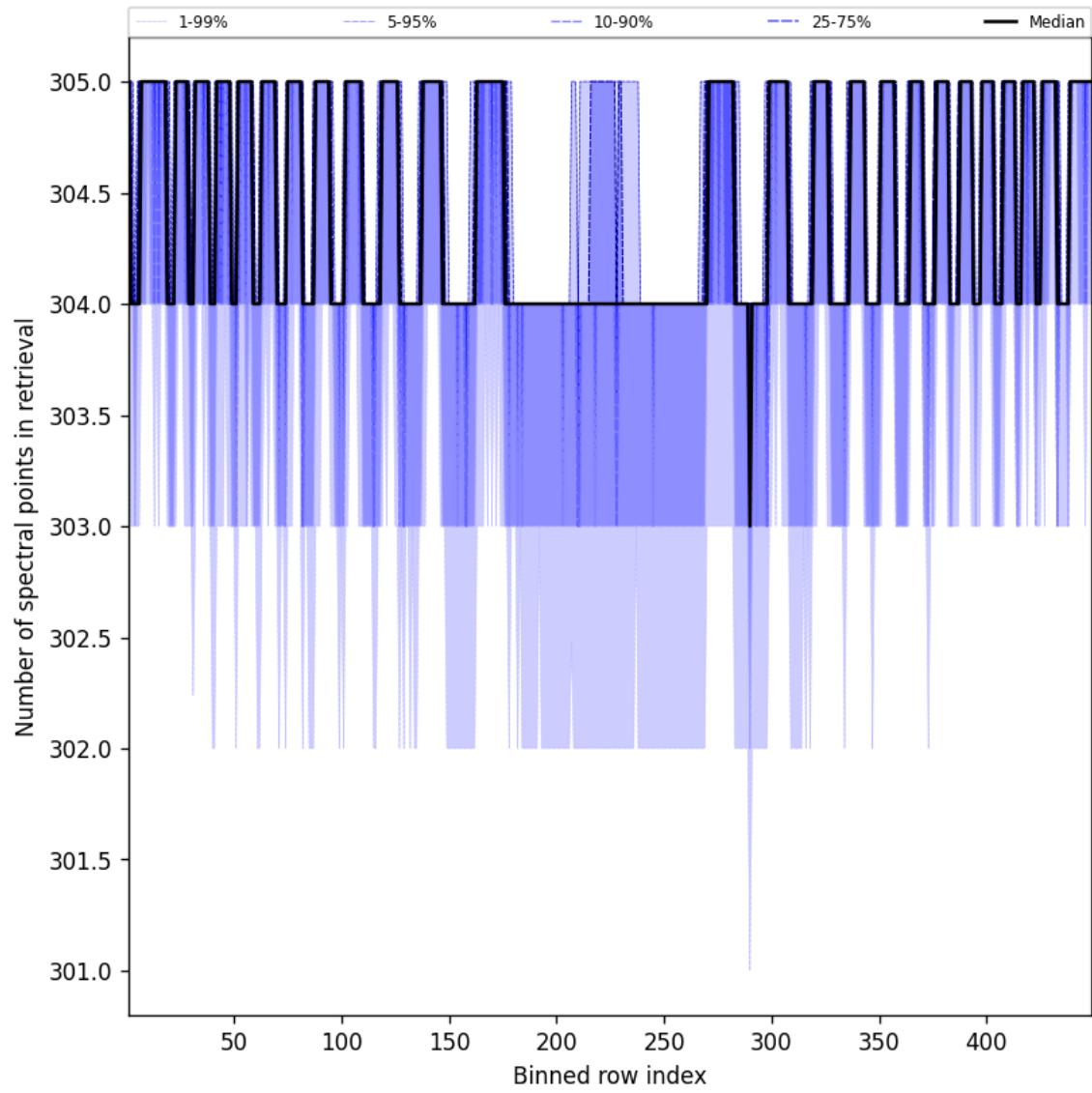
Figure 48: Along track statistics of “Number of spectral points in retrieval” for 2025-10-15 to 2025-10-15
