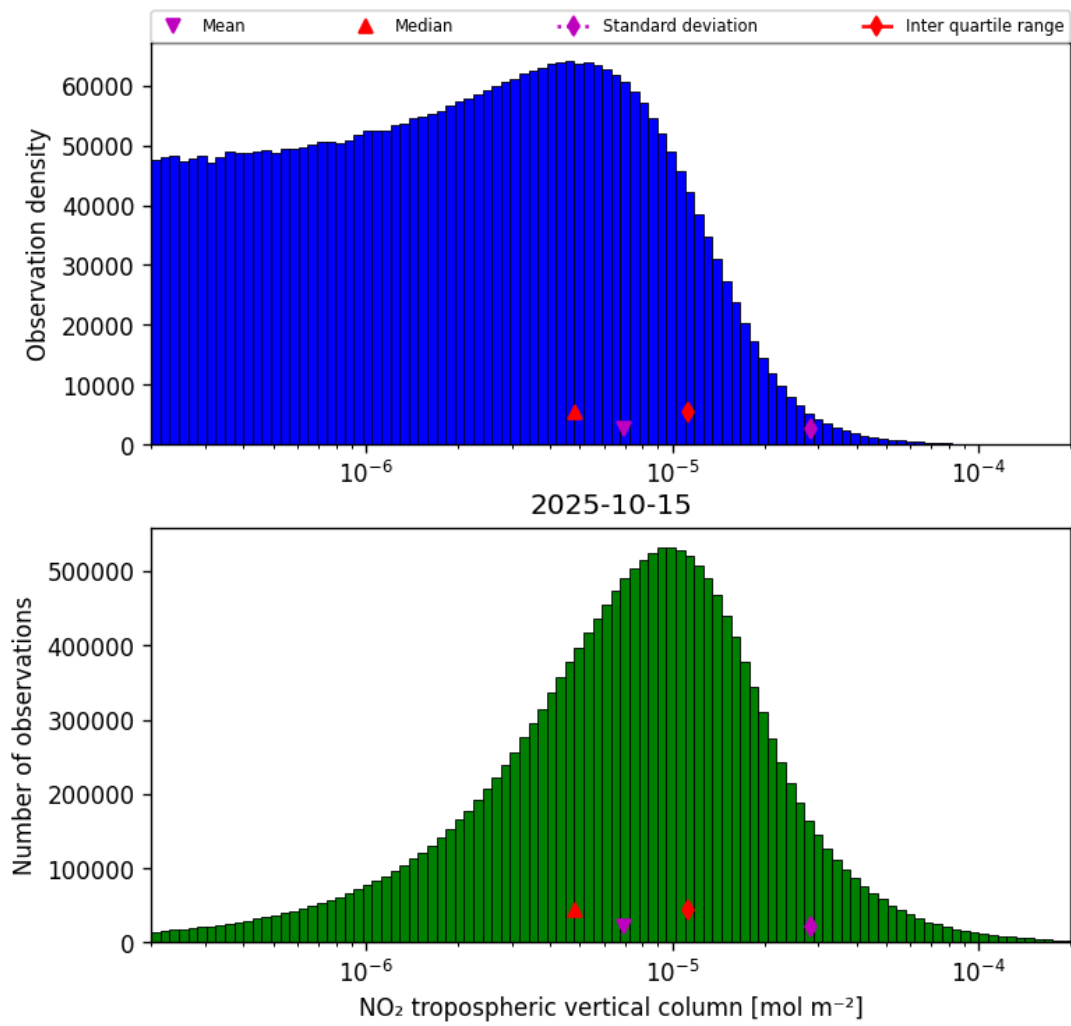
Figure 27: Histogram of “NO 2 tropospheric vertical column” for 2025-10-15 to 2025-10-15
