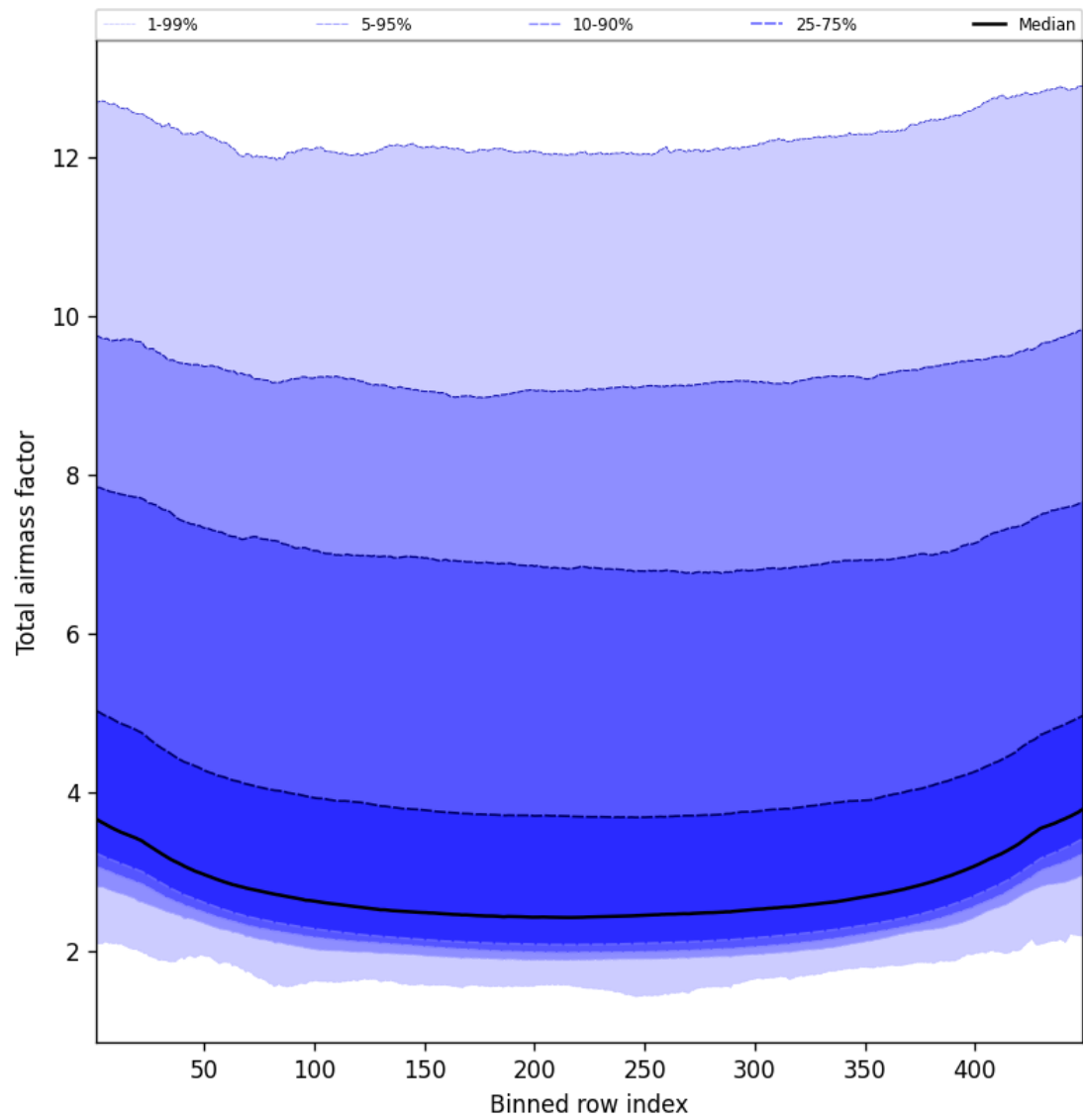
Figure 47: Along track statistics of “Total airmass factor” for 2025-10-15 to 2025-10-15
