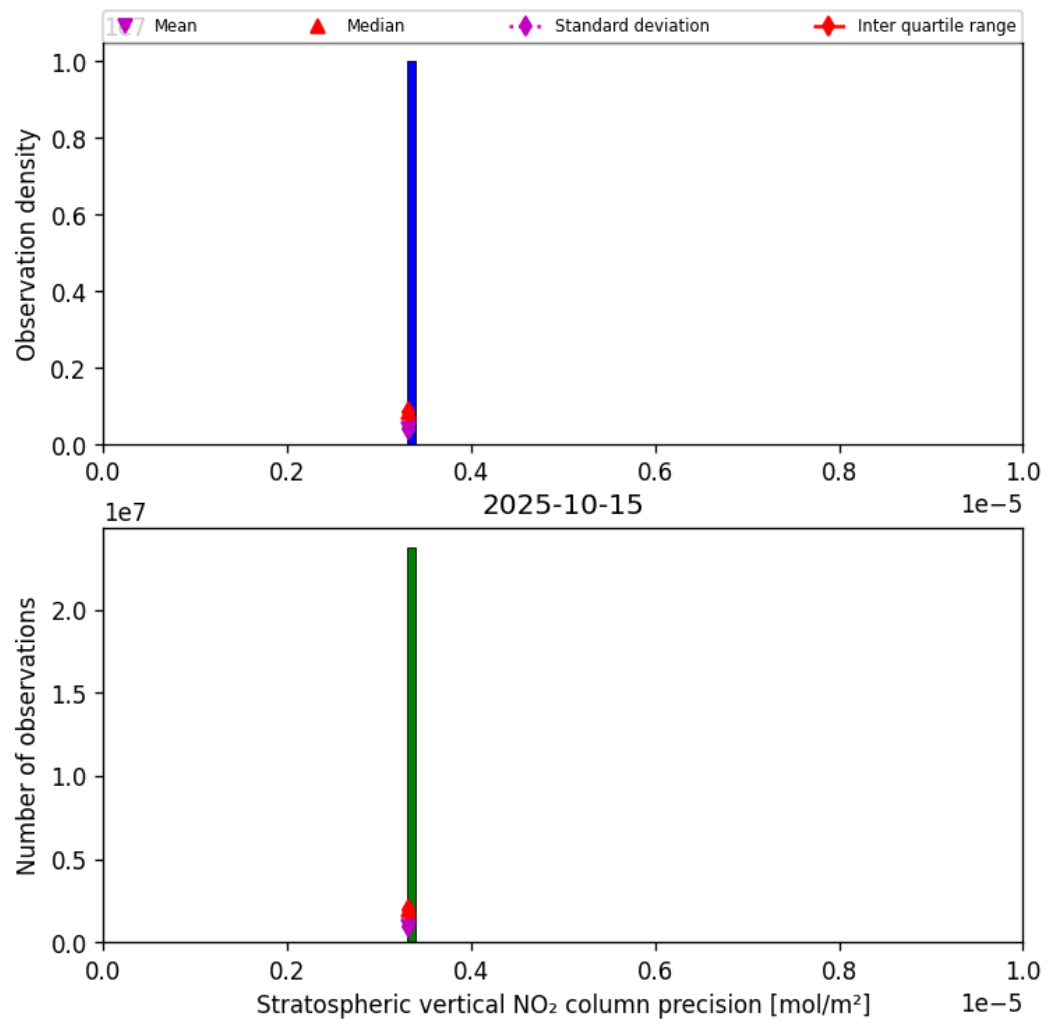
Figure 35: Histogram of “Stratospheric vertical NO 2 column precision” for 2025-10-15 to 2025-10-15
