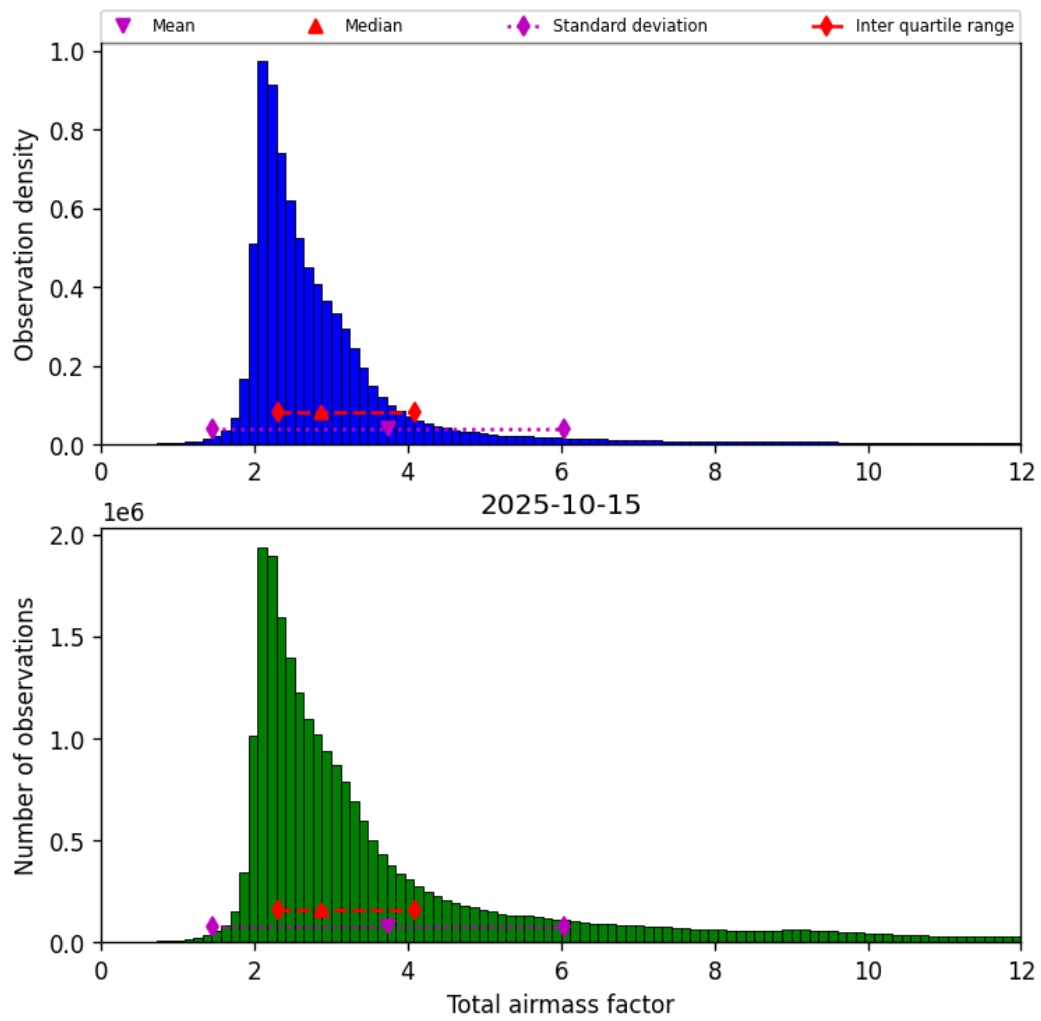
Figure 30: Histogram of “Total airmass factor” for 2025-10-15 to 2025-10-15
