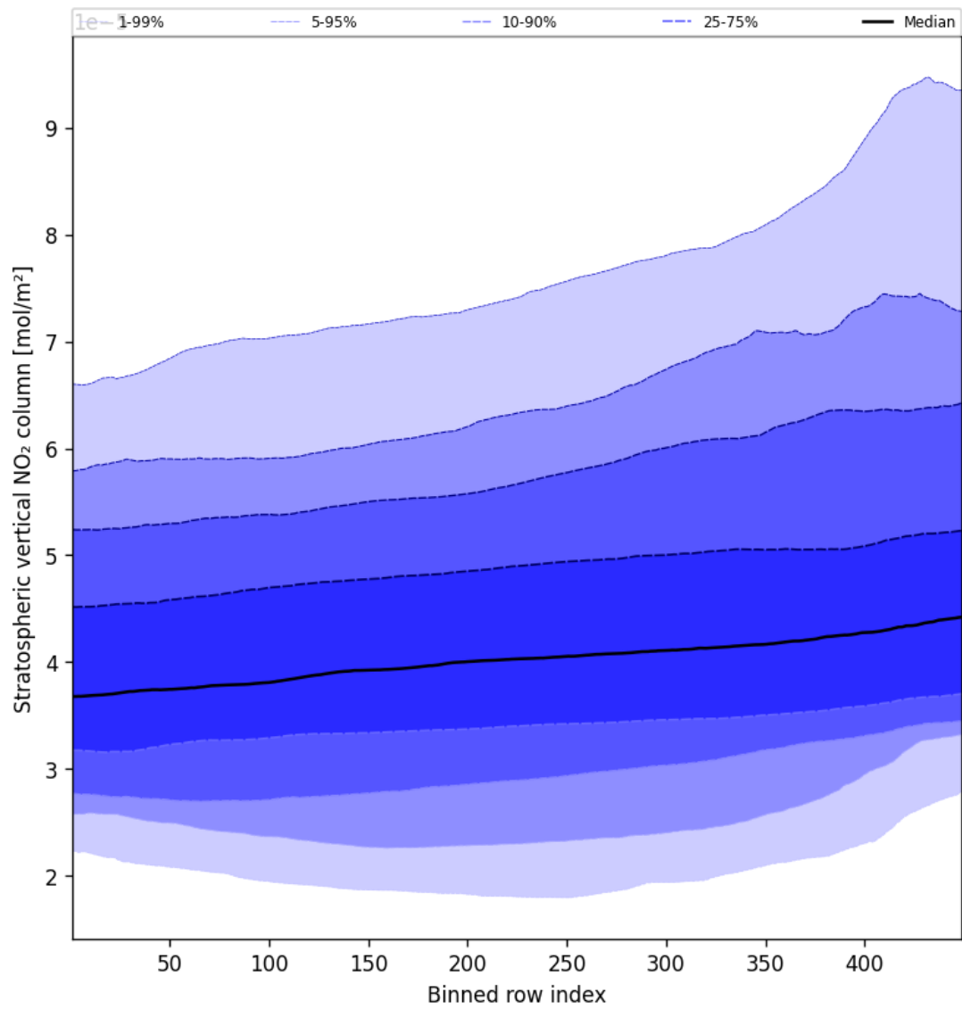
Figure 51: Along track statistics of “Stratospheric vertical NO 2 column” for 2025-10-15 to 2025-10-15
