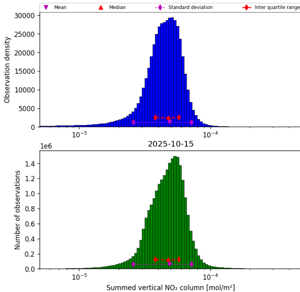
Figure 38: Histogram of “Summed vertical NO 2 column” for 2025-10-15 to 2025-10-15
