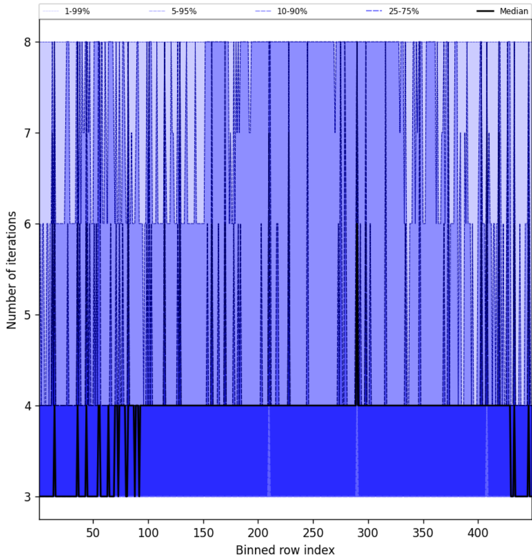
Figure 49: Along track statistics of “Number of iterations” for 2025-10-15 to 2025-10-15
