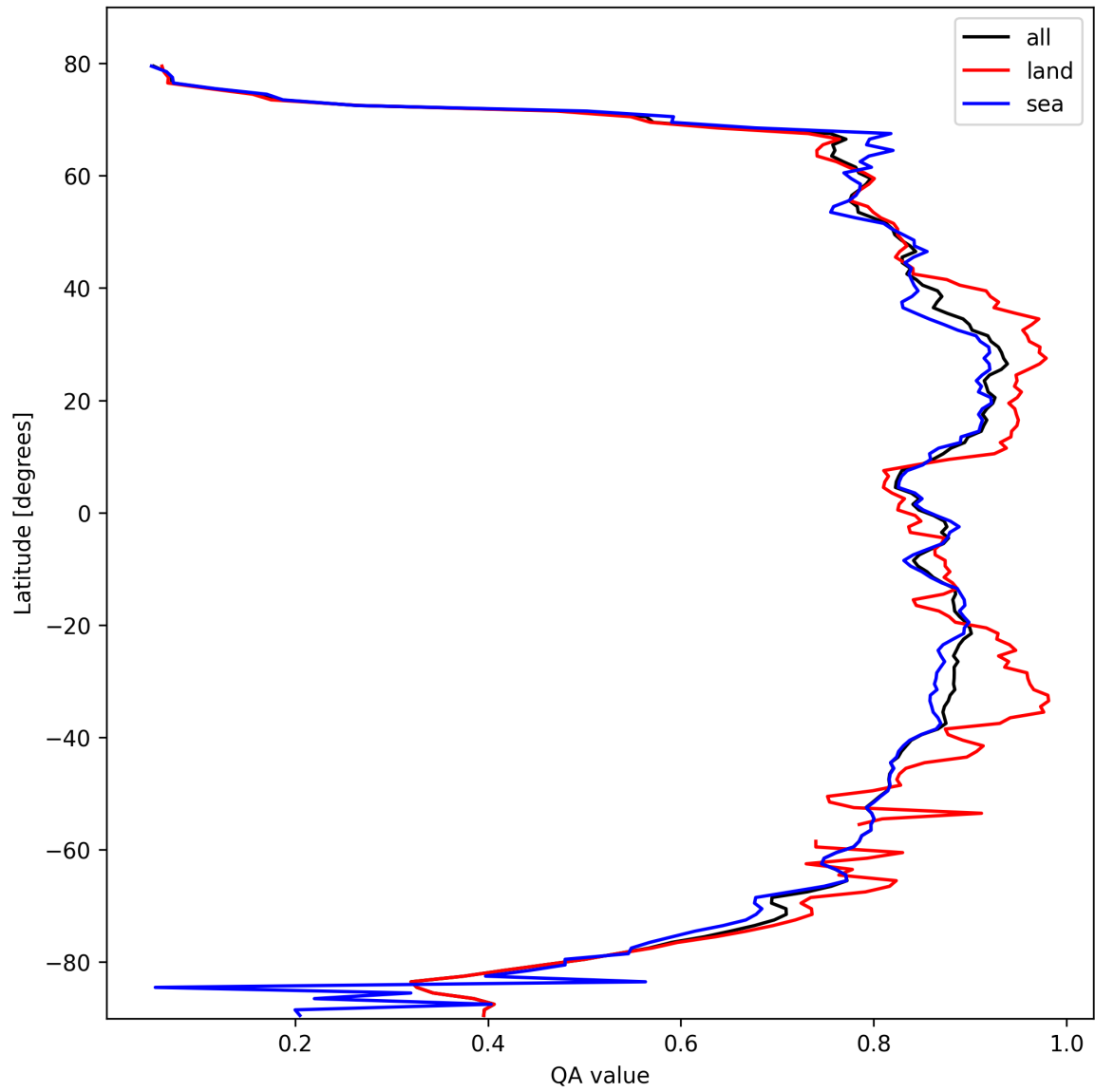
Figure 9: Zonal average of “QA value” for 2025-10-15 to 2025-10-15.
