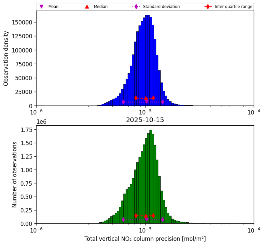
Figure 37: Histogram of "Total vertical NO 2 column precision" for 2025-10-15 to 2025-10-15
