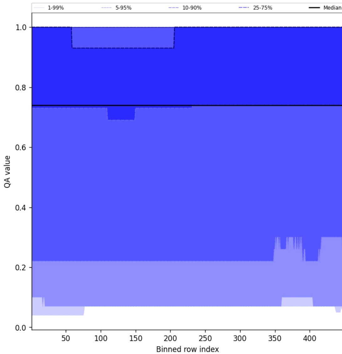
Figure 43: Along track statistics of “QA value” for 2025-10-15 to 2025-10-15
