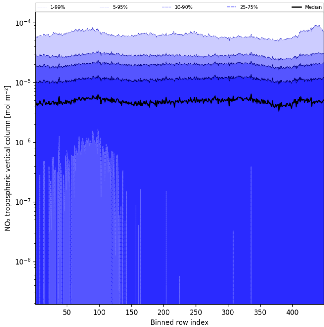
Figure 44: Along track statistics of “NO 2 tropospheric vertical column” for 2025-10-15 to 2025-10-15
