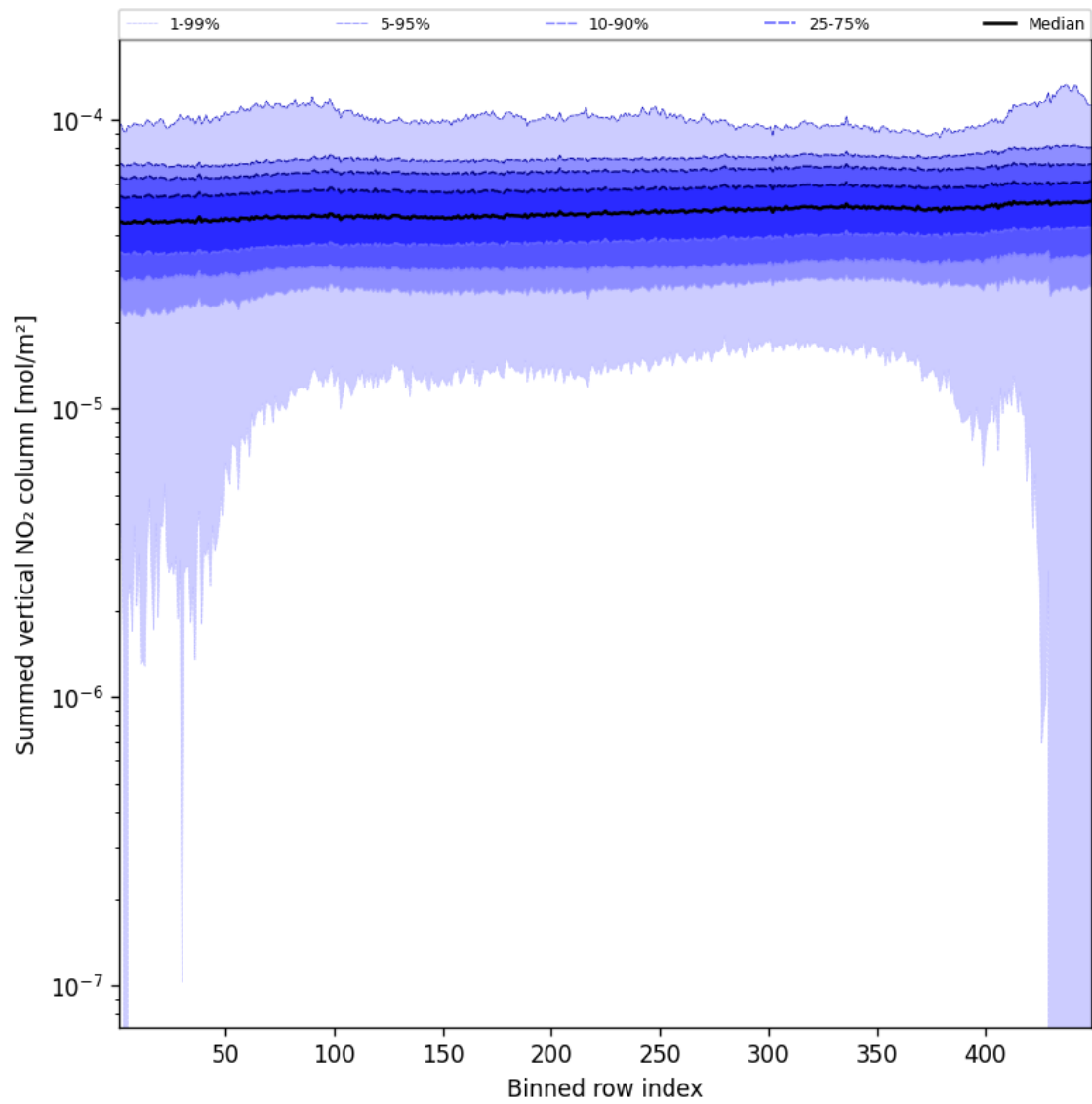
Figure 55: Along track statistics of “Summed vertical NO 2 column” for 2025-10-15 to 2025-10-15
