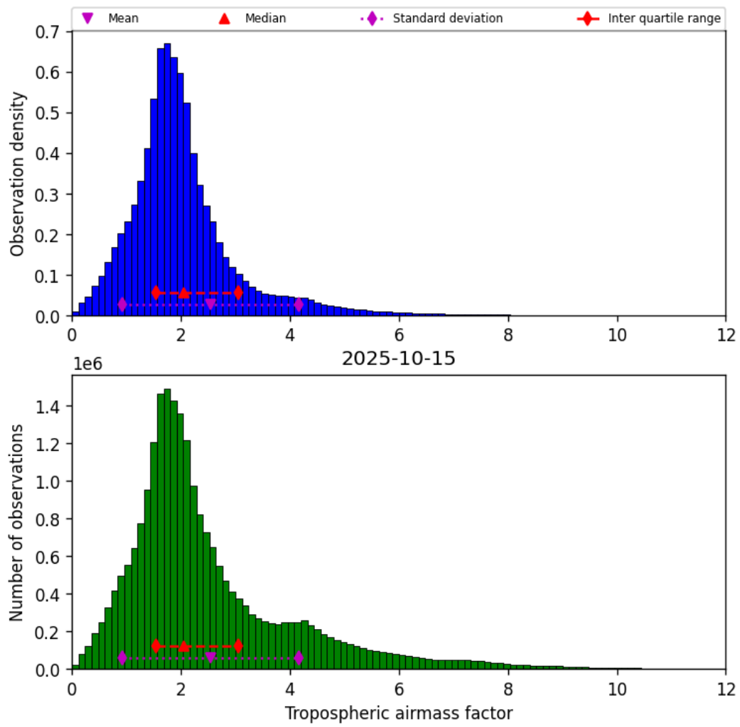
Figure 29: Histogram of “Tropospheric airmass factor” for 2025-10-15 to 2025-10-15
