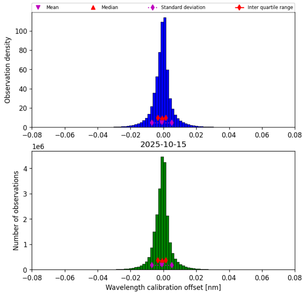
Figure 33: Histogram of “Wavelength calibration offset” for 2025-10-15 to 2025-10-15
