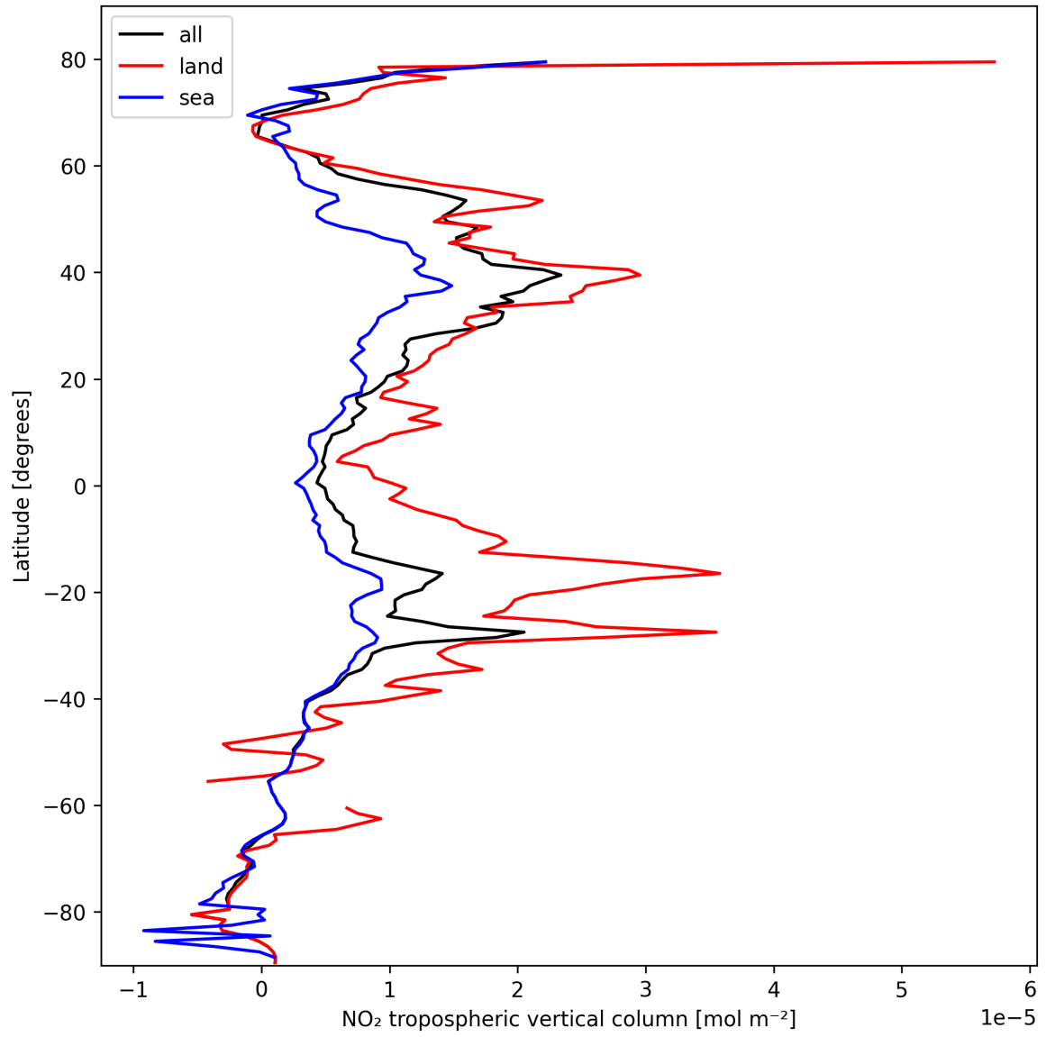
Figure 10: Zonal average of “NO 2 tropospheric vertical column” for 2025-10-16 to 2025-10-17.
