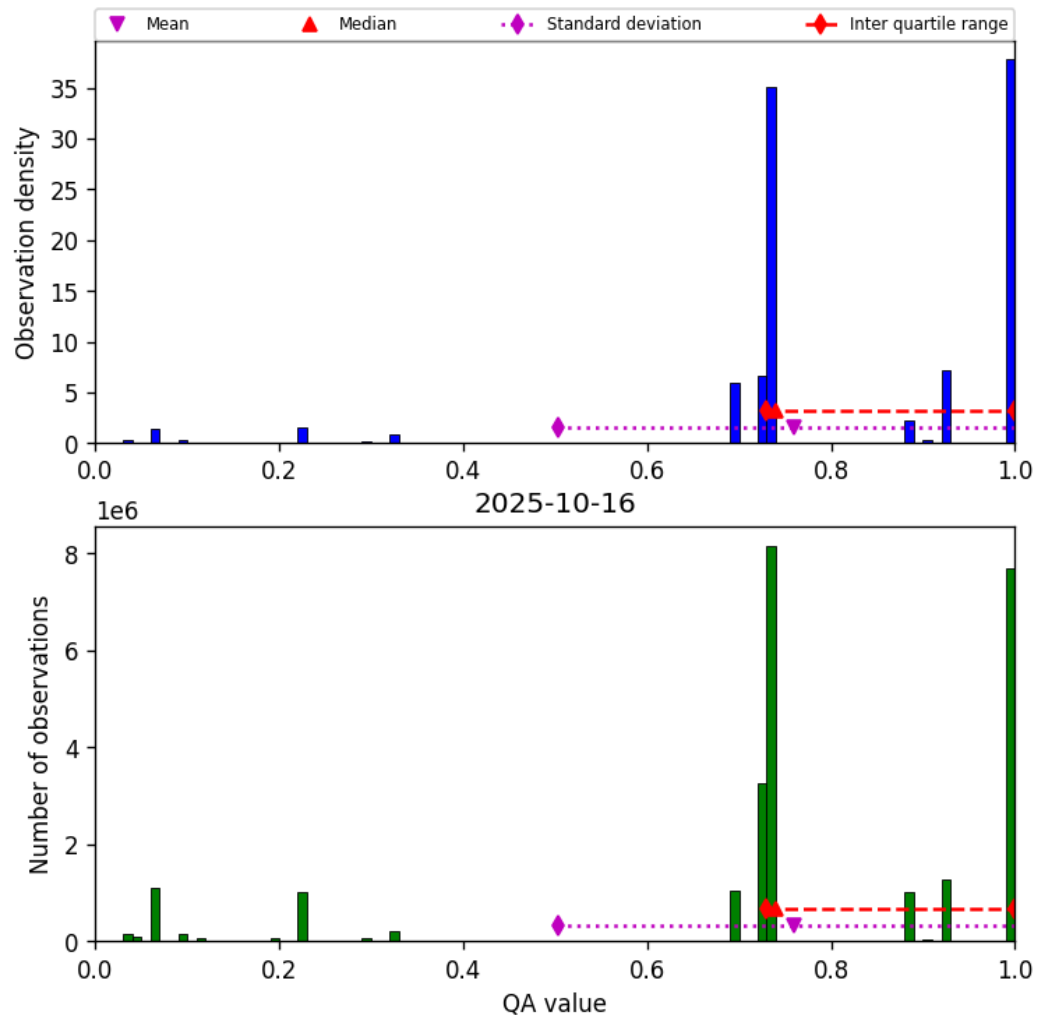
Figure 26: Histogram of “QA value” for 2025-10-16 to 2025-10-17
