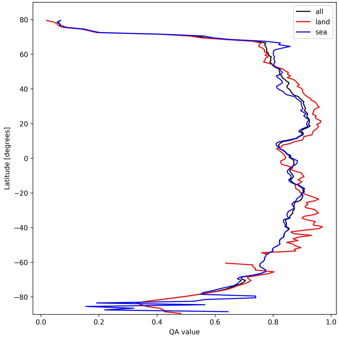
Figure 9: Zonal average of “QA value” for 2025-10-16 to 2025-10-17.
