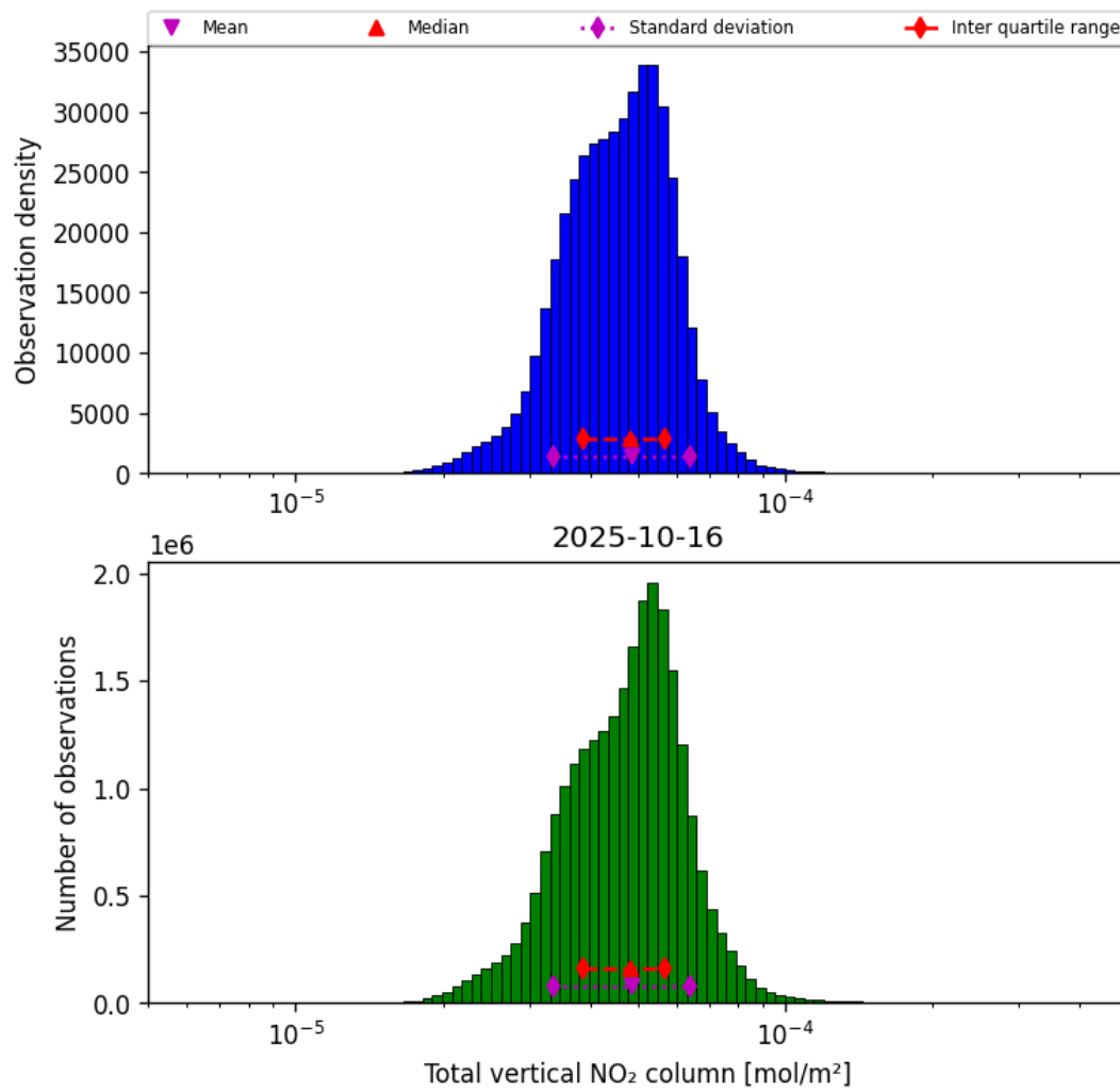
Figure 36: Histogram of “Total vertical NO 2 column” for 2025-10-16 to 2025-10-17
