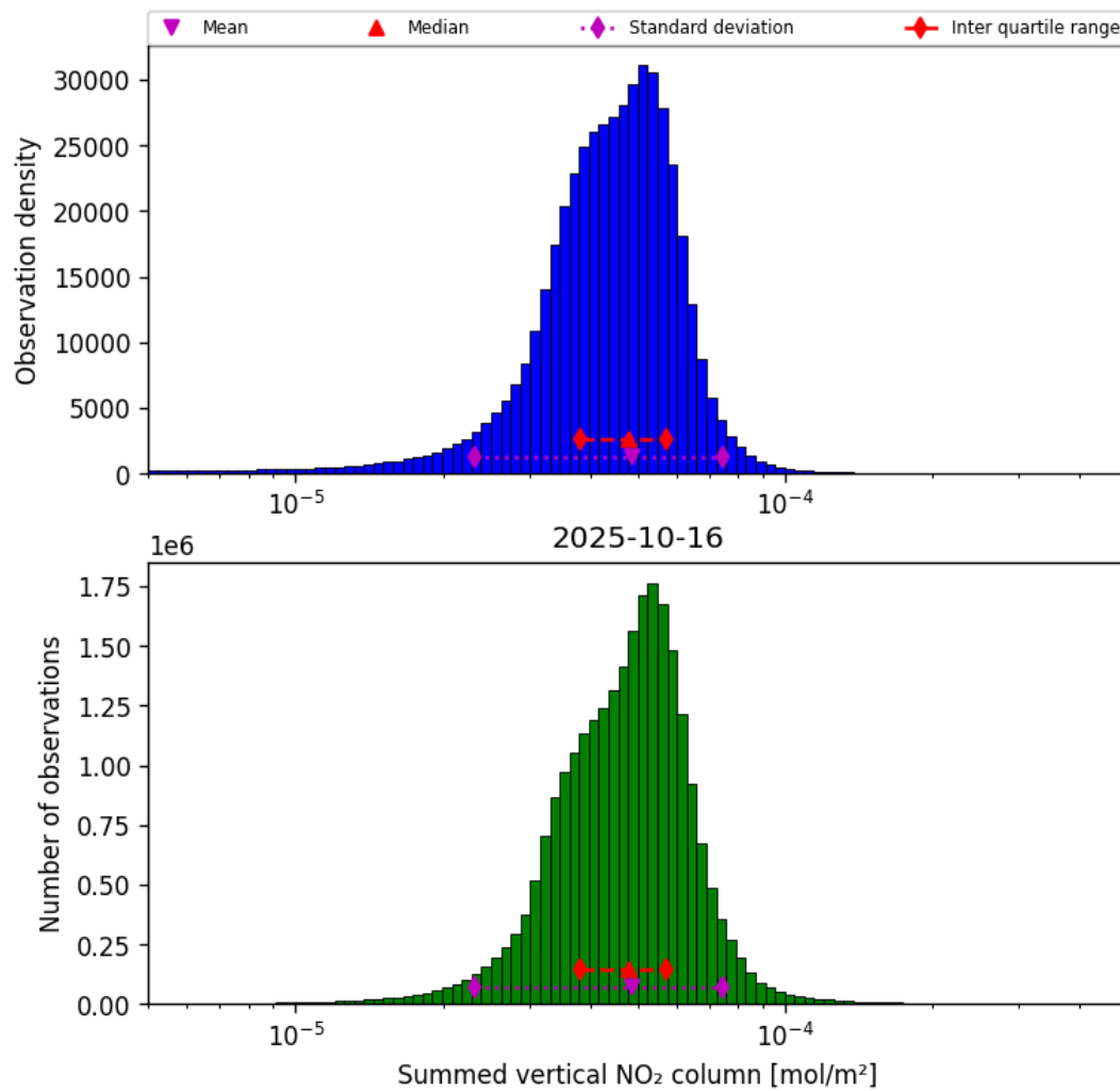
Figure 38: Histogram of “Summed vertical NO 2 column” for 2025-10-16 to 2025-10-17
