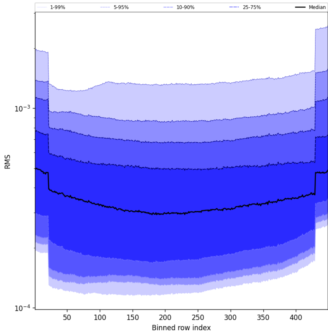
Figure 58: Along track statistics of “RMS” for 2025-10-16 to 2025-10-17
