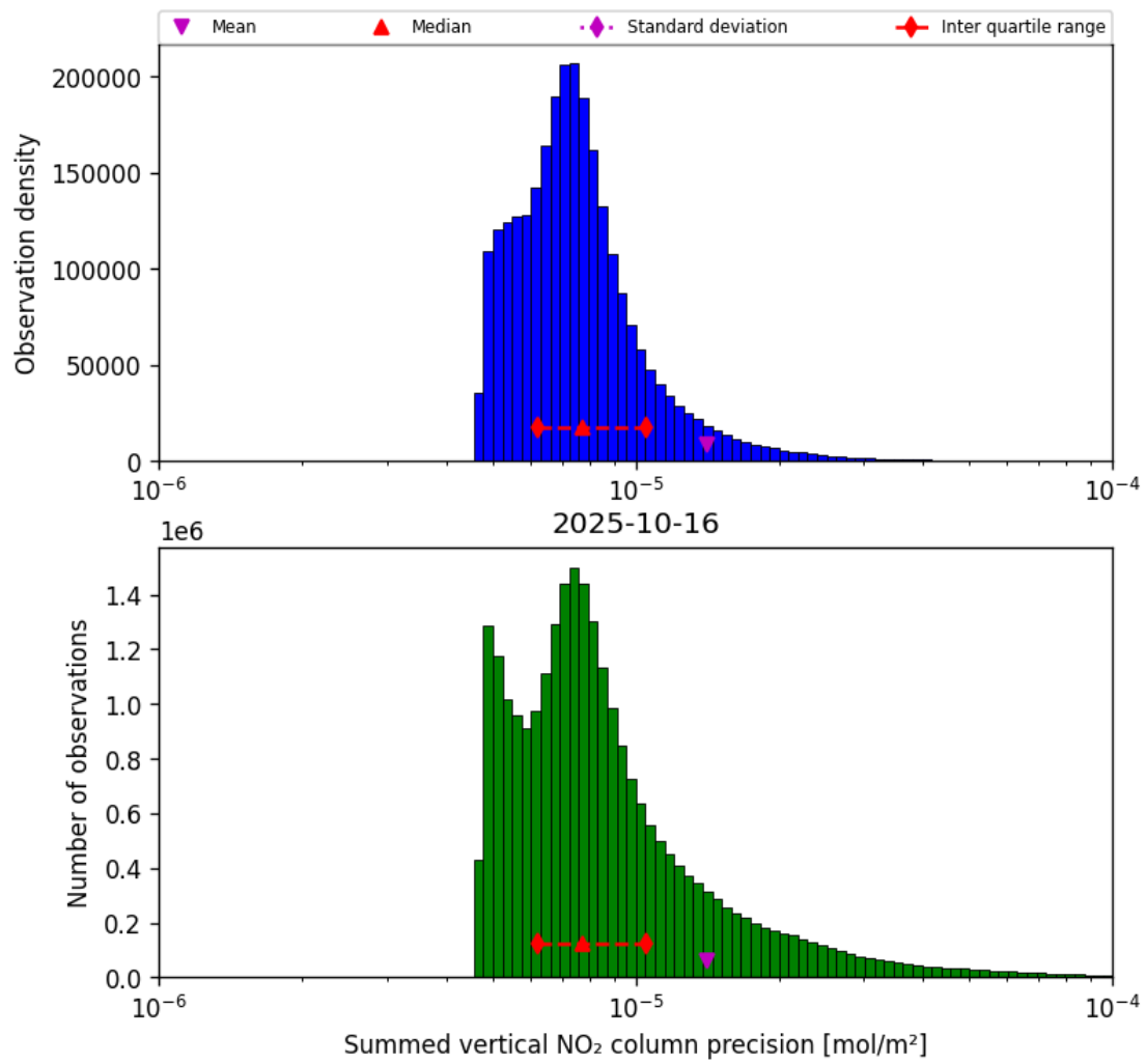
Figure 39: Histogram of “Summed vertical NO 2 column precision” for 2025-10-16 to 2025-10-17
