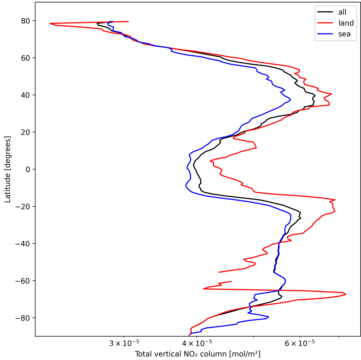
Figure 19: Zonal average of “Total vertical NO 2 column” for 2025-10-16 to 2025-10-17.
