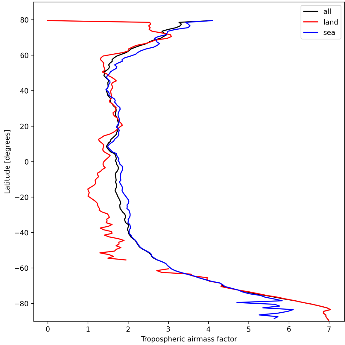
Figure 12: Zonal average of “Tropospheric airmass factor” for 2025-10-16 to 2025-10-17.
