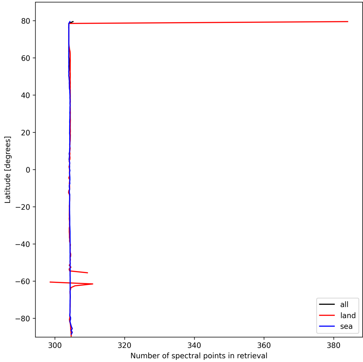
Figure 14: Zonal average of “Number of spectral points in retrieval” for 2025-10-16 to 2025-10-17.
