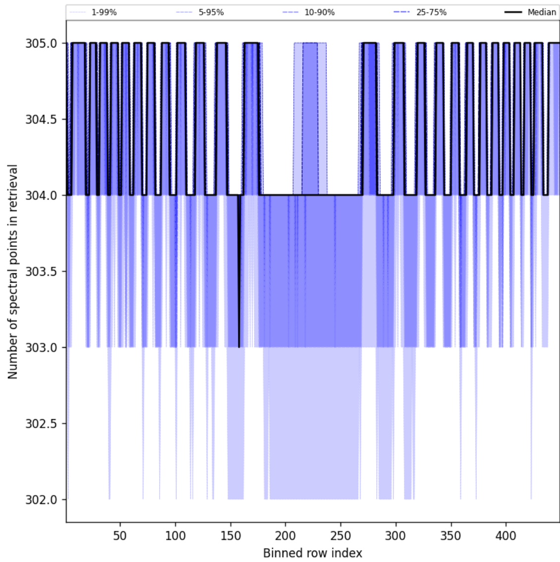
Figure 48: Along track statistics of “Number of spectral points in retrieval” for 2025-10-16 to 2025-10-17
