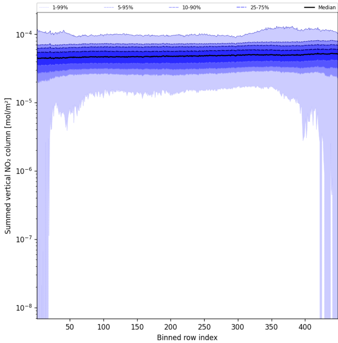
Figure 55: Along track statistics of “Summed vertical NO 2 column” for 2025-10-16 to 2025-10-17
