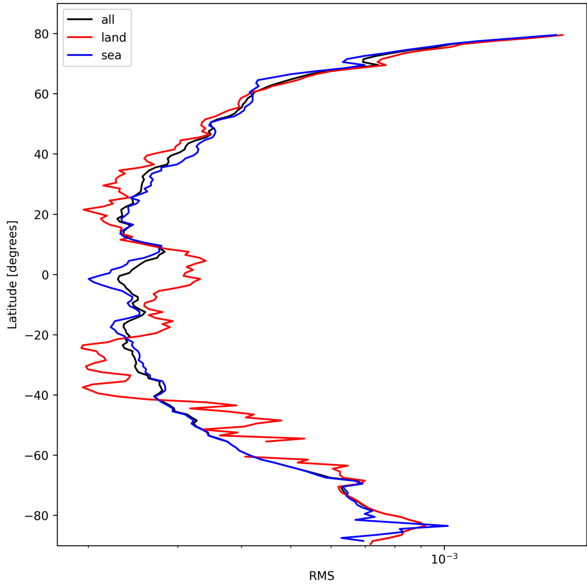
Figure 24: Zonal average of “RMS” for 2025-10-16 to 2025-10-17.
