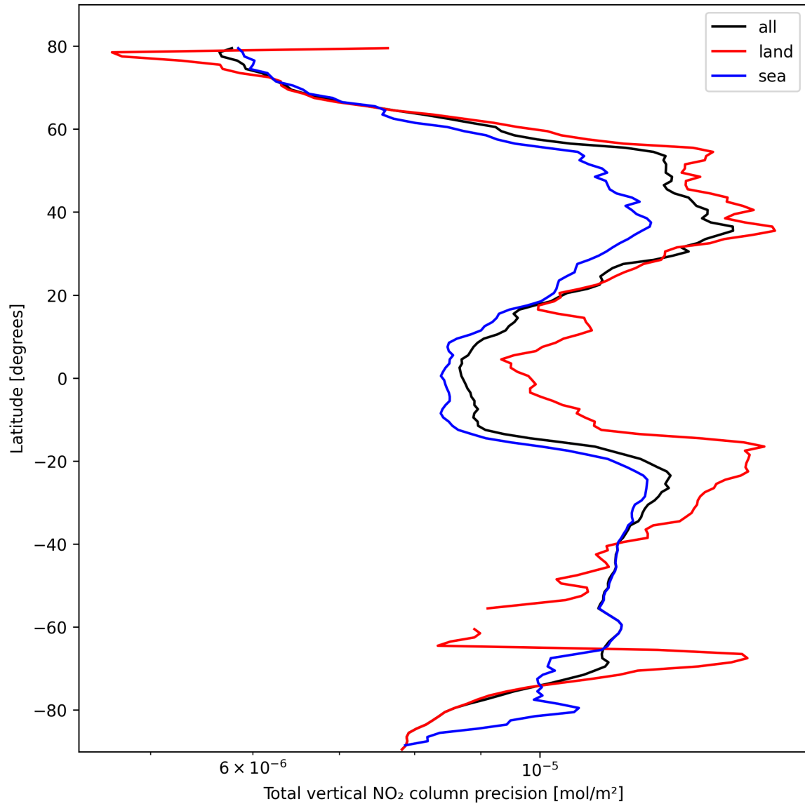
Figure 20: Zonal average of “Total vertical NO 2 column precision” for 2025-10-16 to 2025-10-17.
