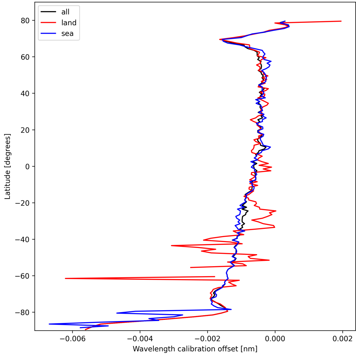
Figure 16: Zonal average of “Wavelength calibration offset” for 2025-10-16 to 2025-10-17.
