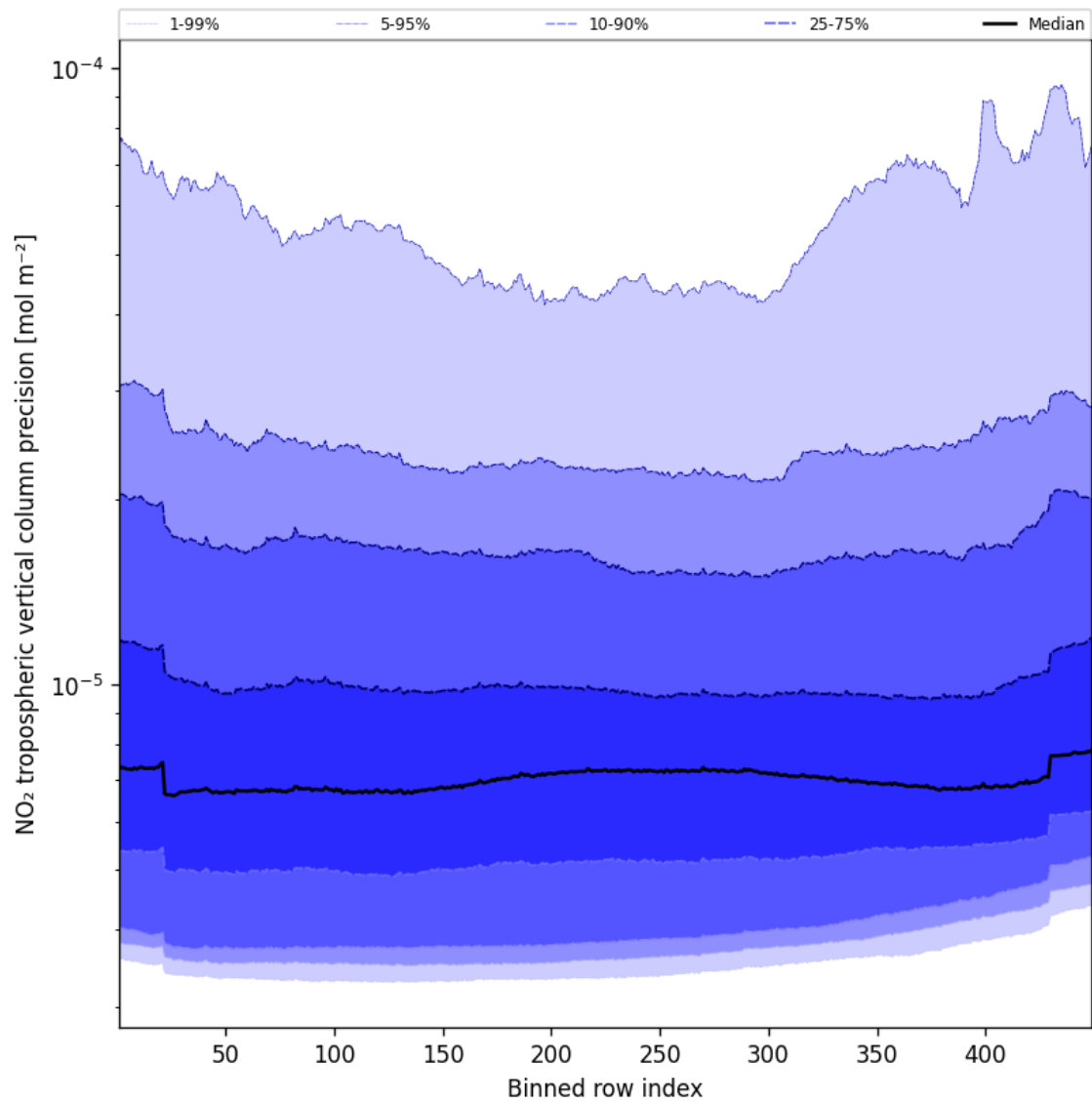
Figure 45: Along track statistics of “NO 2 tropospheric vertical column precision” for 2025-10-16 to 2025-10-17
