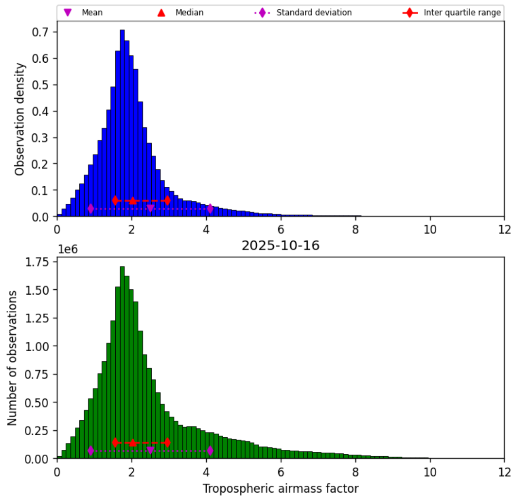
Figure 29: Histogram of “Tropospheric airmass factor” for 2025-10-16 to 2025-10-17
