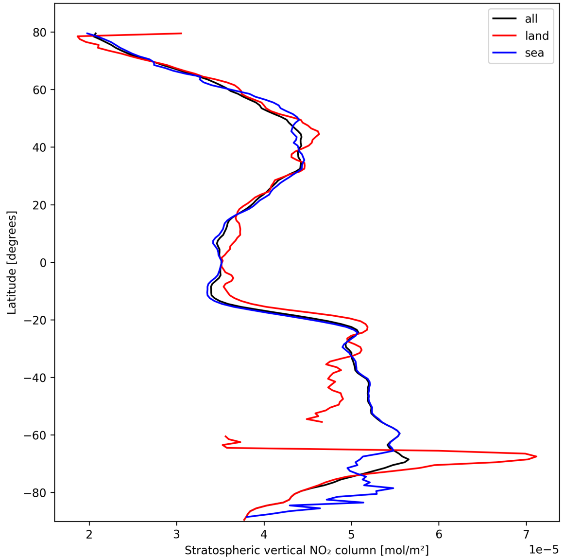
Figure 17: Zonal average of “Stratospheric vertical NO 2 column” for 2025-10-16 to 2025-10-17.
