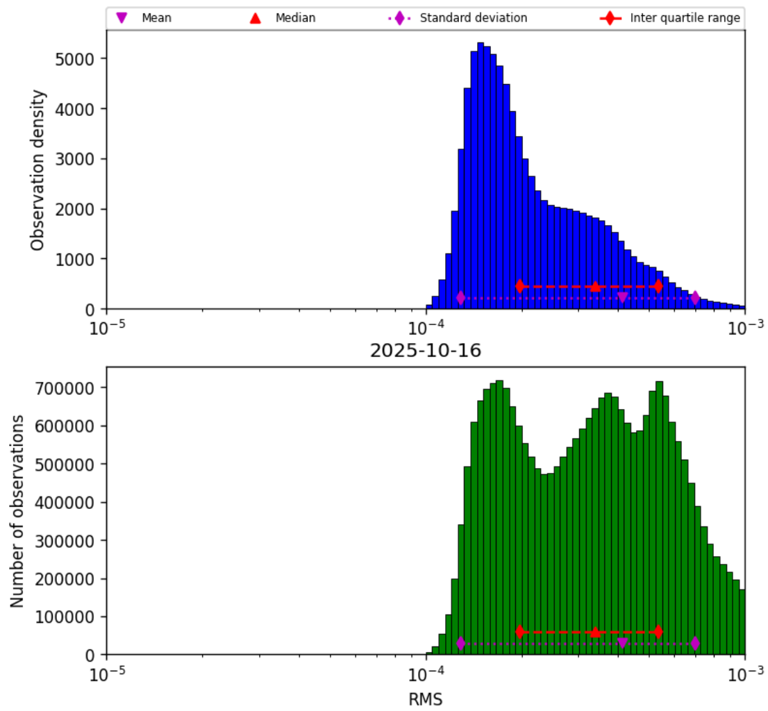
Figure 41: Histogram of “RMS” for 2025-10-16 to 2025-10-17
