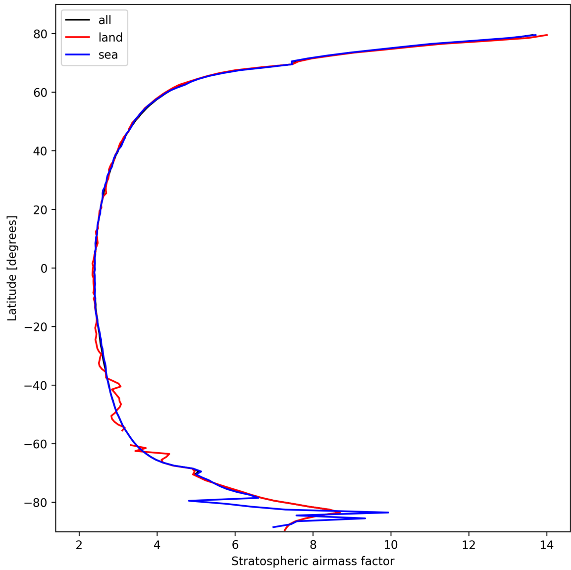
Figure 25: Zonal average of “Stratospheric air mass factor” for 2025-10-16 to 2025-10-17.
