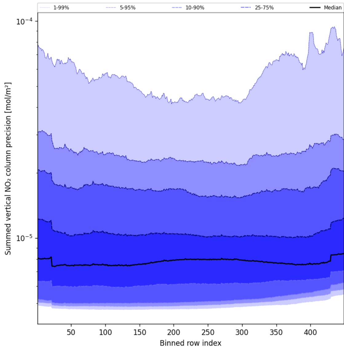
Figure 56: Along track statistics of “Summed vertical NO 2 column precision” for 2025-10-16 to 2025-10-17
