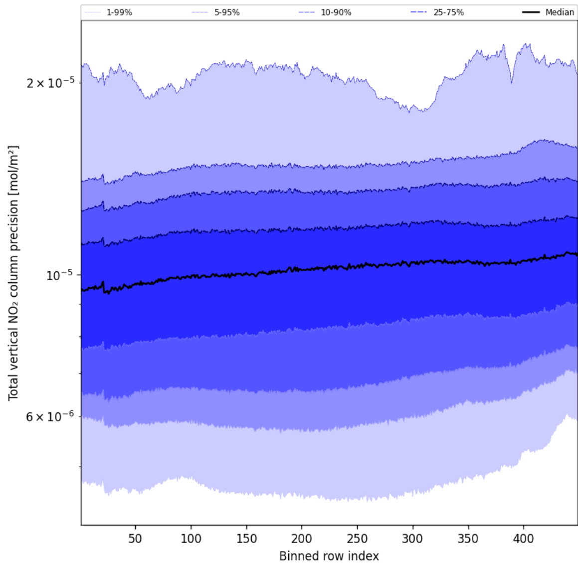
Figure 54: Along track statistics of “Total vertical NO 2 column precision” for 2025-10-16 to 2025-10-17
