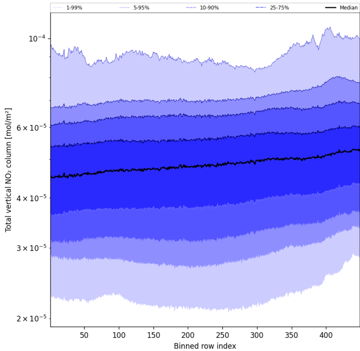
Figure 53: Along track statistics of “Total vertical NO 2 column” for 2025-10-16 to 2025-10-17
