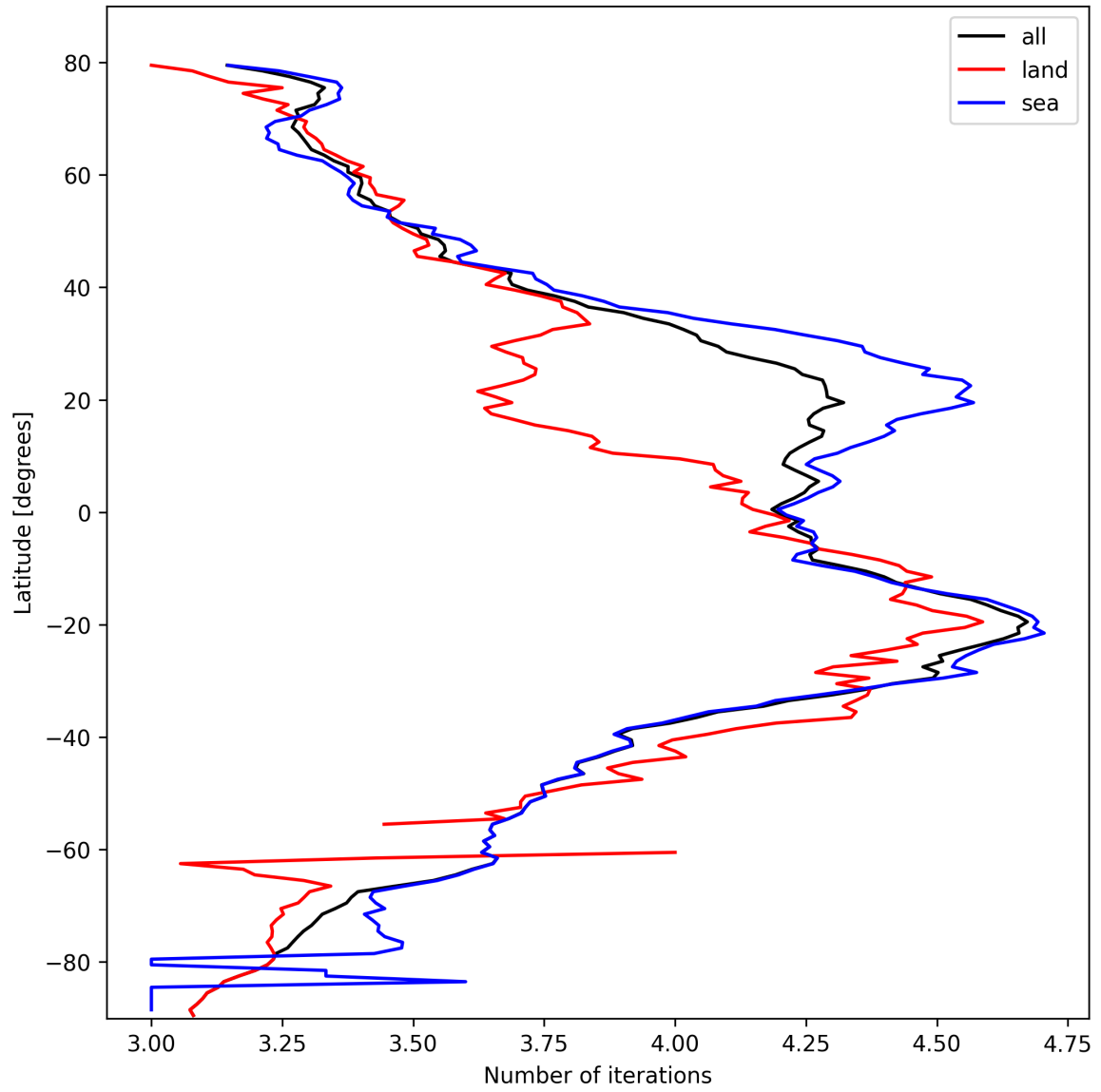
Figure 15: Zonal average of “Number of iterations” for 2025-10-16 to 2025-10-17.
