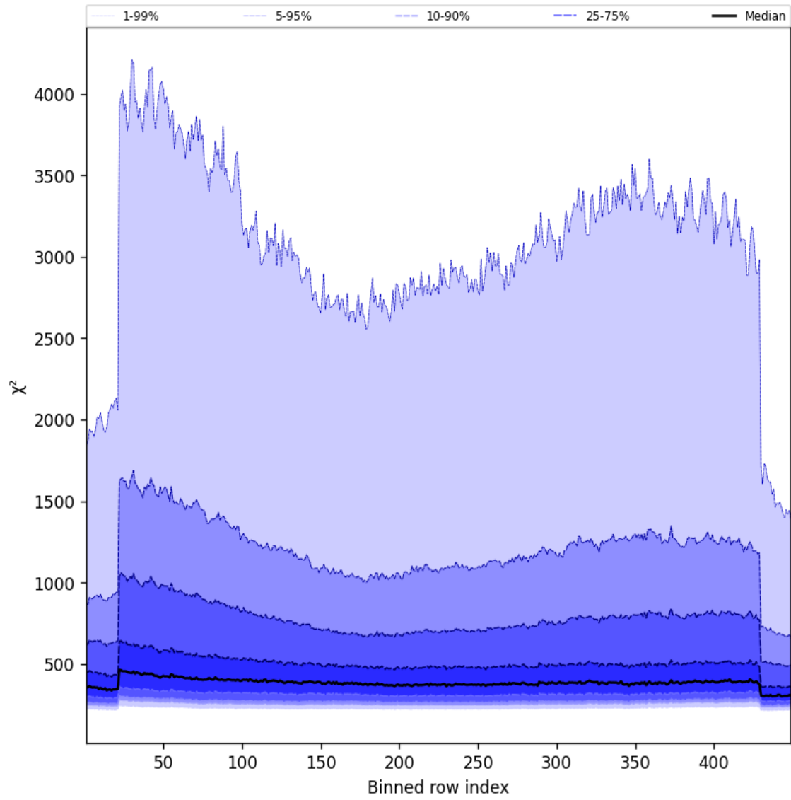
Figure 57: Along track statistics of “ \chi^2 ” for 2025-10-16 to 2025-10-17
