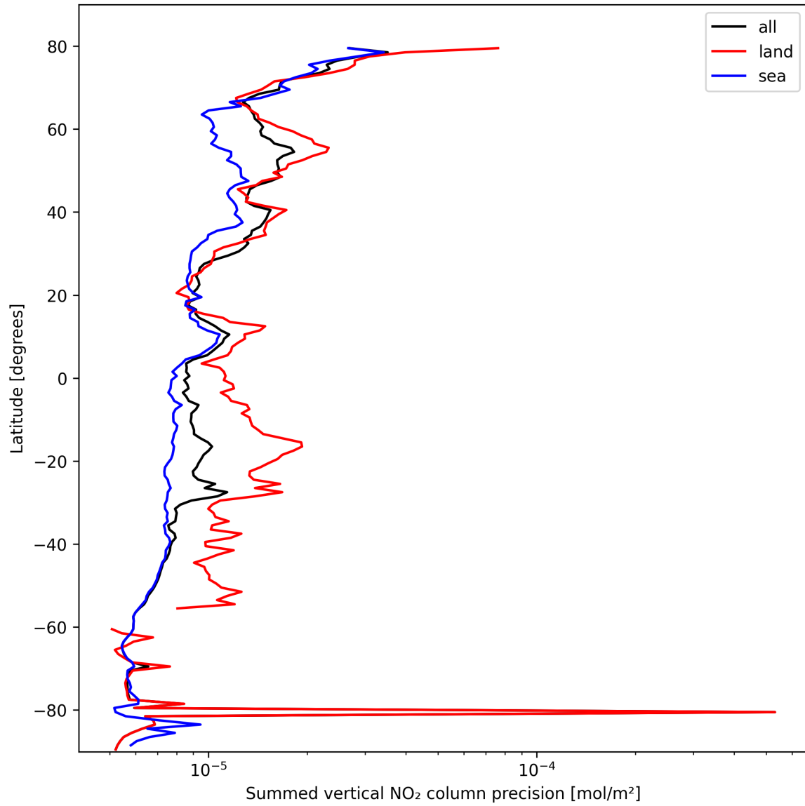
Figure 22: Zonal average of “Summed vertical NO 2 column precision” for 2025-10-16 to 2025-10-17.
