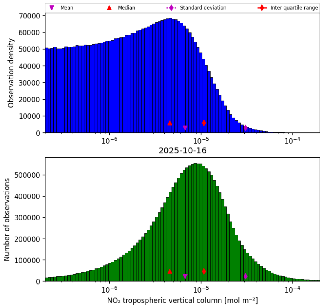
Figure 27: Histogram of “NO 2 tropospheric vertical column” for 2025-10-16 to 2025-10-17
