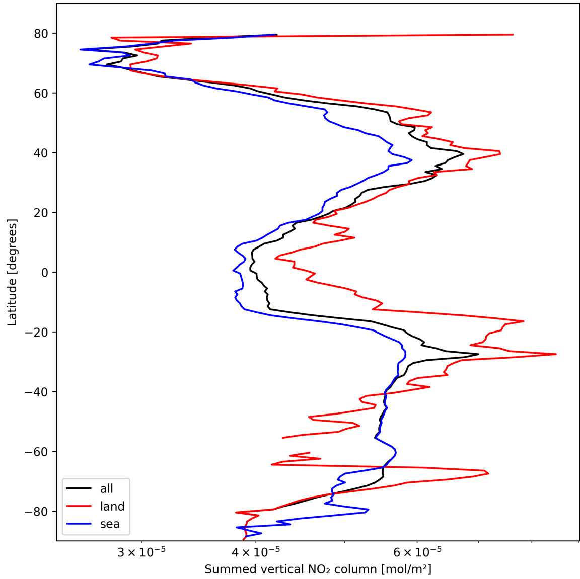
Figure 21: Zonal average of “Summed vertical NO 2 column” for 2025-10-16 to 2025-10-17.
