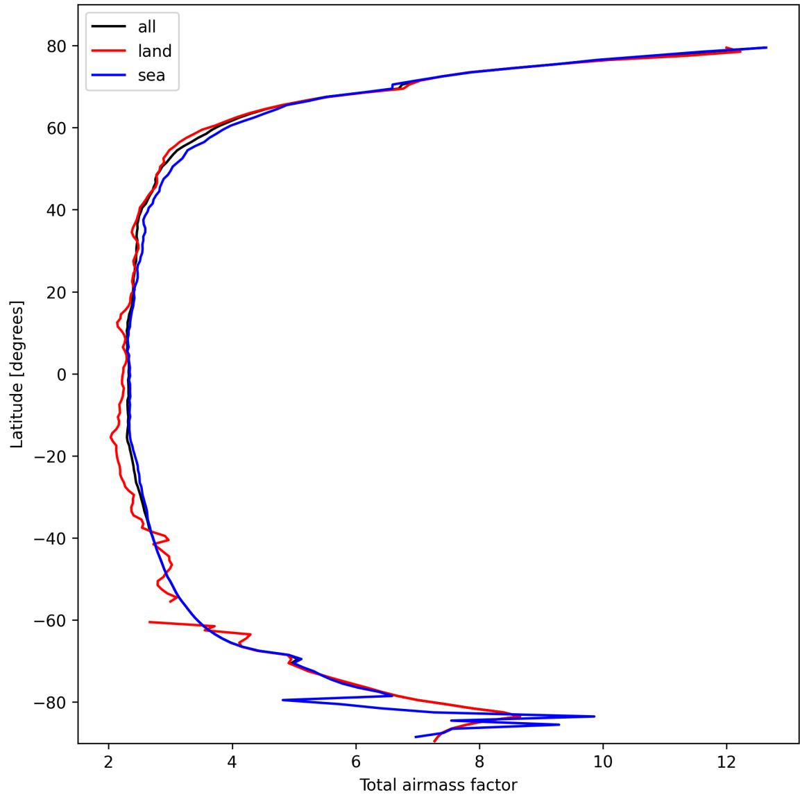
Figure 13: Zonal average of “Total airmass factor” for 2025-10-16 to 2025-10-17.
