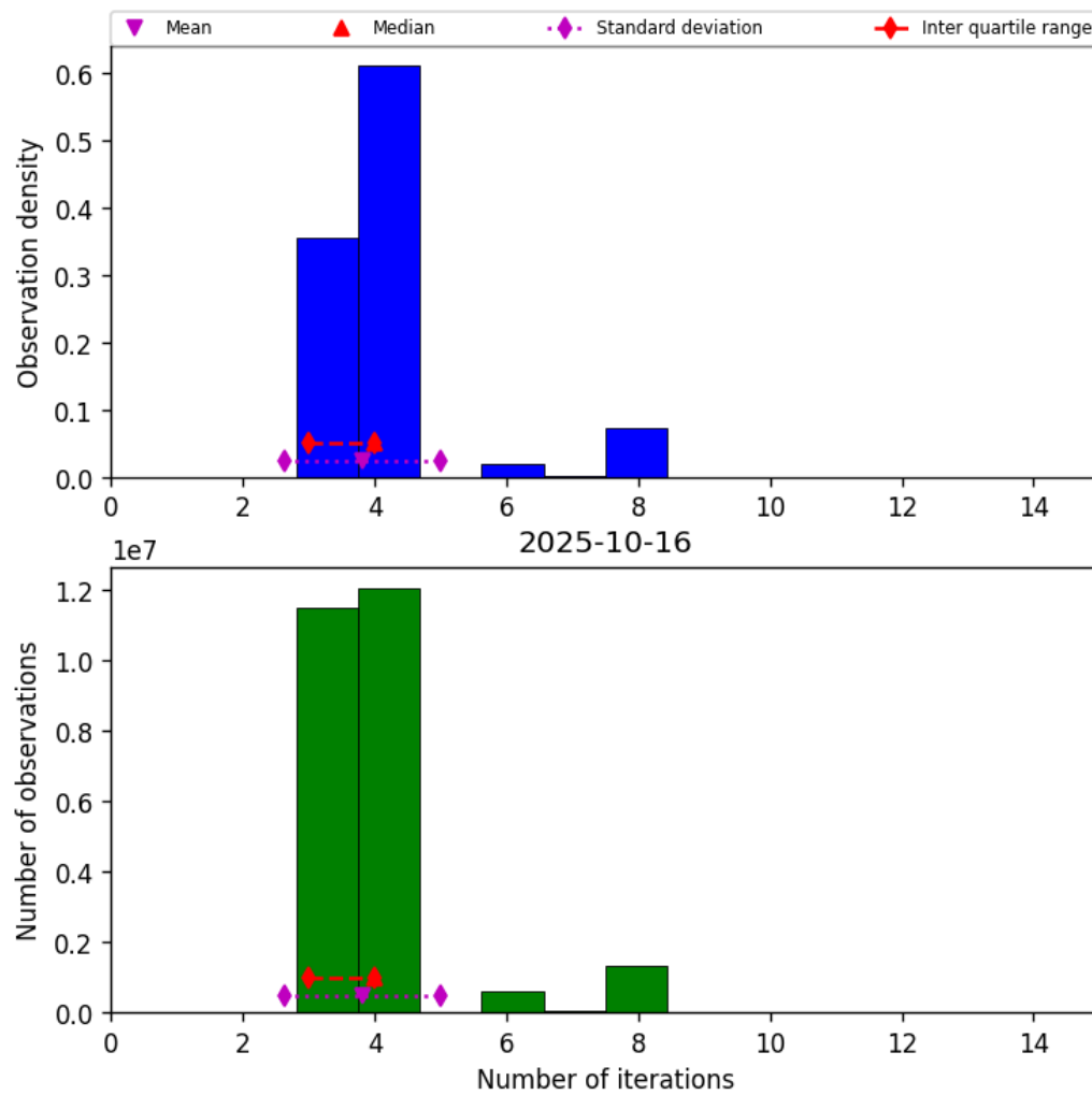
Figure 32: Histogram of “Number of iterations” for 2025-10-16 to 2025-10-17
