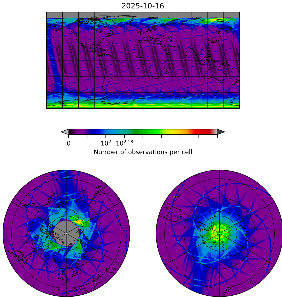
Figure 8: Map of the number of observations for 2025-10-16 to 2025-10-17
