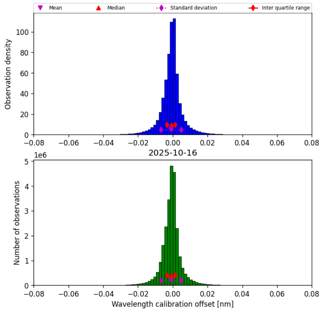
Figure 33: Histogram of “Wavelength calibration offset” for 2025-10-16 to 2025-10-17
