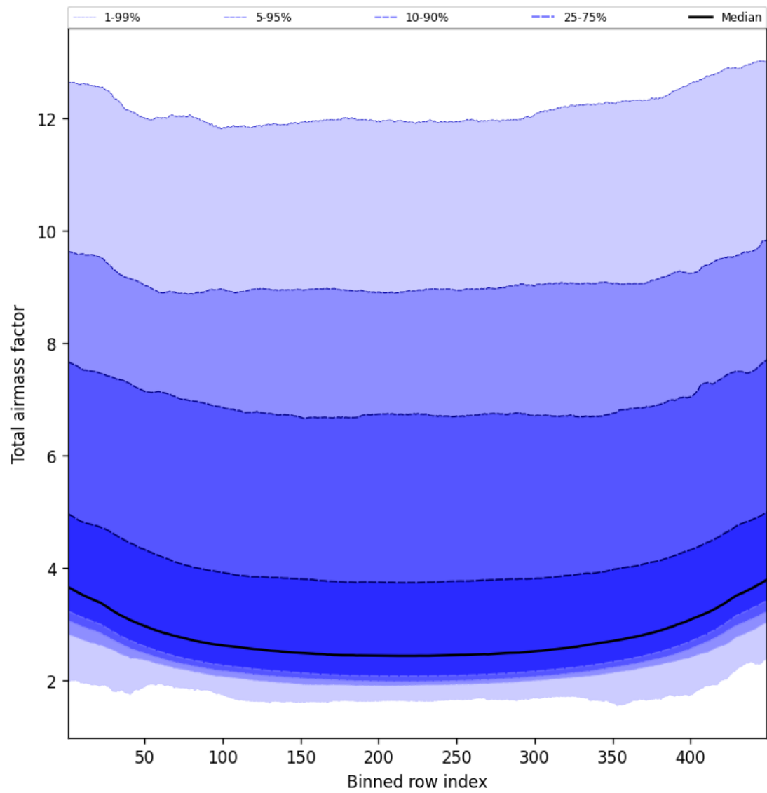
Figure 47: Along track statistics of “Total airmass factor” for 2025-10-16 to 2025-10-17
