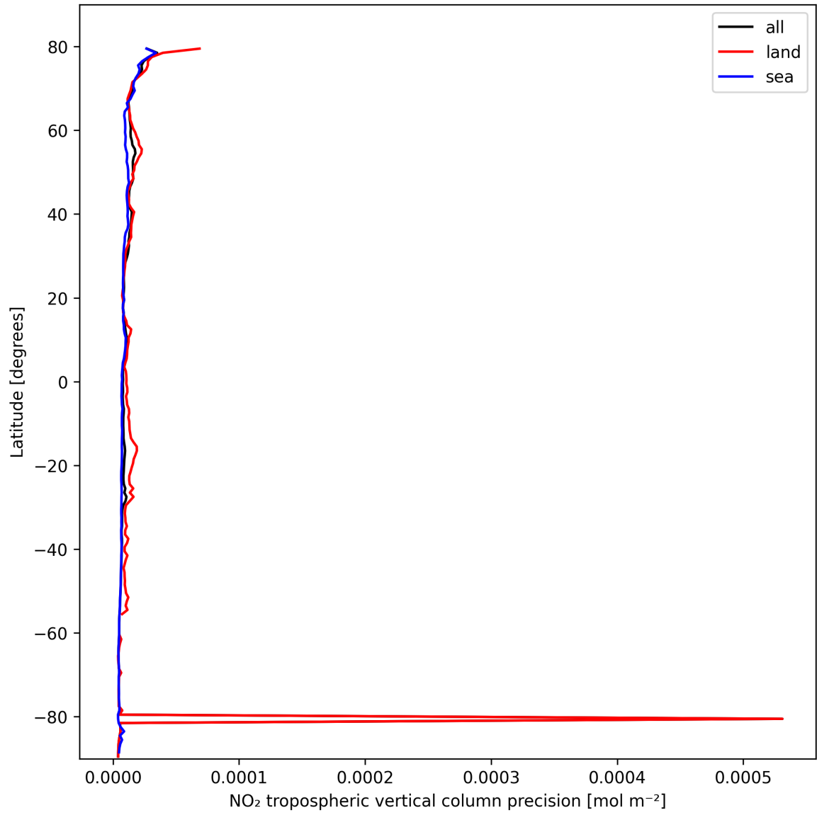
Figure 11: Zonal average of “NO 2 tropospheric vertical column precision” for 2025-10-16 to 2025-10-17.
