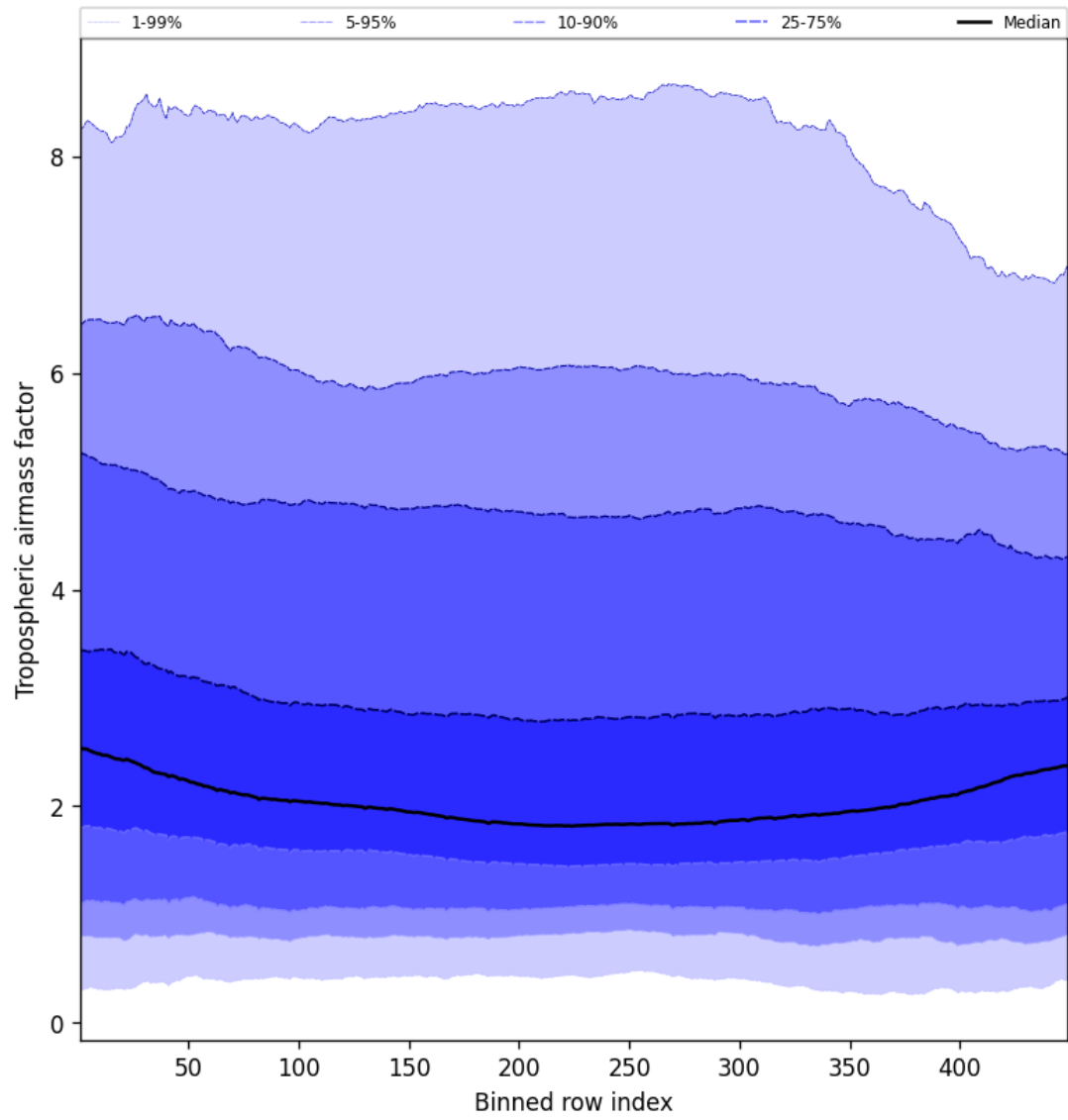
Figure 46: Along track statistics of “Tropospheric airmass factor” for 2025-10-16 to 2025-10-17
