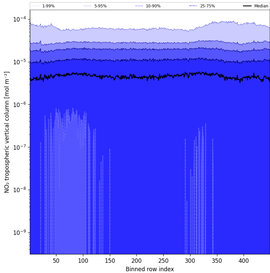
Figure 44: Along track statistics of “NO 2 tropospheric vertical column” for 2025-10-16 to 2025-10-17
