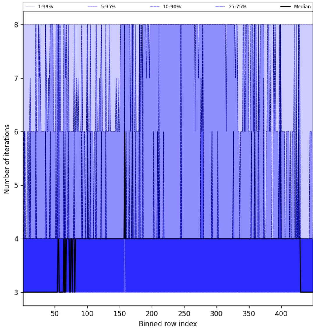
Figure 49: Along track statistics of “Number of iterations” for 2025-10-16 to 2025-10-17
