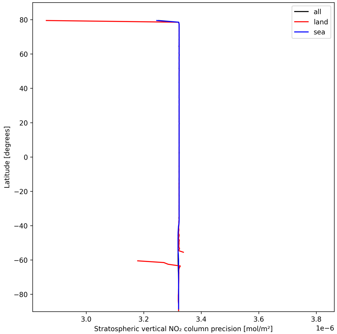
Figure 18: Zonal average of “Stratospheric vertical NO 2 column precision” for 2025-10-16 to 2025-10-17.
