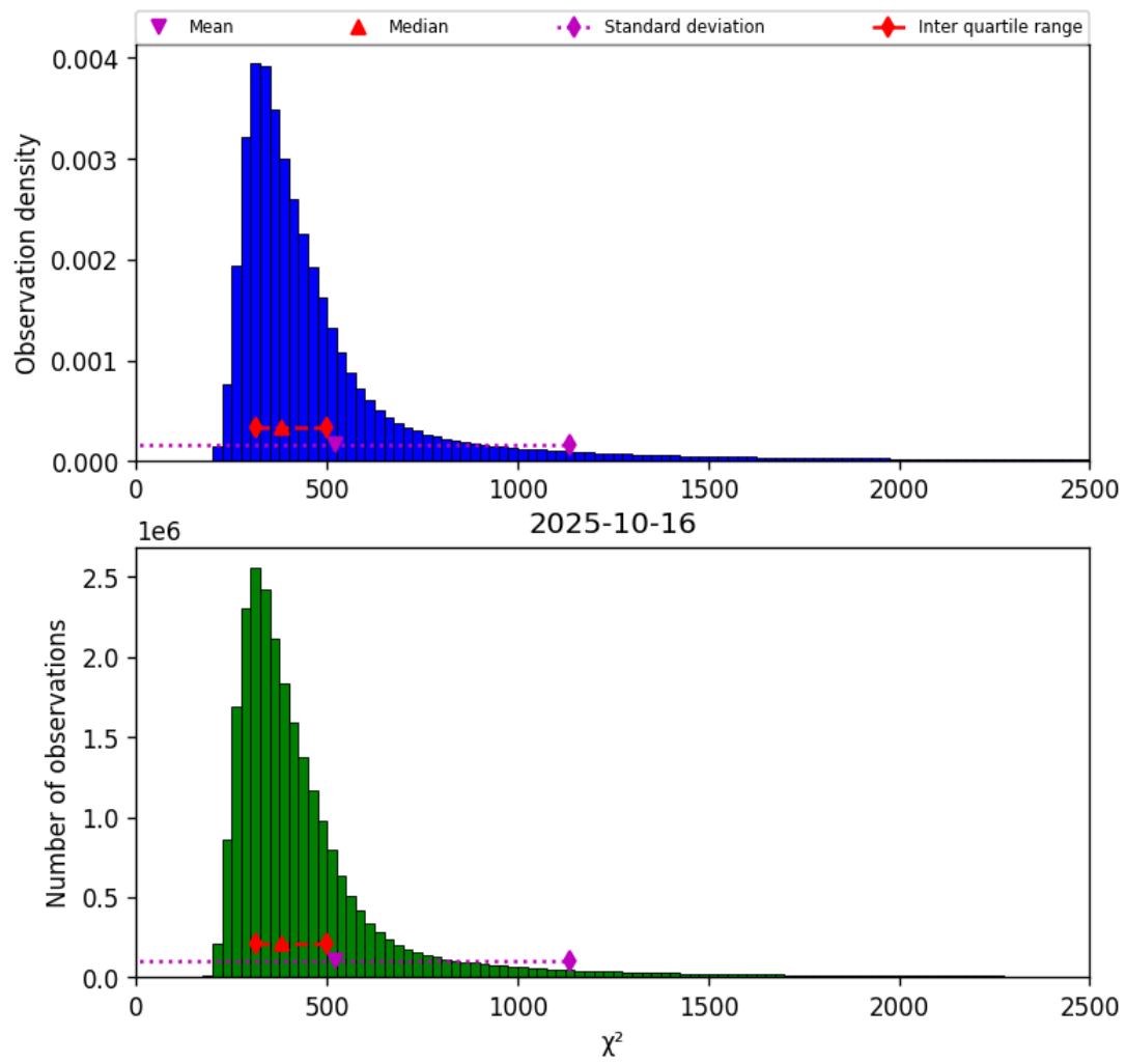
Figure 40: Histogram of “ \chi^2 ” for 2025-10-16 to 2025-10-17
