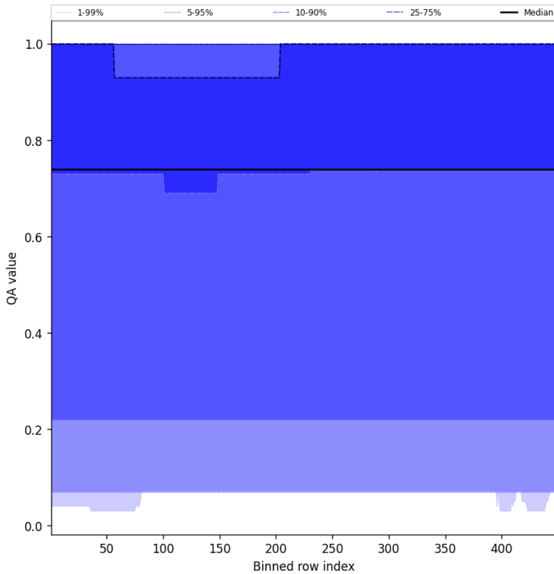
Figure 43: Along track statistics of “QA value” for 2025-10-16 to 2025-10-17
