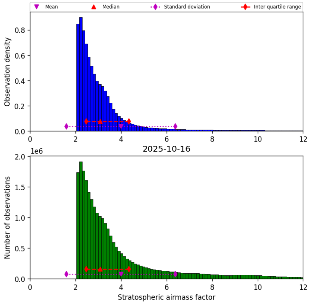
Figure 42: Histogram of “Stratospheric airmass factor” for 2025-10-16 to 2025-10-17
