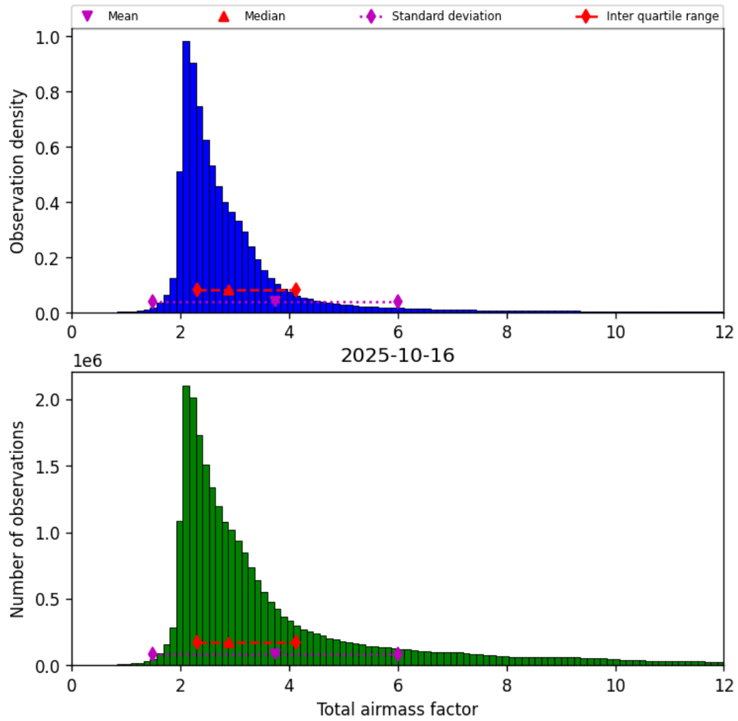
Figure 30: Histogram of “Total airmass factor” for 2025-10-16 to 2025-10-17
