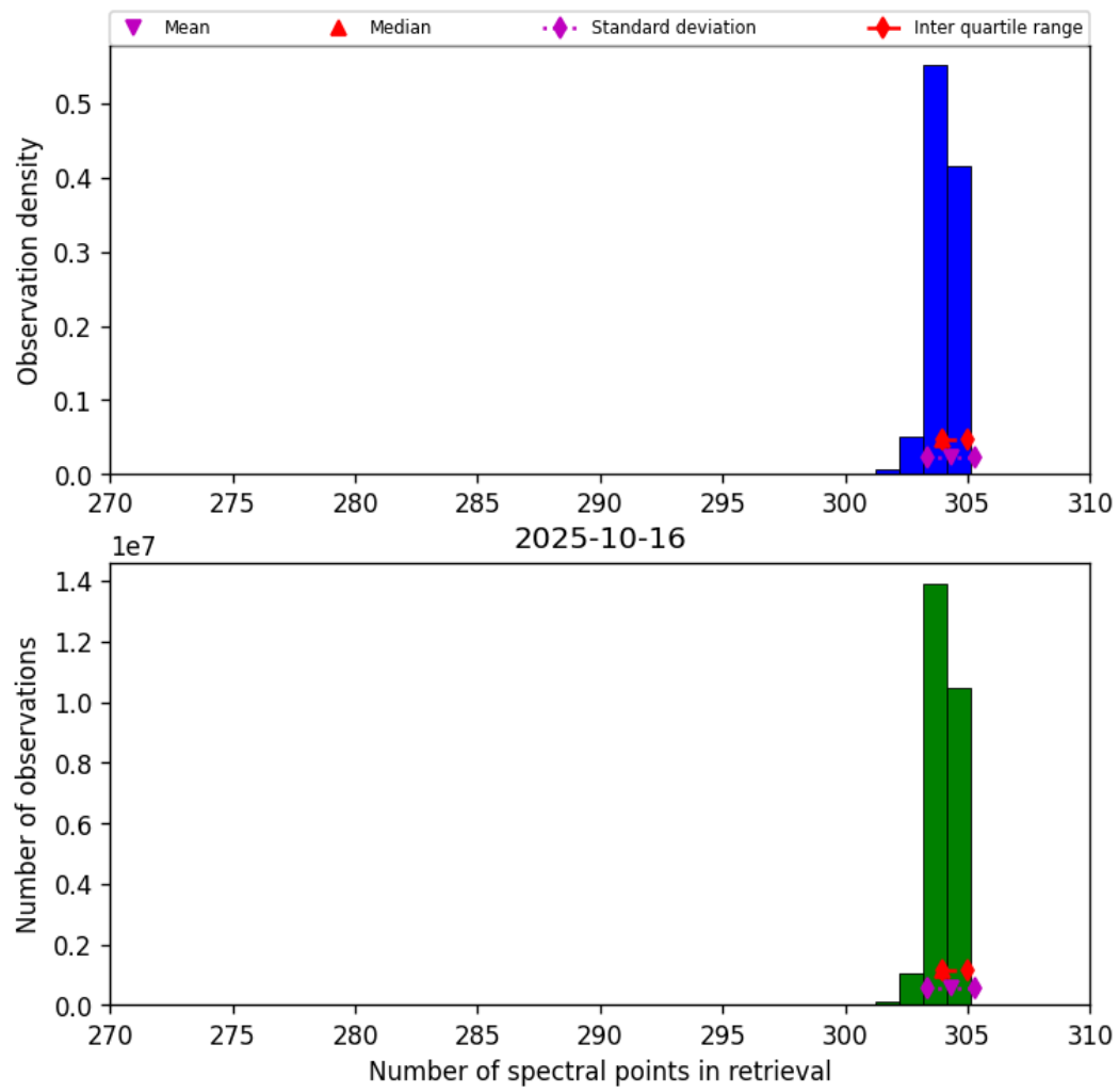
Figure 31: Histogram of “Number of spectral points in retrieval” for 2025-10-16 to 2025-10-17
