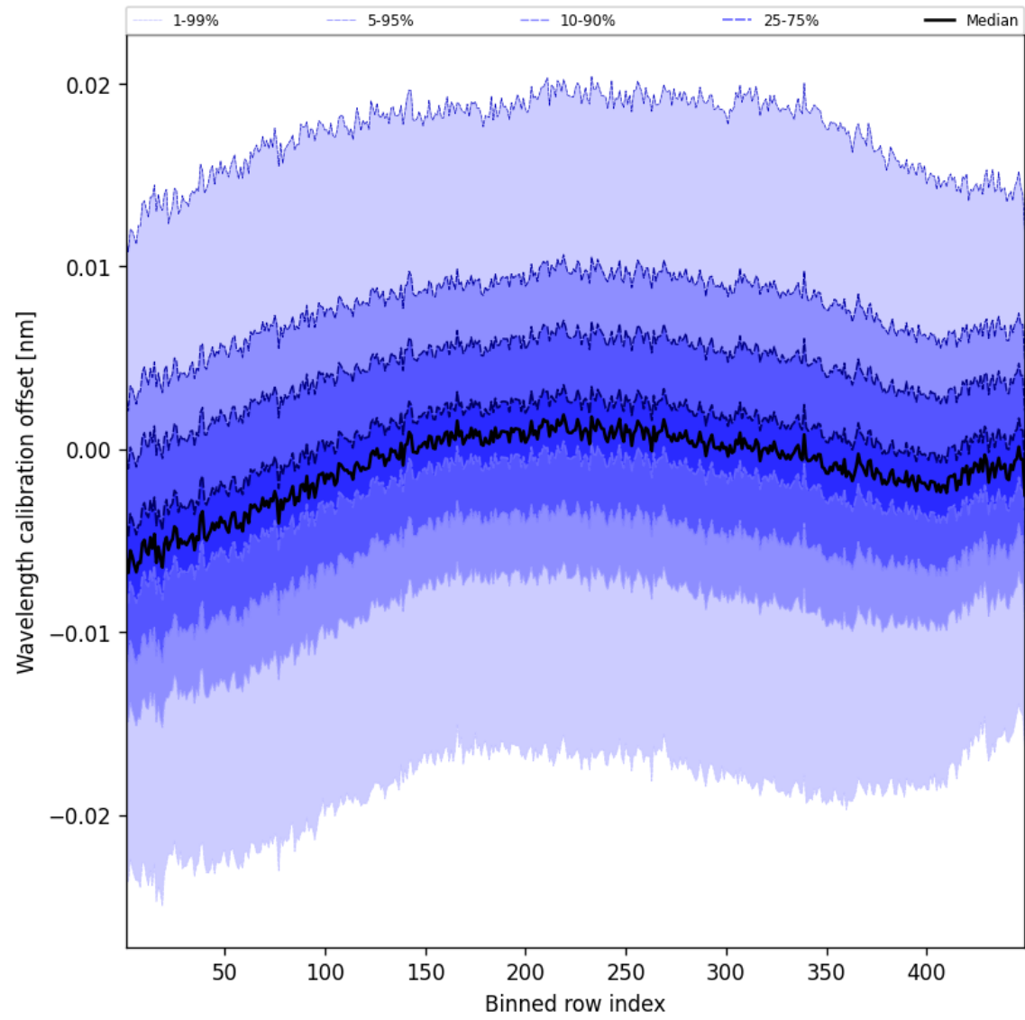
Figure 50: Along track statistics of “Wavelength calibration offset” for 2025-10-16 to 2025-10-17
