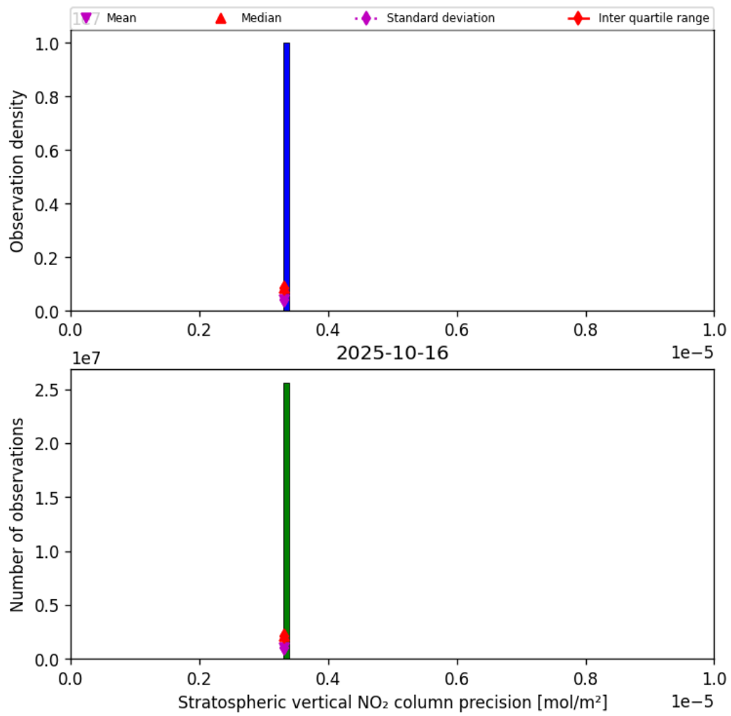
Figure 35: Histogram of “Stratospheric vertical NO 2 column precision” for 2025-10-16 to 2025-10-17
