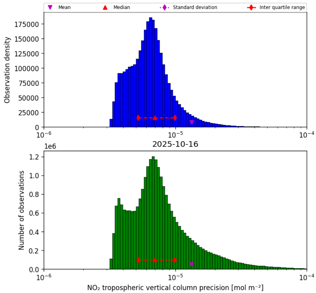
Figure 28: Histogram of “NO 2 tropospheric vertical column precision” for 2025-10-16 to 2025-10-17
