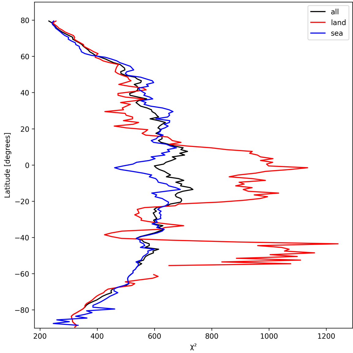
Figure 23: Zonal average of “ \chi^2 ” for 2025-10-16 to 2025-10-17.
