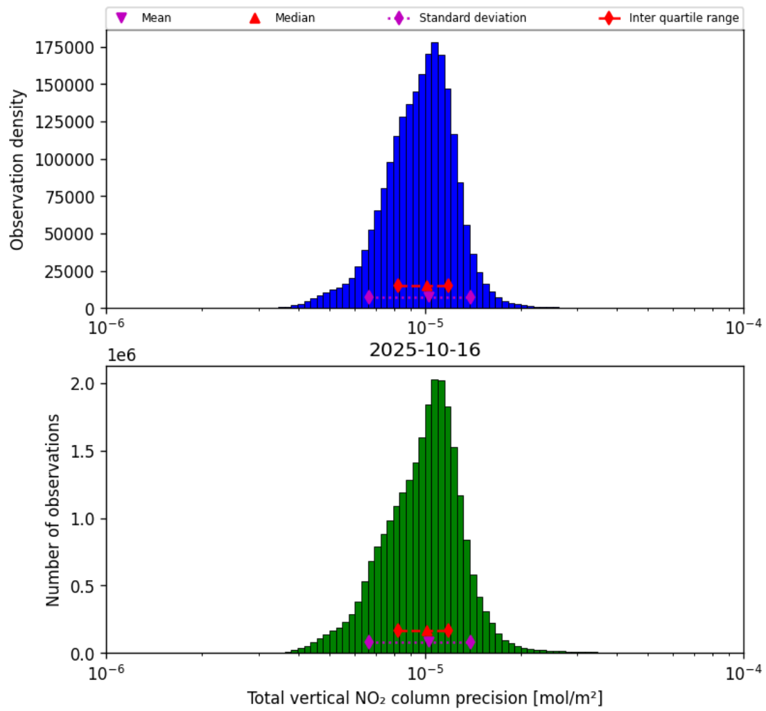
Figure 37: Histogram of "Total vertical NO 2 column precision" for 2025-10-16 to 2025-10-17
