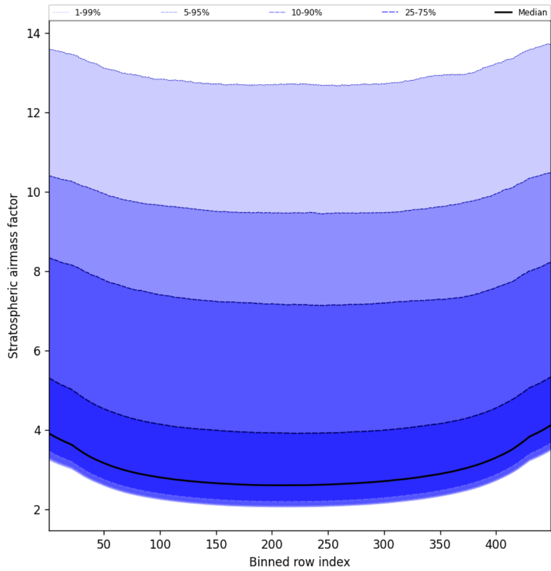
Figure 59: Along track statistics of “Stratospheric airmass factor” for 2025-10-16 to 2025-10-17
