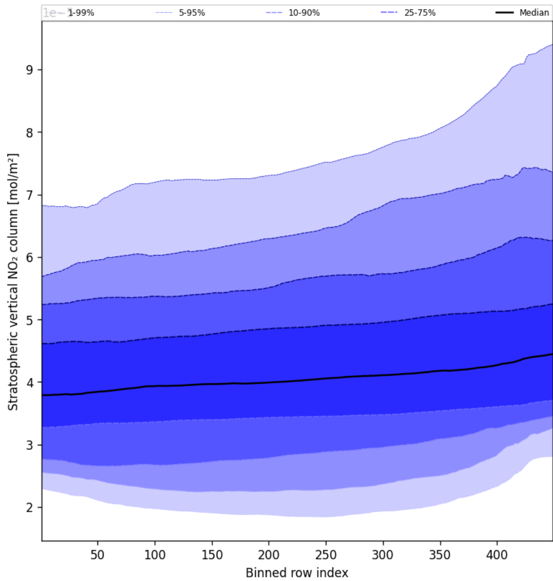
Figure 51: Along track statistics of “Stratospheric vertical NO 2 column” for 2025-10-16 to 2025-10-17
