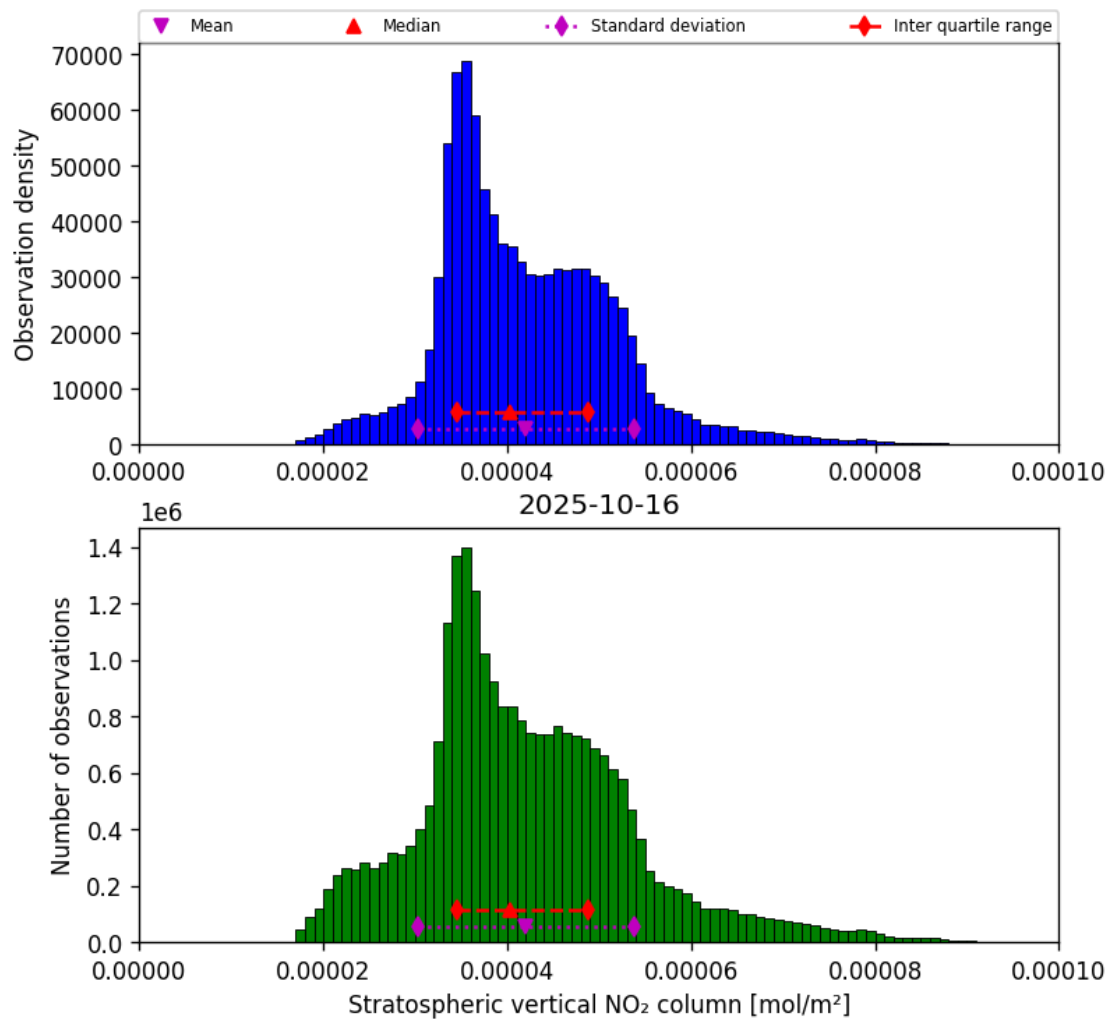
Figure 34: Histogram of “Stratospheric vertical NO 2 column” for 2025-10-16 to 2025-10-17
