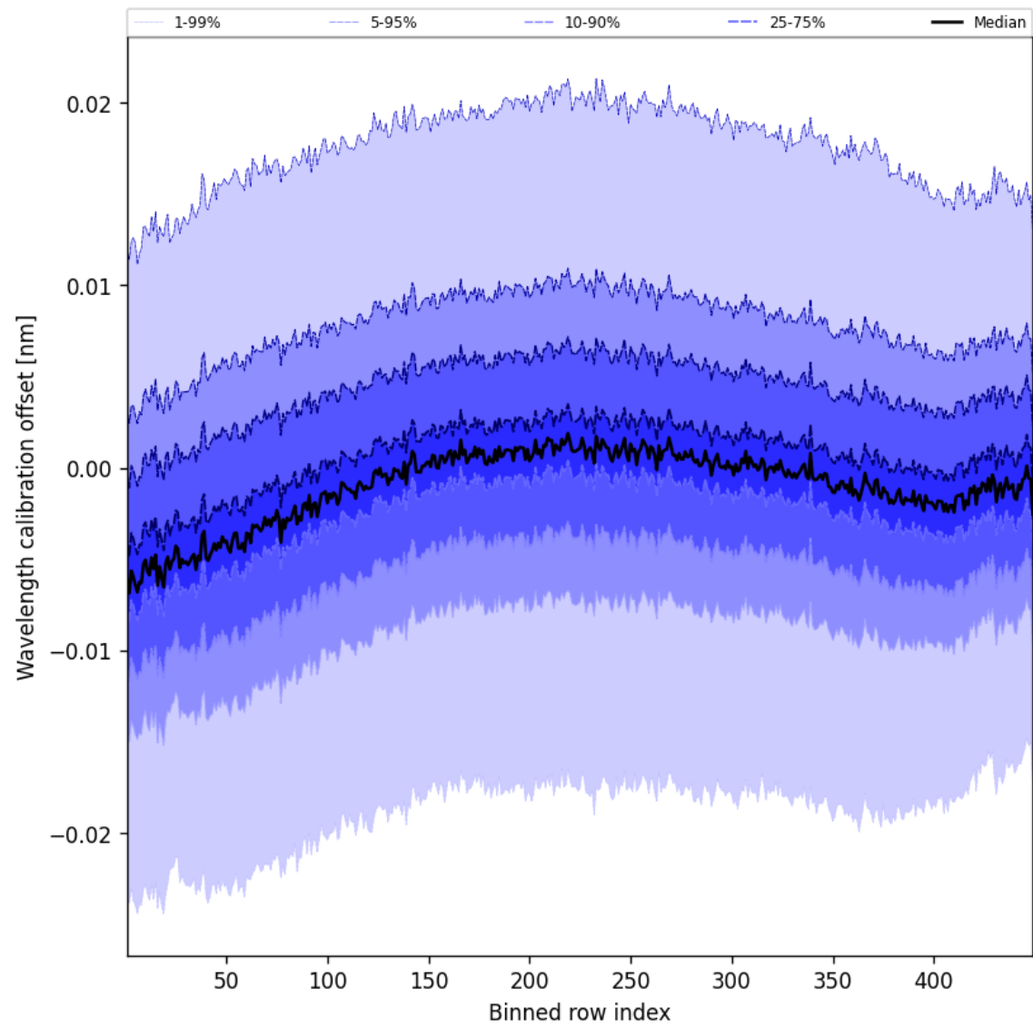
Figure 50: Along track statistics of “Wavelength calibration offset” for 2025-10-17 to 2025-10-18
