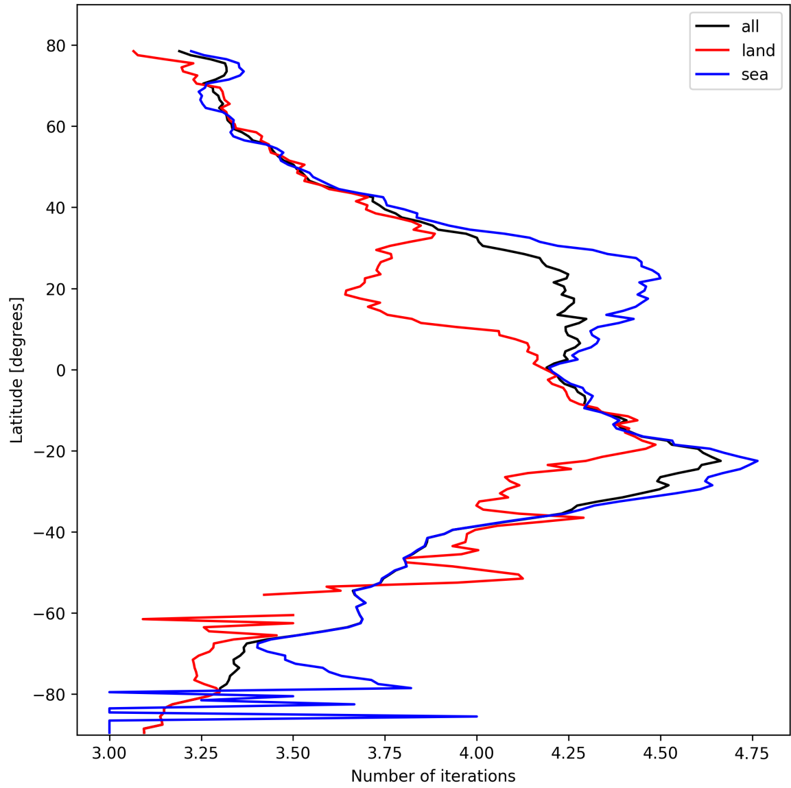
Figure 15: Zonal average of “Number of iterations” for 2025-10-17 to 2025-10-18.
