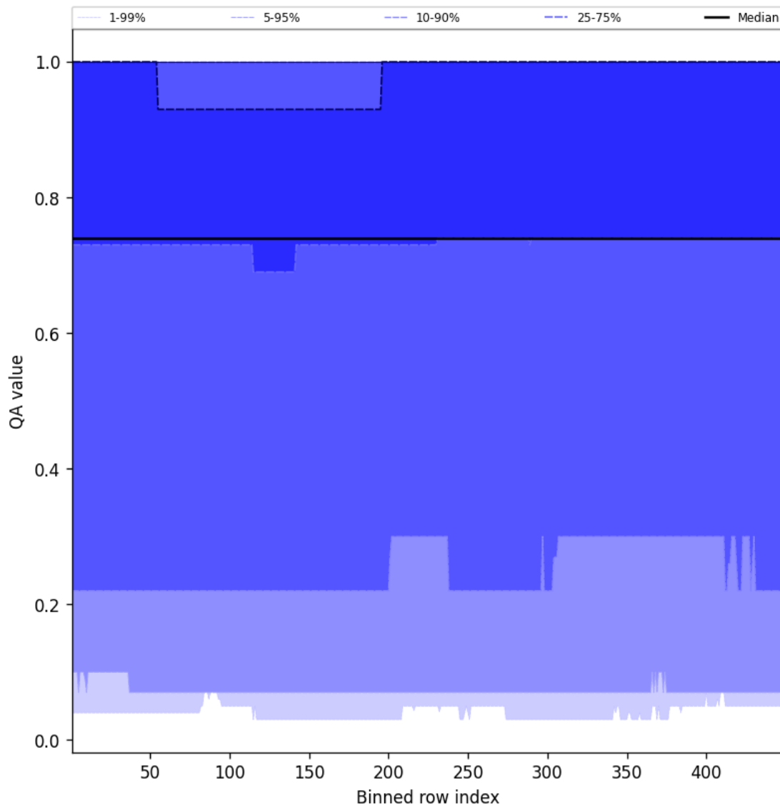
Figure 43: Along track statistics of “QA value” for 2025-10-17 to 2025-10-18
