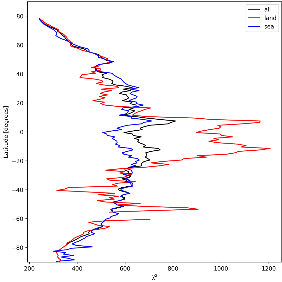
Figure 23: Zonal average of “ \chi^2 ” for 2025-10-17 to 2025-10-18.
