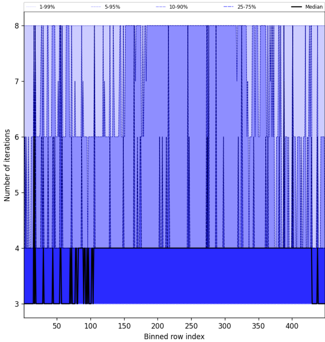
Figure 49: Along track statistics of “Number of iterations” for 2025-10-17 to 2025-10-18
