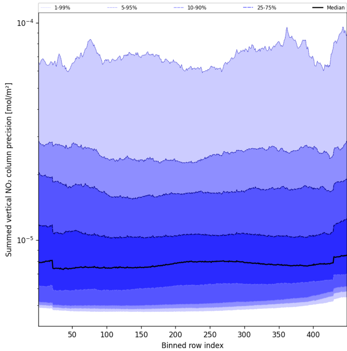
Figure 56: Along track statistics of “Summed vertical NO 2 column precision” for 2025-10-17 to 2025-10-18
