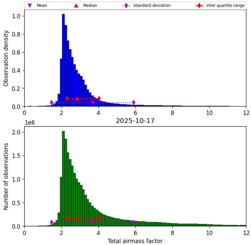
Figure 30: Histogram of “Total airmass factor” for 2025-10-17 to 2025-10-18
