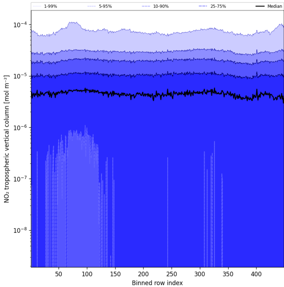
Figure 44: Along track statistics of “NO 2 tropospheric vertical column” for 2025-10-17 to 2025-10-18
