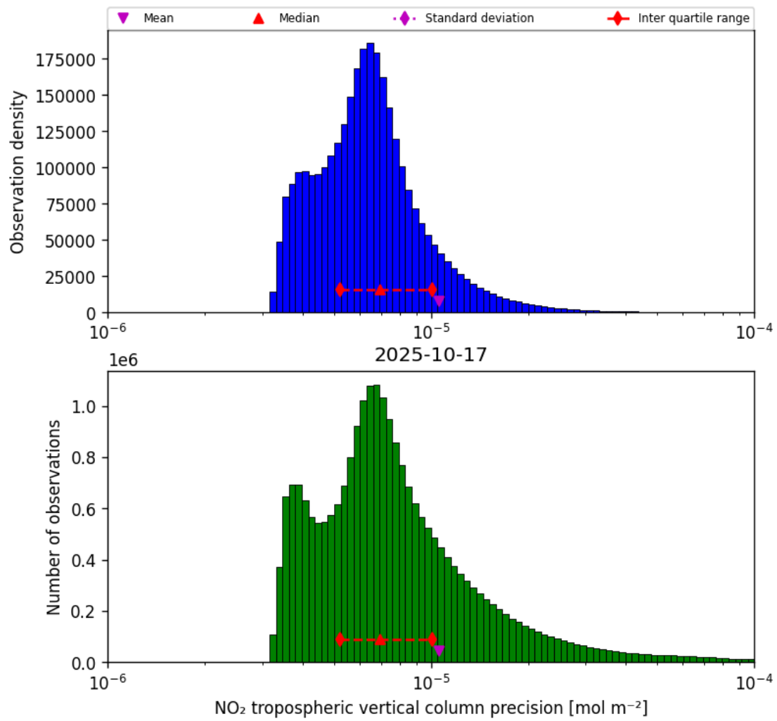
Figure 28: Histogram of “NO 2 tropospheric vertical column precision” for 2025-10-17 to 2025-10-18
