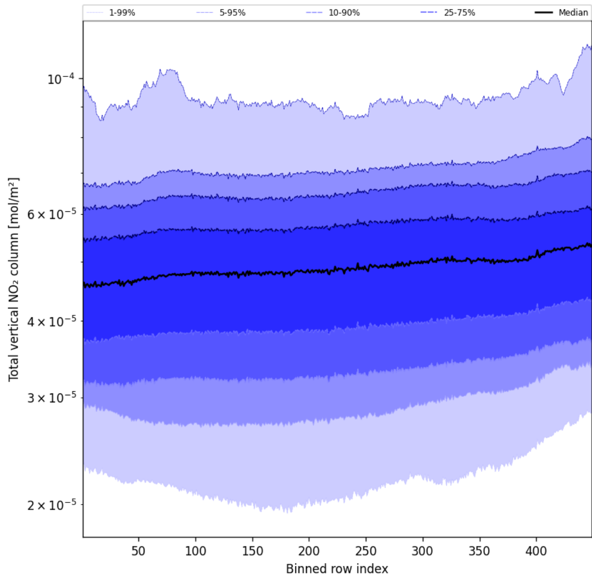
Figure 53: Along track statistics of “Total vertical NO 2 column” for 2025-10-17 to 2025-10-18
