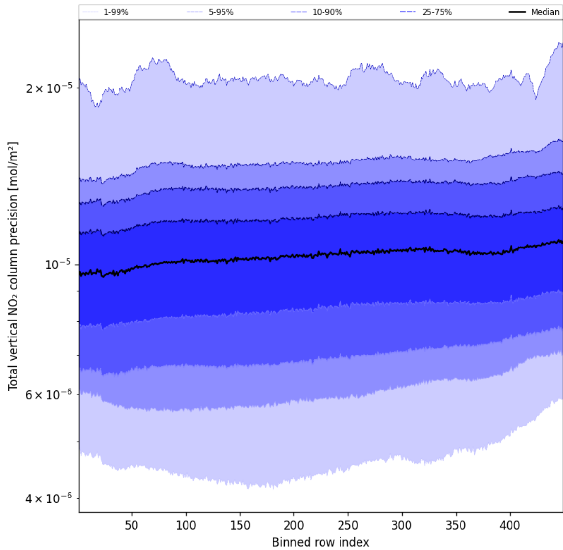
Figure 54: Along track statistics of “Total vertical NO 2 column precision” for 2025-10-17 to 2025-10-18
