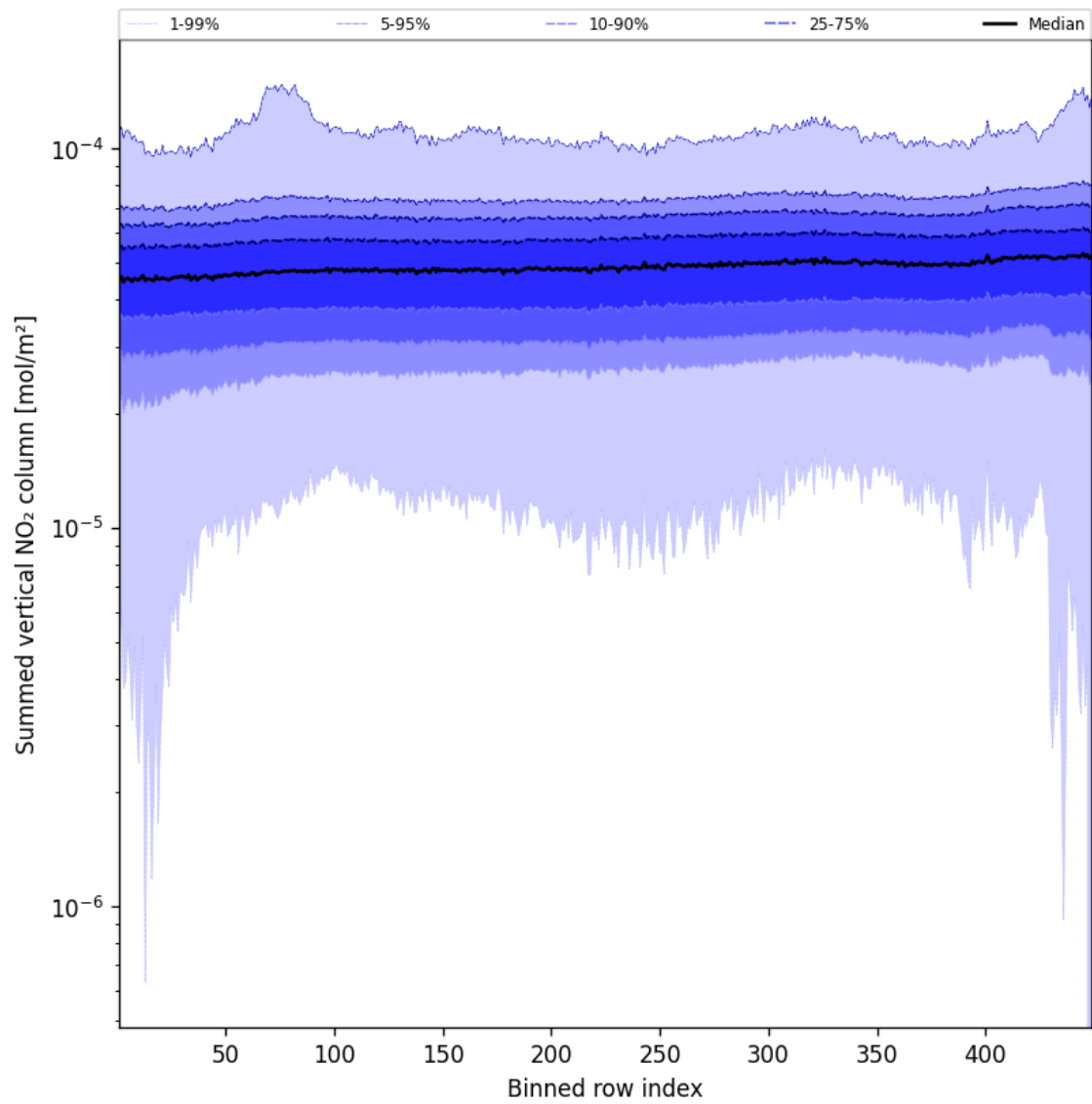
Figure 55: Along track statistics of “Summed vertical NO 2 column” for 2025-10-17 to 2025-10-18
