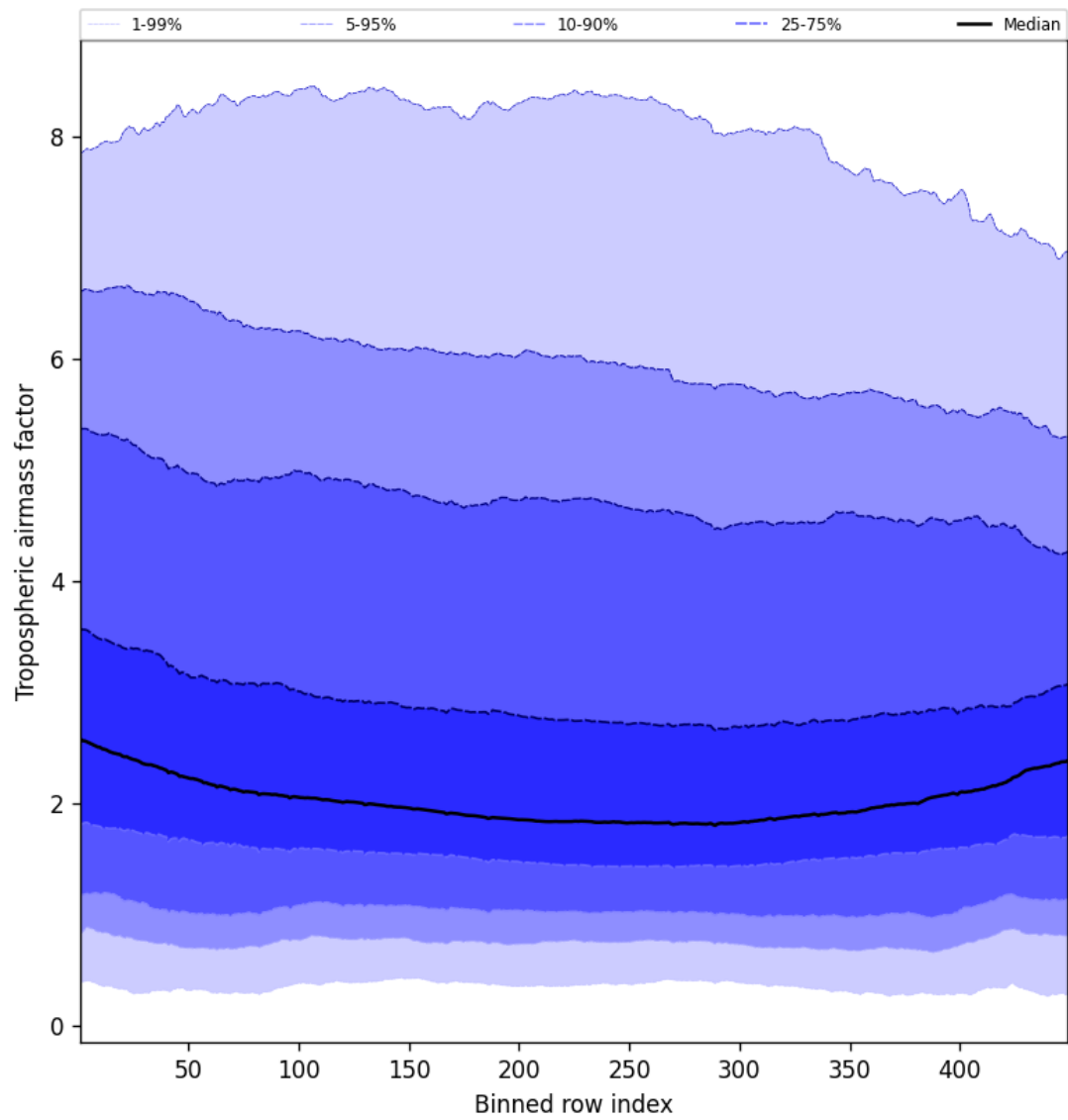
Figure 46: Along track statistics of “Tropospheric airmass factor” for 2025-10-17 to 2025-10-18
