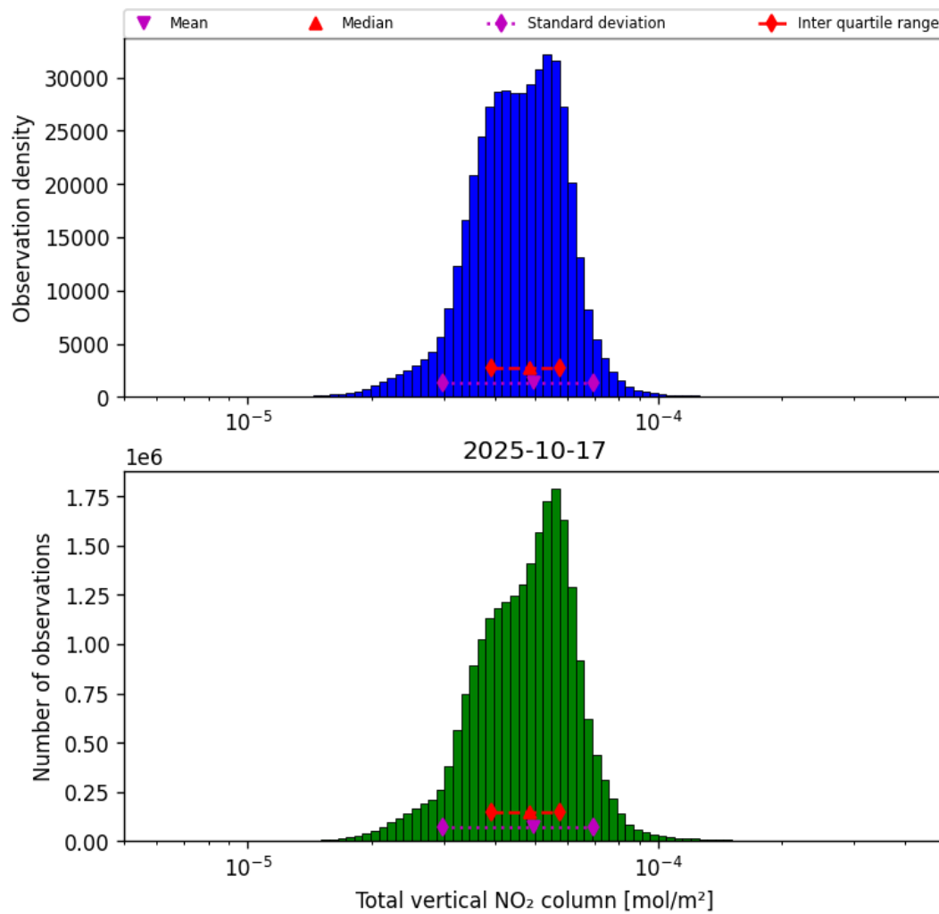
Figure 36: Histogram of “Total vertical NO 2 column” for 2025-10-17 to 2025-10-18
