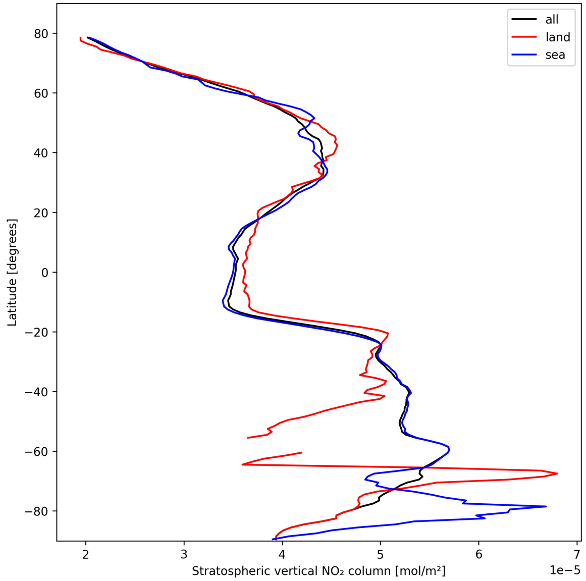
Figure 17: Zonal average of “Stratospheric vertical NO 2 column” for 2025-10-17 to 2025-10-18.
