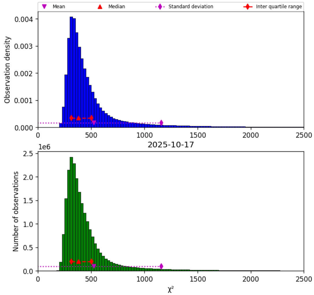
Figure 40: Histogram of “ \chi^2 ” for 2025-10-17 to 2025-10-18
