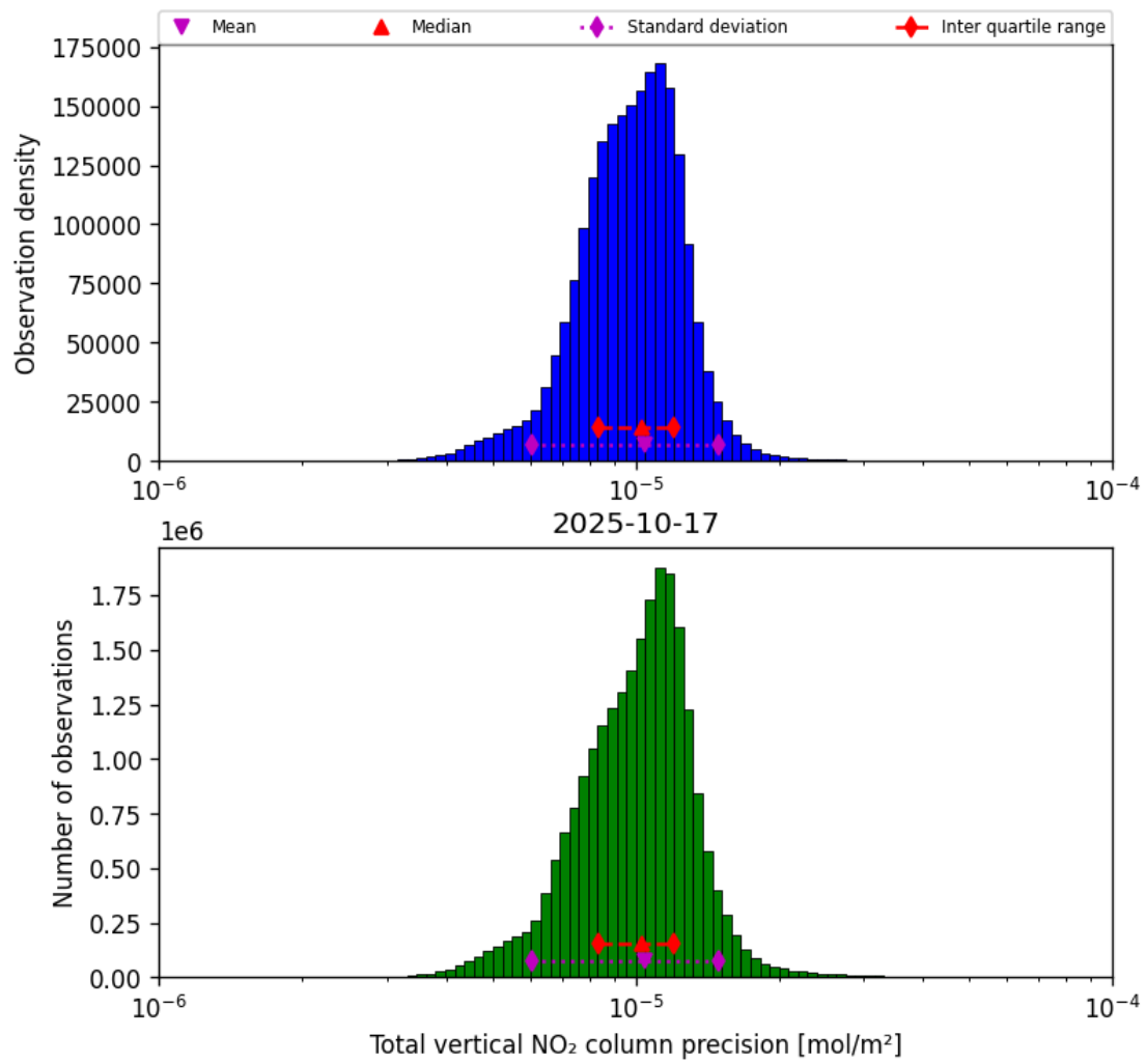
Figure 37: Histogram of “Total vertical NO 2 column precision” for 2025-10-17 to 2025-10-18
