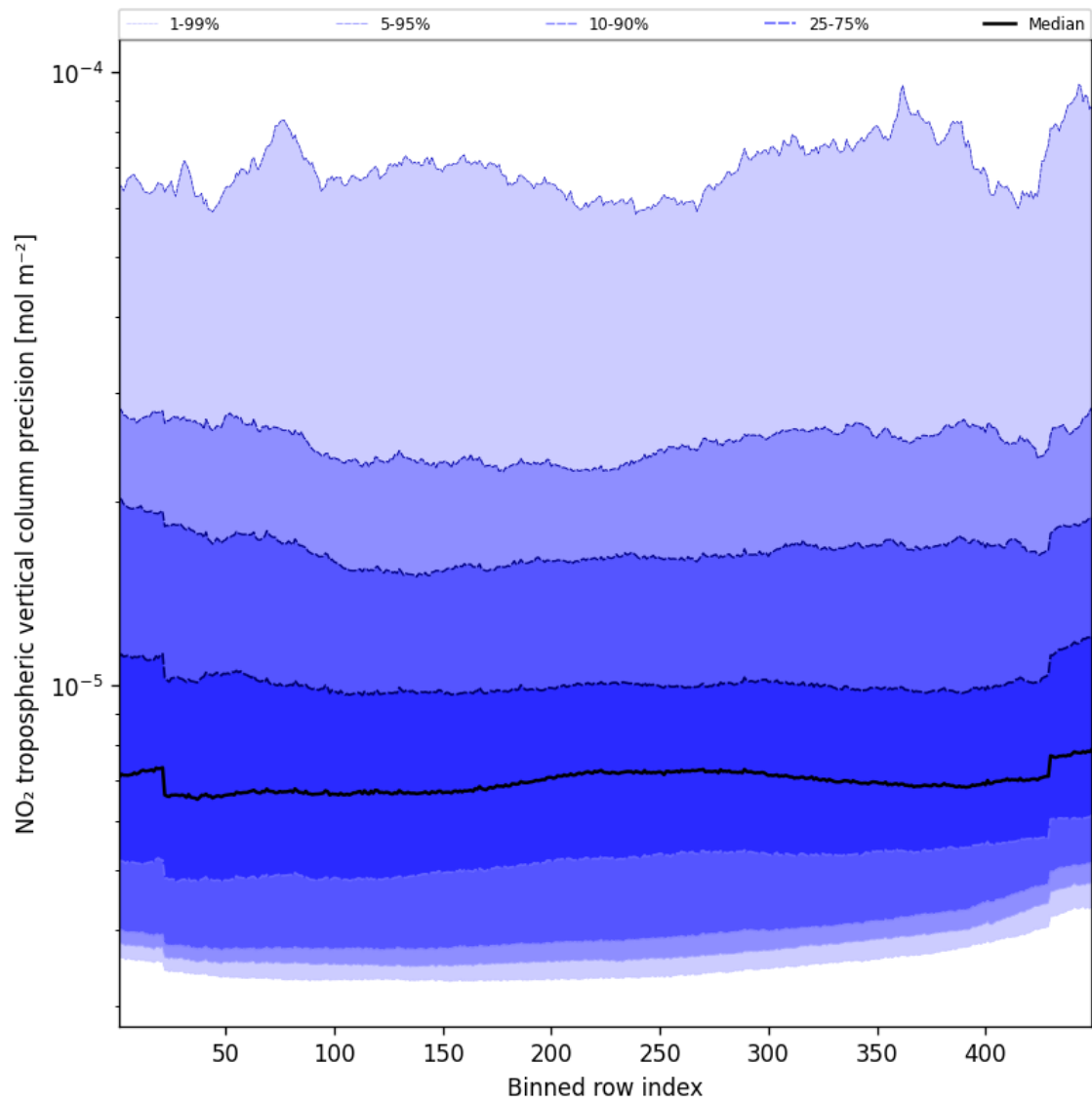
Figure 45: Along track statistics of “NO 2 tropospheric vertical column precision” for 2025-10-17 to 2025-10-18
