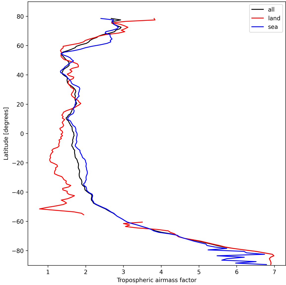
Figure 12: Zonal average of “Tropospheric air mass factor” for 2025-10-17 to 2025-10-18.
