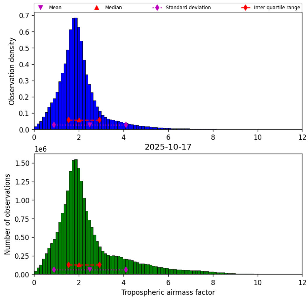
Figure 29: Histogram of “Tropospheric airmass factor” for 2025-10-17 to 2025-10-18
