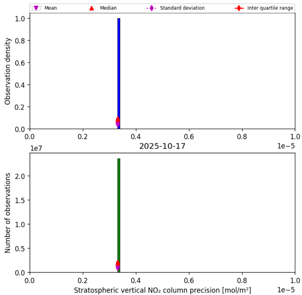
Figure 35: Histogram of “Stratospheric vertical NO 2 column precision” for 2025-10-17 to 2025-10-18
