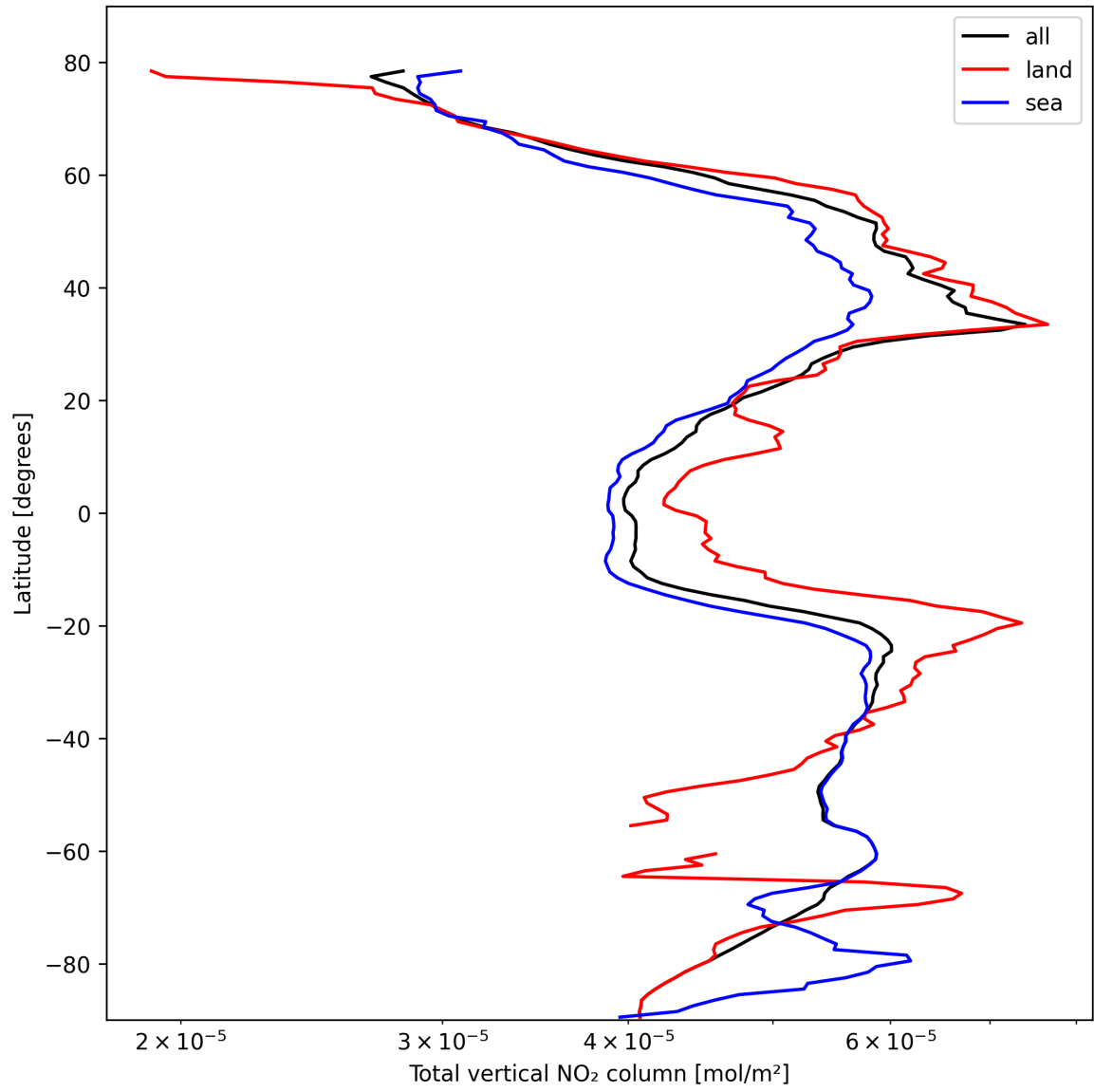
Figure 19: Zonal average of “Total vertical NO 2 column” for 2025-10-17 to 2025-10-18.
