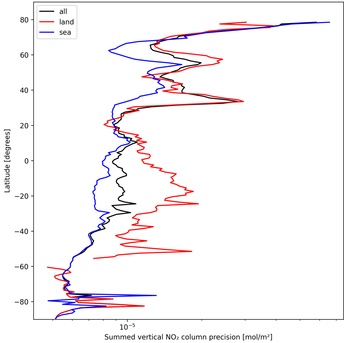
Figure 22: Zonal average of “Summed vertical NO 2 column precision” for 2025-10-17 to 2025-10-18.
