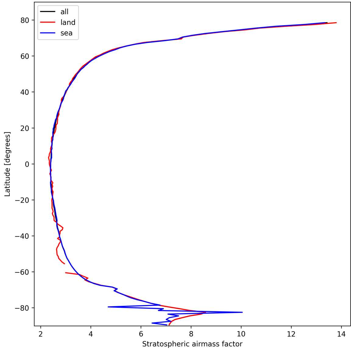
Figure 25: Zonal average of “Stratospheric air mass factor” for 2025-10-17 to 2025-10-18.
