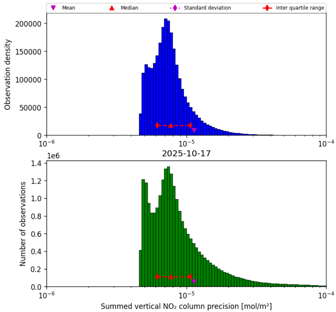
Figure 39: Histogram of “Summed vertical NO 2 column precision” for 2025-10-17 to 2025-10-18
