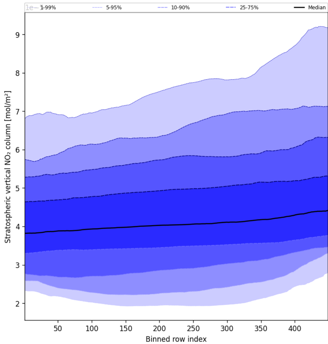
Figure 51: Along track statistics of “Stratospheric vertical NO 2 column” for 2025-10-17 to 2025-10-18
