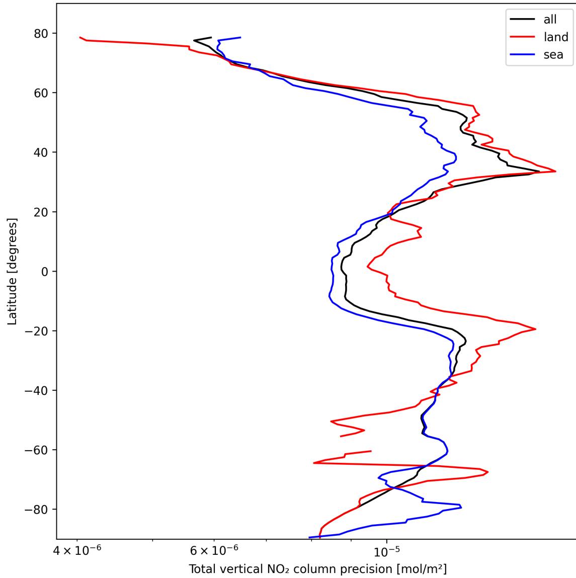
Figure 20: Zonal average of “Total vertical NO 2 column precision” for 2025-10-17 to 2025-10-18.
