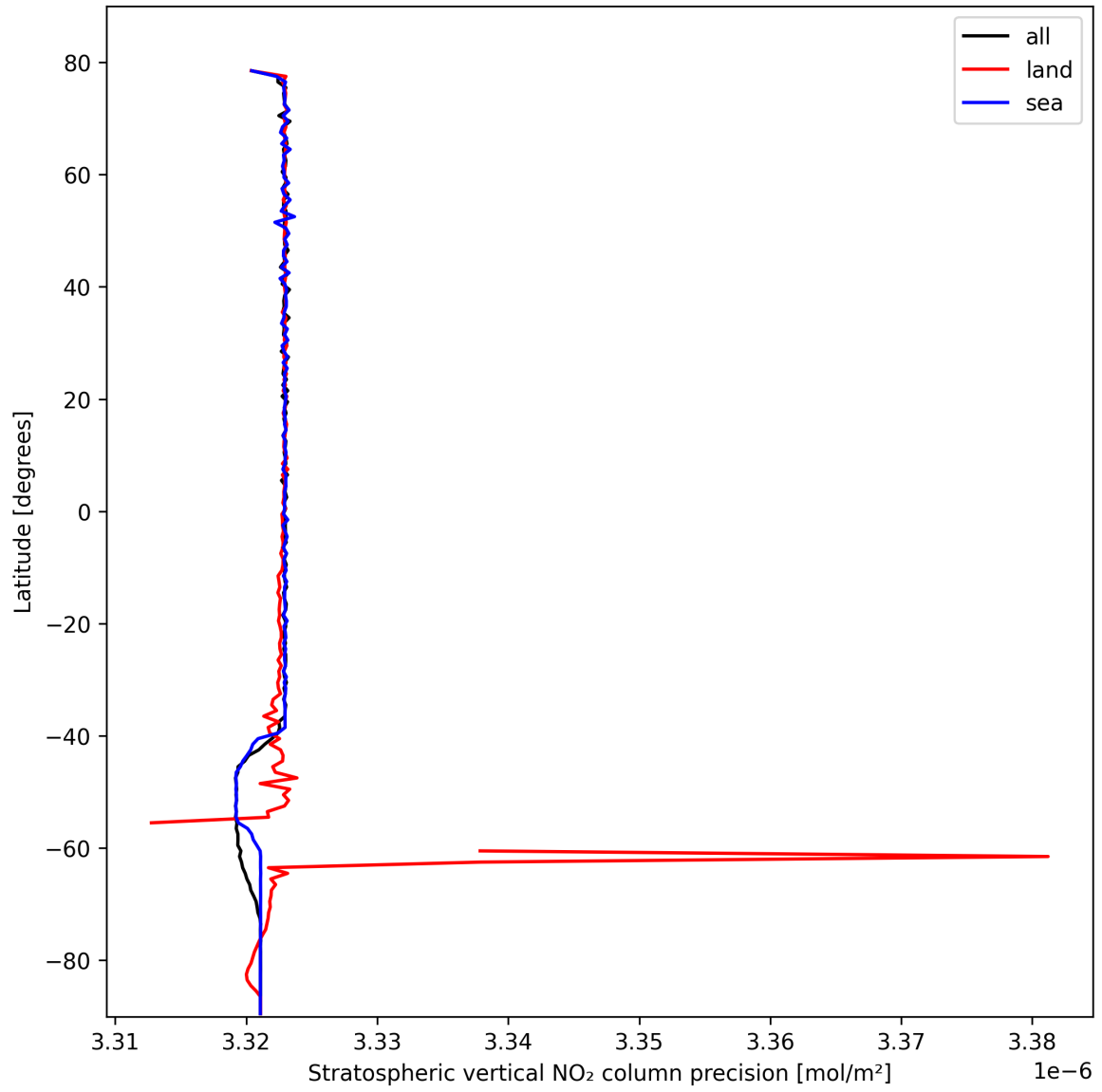
Figure 18: Zonal average of “Stratospheric vertical NO 2 column precision” for 2025-10-17 to 2025-10-18.
