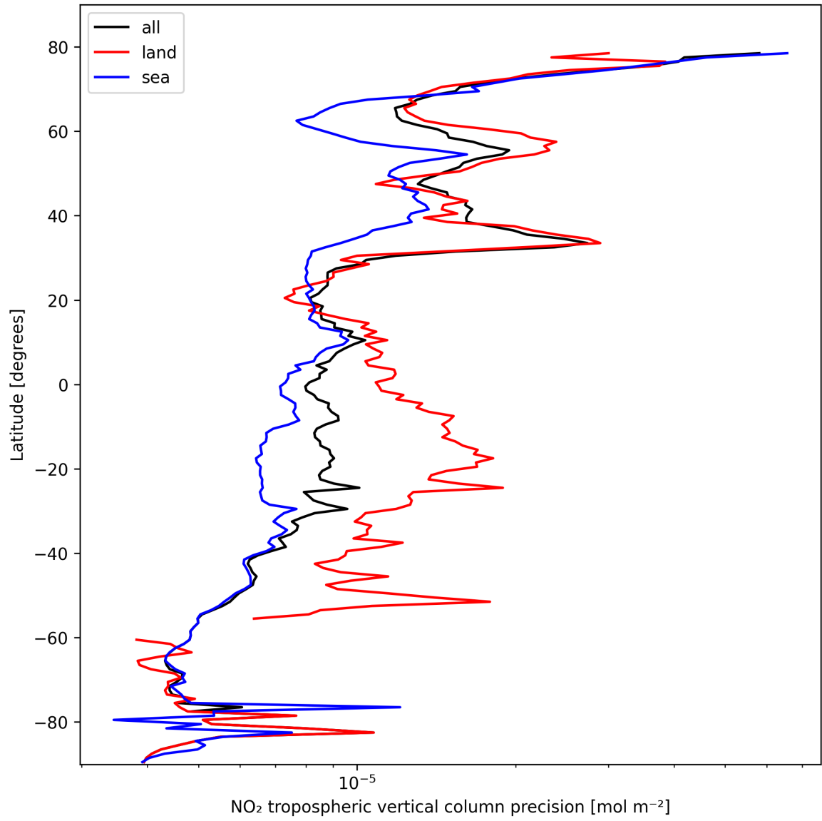
Figure 11: Zonal average of “NO 2 tropospheric vertical column precision” for 2025-10-17 to 2025-10-18.
