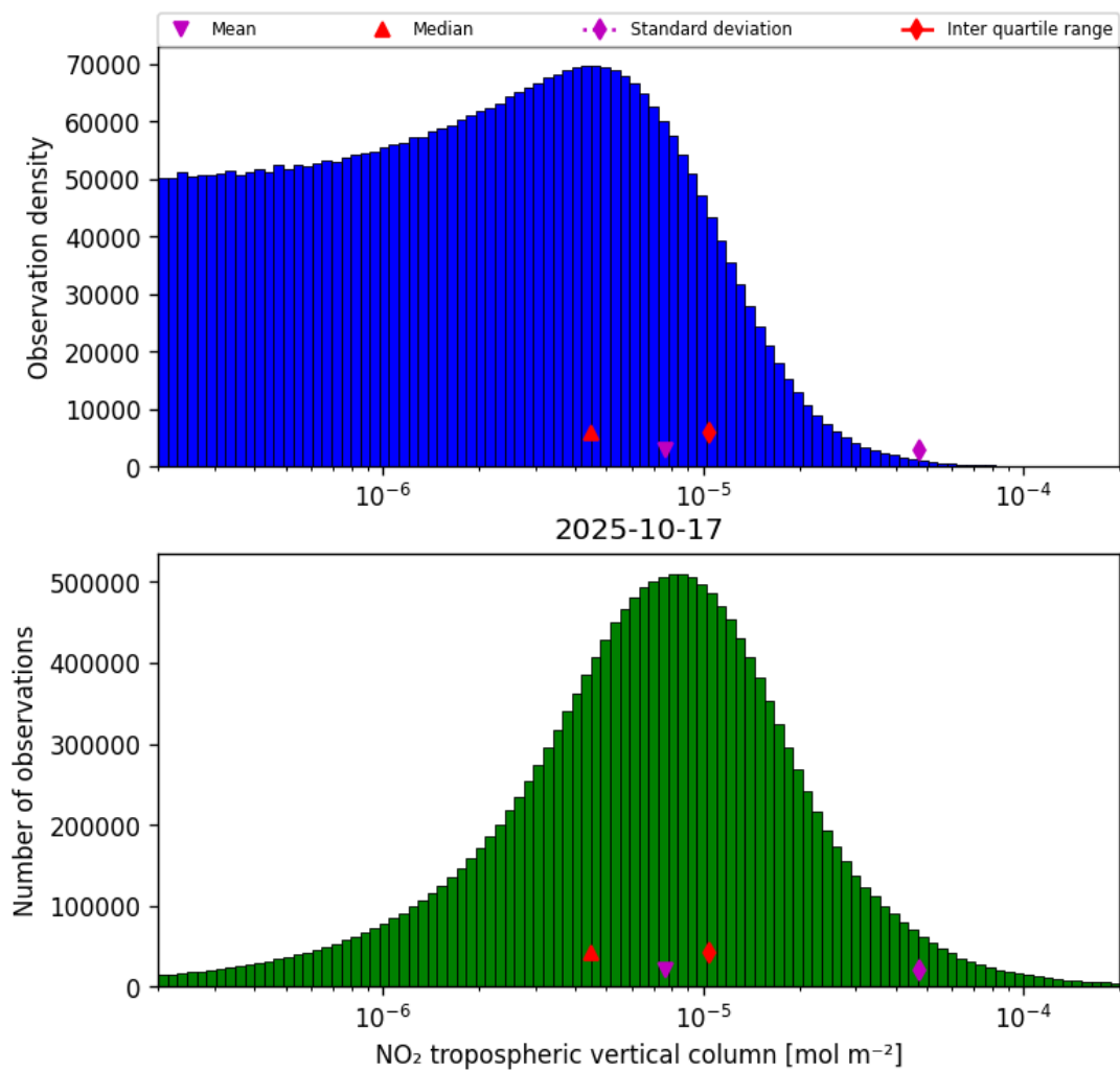
Figure 27: Histogram of “NO 2 tropospheric vertical column” for 2025-10-17 to 2025-10-18
