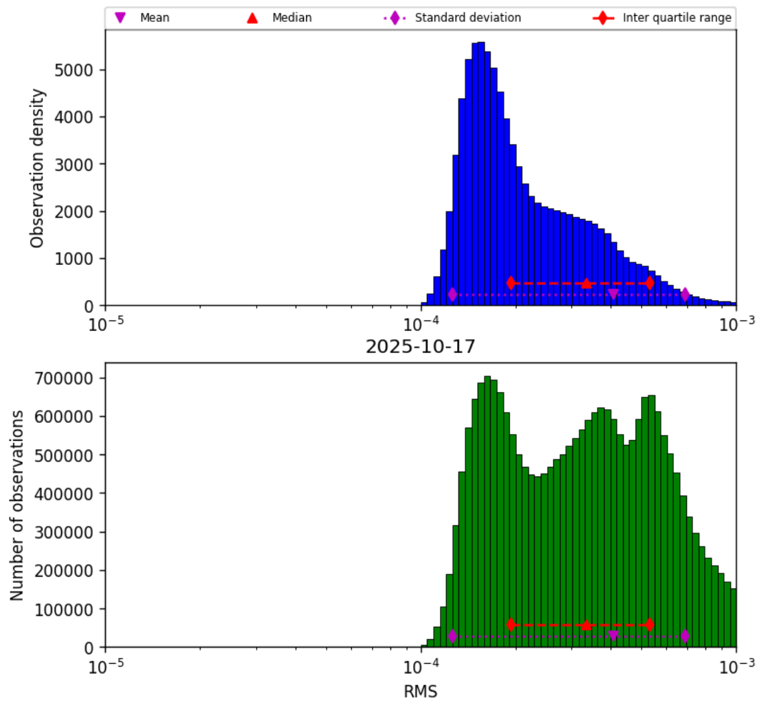
Figure 41: Histogram of “RMS” for 2025-10-17 to 2025-10-18
