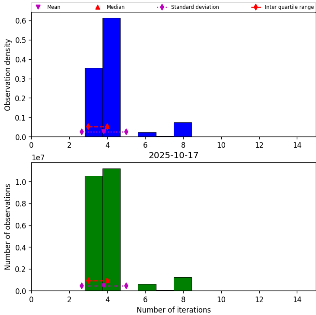
Figure 32: Histogram of “Number of iterations” for 2025-10-17 to 2025-10-18
