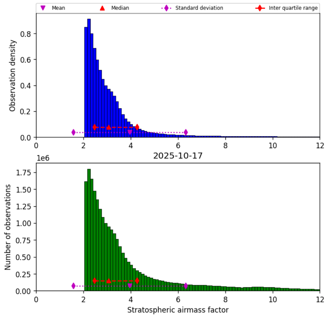
Figure 42: Histogram of “Stratospheric airmass factor” for 2025-10-17 to 2025-10-18
