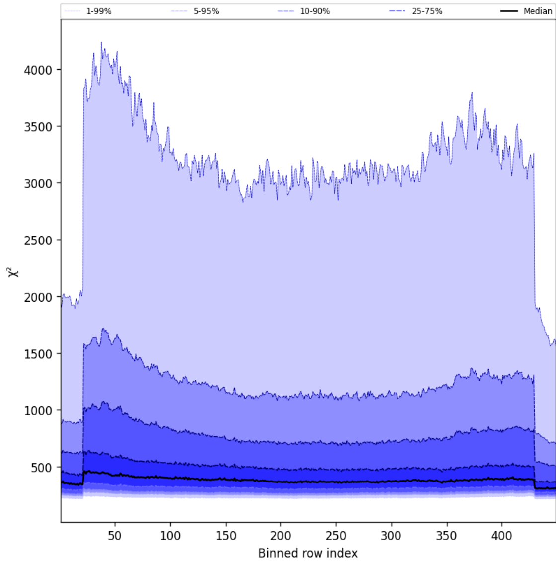
Figure 57: Along track statistics of “ \chi^2 ” for 2025-10-17 to 2025-10-18
