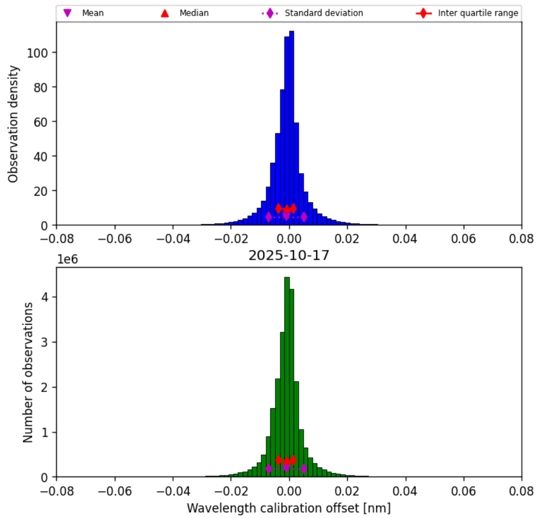
Figure 33: Histogram of “Wavelength calibration offset” for 2025-10-17 to 2025-10-18
