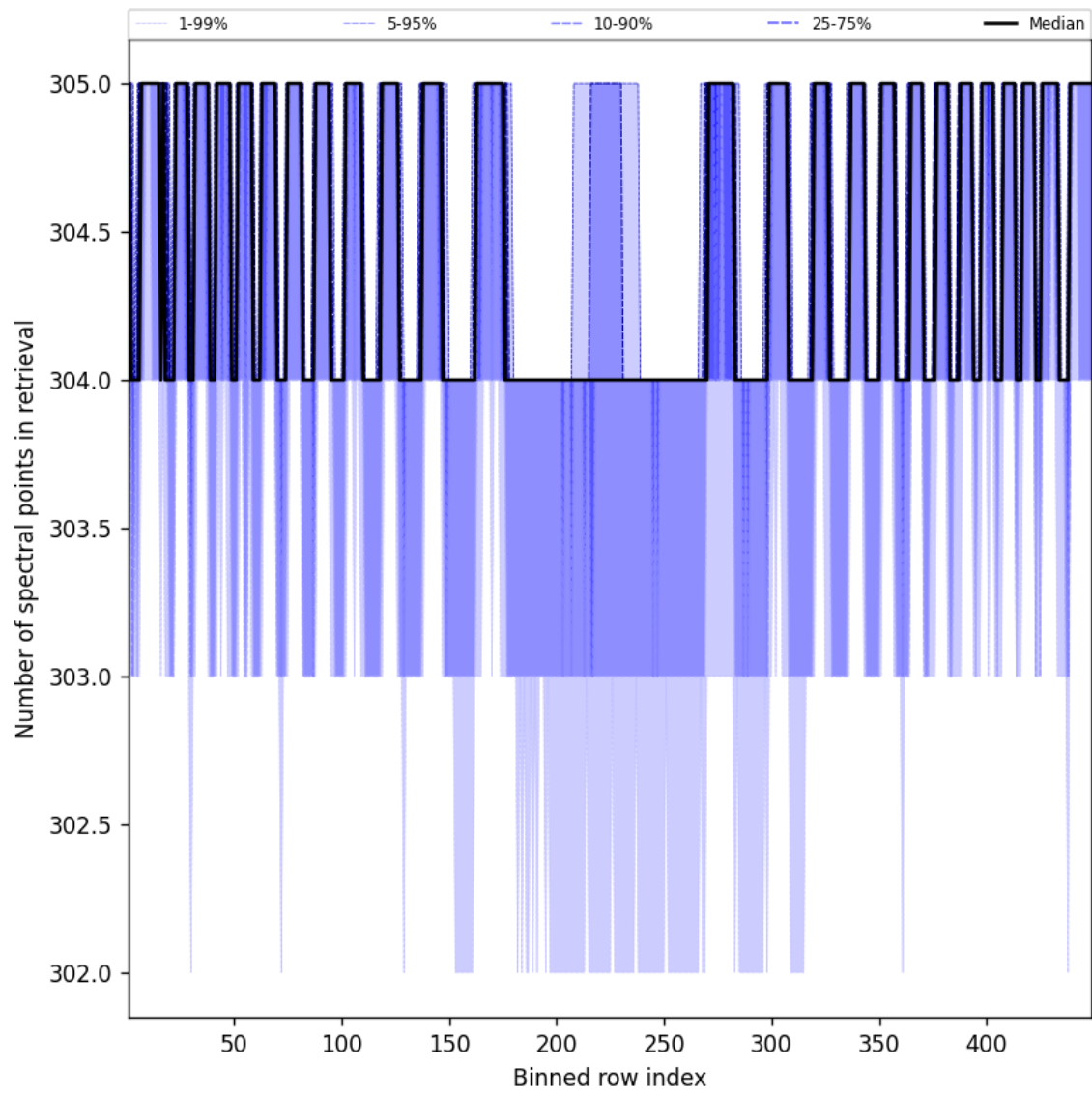
Figure 48: Along track statistics of “Number of spectral points in retrieval” for 2025-10-17 to 2025-10-18
