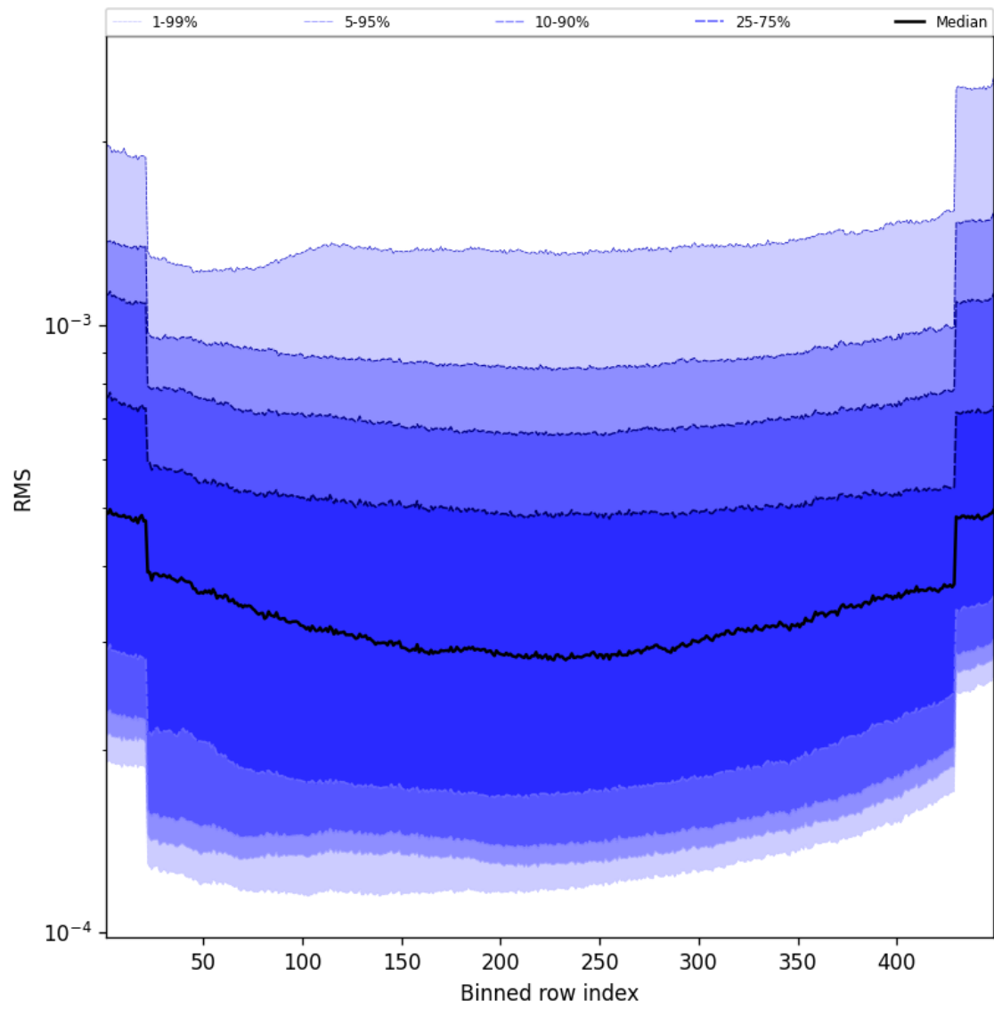
Figure 58: Along track statistics of “RMS” for 2025-10-17 to 2025-10-18
