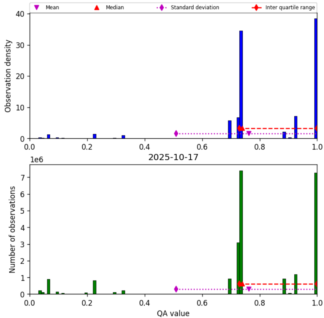
Figure 26: Histogram of “QA value” for 2025-10-17 to 2025-10-18
