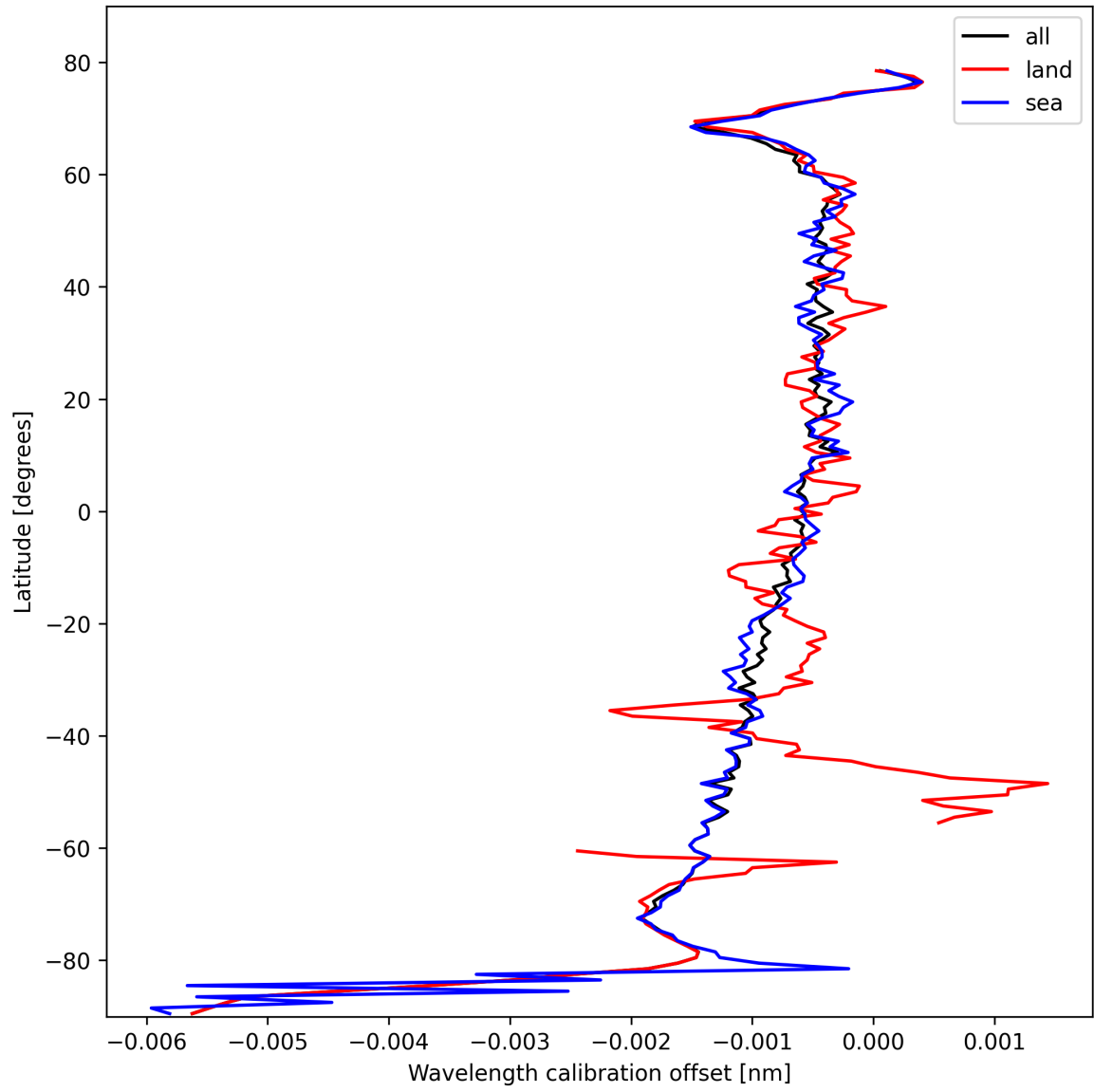
Figure 16: Zonal average of “Wavelength calibration offset” for 2025-10-17 to 2025-10-18.
