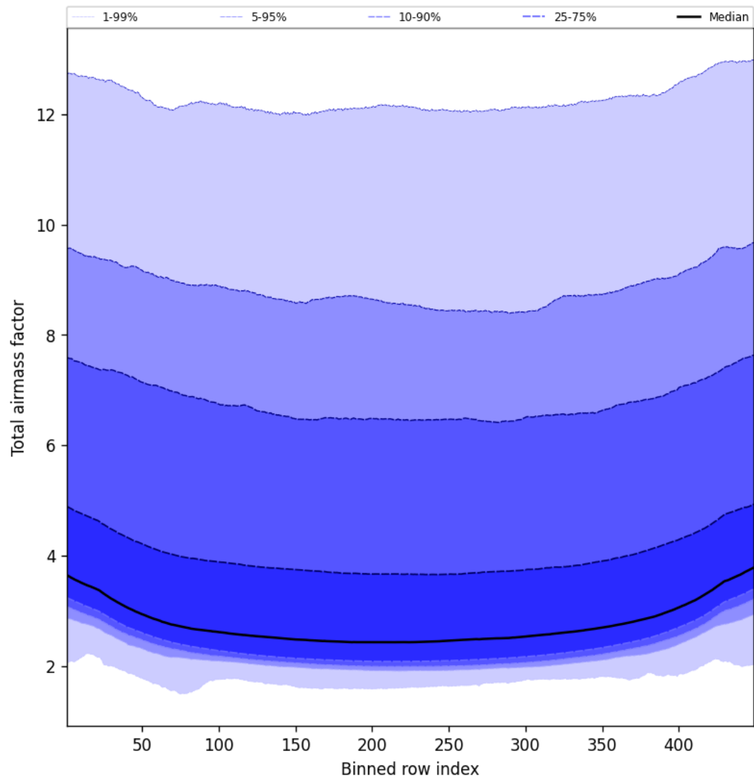
Figure 47: Along track statistics of “Total airmass factor” for 2025-10-17 to 2025-10-18
