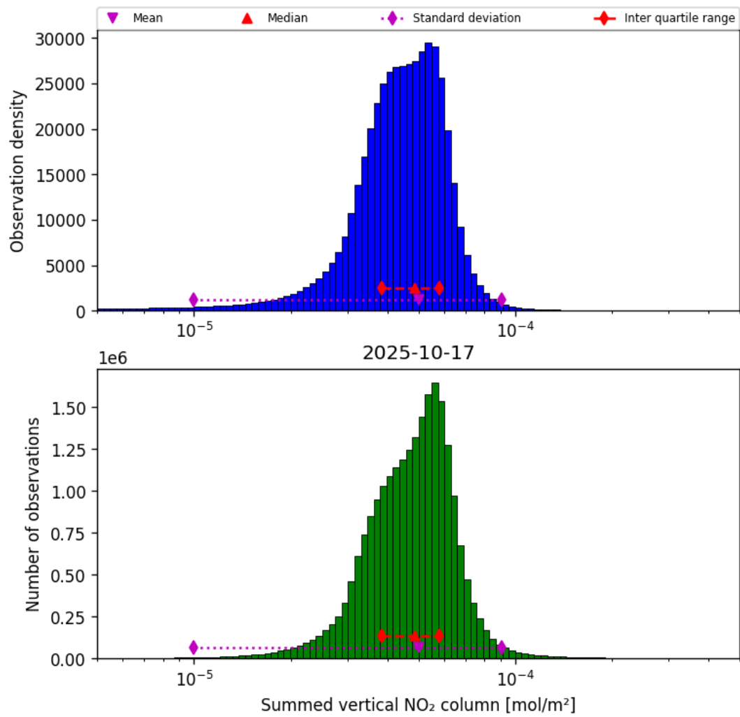
Figure 38: Histogram of “Summed vertical NO 2 column” for 2025-10-17 to 2025-10-18
