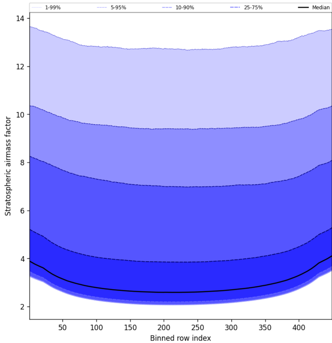
Figure 59: Along track statistics of “Stratospheric airmass factor” for 2025-10-17 to 2025-10-18
