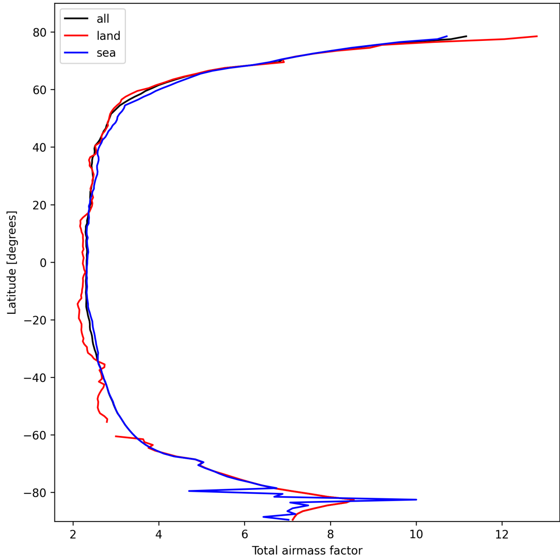
Figure 13: Zonal average of “Total airmass factor” for 2025-10-17 to 2025-10-18.
