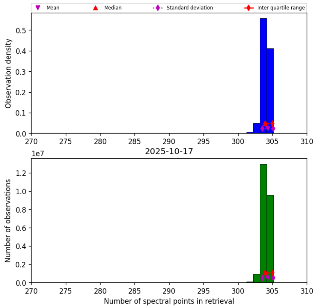
Figure 31: Histogram of “Number of spectral points in retrieval” for 2025-10-17 to 2025-10-18
