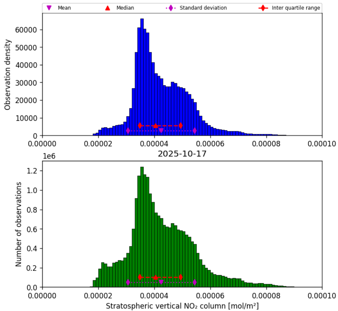
Figure 34: Histogram of “Stratospheric vertical NO 2 column” for 2025-10-17 to 2025-10-18
