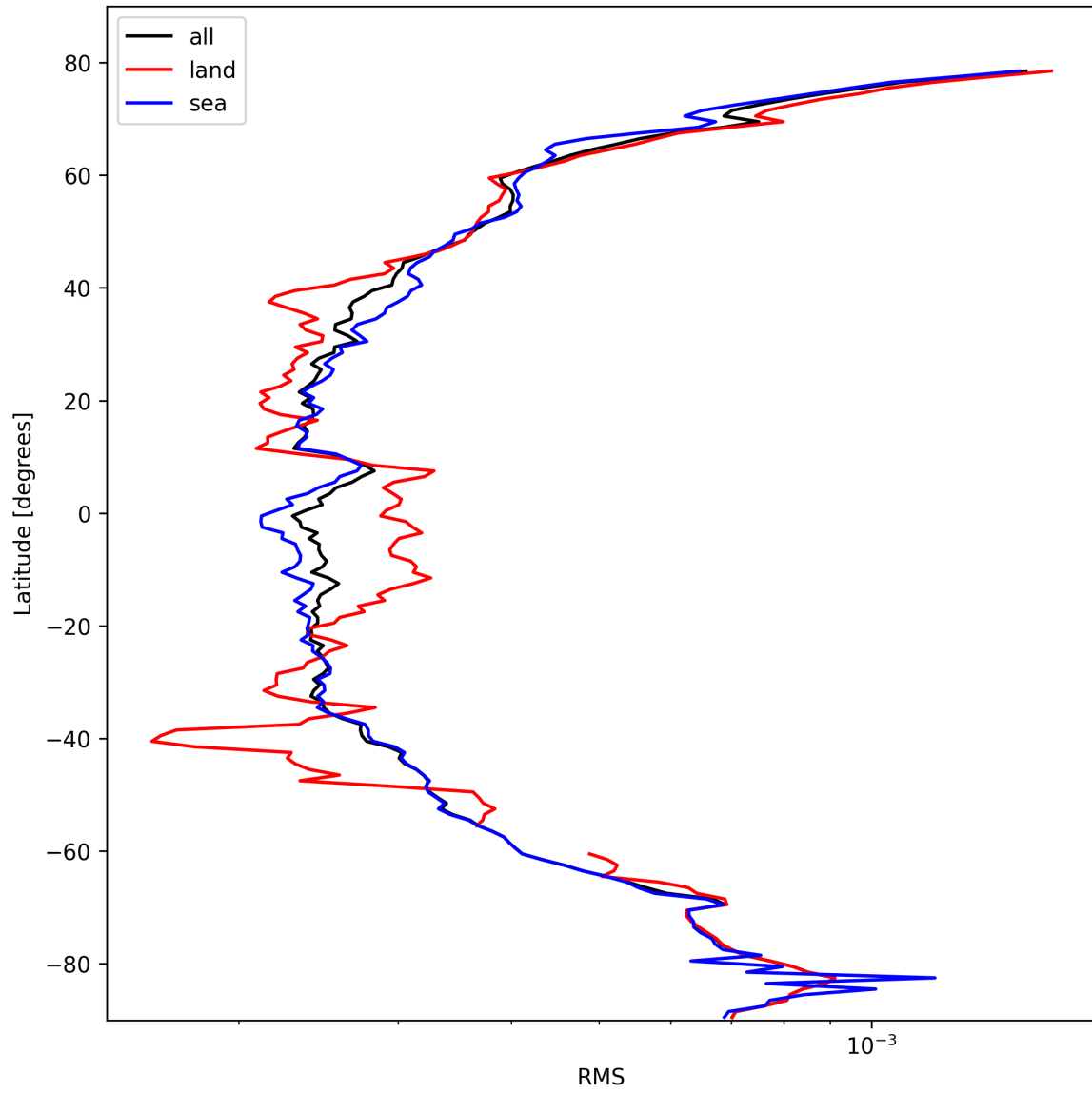
Figure 24: Zonal average of “RMS” for 2025-10-17 to 2025-10-18.
