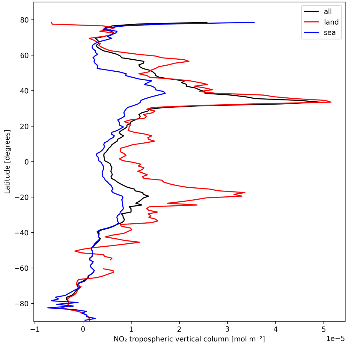
Figure 10: Zonal average of “NO 2 tropospheric vertical column” for 2025-10-17 to 2025-10-18.
