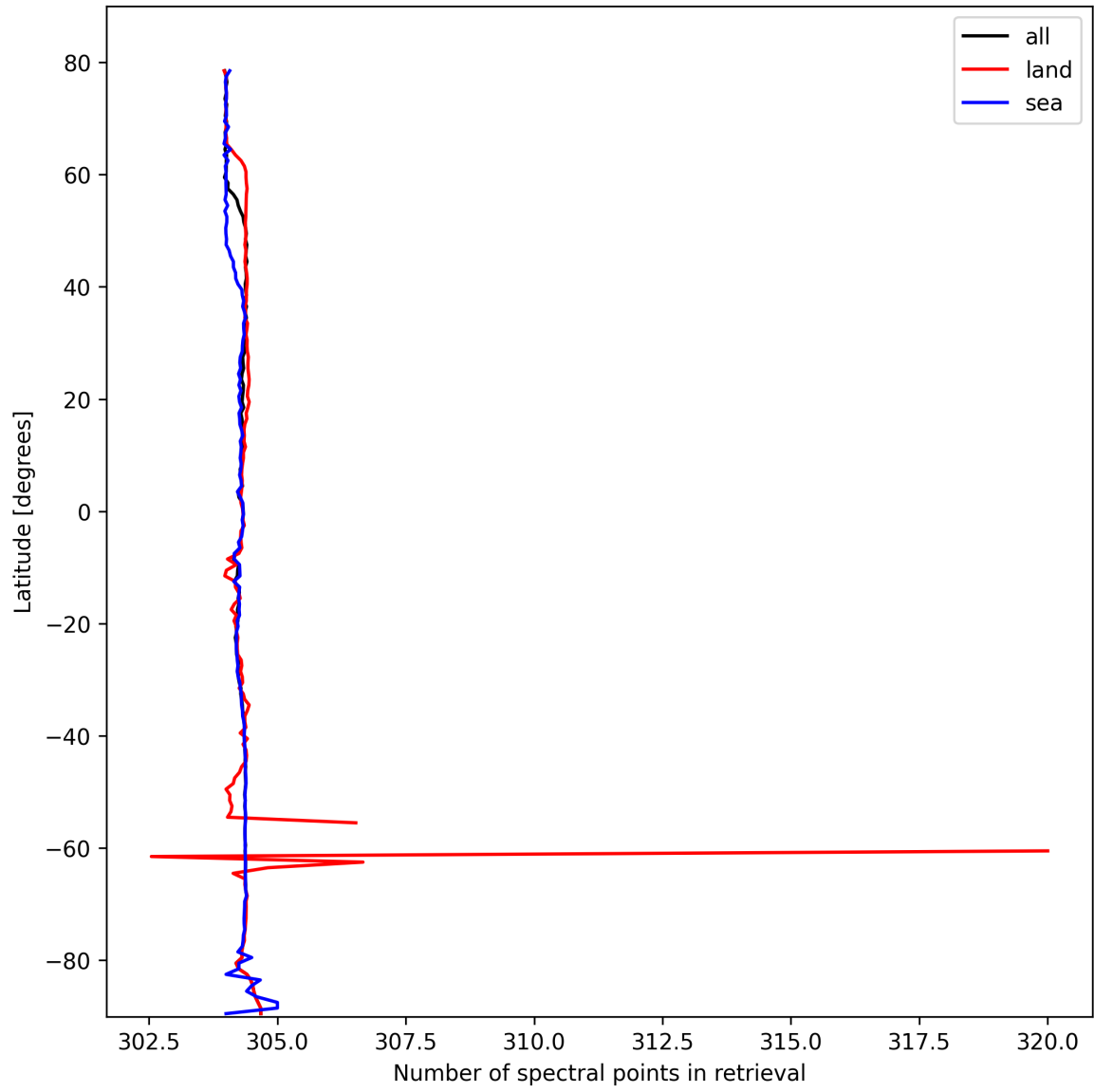
Figure 14: Zonal average of “Number of spectral points in retrieval” for 2025-10-17 to 2025-10-18.
