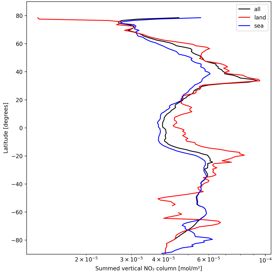
Figure 21: Zonal average of “Summed vertical NO 2 column” for 2025-10-17 to 2025-10-18.
