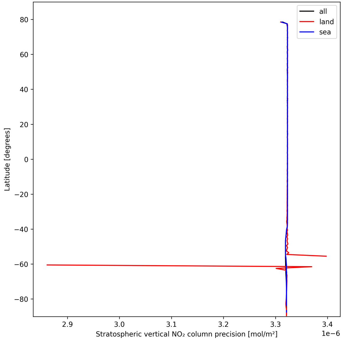
Figure 18: Zonal average of "Stratospheric vertical NO 2 column precision" for 2025-10-18 to 2025-10-19.
