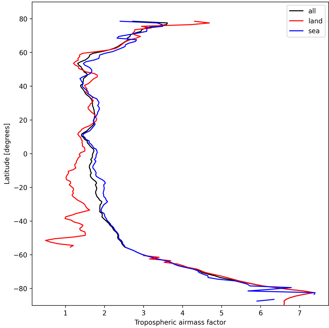
Figure 12: Zonal average of “Tropospheric airmass factor” for 2025-10-18 to 2025-10-19.
