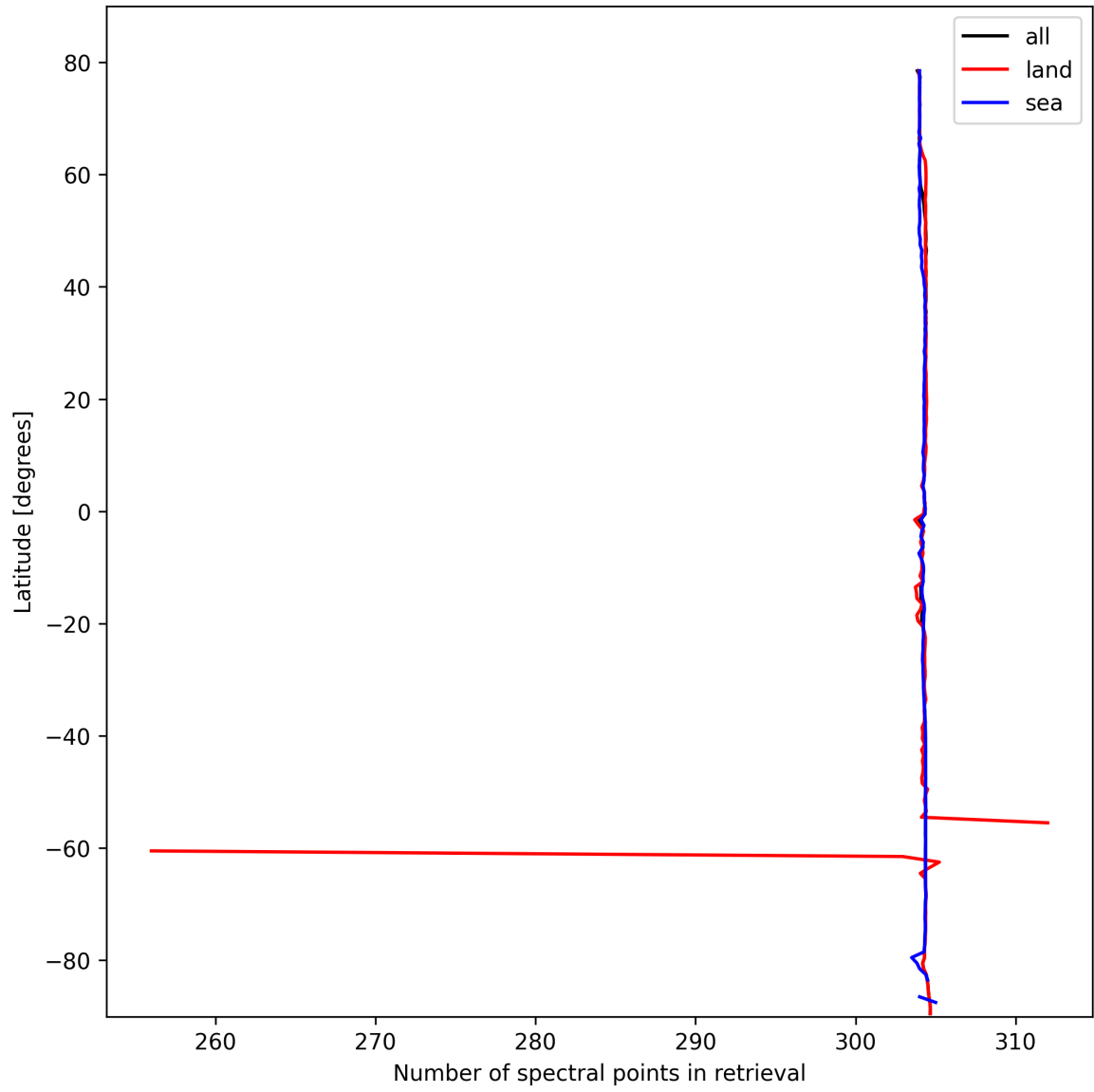
Figure 14: Zonal average of “Number of spectral points in retrieval” for 2025-10-18 to 2025-10-19.
