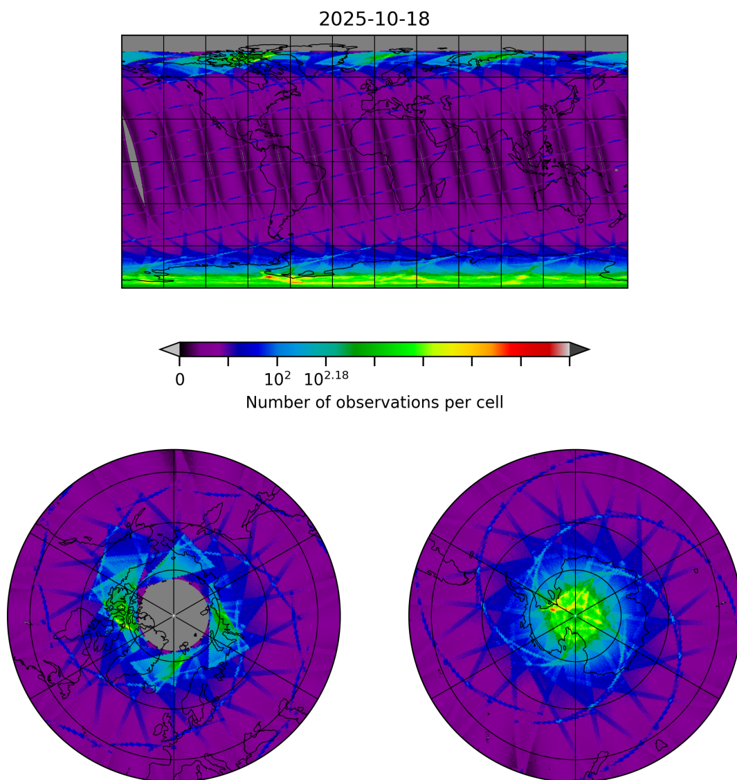
Figure 8: Map of the number of observations for 2025-10-18 to 2025-10-19
