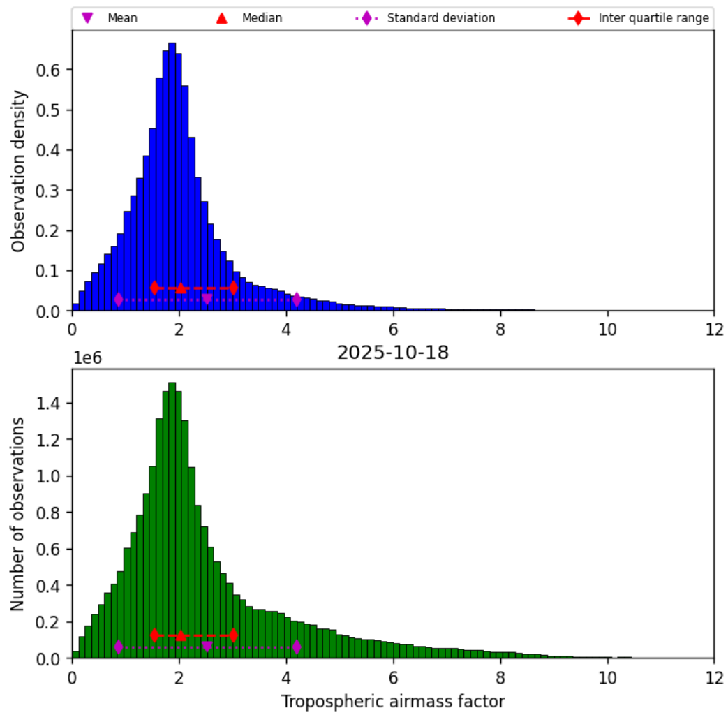
Figure 29: Histogram of “Tropospheric airmass factor” for 2025-10-18 to 2025-10-19
