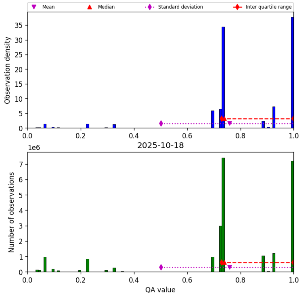
Figure 26: Histogram of “QA value” for 2025-10-18 to 2025-10-19
