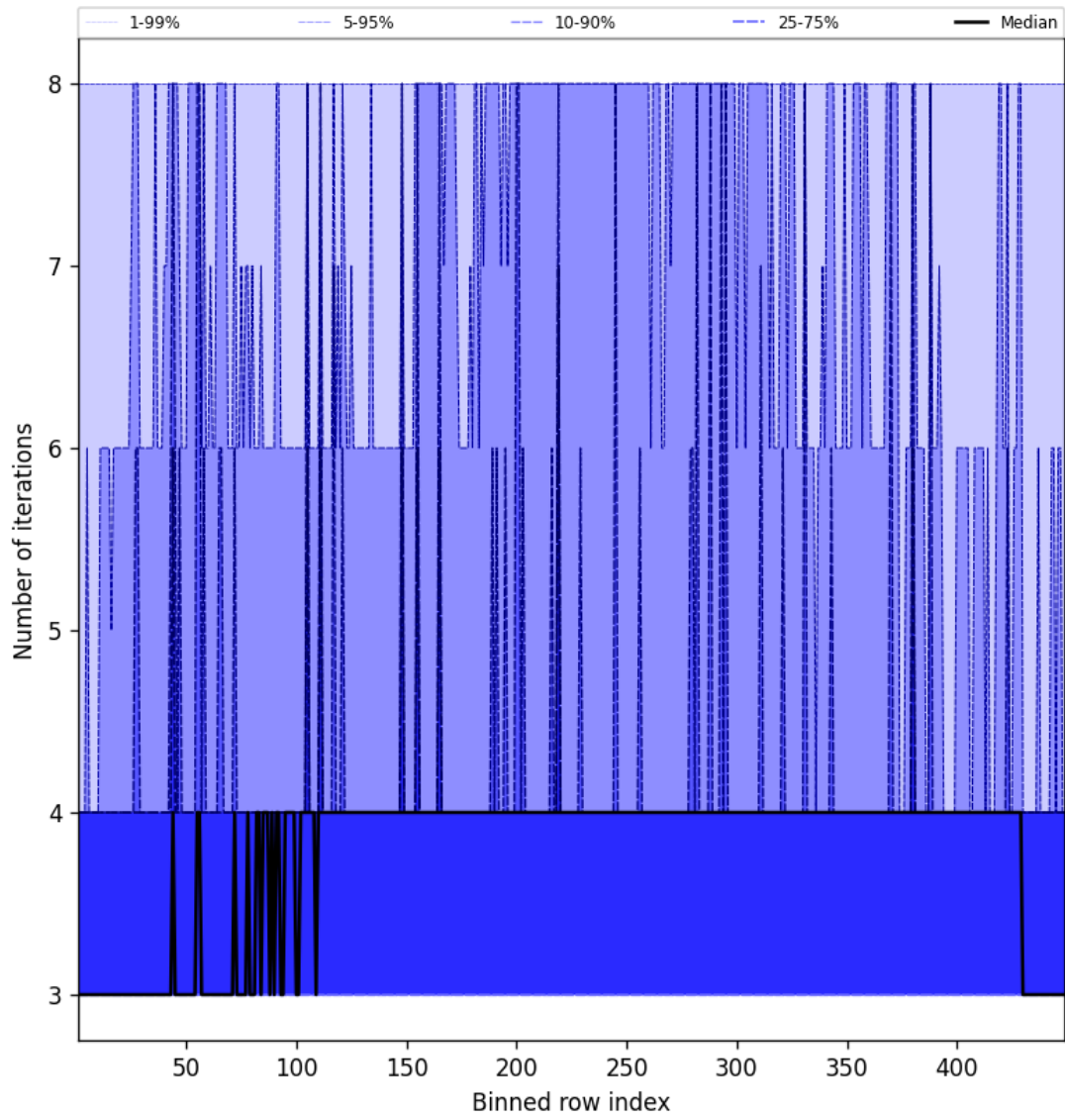
Figure 49: Along track statistics of “Number of iterations” for 2025-10-18 to 2025-10-19
