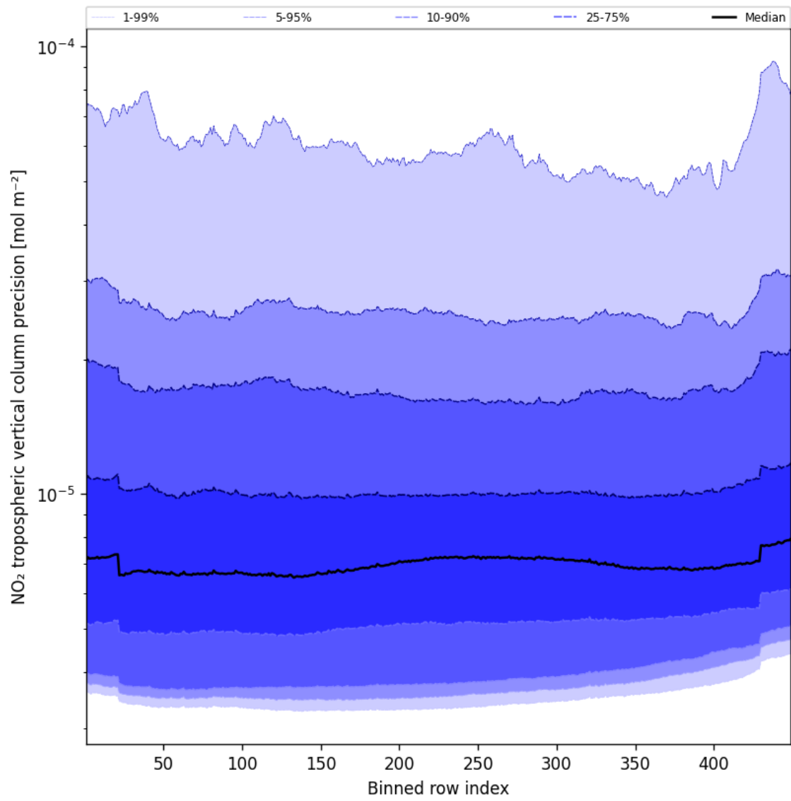
Figure 45: Along track statistics of “NO 2 tropospheric vertical column precision” for 2025-10-18 to 2025-10-19
