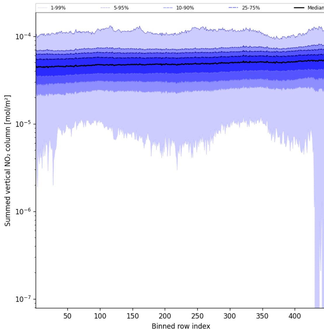
Figure 55: Along track statistics of “Summed vertical NO 2 column” for 2025-10-18 to 2025-10-19
