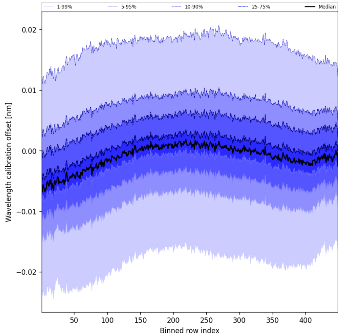
Figure 50: Along track statistics of “Wavelength calibration offset” for 2025-10-18 to 2025-10-19
