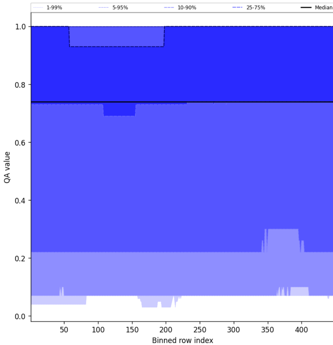
Figure 43: Along track statistics of "QA value" for 2025-10-18 to 2025-10-19
