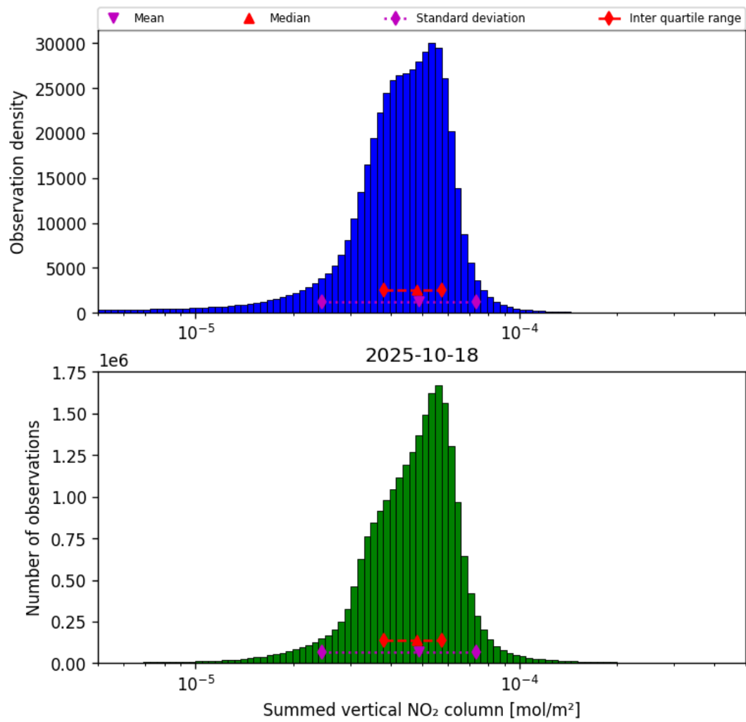
Figure 38: Histogram of “Summed vertical NO 2 column” for 2025-10-18 to 2025-10-19
