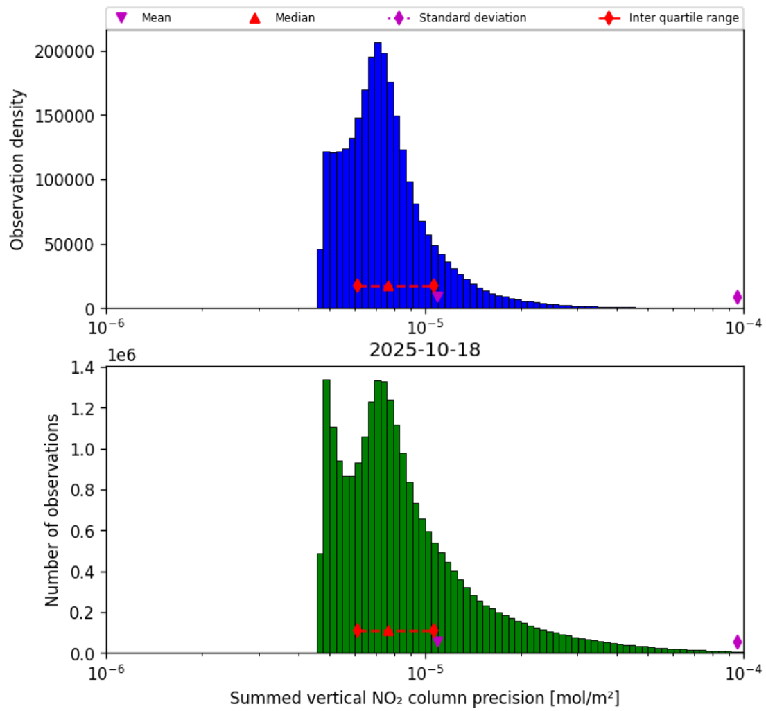
Figure 39: Histogram of “Summed vertical NO 2 column precision” for 2025-10-18 to 2025-10-19
