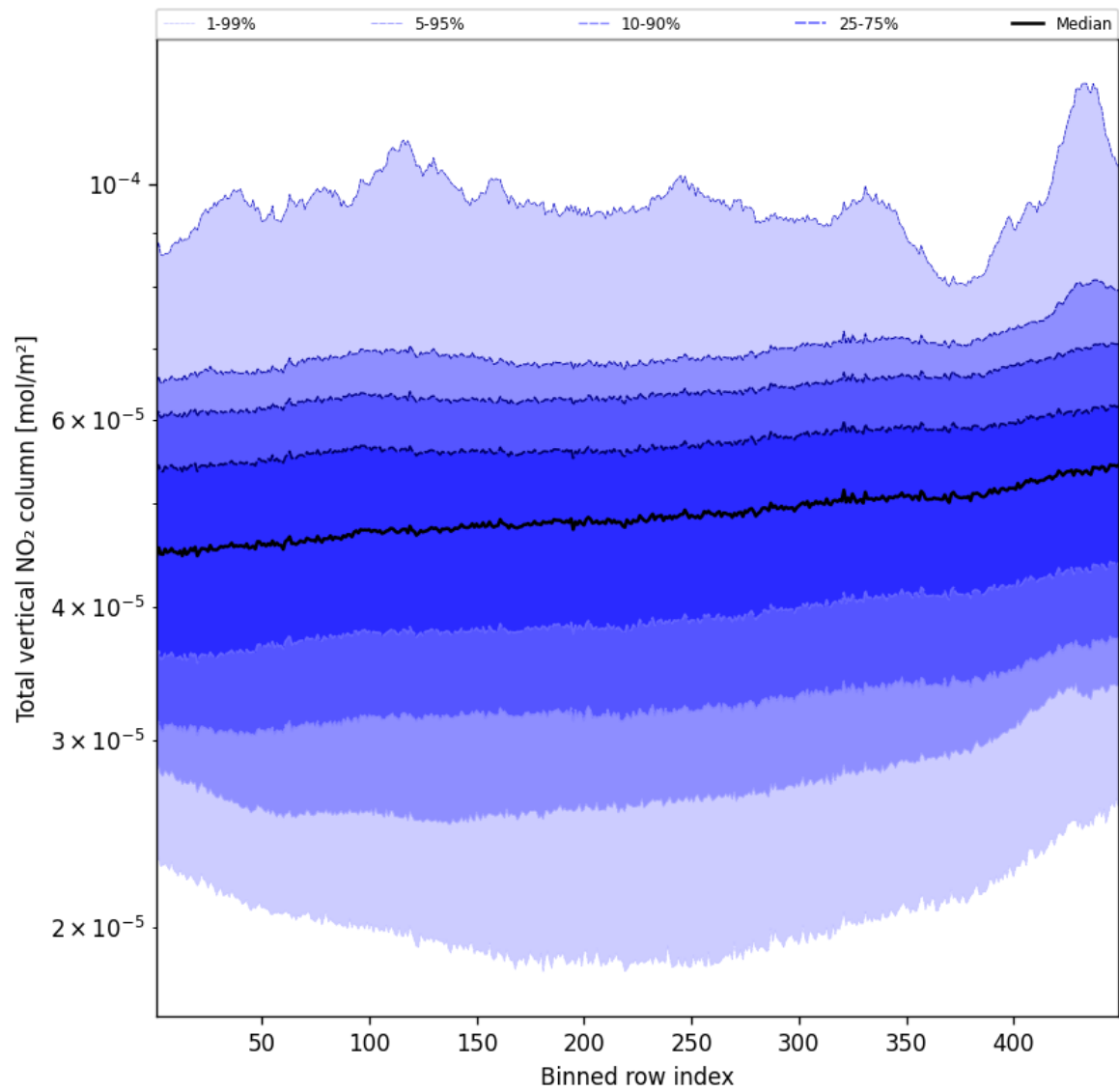
Figure 53: Along track statistics of “Total vertical NO 2 column” for 2025-10-18 to 2025-10-19
