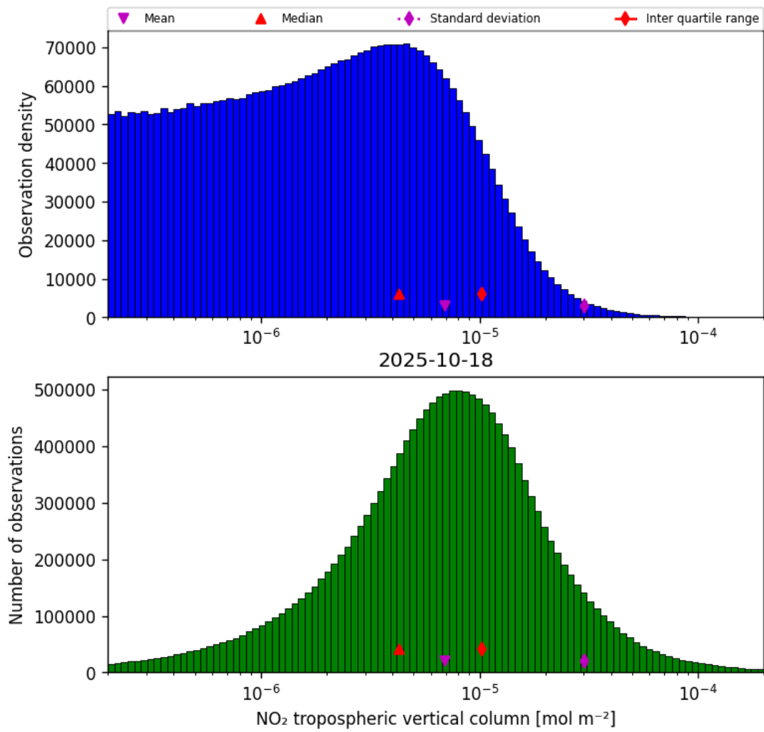
Figure 27: Histogram of “NO 2 tropospheric vertical column” for 2025-10-18 to 2025-10-19
