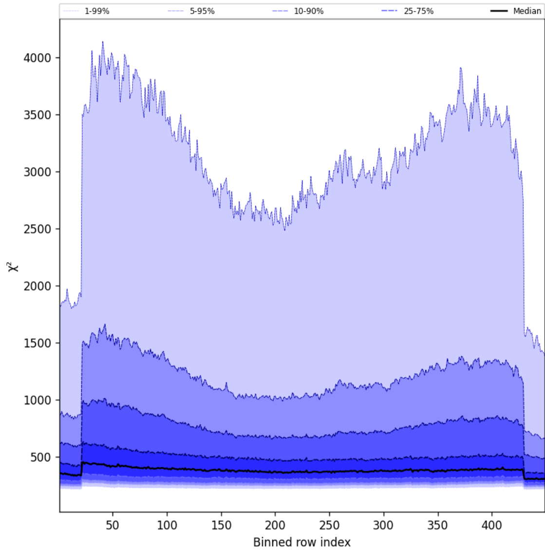
Figure 57: Along track statistics of “ \chi^2 ” for 2025-10-18 to 2025-10-19
