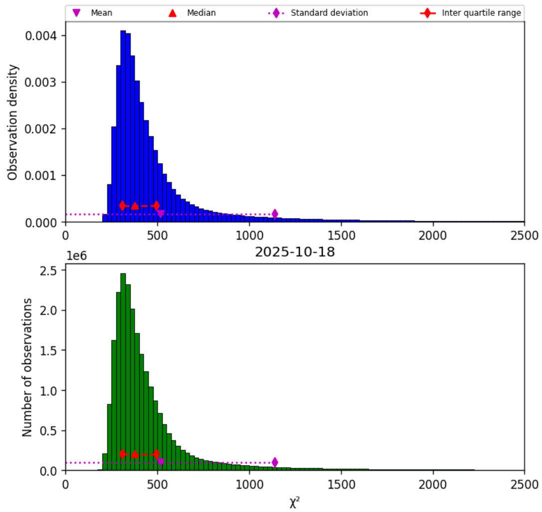
Figure 40: Histogram of “ \chi^2 ” for 2025-10-18 to 2025-10-19
