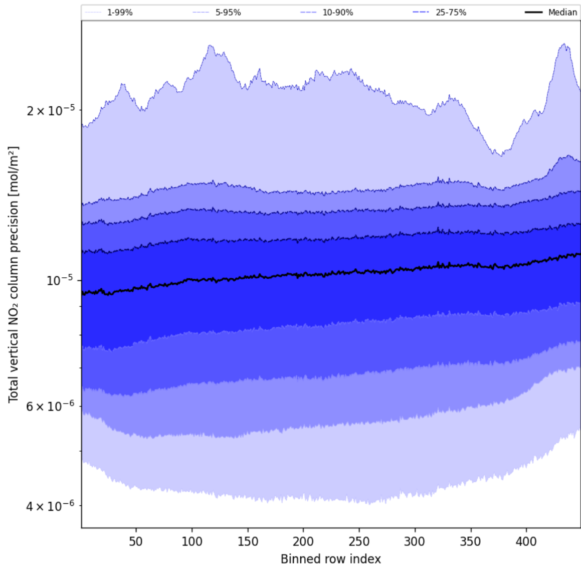
Figure 54: Along track statistics of "Total vertical NO 2 column precision" for 2025-10-18 to 2025-10-19
