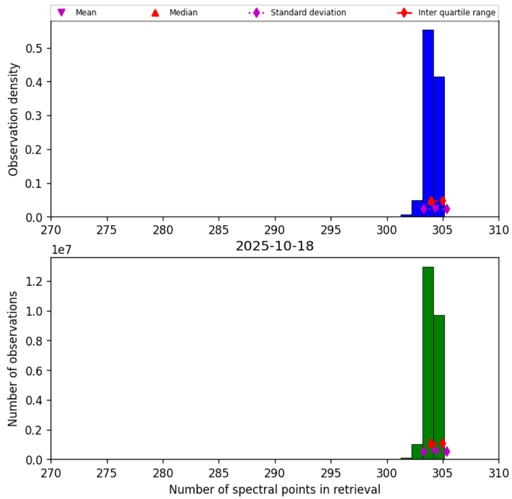
Figure 31: Histogram of “Number of spectral points in retrieval” for 2025-10-18 to 2025-10-19
