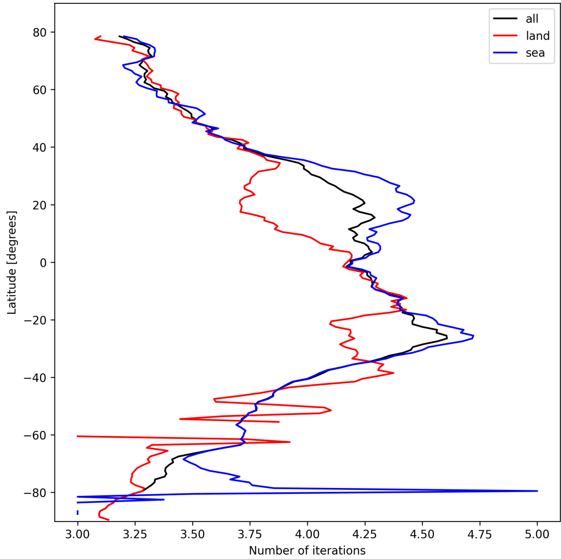
Figure 15: Zonal average of “Number of iterations” for 2025-10-18 to 2025-10-19.
