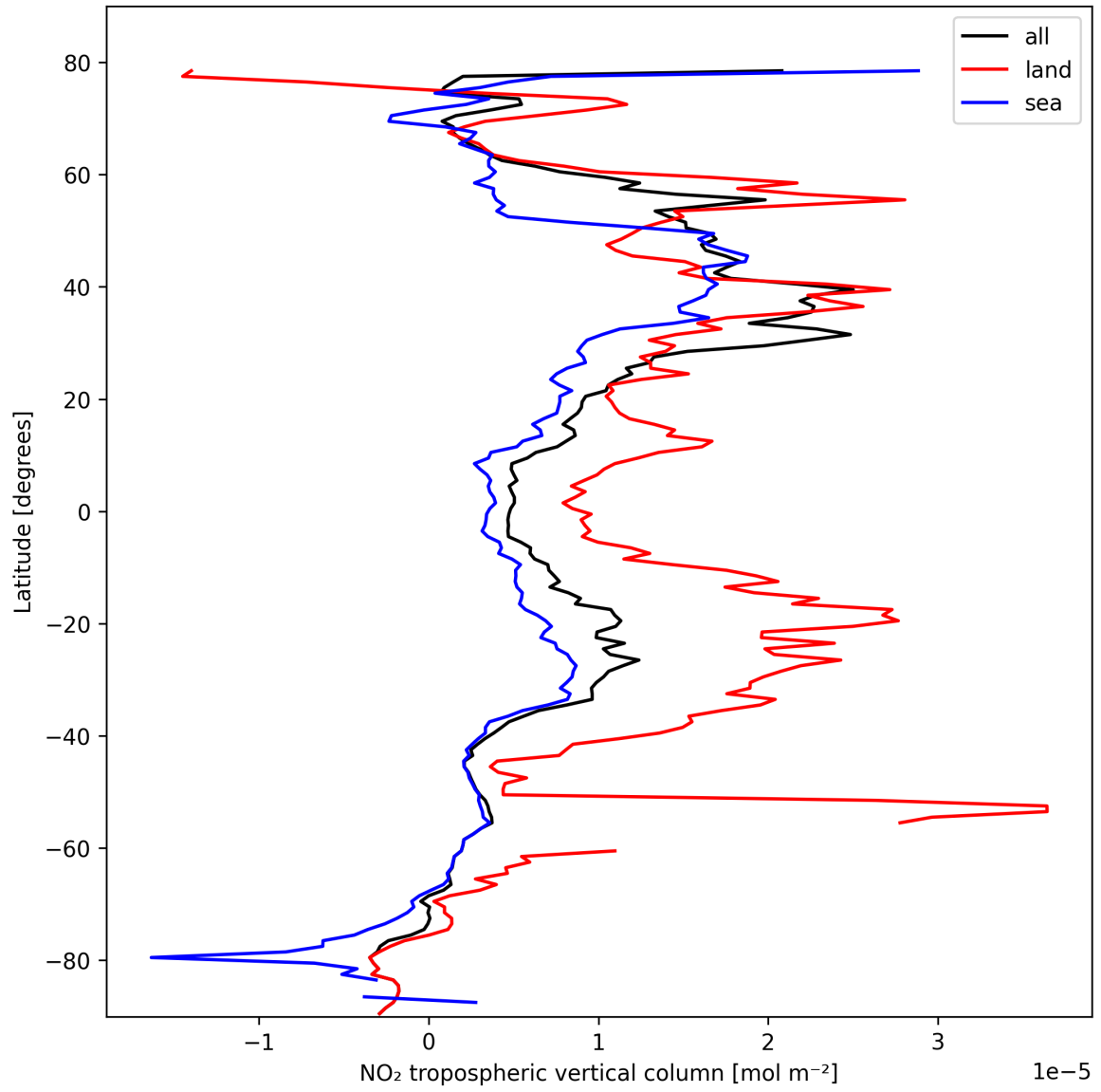
Figure 10: Zonal average of “NO 2 tropospheric vertical column” for 2025-10-18 to 2025-10-19.
