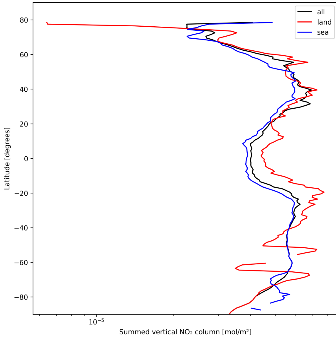
Figure 21: Zonal average of “Summed vertical NO 2 column” for 2025-10-18 to 2025-10-19.
