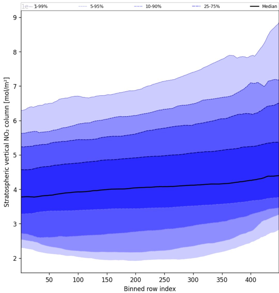
Figure 51: Along track statistics of “Stratospheric vertical NO 2 column” for 2025-10-18 to 2025-10-19
