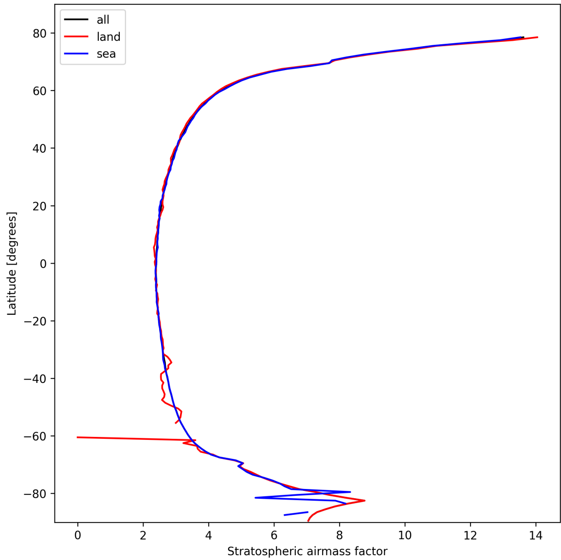
Figure 25: Zonal average of “Stratospheric airmass factor” for 2025-10-18 to 2025-10-19.
