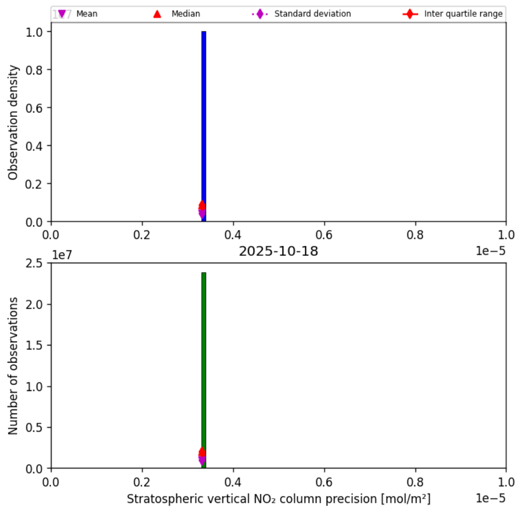
Figure 35: Histogram of “Stratospheric vertical NO 2 column precision” for 2025-10-18 to 2025-10-19
