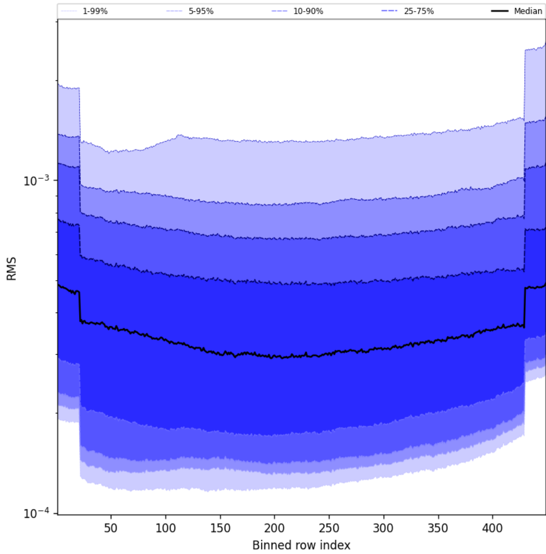
Figure 58: Along track statistics of “RMS” for 2025-10-18 to 2025-10-19
