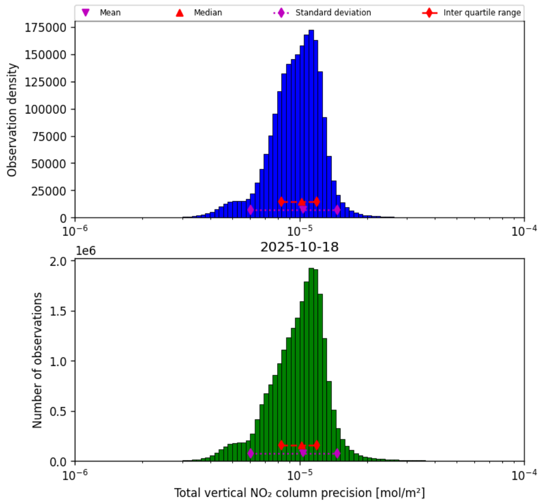
Figure 37: Histogram of "Total vertical NO 2 column precision" for 2025-10-18 to 2025-10-19
