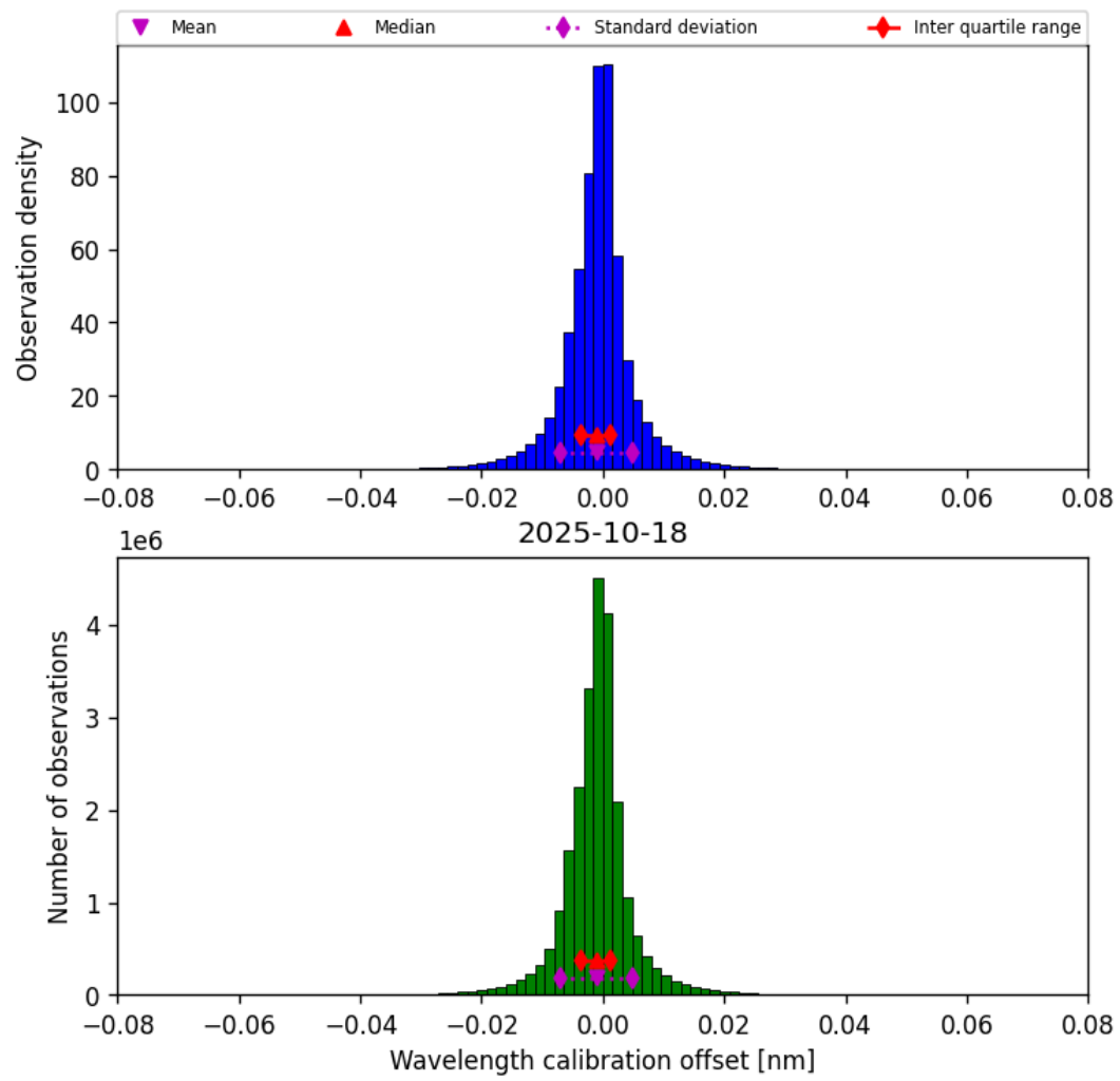
Figure 33: Histogram of “Wavelength calibration offset” for 2025-10-18 to 2025-10-19
