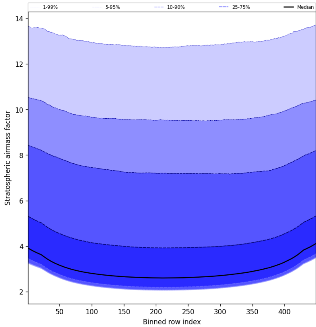
Figure 59: Along track statistics of “Stratospheric airmass factor” for 2025-10-18 to 2025-10-19
