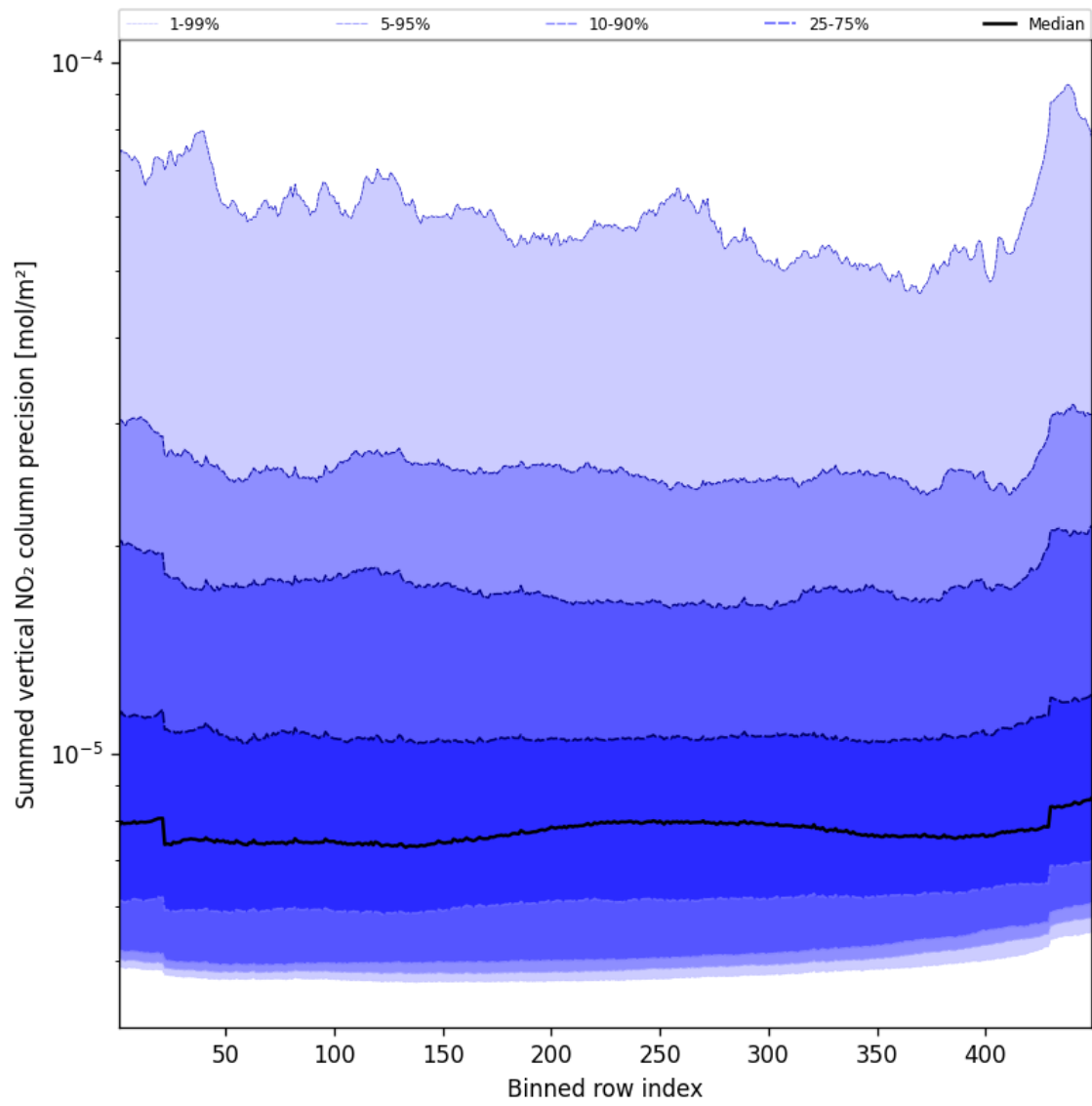
Figure 56: Along track statistics of “Summed vertical NO 2 column precision” for 2025-10-18 to 2025-10-19
