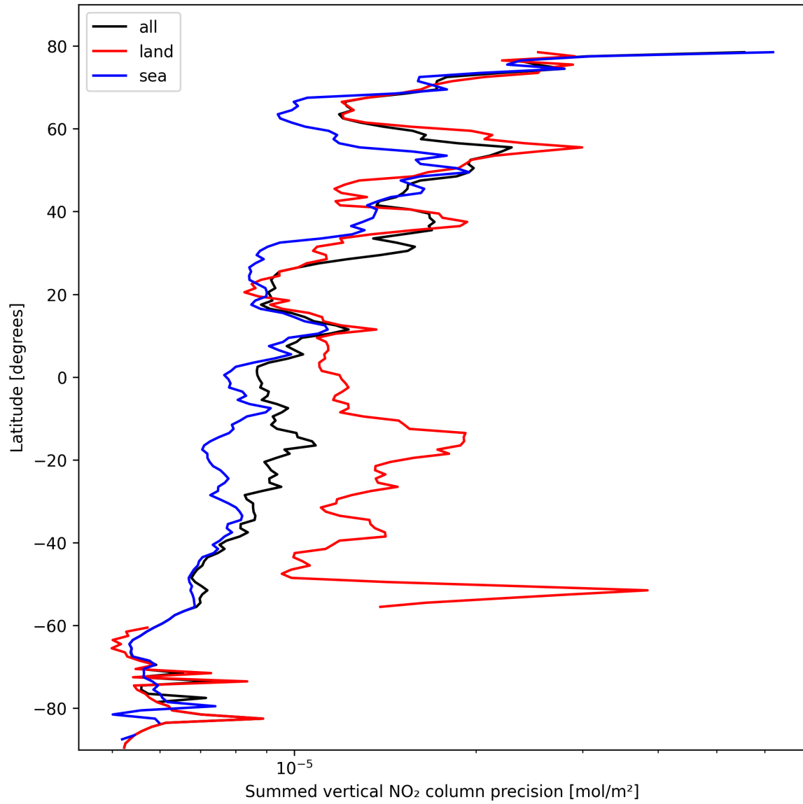
Figure 22: Zonal average of “Summed vertical NO 2 column precision” for 2025-10-18 to 2025-10-19.
