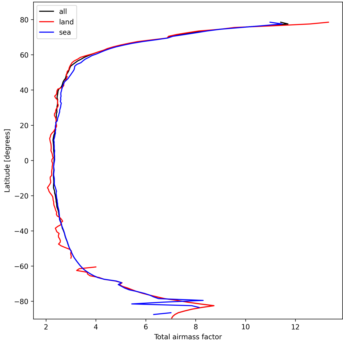
Figure 13: Zonal average of “Total airmass factor” for 2025-10-18 to 2025-10-19.
