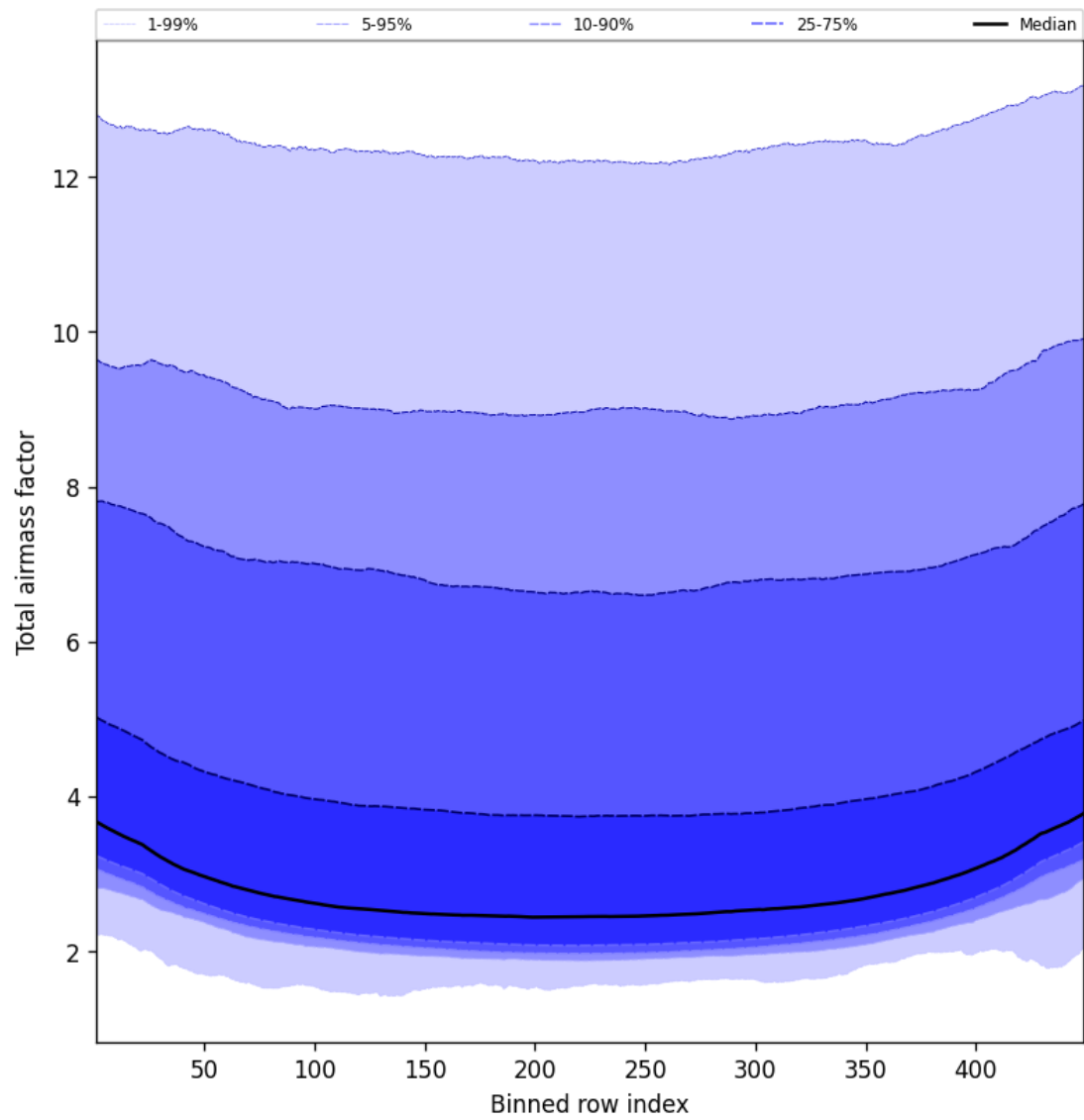
Figure 47: Along track statistics of “Total airmass factor” for 2025-10-18 to 2025-10-19
