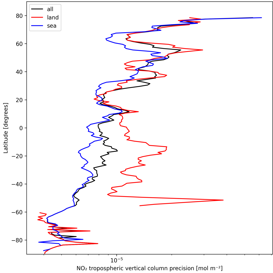
Figure 11: Zonal average of “NO 2 tropospheric vertical column precision” for 2025-10-18 to 2025-10-19.
