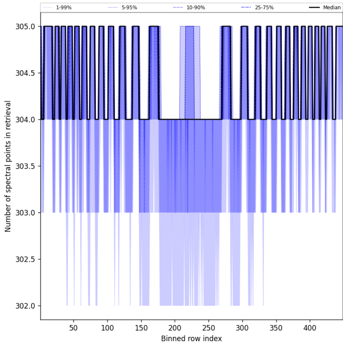
Figure 48: Along track statistics of “Number of spectral points in retrieval” for 2025-10-18 to 2025-10-19
