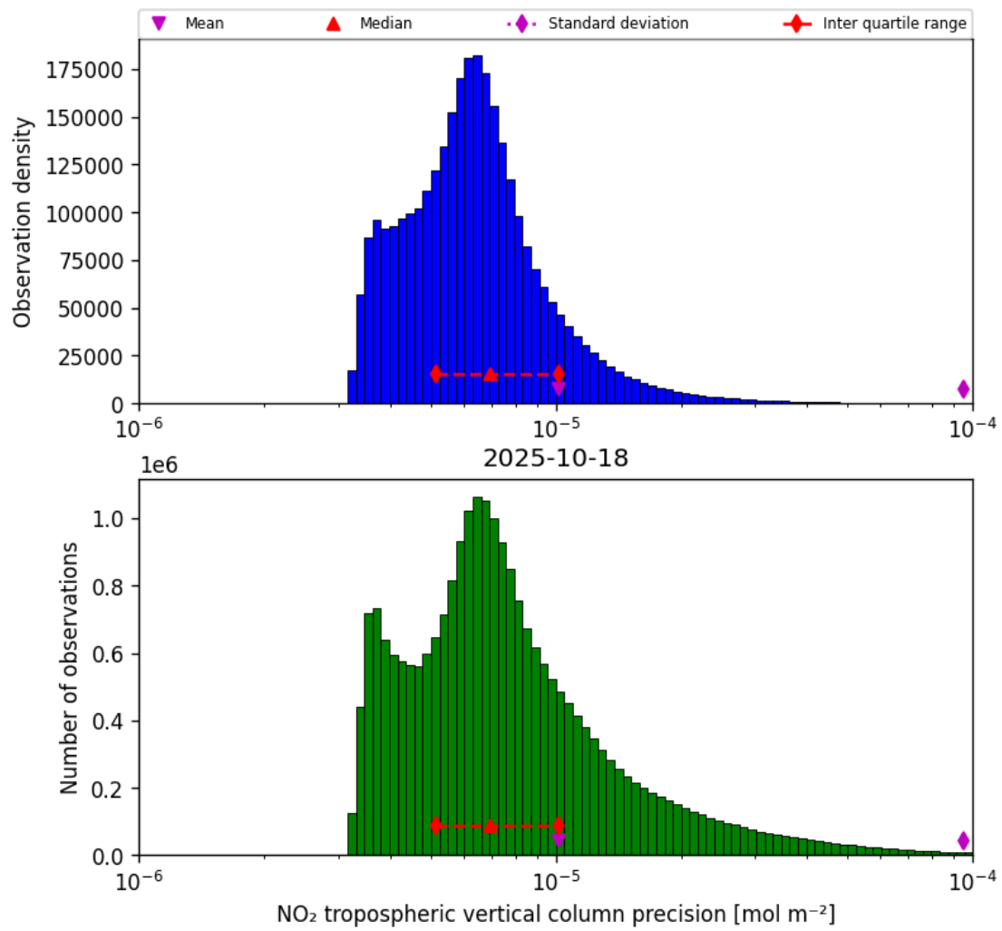
Figure 28: Histogram of “NO 2 tropospheric vertical column precision” for 2025-10-18 to 2025-10-19
