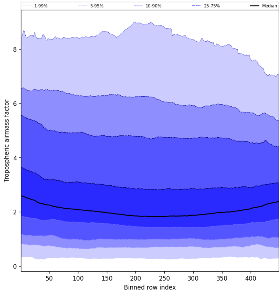
Figure 46: Along track statistics of “Tropospheric airmass factor” for 2025-10-18 to 2025-10-19
