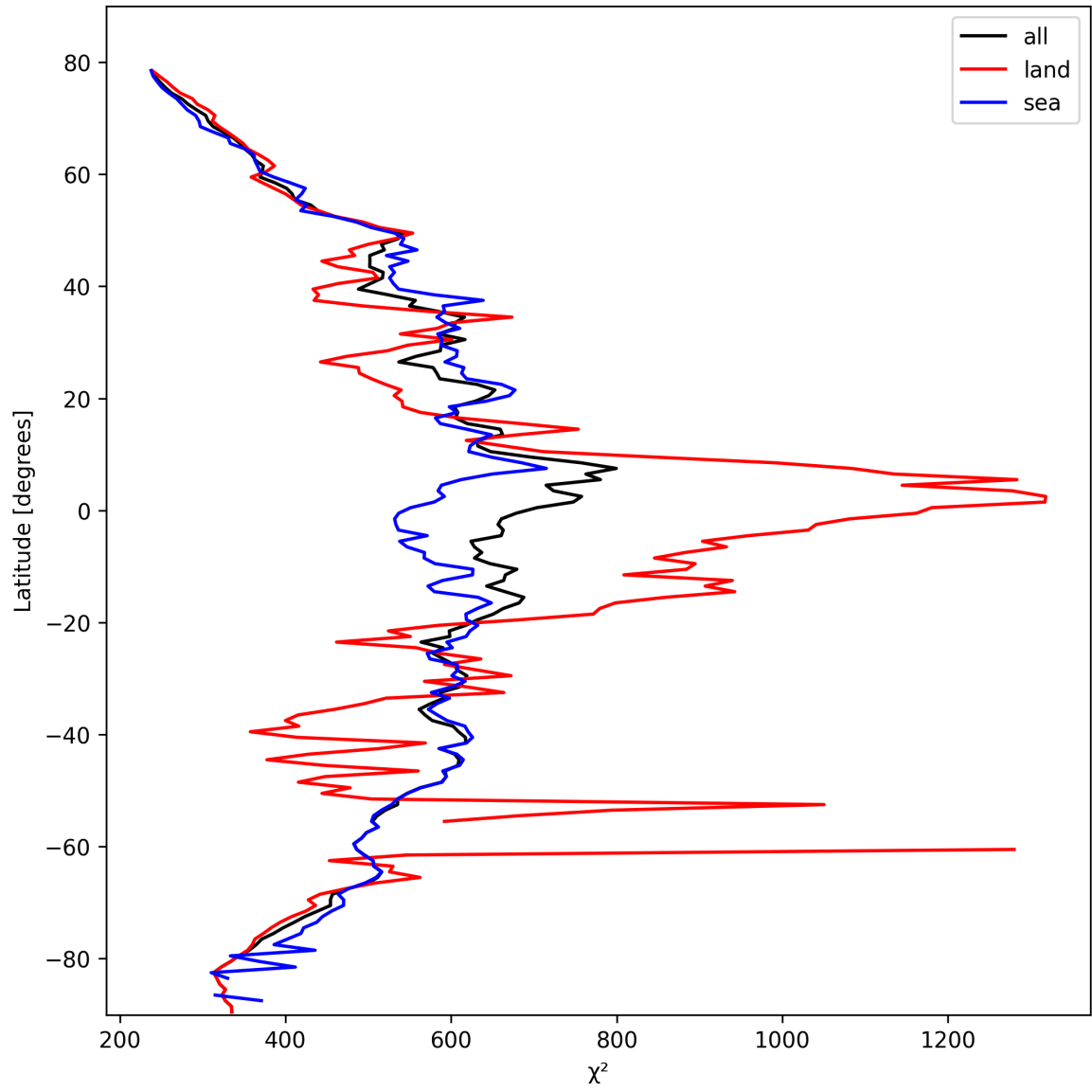
Figure 23: Zonal average of “ \chi^2 ” for 2025-10-18 to 2025-10-19.
