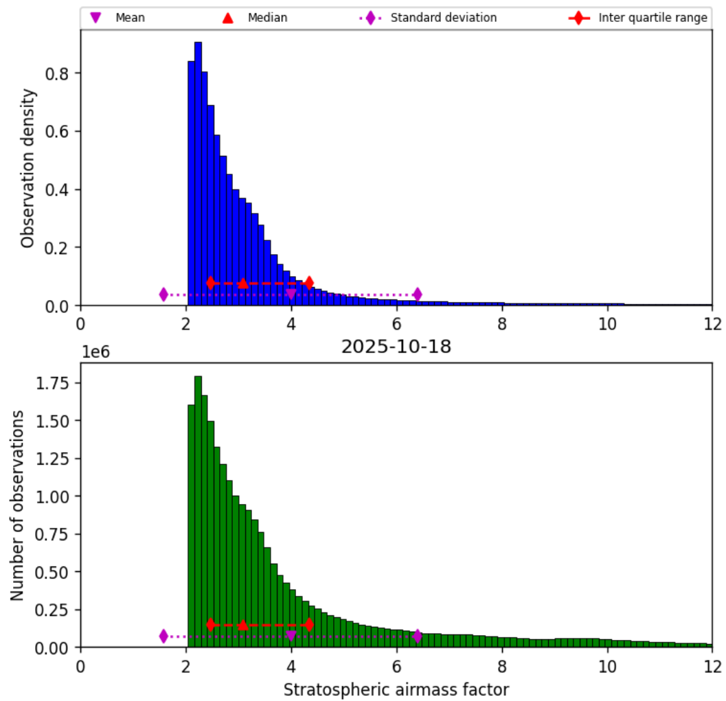
Figure 42: Histogram of “Stratospheric airmass factor” for 2025-10-18 to 2025-10-19
