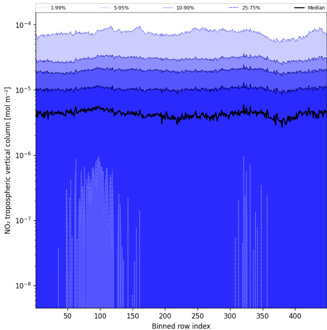
Figure 44: Along track statistics of “NO 2 tropospheric vertical column” for 2025-10-18 to 2025-10-19
