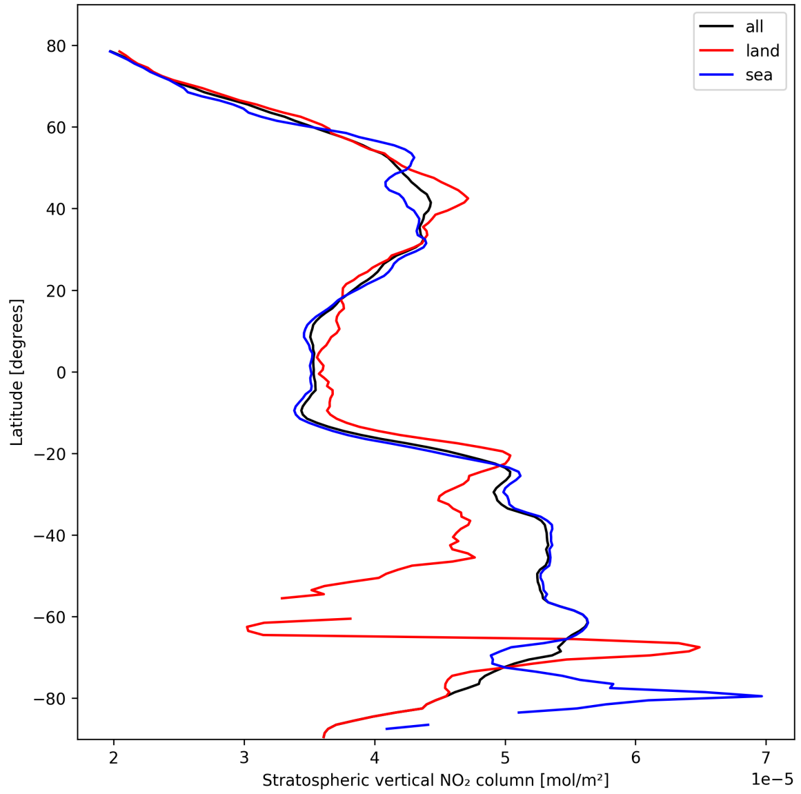
Figure 17: Zonal average of “Stratospheric vertical NO 2 column” for 2025-10-18 to 2025-10-19.
