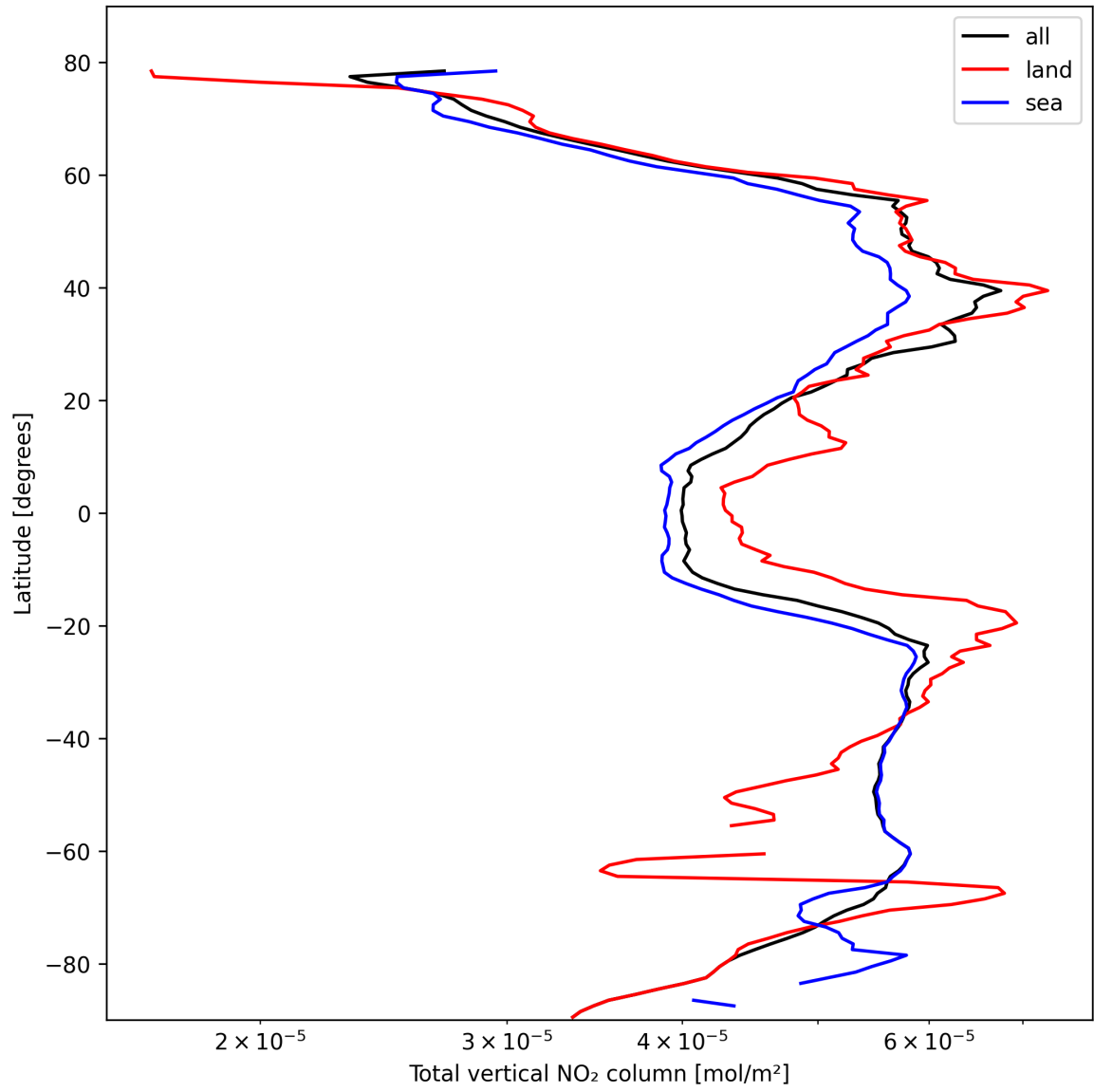
Figure 19: Zonal average of “Total vertical NO 2 column” for 2025-10-18 to 2025-10-19.
