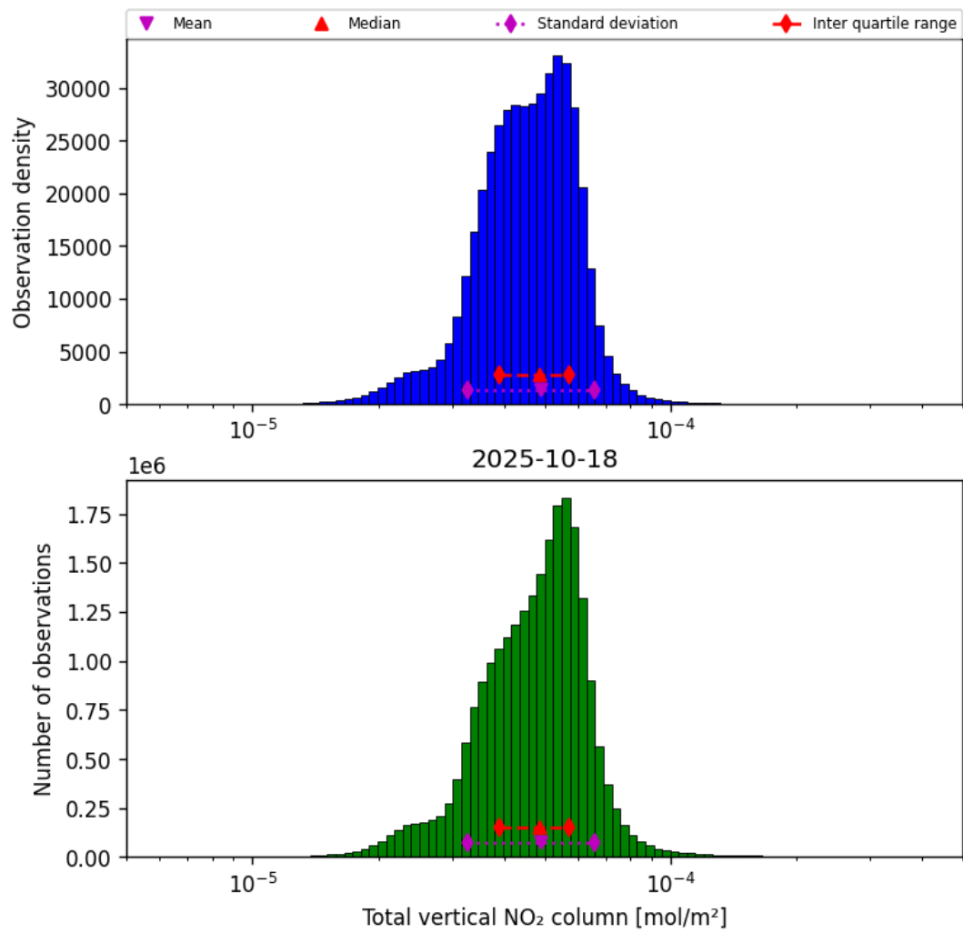
Figure 36: Histogram of “Total vertical NO 2 column” for 2025-10-18 to 2025-10-19
