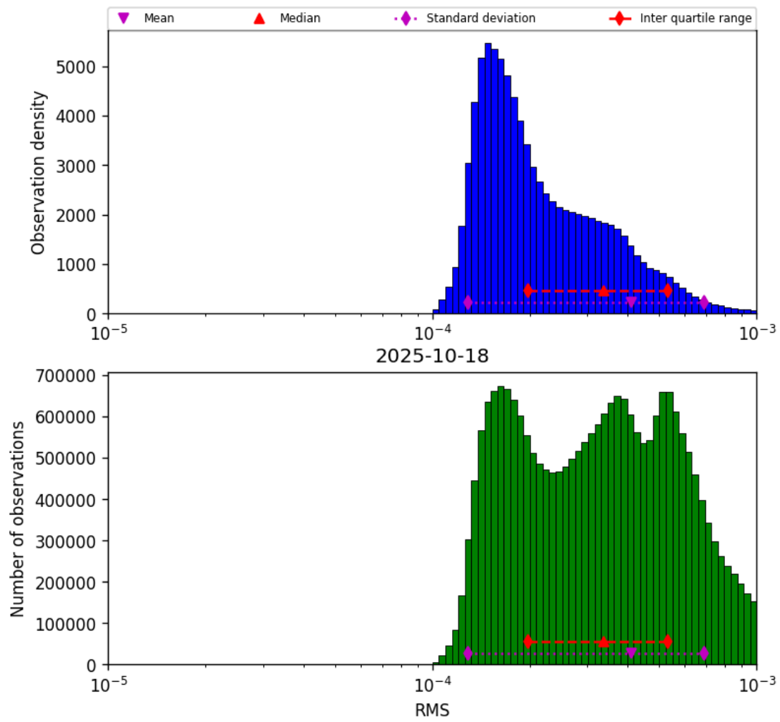
Figure 41: Histogram of “RMS” for 2025-10-18 to 2025-10-19
