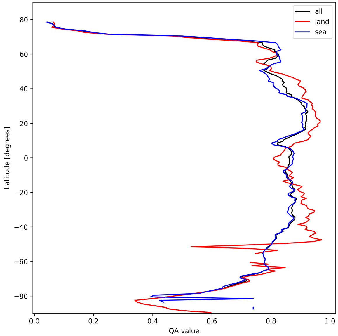
Figure 9: Zonal average of “QA value” for 2025-10-18 to 2025-10-19.
