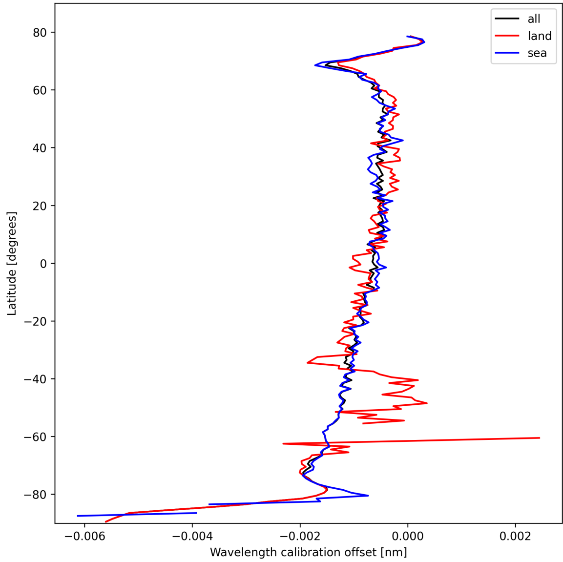
Figure 16: Zonal average of “Wavelength calibration offset” for 2025-10-18 to 2025-10-19.
