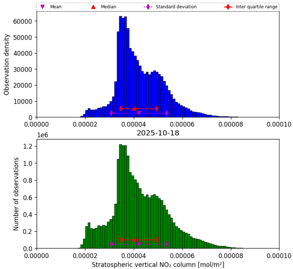
Figure 34: Histogram of “Stratospheric vertical NO 2 column” for 2025-10-18 to 2025-10-19
