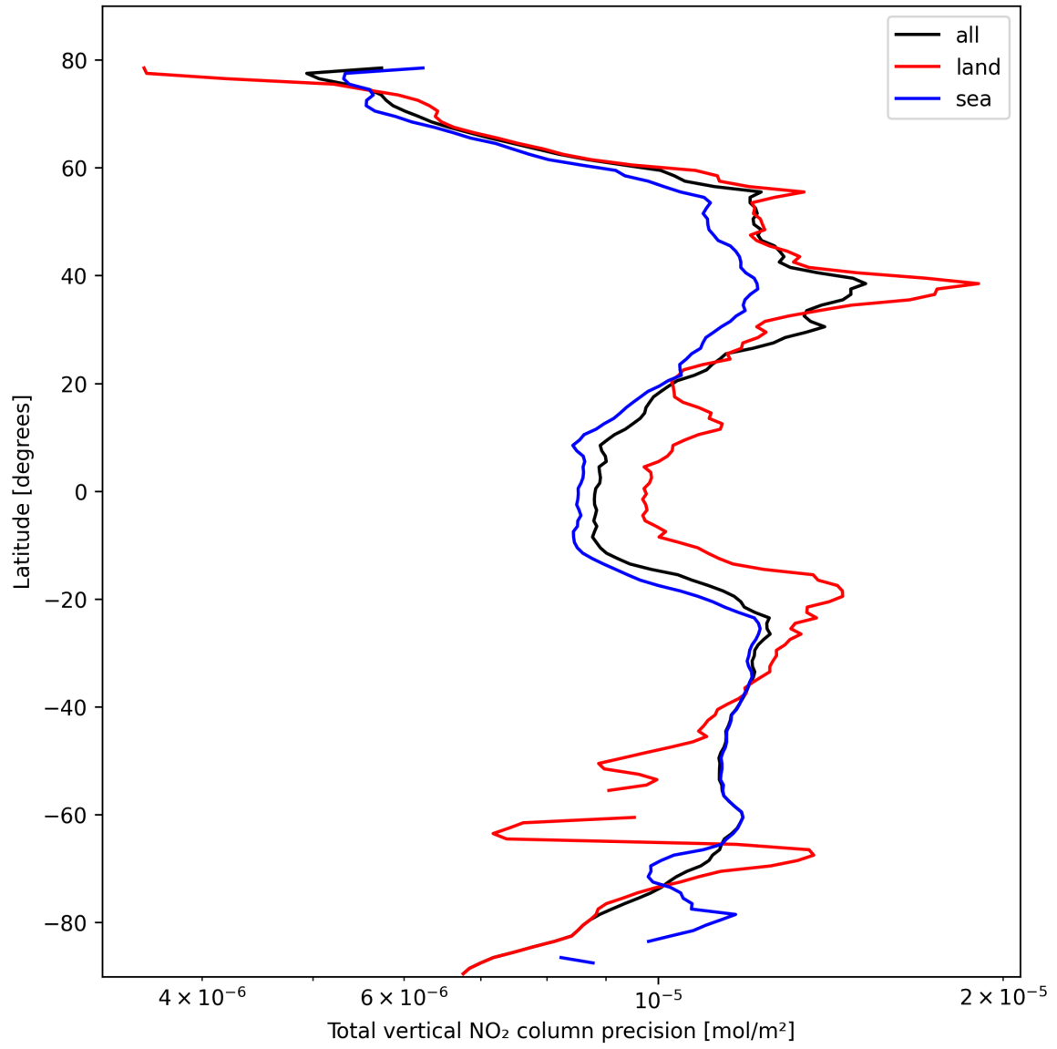
Figure 20: Zonal average of “Total vertical NO 2 column precision” for 2025-10-18 to 2025-10-19.
