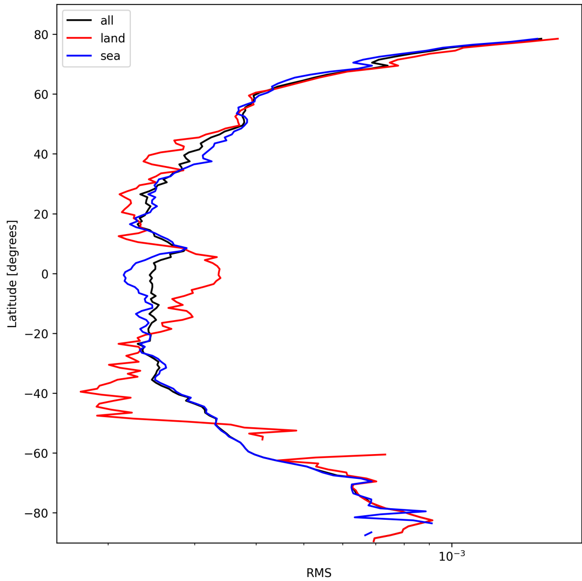
Figure 24: Zonal average of “RMS” for 2025-10-18 to 2025-10-19.
