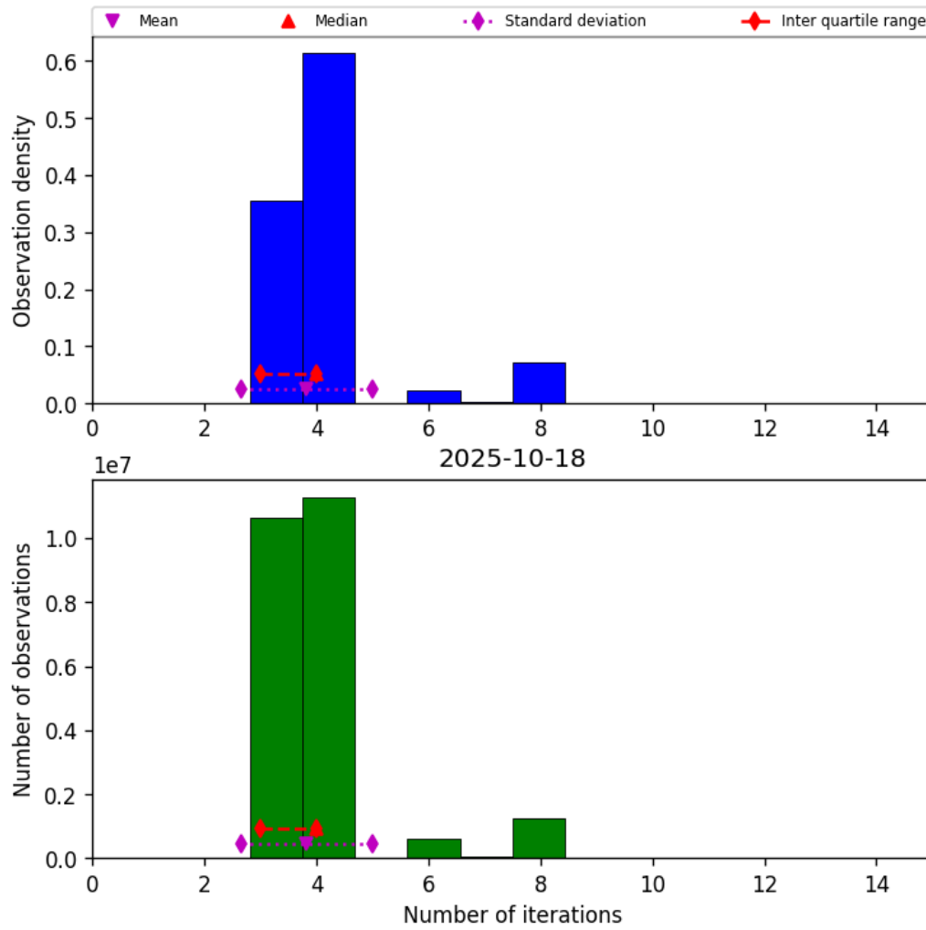
Figure 32: Histogram of “Number of iterations” for 2025-10-18 to 2025-10-19
