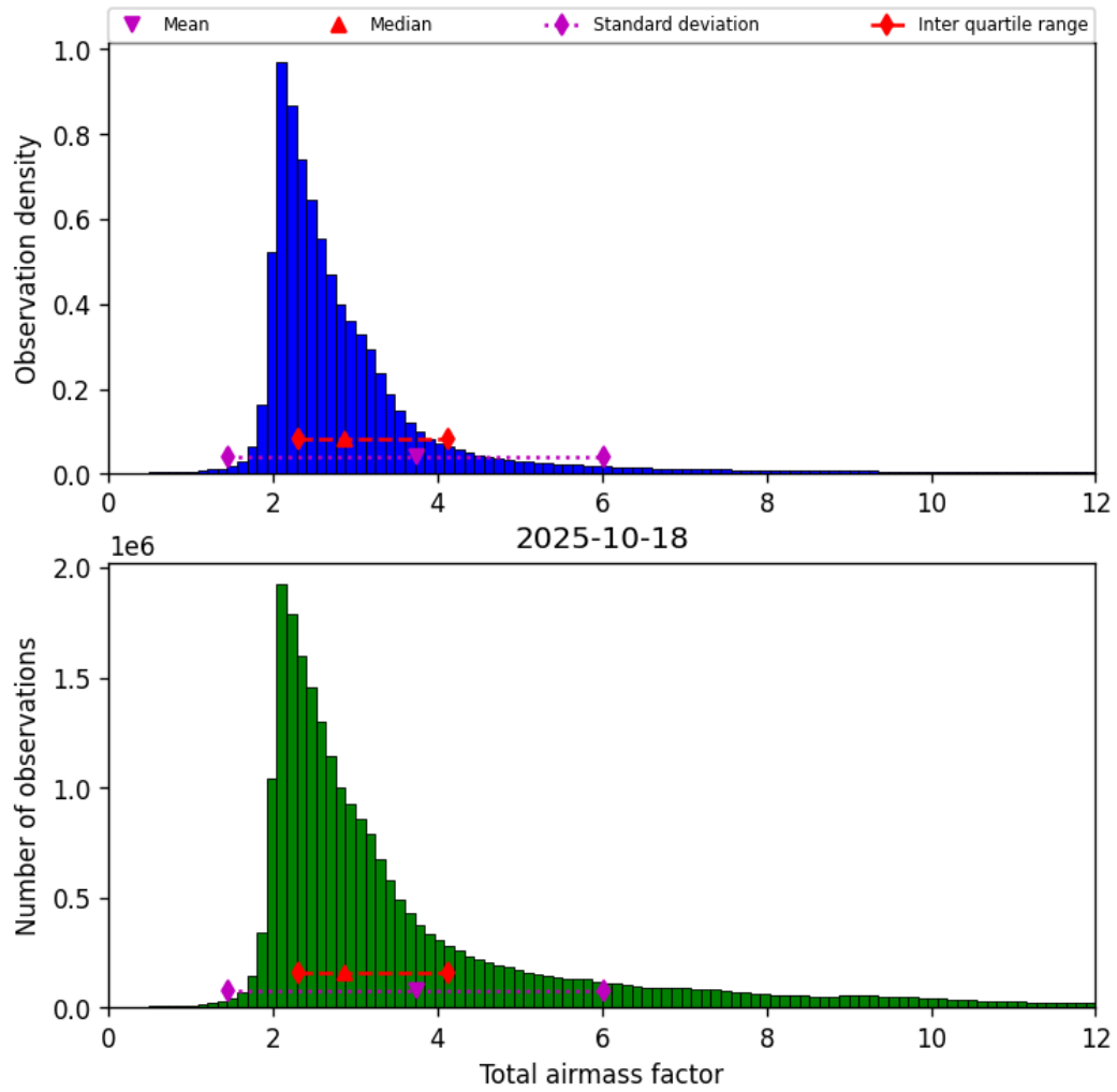
Figure 30: Histogram of “Total airmass factor” for 2025-10-18 to 2025-10-19
