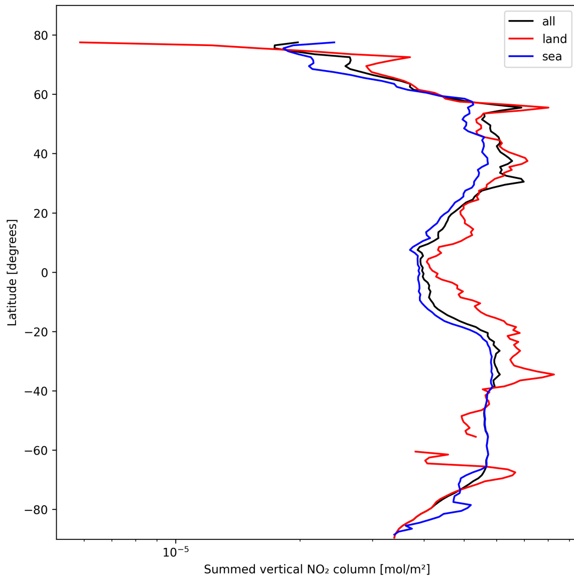
Figure 21: Zonal average of “Summed vertical NO 2 column” for 2025-10-19 to 2025-10-20.
