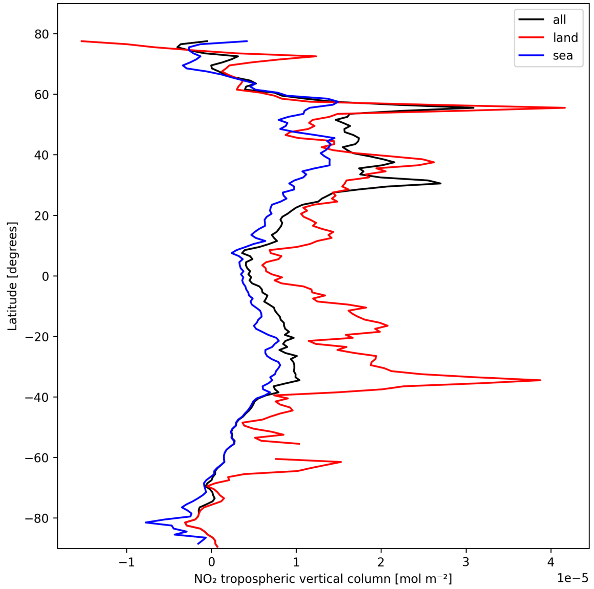
Figure 10: Zonal average of “NO 2 tropospheric vertical column” for 2025-10-19 to 2025-10-20.
