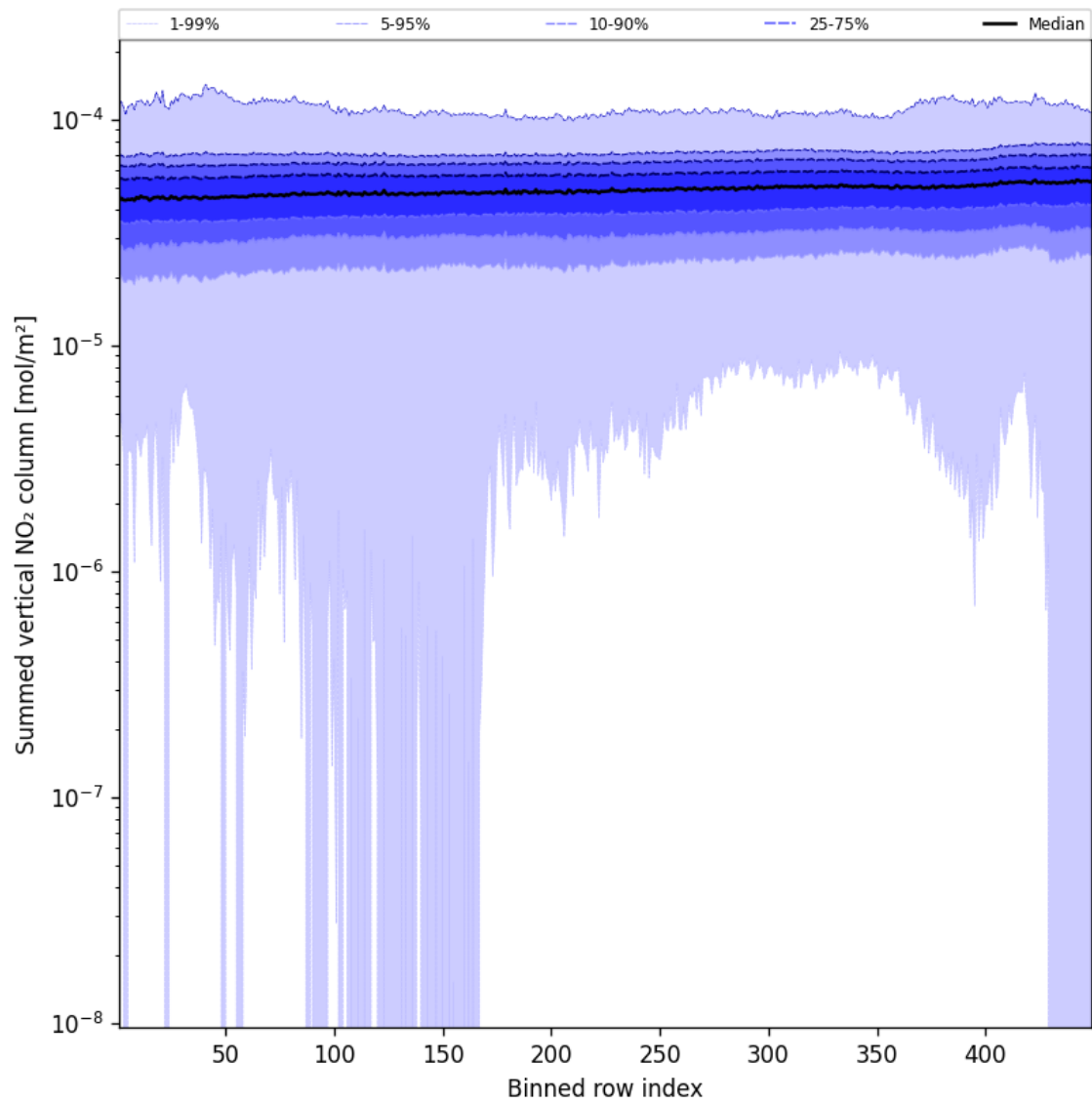
Figure 55: Along track statistics of “Summed vertical NO 2 column” for 2025-10-19 to 2025-10-20
