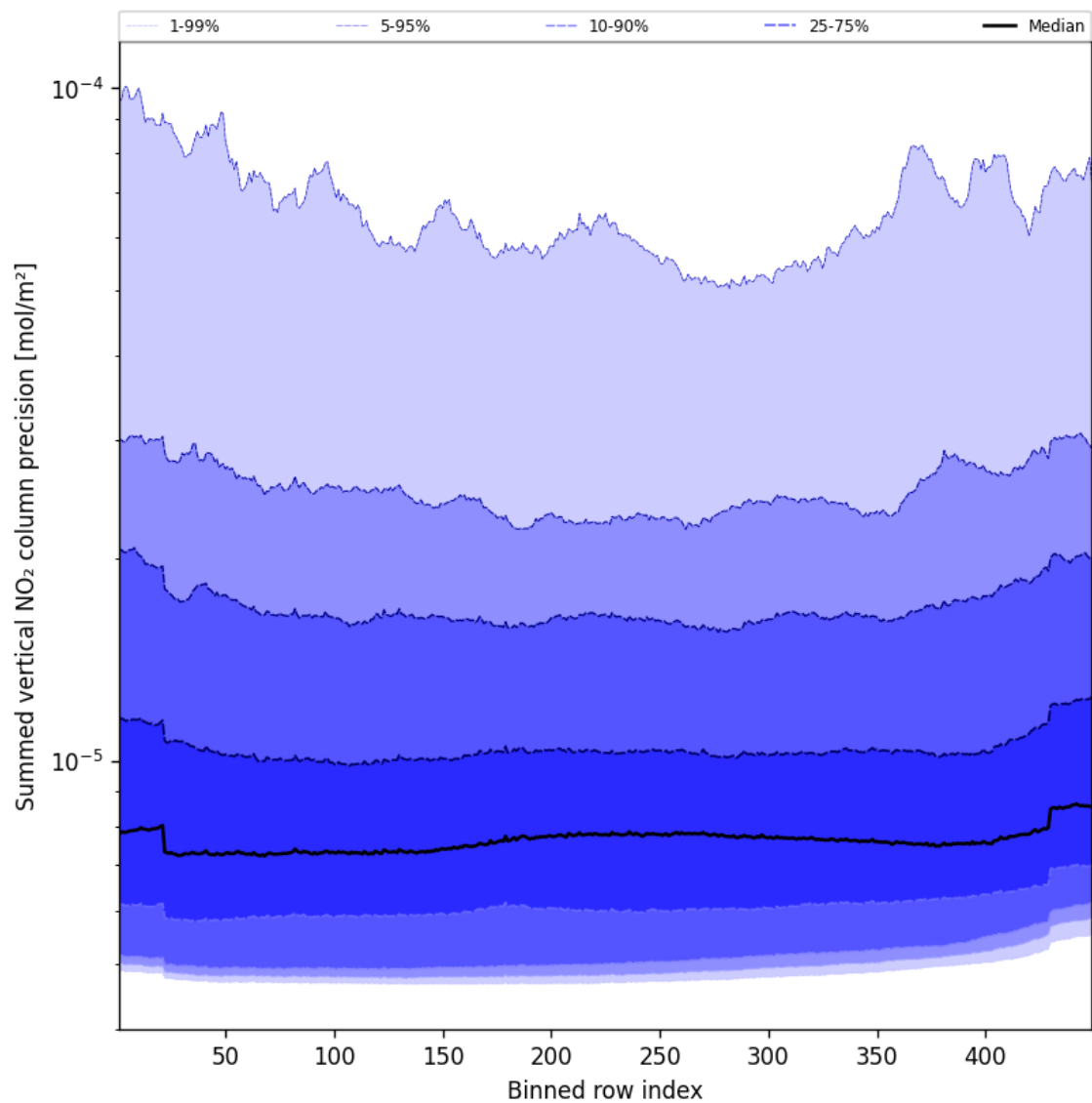
Figure 56: Along track statistics of “Summed vertical NO 2 column precision” for 2025-10-19 to 2025-10-20
