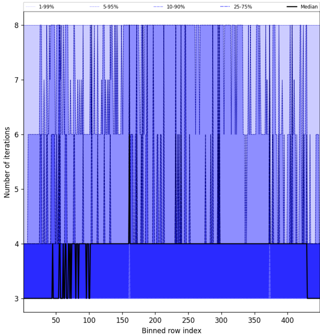
Figure 49: Along track statistics of “Number of iterations” for 2025-10-19 to 2025-10-20
