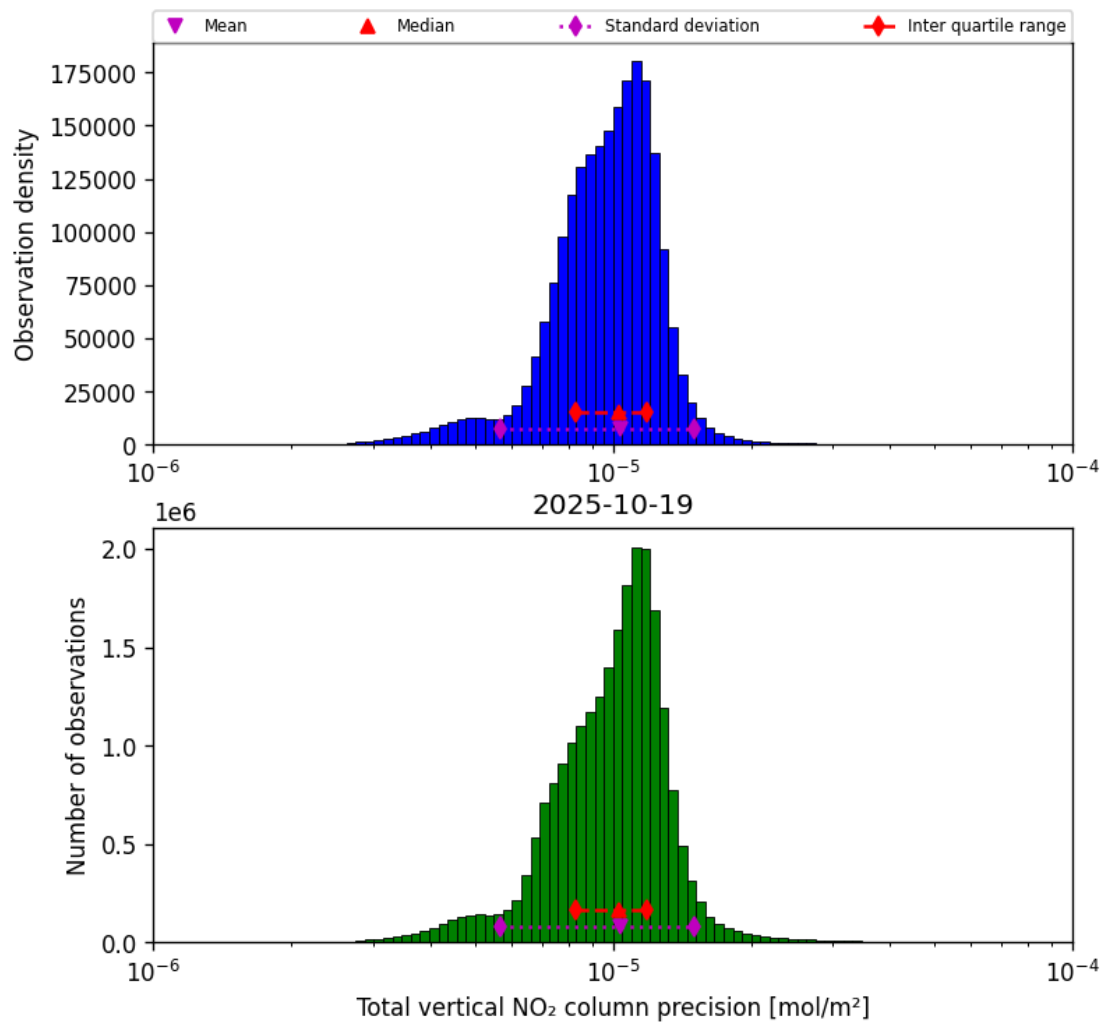
Figure 37: Histogram of "Total vertical NO 2 column precision" for 2025-10-19 to 2025-10-20
