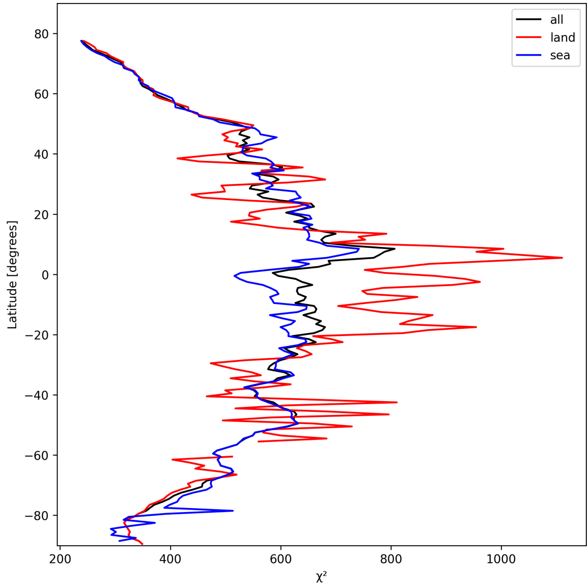
Figure 23: Zonal average of “ \chi^2 ” for 2025-10-19 to 2025-10-20.
