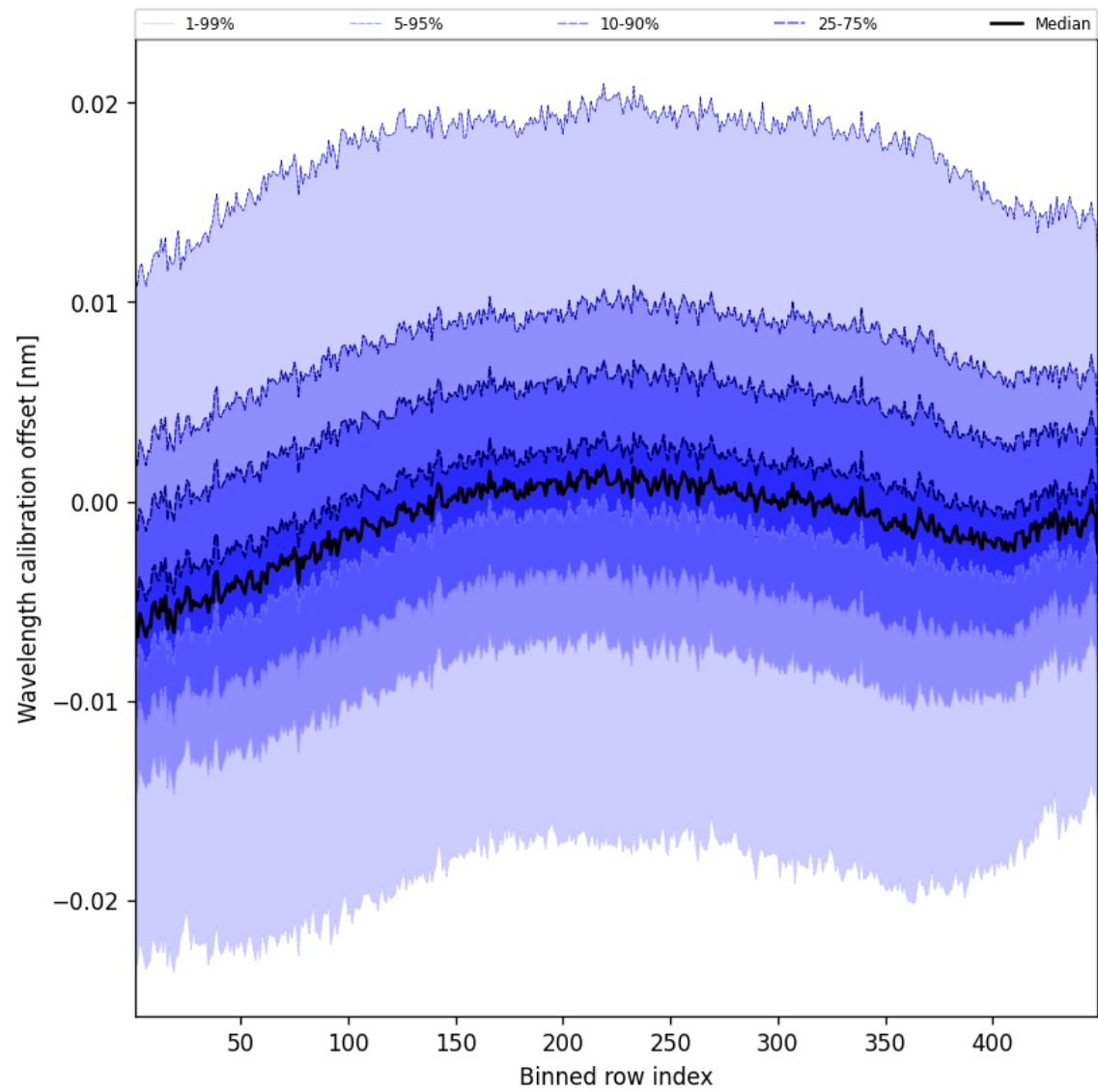
Figure 50: Along track statistics of “Wavelength calibration offset” for 2025-10-19 to 2025-10-20
