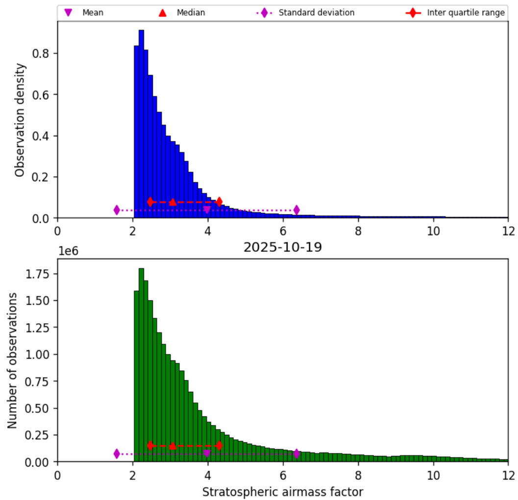
Figure 42: Histogram of “Stratospheric airmass factor” for 2025-10-19 to 2025-10-20
