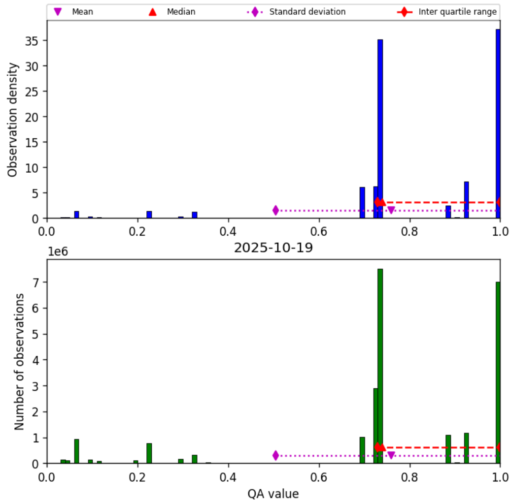
Figure 26: Histogram of “QA value” for 2025-10-19 to 2025-10-20
