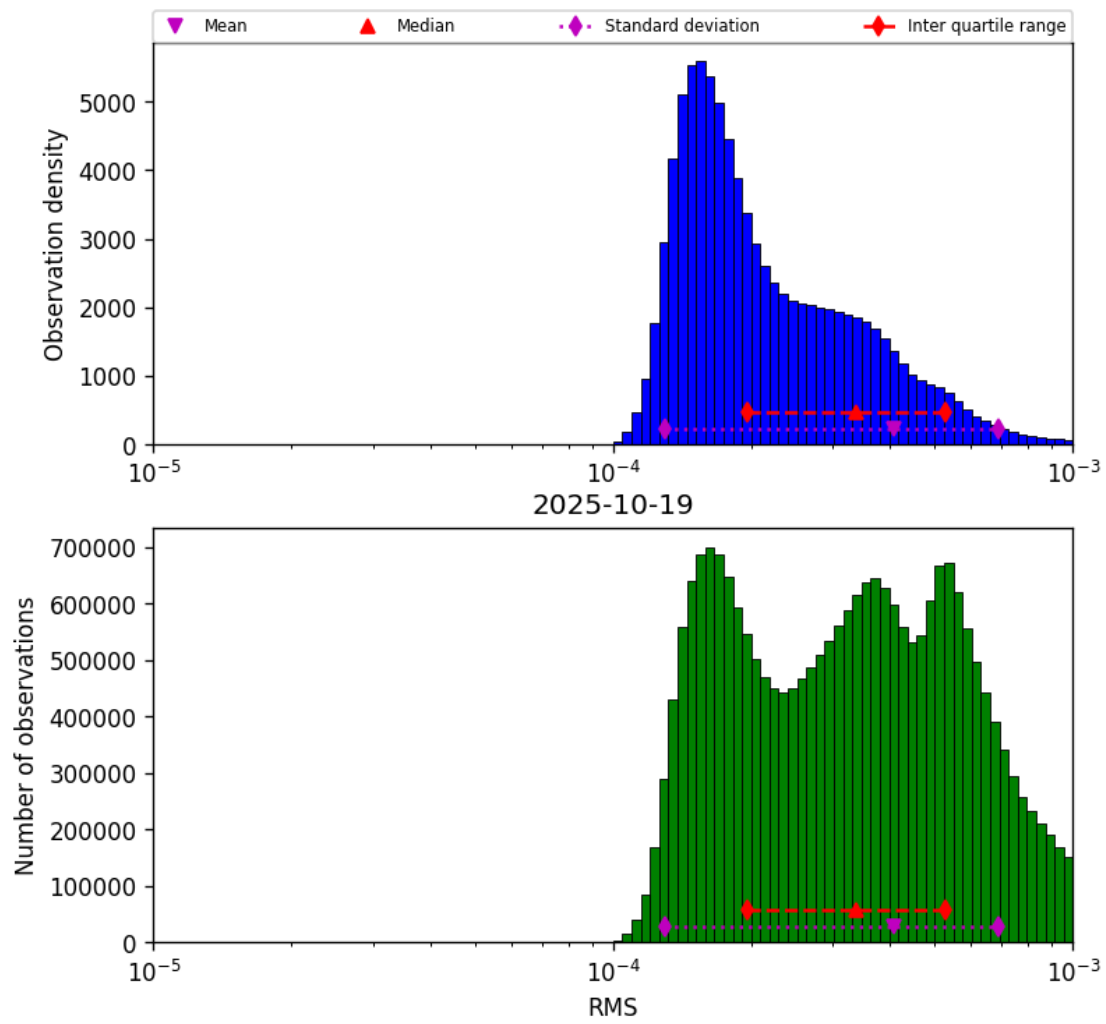
Figure 41: Histogram of “RMS” for 2025-10-19 to 2025-10-20
