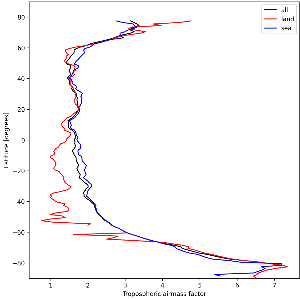
Figure 12: Zonal average of “Tropospheric airmass factor” for 2025-10-19 to 2025-10-20.
