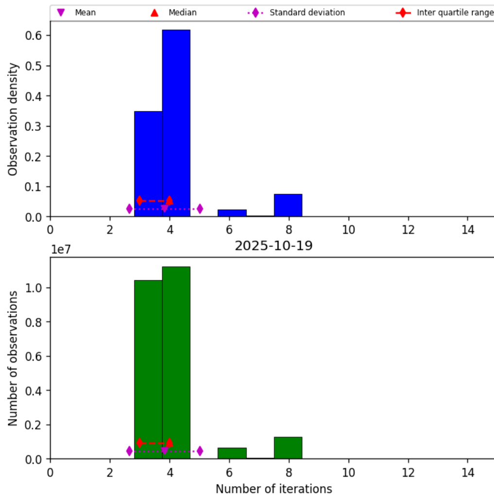
Figure 32: Histogram of “Number of iterations” for 2025-10-19 to 2025-10-20
