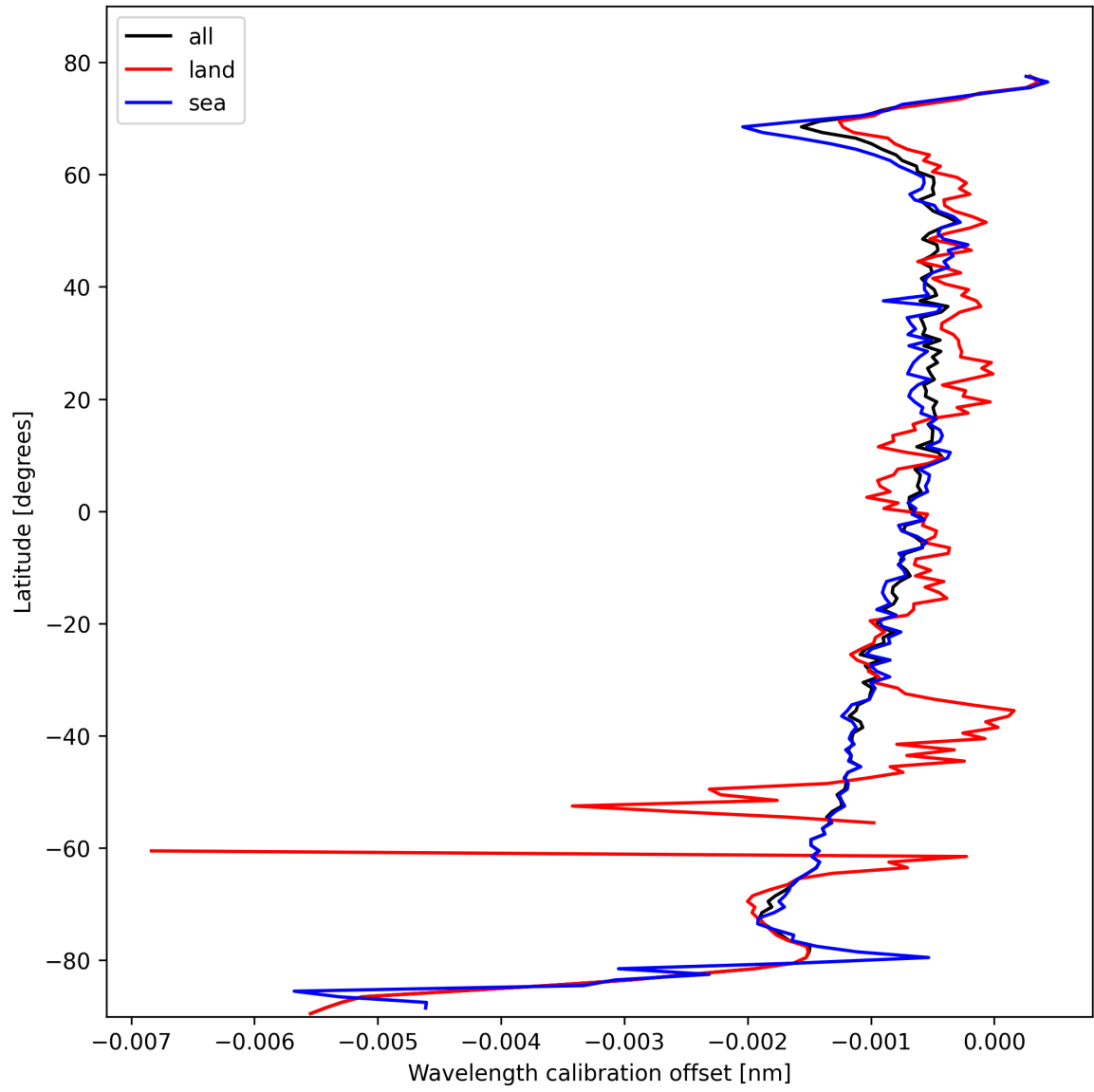
Figure 16: Zonal average of “Wavelength calibration offset” for 2025-10-19 to 2025-10-20.
