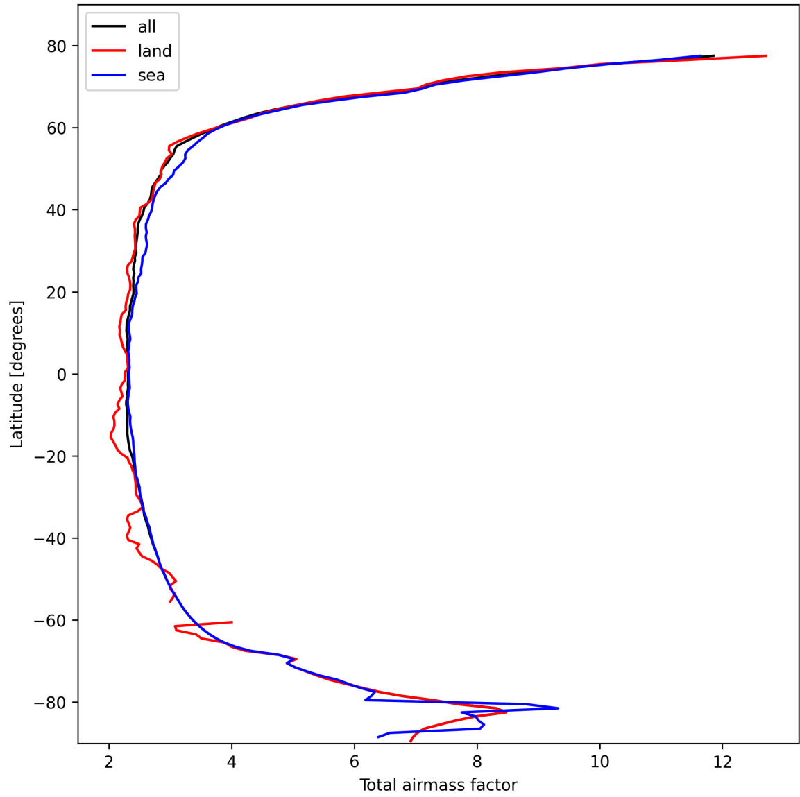
Figure 13: Zonal average of “Total airmass factor” for 2025-10-19 to 2025-10-20.
