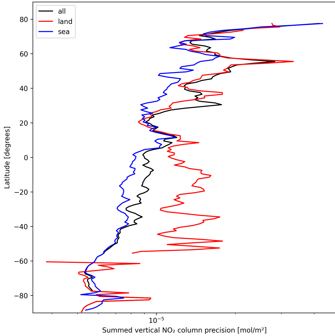
Figure 22: Zonal average of “Summed vertical NO 2 column precision” for 2025-10-19 to 2025-10-20.
