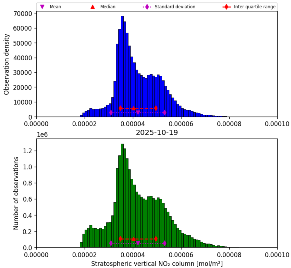
Figure 34: Histogram of “Stratospheric vertical NO 2 column” for 2025-10-19 to 2025-10-20
