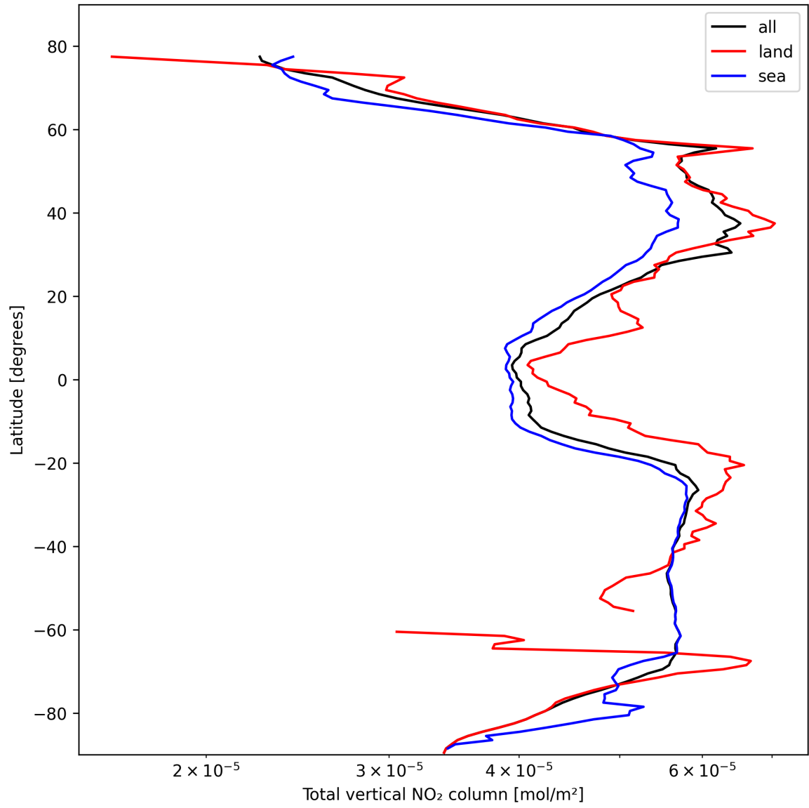
Figure 19: Zonal average of “Total vertical NO 2 column” for 2025-10-19 to 2025-10-20.
