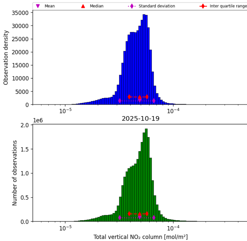
Figure 36: Histogram of “Total vertical NO 2 column” for 2025-10-19 to 2025-10-20
