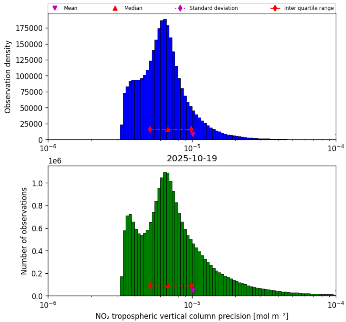
Figure 28: Histogram of “NO 2 tropospheric vertical column precision” for 2025-10-19 to 2025-10-20
