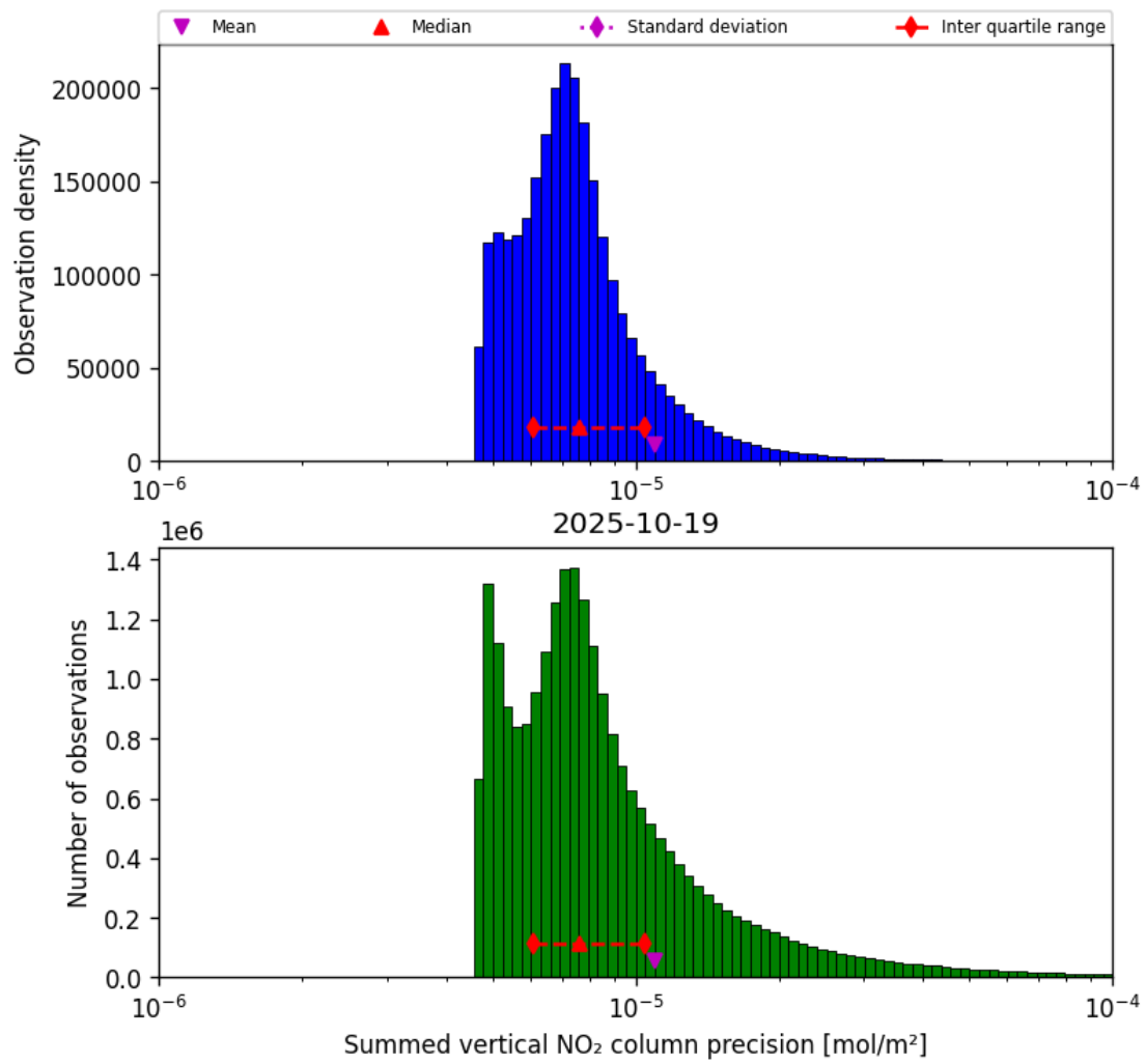
Figure 39: Histogram of "Summed vertical NO 2 column precision" for 2025-10-19 to 2025-10-20
