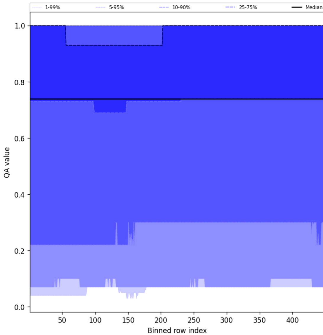
Figure 43: Along track statistics of "QA value" for 2025-10-19 to 2025-10-20
