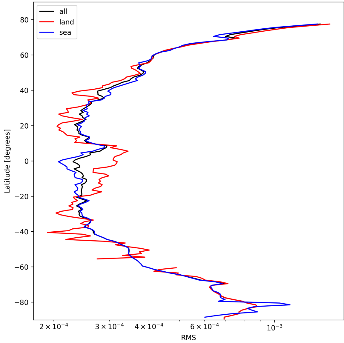
Figure 24: Zonal average of “RMS” for 2025-10-19 to 2025-10-20.
