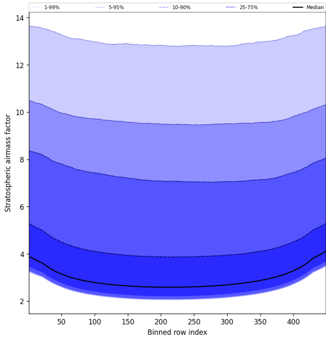
Figure 59: Along track statistics of “Stratospheric air mass factor” for 2025-10-19 to 2025-10-20
