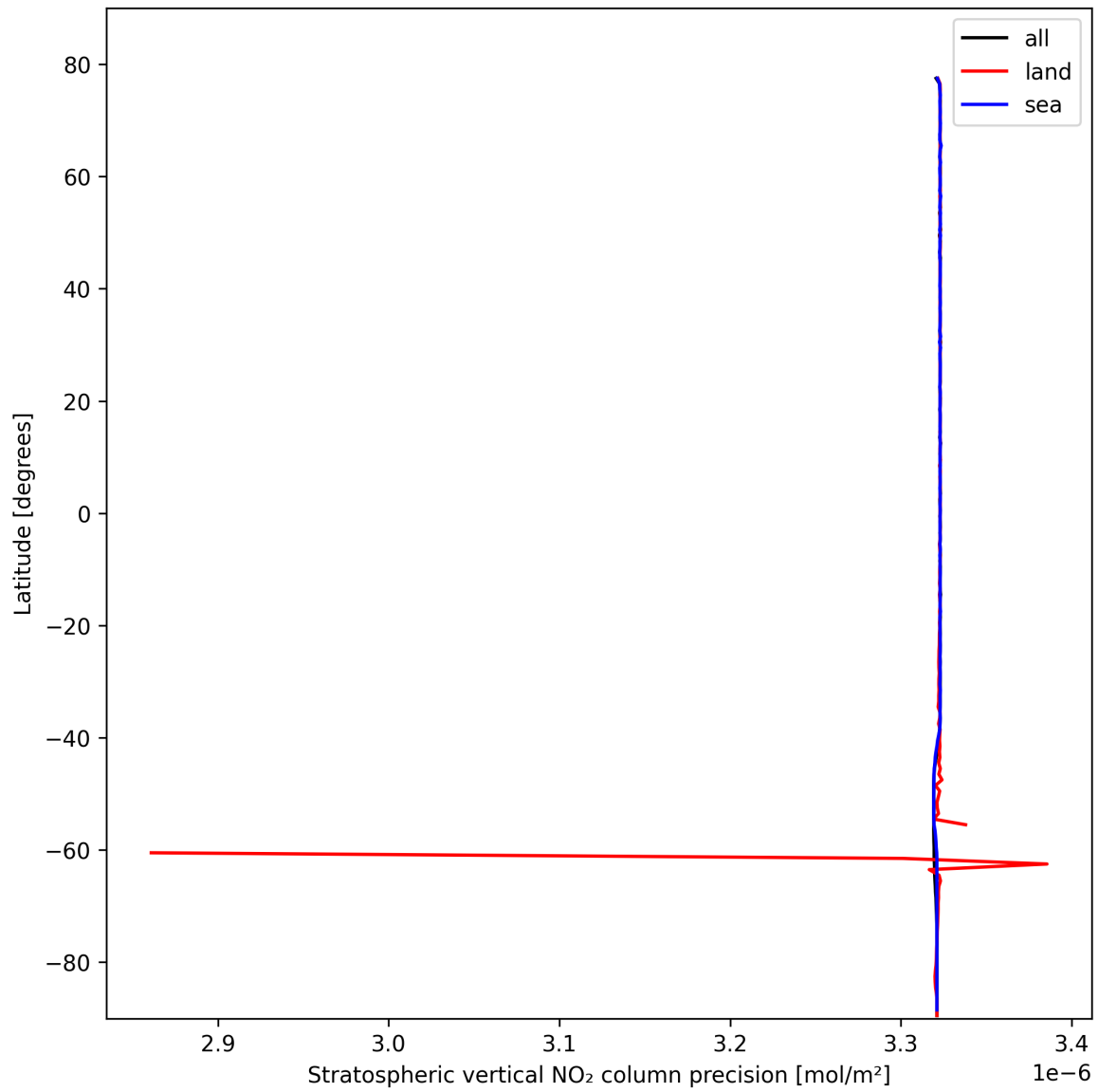
Figure 18: Zonal average of “Stratospheric vertical NO 2 column precision” for 2025-10-19 to 2025-10-20.
