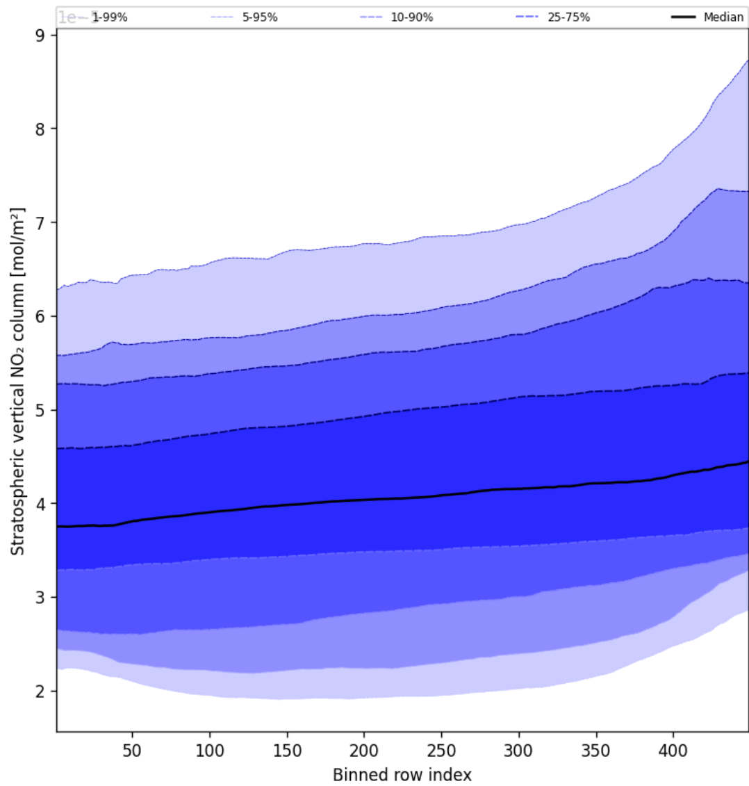
Figure 51: Along track statistics of “Stratospheric vertical NO 2 column” for 2025-10-19 to 2025-10-20
