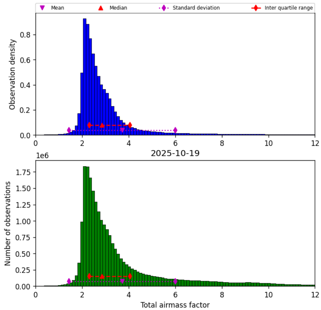
Figure 30: Histogram of “Total airmass factor” for 2025-10-19 to 2025-10-20
