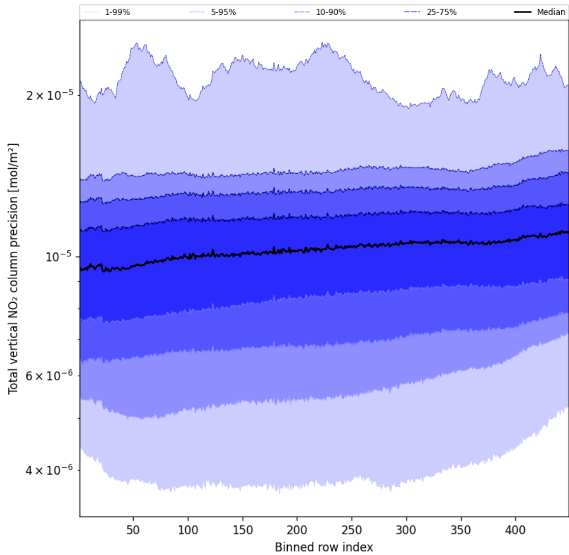
Figure 54: Along track statistics of "Total vertical NO 2 column precision" for 2025-10-19 to 2025-10-20
