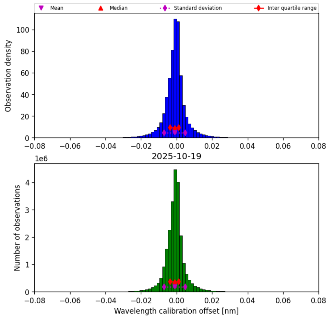
Figure 33: Histogram of “Wavelength calibration offset” for 2025-10-19 to 2025-10-20
