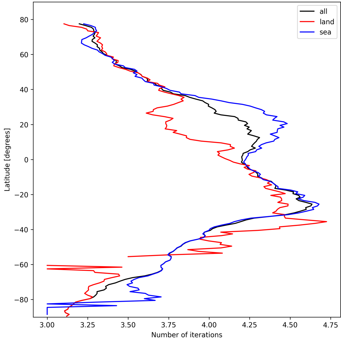
Figure 15: Zonal average of “Number of iterations” for 2025-10-19 to 2025-10-20.
