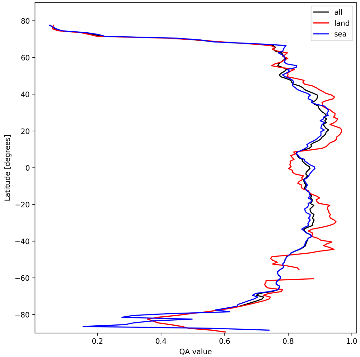
Figure 9: Zonal average of “QA value” for 2025-10-19 to 2025-10-20.
