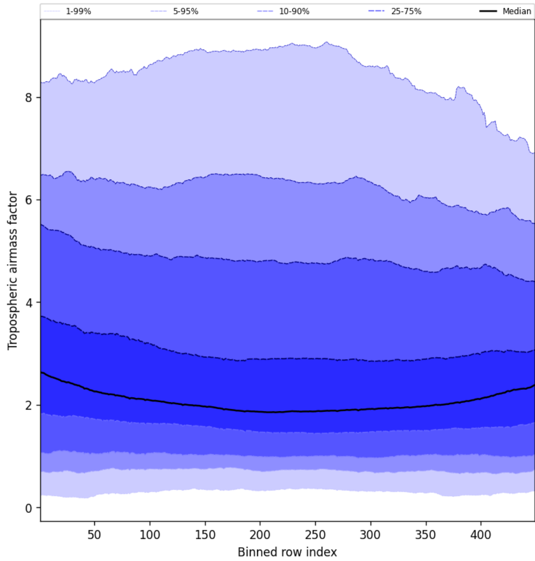
Figure 46: Along track statistics of “Tropospheric air mass factor” for 2025-10-19 to 2025-10-20
