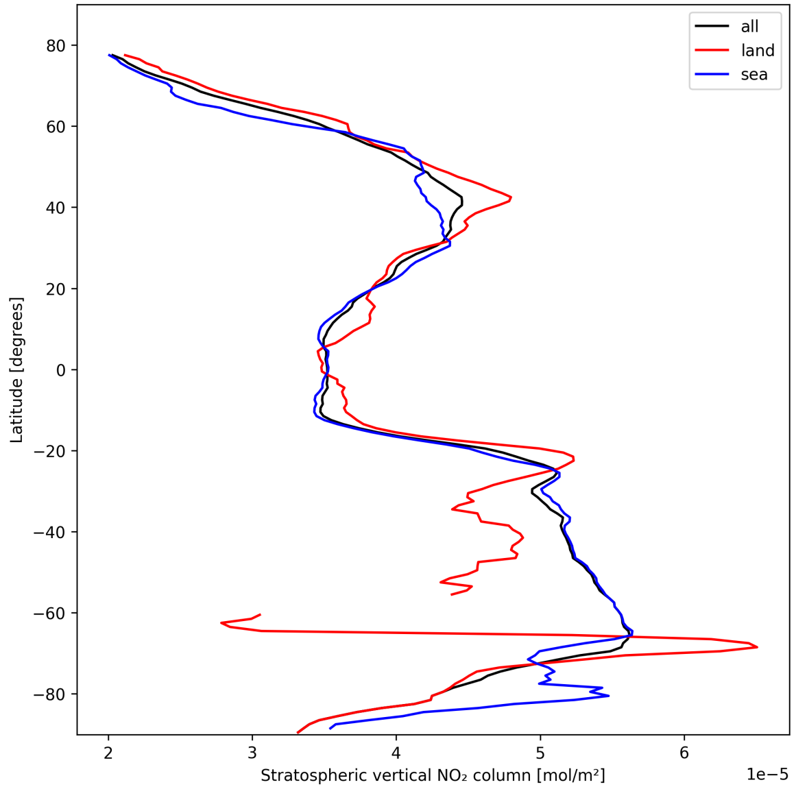
Figure 17: Zonal average of “Stratospheric vertical NO 2 column” for 2025-10-19 to 2025-10-20.
