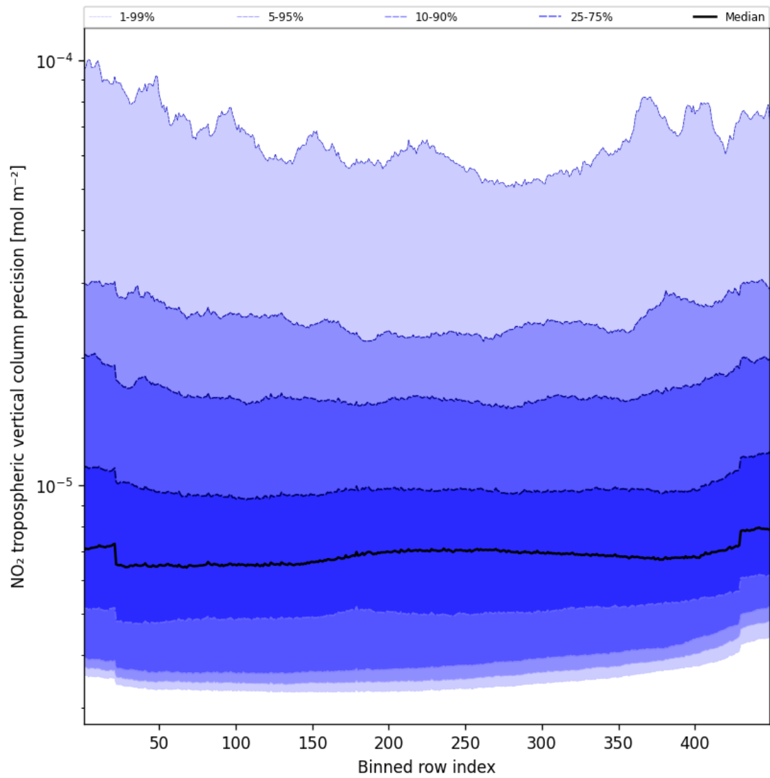
Figure 45: Along track statistics of “NO 2 tropospheric vertical column precision” for 2025-10-19 to 2025-10-20
