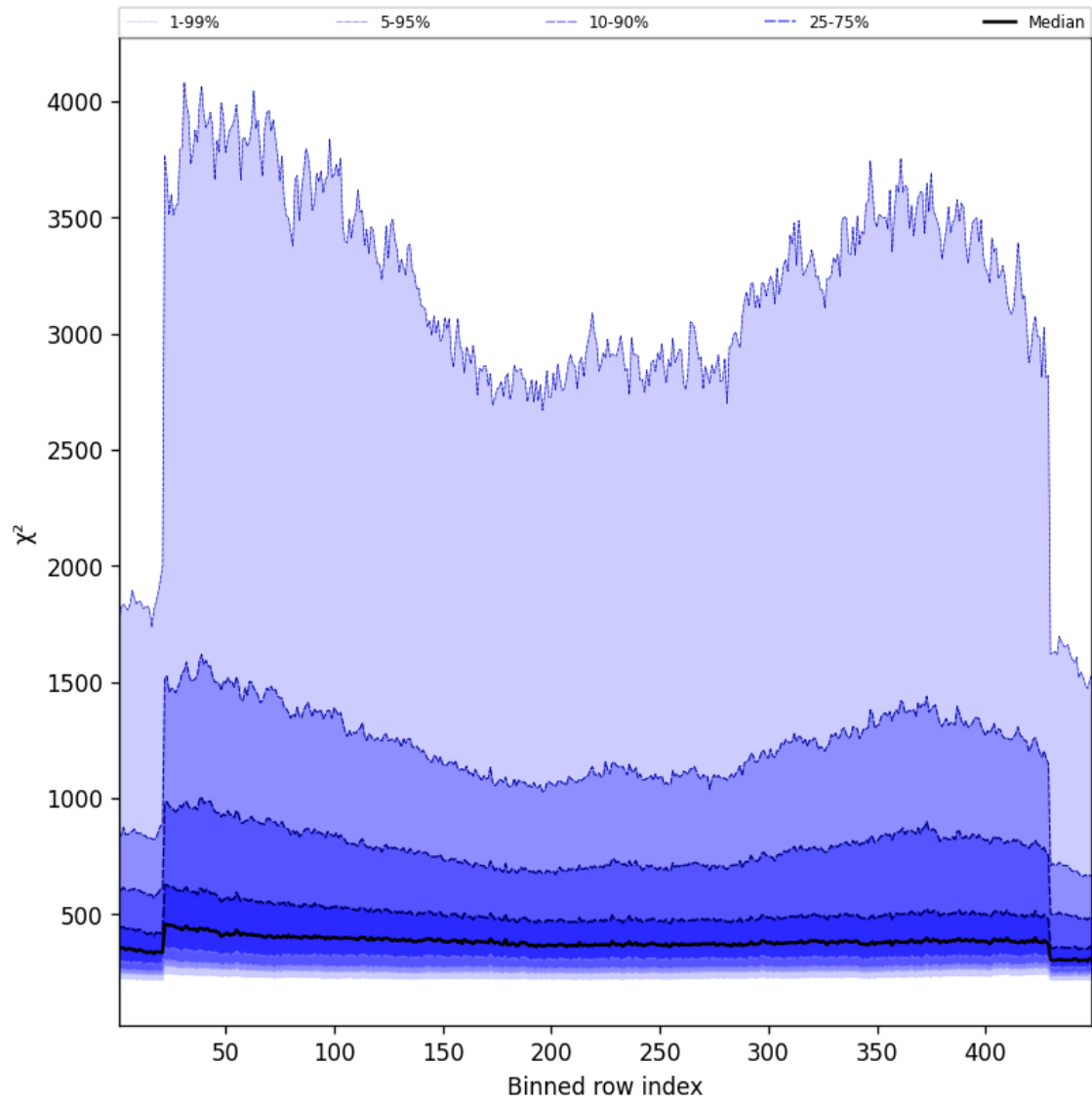
Figure 57: Along track statistics of “ \chi^2 ” for 2025-10-19 to 2025-10-20
