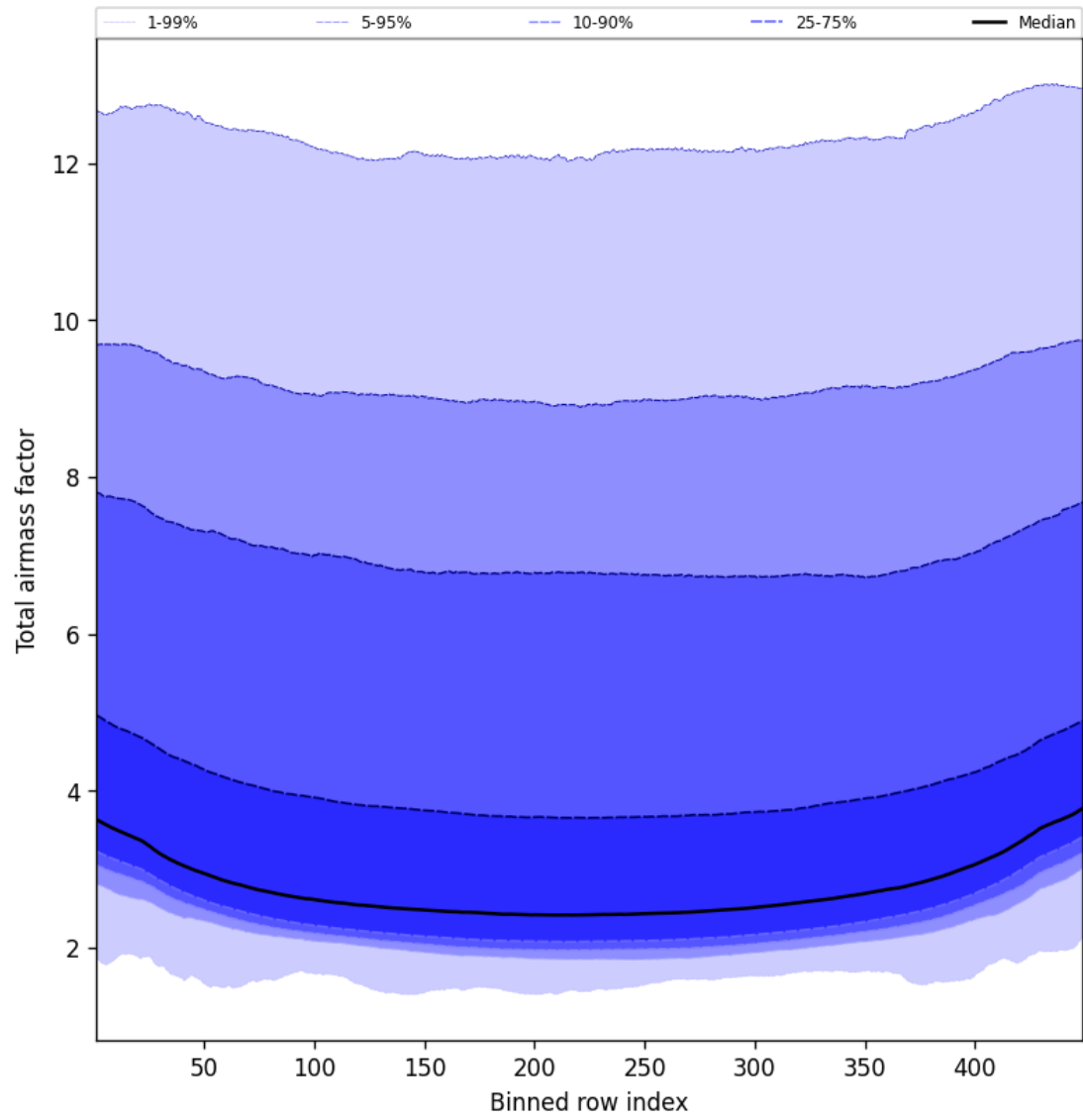
Figure 47: Along track statistics of “Total airmass factor” for 2025-10-19 to 2025-10-20
