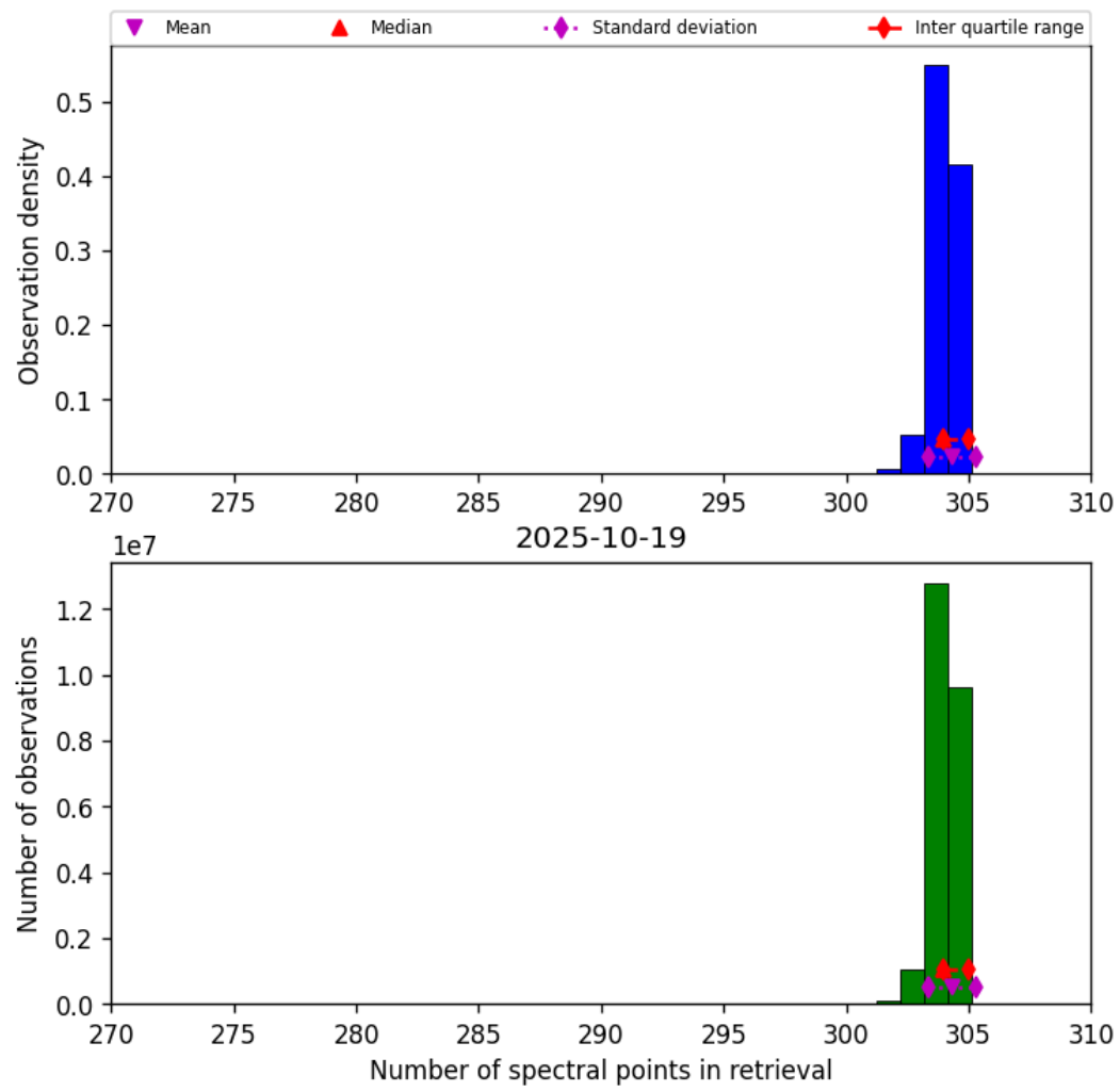
Figure 31: Histogram of “Number of spectral points in retrieval” for 2025-10-19 to 2025-10-20
