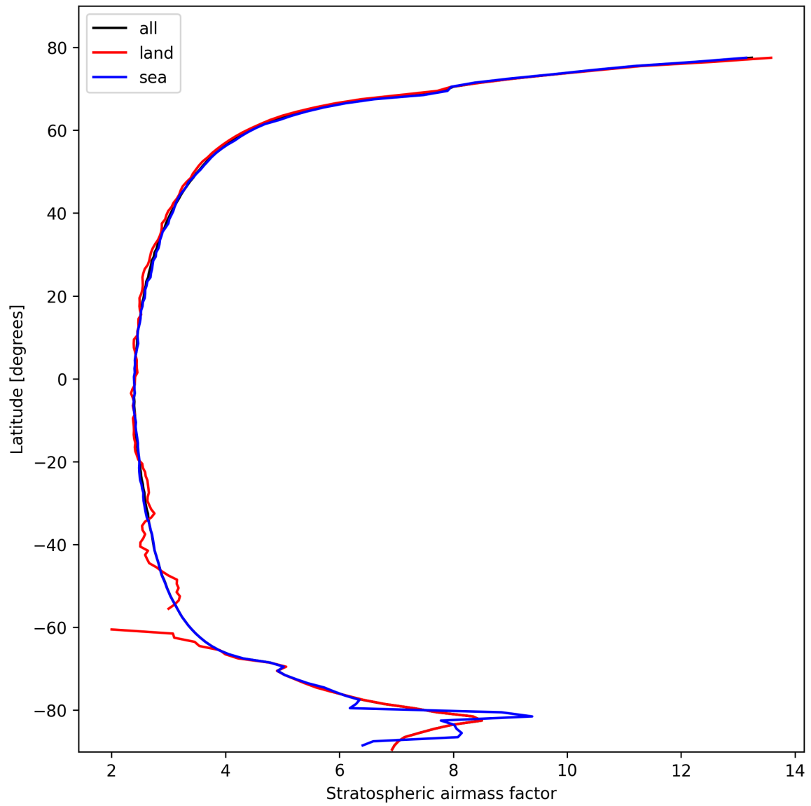
Figure 25: Zonal average of “Stratospheric airmass factor” for 2025-10-19 to 2025-10-20.
