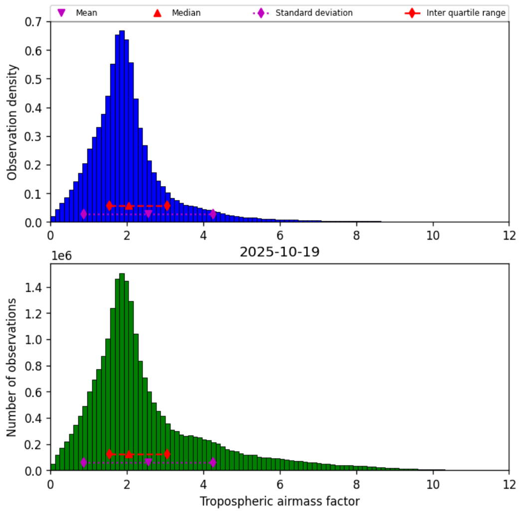
Figure 29: Histogram of “Tropospheric airmass factor” for 2025-10-19 to 2025-10-20
