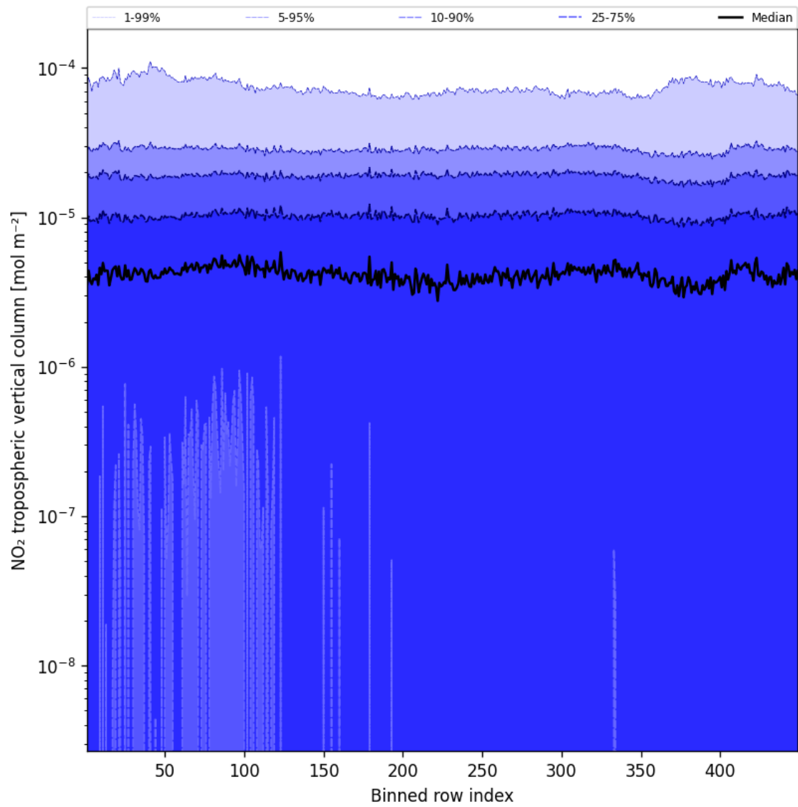
Figure 44: Along track statistics of “NO 2 tropospheric vertical column” for 2025-10-19 to 2025-10-20
