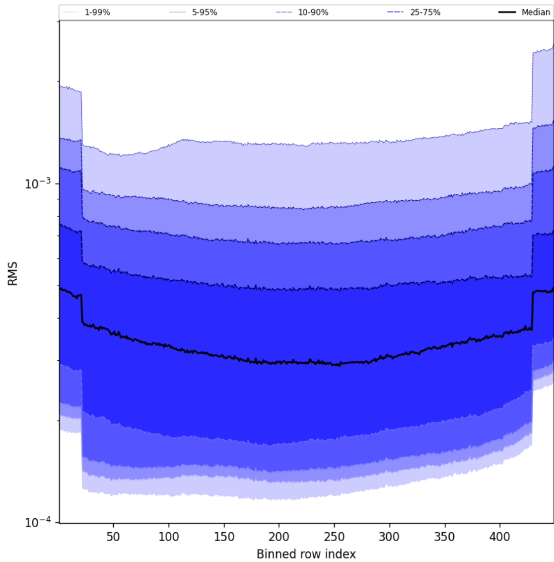
Figure 58: Along track statistics of “RMS” for 2025-10-19 to 2025-10-20
