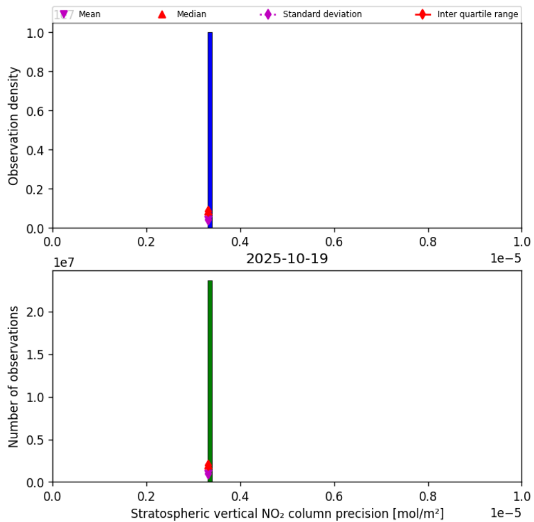
Figure 35: Histogram of “Stratospheric vertical NO 2 column precision” for 2025-10-19 to 2025-10-20
