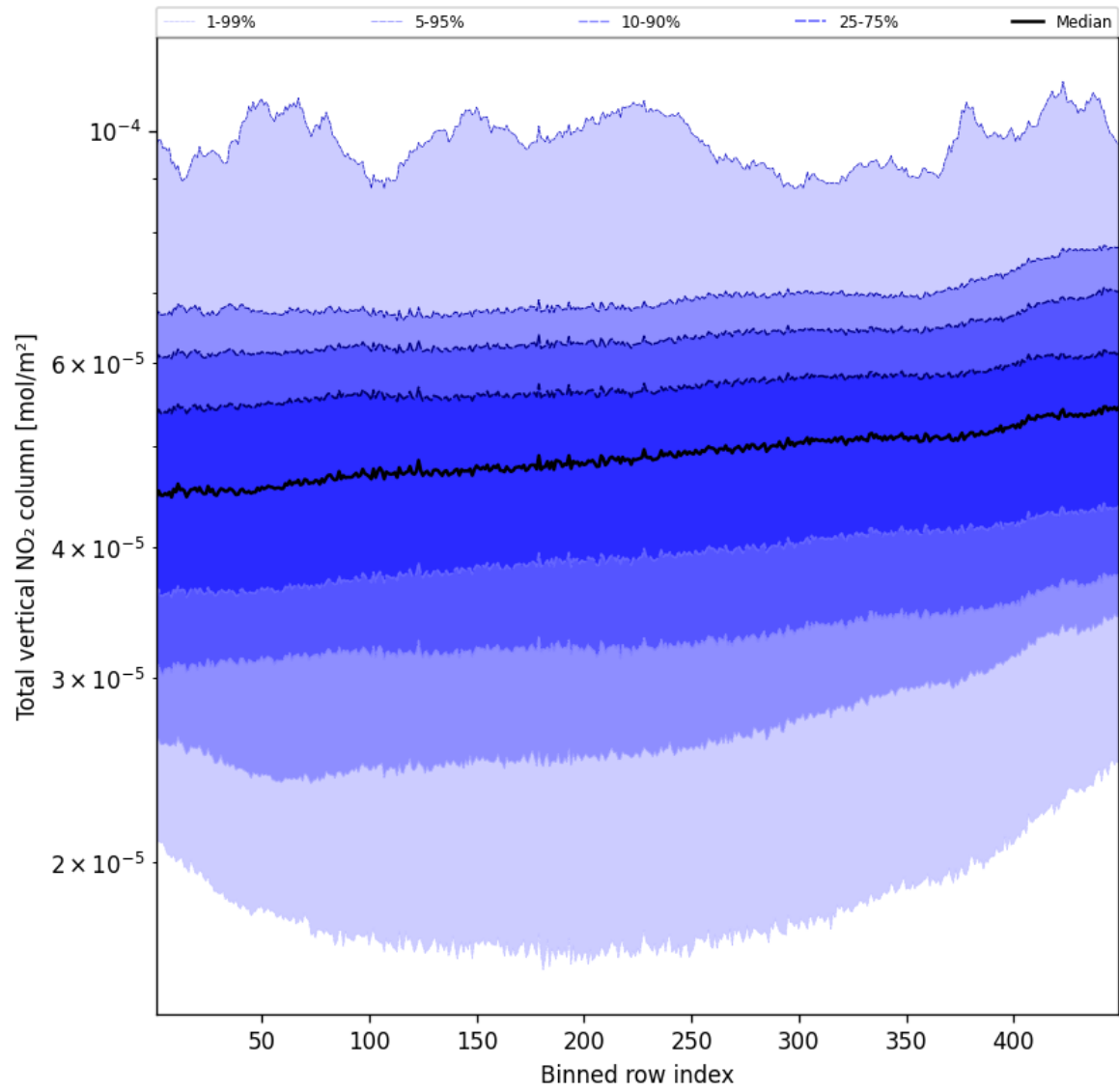
Figure 53: Along track statistics of “Total vertical NO 2 column” for 2025-10-19 to 2025-10-20
