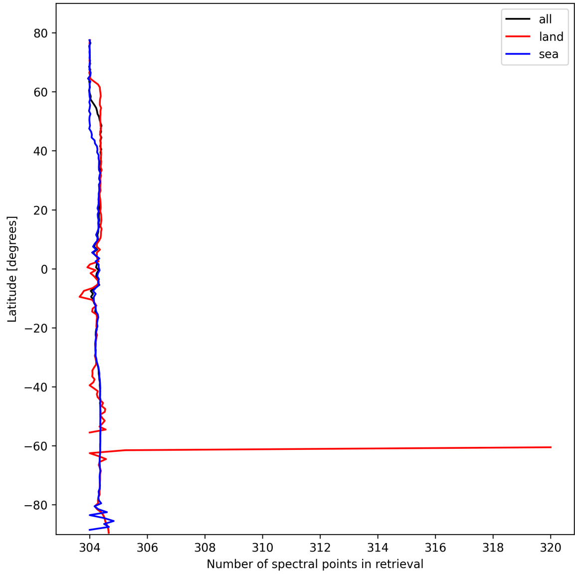
Figure 14: Zonal average of “Number of spectral points in retrieval” for 2025-10-19 to 2025-10-20.
