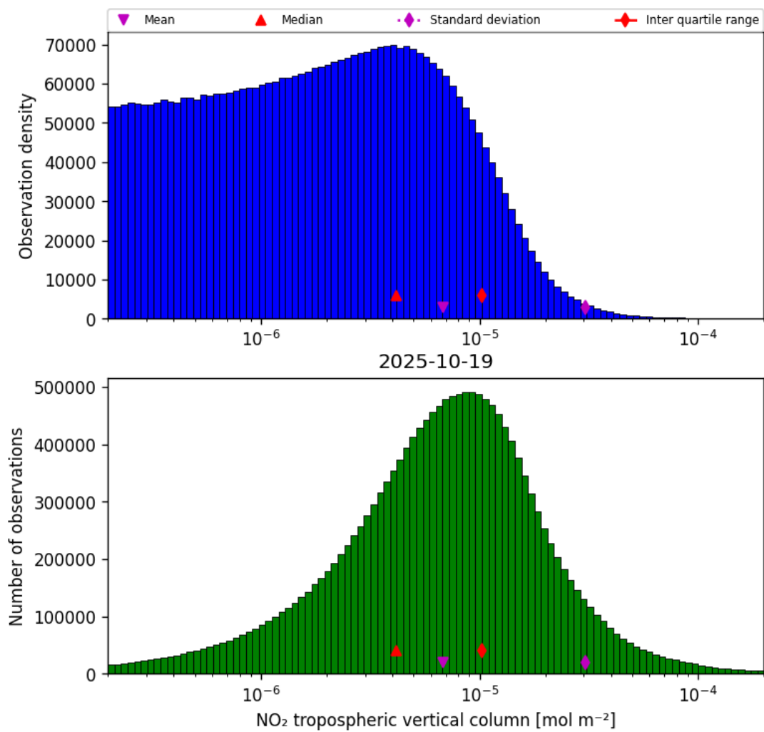
Figure 27: Histogram of “NO 2 tropospheric vertical column” for 2025-10-19 to 2025-10-20
