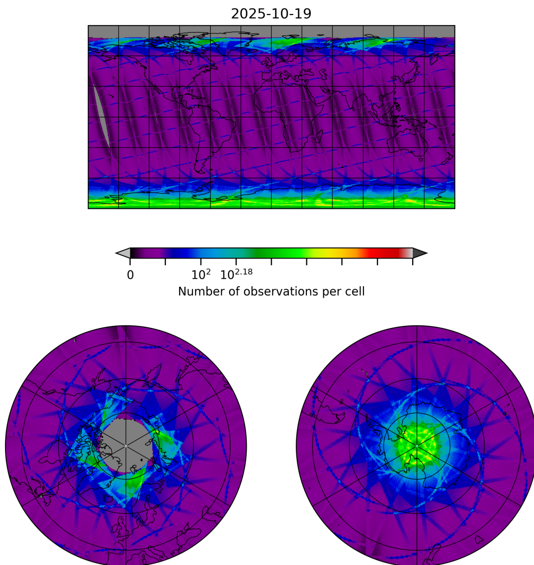
Figure 8: Map of the number of observations for 2025-10-19 to 2025-10-20
