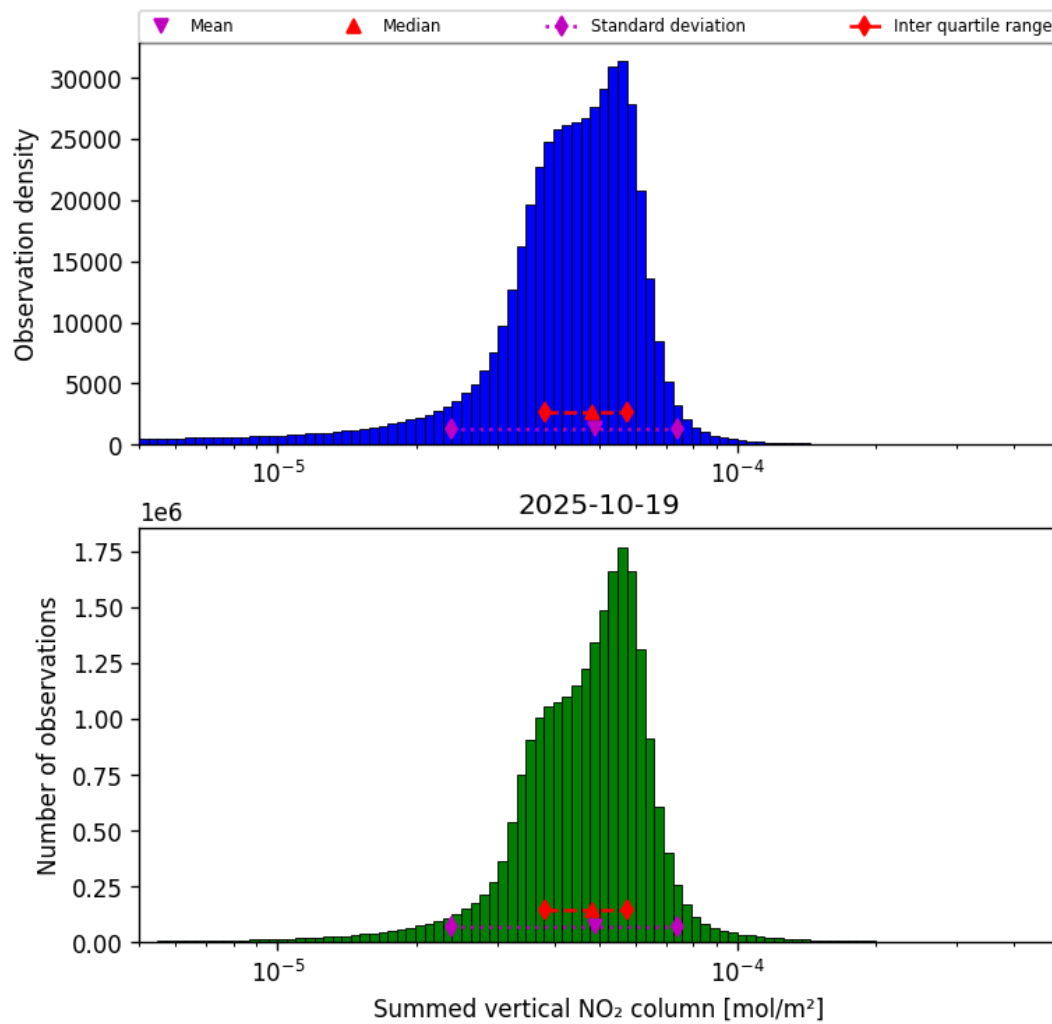
Figure 38: Histogram of “Summed vertical NO 2 column” for 2025-10-19 to 2025-10-20
