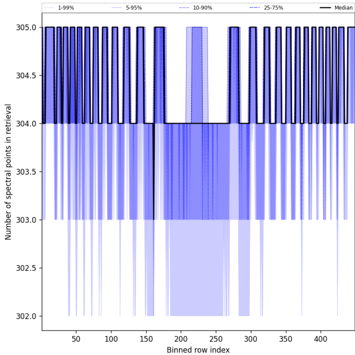
Figure 48: Along track statistics of “Number of spectral points in retrieval” for 2025-10-19 to 2025-10-20
