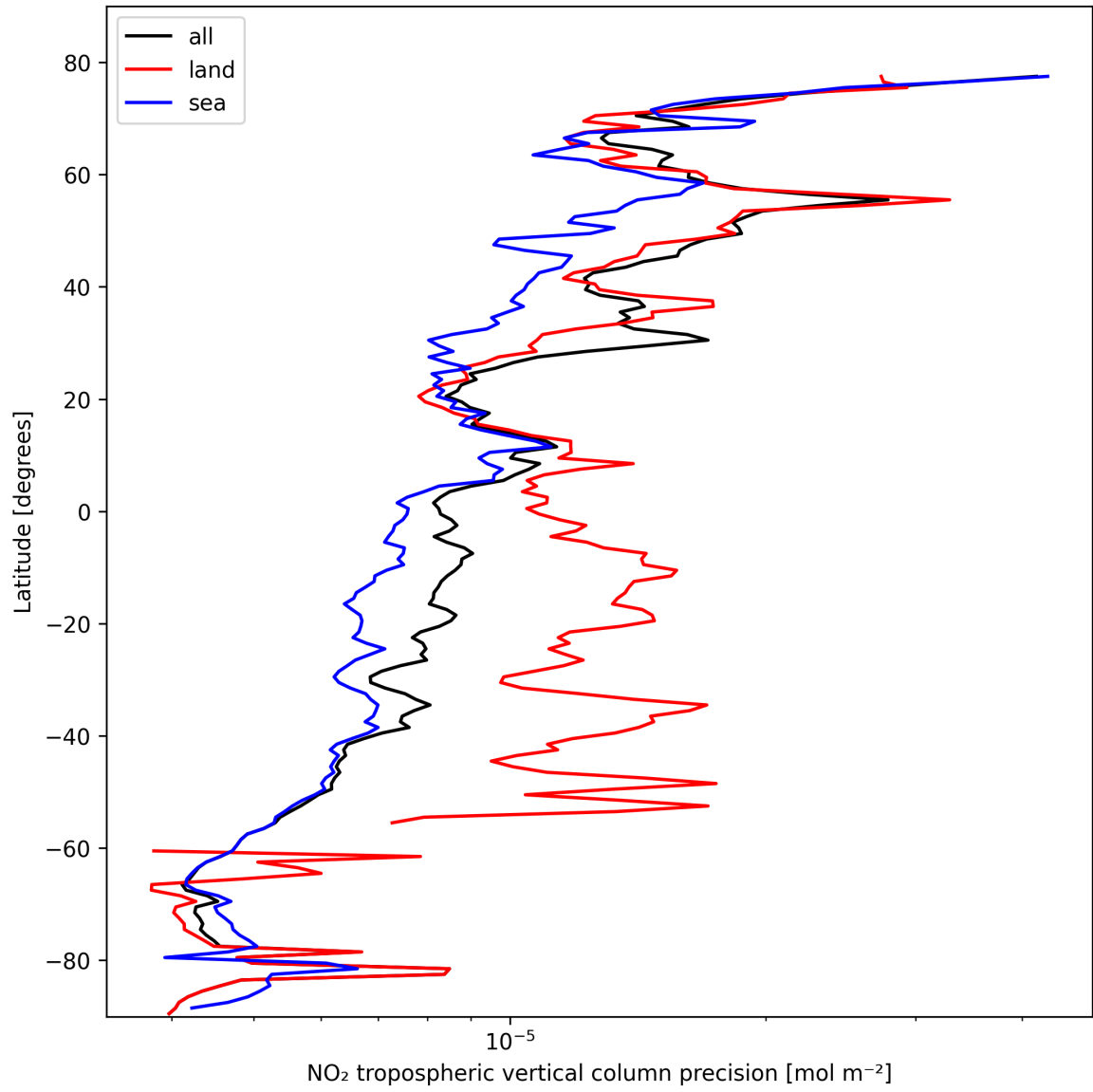
Figure 11: Zonal average of “NO 2 tropospheric vertical column precision” for 2025-10-19 to 2025-10-20.
