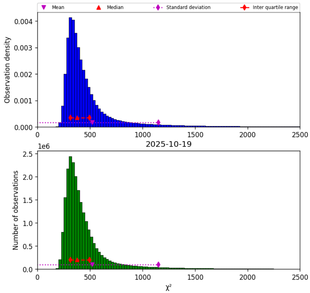
Figure 40: Histogram of “ \chi^2 ” for 2025-10-19 to 2025-10-20
