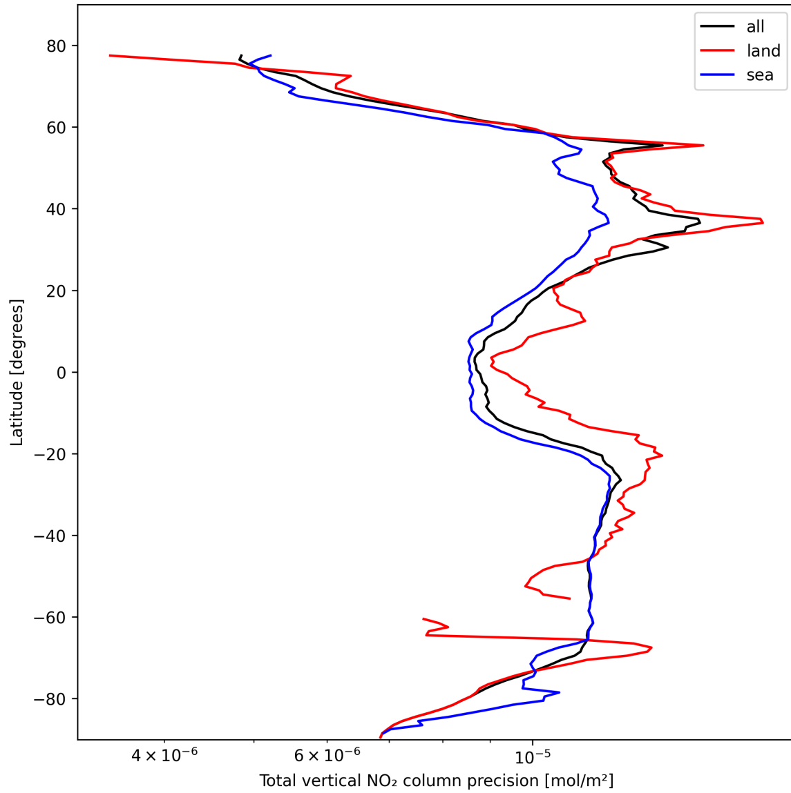
Figure 20: Zonal average of “Total vertical NO 2 column precision” for 2025-10-19 to 2025-10-20.
