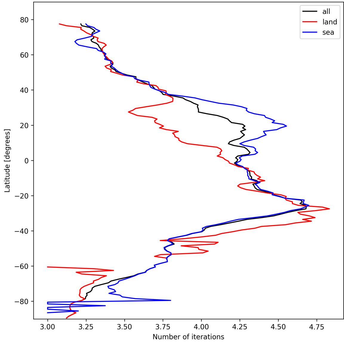
Figure 15: Zonal average of “Number of iterations” for 2025-10-20 to 2025-10-20.
