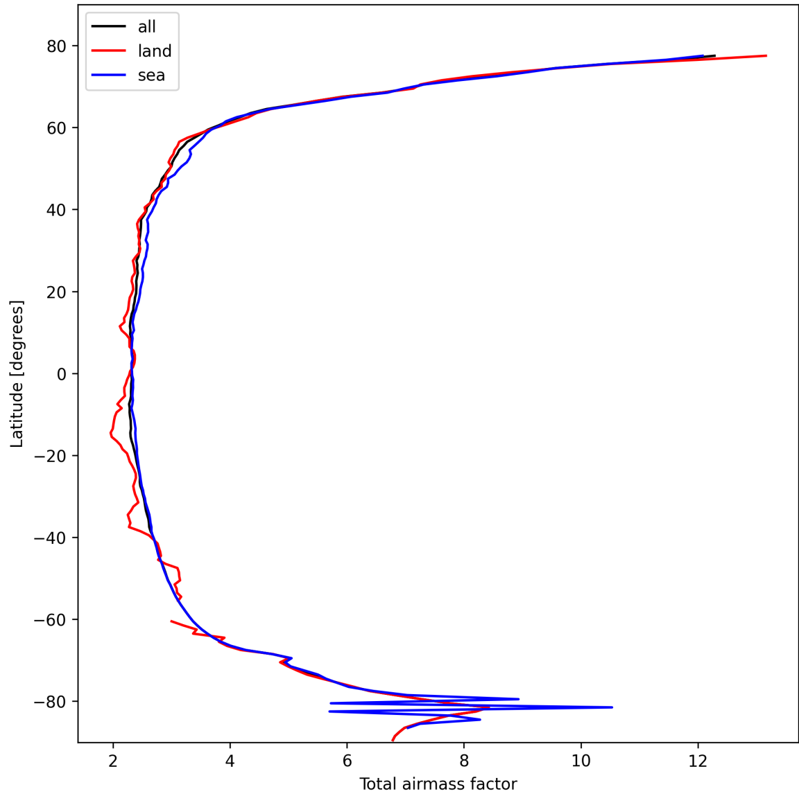
Figure 13: Zonal average of “Total airmass factor” for 2025-10-20 to 2025-10-20.
