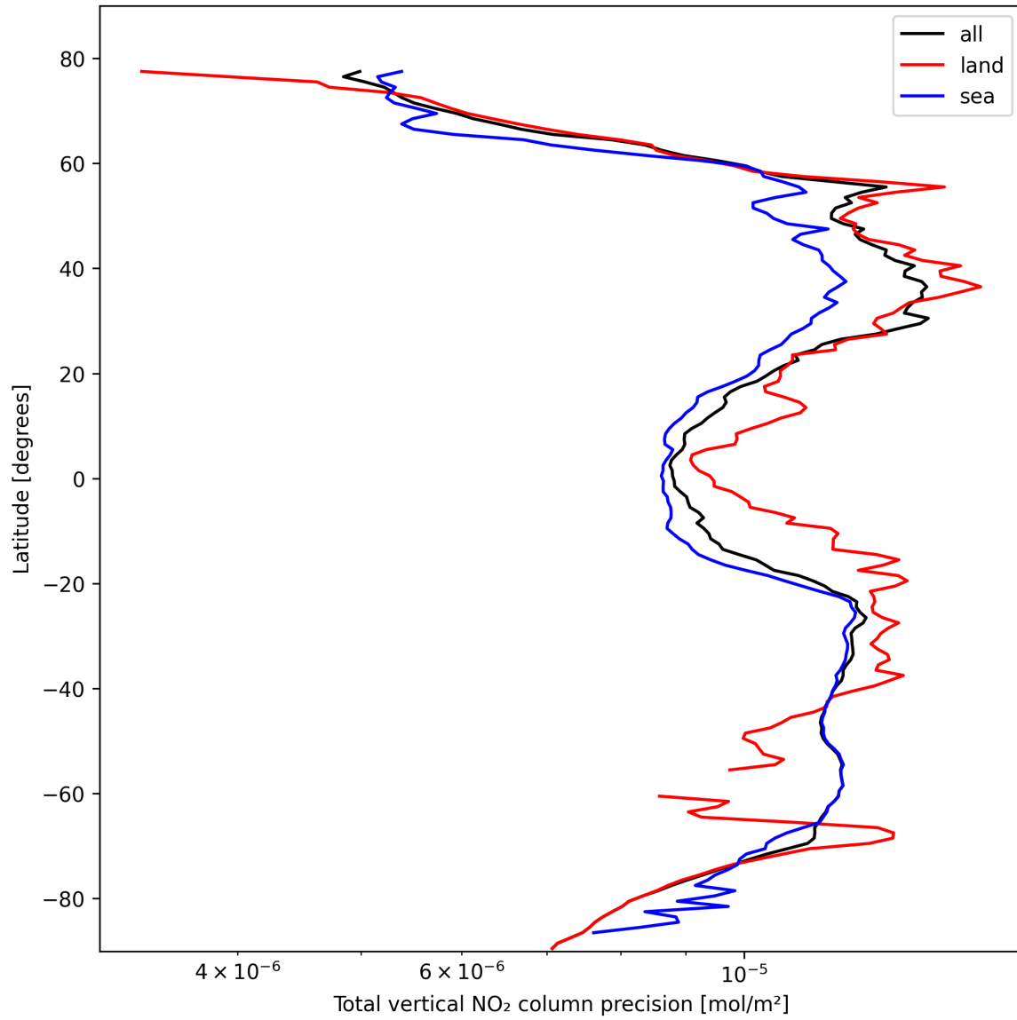
Figure 20: Zonal average of “Total vertical NO 2 column precision” for 2025-10-20 to 2025-10-20.
