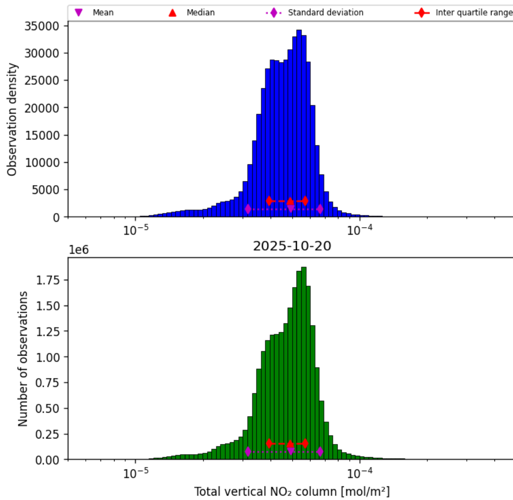
Figure 36: Histogram of "Total vertical NO 2 column" for 2025-10-20 to 2025-10-20
