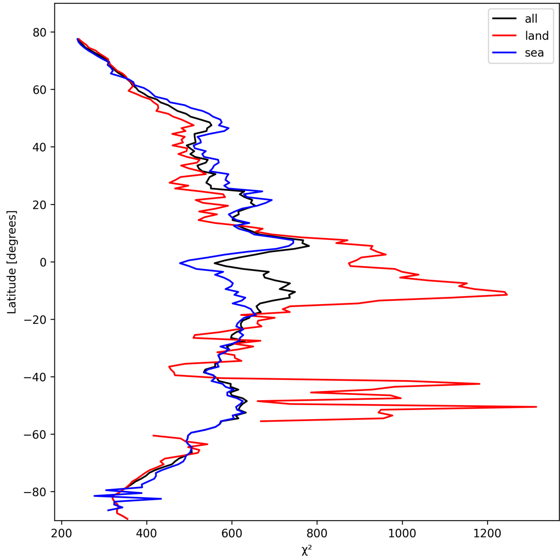
Figure 23: Zonal average of “ \chi^2 ” for 2025-10-20 to 2025-10-20.
