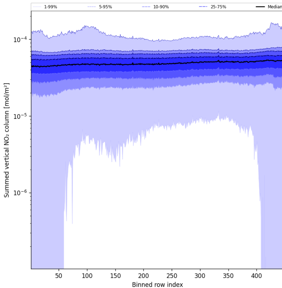
Figure 55: Along track statistics of “Summed vertical NO 2 column” for 2025-10-20 to 2025-10-20
