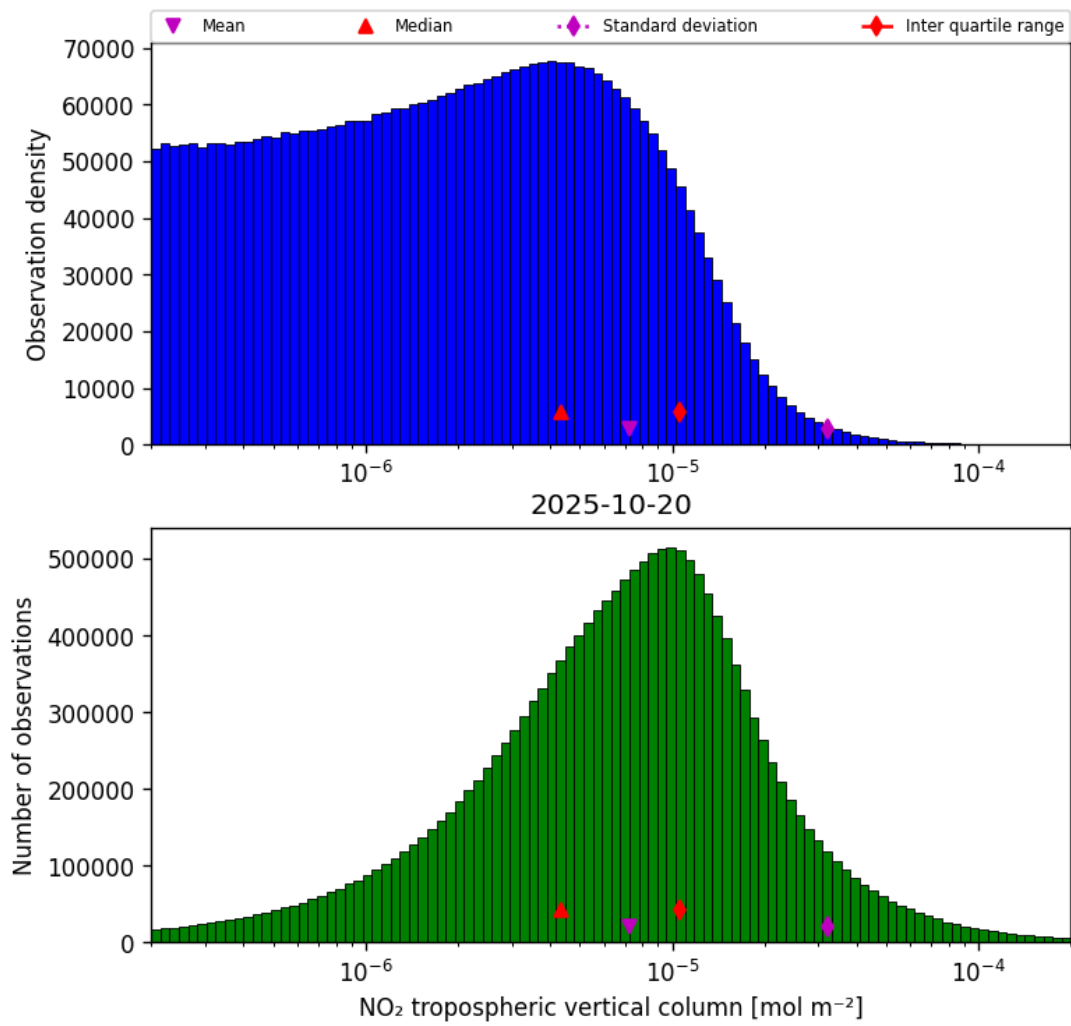
Figure 27: Histogram of “NO 2 tropospheric vertical column” for 2025-10-20 to 2025-10-20
