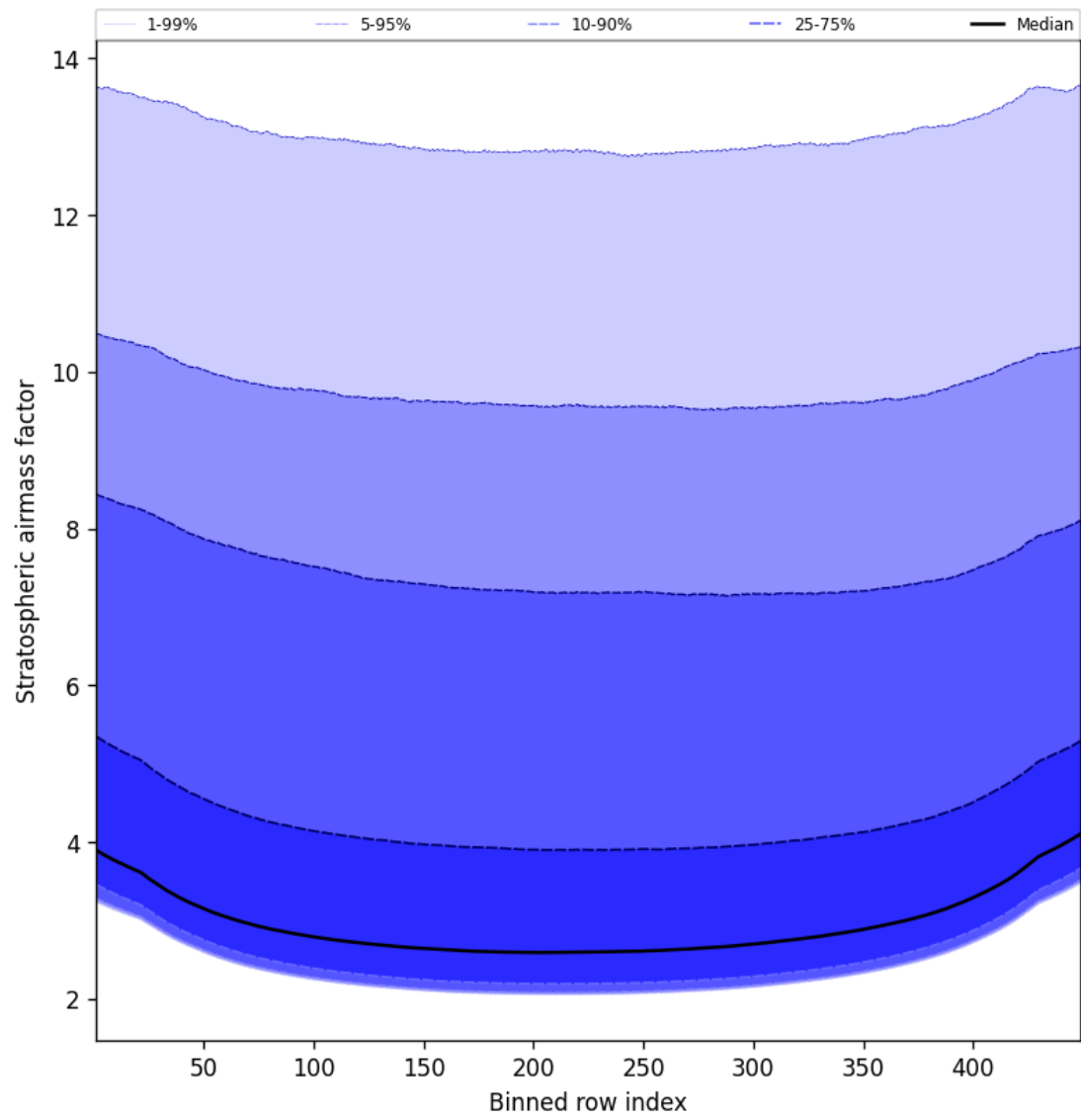
Figure 59: Along track statistics of “Stratospheric air mass factor” for 2025-10-20 to 2025-10-20
