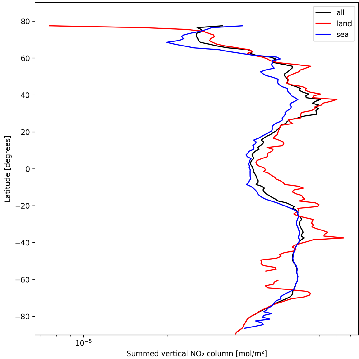
Figure 21: Zonal average of “Summed vertical NO 2 column” for 2025-10-20 to 2025-10-20.
