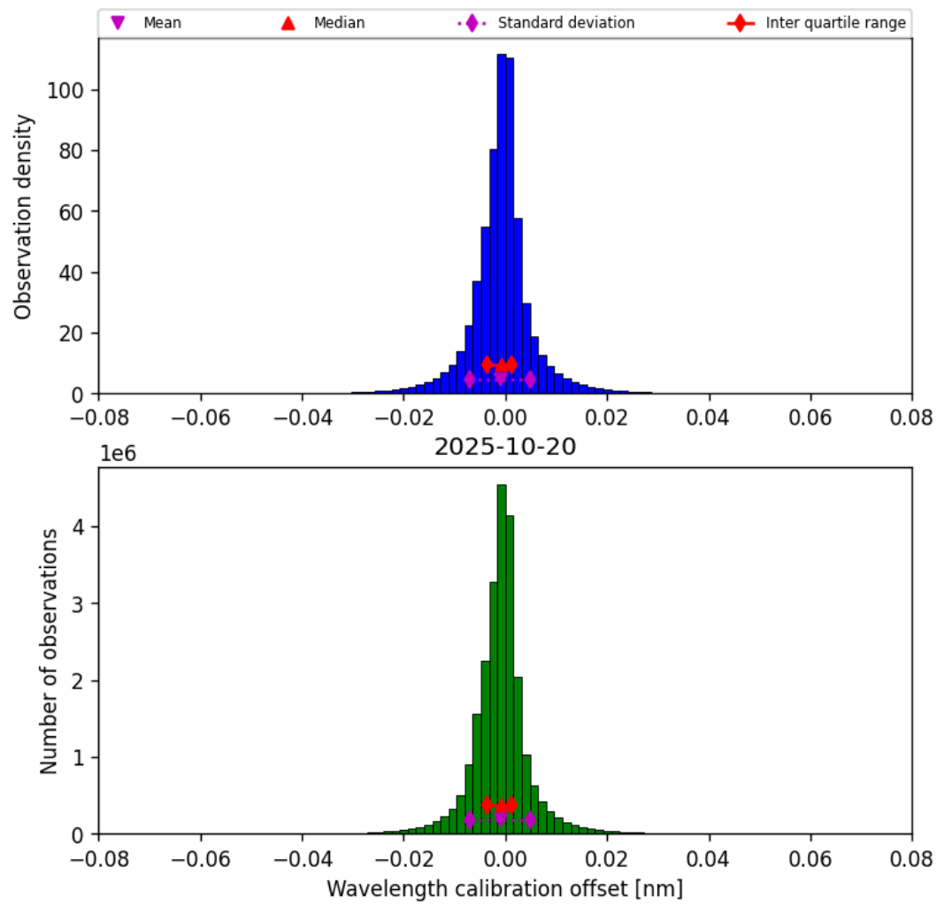
Figure 33: Histogram of “Wavelength calibration offset” for 2025-10-20 to 2025-10-20
