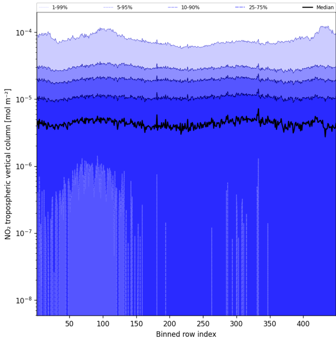
Figure 44: Along track statistics of “NO 2 tropospheric vertical column” for 2025-10-20 to 2025-10-20
