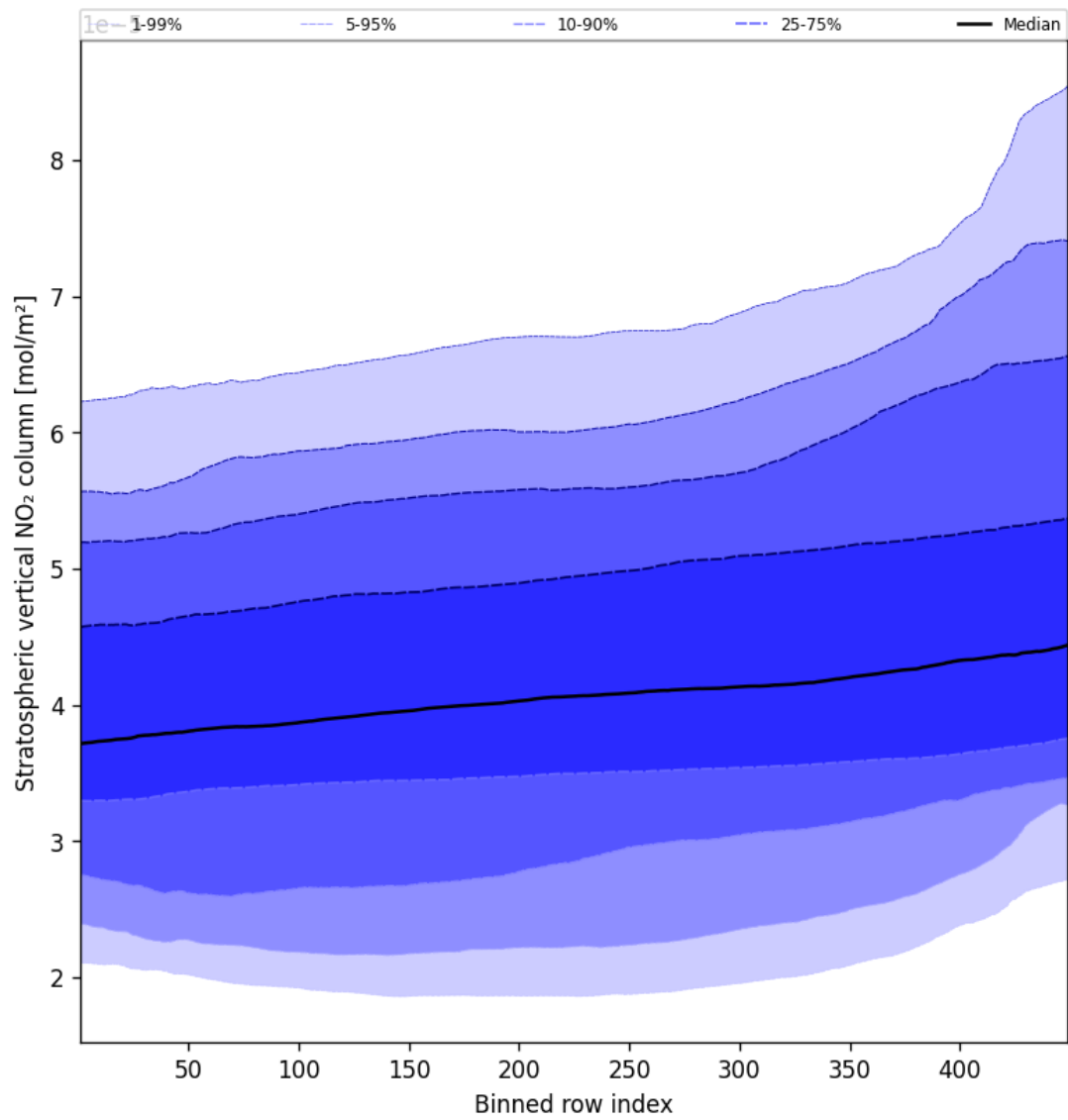
Figure 51: Along track statistics of “Stratospheric vertical NO 2 column” for 2025-10-20 to 2025-10-20
