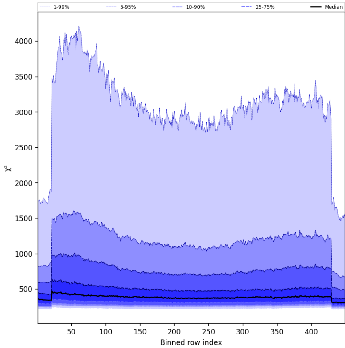
Figure 57: Along track statistics of “ \chi^2 ” for 2025-10-20 to 2025-10-20
