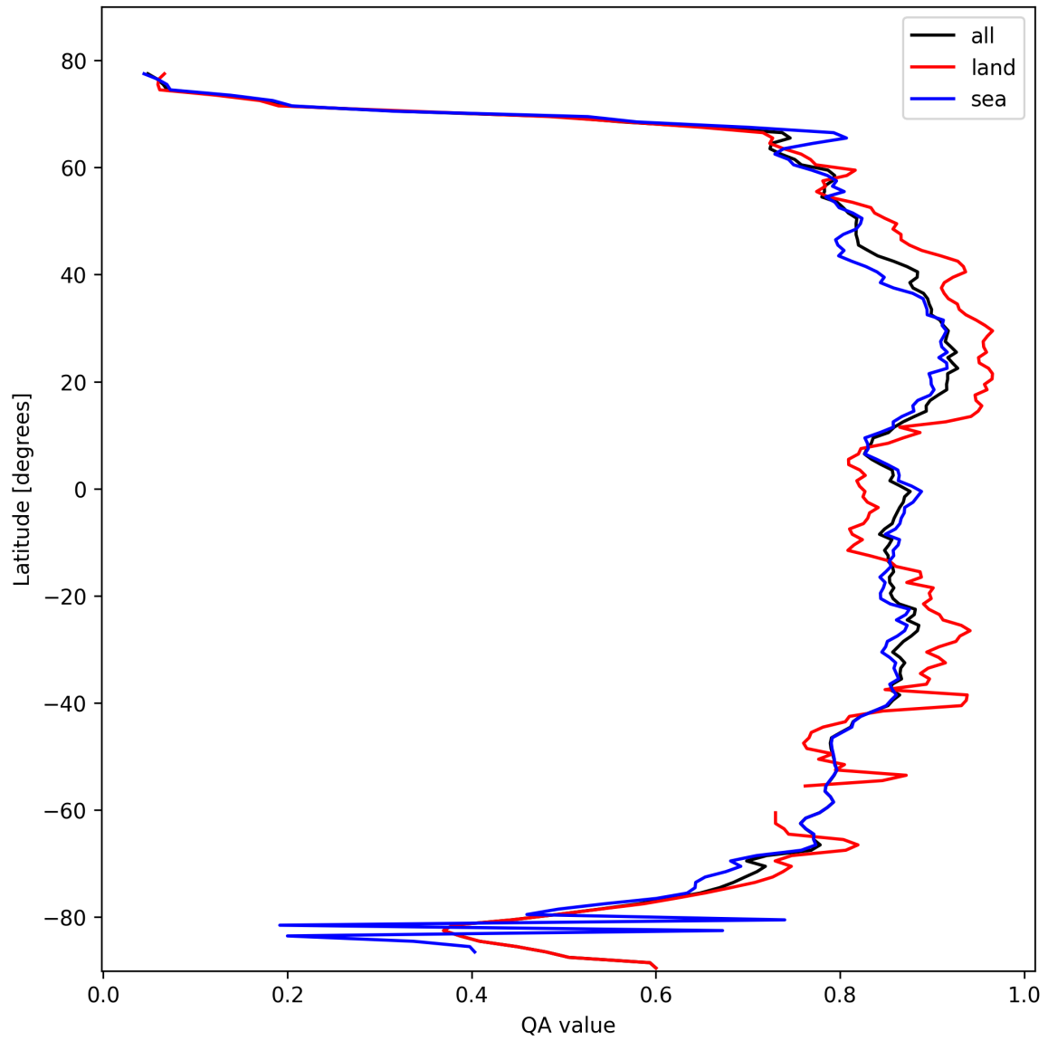
Figure 9: Zonal average of “QA value” for 2025-10-20 to 2025-10-20.
