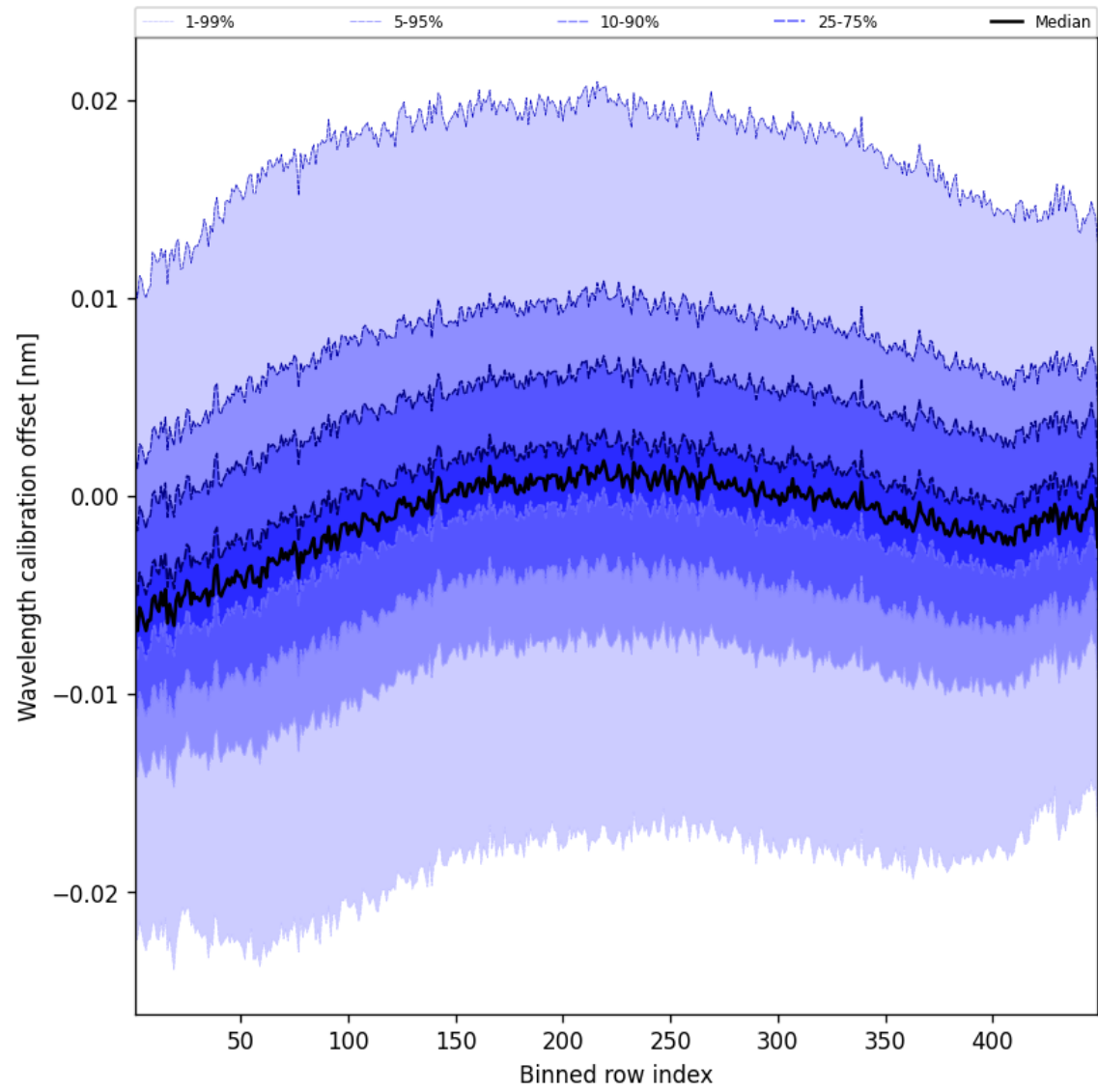
Figure 50: Along track statistics of “Wavelength calibration offset” for 2025-10-20 to 2025-10-20
