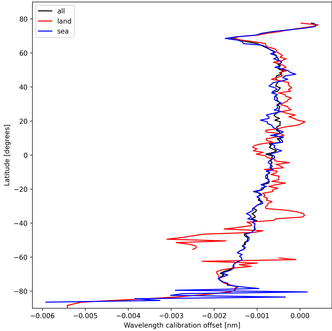
Figure 16: Zonal average of “Wavelength calibration offset” for 2025-10-20 to 2025-10-20.
