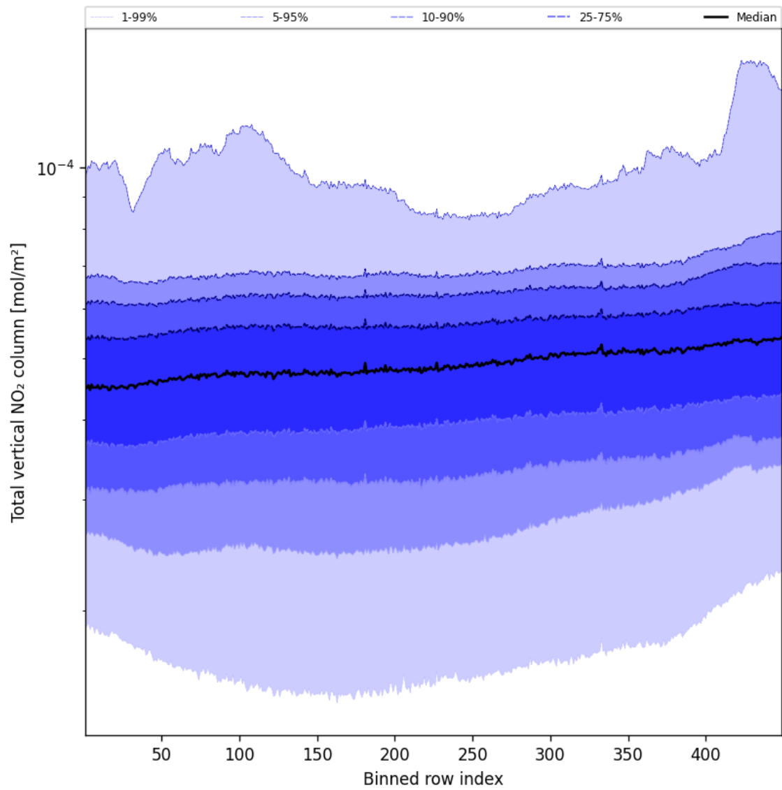
Figure 53: Along track statistics of “Total vertical NO 2 column” for 2025-10-20 to 2025-10-20
