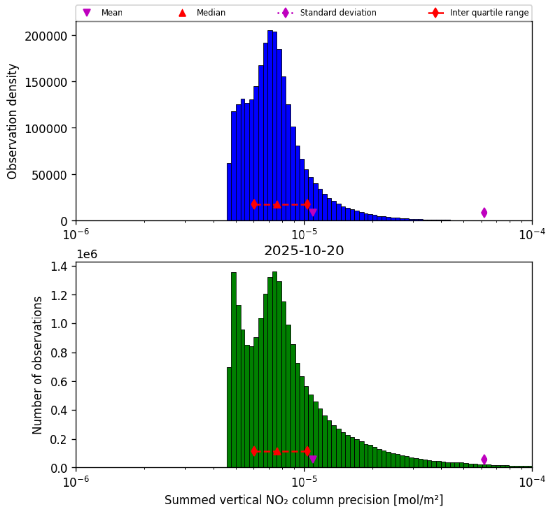
Figure 39: Histogram of "Summed vertical NO 2 column precision" for 2025-10-20 to 2025-10-20
