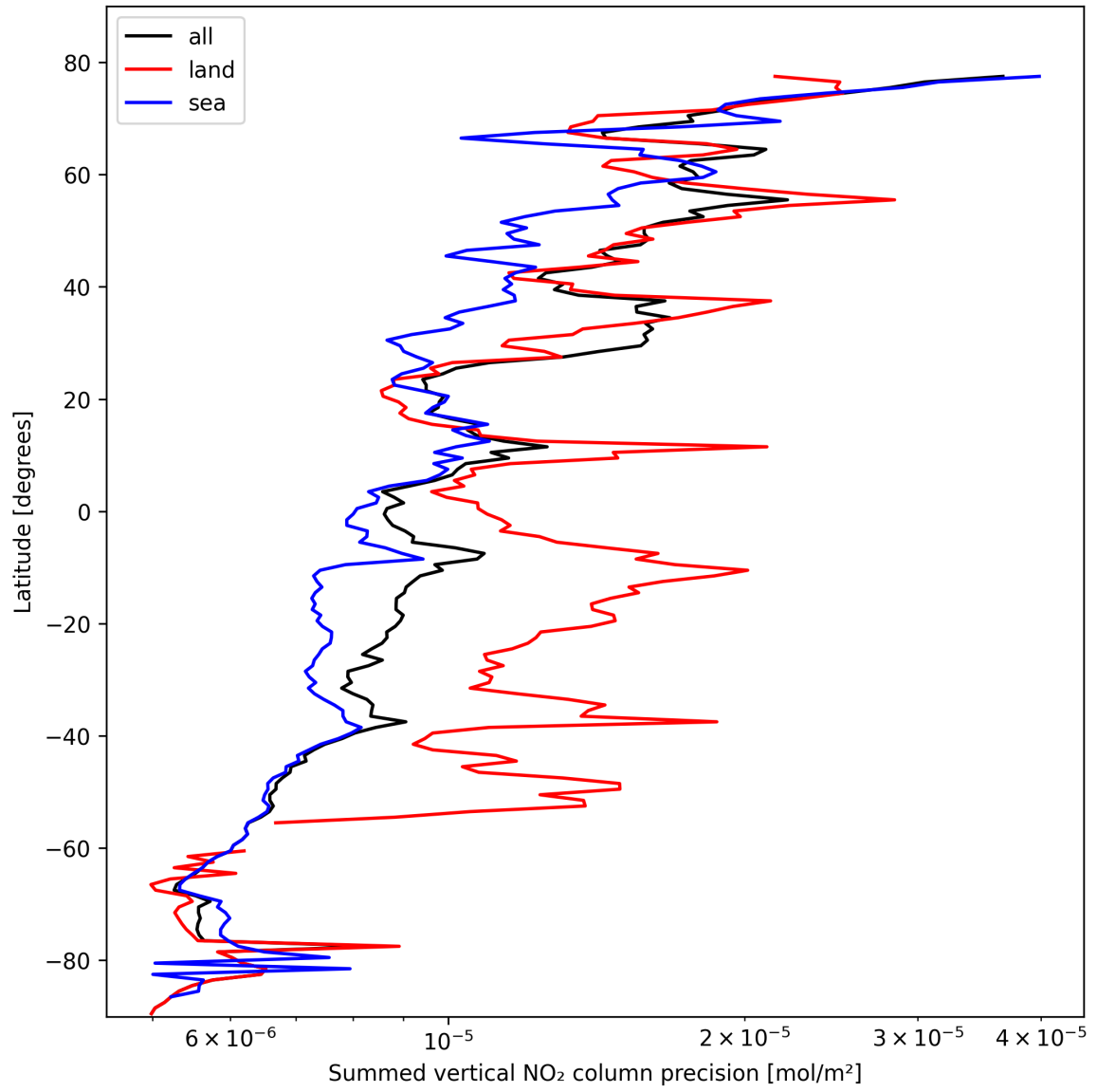
Figure 22: Zonal average of “Summed vertical NO 2 column precision” for 2025-10-20 to 2025-10-20.
