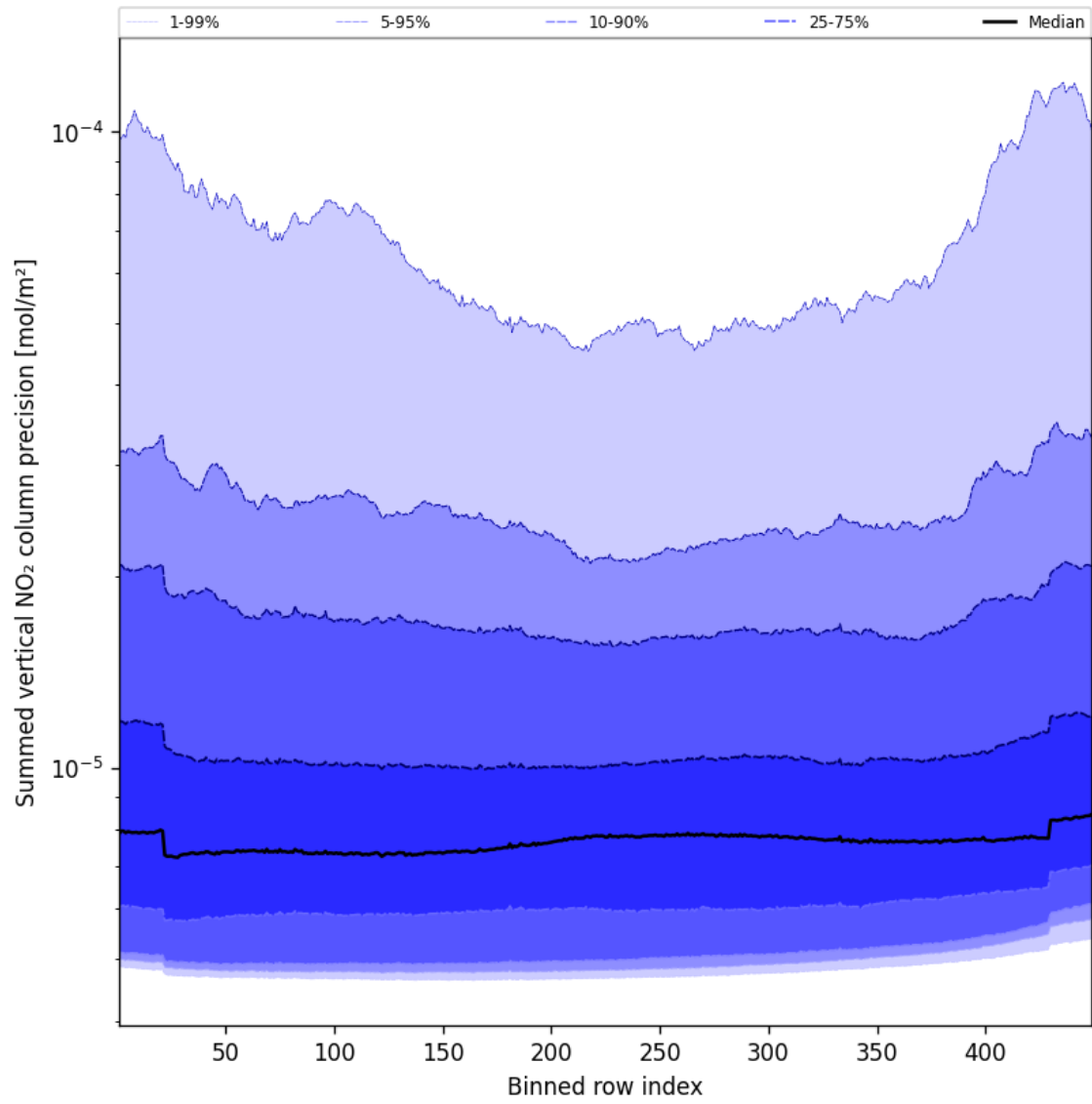
Figure 56: Along track statistics of “Summed vertical NO 2 column precision” for 2025-10-20 to 2025-10-20
