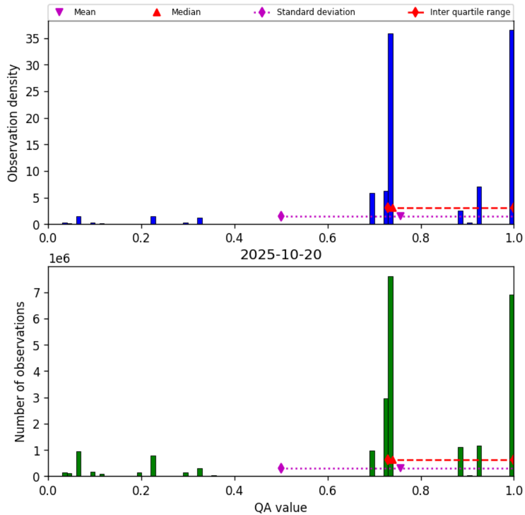
Figure 26: Histogram of “QA value” for 2025-10-20 to 2025-10-20
