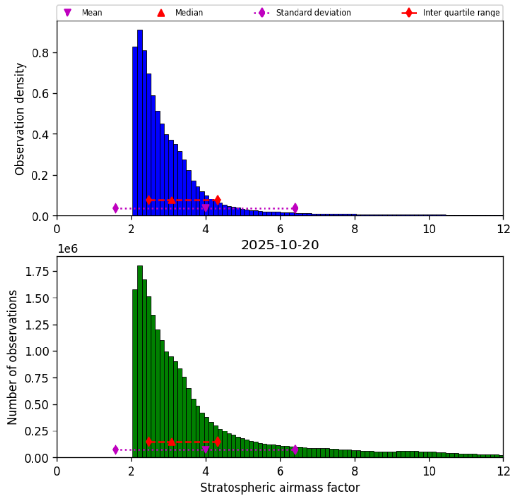
Figure 42: Histogram of “Stratospheric airmass factor” for 2025-10-20 to 2025-10-20
