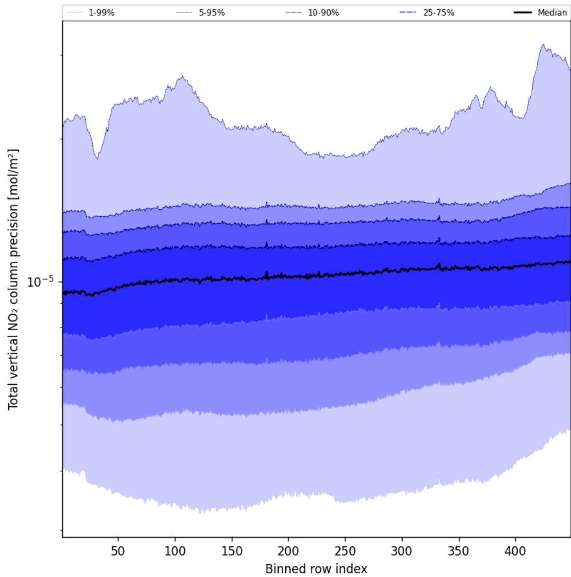
Figure 54: Along track statistics of “Total vertical NO 2 column precision” for 2025-10-20 to 2025-10-20
