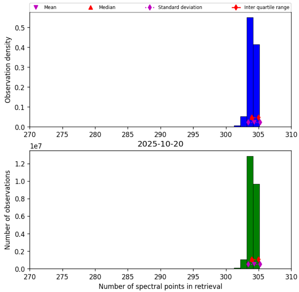
Figure 31: Histogram of “Number of spectral points in retrieval” for 2025-10-20 to 2025-10-20
