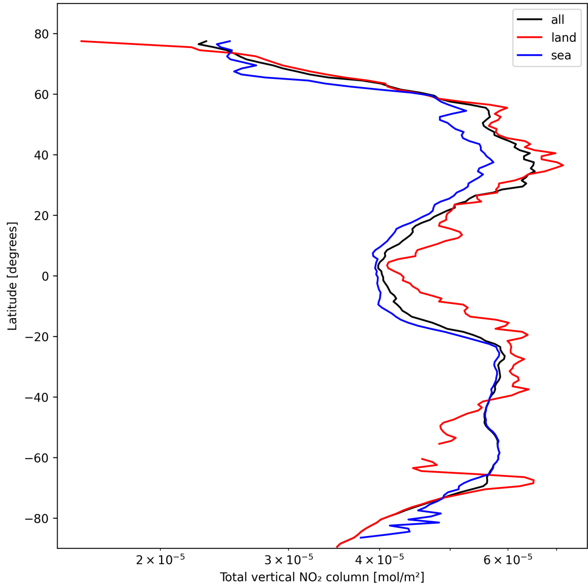
Figure 19: Zonal average of “Total vertical NO 2 column” for 2025-10-20 to 2025-10-20.
