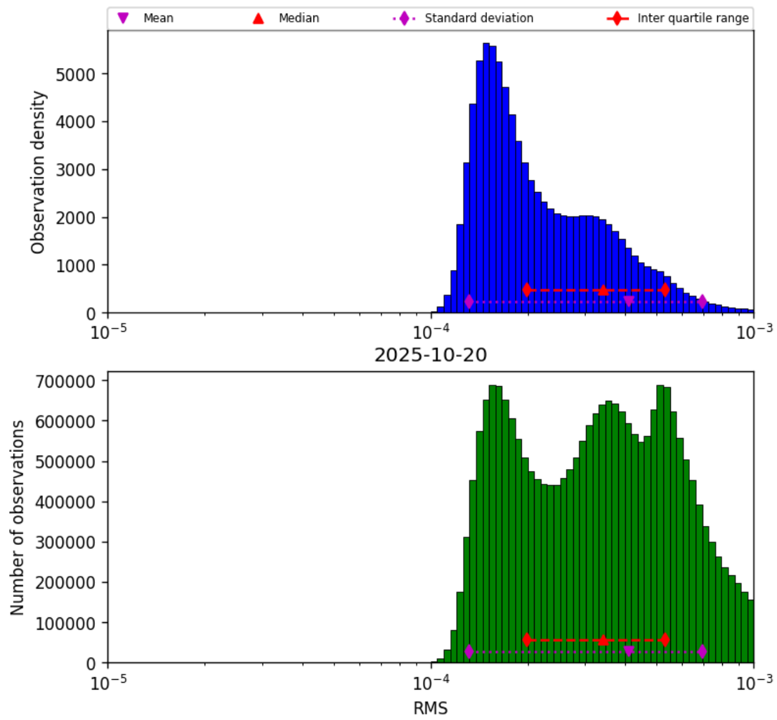
Figure 41: Histogram of “RMS” for 2025-10-20 to 2025-10-20
