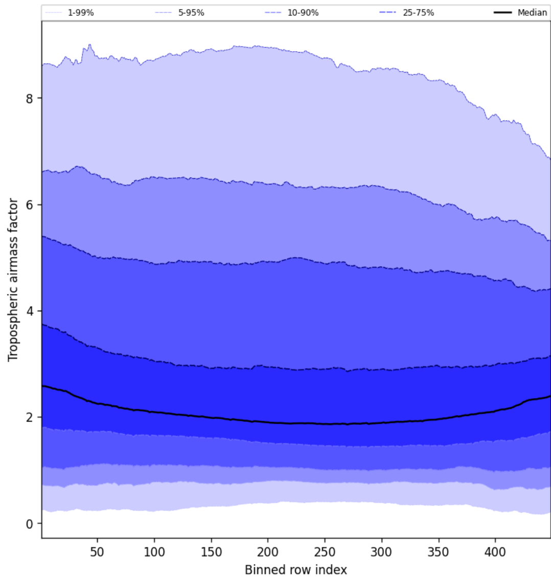
Figure 46: Along track statistics of “Tropospheric airmass factor” for 2025-10-20 to 2025-10-20
