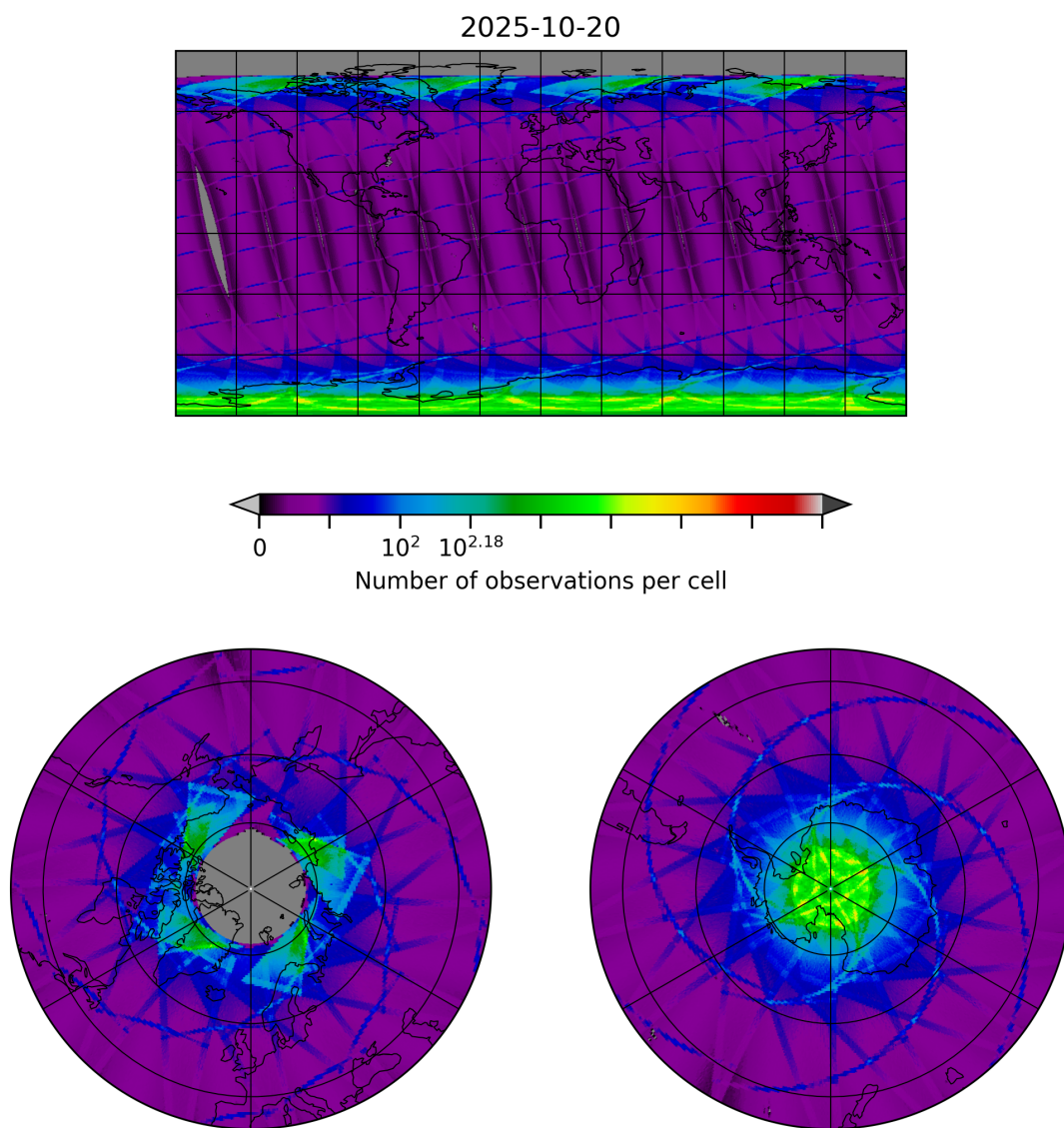
Figure 8: Map of the number of observations for 2025-10-20 to 2025-10-20
