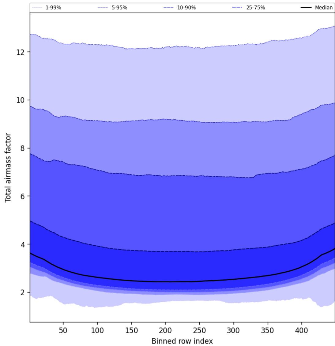
Figure 47: Along track statistics of “Total airmass factor” for 2025-10-20 to 2025-10-20
