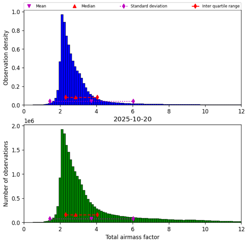
Figure 30: Histogram of “Total airmass factor” for 2025-10-20 to 2025-10-20
