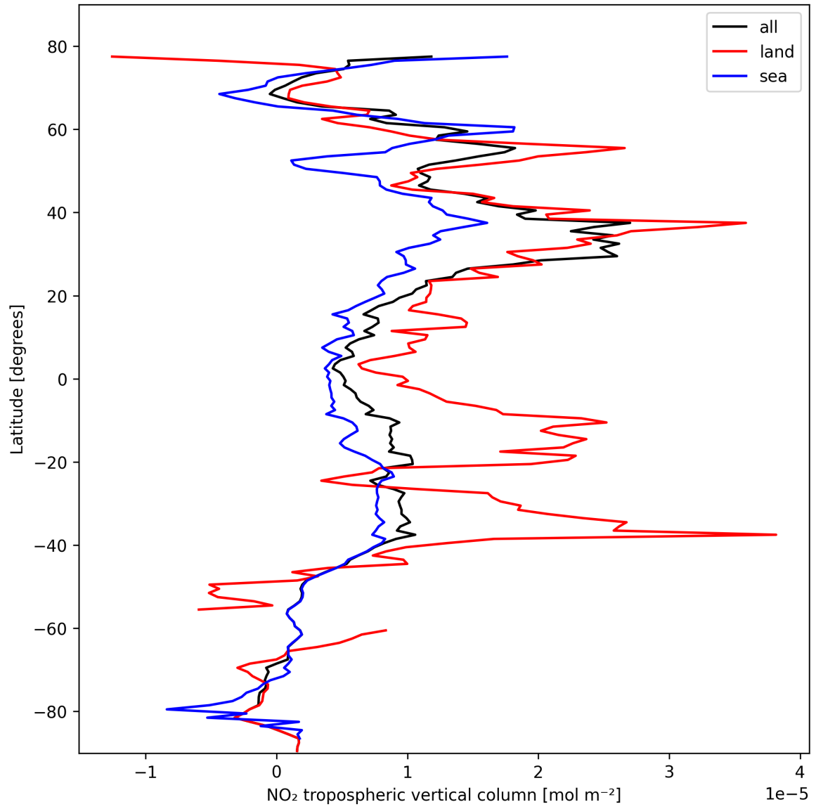
Figure 10: Zonal average of “NO 2 tropospheric vertical column” for 2025-10-20 to 2025-10-20.
