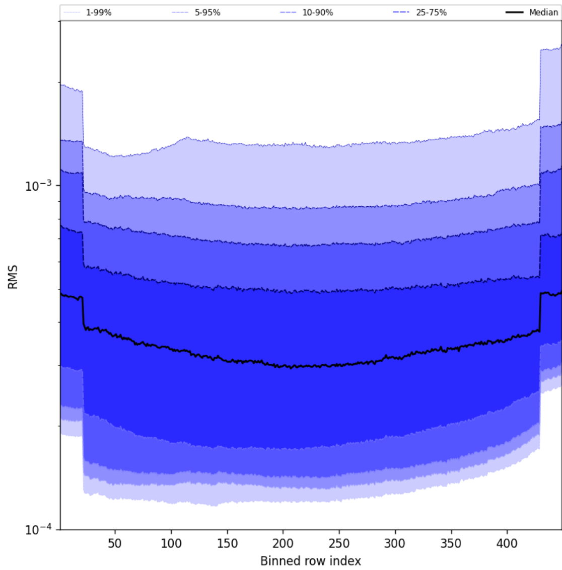
Figure 58: Along track statistics of “RMS” for 2025-10-20 to 2025-10-20
