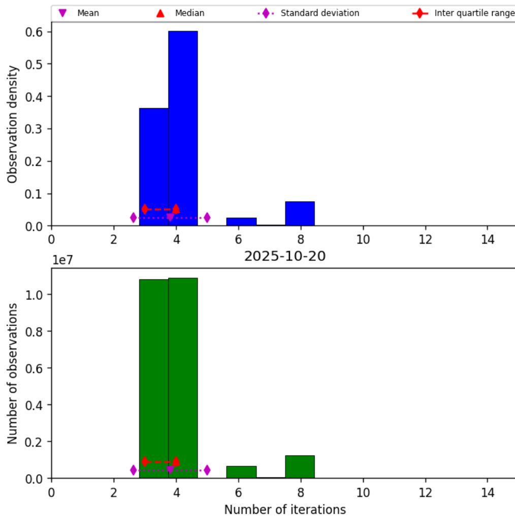
Figure 32: Histogram of “Number of iterations” for 2025-10-20 to 2025-10-20
