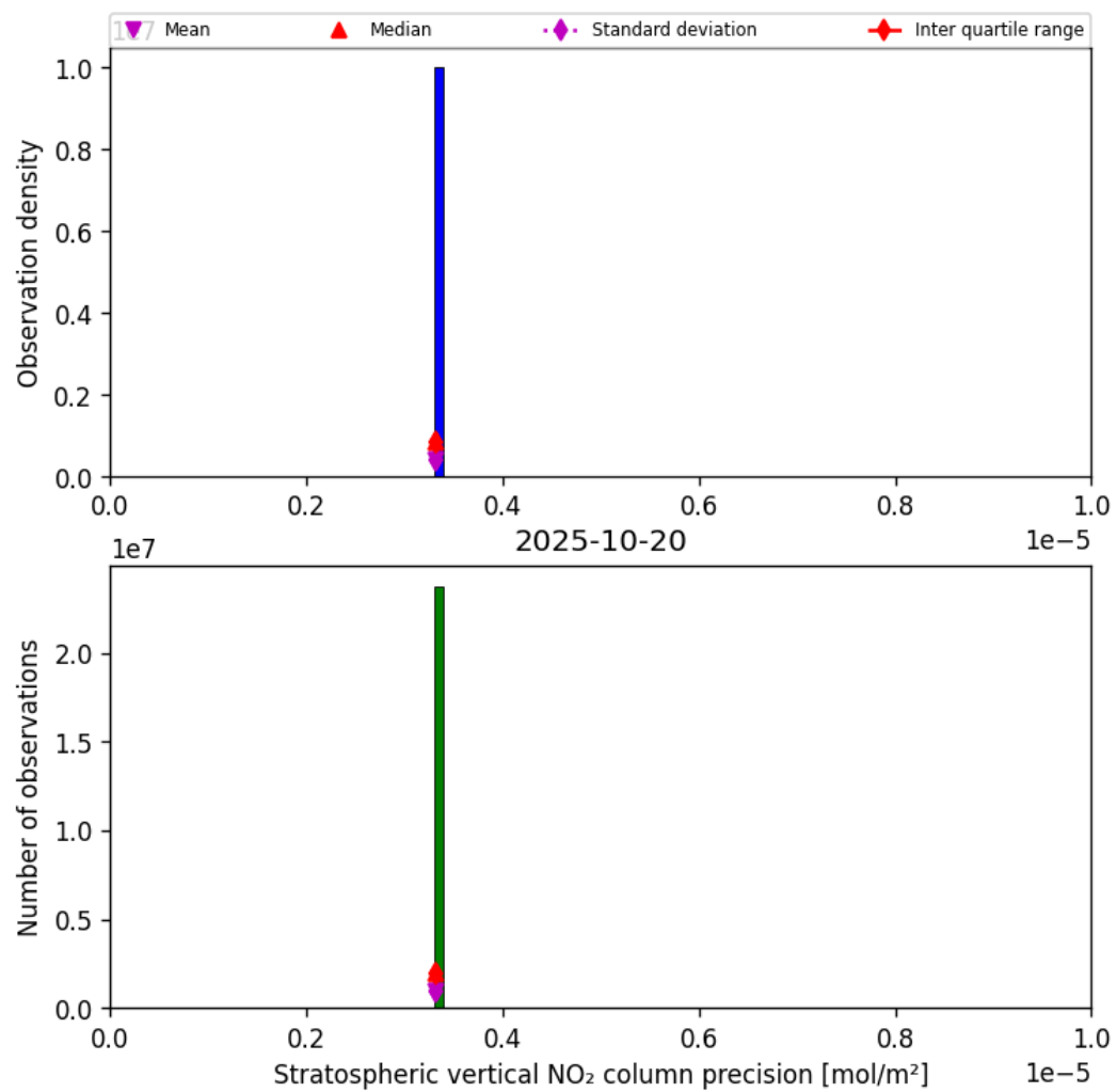
Figure 35: Histogram of “Stratospheric vertical NO 2 column precision” for 2025-10-20 to 2025-10-20
