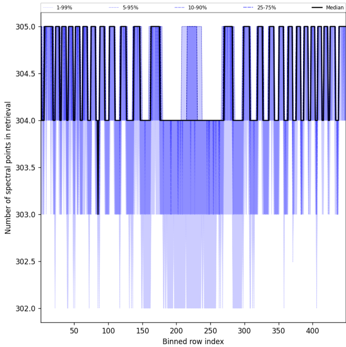
Figure 48: Along track statistics of “Number of spectral points in retrieval” for 2025-10-20 to 2025-10-20
