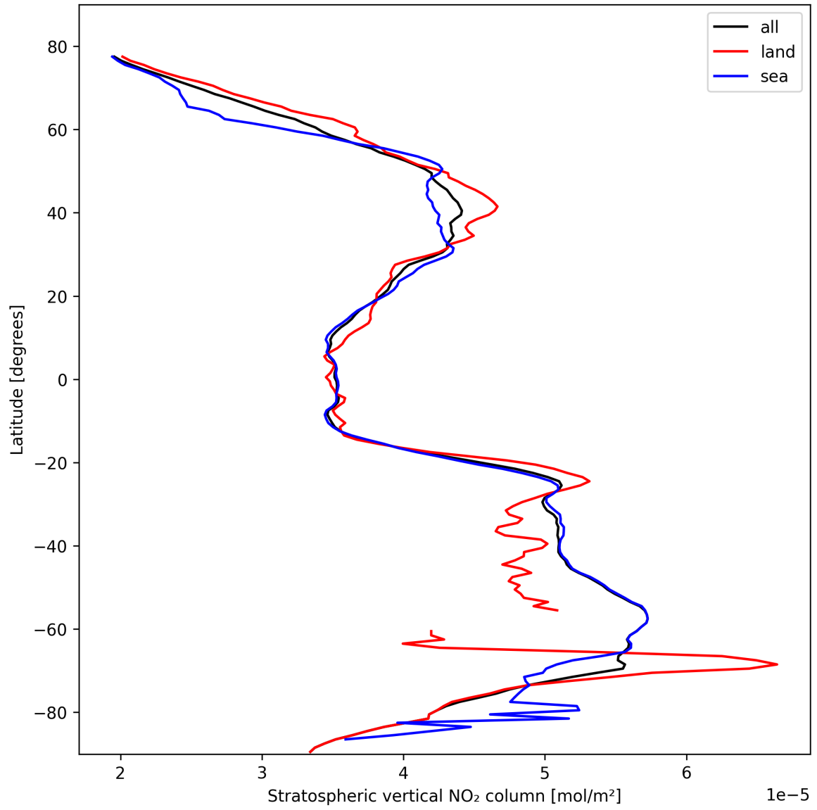
Figure 17: Zonal average of “Stratospheric vertical NO 2 column” for 2025-10-20 to 2025-10-20.
