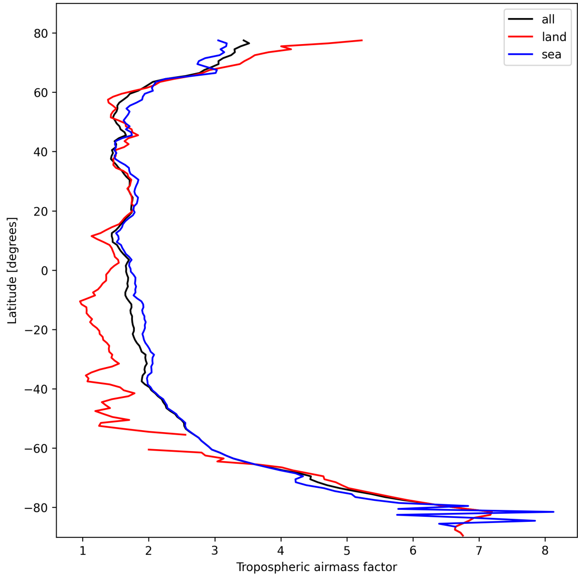
Figure 12: Zonal average of “Tropospheric airmass factor” for 2025-10-20 to 2025-10-20.
