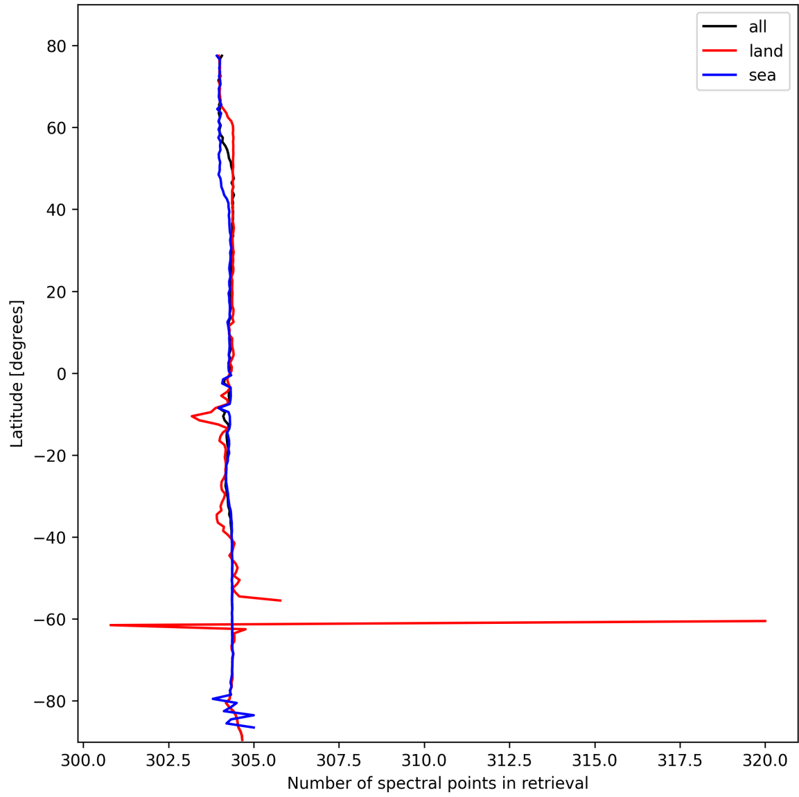
Figure 14: Zonal average of “Number of spectral points in retrieval” for 2025-10-20 to 2025-10-20.
