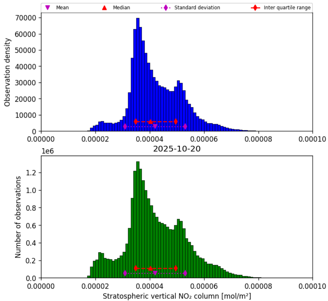
Figure 34: Histogram of “Stratospheric vertical NO 2 column” for 2025-10-20 to 2025-10-20
