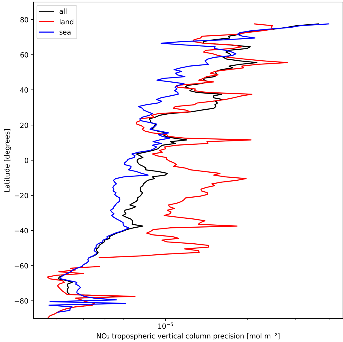
Figure 11: Zonal average of “NO 2 tropospheric vertical column precision” for 2025-10-20 to 2025-10-20.
