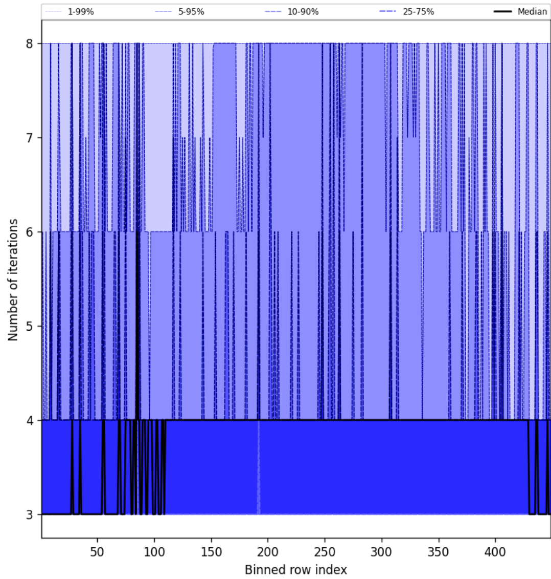
Figure 49: Along track statistics of “Number of iterations” for 2025-10-20 to 2025-10-20
