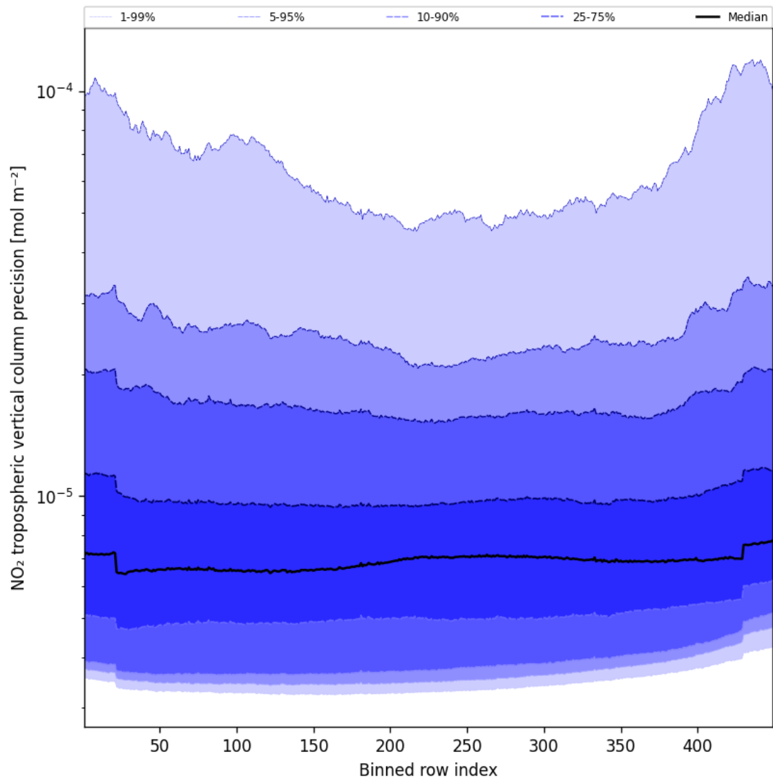
Figure 45: Along track statistics of “NO 2 tropospheric vertical column precision” for 2025-10-20 to 2025-10-20
