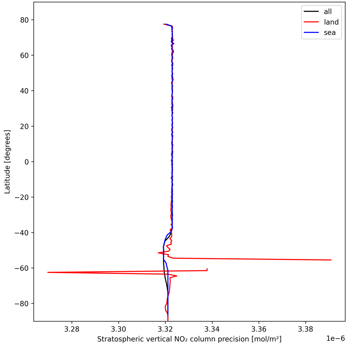
Figure 18: Zonal average of “Stratospheric vertical NO 2 column precision” for 2025-10-20 to 2025-10-20.
