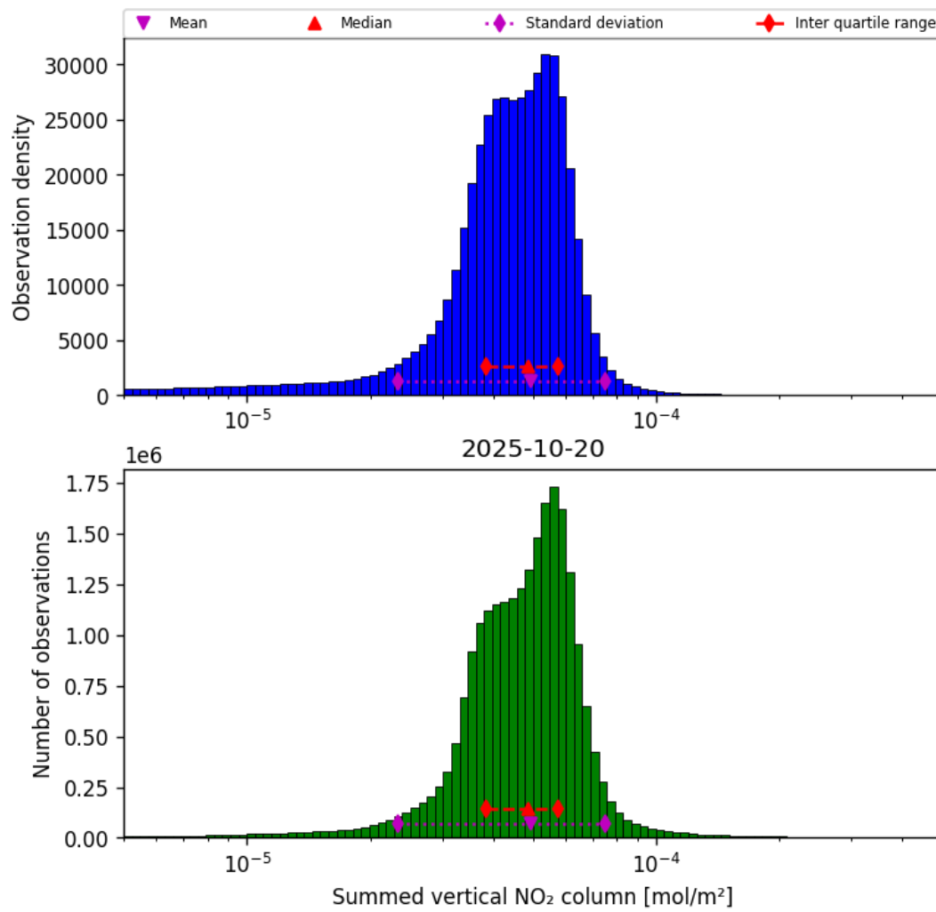
Figure 38: Histogram of "Summed vertical NO 2 column" for 2025-10-20 to 2025-10-20
