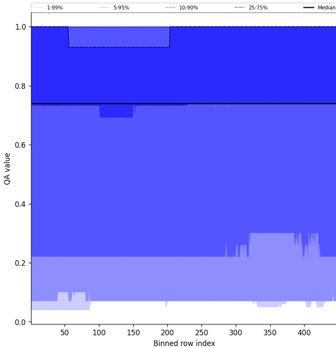
Figure 43: Along track statistics of “QA value” for 2025-10-20 to 2025-10-20
