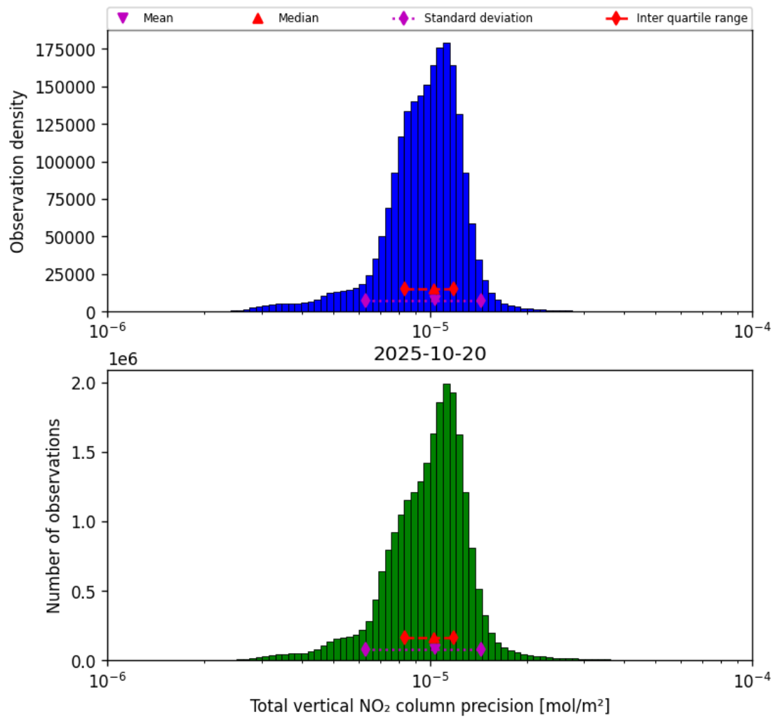
Figure 37: Histogram of "Total vertical NO 2 column precision" for 2025-10-20 to 2025-10-20
