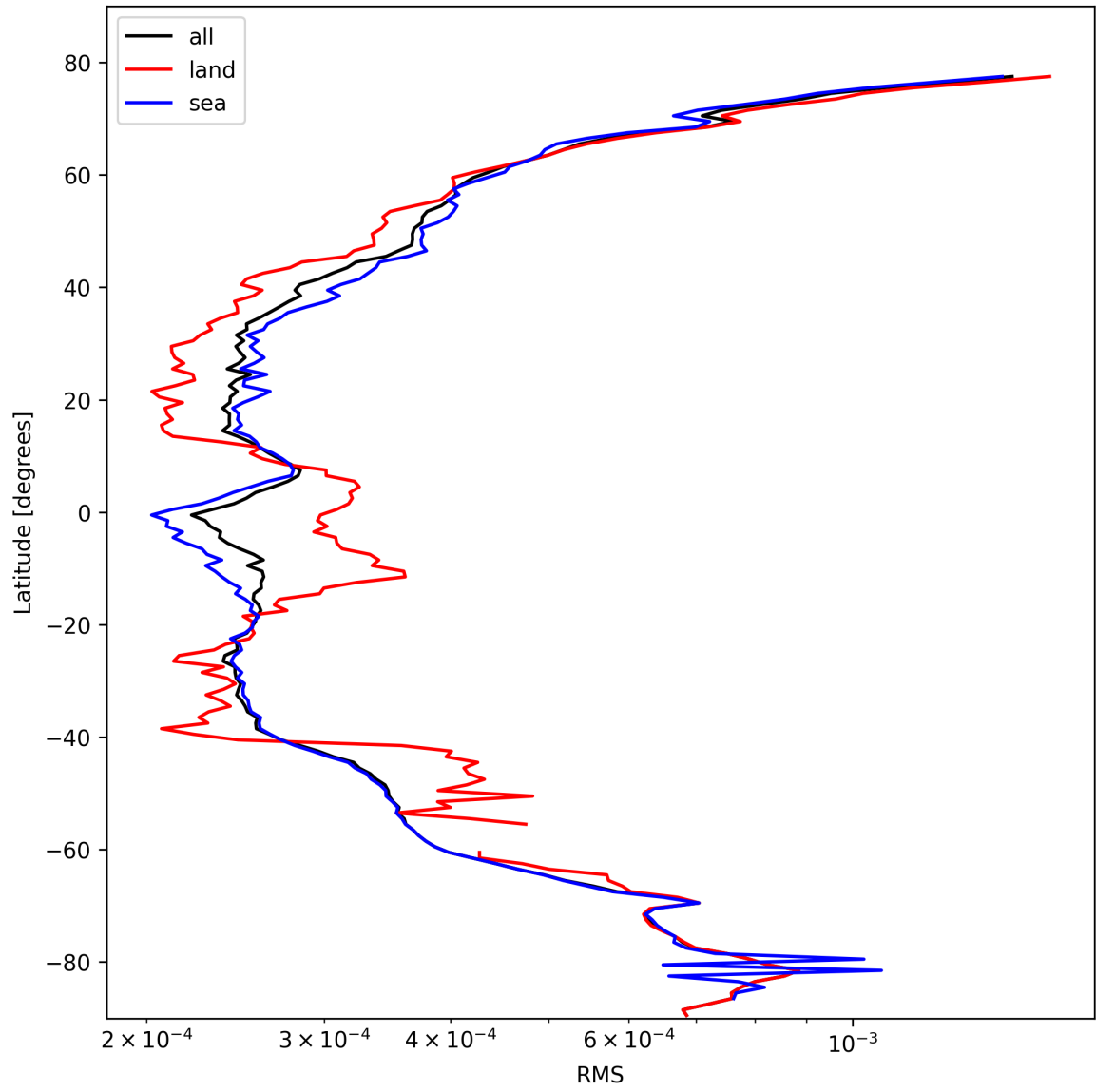
Figure 24: Zonal average of “RMS” for 2025-10-20 to 2025-10-20.
