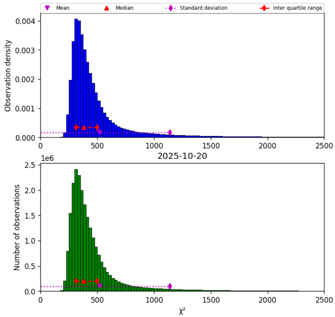
Figure 40: Histogram of “ \chi^2 ” for 2025-10-20 to 2025-10-20
