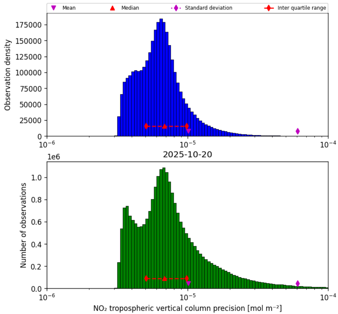
Figure 28: Histogram of “NO 2 tropospheric vertical column precision” for 2025-10-20 to 2025-10-20
