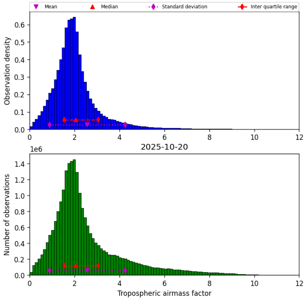
Figure 29: Histogram of “Tropospheric airmass factor” for 2025-10-20 to 2025-10-20
