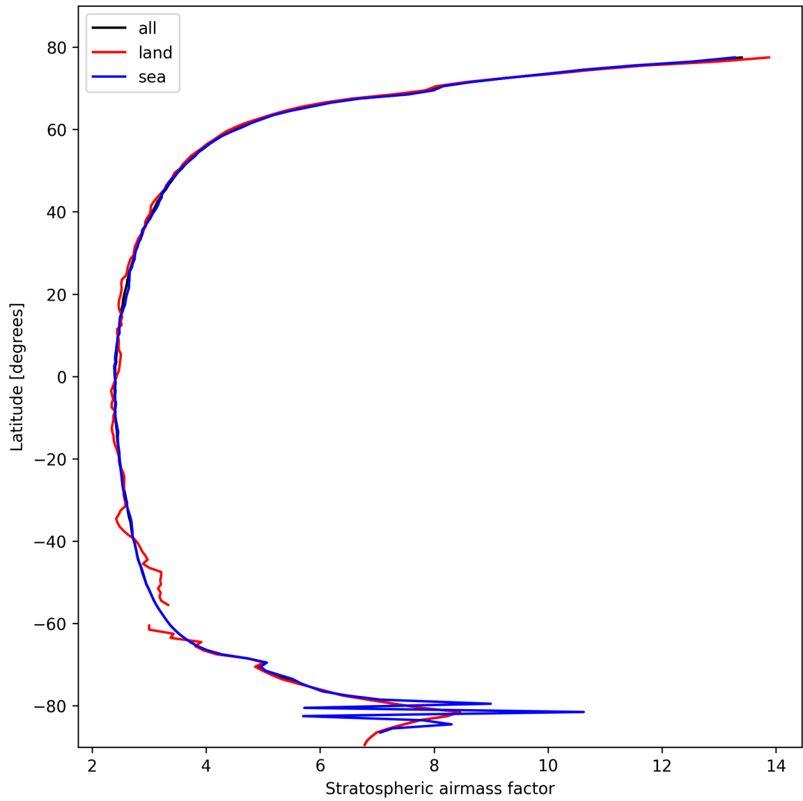
Figure 25: Zonal average of “Stratospheric airmass factor” for 2025-10-20 to 2025-10-20.
