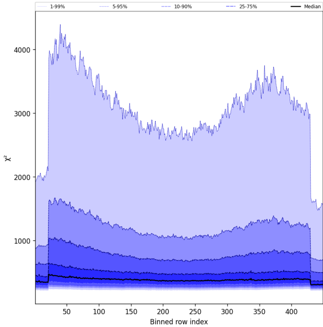
Figure 57: Along track statistics of “ \chi^2 ” for 2025-10-21 to 2025-10-22
