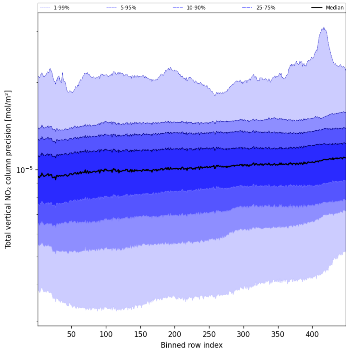
Figure 54: Along track statistics of “Total vertical NO 2 column precision” for 2025-10-21 to 2025-10-22
