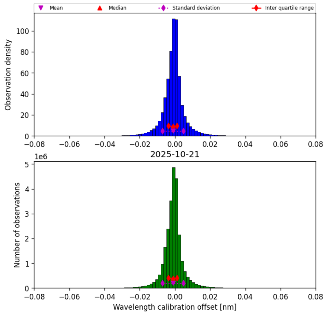
Figure 33: Histogram of “Wavelength calibration offset” for 2025-10-21 to 2025-10-22
