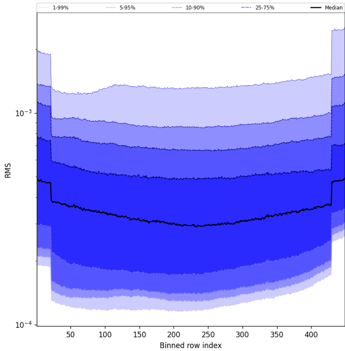
Figure 58: Along track statistics of “RMS” for 2025-10-21 to 2025-10-22
