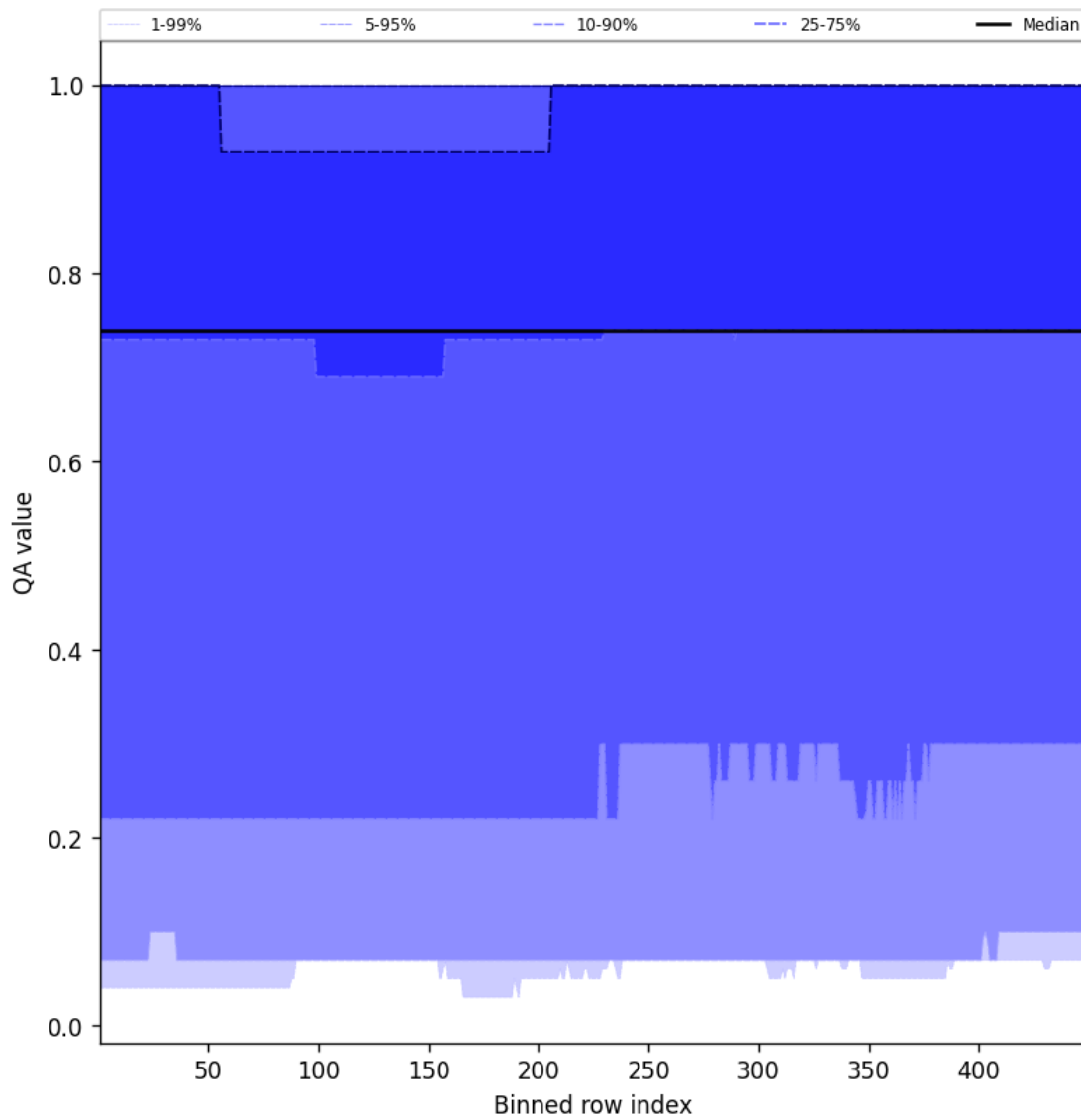
Figure 43: Along track statistics of “QA value” for 2025-10-21 to 2025-10-22
