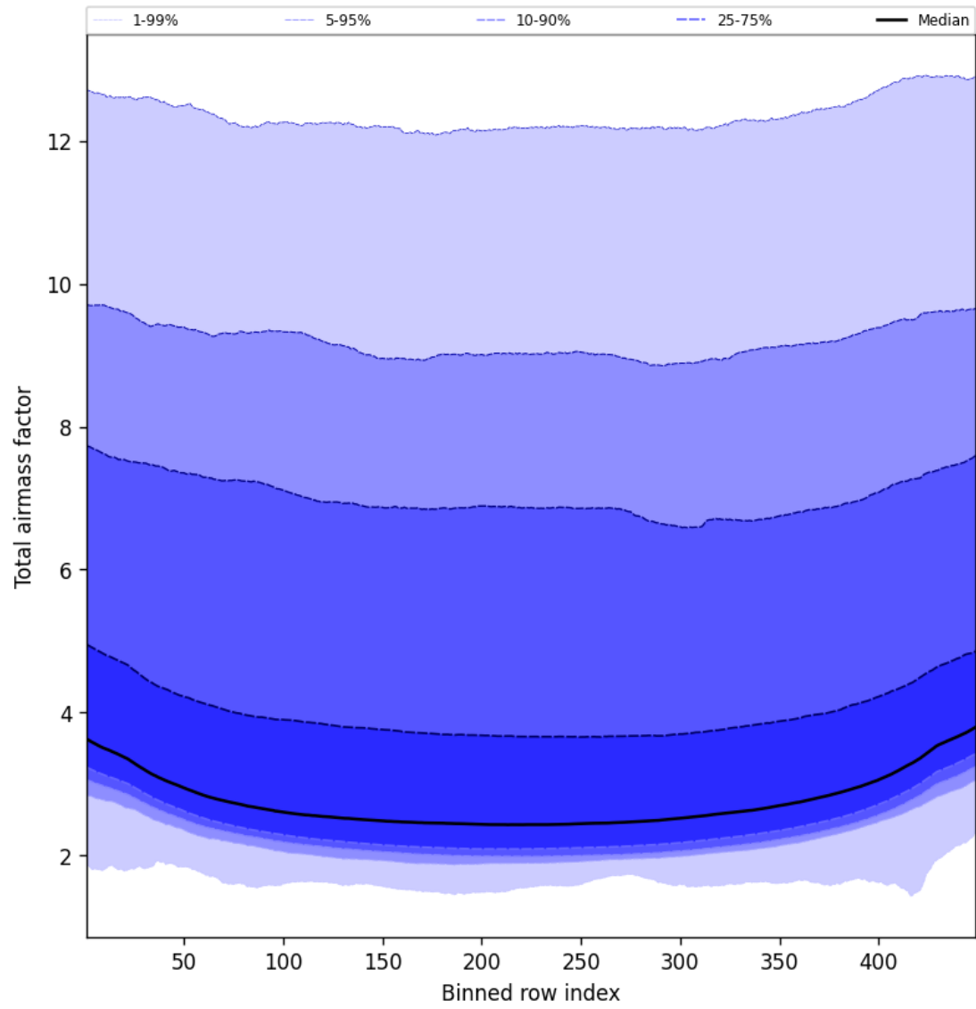
Figure 47: Along track statistics of “Total airmass factor” for 2025-10-21 to 2025-10-22
