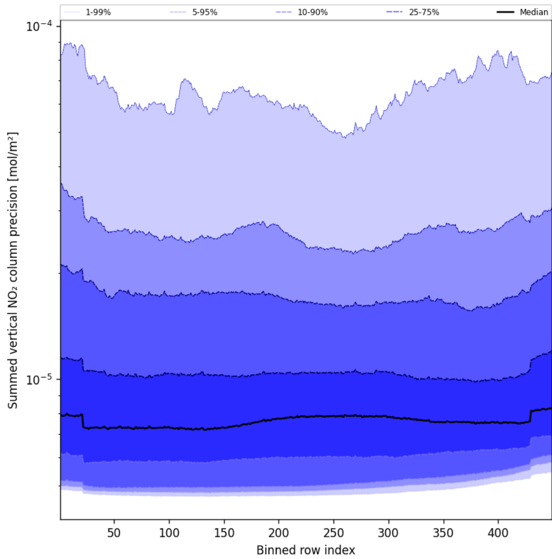
Figure 56: Along track statistics of “Summed vertical NO 2 column precision” for 2025-10-21 to 2025-10-22
