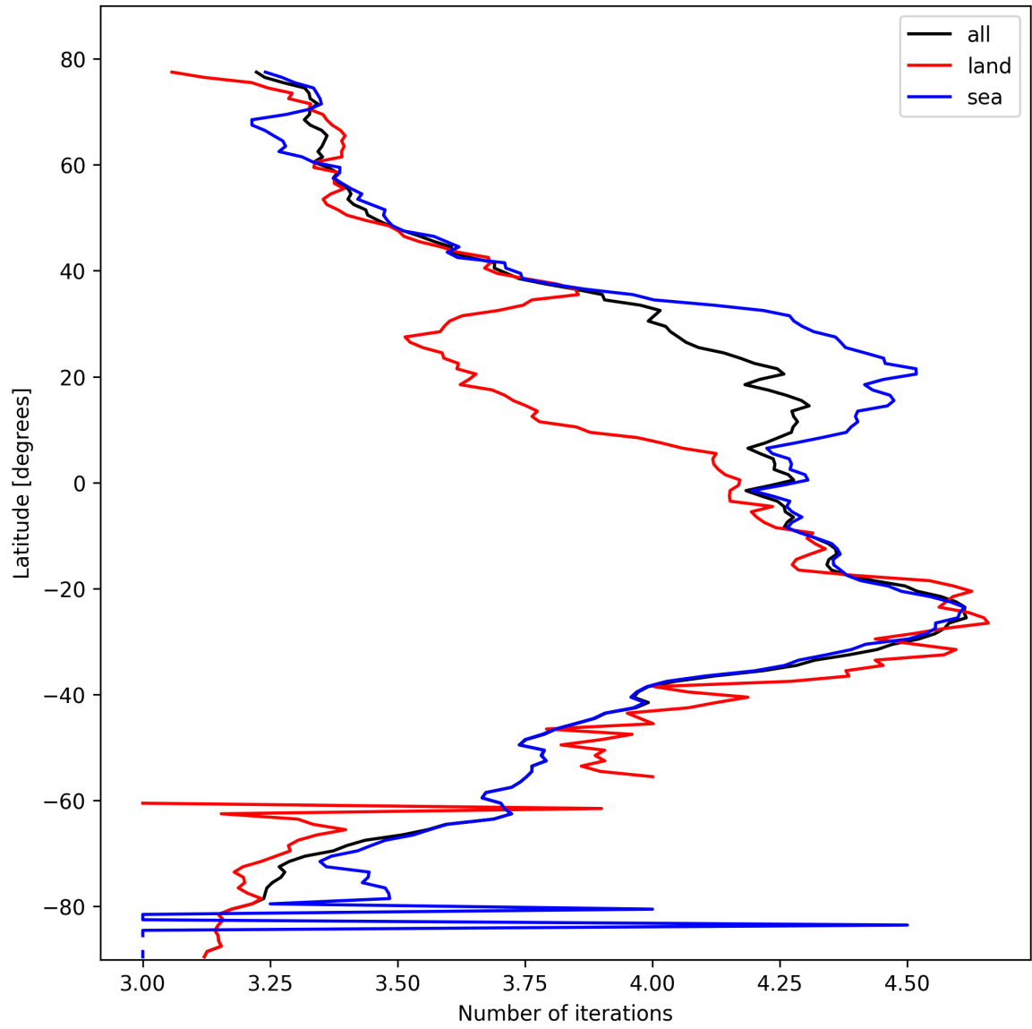
Figure 15: Zonal average of “Number of iterations” for 2025-10-21 to 2025-10-22.
