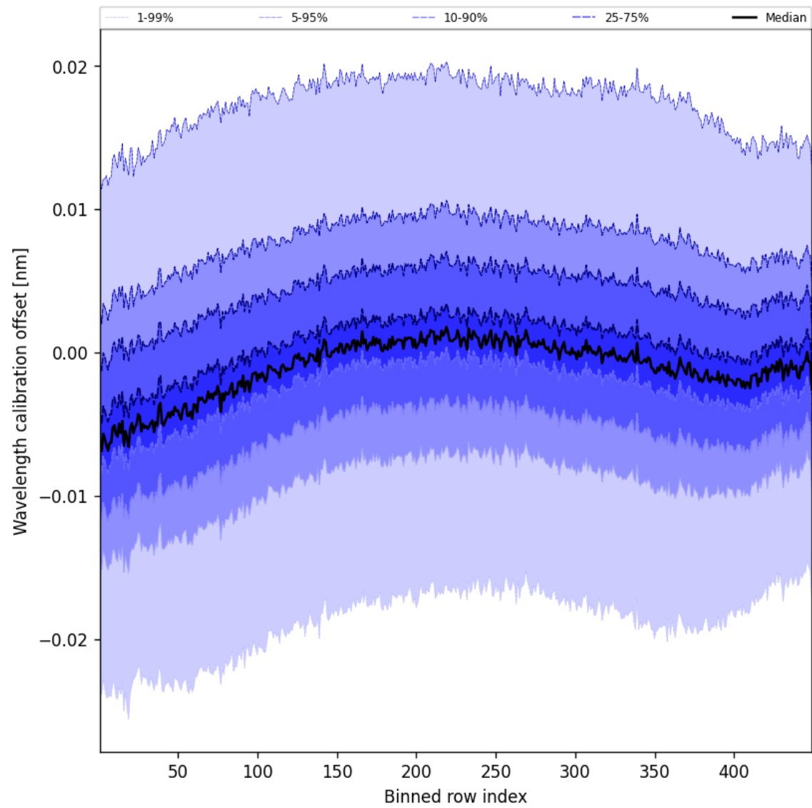
Figure 50: Along track statistics of “Wavelength calibration offset” for 2025-10-21 to 2025-10-22
