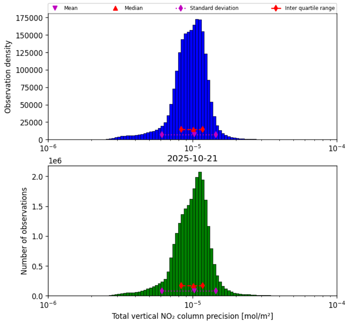
Figure 37: Histogram of “Total vertical NO 2 column precision” for 2025-10-21 to 2025-10-22
