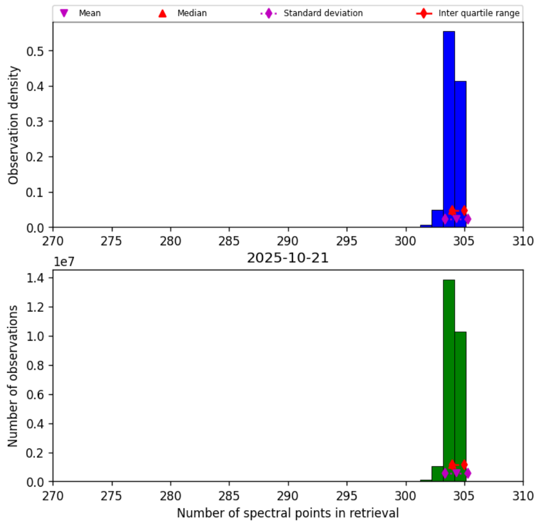
Figure 31: Histogram of “Number of spectral points in retrieval” for 2025-10-21 to 2025-10-22
