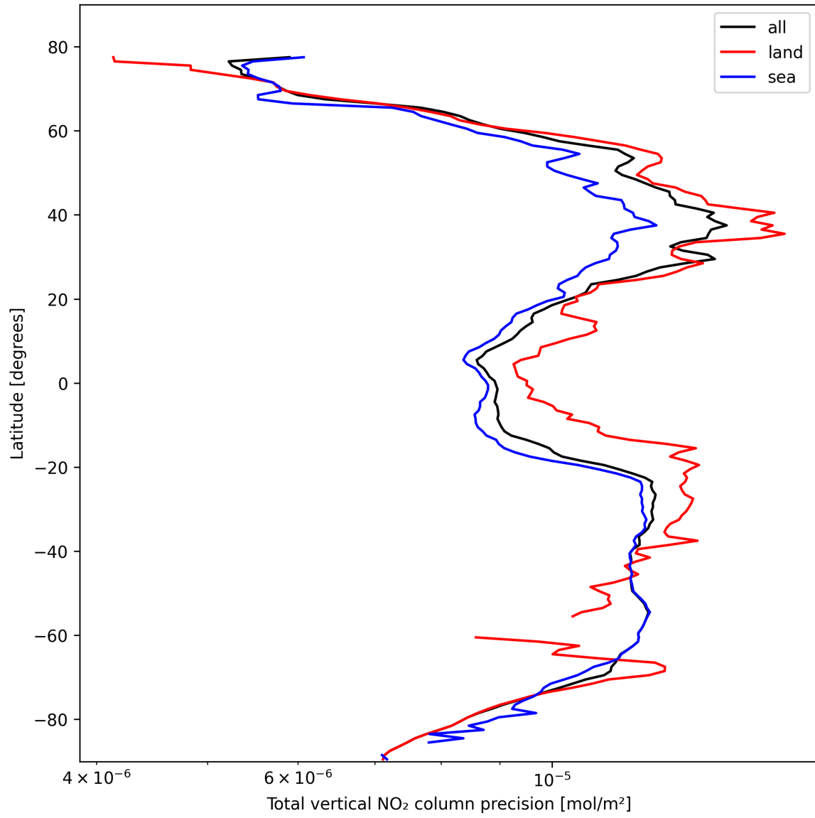
Figure 20: Zonal average of “Total vertical NO 2 column precision” for 2025-10-21 to 2025-10-22.
