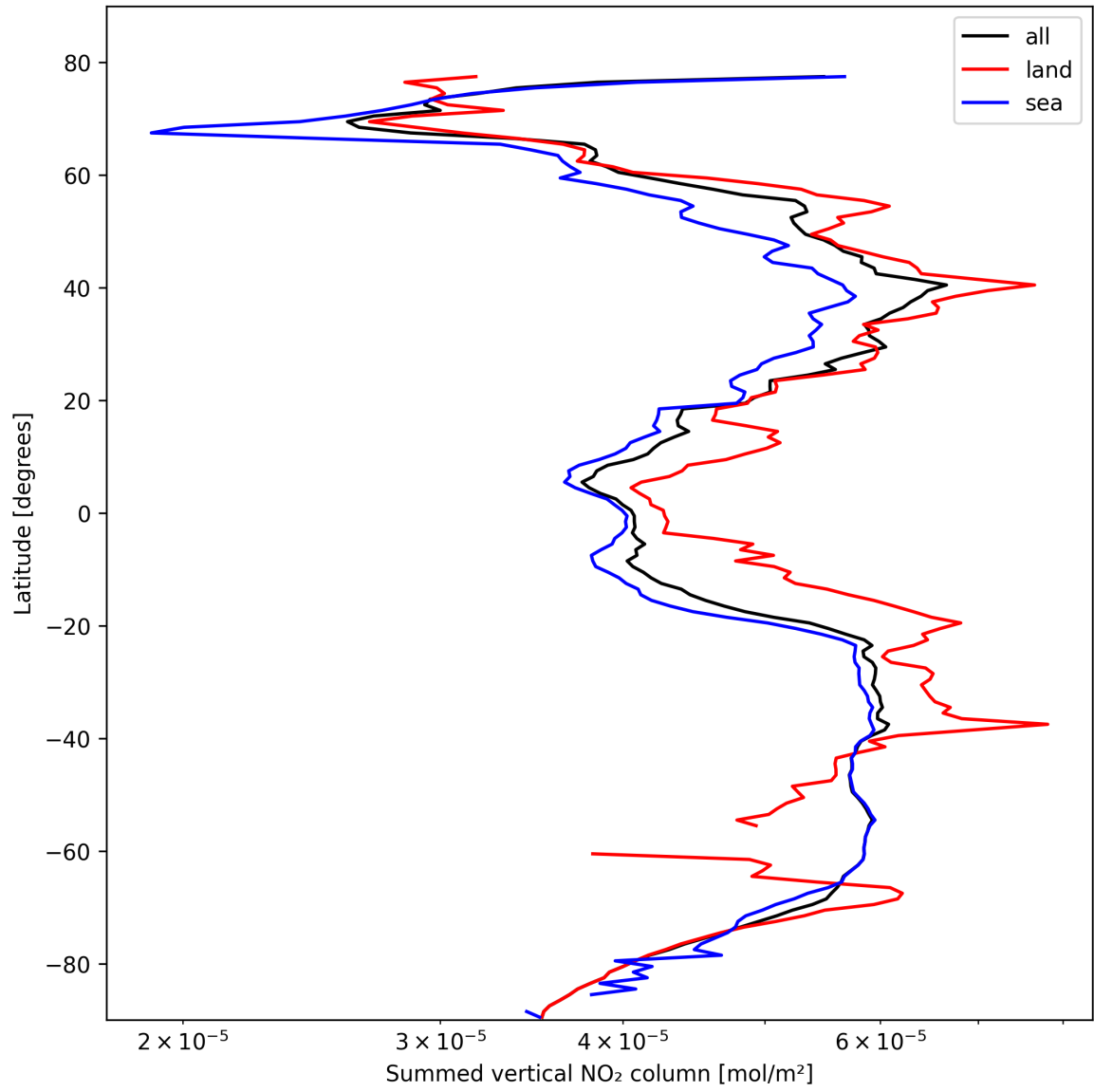
Figure 21: Zonal average of “Summed vertical NO 2 column” for 2025-10-21 to 2025-10-22.
