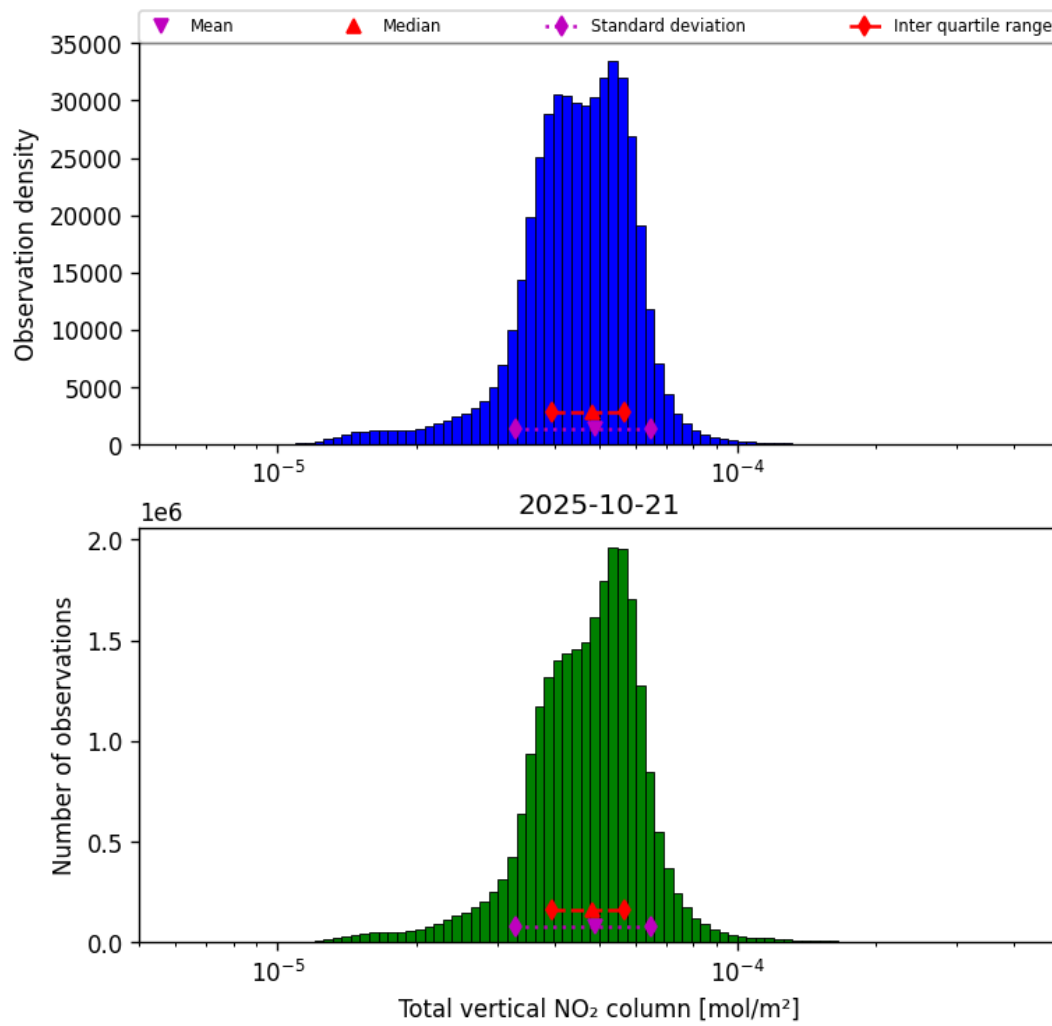
Figure 36: Histogram of “Total vertical NO 2 column” for 2025-10-21 to 2025-10-22
