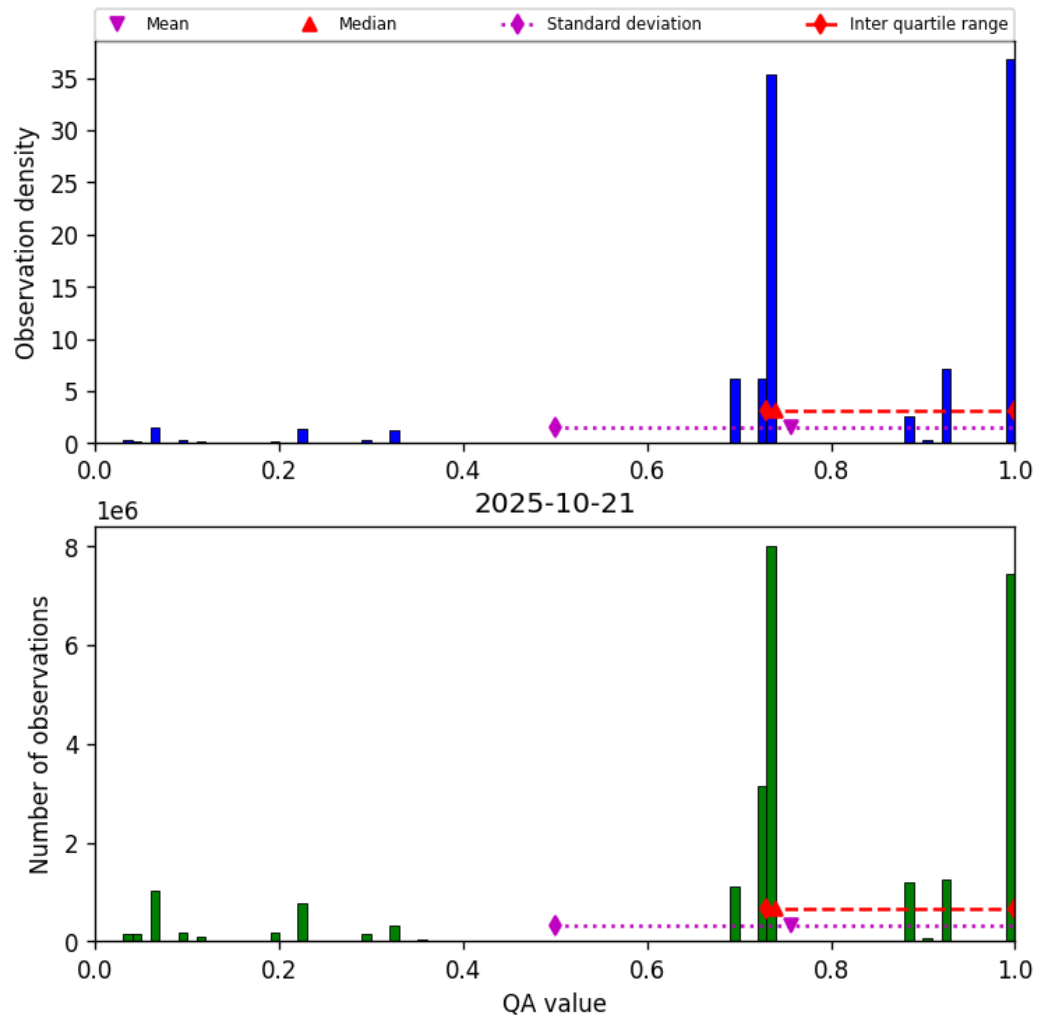
Figure 26: Histogram of “QA value” for 2025-10-21 to 2025-10-22
