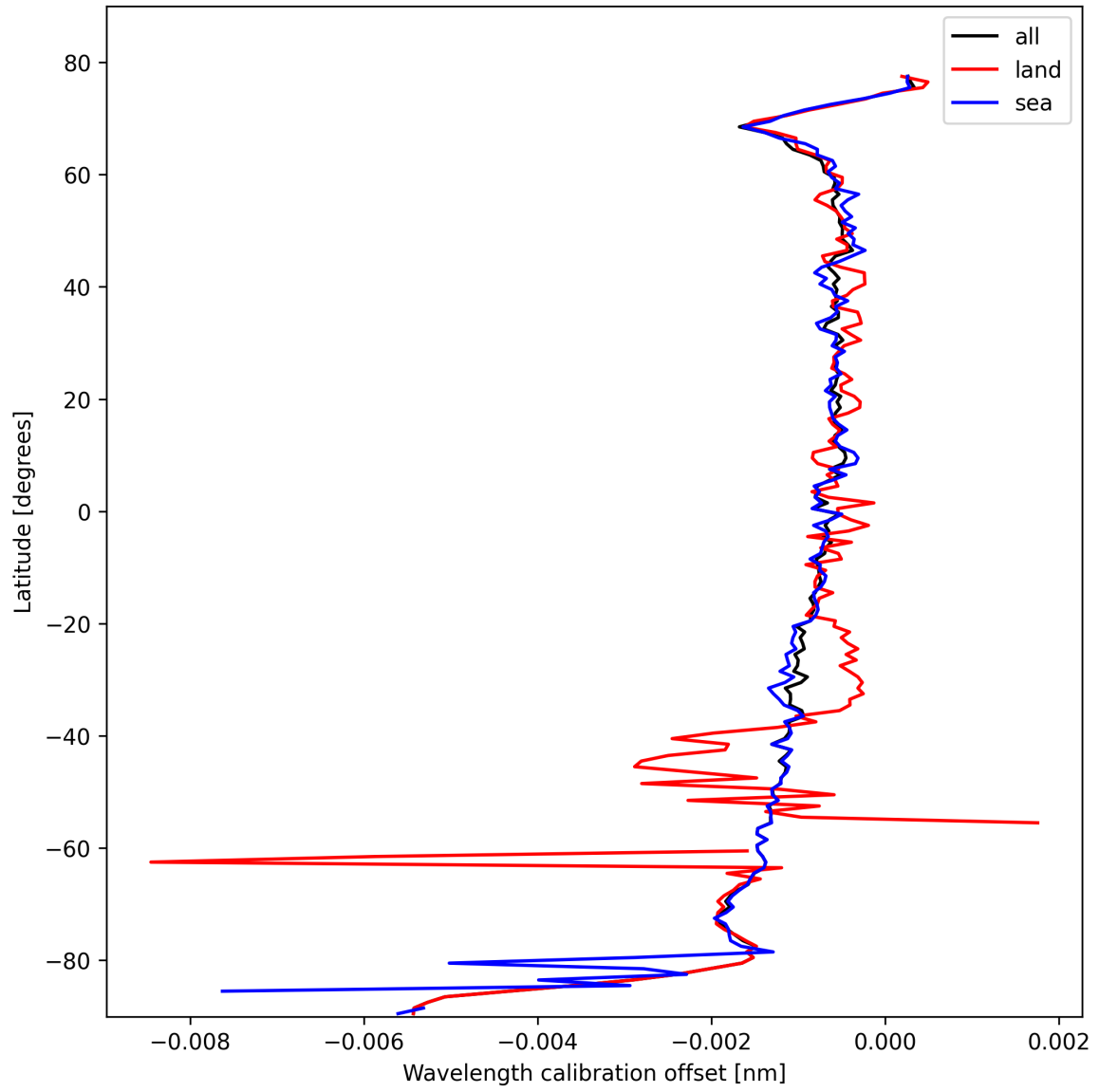
Figure 16: Zonal average of “Wavelength calibration offset” for 2025-10-21 to 2025-10-22.
