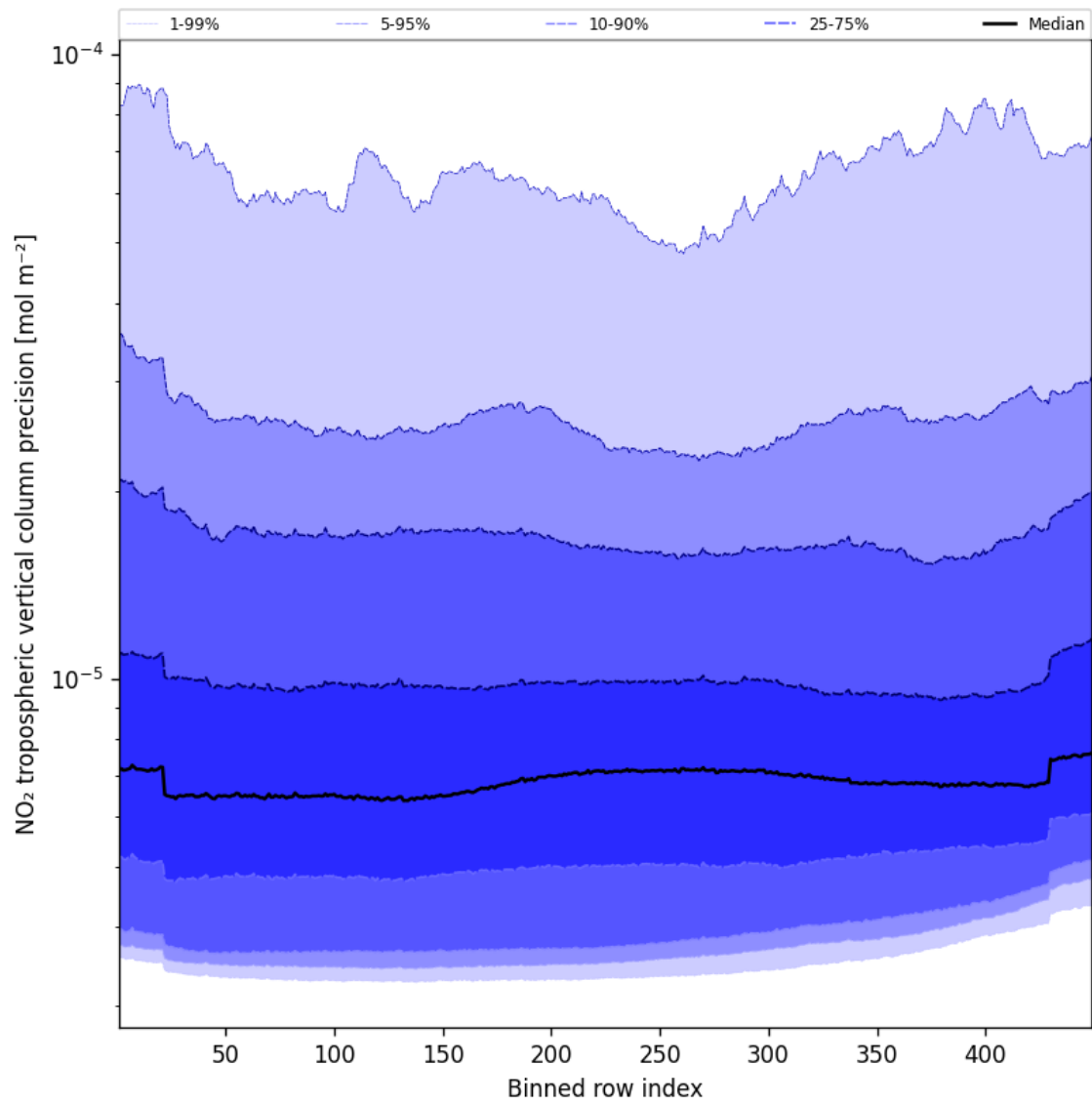
Figure 45: Along track statistics of “NO 2 tropospheric vertical column precision” for 2025-10-21 to 2025-10-22
