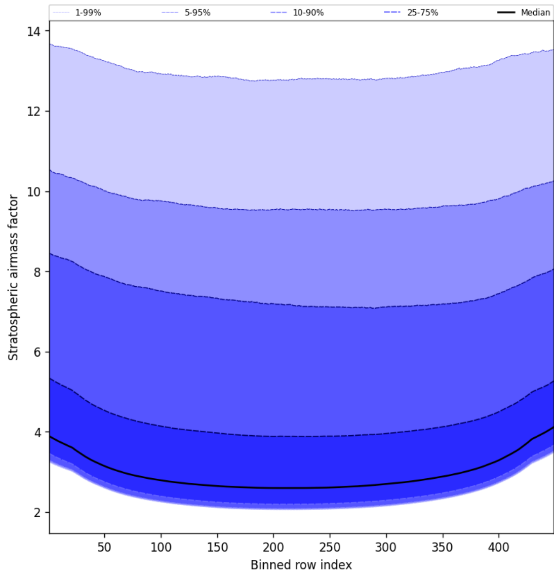
Figure 59: Along track statistics of “Stratospheric air mass factor” for 2025-10-21 to 2025-10-22
