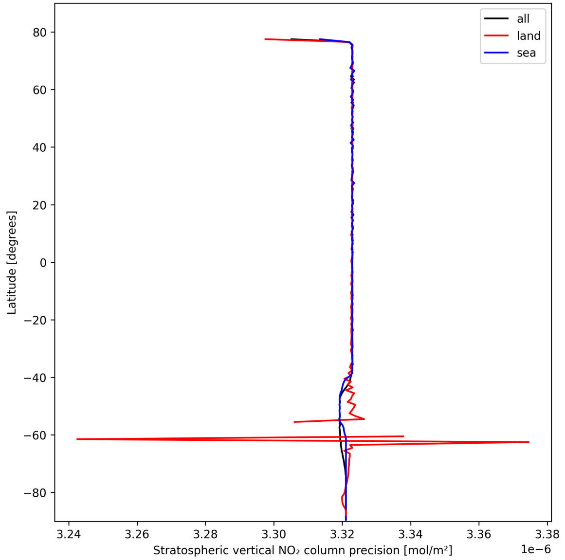
Figure 18: Zonal average of "Stratospheric vertical NO 2 column precision" for 2025-10-21 to 2025-10-22.
