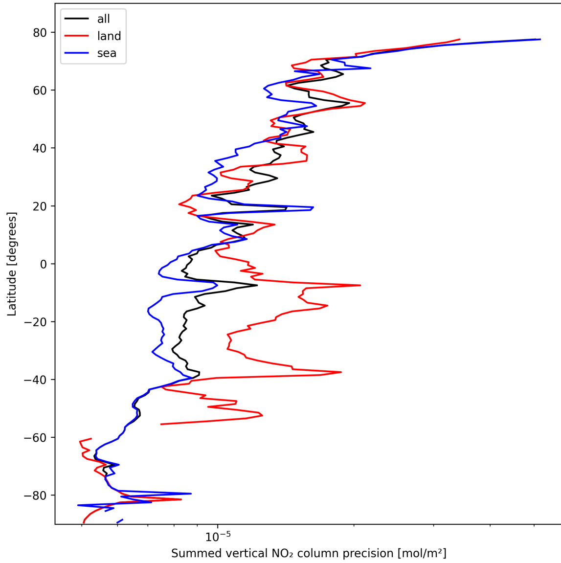
Figure 22: Zonal average of “Summed vertical NO 2 column precision” for 2025-10-21 to 2025-10-22.
