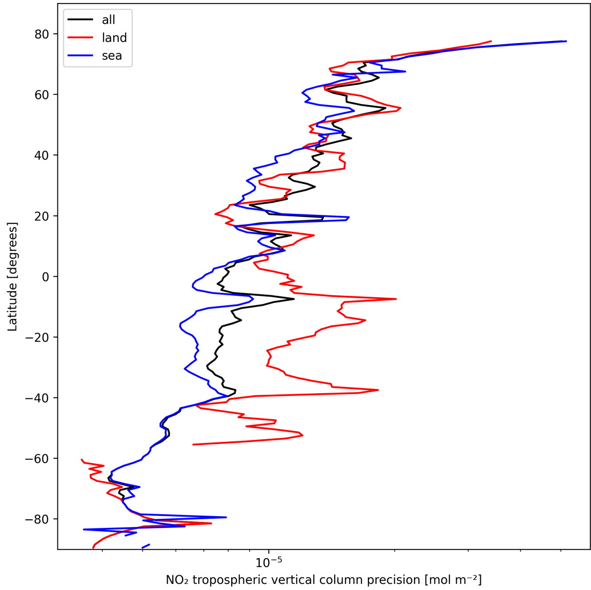
Figure 11: Zonal average of “NO 2 tropospheric vertical column precision” for 2025-10-21 to 2025-10-22.
