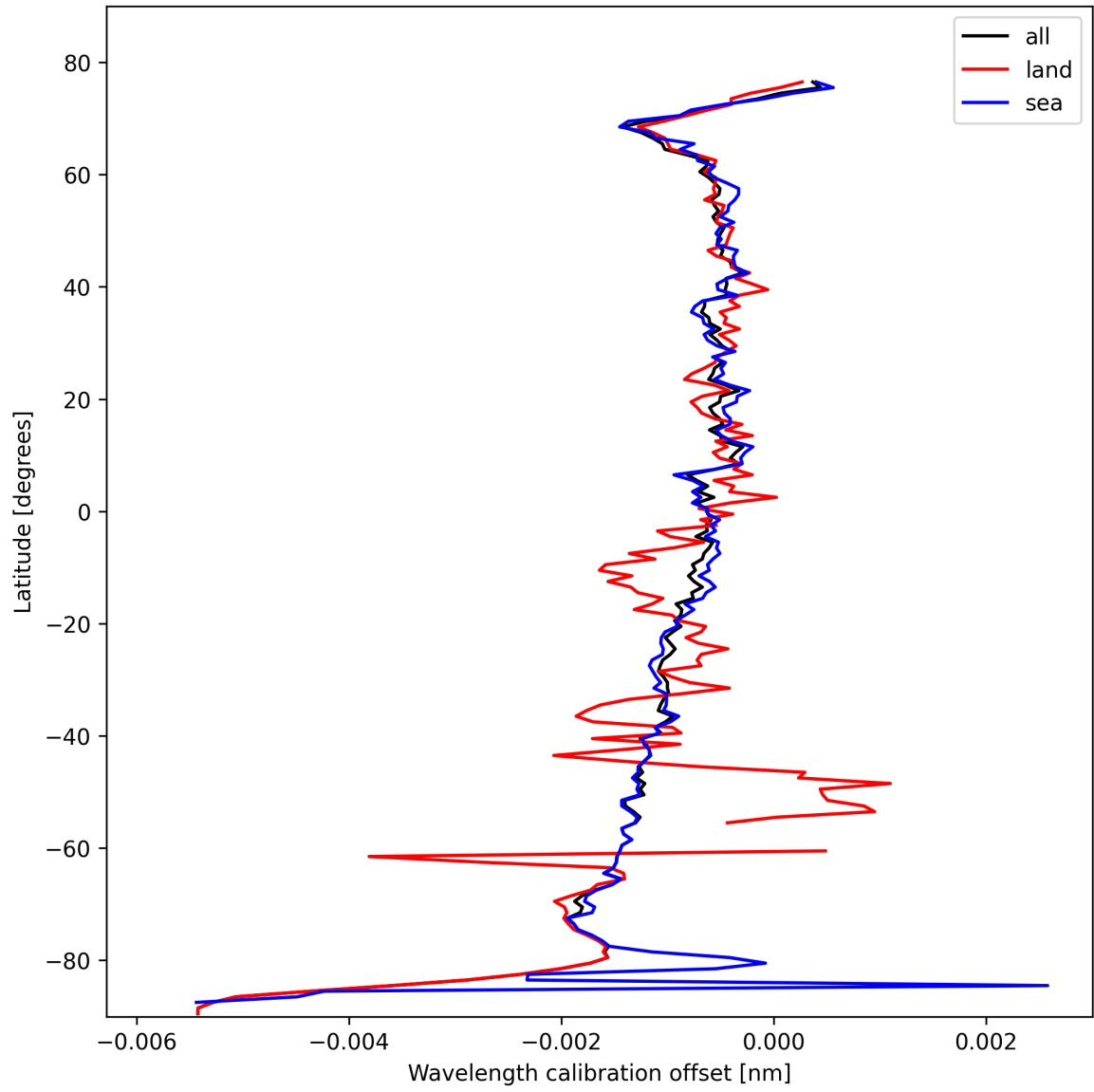
Figure 16: Zonal average of “Wavelength calibration offset” for 2025-10-22 to 2025-10-23.
