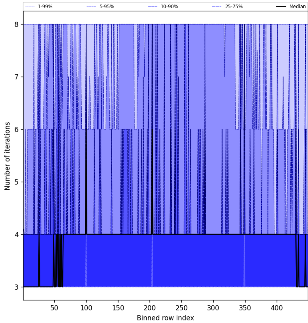
Figure 49: Along track statistics of “Number of iterations” for 2025-10-22 to 2025-10-23
