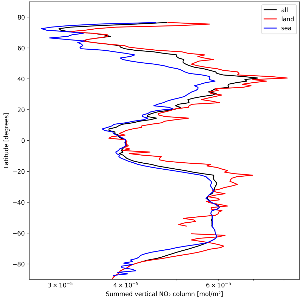
Figure 21: Zonal average of “Summed vertical NO 2 column” for 2025-10-22 to 2025-10-23.
