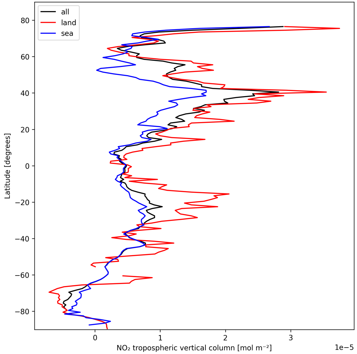
Figure 10: Zonal average of “NO 2 tropospheric vertical column” for 2025-10-22 to 2025-10-23.
