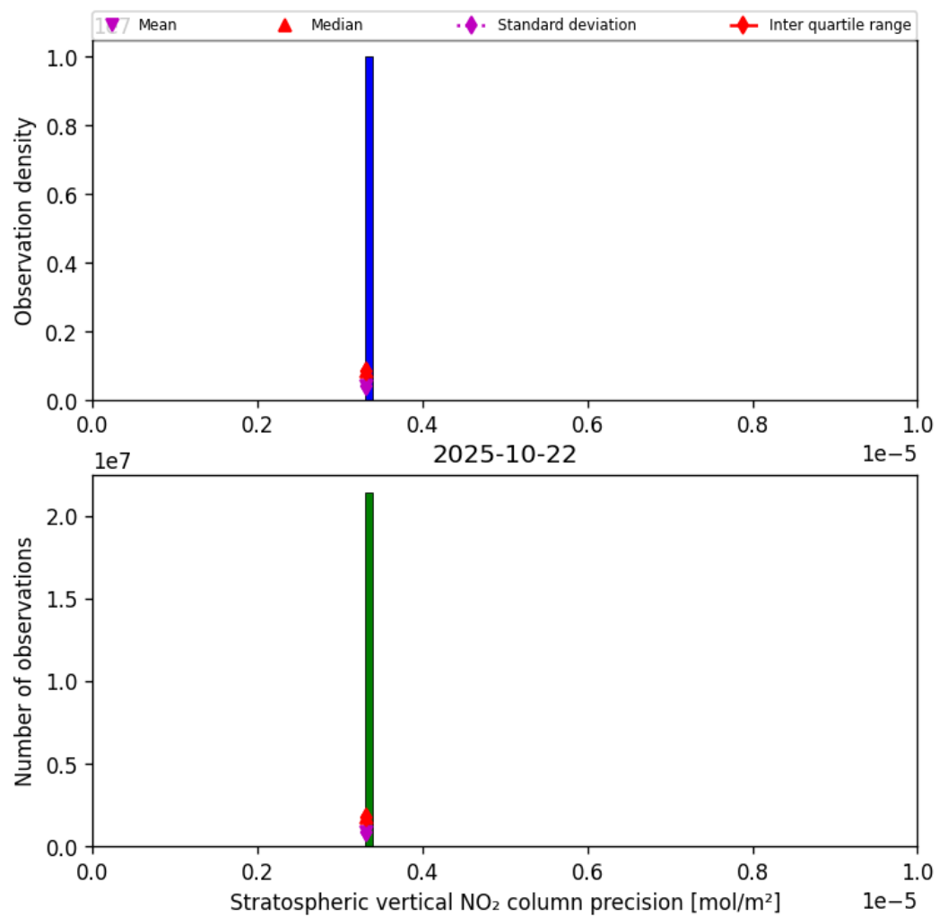
Figure 35: Histogram of “Stratospheric vertical NO 2 column precision” for 2025-10-22 to 2025-10-23
