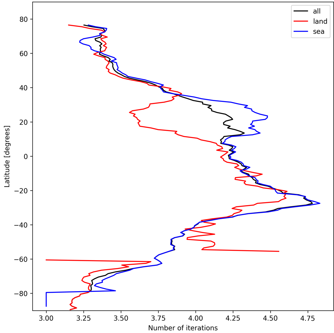
Figure 15: Zonal average of “Number of iterations” for 2025-10-22 to 2025-10-23.
