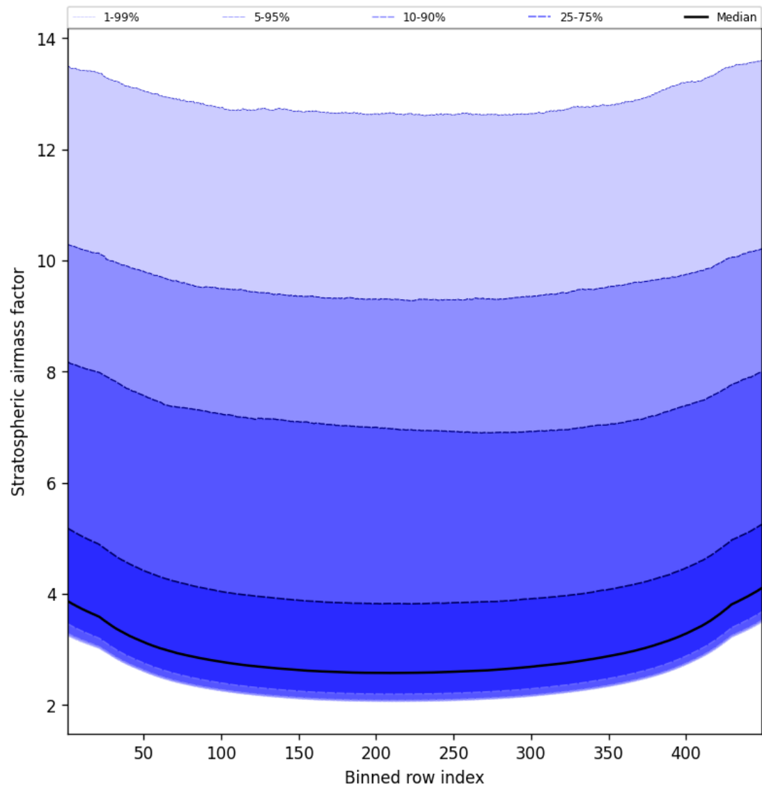
Figure 59: Along track statistics of “Stratospheric airmass factor” for 2025-10-22 to 2025-10-23
