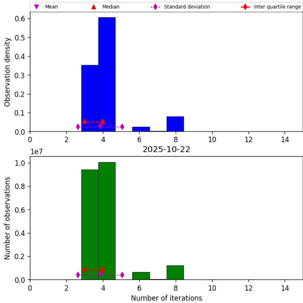
Figure 32: Histogram of “Number of iterations” for 2025-10-22 to 2025-10-23
