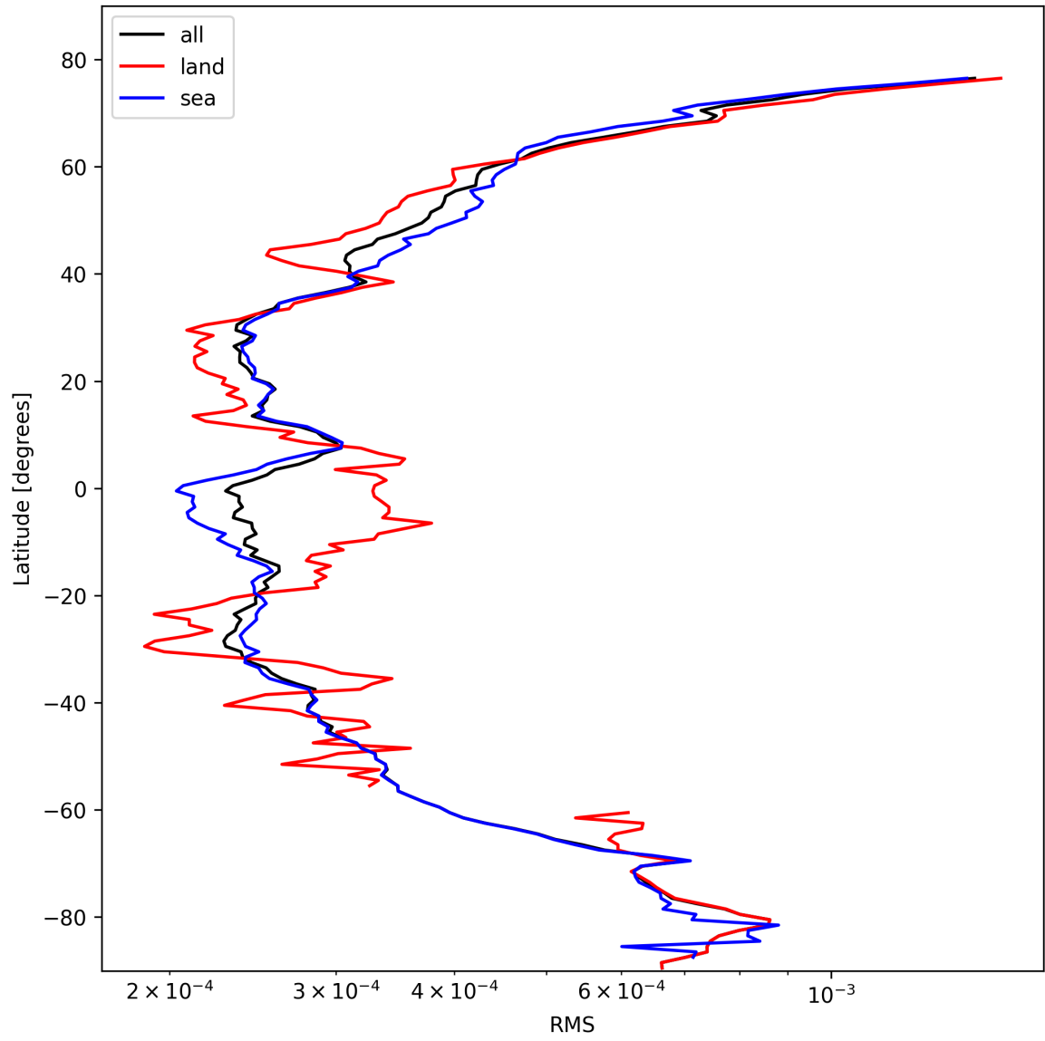
Figure 24: Zonal average of “RMS” for 2025-10-22 to 2025-10-23.
