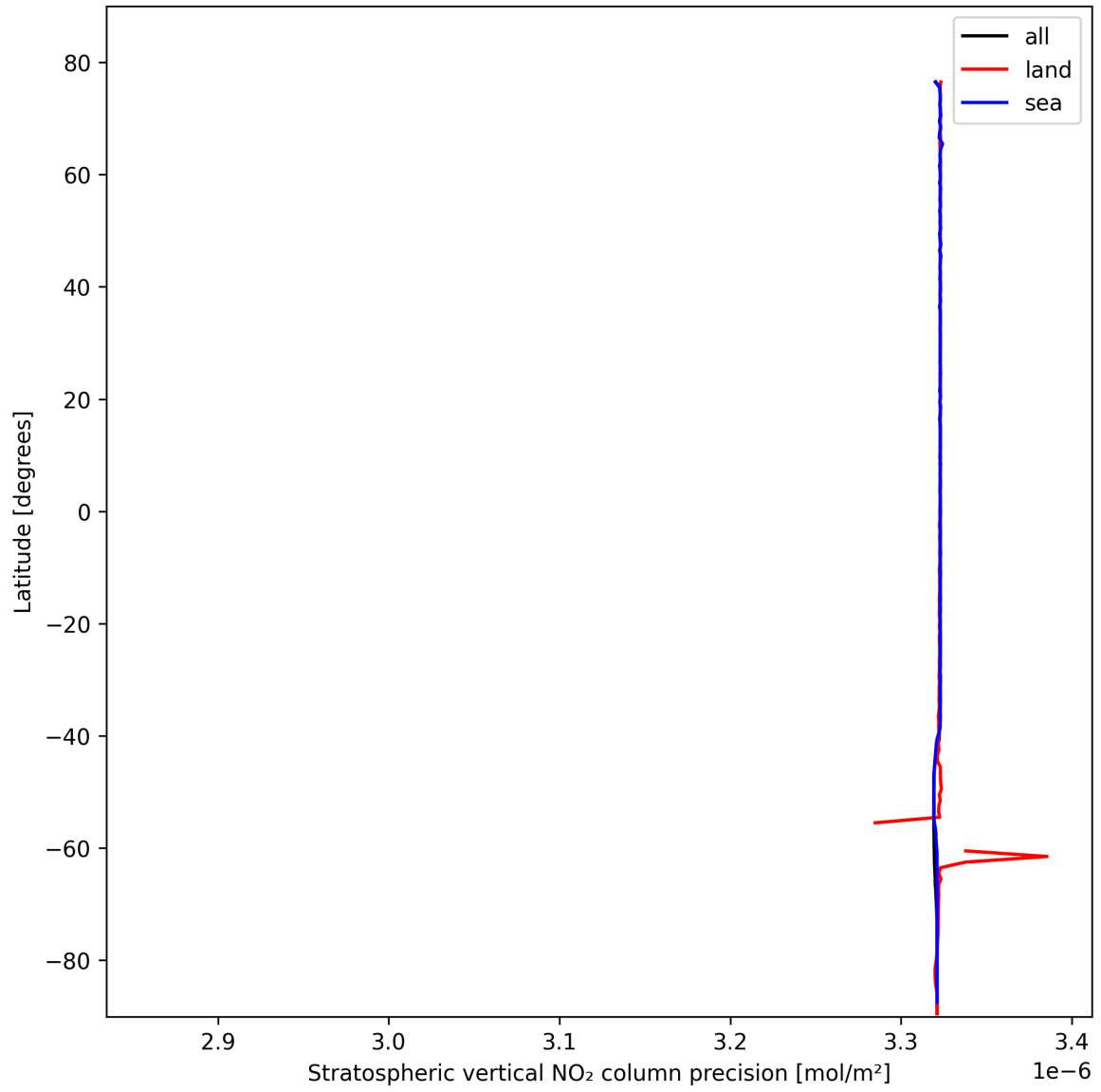
Figure 18: Zonal average of “Stratospheric vertical NO 2 column precision” for 2025-10-22 to 2025-10-23.
