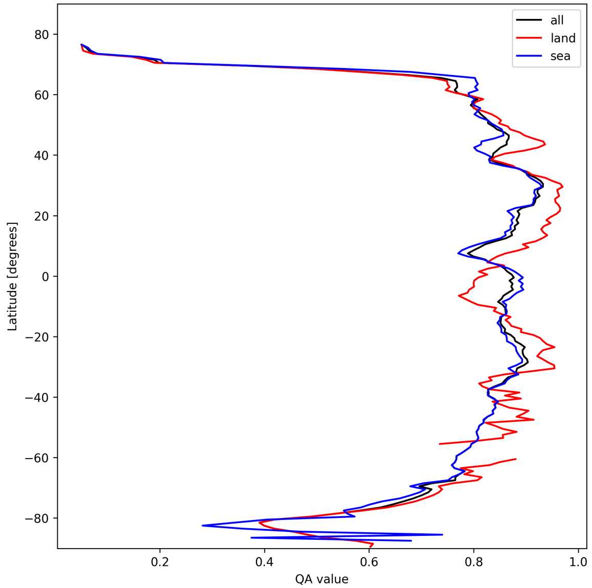
Figure 9: Zonal average of “QA value” for 2025-10-22 to 2025-10-23.
