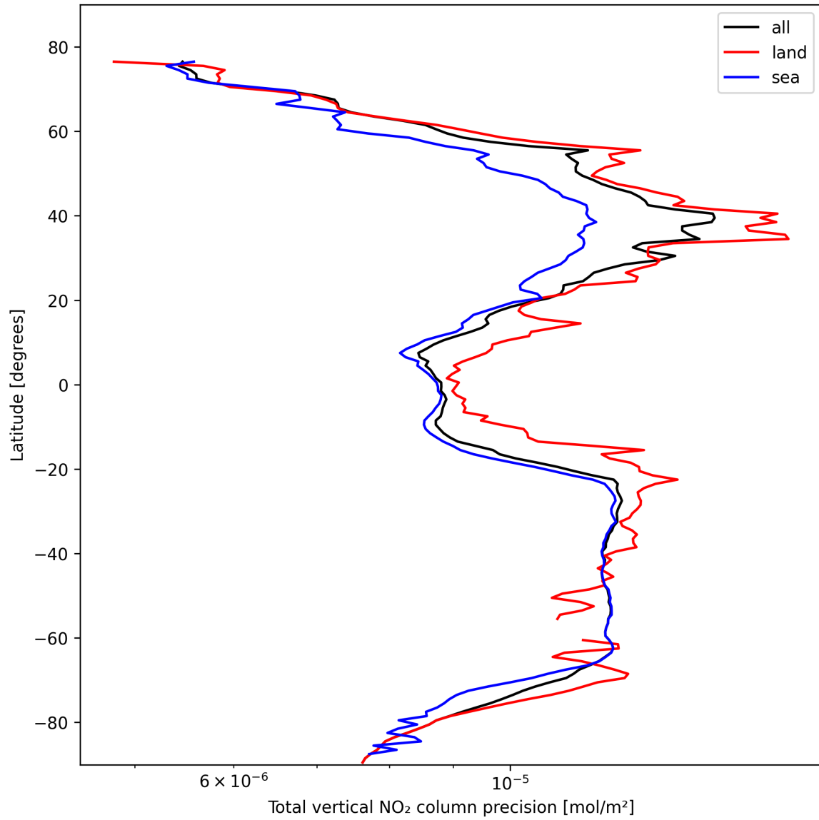
Figure 20: Zonal average of “Total vertical NO 2 column precision” for 2025-10-22 to 2025-10-23.
