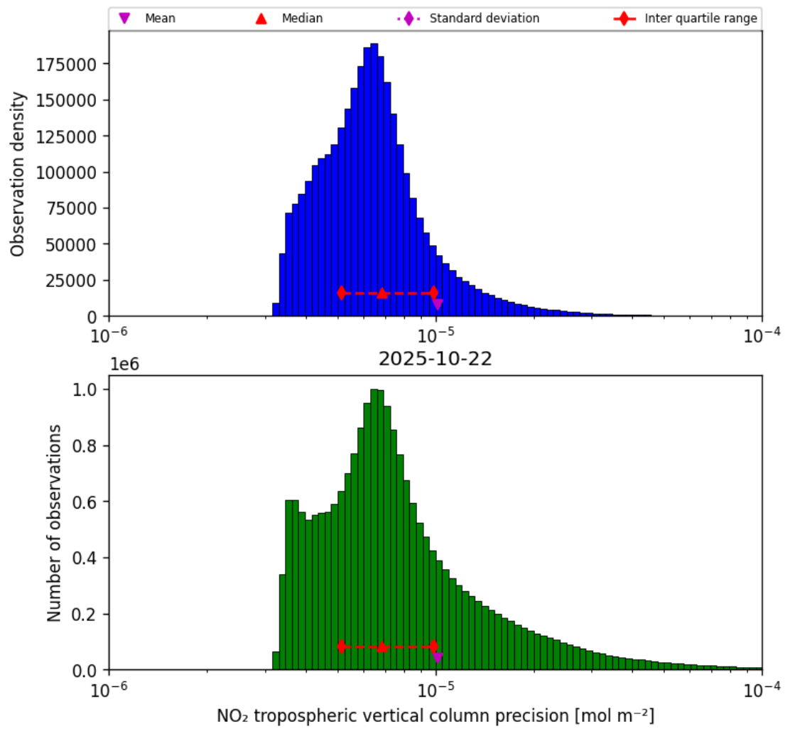
Figure 28: Histogram of "NO 2 tropospheric vertical column precision" for 2025-10-22 to 2025-10-23
