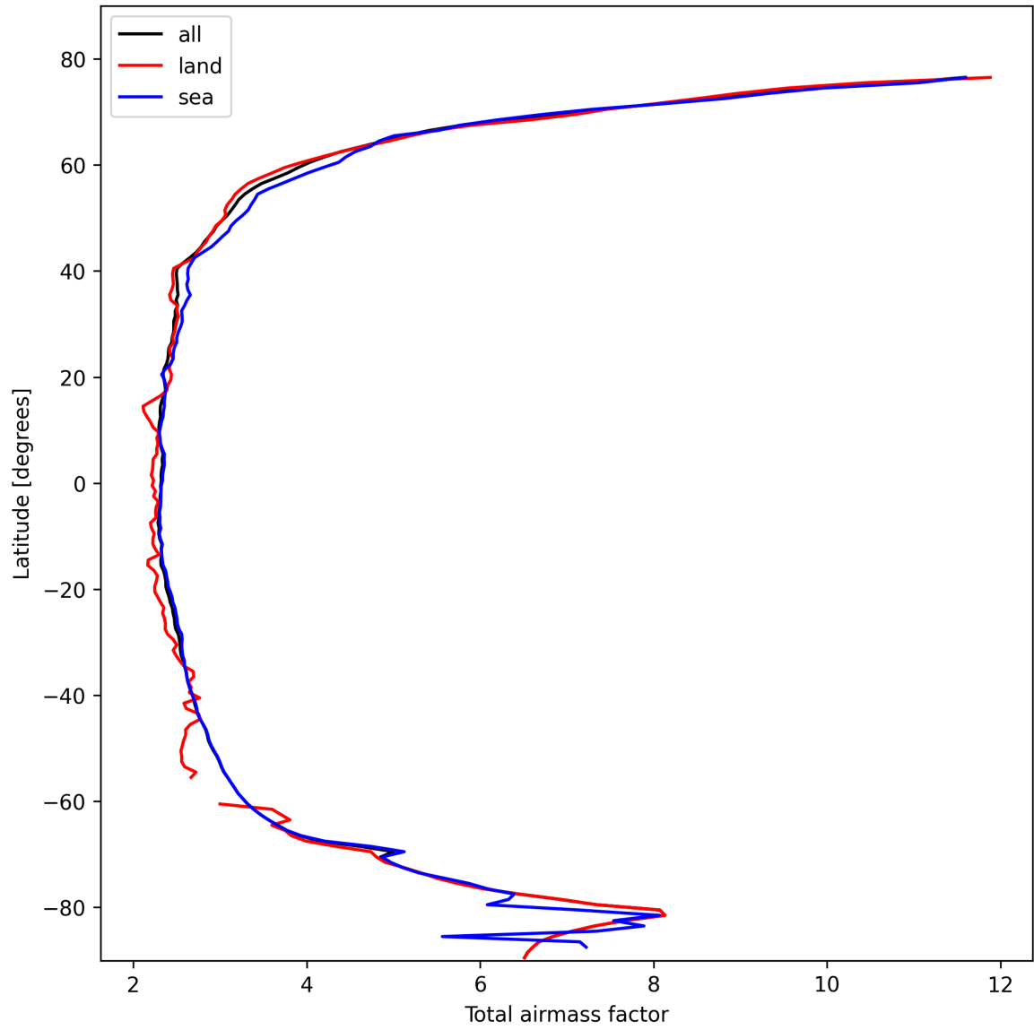
Figure 13: Zonal average of “Total airmass factor” for 2025-10-22 to 2025-10-23.
