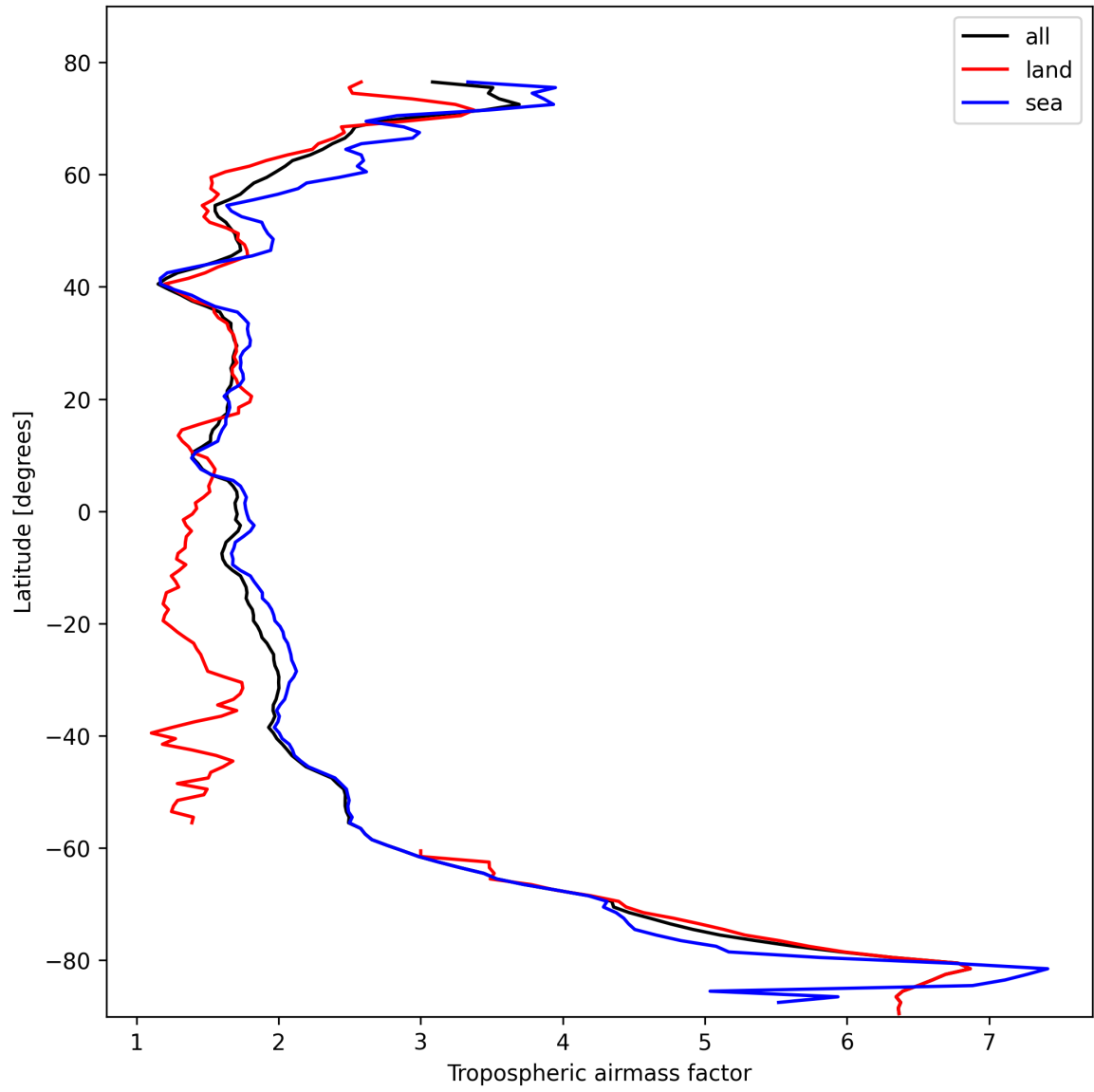
Figure 12: Zonal average of “Tropospheric airmass factor” for 2025-10-22 to 2025-10-23.
