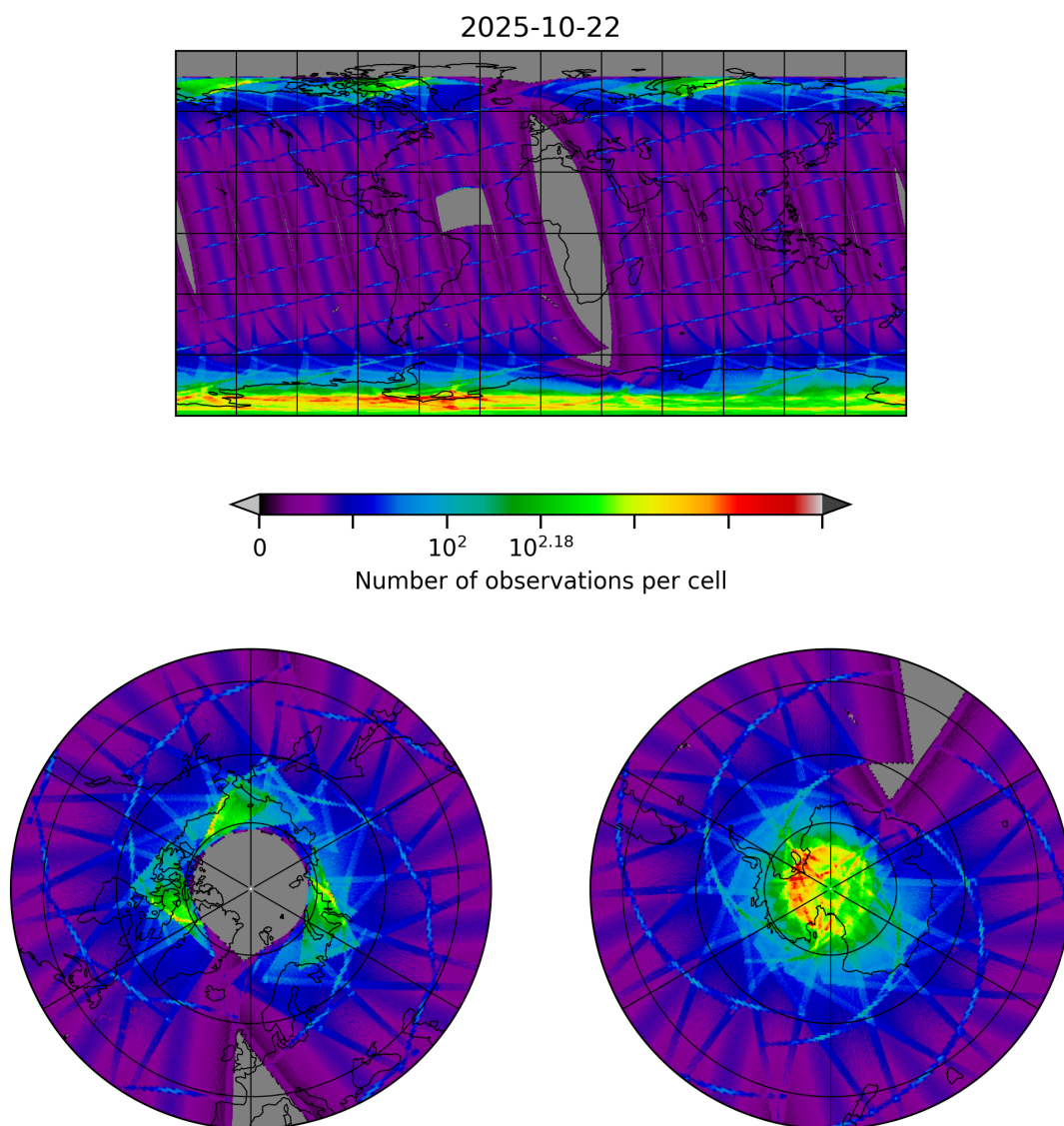
Figure 8: Map of the number of observations for 2025-10-22 to 2025-10-23
