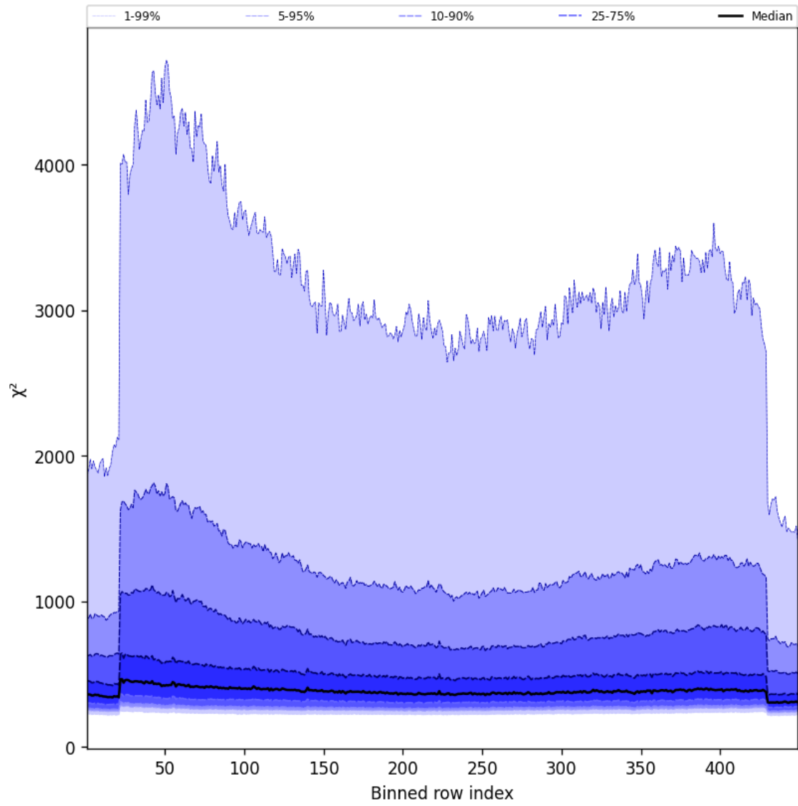
Figure 57: Along track statistics of “ \chi^2 ” for 2025-10-22 to 2025-10-23
