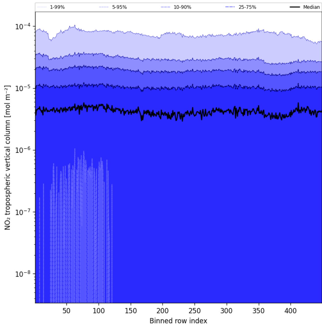
Figure 44: Along track statistics of “NO 2 tropospheric vertical column” for 2025-10-22 to 2025-10-23
