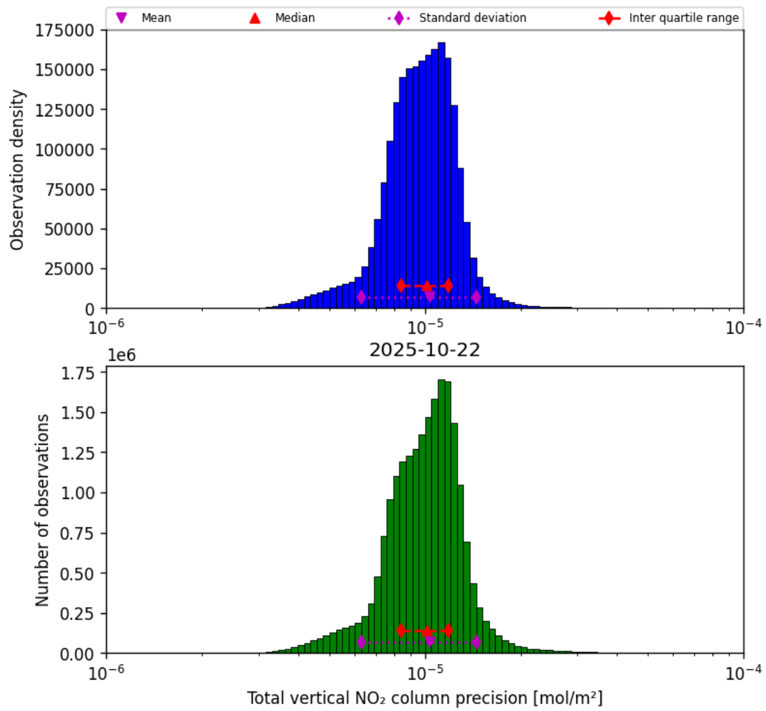
Figure 37: Histogram of “Total vertical NO 2 column precision” for 2025-10-22 to 2025-10-23
