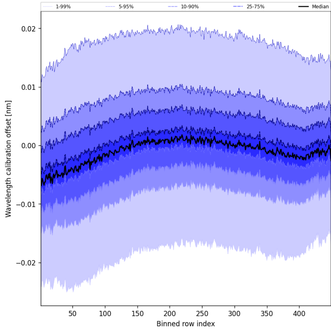
Figure 50: Along track statistics of “Wavelength calibration offset” for 2025-10-22 to 2025-10-23
