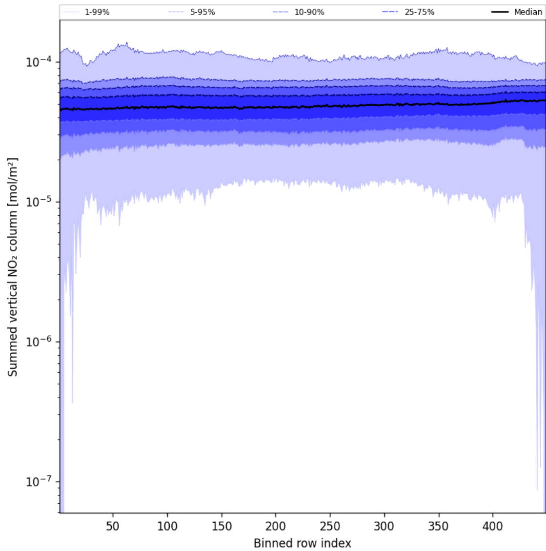
Figure 55: Along track statistics of “Summed vertical NO 2 column” for 2025-10-22 to 2025-10-23
