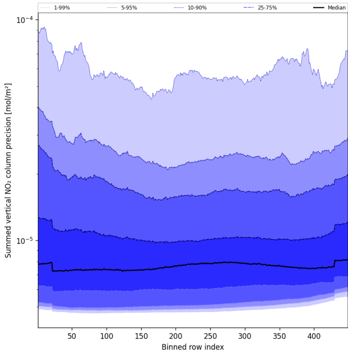
Figure 56: Along track statistics of “Summed vertical NO 2 column precision” for 2025-10-22 to 2025-10-23
