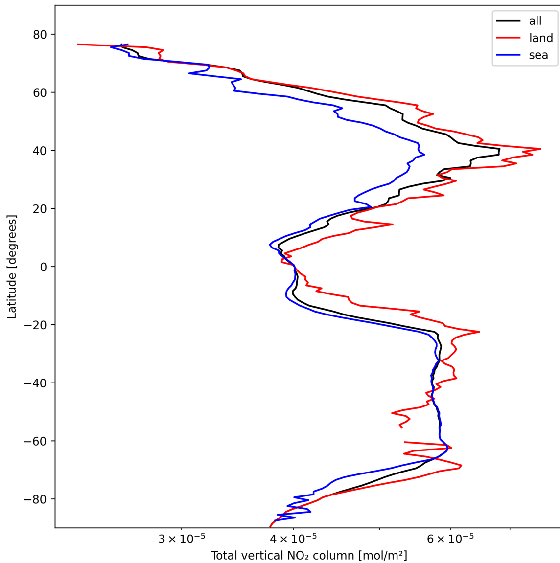
Figure 19: Zonal average of “Total vertical NO 2 column” for 2025-10-22 to 2025-10-23.
