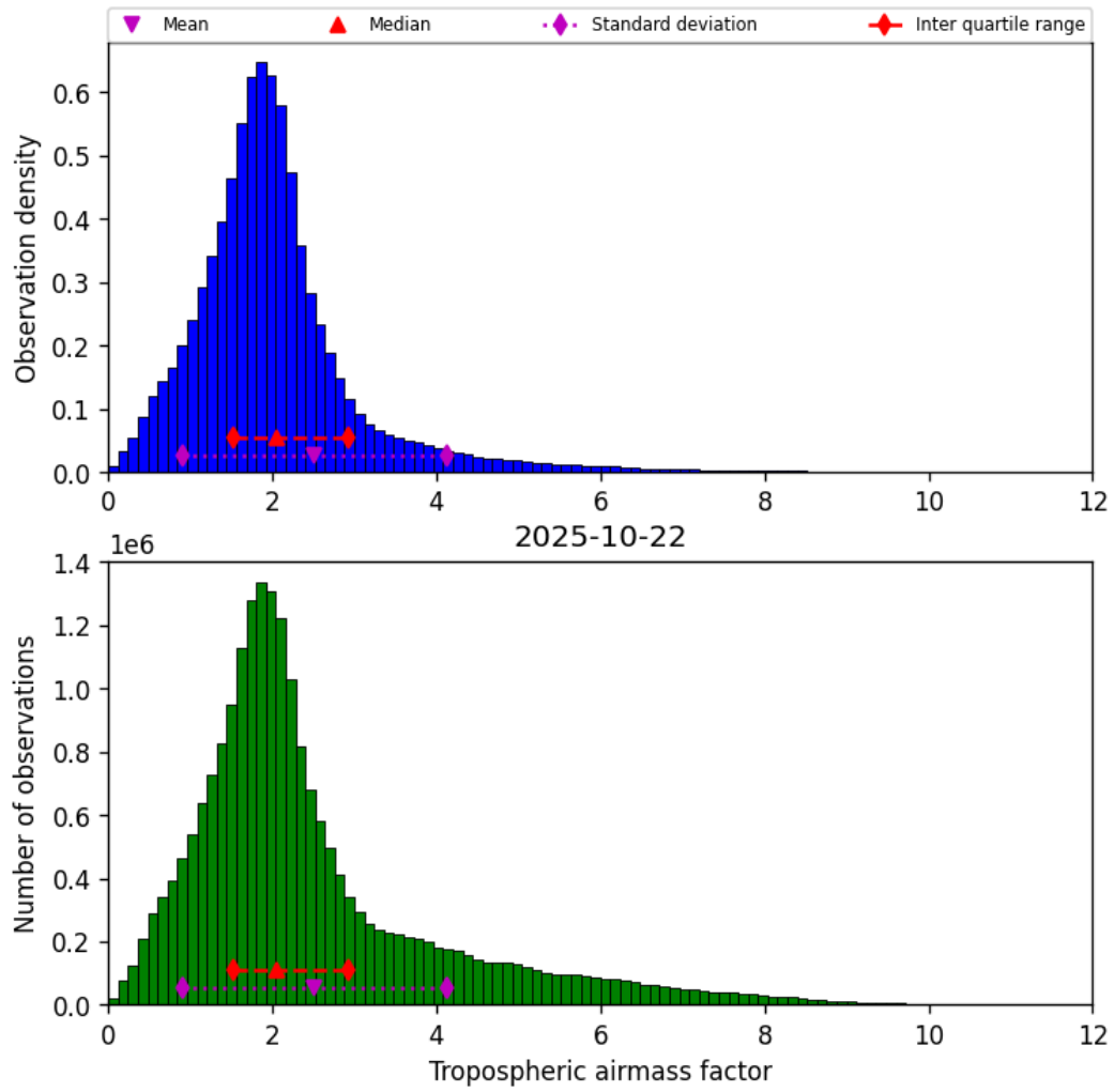
Figure 29: Histogram of “Tropospheric airmass factor” for 2025-10-22 to 2025-10-23
