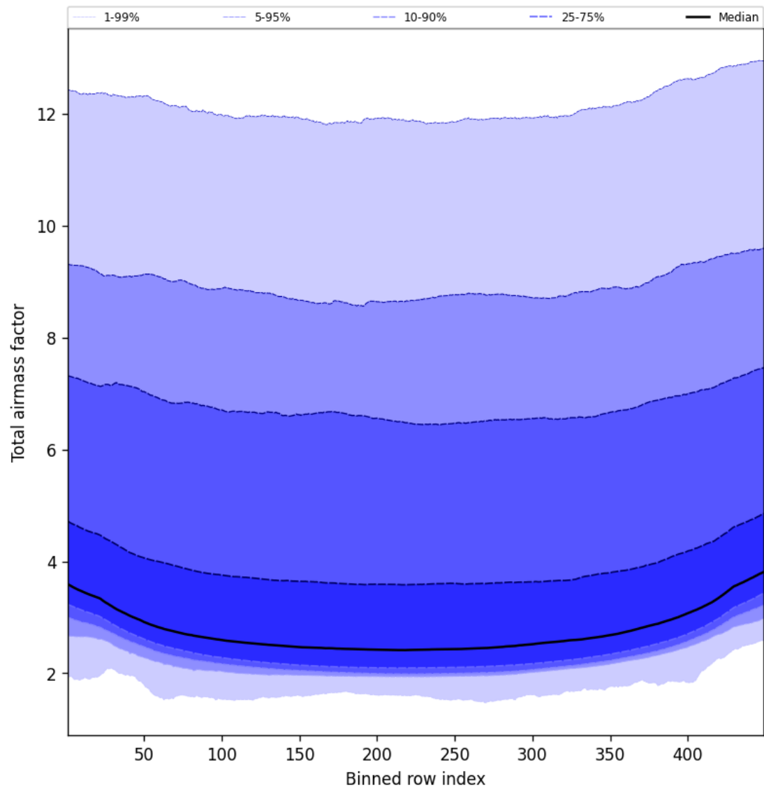
Figure 47: Along track statistics of “Total airmass factor” for 2025-10-22 to 2025-10-23
