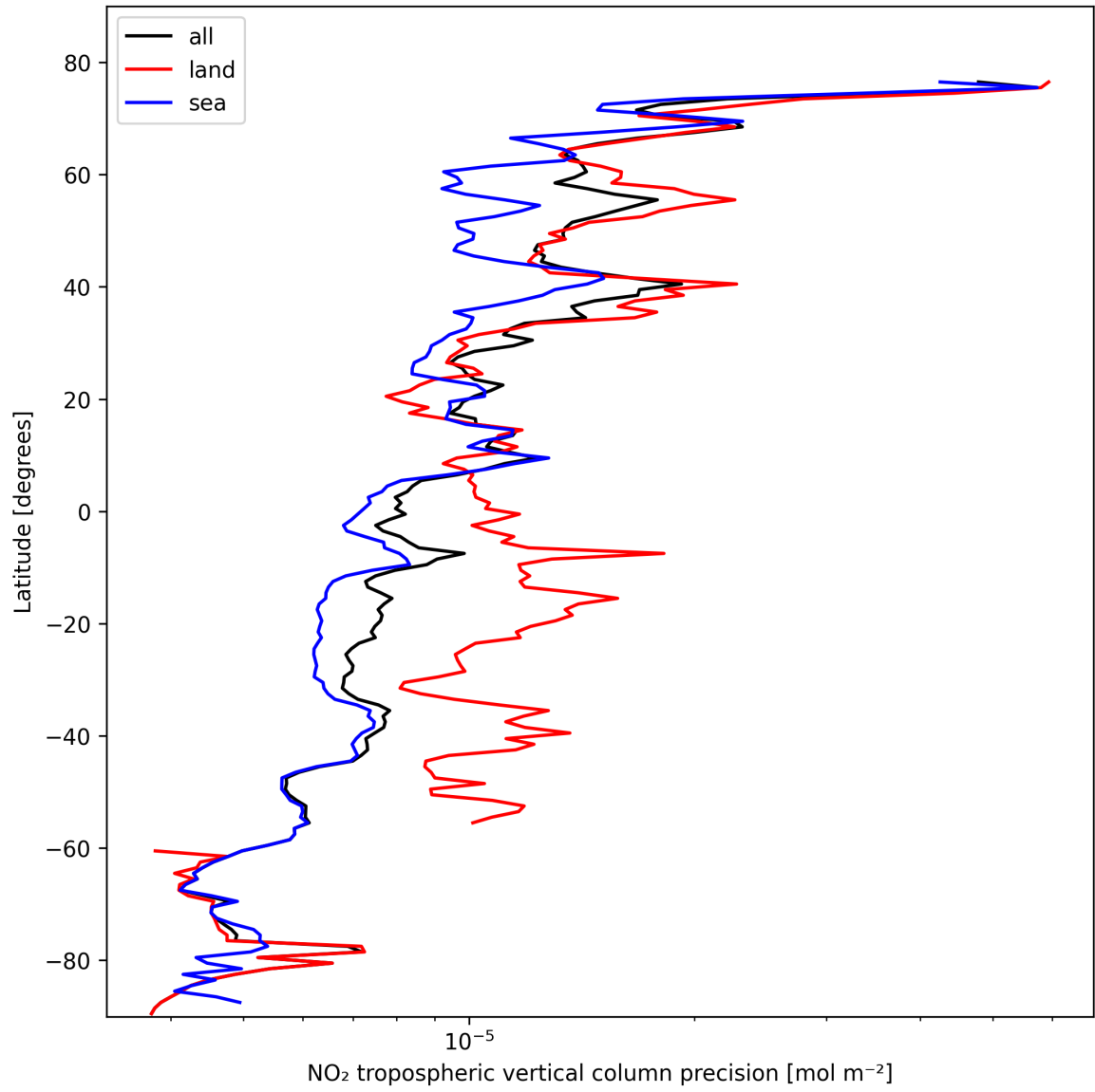
Figure 11: Zonal average of “NO 2 tropospheric vertical column precision” for 2025-10-22 to 2025-10-23.
