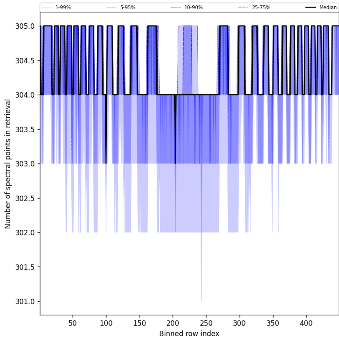
Figure 48: Along track statistics of “Number of spectral points in retrieval” for 2025-10-22 to 2025-10-23
