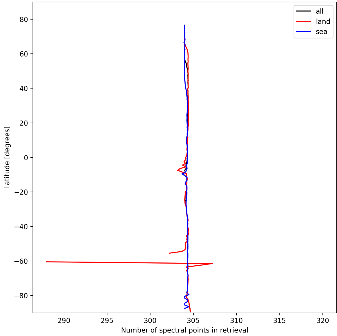
Figure 14: Zonal average of “Number of spectral points in retrieval” for 2025-10-22 to 2025-10-23.
