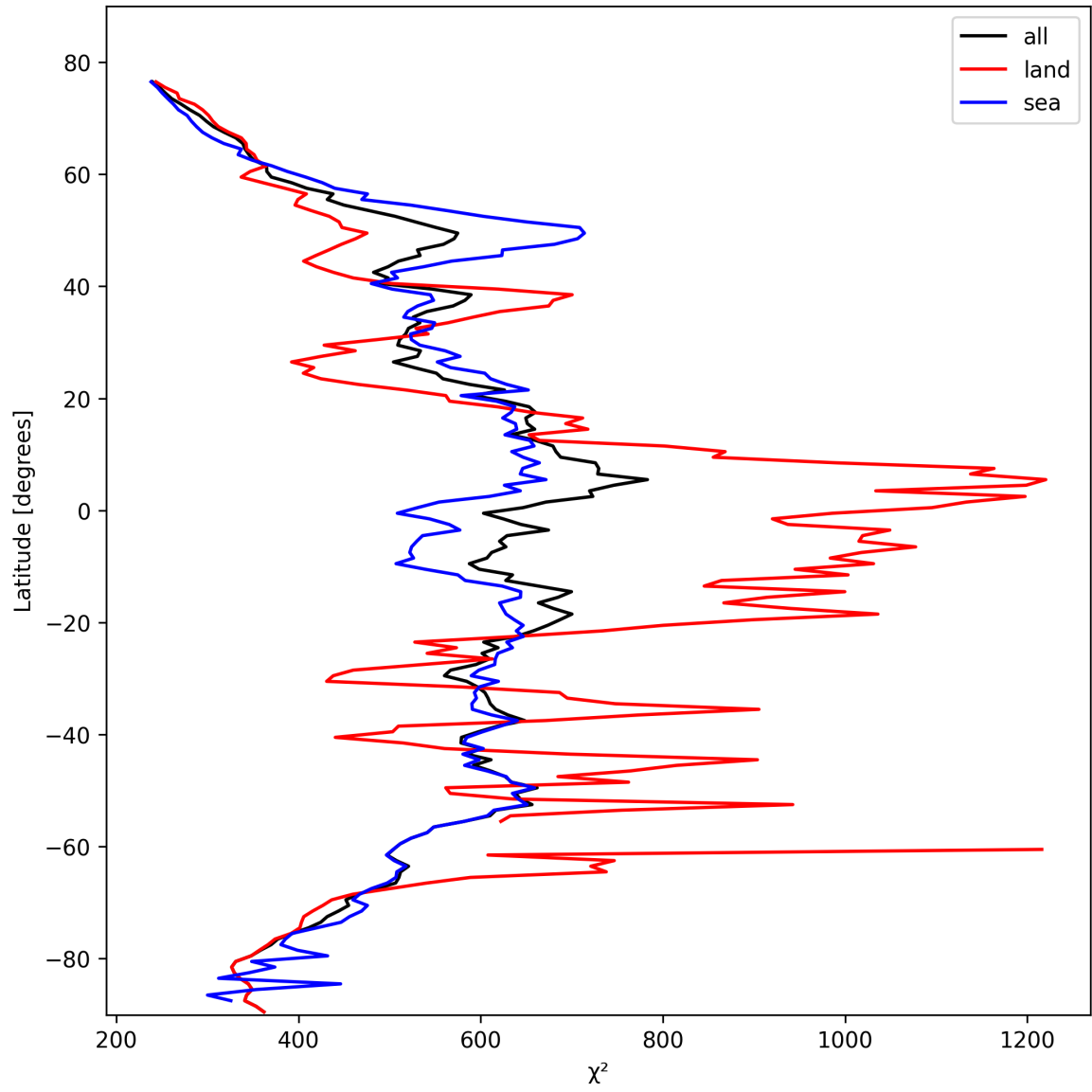
Figure 23: Zonal average of “ \chi^2 ” for 2025-10-22 to 2025-10-23.
