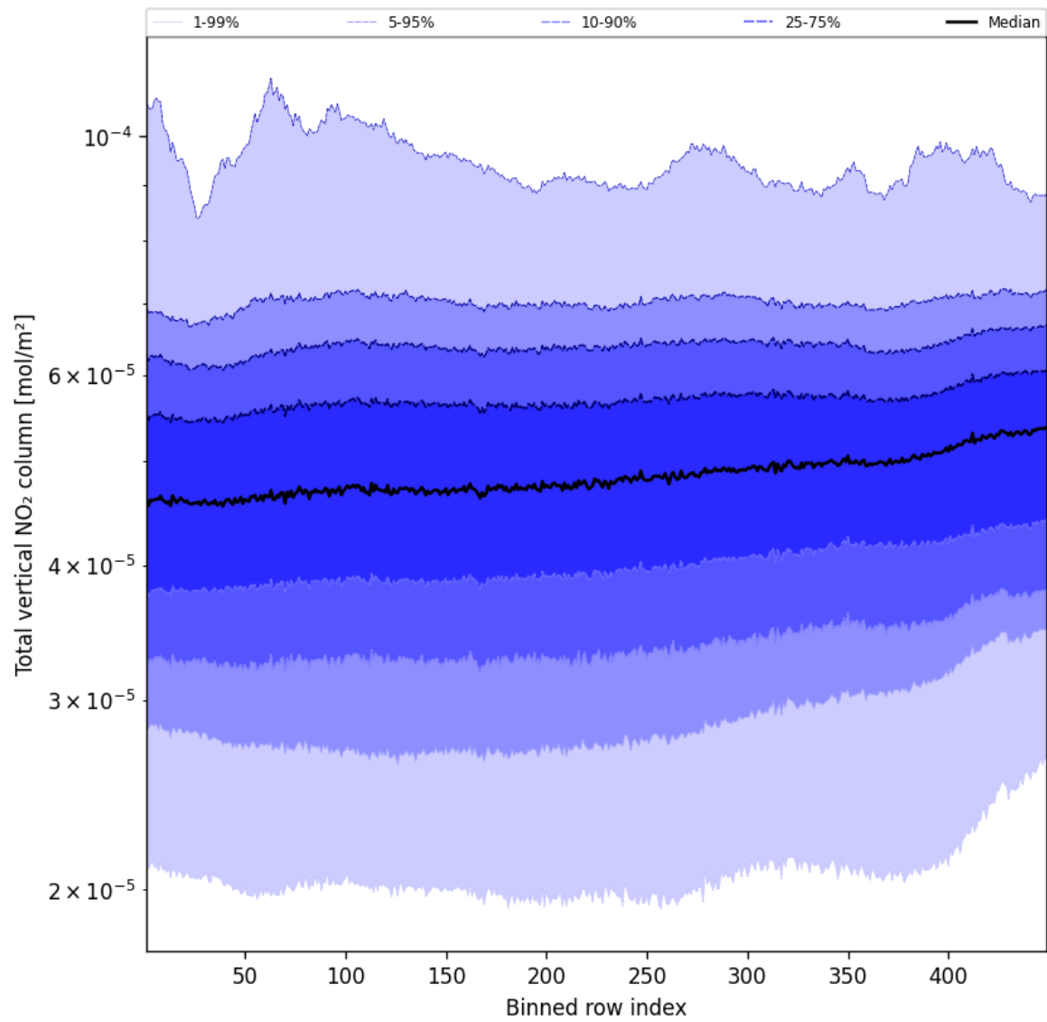
Figure 53: Along track statistics of “Total vertical NO 2 column” for 2025-10-22 to 2025-10-23
