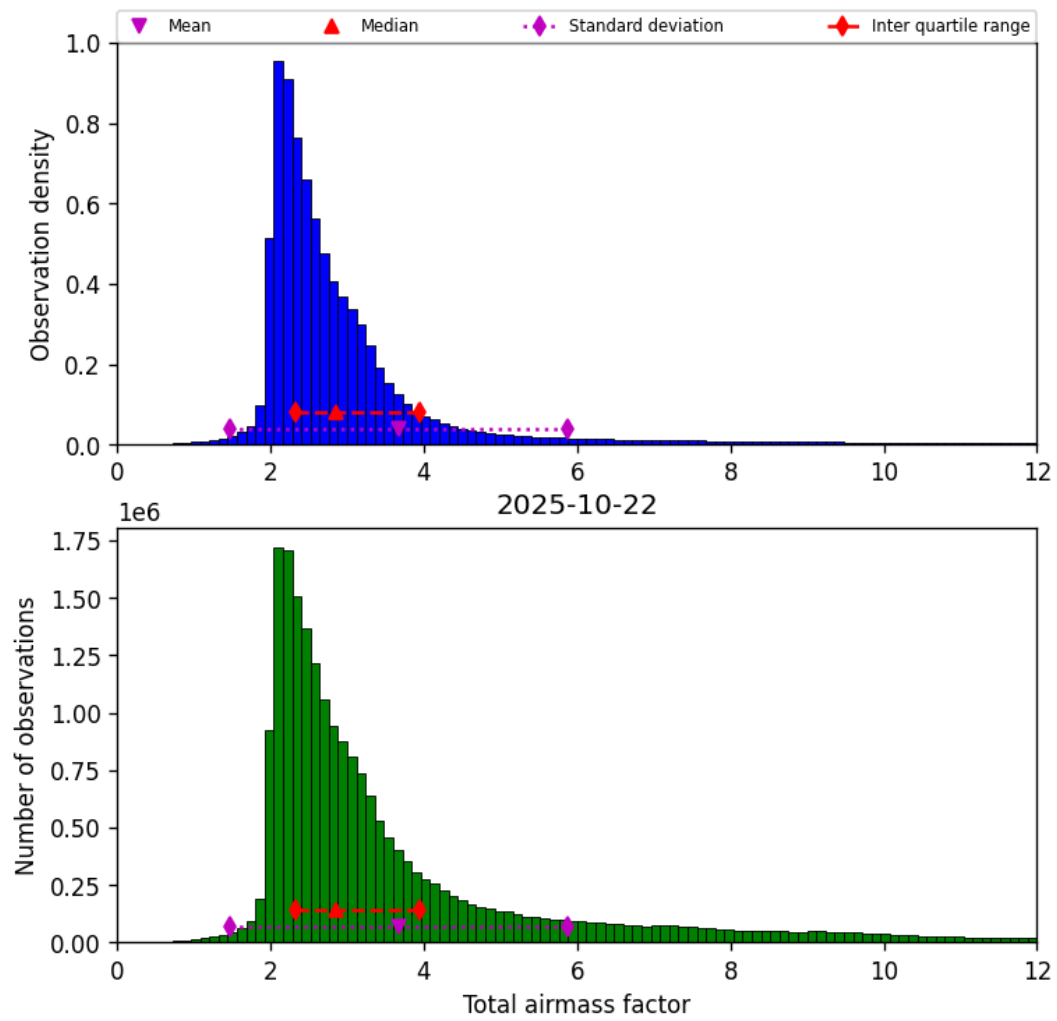
Figure 30: Histogram of “Total airmass factor” for 2025-10-22 to 2025-10-23
