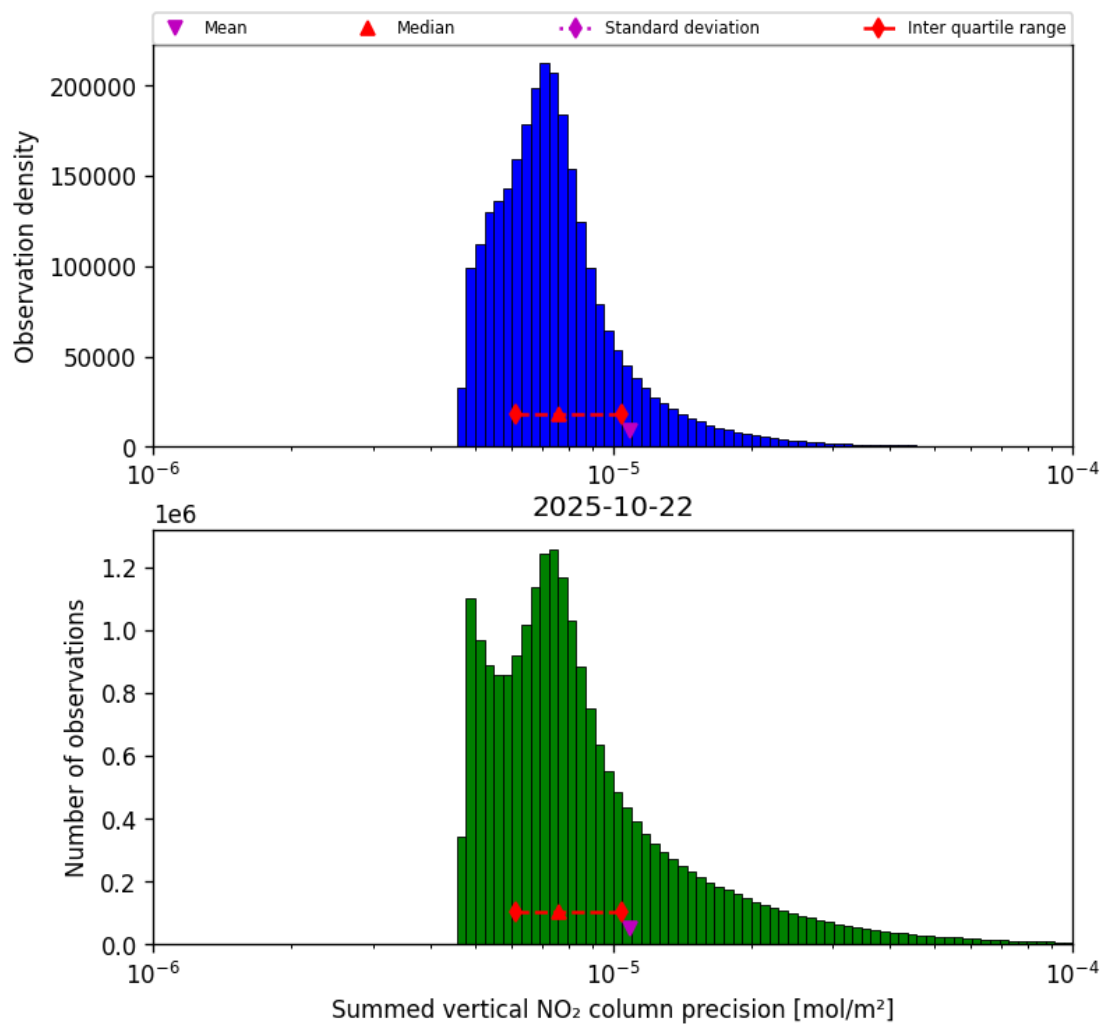
Figure 39: Histogram of “Summed vertical NO 2 column precision” for 2025-10-22 to 2025-10-23
