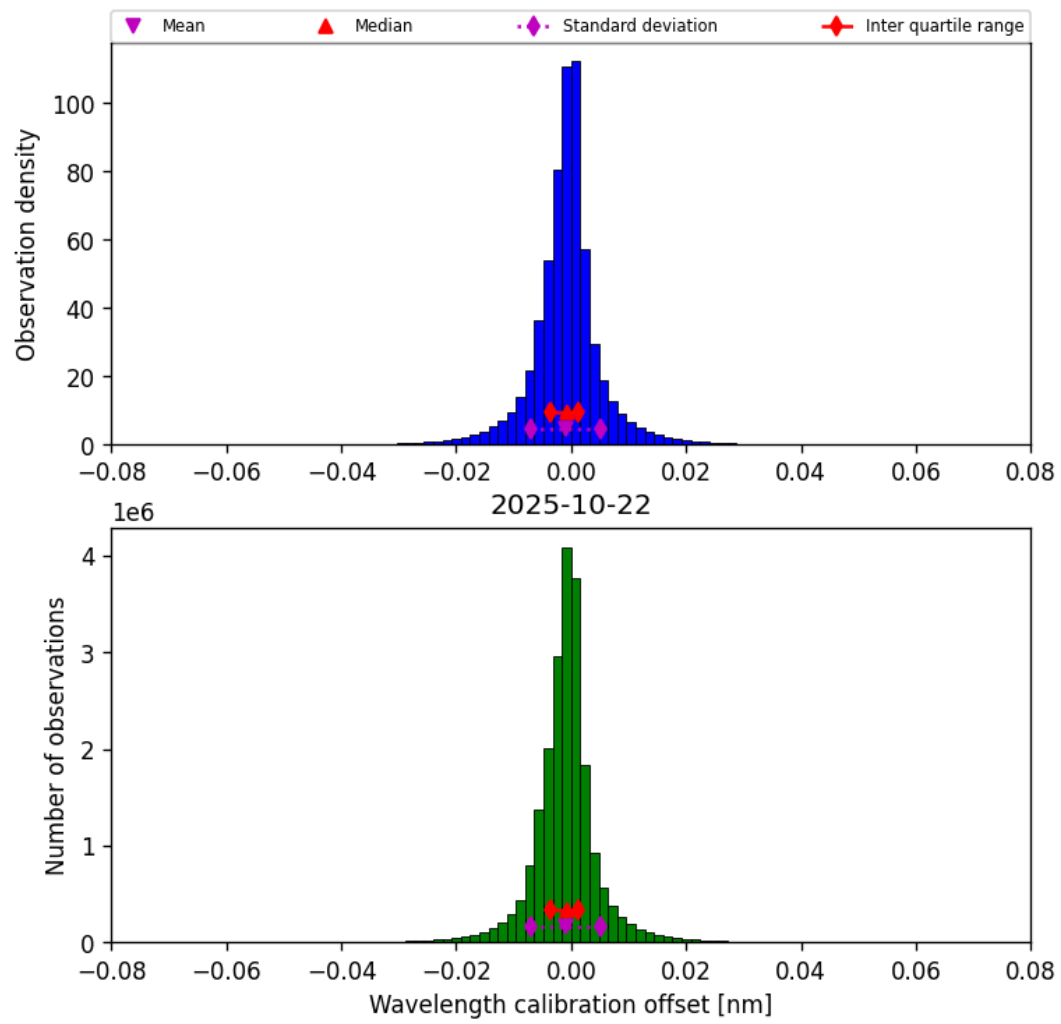
Figure 33: Histogram of “Wavelength calibration offset” for 2025-10-22 to 2025-10-23
