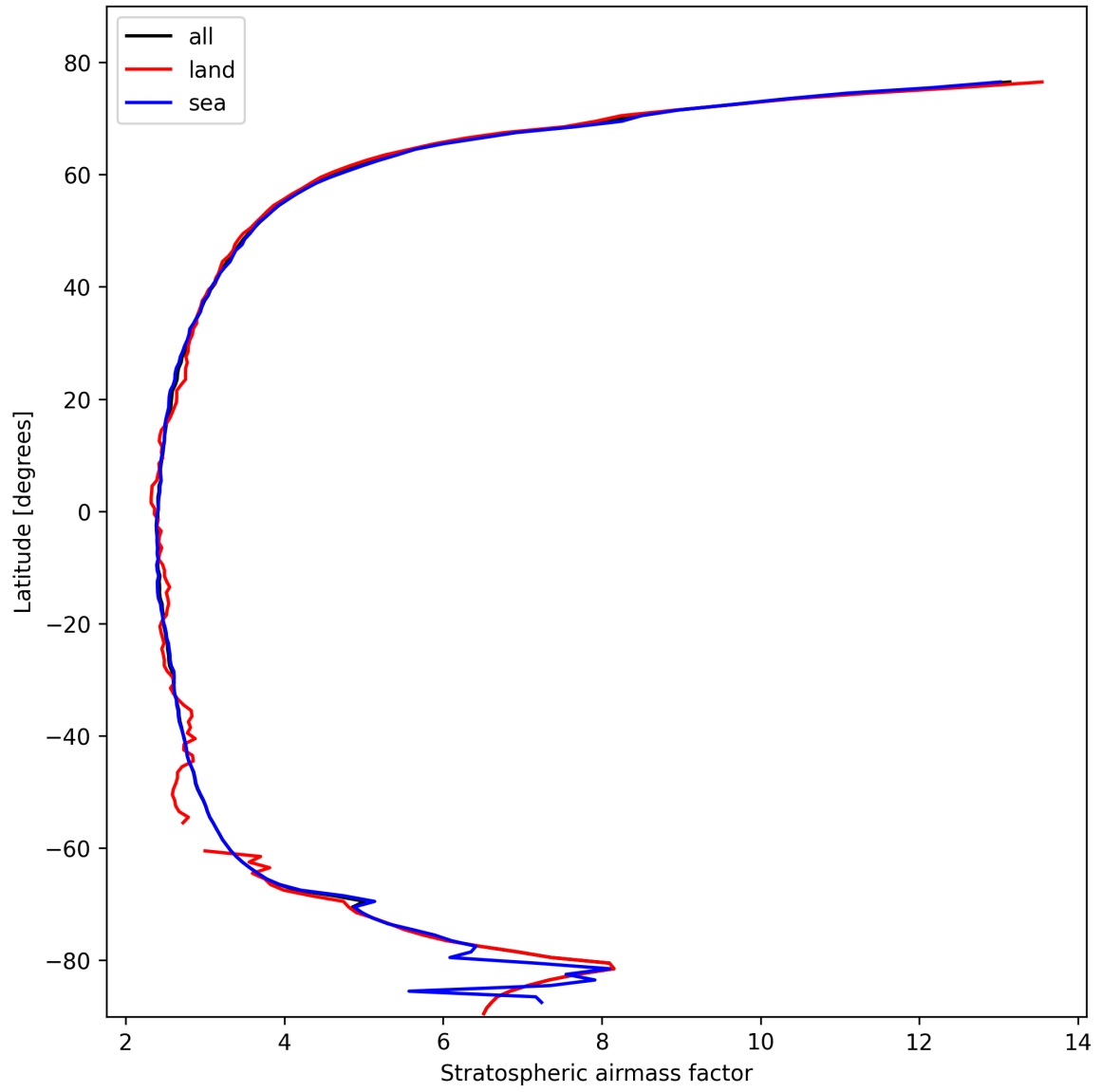
Figure 25: Zonal average of “Stratospheric airmass factor” for 2025-10-22 to 2025-10-23.
