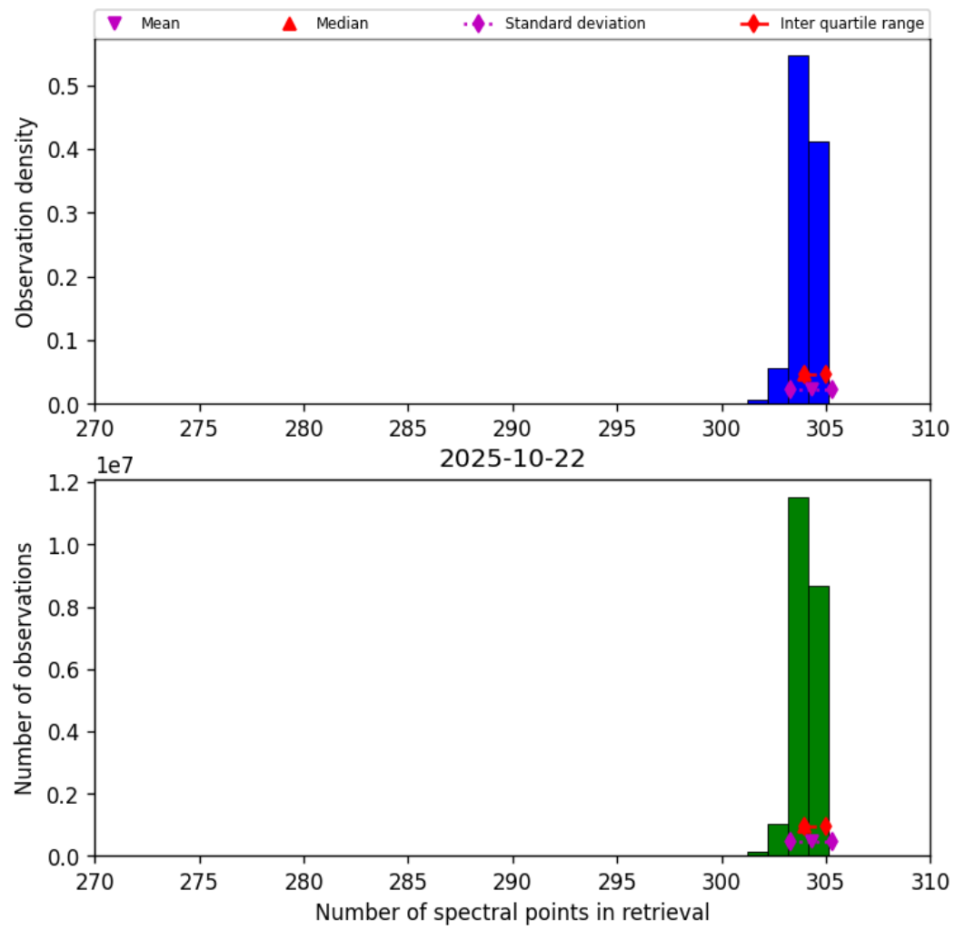
Figure 31: Histogram of “Number of spectral points in retrieval” for 2025-10-22 to 2025-10-23
