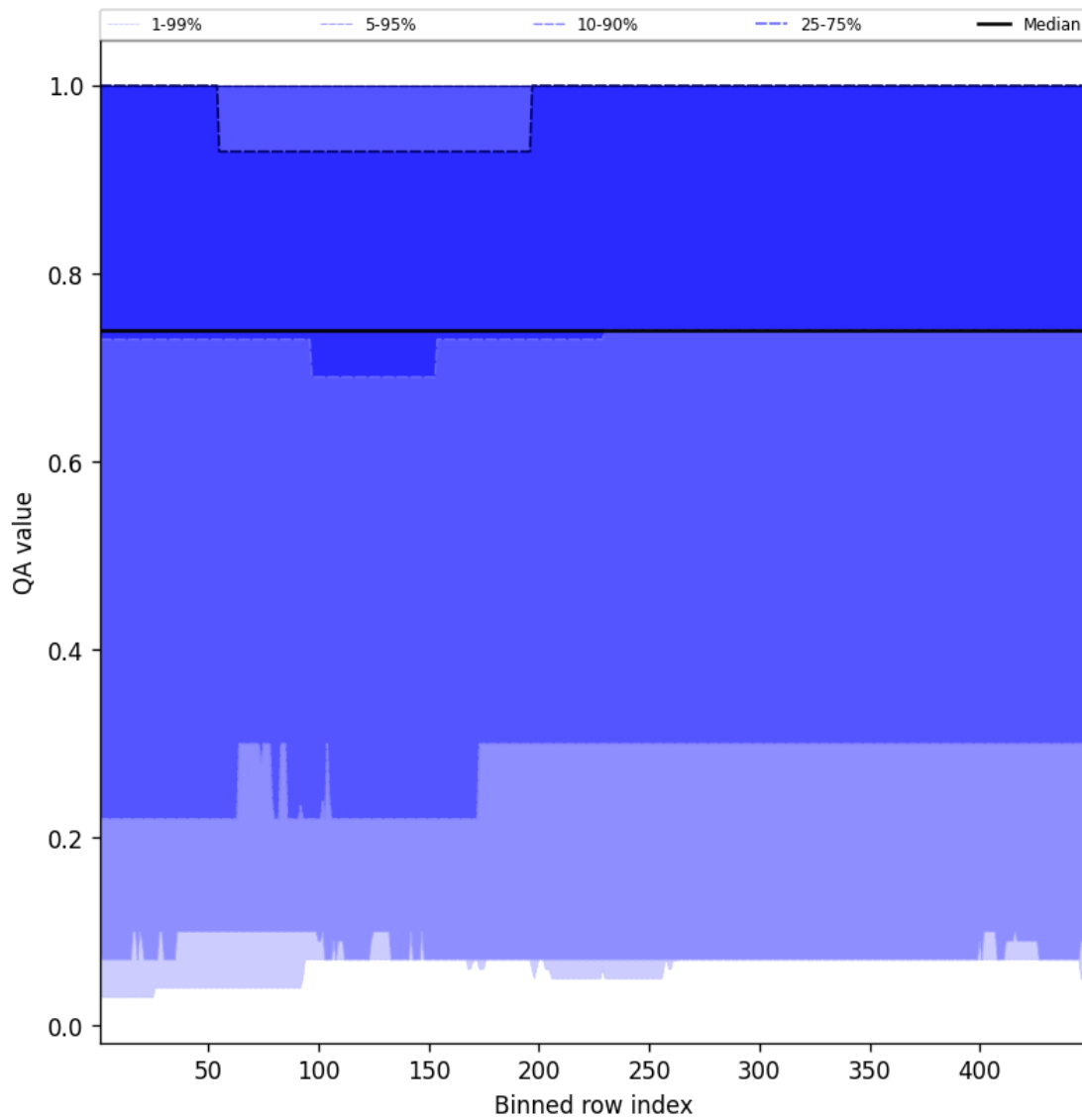
Figure 43: Along track statistics of “QA value” for 2025-10-22 to 2025-10-23
