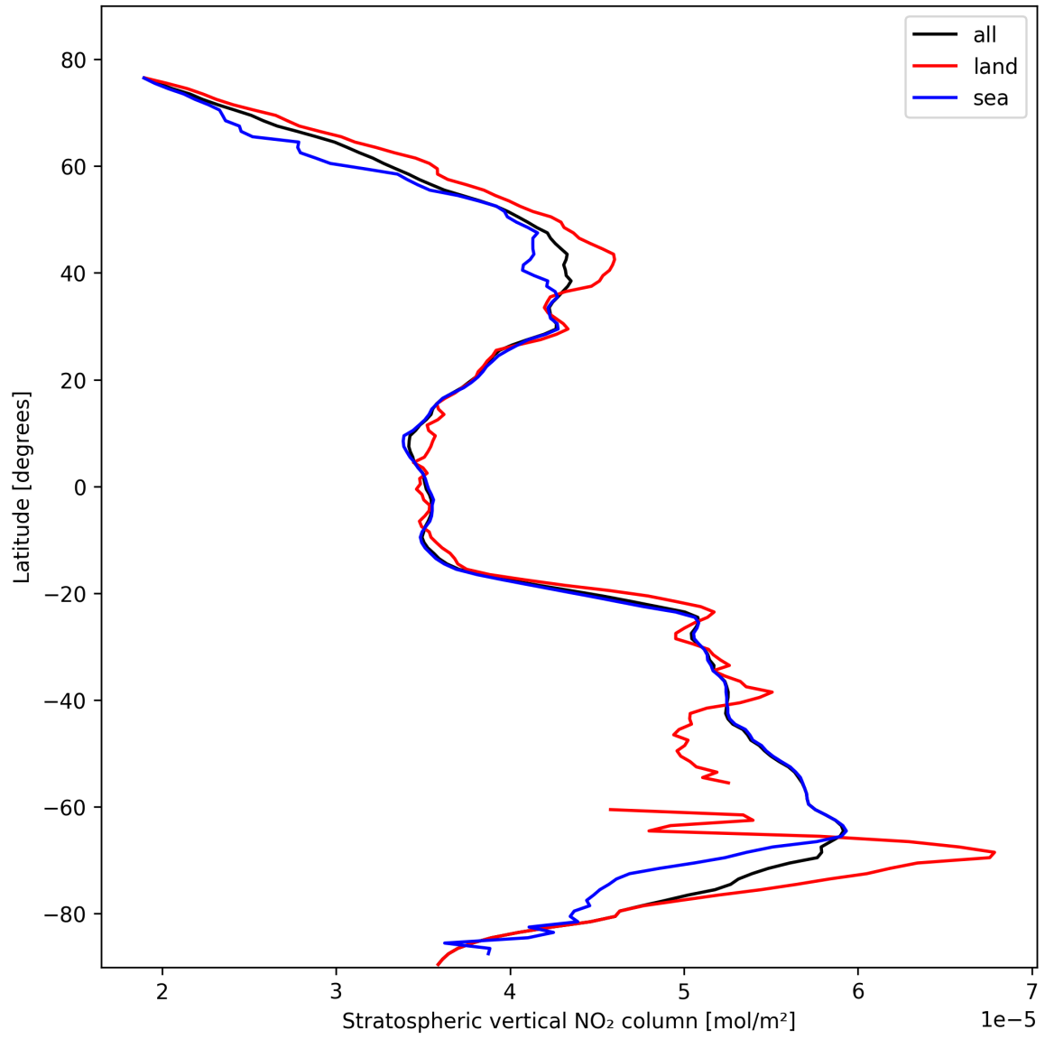
Figure 17: Zonal average of “Stratospheric vertical NO 2 column” for 2025-10-22 to 2025-10-23.
