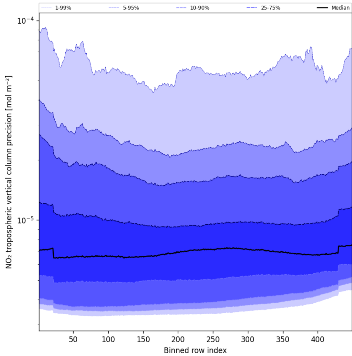
Figure 45: Along track statistics of “NO 2 tropospheric vertical column precision” for 2025-10-22 to 2025-10-23
