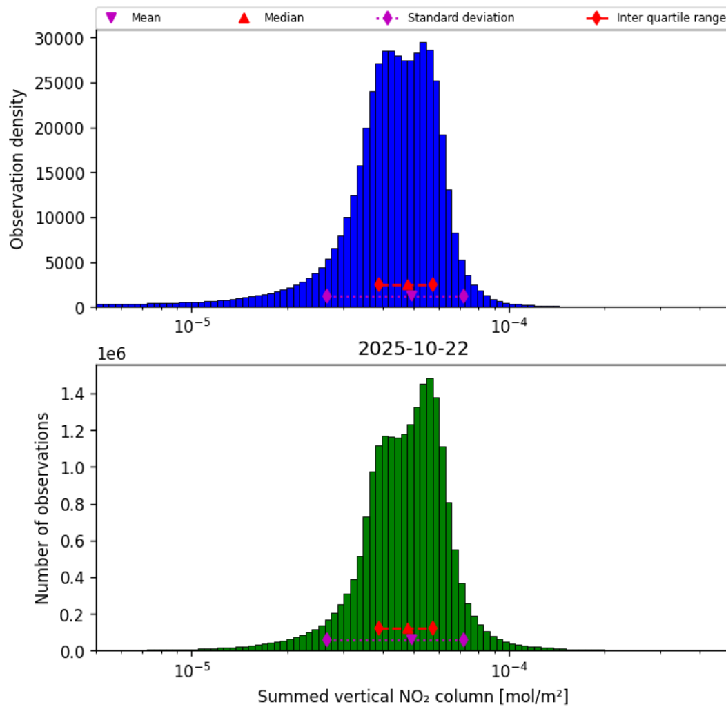
Figure 38: Histogram of “Summed vertical NO 2 column” for 2025-10-22 to 2025-10-23
