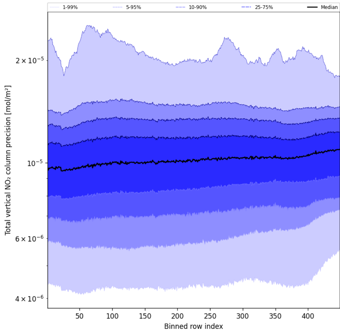
Figure 54: Along track statistics of “Total vertical NO 2 column precision” for 2025-10-22 to 2025-10-23
