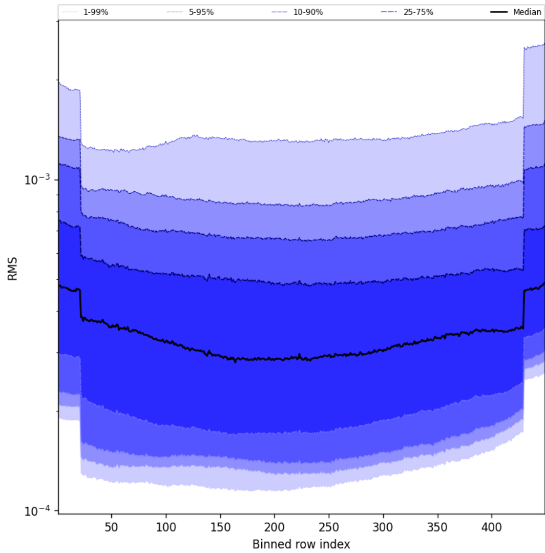
Figure 58: Along track statistics of “RMS” for 2025-10-22 to 2025-10-23
