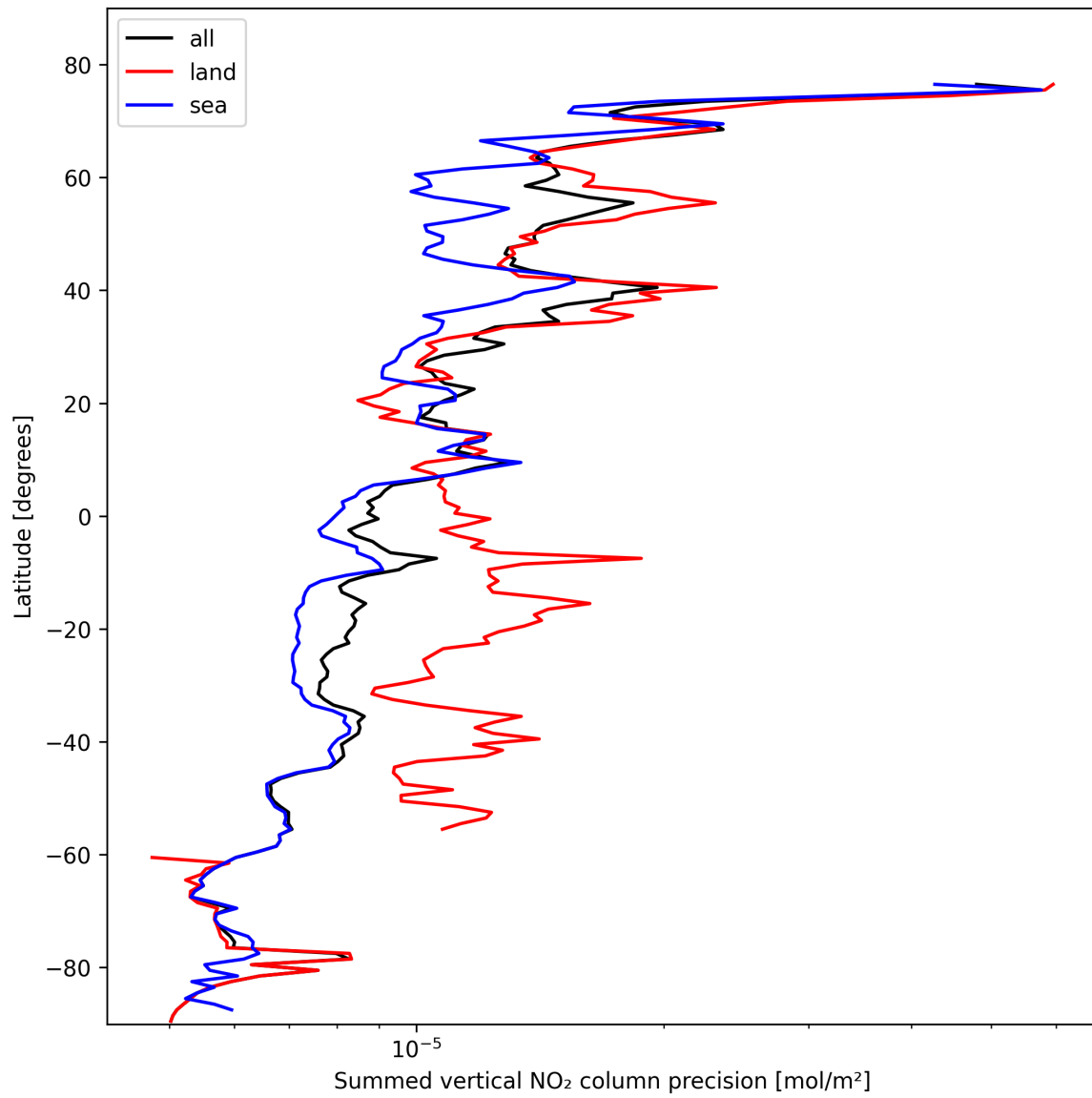
Figure 22: Zonal average of “Summed vertical NO 2 column precision” for 2025-10-22 to 2025-10-23.
