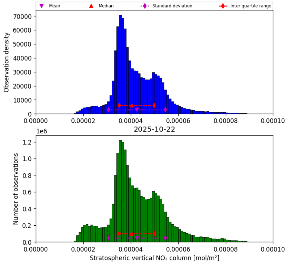
Figure 34: Histogram of “Stratospheric vertical NO 2 column” for 2025-10-22 to 2025-10-23
