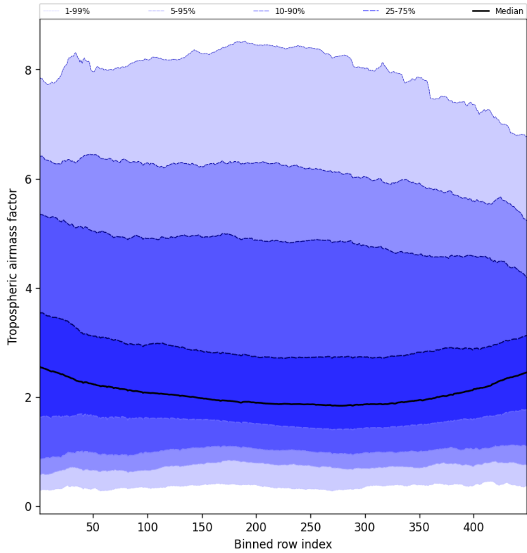
Figure 46: Along track statistics of “Tropospheric air mass factor” for 2025-10-22 to 2025-10-23
