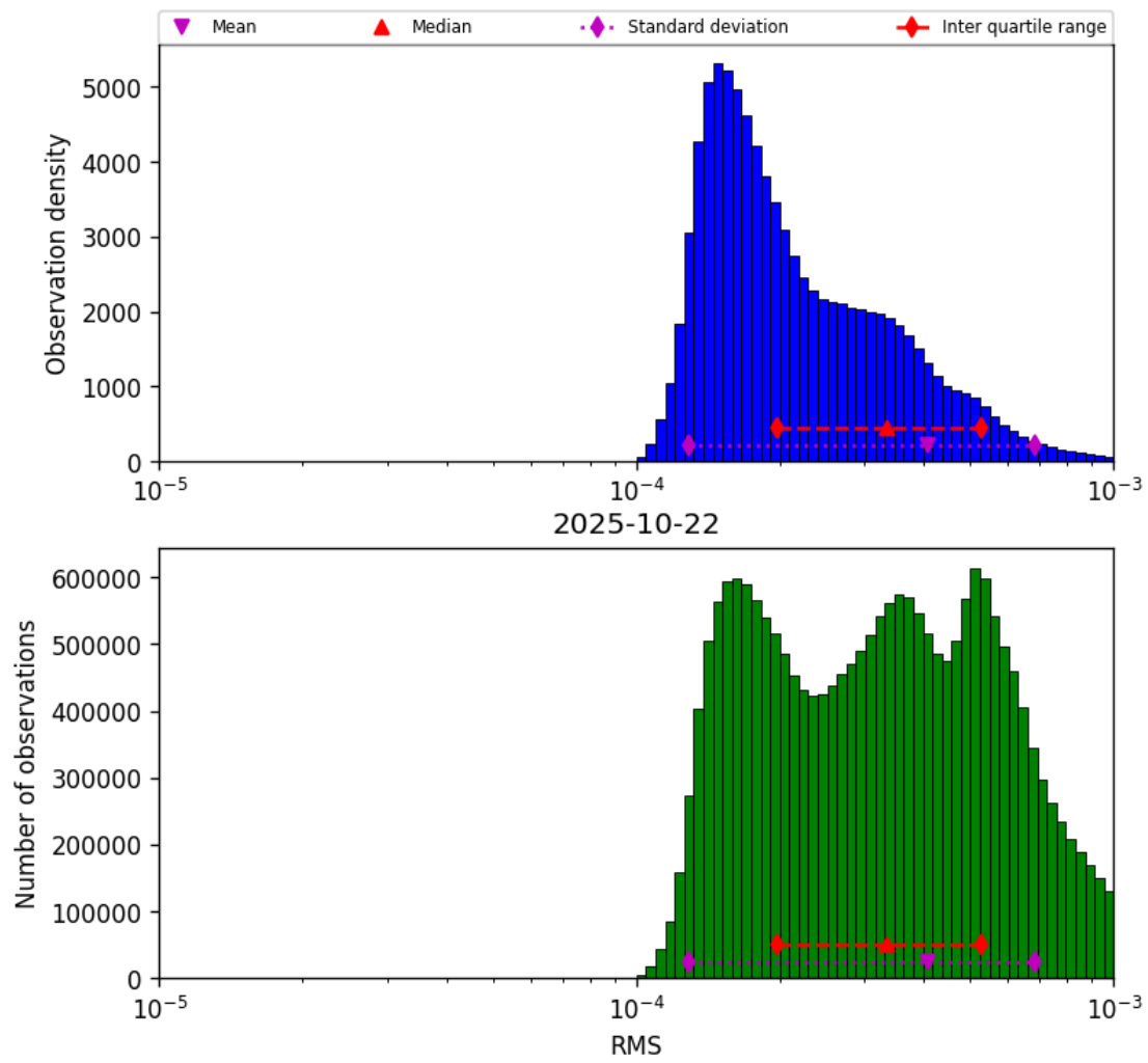
Figure 41: Histogram of “RMS” for 2025-10-22 to 2025-10-23
