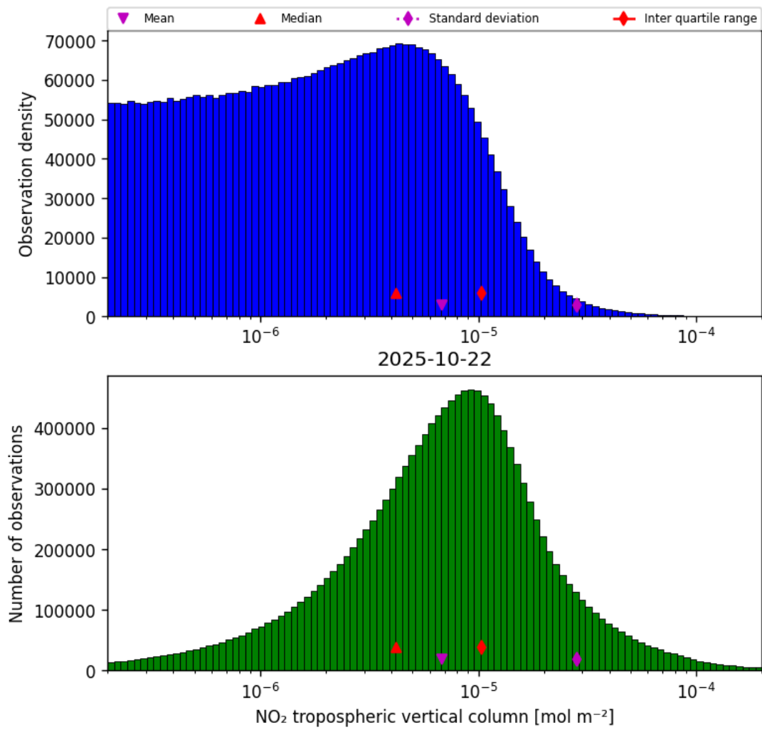
Figure 27: Histogram of “NO 2 tropospheric vertical column” for 2025-10-22 to 2025-10-23
