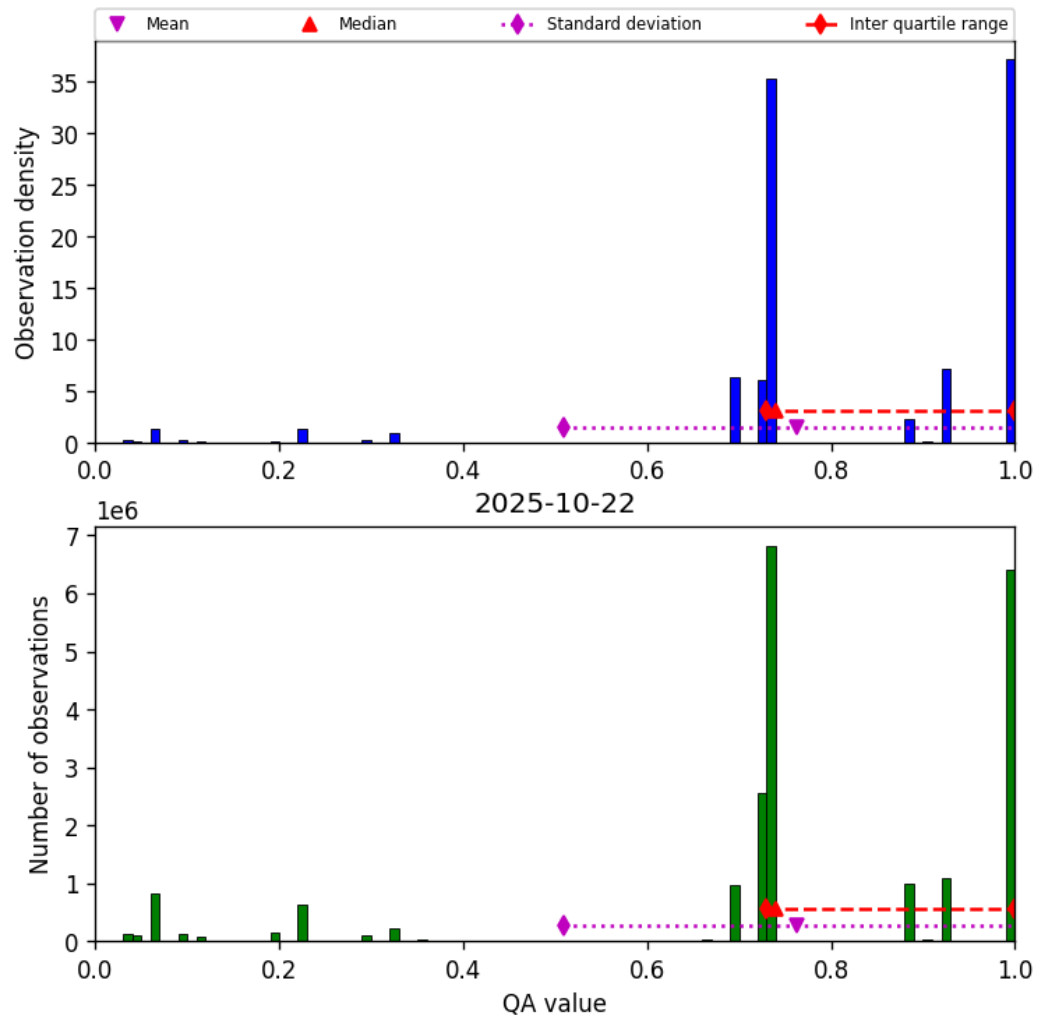
Figure 26: Histogram of “QA value” for 2025-10-22 to 2025-10-23
