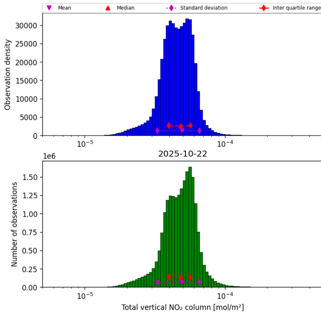
Figure 36: Histogram of “Total vertical NO 2 column” for 2025-10-22 to 2025-10-23
