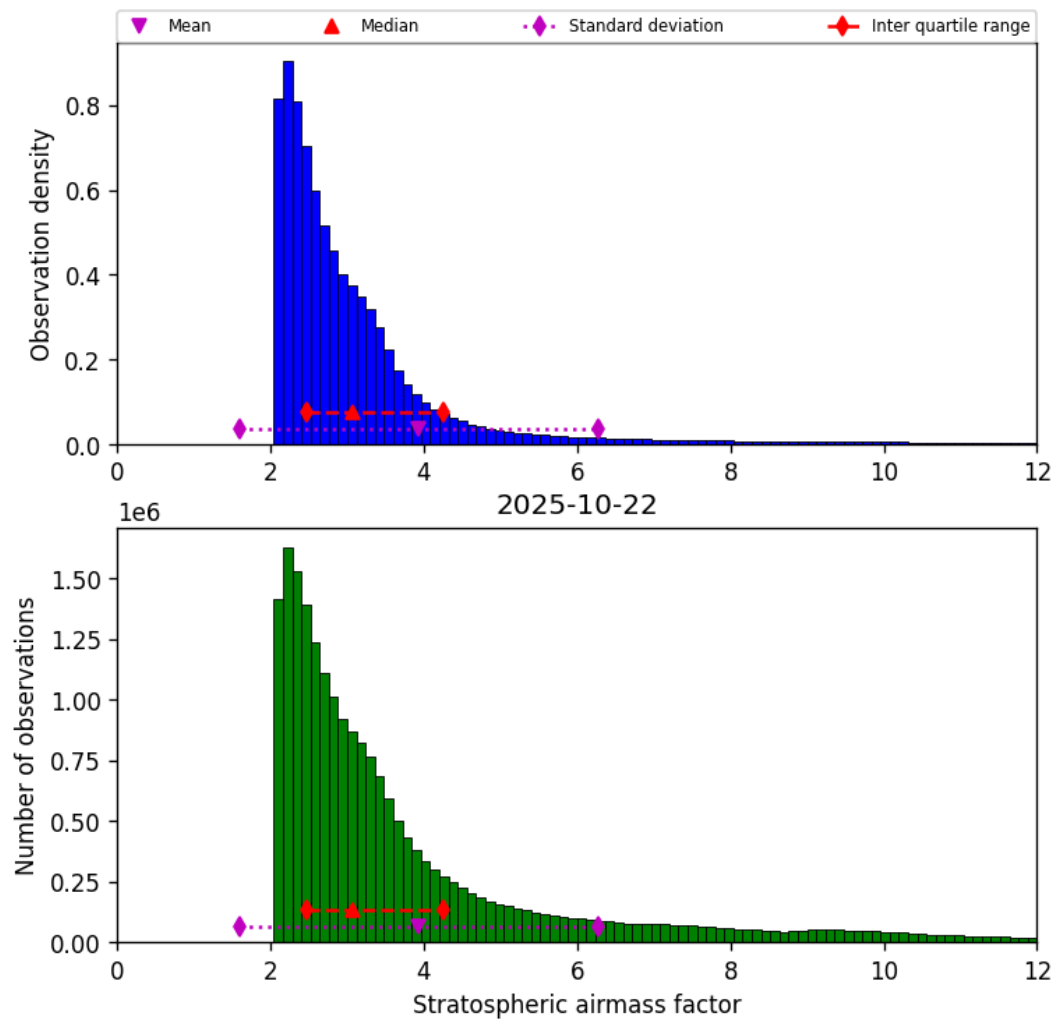
Figure 42: Histogram of “Stratospheric airmass factor” for 2025-10-22 to 2025-10-23
