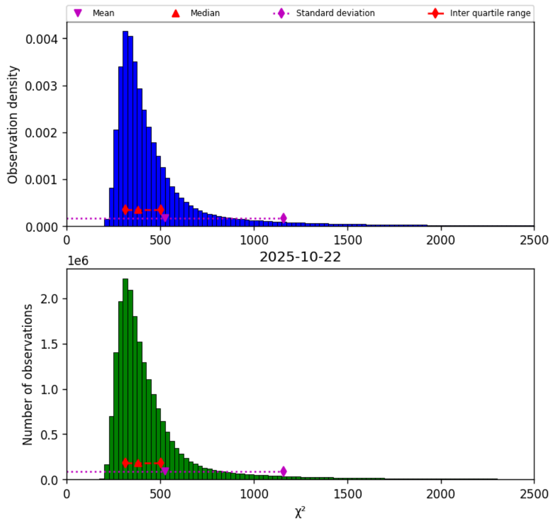
Figure 40: Histogram of “ \chi^2 ” for 2025-10-22 to 2025-10-23
