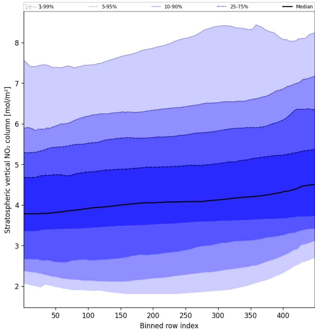
Figure 51: Along track statistics of "Stratospheric vertical NO 2 column" for 2025-10-22 to 2025-10-23
