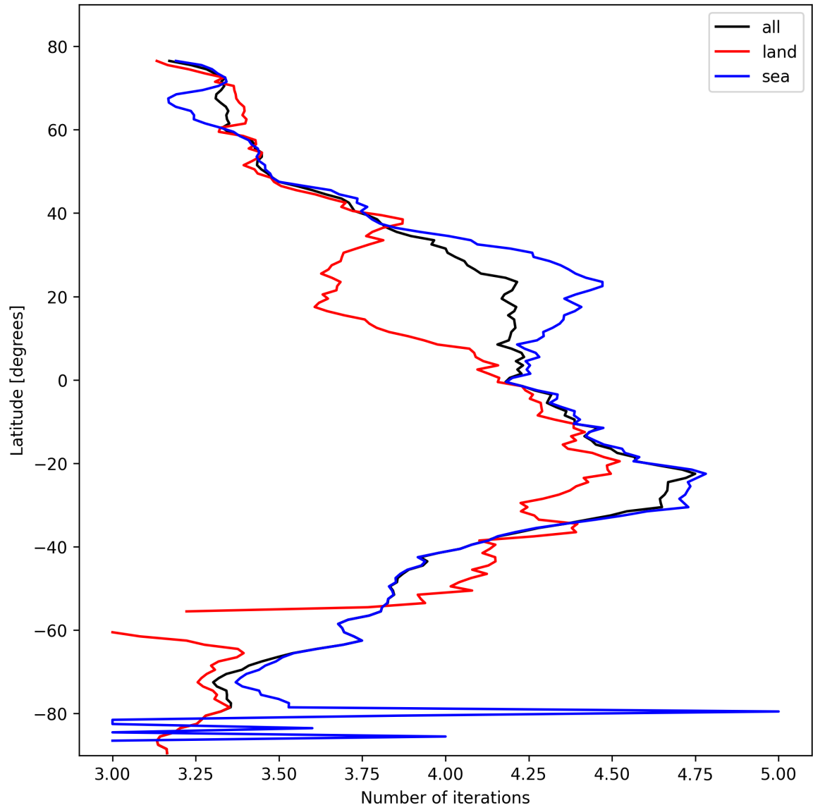
Figure 15: Zonal average of “Number of iterations” for 2025-10-23 to 2025-10-24.
