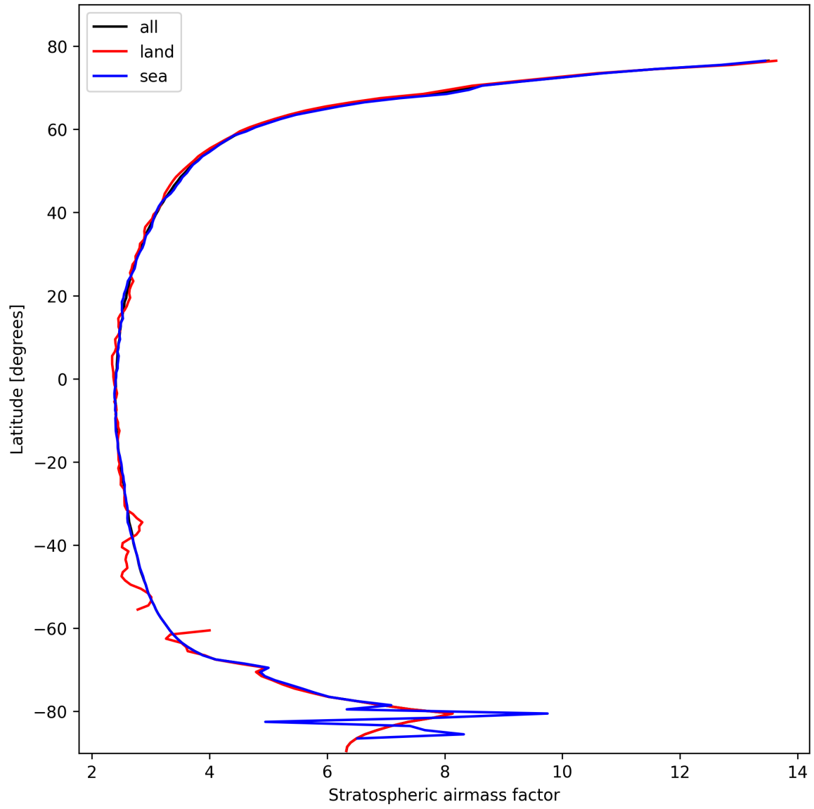
Figure 25: Zonal average of “Stratospheric air mass factor” for 2025-10-23 to 2025-10-24.
