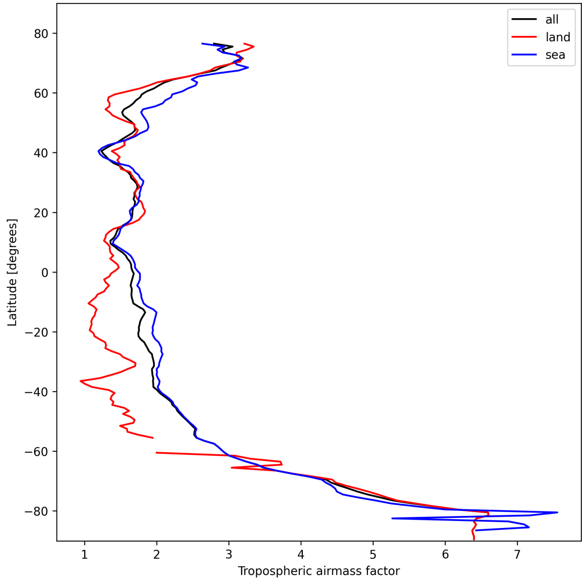
Figure 12: Zonal average of “Tropospheric airmass factor” for 2025-10-23 to 2025-10-24.
