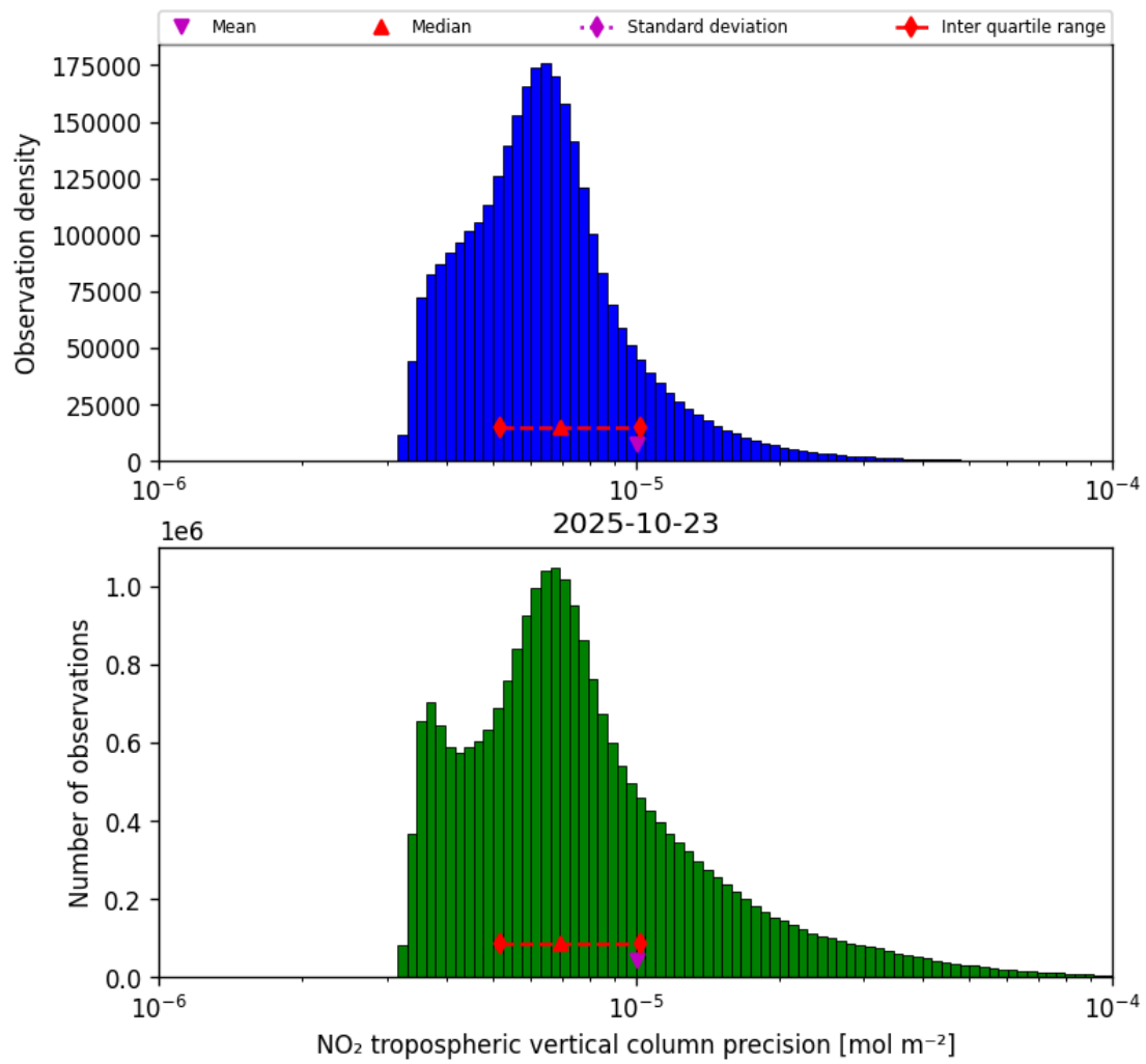
Figure 28: Histogram of “NO 2 tropospheric vertical column precision” for 2025-10-23 to 2025-10-24
