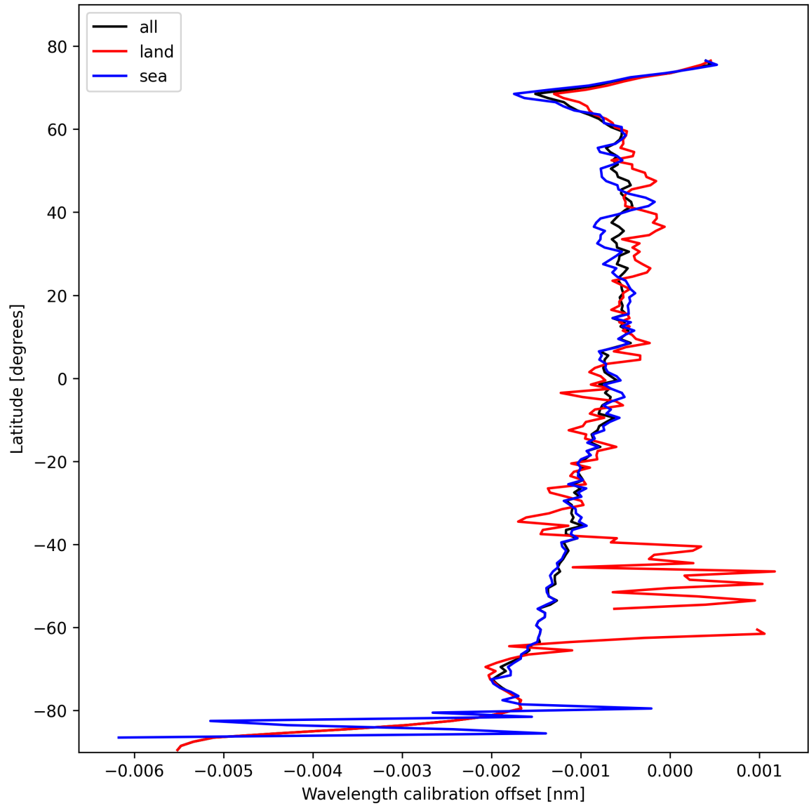
Figure 16: Zonal average of “Wavelength calibration offset” for 2025-10-23 to 2025-10-24.
