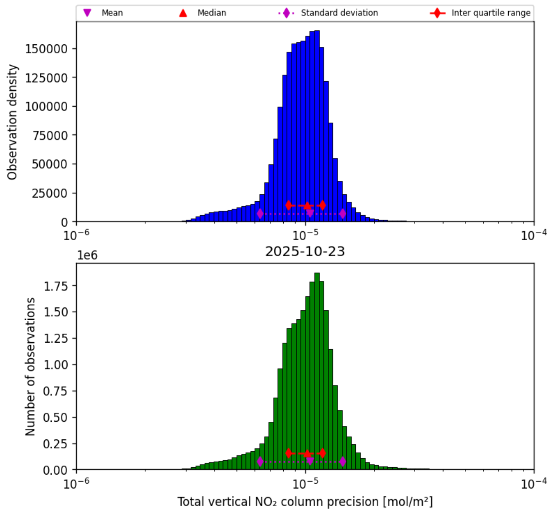
Figure 37: Histogram of "Total vertical NO 2 column precision" for 2025-10-23 to 2025-10-24
