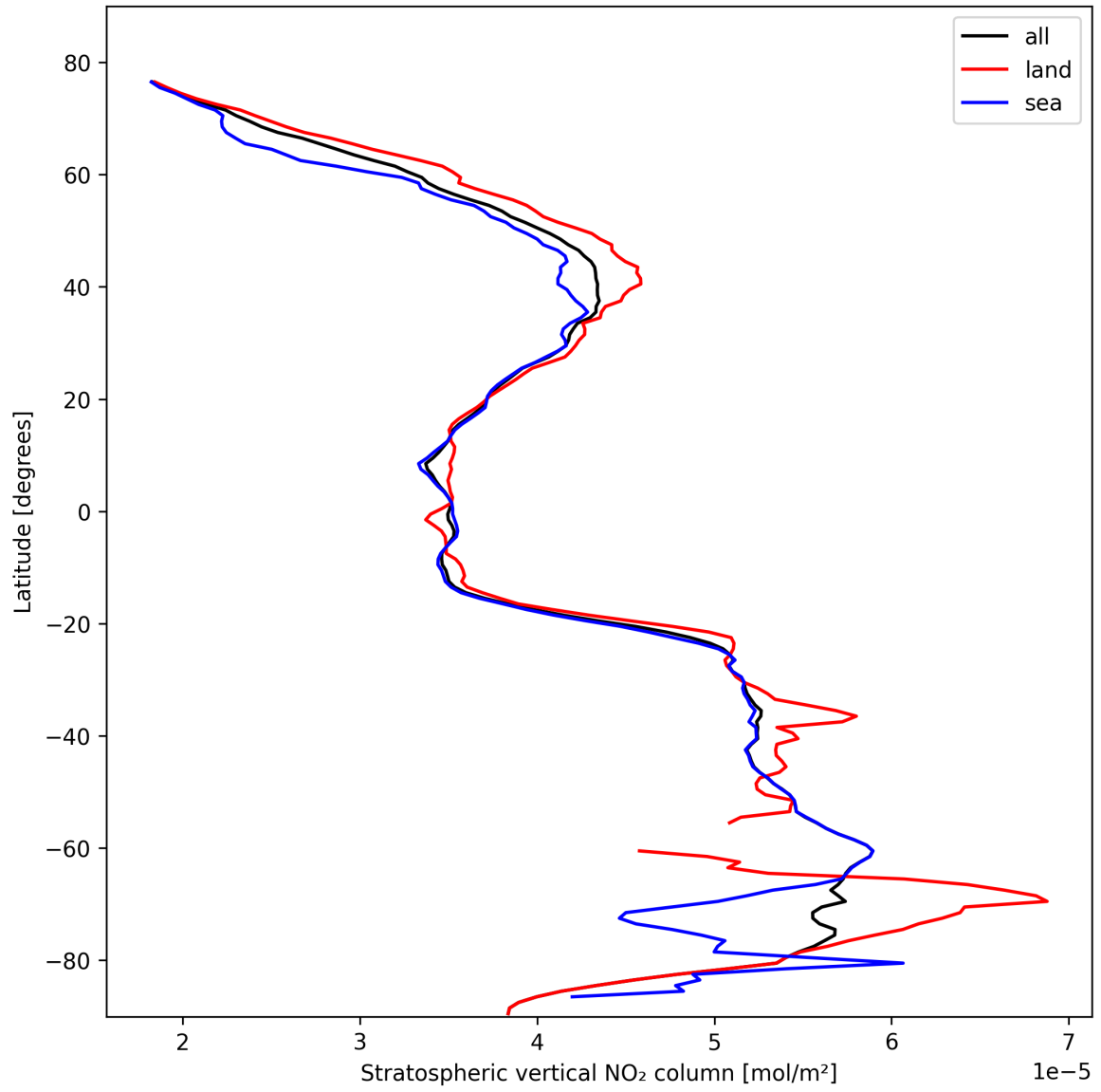
Figure 17: Zonal average of “Stratospheric vertical NO 2 column” for 2025-10-23 to 2025-10-24.
