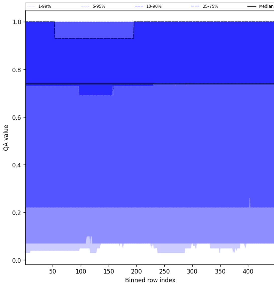
Figure 43: Along track statistics of “QA value” for 2025-10-23 to 2025-10-24
