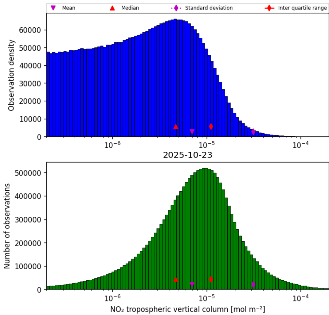
Figure 27: Histogram of “NO 2 tropospheric vertical column” for 2025-10-23 to 2025-10-24
