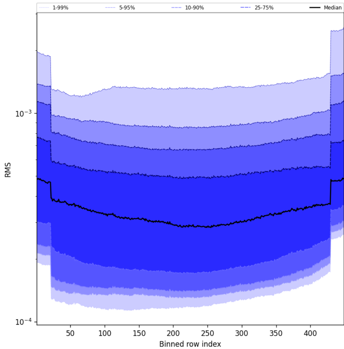
Figure 58: Along track statistics of “RMS” for 2025-10-23 to 2025-10-24
