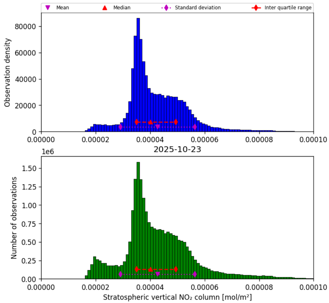
Figure 34: Histogram of “Stratospheric vertical NO 2 column” for 2025-10-23 to 2025-10-24
