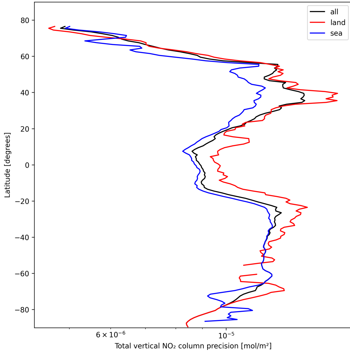
Figure 20: Zonal average of “Total vertical NO 2 column precision” for 2025-10-23 to 2025-10-24.
