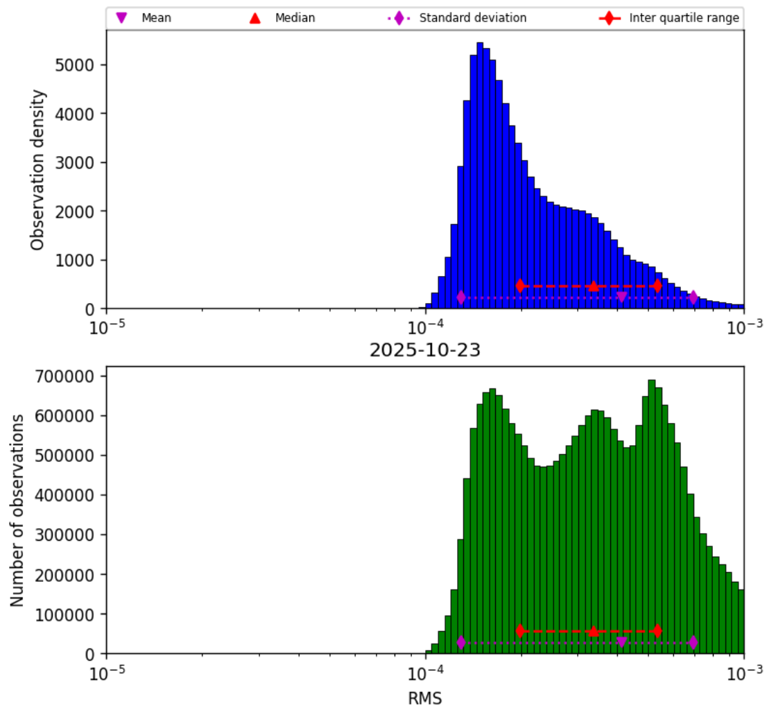
Figure 41: Histogram of “RMS” for 2025-10-23 to 2025-10-24
