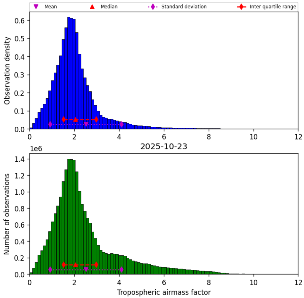
Figure 29: Histogram of “Tropospheric airmass factor” for 2025-10-23 to 2025-10-24
