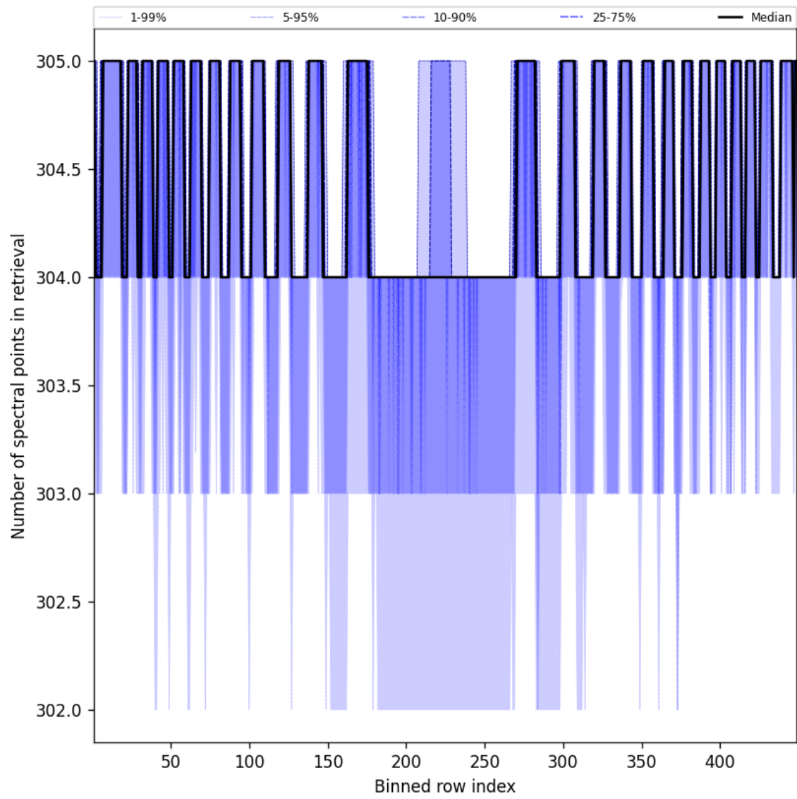
Figure 48: Along track statistics of “Number of spectral points in retrieval” for 2025-10-23 to 2025-10-24
