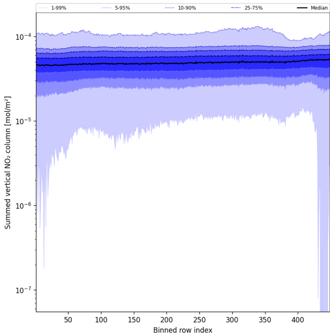
Figure 55: Along track statistics of “Summed vertical NO 2 column” for 2025-10-23 to 2025-10-24
