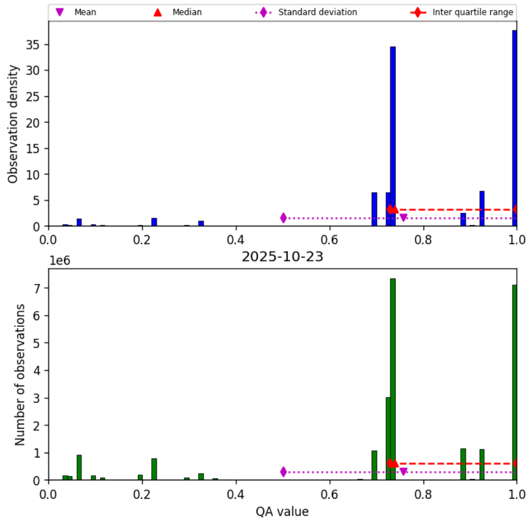
Figure 26: Histogram of “QA value” for 2025-10-23 to 2025-10-24
