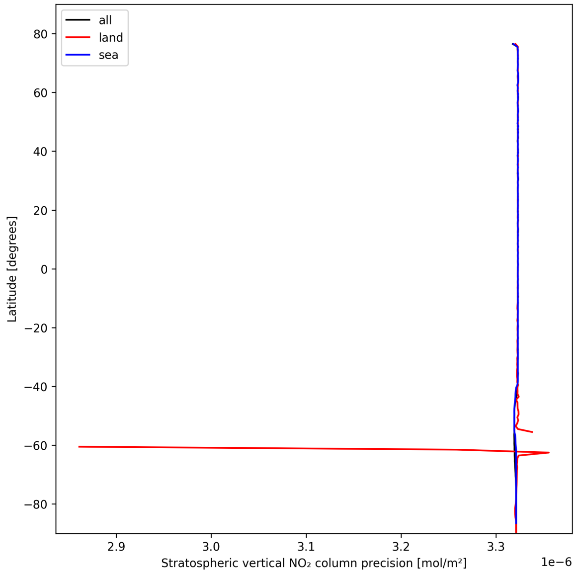
Figure 18: Zonal average of “Stratospheric vertical NO 2 column precision” for 2025-10-23 to 2025-10-24.
