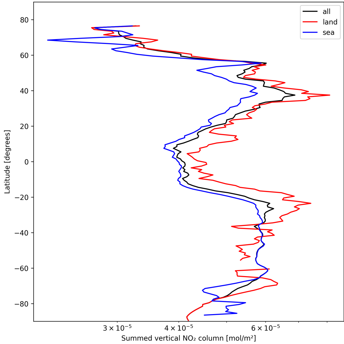
Figure 21: Zonal average of “Summed vertical NO 2 column” for 2025-10-23 to 2025-10-24.
