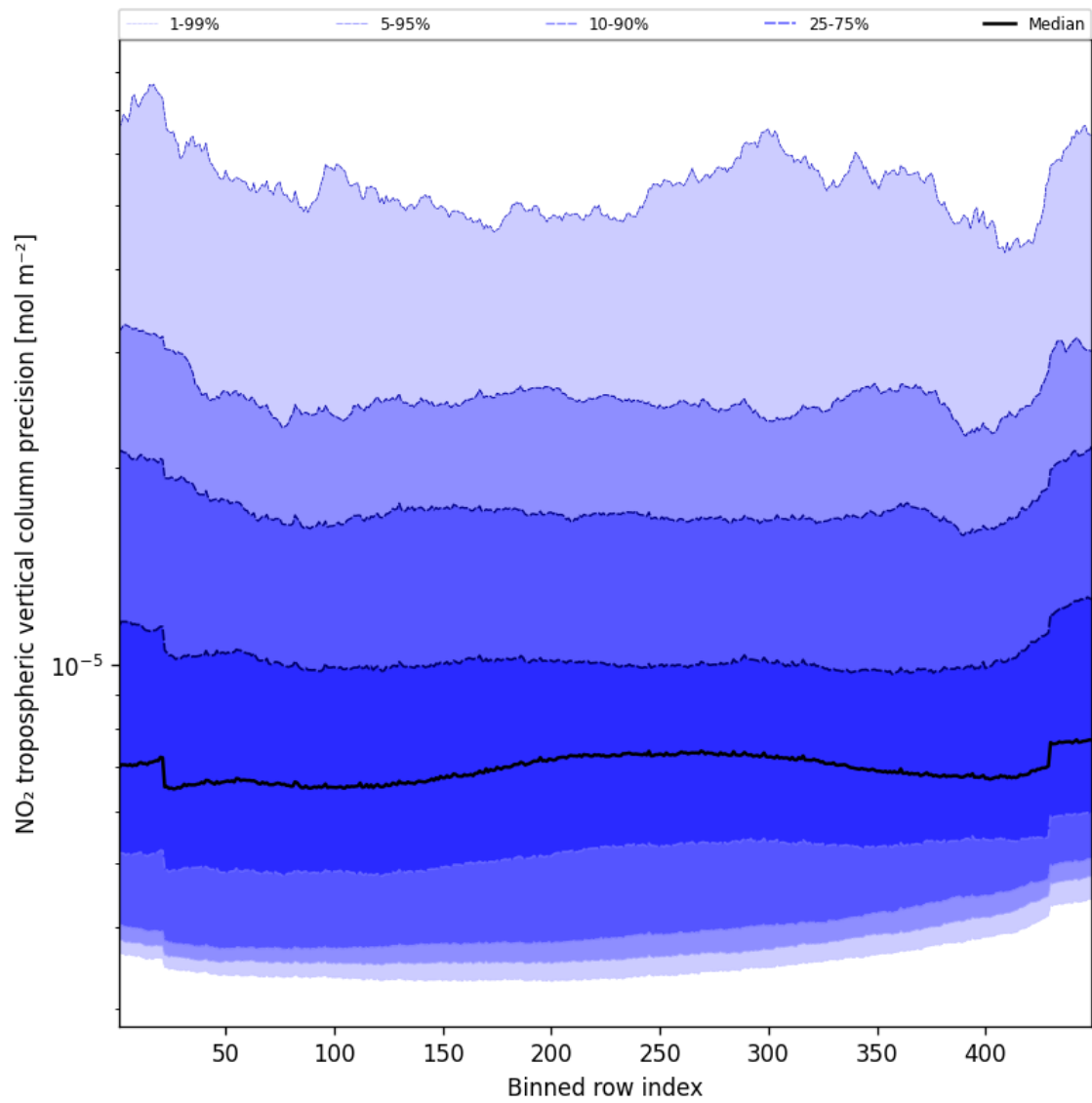
Figure 45: Along track statistics of “NO 2 tropospheric vertical column precision” for 2025-10-23 to 2025-10-24
