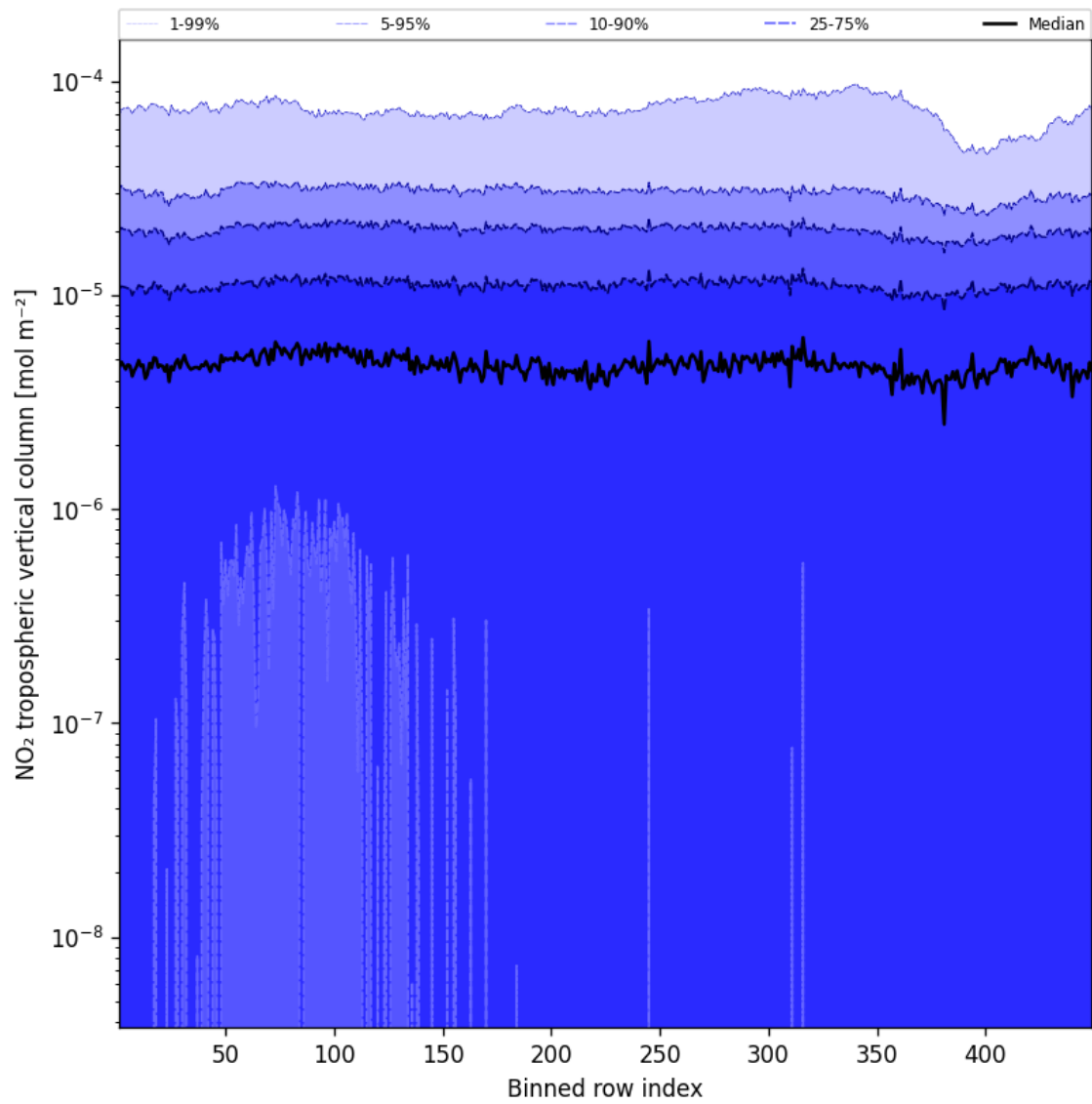
Figure 44: Along track statistics of “NO 2 tropospheric vertical column” for 2025-10-23 to 2025-10-24
