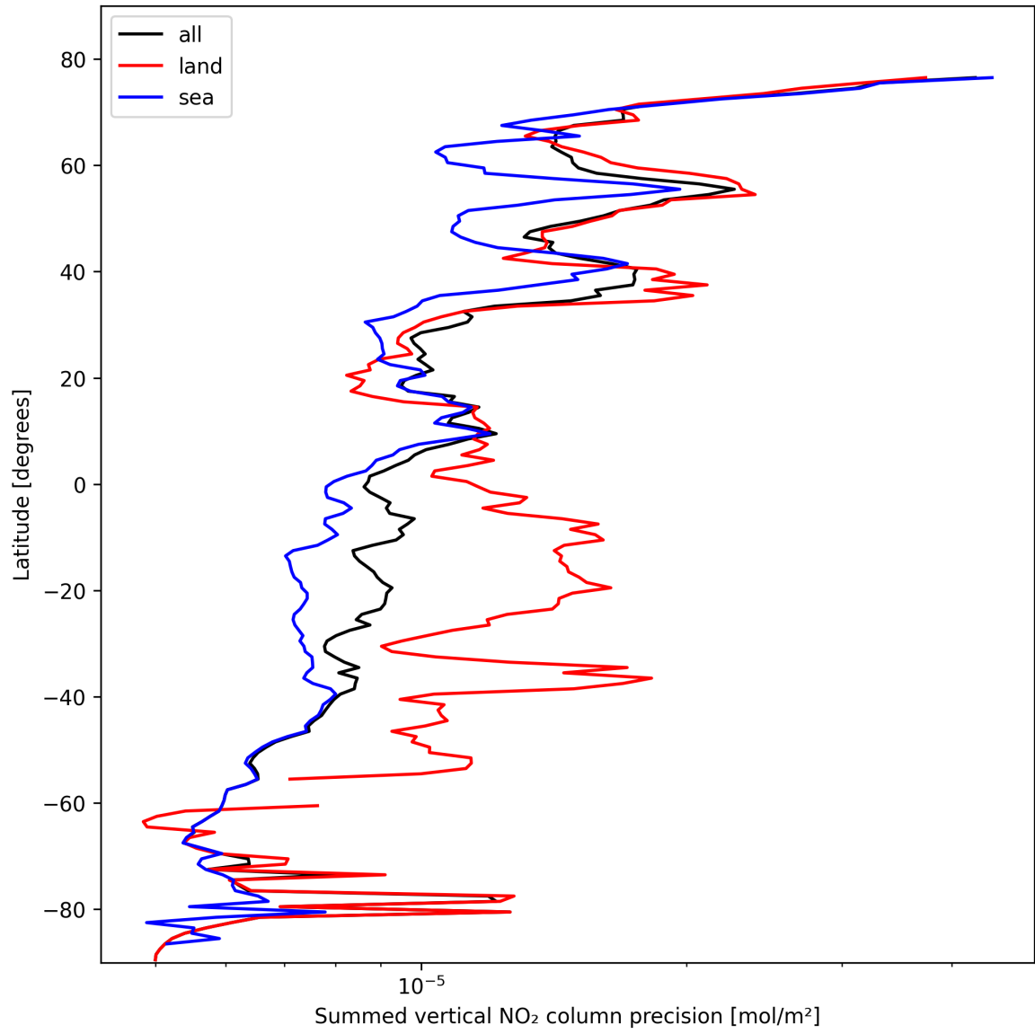
Figure 22: Zonal average of “Summed vertical NO 2 column precision” for 2025-10-23 to 2025-10-24.
