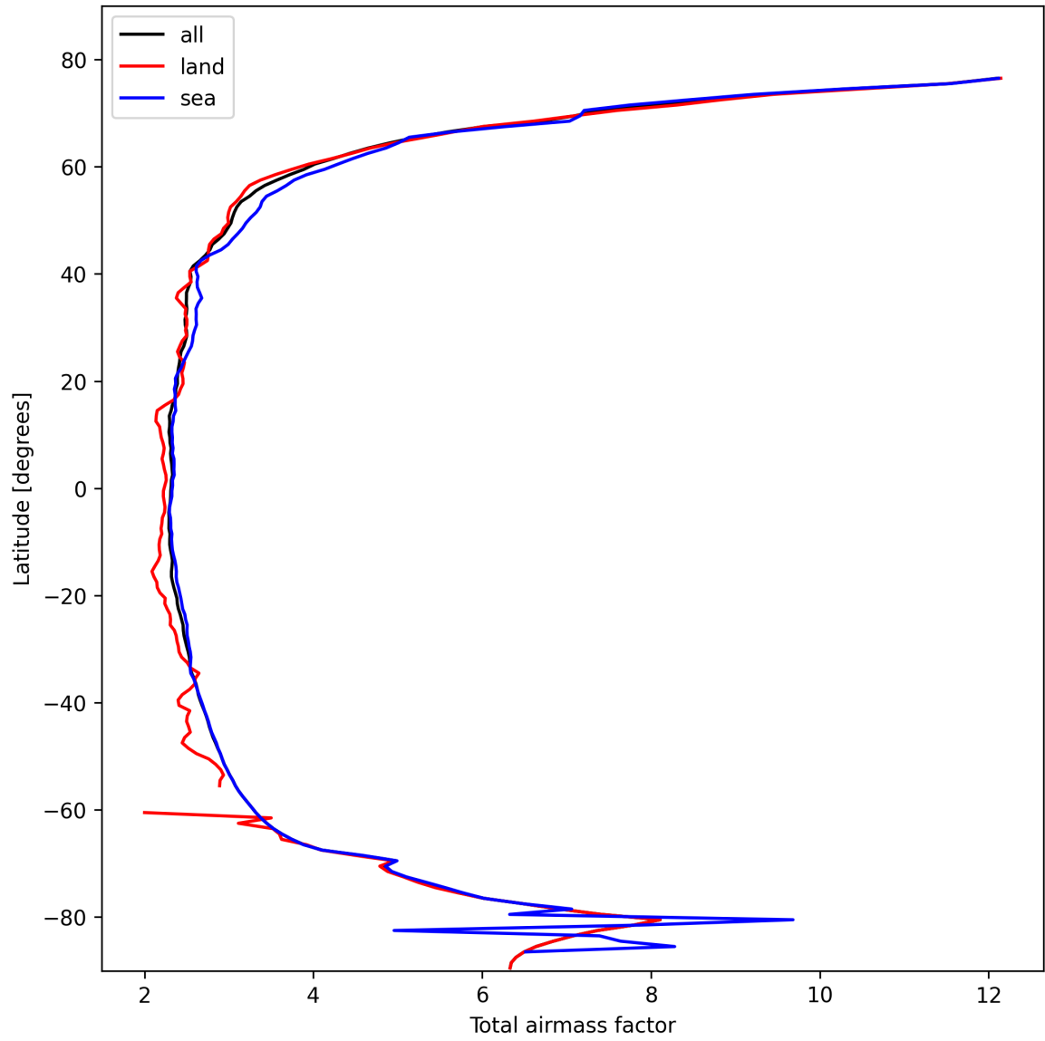
Figure 13: Zonal average of “Total airmass factor” for 2025-10-23 to 2025-10-24.
