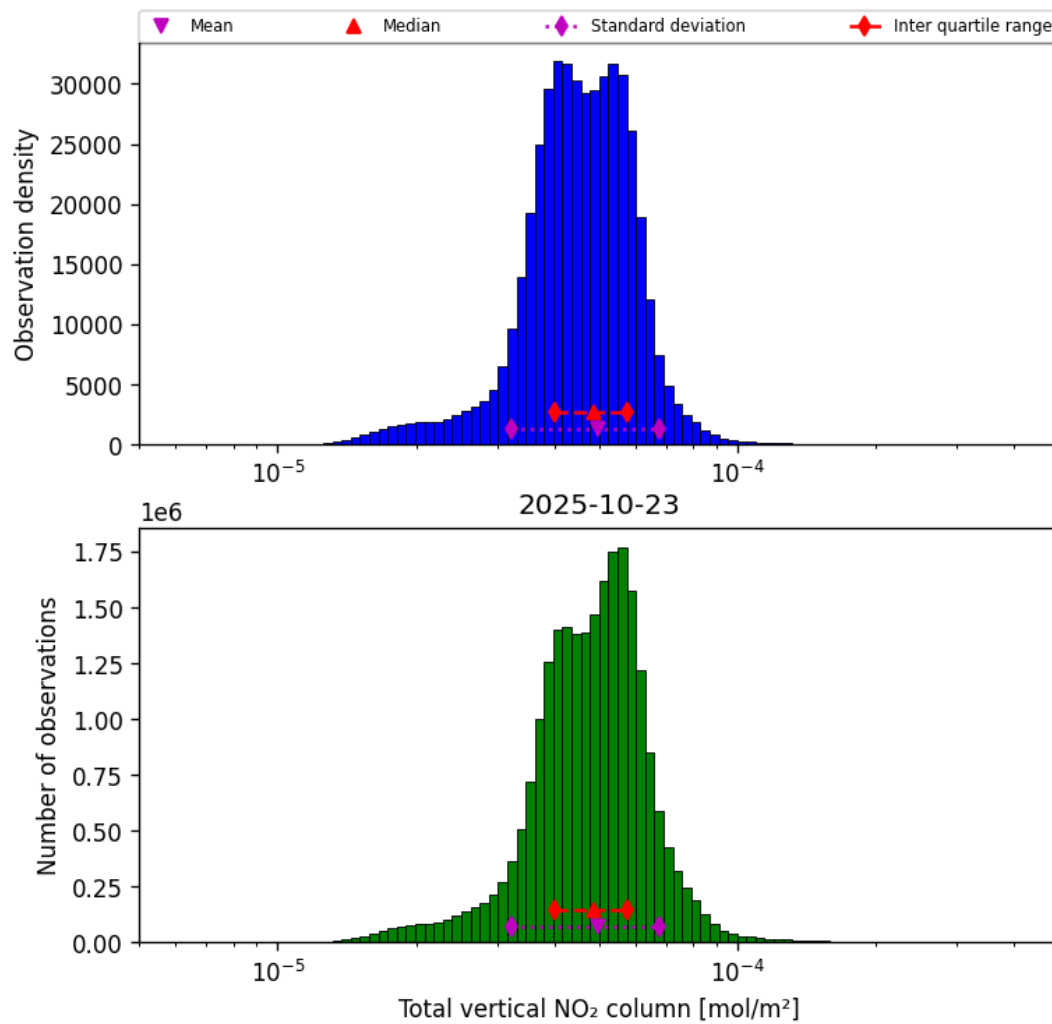
Figure 36: Histogram of “Total vertical NO 2 column” for 2025-10-23 to 2025-10-24
