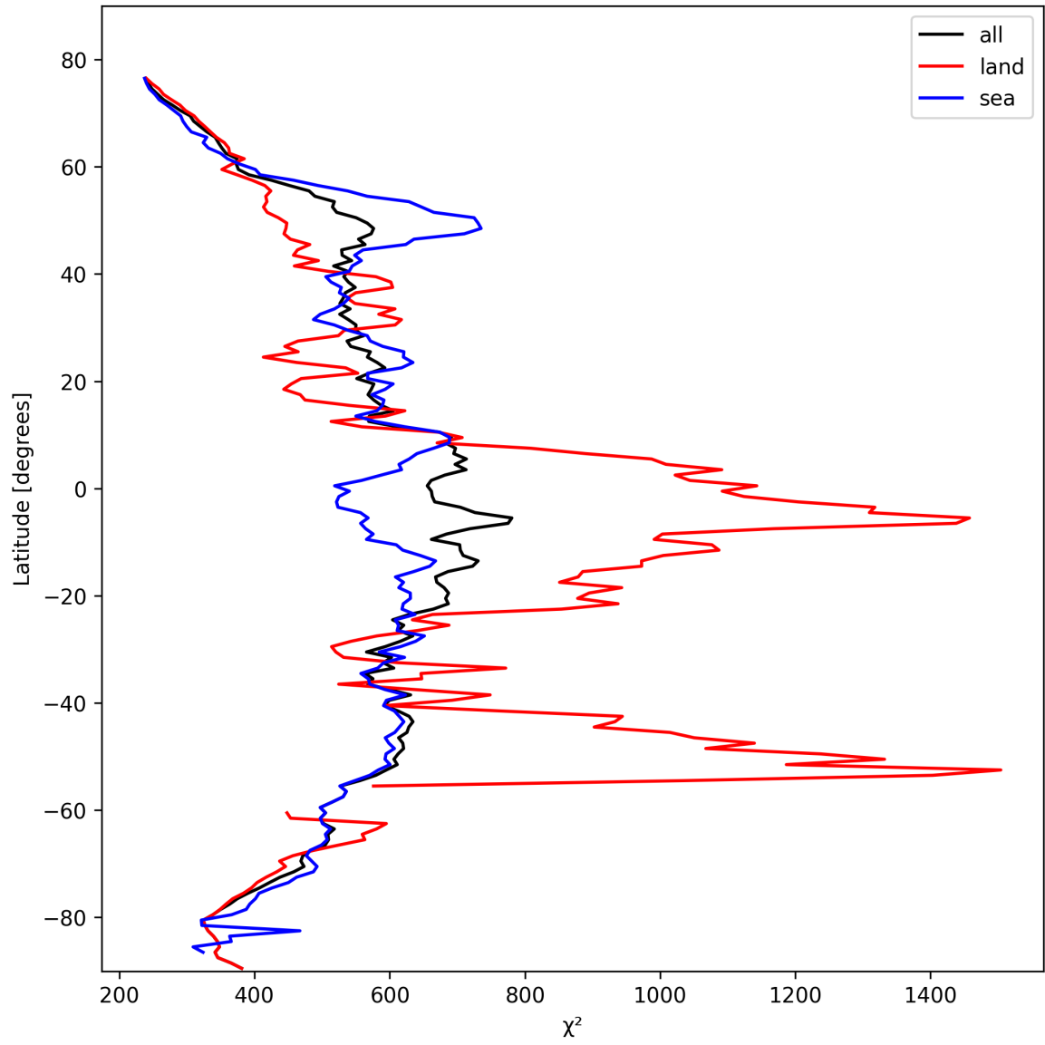
Figure 23: Zonal average of “ \chi^2 ” for 2025-10-23 to 2025-10-24.
