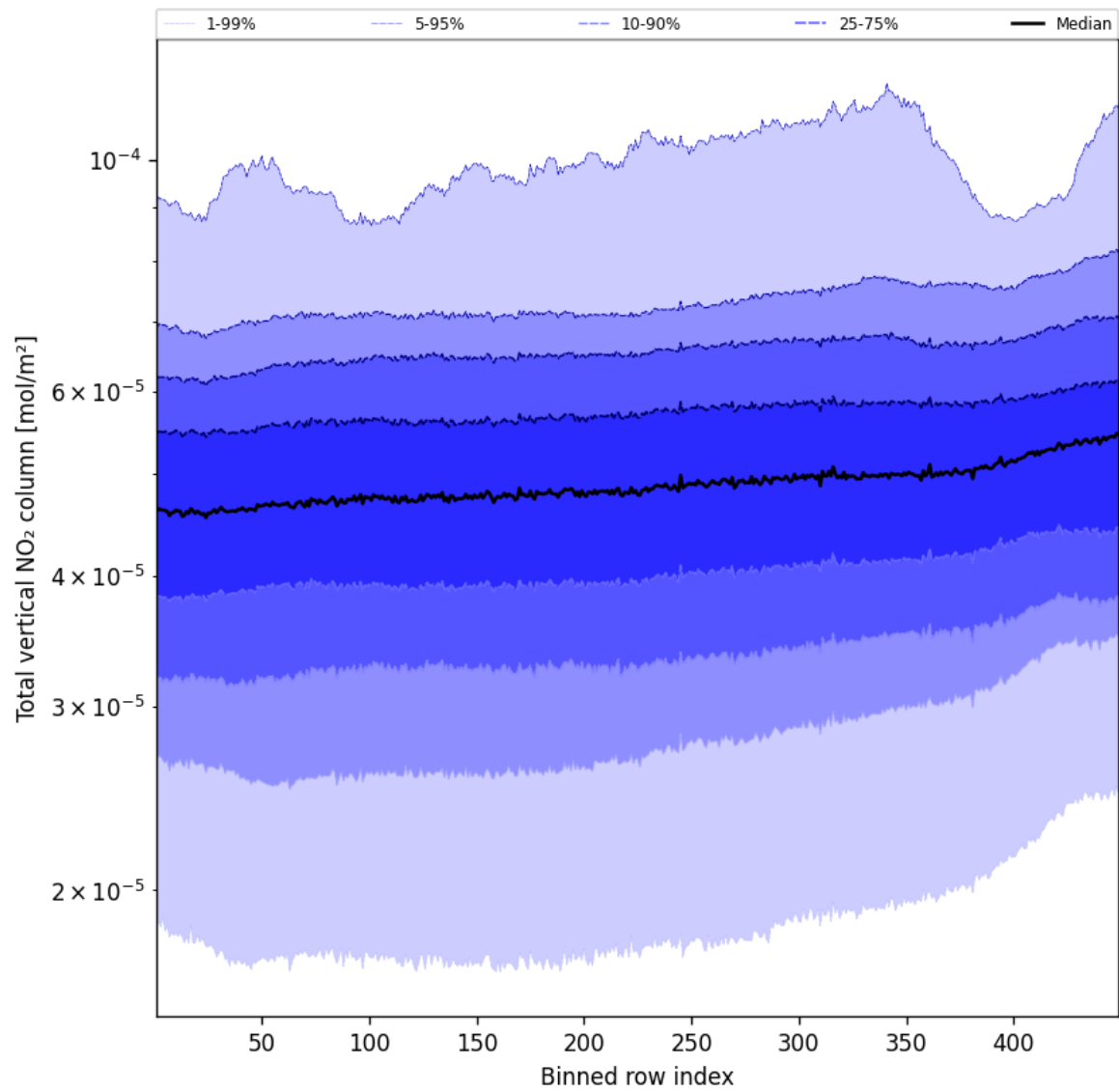
Figure 53: Along track statistics of “Total vertical NO 2 column” for 2025-10-23 to 2025-10-24
