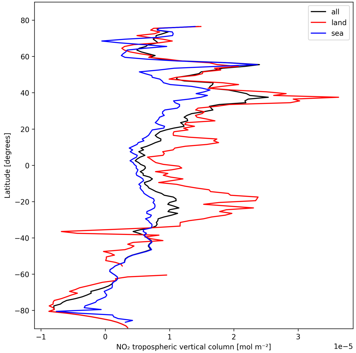
Figure 10: Zonal average of “NO 2 tropospheric vertical column” for 2025-10-23 to 2025-10-24.
