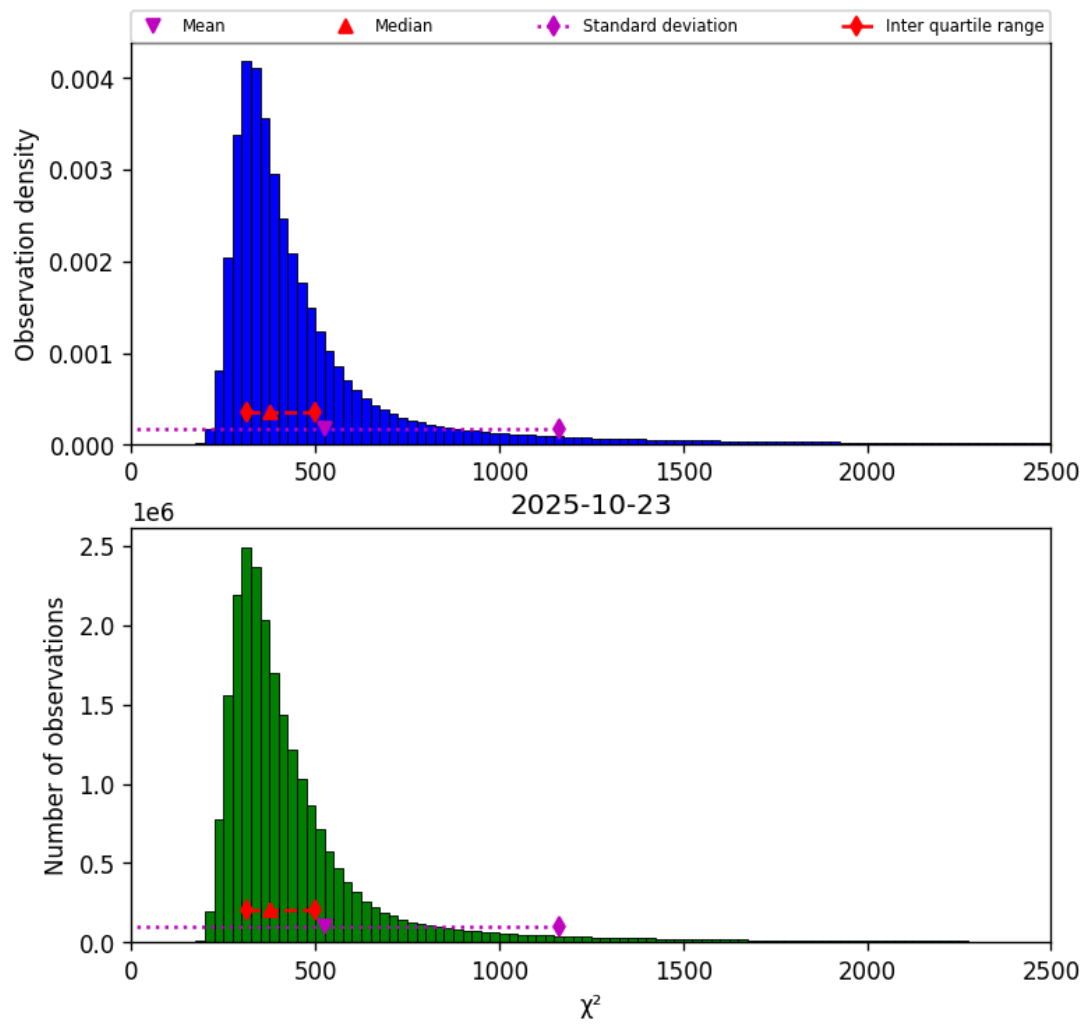
Figure 40: Histogram of “ \chi^2 ” for 2025-10-23 to 2025-10-24
