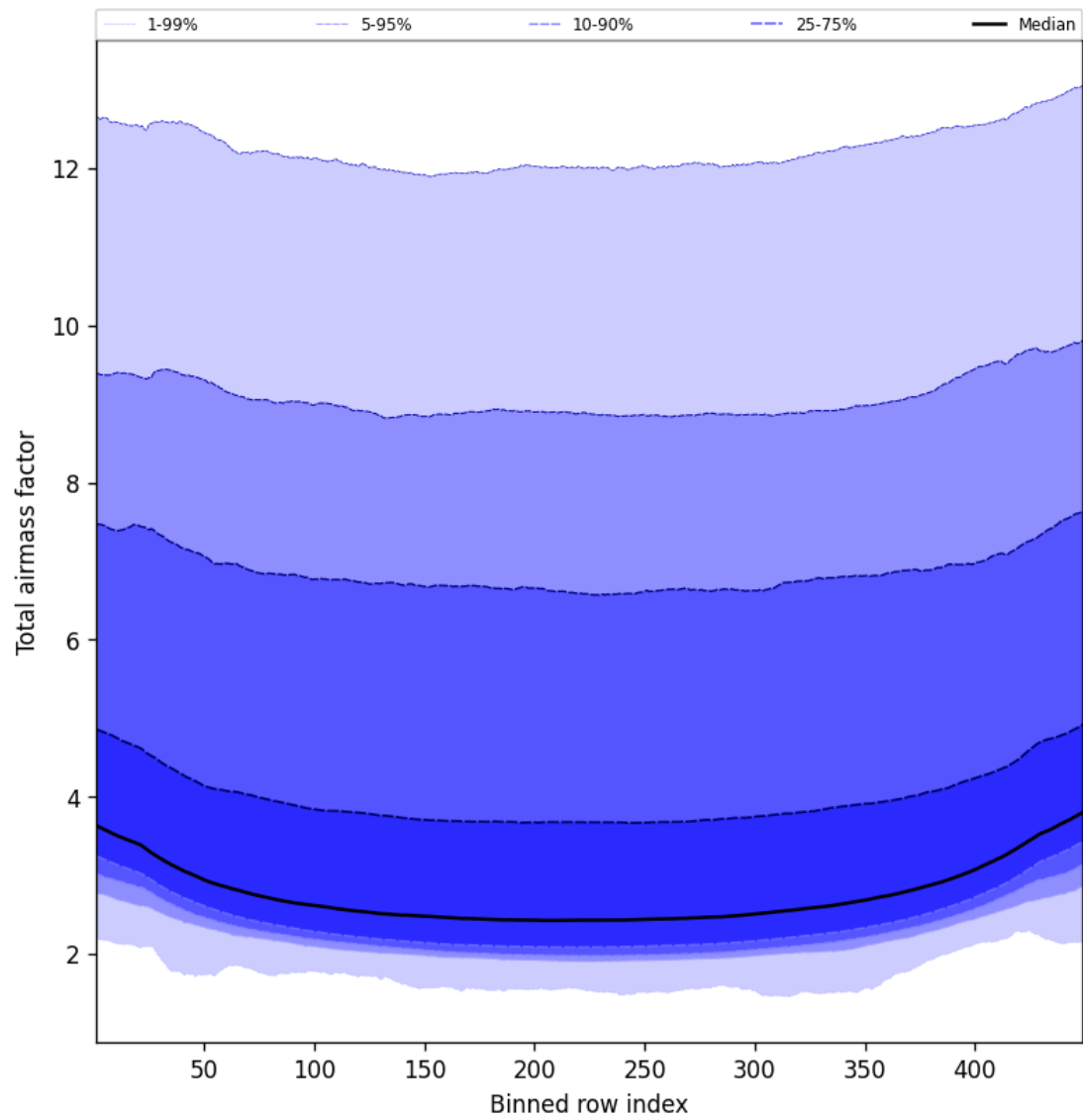
Figure 47: Along track statistics of “Total airmass factor” for 2025-10-23 to 2025-10-24
