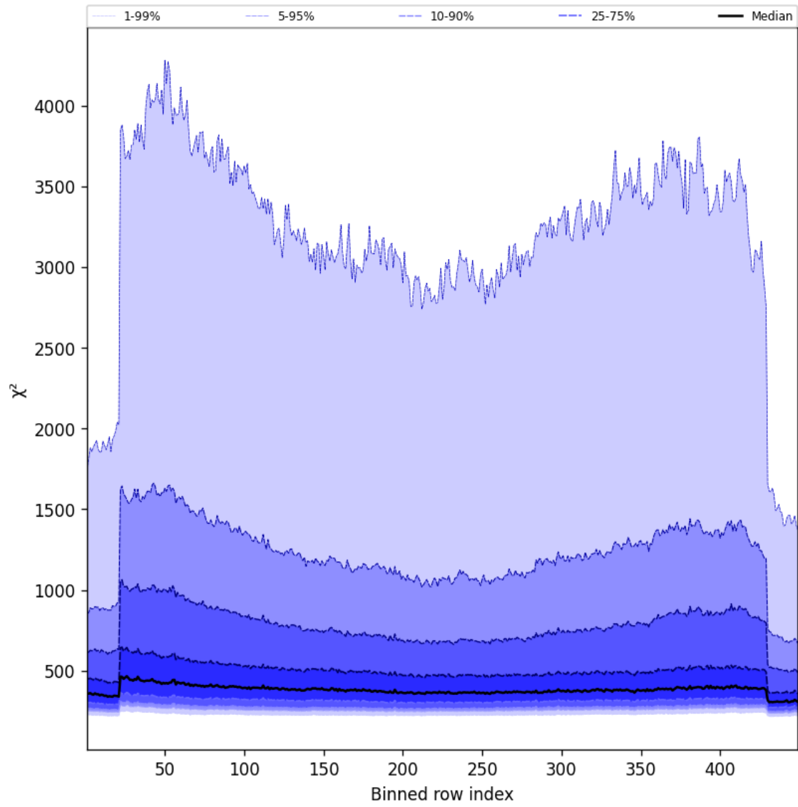
Figure 57: Along track statistics of “ \chi^2 ” for 2025-10-23 to 2025-10-24
