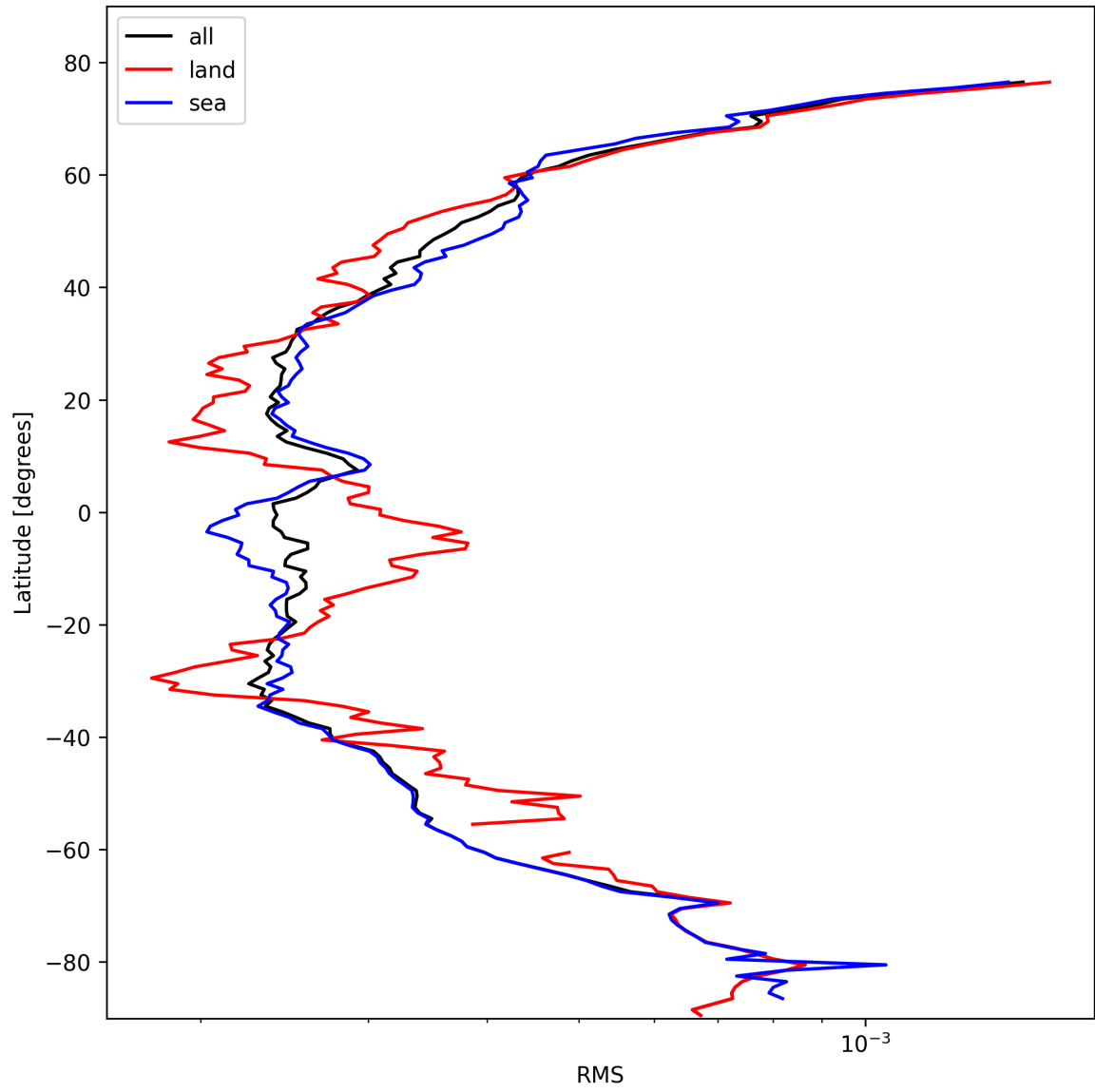
Figure 24: Zonal average of “RMS” for 2025-10-23 to 2025-10-24.
