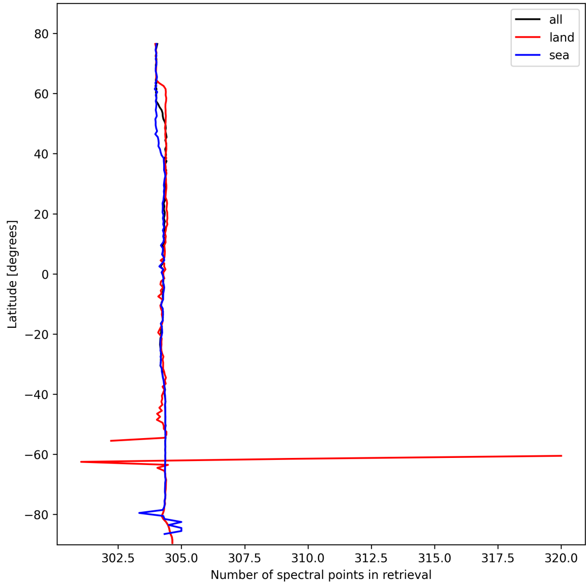
Figure 14: Zonal average of “Number of spectral points in retrieval” for 2025-10-23 to 2025-10-24.
