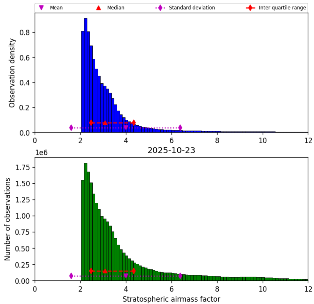
Figure 42: Histogram of “Stratospheric airmass factor” for 2025-10-23 to 2025-10-24
