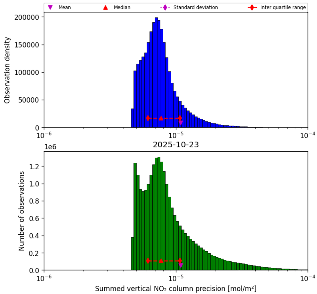
Figure 39: Histogram of “Summed vertical NO 2 column precision” for 2025-10-23 to 2025-10-24
