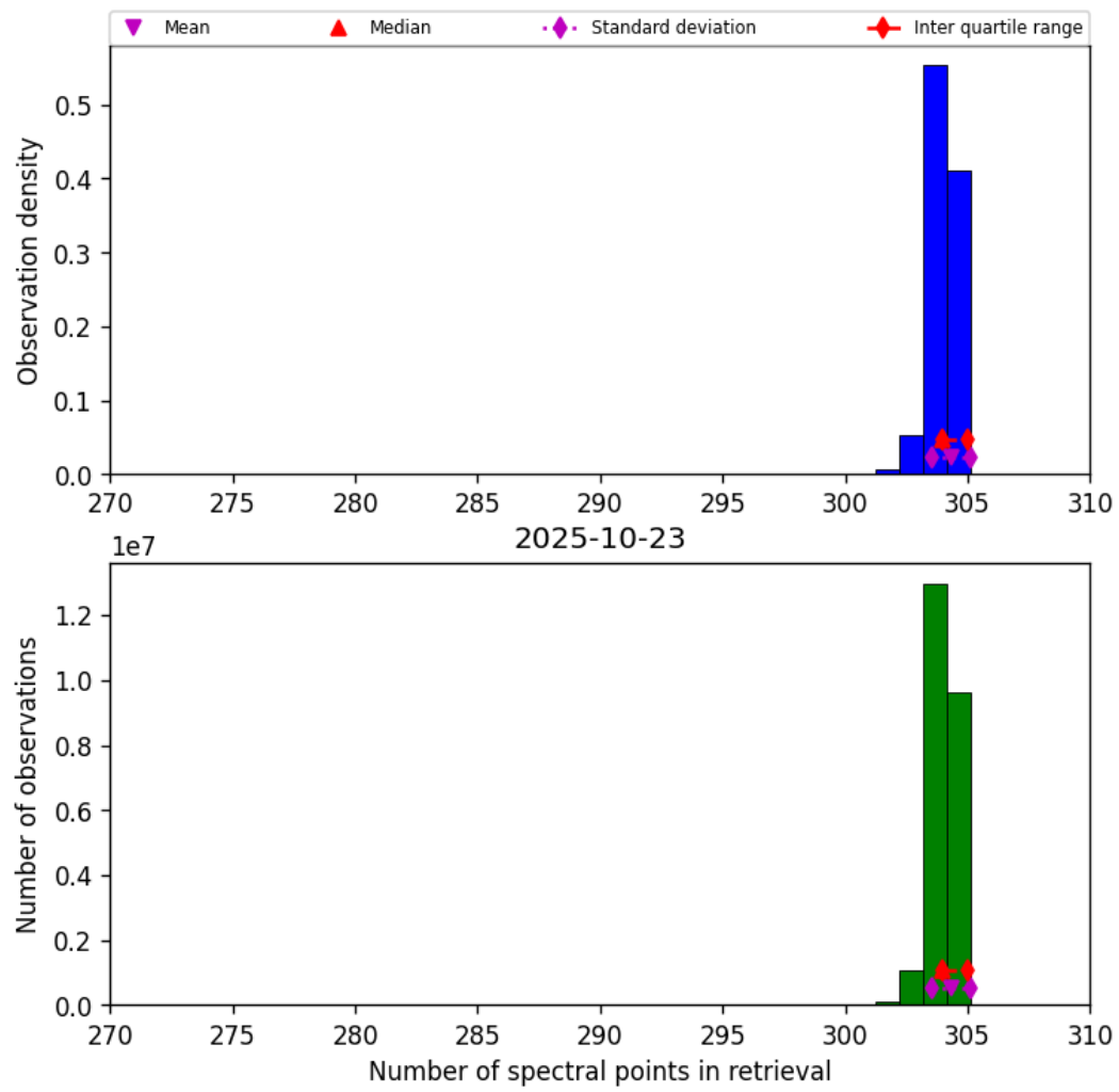
Figure 31: Histogram of “Number of spectral points in retrieval” for 2025-10-23 to 2025-10-24
