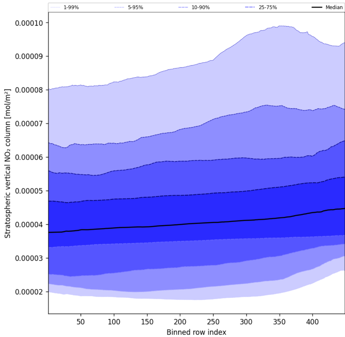
Figure 51: Along track statistics of “Stratospheric vertical NO 2 column” for 2025-10-23 to 2025-10-24
