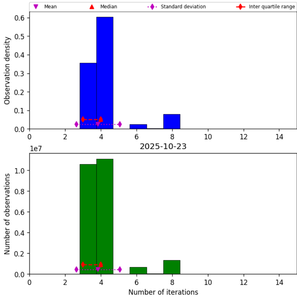
Figure 32: Histogram of “Number of iterations” for 2025-10-23 to 2025-10-24
