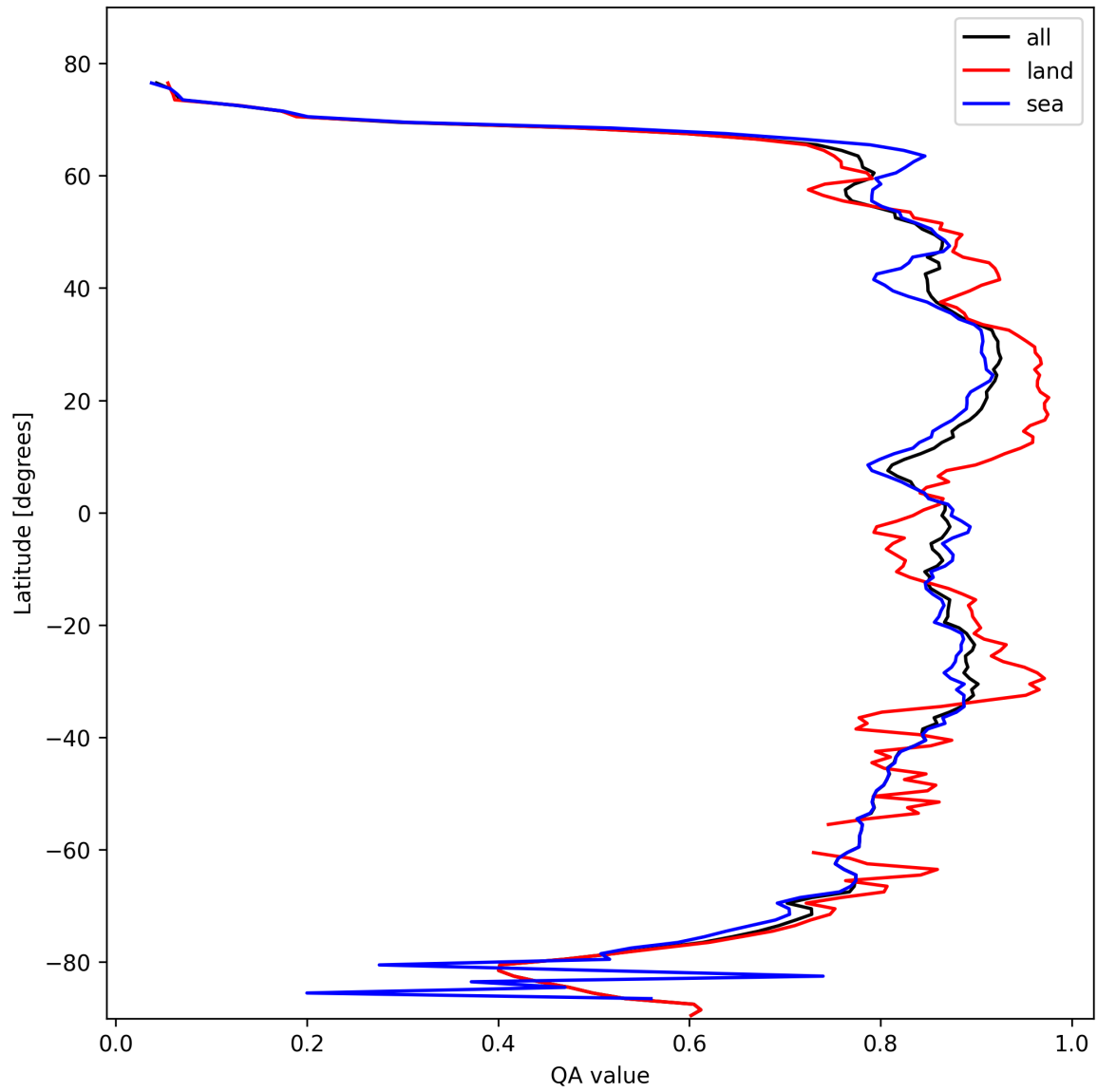
Figure 9: Zonal average of “QA value” for 2025-10-23 to 2025-10-24.
