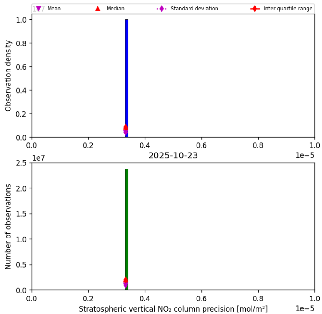
Figure 35: Histogram of “Stratospheric vertical NO 2 column precision” for 2025-10-23 to 2025-10-24
