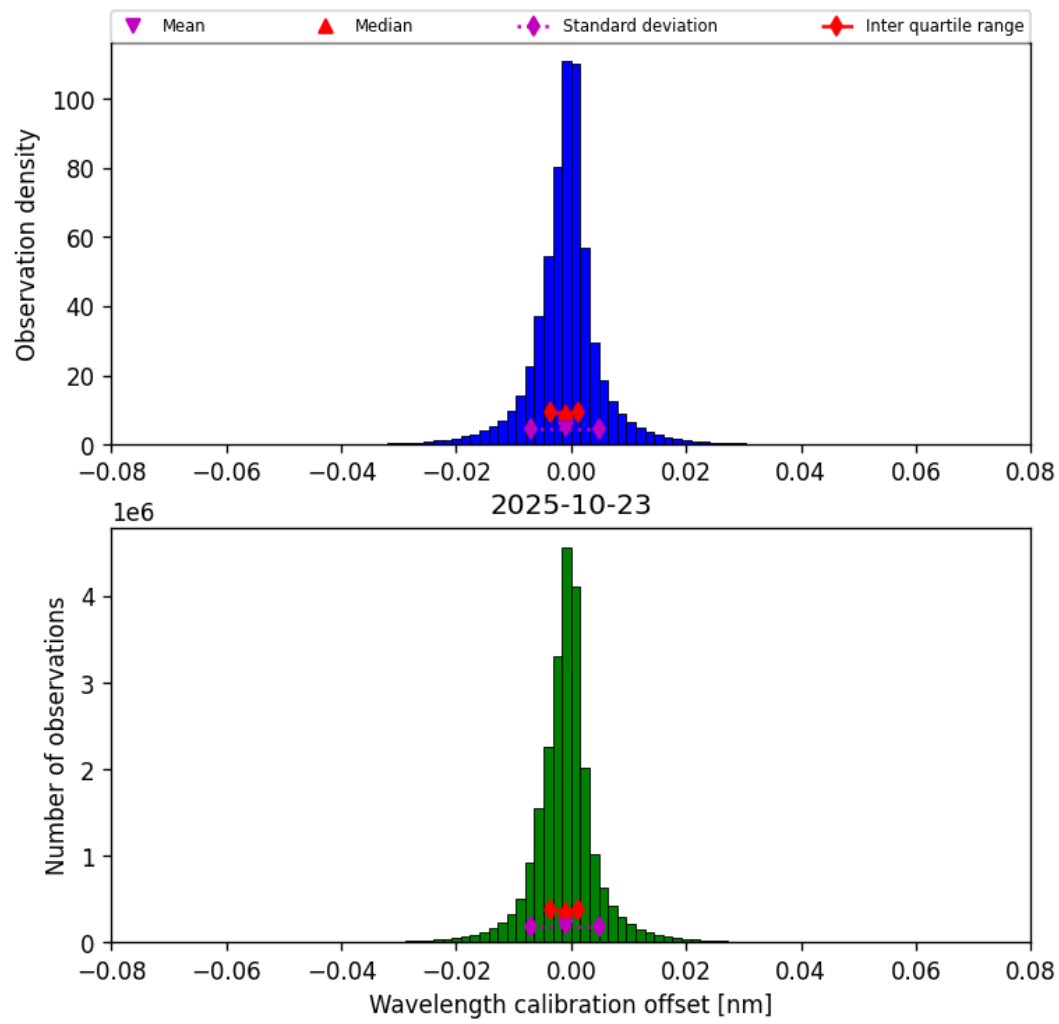
Figure 33: Histogram of “Wavelength calibration offset” for 2025-10-23 to 2025-10-24
