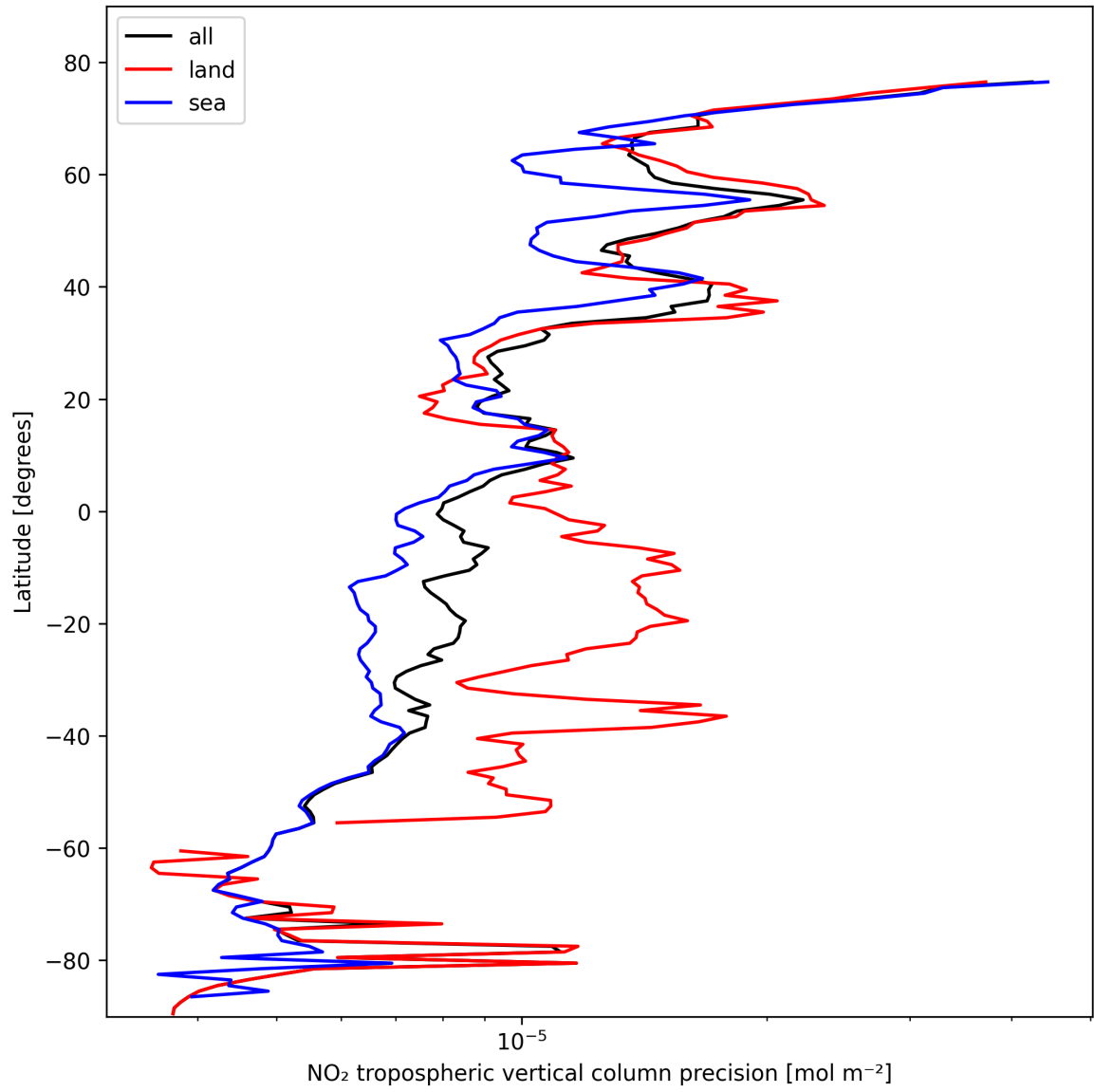
Figure 11: Zonal average of “NO 2 tropospheric vertical column precision” for 2025-10-23 to 2025-10-24.
