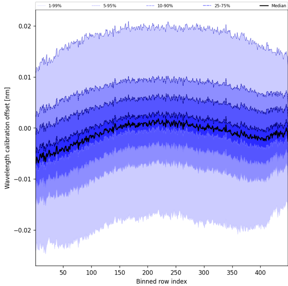
Figure 50: Along track statistics of “Wavelength calibration offset” for 2025-10-23 to 2025-10-24
