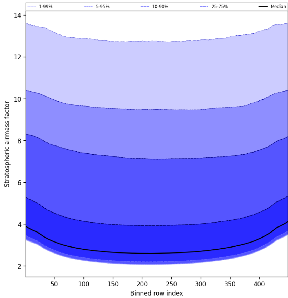
Figure 59: Along track statistics of “Stratospheric airmass factor” for 2025-10-23 to 2025-10-24
