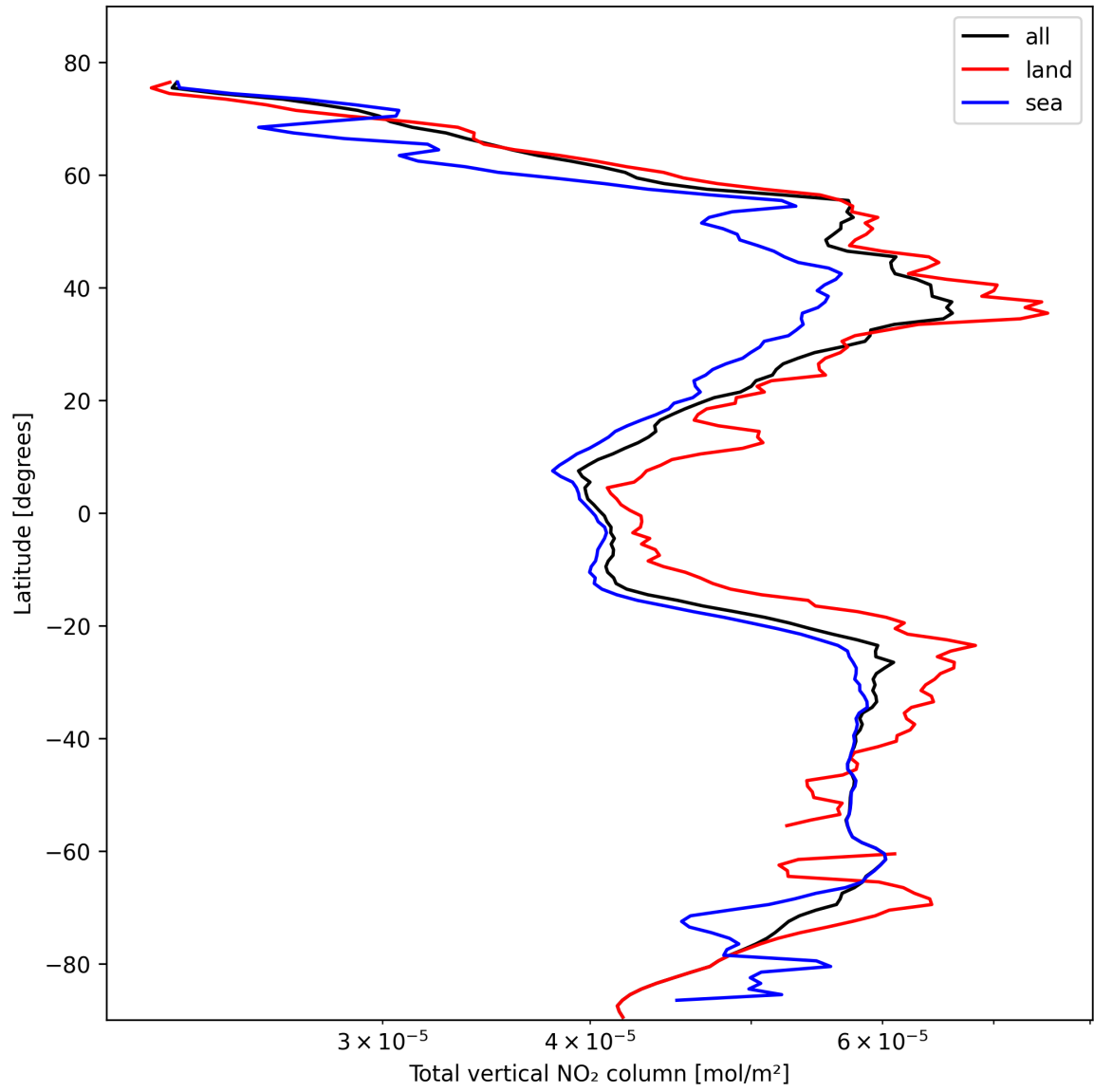
Figure 19: Zonal average of “Total vertical NO 2 column” for 2025-10-23 to 2025-10-24.
