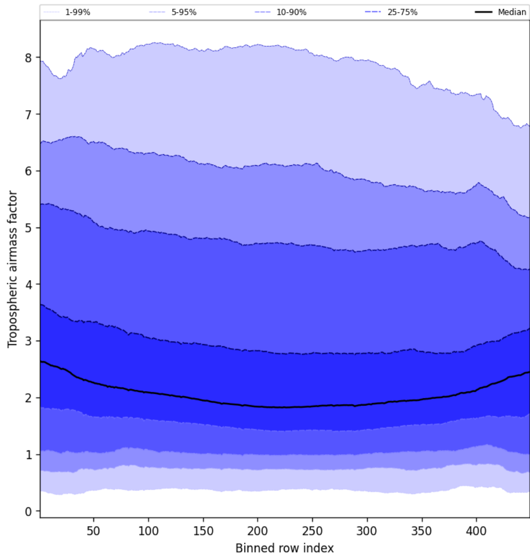
Figure 46: Along track statistics of “Tropospheric air mass factor” for 2025-10-23 to 2025-10-24
