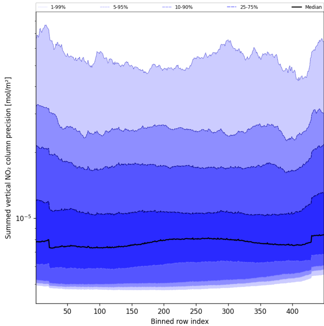
Figure 56: Along track statistics of “Summed vertical NO 2 column precision” for 2025-10-23 to 2025-10-24
