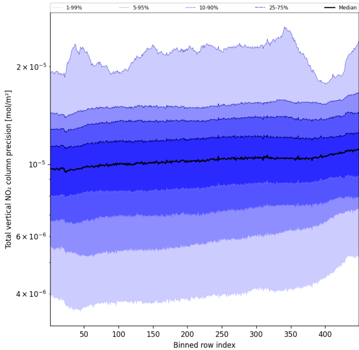
Figure 54: Along track statistics of “Total vertical NO 2 column precision” for 2025-10-23 to 2025-10-24
