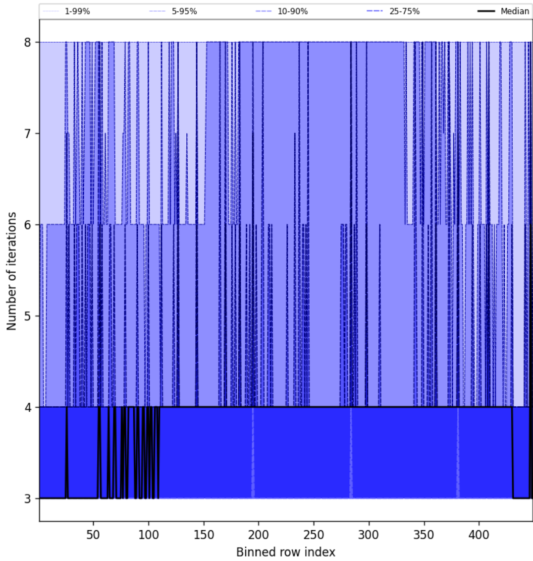
Figure 49: Along track statistics of “Number of iterations” for 2025-10-23 to 2025-10-24
