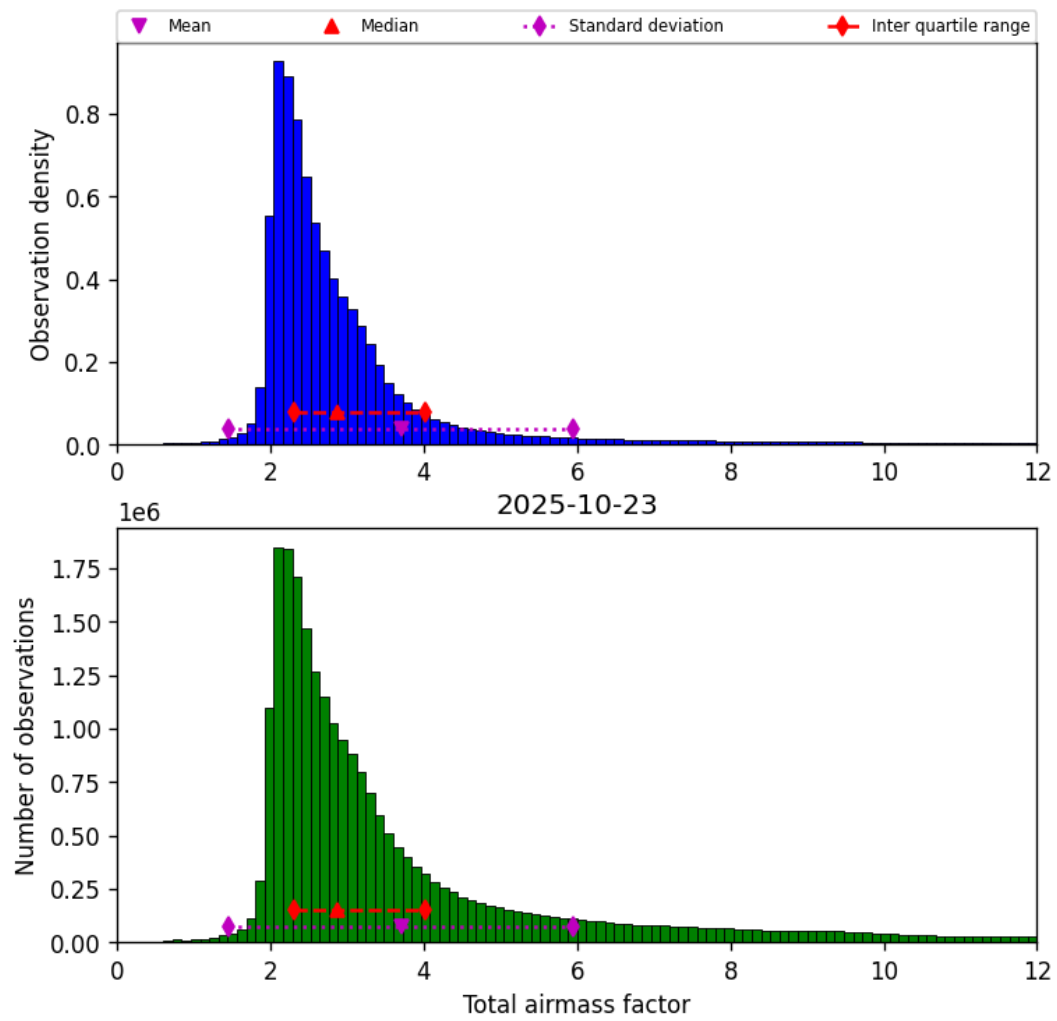
Figure 30: Histogram of “Total airmass factor” for 2025-10-23 to 2025-10-24
