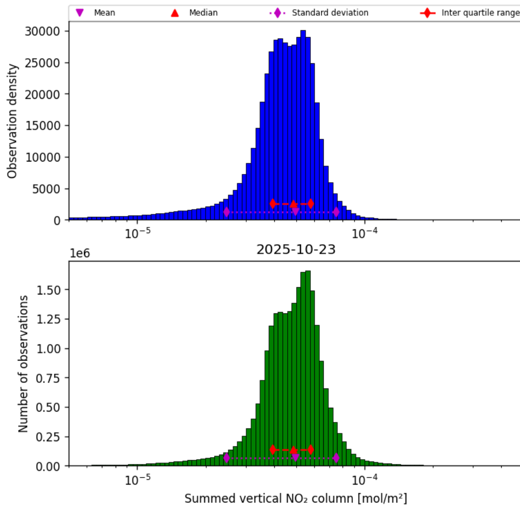
Figure 38: Histogram of “Summed vertical NO 2 column” for 2025-10-23 to 2025-10-24
