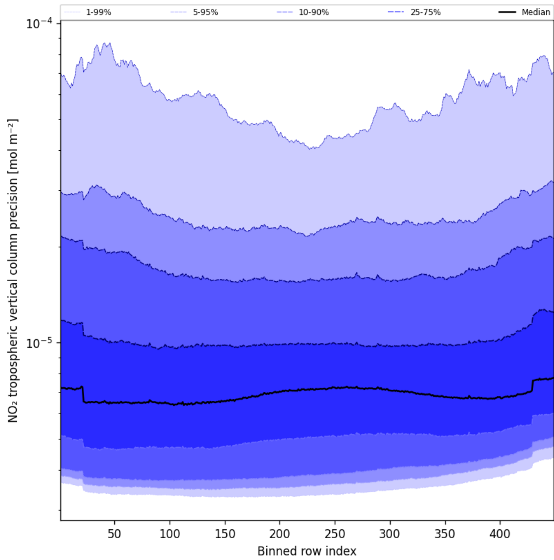
Figure 45: Along track statistics of “NO 2 tropospheric vertical column precision” for 2025-10-24 to 2025-10-25
