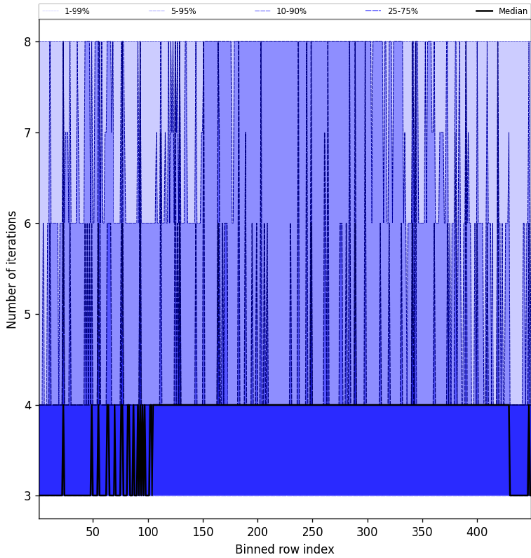
Figure 49: Along track statistics of “Number of iterations” for 2025-10-24 to 2025-10-25
