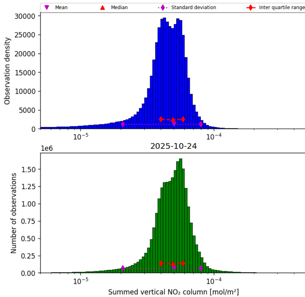
Figure 38: Histogram of “Summed vertical NO 2 column” for 2025-10-24 to 2025-10-25
