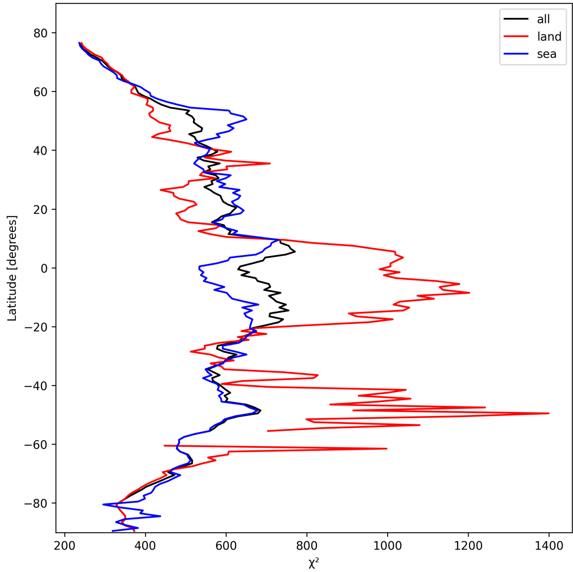
Figure 23: Zonal average of “ \chi^2 ” for 2025-10-24 to 2025-10-25.
