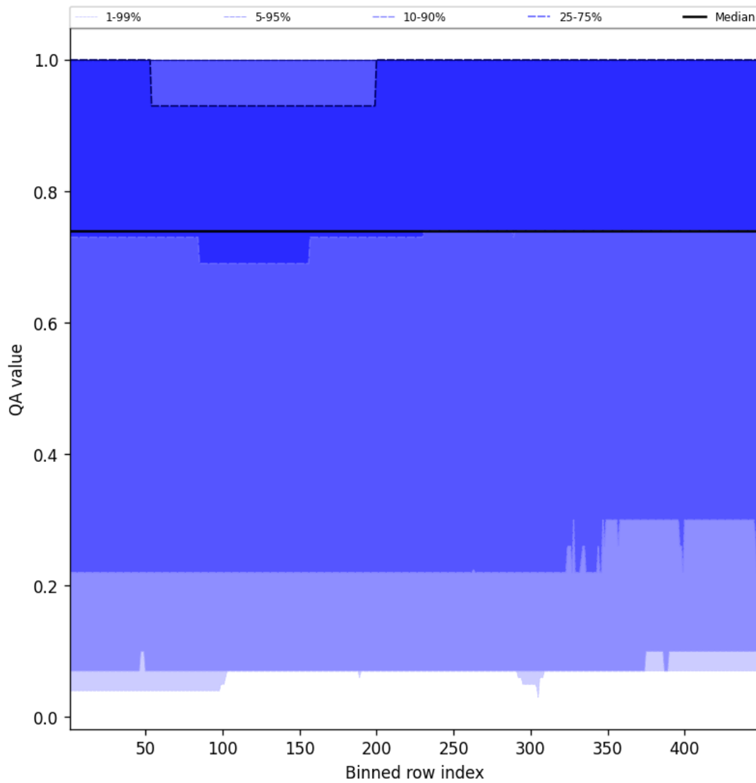
Figure 43: Along track statistics of “QA value” for 2025-10-24 to 2025-10-25
