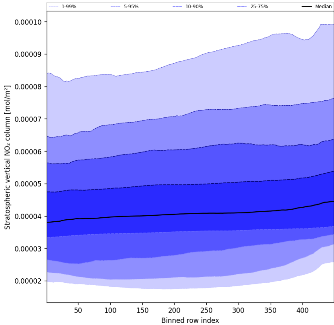
Figure 51: Along track statistics of “Stratospheric vertical NO 2 column” for 2025-10-24 to 2025-10-25
