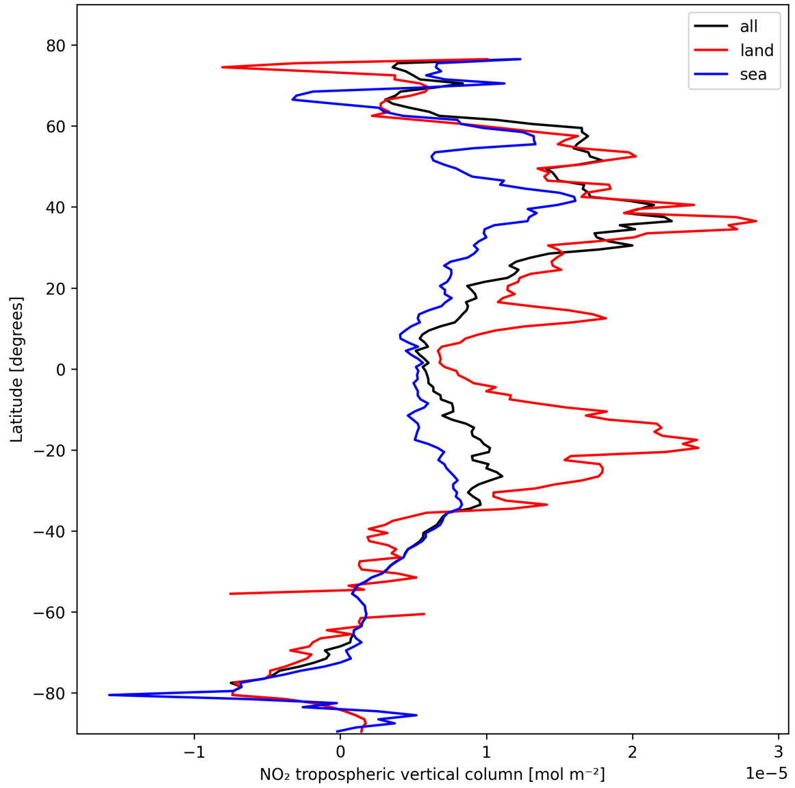
Figure 10: Zonal average of “NO 2 tropospheric vertical column” for 2025-10-24 to 2025-10-25.
