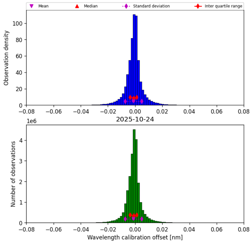
Figure 33: Histogram of “Wavelength calibration offset” for 2025-10-24 to 2025-10-25
