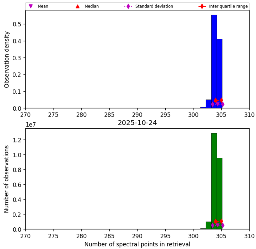
Figure 31: Histogram of “Number of spectral points in retrieval” for 2025-10-24 to 2025-10-25
