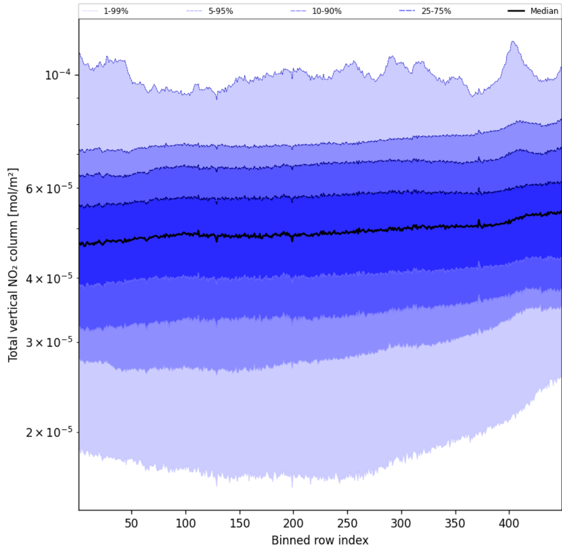
Figure 53: Along track statistics of “Total vertical NO 2 column” for 2025-10-24 to 2025-10-25
