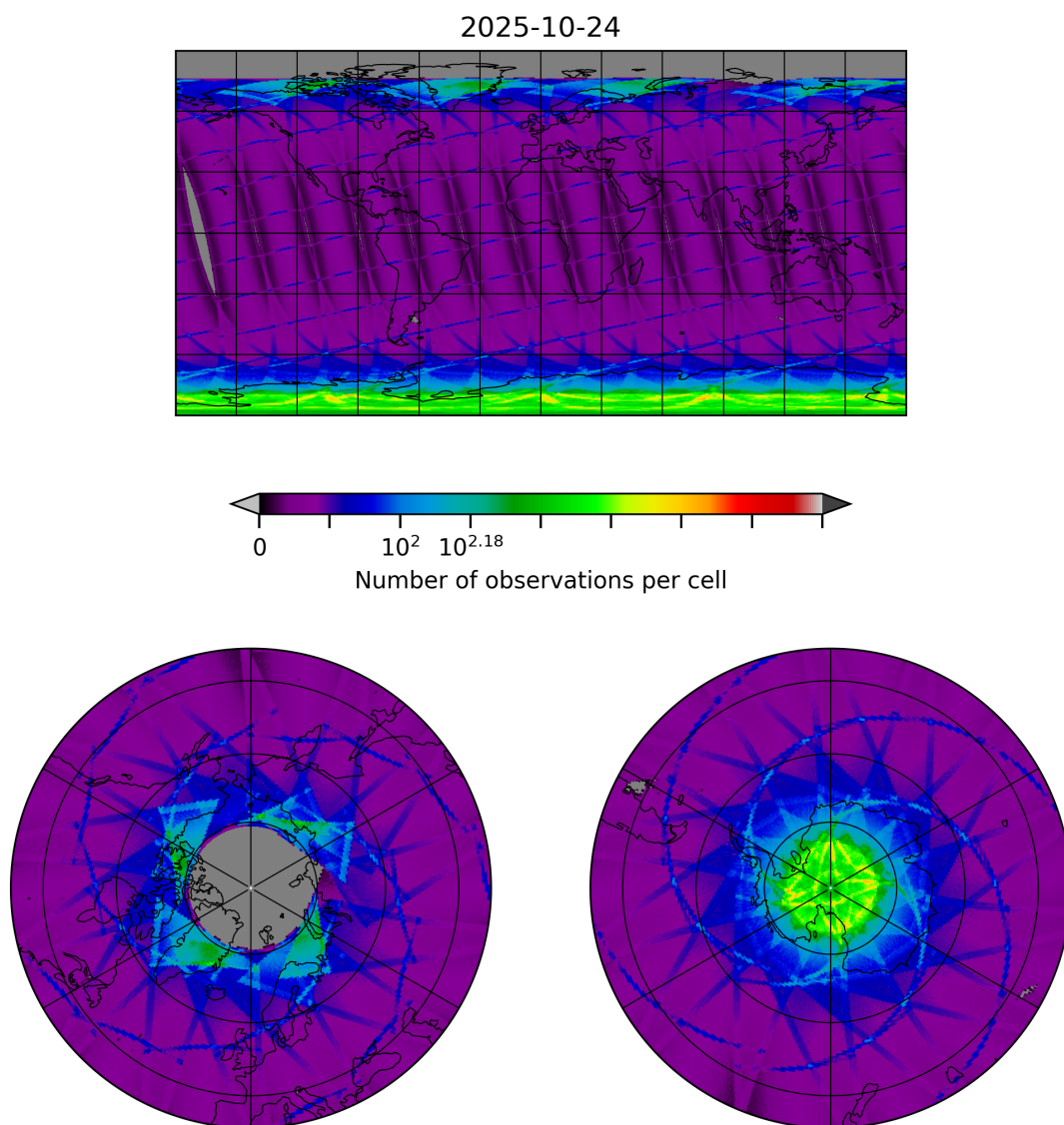
Figure 8: Map of the number of observations for 2025-10-24 to 2025-10-25
