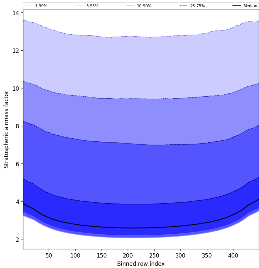
Figure 59: Along track statistics of “Stratospheric airmass factor” for 2025-10-24 to 2025-10-25
