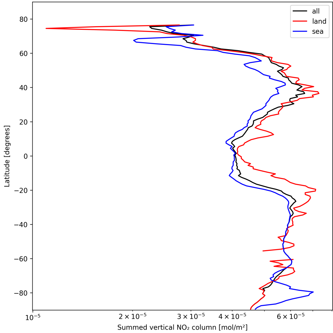
Figure 21: Zonal average of “Summed vertical NO 2 column” for 2025-10-24 to 2025-10-25.
