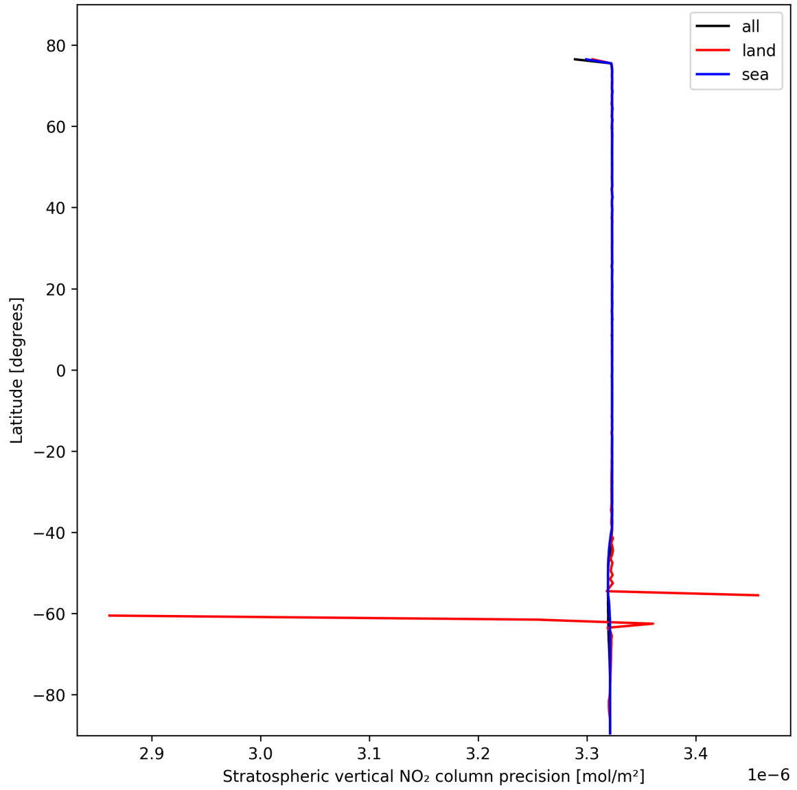
Figure 18: Zonal average of “Stratospheric vertical NO 2 column precision” for 2025-10-24 to 2025-10-25.
