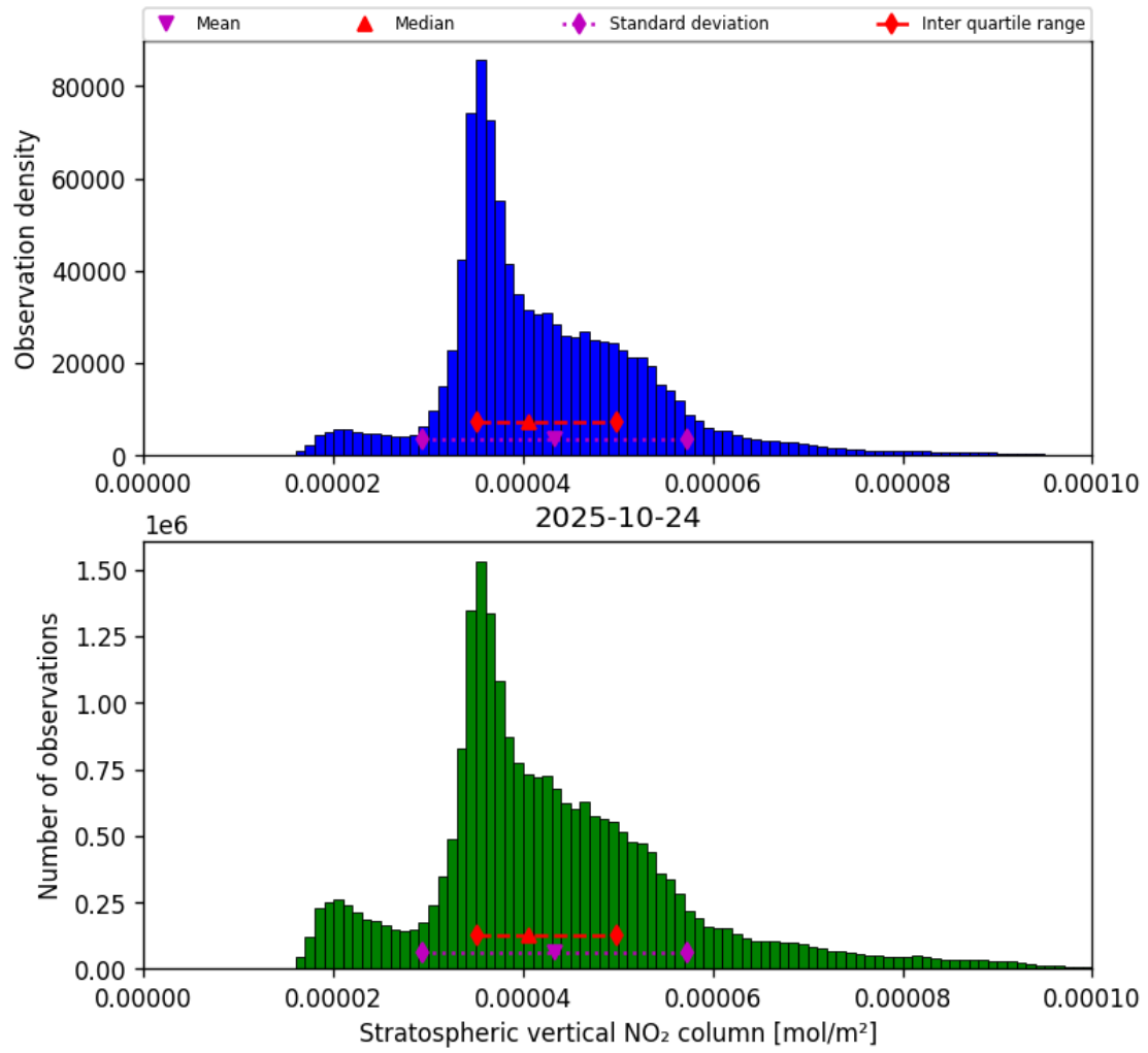
Figure 34: Histogram of “Stratospheric vertical NO 2 column” for 2025-10-24 to 2025-10-25
