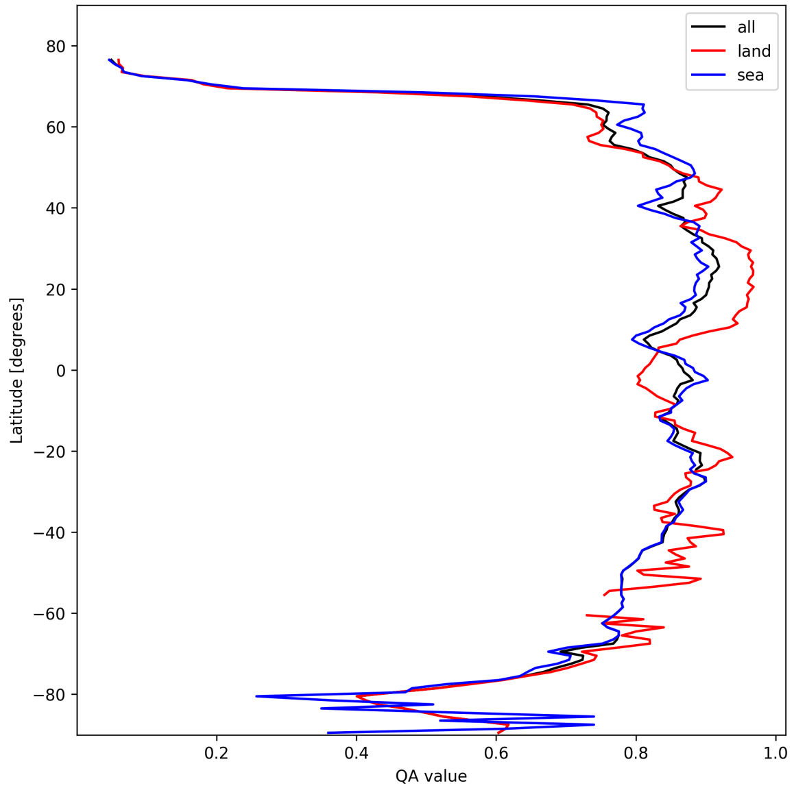
Figure 9: Zonal average of “QA value” for 2025-10-24 to 2025-10-25.
