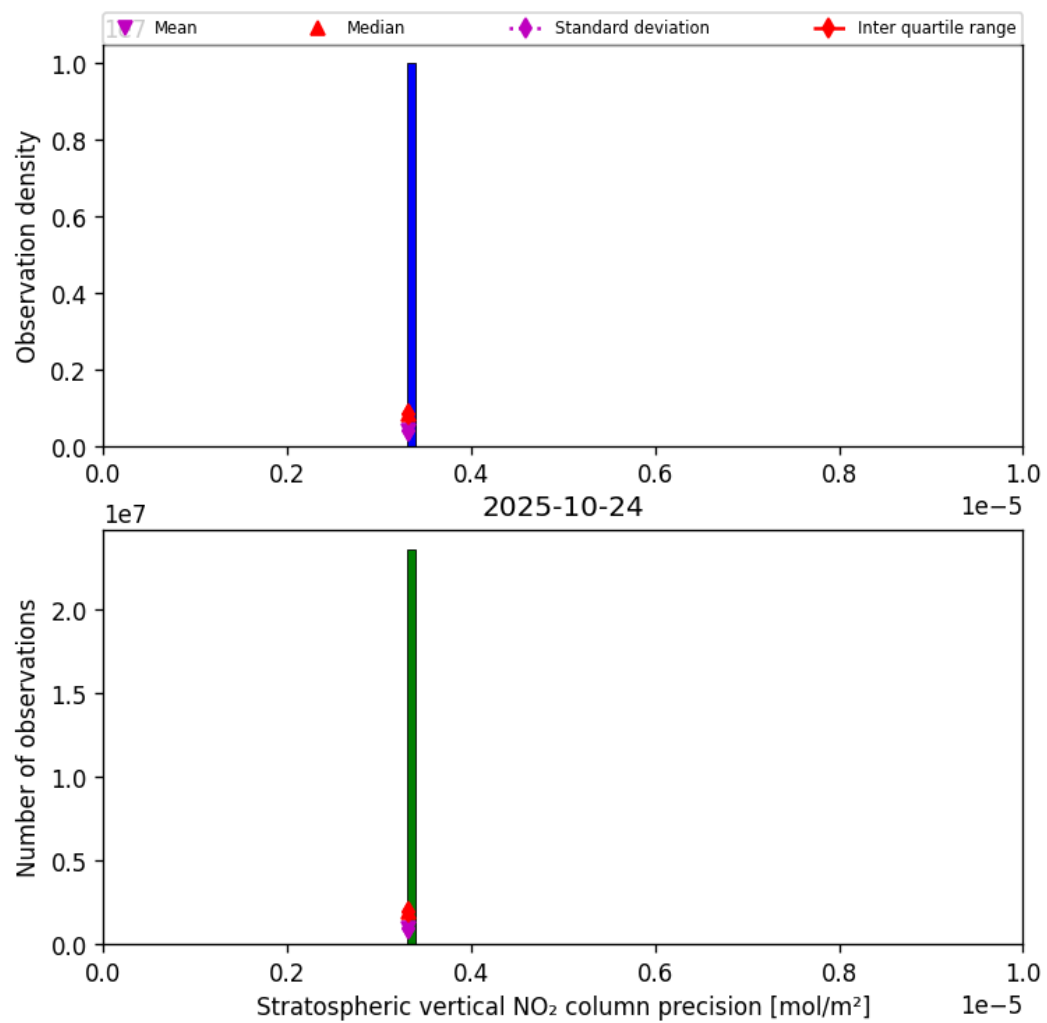
Figure 35: Histogram of “Stratospheric vertical NO 2 column precision” for 2025-10-24 to 2025-10-25
