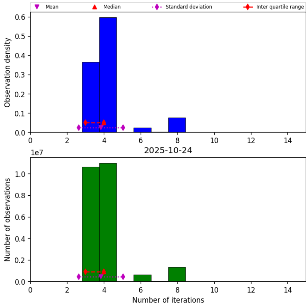
Figure 32: Histogram of “Number of iterations” for 2025-10-24 to 2025-10-25
