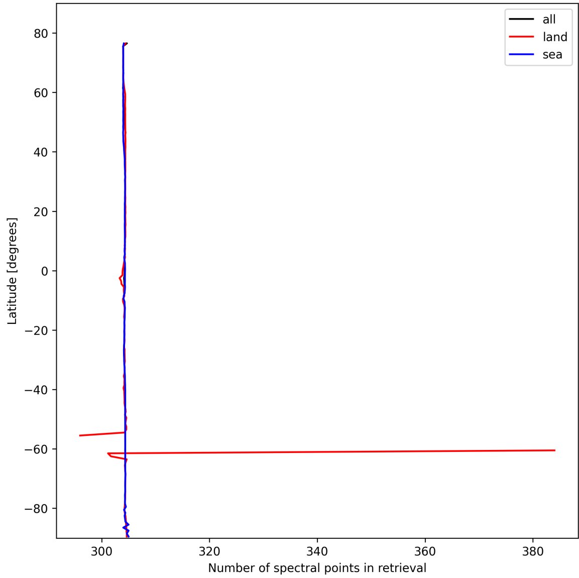
Figure 14: Zonal average of “Number of spectral points in retrieval” for 2025-10-24 to 2025-10-25.
