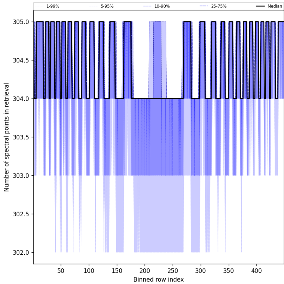
Figure 48: Along track statistics of “Number of spectral points in retrieval” for 2025-10-24 to 2025-10-25
