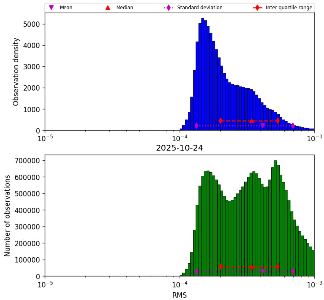
Figure 41: Histogram of “RMS” for 2025-10-24 to 2025-10-25
