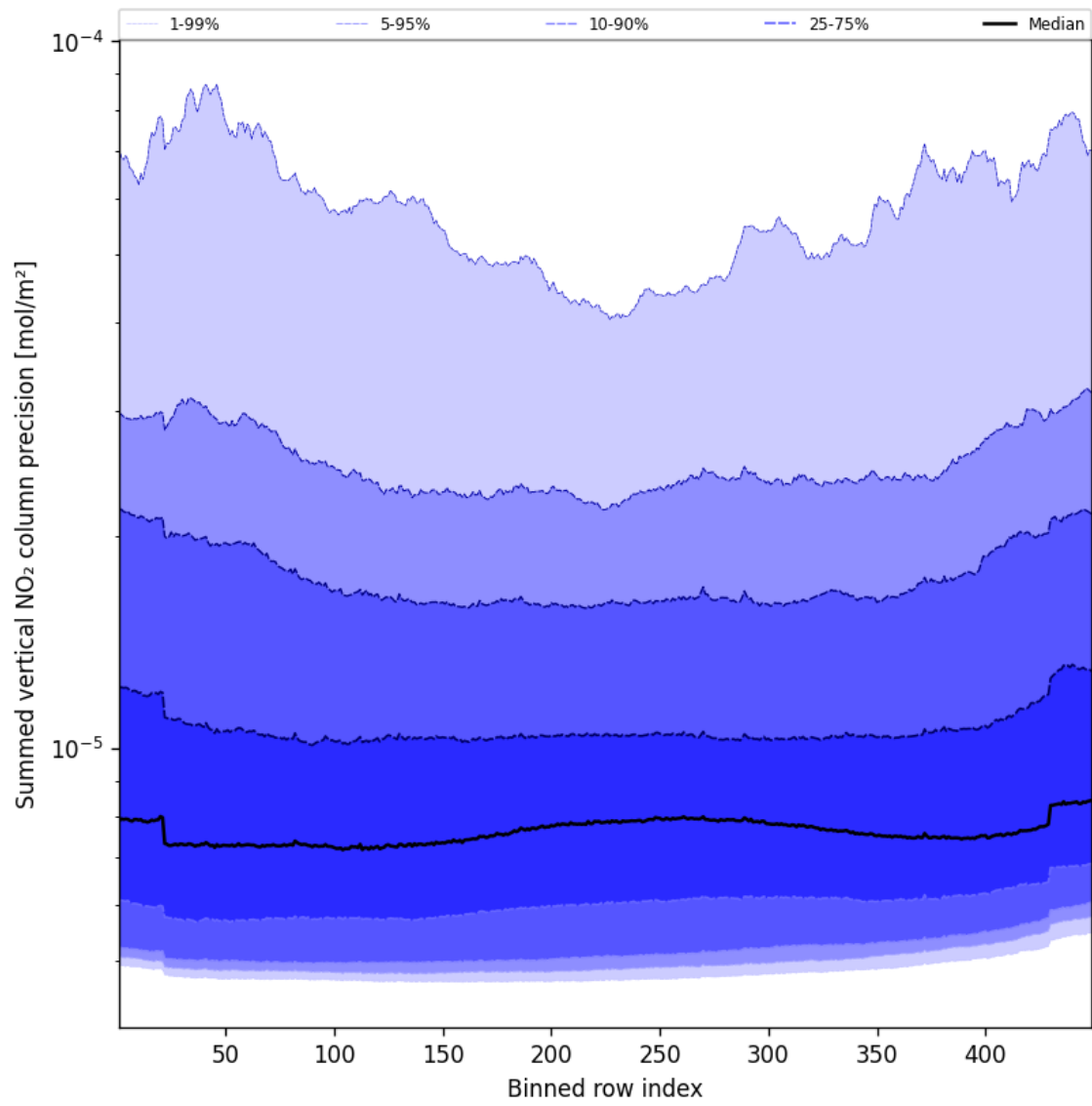
Figure 56: Along track statistics of “Summed vertical NO 2 column precision” for 2025-10-24 to 2025-10-25
