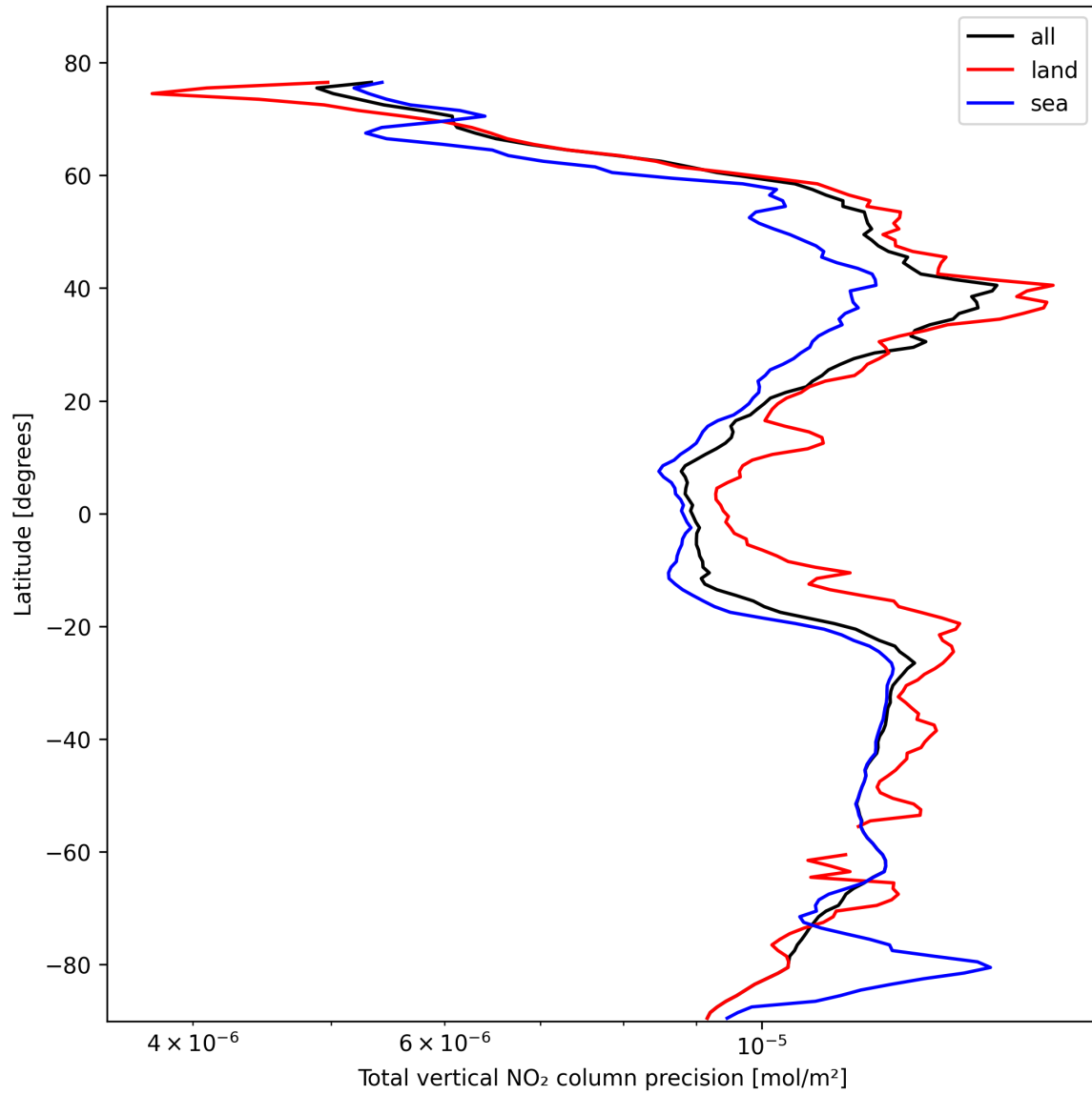
Figure 20: Zonal average of “Total vertical NO 2 column precision” for 2025-10-24 to 2025-10-25.
