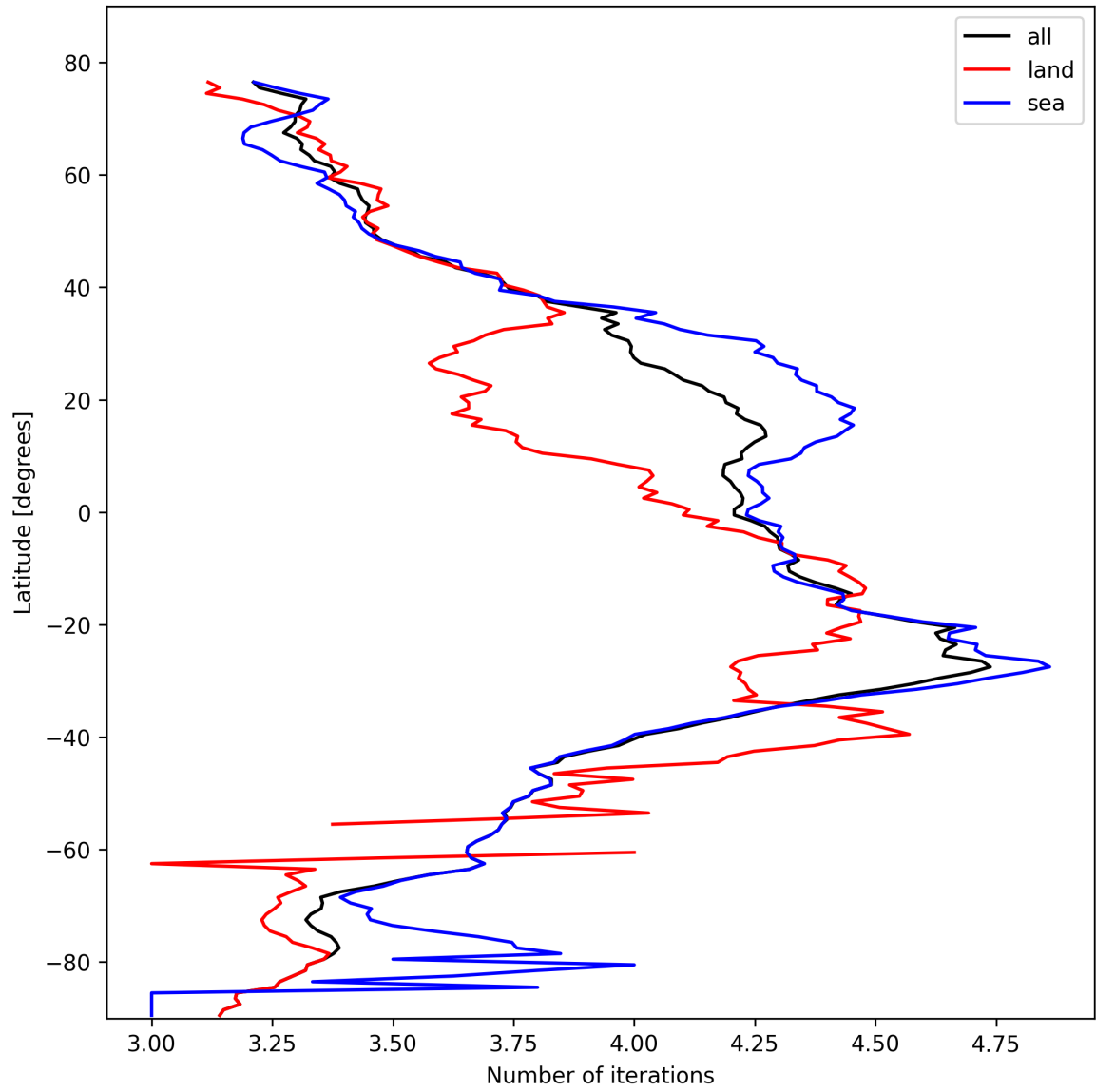
Figure 15: Zonal average of “Number of iterations” for 2025-10-24 to 2025-10-25.
