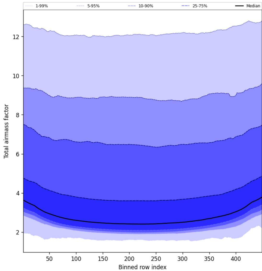
Figure 47: Along track statistics of “Total airmass factor” for 2025-10-24 to 2025-10-25
