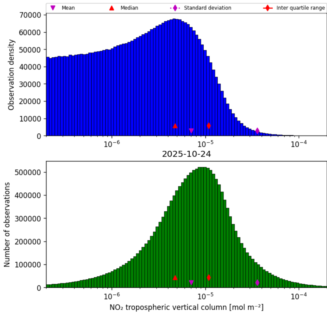
Figure 27: Histogram of “NO 2 tropospheric vertical column” for 2025-10-24 to 2025-10-25
