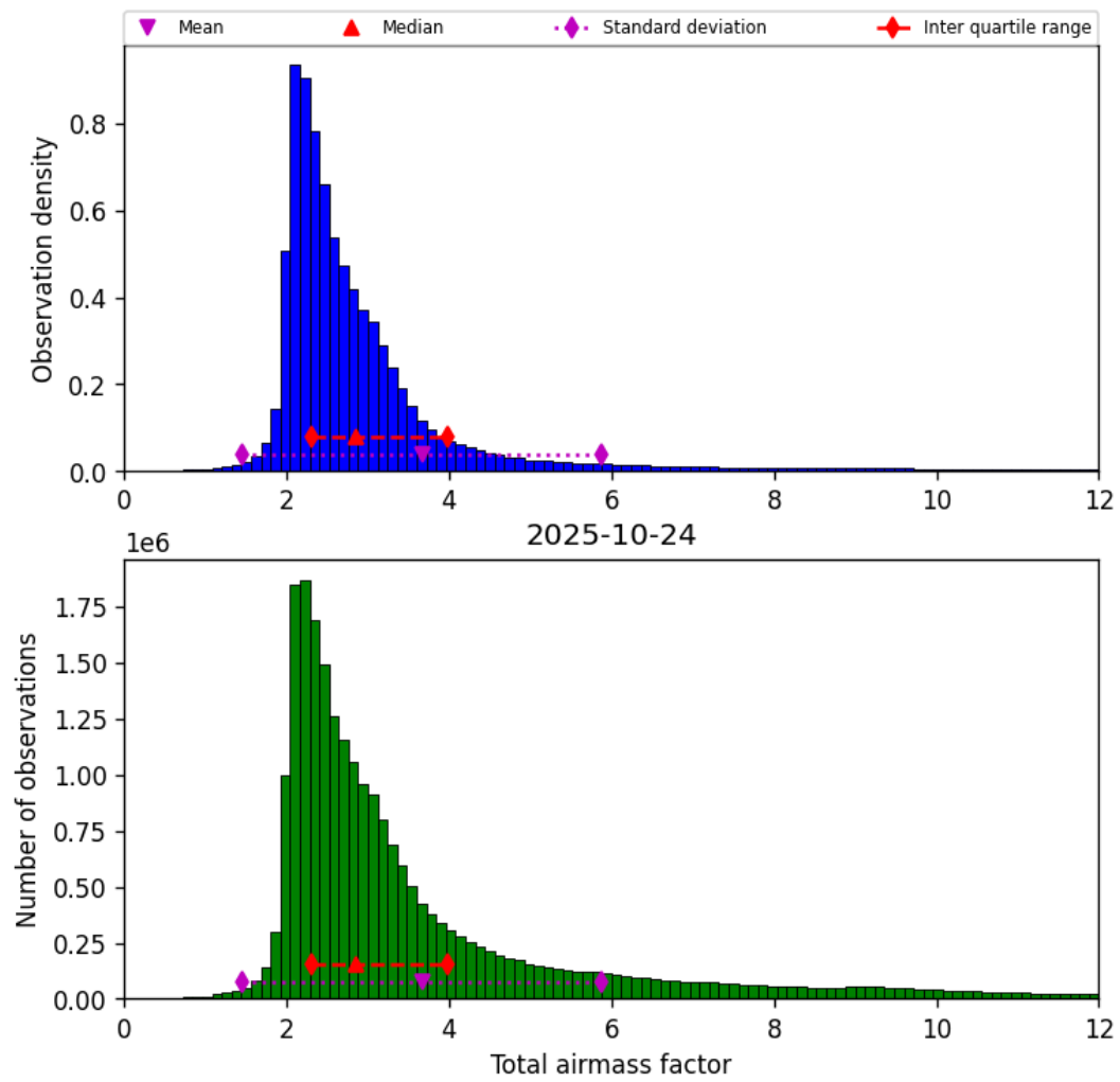
Figure 30: Histogram of “Total airmass factor” for 2025-10-24 to 2025-10-25
