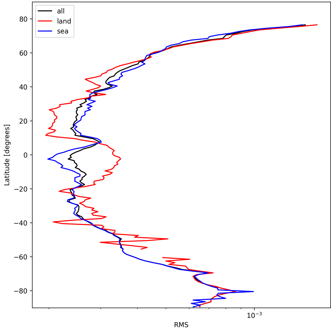
Figure 24: Zonal average of “RMS” for 2025-10-24 to 2025-10-25.
