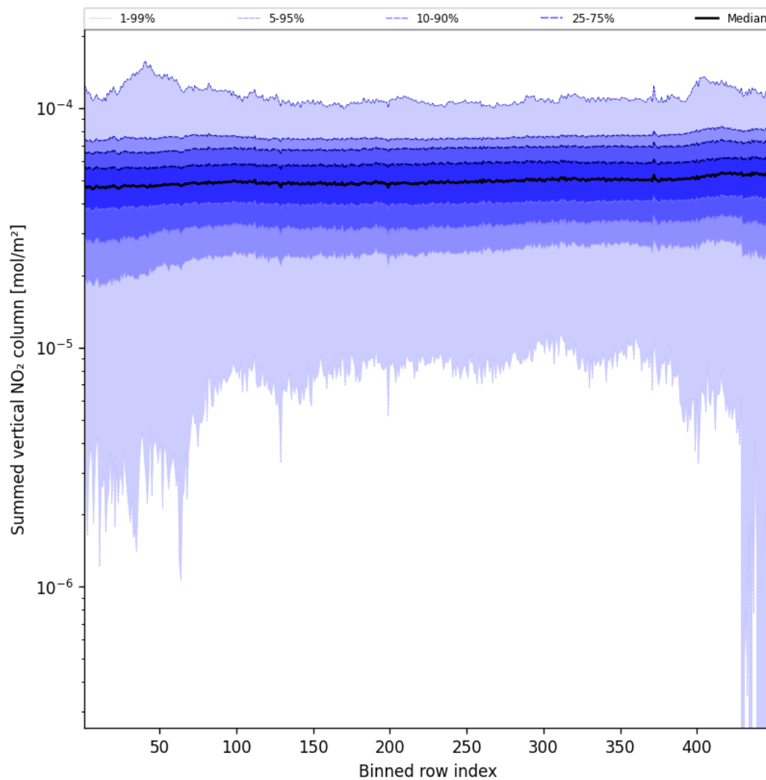
Figure 55: Along track statistics of “Summed vertical NO 2 column” for 2025-10-24 to 2025-10-25
