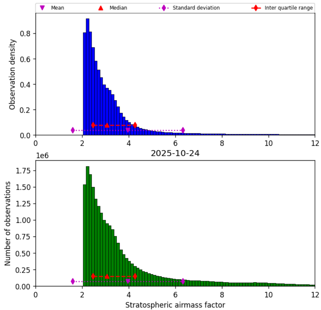
Figure 42: Histogram of “Stratospheric airmass factor” for 2025-10-24 to 2025-10-25
