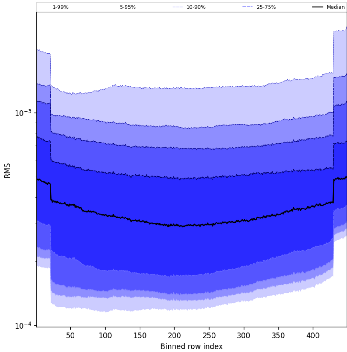
Figure 58: Along track statistics of “RMS” for 2025-10-24 to 2025-10-25
