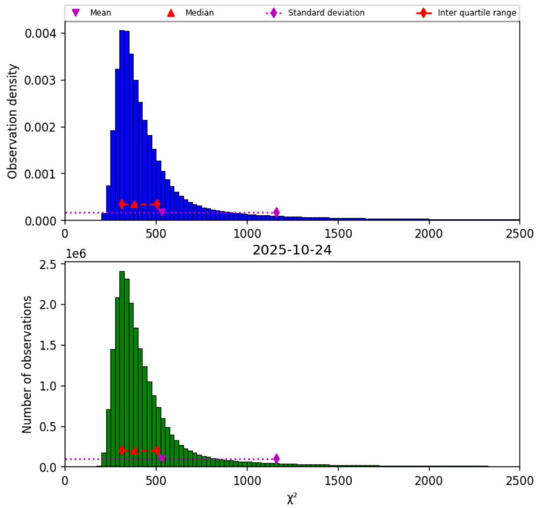
Figure 40: Histogram of “ \chi^2 ” for 2025-10-24 to 2025-10-25
