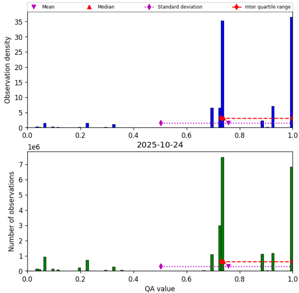
Figure 26: Histogram of “QA value” for 2025-10-24 to 2025-10-25
