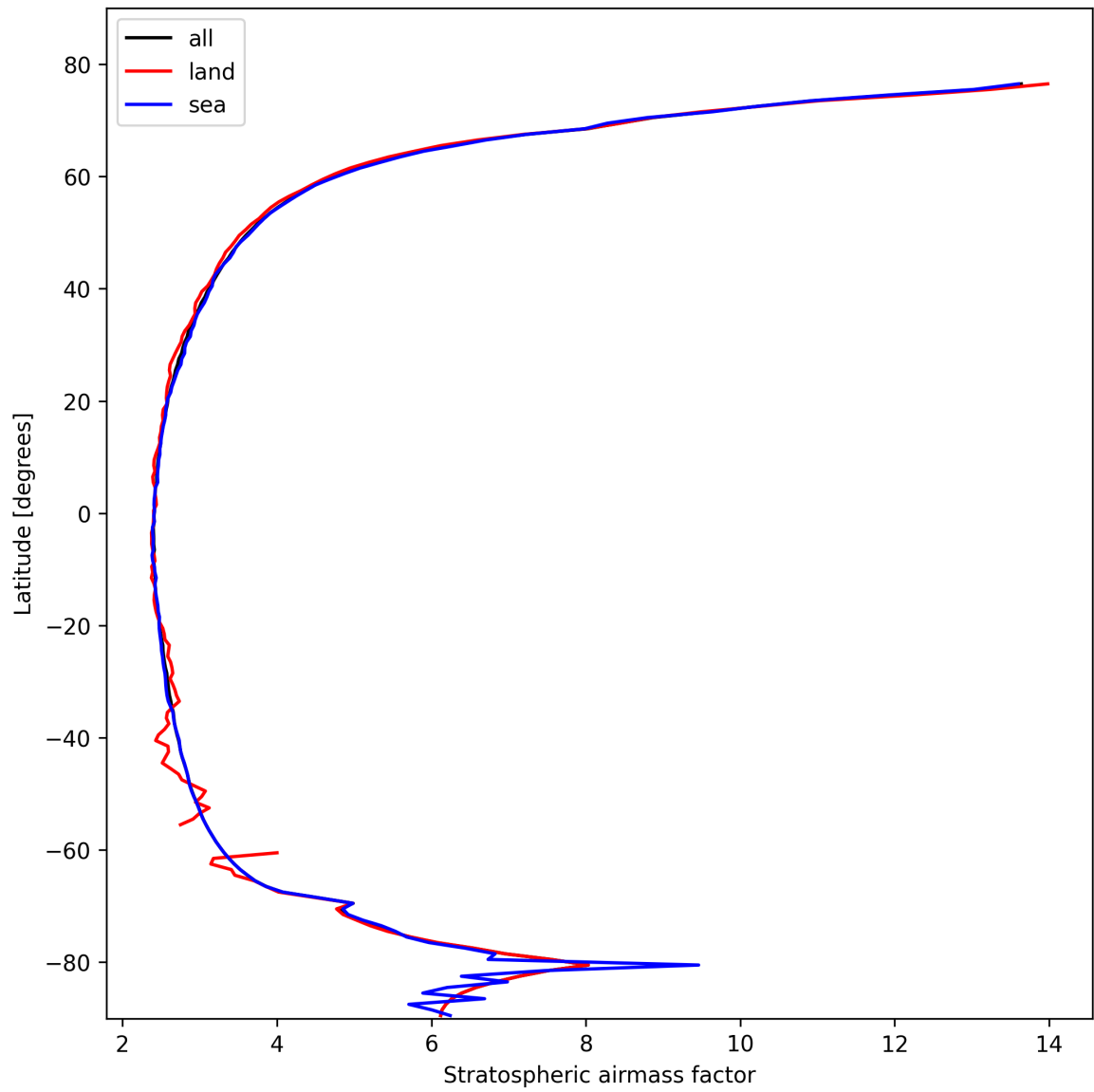
Figure 25: Zonal average of “Stratospheric airmass factor” for 2025-10-24 to 2025-10-25.
