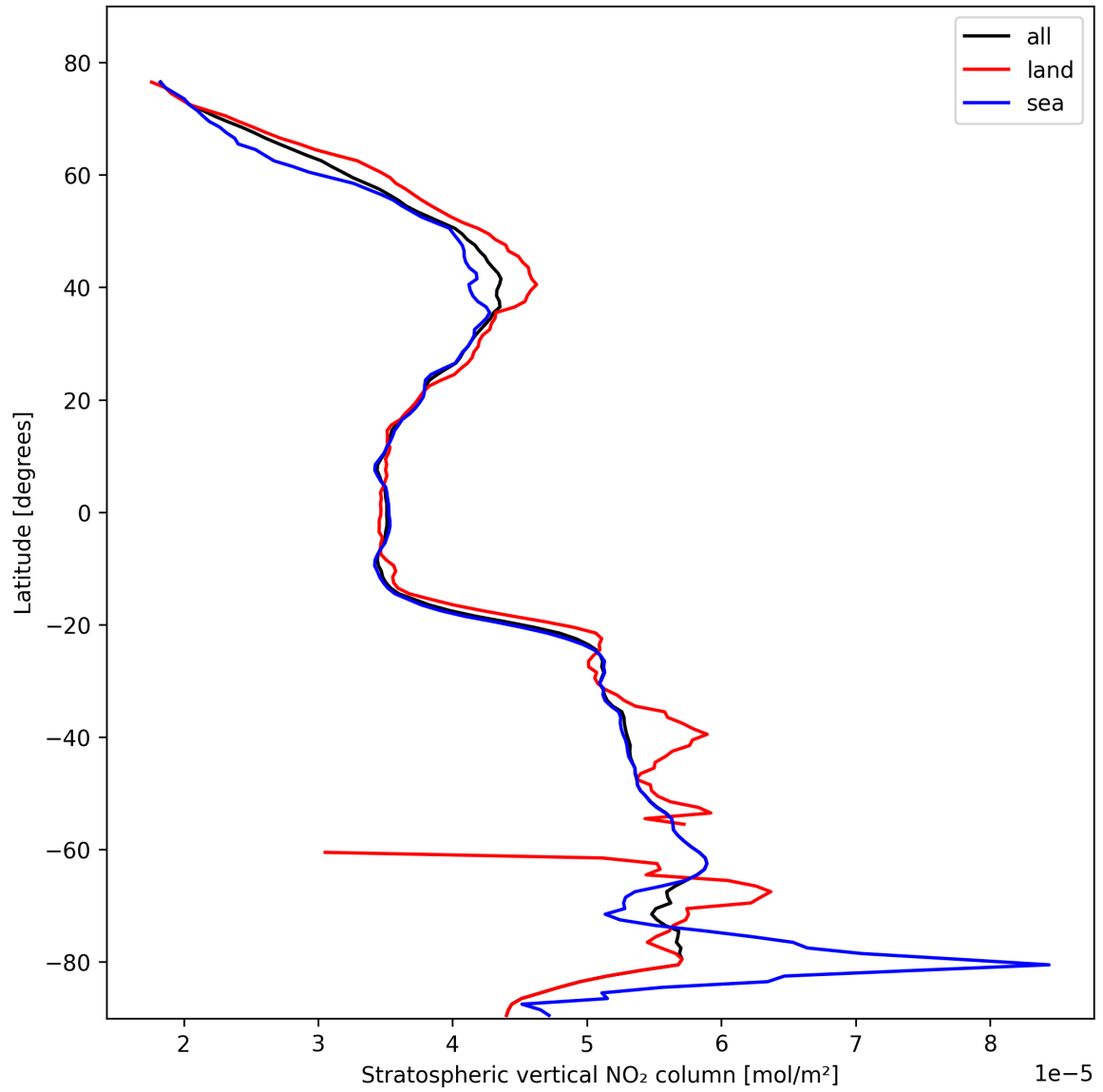
Figure 17: Zonal average of “Stratospheric vertical NO 2 column” for 2025-10-24 to 2025-10-25.
