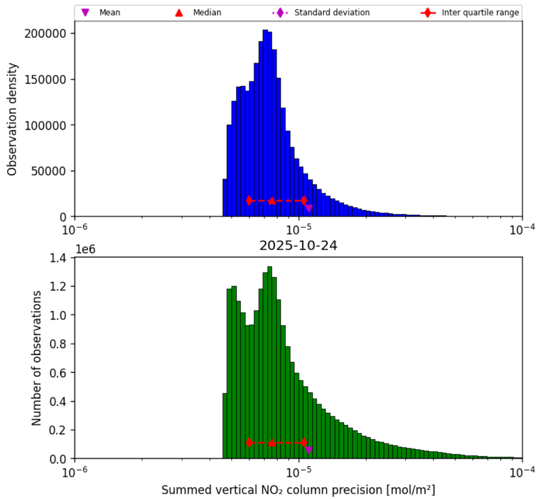
Figure 39: Histogram of “Summed vertical NO 2 column precision” for 2025-10-24 to 2025-10-25
