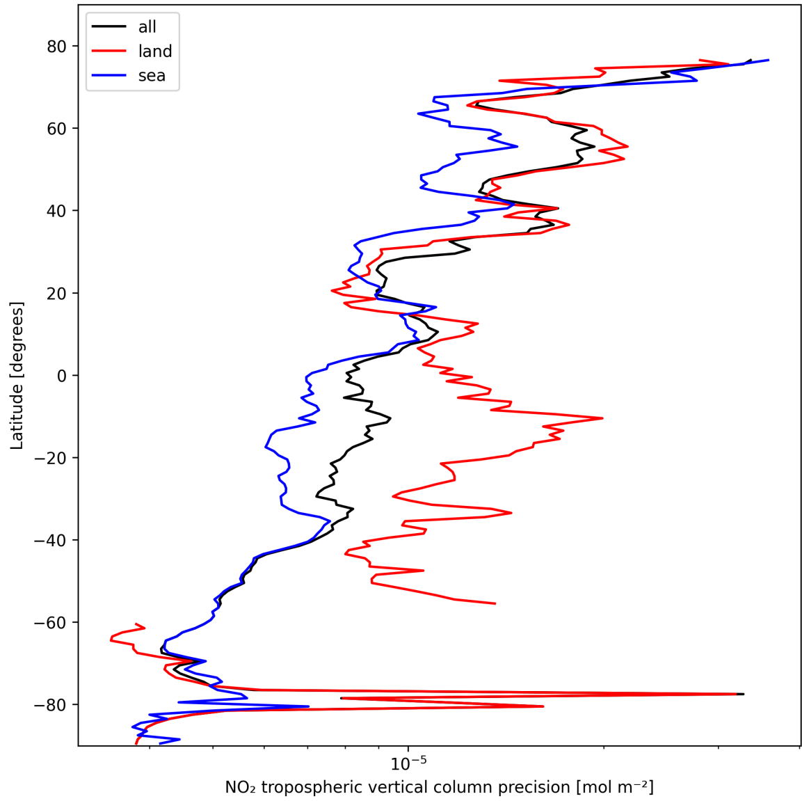
Figure 11: Zonal average of “NO 2 tropospheric vertical column precision” for 2025-10-24 to 2025-10-25.
