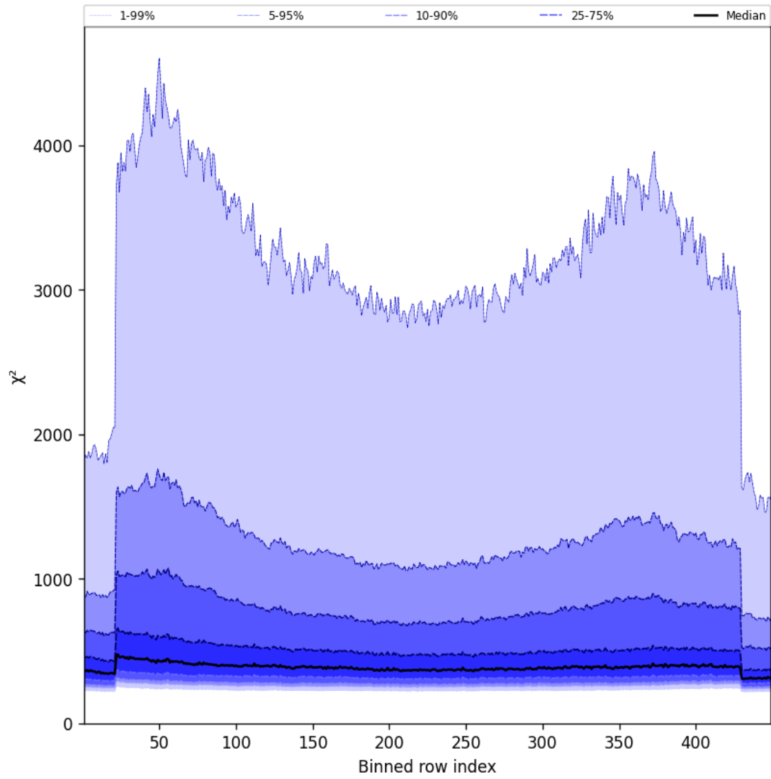
Figure 57: Along track statistics of “ \chi^2 ” for 2025-10-24 to 2025-10-25
