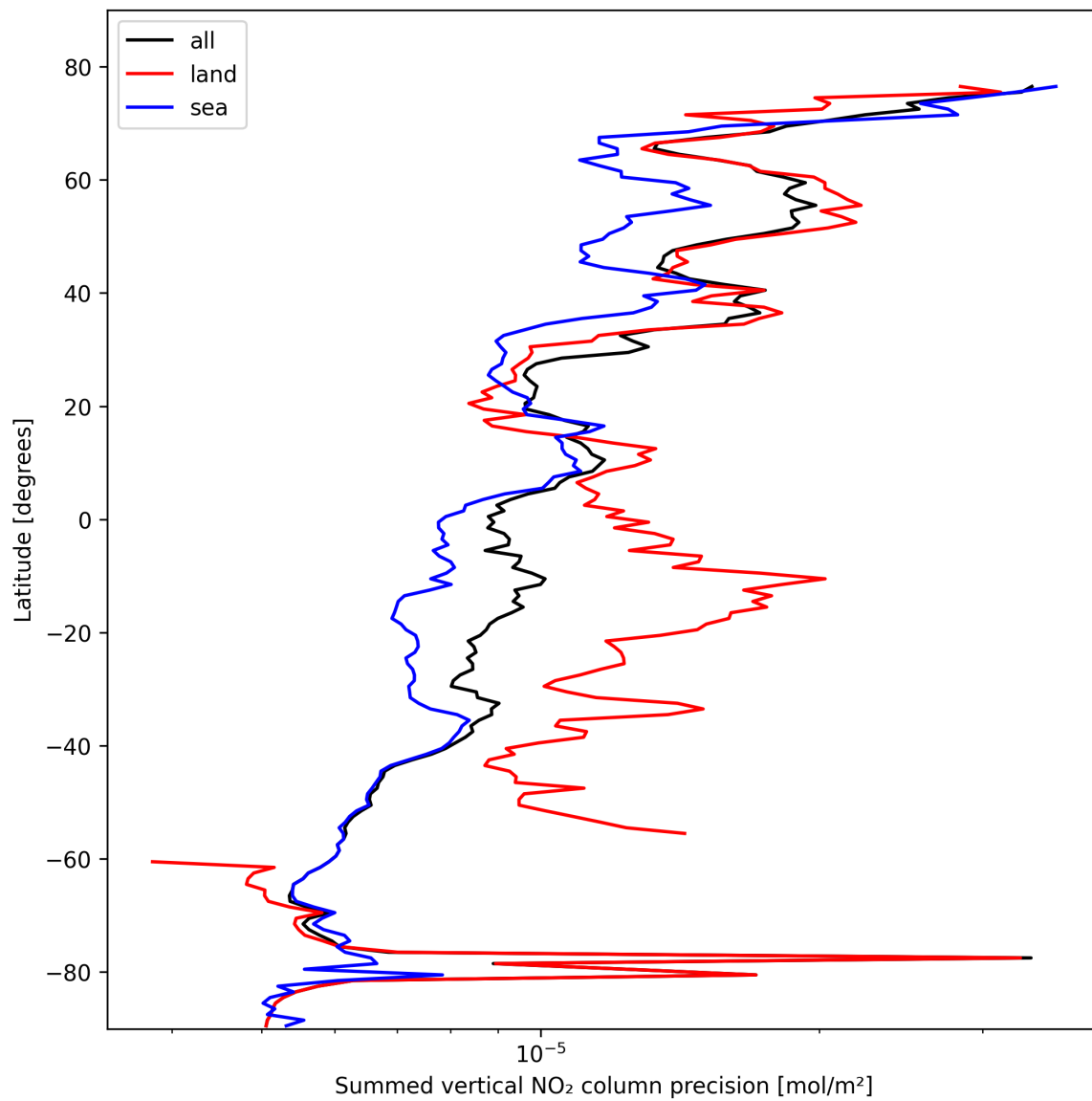
Figure 22: Zonal average of “Summed vertical NO 2 column precision” for 2025-10-24 to 2025-10-25.
