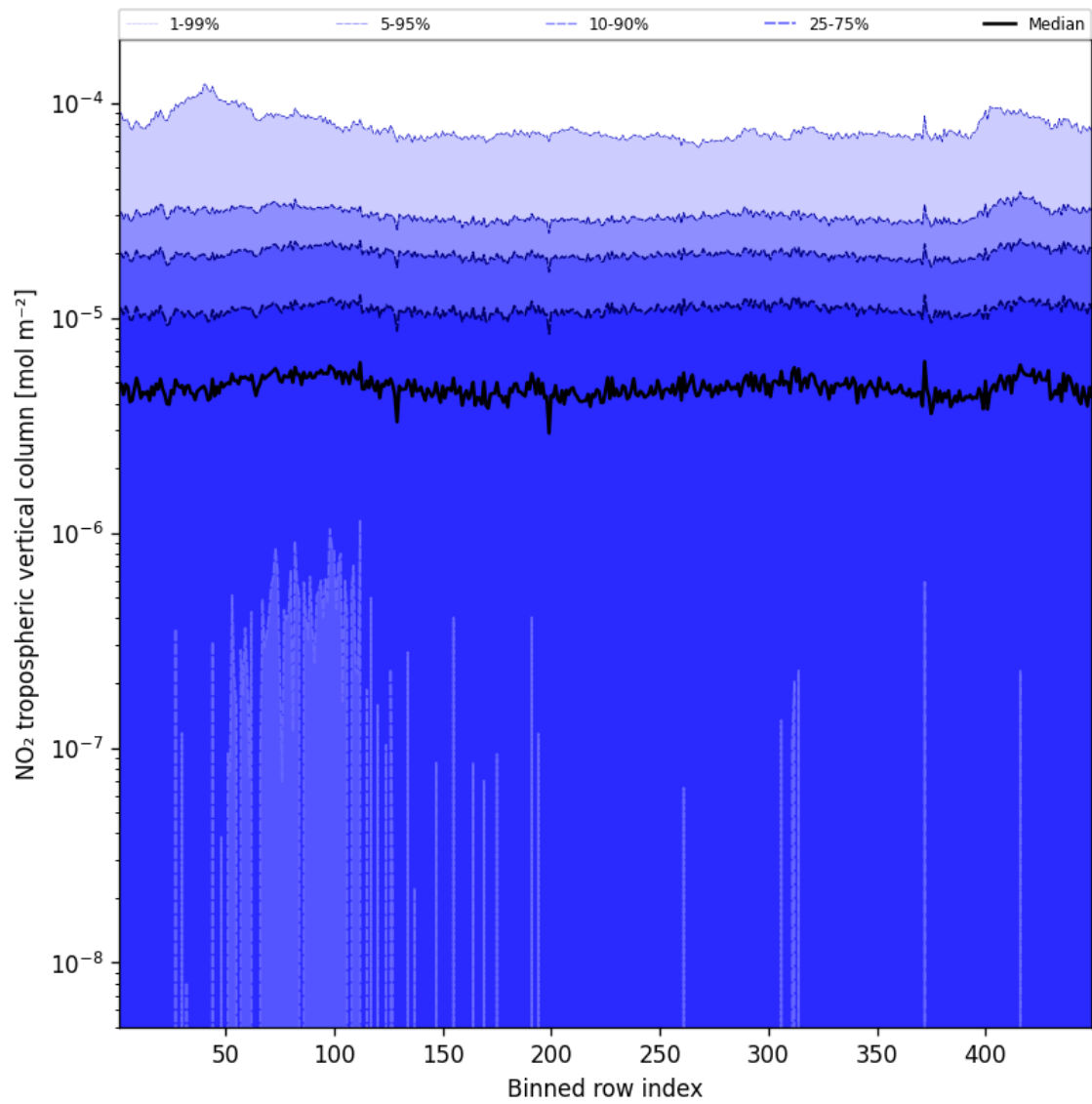
Figure 44: Along track statistics of “NO 2 tropospheric vertical column” for 2025-10-24 to 2025-10-25
