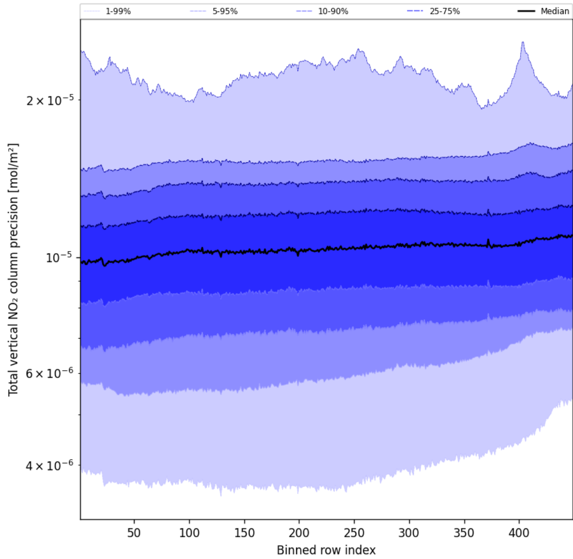
Figure 54: Along track statistics of "Total vertical NO 2 column precision" for 2025-10-24 to 2025-10-25
