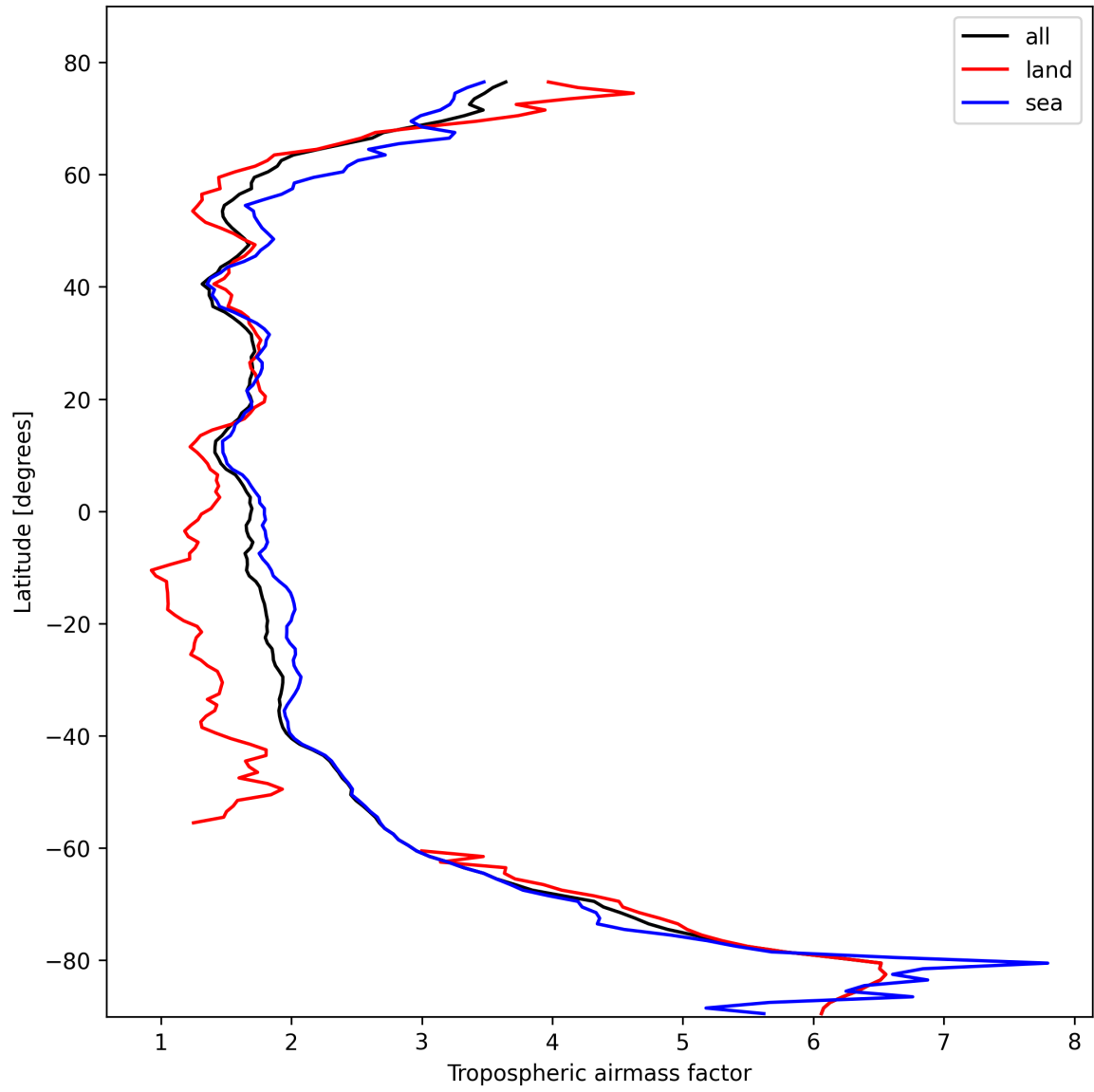
Figure 12: Zonal average of “Tropospheric airmass factor” for 2025-10-24 to 2025-10-25.
