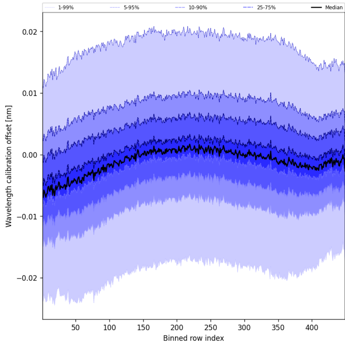
Figure 50: Along track statistics of “Wavelength calibration offset” for 2025-10-24 to 2025-10-25
