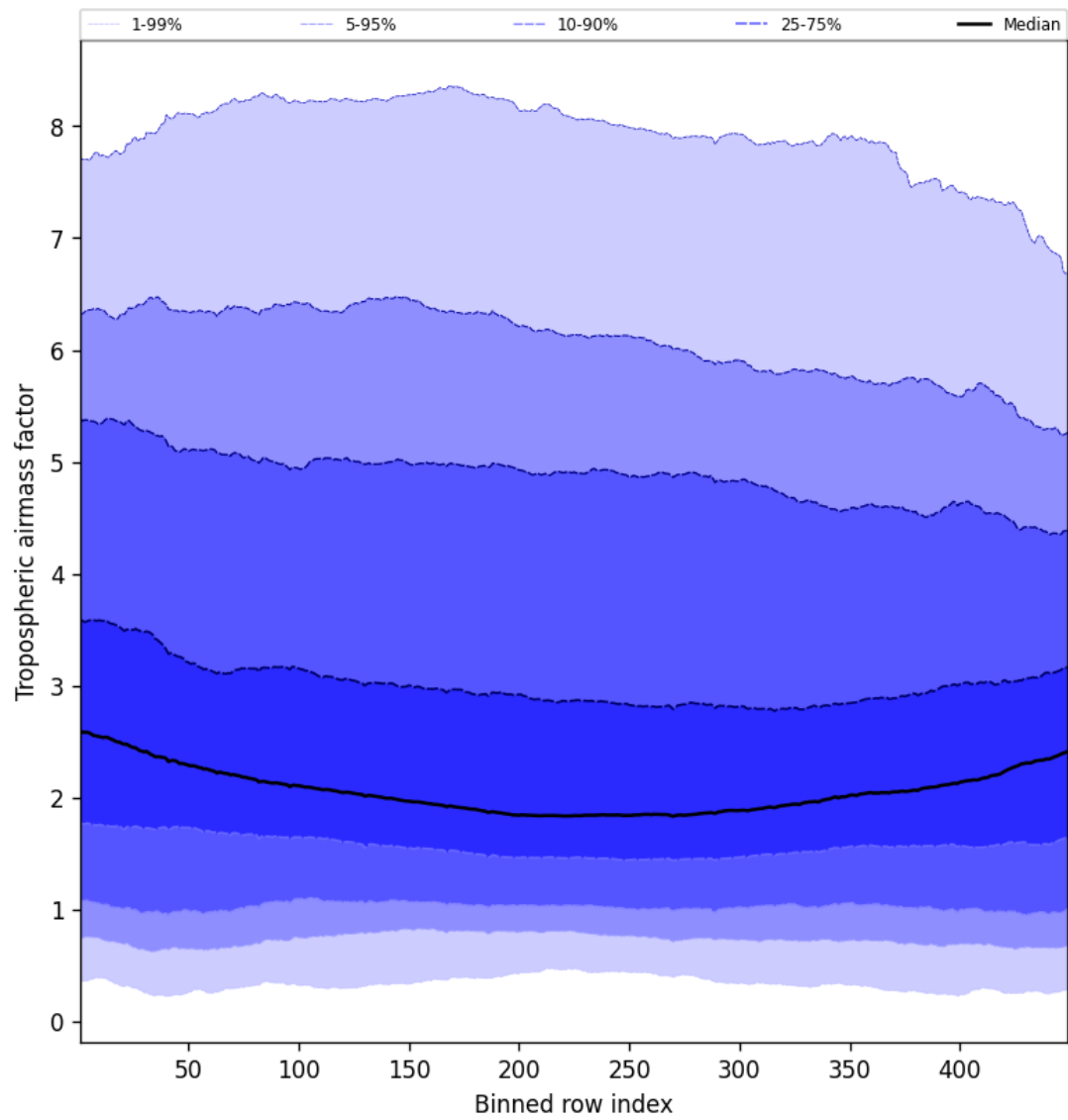
Figure 46: Along track statistics of “Tropospheric air mass factor” for 2025-10-24 to 2025-10-25
