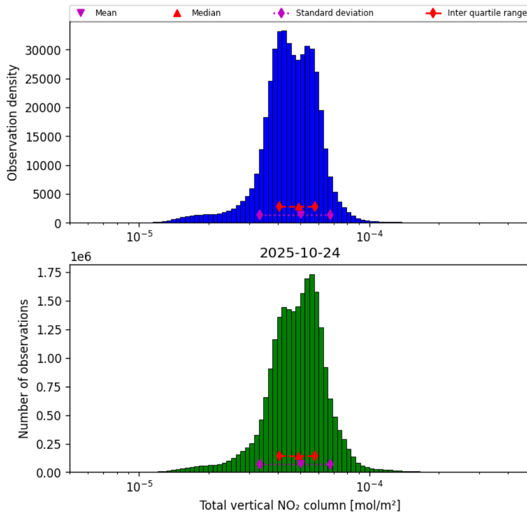
Figure 36: Histogram of “Total vertical NO 2 column” for 2025-10-24 to 2025-10-25
