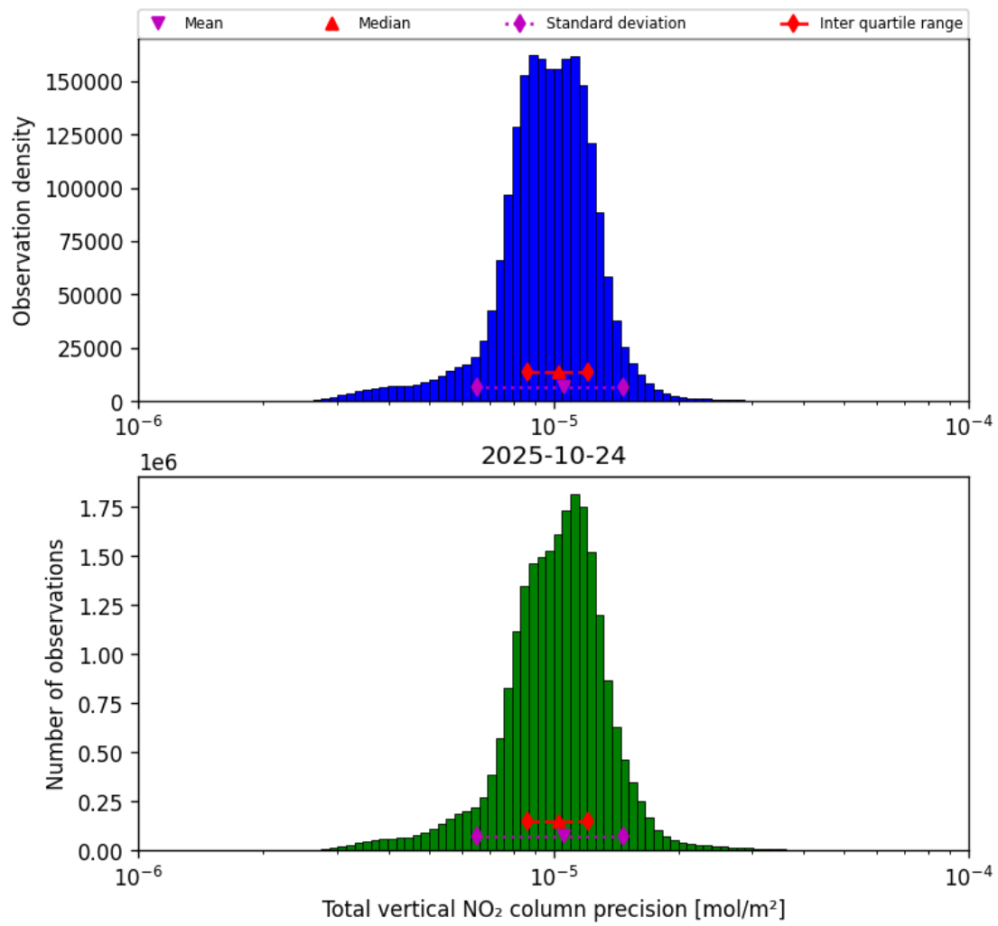
Figure 37: Histogram of “Total vertical NO 2 column precision” for 2025-10-24 to 2025-10-25
