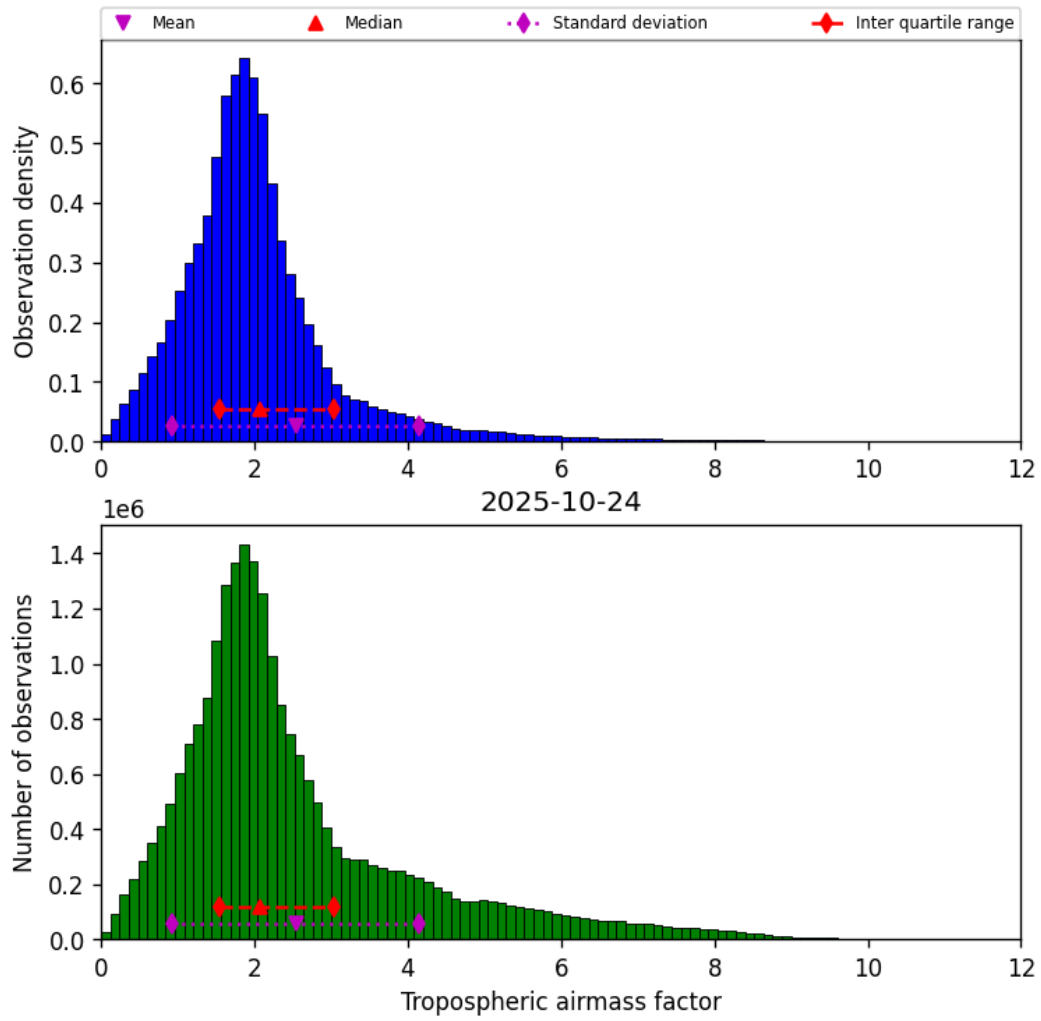
Figure 29: Histogram of “Tropospheric airmass factor” for 2025-10-24 to 2025-10-25
