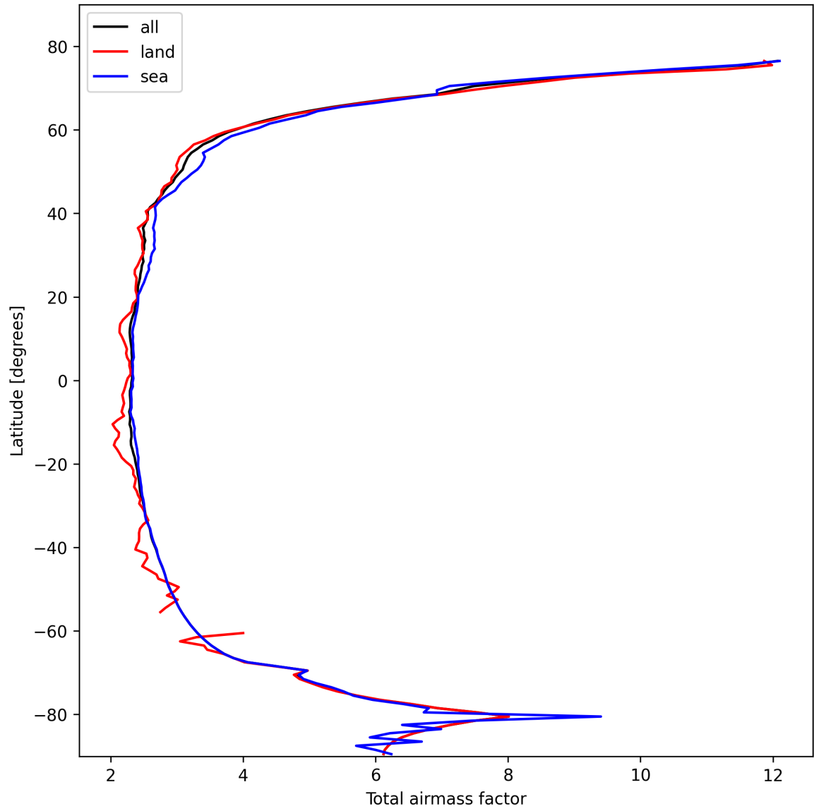
Figure 13: Zonal average of “Total airmass factor” for 2025-10-24 to 2025-10-25.
