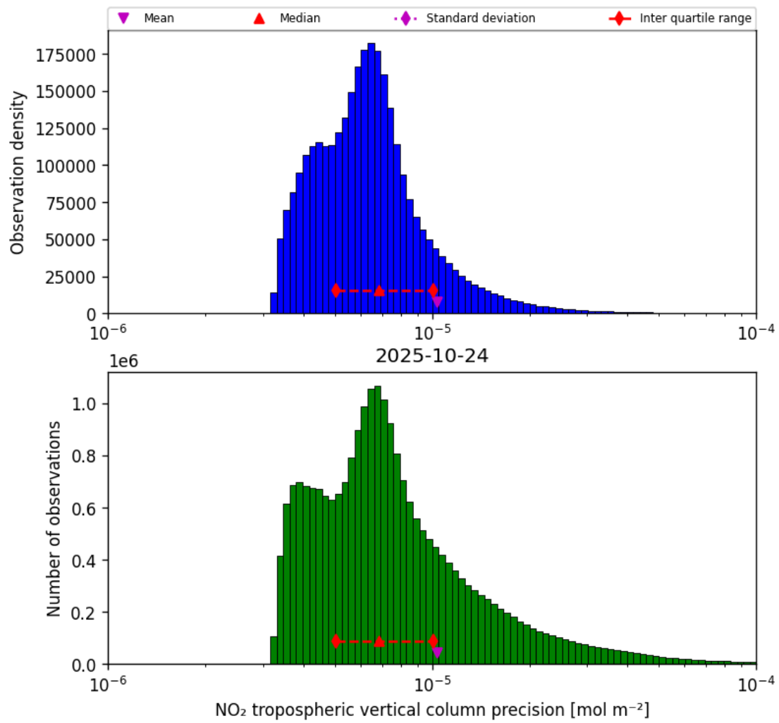
Figure 28: Histogram of “NO 2 tropospheric vertical column precision” for 2025-10-24 to 2025-10-25
