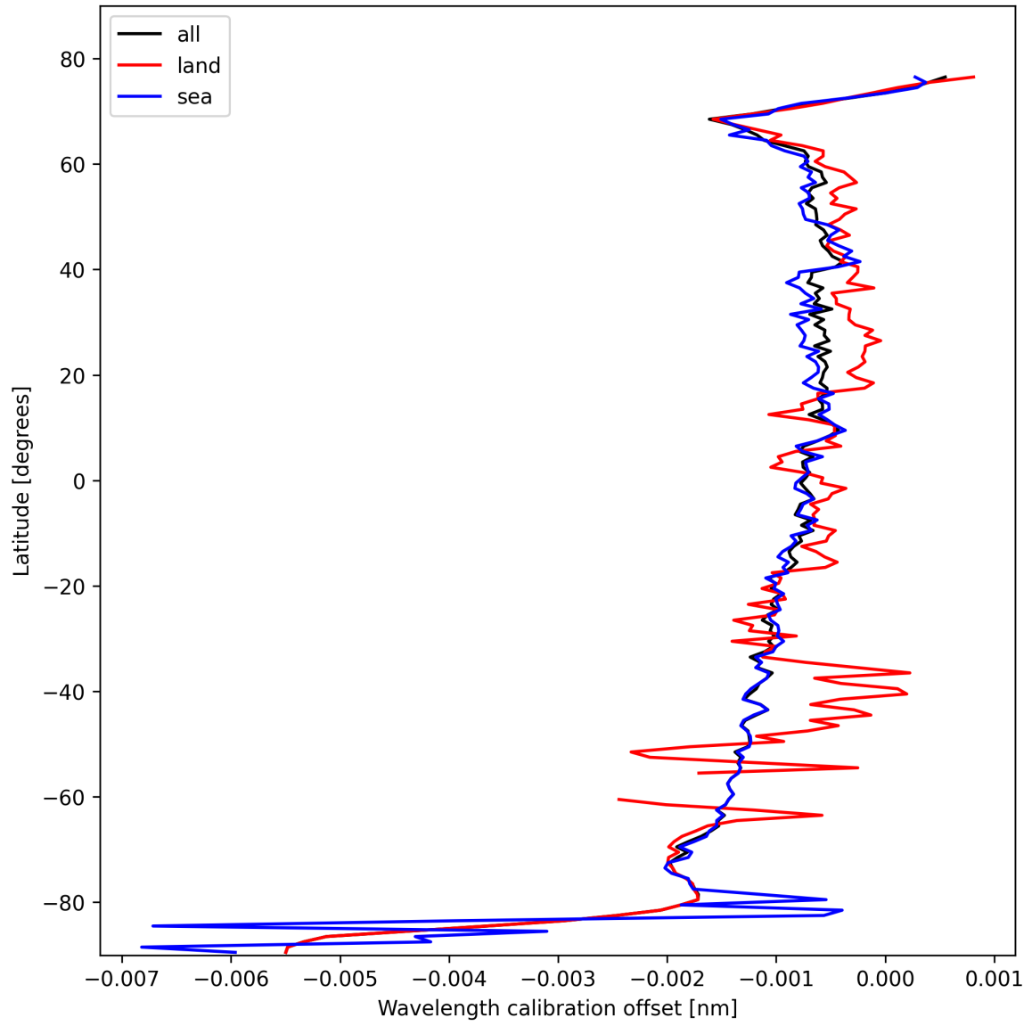
Figure 16: Zonal average of “Wavelength calibration offset” for 2025-10-24 to 2025-10-25.
