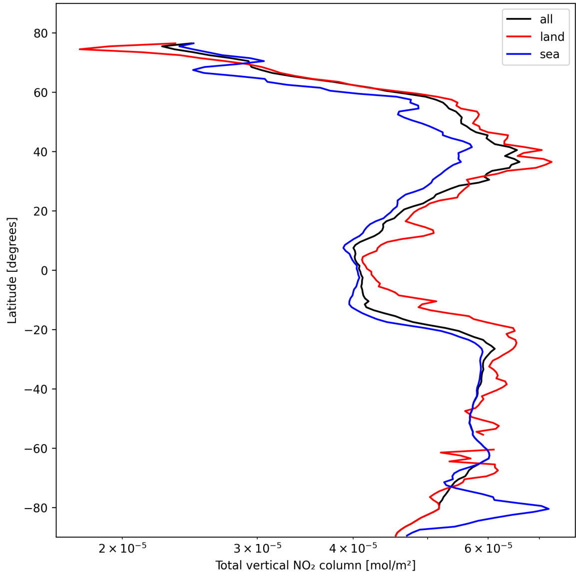
Figure 19: Zonal average of “Total vertical NO 2 column” for 2025-10-24 to 2025-10-25.
