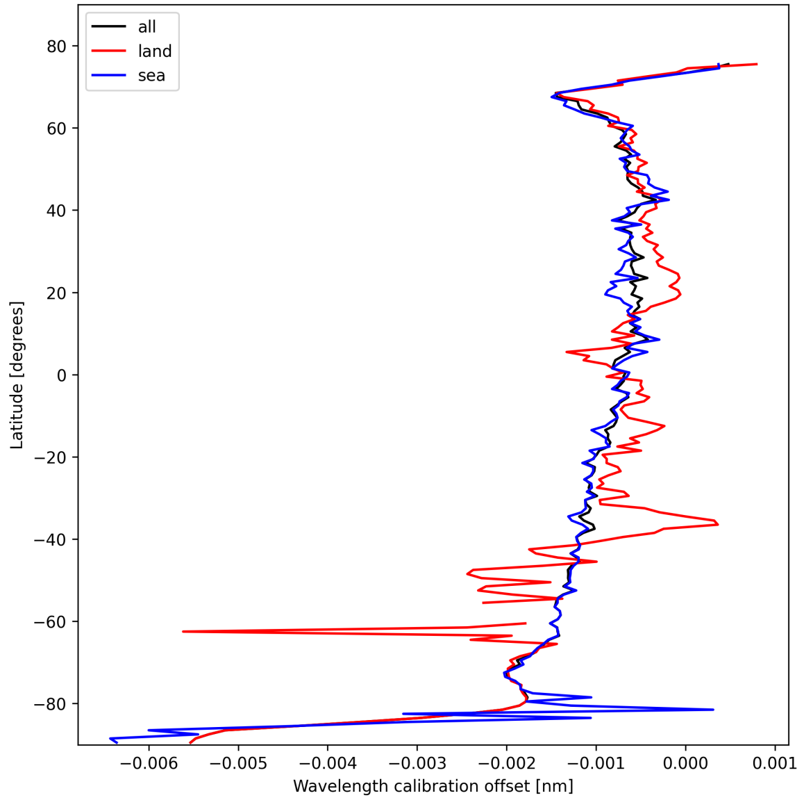
Figure 16: Zonal average of “Wavelength calibration offset” for 2025-10-25 to 2025-10-25.
