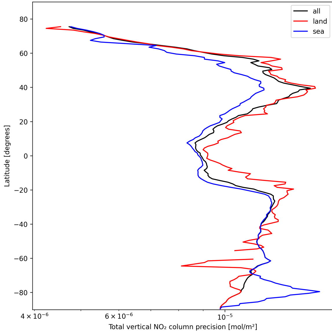
Figure 20: Zonal average of “Total vertical NO 2 column precision” for 2025-10-25 to 2025-10-25.
