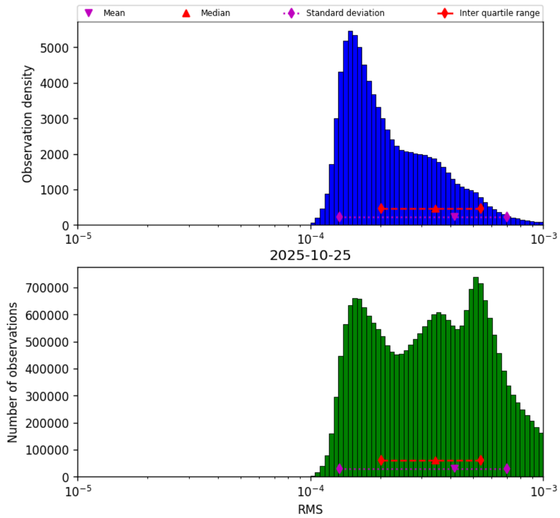
Figure 41: Histogram of “RMS” for 2025-10-25 to 2025-10-25
