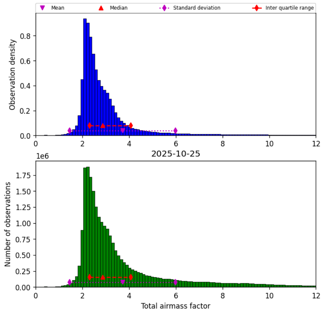
Figure 30: Histogram of “Total airmass factor” for 2025-10-25 to 2025-10-25
