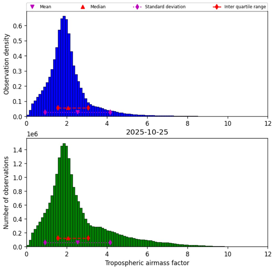
Figure 29: Histogram of “Tropospheric airmass factor” for 2025-10-25 to 2025-10-25
