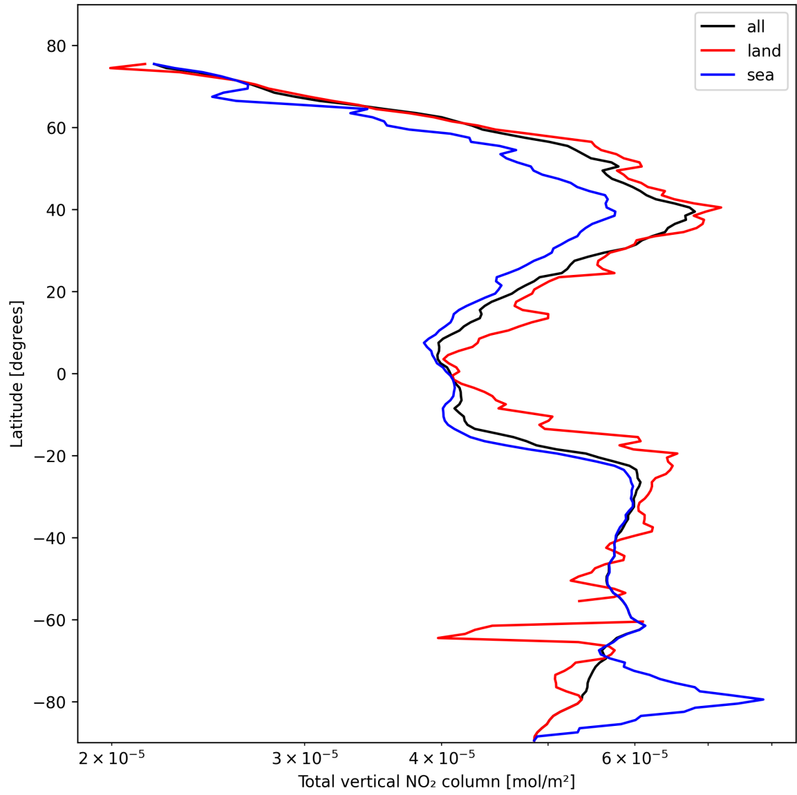
Figure 19: Zonal average of “Total vertical NO 2 column” for 2025-10-25 to 2025-10-25.
