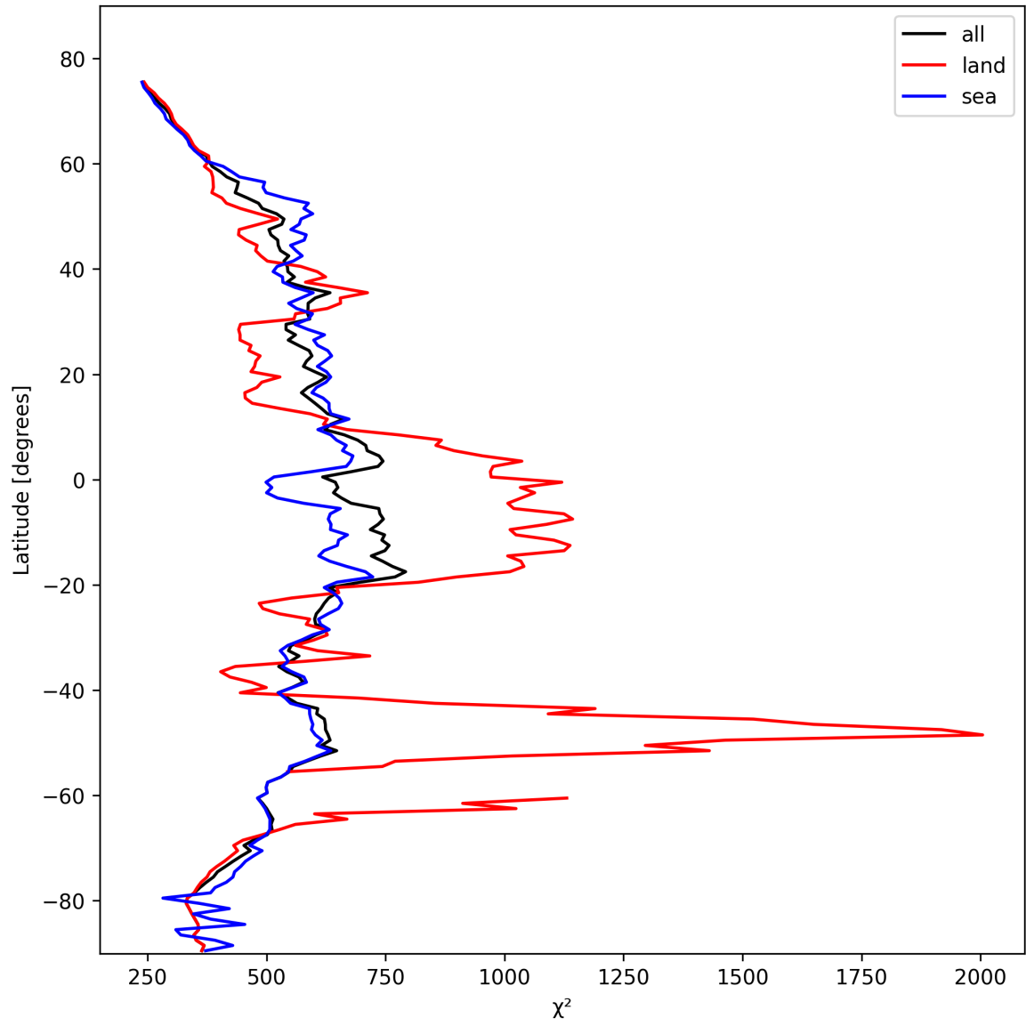
Figure 23: Zonal average of “ \chi^2 ” for 2025-10-25 to 2025-10-25.
