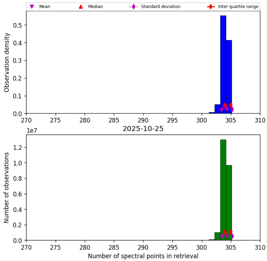
Figure 31: Histogram of “Number of spectral points in retrieval” for 2025-10-25 to 2025-10-25
