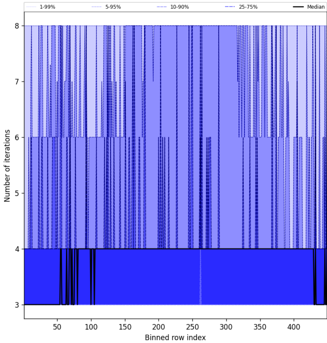
Figure 49: Along track statistics of “Number of iterations” for 2025-10-25 to 2025-10-25
