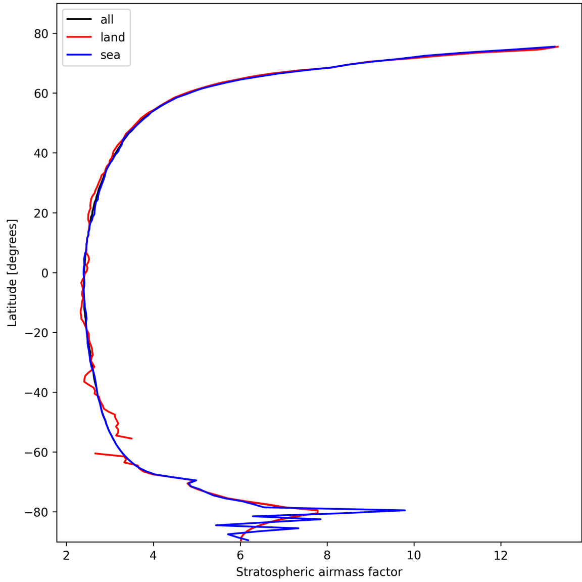
Figure 25: Zonal average of “Stratospheric air mass factor” for 2025-10-25 to 2025-10-25.
