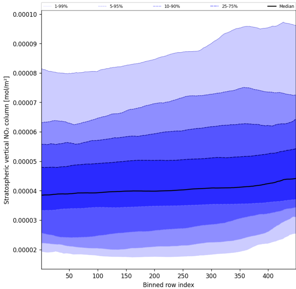
Figure 51: Along track statistics of “Stratospheric vertical NO 2 column” for 2025-10-25 to 2025-10-25
