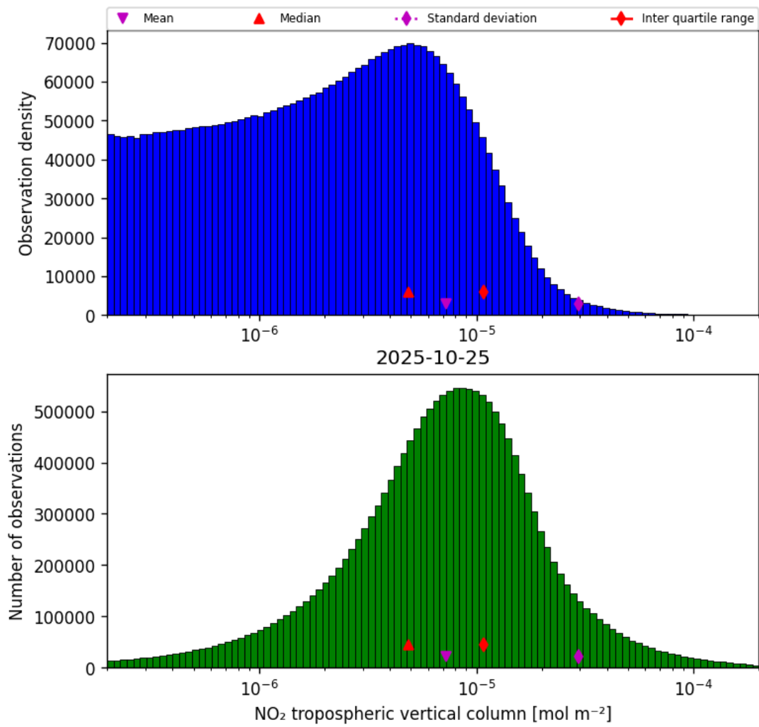
Figure 27: Histogram of “ \text{NO}_2 tropospheric vertical column” for 2025-10-25 to 2025-10-25
