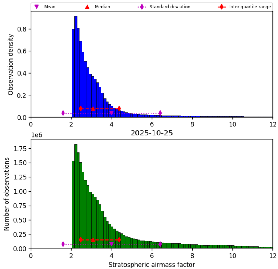
Figure 42: Histogram of “Stratospheric airmass factor” for 2025-10-25 to 2025-10-25
