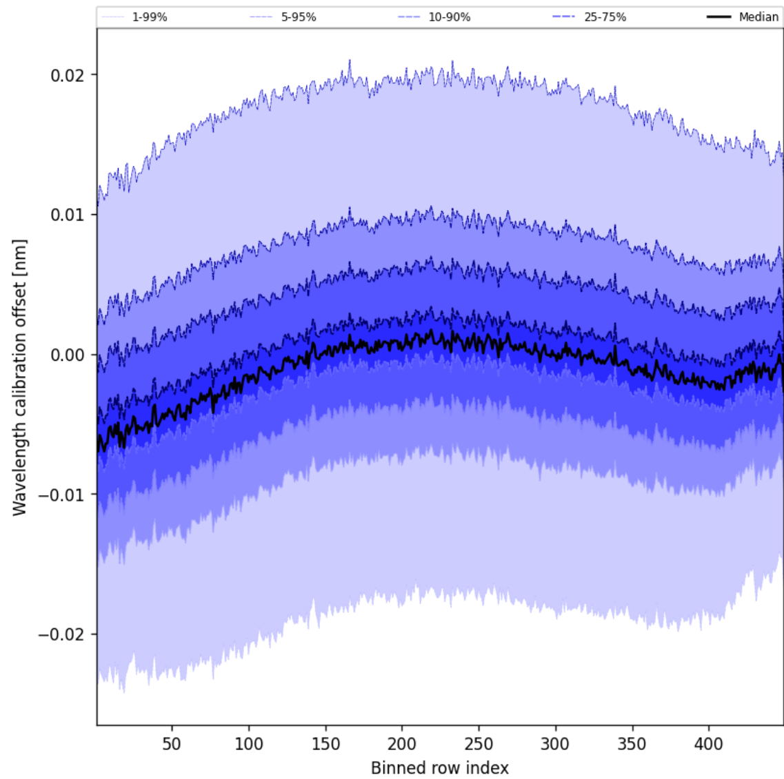
Figure 50: Along track statistics of “Wavelength calibration offset” for 2025-10-25 to 2025-10-25
