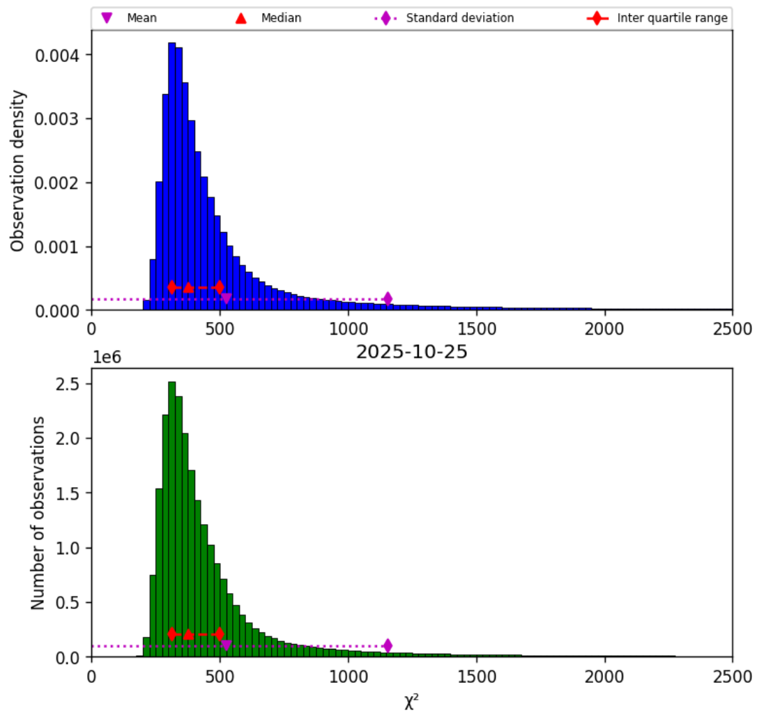
Figure 40: Histogram of “ \chi^2 ” for 2025-10-25 to 2025-10-25
