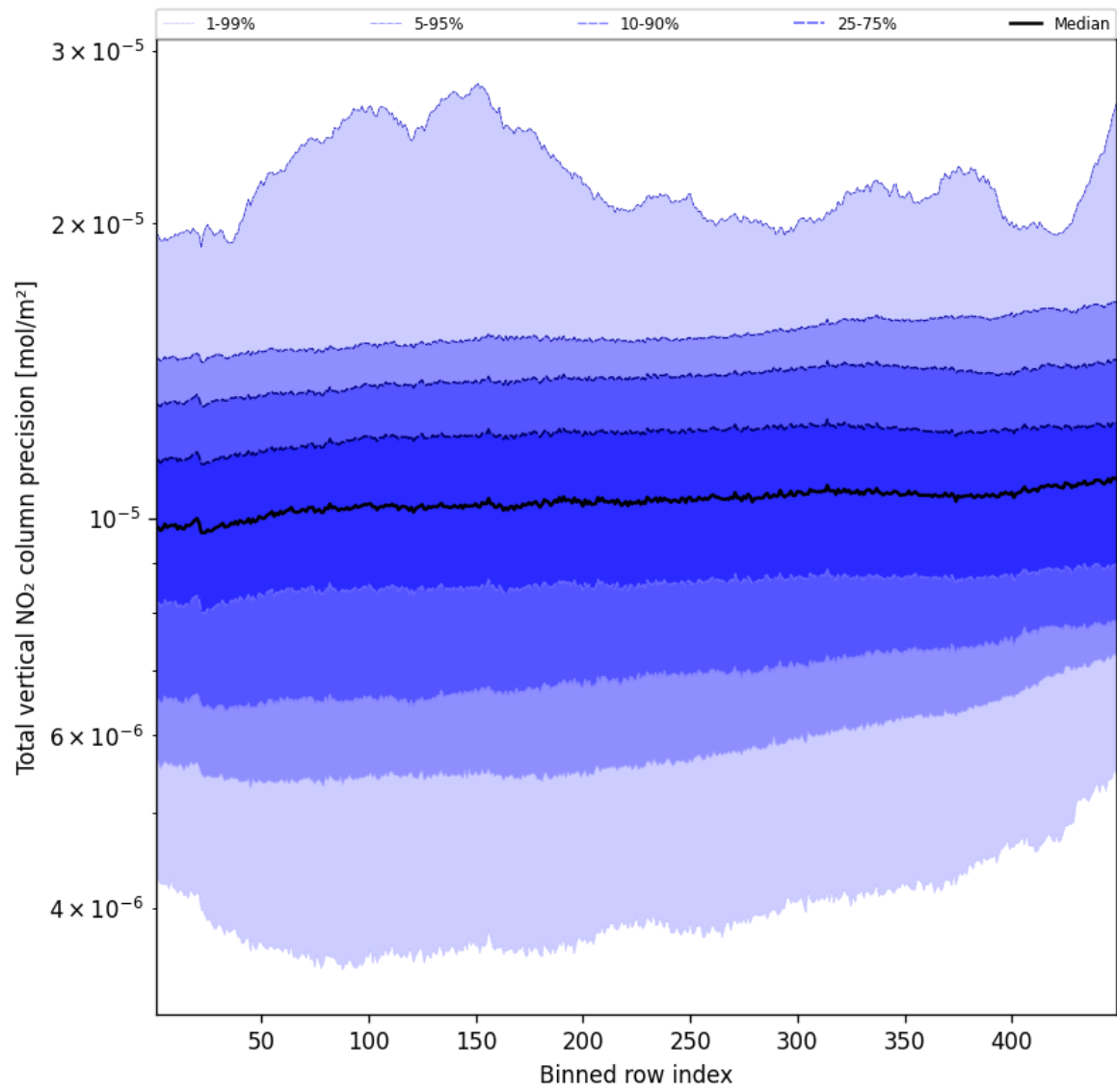
Figure 54: Along track statistics of “Total vertical NO 2 column precision” for 2025-10-25 to 2025-10-25
