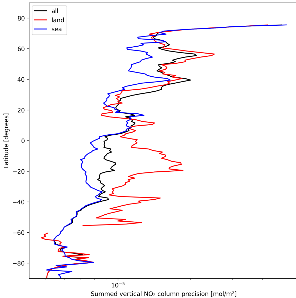
Figure 22: Zonal average of “Summed vertical NO 2 column precision” for 2025-10-25 to 2025-10-25.
