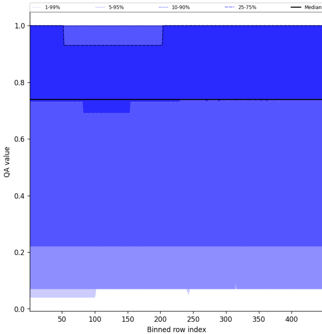
Figure 43: Along track statistics of “QA value” for 2025-10-25 to 2025-10-25
