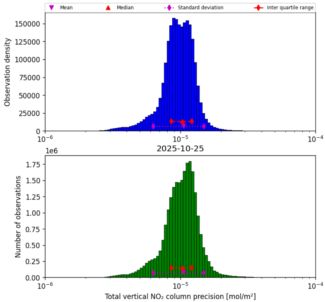
Figure 37: Histogram of “Total vertical NO 2 column precision” for 2025-10-25 to 2025-10-25
