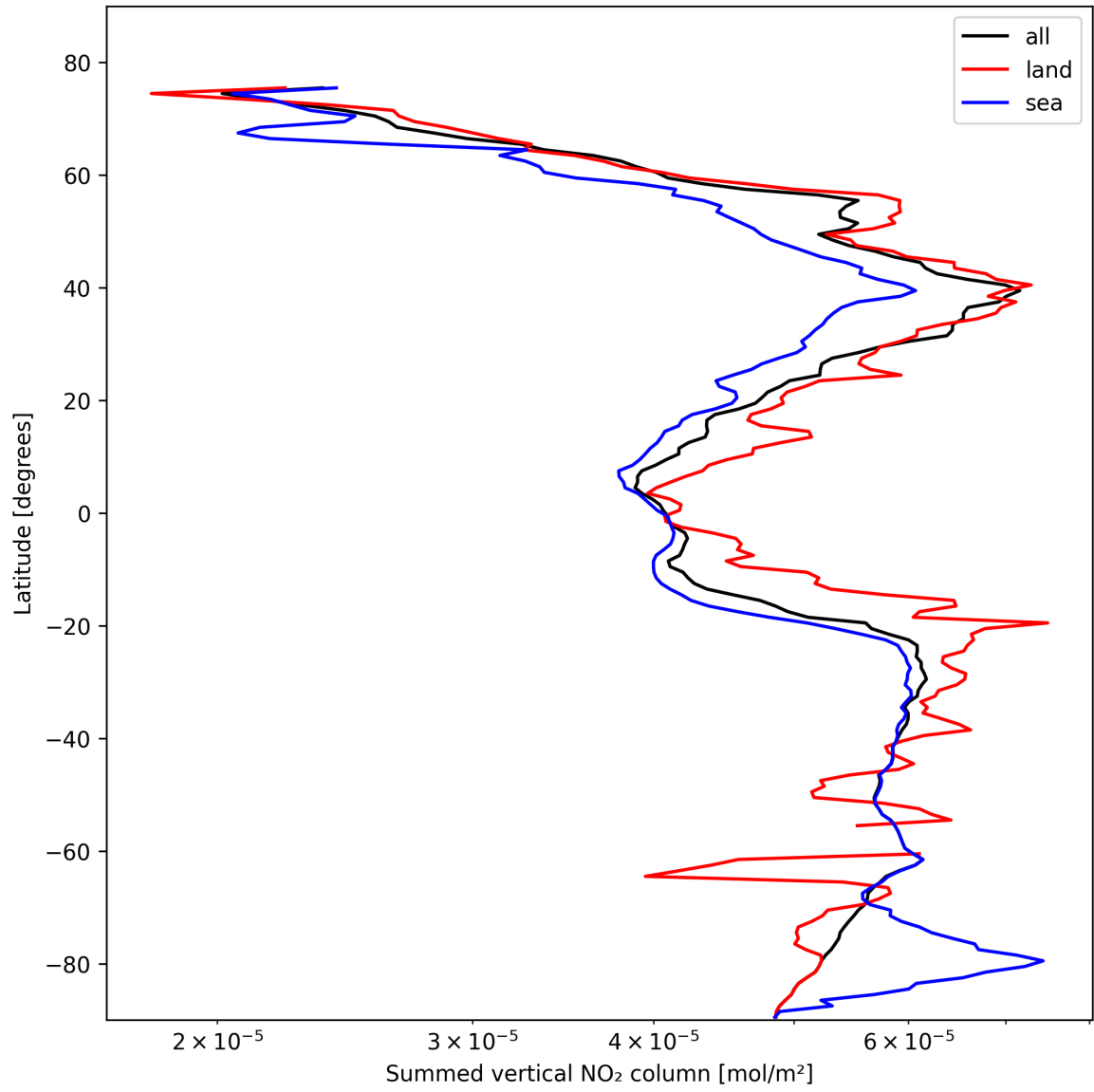
Figure 21: Zonal average of “Summed vertical NO 2 column” for 2025-10-25 to 2025-10-25.
