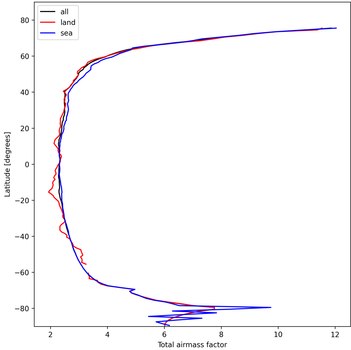
Figure 13: Zonal average of “Total airmass factor” for 2025-10-25 to 2025-10-25.
