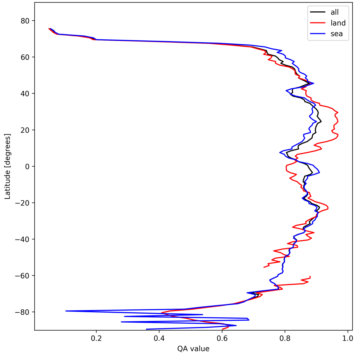
Figure 9: Zonal average of “QA value” for 2025-10-25 to 2025-10-25.
