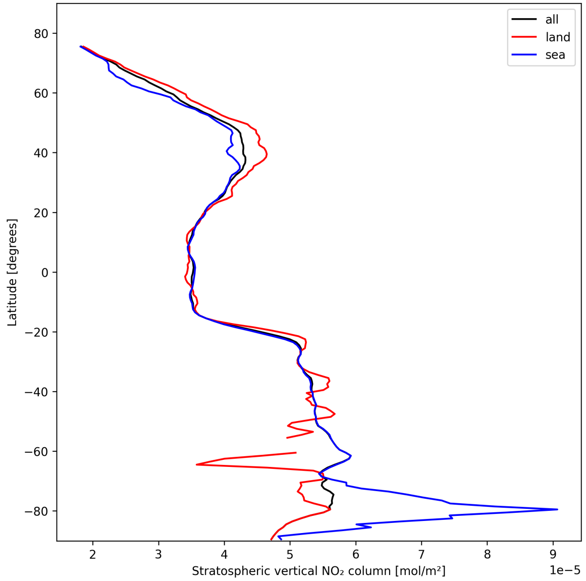
Figure 17: Zonal average of “Stratospheric vertical NO 2 column” for 2025-10-25 to 2025-10-25.
