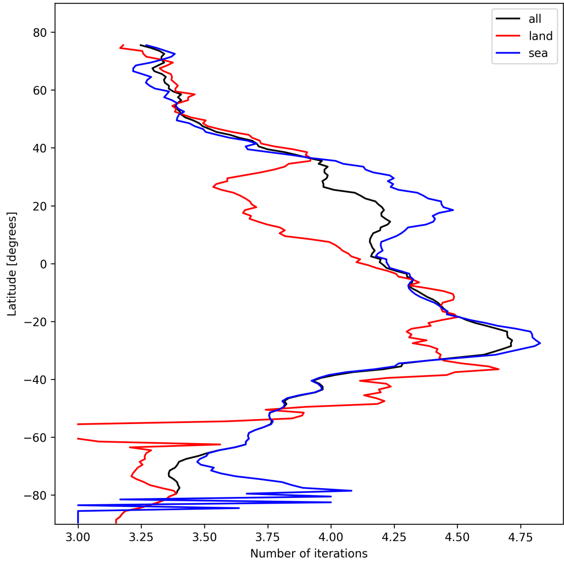
Figure 15: Zonal average of “Number of iterations” for 2025-10-25 to 2025-10-25.
