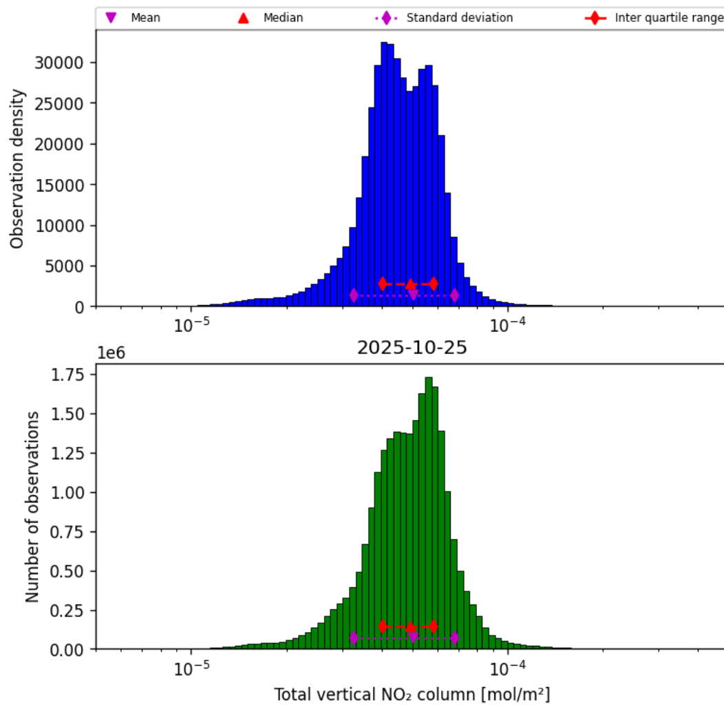
Figure 36: Histogram of “Total vertical NO 2 column” for 2025-10-25 to 2025-10-25
