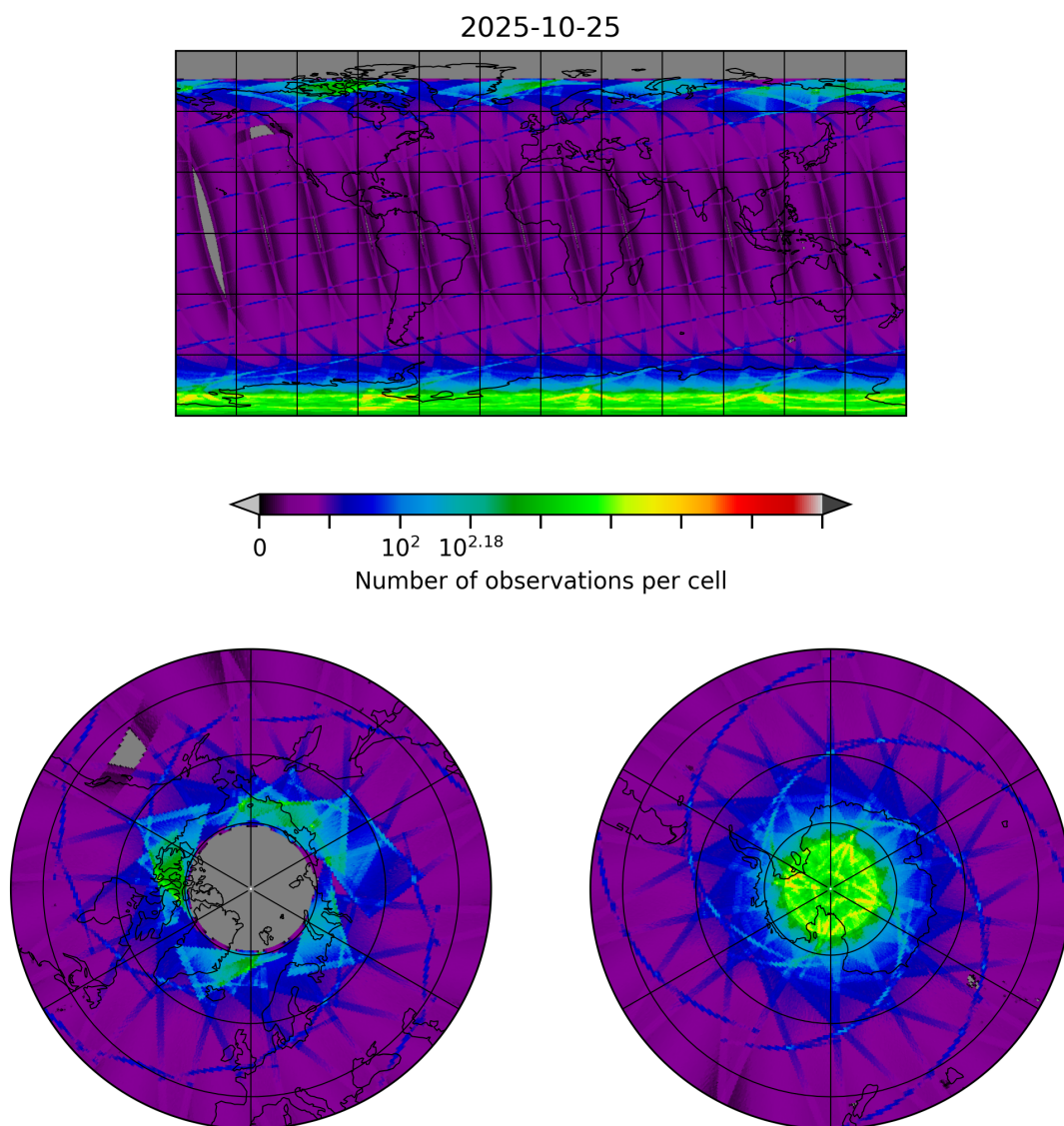
Figure 8: Map of the number of observations for 2025-10-25 to 2025-10-25
