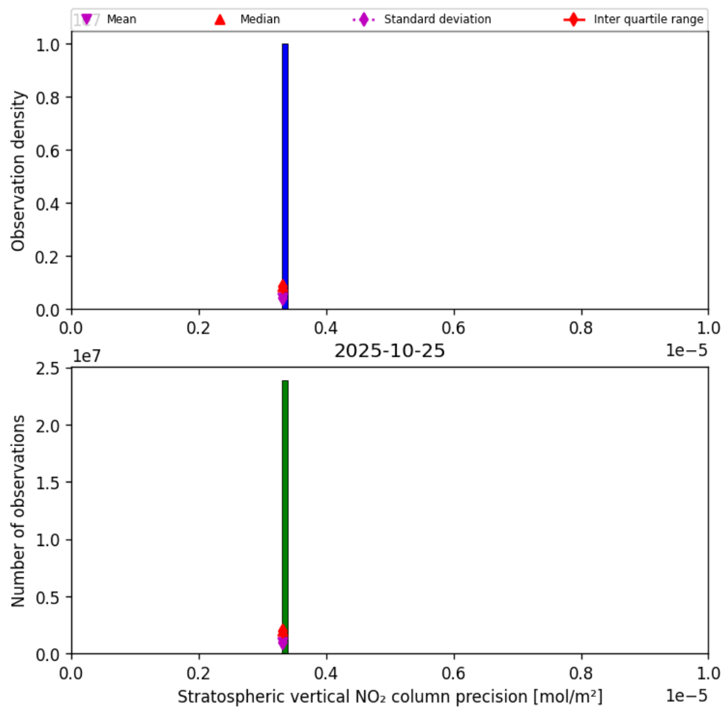
Figure 35: Histogram of “Stratospheric vertical NO 2 column precision” for 2025-10-25 to 2025-10-25
