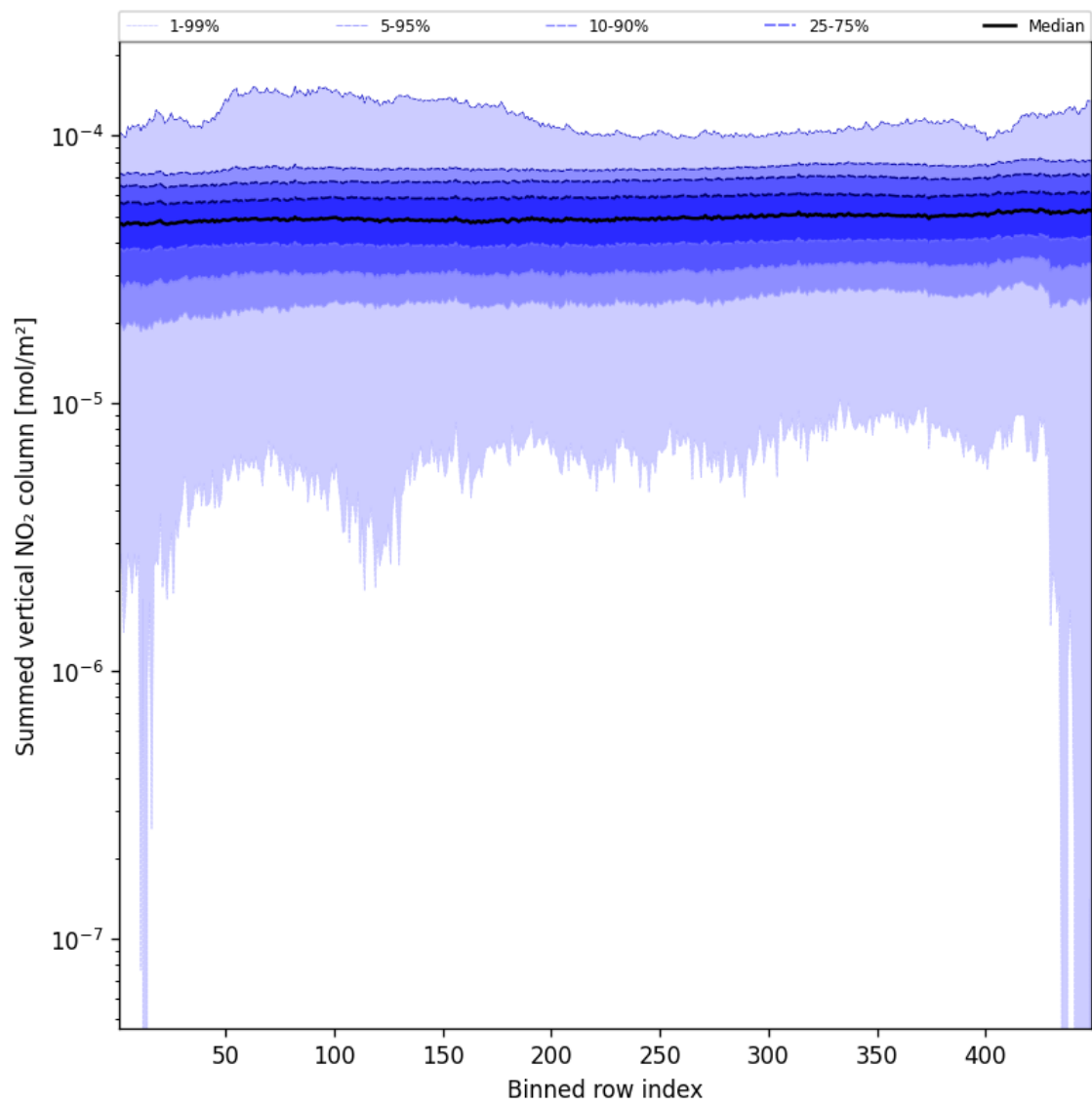
Figure 55: Along track statistics of “Summed vertical NO 2 column” for 2025-10-25 to 2025-10-25
