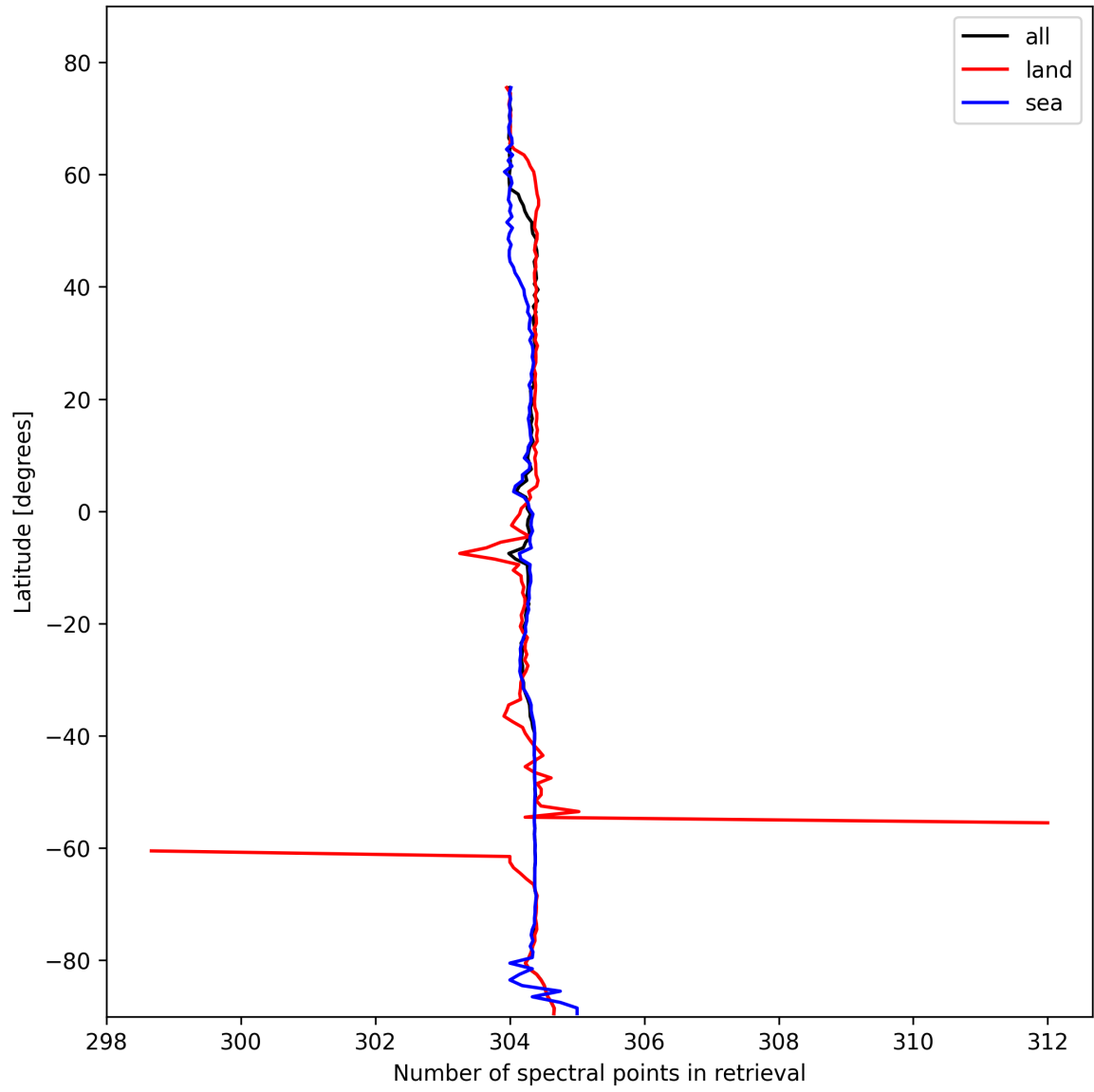
Figure 14: Zonal average of “Number of spectral points in retrieval” for 2025-10-25 to 2025-10-25.
