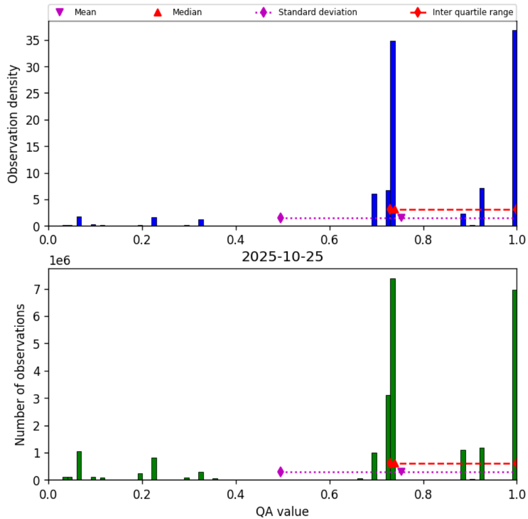
Figure 26: Histogram of “QA value” for 2025-10-25 to 2025-10-25
