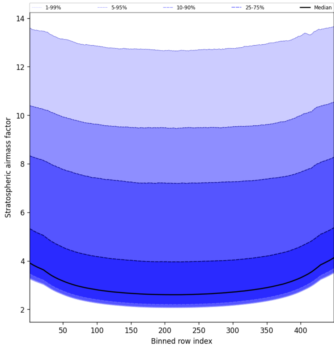
Figure 59: Along track statistics of “Stratospheric air mass factor” for 2025-10-25 to 2025-10-25
