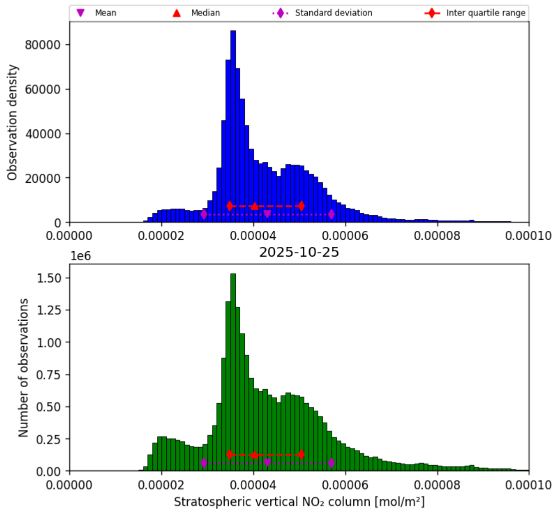
Figure 34: Histogram of “Stratospheric vertical NO 2 column” for 2025-10-25 to 2025-10-25
