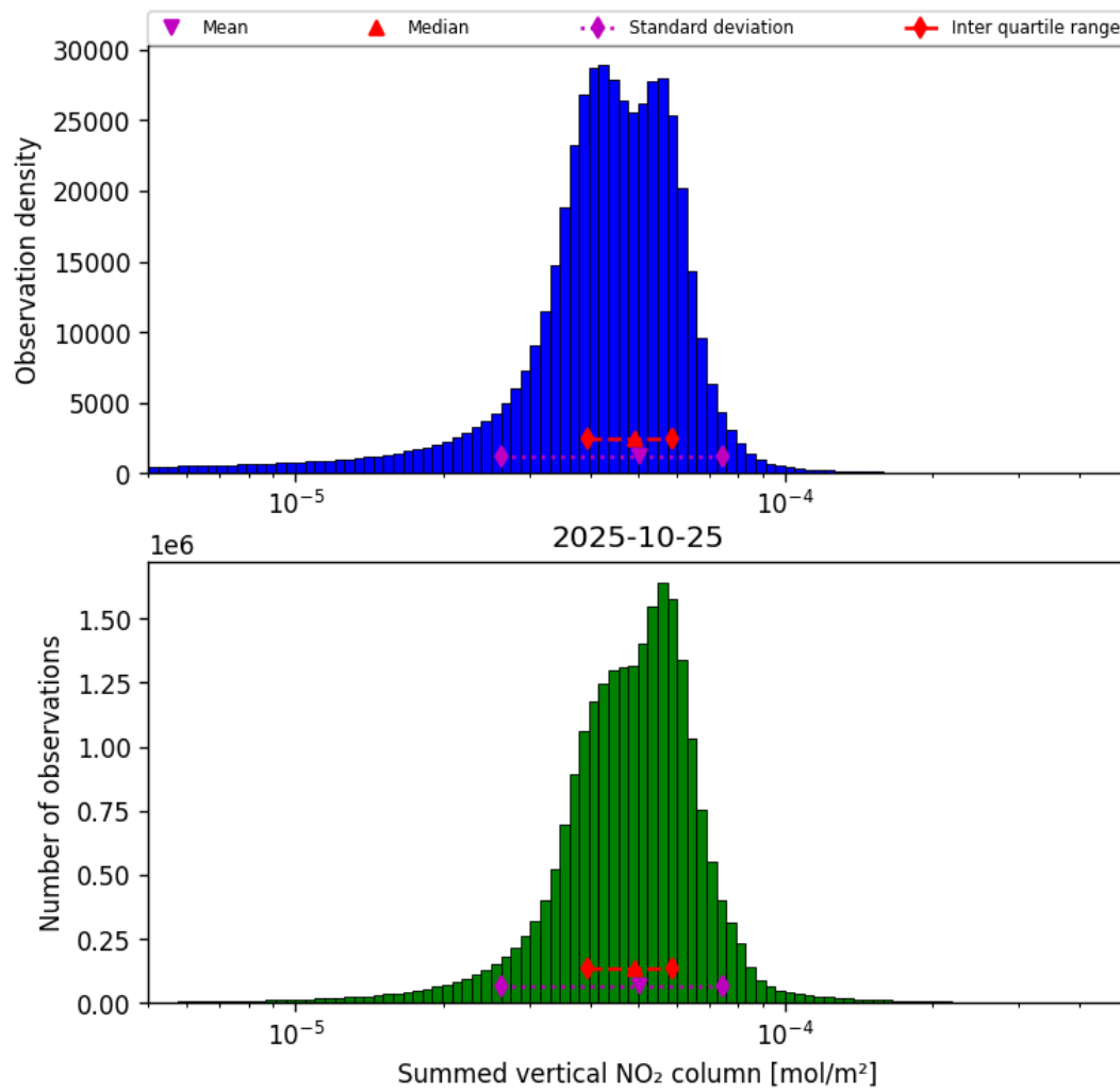
Figure 38: Histogram of “Summed vertical NO 2 column” for 2025-10-25 to 2025-10-25
