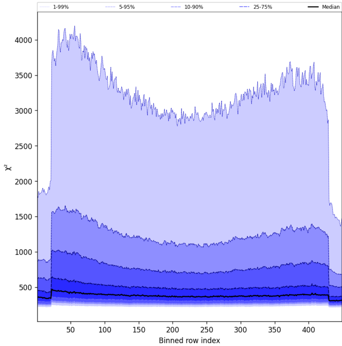
Figure 57: Along track statistics of “ \chi^2 ” for 2025-10-25 to 2025-10-25
