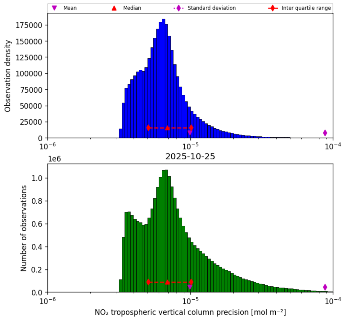
Figure 28: Histogram of "NO 2 tropospheric vertical column precision" for 2025-10-25 to 2025-10-25
