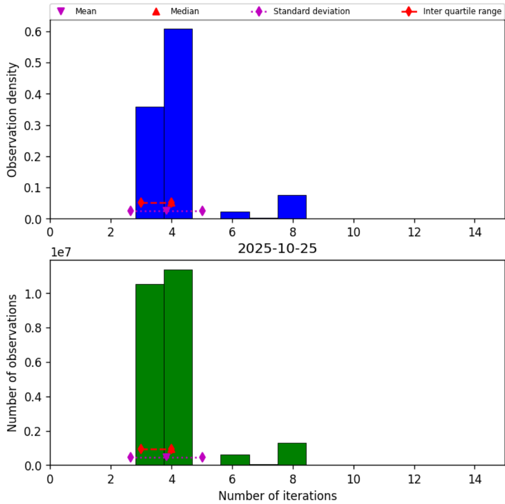
Figure 32: Histogram of “Number of iterations” for 2025-10-25 to 2025-10-25
