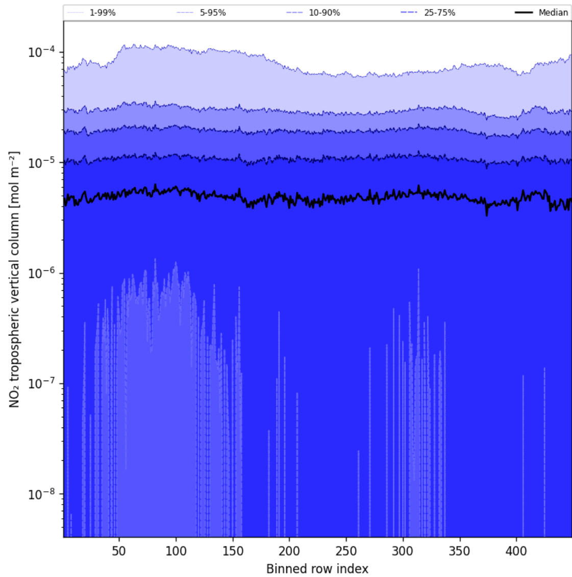
Figure 44: Along track statistics of “NO 2 tropospheric vertical column” for 2025-10-25 to 2025-10-25
