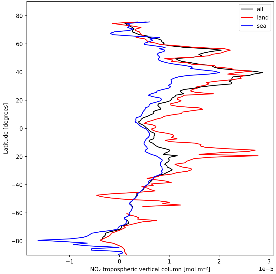
Figure 10: Zonal average of “NO 2 tropospheric vertical column” for 2025-10-25 to 2025-10-25.
