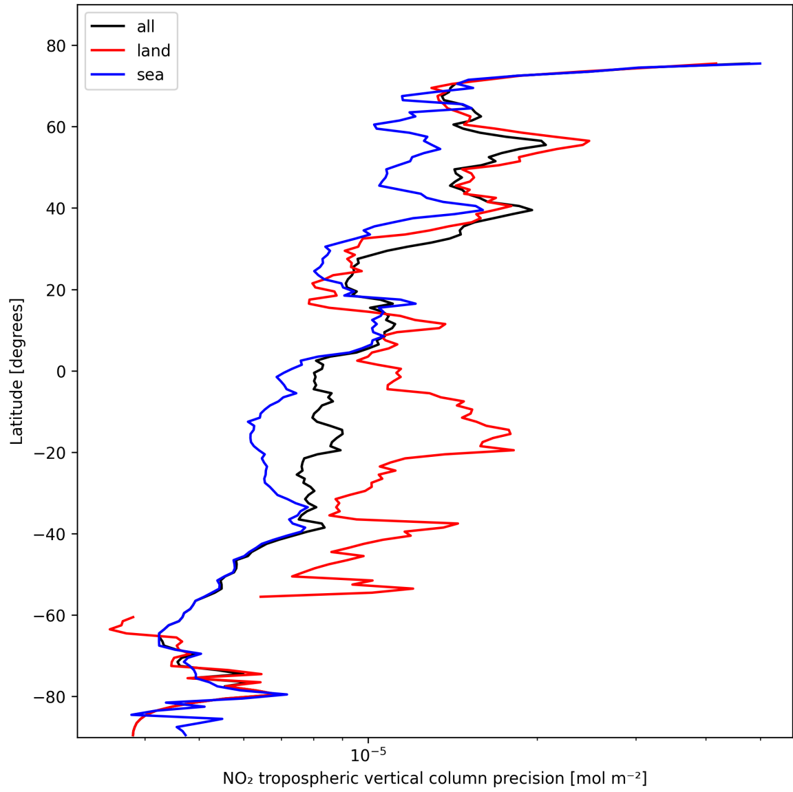
Figure 11: Zonal average of “NO 2 tropospheric vertical column precision” for 2025-10-25 to 2025-10-25.
