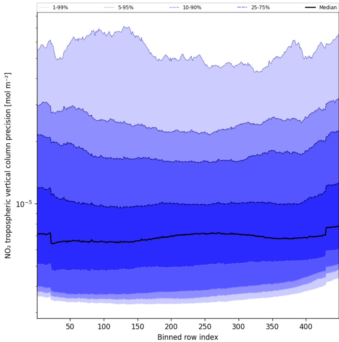
Figure 45: Along track statistics of “NO 2 tropospheric vertical column precision” for 2025-10-25 to 2025-10-25
