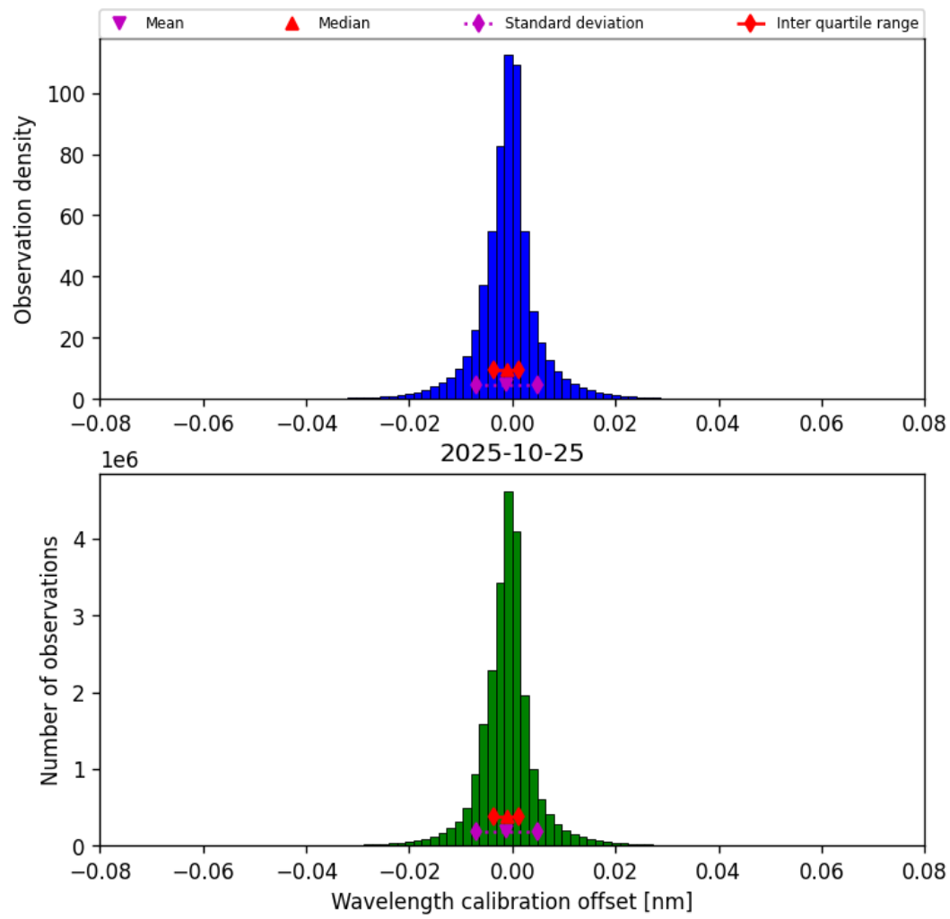
Figure 33: Histogram of “Wavelength calibration offset” for 2025-10-25 to 2025-10-25
