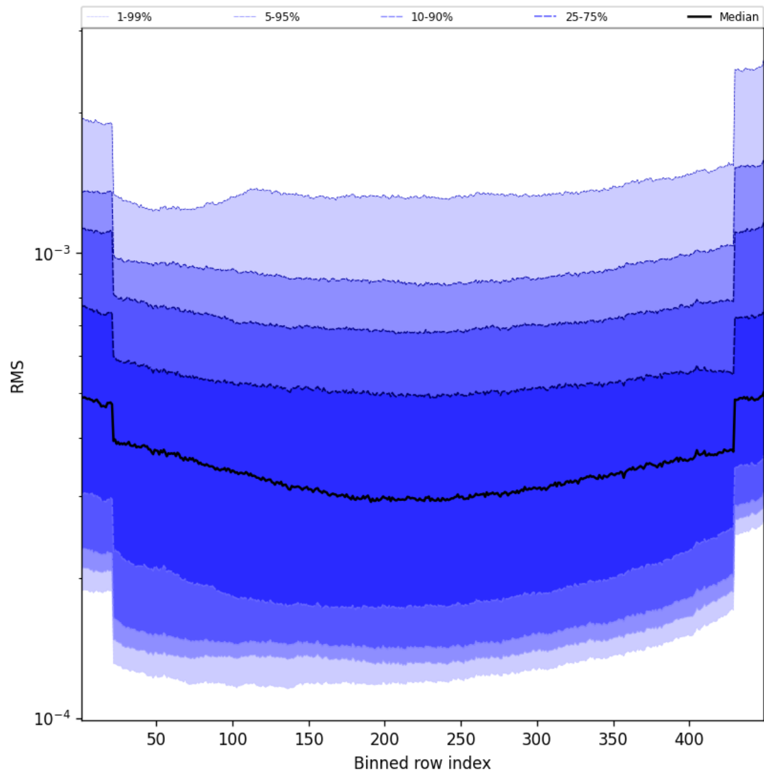
Figure 58: Along track statistics of “RMS” for 2025-10-25 to 2025-10-25
