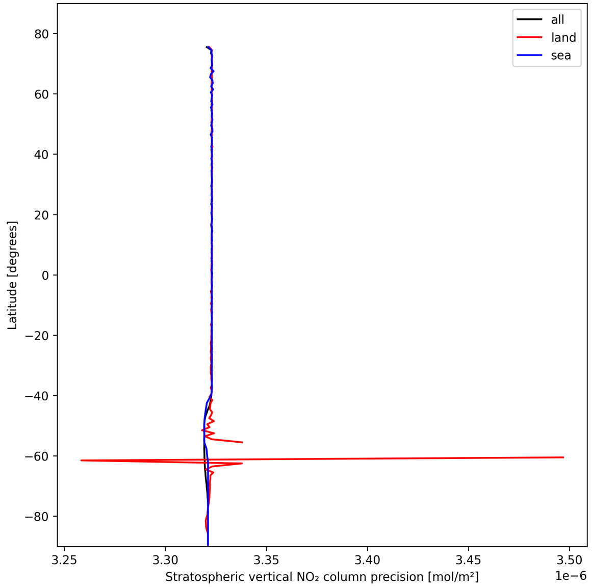
Figure 18: Zonal average of “Stratospheric vertical NO 2 column precision” for 2025-10-25 to 2025-10-25.
