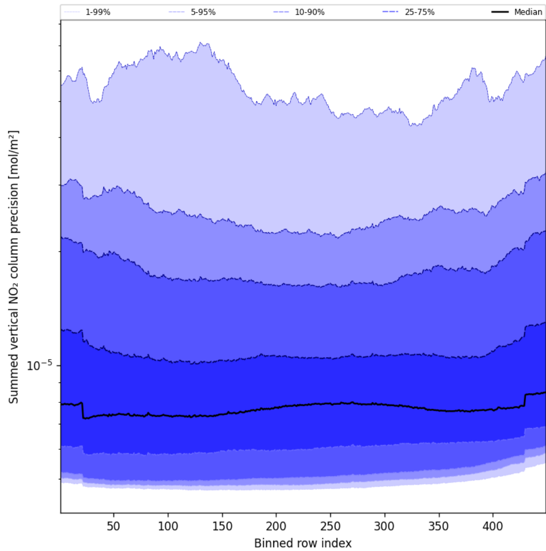
Figure 56: Along track statistics of “Summed vertical NO 2 column precision” for 2025-10-25 to 2025-10-25
