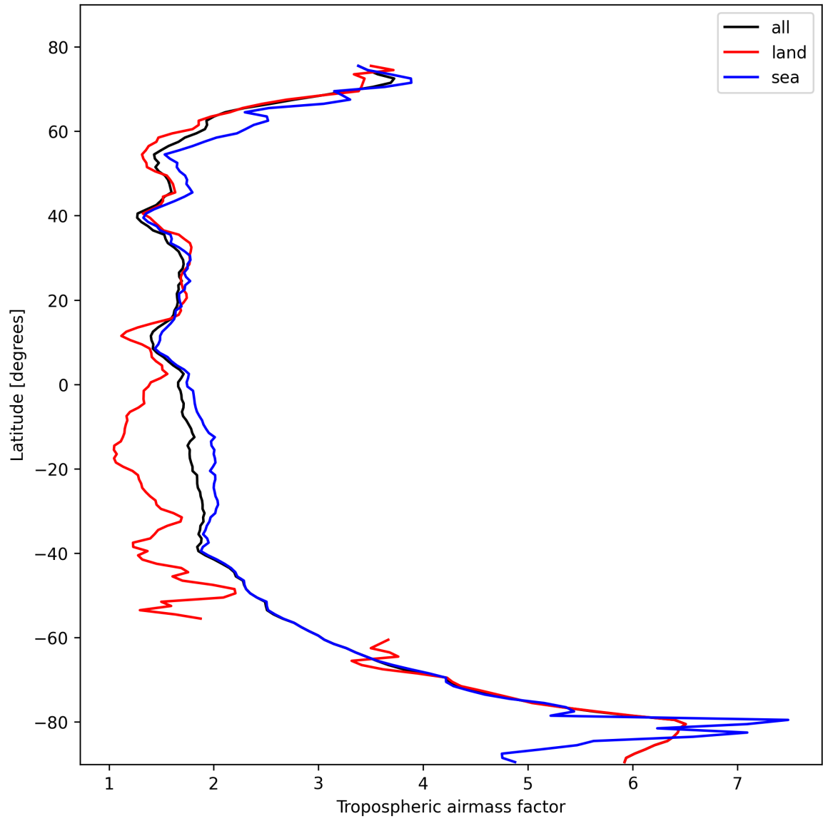
Figure 12: Zonal average of “Tropospheric airmass factor” for 2025-10-25 to 2025-10-25.
