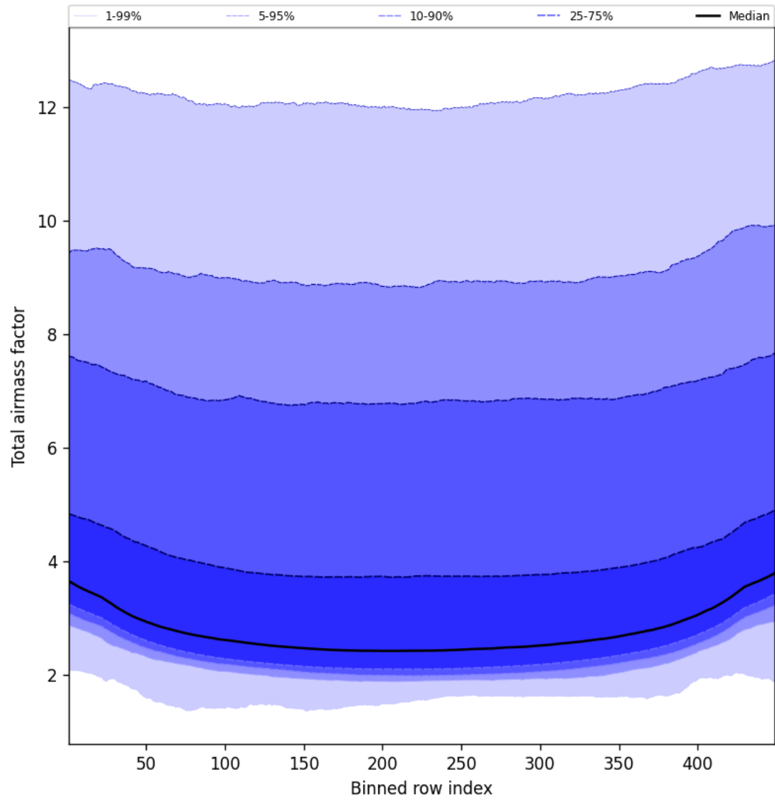
Figure 47: Along track statistics of “Total airmass factor” for 2025-10-25 to 2025-10-25
