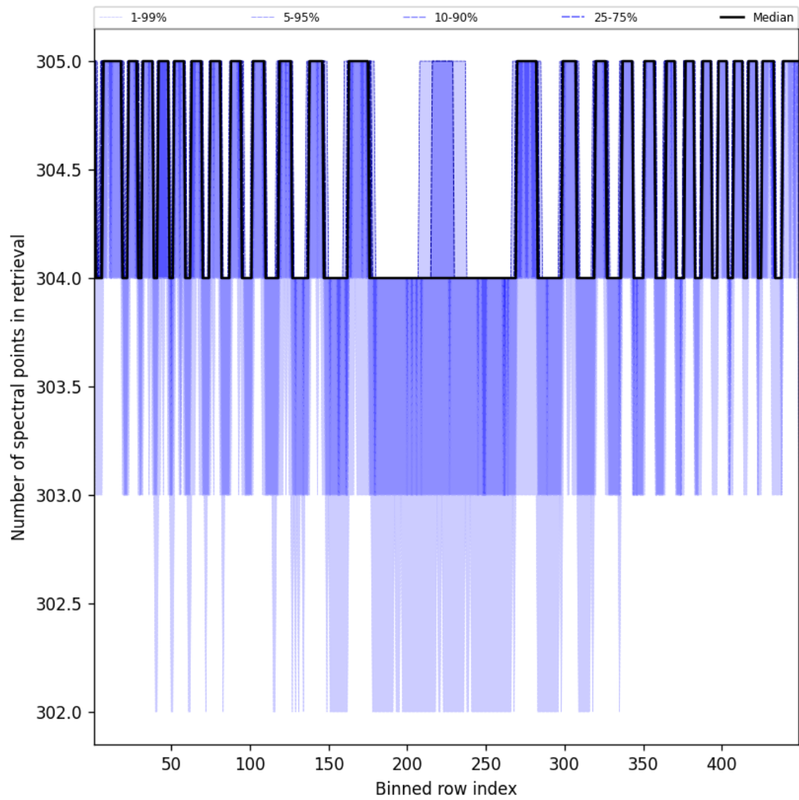
Figure 48: Along track statistics of “Number of spectral points in retrieval” for 2025-10-25 to 2025-10-25
