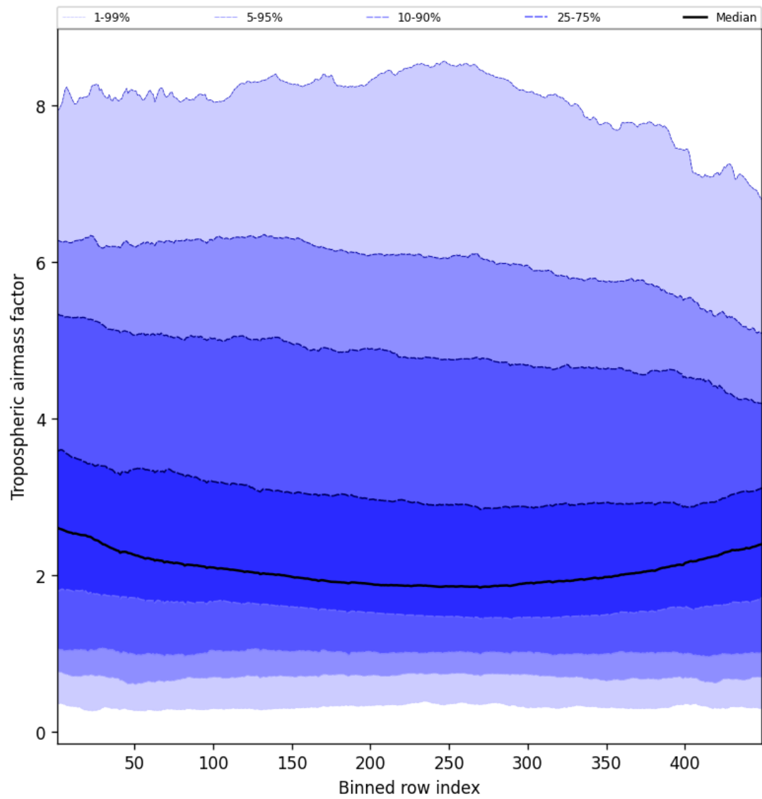
Figure 46: Along track statistics of “Tropospheric air mass factor” for 2025-10-25 to 2025-10-25
