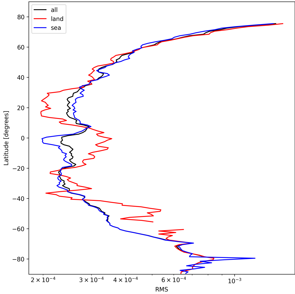
Figure 24: Zonal average of “RMS” for 2025-10-25 to 2025-10-25.
