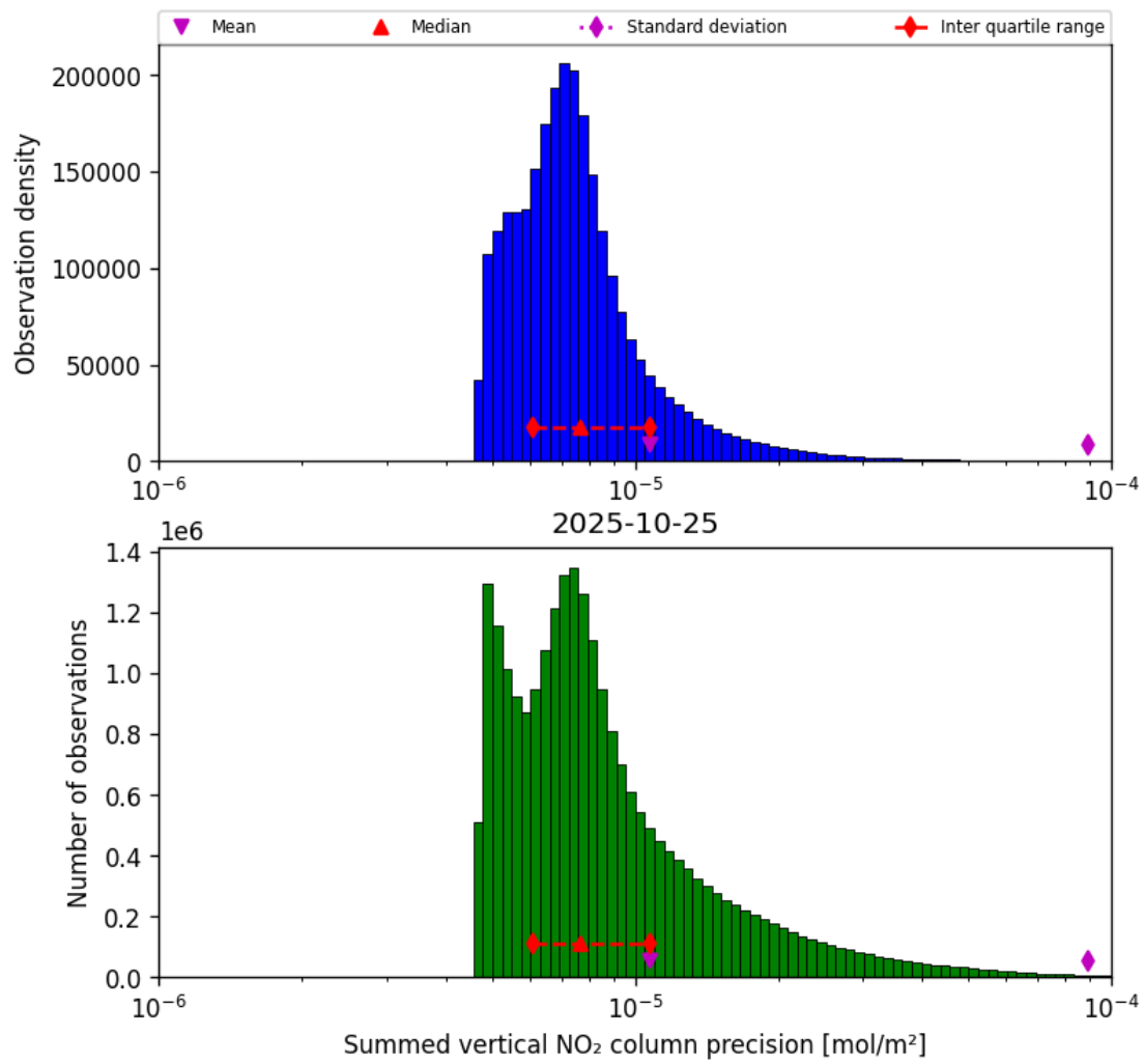
Figure 39: Histogram of “Summed vertical NO 2 column precision” for 2025-10-25 to 2025-10-25
