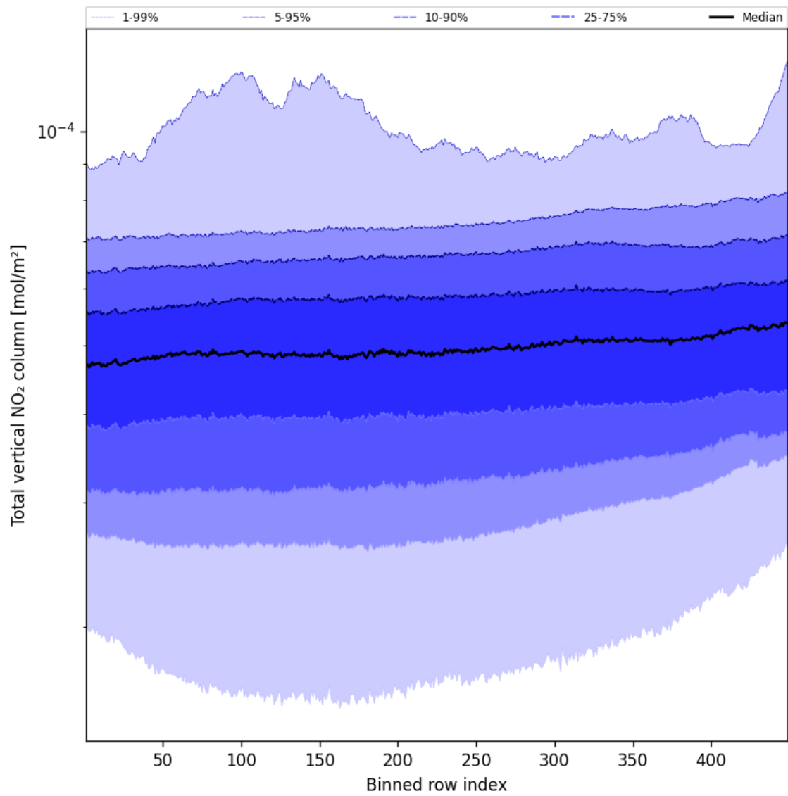
Figure 53: Along track statistics of “Total vertical NO 2 column” for 2025-10-25 to 2025-10-25
