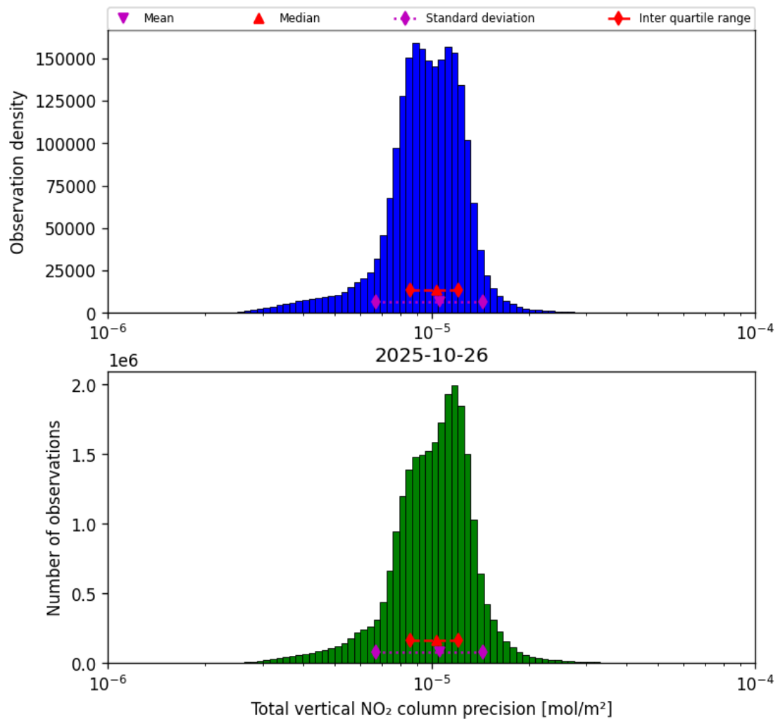
Figure 37: Histogram of “Total vertical NO 2 column precision” for 2025-10-26 to 2025-10-27
