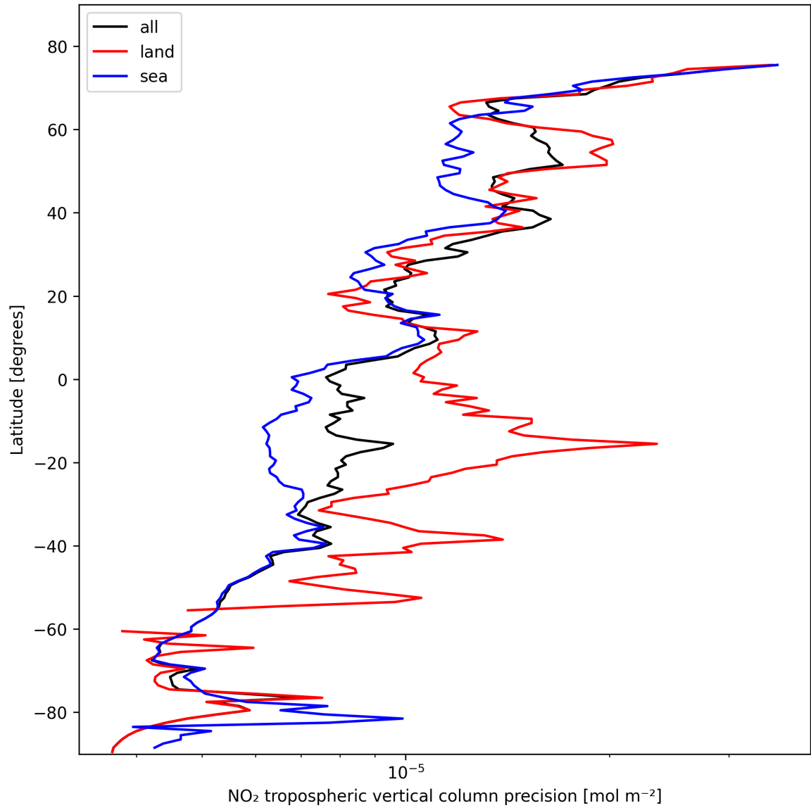
Figure 11: Zonal average of “NO 2 tropospheric vertical column precision” for 2025-10-26 to 2025-10-27.
