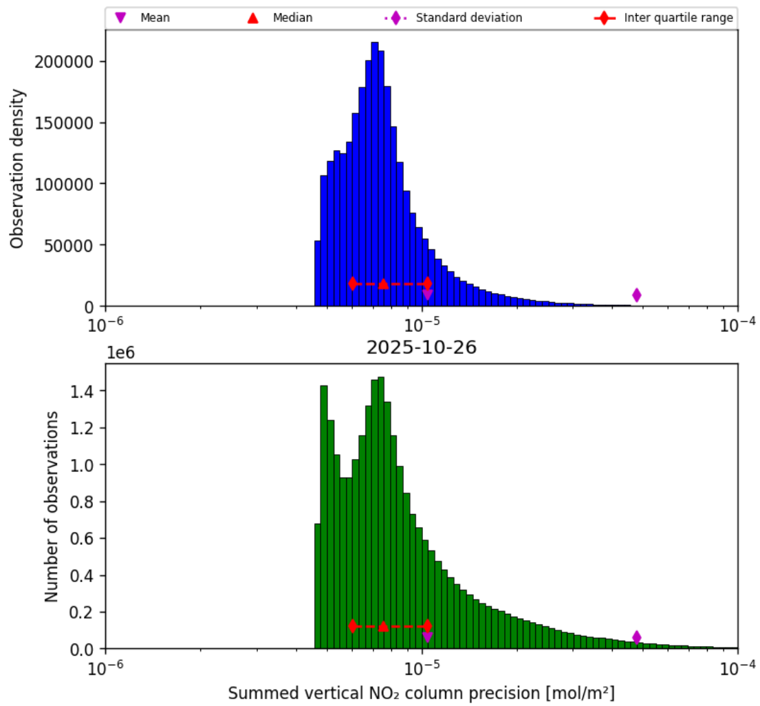
Figure 39: Histogram of “Summed vertical NO 2 column precision” for 2025-10-26 to 2025-10-27
