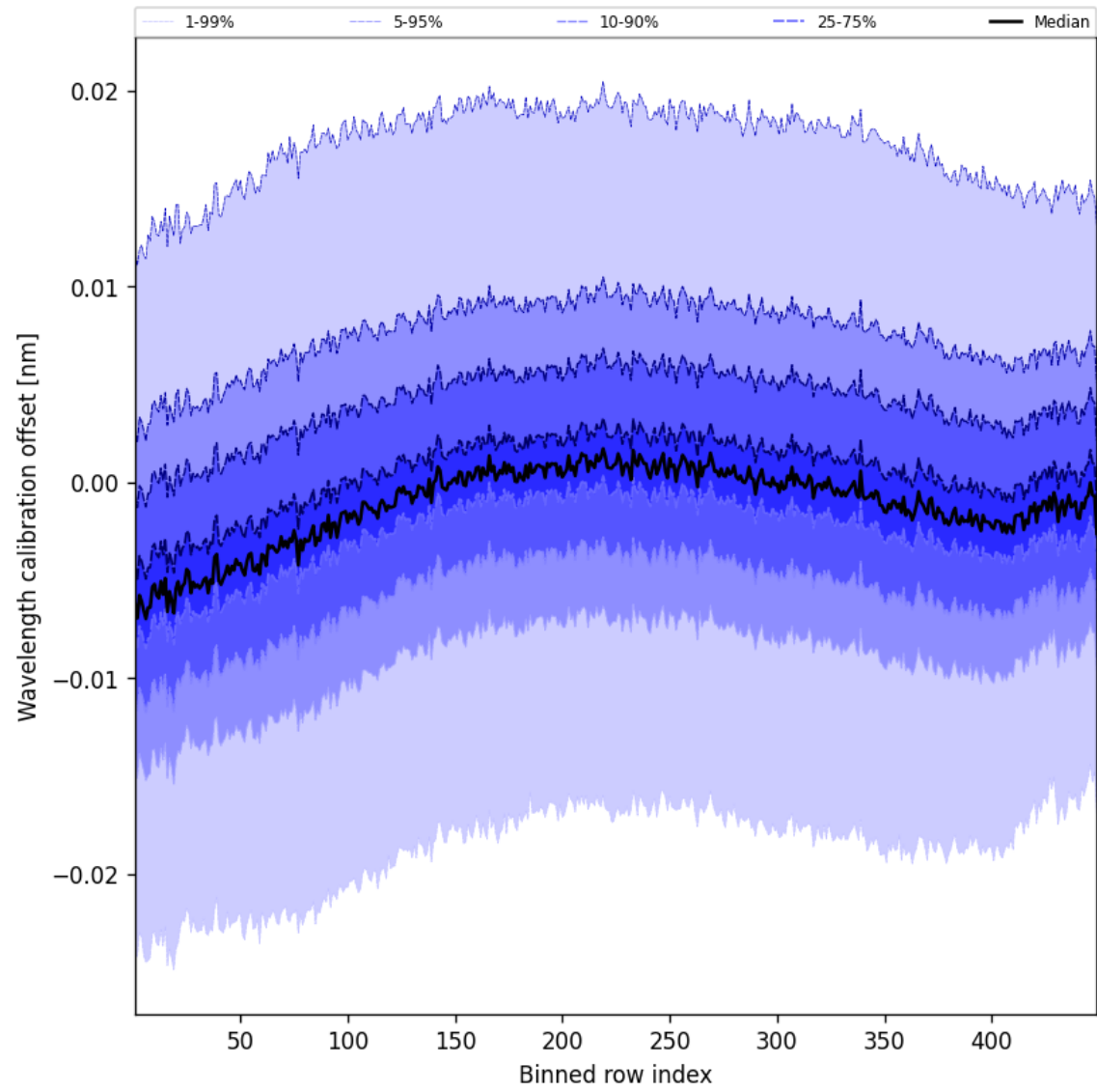
Figure 50: Along track statistics of “Wavelength calibration offset” for 2025-10-26 to 2025-10-27
