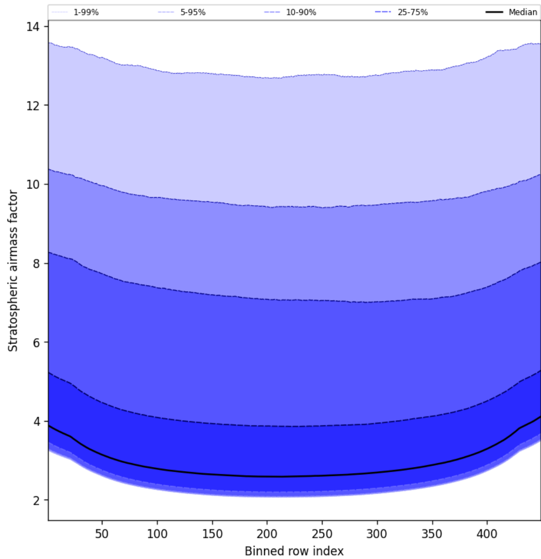
Figure 59: Along track statistics of “Stratospheric airmass factor” for 2025-10-26 to 2025-10-27
