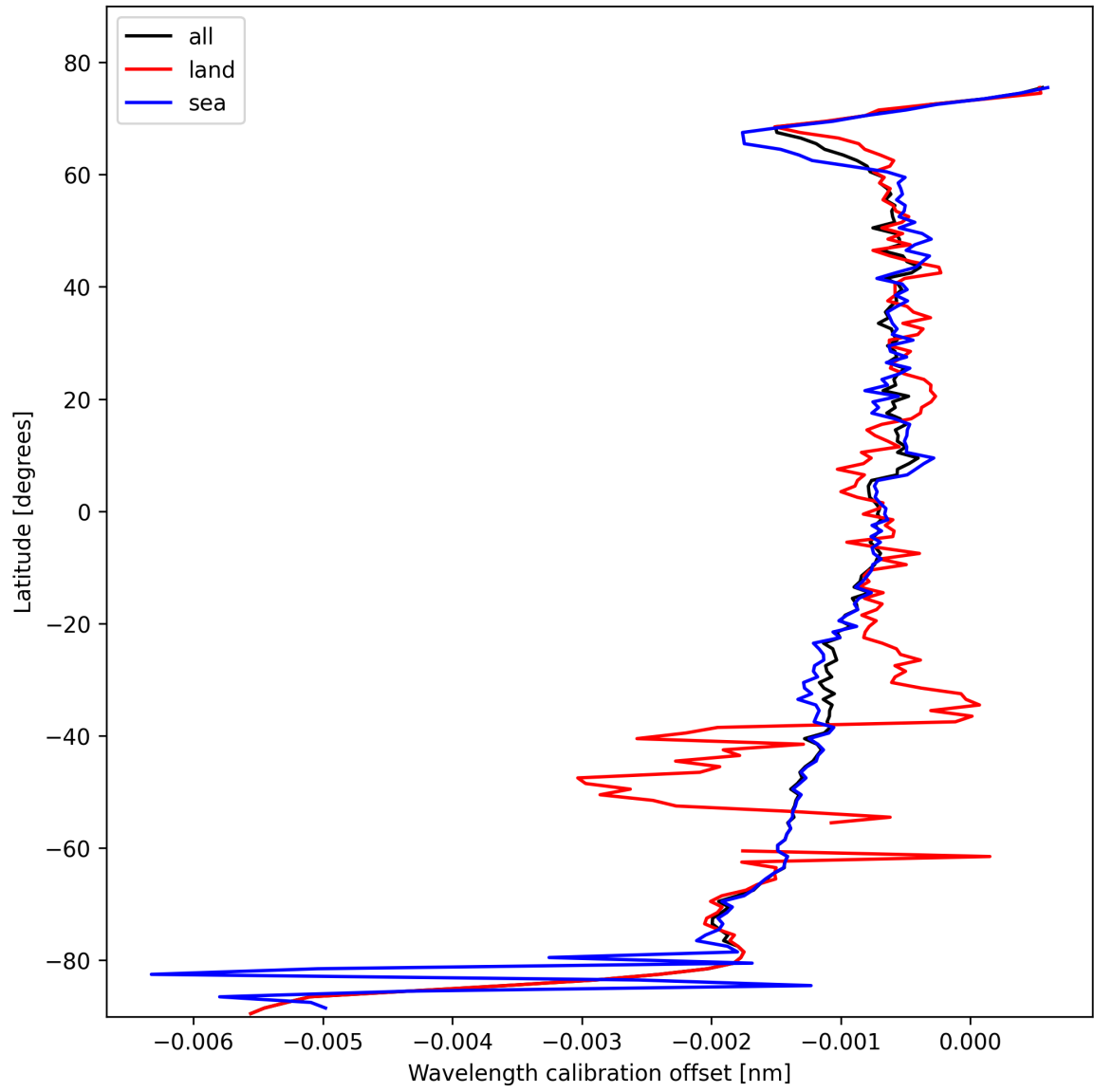
Figure 16: Zonal average of “Wavelength calibration offset” for 2025-10-26 to 2025-10-27.
