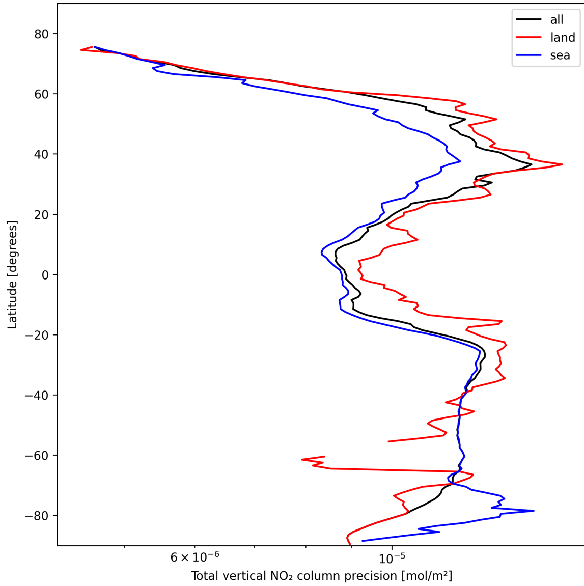
Figure 20: Zonal average of “Total vertical NO 2 column precision” for 2025-10-26 to 2025-10-27.
