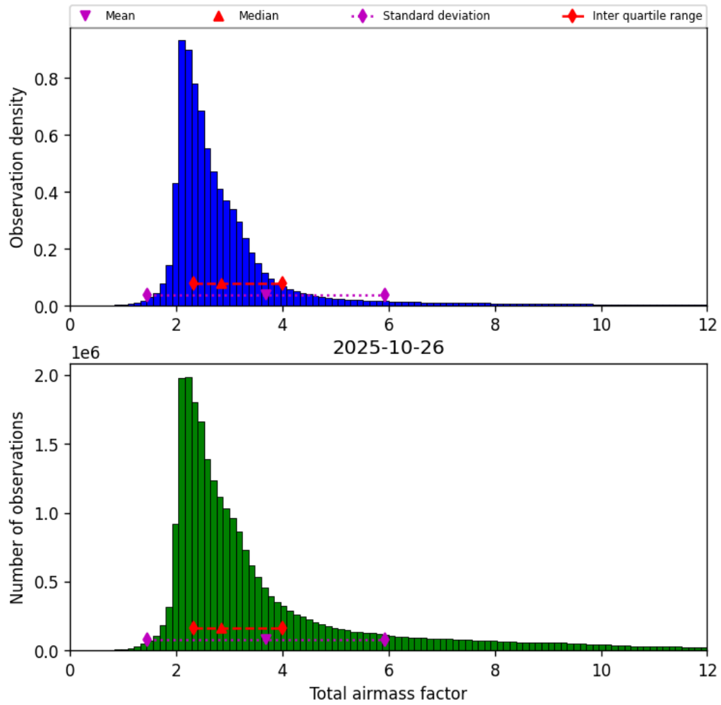
Figure 30: Histogram of “Total airmass factor” for 2025-10-26 to 2025-10-27
