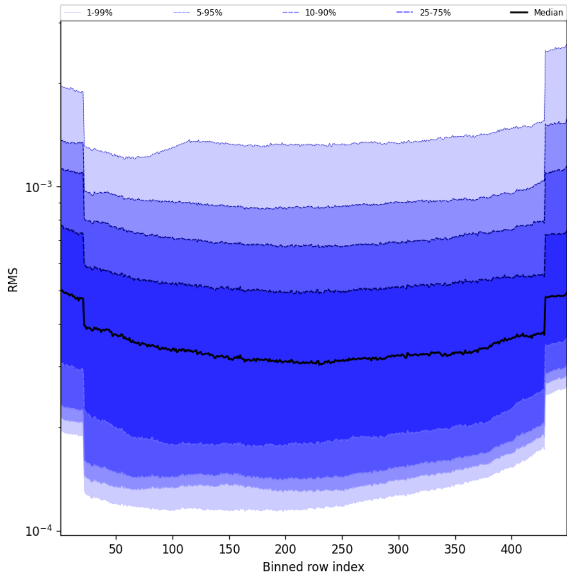
Figure 58: Along track statistics of “RMS” for 2025-10-27 to 2025-10-28
