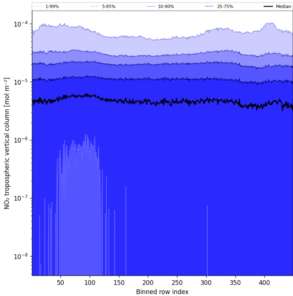
Figure 44: Along track statistics of “NO 2 tropospheric vertical column” for 2025-10-27 to 2025-10-28
