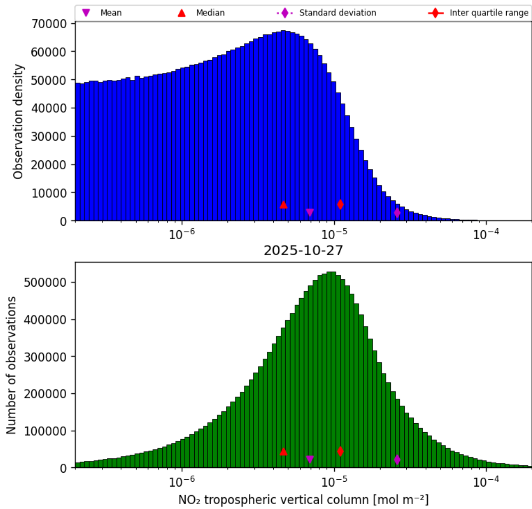
Figure 27: Histogram of “NO 2 tropospheric vertical column” for 2025-10-27 to 2025-10-28
