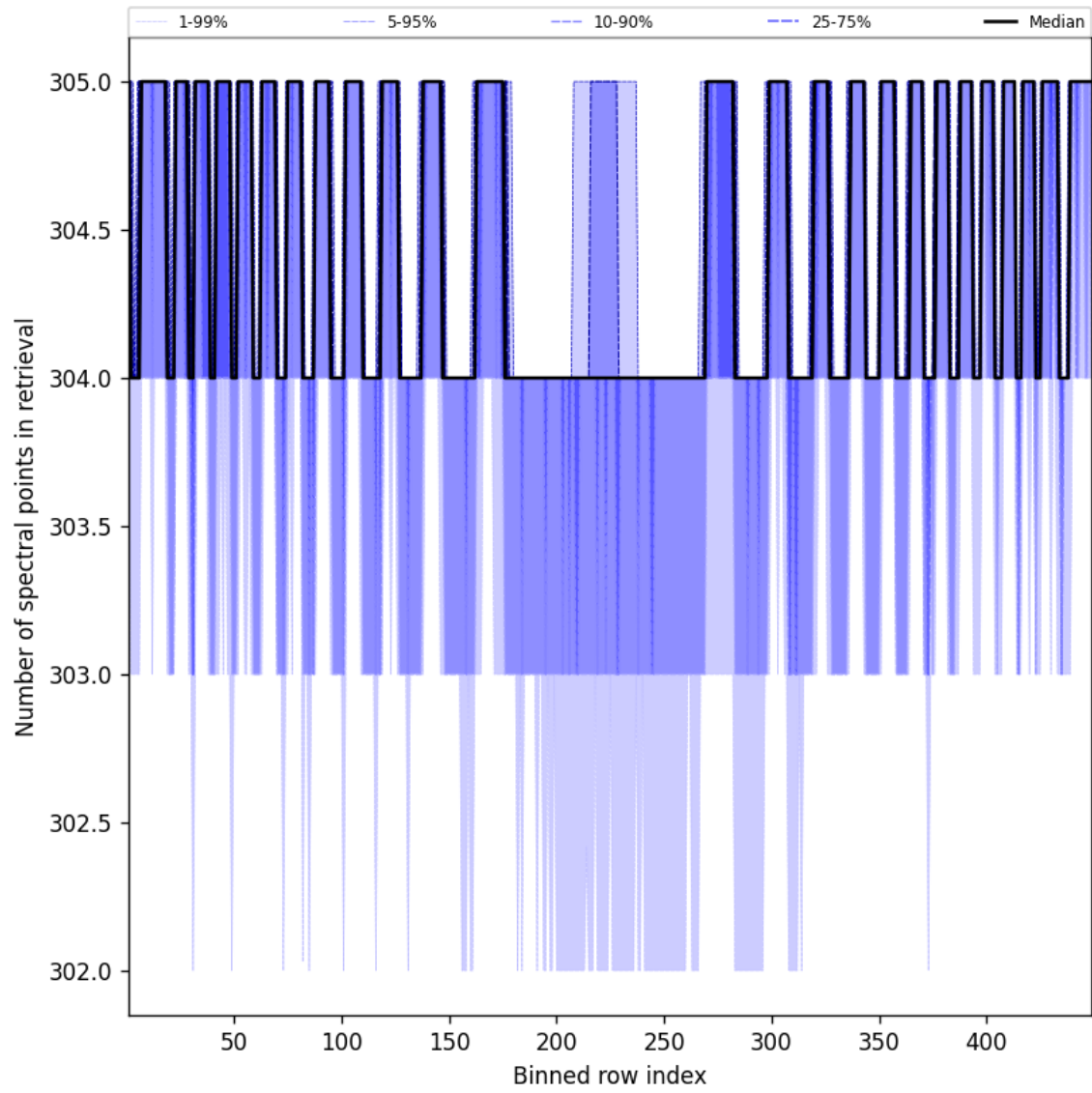
Figure 48: Along track statistics of “Number of spectral points in retrieval” for 2025-10-27 to 2025-10-28
