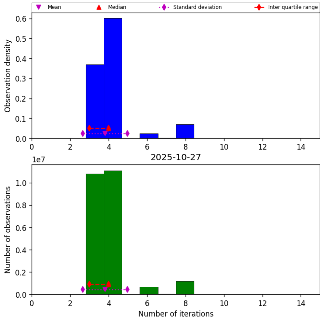
Figure 32: Histogram of “Number of iterations” for 2025-10-27 to 2025-10-28
