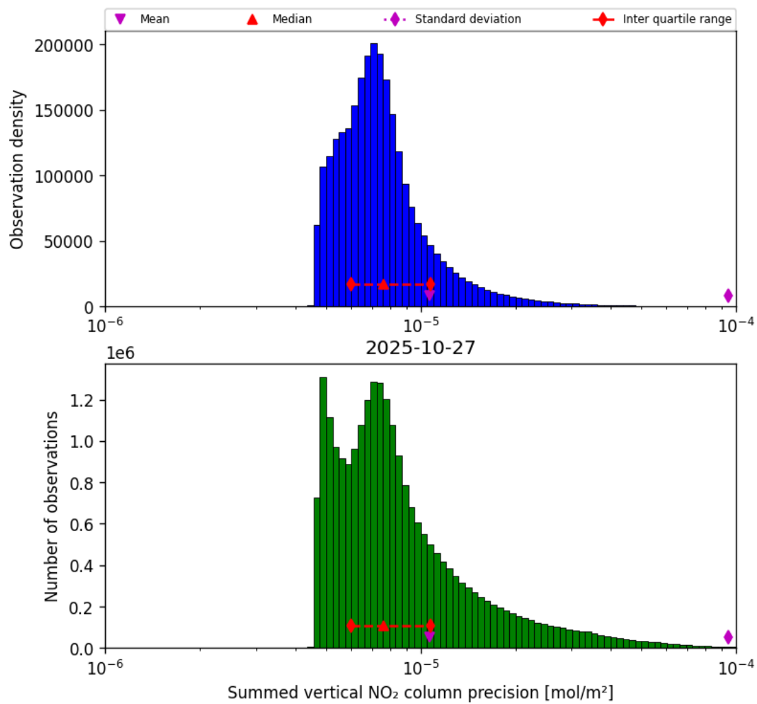
Figure 39: Histogram of “Summed vertical NO 2 column precision” for 2025-10-27 to 2025-10-28
