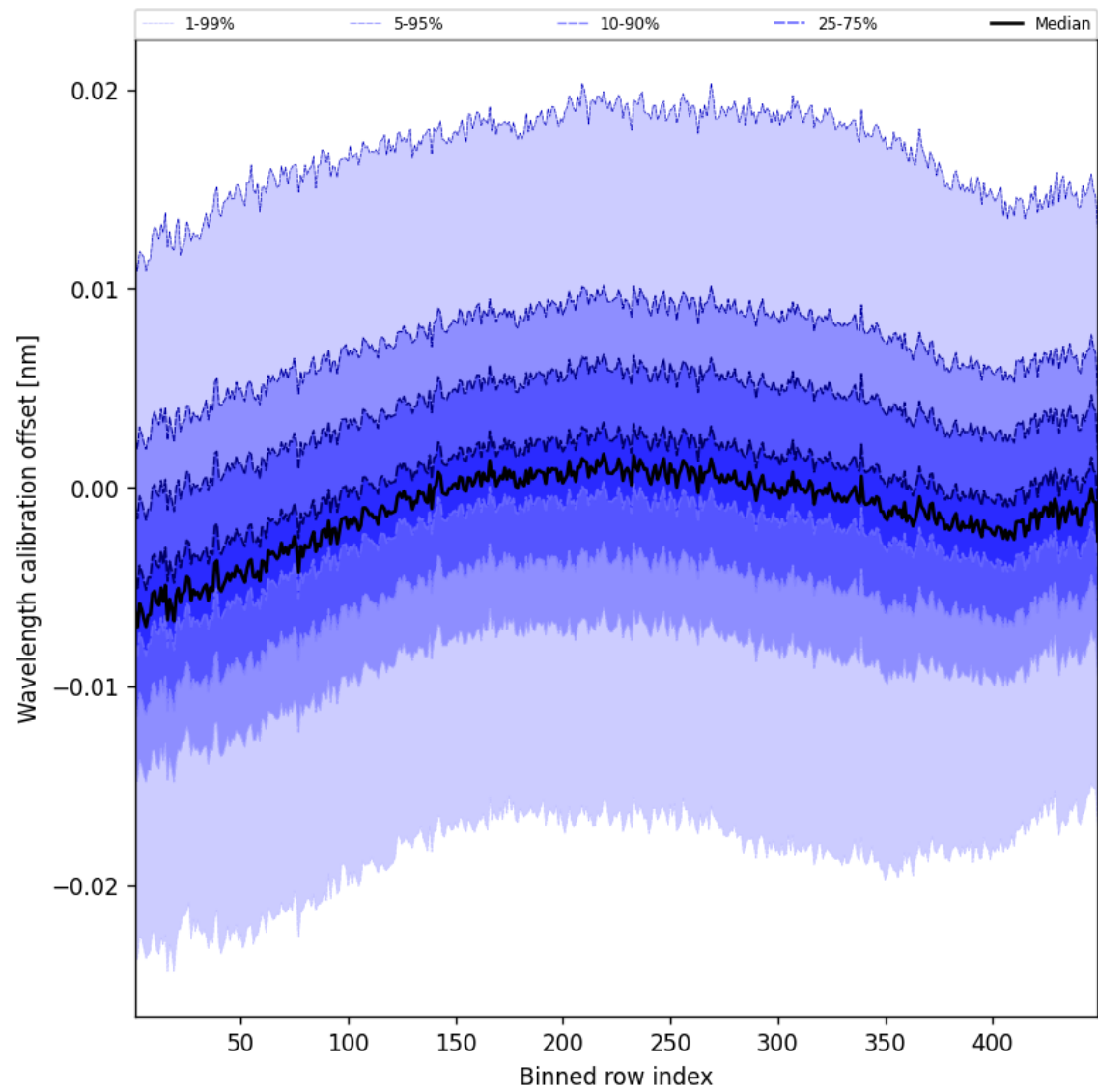
Figure 50: Along track statistics of “Wavelength calibration offset” for 2025-10-27 to 2025-10-28
