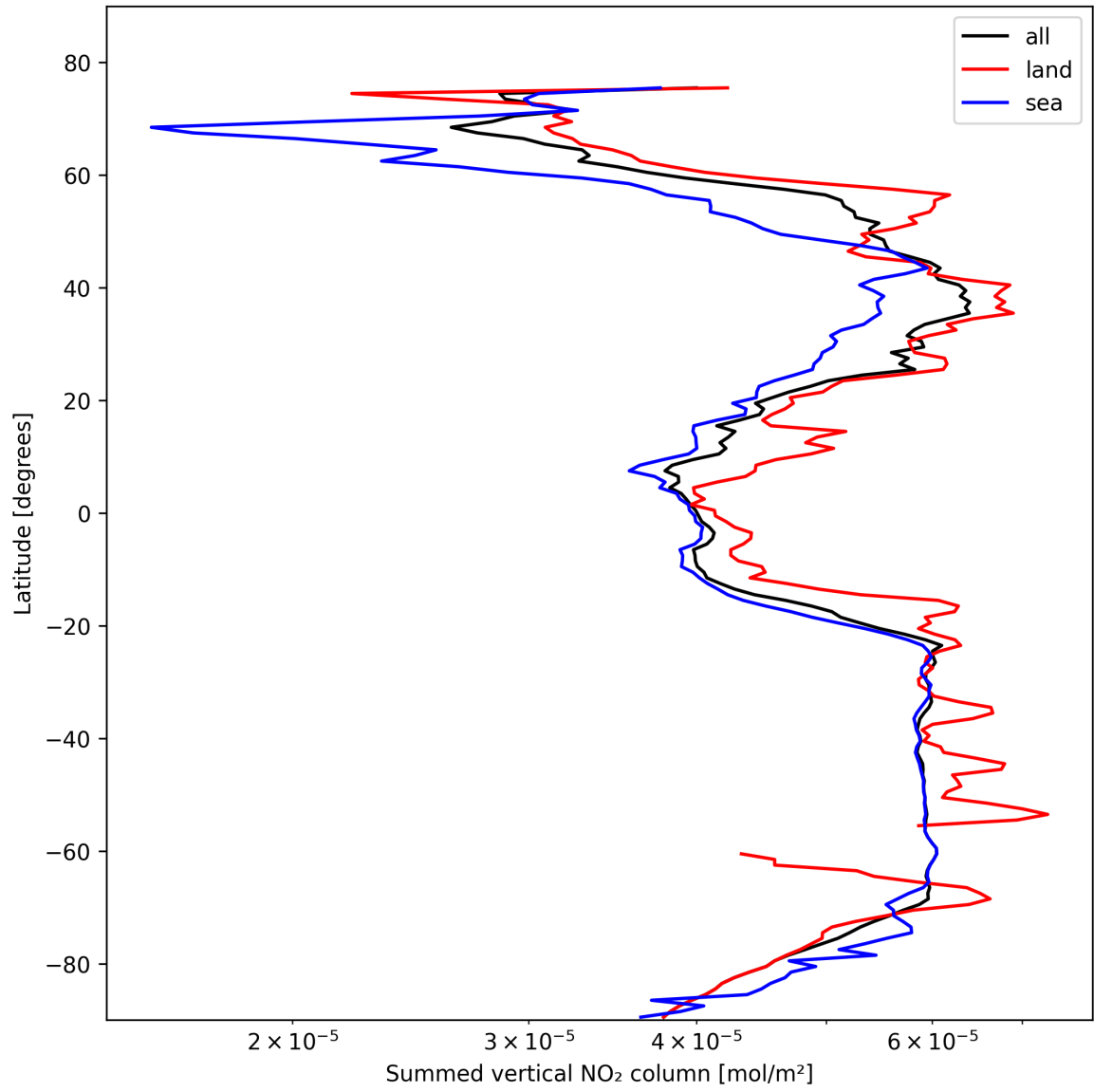
Figure 21: Zonal average of “Summed vertical NO 2 column” for 2025-10-27 to 2025-10-28.
