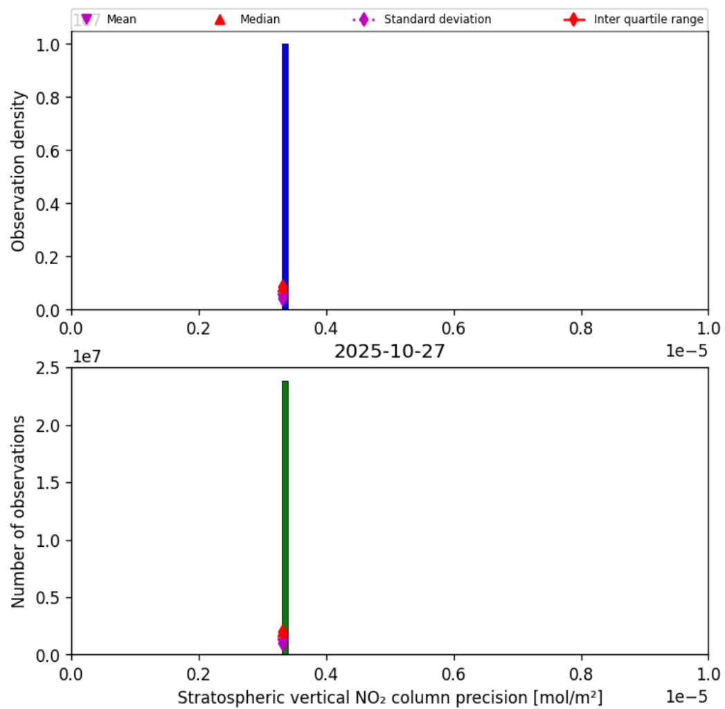
Figure 35: Histogram of “Stratospheric vertical NO 2 column precision” for 2025-10-27 to 2025-10-28
