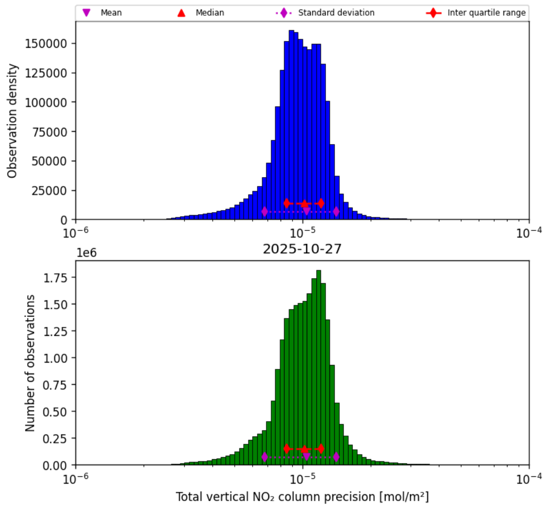
Figure 37: Histogram of “Total vertical NO 2 column precision” for 2025-10-27 to 2025-10-28
