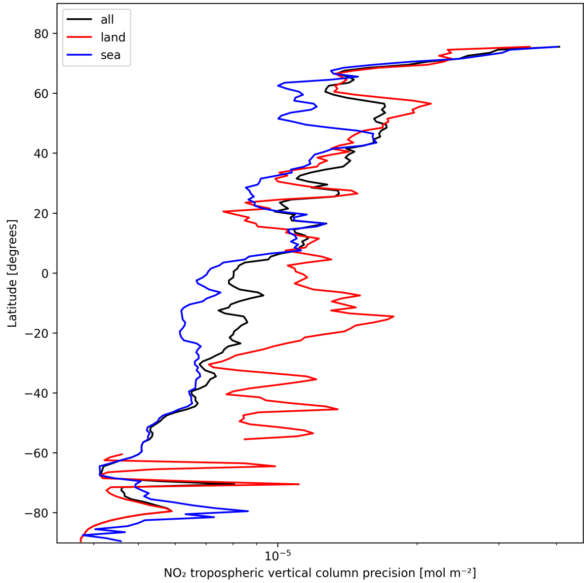
Figure 11: Zonal average of “NO 2 tropospheric vertical column precision” for 2025-10-27 to 2025-10-28.
