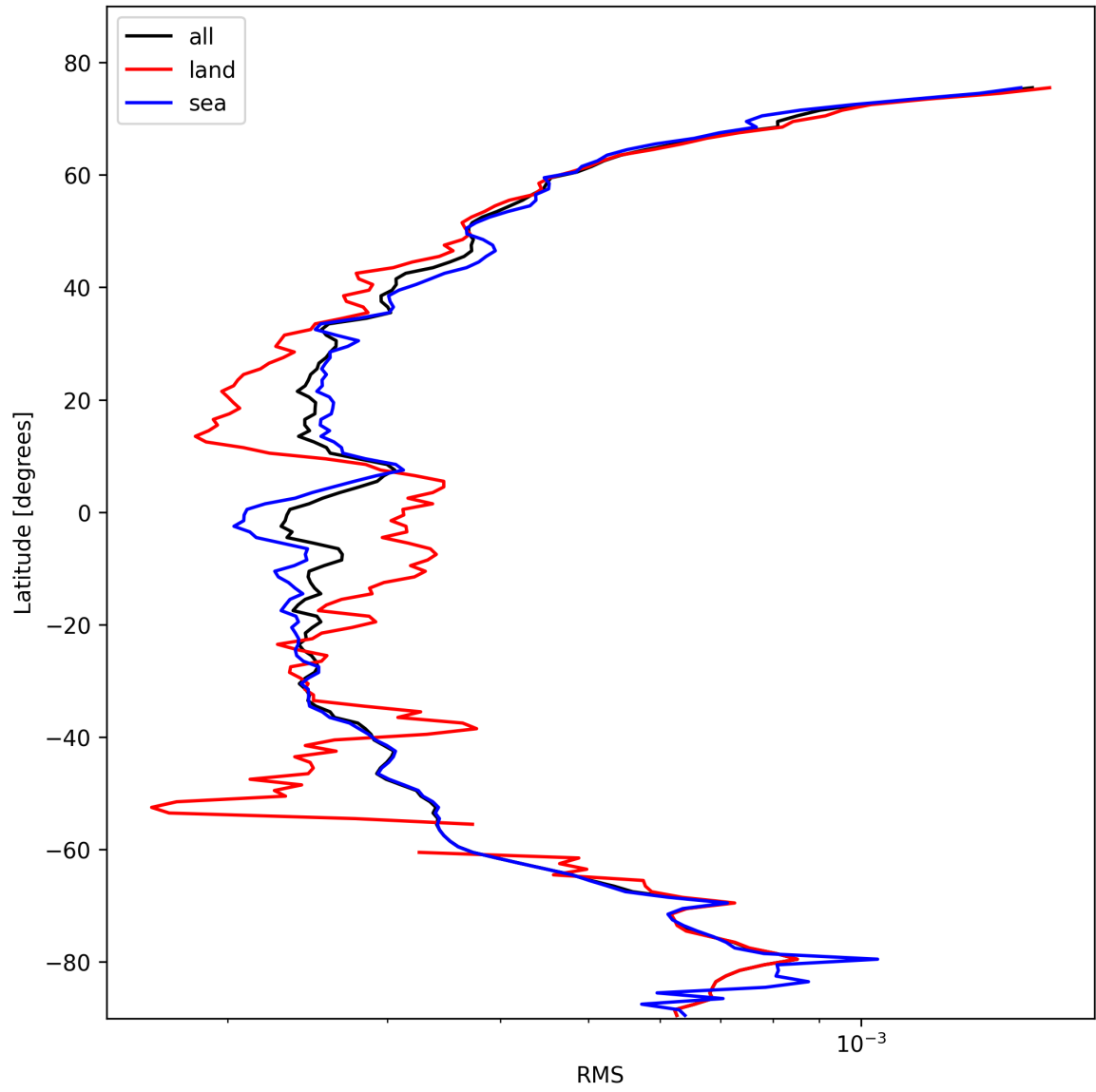
Figure 24: Zonal average of “RMS” for 2025-10-27 to 2025-10-28.
