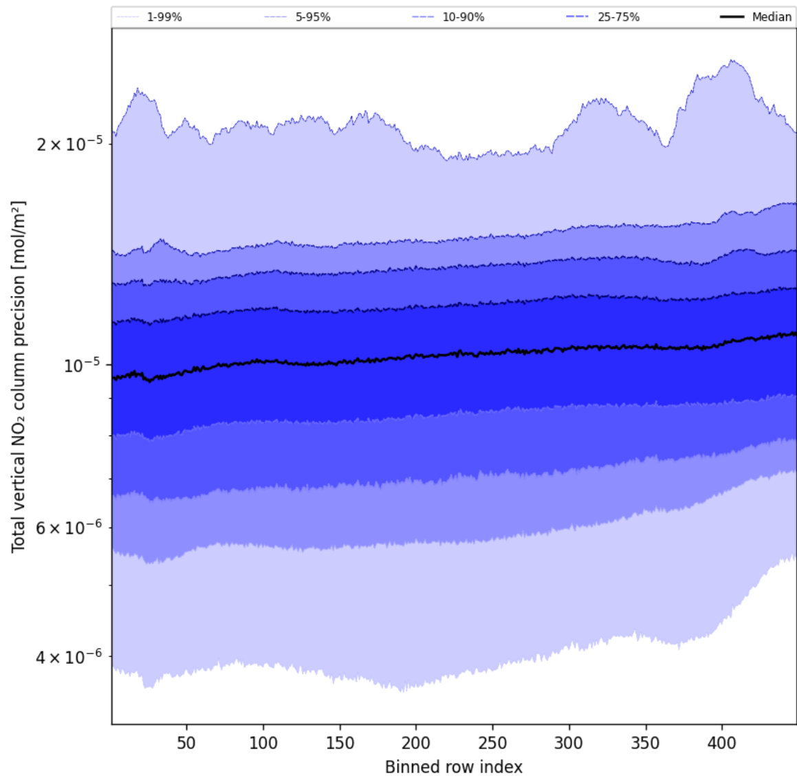
Figure 54: Along track statistics of "Total vertical NO 2 column precision" for 2025-10-27 to 2025-10-28
