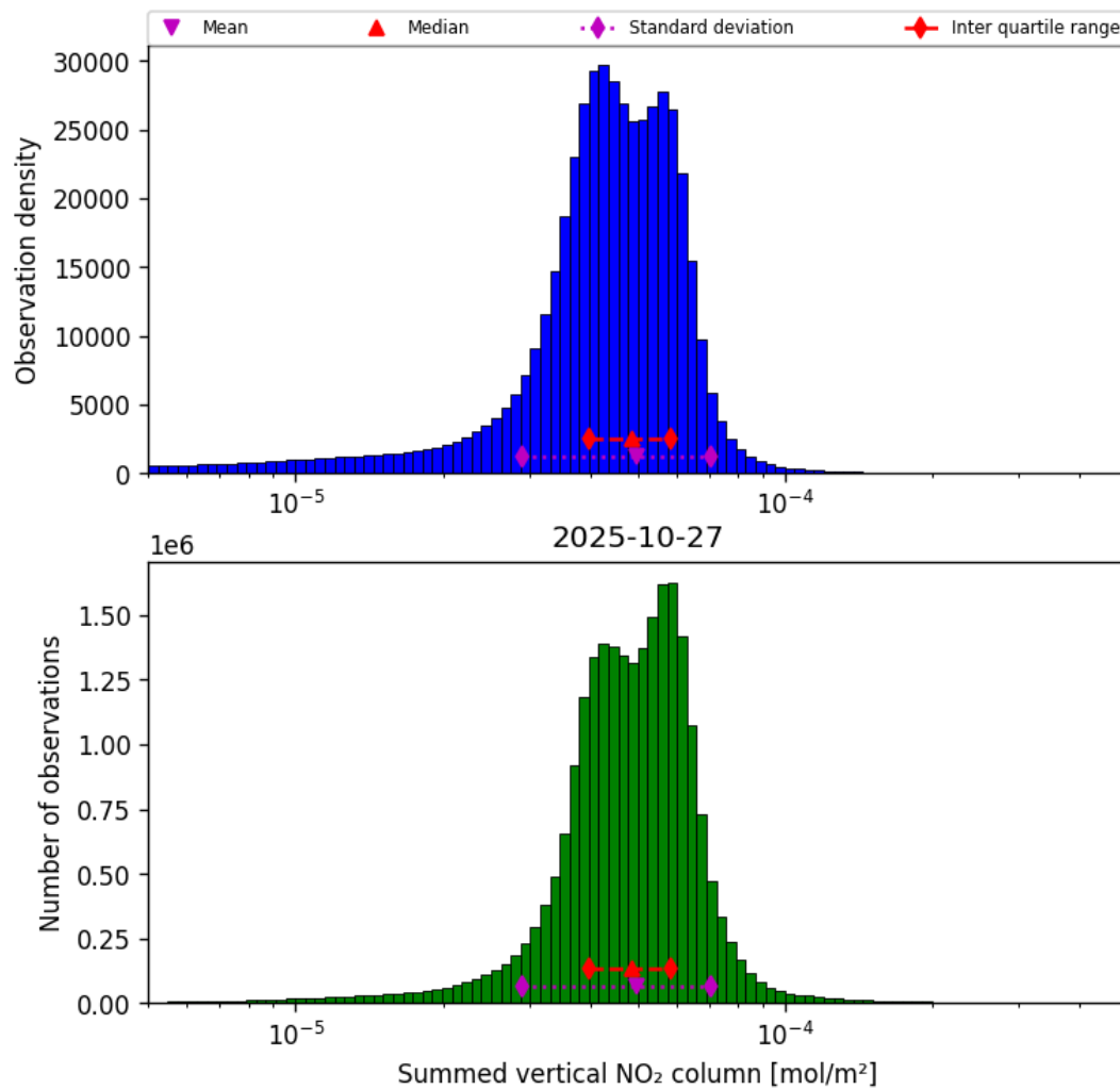
Figure 38: Histogram of “Summed vertical NO 2 column” for 2025-10-27 to 2025-10-28
