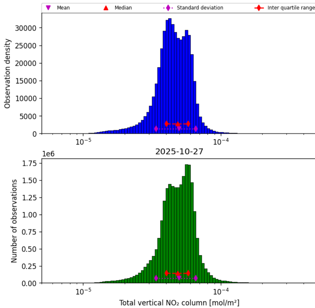
Figure 36: Histogram of "Total vertical NO 2 column" for 2025-10-27 to 2025-10-28
