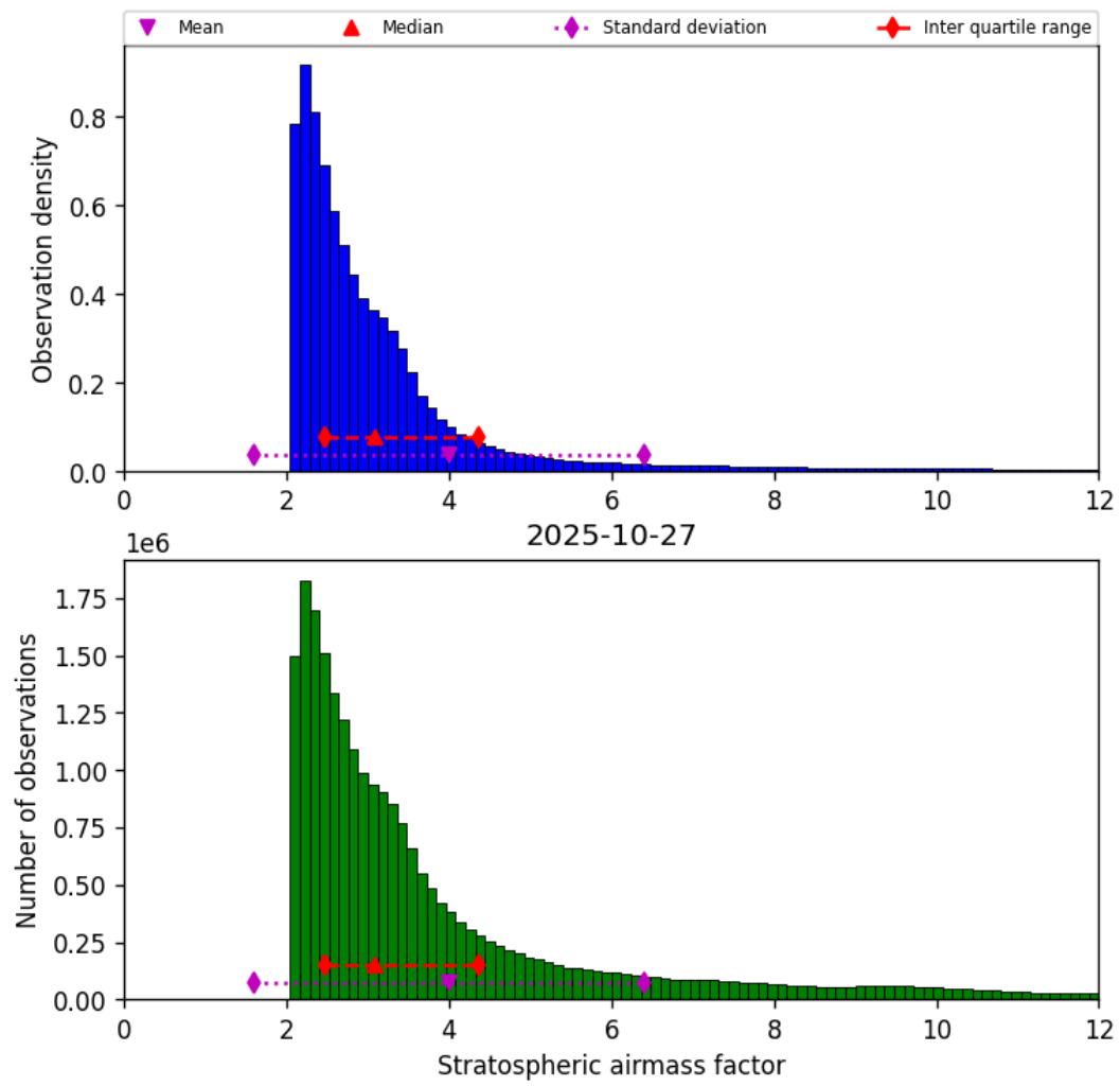
Figure 42: Histogram of “Stratospheric airmass factor” for 2025-10-27 to 2025-10-28
