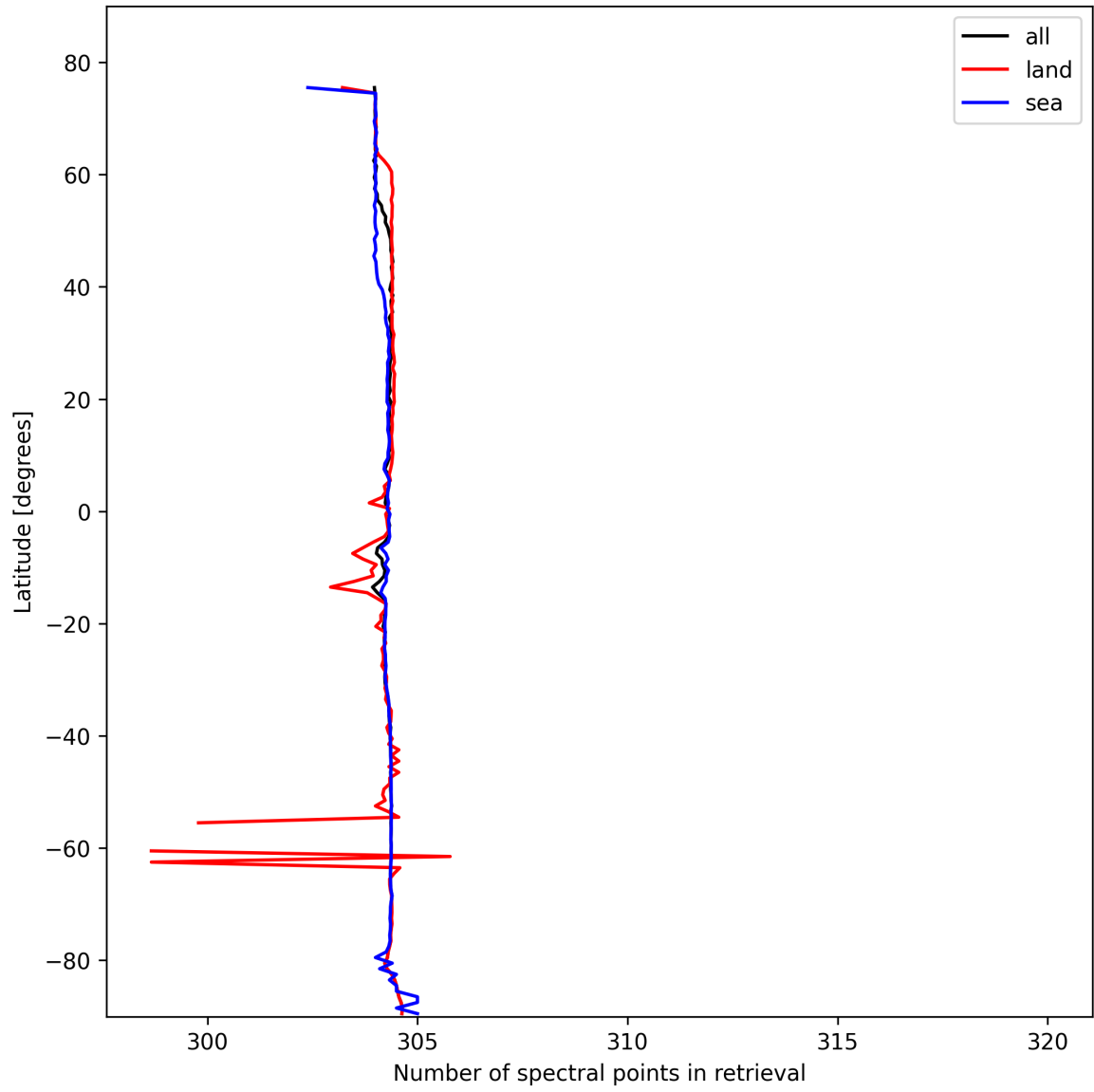
Figure 14: Zonal average of “Number of spectral points in retrieval” for 2025-10-27 to 2025-10-28.
