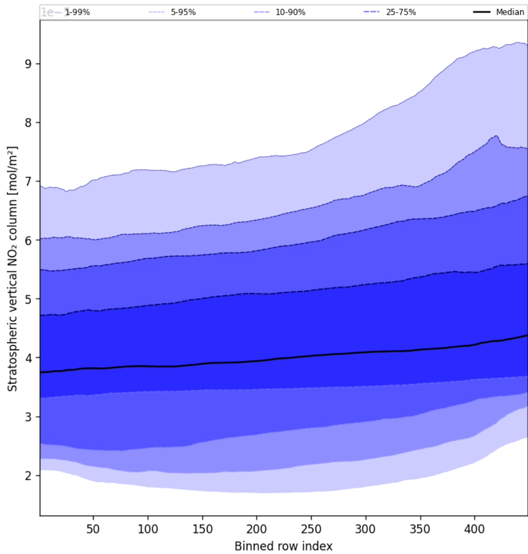
Figure 51: Along track statistics of “Stratospheric vertical NO 2 column” for 2025-10-27 to 2025-10-28
