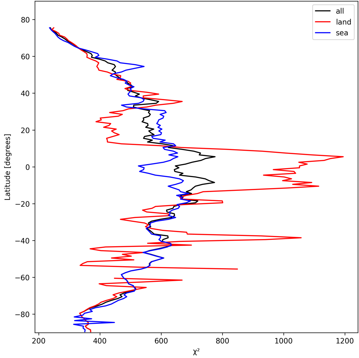
Figure 23: Zonal average of “ \chi^2 ” for 2025-10-27 to 2025-10-28.
