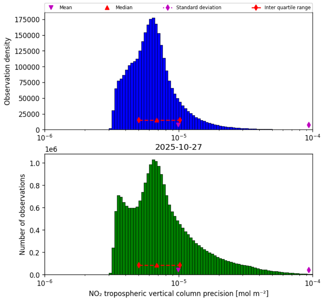
Figure 28: Histogram of “NO 2 tropospheric vertical column precision” for 2025-10-27 to 2025-10-28
