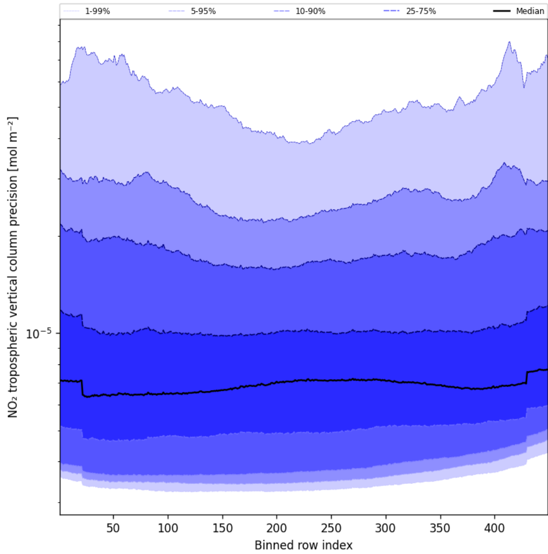
Figure 45: Along track statistics of “NO 2 tropospheric vertical column precision” for 2025-10-27 to 2025-10-28
