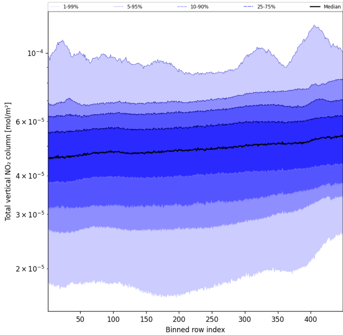
Figure 53: Along track statistics of “Total vertical NO 2 column” for 2025-10-27 to 2025-10-28
