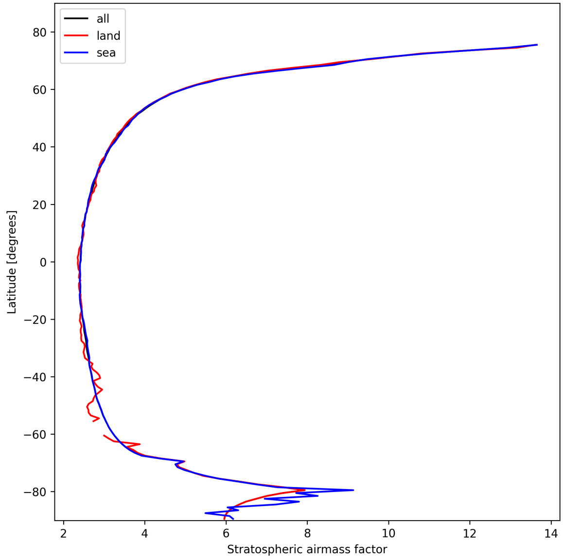
Figure 25: Zonal average of “Stratospheric air mass factor” for 2025-10-27 to 2025-10-28.
