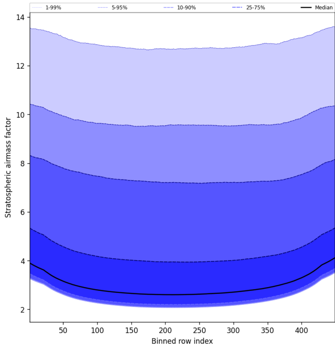
Figure 59: Along track statistics of “Stratospheric airmass factor” for 2025-10-27 to 2025-10-28
