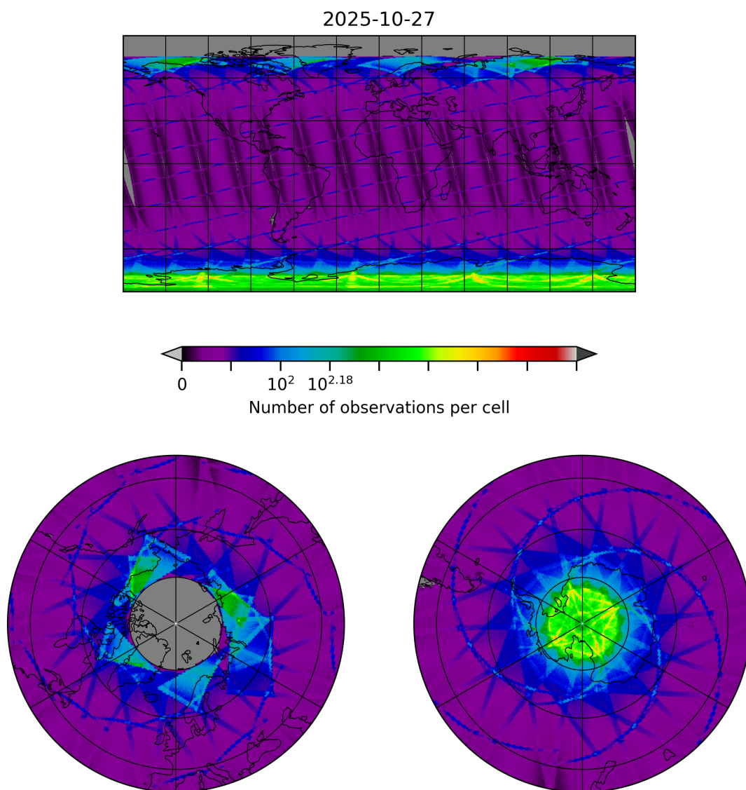
Figure 8: Map of the number of observations for 2025-10-27 to 2025-10-28
