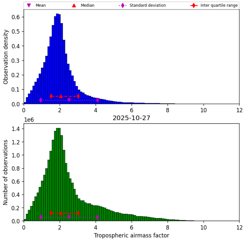
Figure 29: Histogram of “Tropospheric airmass factor” for 2025-10-27 to 2025-10-28
