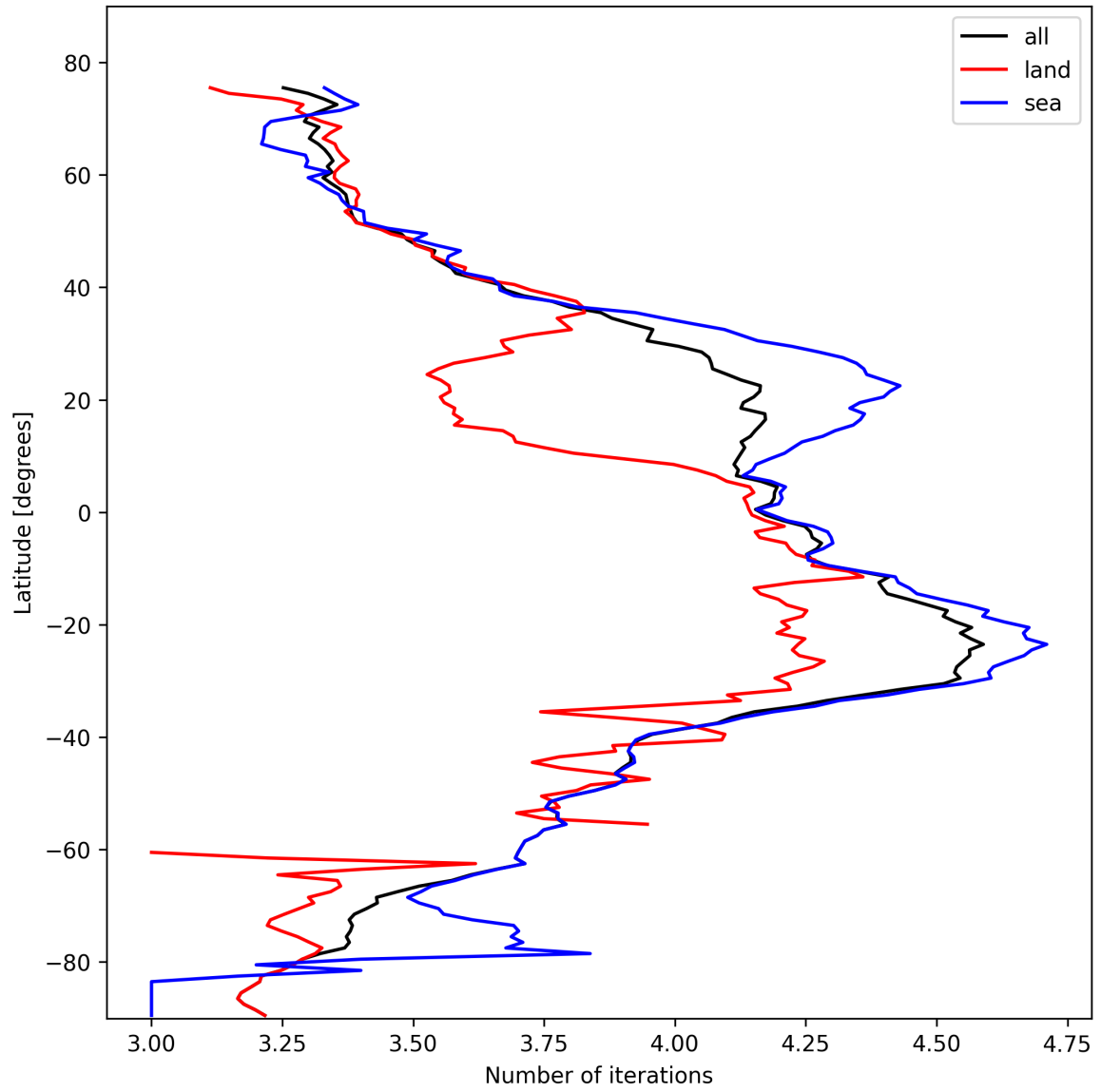
Figure 15: Zonal average of “Number of iterations” for 2025-10-27 to 2025-10-28.
