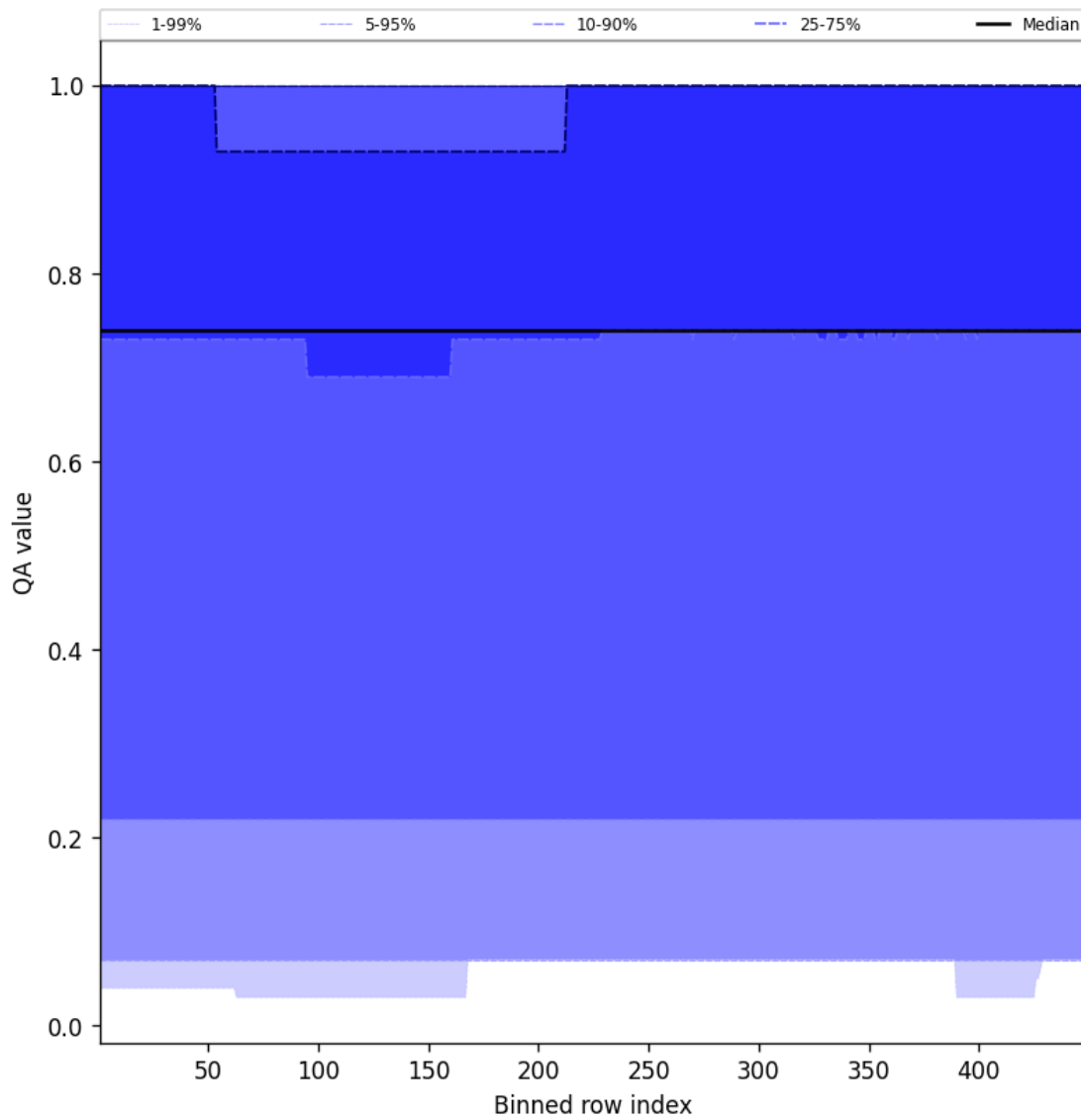
Figure 43: Along track statistics of “QA value” for 2025-10-27 to 2025-10-28
