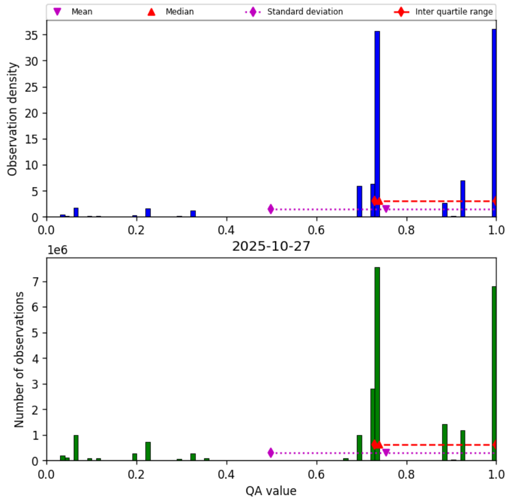
Figure 26: Histogram of “QA value” for 2025-10-27 to 2025-10-28
