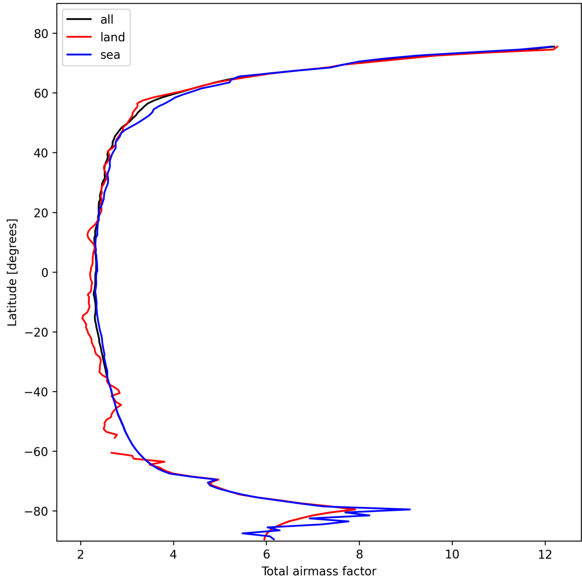
Figure 13: Zonal average of “Total airmass factor” for 2025-10-27 to 2025-10-28.
