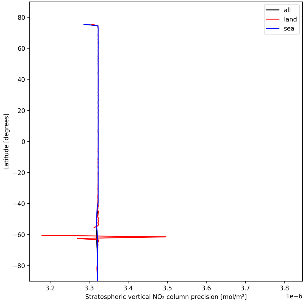
Figure 18: Zonal average of “Stratospheric vertical NO 2 column precision” for 2025-10-27 to 2025-10-28.
