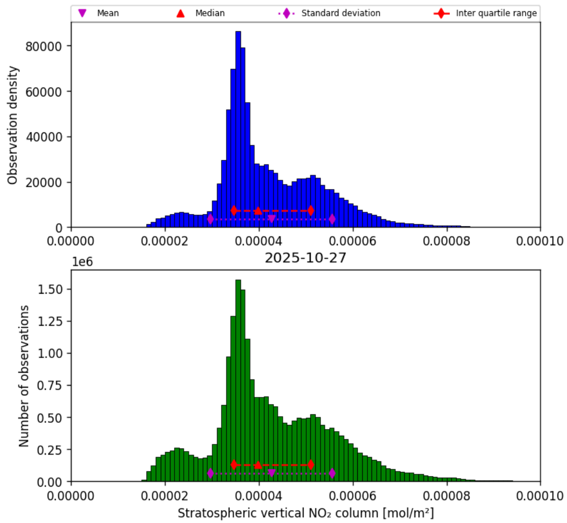
Figure 34: Histogram of “Stratospheric vertical NO 2 column” for 2025-10-27 to 2025-10-28
