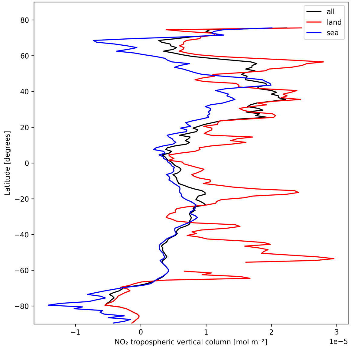
Figure 10: Zonal average of “NO 2 tropospheric vertical column” for 2025-10-27 to 2025-10-28.
