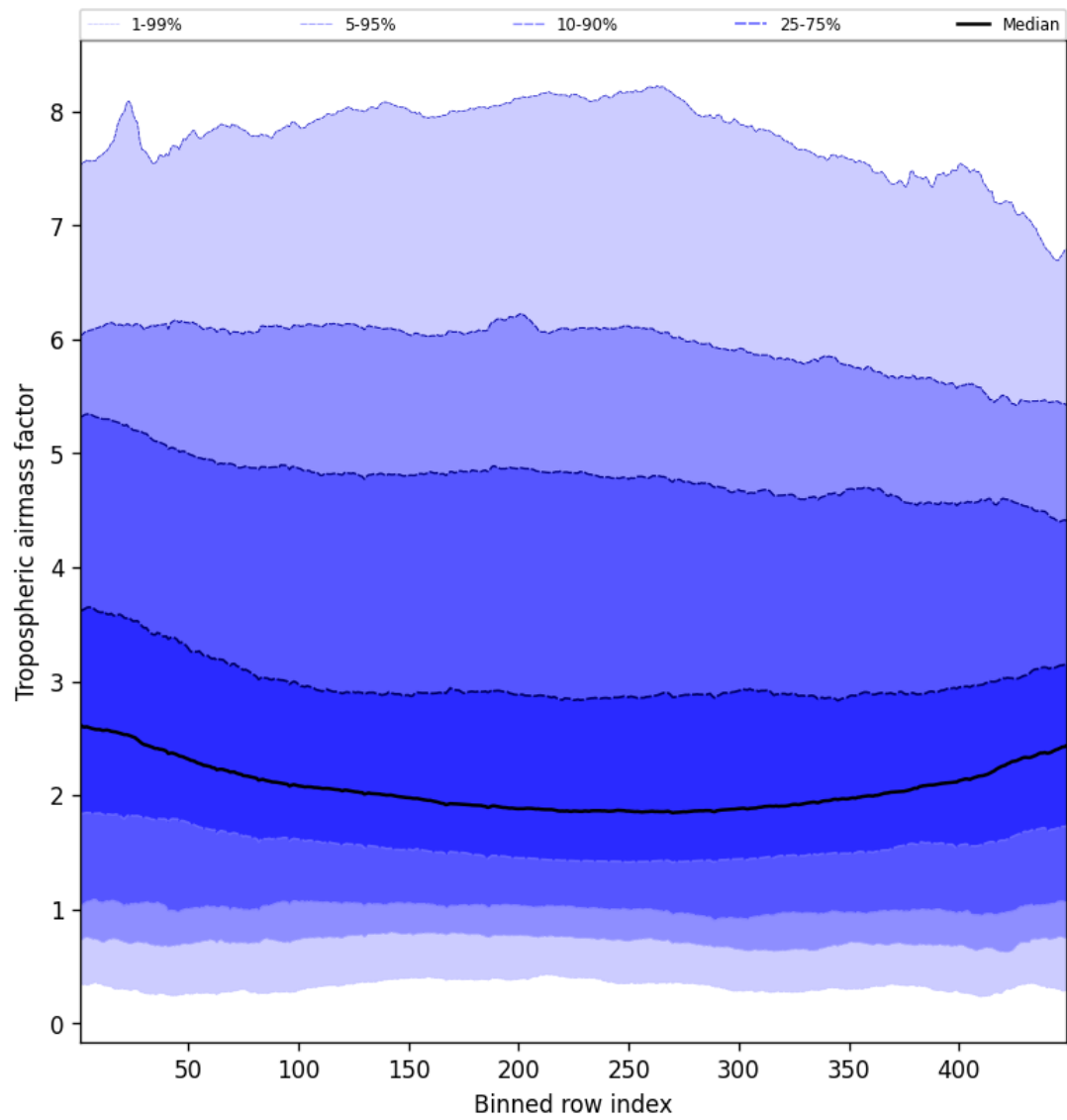
Figure 46: Along track statistics of “Tropospheric airmass factor” for 2025-10-27 to 2025-10-28
