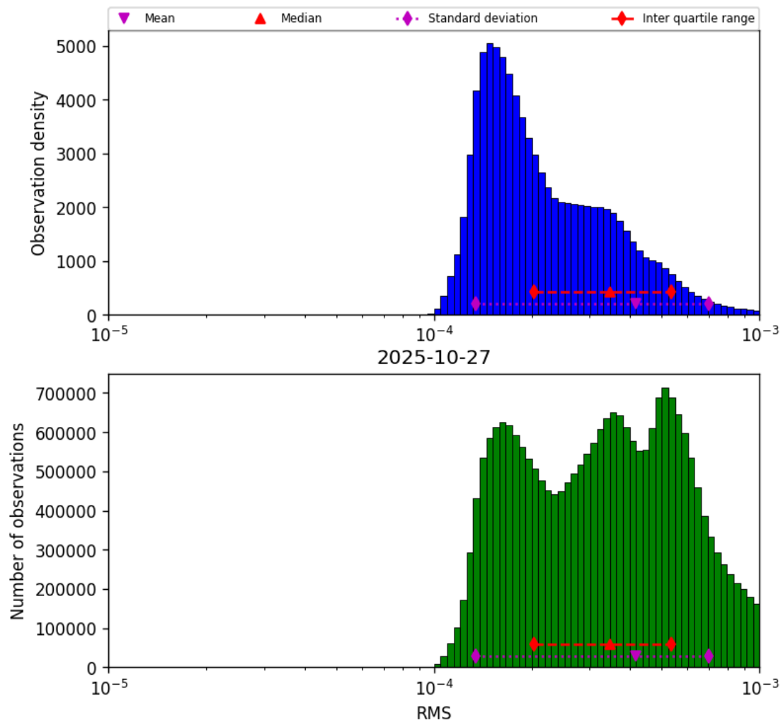
Figure 41: Histogram of “RMS” for 2025-10-27 to 2025-10-28
