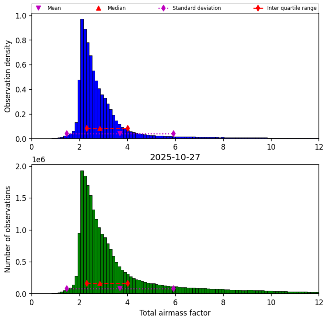
Figure 30: Histogram of “Total airmass factor” for 2025-10-27 to 2025-10-28
