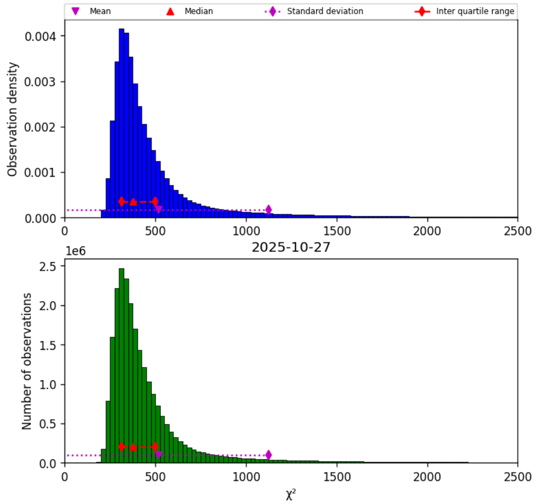
Figure 40: Histogram of “ \chi^2 ” for 2025-10-27 to 2025-10-28
