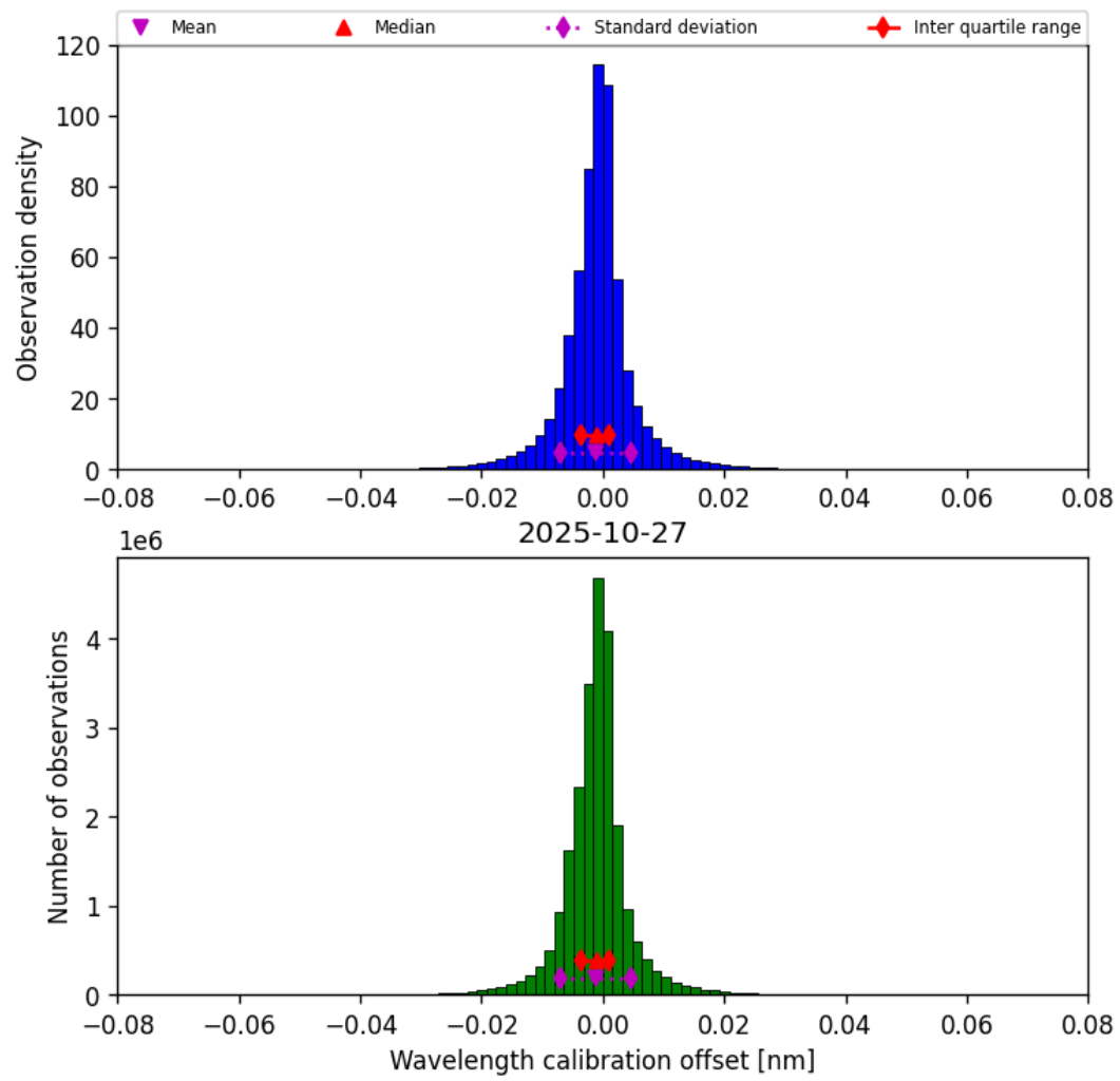
Figure 33: Histogram of “Wavelength calibration offset” for 2025-10-27 to 2025-10-28
