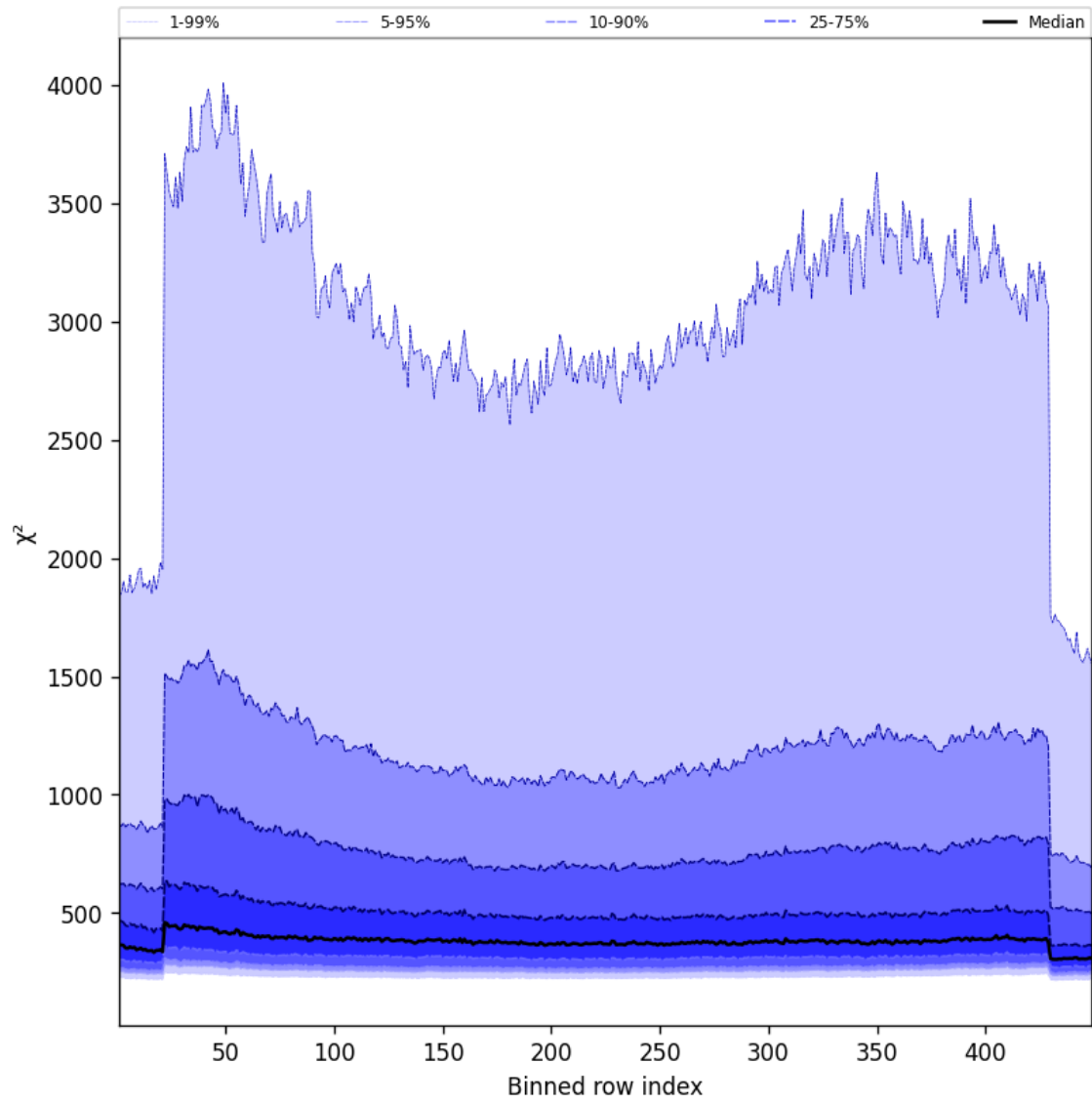
Figure 57: Along track statistics of “ \chi^2 ” for 2025-10-27 to 2025-10-28
