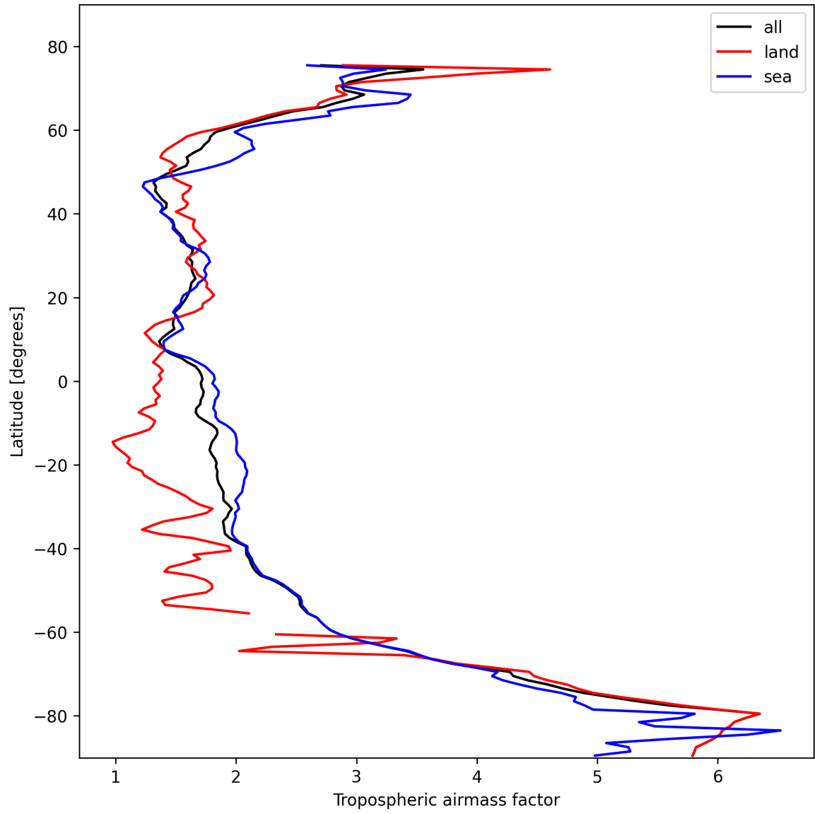
Figure 12: Zonal average of “Tropospheric airmass factor” for 2025-10-27 to 2025-10-28.
