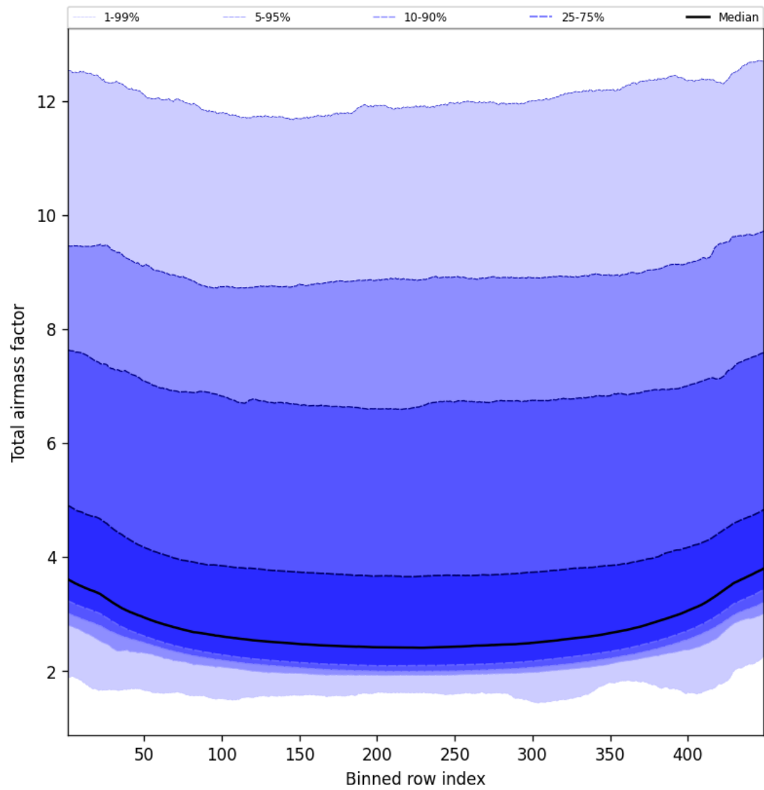
Figure 47: Along track statistics of “Total airmass factor” for 2025-10-27 to 2025-10-28
