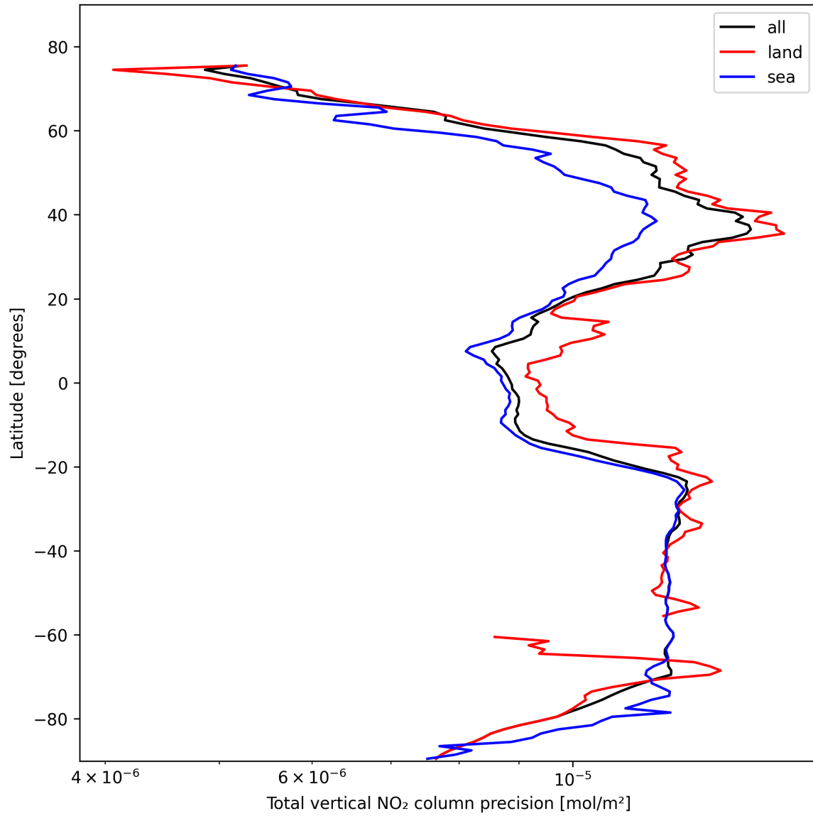
Figure 20: Zonal average of “Total vertical NO 2 column precision” for 2025-10-27 to 2025-10-28.
