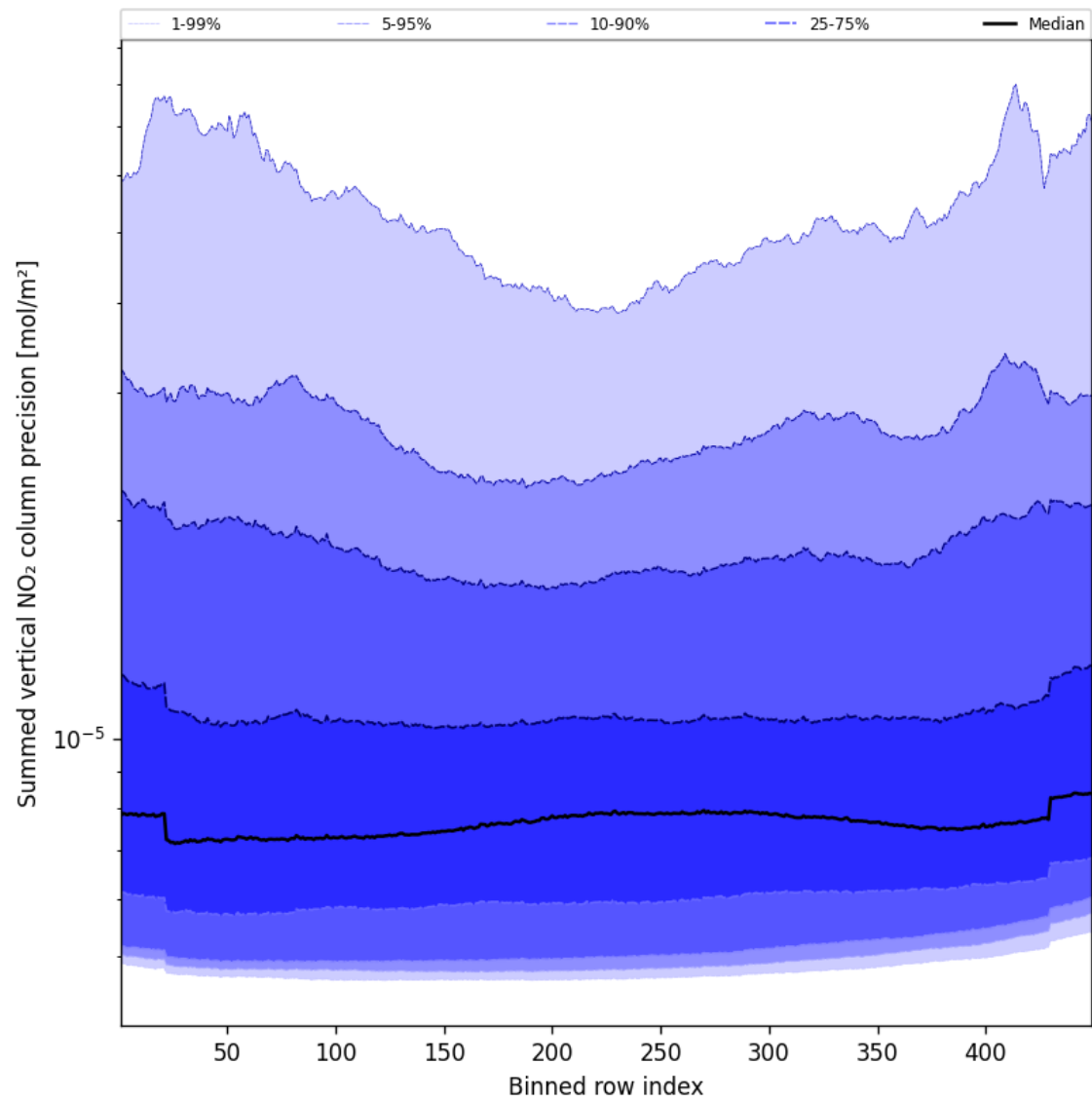
Figure 56: Along track statistics of “Summed vertical NO 2 column precision” for 2025-10-27 to 2025-10-28
