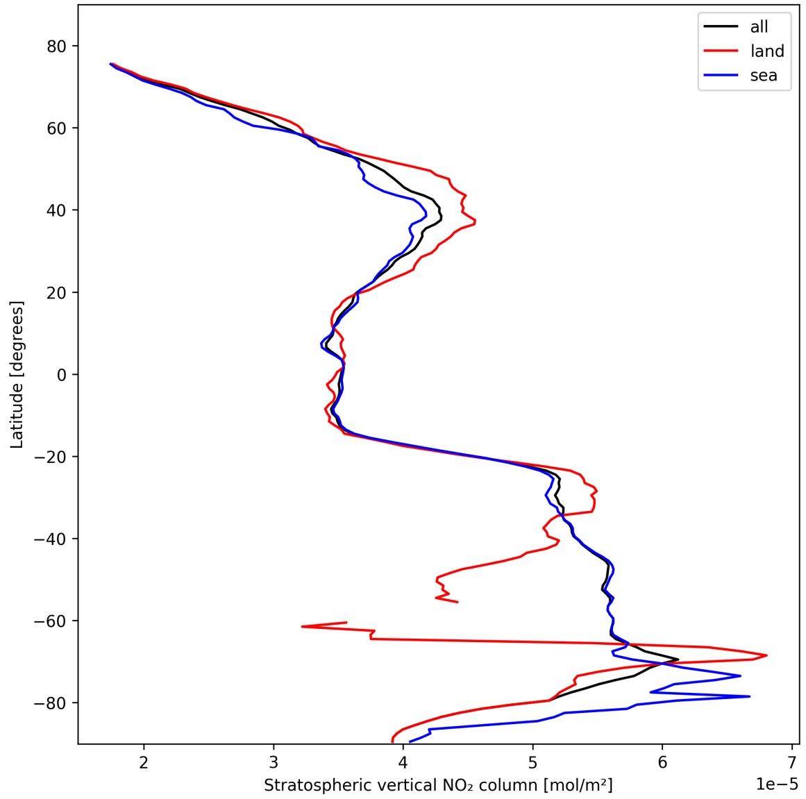
Figure 17: Zonal average of “Stratospheric vertical NO 2 column” for 2025-10-27 to 2025-10-28.
