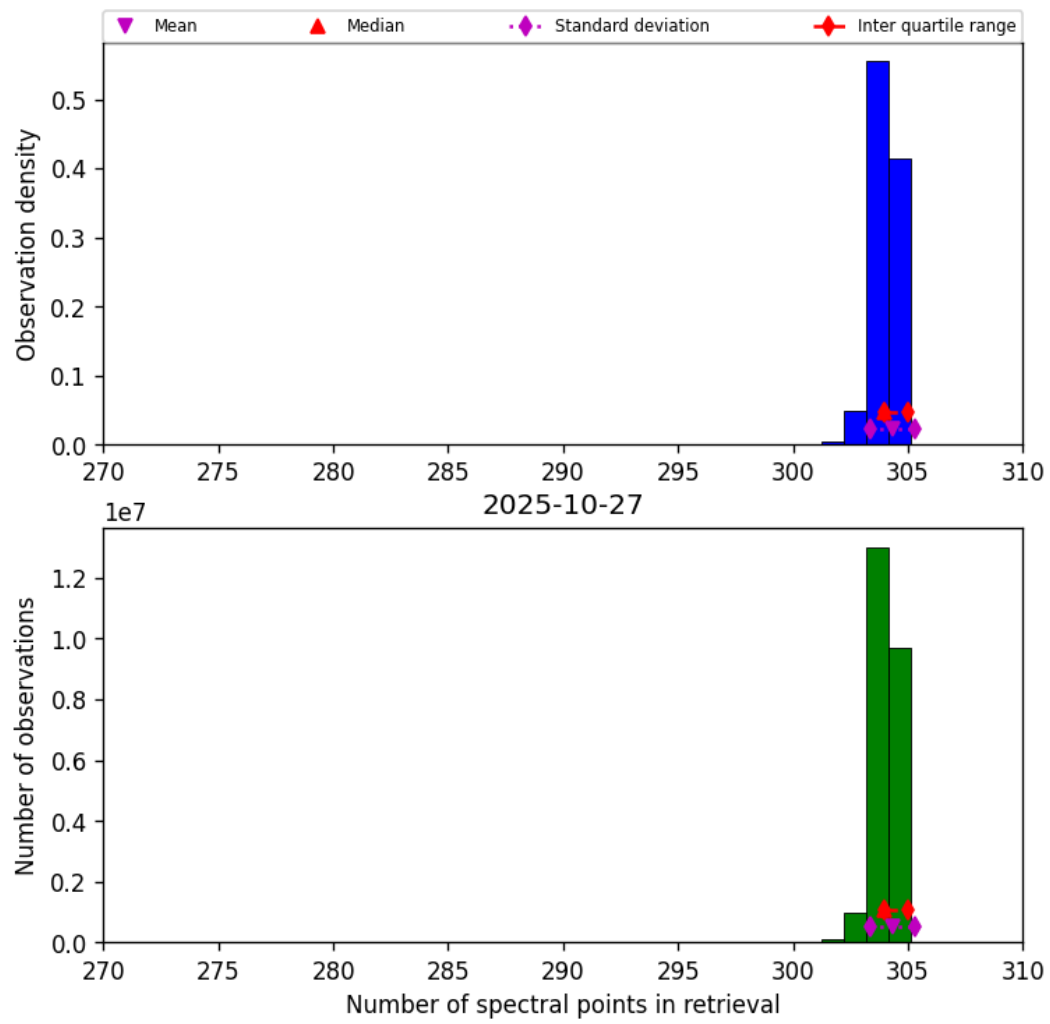
Figure 31: Histogram of “Number of spectral points in retrieval” for 2025-10-27 to 2025-10-28
