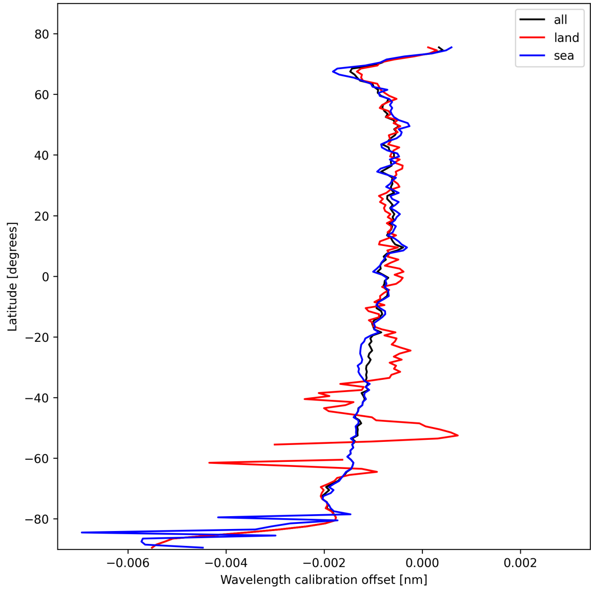
Figure 16: Zonal average of “Wavelength calibration offset” for 2025-10-27 to 2025-10-28.
