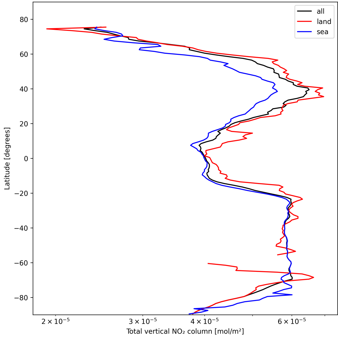
Figure 19: Zonal average of “Total vertical NO 2 column” for 2025-10-27 to 2025-10-28.
