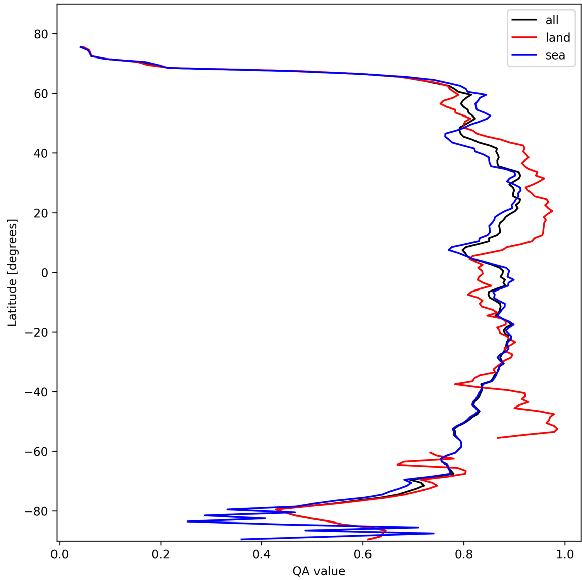
Figure 9: Zonal average of “QA value” for 2025-10-27 to 2025-10-28.
