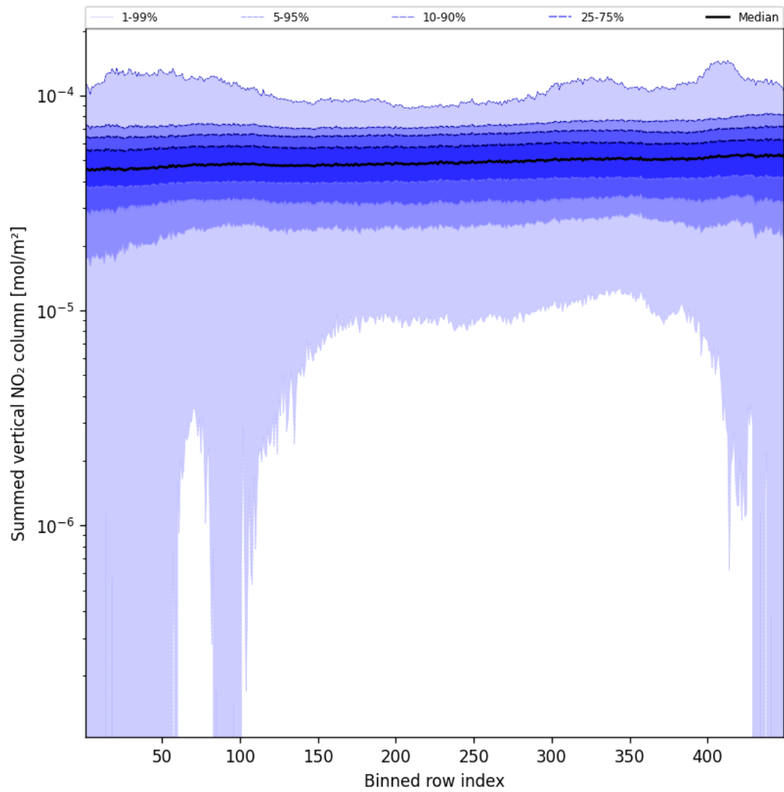
Figure 55: Along track statistics of “Summed vertical NO 2 column” for 2025-10-27 to 2025-10-28
