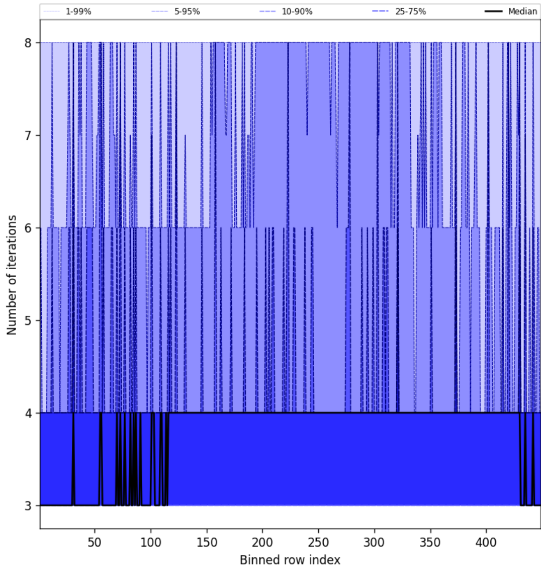
Figure 49: Along track statistics of “Number of iterations” for 2025-10-27 to 2025-10-28
