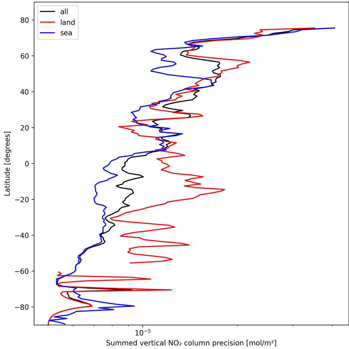
Figure 22: Zonal average of “Summed vertical NO 2 column precision” for 2025-10-27 to 2025-10-28.
