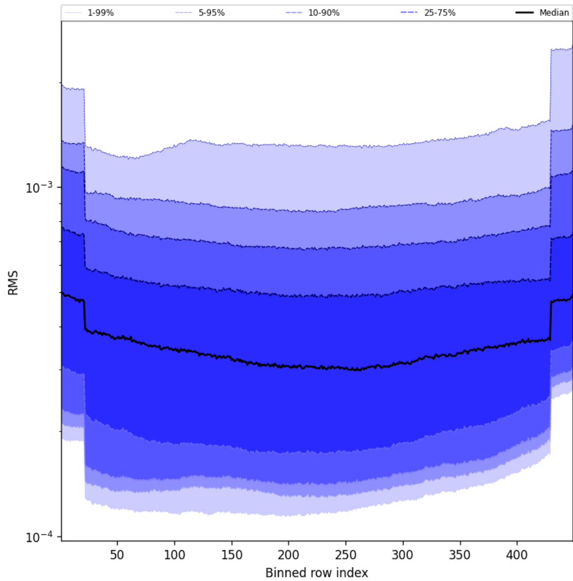
Figure 58: Along track statistics of “RMS” for 2025-10-28 to 2025-10-29
