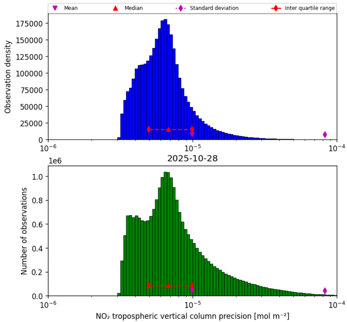
Figure 28: Histogram of “NO 2 tropospheric vertical column precision” for 2025-10-28 to 2025-10-29
