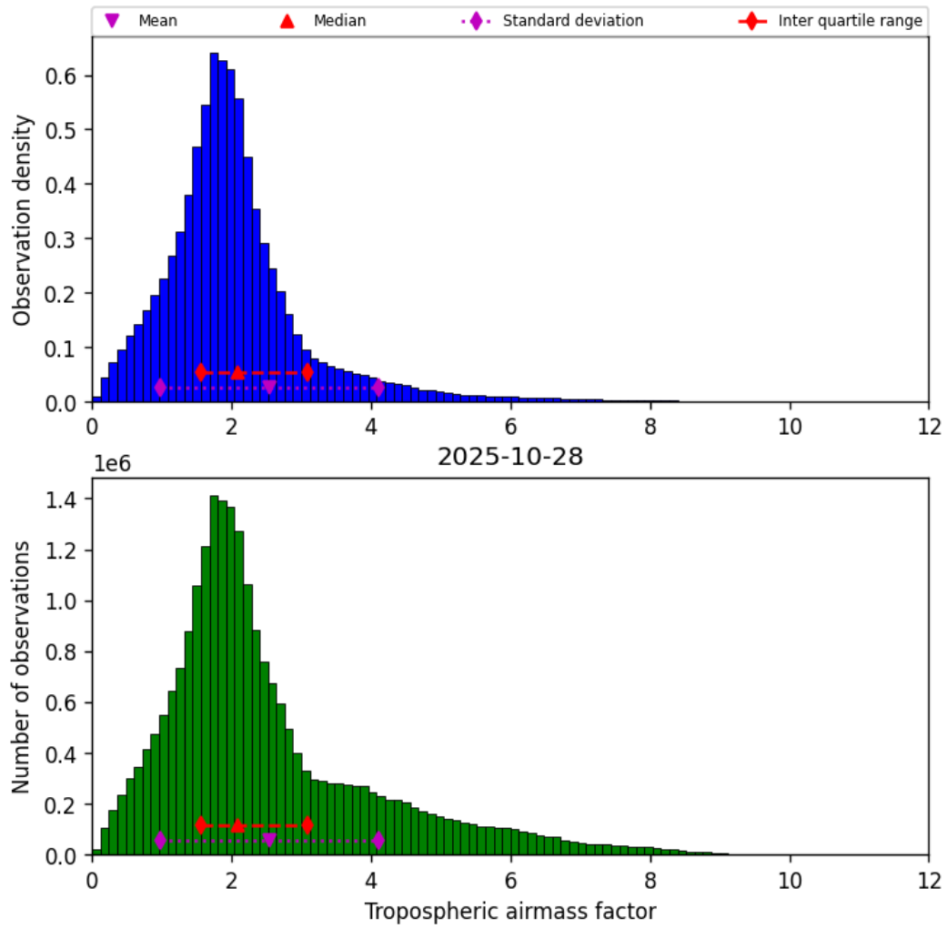
Figure 29: Histogram of “Tropospheric airmass factor” for 2025-10-28 to 2025-10-29
