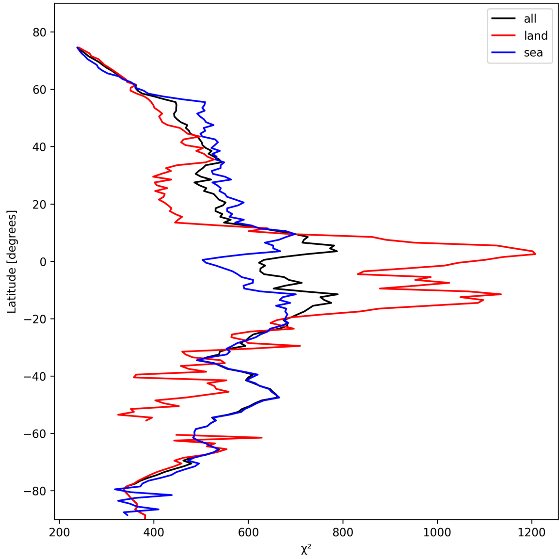
Figure 23: Zonal average of “ \chi^2 ” for 2025-10-28 to 2025-10-29.
