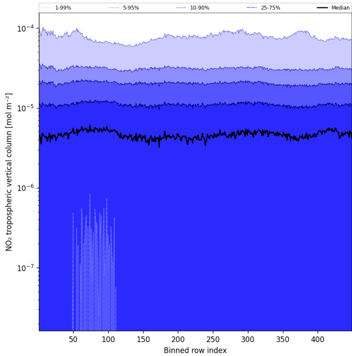
Figure 44: Along track statistics of “NO 2 tropospheric vertical column” for 2025-10-28 to 2025-10-29
