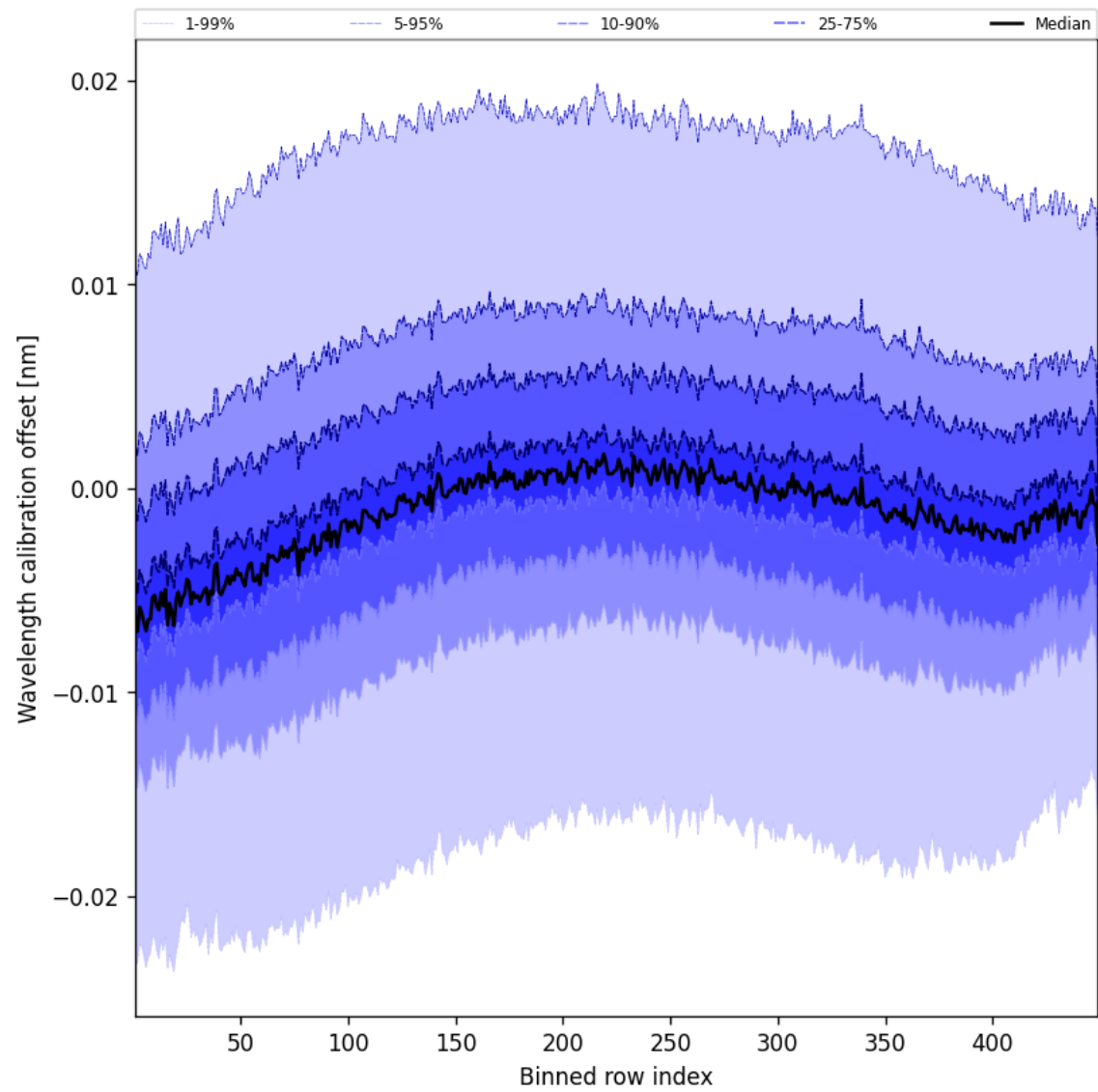
Figure 50: Along track statistics of “Wavelength calibration offset” for 2025-10-28 to 2025-10-29
