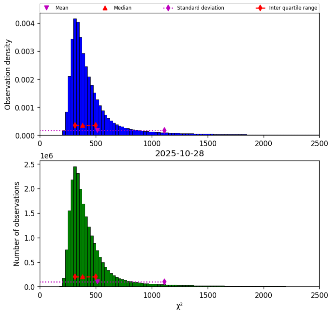
Figure 40: Histogram of “ \chi^2 ” for 2025-10-28 to 2025-10-29
