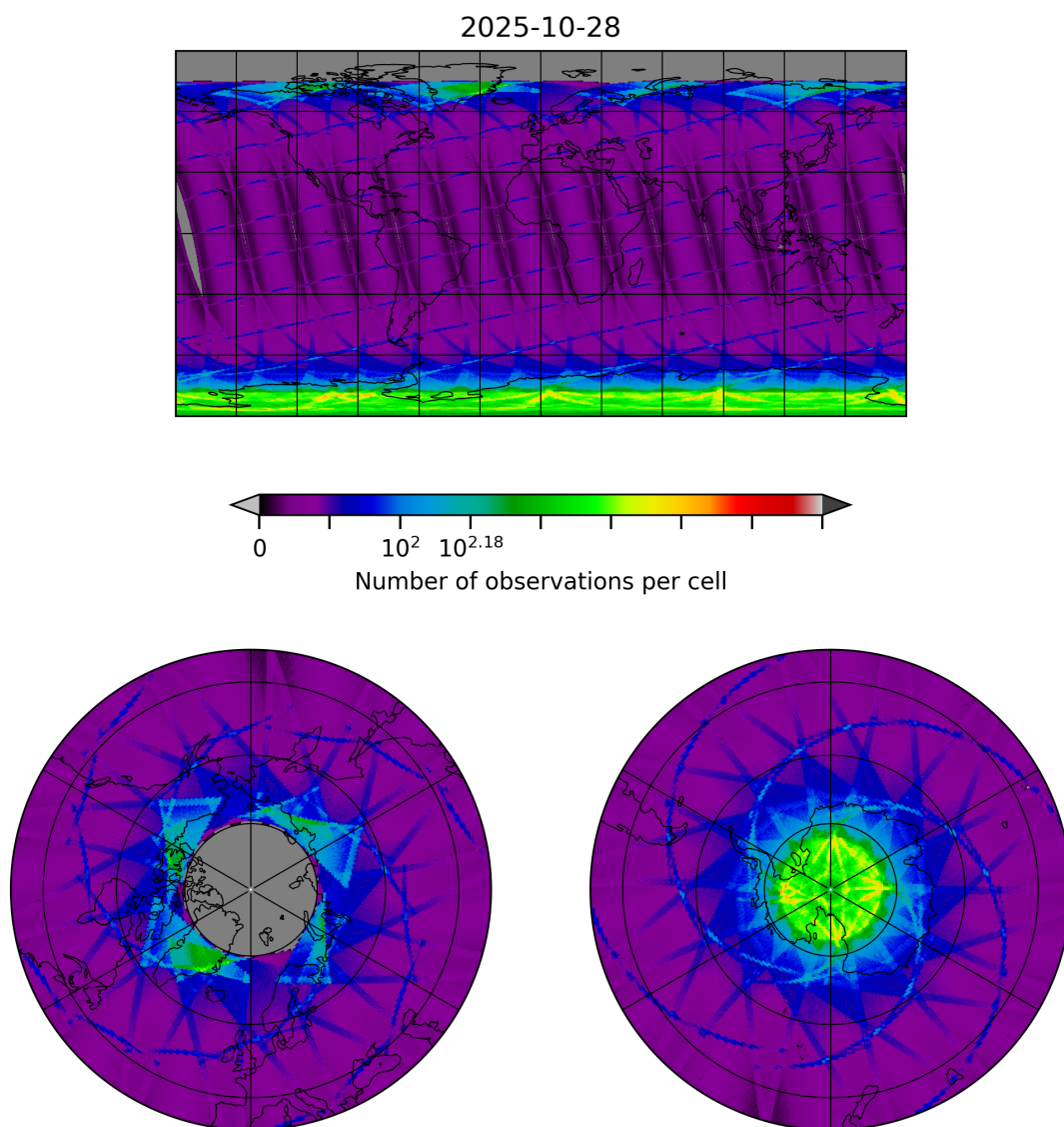
Figure 8: Map of the number of observations for 2025-10-28 to 2025-10-29
