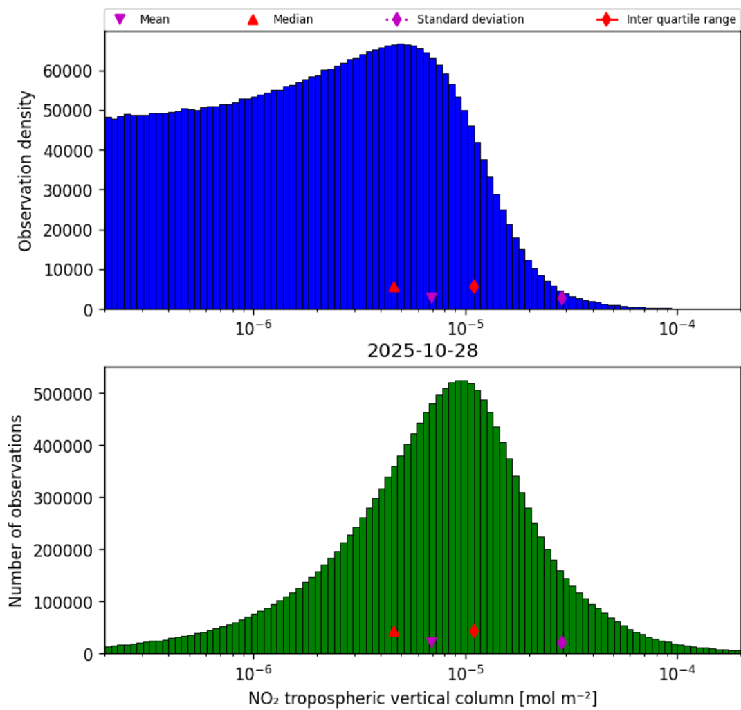
Figure 27: Histogram of “NO 2 tropospheric vertical column” for 2025-10-28 to 2025-10-29
