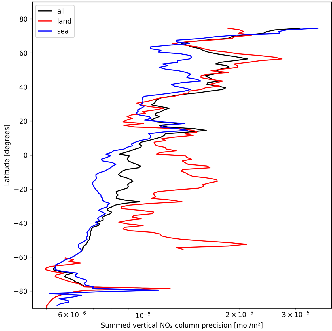
Figure 22: Zonal average of “Summed vertical NO 2 column precision” for 2025-10-28 to 2025-10-29.
