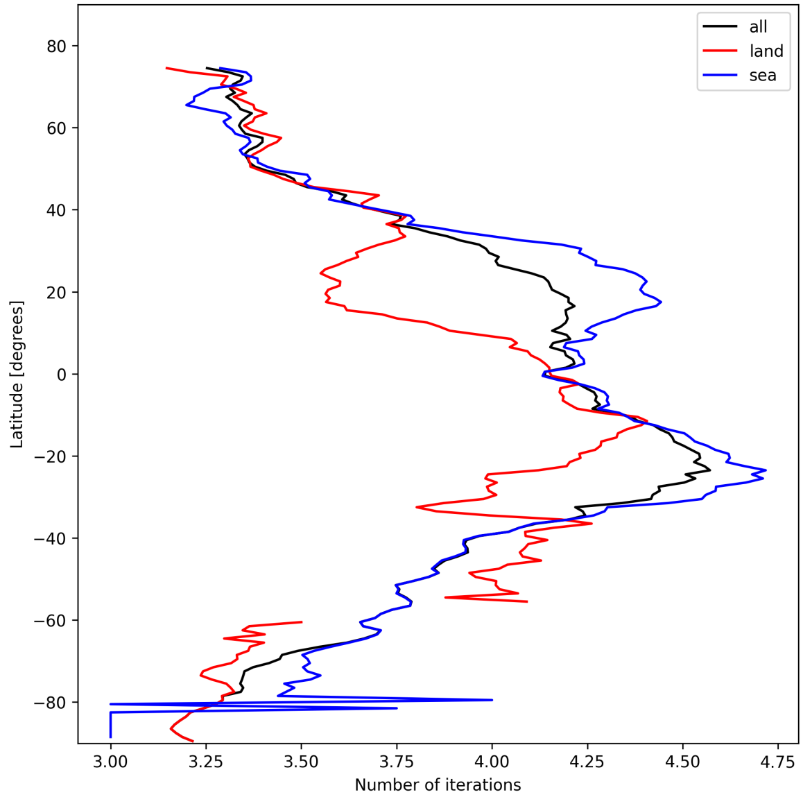
Figure 15: Zonal average of “Number of iterations” for 2025-10-28 to 2025-10-29.
