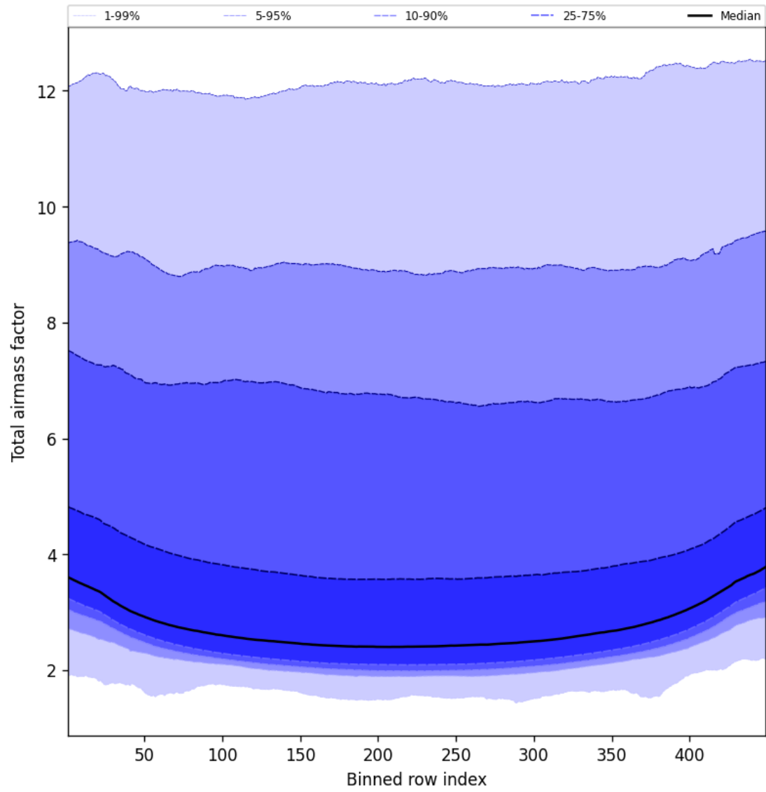
Figure 47: Along track statistics of “Total airmass factor” for 2025-10-28 to 2025-10-29
