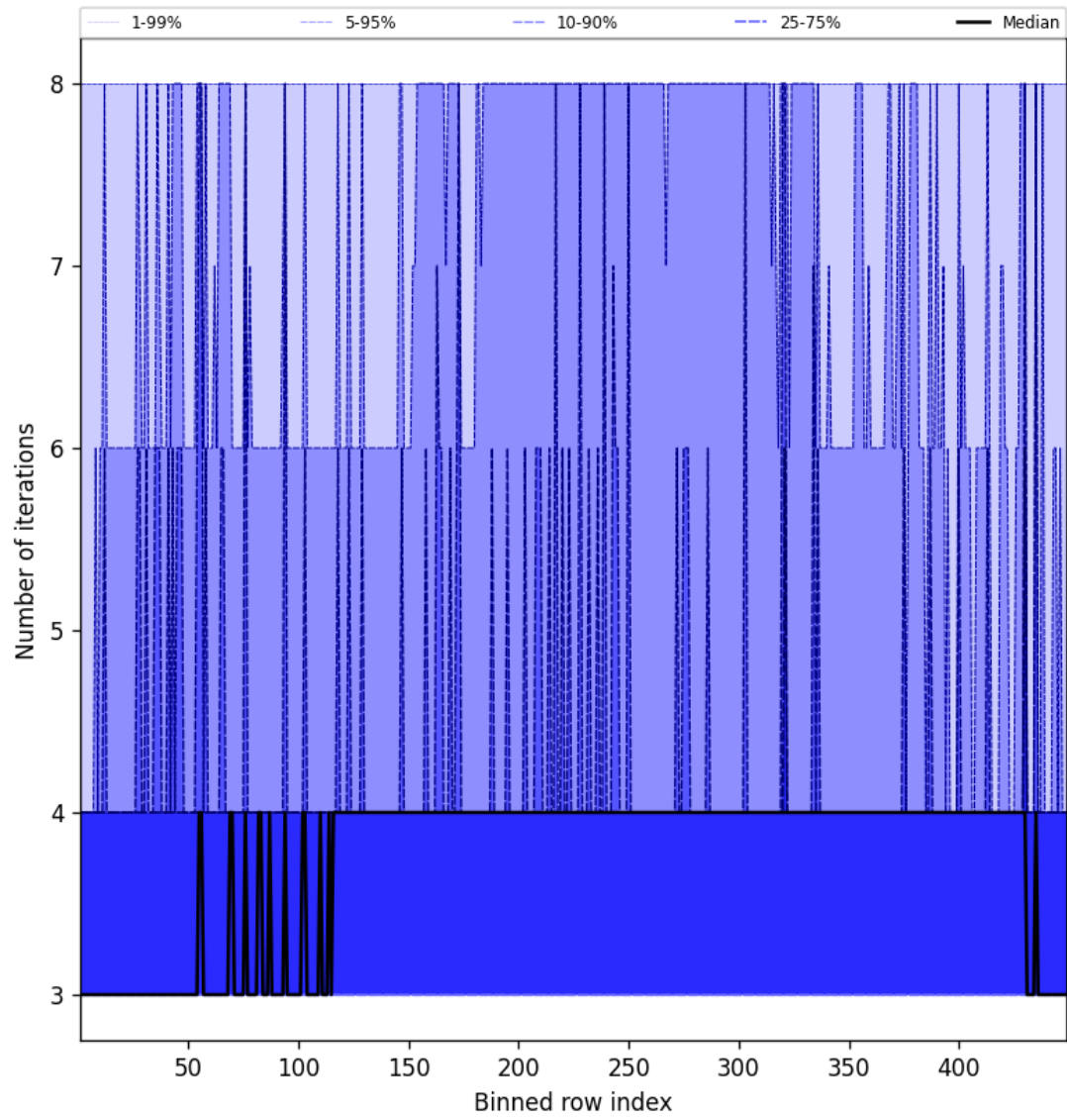
Figure 49: Along track statistics of “Number of iterations” for 2025-10-28 to 2025-10-29
