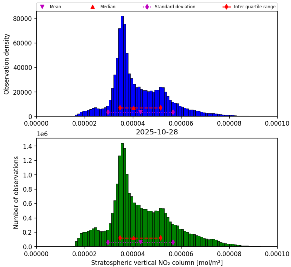
Figure 34: Histogram of “Stratospheric vertical NO 2 column” for 2025-10-28 to 2025-10-29
