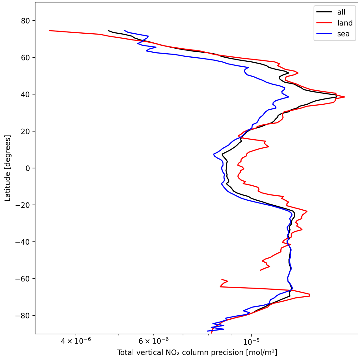
Figure 20: Zonal average of “Total vertical NO 2 column precision” for 2025-10-28 to 2025-10-29.
