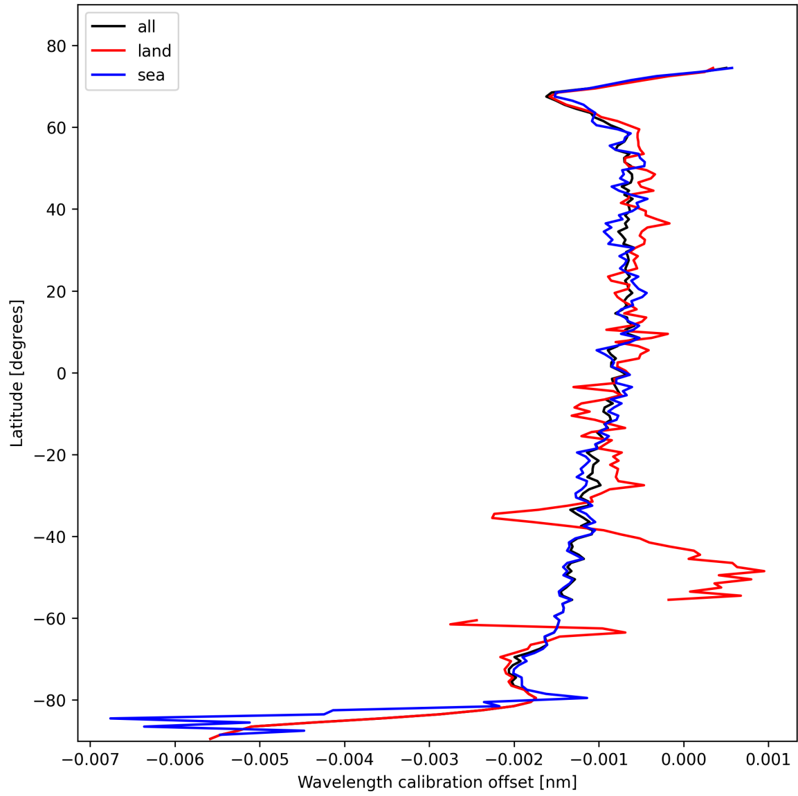
Figure 16: Zonal average of “Wavelength calibration offset” for 2025-10-28 to 2025-10-29.
