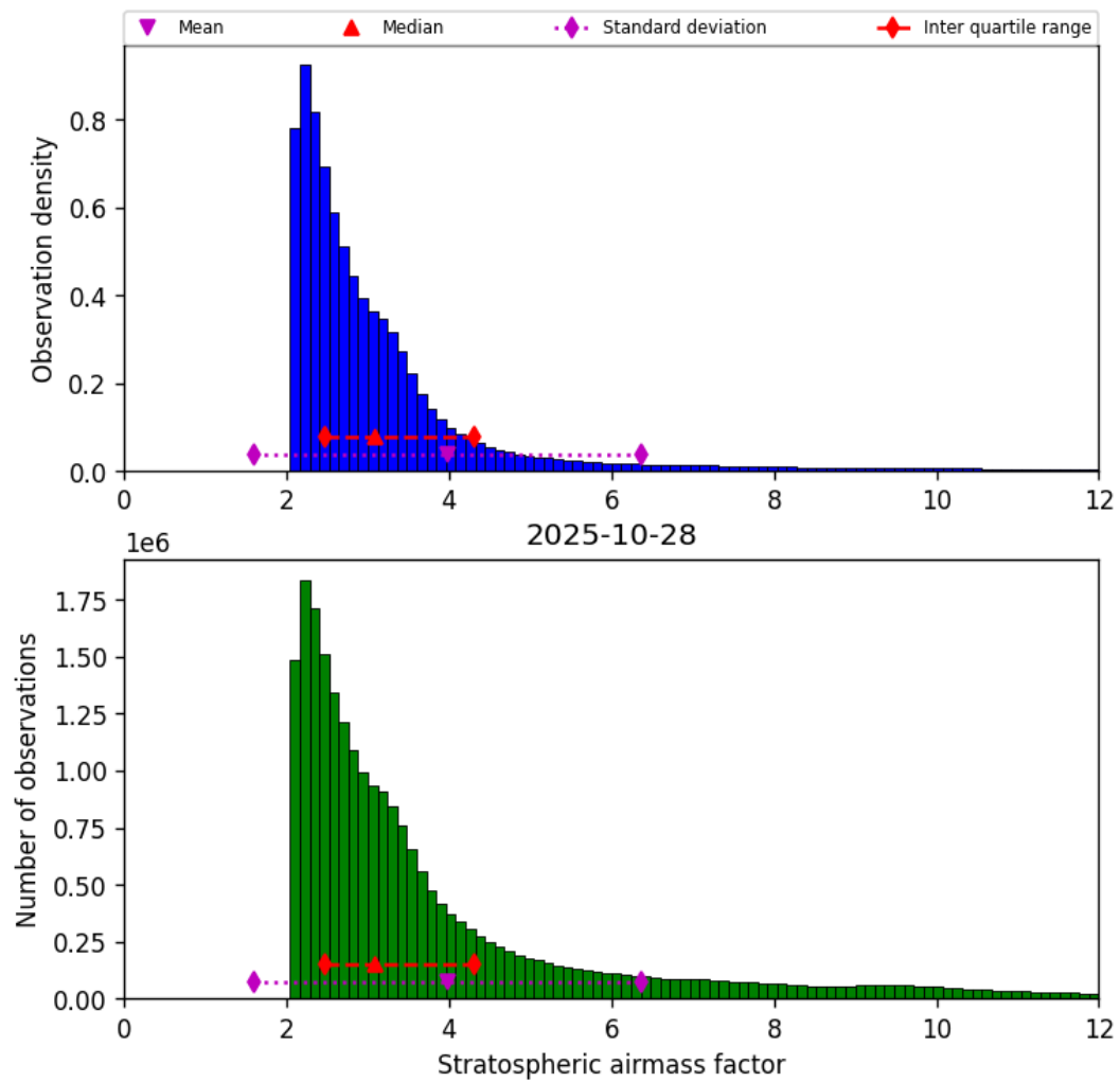
Figure 42: Histogram of “Stratospheric airmass factor” for 2025-10-28 to 2025-10-29
