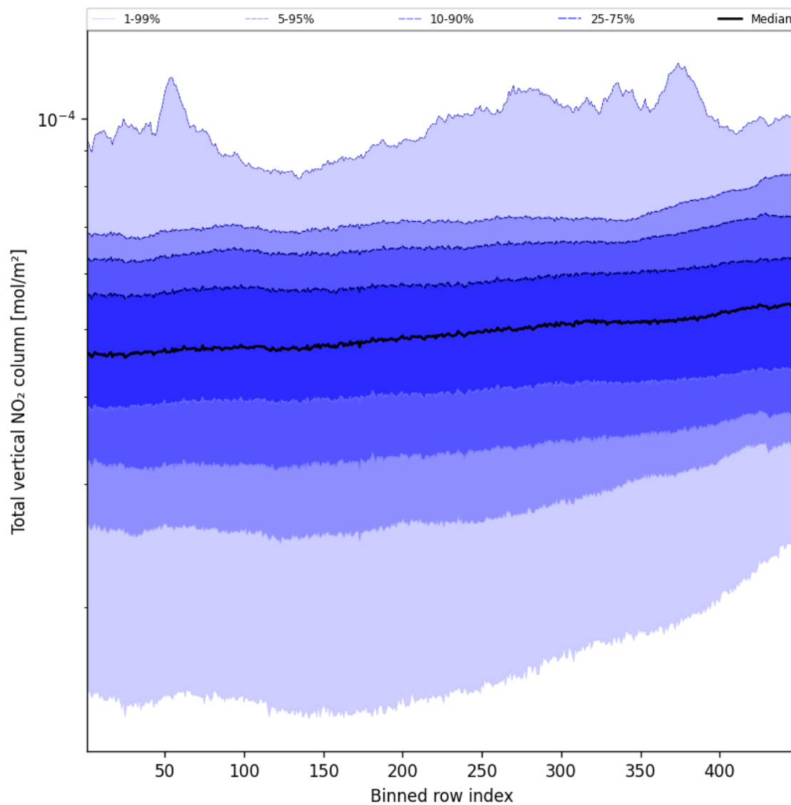
Figure 53: Along track statistics of “Total vertical NO 2 column” for 2025-10-28 to 2025-10-29
