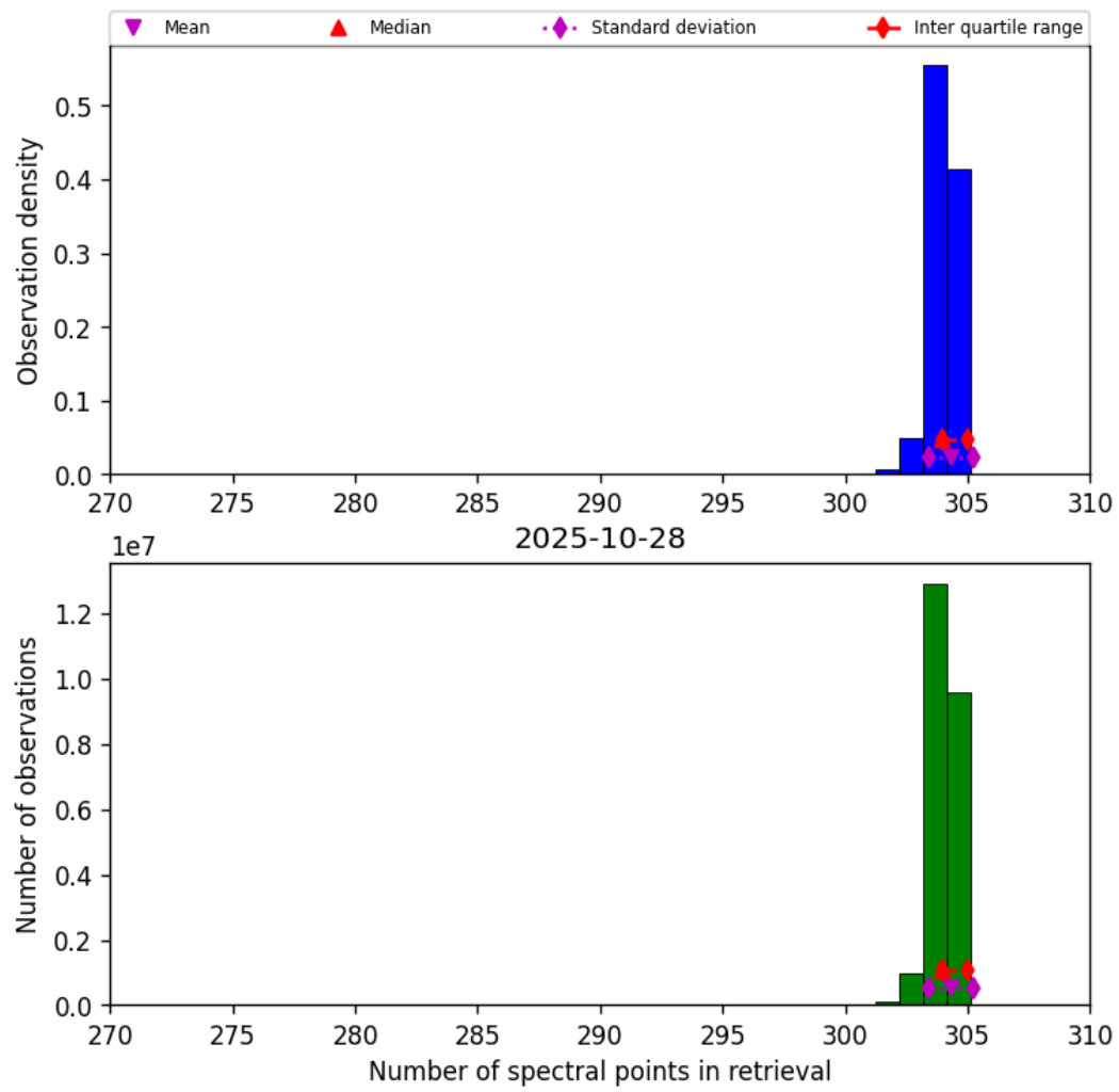
Figure 31: Histogram of “Number of spectral points in retrieval” for 2025-10-28 to 2025-10-29
