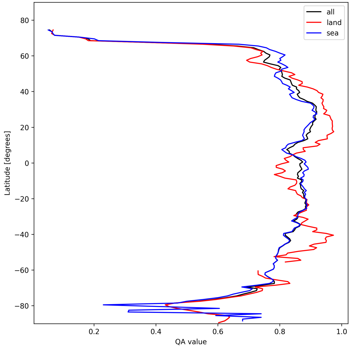
Figure 9: Zonal average of “QA value” for 2025-10-28 to 2025-10-29.
