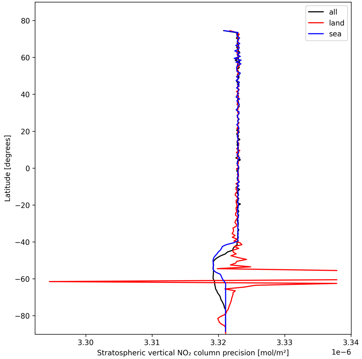
Figure 18: Zonal average of “Stratospheric vertical NO 2 column precision” for 2025-10-28 to 2025-10-29.
