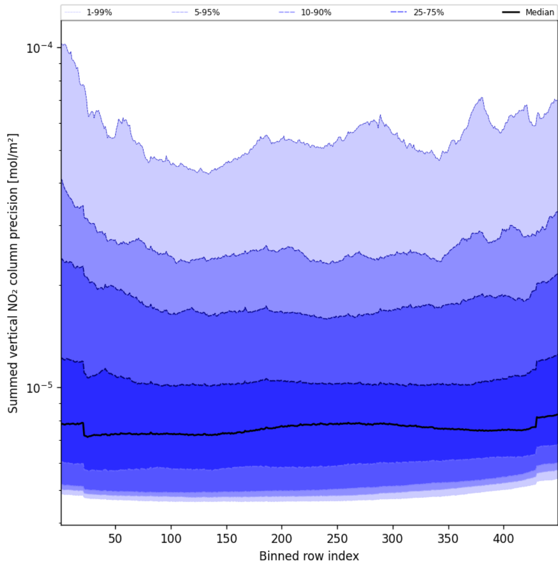
Figure 56: Along track statistics of “Summed vertical NO 2 column precision” for 2025-10-28 to 2025-10-29
