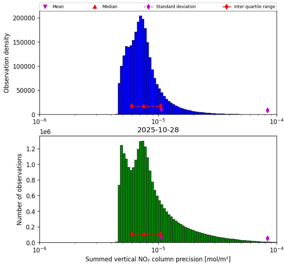
Figure 39: Histogram of “Summed vertical NO 2 column precision” for 2025-10-28 to 2025-10-29
