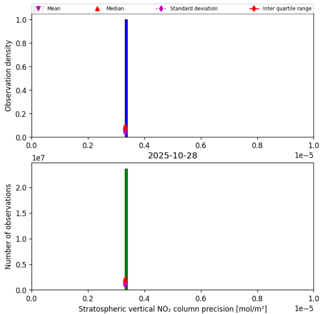
Figure 35: Histogram of “Stratospheric vertical NO 2 column precision” for 2025-10-28 to 2025-10-29
