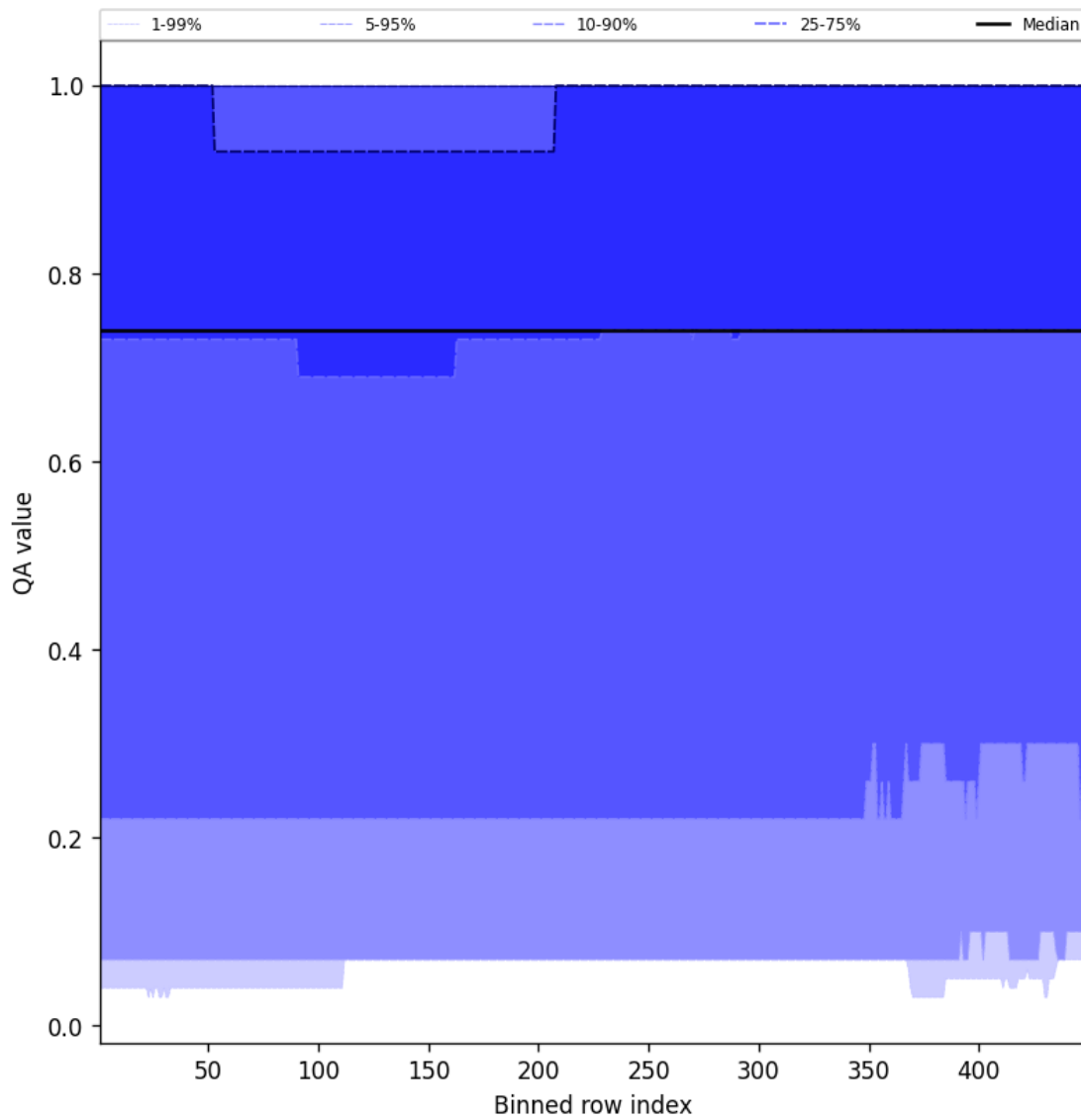
Figure 43: Along track statistics of “QA value” for 2025-10-28 to 2025-10-29
