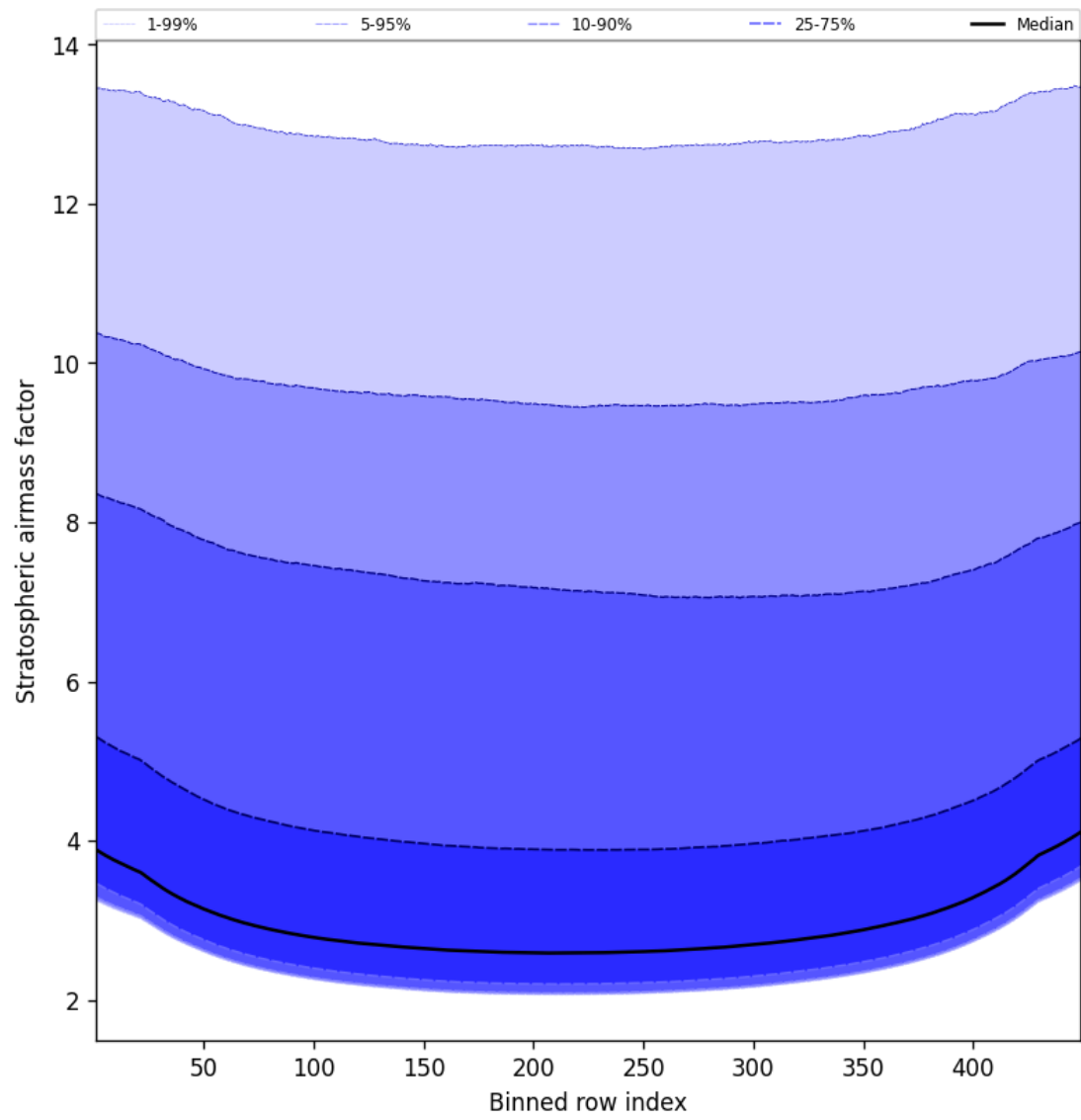
Figure 59: Along track statistics of “Stratospheric airmass factor” for 2025-10-28 to 2025-10-29
