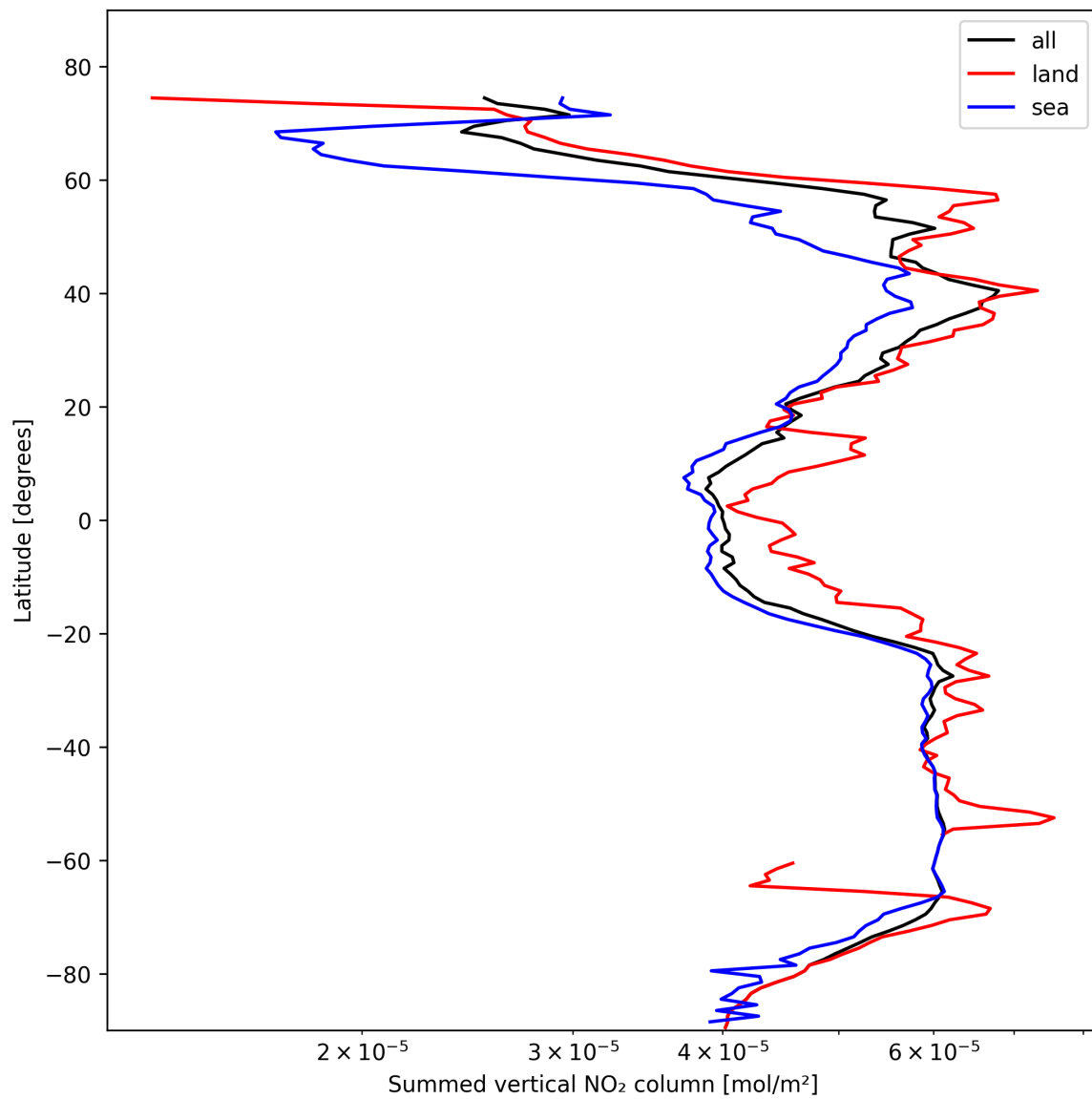
Figure 21: Zonal average of “Summed vertical NO 2 column” for 2025-10-28 to 2025-10-29.
