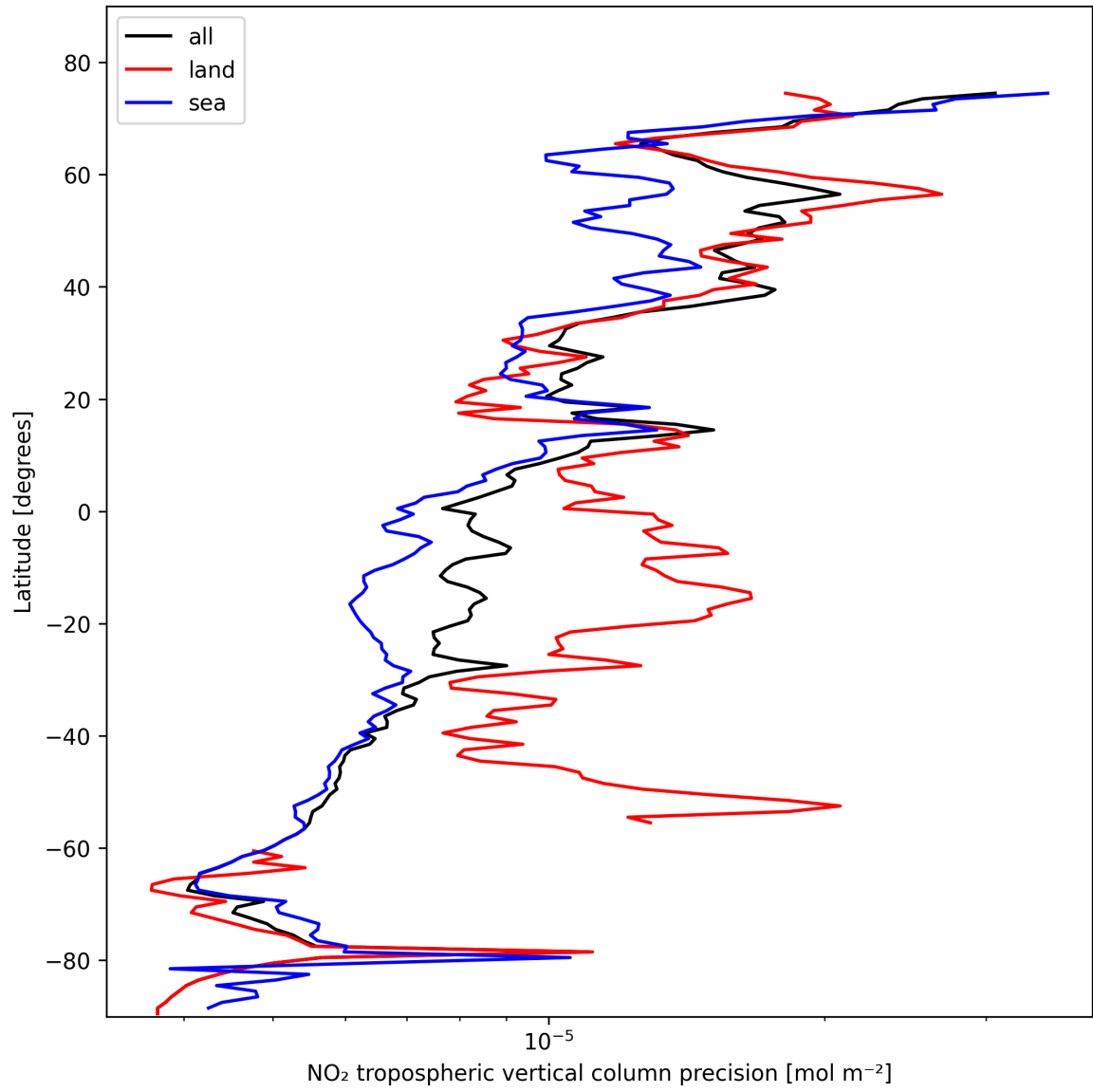
Figure 11: Zonal average of “NO 2 tropospheric vertical column precision” for 2025-10-28 to 2025-10-29.
