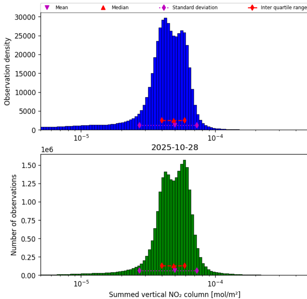
Figure 38: Histogram of “Summed vertical NO 2 column” for 2025-10-28 to 2025-10-29
