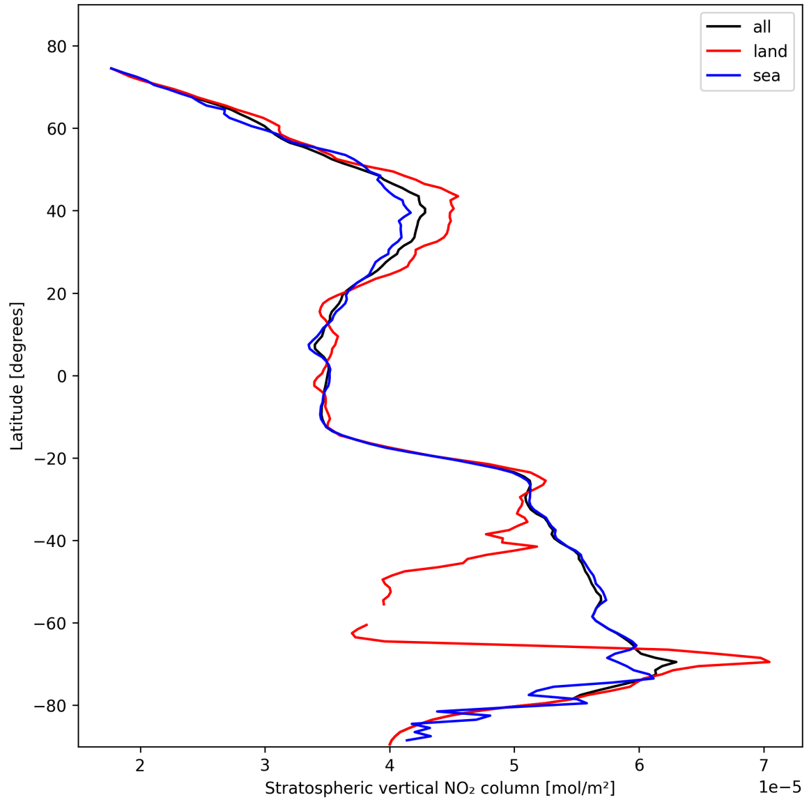
Figure 17: Zonal average of “Stratospheric vertical NO 2 column” for 2025-10-28 to 2025-10-29.
