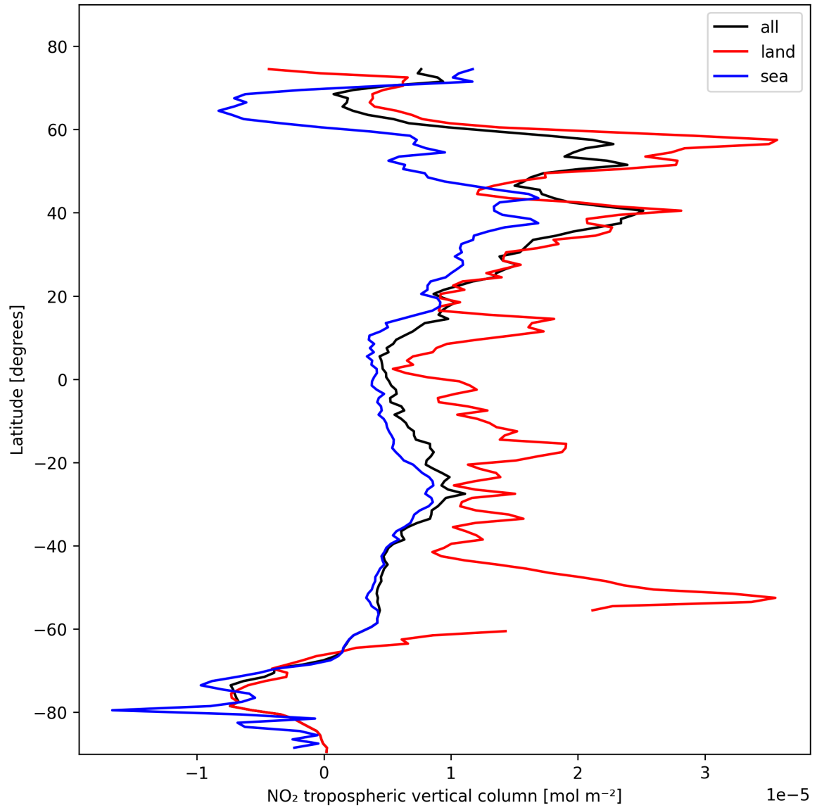
Figure 10: Zonal average of “NO 2 tropospheric vertical column” for 2025-10-28 to 2025-10-29.
