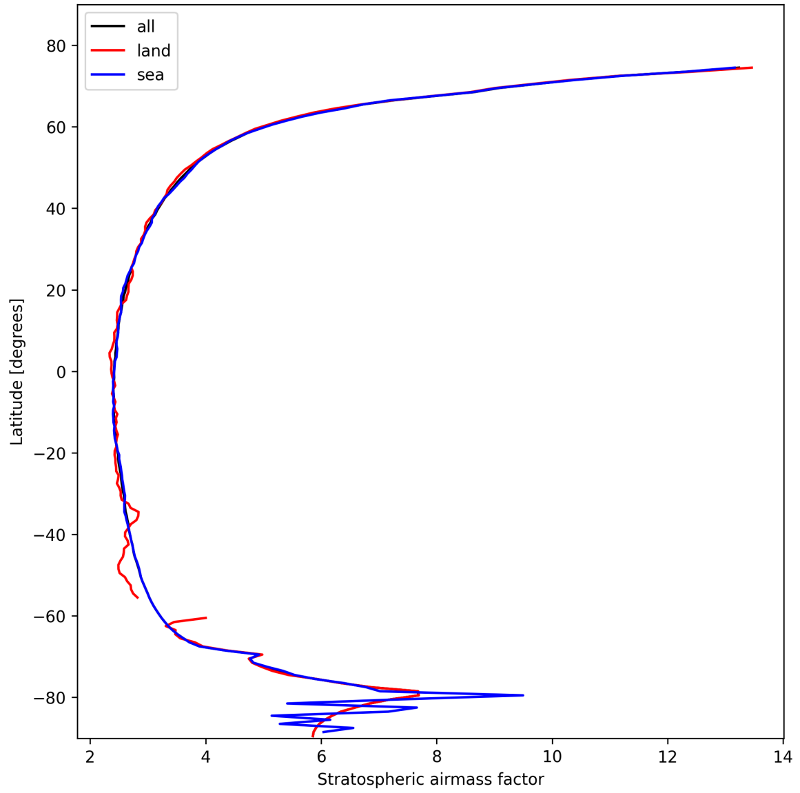
Figure 25: Zonal average of “Stratospheric airmass factor” for 2025-10-28 to 2025-10-29.
