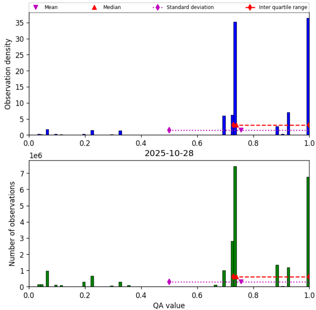
Figure 26: Histogram of “QA value” for 2025-10-28 to 2025-10-29
