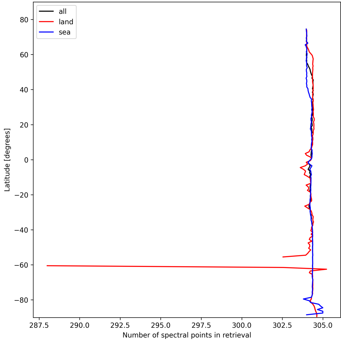
Figure 14: Zonal average of “Number of spectral points in retrieval” for 2025-10-28 to 2025-10-29.
