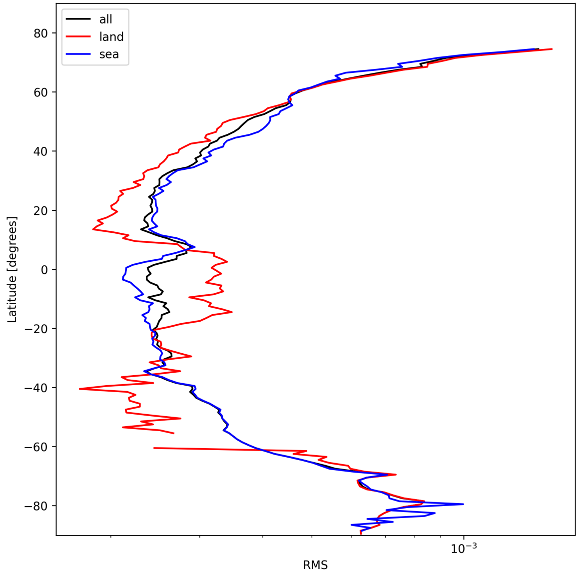
Figure 24: Zonal average of “RMS” for 2025-10-28 to 2025-10-29.
