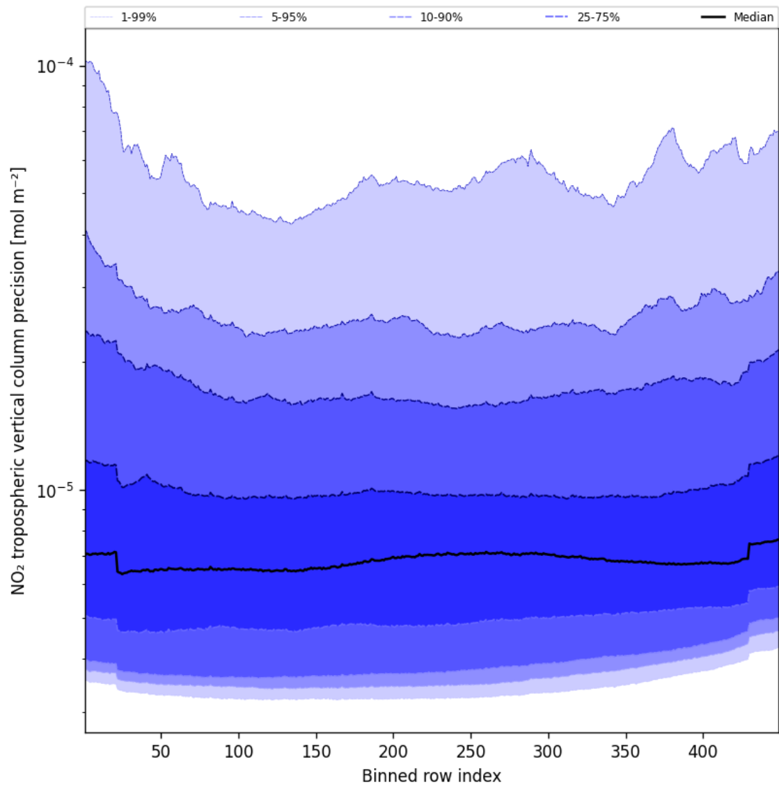
Figure 45: Along track statistics of “NO 2 tropospheric vertical column precision” for 2025-10-28 to 2025-10-29
