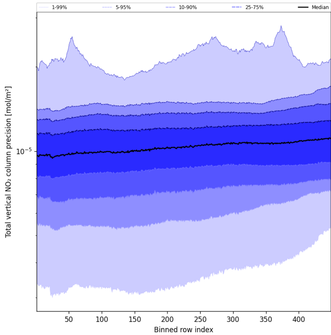
Figure 54: Along track statistics of “Total vertical NO 2 column precision” for 2025-10-28 to 2025-10-29
