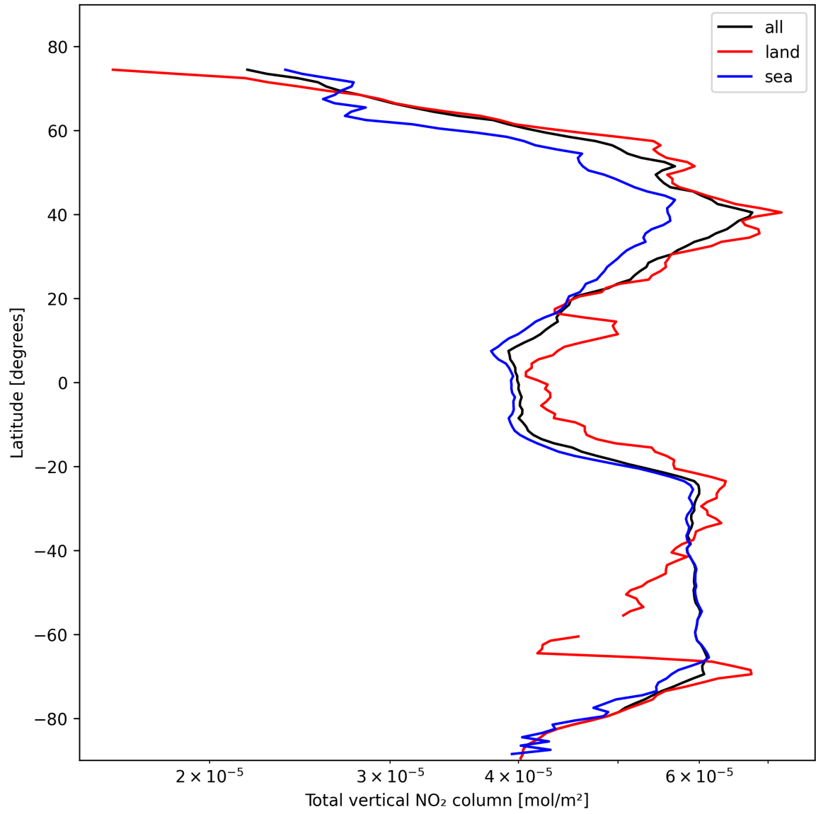
Figure 19: Zonal average of “Total vertical NO 2 column” for 2025-10-28 to 2025-10-29.
