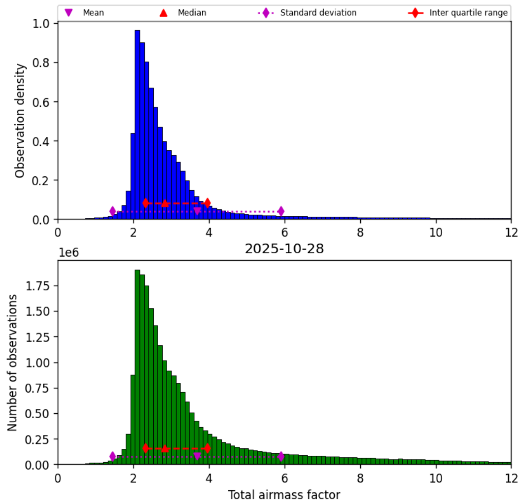
Figure 30: Histogram of “Total airmass factor” for 2025-10-28 to 2025-10-29
