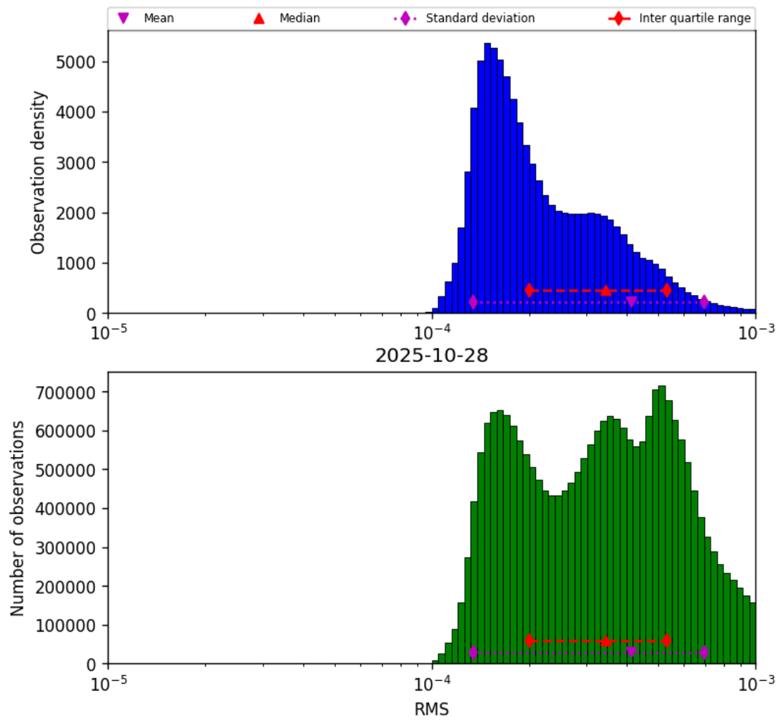
Figure 41: Histogram of “RMS” for 2025-10-28 to 2025-10-29
