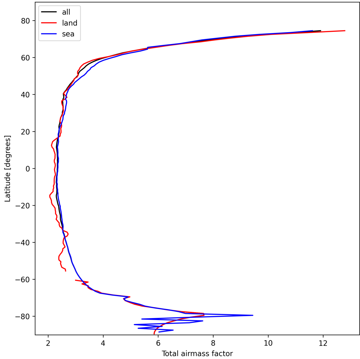
Figure 13: Zonal average of “Total airmass factor” for 2025-10-28 to 2025-10-29.
