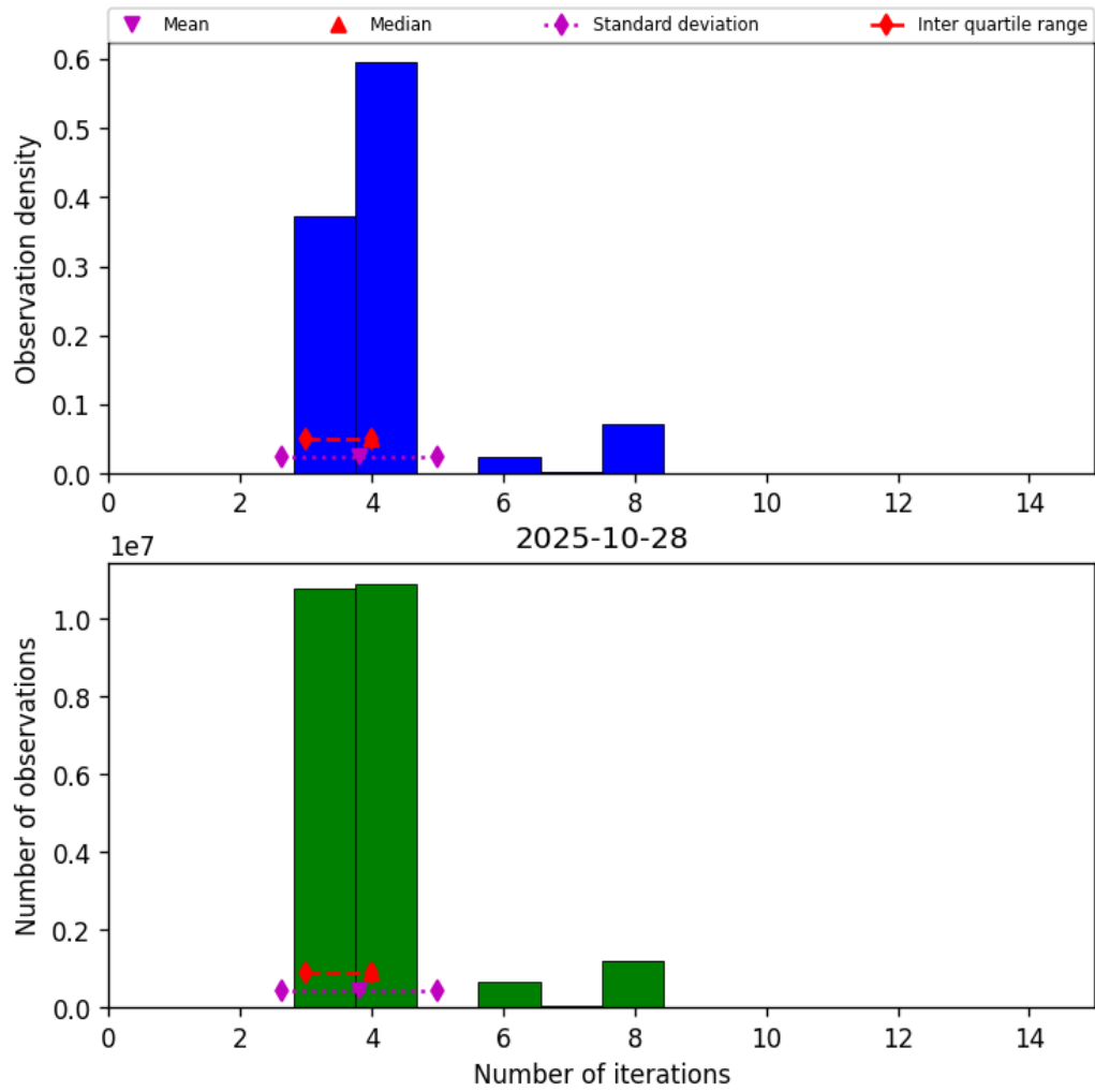
Figure 32: Histogram of “Number of iterations” for 2025-10-28 to 2025-10-29
