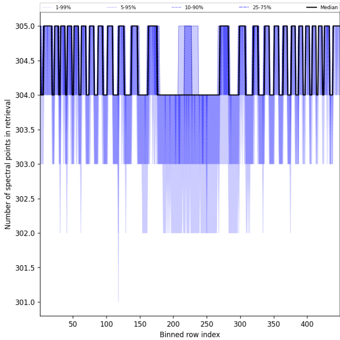
Figure 48: Along track statistics of “Number of spectral points in retrieval” for 2025-10-28 to 2025-10-29
