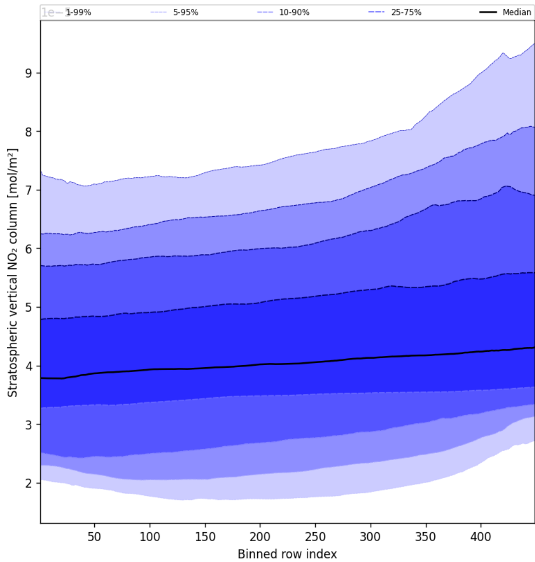
Figure 51: Along track statistics of “Stratospheric vertical NO 2 column” for 2025-10-28 to 2025-10-29
