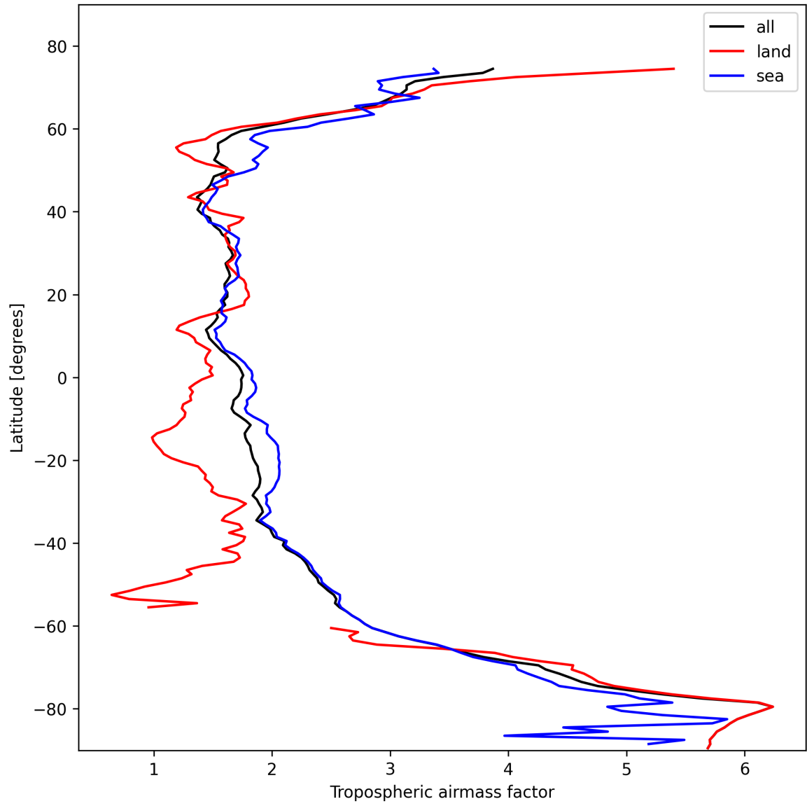
Figure 12: Zonal average of “Tropospheric airmass factor” for 2025-10-28 to 2025-10-29.
