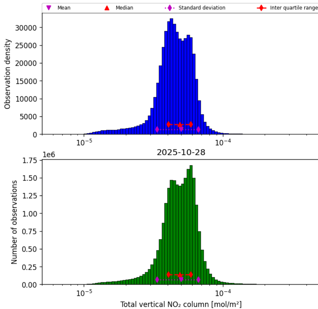
Figure 36: Histogram of "Total vertical NO 2 column" for 2025-10-28 to 2025-10-29
