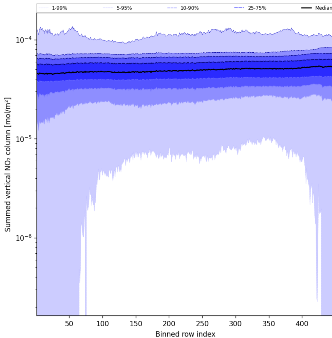
Figure 55: Along track statistics of “Summed vertical NO 2 column” for 2025-10-28 to 2025-10-29
