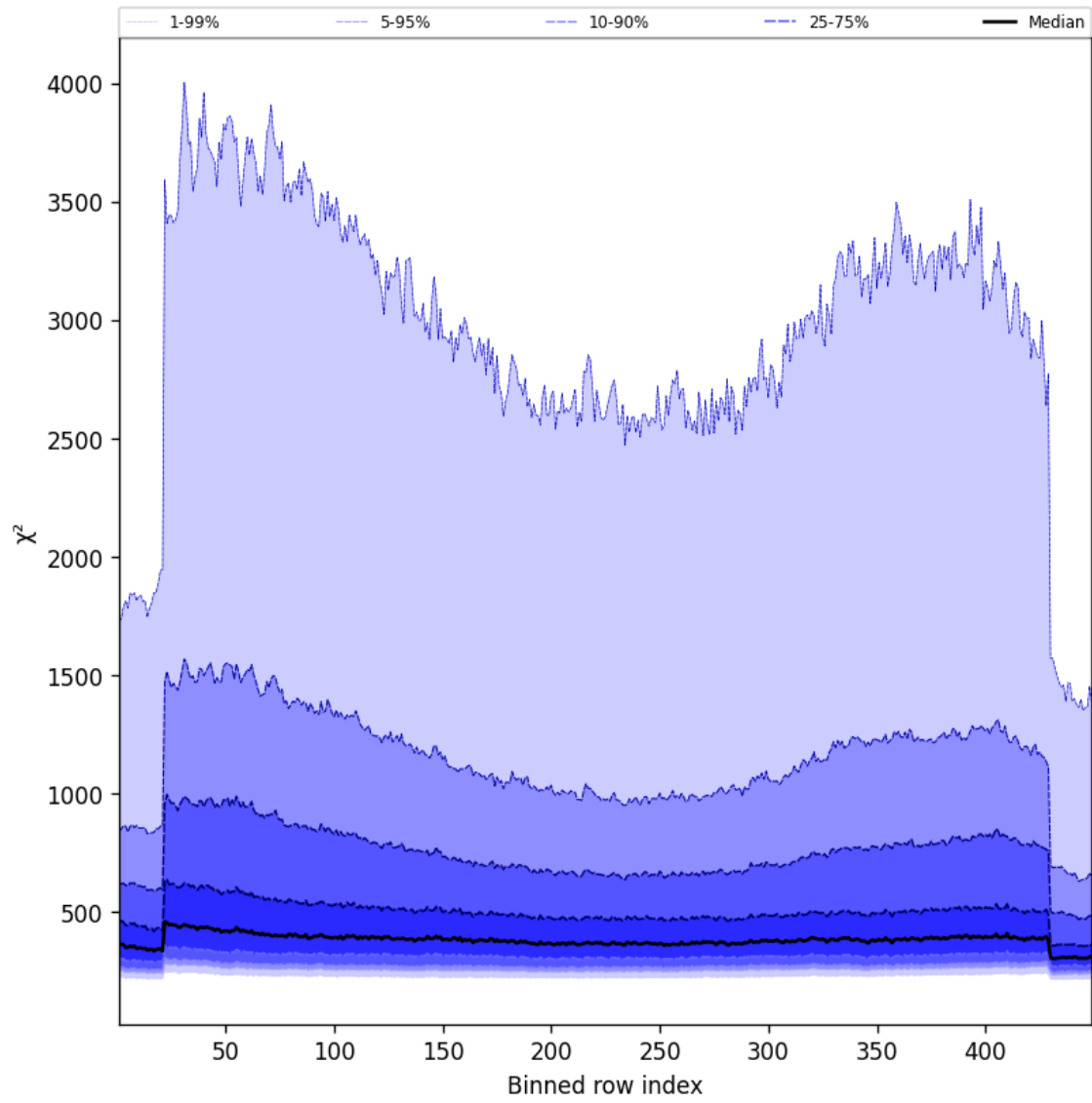
Figure 57: Along track statistics of “ \chi^2 ” for 2025-10-28 to 2025-10-29
