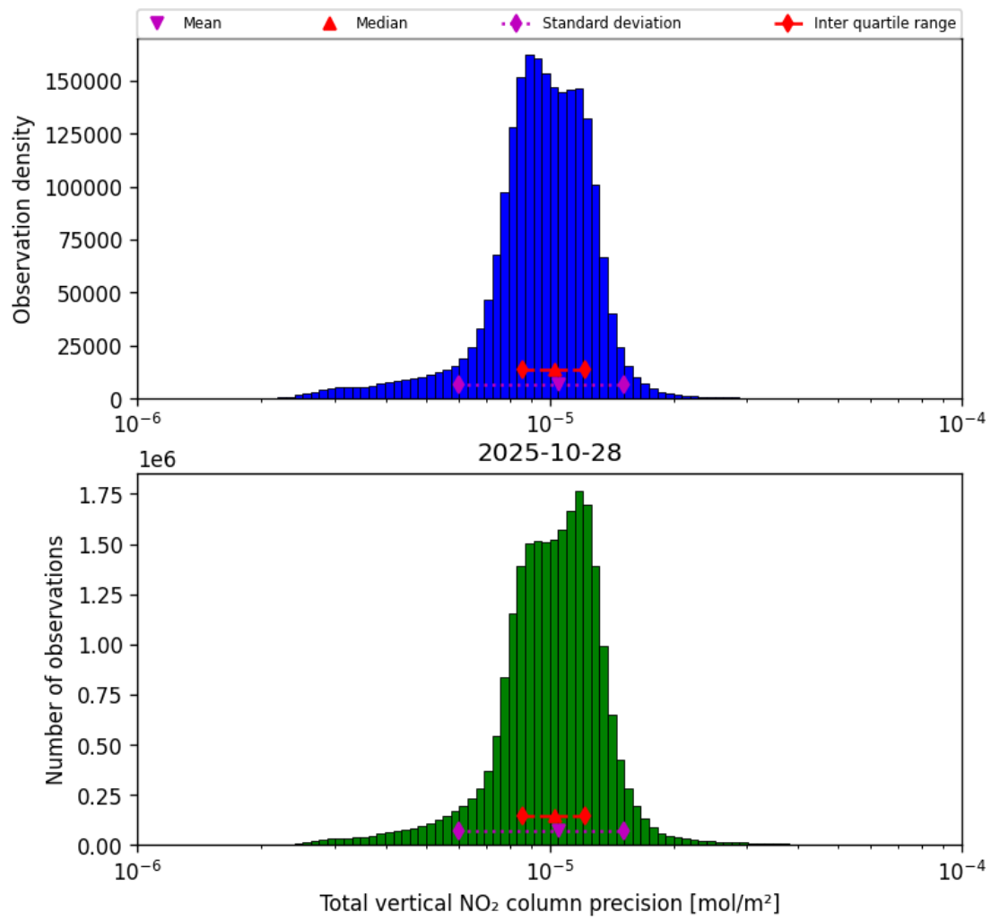
Figure 37: Histogram of “Total vertical NO 2 column precision” for 2025-10-28 to 2025-10-29
