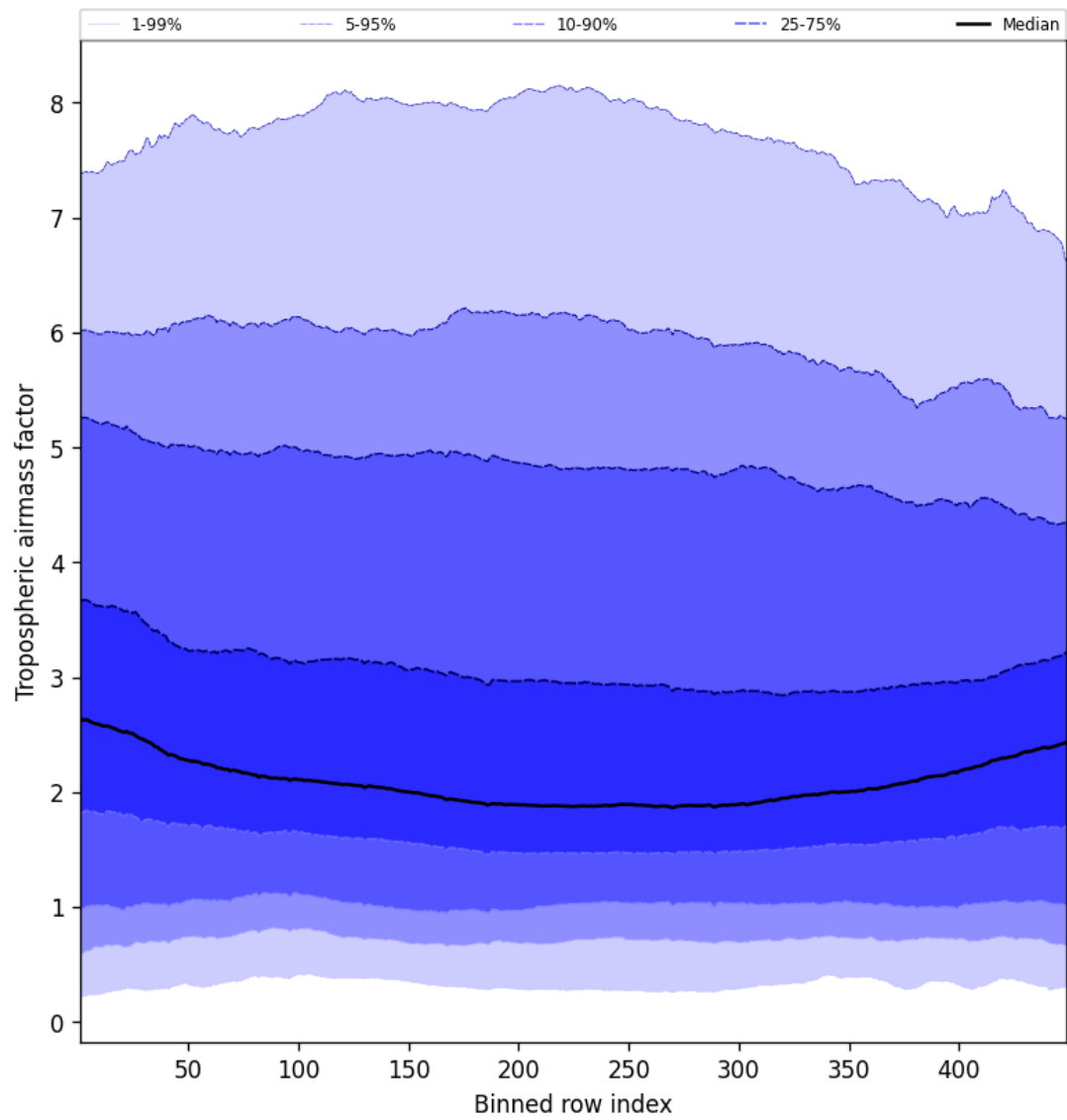
Figure 46: Along track statistics of “Tropospheric airmass factor” for 2025-10-28 to 2025-10-29
