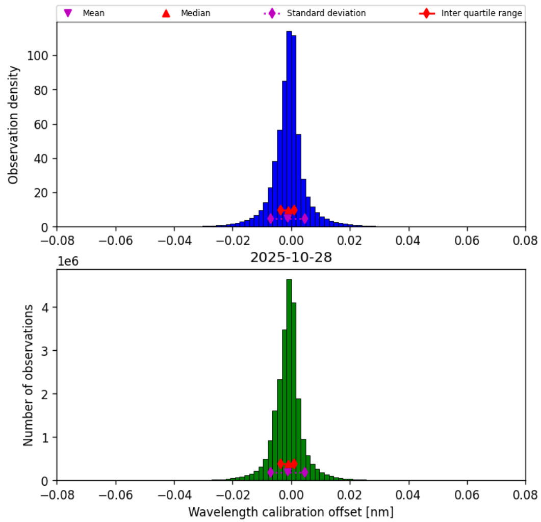
Figure 33: Histogram of “Wavelength calibration offset” for 2025-10-28 to 2025-10-29
