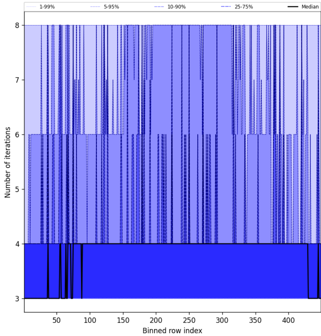
Figure 49: Along track statistics of “Number of iterations” for 2025-10-29 to 2025-10-30
