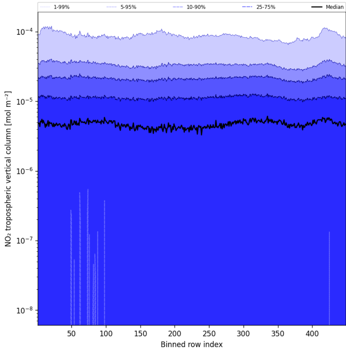
Figure 44: Along track statistics of “NO 2 tropospheric vertical column” for 2025-10-29 to 2025-10-30
