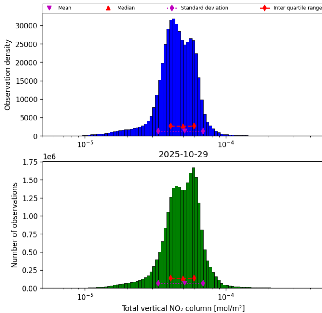
Figure 36: Histogram of “Total vertical NO 2 column” for 2025-10-29 to 2025-10-30
