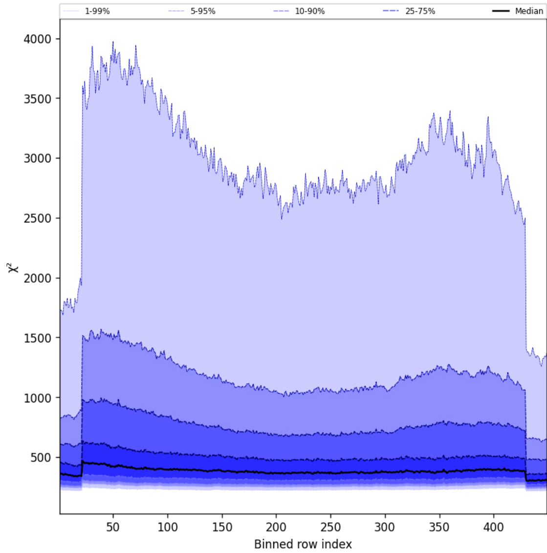
Figure 57: Along track statistics of “ \chi^2 ” for 2025-10-29 to 2025-10-30
