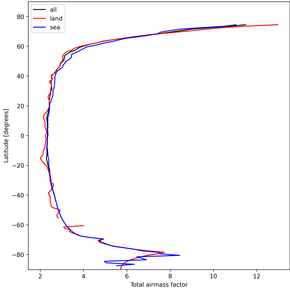
Figure 13: Zonal average of “Total airmass factor” for 2025-10-29 to 2025-10-30.
