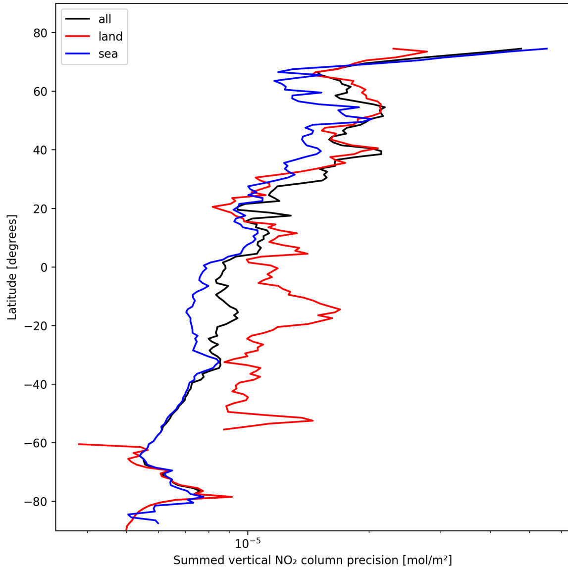
Figure 22: Zonal average of “Summed vertical NO 2 column precision” for 2025-10-29 to 2025-10-30.
