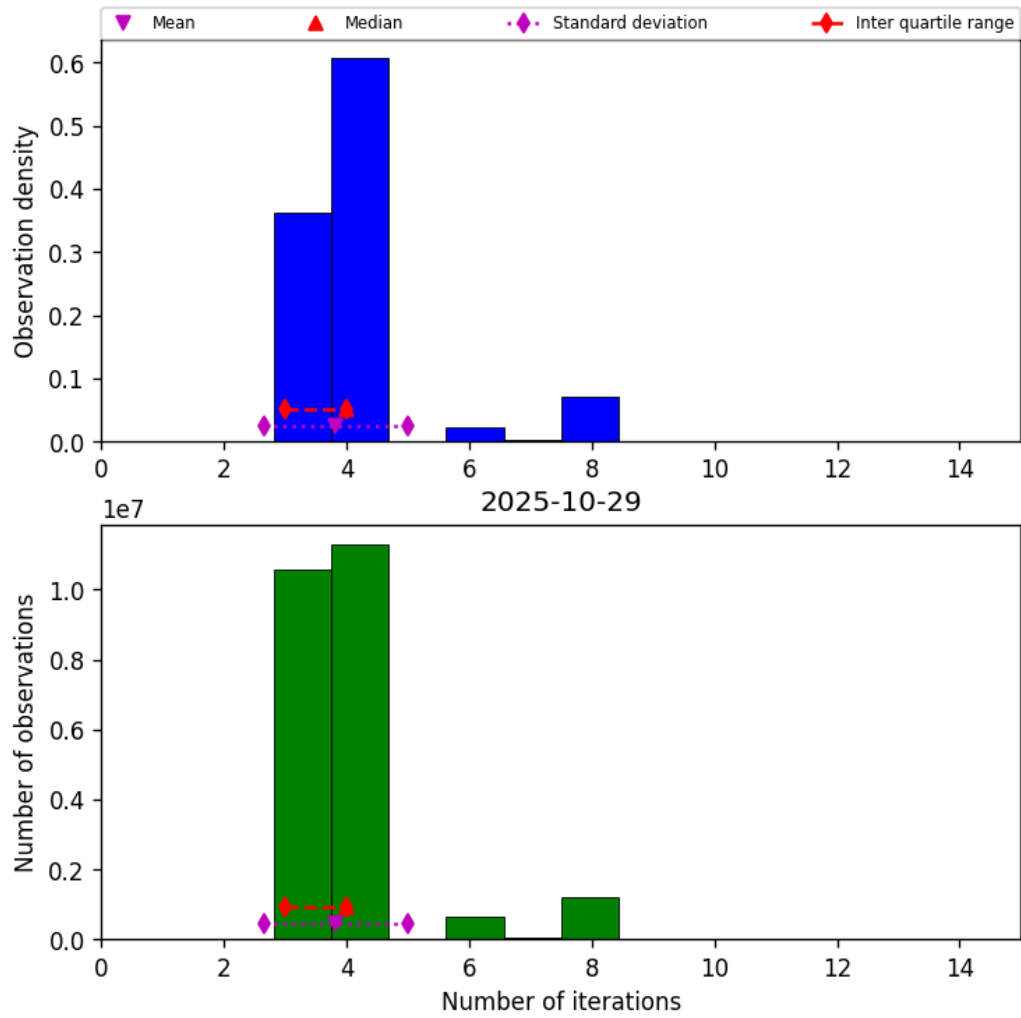
Figure 32: Histogram of “Number of iterations” for 2025-10-29 to 2025-10-30
