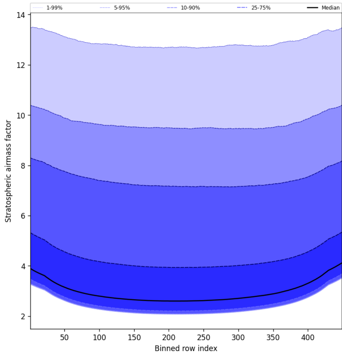
Figure 59: Along track statistics of “Stratospheric airmass factor” for 2025-10-29 to 2025-10-30
