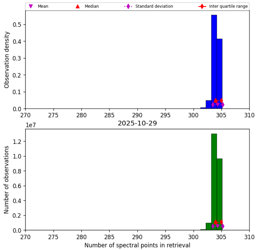
Figure 31: Histogram of “Number of spectral points in retrieval” for 2025-10-29 to 2025-10-30
