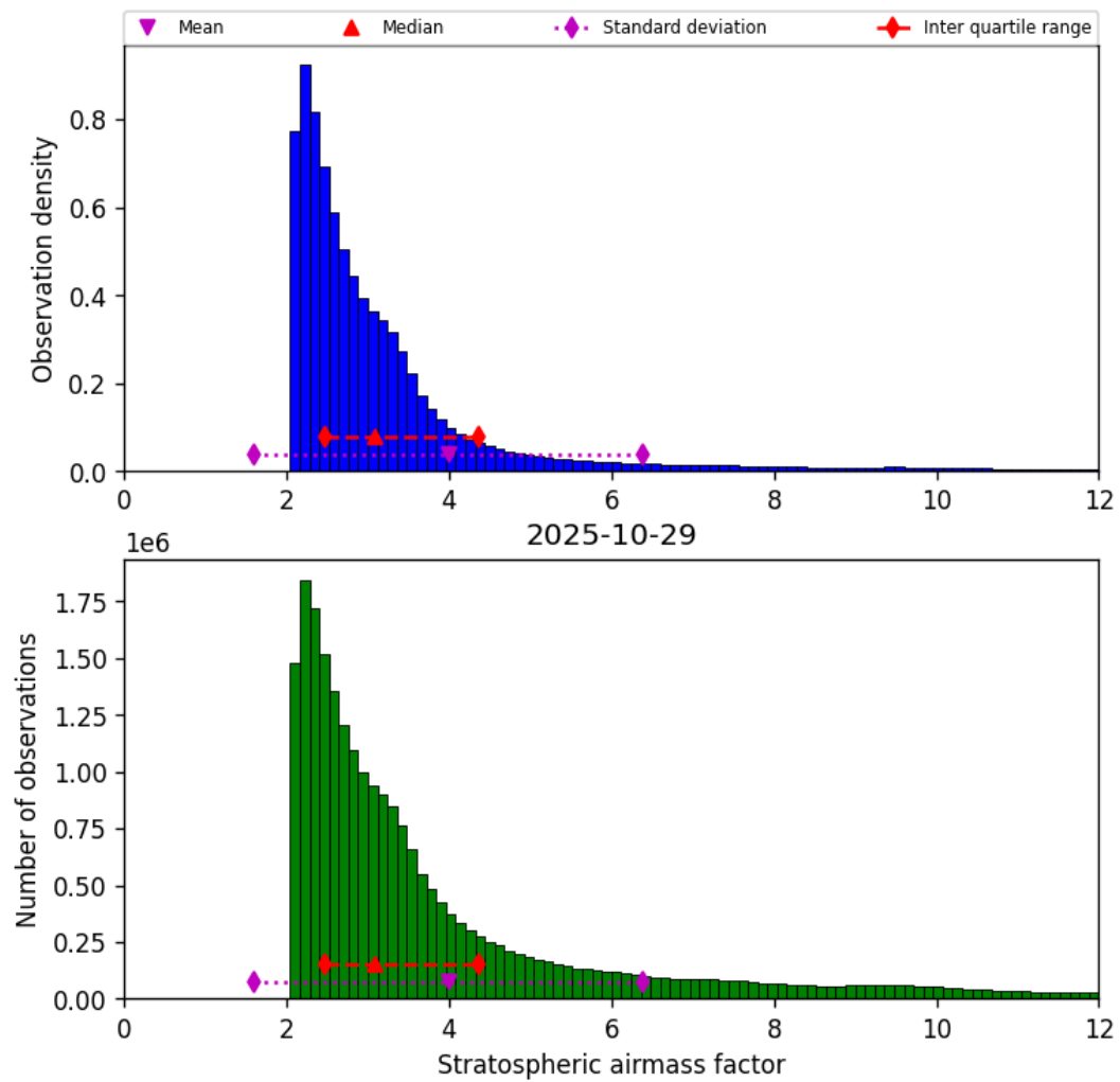
Figure 42: Histogram of “Stratospheric airmass factor” for 2025-10-29 to 2025-10-30
