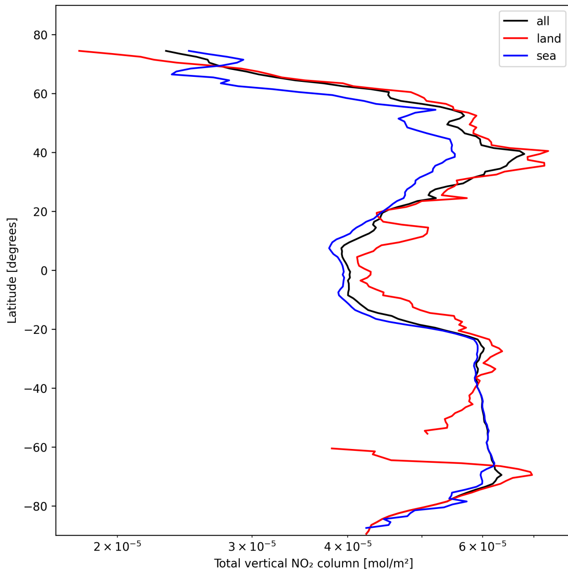
Figure 19: Zonal average of “Total vertical NO 2 column” for 2025-10-29 to 2025-10-30.
