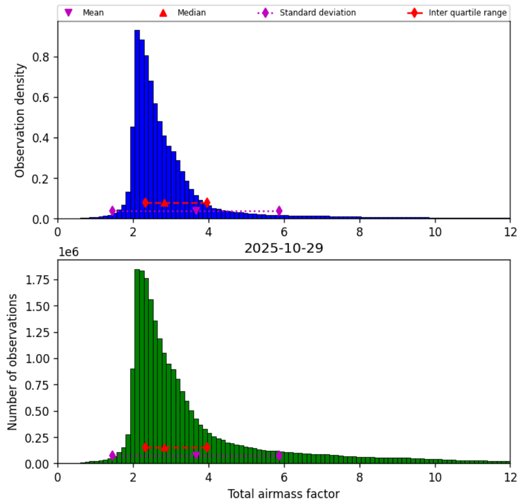
Figure 30: Histogram of “Total airmass factor” for 2025-10-29 to 2025-10-30
