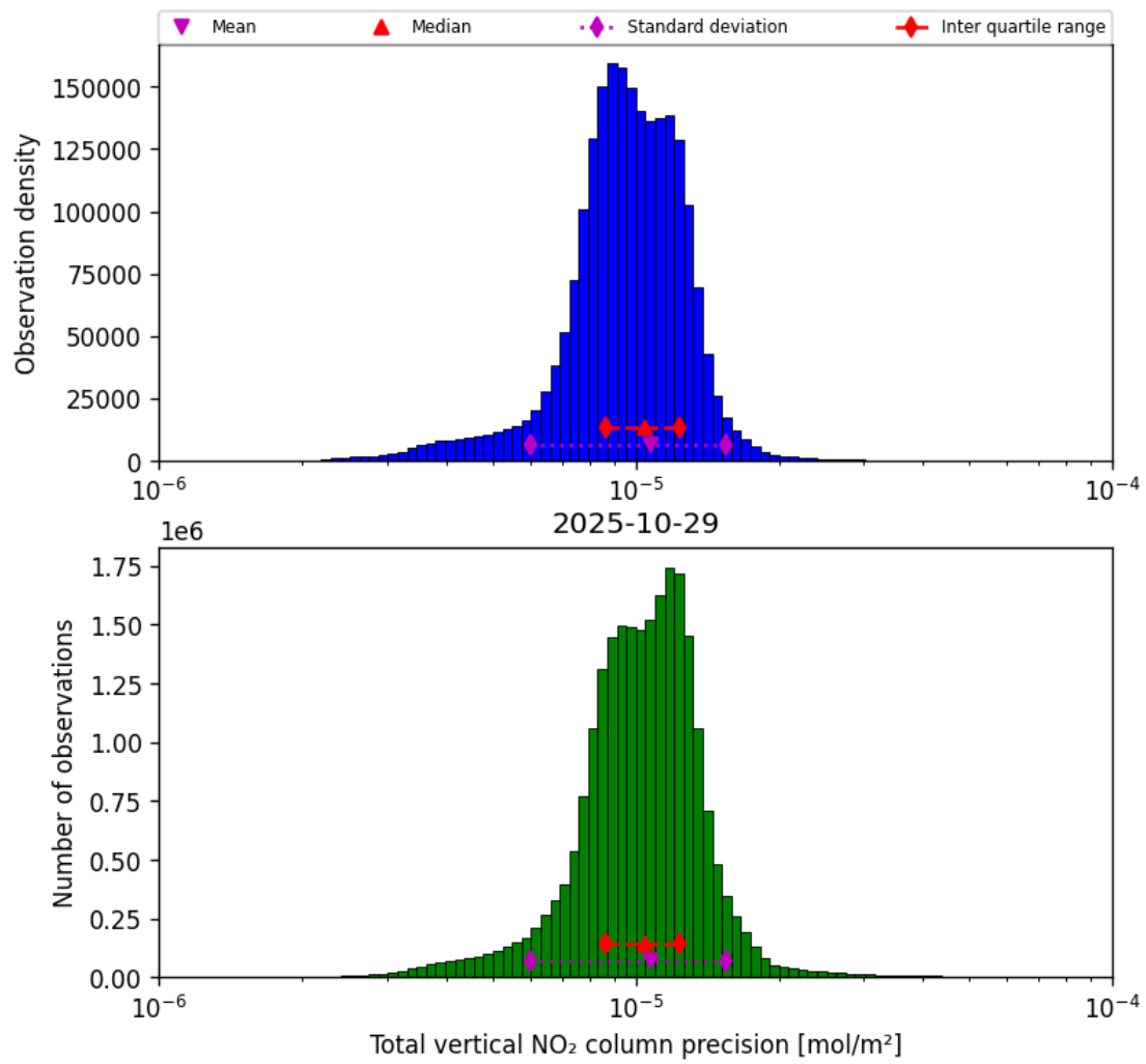
Figure 37: Histogram of “Total vertical NO 2 column precision” for 2025-10-29 to 2025-10-30
