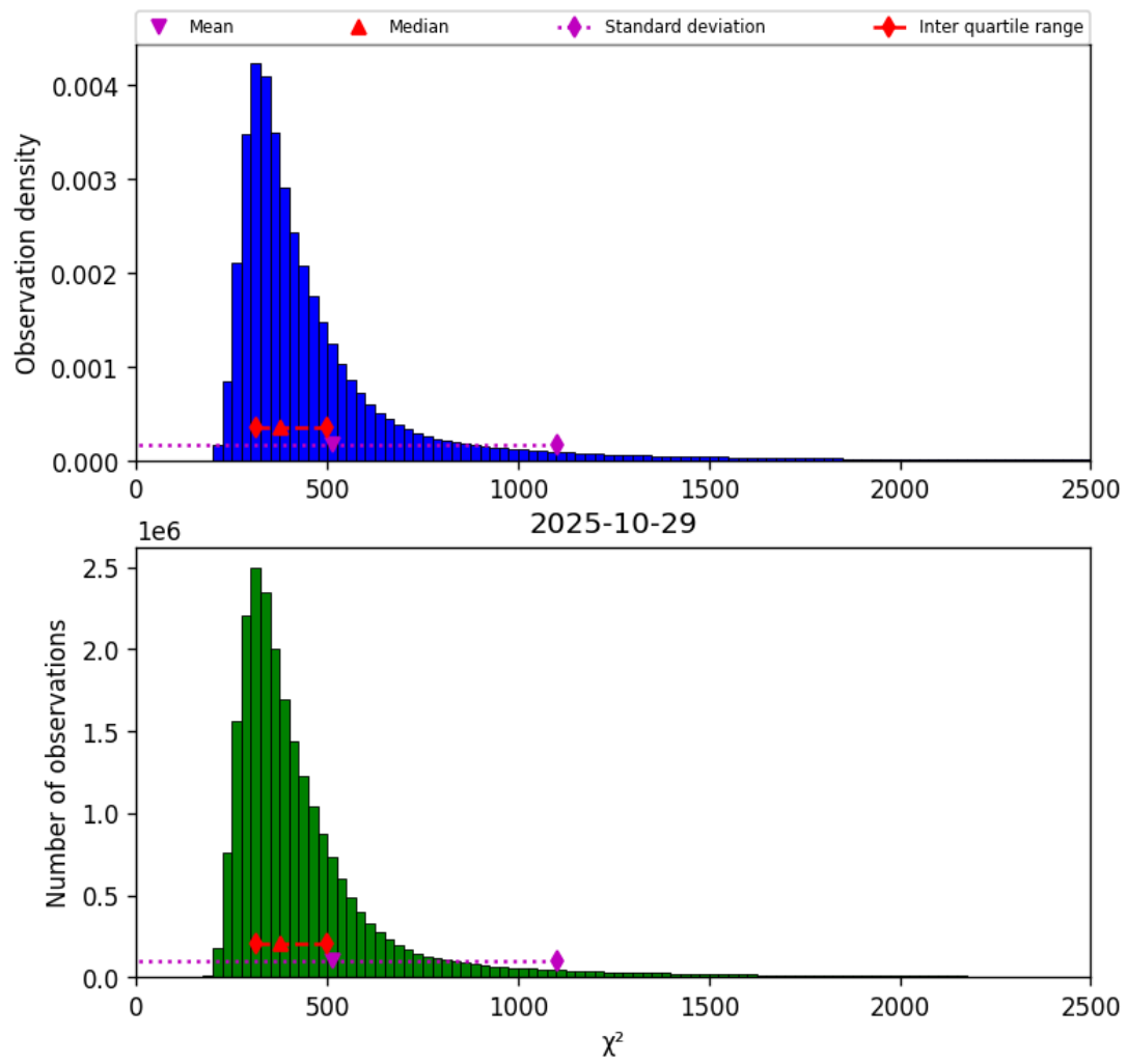
Figure 40: Histogram of “ \chi^2 ” for 2025-10-29 to 2025-10-30
