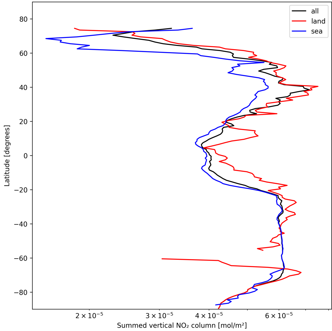
Figure 21: Zonal average of “Summed vertical NO 2 column” for 2025-10-29 to 2025-10-30.
