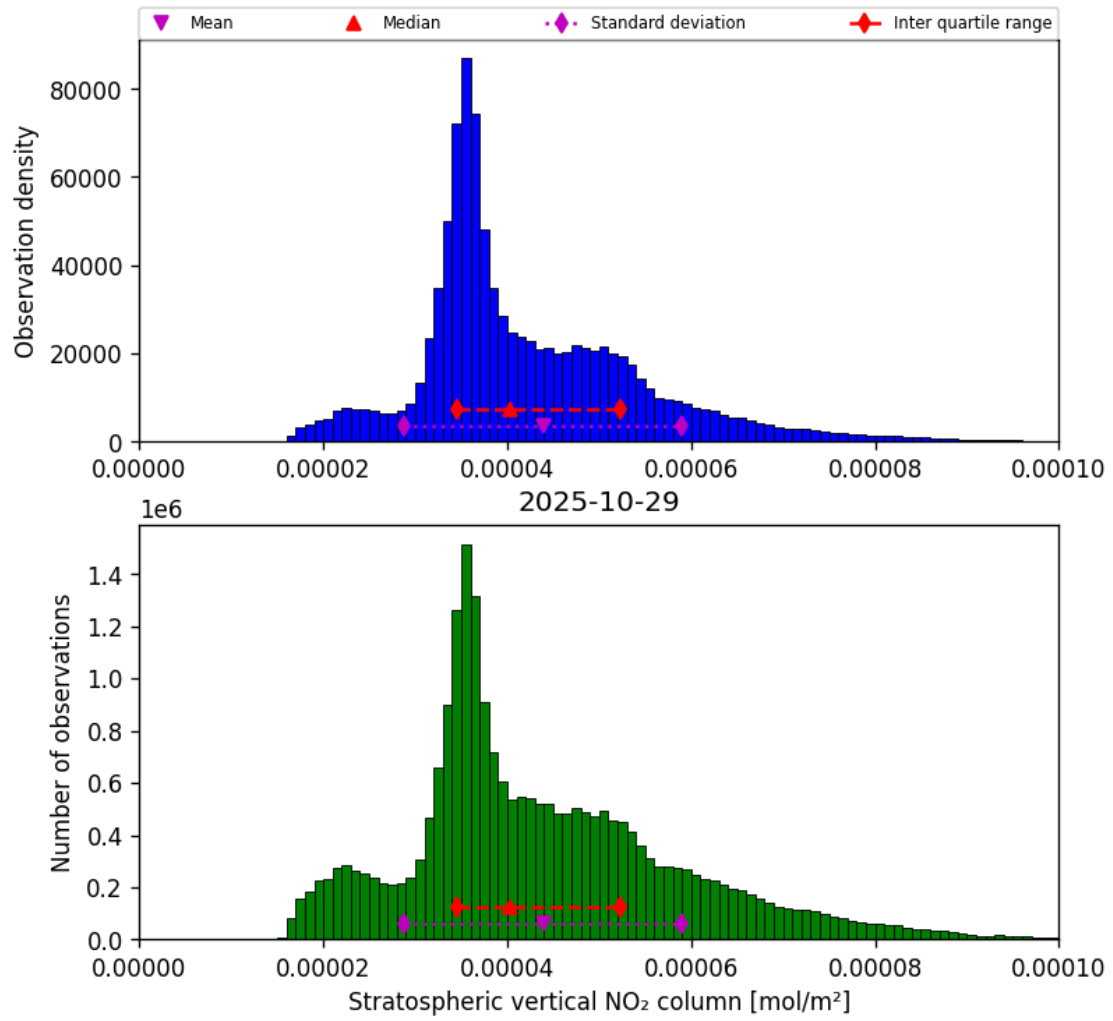
Figure 34: Histogram of “Stratospheric vertical NO 2 column” for 2025-10-29 to 2025-10-30
