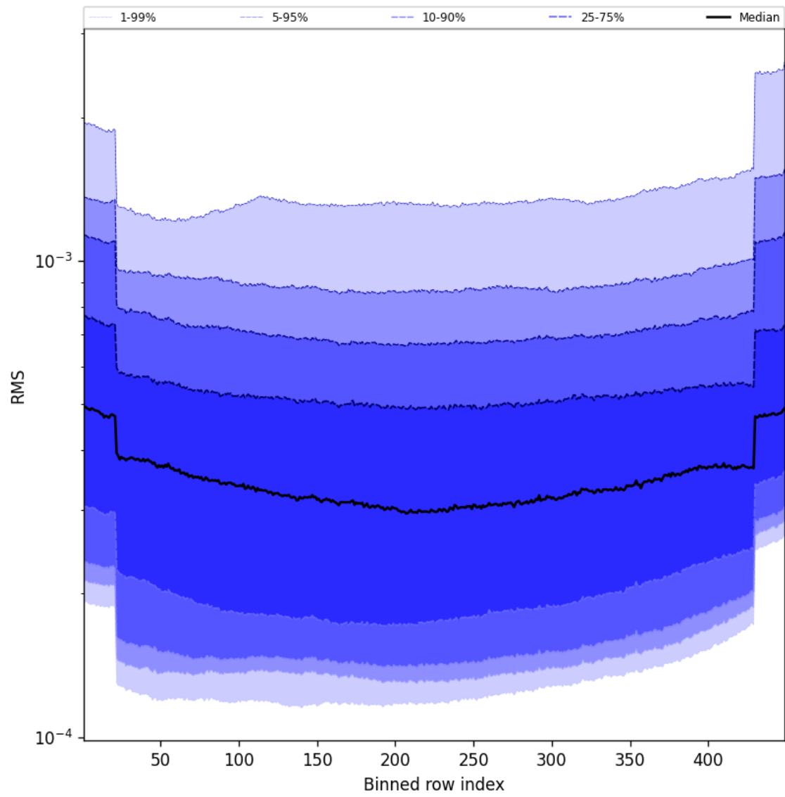
Figure 58: Along track statistics of “RMS” for 2025-10-29 to 2025-10-30
