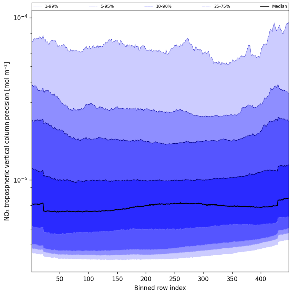
Figure 45: Along track statistics of "NO 2 tropospheric vertical column precision" for 2025-10-29 to 2025-10-30
