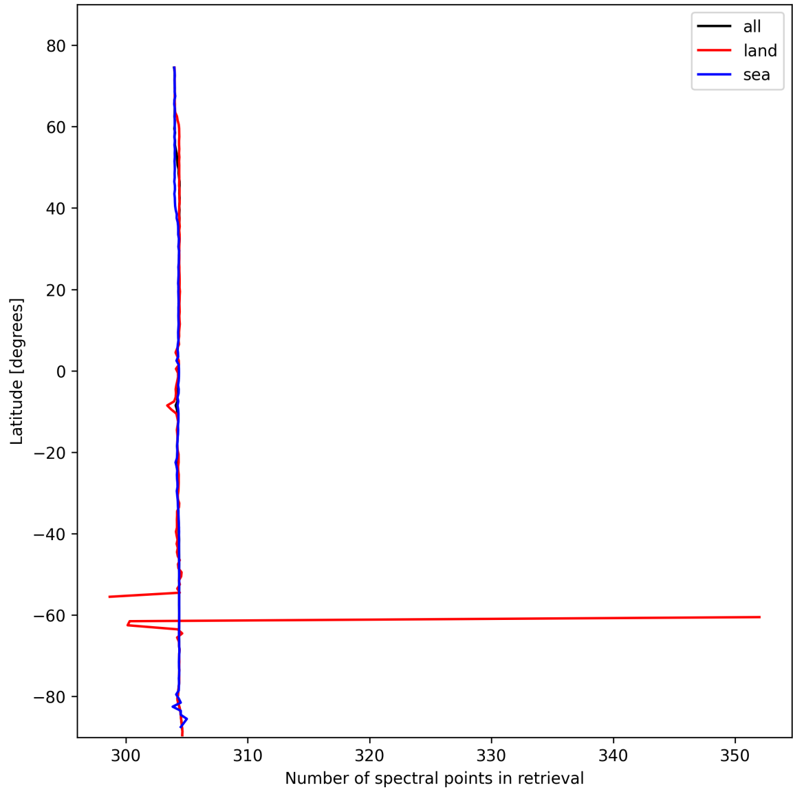
Figure 14: Zonal average of “Number of spectral points in retrieval” for 2025-10-29 to 2025-10-30.
