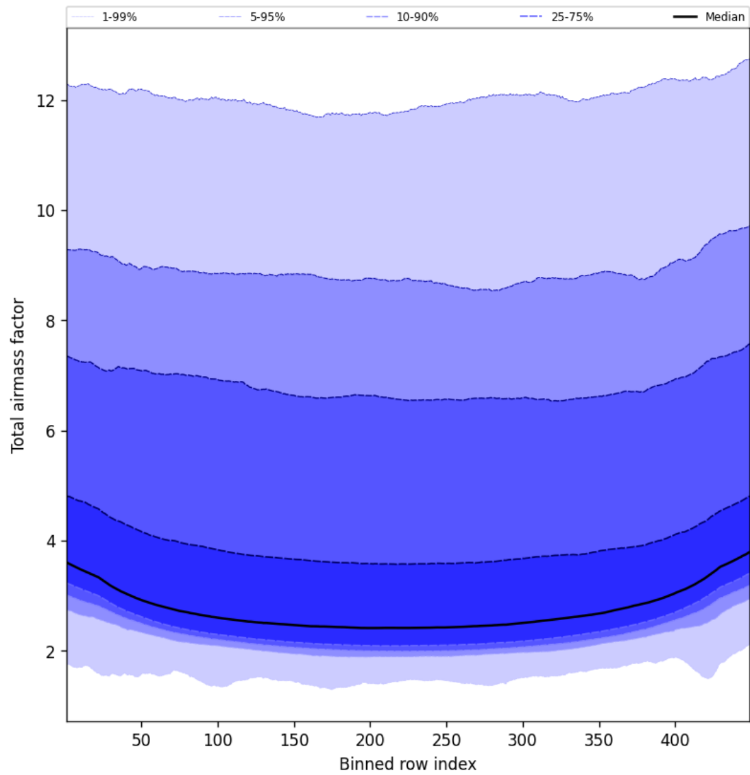
Figure 47: Along track statistics of “Total airmass factor” for 2025-10-29 to 2025-10-30
