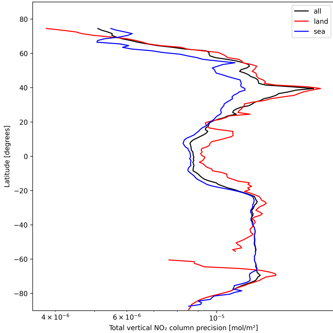
Figure 20: Zonal average of “Total vertical NO 2 column precision” for 2025-10-29 to 2025-10-30.
