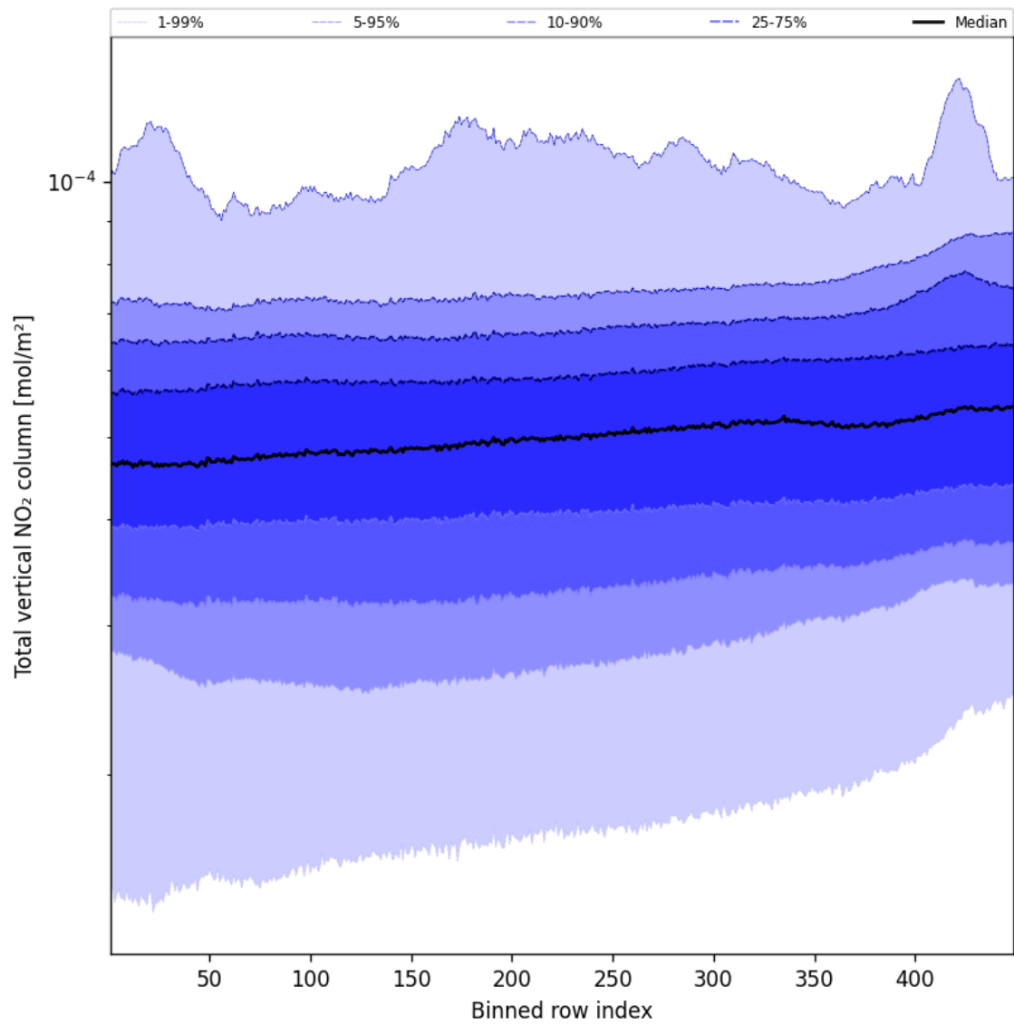
Figure 53: Along track statistics of “Total vertical NO 2 column” for 2025-10-29 to 2025-10-30
