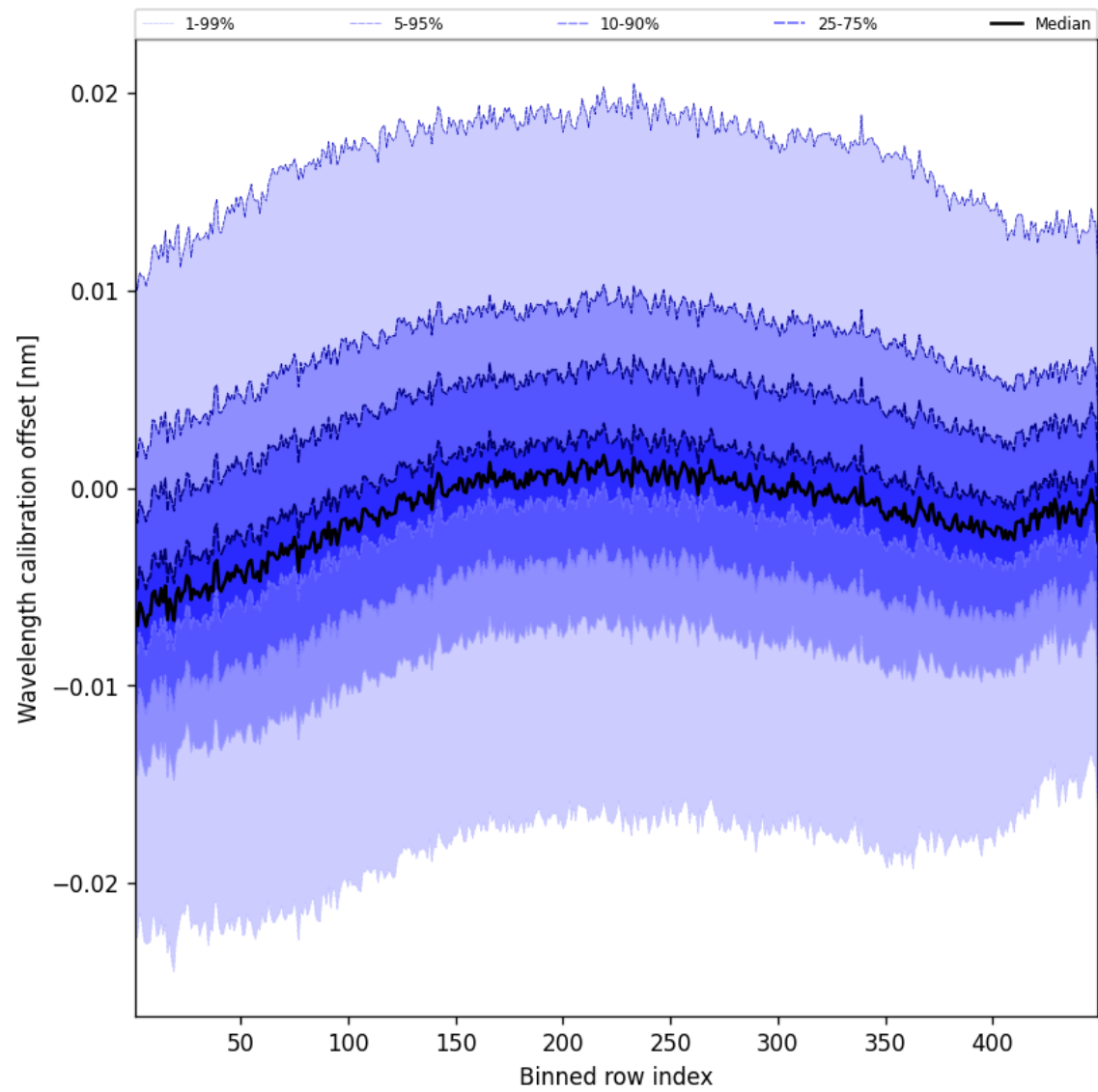
Figure 50: Along track statistics of “Wavelength calibration offset” for 2025-10-29 to 2025-10-30
