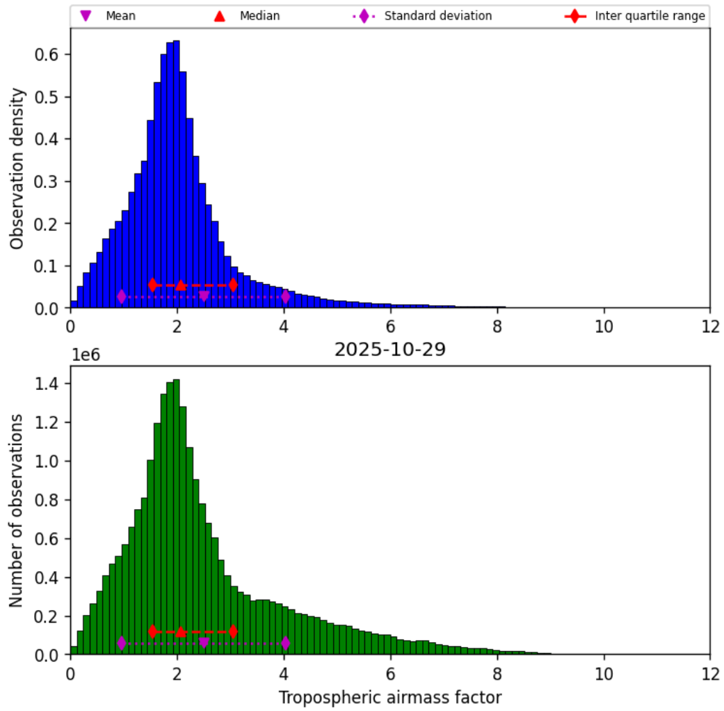
Figure 29: Histogram of “Tropospheric airmass factor” for 2025-10-29 to 2025-10-30
