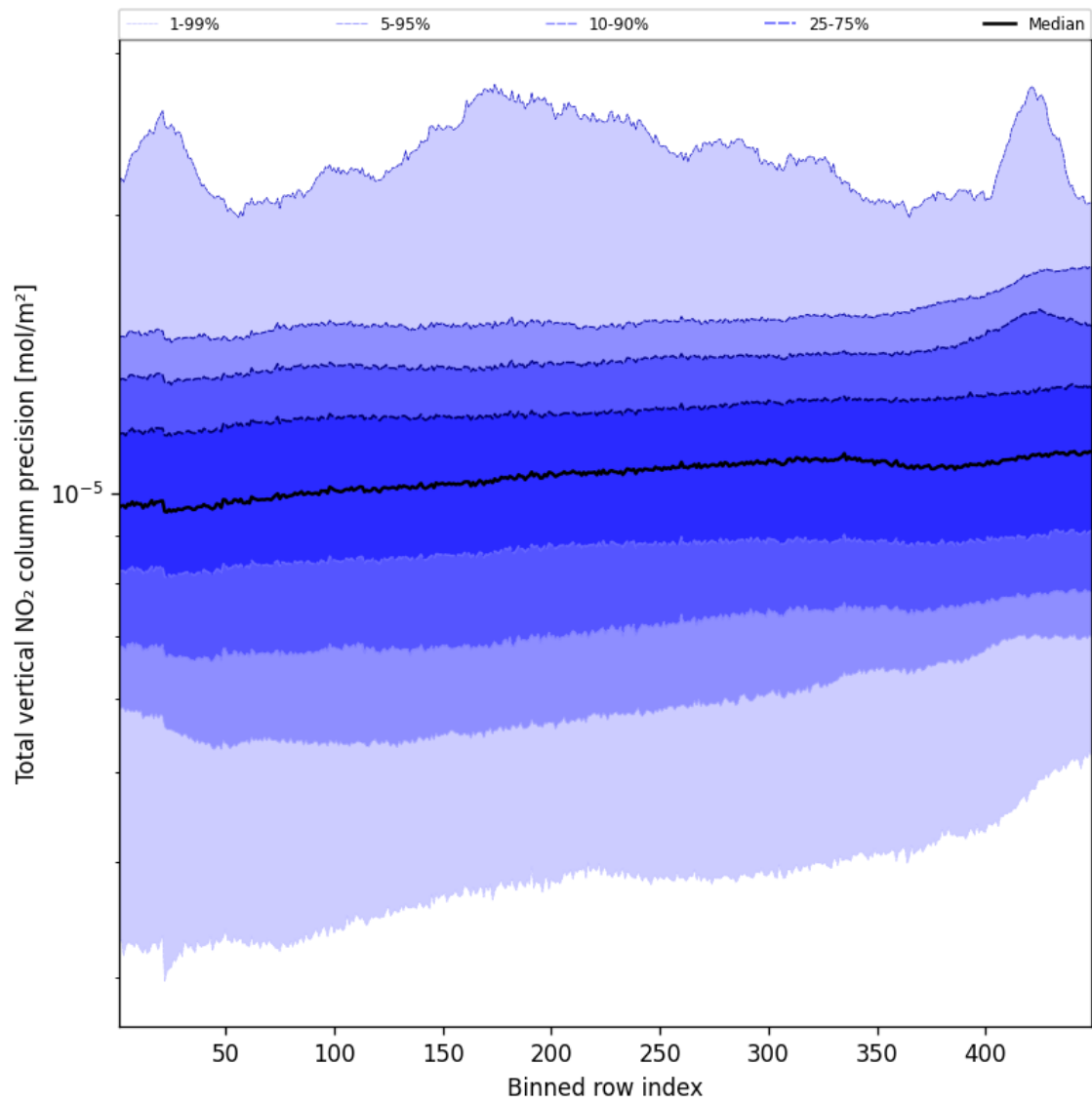
Figure 54: Along track statistics of “Total vertical NO 2 column precision” for 2025-10-29 to 2025-10-30
