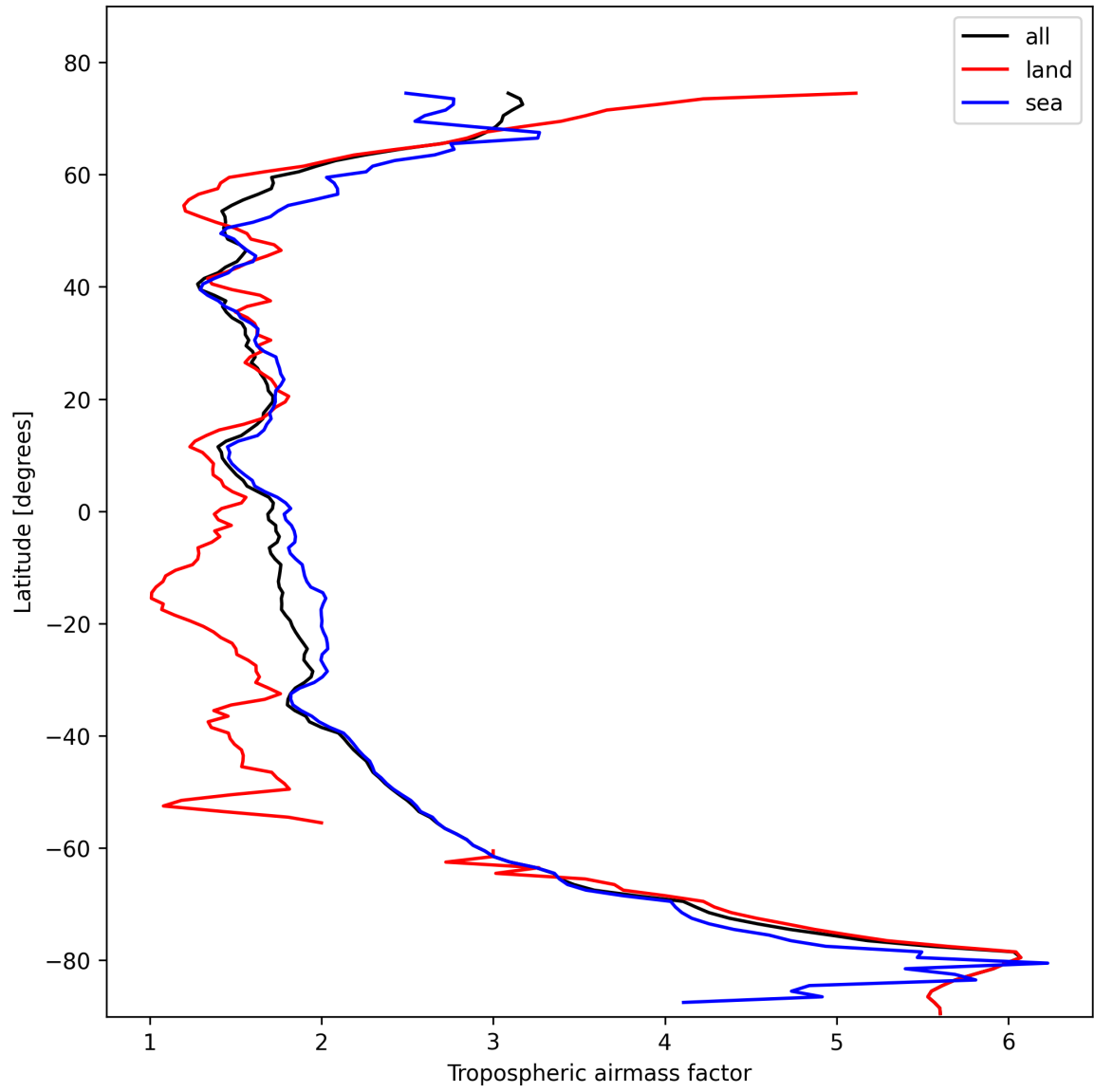
Figure 12: Zonal average of “Tropospheric airmass factor” for 2025-10-29 to 2025-10-30.
