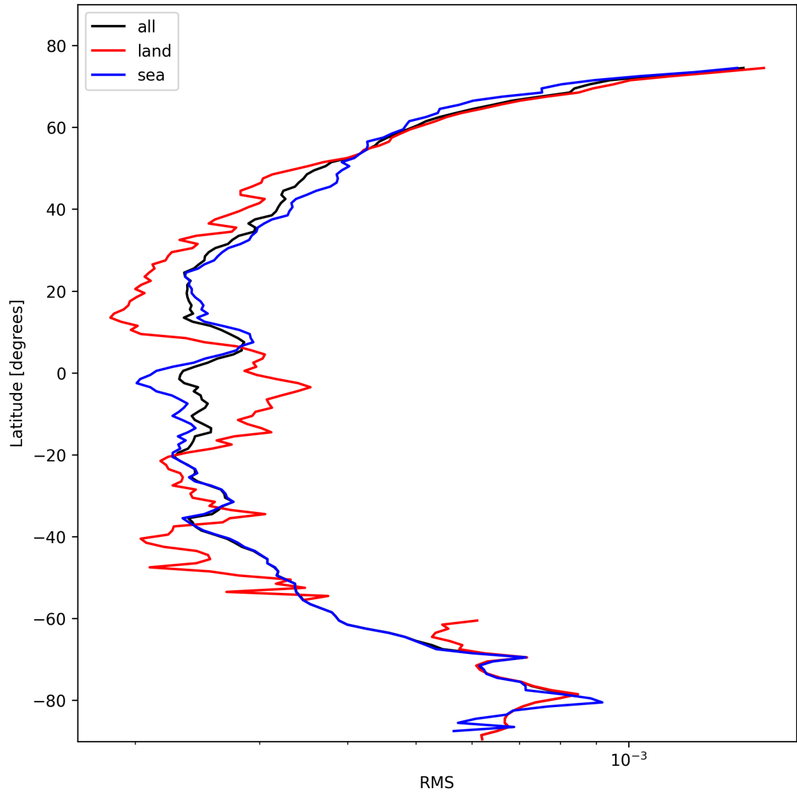
Figure 24: Zonal average of “RMS” for 2025-10-29 to 2025-10-30.
