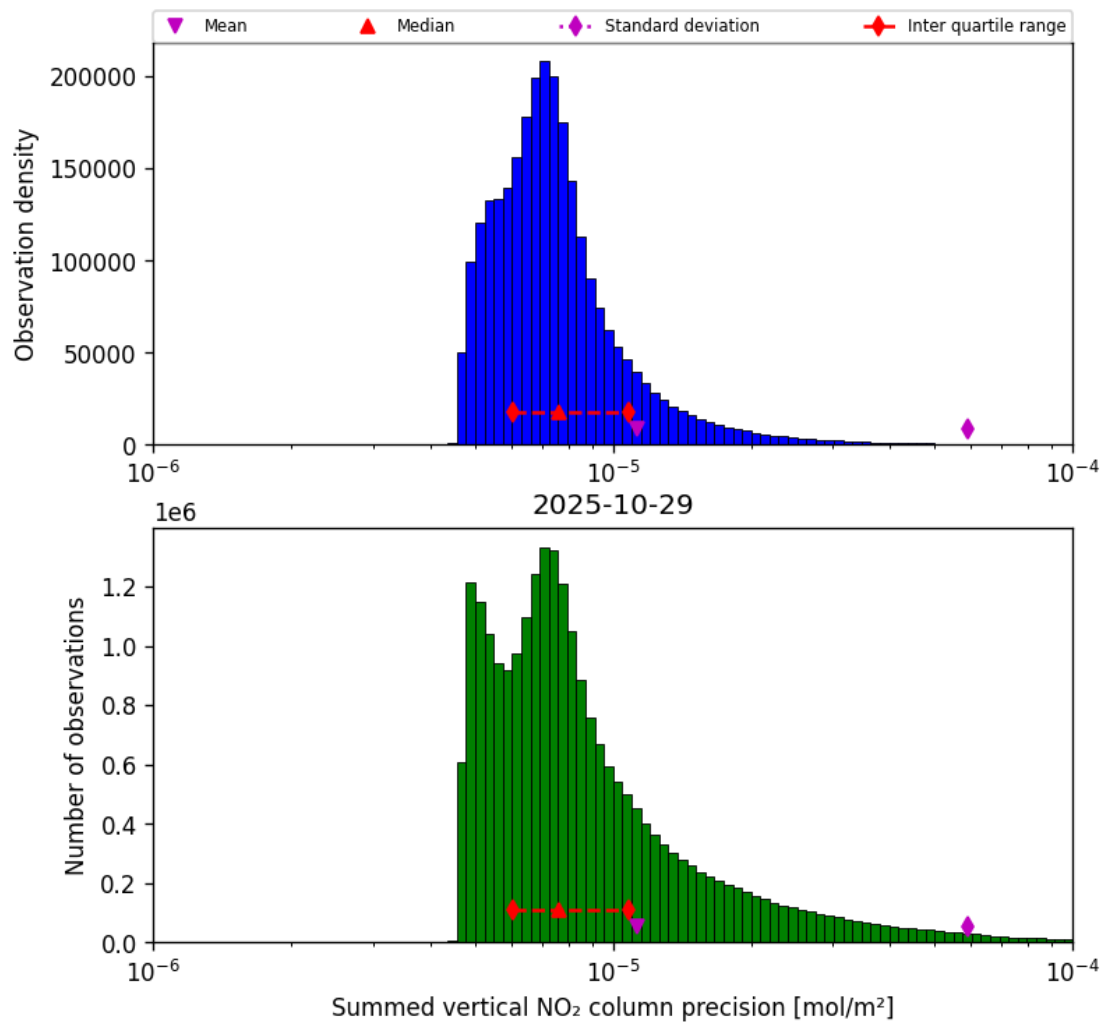
Figure 39: Histogram of "Summed vertical NO 2 column precision" for 2025-10-29 to 2025-10-30
