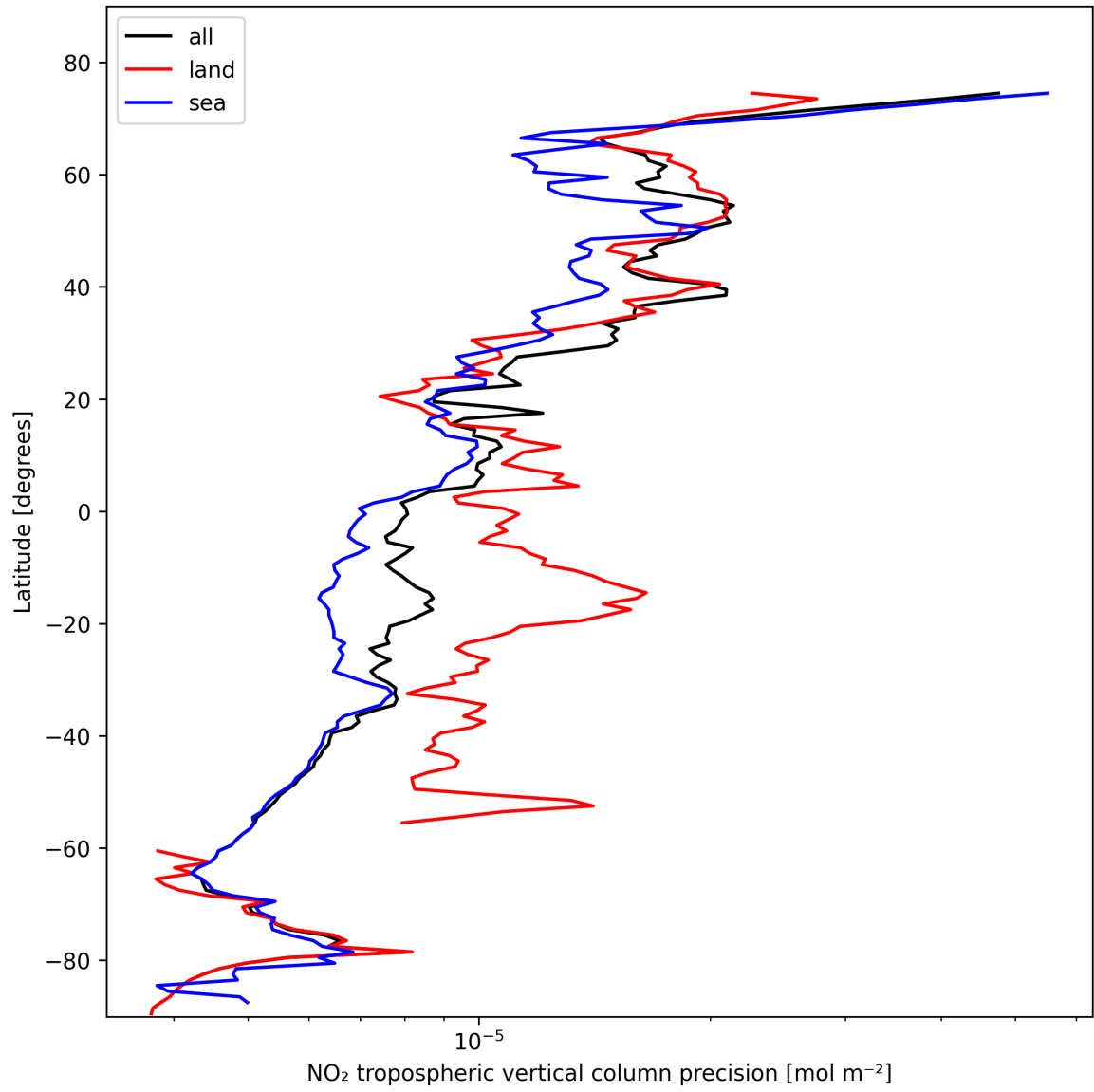
Figure 11: Zonal average of “NO 2 tropospheric vertical column precision” for 2025-10-29 to 2025-10-30.
