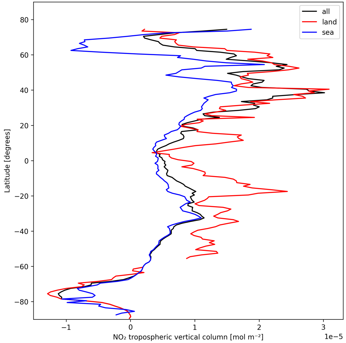
Figure 10: Zonal average of “NO 2 tropospheric vertical column” for 2025-10-29 to 2025-10-30.
