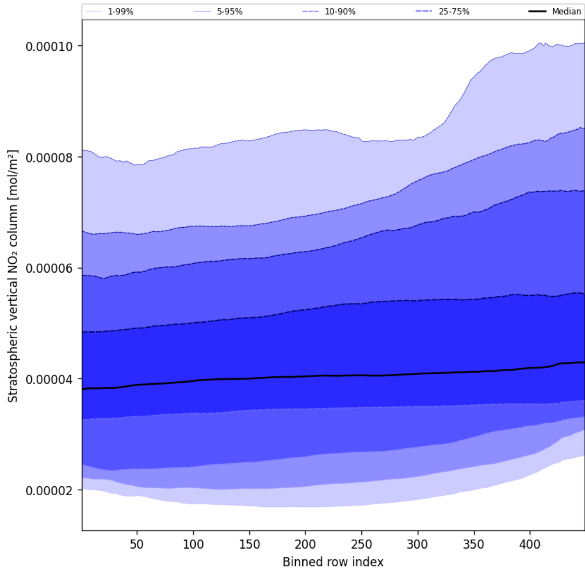
Figure 51: Along track statistics of “Stratospheric vertical NO 2 column” for 2025-10-29 to 2025-10-30
