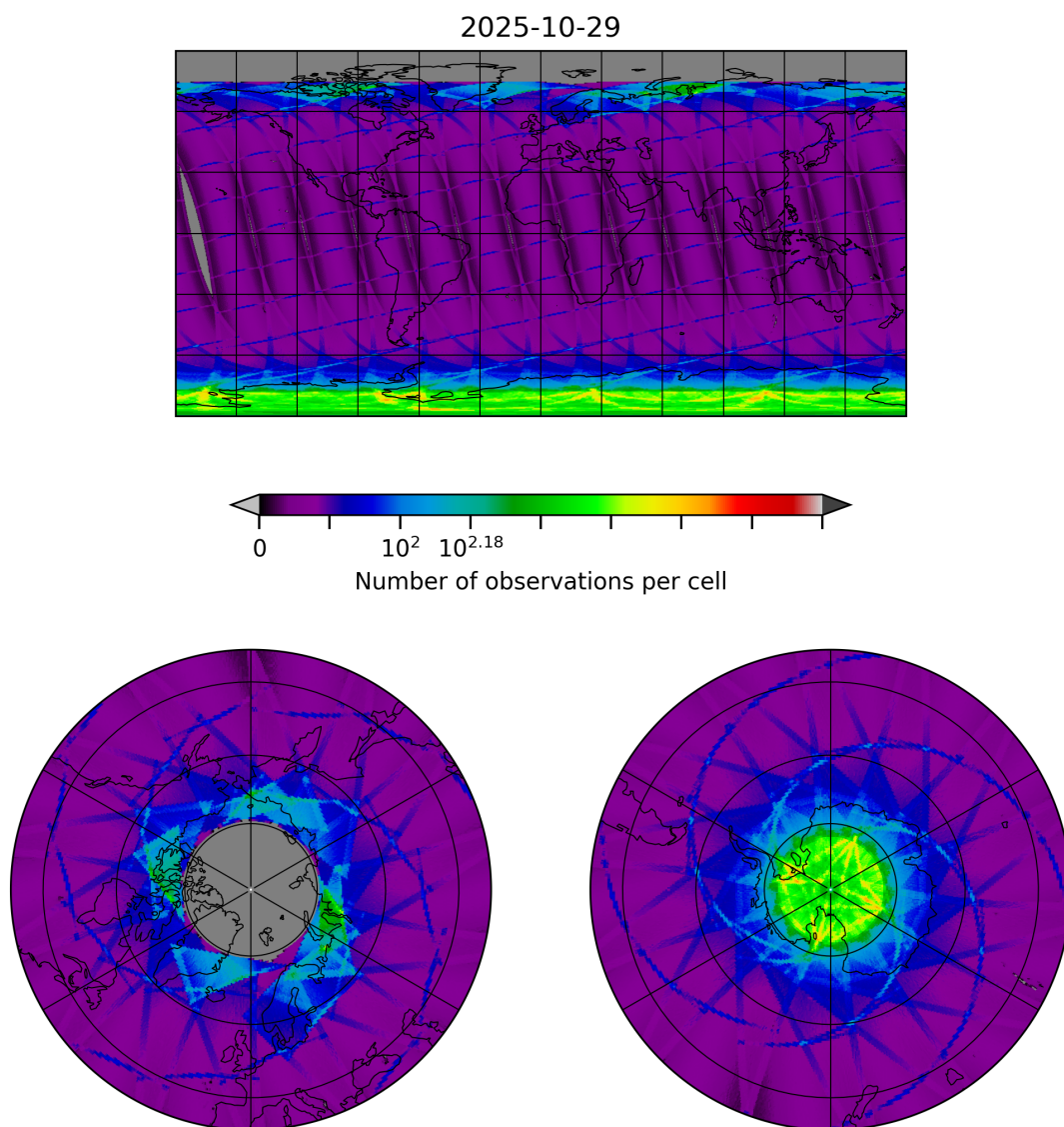
Figure 8: Map of the number of observations for 2025-10-29 to 2025-10-30
