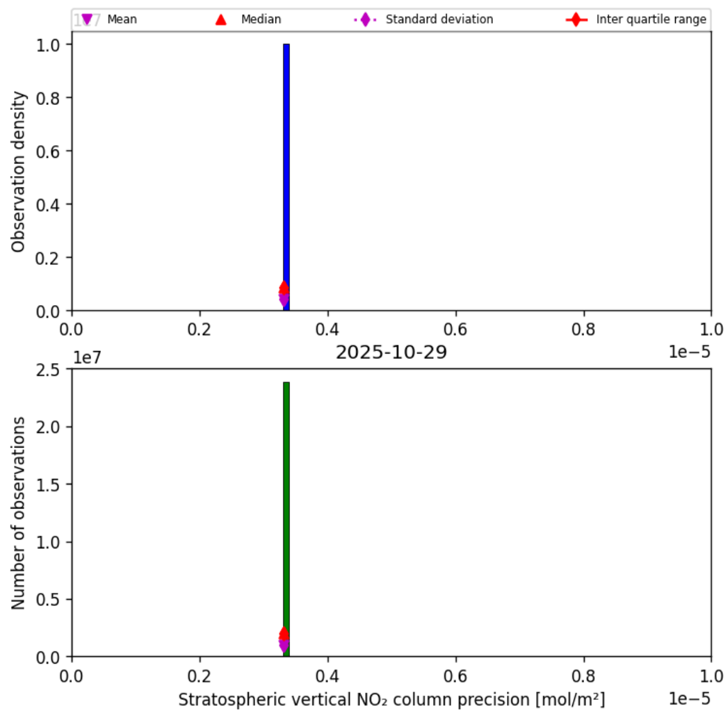
Figure 35: Histogram of “Stratospheric vertical NO 2 column precision” for 2025-10-29 to 2025-10-30
