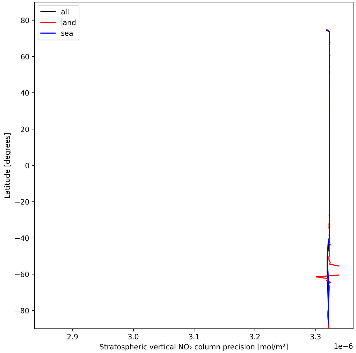
Figure 18: Zonal average of "Stratospheric vertical NO 2 column precision" for 2025-10-29 to 2025-10-30.
