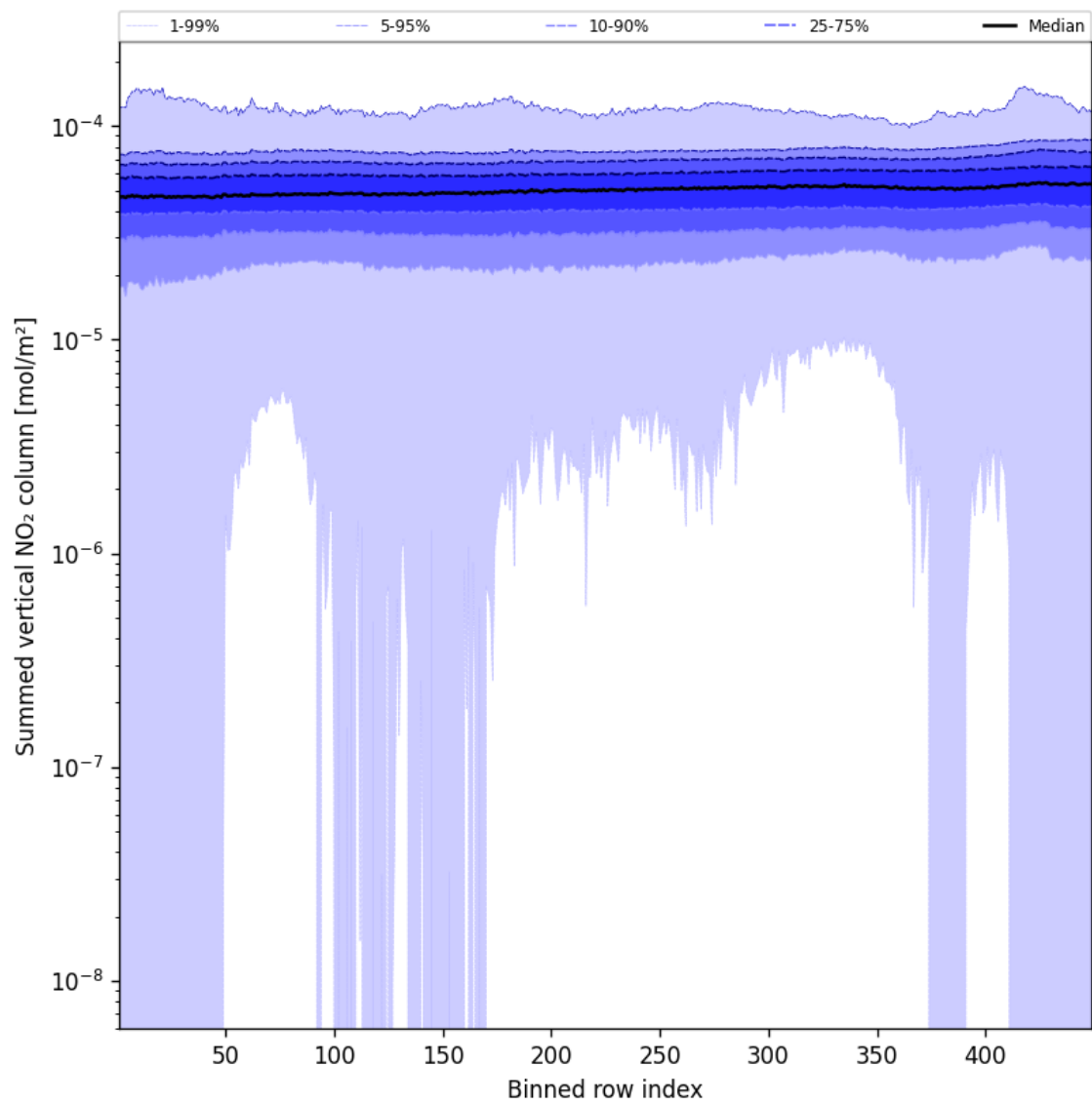
Figure 55: Along track statistics of “Summed vertical NO 2 column” for 2025-10-29 to 2025-10-30
