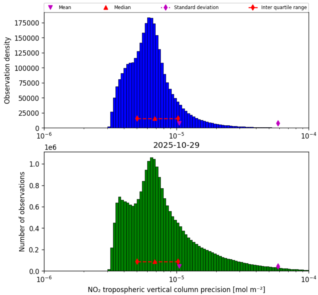
Figure 28: Histogram of “NO 2 tropospheric vertical column precision” for 2025-10-29 to 2025-10-30
