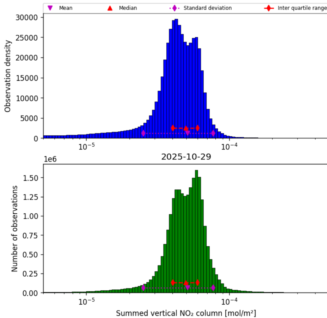
Figure 38: Histogram of “Summed vertical NO 2 column” for 2025-10-29 to 2025-10-30
