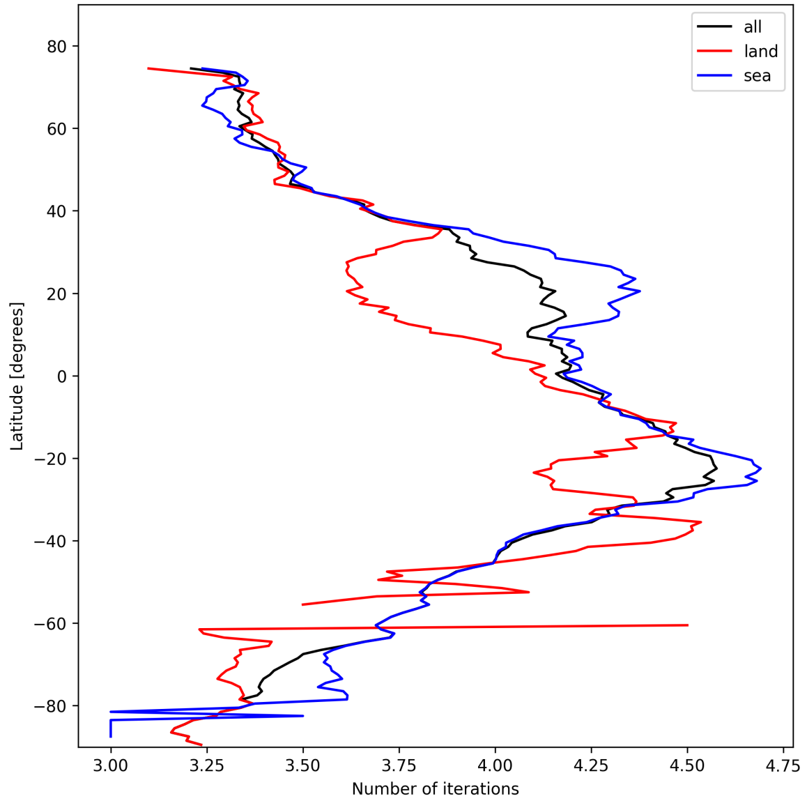
Figure 15: Zonal average of “Number of iterations” for 2025-10-29 to 2025-10-30.
