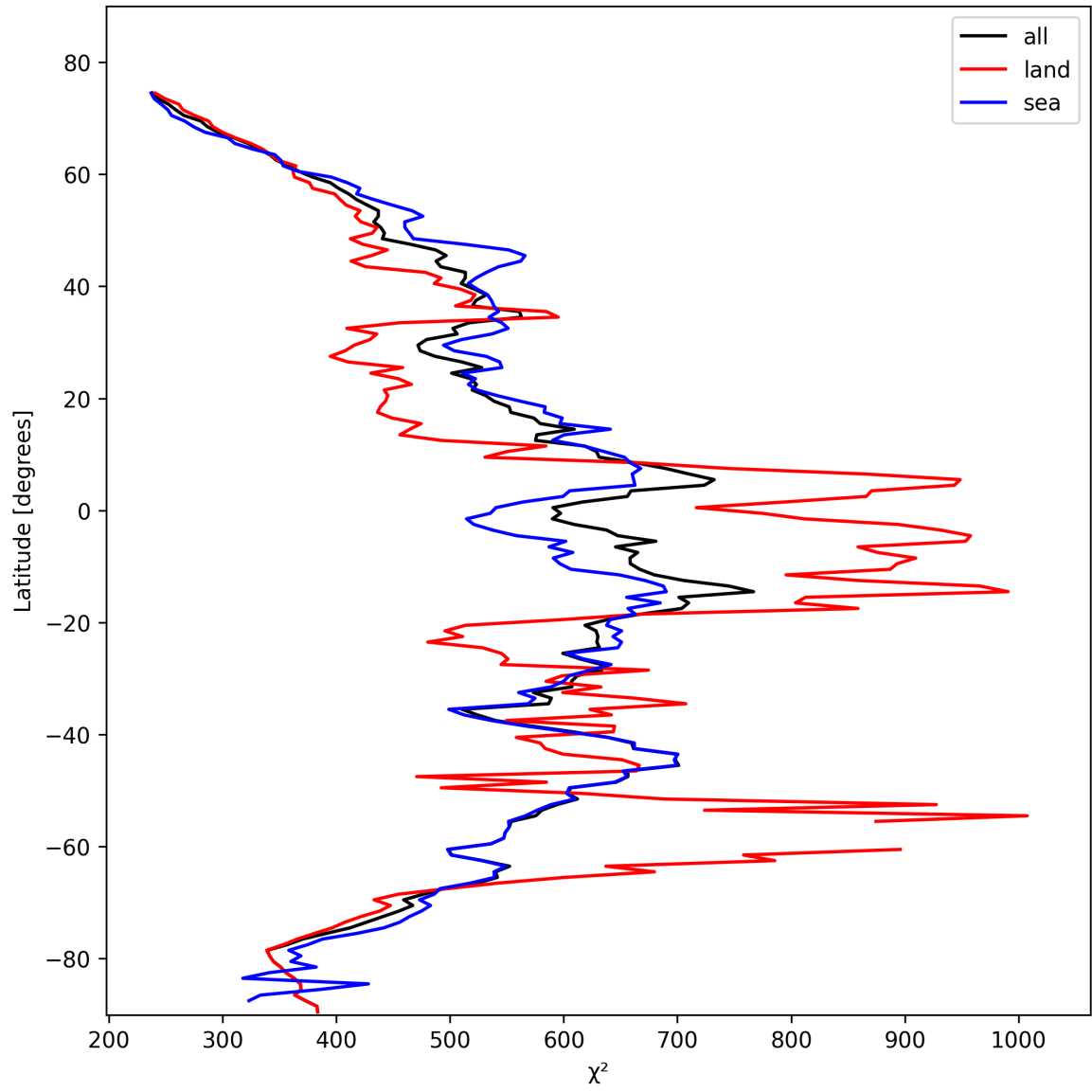
Figure 23: Zonal average of “ \chi^2 ” for 2025-10-29 to 2025-10-30.
