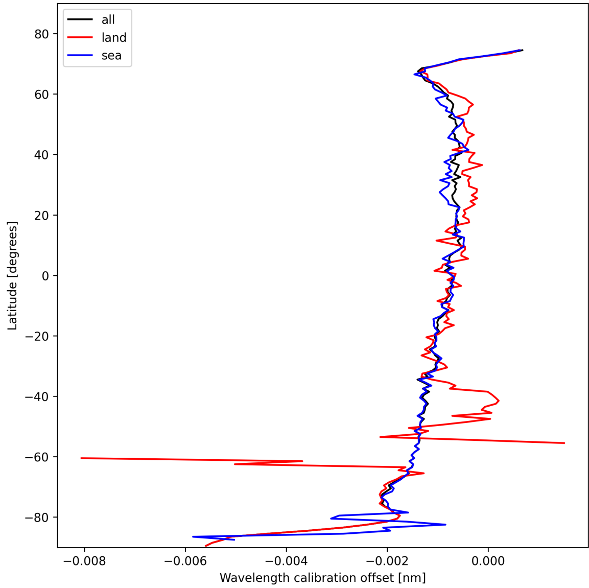
Figure 16: Zonal average of “Wavelength calibration offset” for 2025-10-29 to 2025-10-30.
