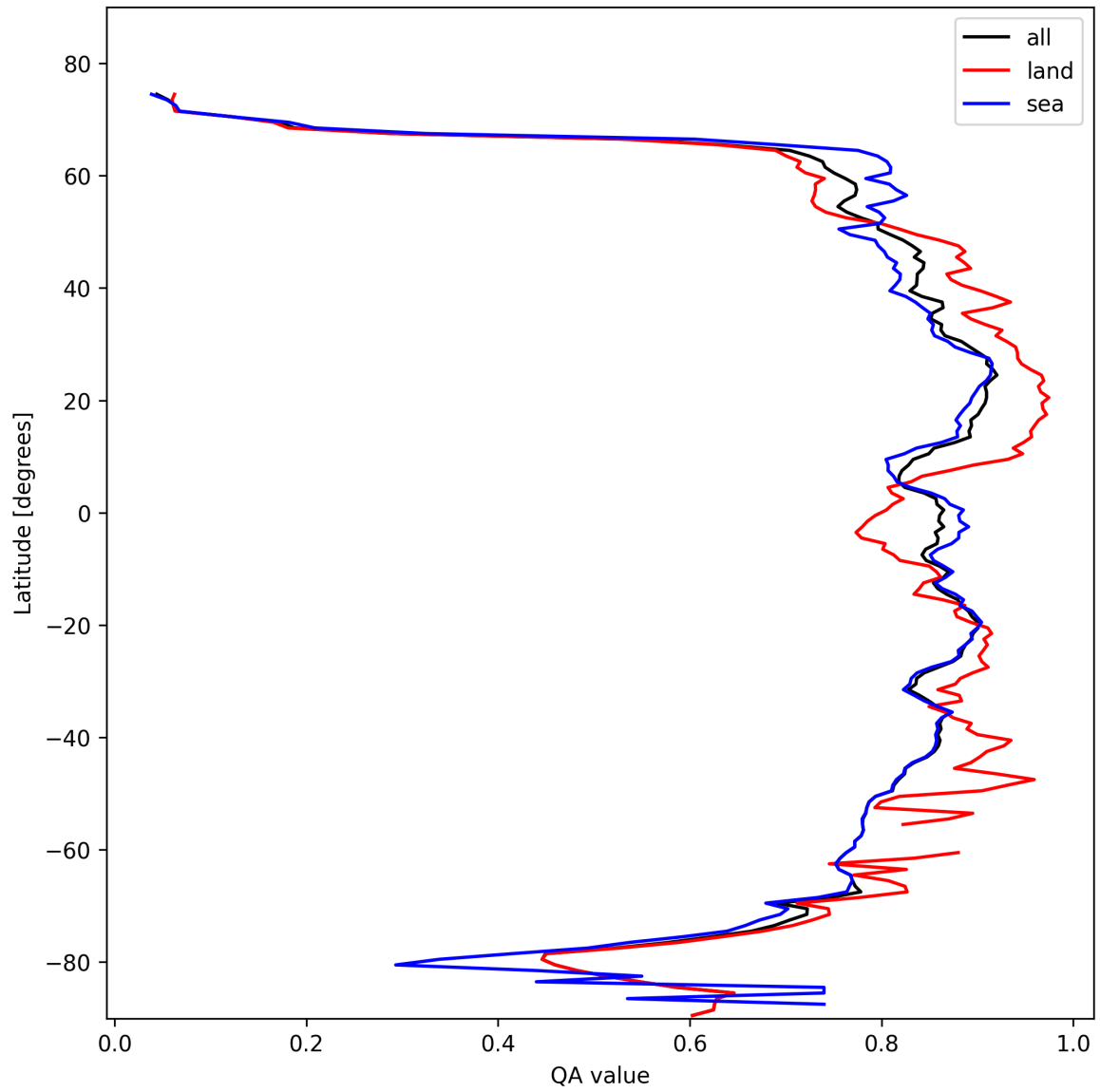
Figure 9: Zonal average of “QA value” for 2025-10-29 to 2025-10-30.
