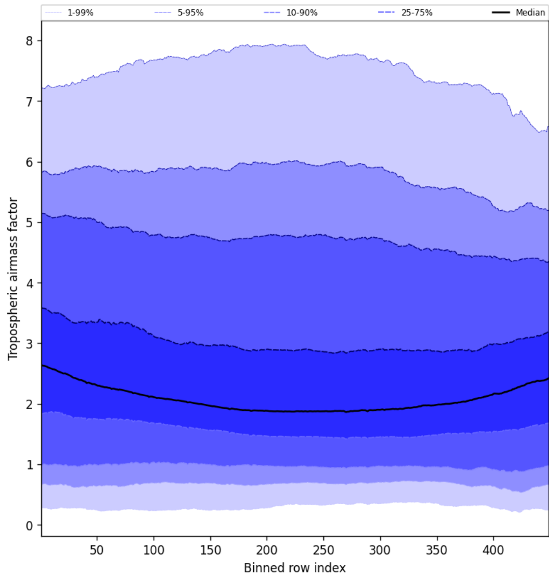
Figure 46: Along track statistics of “Tropospheric airmass factor” for 2025-10-29 to 2025-10-30
