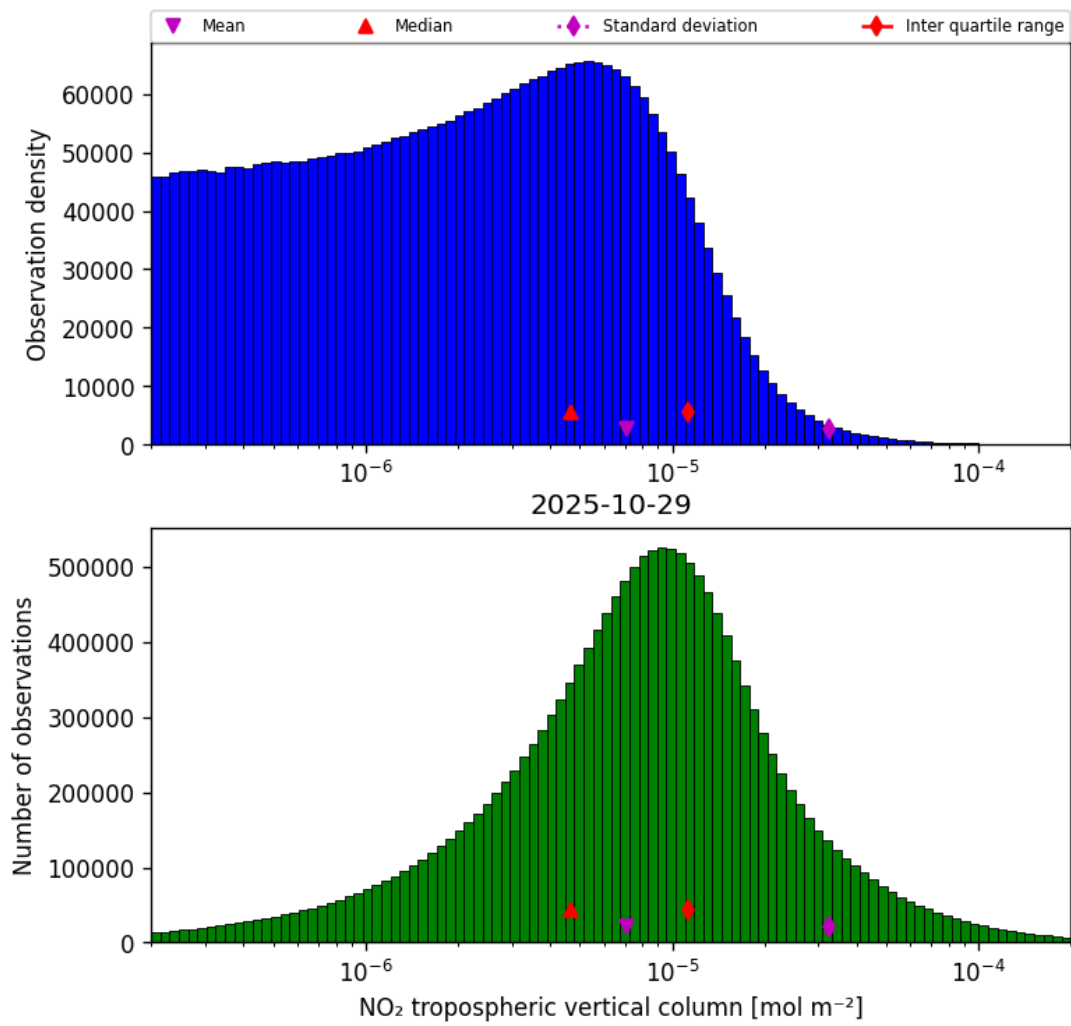
Figure 27: Histogram of “NO 2 tropospheric vertical column” for 2025-10-29 to 2025-10-30
