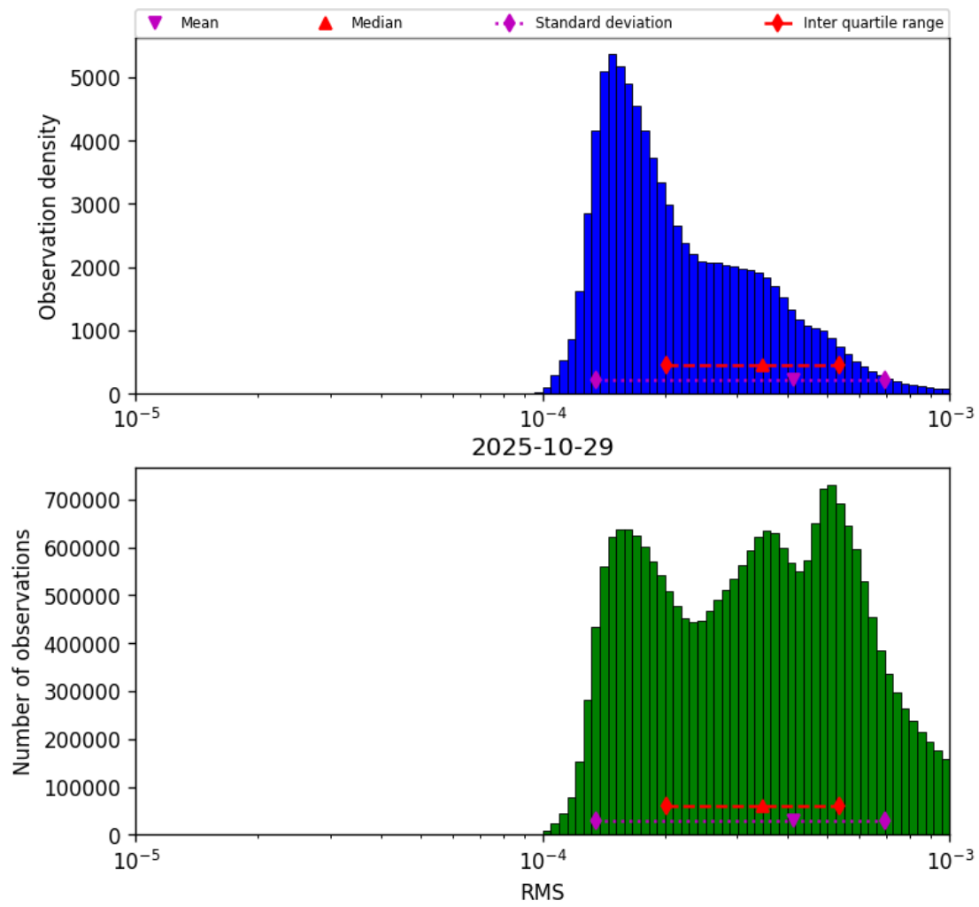
Figure 41: Histogram of “RMS” for 2025-10-29 to 2025-10-30
