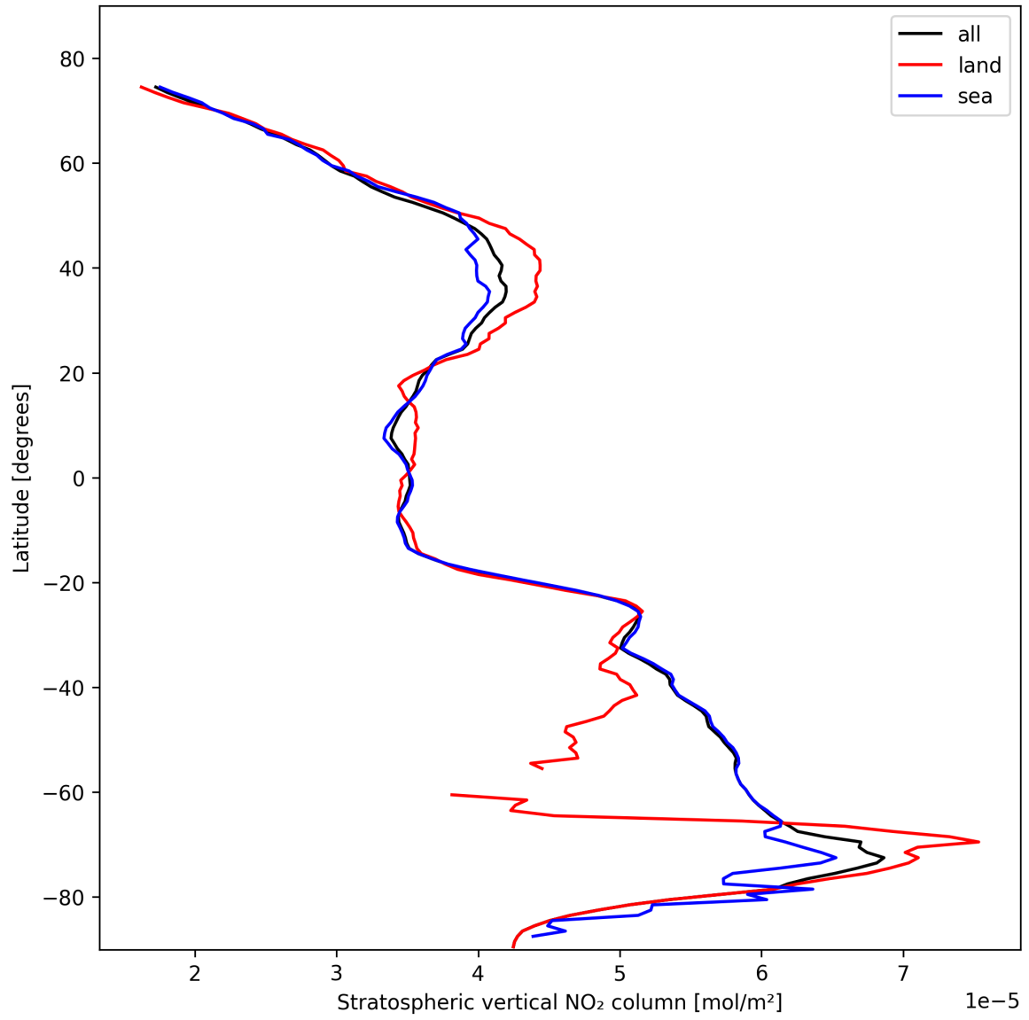
Figure 17: Zonal average of “Stratospheric vertical NO 2 column” for 2025-10-29 to 2025-10-30.
