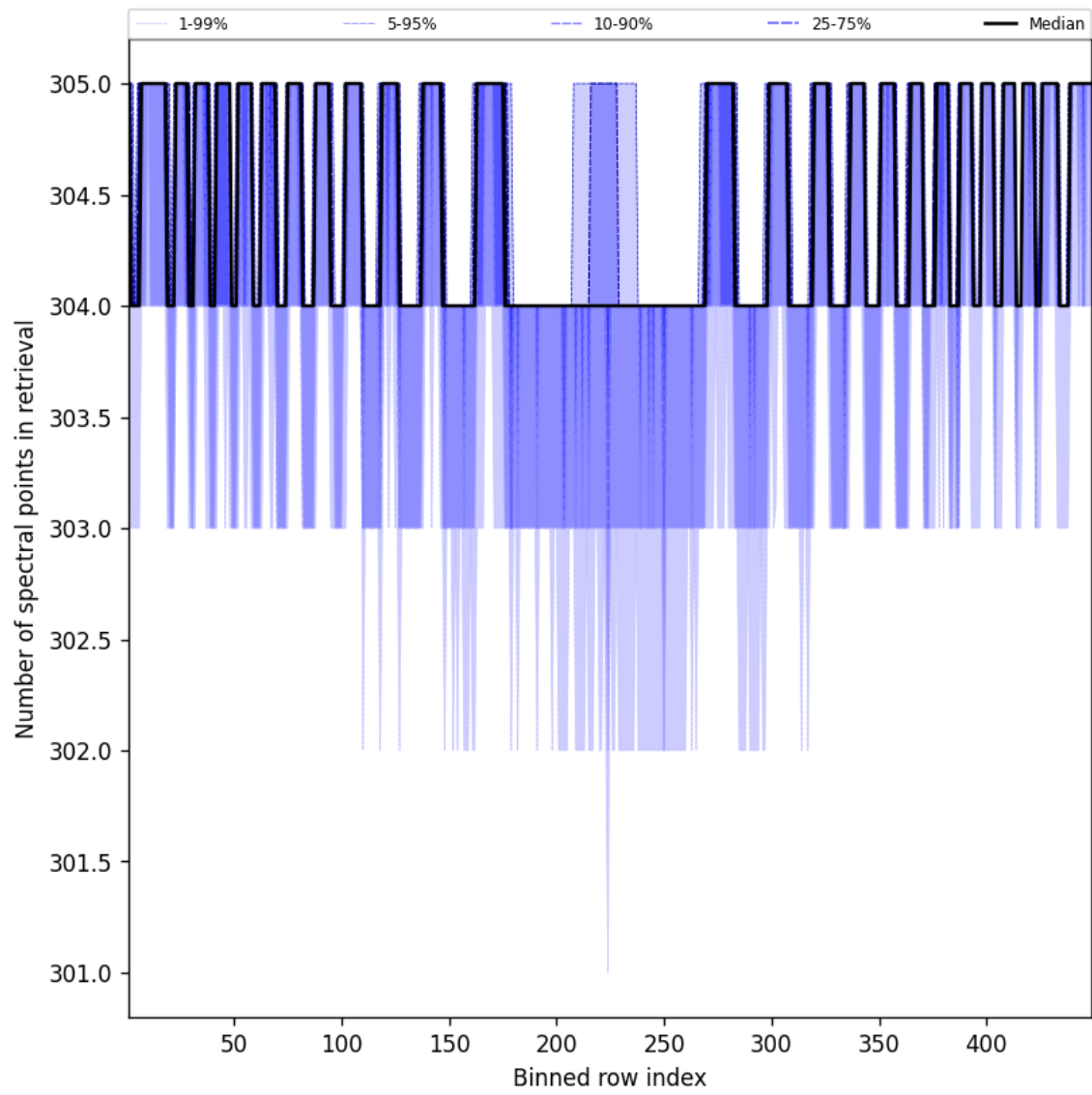
Figure 48: Along track statistics of “Number of spectral points in retrieval” for 2025-10-29 to 2025-10-30
