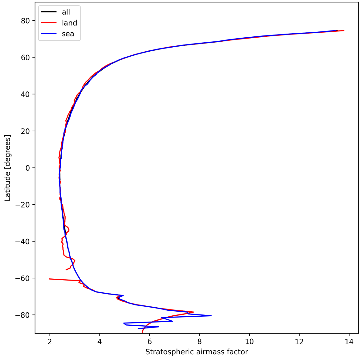
Figure 25: Zonal average of “Stratospheric airmass factor” for 2025-10-29 to 2025-10-30.
