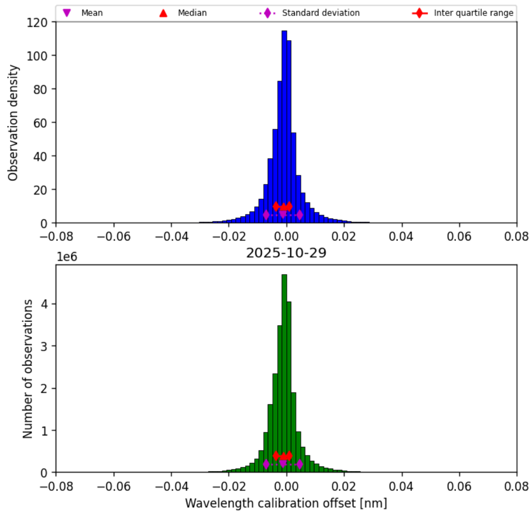
Figure 33: Histogram of “Wavelength calibration offset” for 2025-10-29 to 2025-10-30
