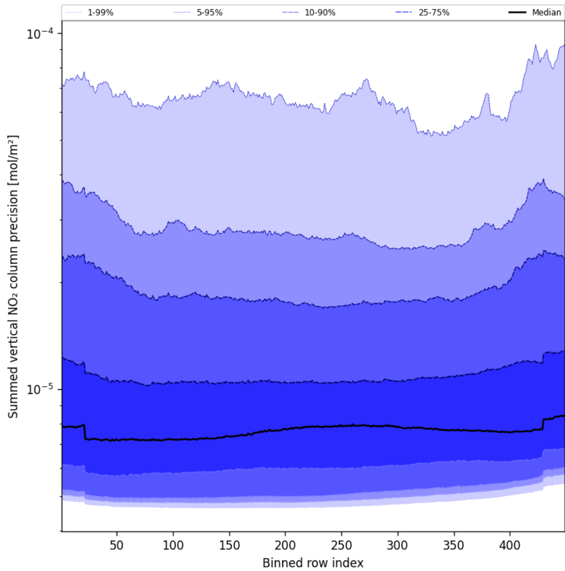
Figure 56: Along track statistics of “Summed vertical NO 2 column precision” for 2025-10-29 to 2025-10-30
