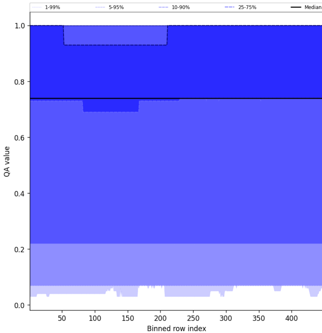
Figure 43: Along track statistics of “QA value” for 2025-10-29 to 2025-10-30
