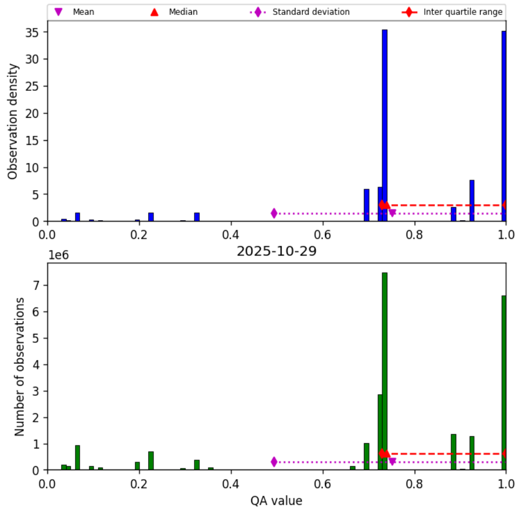
Figure 26: Histogram of “QA value” for 2025-10-29 to 2025-10-30
