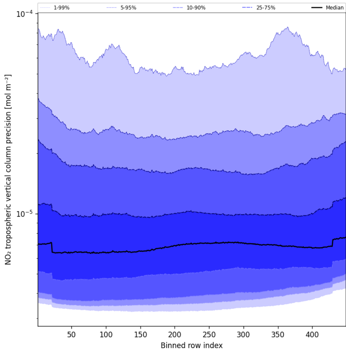
Figure 45: Along track statistics of “NO 2 tropospheric vertical column precision” for 2025-10-30 to 2025-10-30
