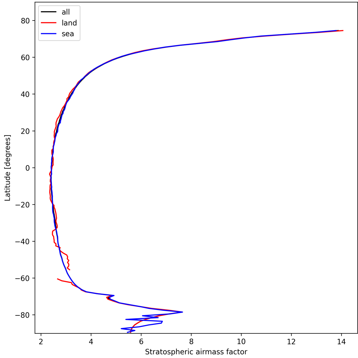
Figure 25: Zonal average of “Stratospheric air mass factor” for 2025-10-30 to 2025-10-30.
