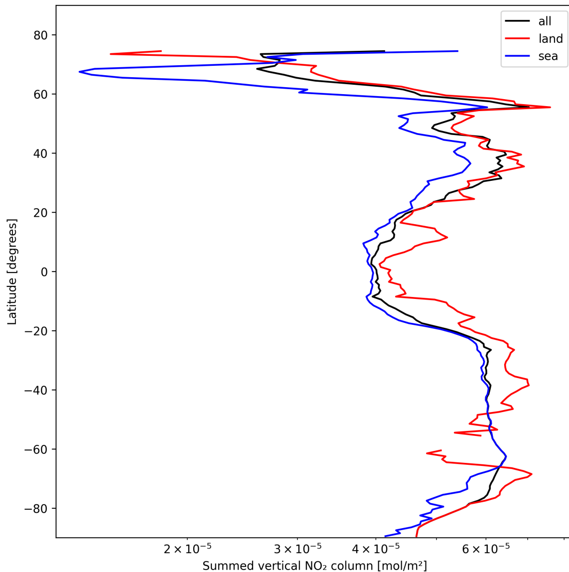
Figure 21: Zonal average of “Summed vertical NO 2 column” for 2025-10-30 to 2025-10-30.
