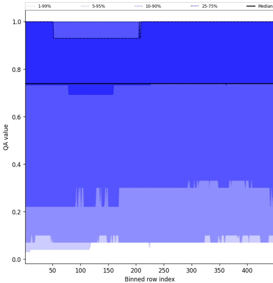
Figure 43: Along track statistics of “QA value” for 2025-10-30 to 2025-10-30
