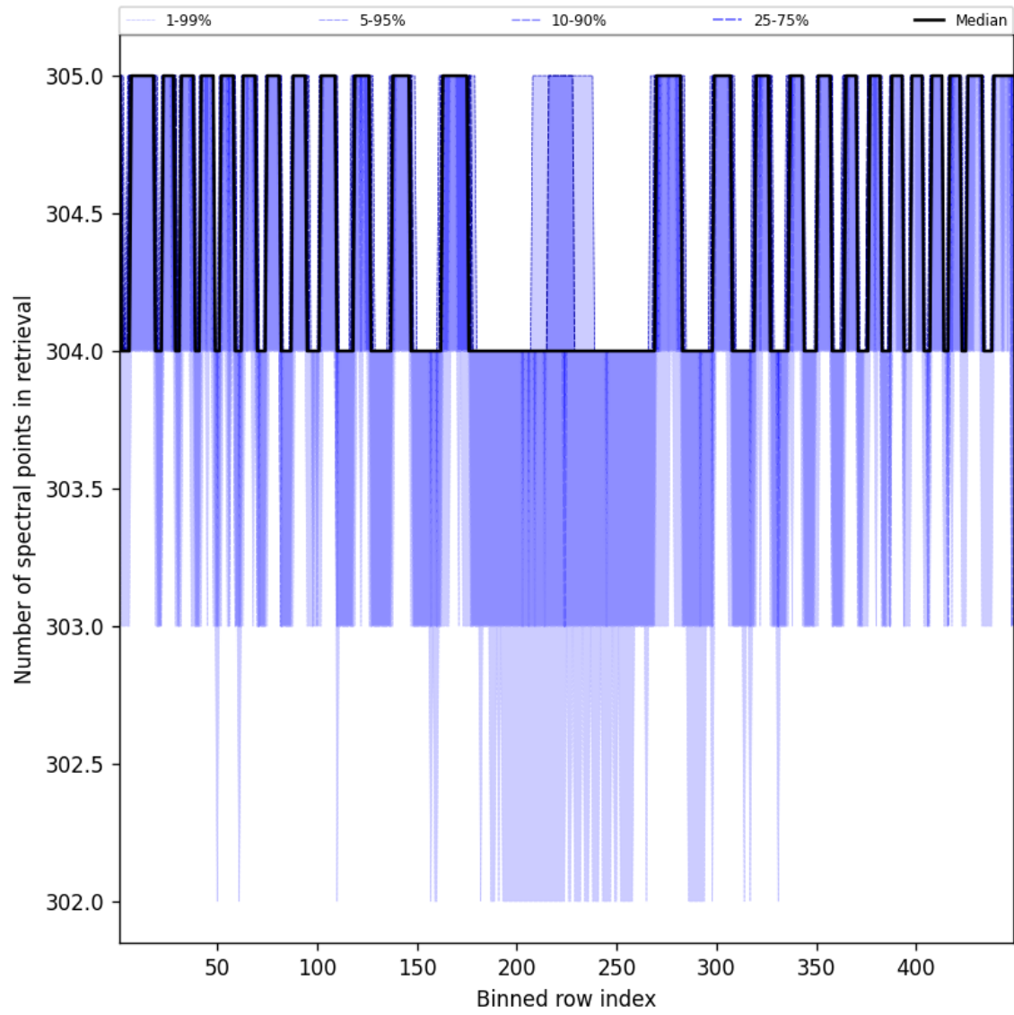
Figure 48: Along track statistics of “Number of spectral points in retrieval” for 2025-10-30 to 2025-10-30
