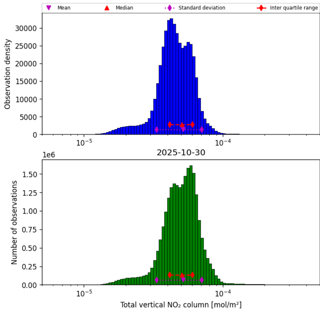
Figure 36: Histogram of “Total vertical NO 2 column” for 2025-10-30 to 2025-10-30
