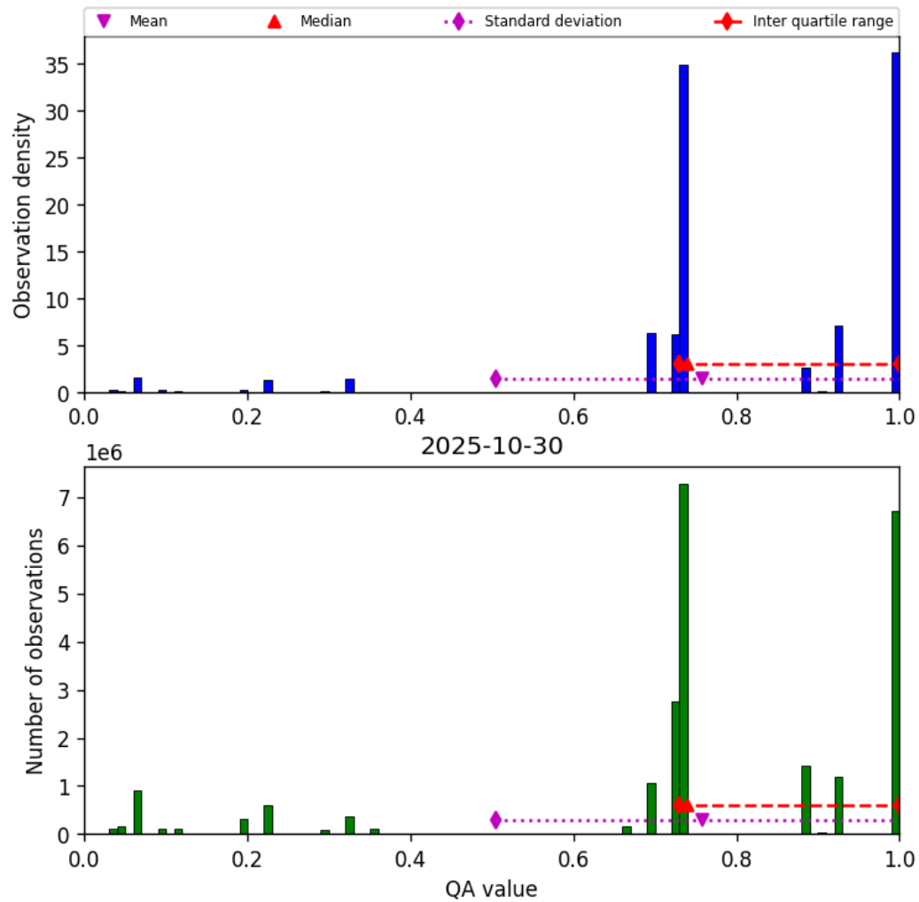
Figure 26: Histogram of “QA value” for 2025-10-30 to 2025-10-30
