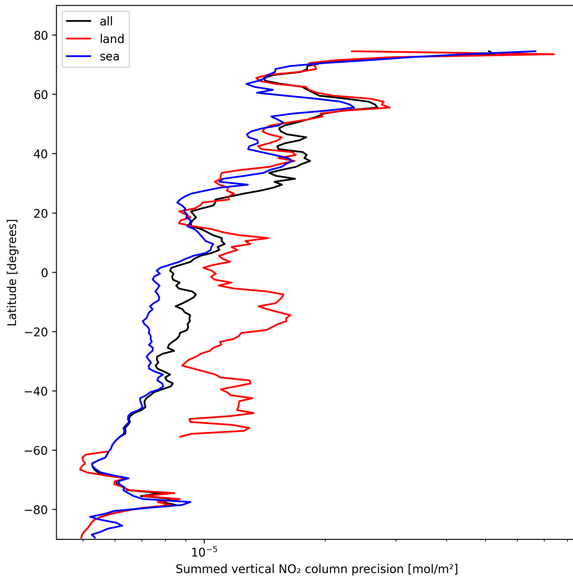
Figure 22: Zonal average of “Summed vertical NO 2 column precision” for 2025-10-30 to 2025-10-30.
