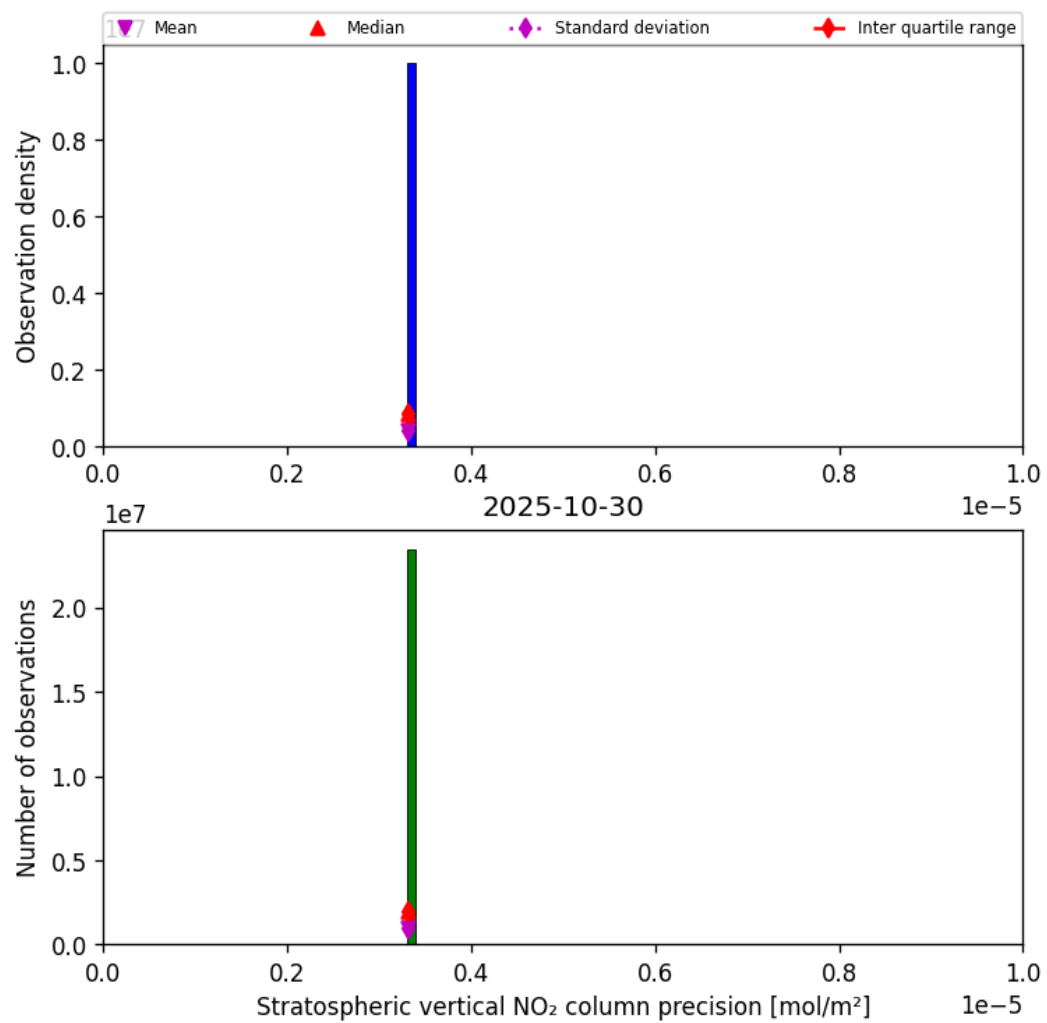
Figure 35: Histogram of “Stratospheric vertical NO 2 column precision” for 2025-10-30 to 2025-10-30
