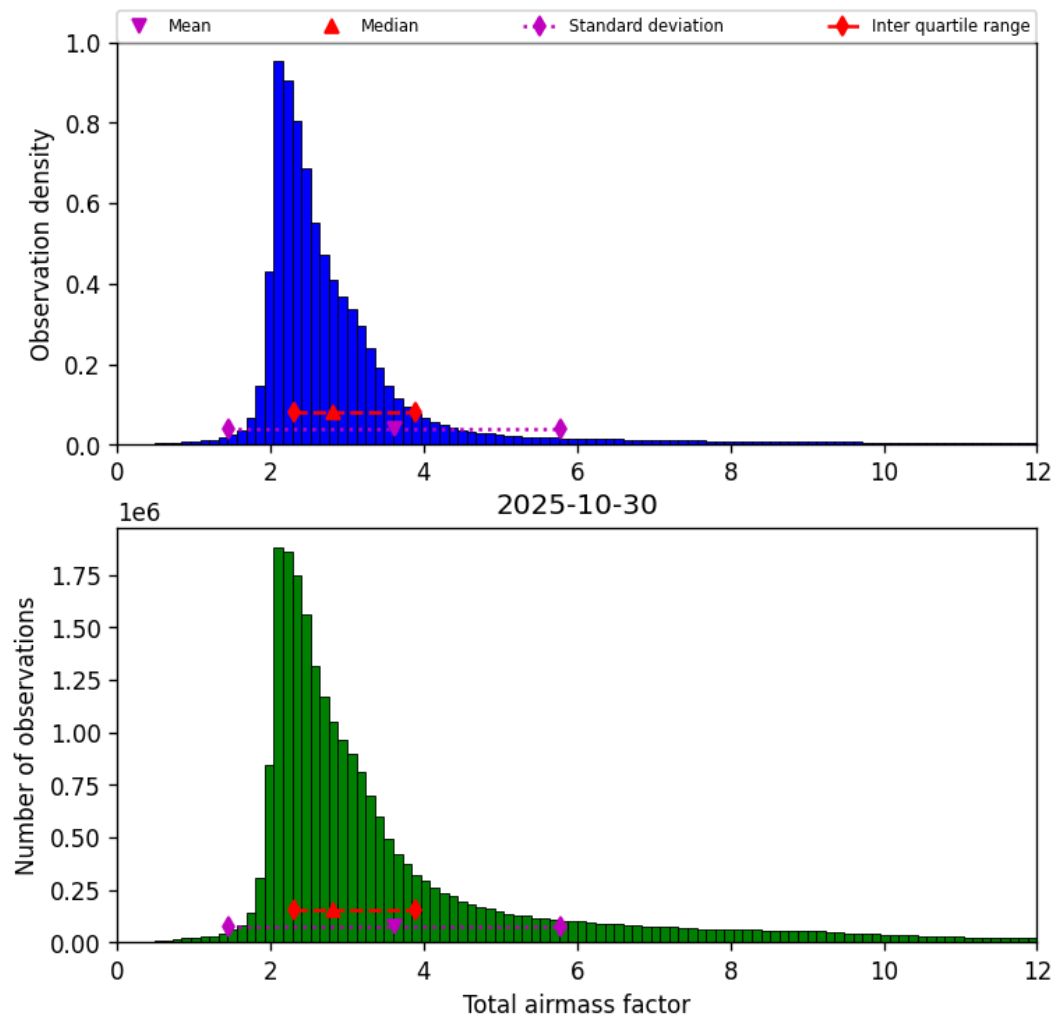
Figure 30: Histogram of “Total airmass factor” for 2025-10-30 to 2025-10-30
