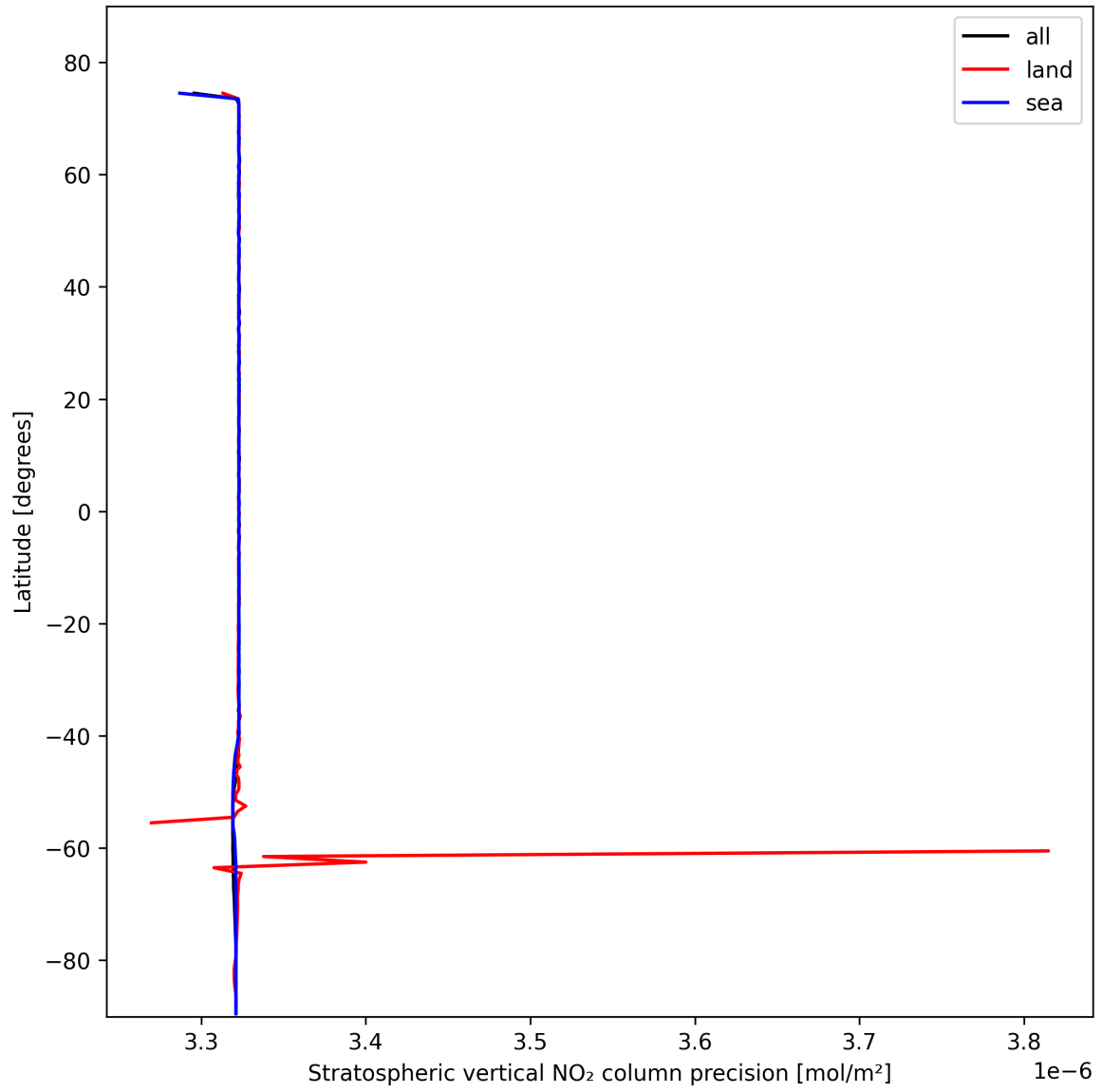
Figure 18: Zonal average of “Stratospheric vertical NO 2 column precision” for 2025-10-30 to 2025-10-30.
