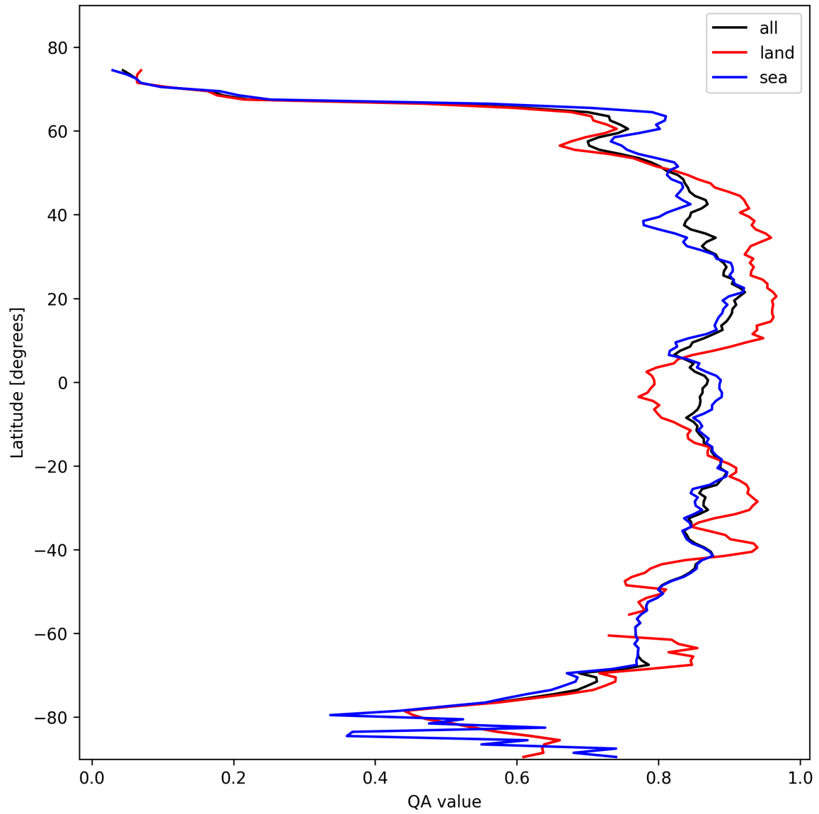
Figure 9: Zonal average of “QA value” for 2025-10-30 to 2025-10-30.
