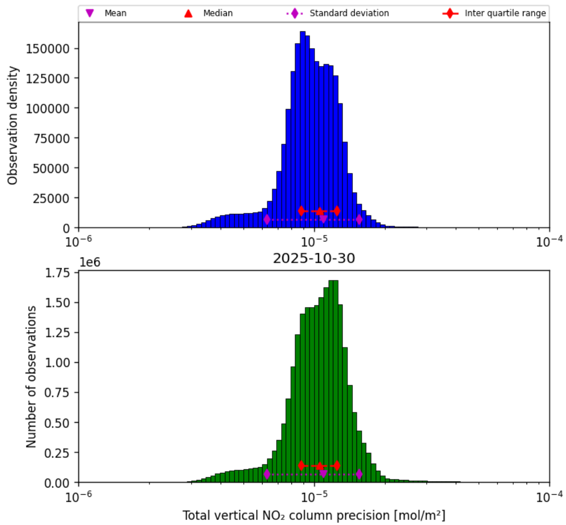
Figure 37: Histogram of "Total vertical NO 2 column precision" for 2025-10-30 to 2025-10-30
