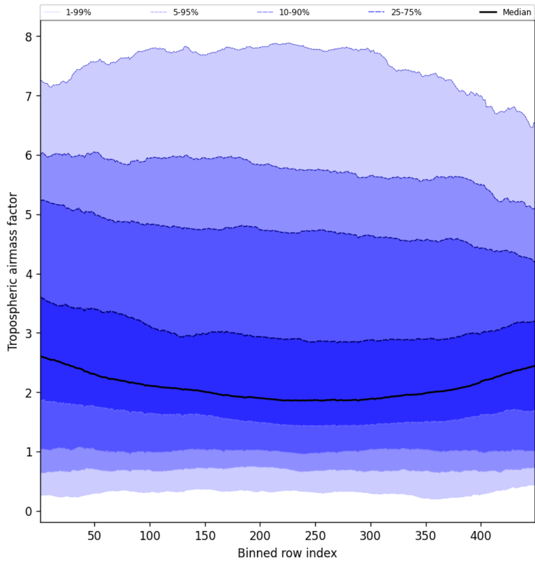
Figure 46: Along track statistics of “Tropospheric air mass factor” for 2025-10-30 to 2025-10-30
