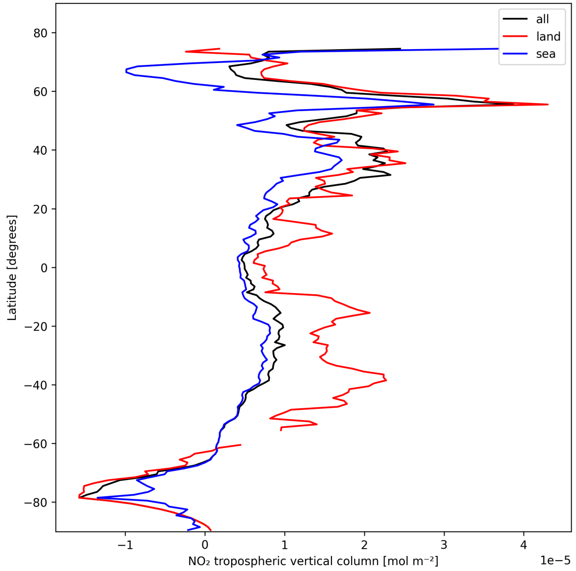
Figure 10: Zonal average of “NO 2 tropospheric vertical column” for 2025-10-30 to 2025-10-30.
