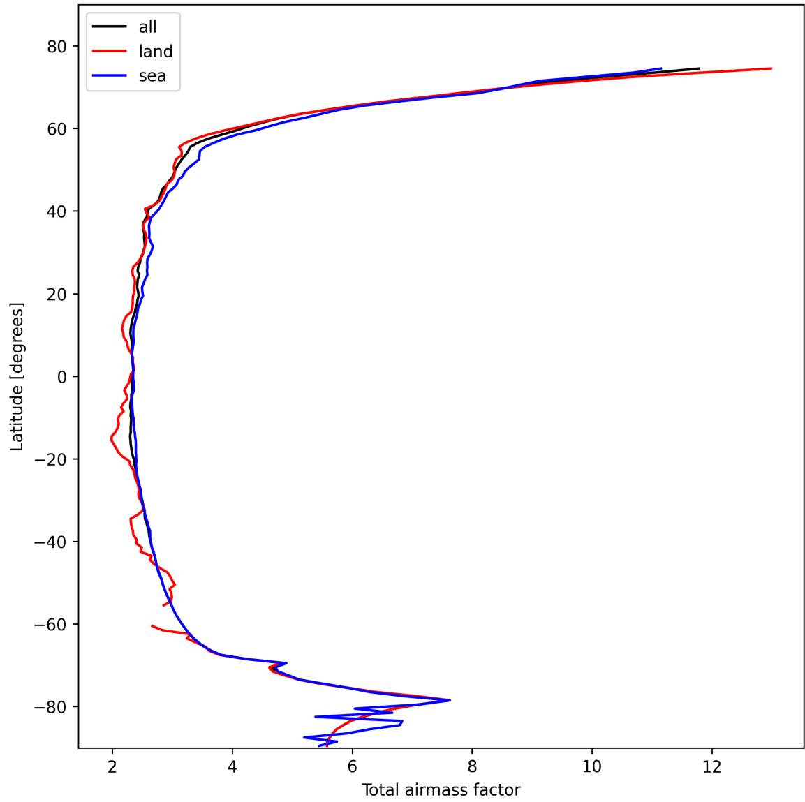
Figure 13: Zonal average of “Total airmass factor” for 2025-10-30 to 2025-10-30.
