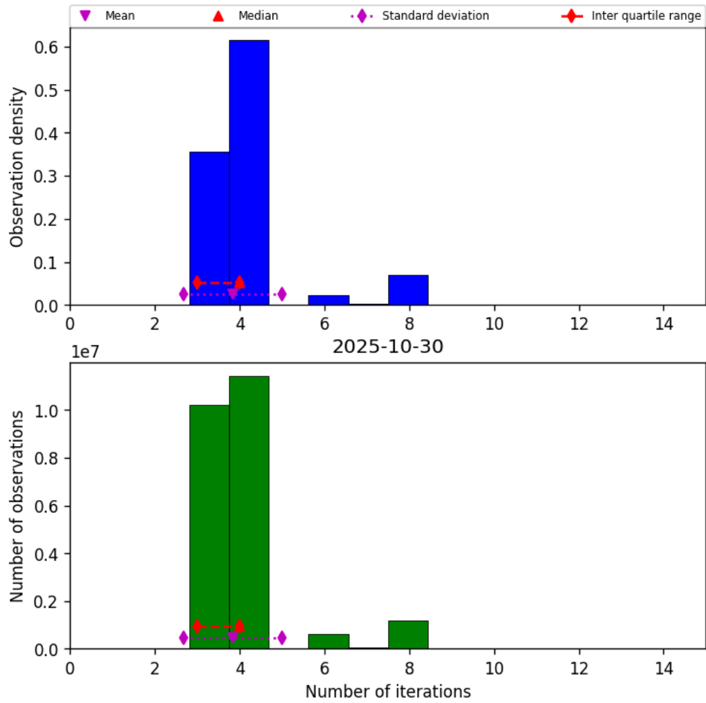
Figure 32: Histogram of “Number of iterations” for 2025-10-30 to 2025-10-30
