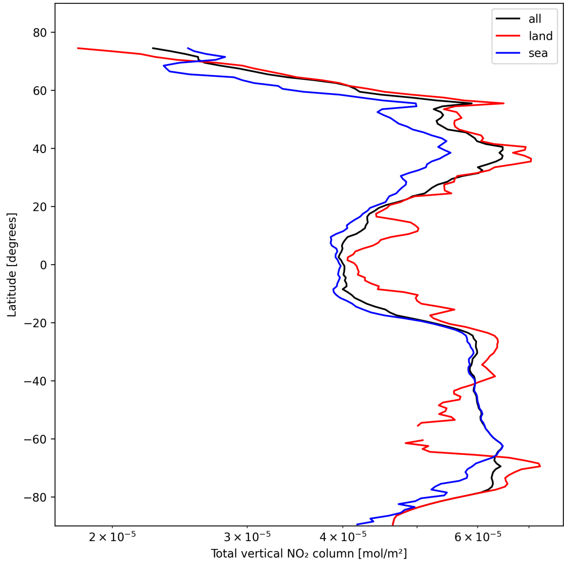
Figure 19: Zonal average of “Total vertical NO 2 column” for 2025-10-30 to 2025-10-30.
