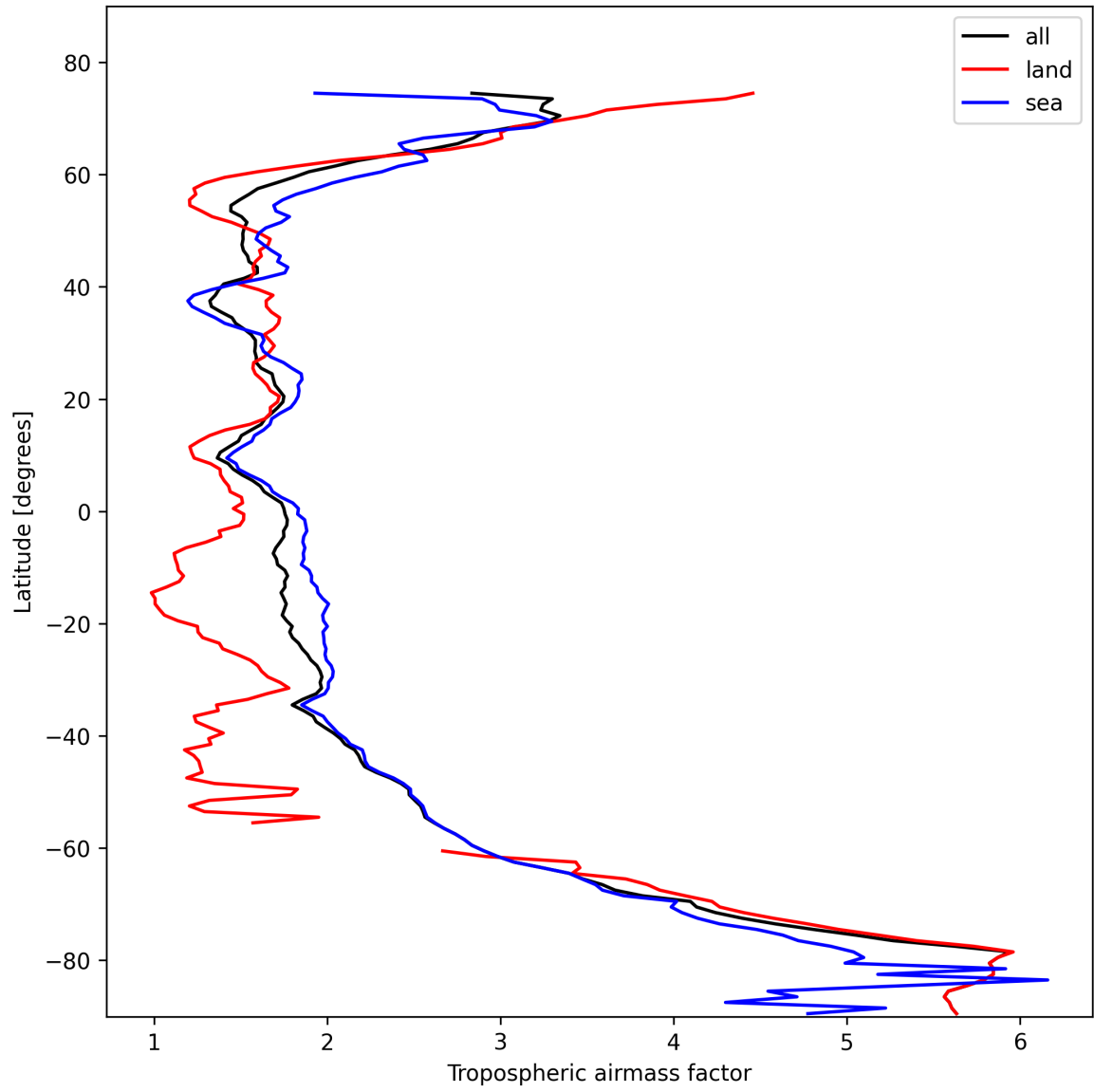
Figure 12: Zonal average of “Tropospheric airmass factor” for 2025-10-30 to 2025-10-30.
