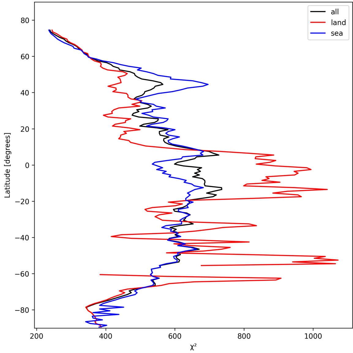
Figure 23: Zonal average of “ \chi^2 ” for 2025-10-30 to 2025-10-30.
