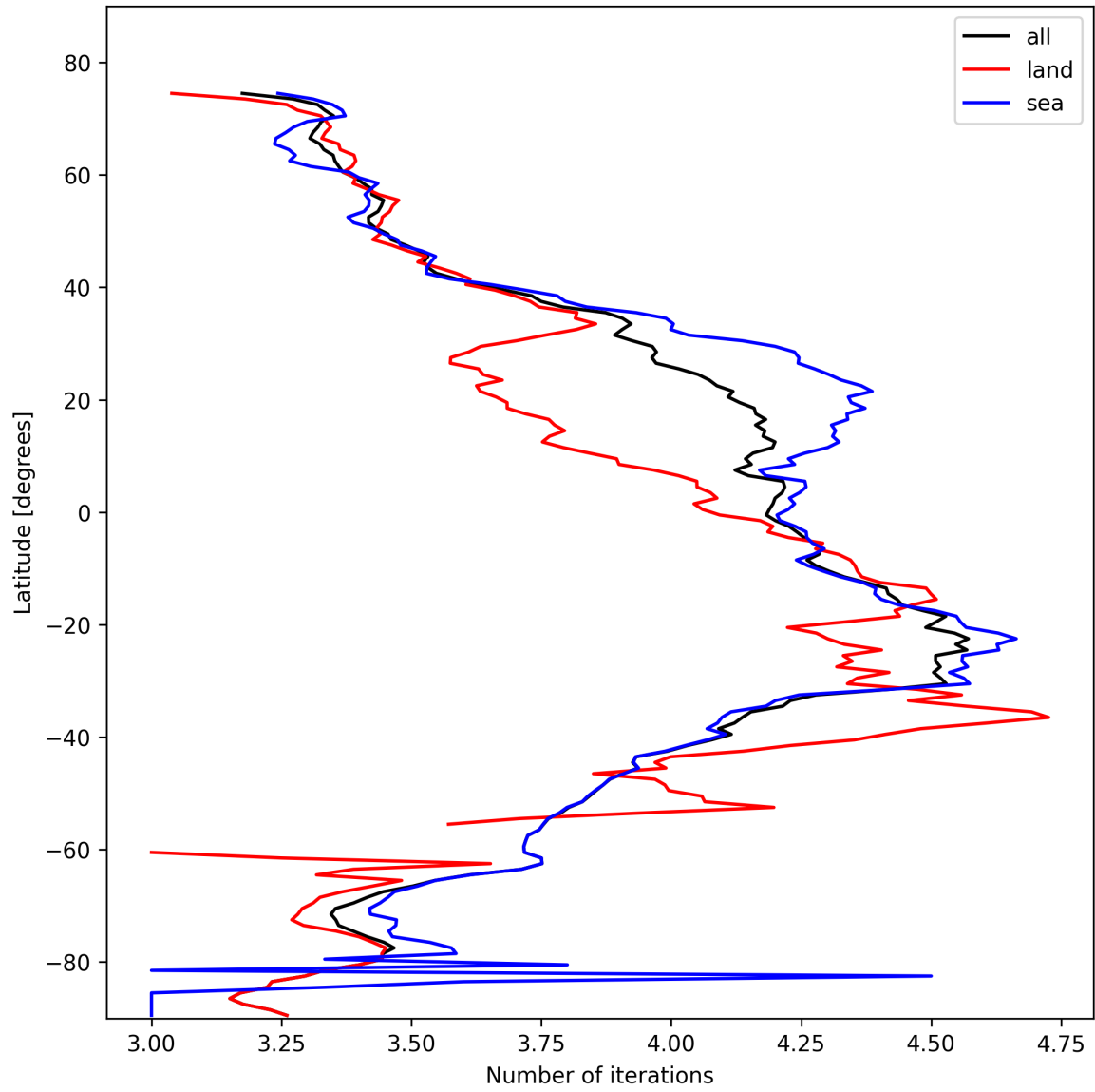
Figure 15: Zonal average of “Number of iterations” for 2025-10-30 to 2025-10-30.
