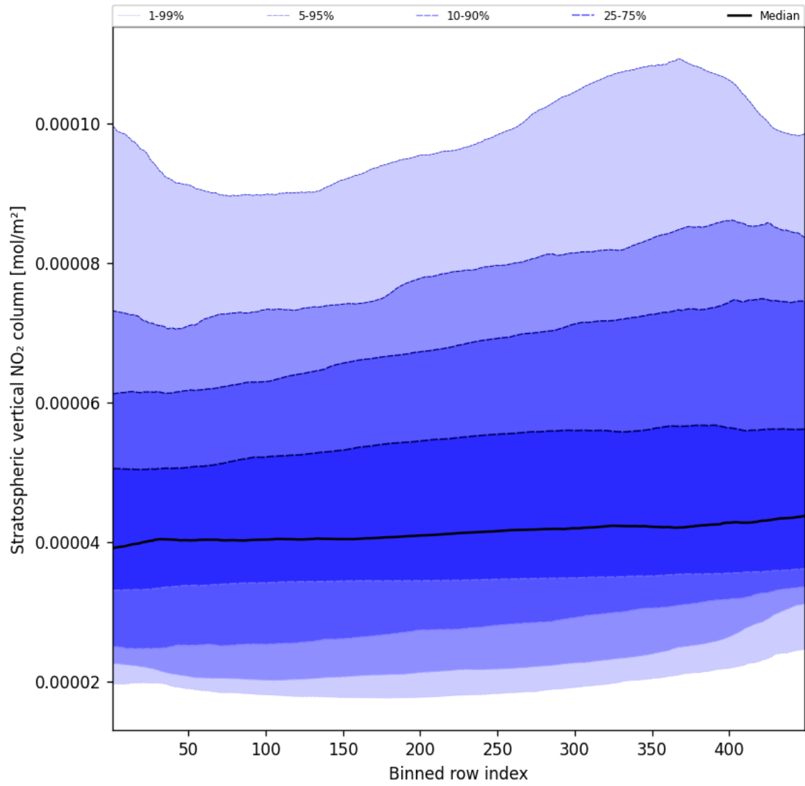
Figure 51: Along track statistics of “Stratospheric vertical NO 2 column” for 2025-10-30 to 2025-10-30
