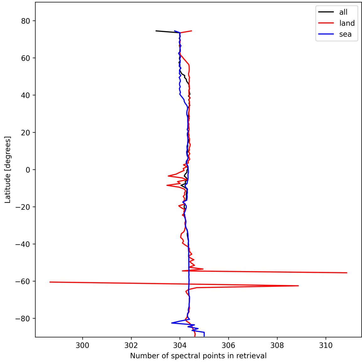
Figure 14: Zonal average of “Number of spectral points in retrieval” for 2025-10-30 to 2025-10-30.
