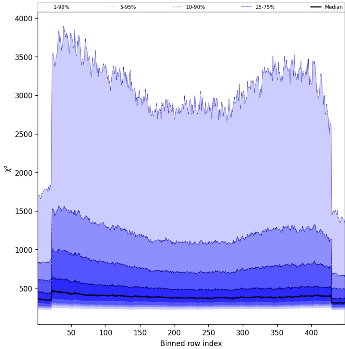
Figure 57: Along track statistics of “ \chi^2 ” for 2025-10-30 to 2025-10-30
