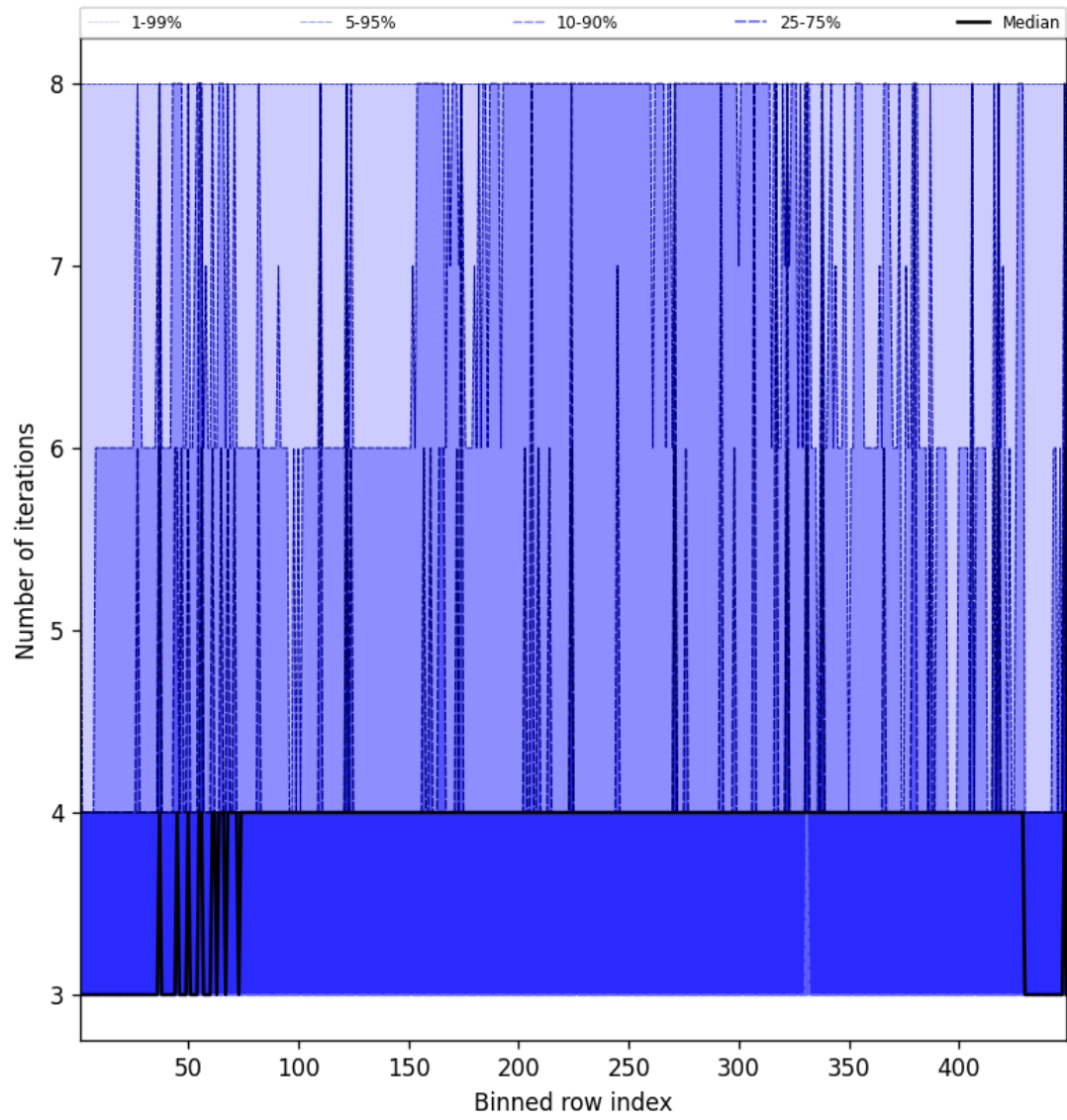
Figure 49: Along track statistics of “Number of iterations” for 2025-10-30 to 2025-10-30
