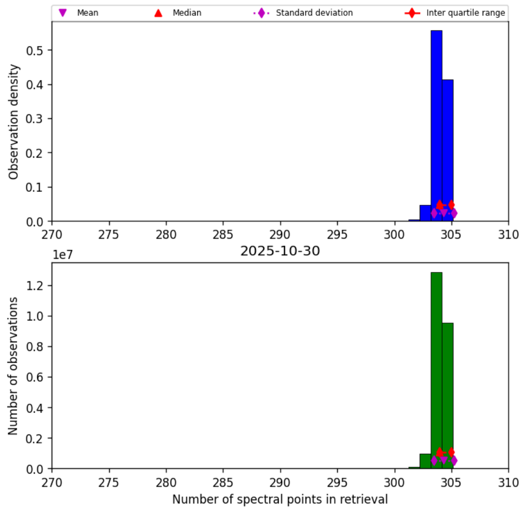
Figure 31: Histogram of “Number of spectral points in retrieval” for 2025-10-30 to 2025-10-30
