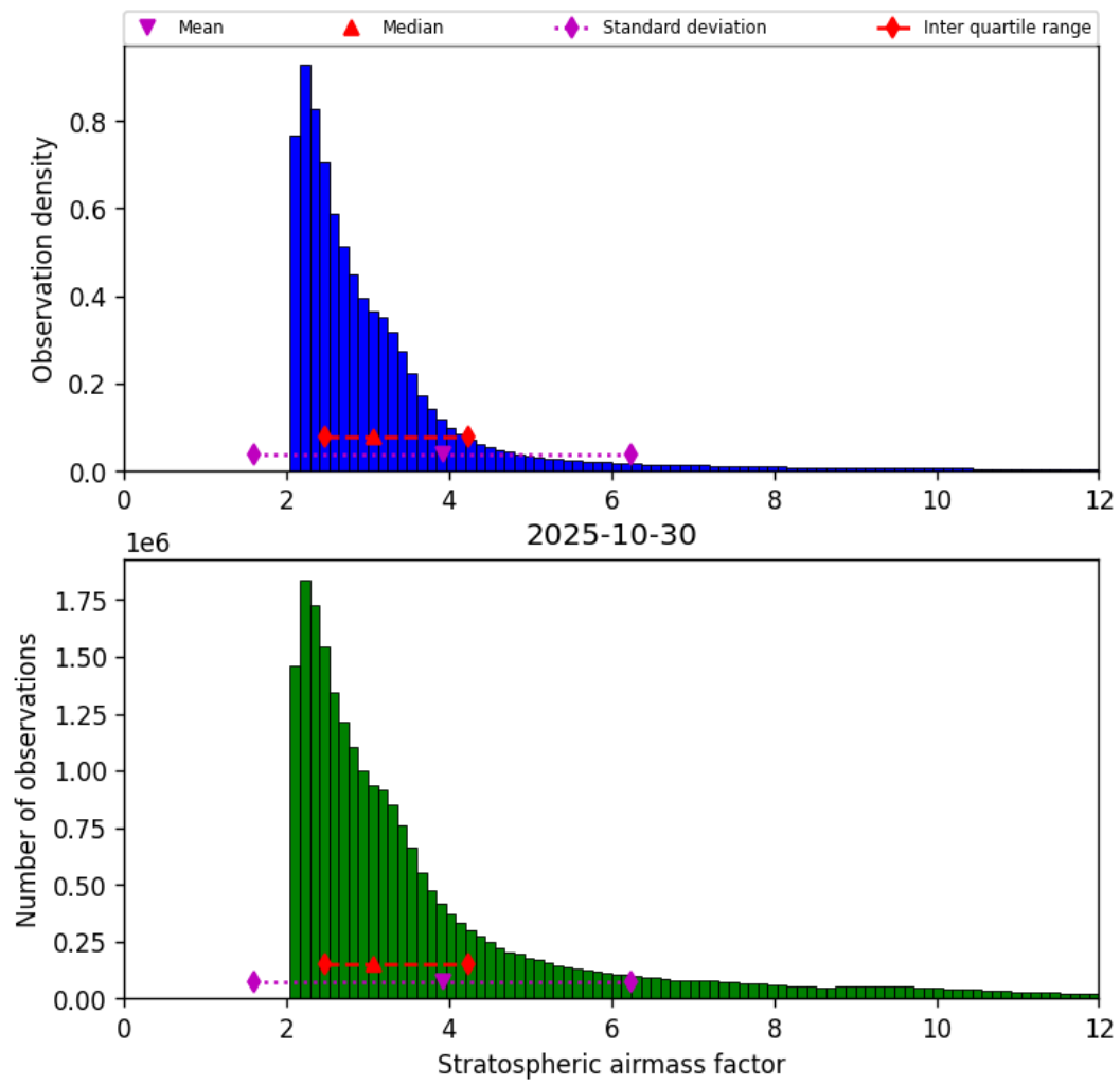
Figure 42: Histogram of “Stratospheric airmass factor” for 2025-10-30 to 2025-10-30
