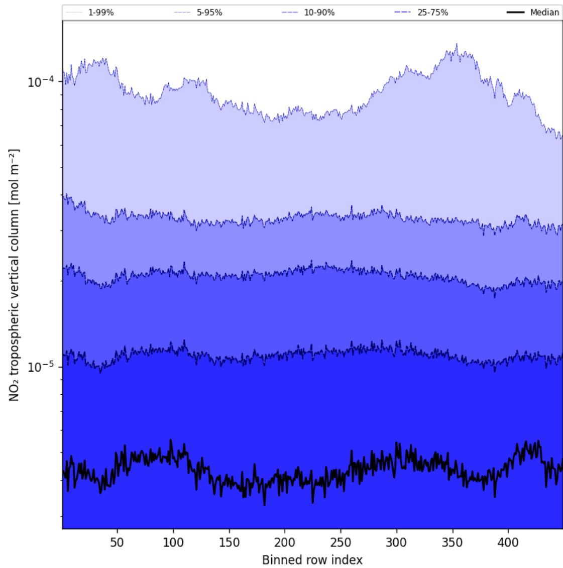
Figure 44: Along track statistics of “NO 2 tropospheric vertical column” for 2025-10-30 to 2025-10-30
