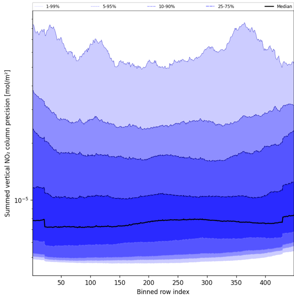
Figure 56: Along track statistics of “Summed vertical NO 2 column precision” for 2025-10-30 to 2025-10-30
