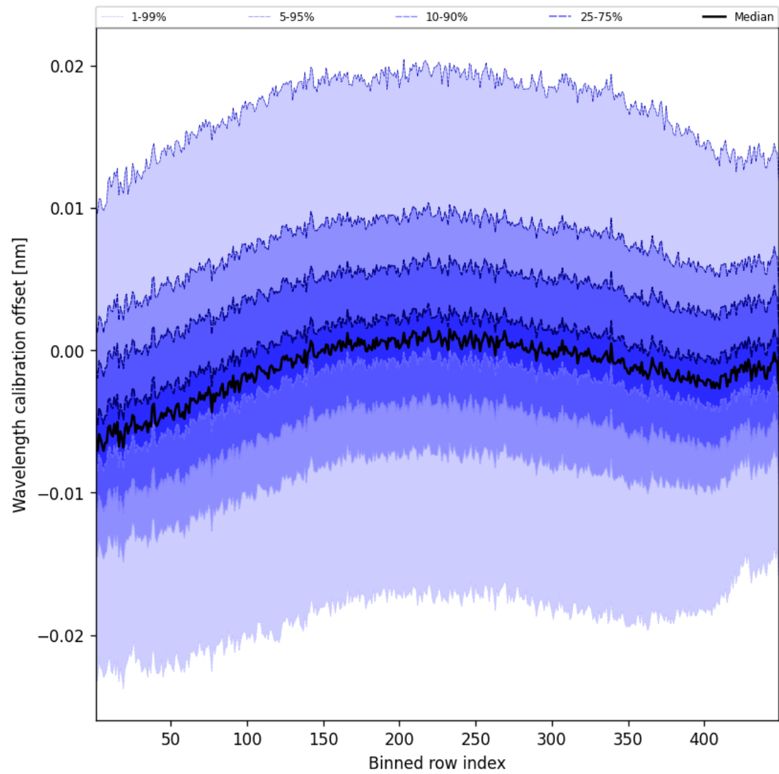
Figure 50: Along track statistics of “Wavelength calibration offset” for 2025-10-30 to 2025-10-30
