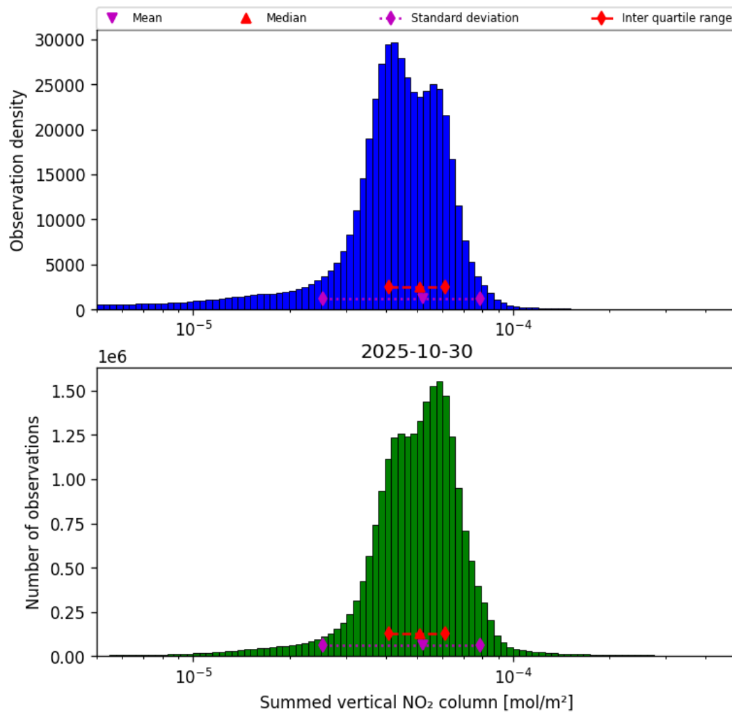
Figure 38: Histogram of "Summed vertical NO 2 column" for 2025-10-30 to 2025-10-30
