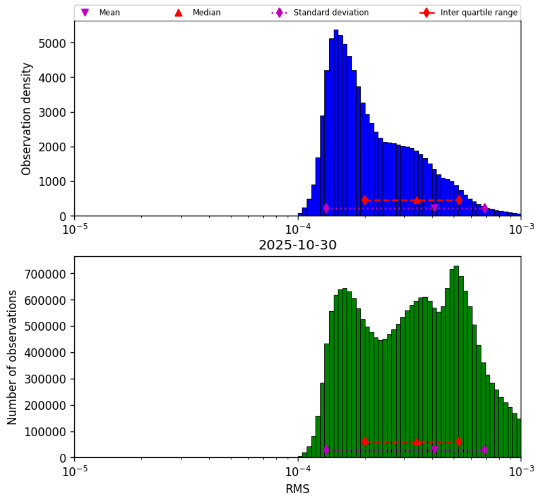
Figure 41: Histogram of “RMS” for 2025-10-30 to 2025-10-30
