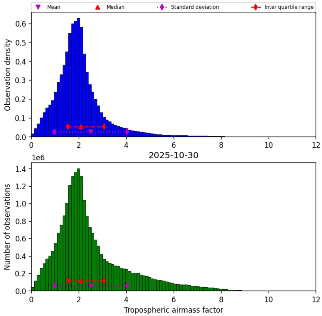
Figure 29: Histogram of “Tropospheric airmass factor” for 2025-10-30 to 2025-10-30
