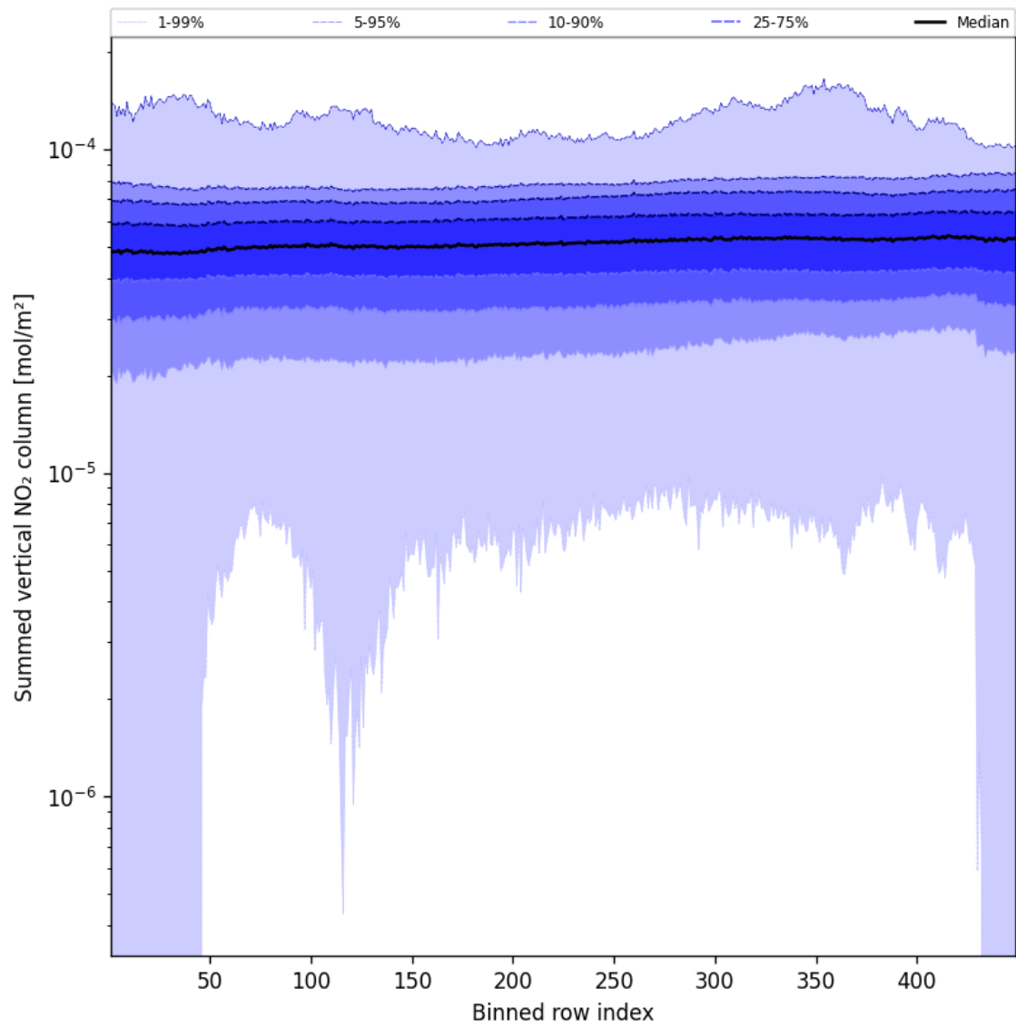
Figure 55: Along track statistics of “Summed vertical NO 2 column” for 2025-10-30 to 2025-10-30
