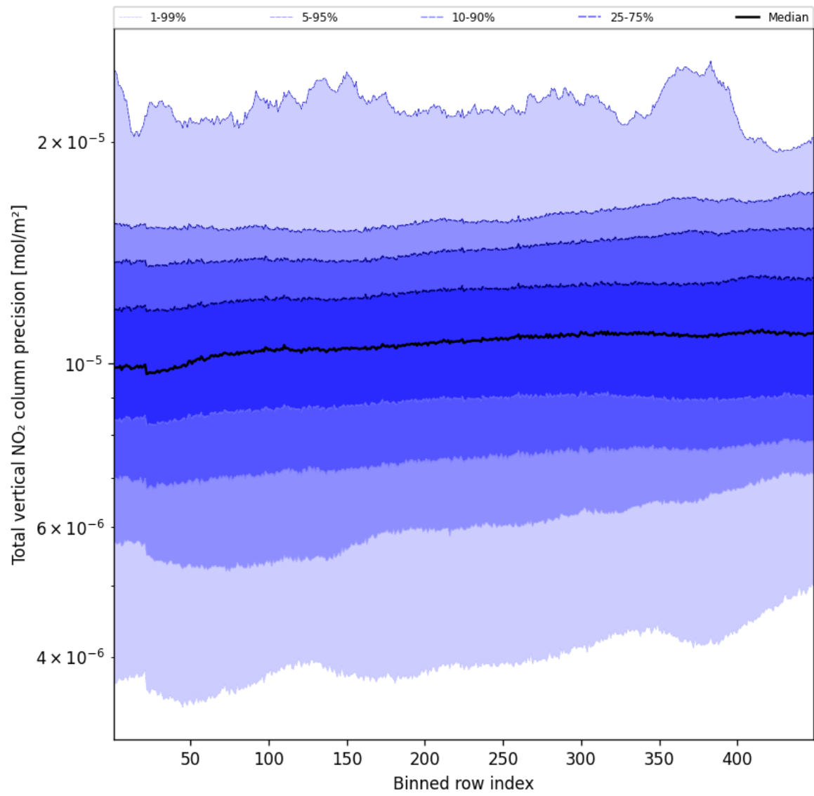
Figure 54: Along track statistics of “Total vertical NO 2 column precision” for 2025-10-30 to 2025-10-30
