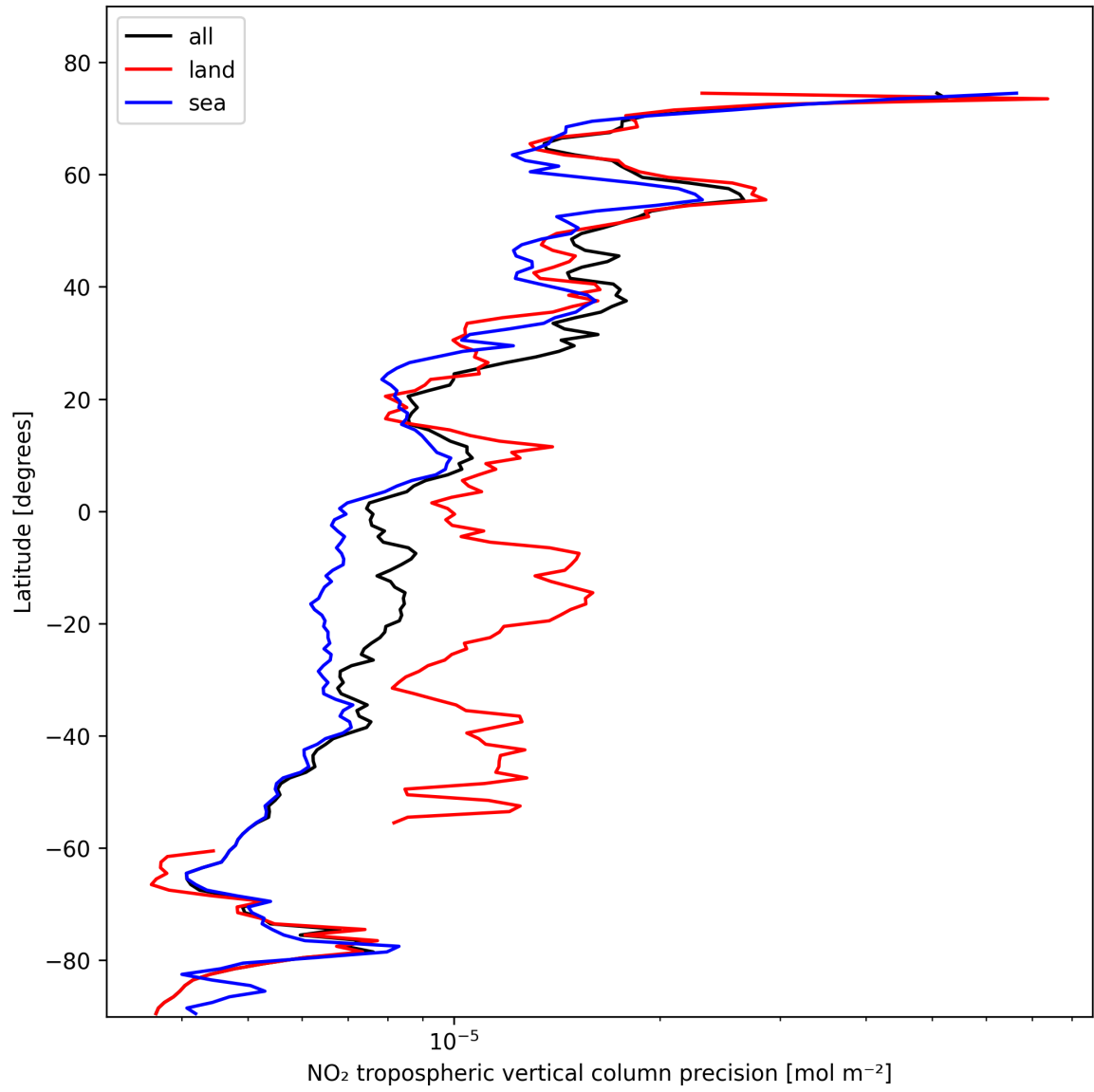
Figure 11: Zonal average of “NO 2 tropospheric vertical column precision” for 2025-10-30 to 2025-10-30.
