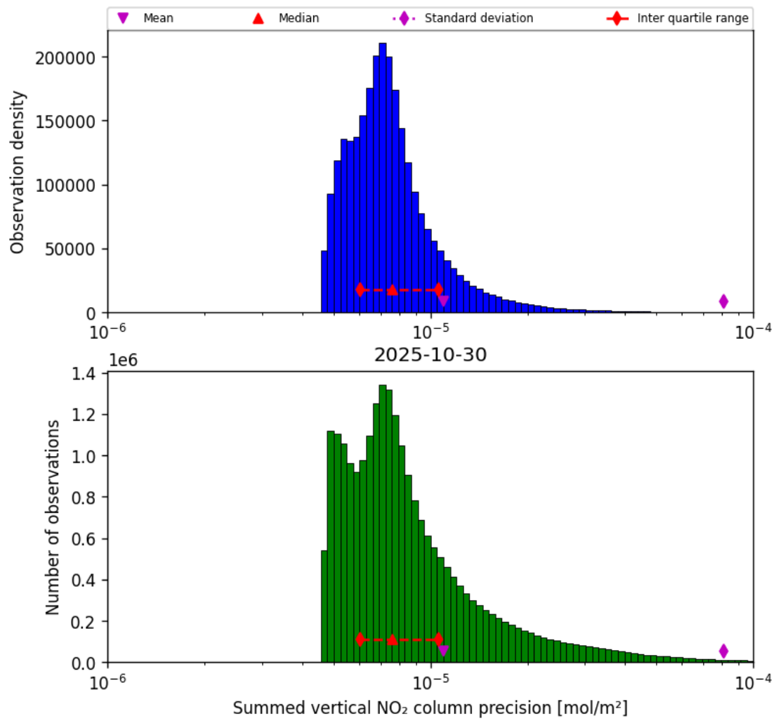
Figure 39: Histogram of "Summed vertical NO 2 column precision" for 2025-10-30 to 2025-10-30
