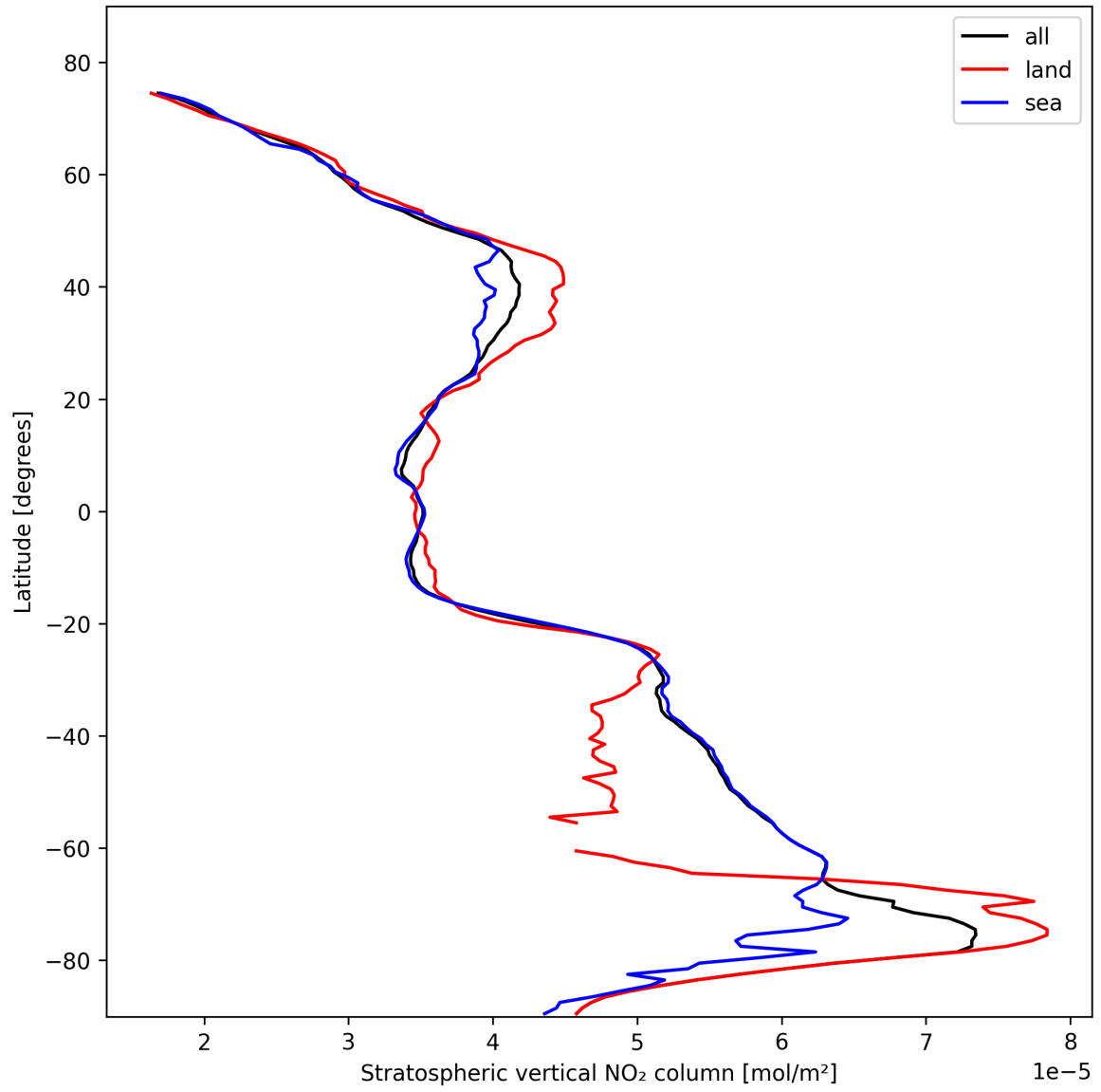
Figure 17: Zonal average of “Stratospheric vertical NO 2 column” for 2025-10-30 to 2025-10-30.
