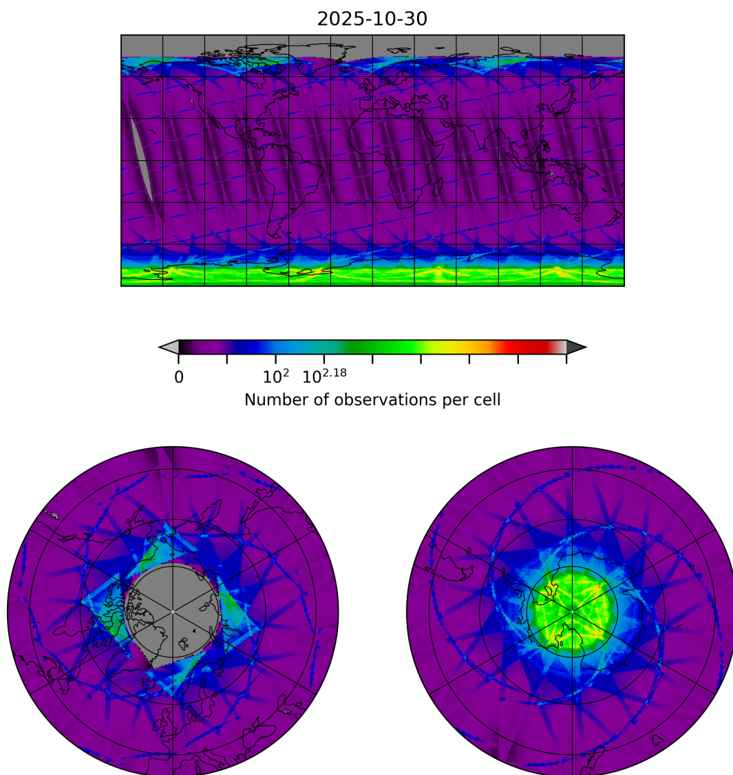
Figure 8: Map of the number of observations for 2025-10-30 to 2025-10-30
