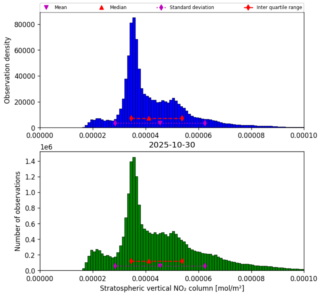
Figure 34: Histogram of “Stratospheric vertical NO 2 column” for 2025-10-30 to 2025-10-30
