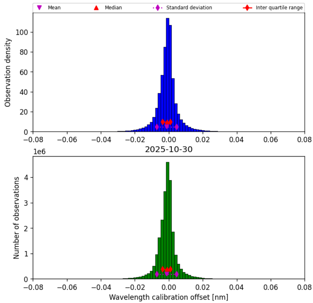
Figure 33: Histogram of “Wavelength calibration offset” for 2025-10-30 to 2025-10-30
