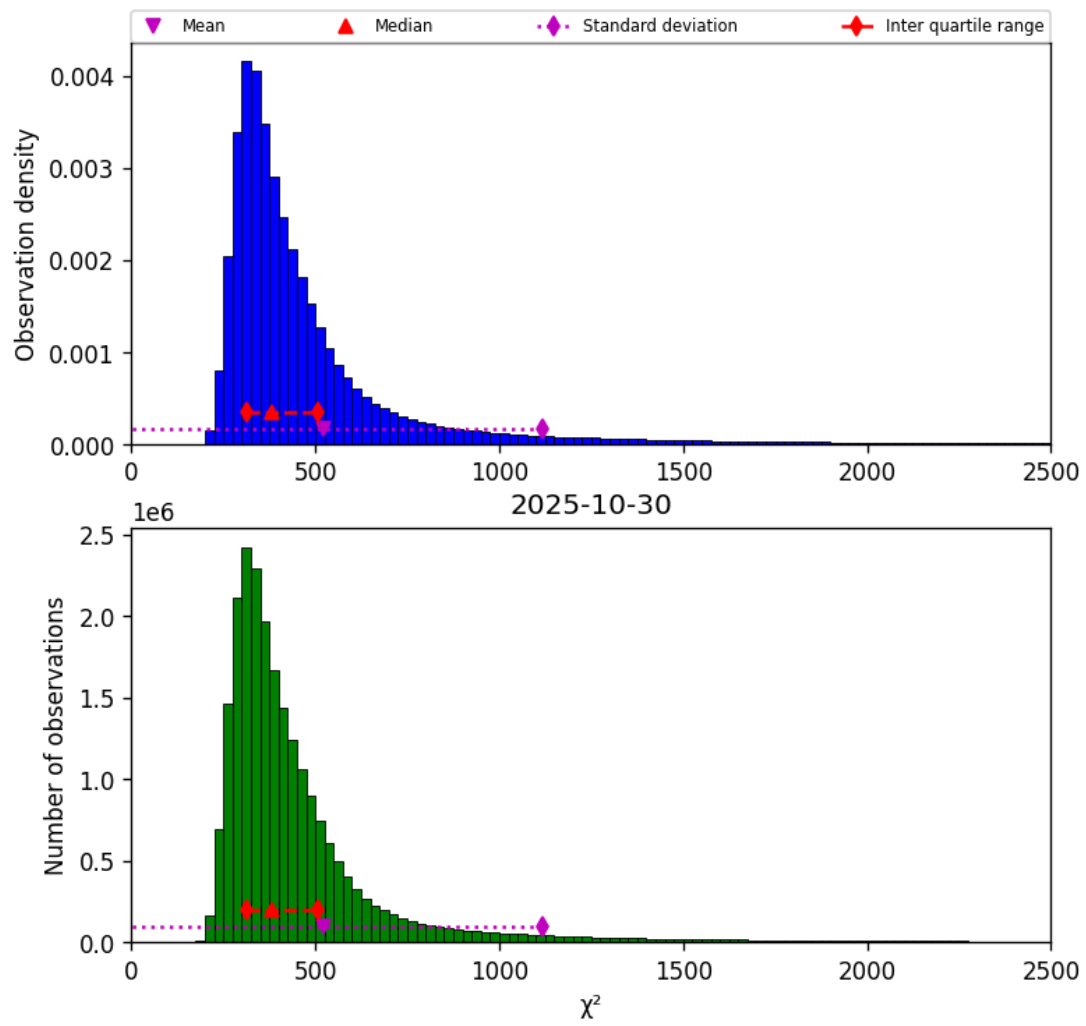
Figure 40: Histogram of “ \chi^2 ” for 2025-10-30 to 2025-10-30
