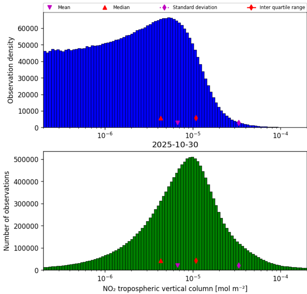
Figure 27: Histogram of “NO 2 tropospheric vertical column” for 2025-10-30 to 2025-10-30
