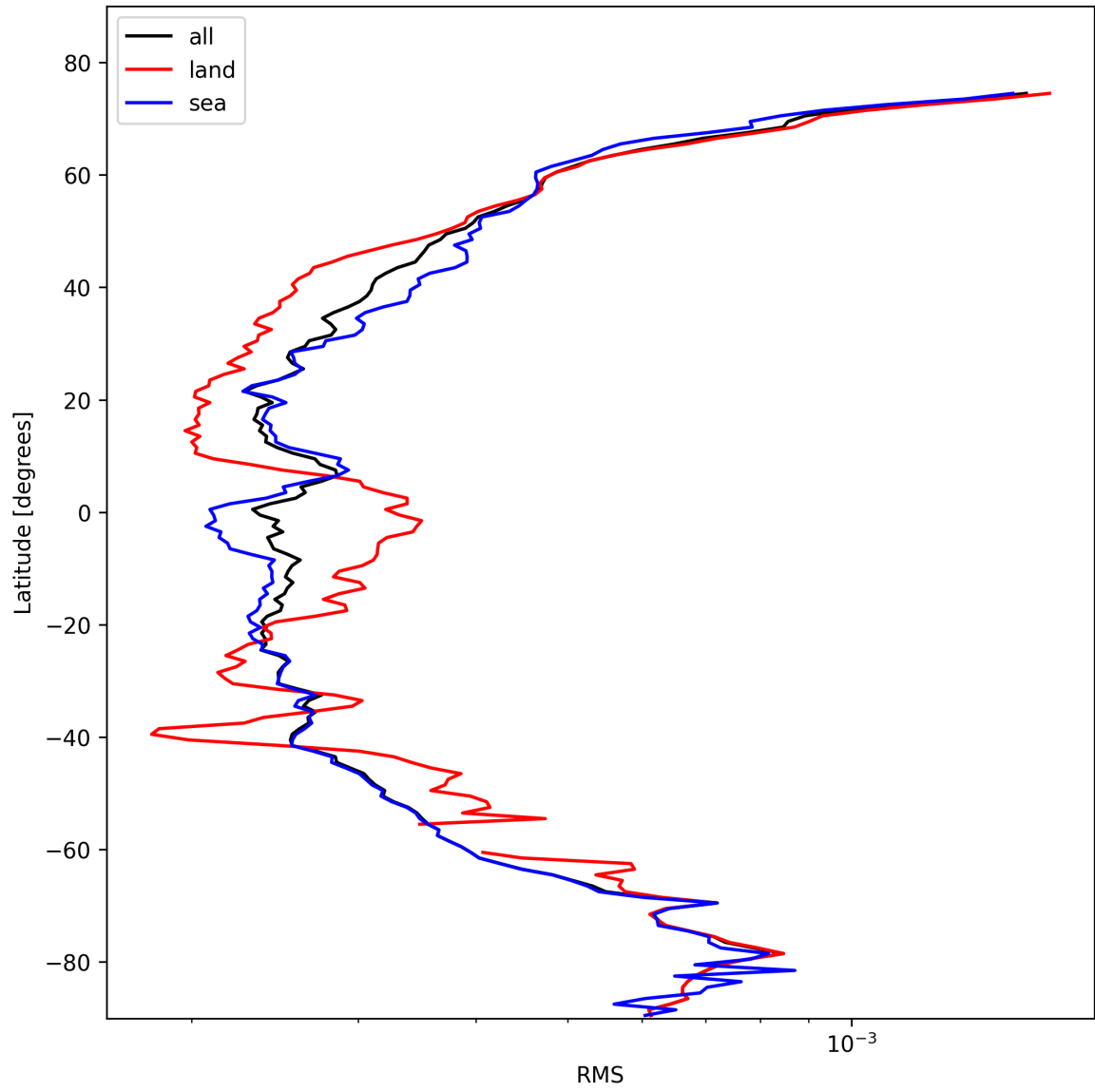
Figure 24: Zonal average of “RMS” for 2025-10-30 to 2025-10-30.
