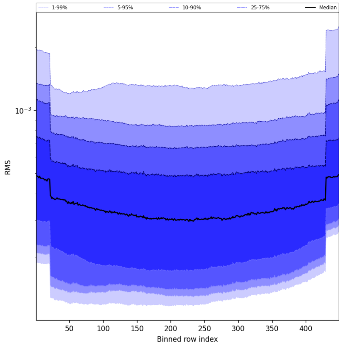
Figure 58: Along track statistics of “RMS” for 2025-10-30 to 2025-10-30
