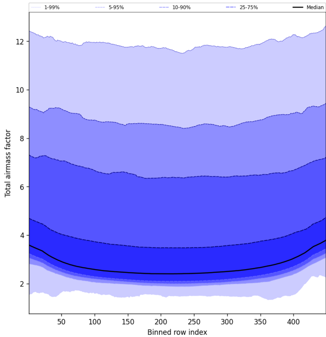
Figure 47: Along track statistics of “Total airmass factor” for 2025-10-30 to 2025-10-30
