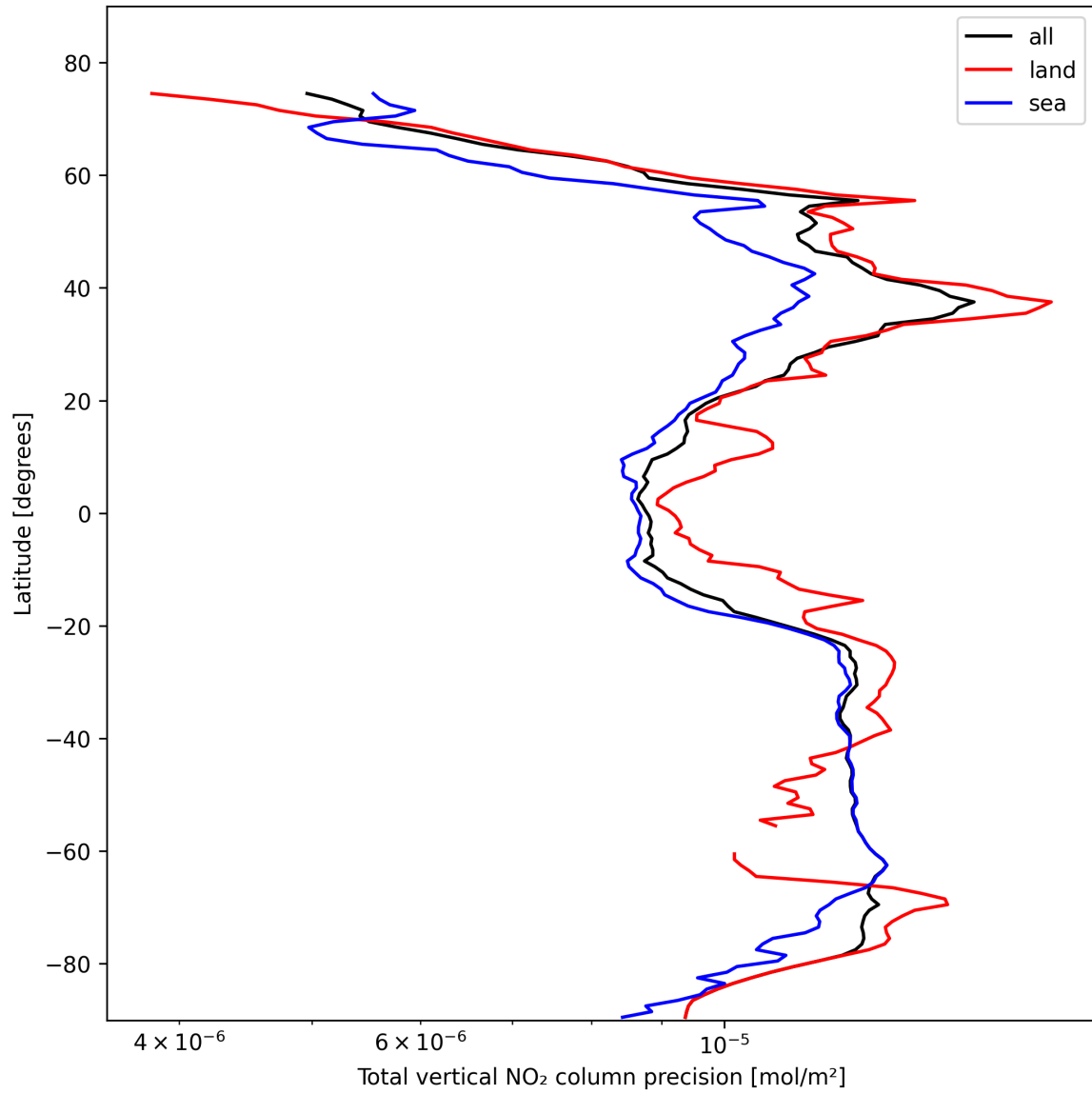
Figure 20: Zonal average of “Total vertical NO 2 column precision” for 2025-10-30 to 2025-10-30.
