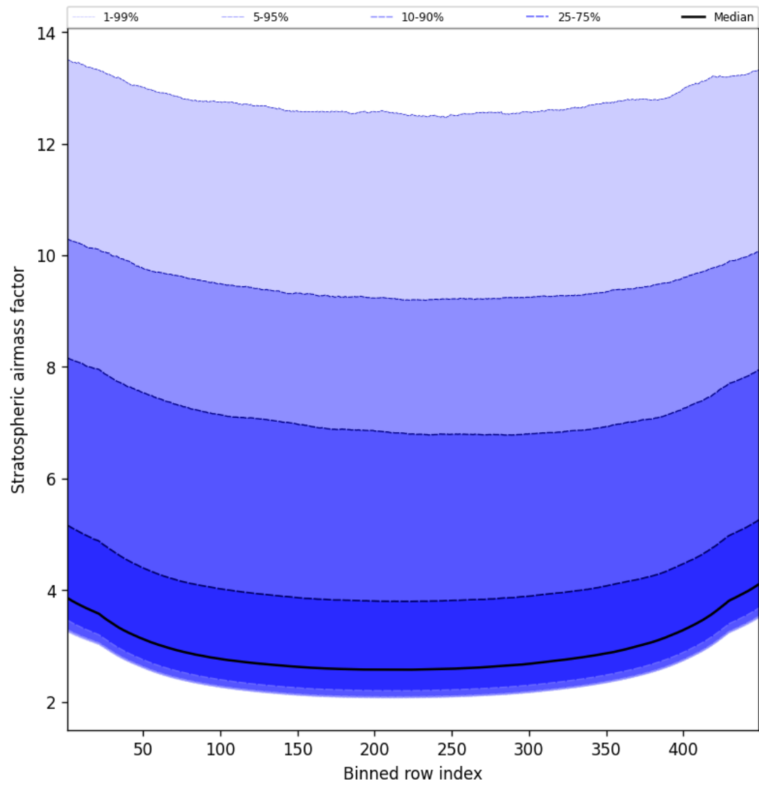
Figure 59: Along track statistics of “Stratospheric airmass factor” for 2025-10-30 to 2025-10-30
