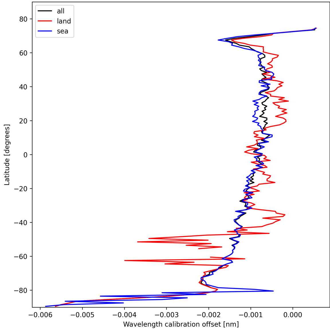
Figure 16: Zonal average of “Wavelength calibration offset” for 2025-10-30 to 2025-10-30.
