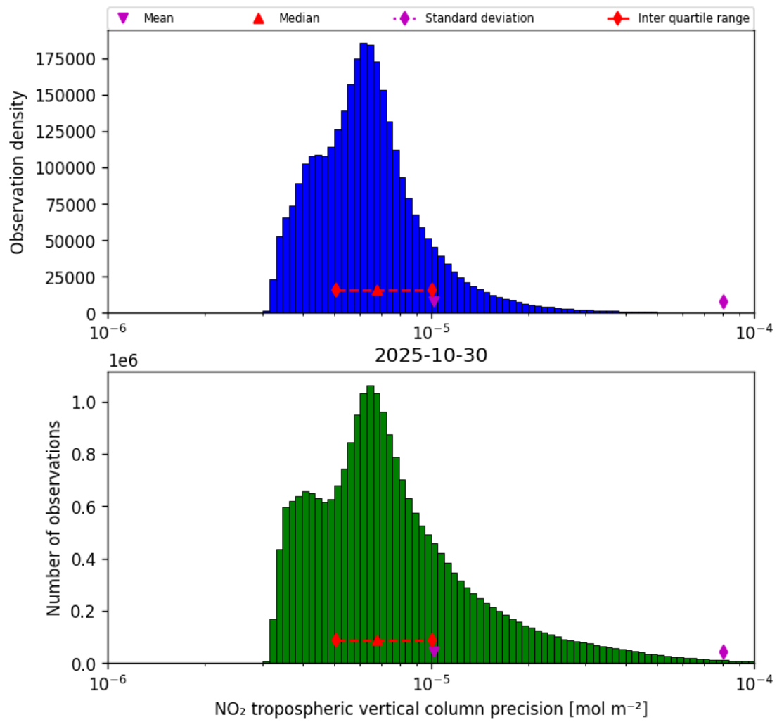
Figure 28: Histogram of “NO 2 tropospheric vertical column precision” for 2025-10-30 to 2025-10-30
