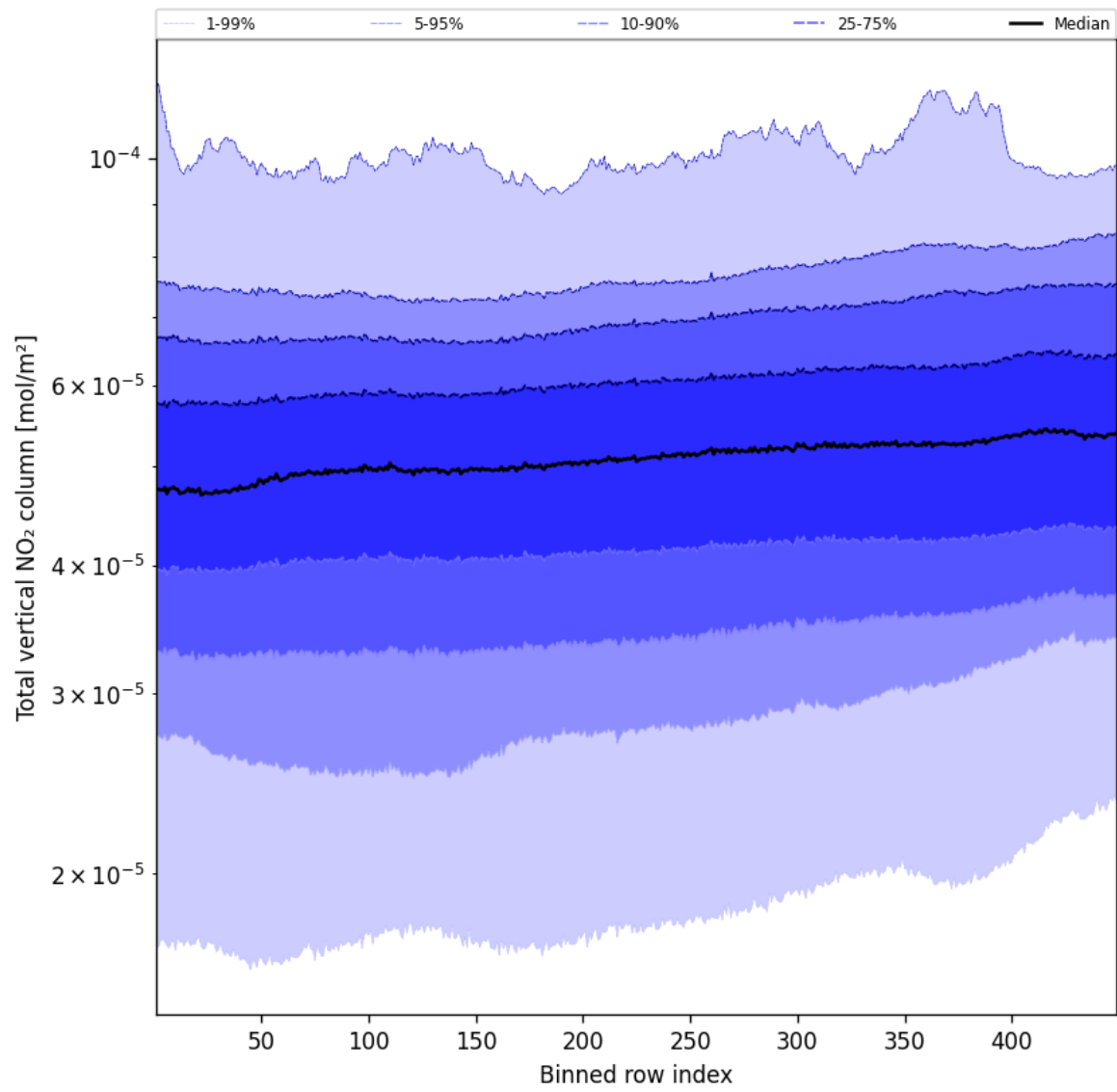
Figure 53: Along track statistics of “Total vertical NO 2 column” for 2025-10-30 to 2025-10-30
