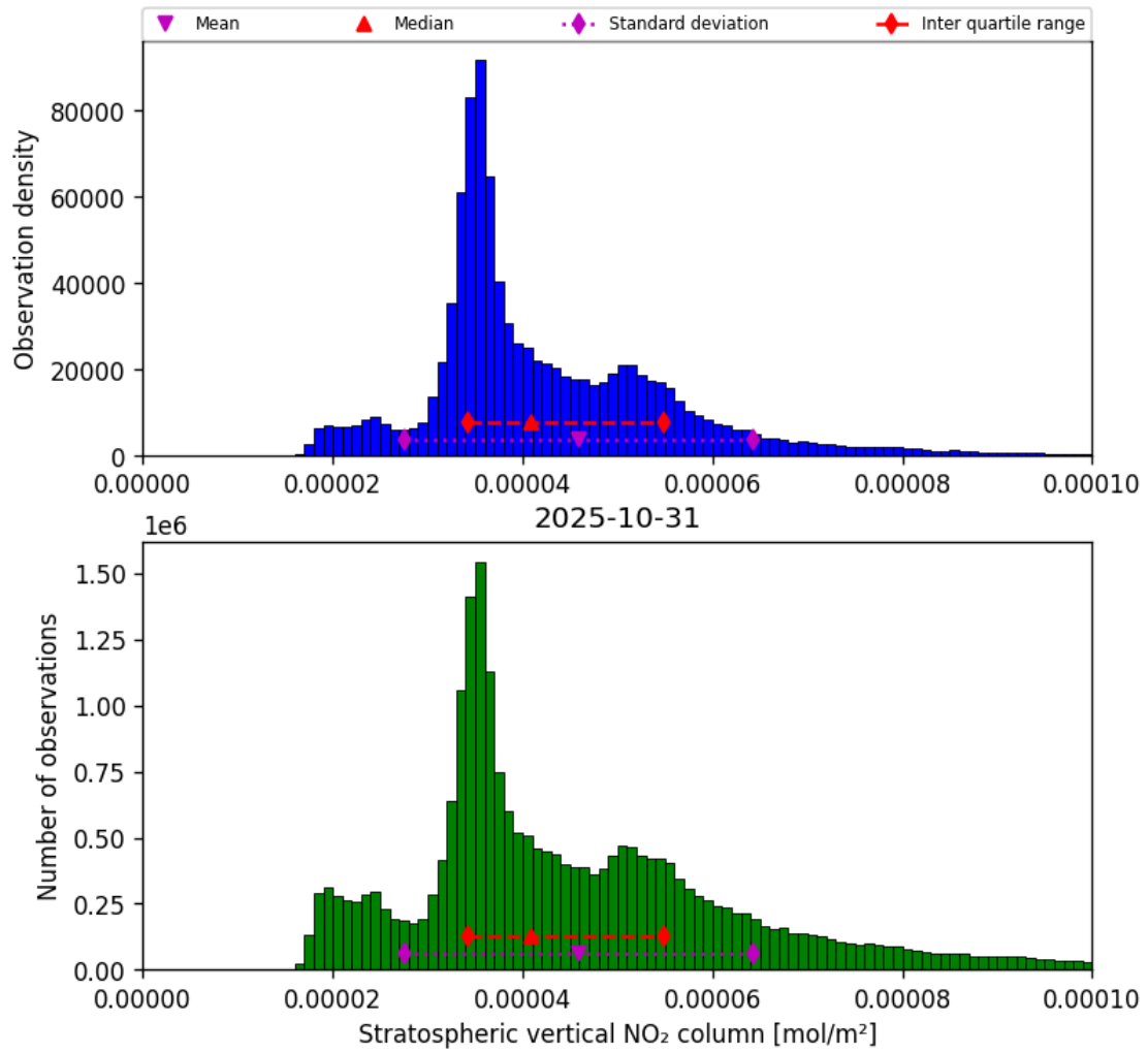
Figure 34: Histogram of “Stratospheric vertical NO 2 column” for 2025-10-31 to 2025-10-31
