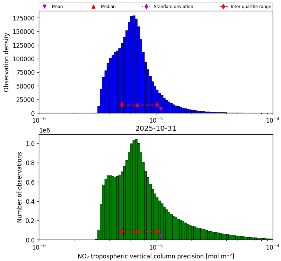
Figure 28: Histogram of "NO 2 tropospheric vertical column precision" for 2025-10-31 to 2025-10-31
