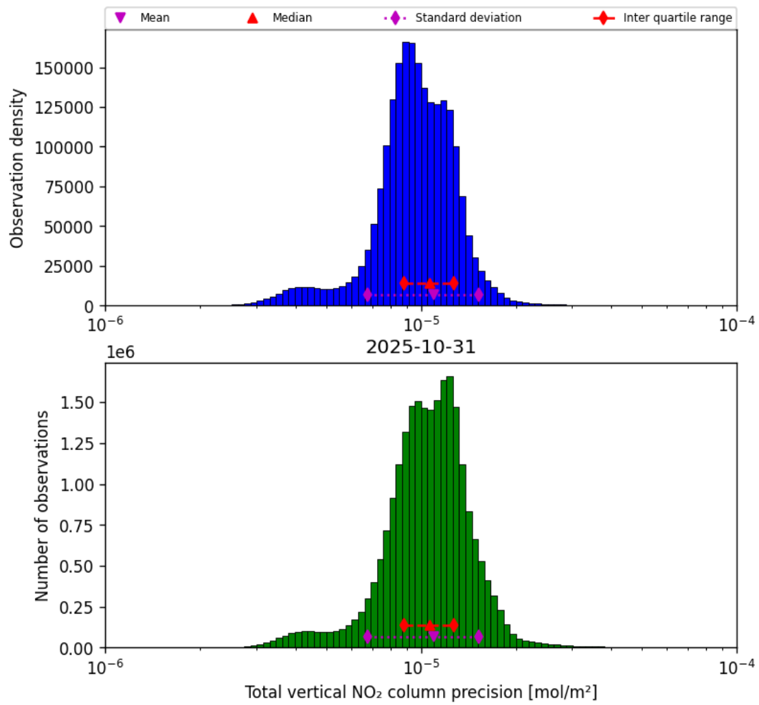
Figure 37: Histogram of "Total vertical NO 2 column precision" for 2025-10-31 to 2025-10-31
