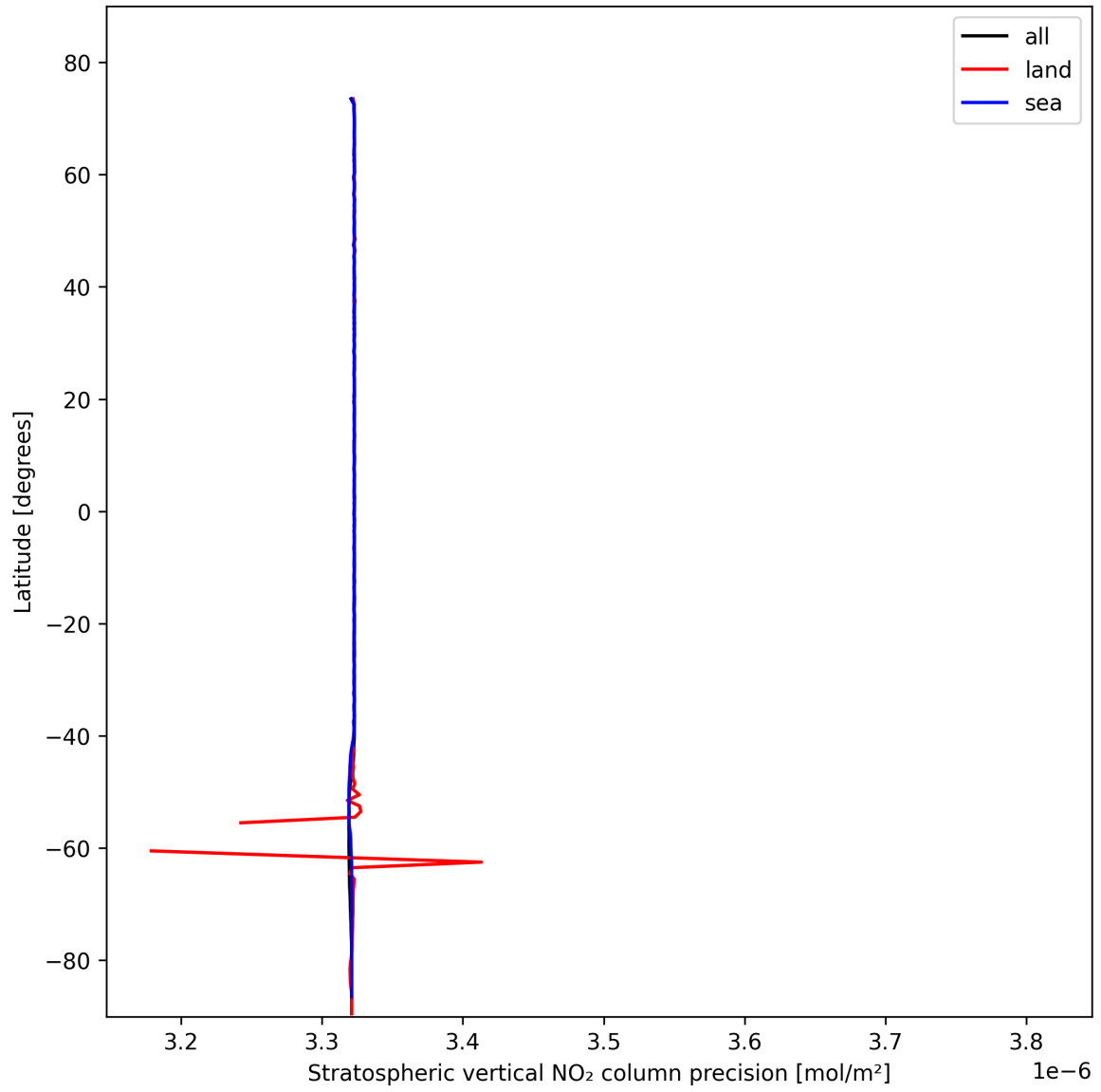
Figure 18: Zonal average of “Stratospheric vertical NO 2 column precision” for 2025-10-31 to 2025-10-31.
