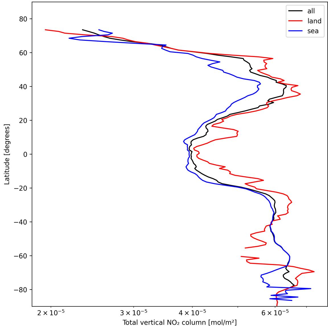
Figure 19: Zonal average of “Total vertical NO 2 column” for 2025-10-31 to 2025-10-31.
