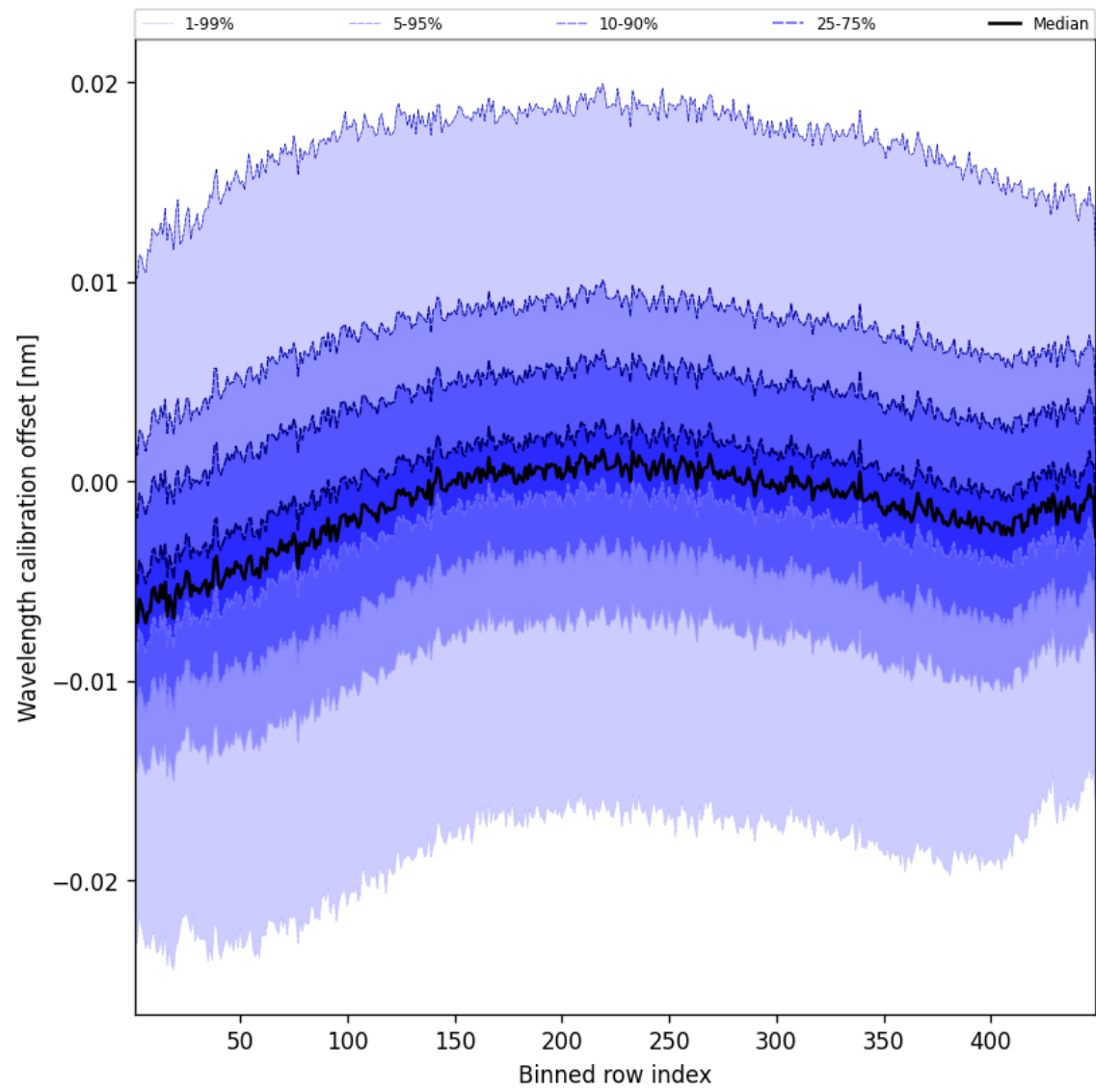
Figure 50: Along track statistics of “Wavelength calibration offset” for 2025-10-31 to 2025-10-31
