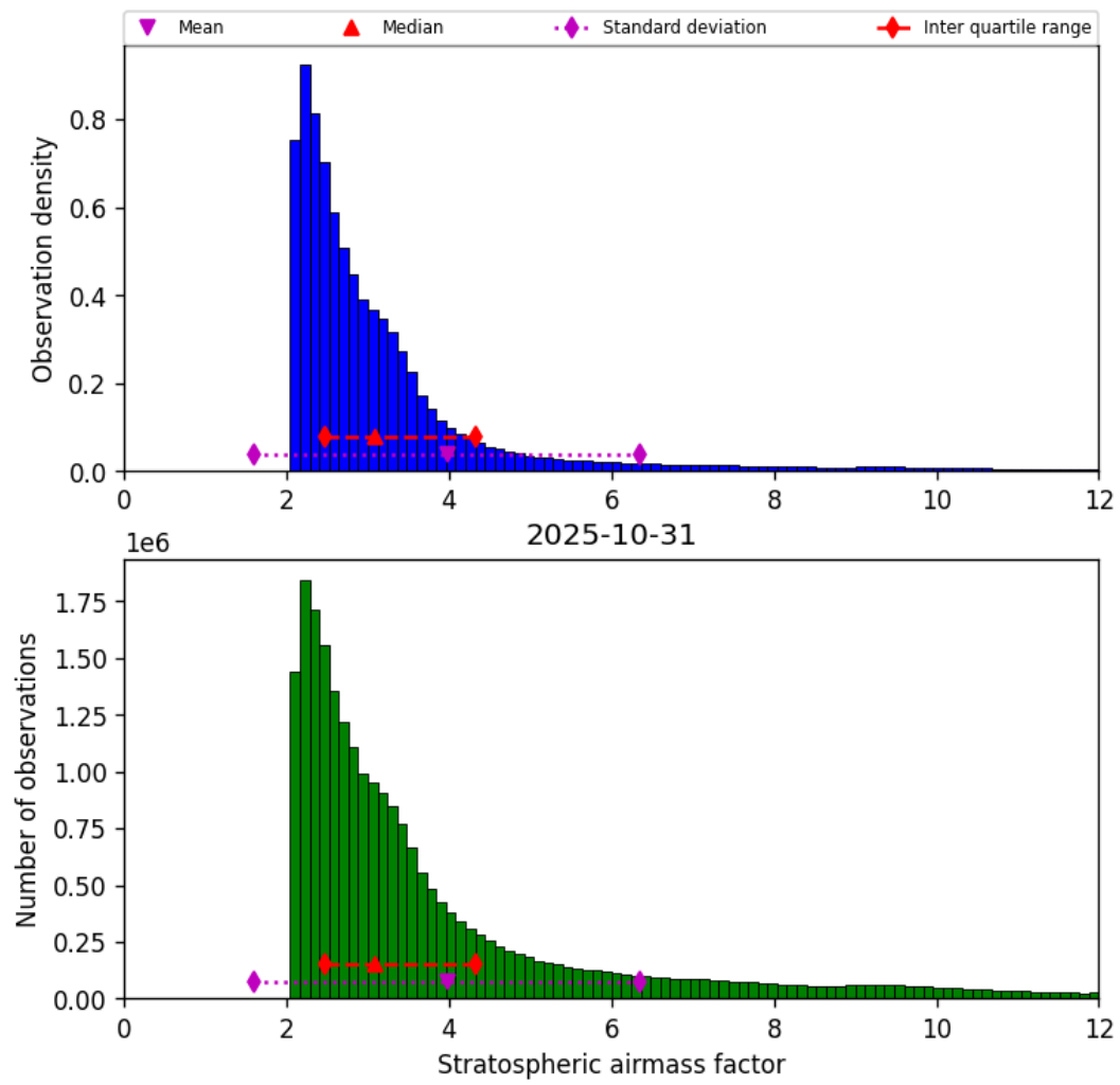
Figure 42: Histogram of “Stratospheric airmass factor” for 2025-10-31 to 2025-10-31
