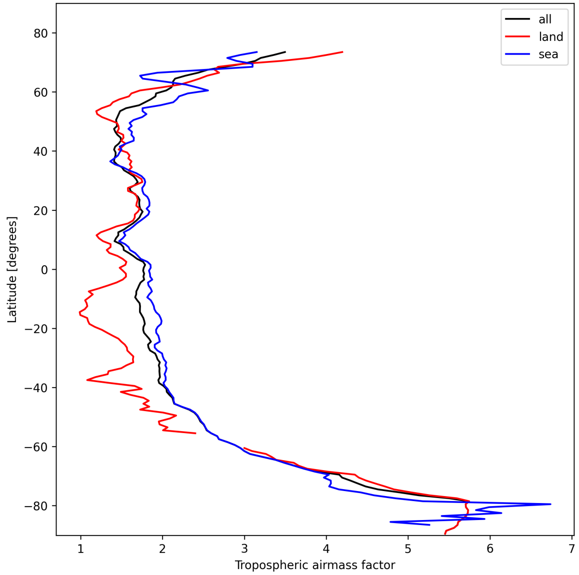
Figure 12: Zonal average of “Tropospheric air mass factor” for 2025-10-31 to 2025-10-31.
