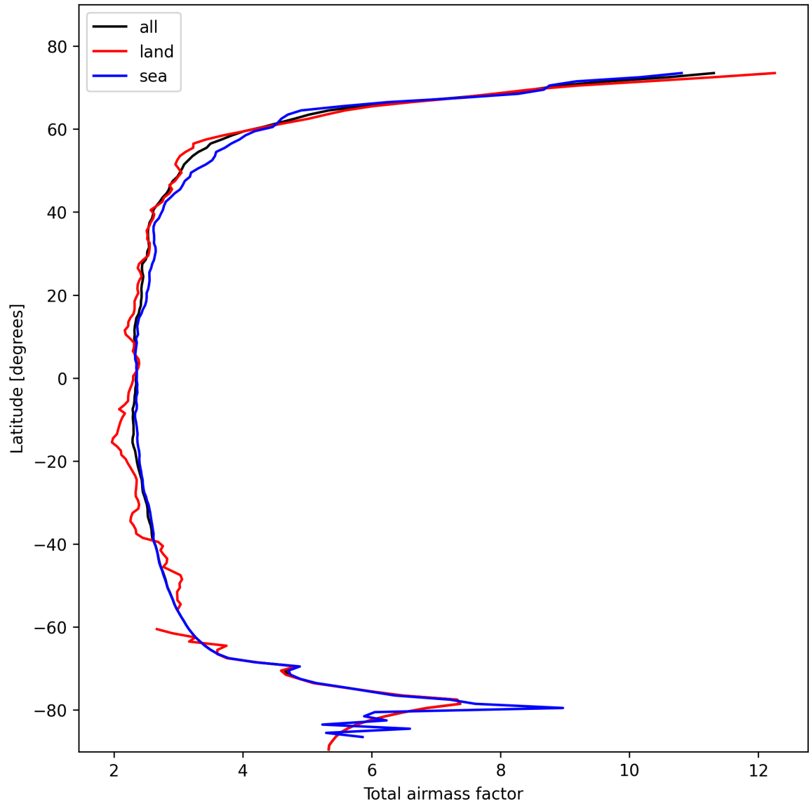
Figure 13: Zonal average of “Total airmass factor” for 2025-10-31 to 2025-10-31.
