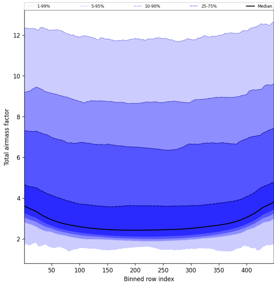
Figure 47: Along track statistics of “Total airmass factor” for 2025-10-31 to 2025-10-31
