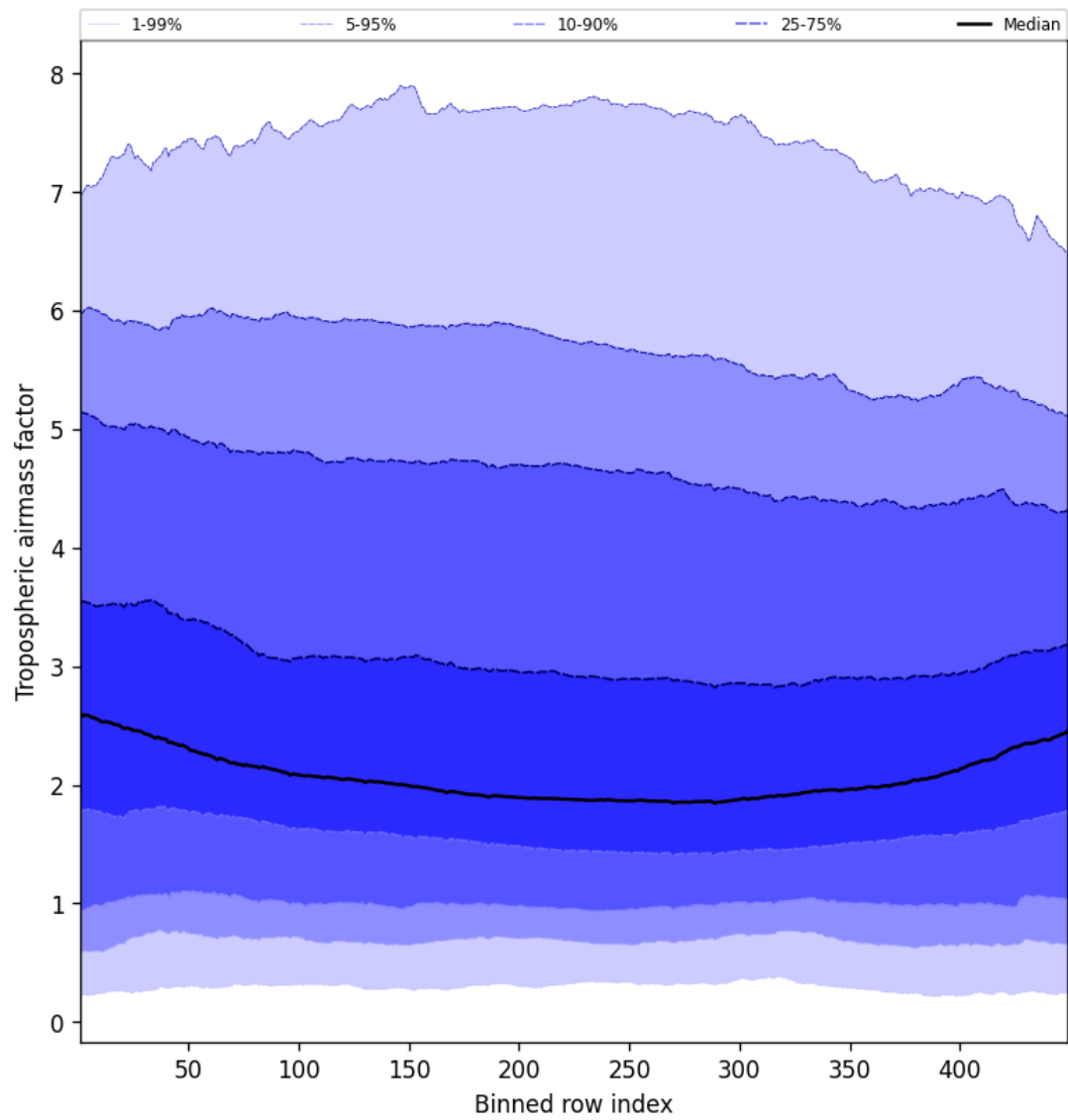
Figure 46: Along track statistics of “Tropospheric airmass factor” for 2025-10-31 to 2025-10-31
