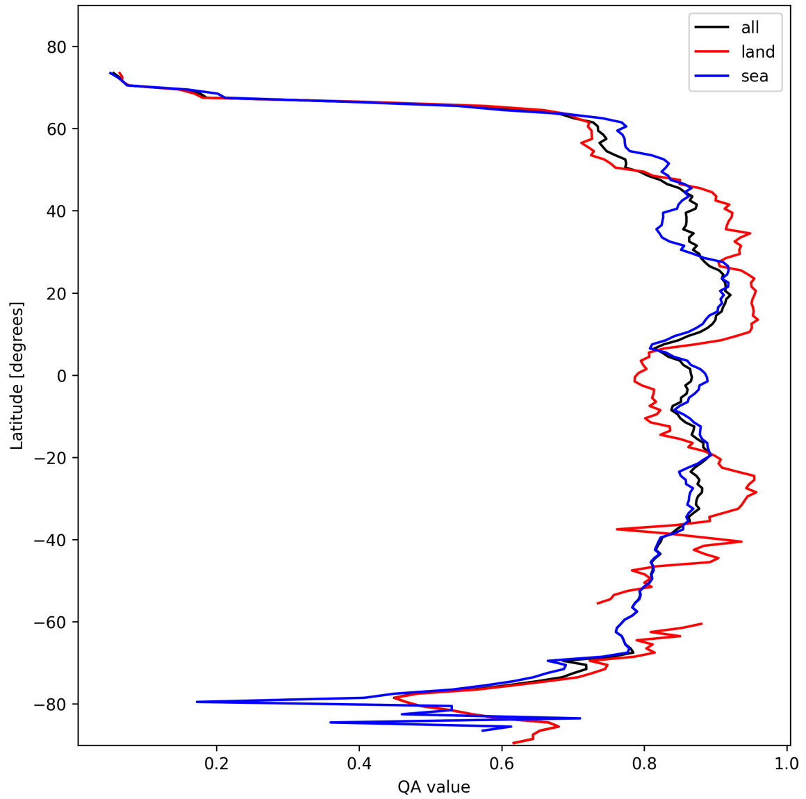
Figure 9: Zonal average of “QA value” for 2025-10-31 to 2025-10-31.
