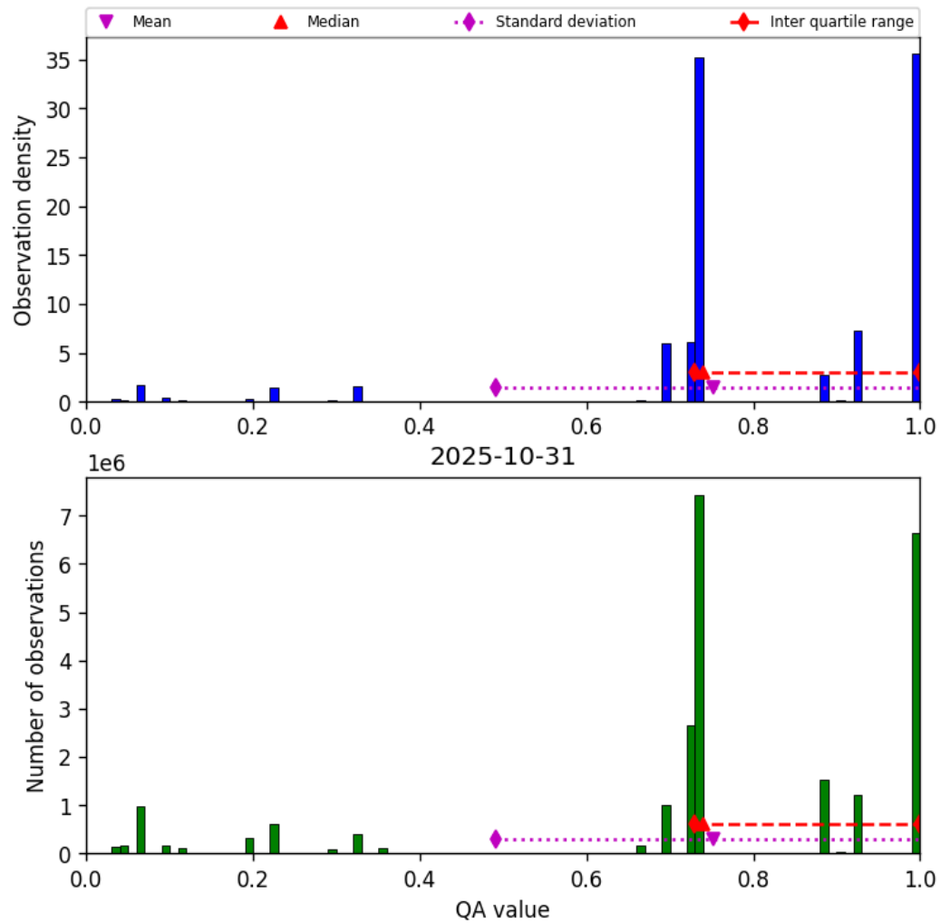
Figure 26: Histogram of “QA value” for 2025-10-31 to 2025-10-31
