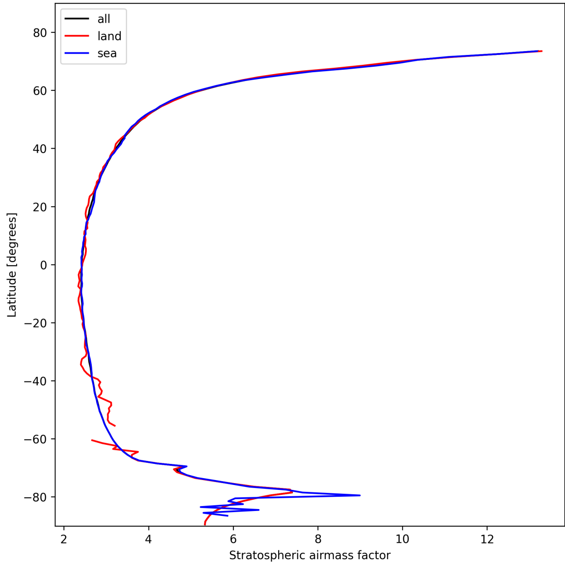
Figure 25: Zonal average of “Stratospheric airmass factor” for 2025-10-31 to 2025-10-31.
