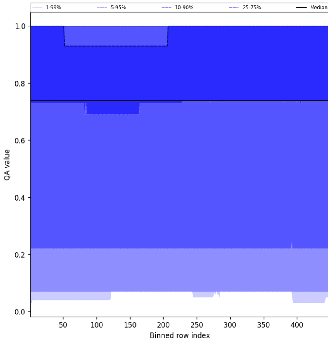
Figure 43: Along track statistics of “QA value” for 2025-10-31 to 2025-10-31
