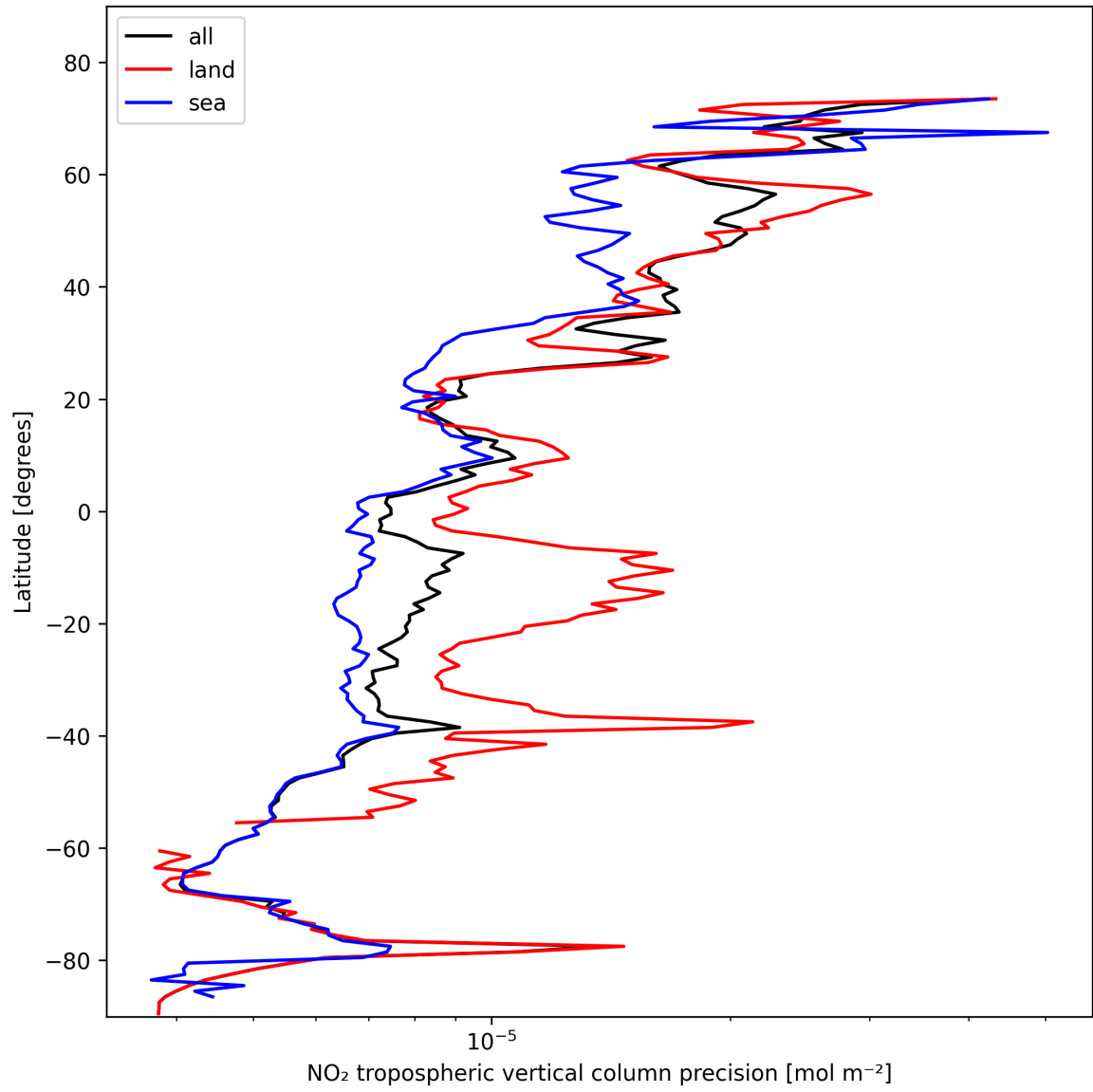
Figure 11: Zonal average of “NO 2 tropospheric vertical column precision” for 2025-10-31 to 2025-10-31.
