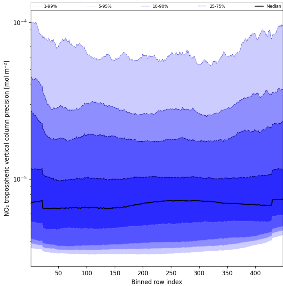
Figure 45: Along track statistics of “NO 2 tropospheric vertical column precision” for 2025-10-31 to 2025-10-31
