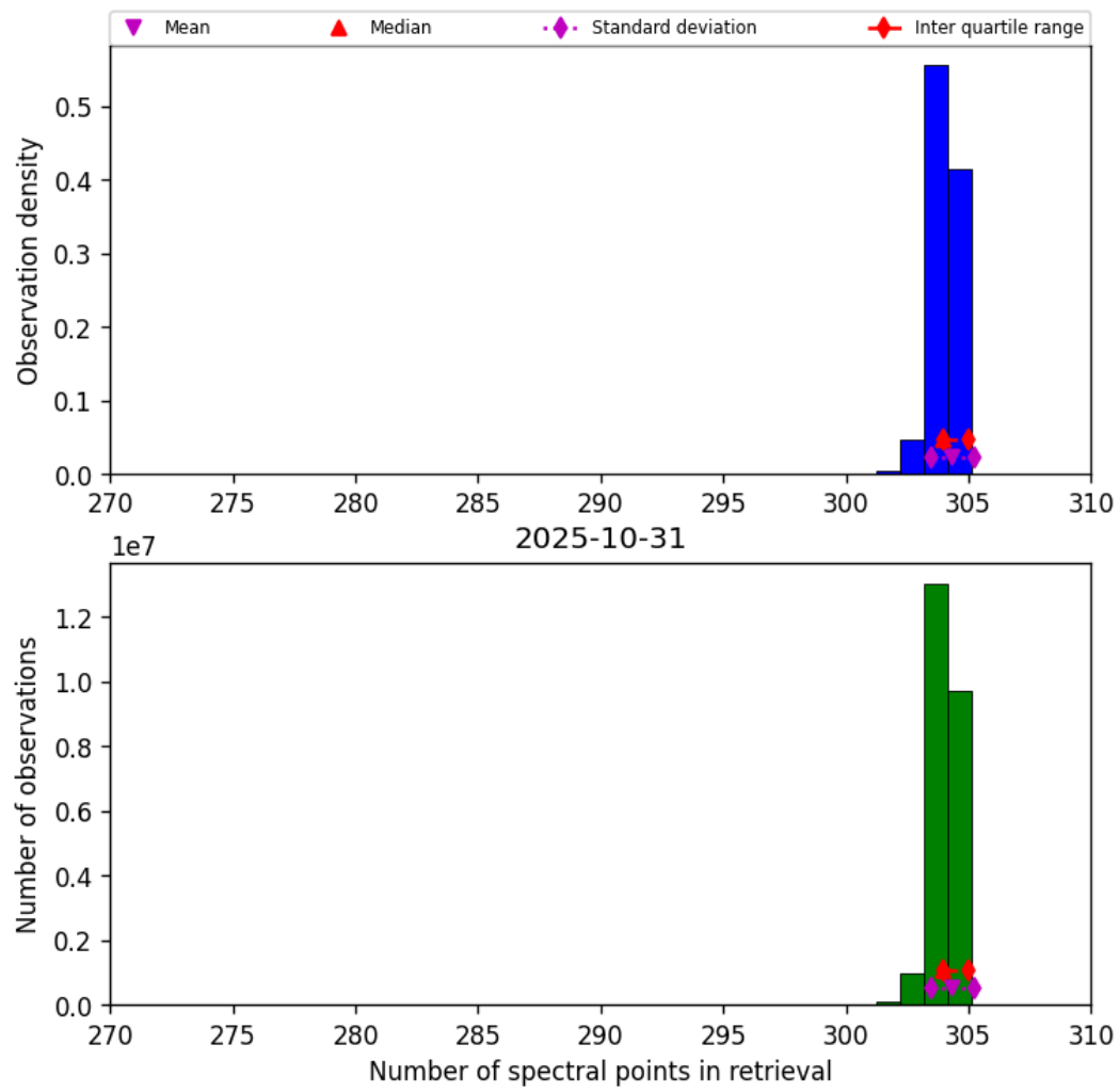
Figure 31: Histogram of “Number of spectral points in retrieval” for 2025-10-31 to 2025-10-31
