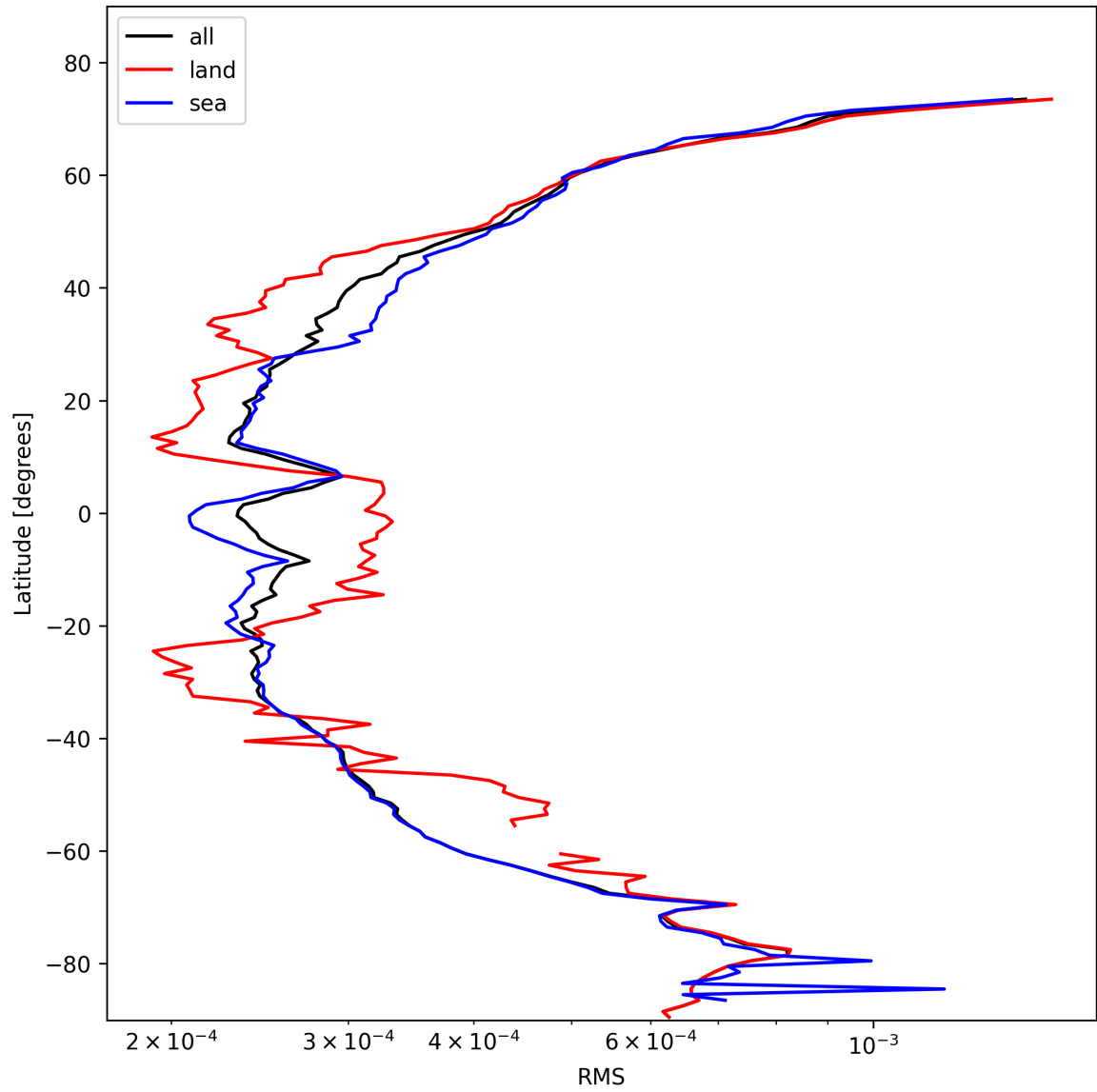
Figure 24: Zonal average of “RMS” for 2025-10-31 to 2025-10-31.
