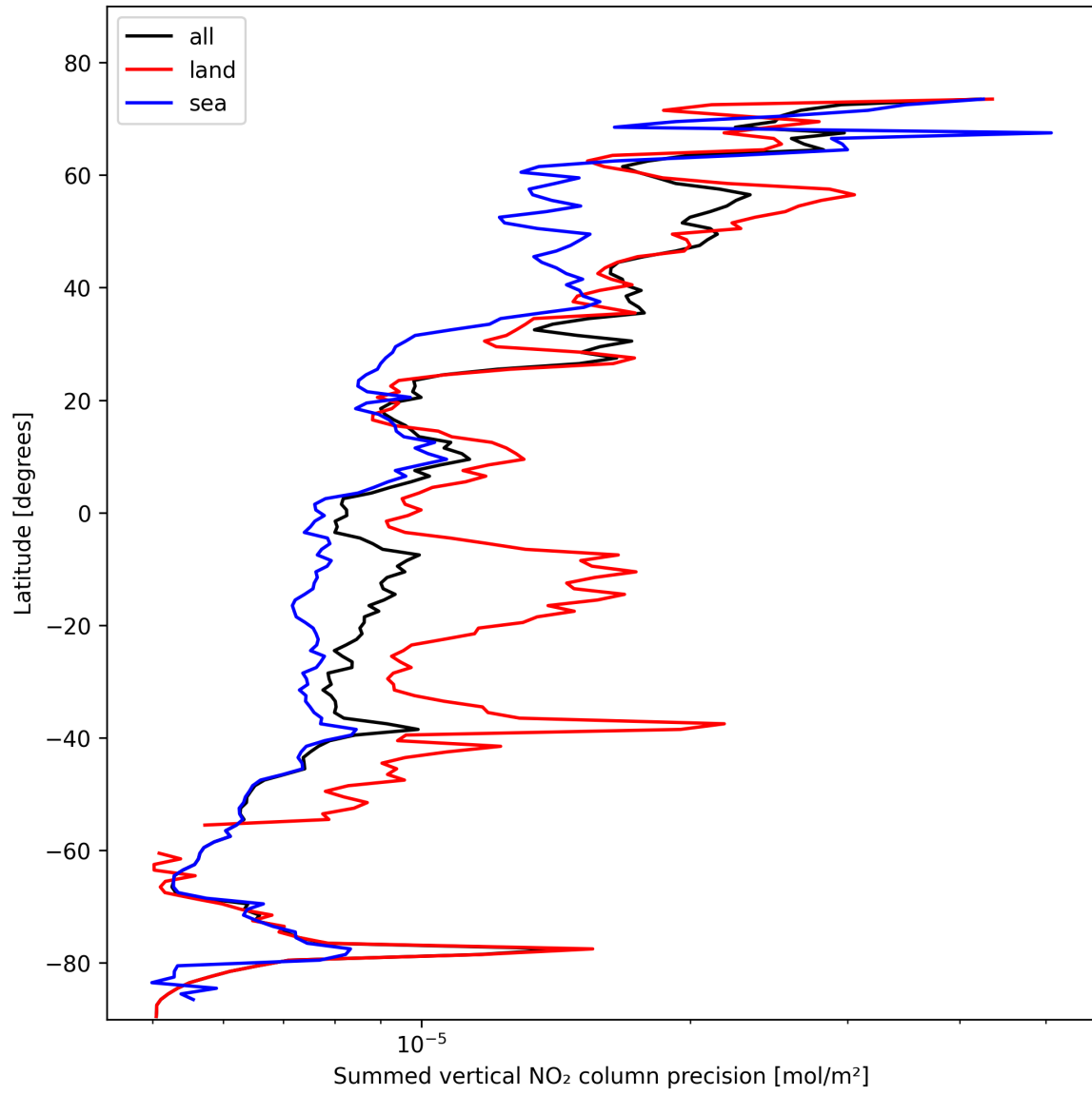
Figure 22: Zonal average of “Summed vertical NO 2 column precision” for 2025-10-31 to 2025-10-31.
