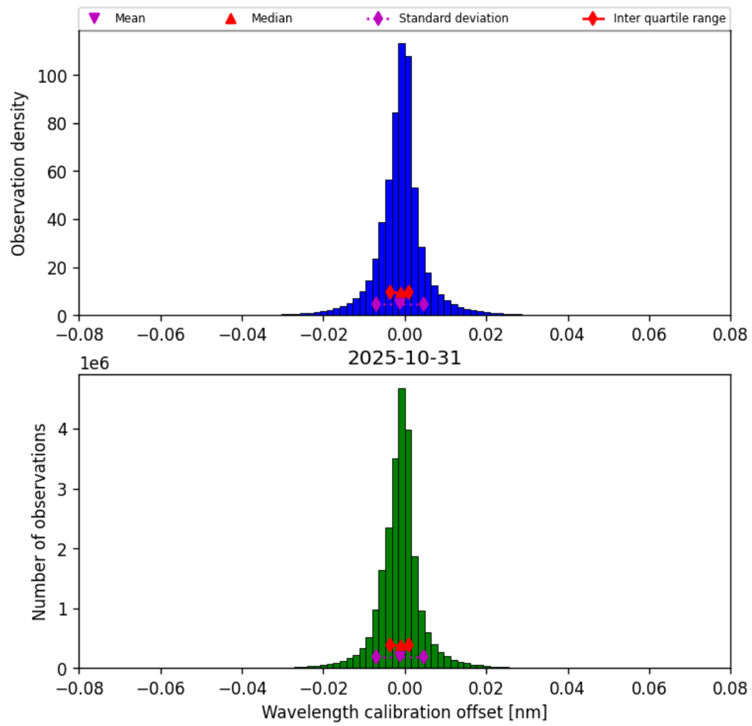
Figure 33: Histogram of “Wavelength calibration offset” for 2025-10-31 to 2025-10-31
