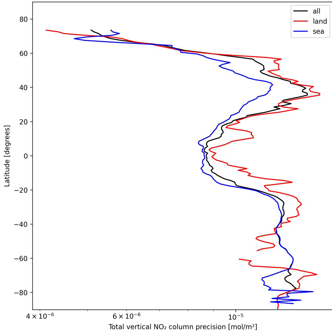
Figure 20: Zonal average of “Total vertical NO 2 column precision” for 2025-10-31 to 2025-10-31.
