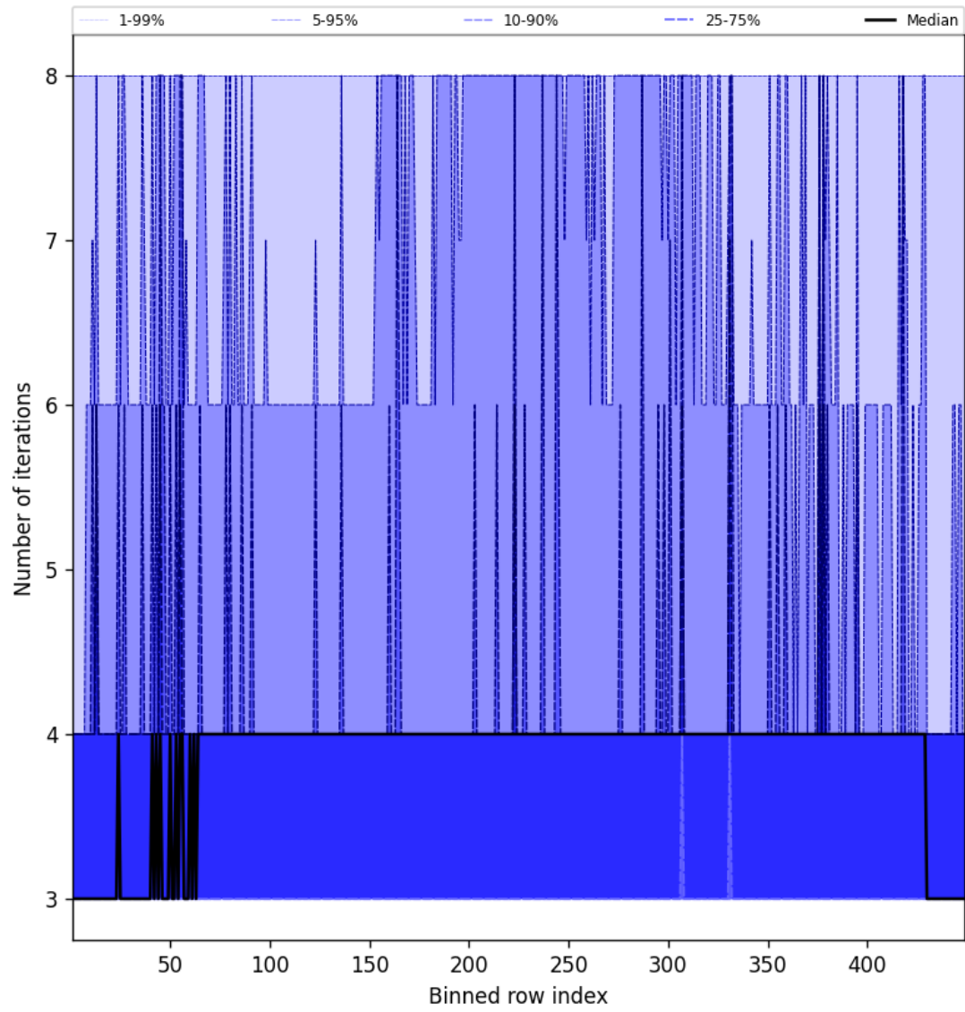
Figure 49: Along track statistics of “Number of iterations” for 2025-10-31 to 2025-10-31
