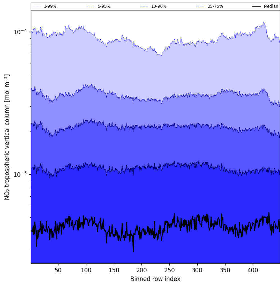
Figure 44: Along track statistics of “NO 2 tropospheric vertical column” for 2025-10-31 to 2025-10-31
