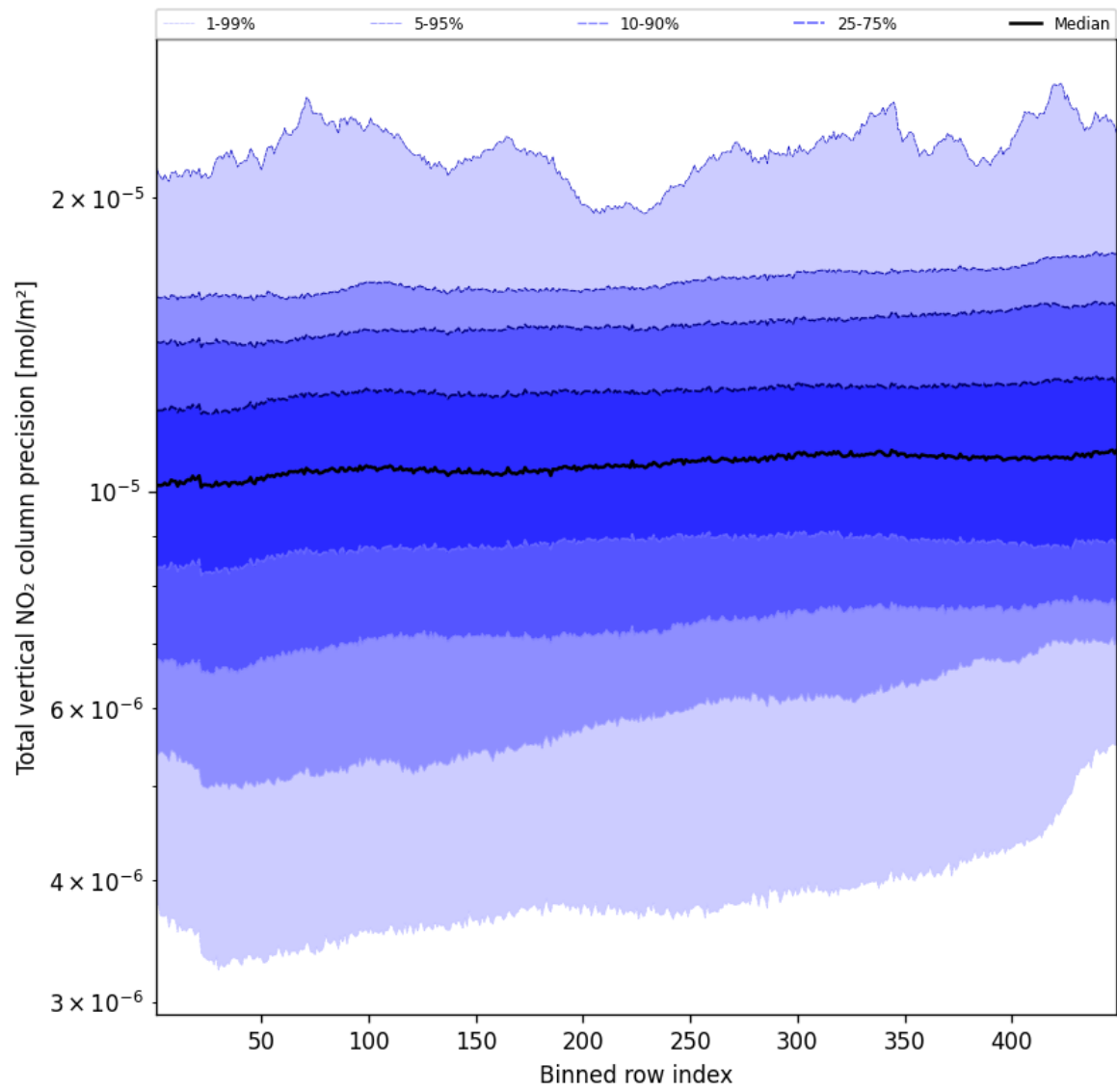
Figure 54: Along track statistics of “Total vertical NO 2 column precision” for 2025-10-31 to 2025-10-31
