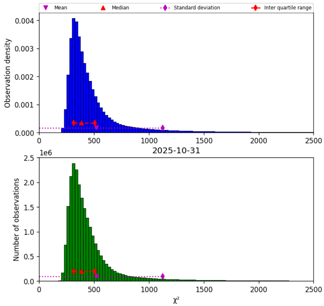
Figure 40: Histogram of “ \chi^2 ” for 2025-10-31 to 2025-10-31
