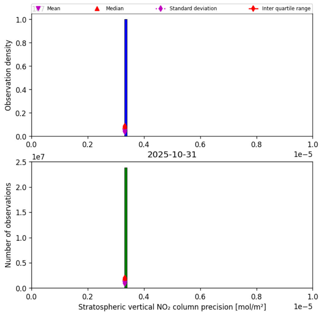
Figure 35: Histogram of “Stratospheric vertical NO 2 column precision” for 2025-10-31 to 2025-10-31
