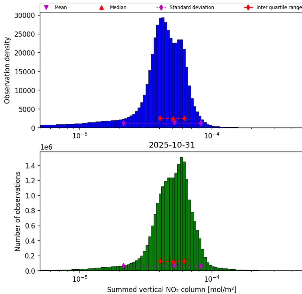
Figure 38: Histogram of "Summed vertical NO 2 column" for 2025-10-31 to 2025-10-31
