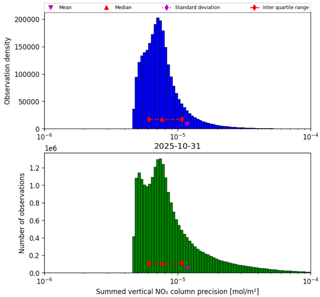
Figure 39: Histogram of "Summed vertical NO 2 column precision" for 2025-10-31 to 2025-10-31
