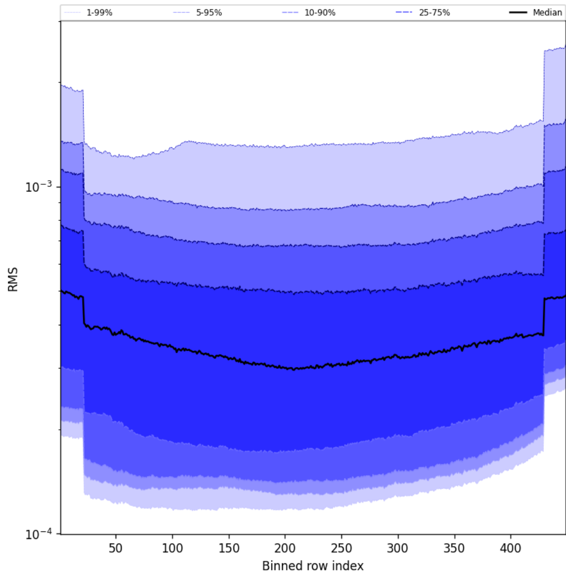
Figure 58: Along track statistics of “RMS” for 2025-10-31 to 2025-10-31
