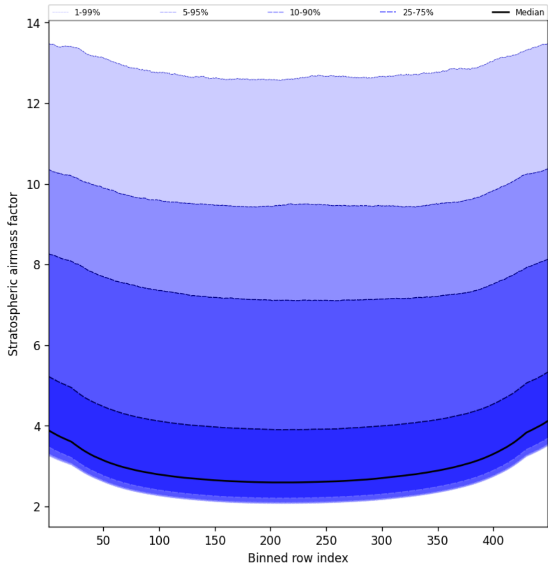
Figure 59: Along track statistics of “Stratospheric airmass factor” for 2025-10-31 to 2025-10-31
