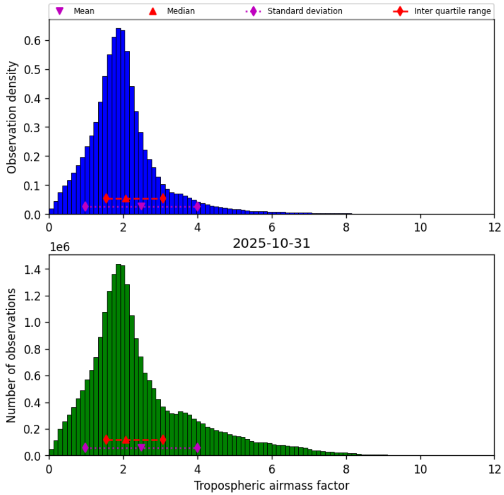
Figure 29: Histogram of “Tropospheric airmass factor” for 2025-10-31 to 2025-10-31
