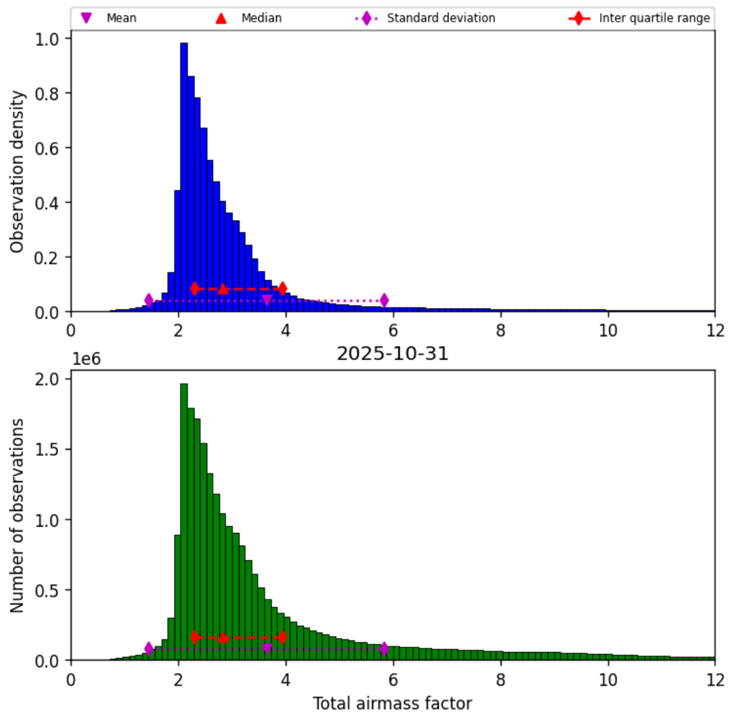
Figure 30: Histogram of “Total airmass factor” for 2025-10-31 to 2025-10-31
