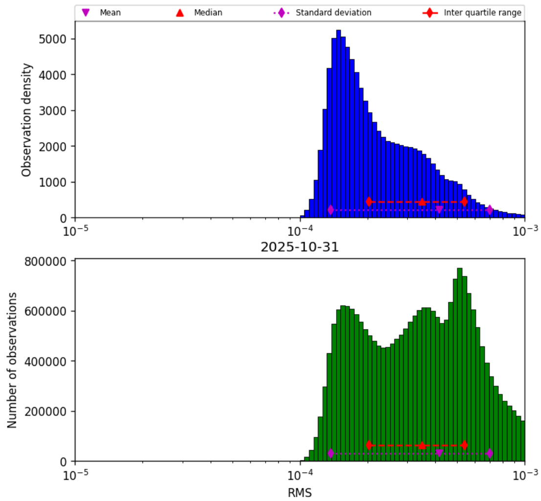
Figure 41: Histogram of “RMS” for 2025-10-31 to 2025-10-31
