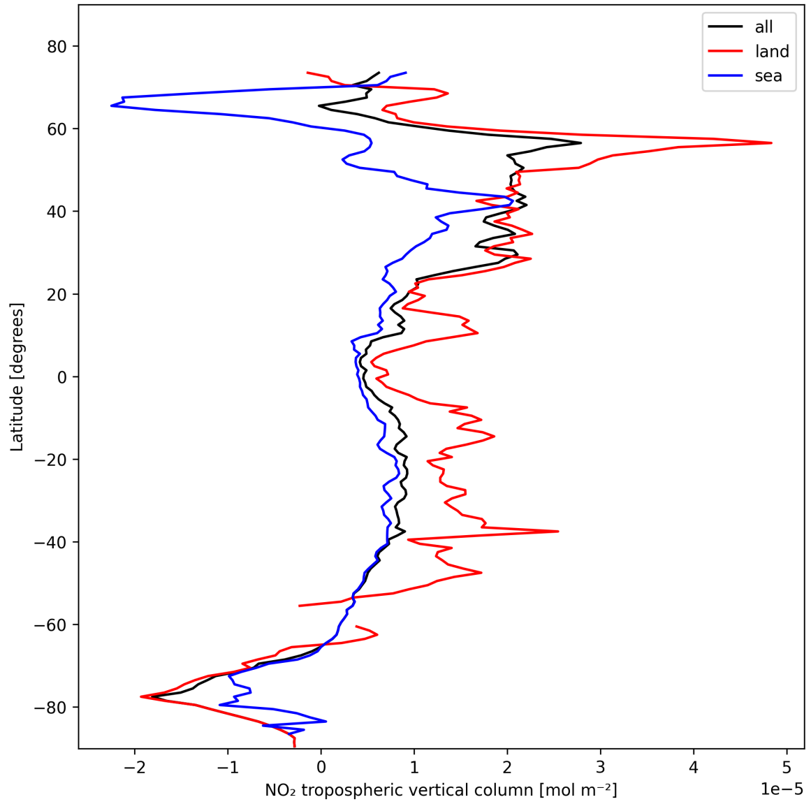
Figure 10: Zonal average of “NO 2 tropospheric vertical column” for 2025-10-31 to 2025-10-31.
