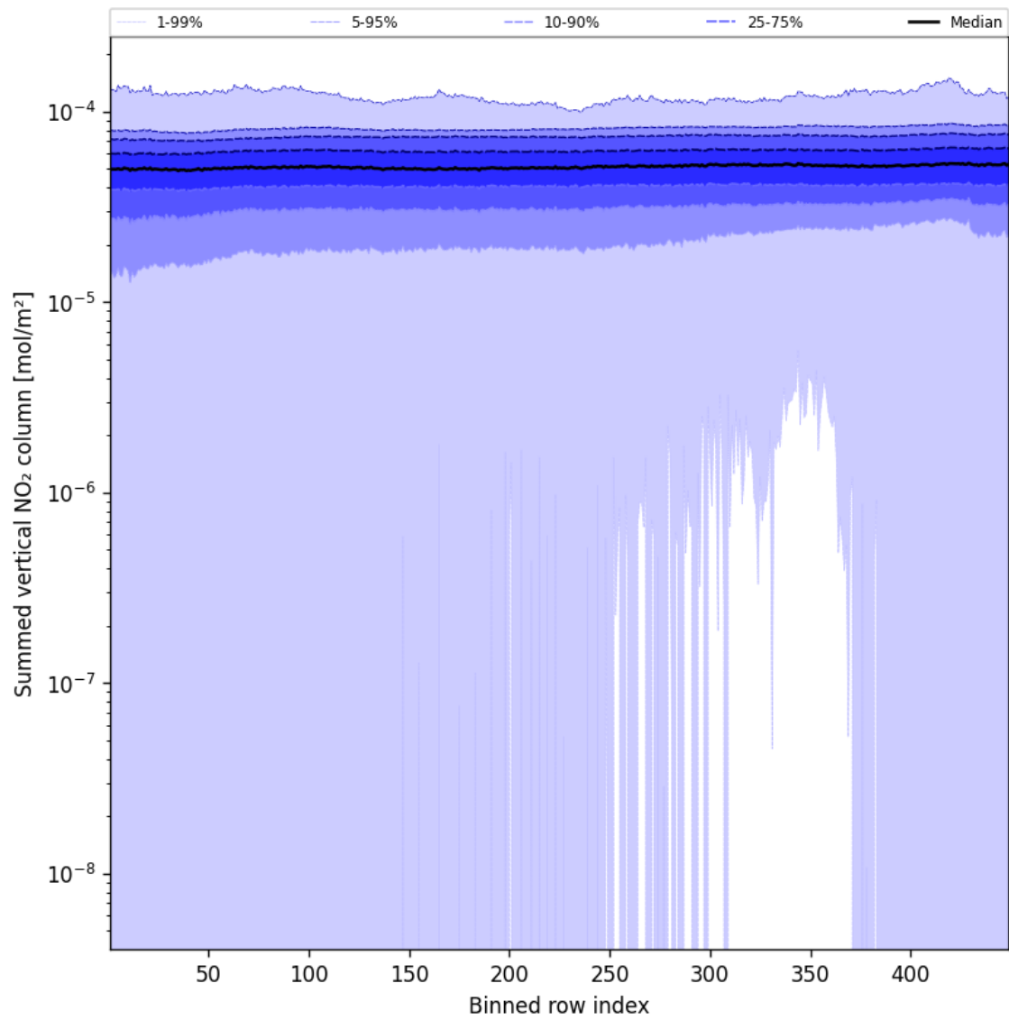
Figure 55: Along track statistics of “Summed vertical NO 2 column” for 2025-10-31 to 2025-10-31
