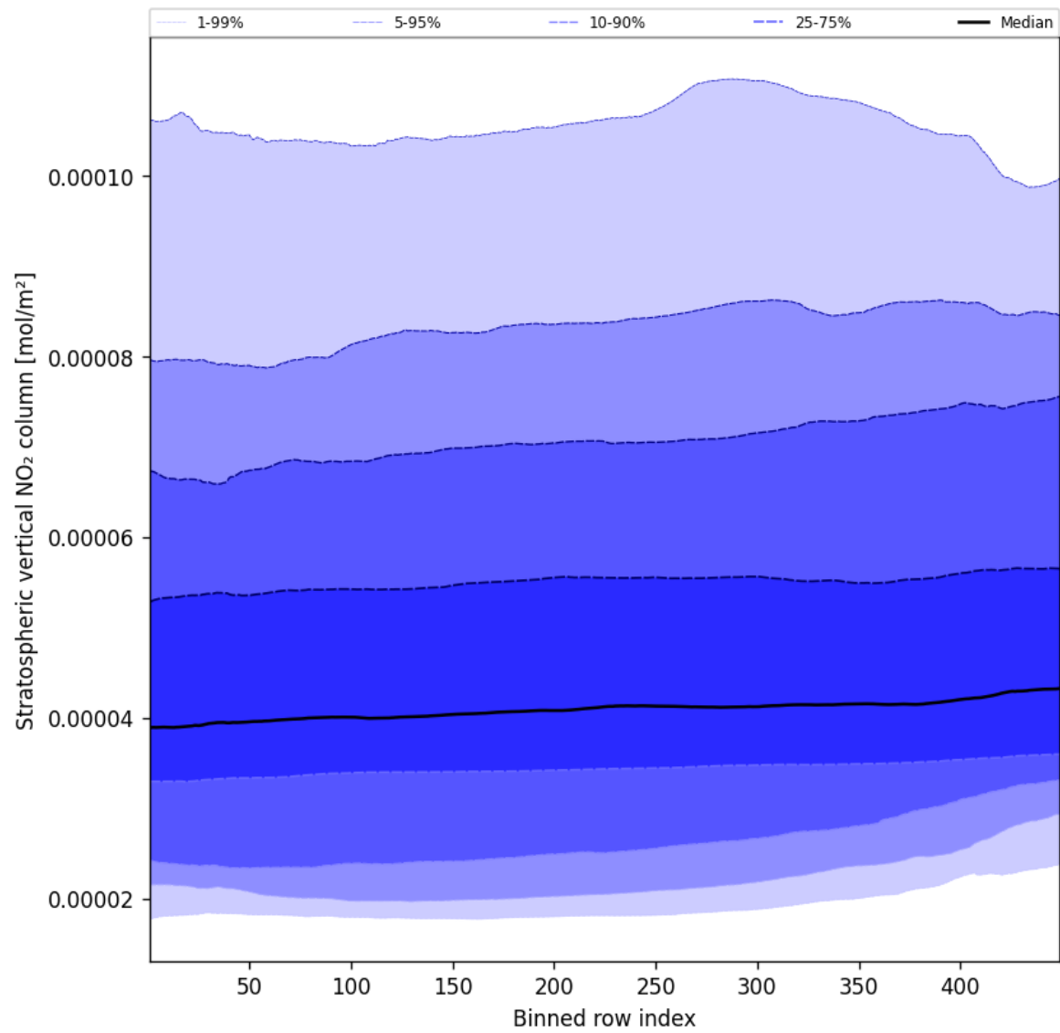
Figure 51: Along track statistics of “Stratospheric vertical NO 2 column” for 2025-10-31 to 2025-10-31
