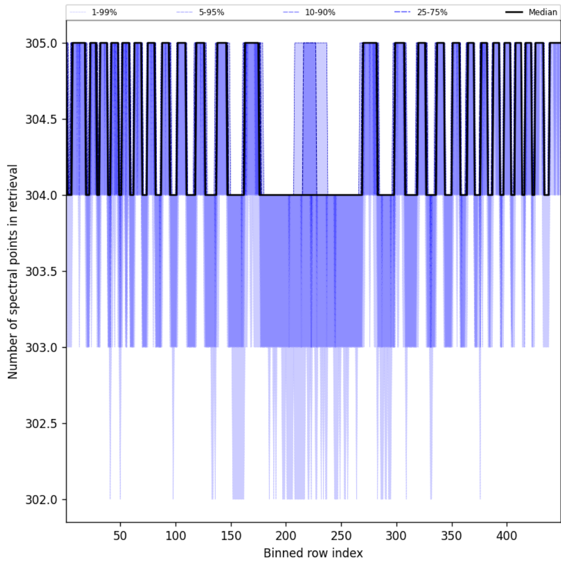
Figure 48: Along track statistics of “Number of spectral points in retrieval” for 2025-10-31 to 2025-10-31
