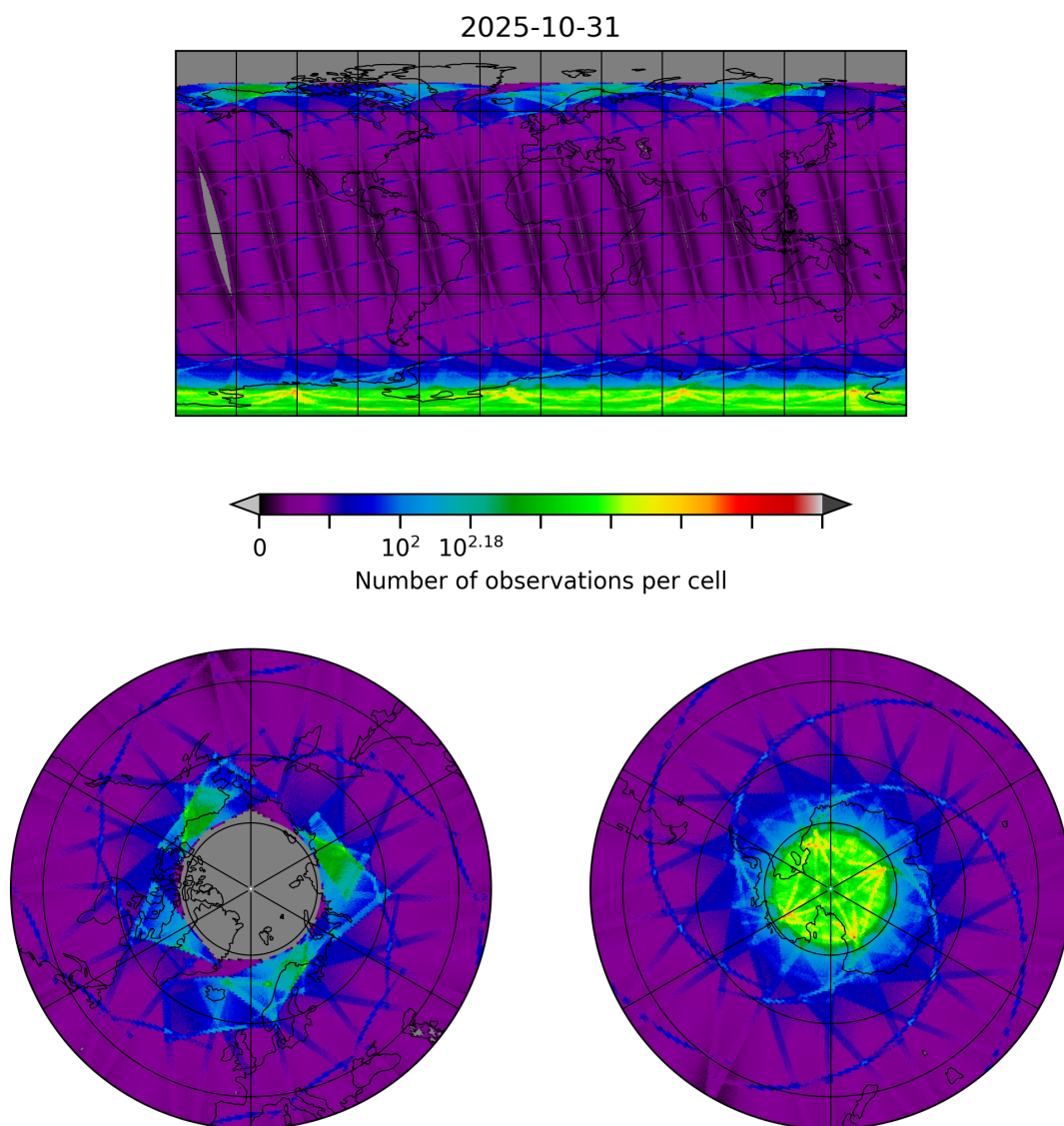
Figure 8: Map of the number of observations for 2025-10-31 to 2025-10-31
