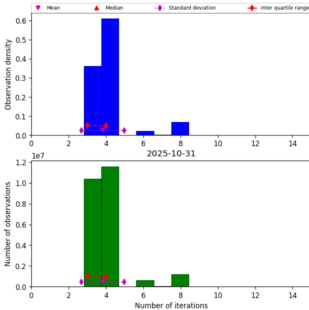
Figure 32: Histogram of “Number of iterations” for 2025-10-31 to 2025-10-31
