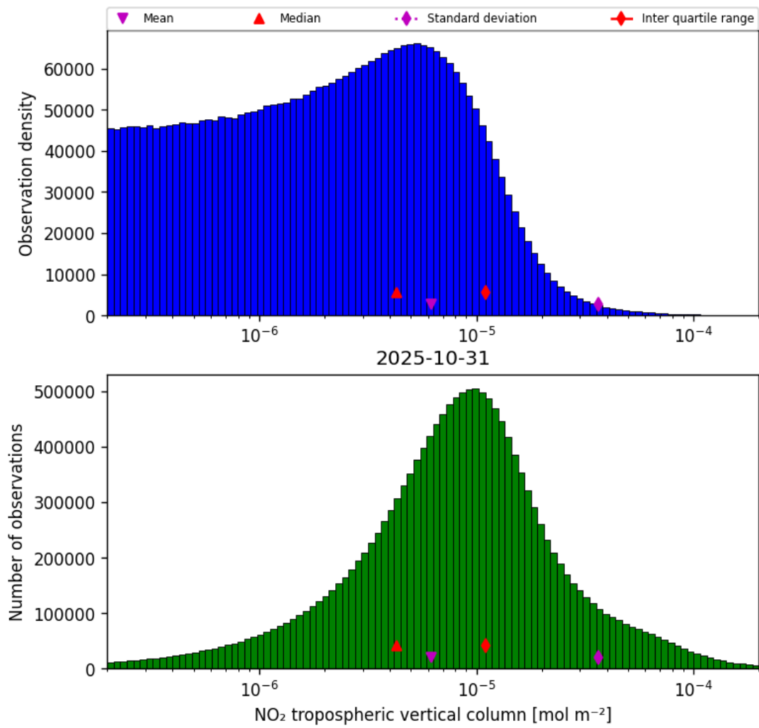
Figure 27: Histogram of “NO 2 tropospheric vertical column” for 2025-10-31 to 2025-10-31
