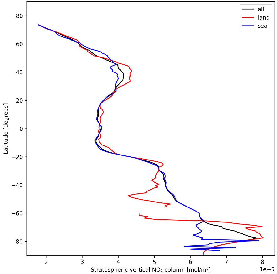
Figure 17: Zonal average of “Stratospheric vertical NO 2 column” for 2025-10-31 to 2025-10-31.
