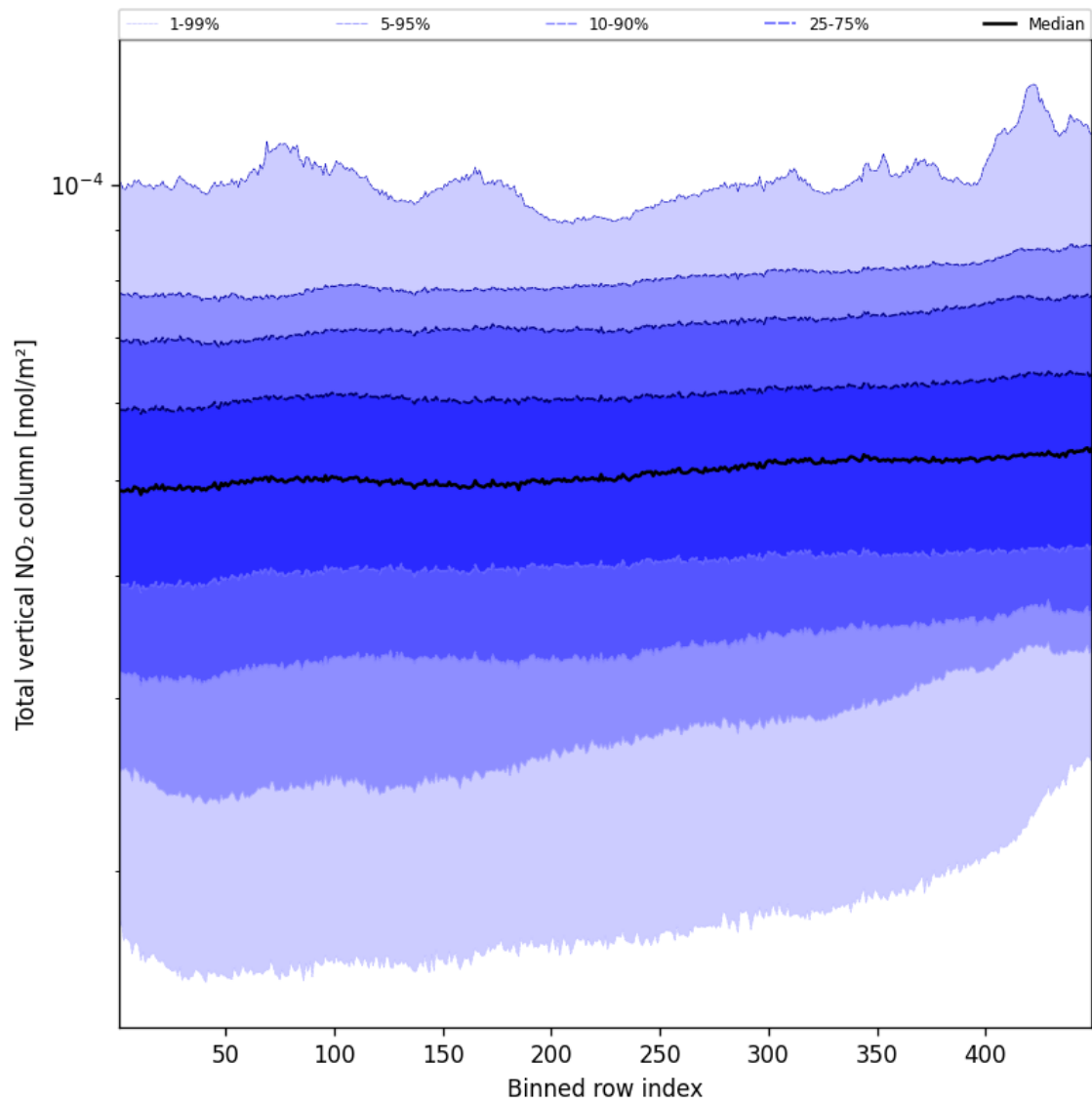
Figure 53: Along track statistics of “Total vertical NO 2 column” for 2025-10-31 to 2025-10-31
