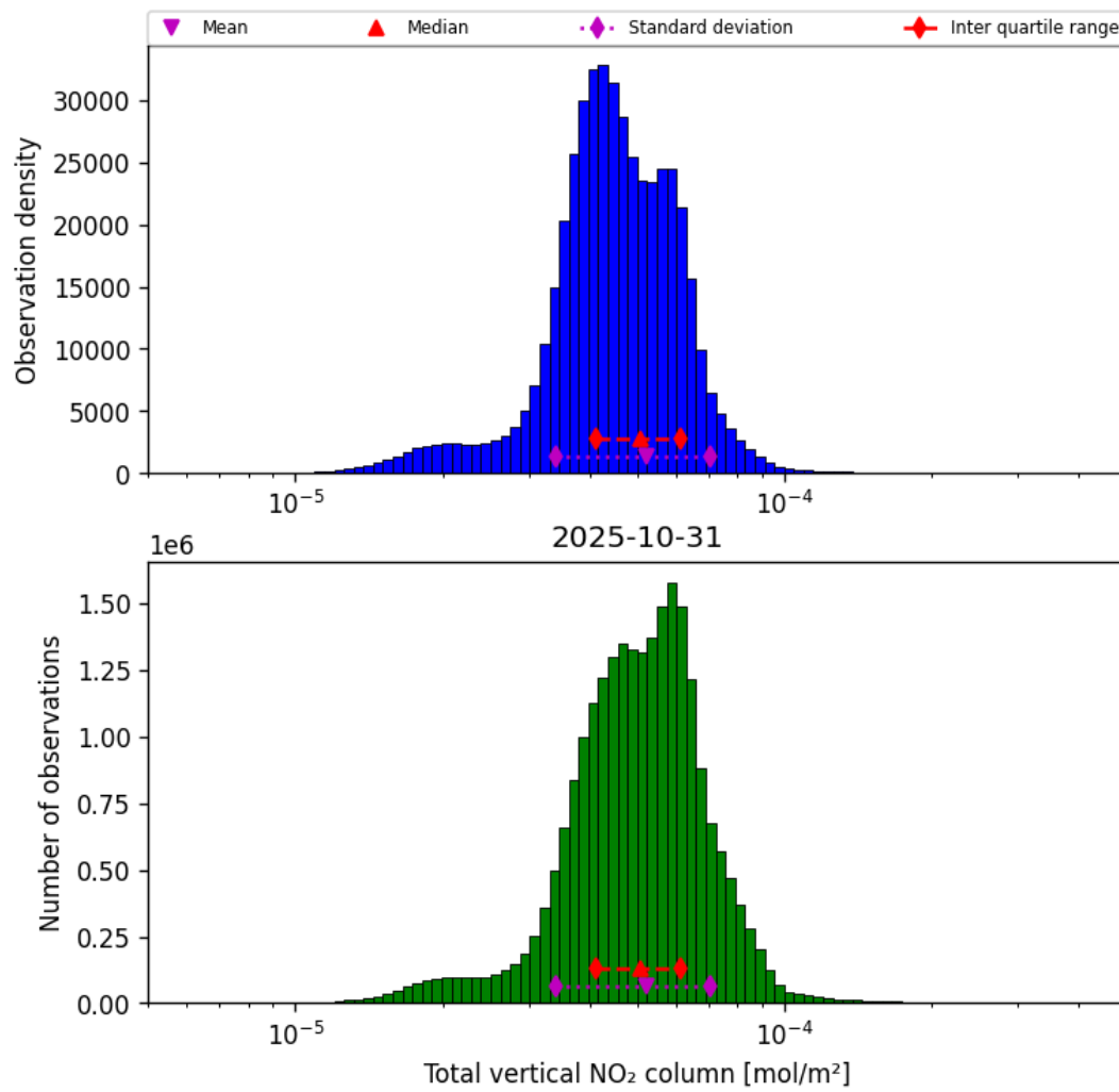
Figure 36: Histogram of "Total vertical NO 2 column" for 2025-10-31 to 2025-10-31
