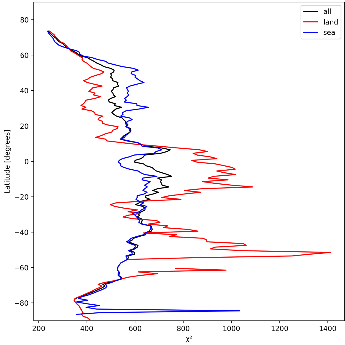
Figure 23: Zonal average of “ \chi^2 ” for 2025-10-31 to 2025-10-31.
