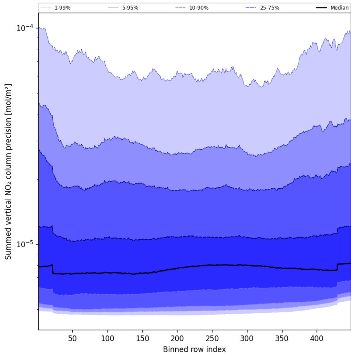
Figure 56: Along track statistics of “Summed vertical NO 2 column precision” for 2025-10-31 to 2025-10-31
