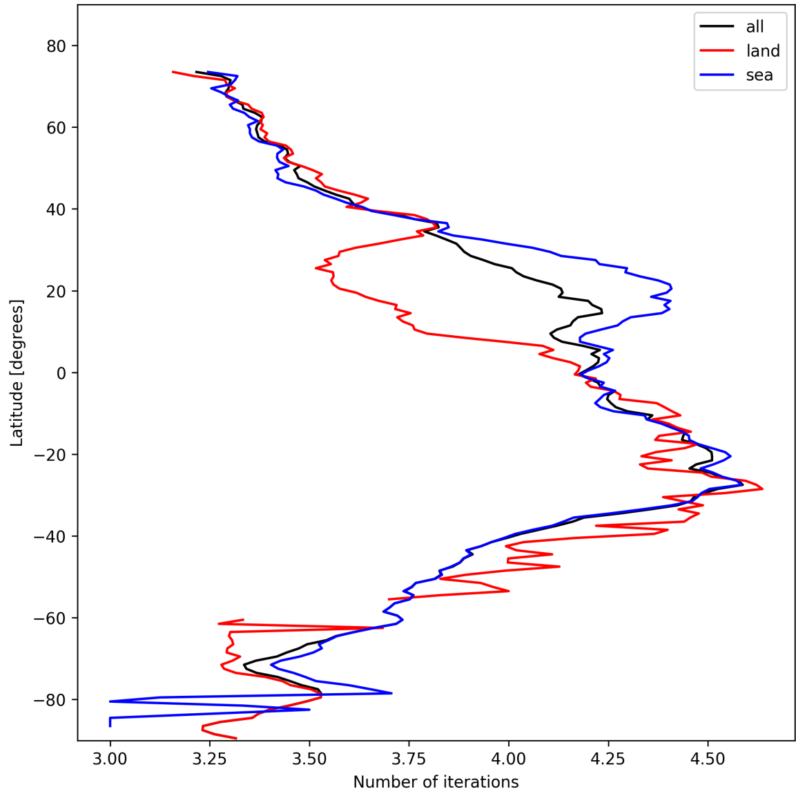
Figure 15: Zonal average of “Number of iterations” for 2025-10-31 to 2025-10-31.
