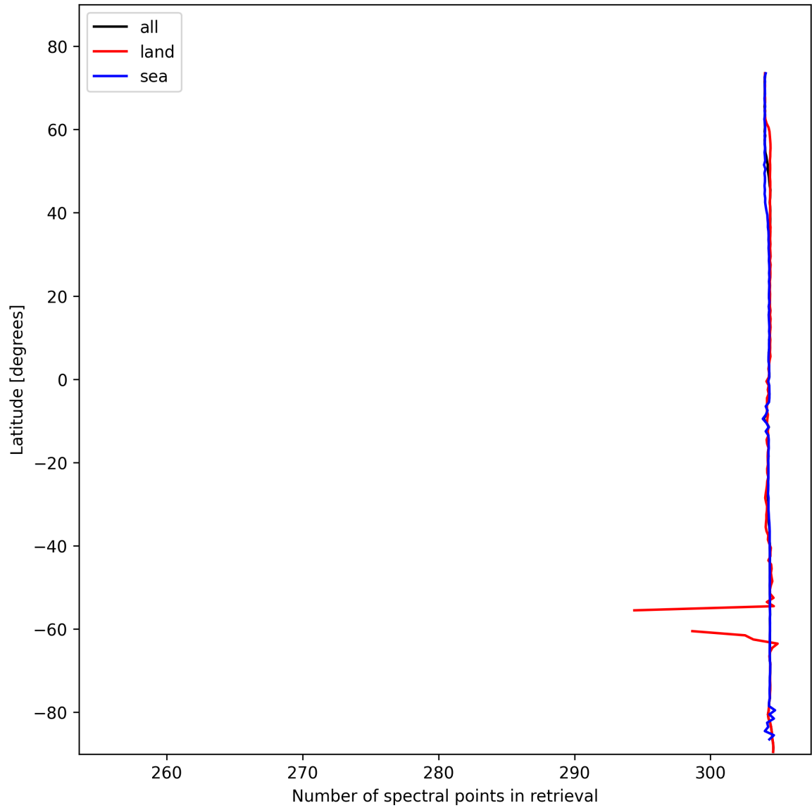
Figure 14: Zonal average of “Number of spectral points in retrieval” for 2025-10-31 to 2025-10-31.
