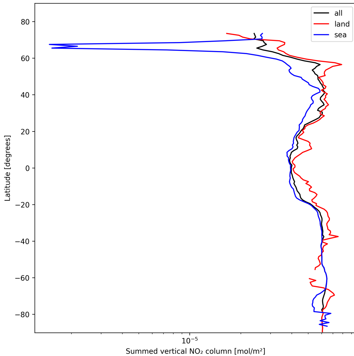
Figure 21: Zonal average of “Summed vertical NO 2 column” for 2025-10-31 to 2025-10-31.
