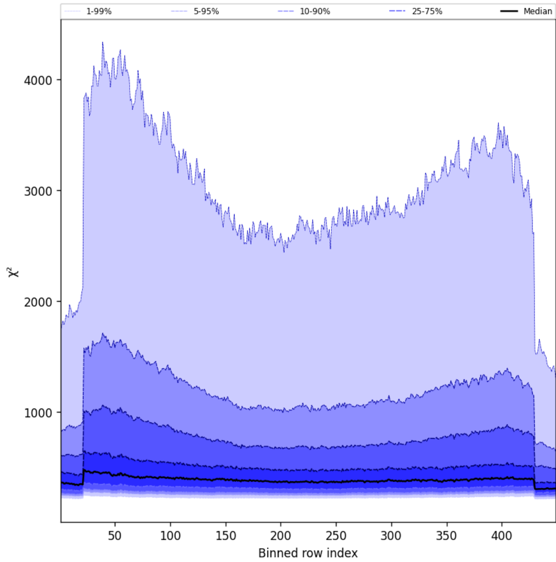
Figure 57: Along track statistics of “ \chi^2 ” for 2025-10-31 to 2025-10-31
