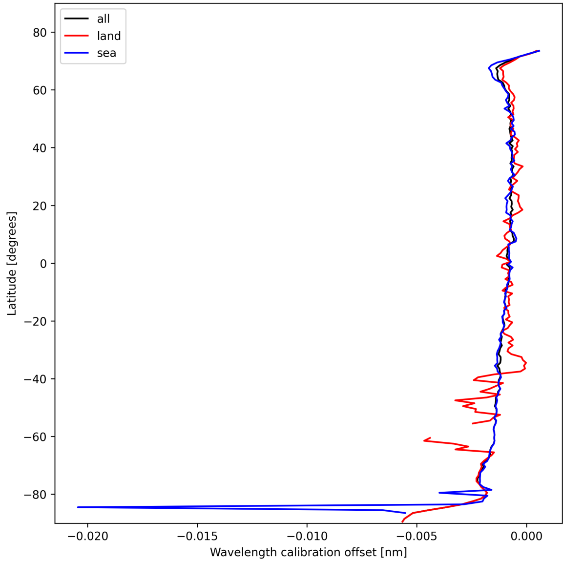
Figure 16: Zonal average of “Wavelength calibration offset” for 2025-10-31 to 2025-10-31.
