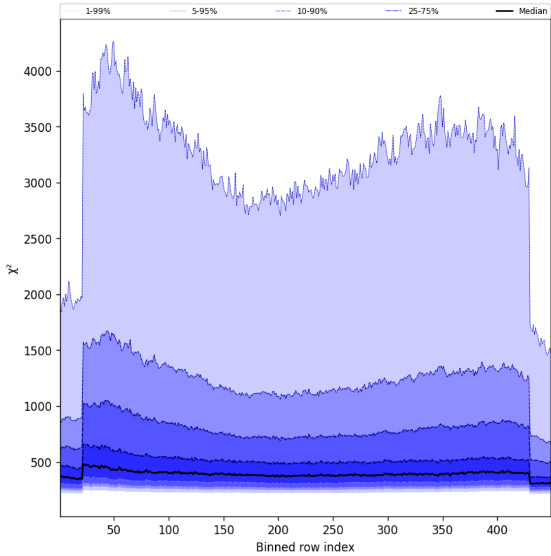
Figure 57: Along track statistics of “ \chi^2 ” for 2025-11-01 to 2025-11-02
