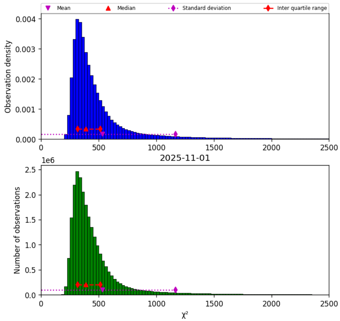
Figure 40: Histogram of “ \chi^2 ” for 2025-11-01 to 2025-11-02
