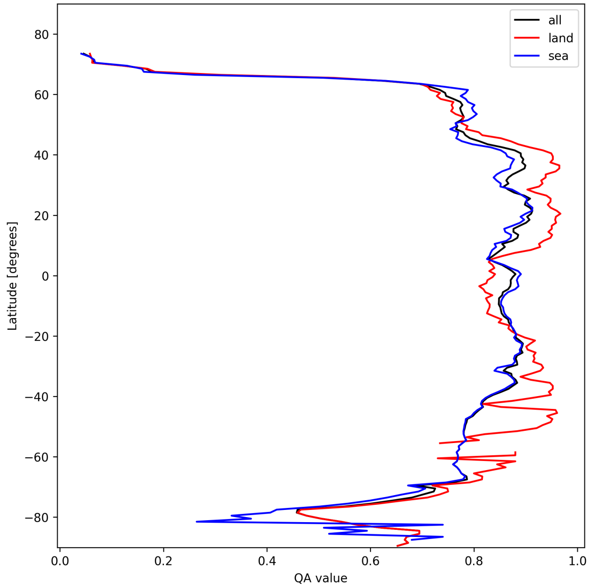
Figure 9: Zonal average of “QA value” for 2025-11-01 to 2025-11-02.
