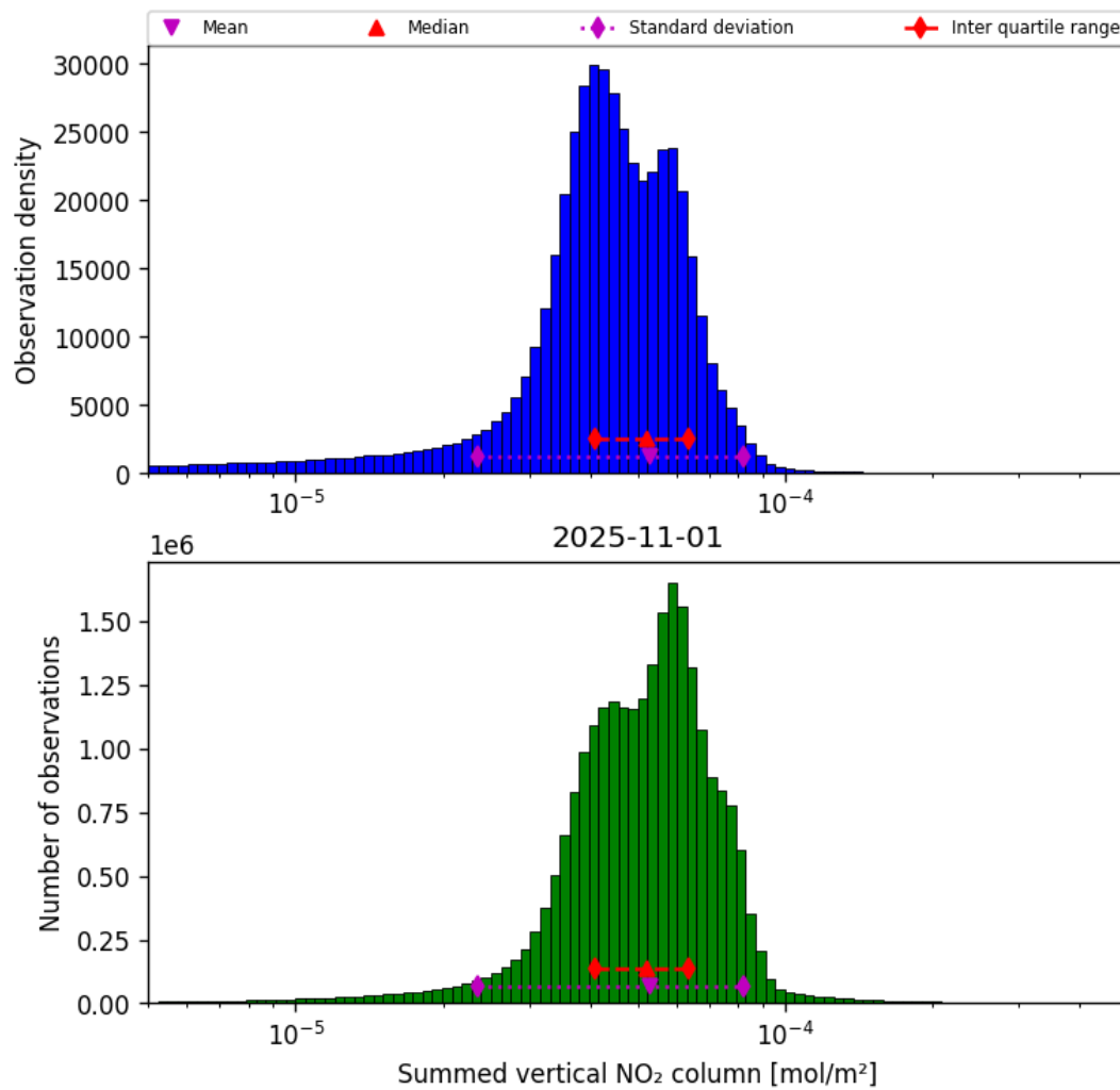
Figure 38: Histogram of “Summed vertical NO 2 column” for 2025-11-01 to 2025-11-02
