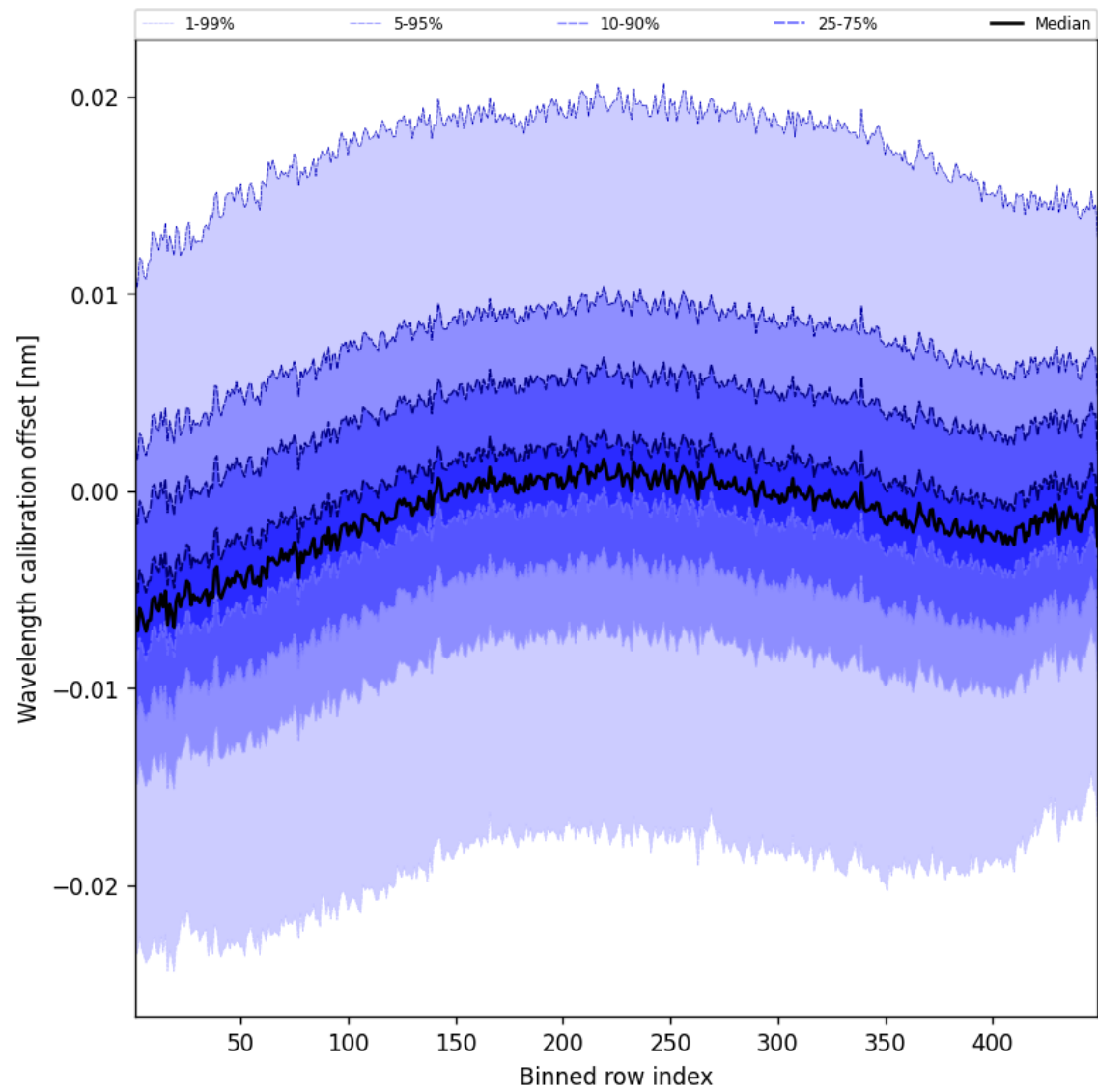
Figure 50: Along track statistics of “Wavelength calibration offset” for 2025-11-01 to 2025-11-02
