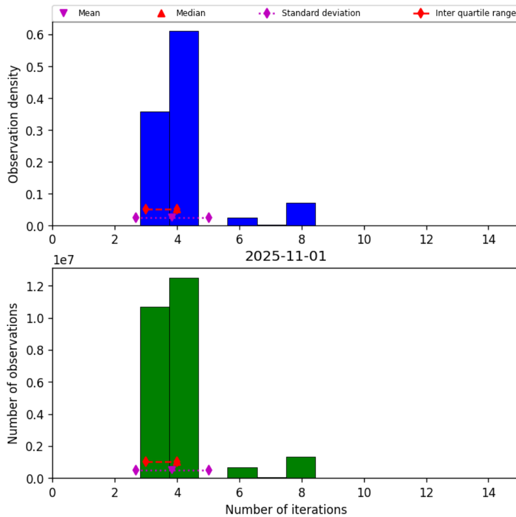
Figure 32: Histogram of “Number of iterations” for 2025-11-01 to 2025-11-02
