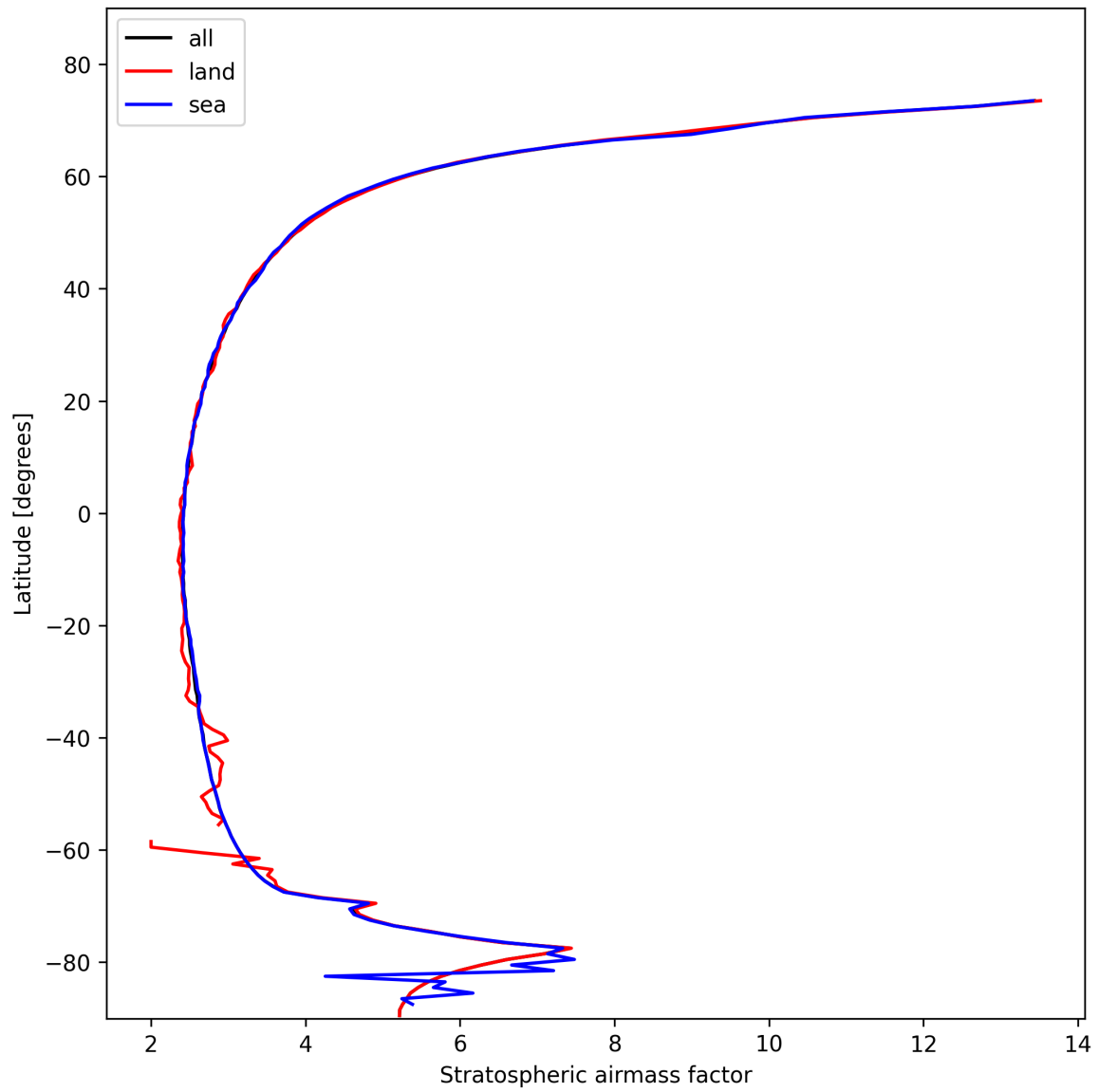
Figure 25: Zonal average of “Stratospheric airmass factor” for 2025-11-01 to 2025-11-02.
