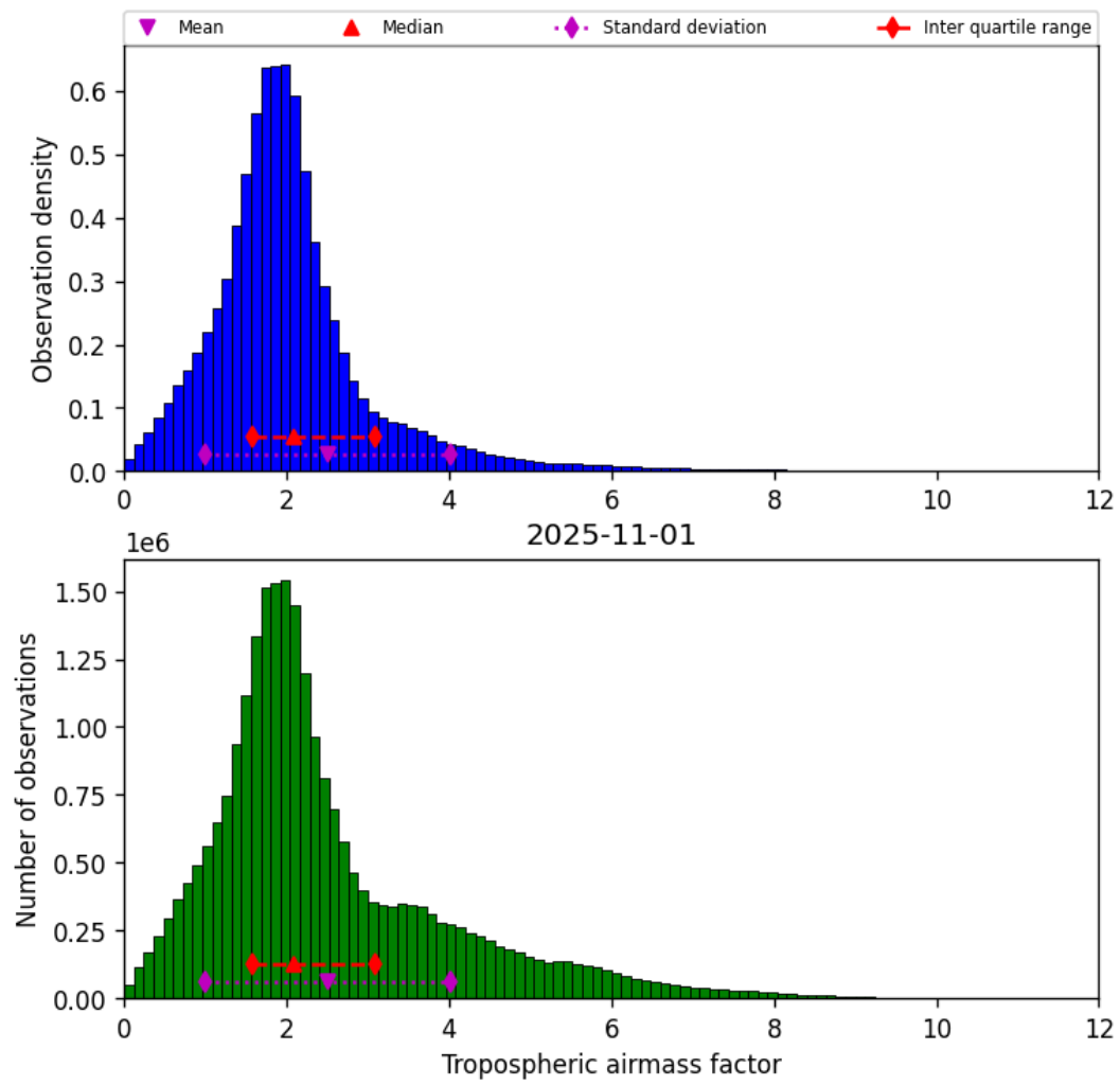
Figure 29: Histogram of “Tropospheric airmass factor” for 2025-11-01 to 2025-11-02
