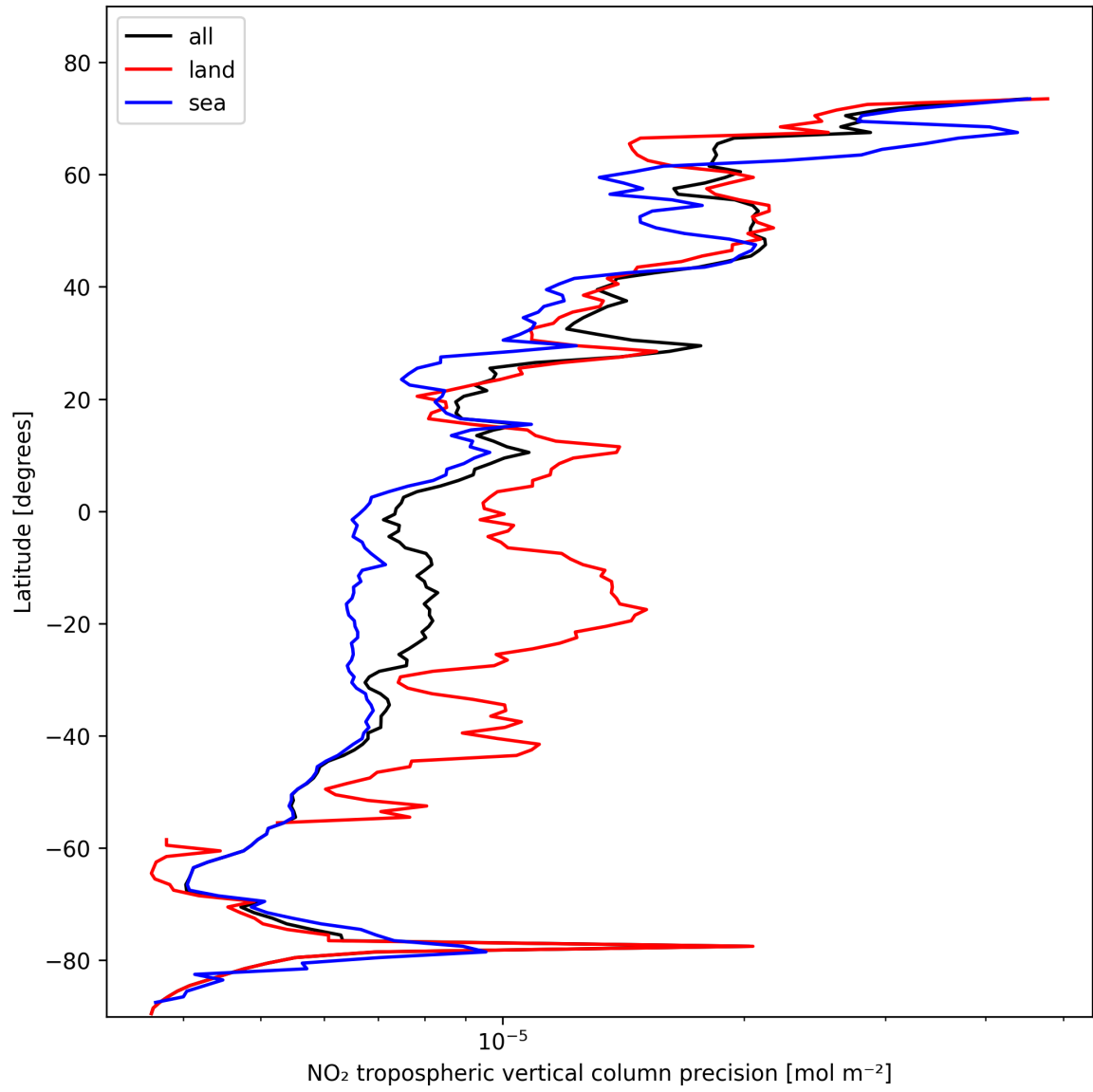
Figure 11: Zonal average of “NO 2 tropospheric vertical column precision” for 2025-11-01 to 2025-11-02.
