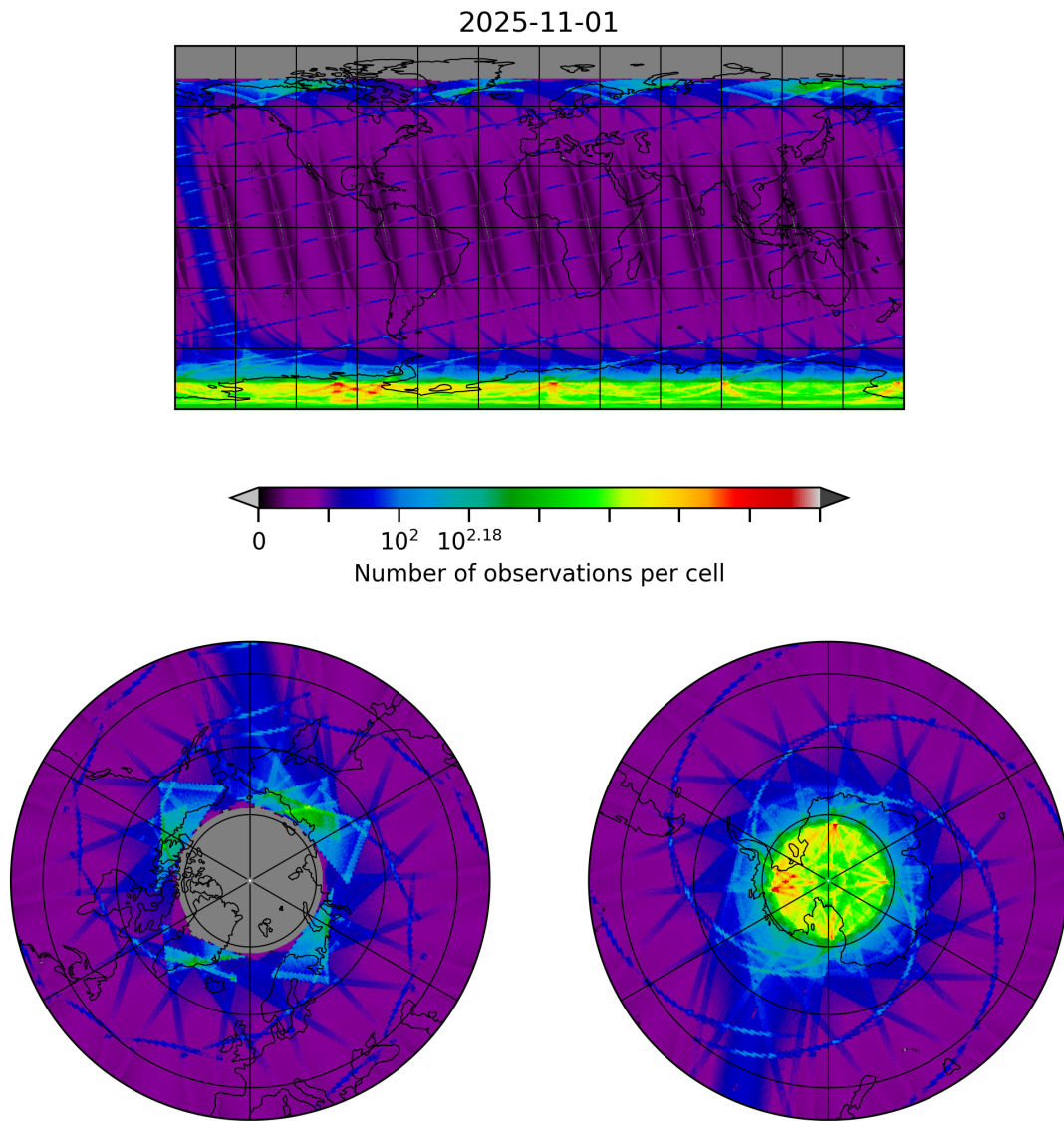
Figure 8: Map of the number of observations for 2025-11-01 to 2025-11-02
