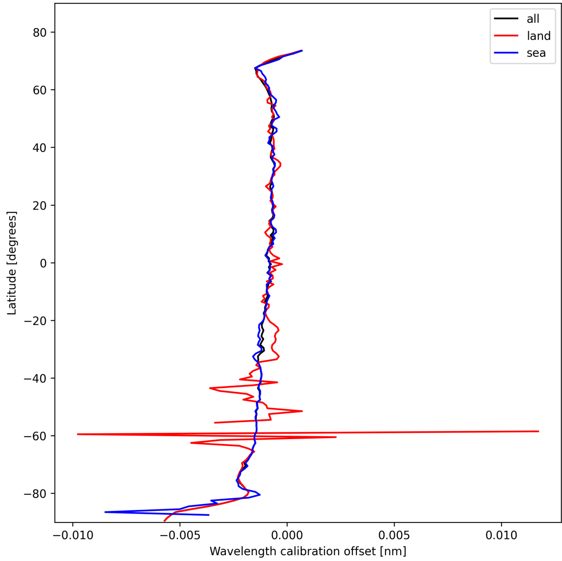
Figure 16: Zonal average of “Wavelength calibration offset” for 2025-11-01 to 2025-11-02.
