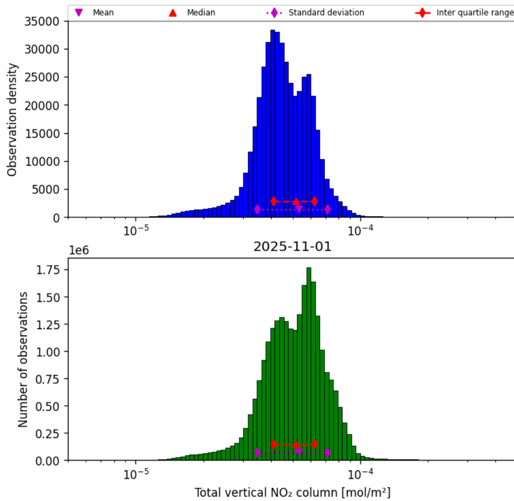
Figure 36: Histogram of “Total vertical NO 2 column” for 2025-11-01 to 2025-11-02
