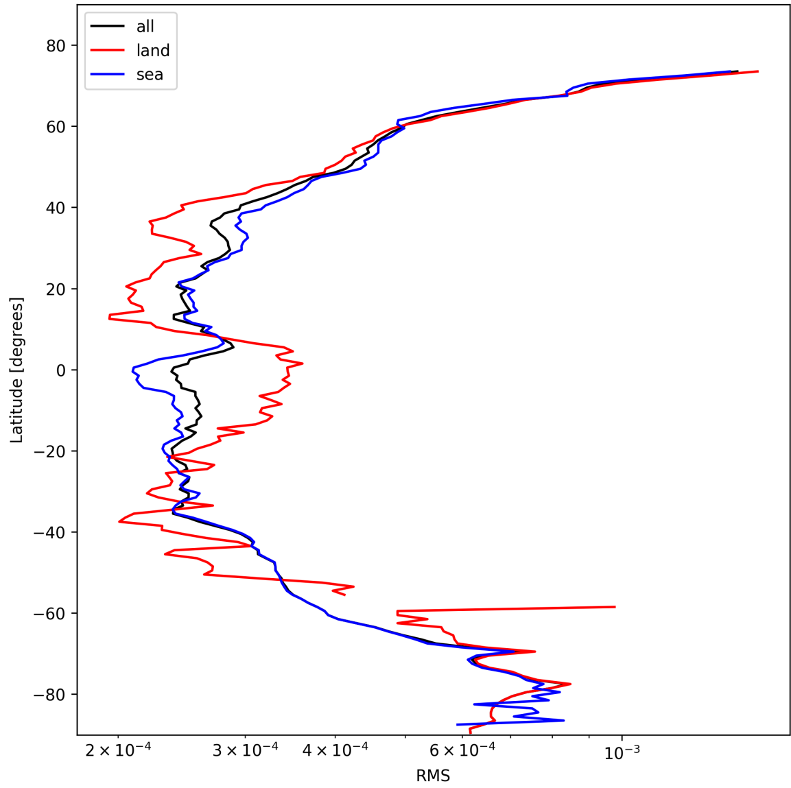
Figure 24: Zonal average of “RMS” for 2025-11-01 to 2025-11-02.
