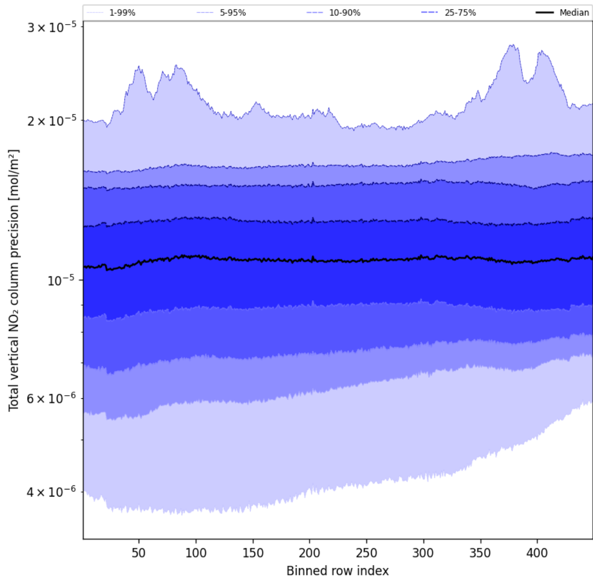
Figure 54: Along track statistics of “Total vertical NO 2 column precision” for 2025-11-01 to 2025-11-02
