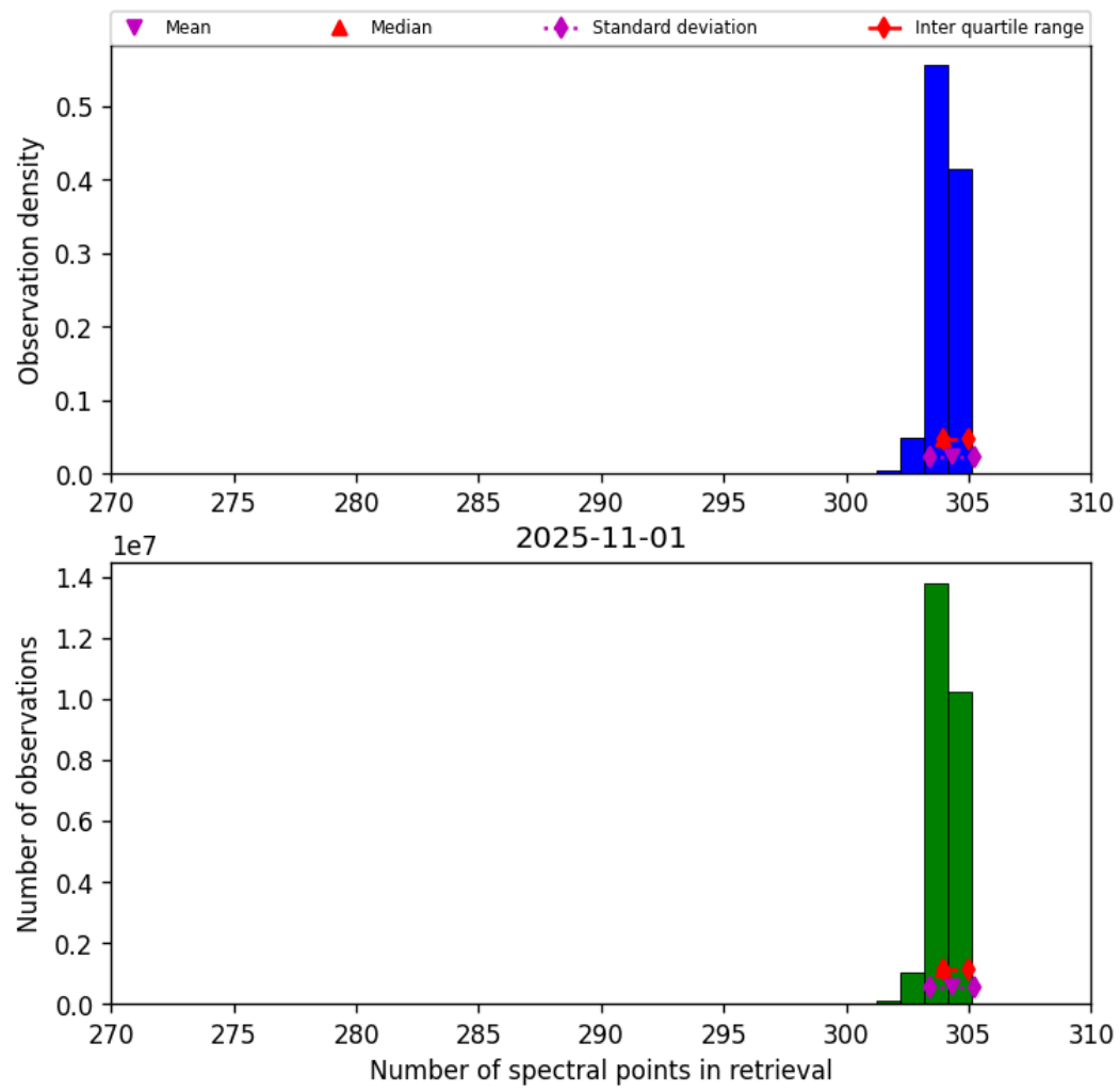
Figure 31: Histogram of “Number of spectral points in retrieval” for 2025-11-01 to 2025-11-02
