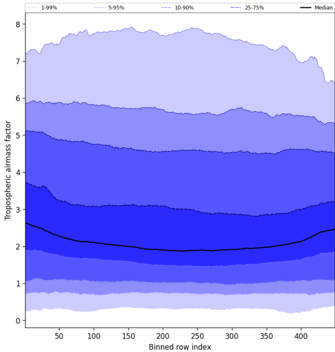
Figure 46: Along track statistics of “Tropospheric airmass factor” for 2025-11-01 to 2025-11-02
