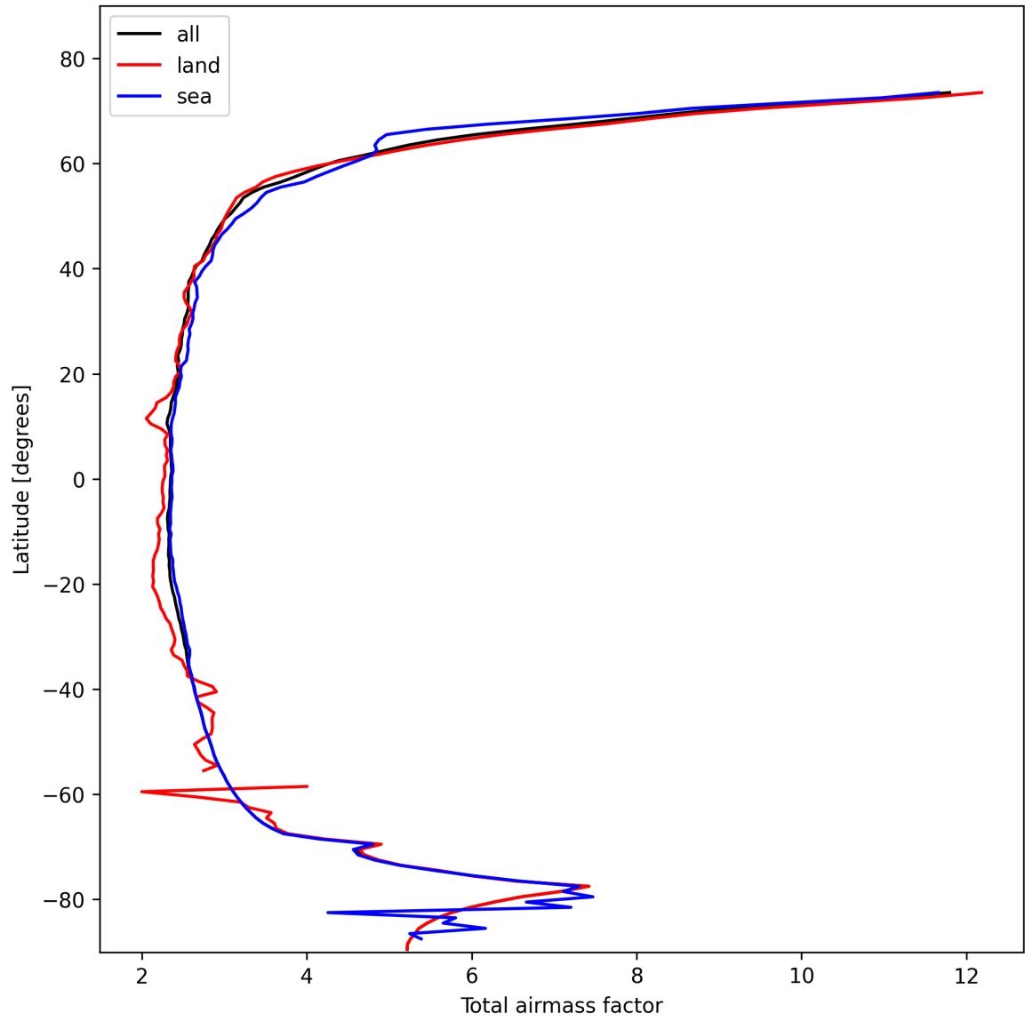
Figure 13: Zonal average of “Total airmass factor” for 2025-11-01 to 2025-11-02.
