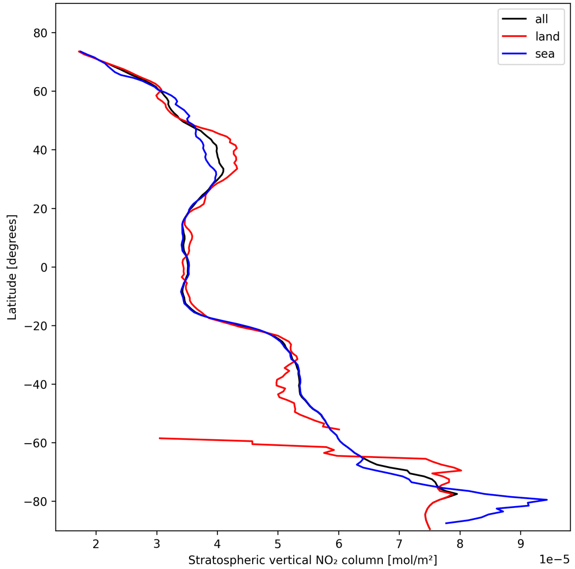
Figure 17: Zonal average of “Stratospheric vertical NO 2 column” for 2025-11-01 to 2025-11-02.
