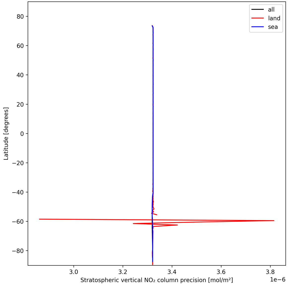
Figure 18: Zonal average of “Stratospheric vertical NO 2 column precision” for 2025-11-01 to 2025-11-02.
