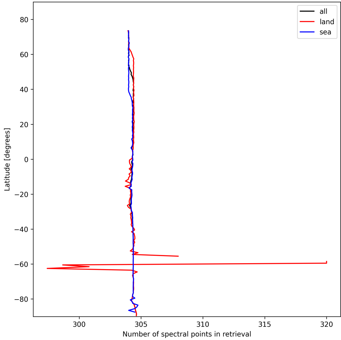
Figure 14: Zonal average of “Number of spectral points in retrieval” for 2025-11-01 to 2025-11-02.
