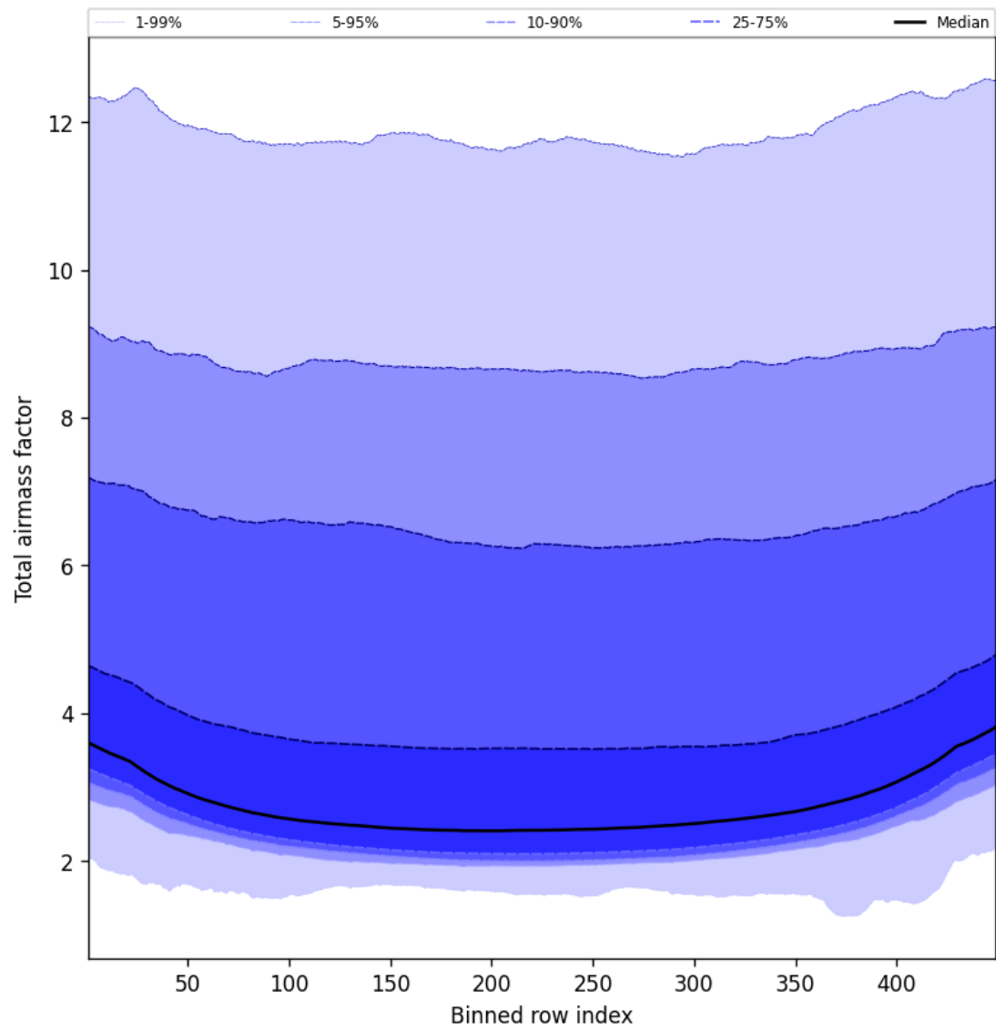
Figure 47: Along track statistics of “Total airmass factor” for 2025-11-01 to 2025-11-02
