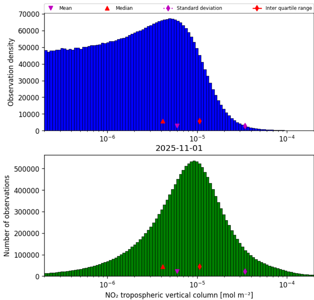
Figure 27: Histogram of “NO 2 tropospheric vertical column” for 2025-11-01 to 2025-11-02
