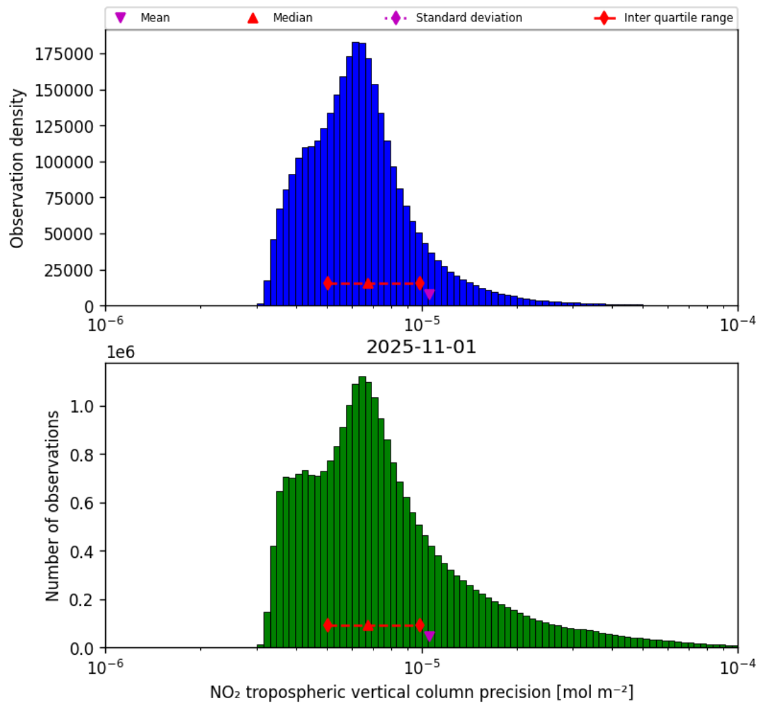
Figure 28: Histogram of “NO 2 tropospheric vertical column precision” for 2025-11-01 to 2025-11-02
