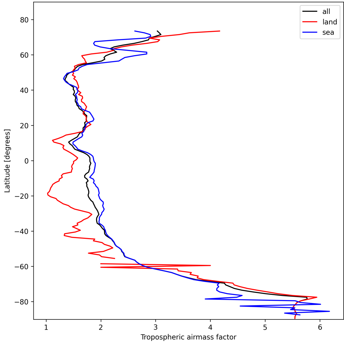
Figure 12: Zonal average of “Tropospheric airmass factor” for 2025-11-01 to 2025-11-02.
