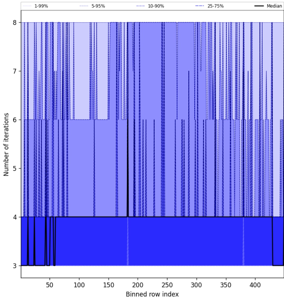
Figure 49: Along track statistics of “Number of iterations” for 2025-11-01 to 2025-11-02
