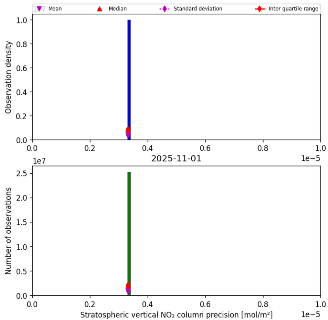
Figure 35: Histogram of “Stratospheric vertical NO 2 column precision” for 2025-11-01 to 2025-11-02
