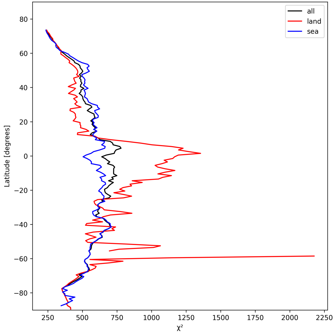
Figure 23: Zonal average of “ \chi^2 ” for 2025-11-01 to 2025-11-02.
