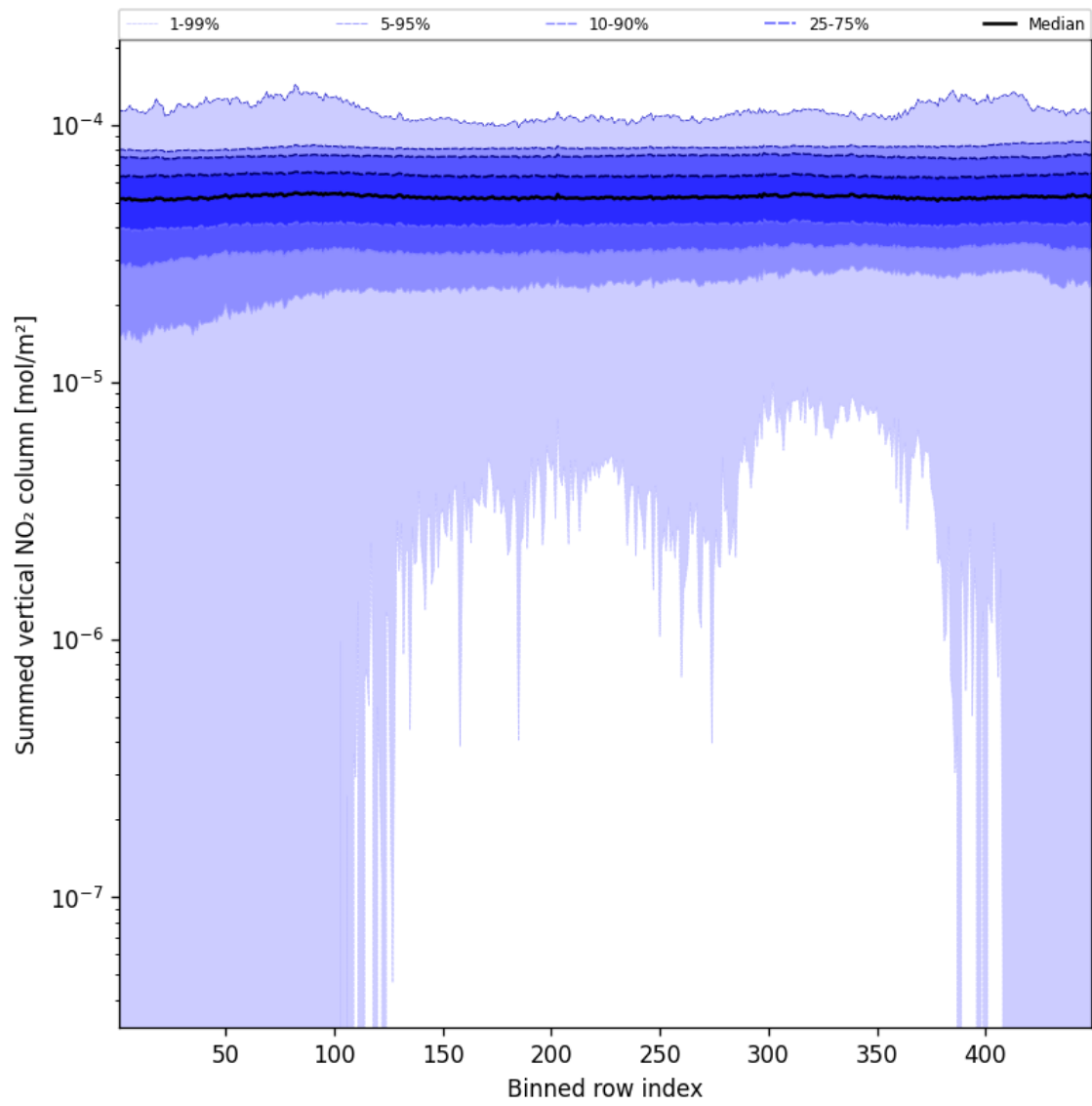
Figure 55: Along track statistics of “Summed vertical NO 2 column” for 2025-11-01 to 2025-11-02
