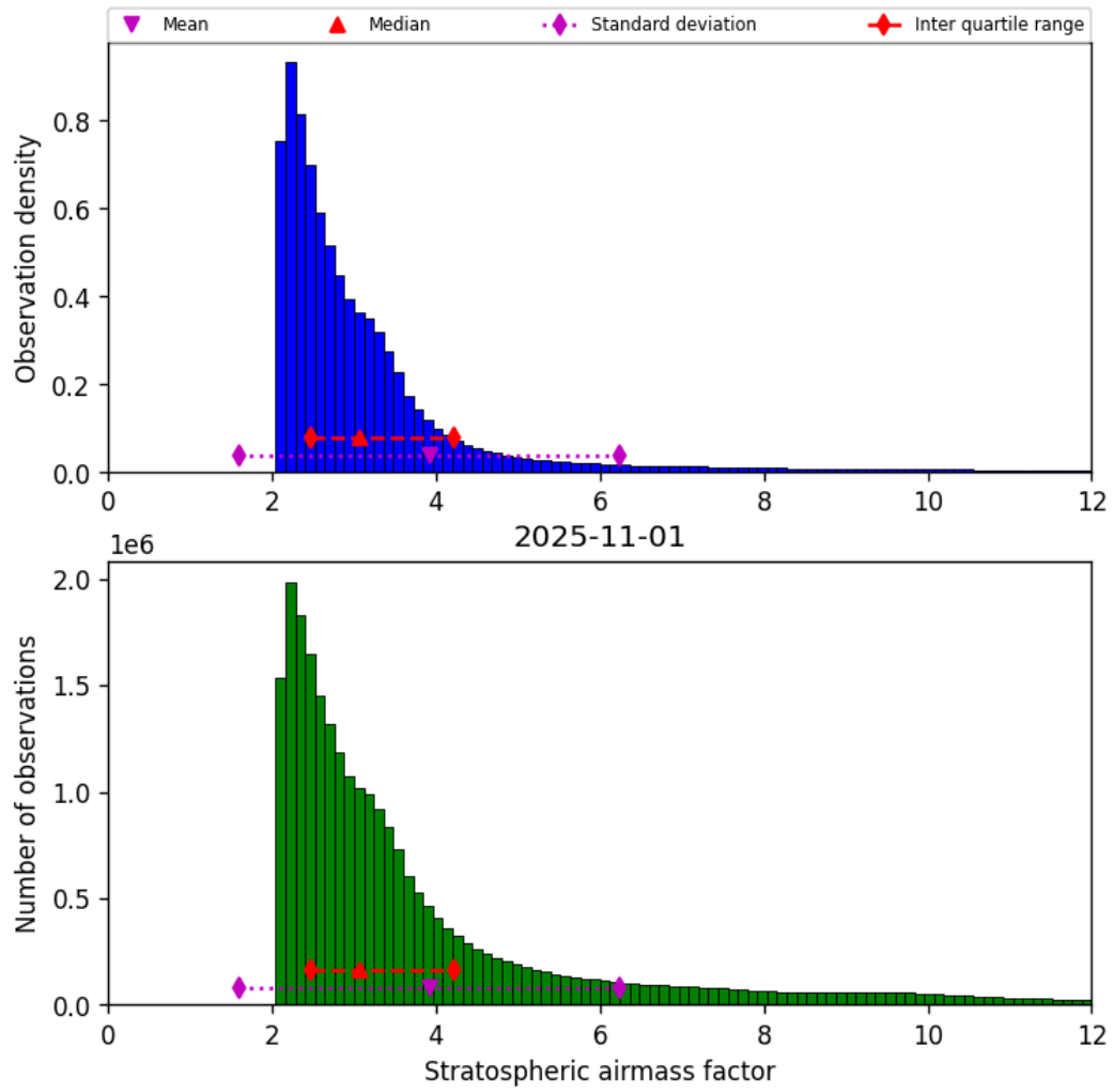
Figure 42: Histogram of “Stratospheric airmass factor” for 2025-11-01 to 2025-11-02
