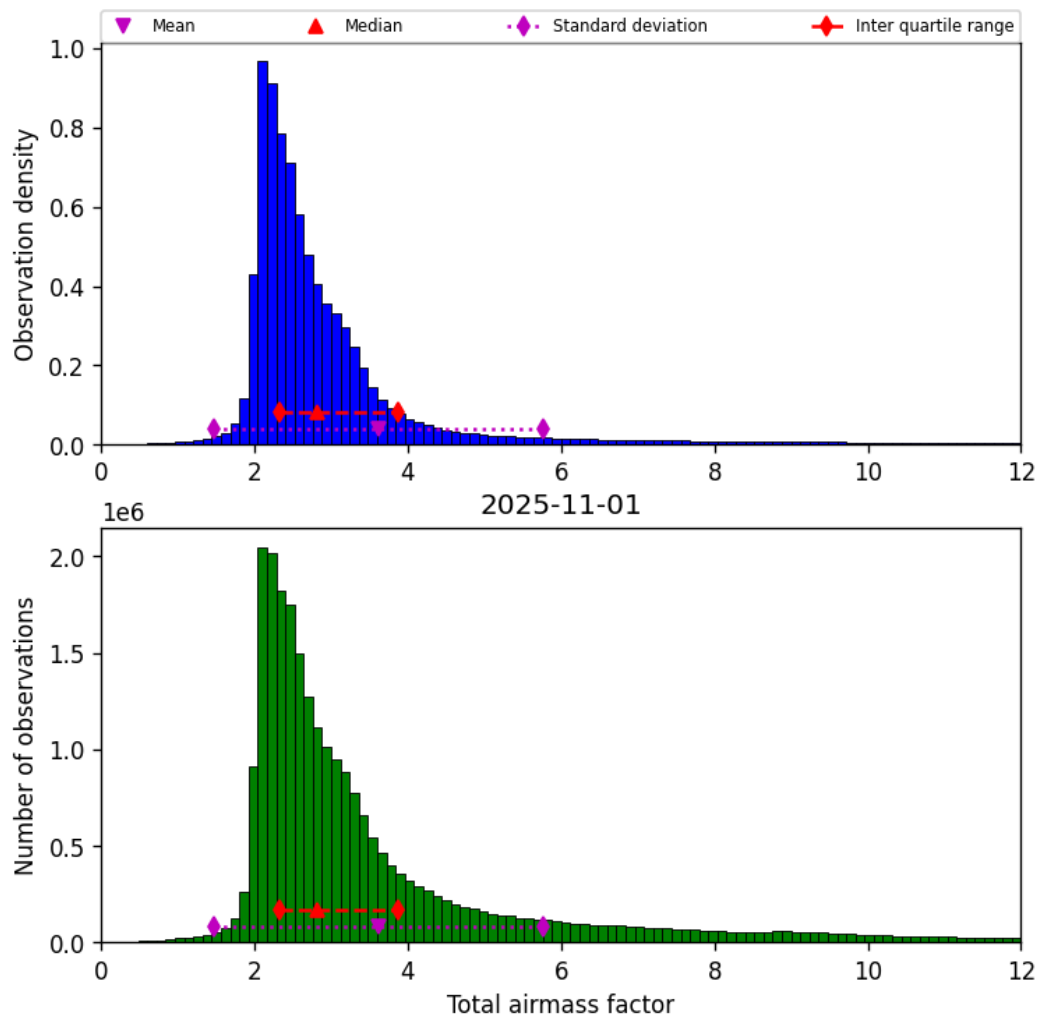
Figure 30: Histogram of “Total airmass factor” for 2025-11-01 to 2025-11-02
