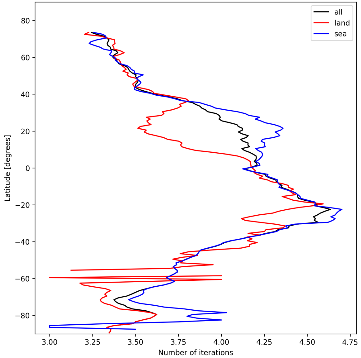
Figure 15: Zonal average of “Number of iterations” for 2025-11-01 to 2025-11-02.
