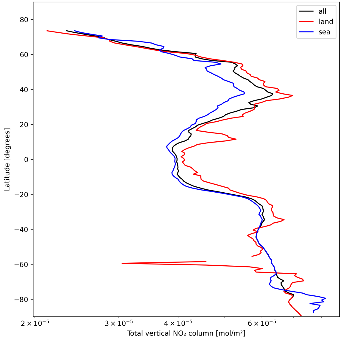
Figure 19: Zonal average of “Total vertical NO 2 column” for 2025-11-01 to 2025-11-02.
