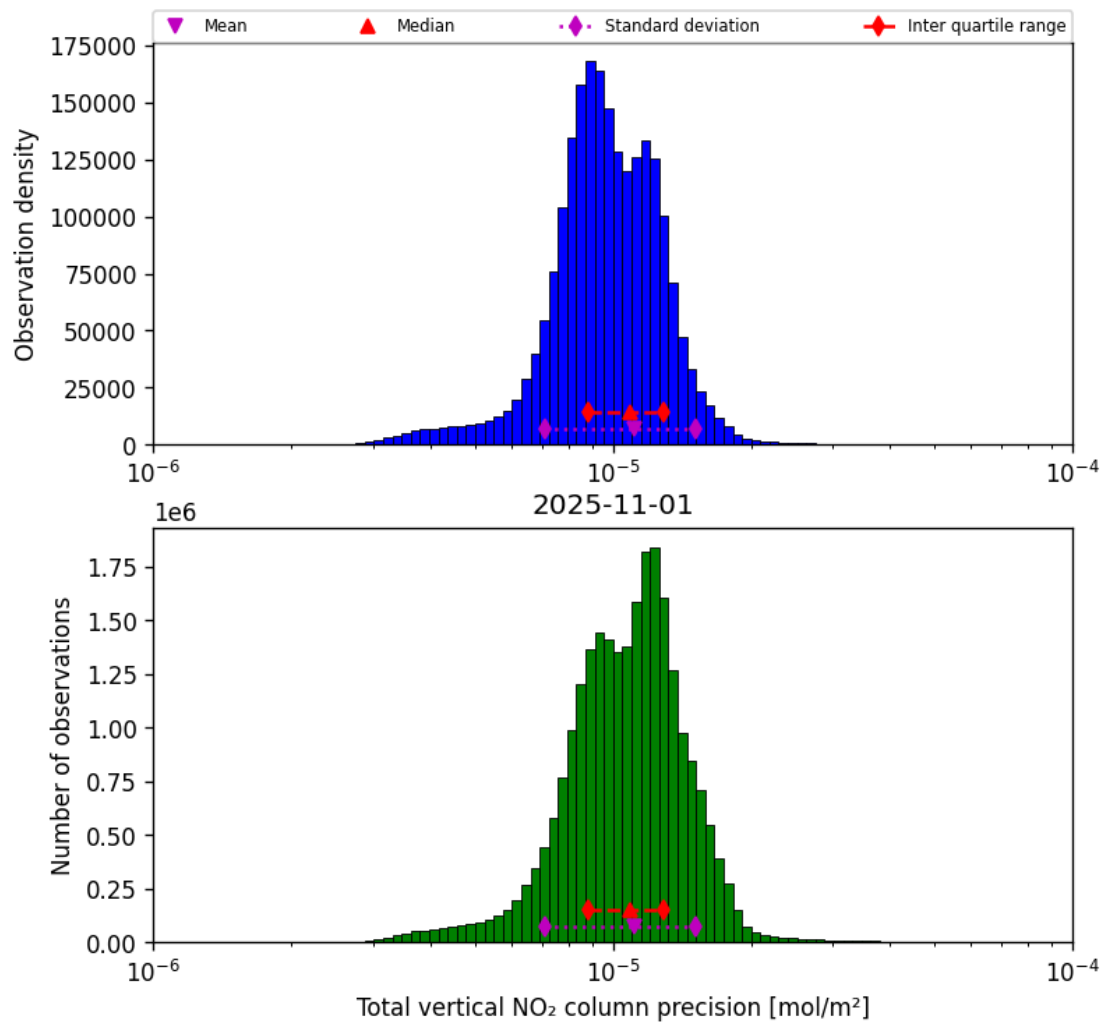
Figure 37: Histogram of “Total vertical NO 2 column precision” for 2025-11-01 to 2025-11-02
