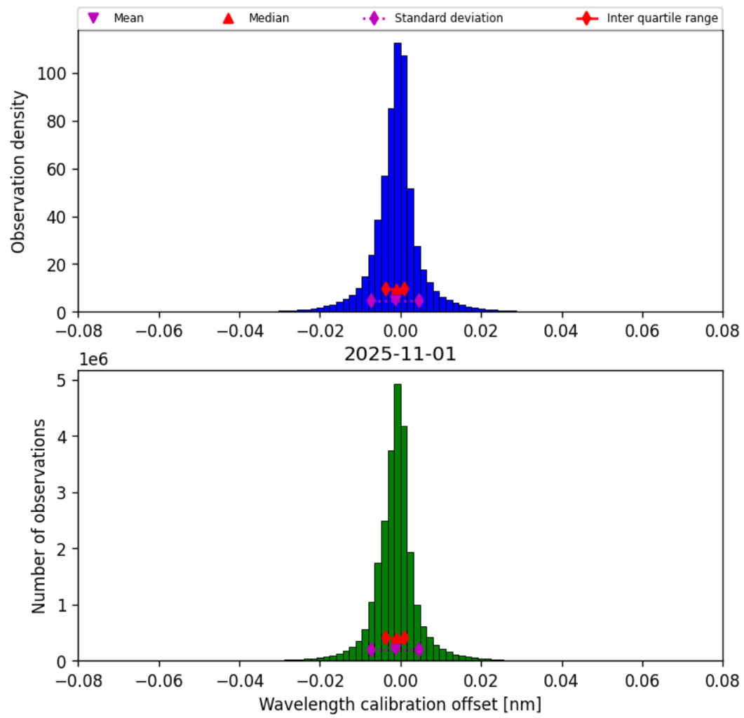
Figure 33: Histogram of “Wavelength calibration offset” for 2025-11-01 to 2025-11-02
