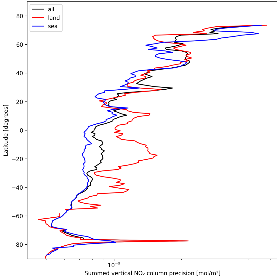
Figure 22: Zonal average of “Summed vertical NO 2 column precision” for 2025-11-01 to 2025-11-02.
