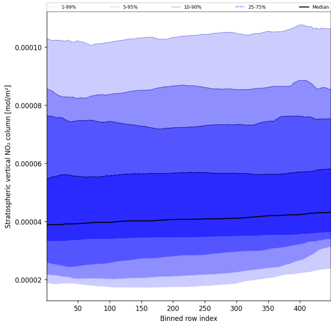
Figure 51: Along track statistics of “Stratospheric vertical NO 2 column” for 2025-11-01 to 2025-11-02
