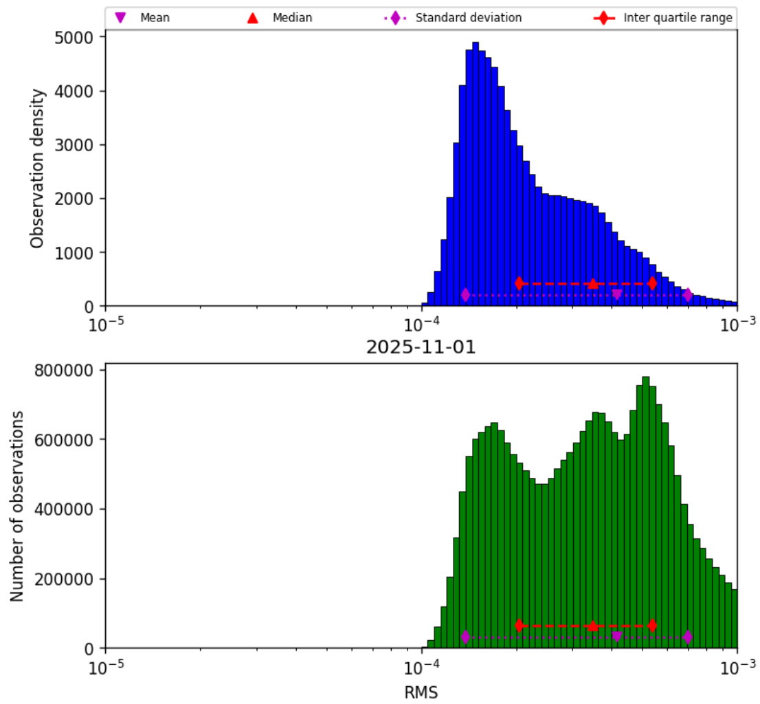
Figure 41: Histogram of “RMS” for 2025-11-01 to 2025-11-02
