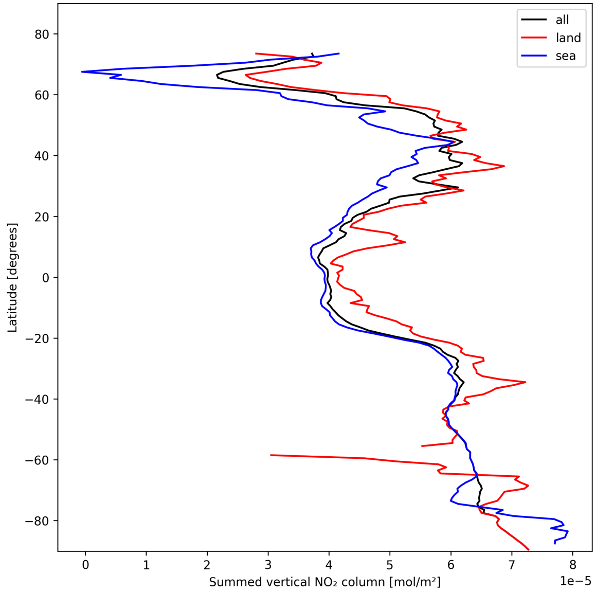
Figure 21: Zonal average of “Summed vertical NO 2 column” for 2025-11-01 to 2025-11-02.
