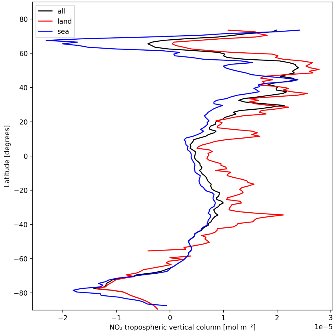
Figure 10: Zonal average of “NO 2 tropospheric vertical column” for 2025-11-01 to 2025-11-02.
