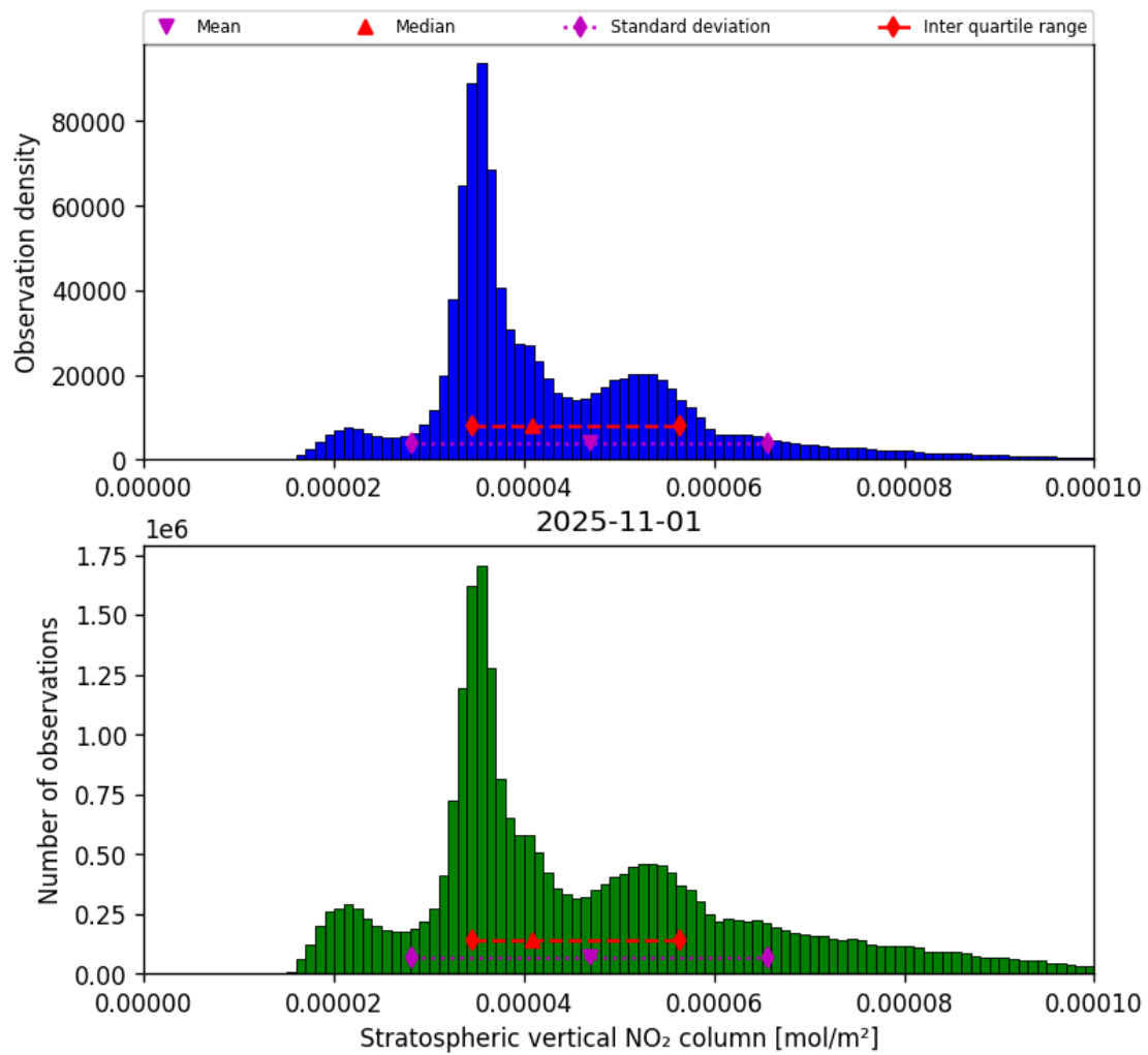
Figure 34: Histogram of “Stratospheric vertical NO 2 column” for 2025-11-01 to 2025-11-02
