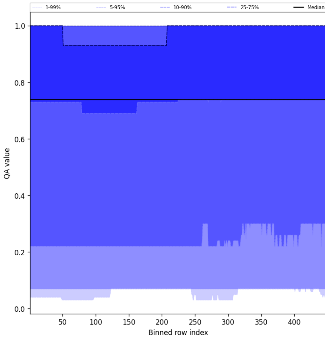
Figure 43: Along track statistics of “QA value” for 2025-11-01 to 2025-11-02
