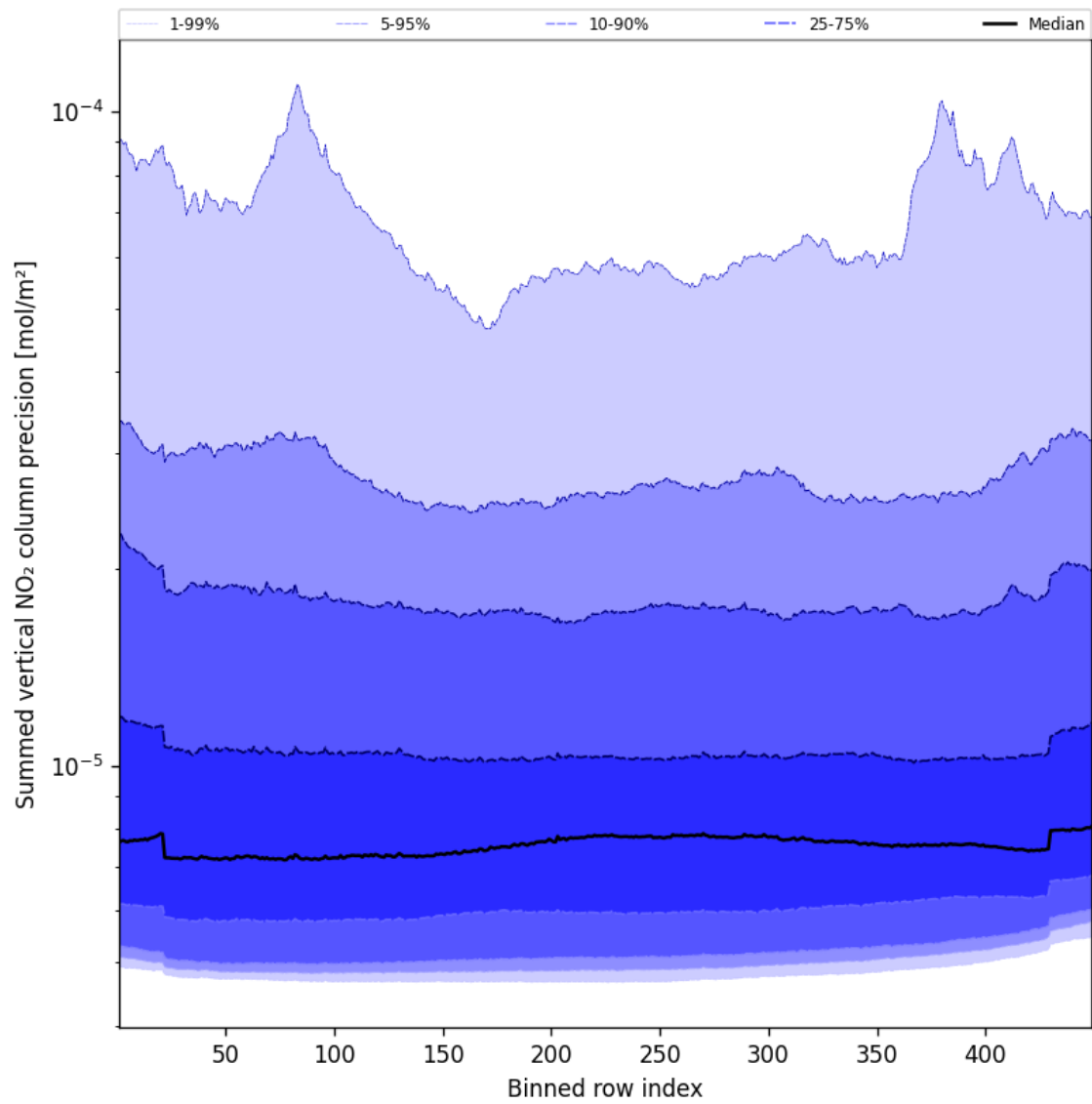
Figure 56: Along track statistics of “Summed vertical NO 2 column precision” for 2025-11-01 to 2025-11-02
