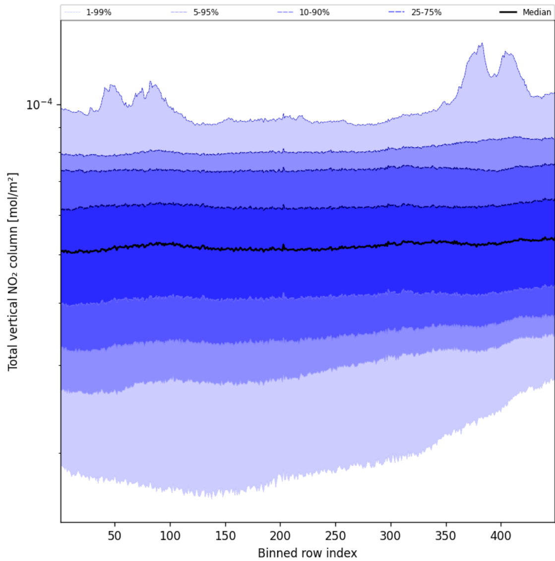
Figure 53: Along track statistics of “Total vertical NO 2 column” for 2025-11-01 to 2025-11-02
