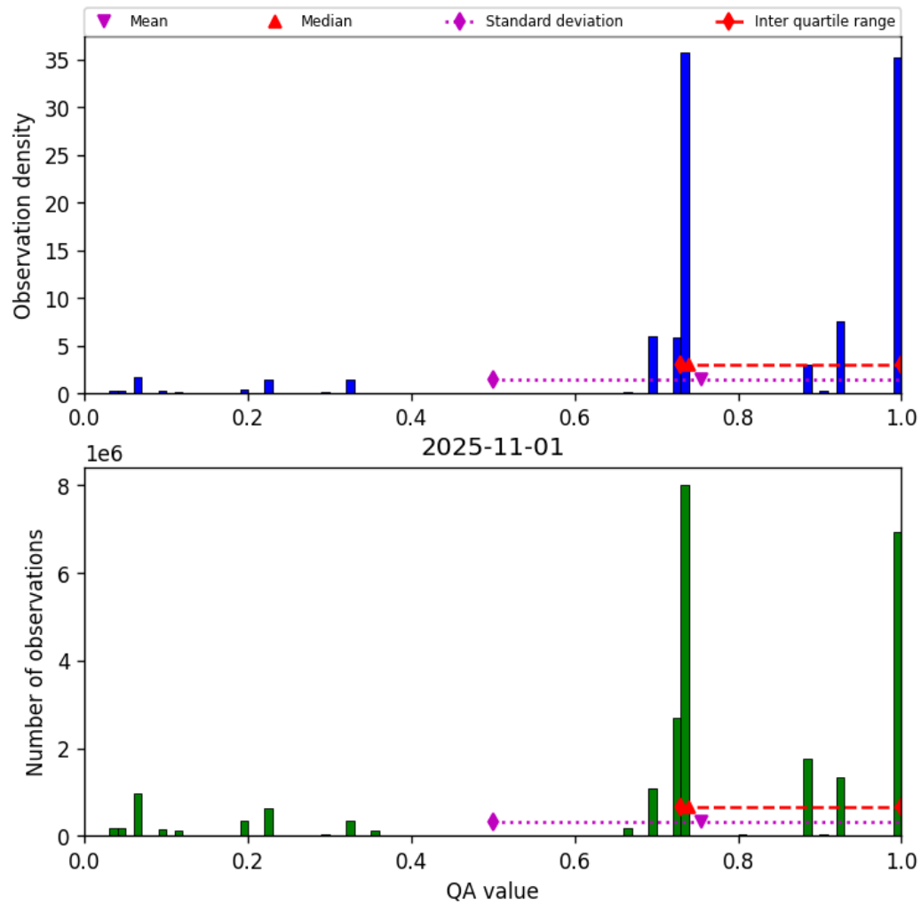
Figure 26: Histogram of “QA value” for 2025-11-01 to 2025-11-02
