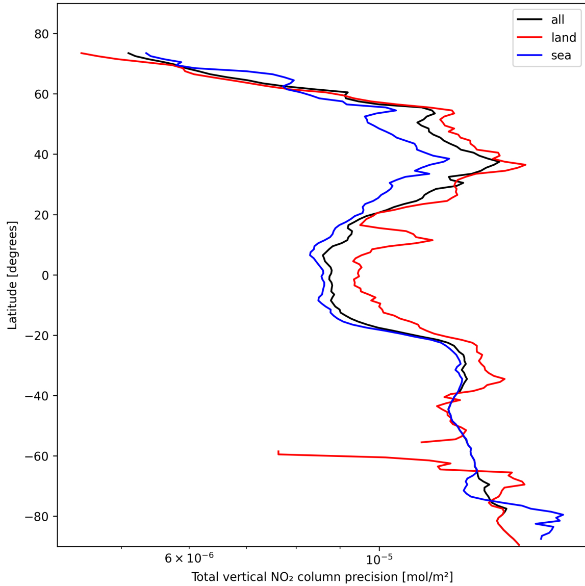
Figure 20: Zonal average of “Total vertical NO 2 column precision” for 2025-11-01 to 2025-11-02.
