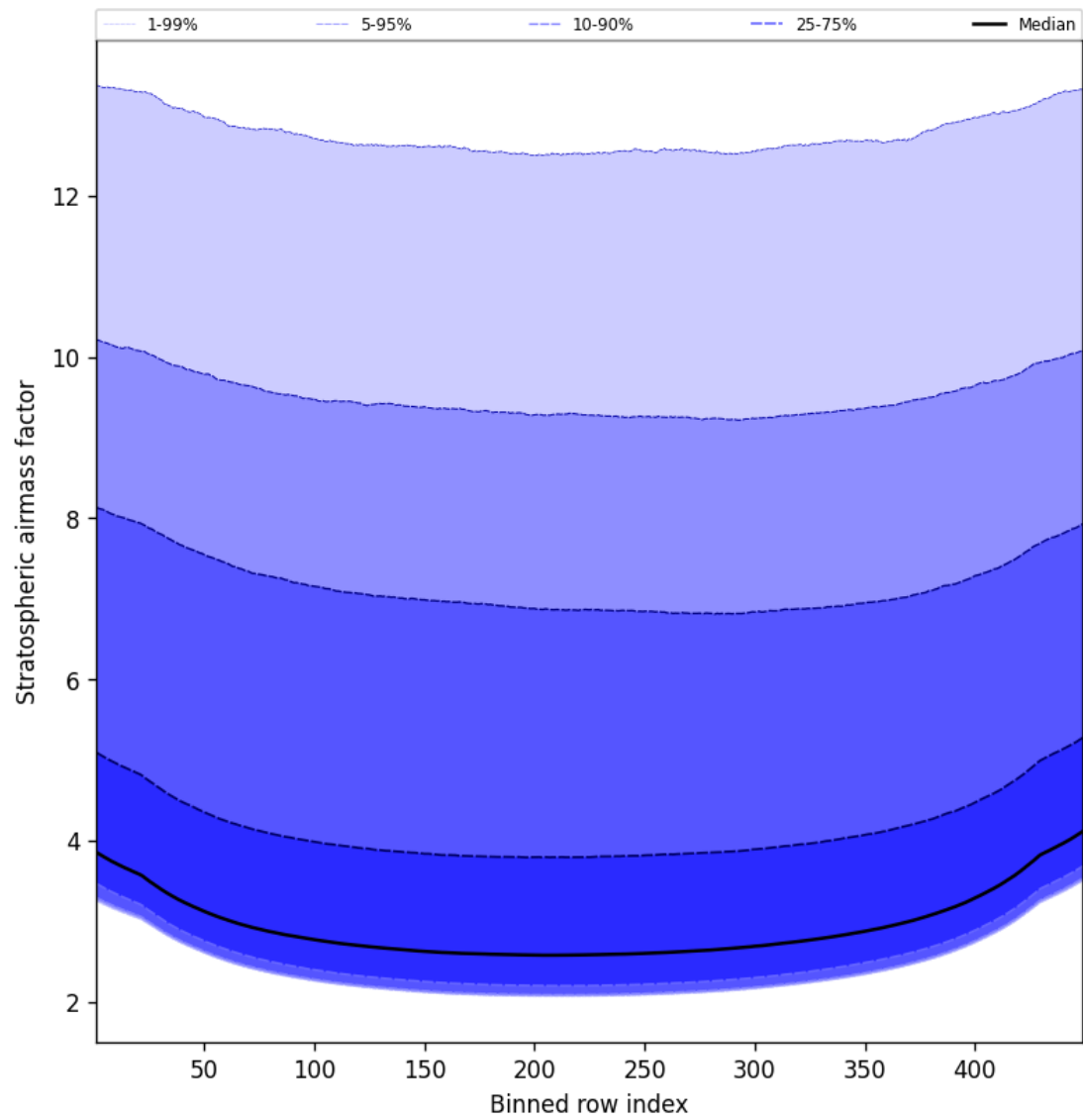
Figure 59: Along track statistics of “Stratospheric airmass factor” for 2025-11-01 to 2025-11-02
