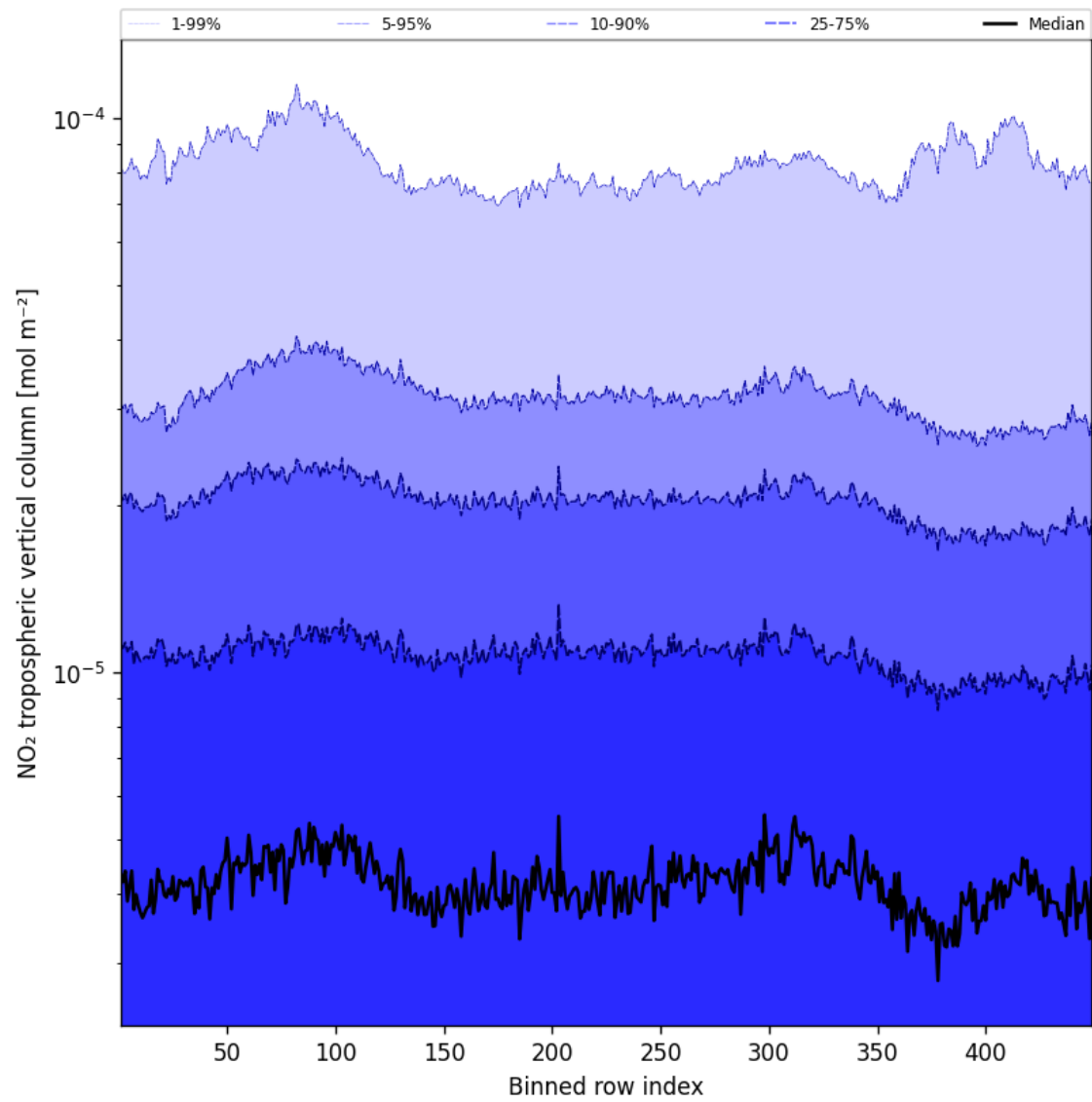
Figure 44: Along track statistics of “NO 2 tropospheric vertical column” for 2025-11-01 to 2025-11-02
