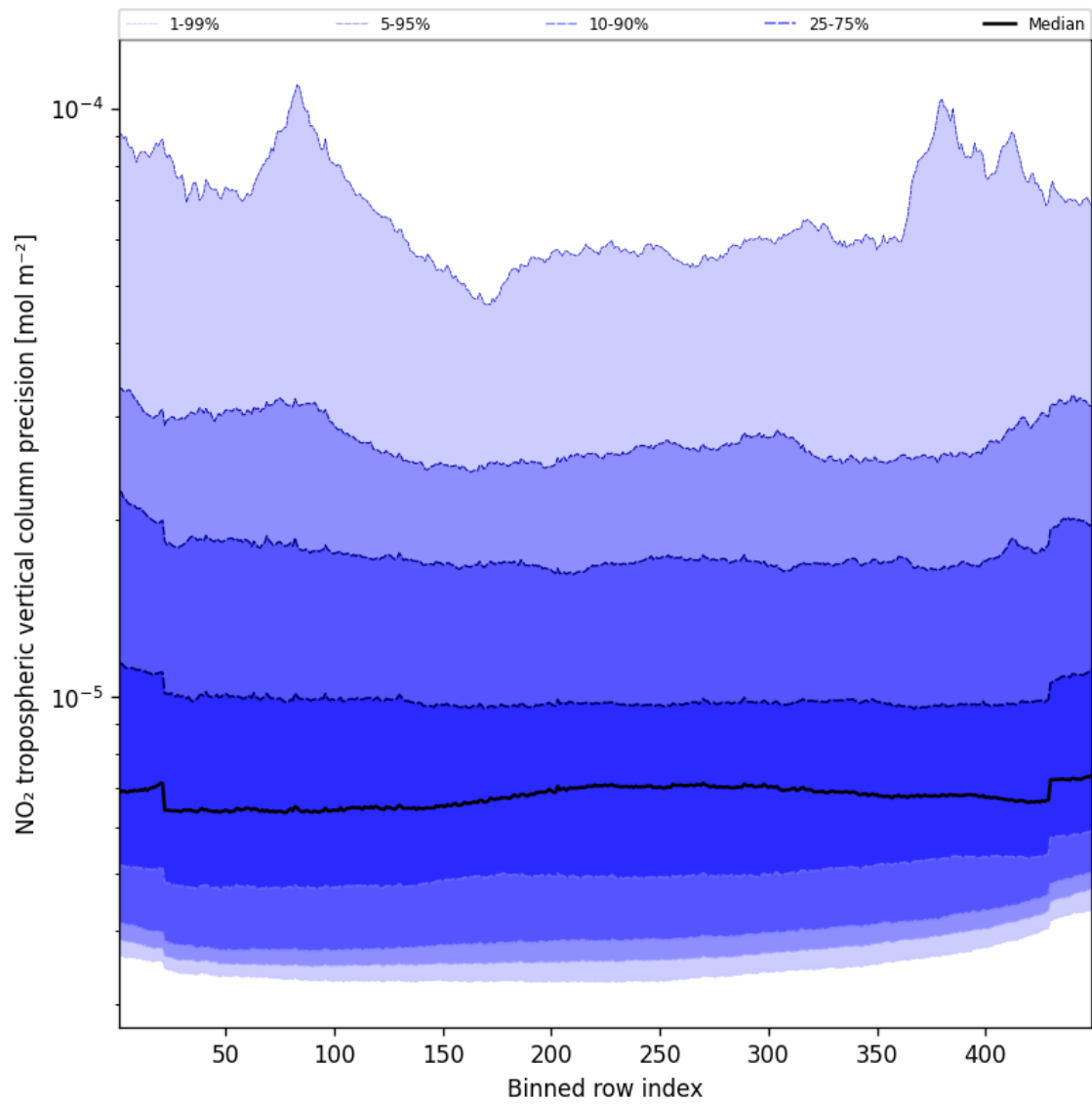
Figure 45: Along track statistics of “NO 2 tropospheric vertical column precision” for 2025-11-01 to 2025-11-02
