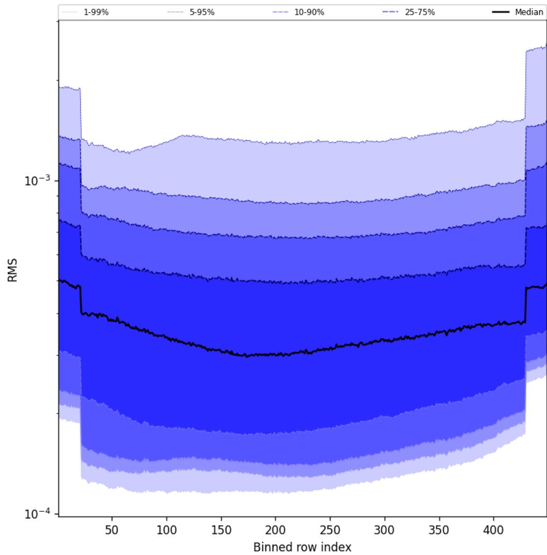
Figure 58: Along track statistics of “RMS” for 2025-11-01 to 2025-11-02
