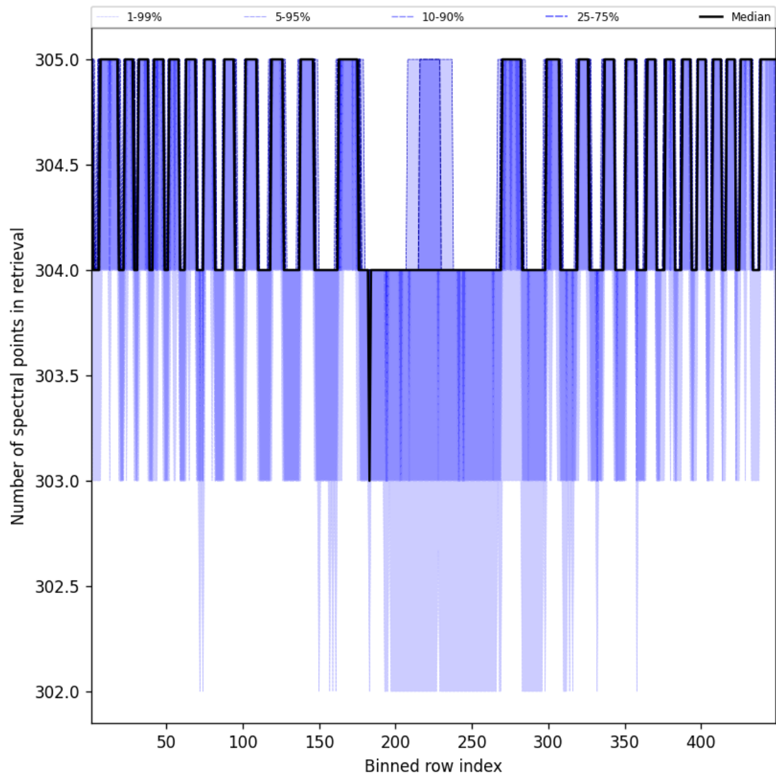
Figure 48: Along track statistics of “Number of spectral points in retrieval” for 2025-11-01 to 2025-11-02
