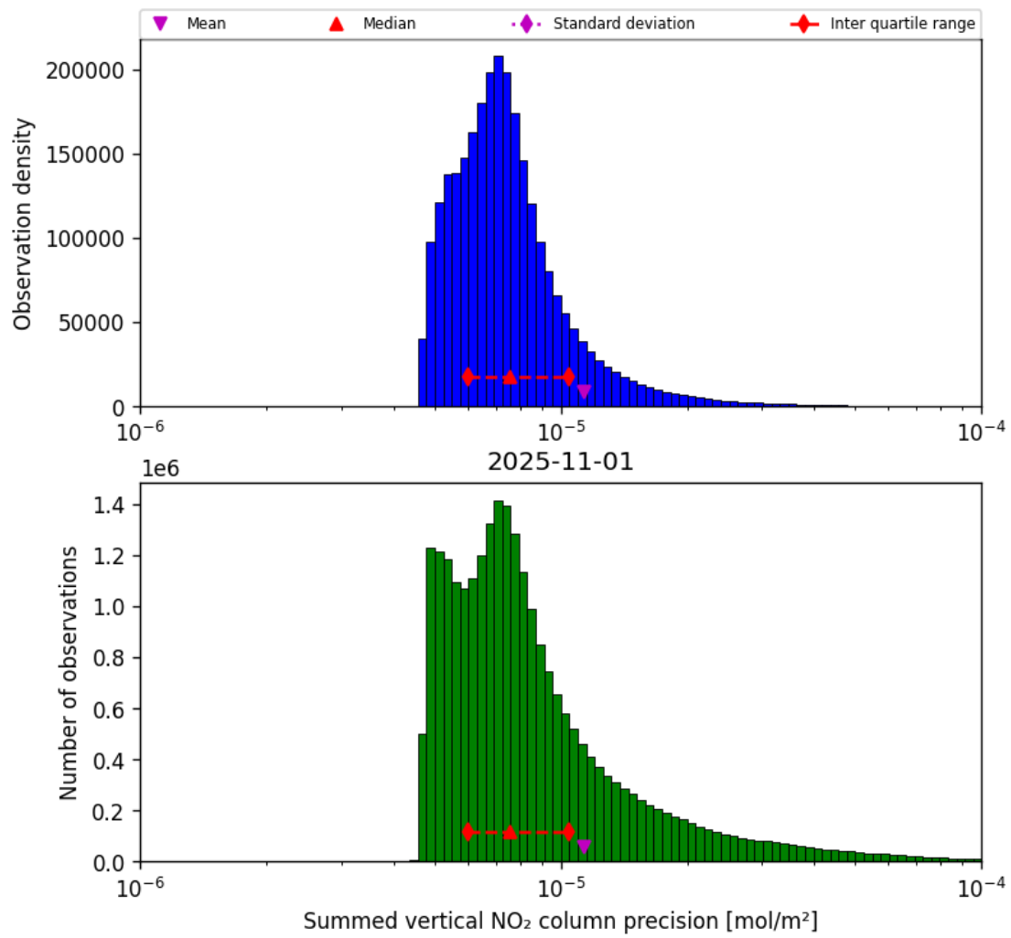
Figure 39: Histogram of "Summed vertical NO 2 column precision" for 2025-11-01 to 2025-11-02
