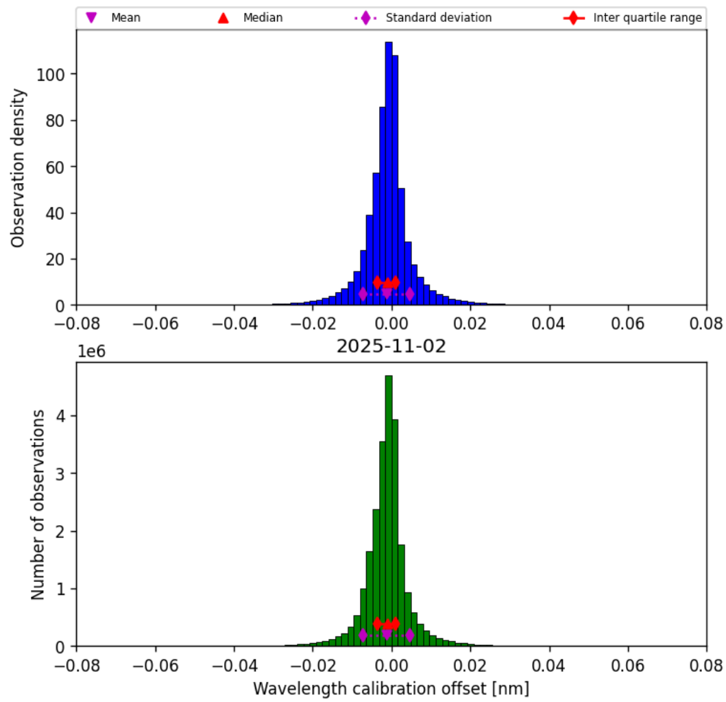
Figure 33: Histogram of “Wavelength calibration offset” for 2025-11-02 to 2025-11-03
