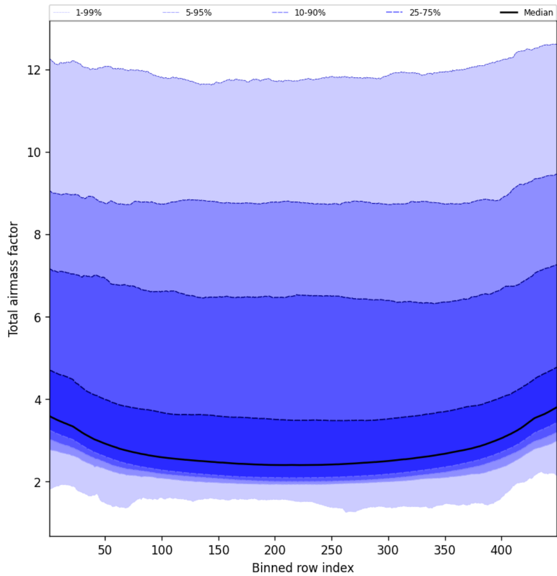
Figure 47: Along track statistics of “Total airmass factor” for 2025-11-02 to 2025-11-03
