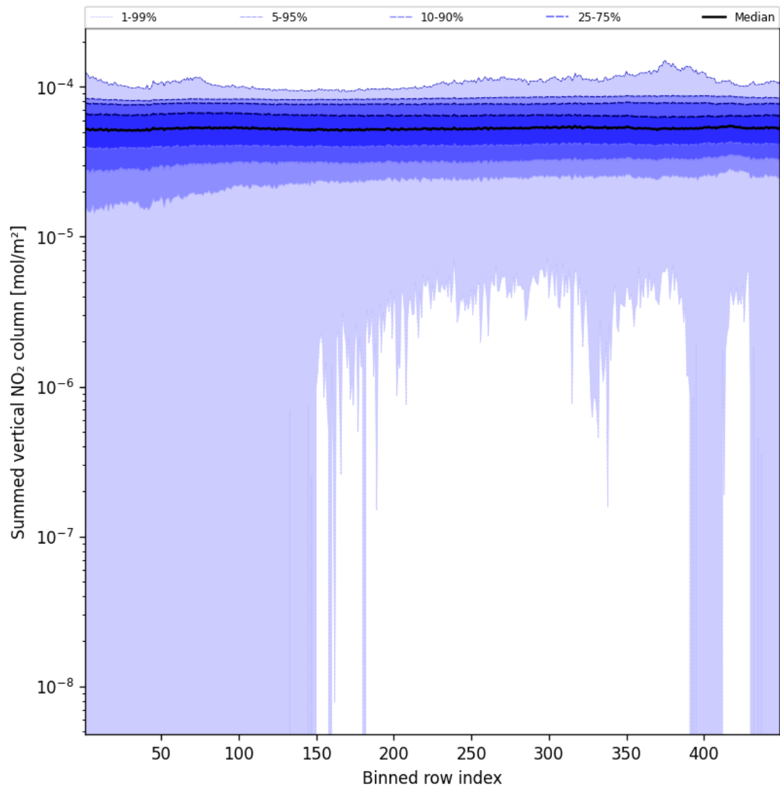
Figure 55: Along track statistics of “Summed vertical NO 2 column” for 2025-11-02 to 2025-11-03
