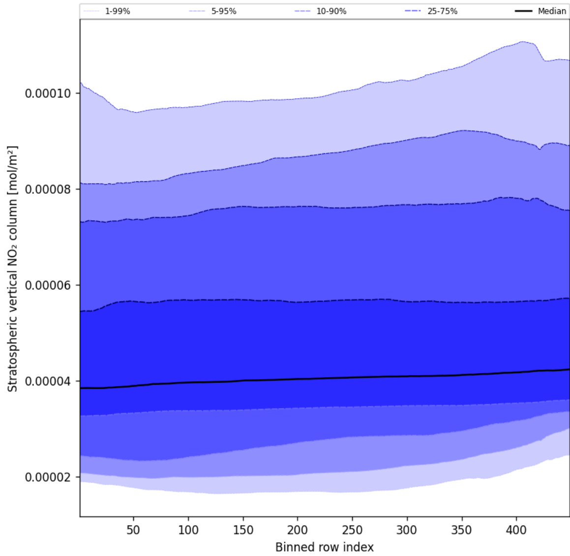
Figure 51: Along track statistics of “Stratospheric vertical NO 2 column” for 2025-11-02 to 2025-11-03
