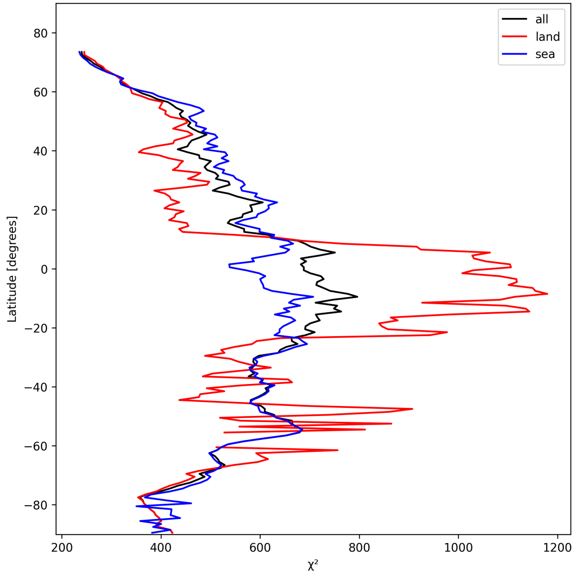
Figure 23: Zonal average of “ \chi^2 ” for 2025-11-02 to 2025-11-03.
