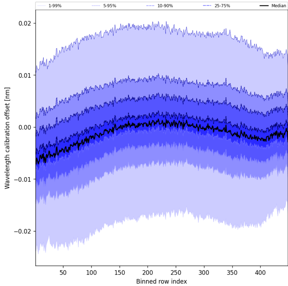
Figure 50: Along track statistics of “Wavelength calibration offset” for 2025-11-02 to 2025-11-03
