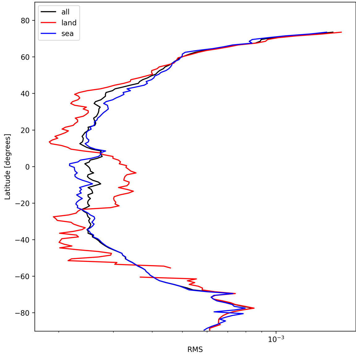
Figure 24: Zonal average of “RMS” for 2025-11-02 to 2025-11-03.
