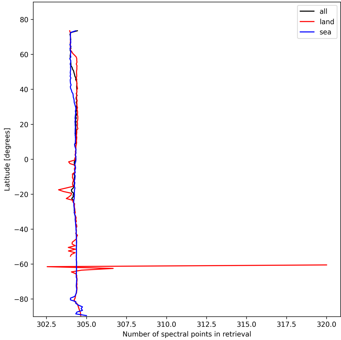
Figure 14: Zonal average of “Number of spectral points in retrieval” for 2025-11-02 to 2025-11-03.
