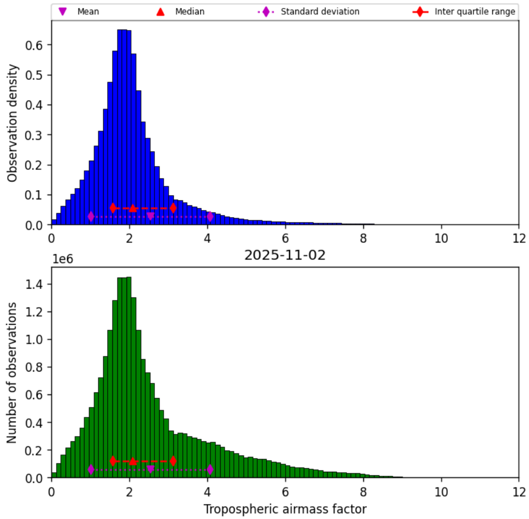
Figure 29: Histogram of “Tropospheric airmass factor” for 2025-11-02 to 2025-11-03
