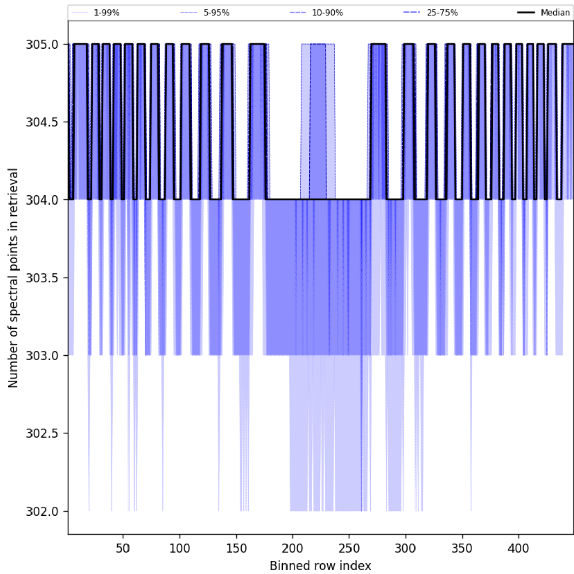
Figure 48: Along track statistics of “Number of spectral points in retrieval” for 2025-11-02 to 2025-11-03
