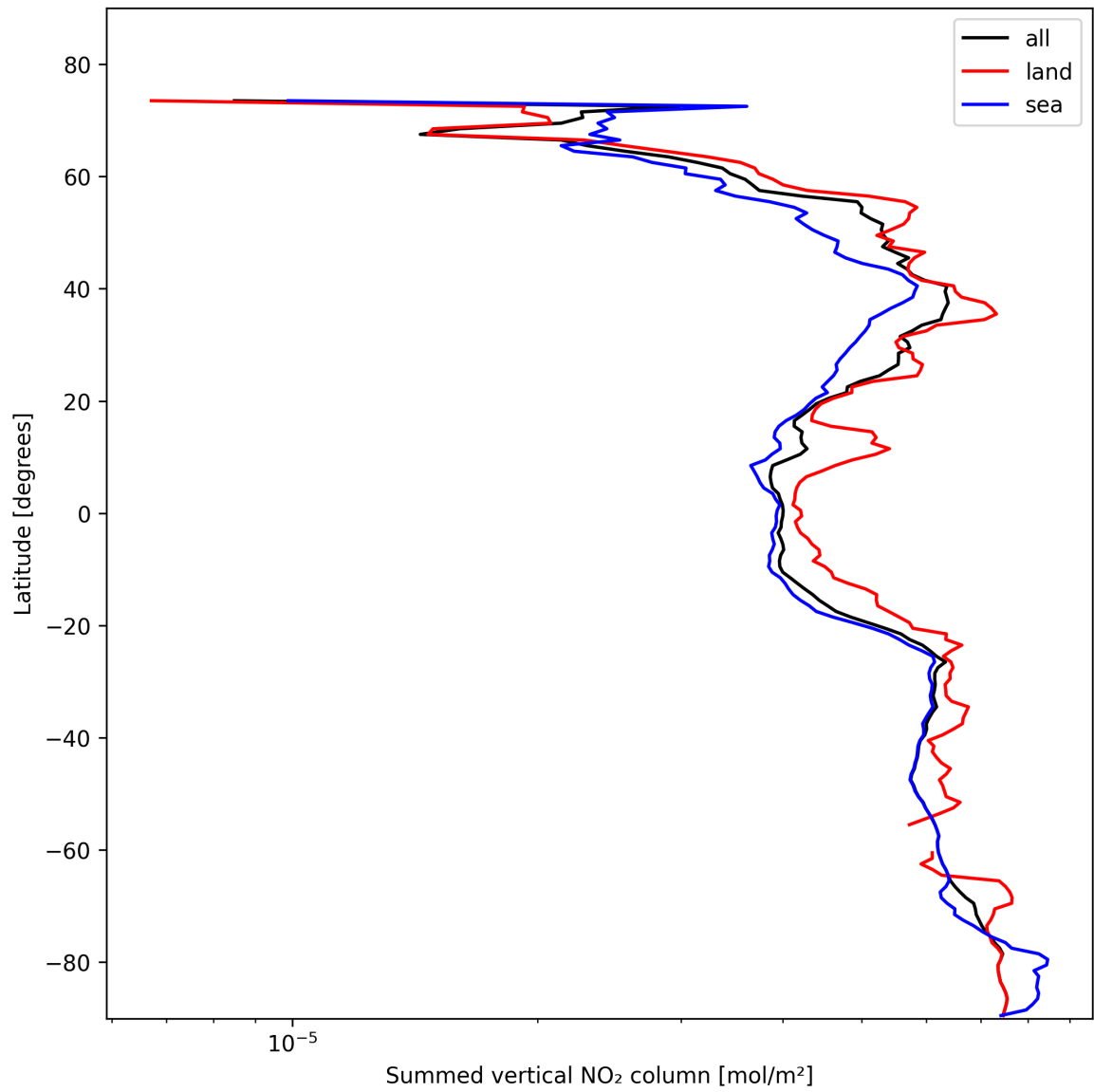
Figure 21: Zonal average of “Summed vertical NO 2 column” for 2025-11-02 to 2025-11-03.
