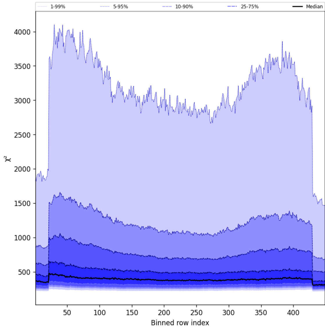
Figure 57: Along track statistics of “ \chi^2 ” for 2025-11-02 to 2025-11-03
