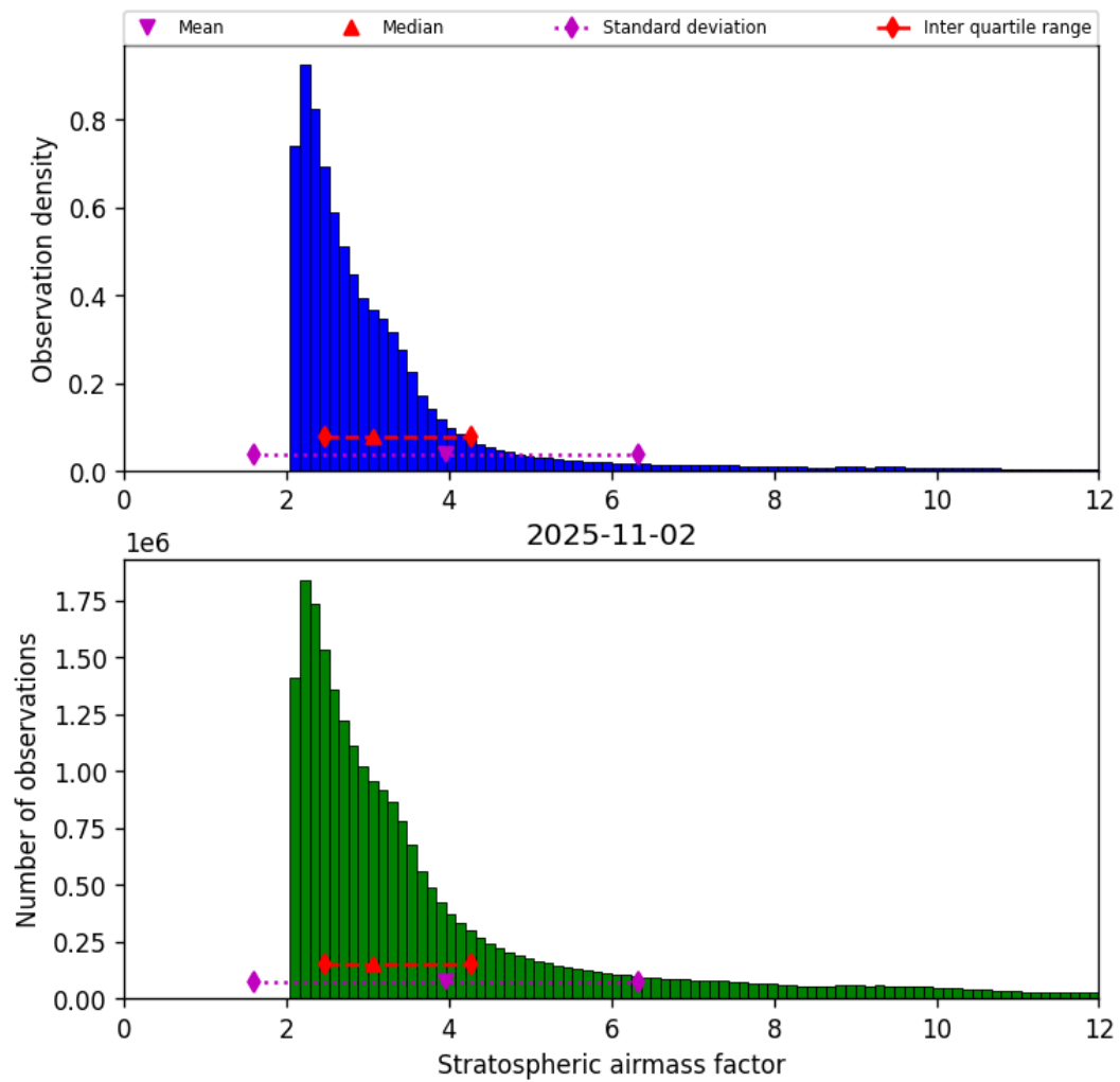
Figure 42: Histogram of “Stratospheric airmass factor” for 2025-11-02 to 2025-11-03
