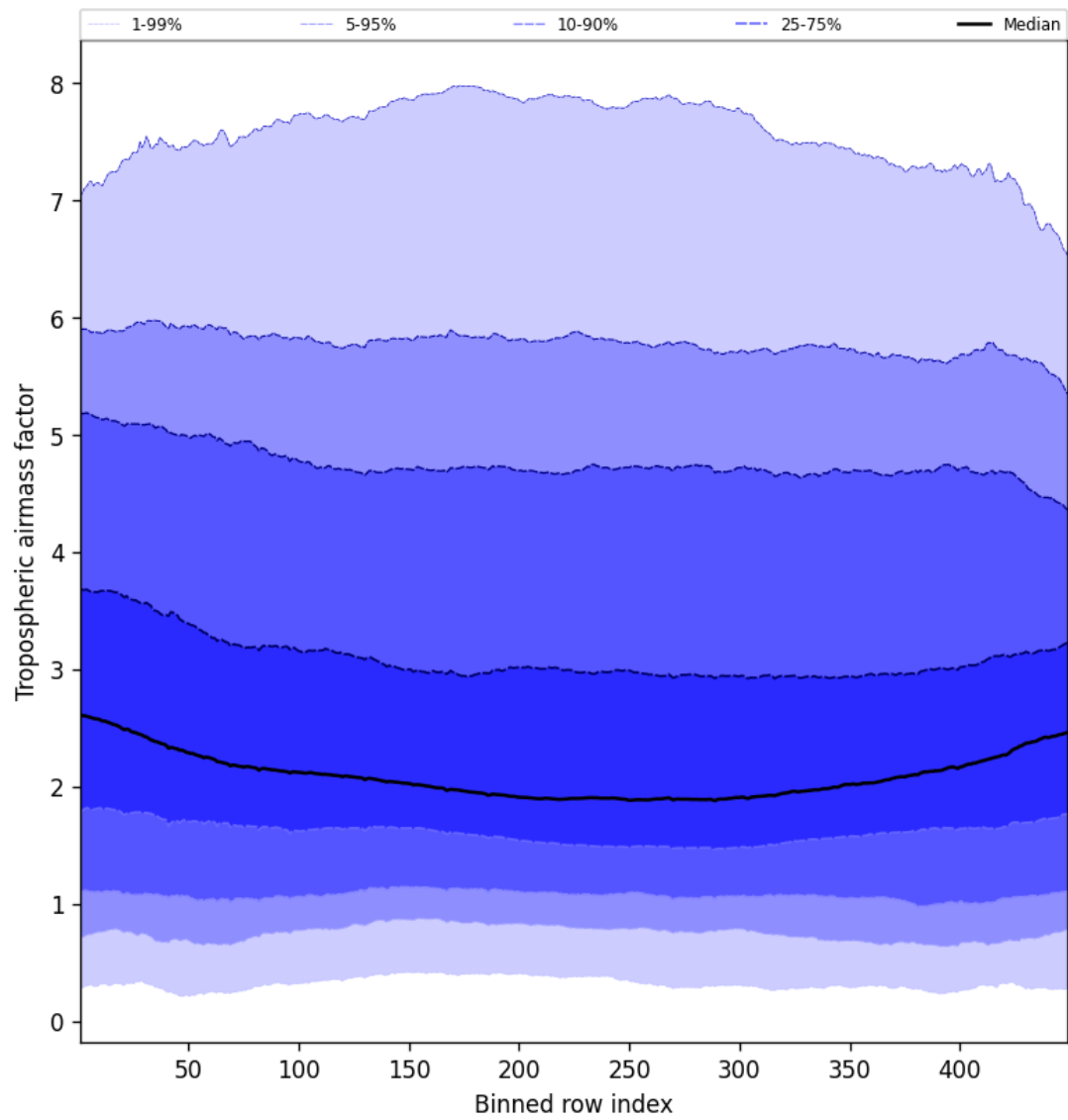
Figure 46: Along track statistics of “Tropospheric airmass factor” for 2025-11-02 to 2025-11-03
