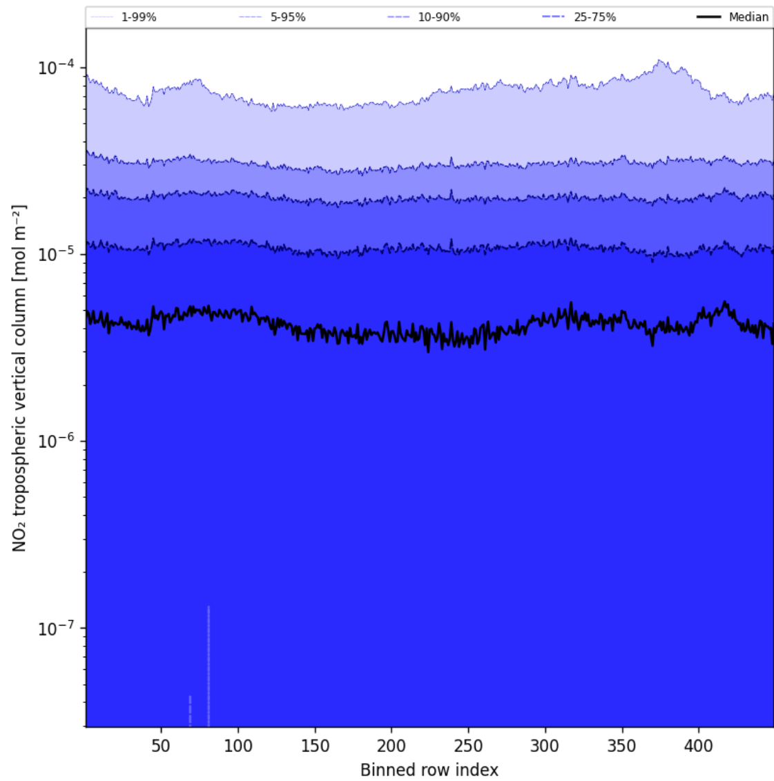
Figure 44: Along track statistics of “NO 2 tropospheric vertical column” for 2025-11-02 to 2025-11-03
