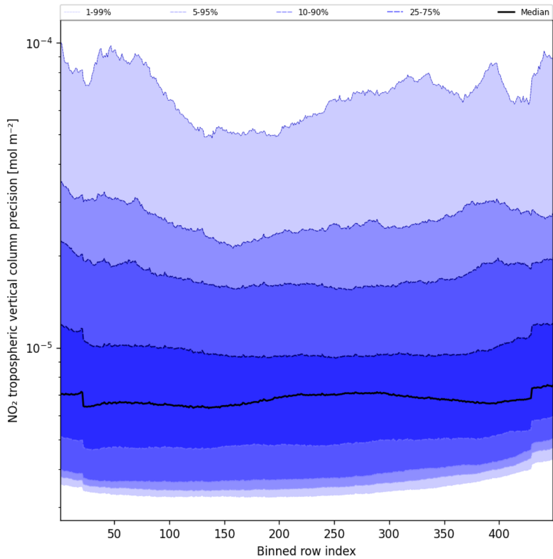
Figure 45: Along track statistics of “NO 2 tropospheric vertical column precision” for 2025-11-02 to 2025-11-03
