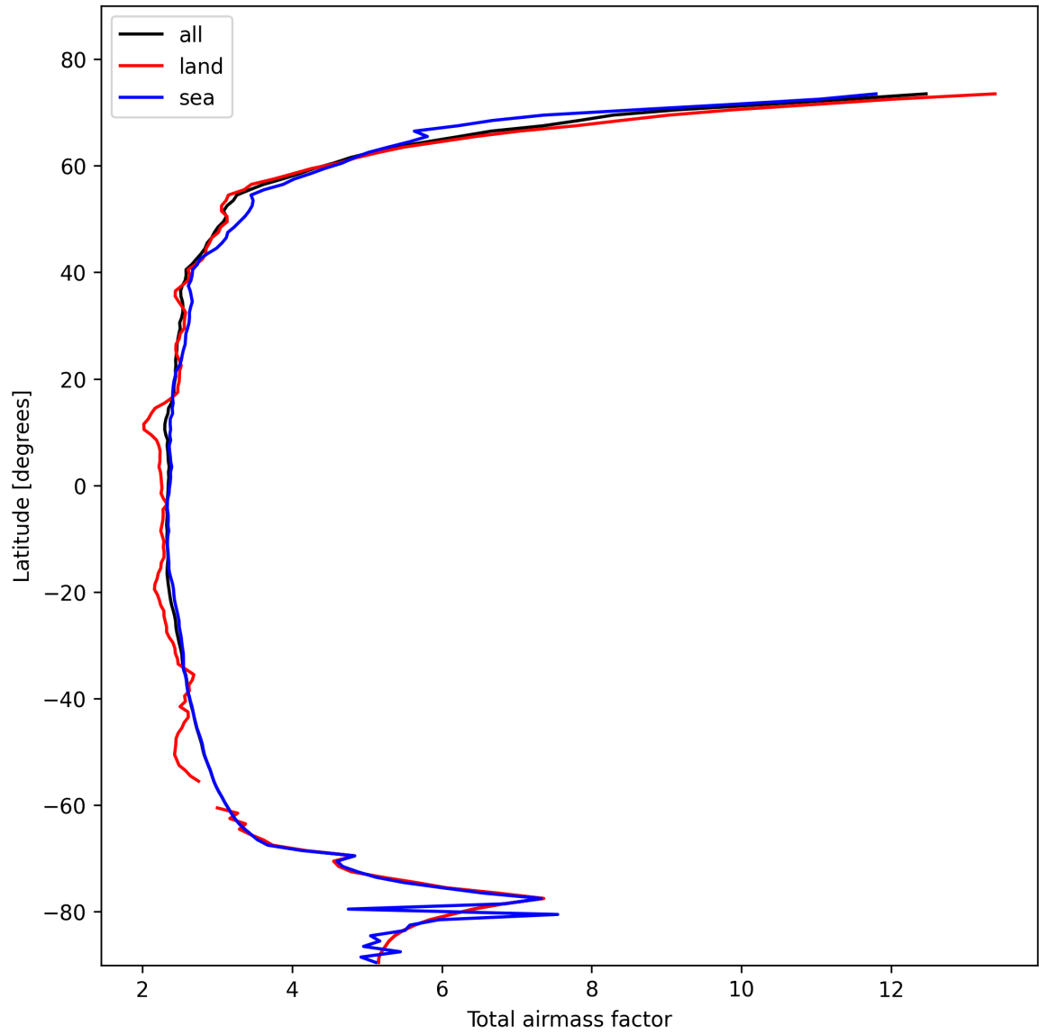
Figure 13: Zonal average of “Total airmass factor” for 2025-11-02 to 2025-11-03.
