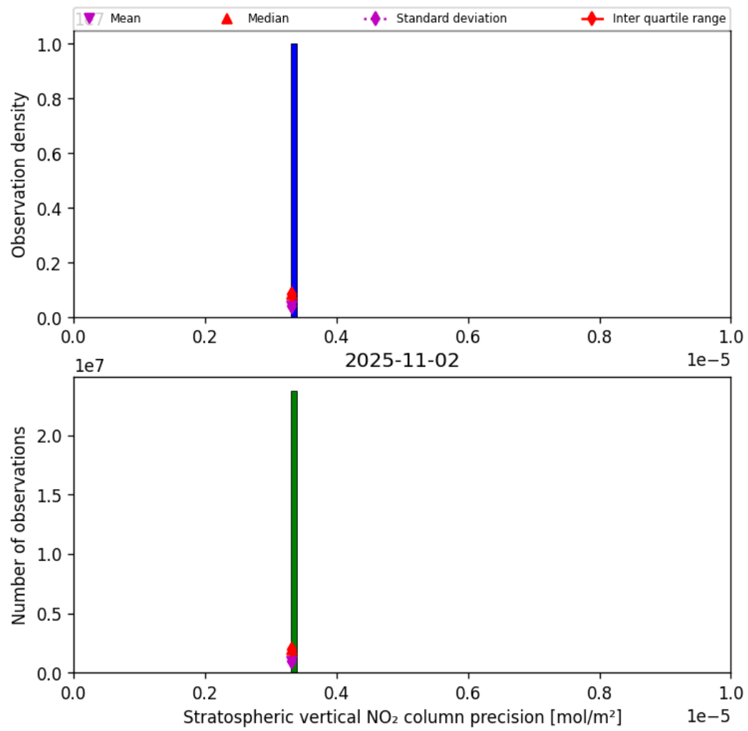
Figure 35: Histogram of “Stratospheric vertical NO 2 column precision” for 2025-11-02 to 2025-11-03
