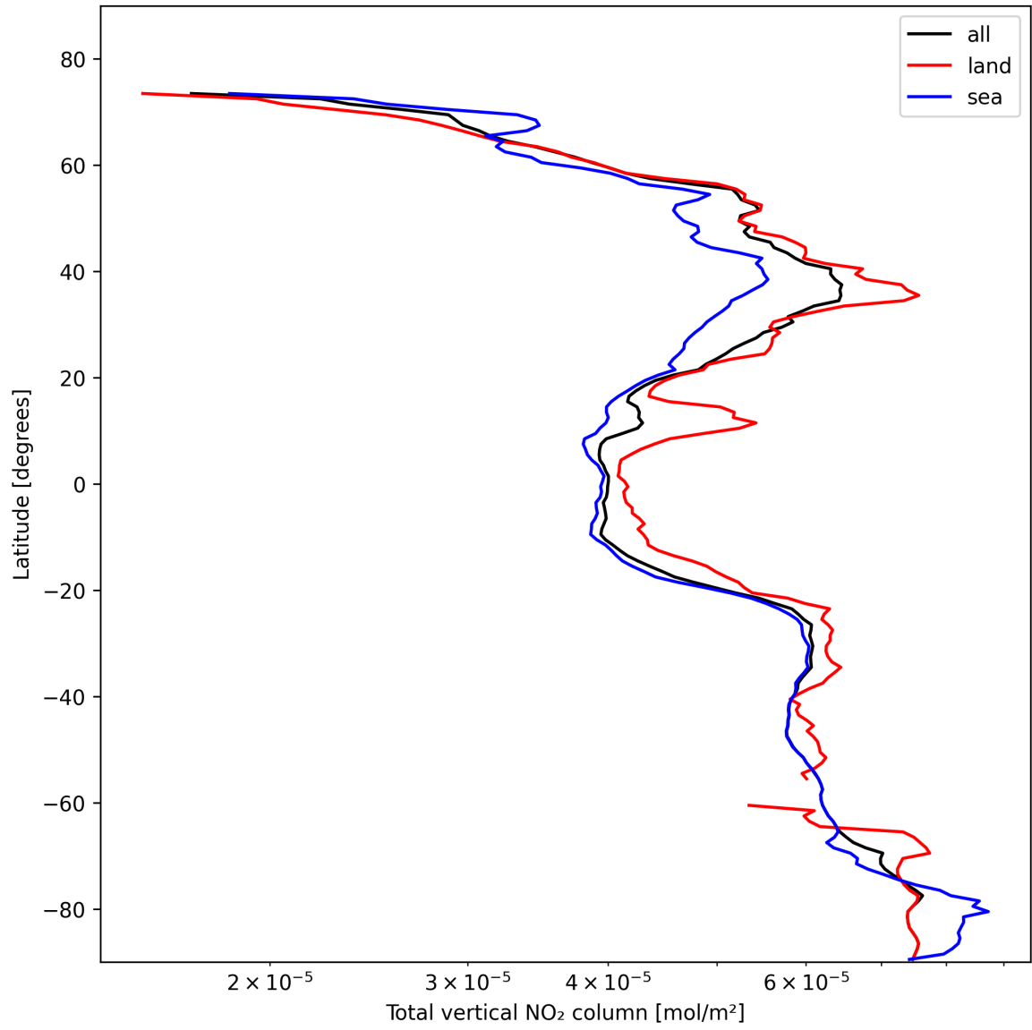
Figure 19: Zonal average of “Total vertical NO 2 column” for 2025-11-02 to 2025-11-03.
