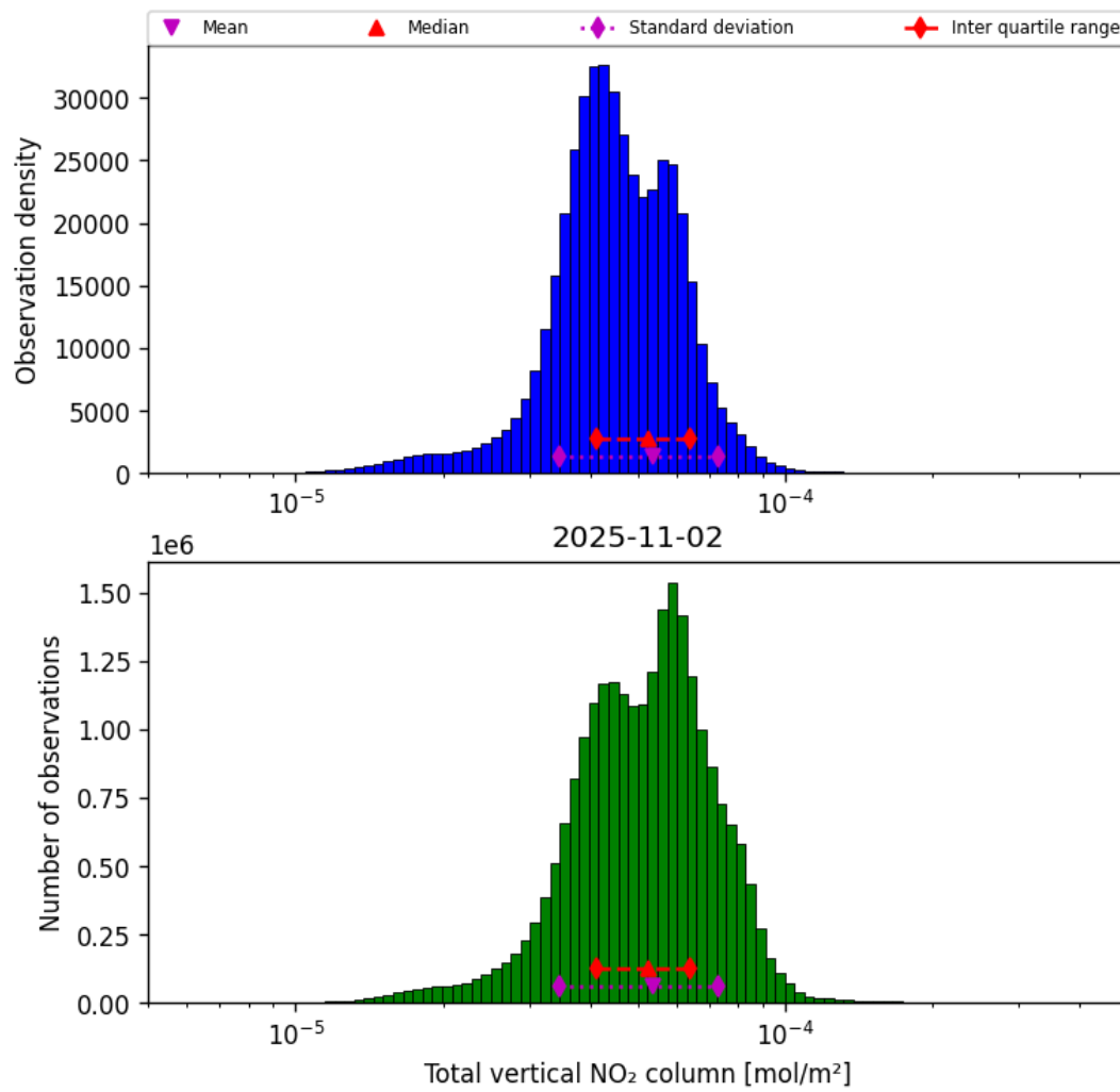
Figure 36: Histogram of “Total vertical NO 2 column” for 2025-11-02 to 2025-11-03
