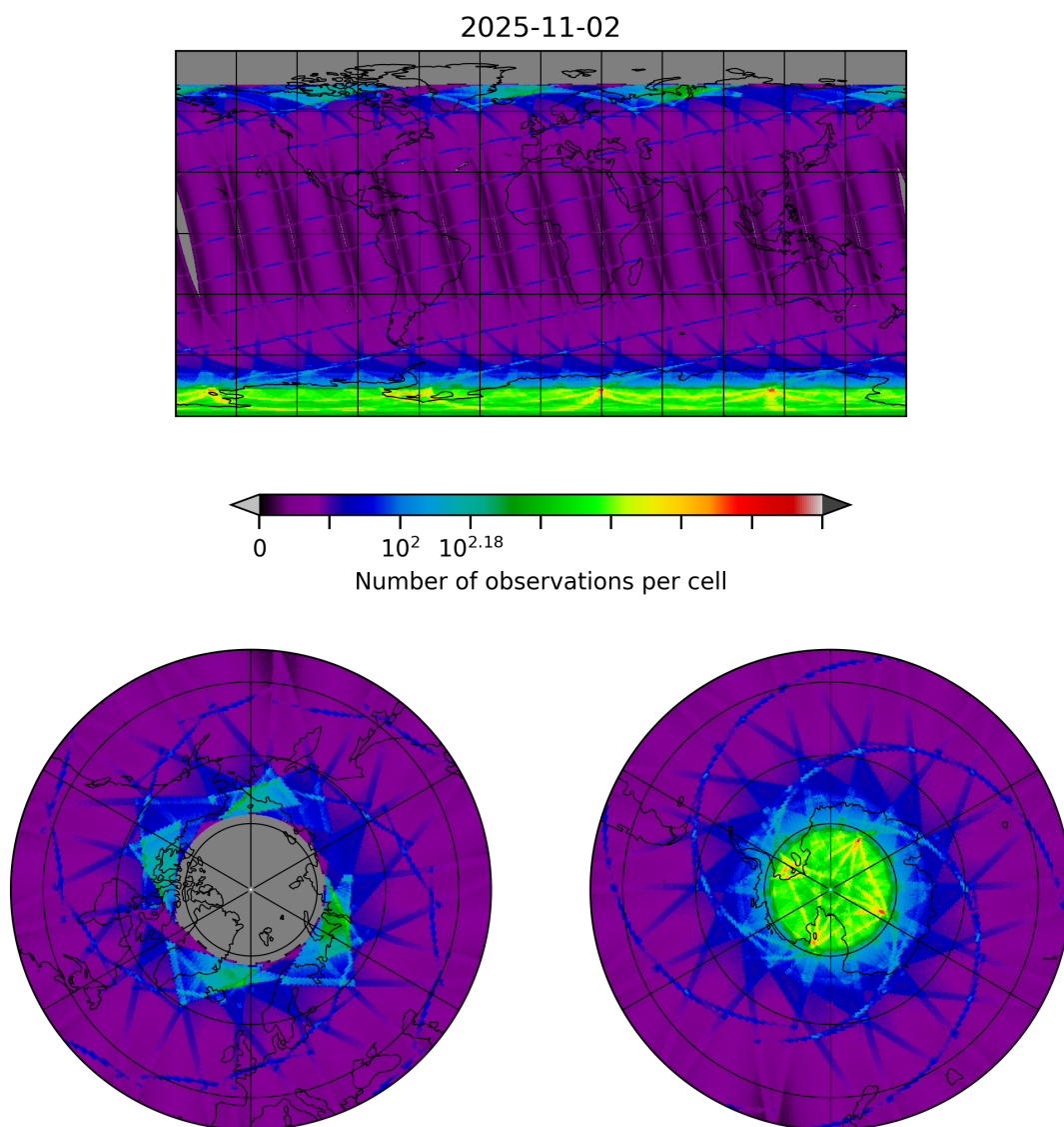
Figure 8: Map of the number of observations for 2025-11-02 to 2025-11-03
