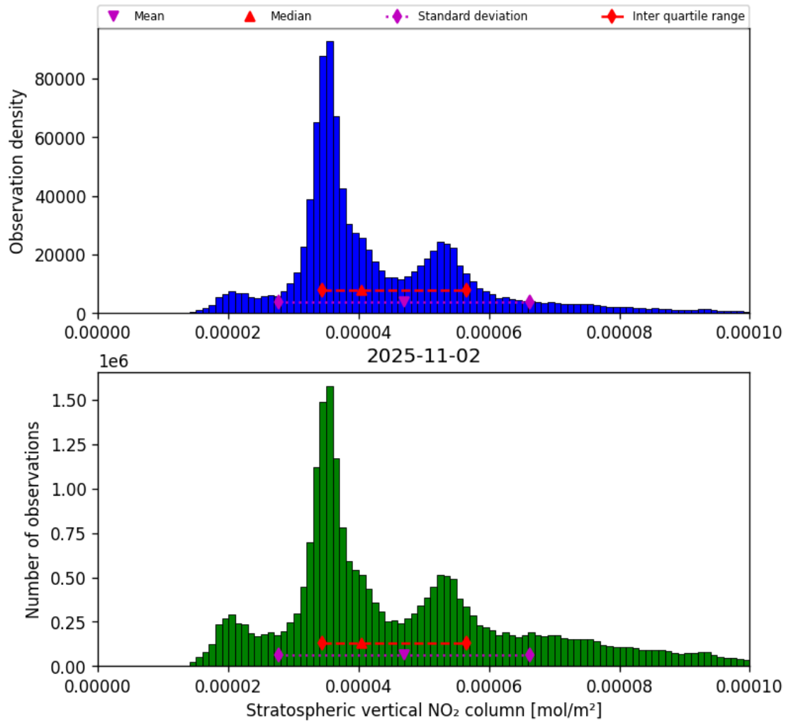
Figure 34: Histogram of “Stratospheric vertical NO 2 column” for 2025-11-02 to 2025-11-03
