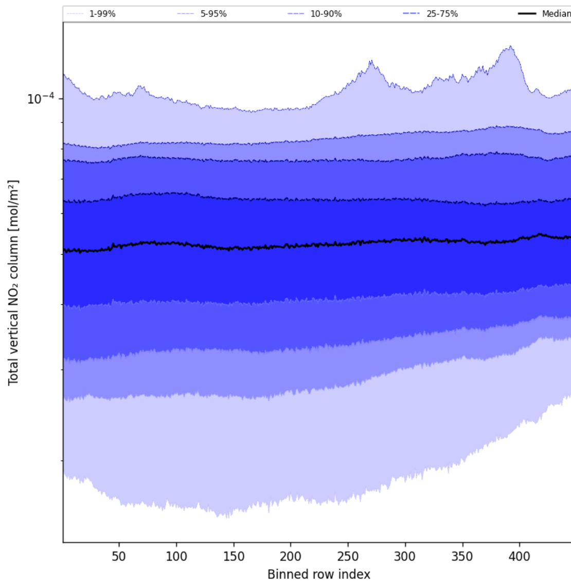
Figure 53: Along track statistics of “Total vertical NO 2 column” for 2025-11-02 to 2025-11-03
