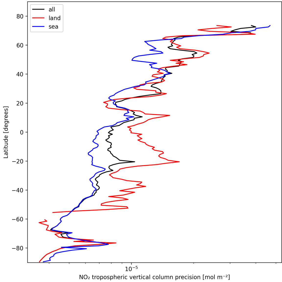
Figure 11: Zonal average of “NO 2 tropospheric vertical column precision” for 2025-11-02 to 2025-11-03.
