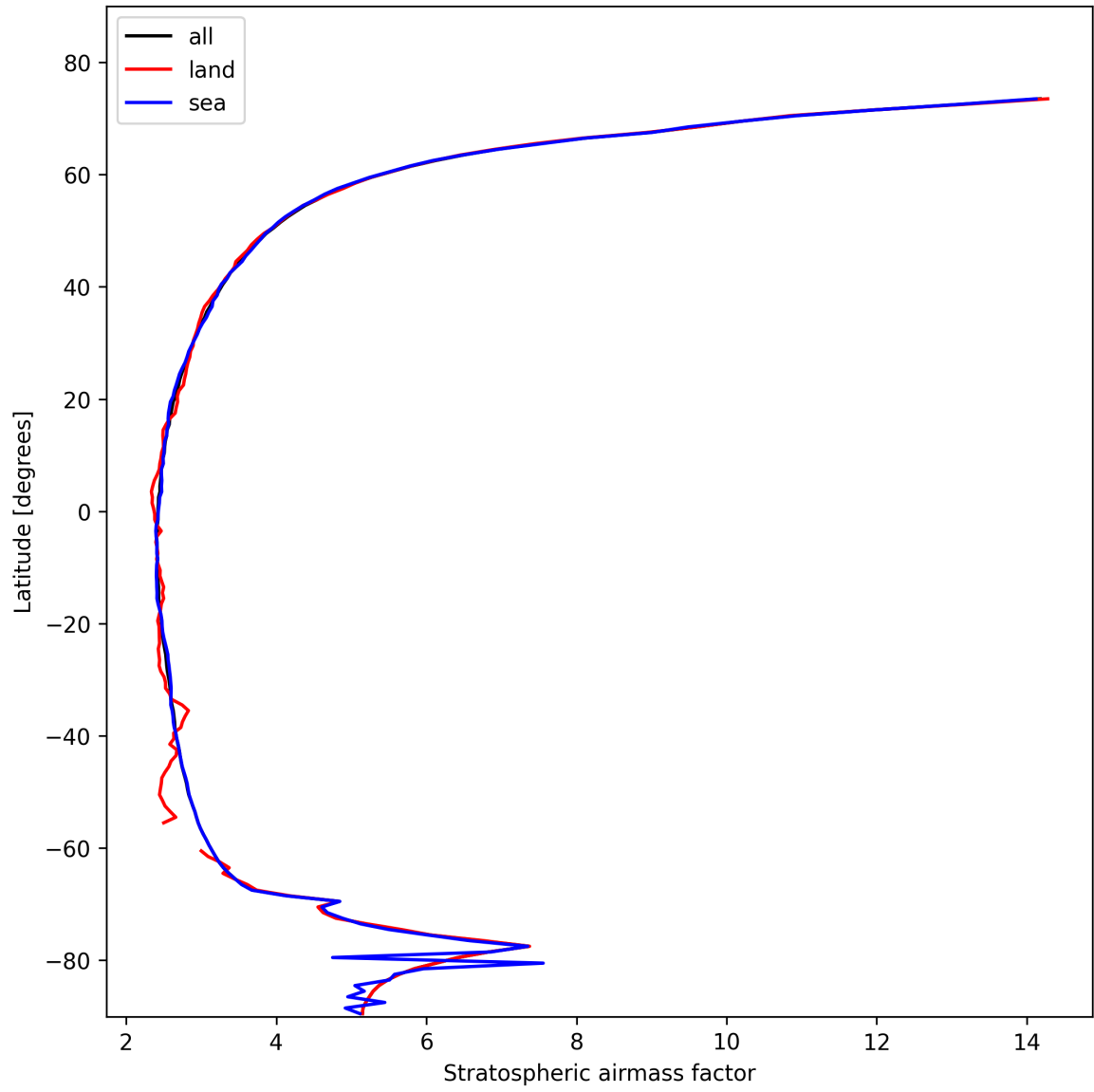
Figure 25: Zonal average of “Stratospheric airmass factor” for 2025-11-02 to 2025-11-03.
