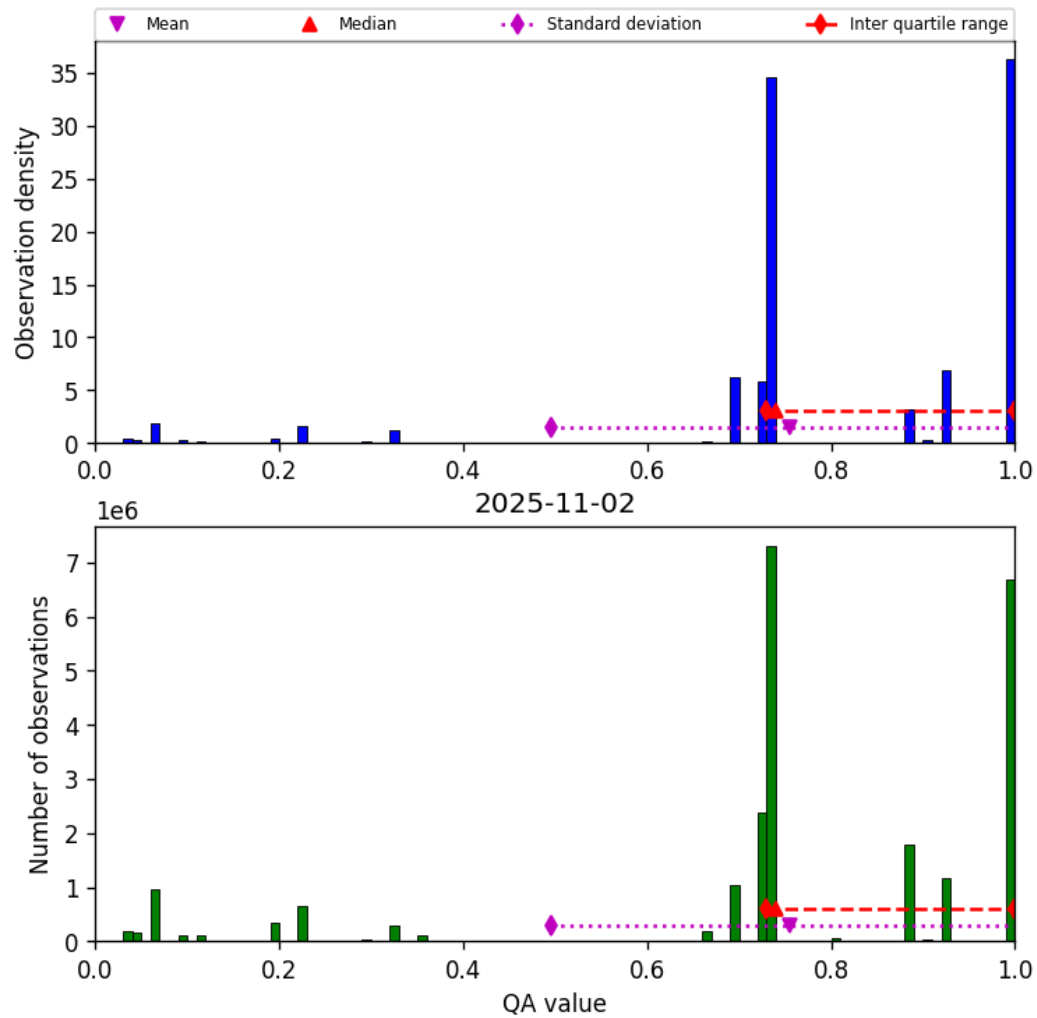
Figure 26: Histogram of “QA value” for 2025-11-02 to 2025-11-03
