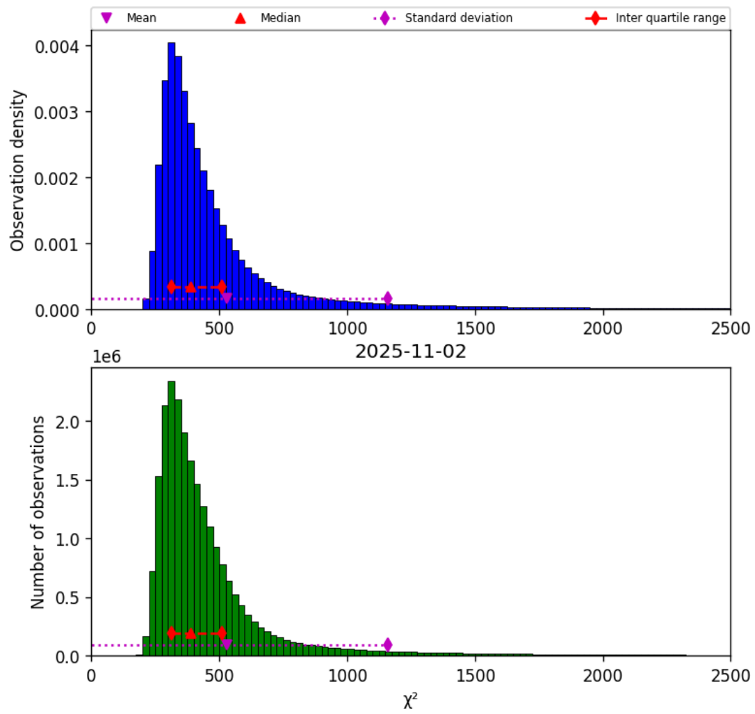
Figure 40: Histogram of “ \chi^2 ” for 2025-11-02 to 2025-11-03
