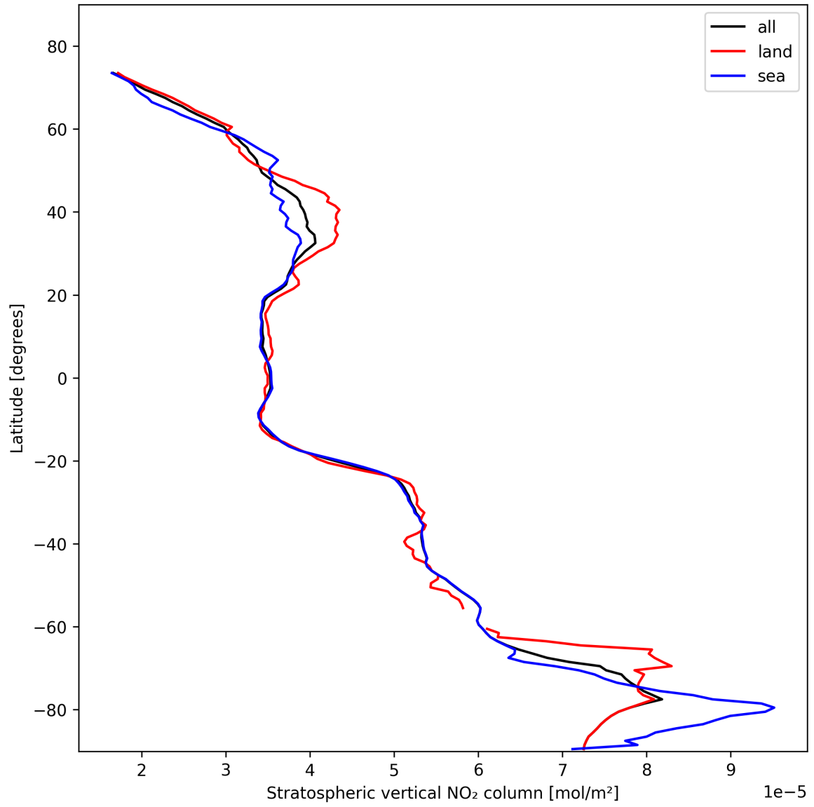
Figure 17: Zonal average of “Stratospheric vertical NO 2 column” for 2025-11-02 to 2025-11-03.
