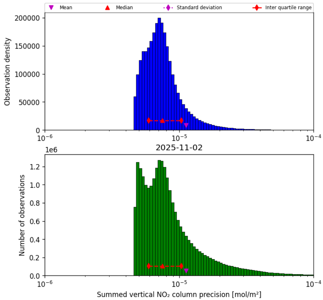
Figure 39: Histogram of “Summed vertical NO 2 column precision” for 2025-11-02 to 2025-11-03
