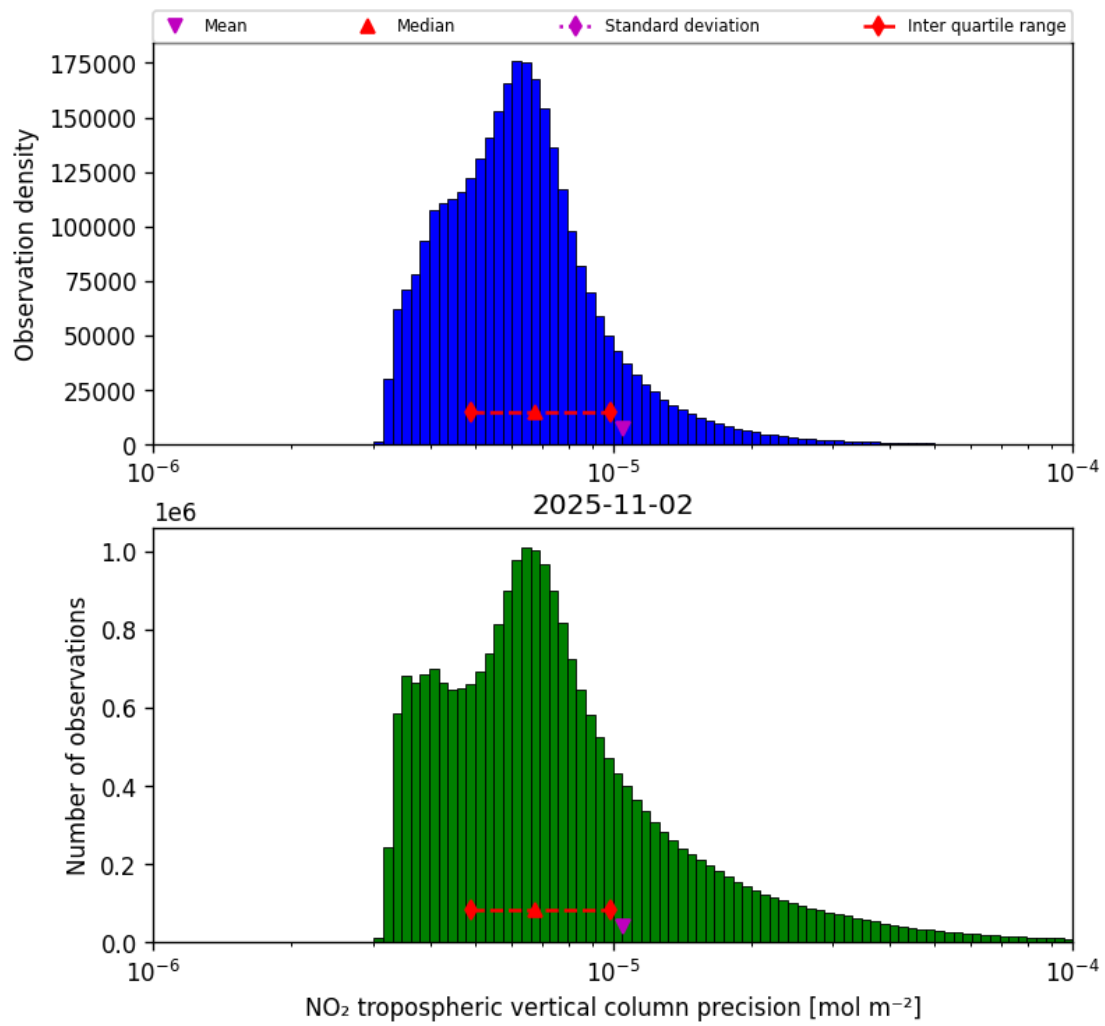
Figure 28: Histogram of “NO 2 tropospheric vertical column precision” for 2025-11-02 to 2025-11-03
