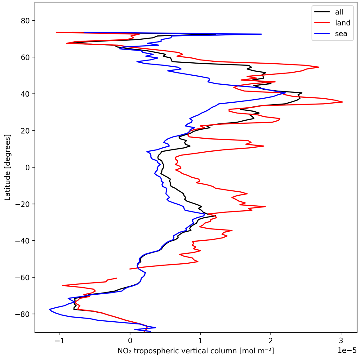
Figure 10: Zonal average of “NO 2 tropospheric vertical column” for 2025-11-02 to 2025-11-03.
