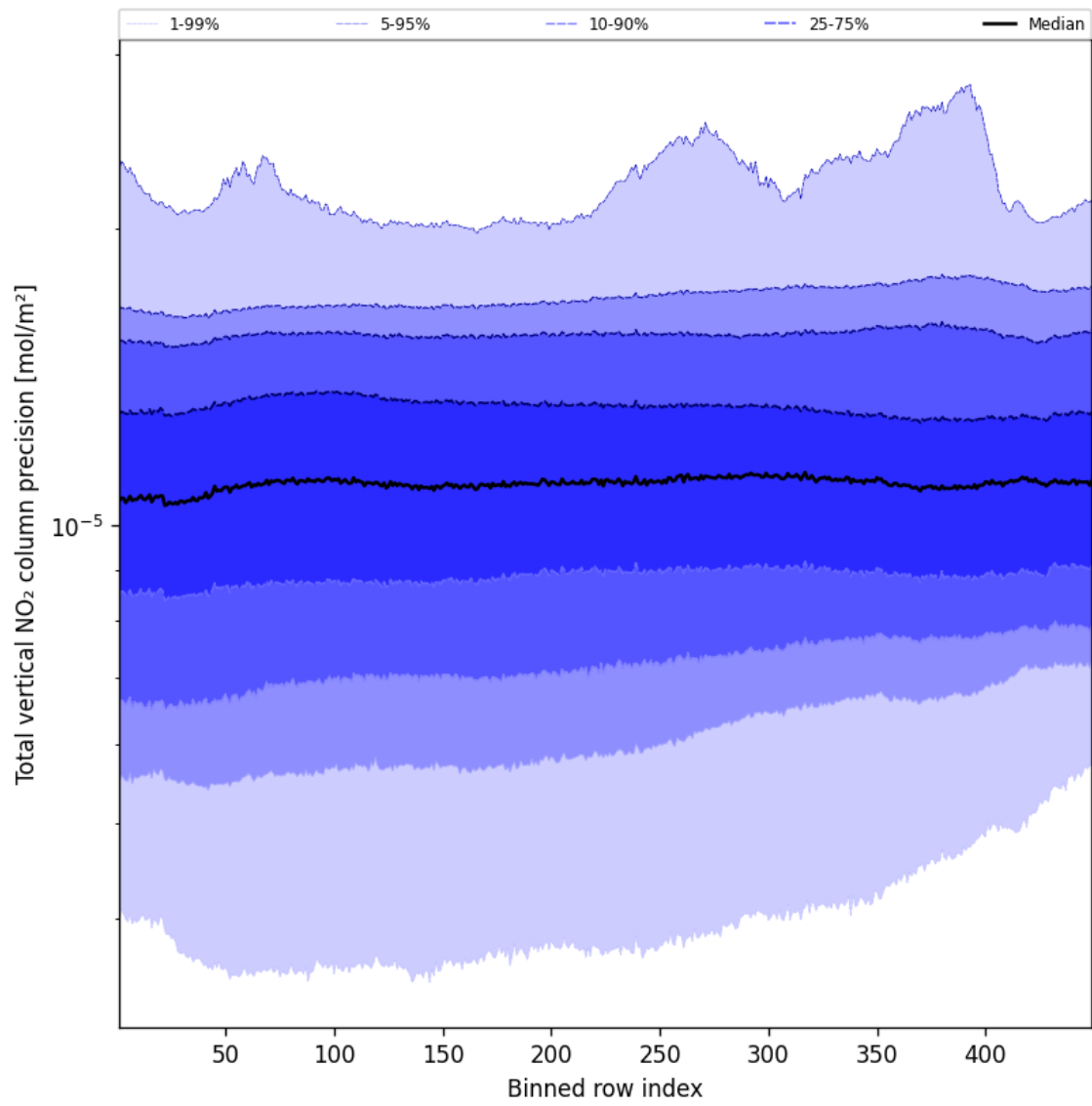
Figure 54: Along track statistics of “Total vertical NO 2 column precision” for 2025-11-02 to 2025-11-03
