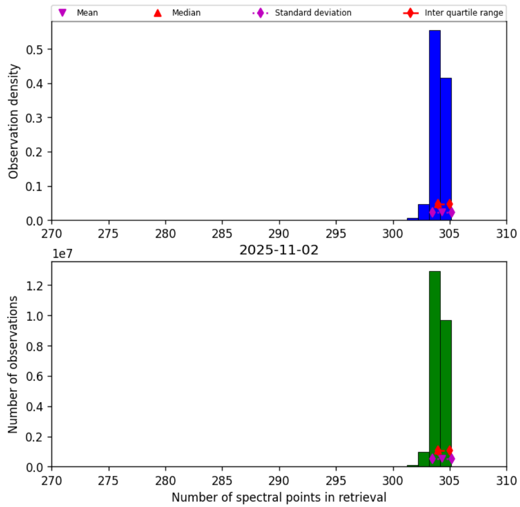
Figure 31: Histogram of “Number of spectral points in retrieval” for 2025-11-02 to 2025-11-03
