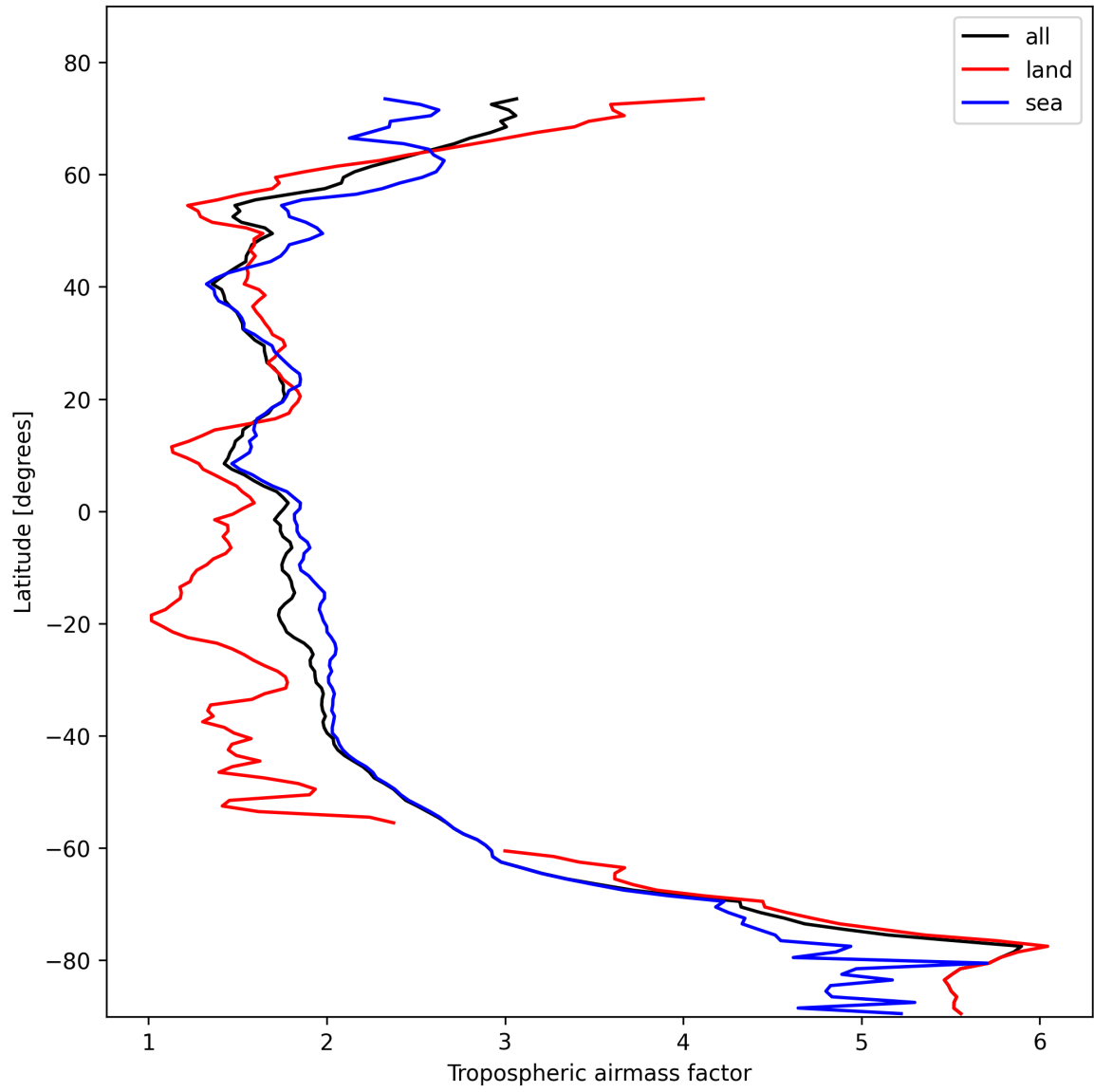
Figure 12: Zonal average of “Tropospheric airmass factor” for 2025-11-02 to 2025-11-03.
