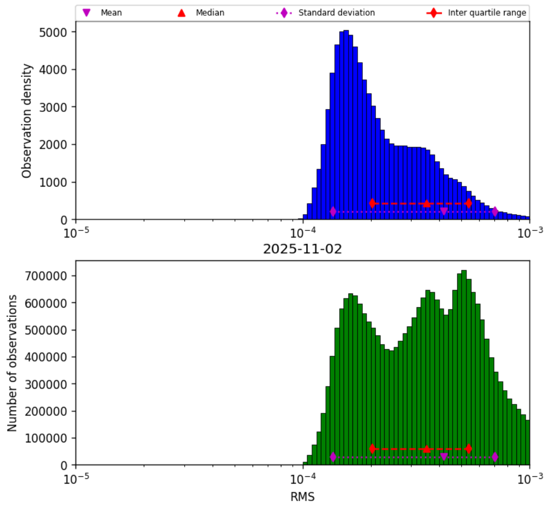
Figure 41: Histogram of “RMS” for 2025-11-02 to 2025-11-03
