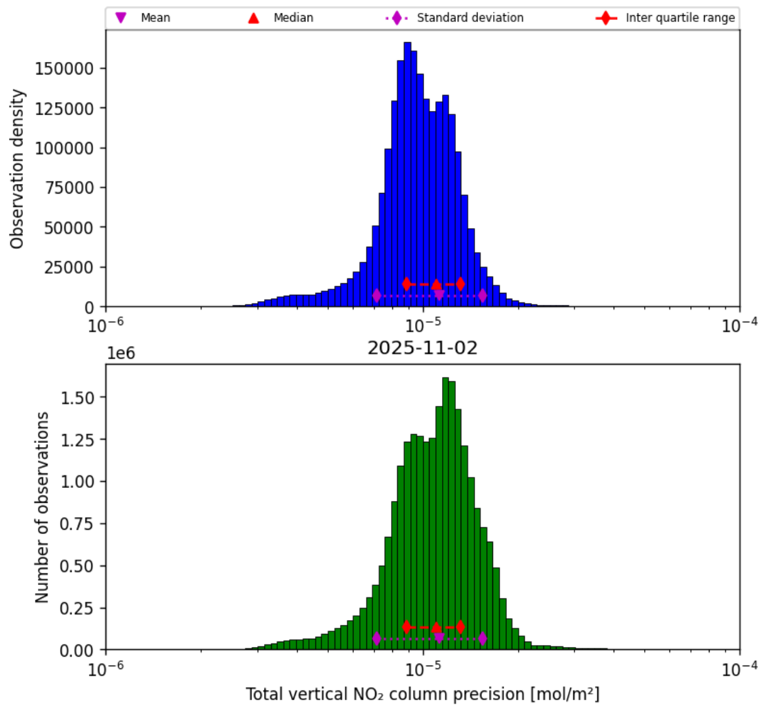
Figure 37: Histogram of “Total vertical NO 2 column precision” for 2025-11-02 to 2025-11-03
