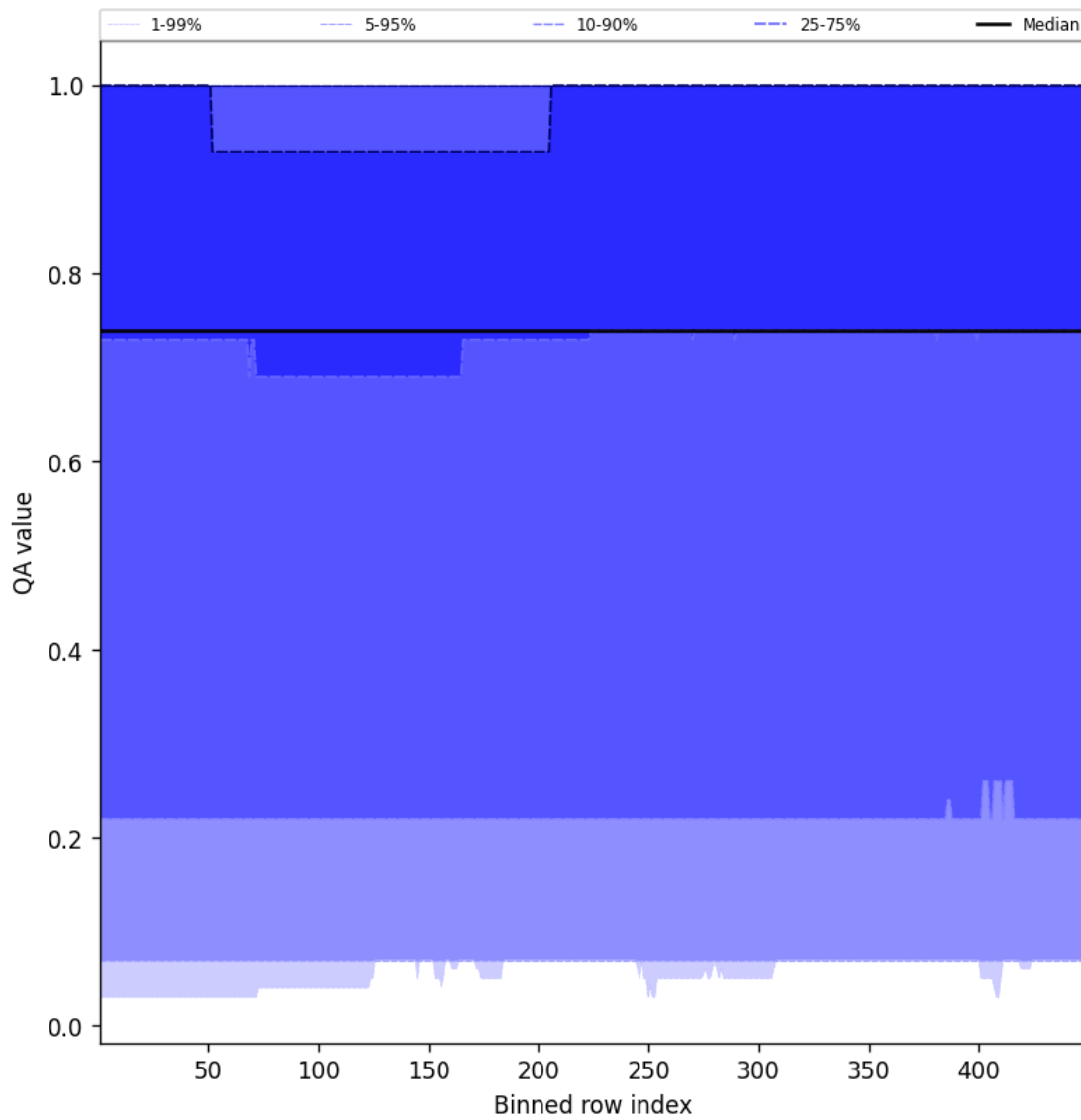
Figure 43: Along track statistics of “QA value” for 2025-11-02 to 2025-11-03
