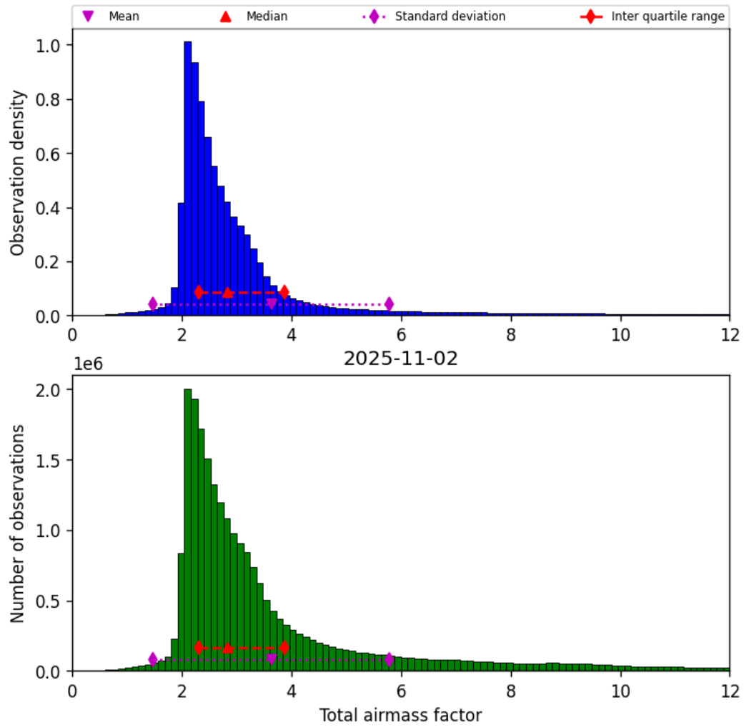
Figure 30: Histogram of “Total airmass factor” for 2025-11-02 to 2025-11-03
