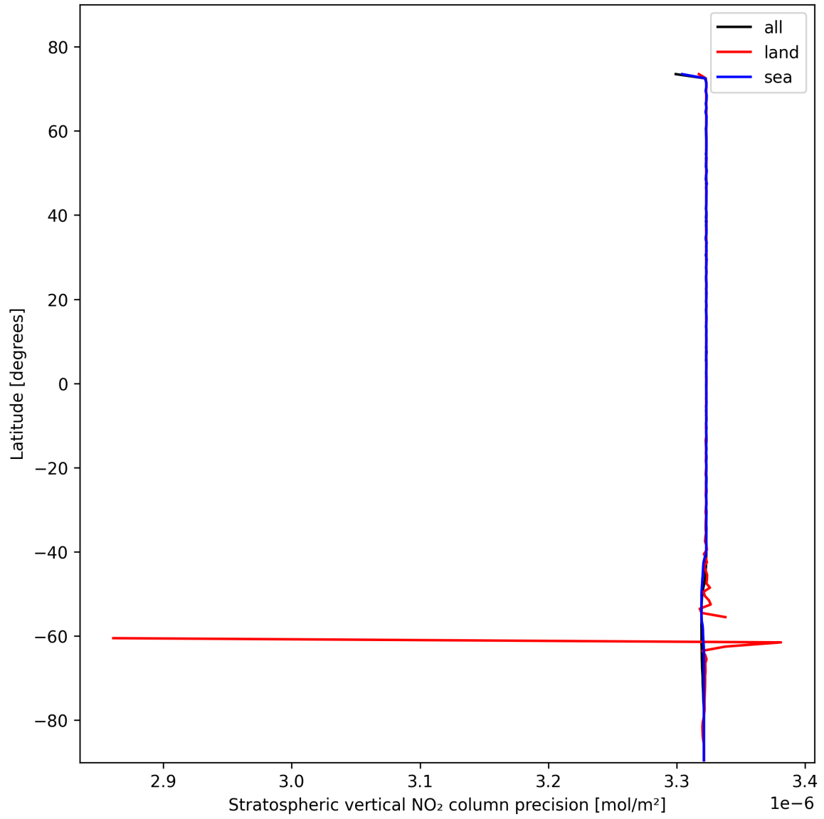
Figure 18: Zonal average of "Stratospheric vertical NO 2 column precision" for 2025-11-02 to 2025-11-03.
