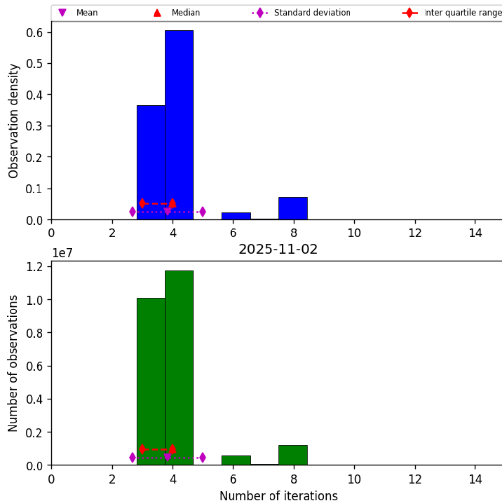
Figure 32: Histogram of “Number of iterations” for 2025-11-02 to 2025-11-03
