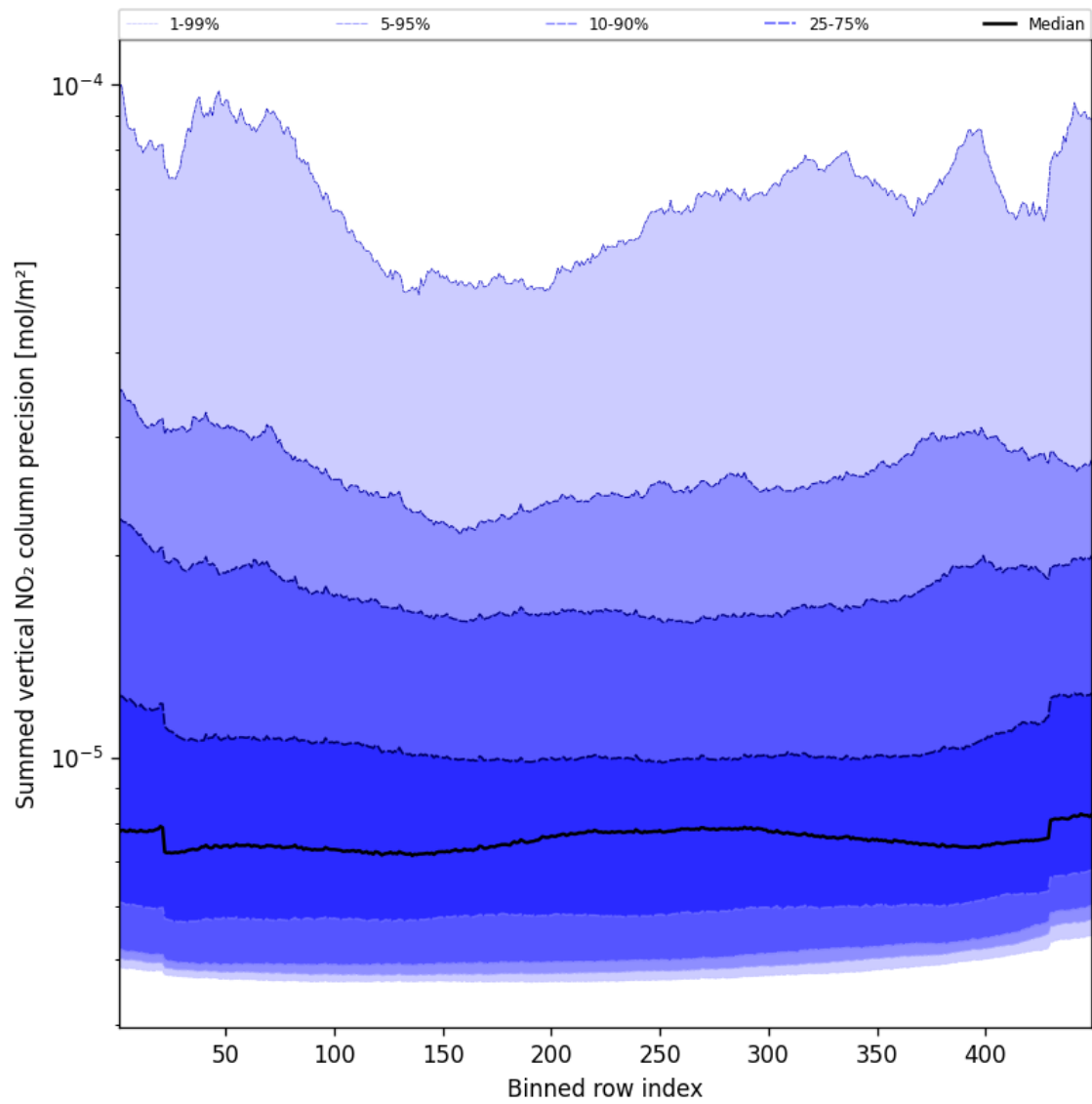
Figure 56: Along track statistics of “Summed vertical NO 2 column precision” for 2025-11-02 to 2025-11-03
