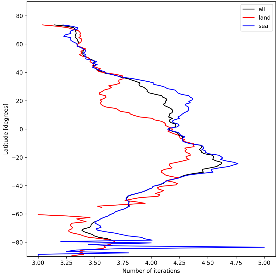
Figure 15: Zonal average of “Number of iterations” for 2025-11-02 to 2025-11-03.
