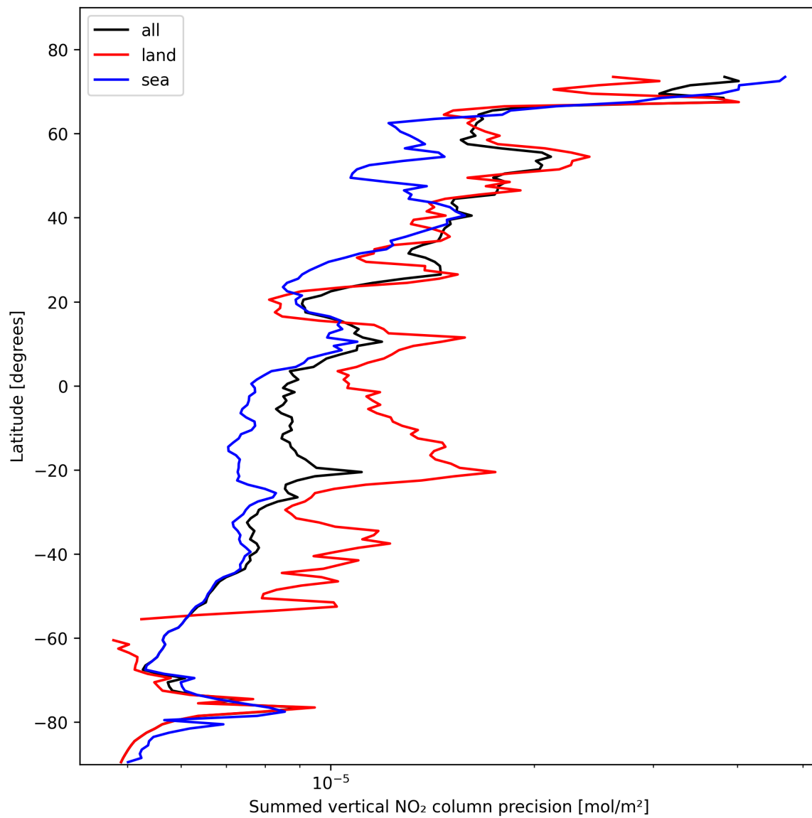
Figure 22: Zonal average of “Summed vertical NO 2 column precision” for 2025-11-02 to 2025-11-03.
