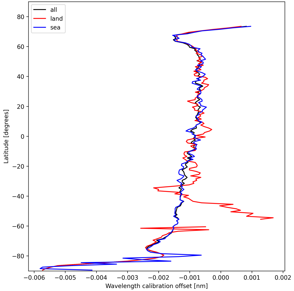
Figure 16: Zonal average of “Wavelength calibration offset” for 2025-11-02 to 2025-11-03.
