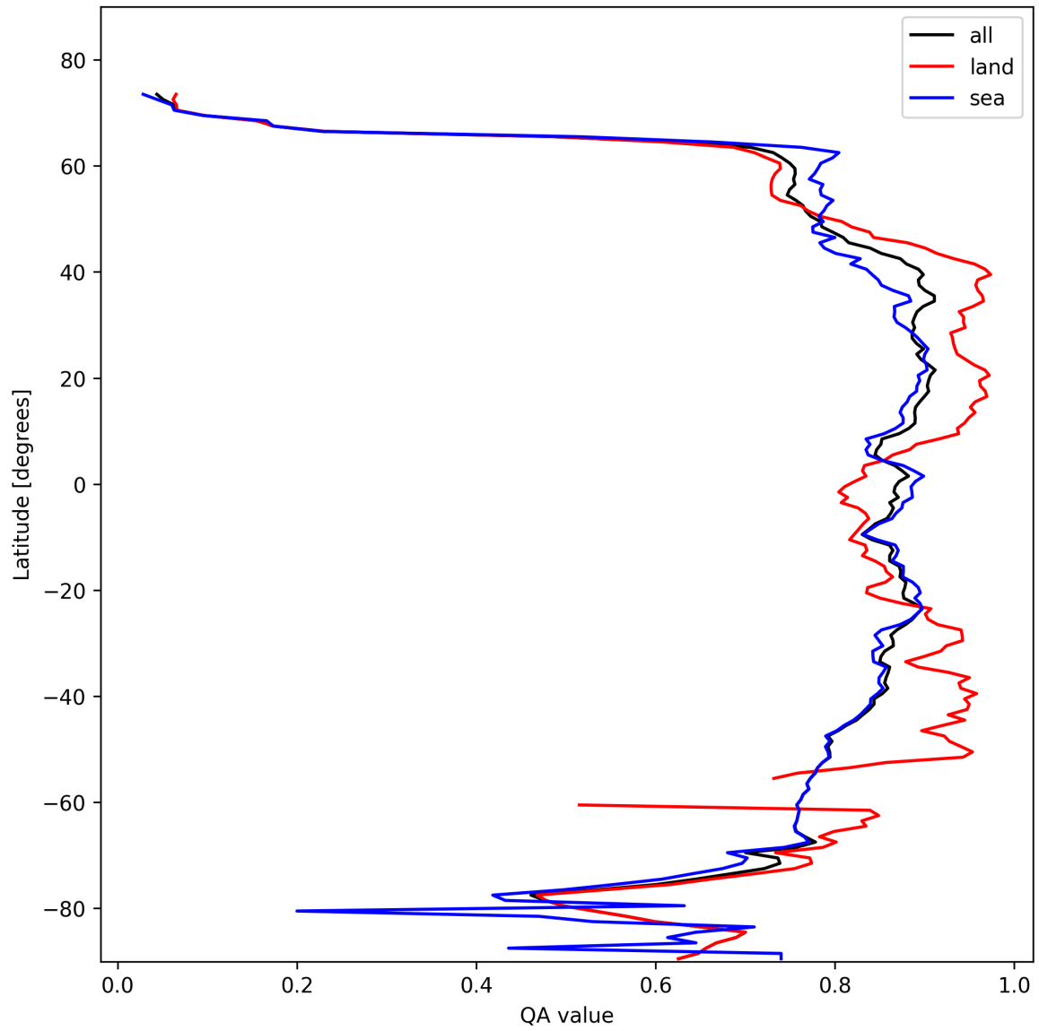
Figure 9: Zonal average of “QA value” for 2025-11-02 to 2025-11-03.
