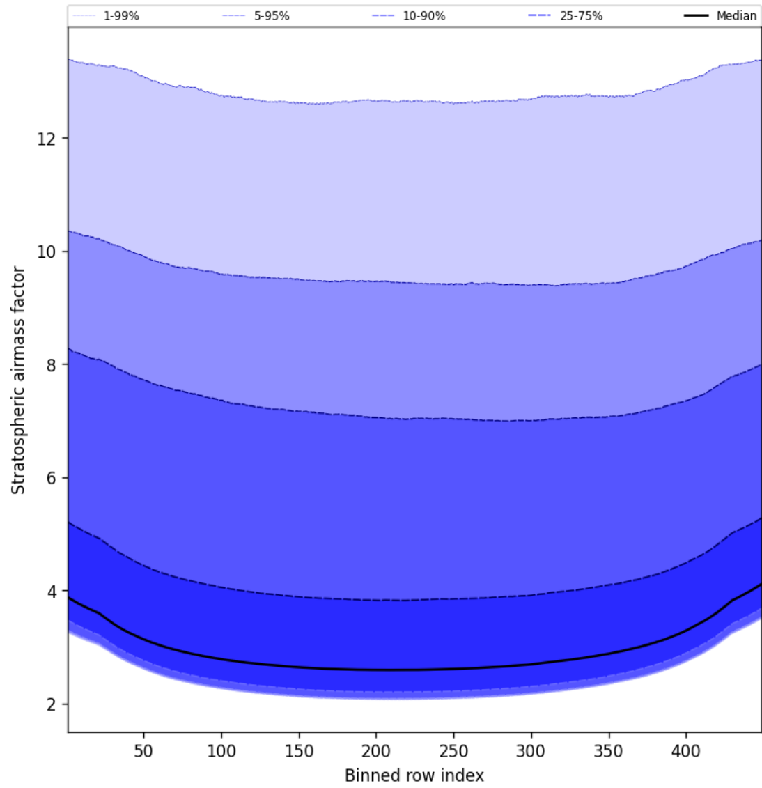
Figure 59: Along track statistics of “Stratospheric airmass factor” for 2025-11-02 to 2025-11-03
