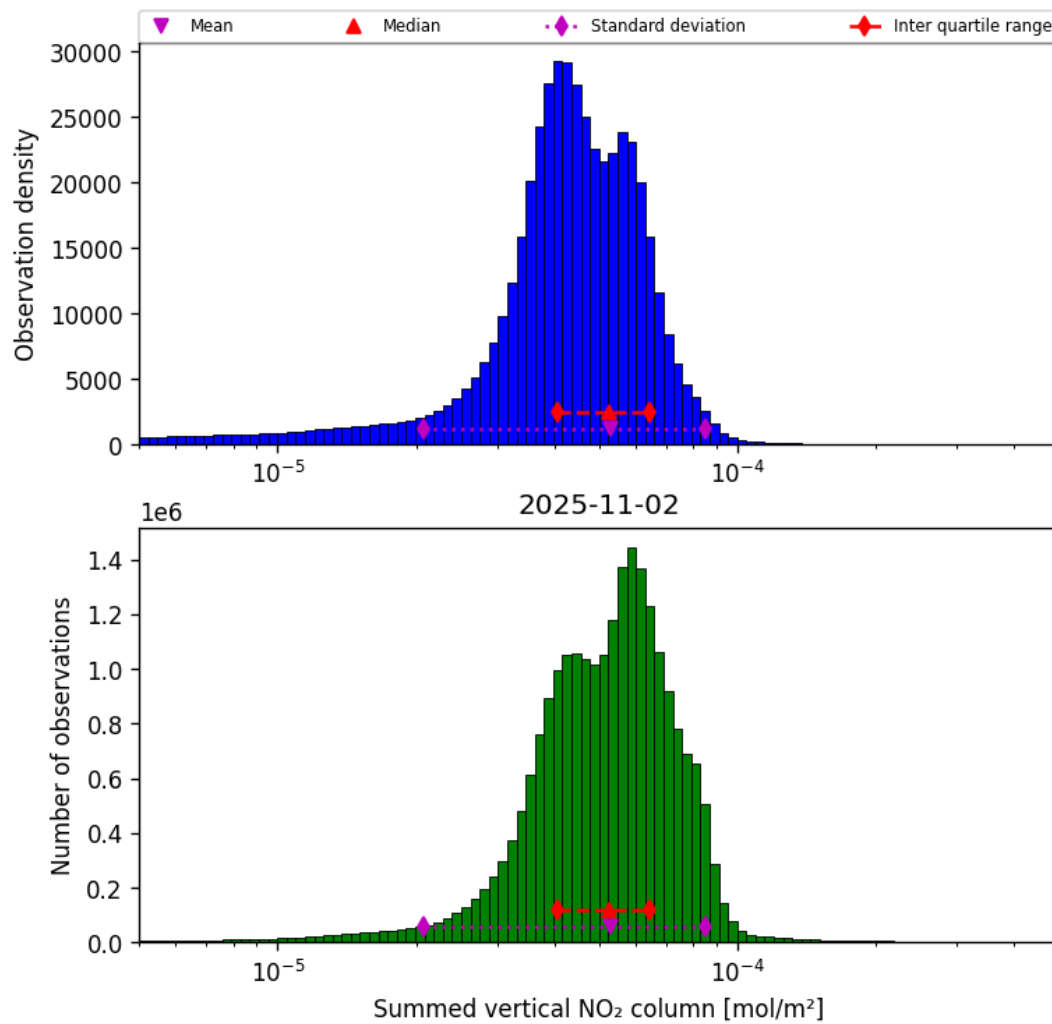
Figure 38: Histogram of "Summed vertical NO 2 column" for 2025-11-02 to 2025-11-03
