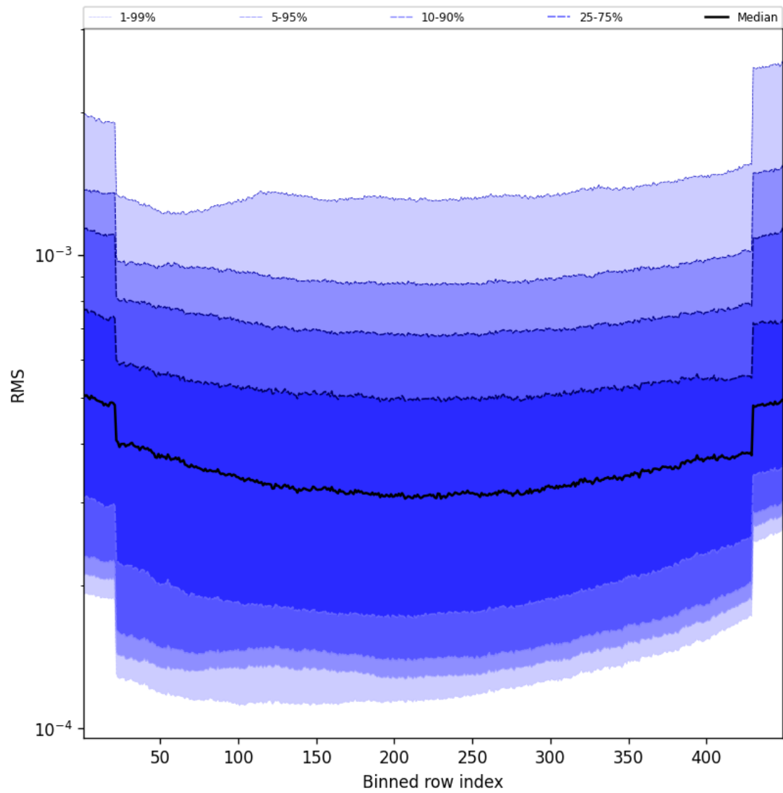
Figure 58: Along track statistics of “RMS” for 2025-11-02 to 2025-11-03
