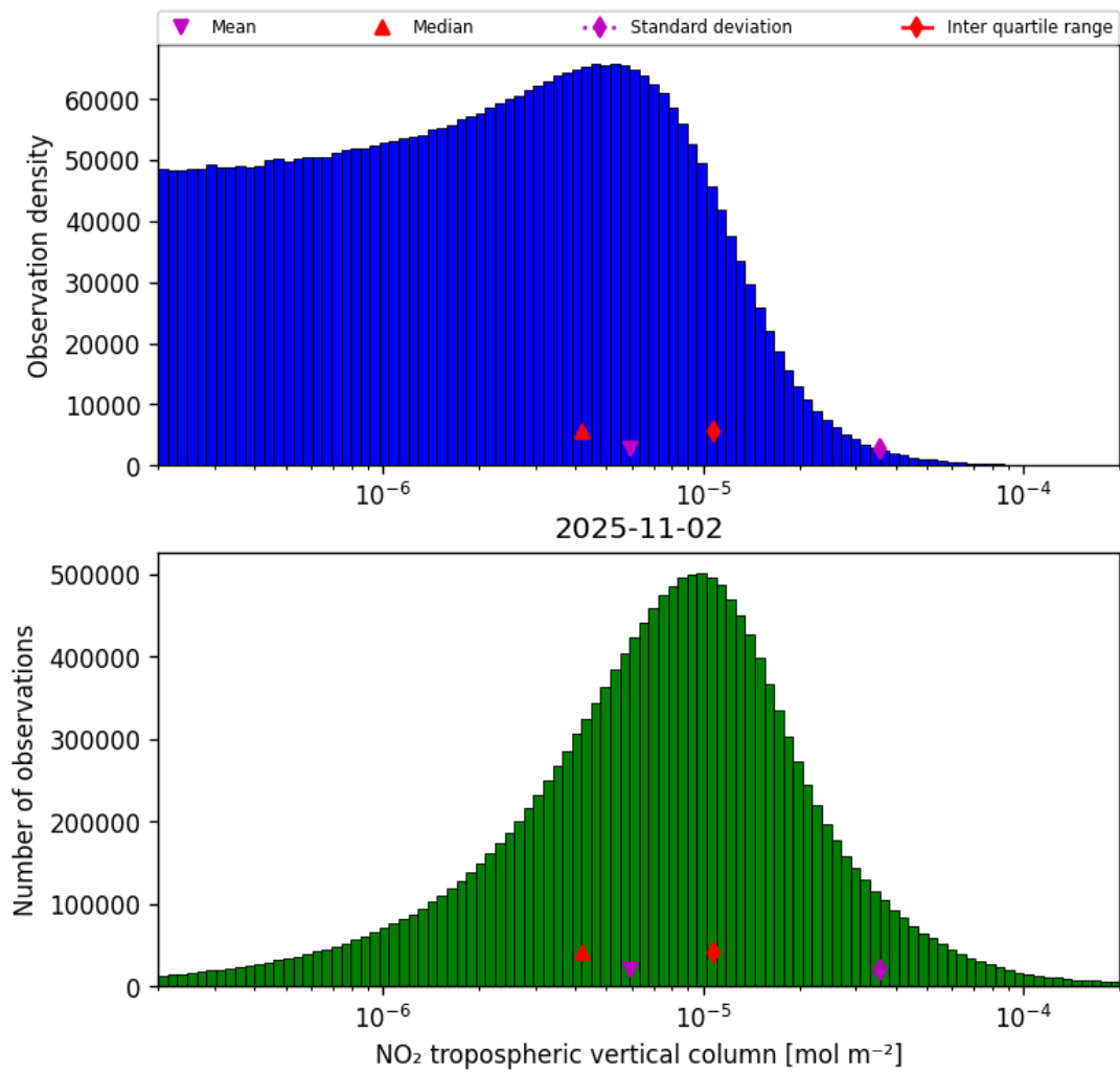
Figure 27: Histogram of “NO 2 tropospheric vertical column” for 2025-11-02 to 2025-11-03
