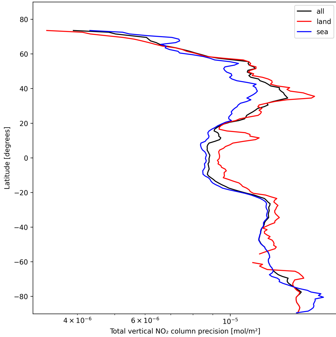
Figure 20: Zonal average of “Total vertical NO 2 column precision” for 2025-11-02 to 2025-11-03.
