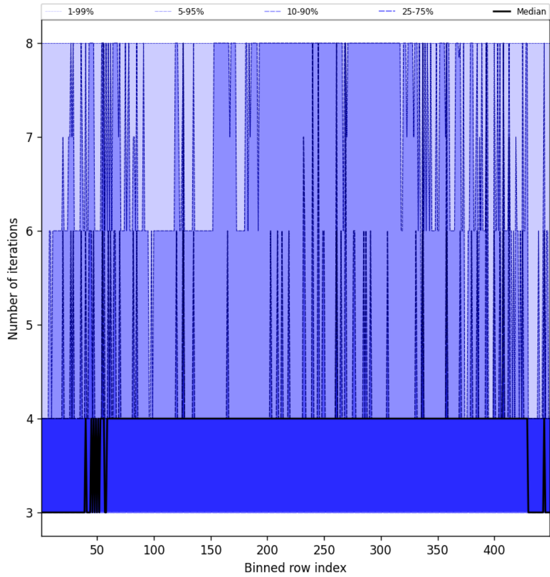
Figure 49: Along track statistics of “Number of iterations” for 2025-11-02 to 2025-11-03
