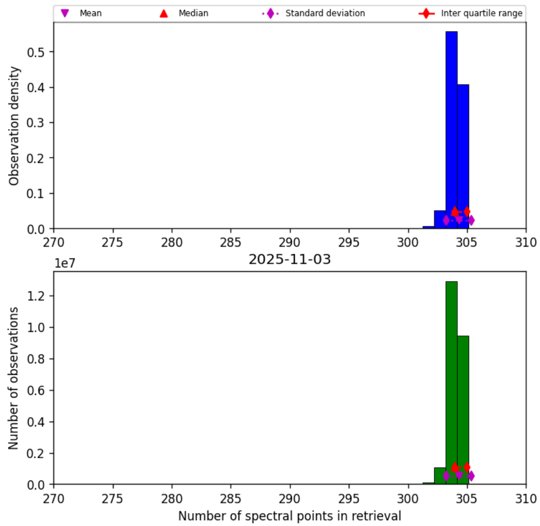
Figure 31: Histogram of “Number of spectral points in retrieval” for 2025-11-03 to 2025-11-04
