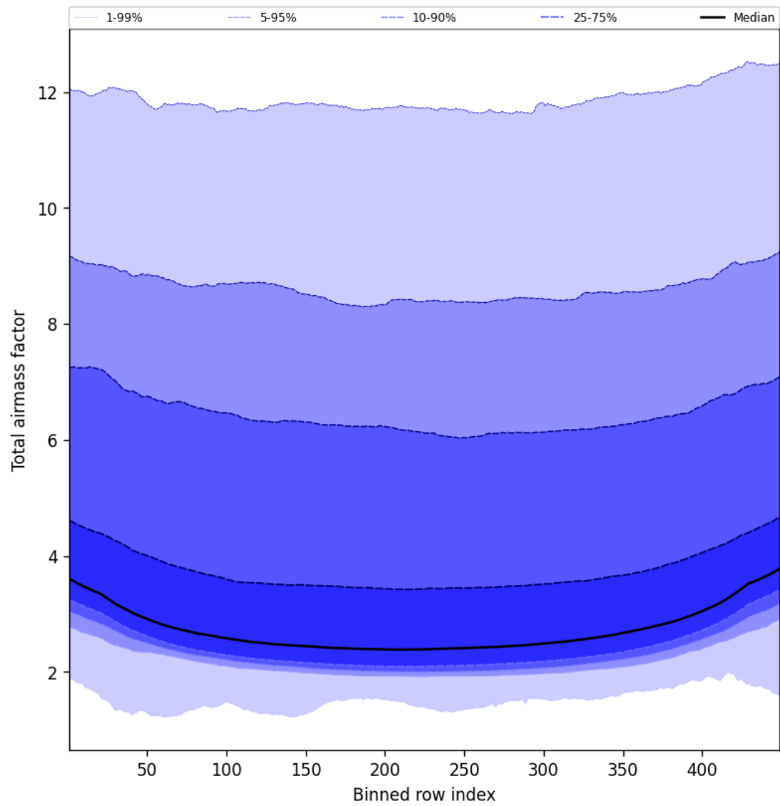
Figure 47: Along track statistics of “Total airmass factor” for 2025-11-03 to 2025-11-04
