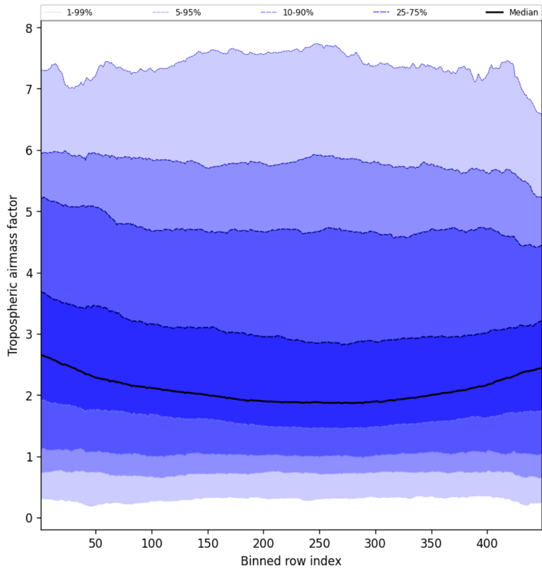
Figure 46: Along track statistics of “Tropospheric air mass factor” for 2025-11-03 to 2025-11-04
