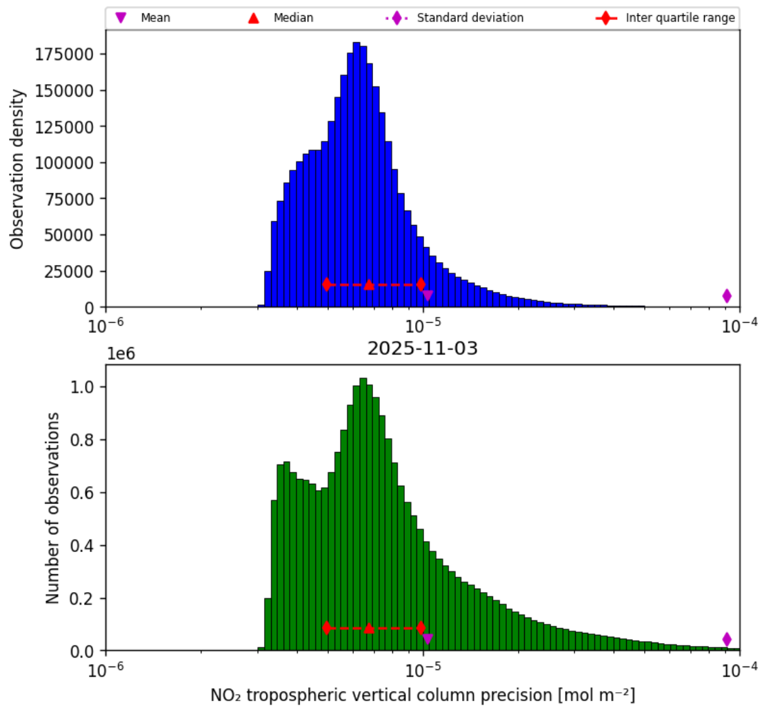
Figure 28: Histogram of “NO 2 tropospheric vertical column precision” for 2025-11-03 to 2025-11-04
