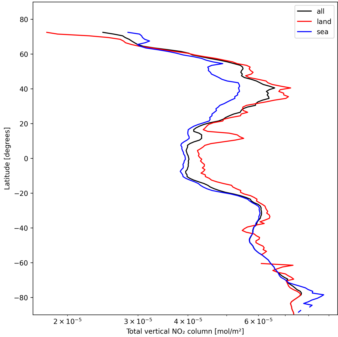
Figure 19: Zonal average of “Total vertical NO 2 column” for 2025-11-03 to 2025-11-04.
