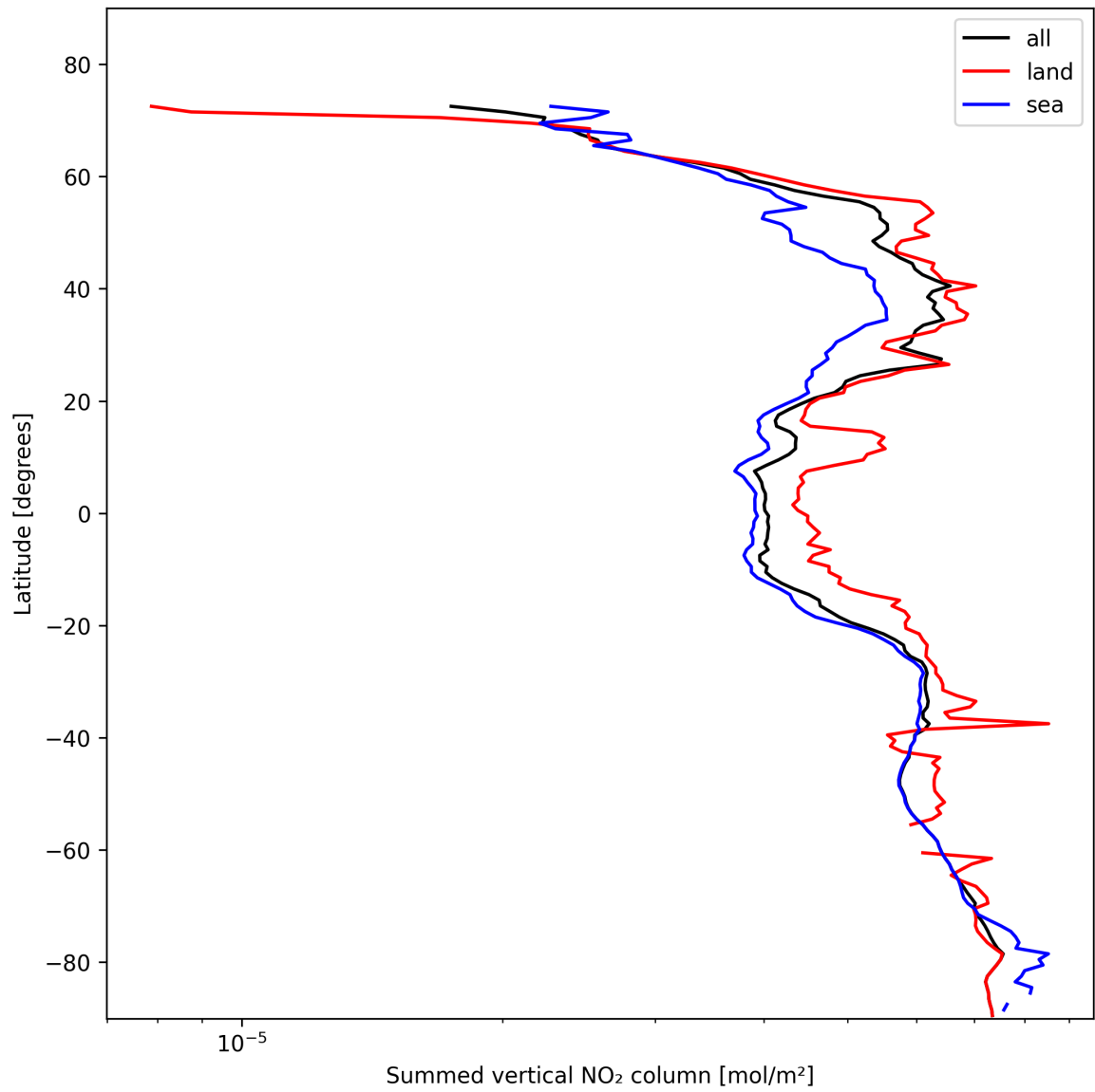
Figure 21: Zonal average of “Summed vertical NO 2 column” for 2025-11-03 to 2025-11-04.
