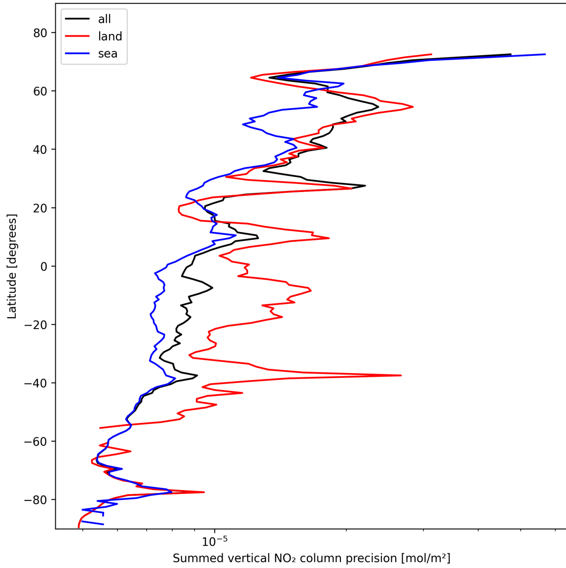
Figure 22: Zonal average of “Summed vertical NO 2 column precision” for 2025-11-03 to 2025-11-04.
