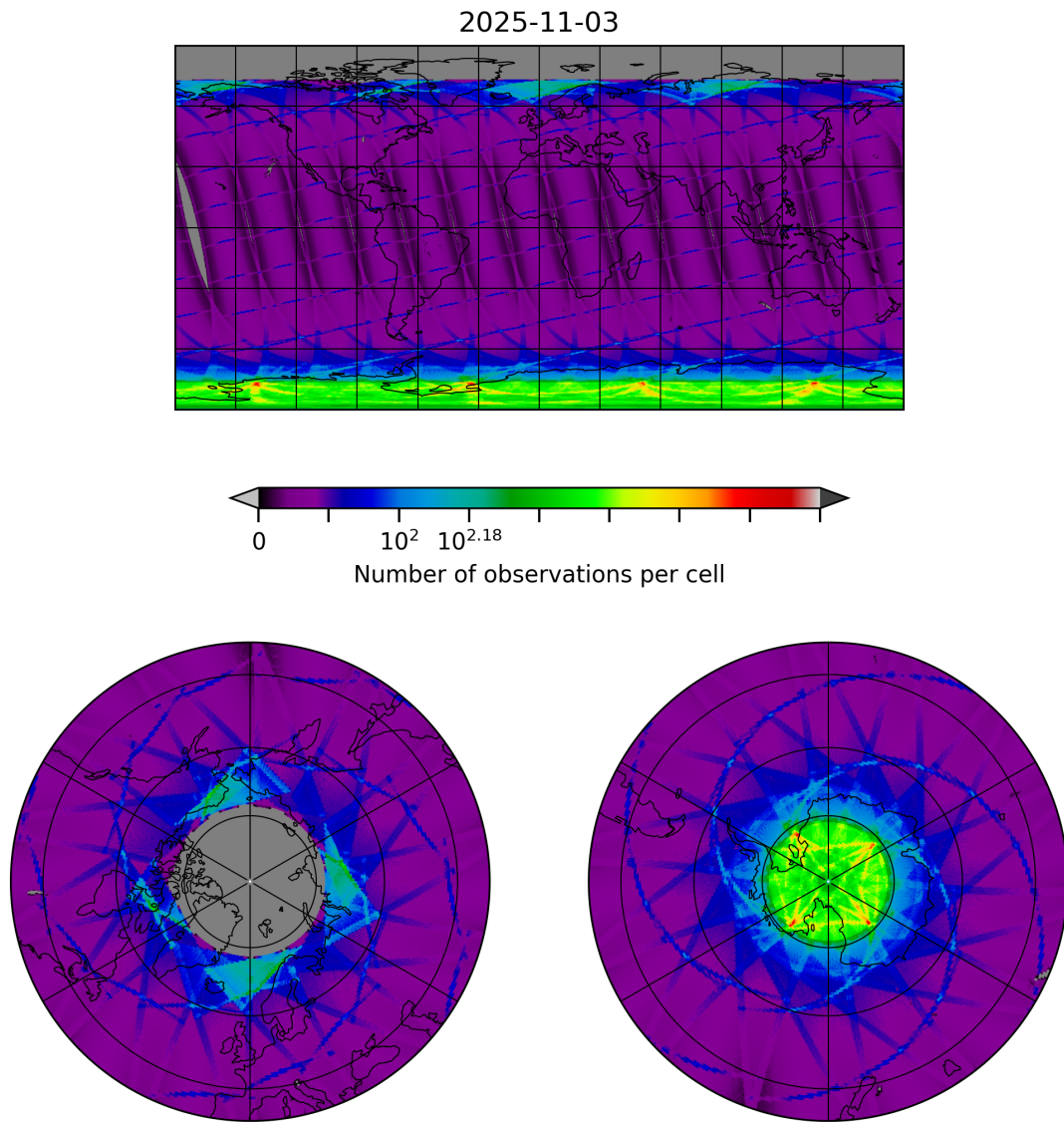
Figure 8: Map of the number of observations for 2025-11-03 to 2025-11-04
