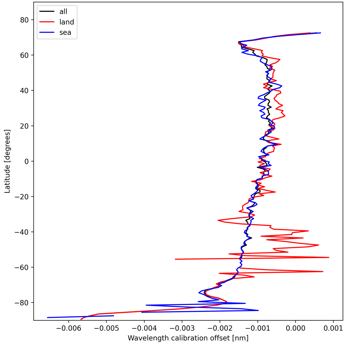
Figure 16: Zonal average of “Wavelength calibration offset” for 2025-11-03 to 2025-11-04.
