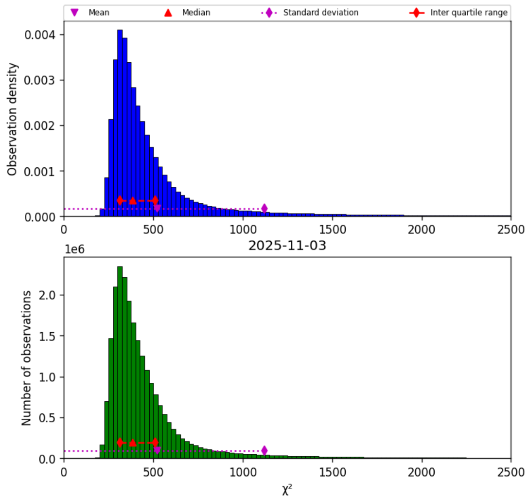
Figure 40: Histogram of “ \chi^2 ” for 2025-11-03 to 2025-11-04
