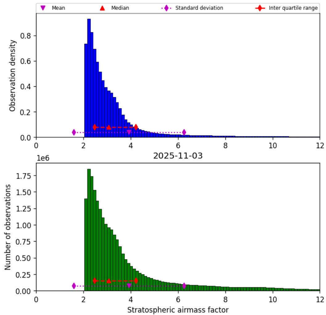
Figure 42: Histogram of “Stratospheric airmass factor” for 2025-11-03 to 2025-11-04
