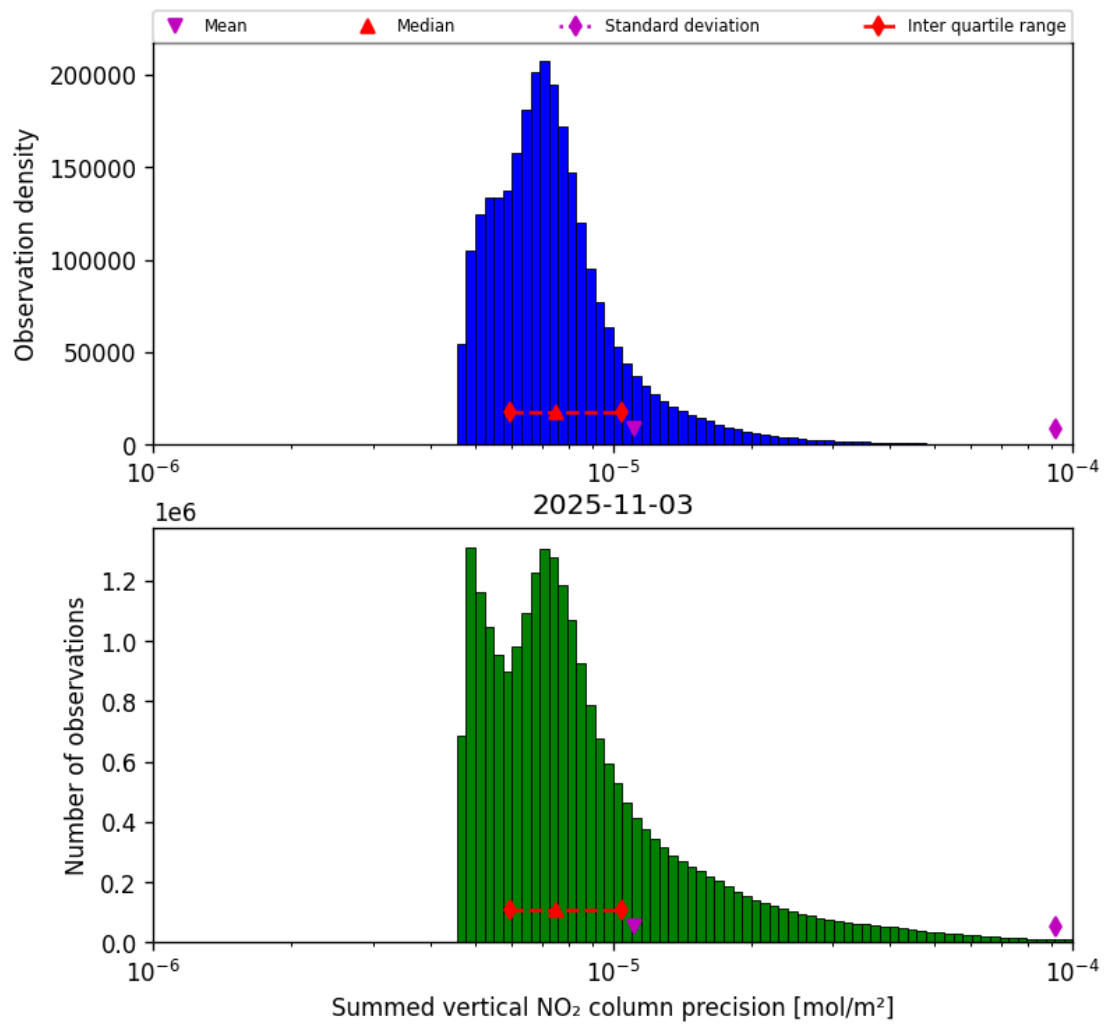
Figure 39: Histogram of "Summed vertical NO 2 column precision" for 2025-11-03 to 2025-11-04
