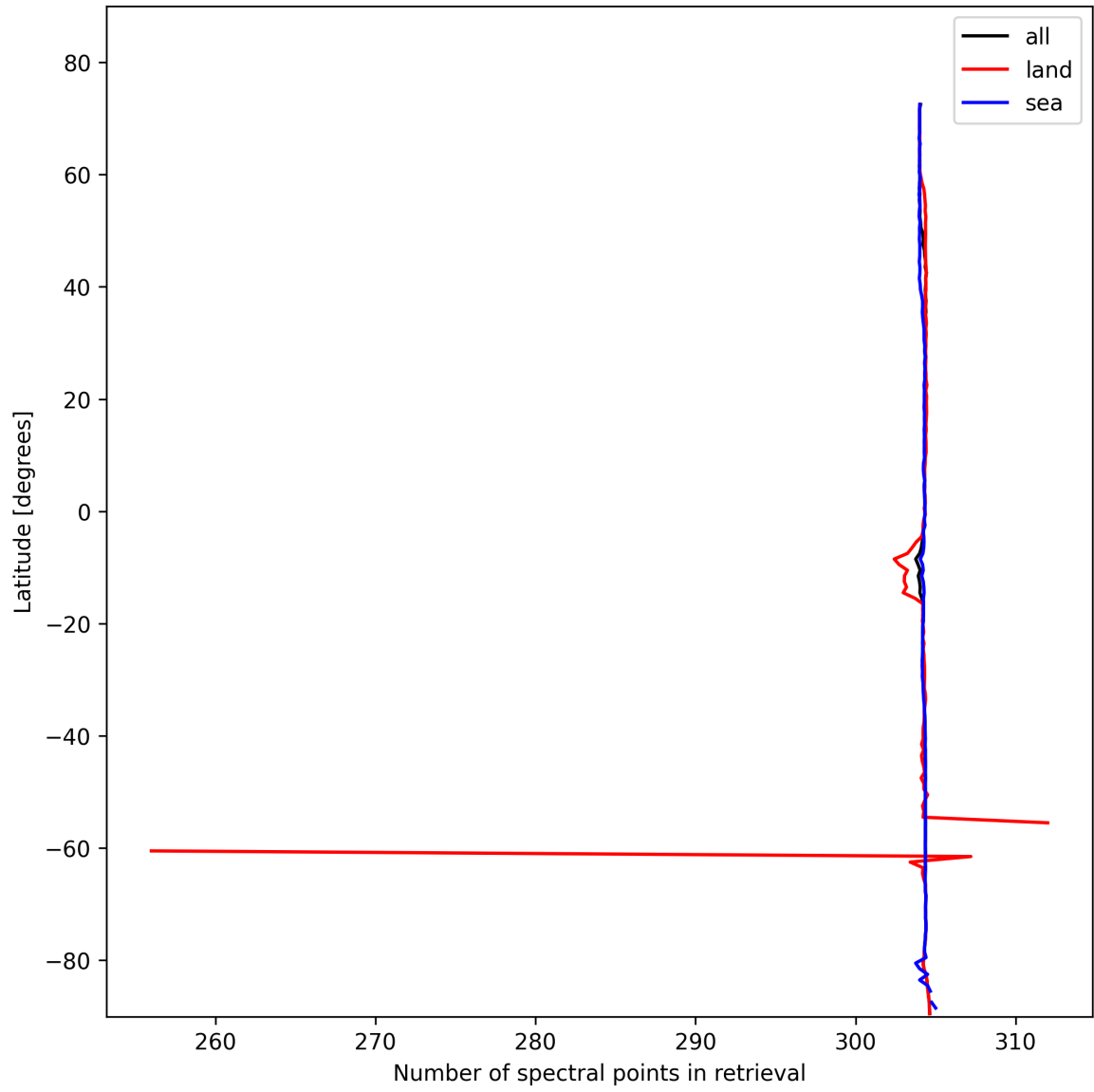
Figure 14: Zonal average of “Number of spectral points in retrieval” for 2025-11-03 to 2025-11-04.
