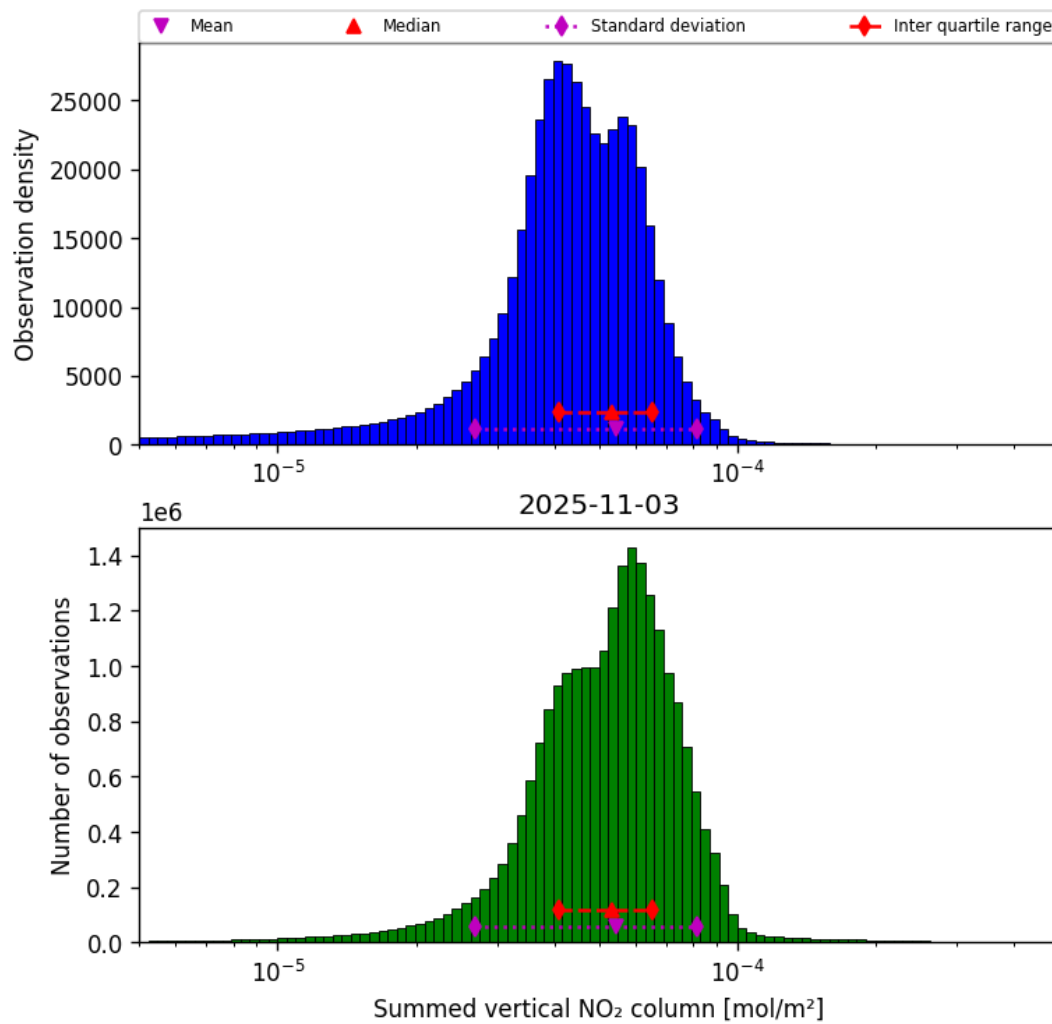
Figure 38: Histogram of “Summed vertical NO 2 column” for 2025-11-03 to 2025-11-04
