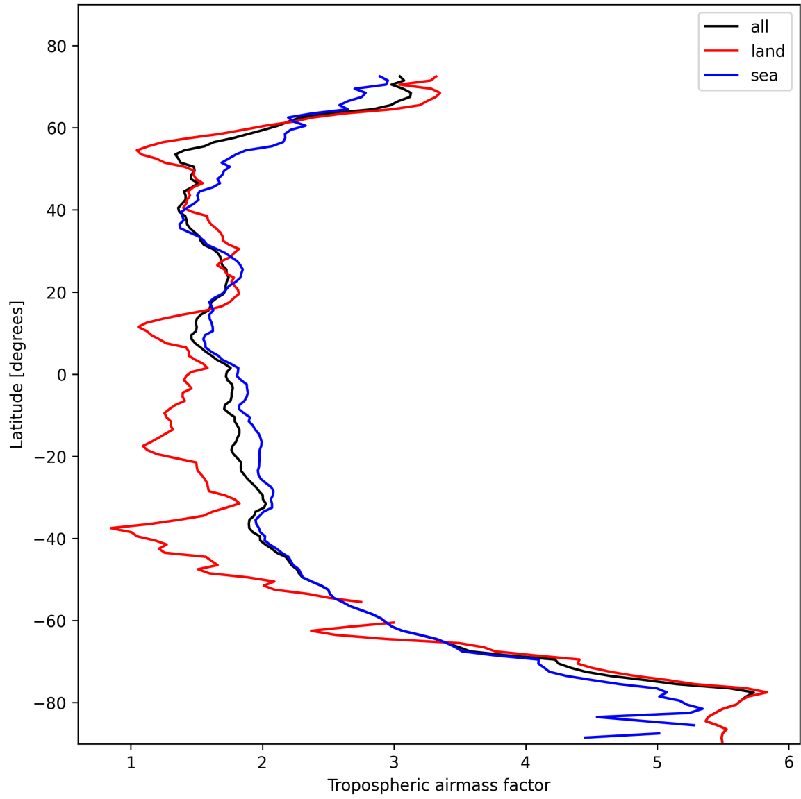
Figure 12: Zonal average of “Tropospheric airmass factor” for 2025-11-03 to 2025-11-04.
