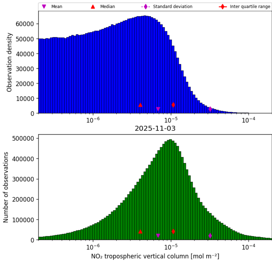
Figure 27: Histogram of “NO 2 tropospheric vertical column” for 2025-11-03 to 2025-11-04
