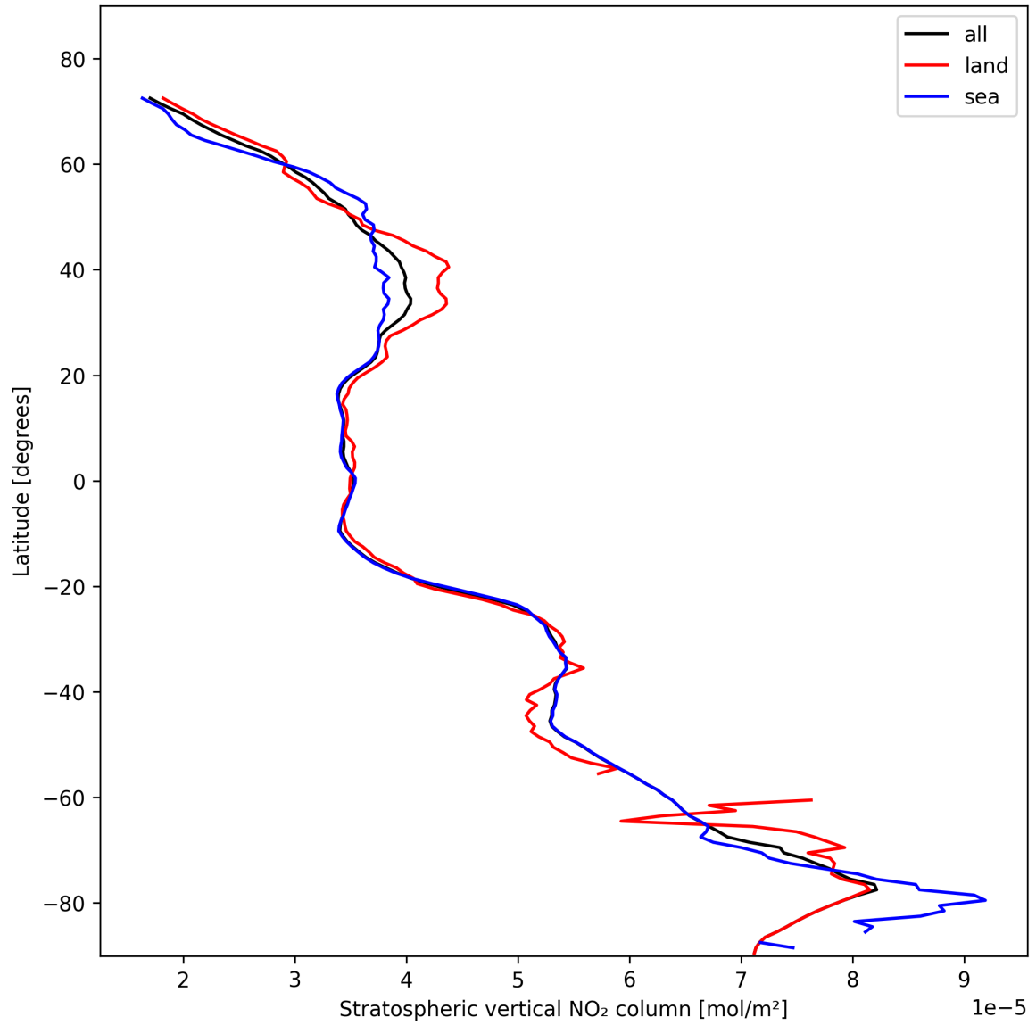
Figure 17: Zonal average of “Stratospheric vertical NO 2 column” for 2025-11-03 to 2025-11-04.
