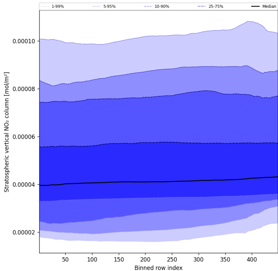
Figure 51: Along track statistics of “Stratospheric vertical NO 2 column” for 2025-11-03 to 2025-11-04
