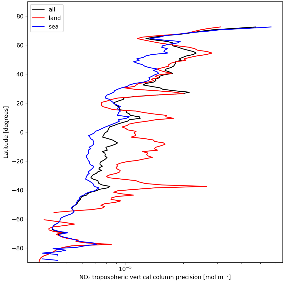
Figure 11: Zonal average of “NO 2 tropospheric vertical column precision” for 2025-11-03 to 2025-11-04.
