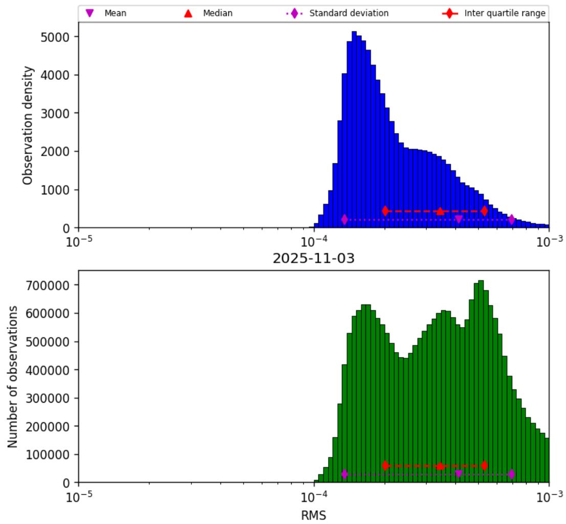
Figure 41: Histogram of “RMS” for 2025-11-03 to 2025-11-04
