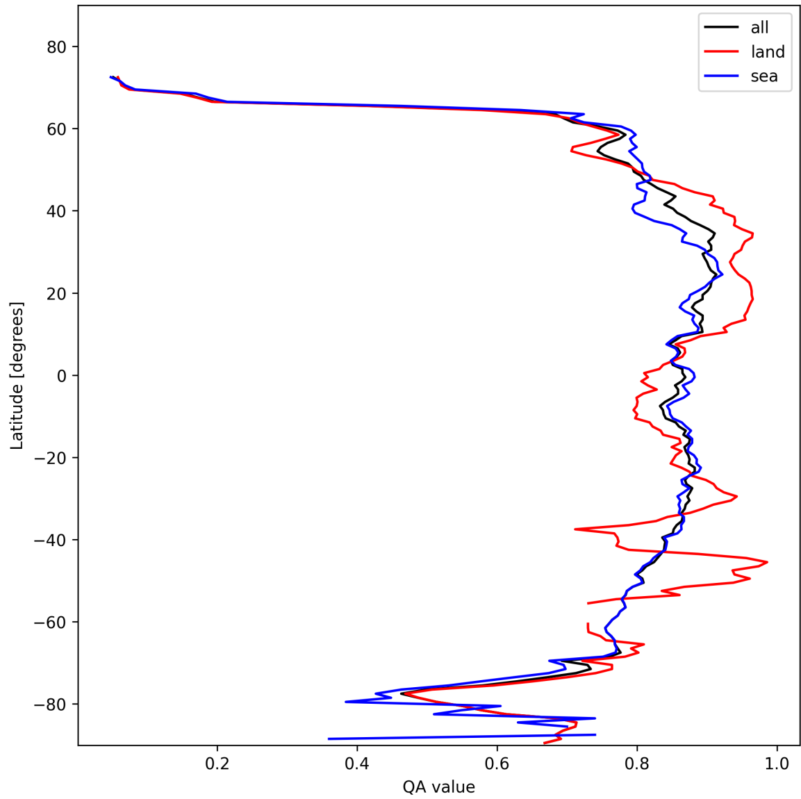
Figure 9: Zonal average of “QA value” for 2025-11-03 to 2025-11-04.
