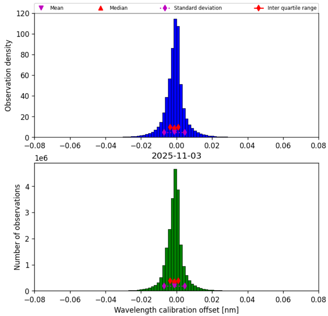
Figure 33: Histogram of “Wavelength calibration offset” for 2025-11-03 to 2025-11-04
