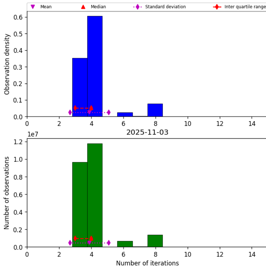
Figure 32: Histogram of “Number of iterations” for 2025-11-03 to 2025-11-04
