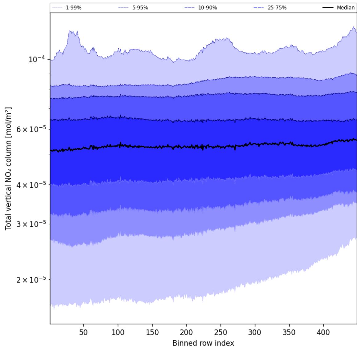
Figure 53: Along track statistics of “Total vertical NO 2 column” for 2025-11-03 to 2025-11-04
