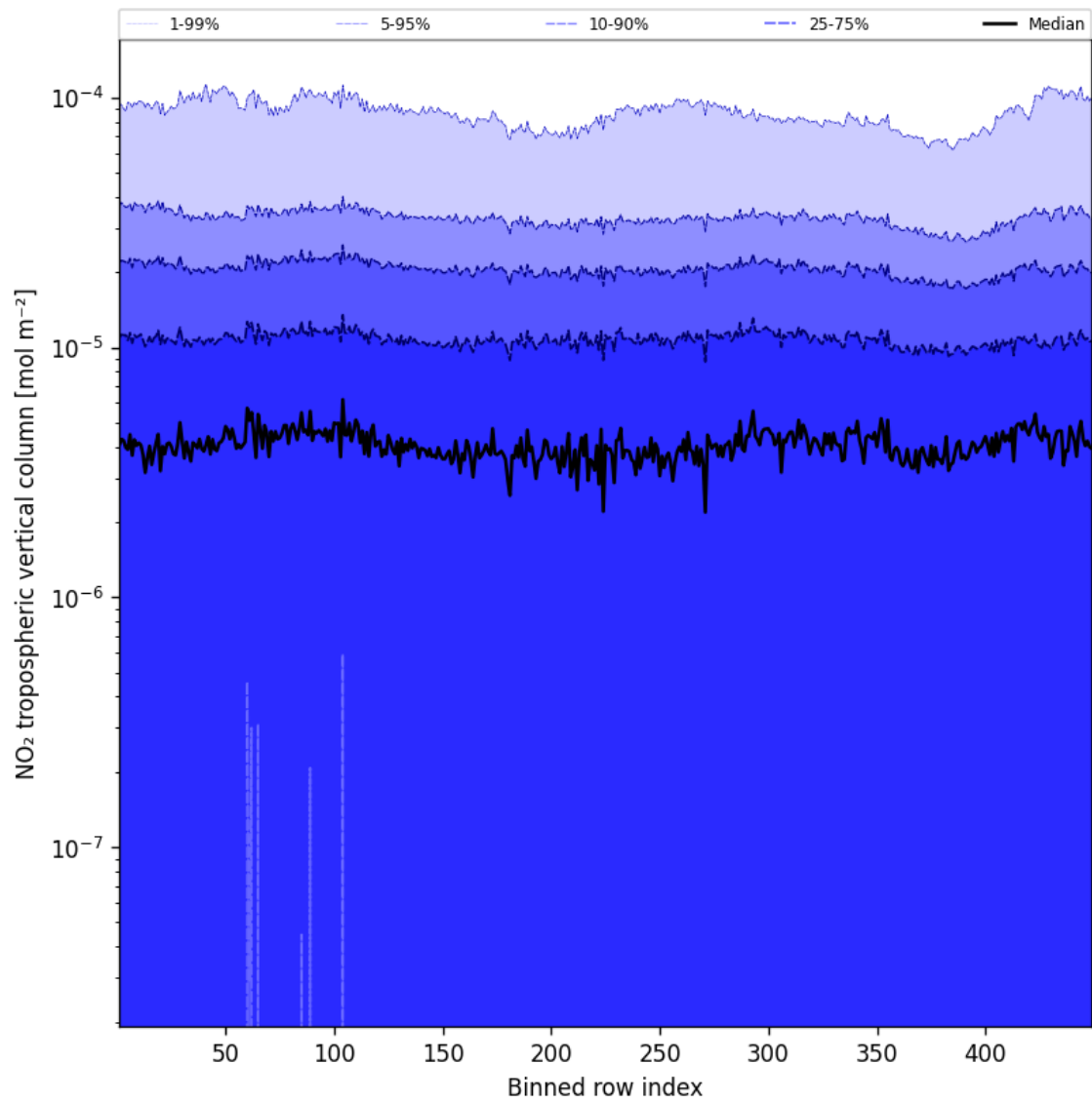
Figure 44: Along track statistics of “NO 2 tropospheric vertical column” for 2025-11-03 to 2025-11-04
