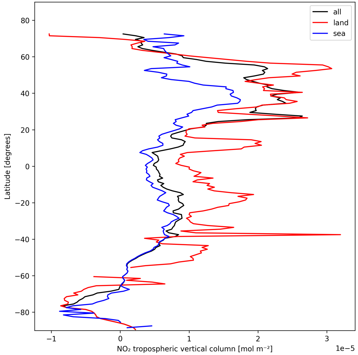
Figure 10: Zonal average of “NO 2 tropospheric vertical column” for 2025-11-03 to 2025-11-04.
