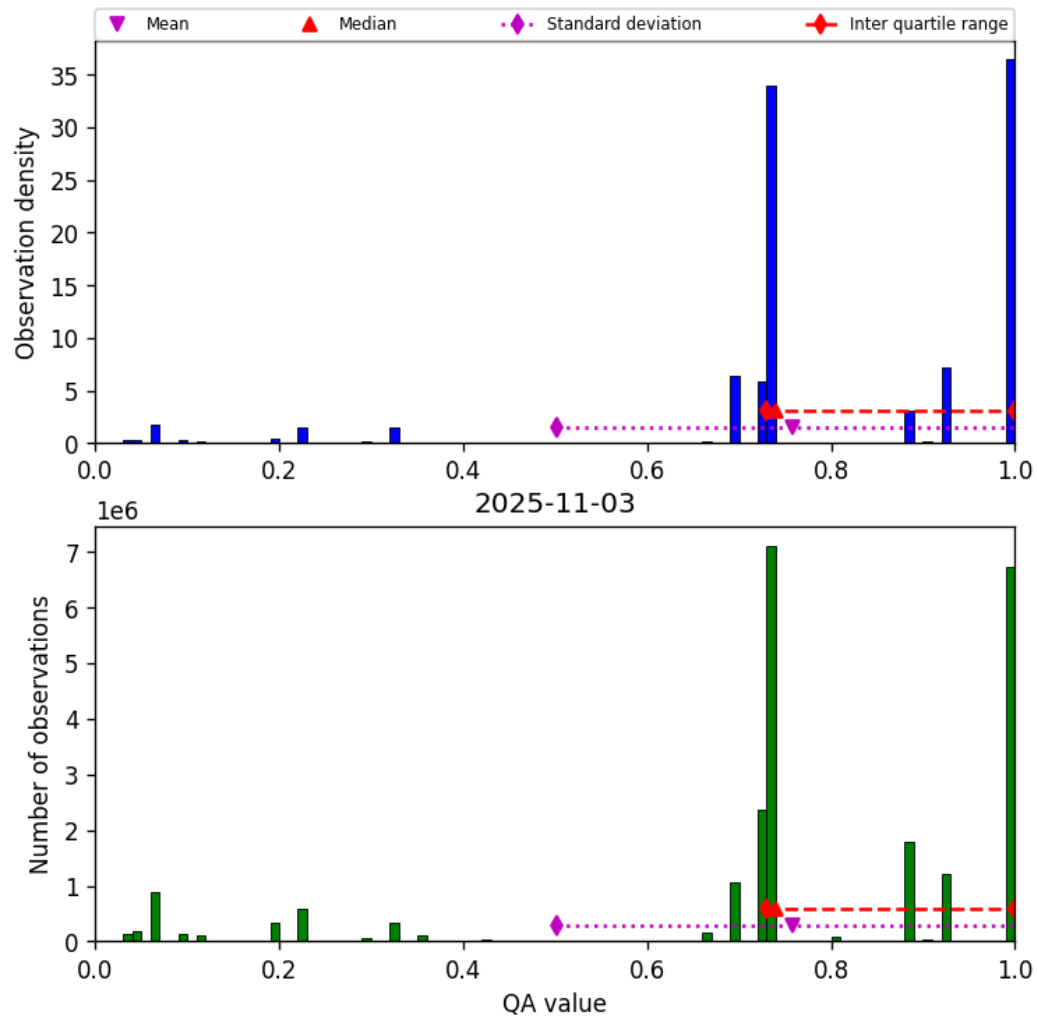
Figure 26: Histogram of “QA value” for 2025-11-03 to 2025-11-04
