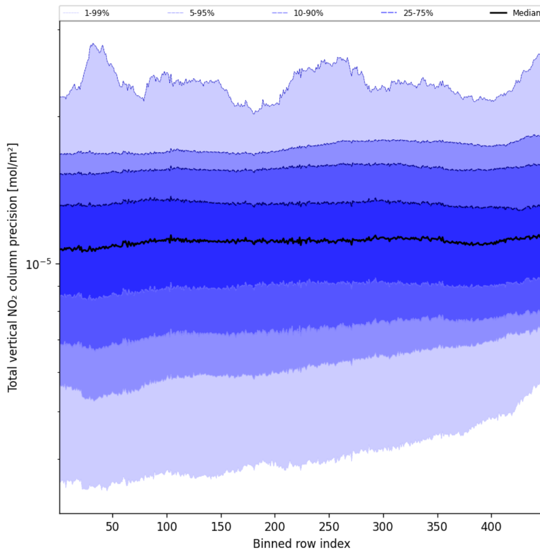
Figure 54: Along track statistics of “Total vertical NO 2 column precision” for 2025-11-03 to 2025-11-04
