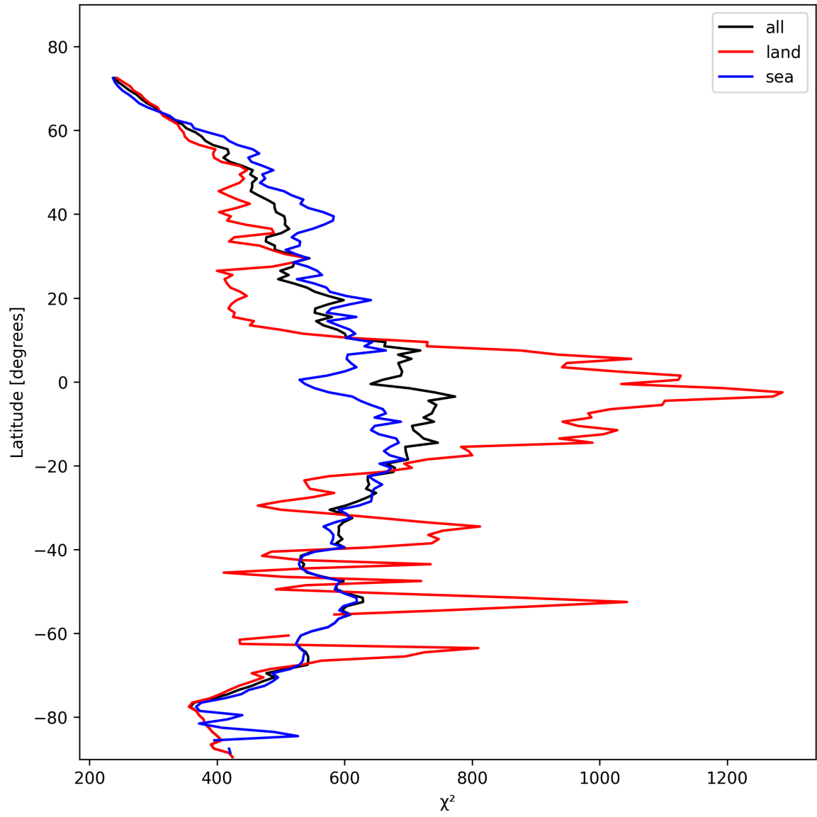
Figure 23: Zonal average of “ \chi^2 ” for 2025-11-03 to 2025-11-04.
