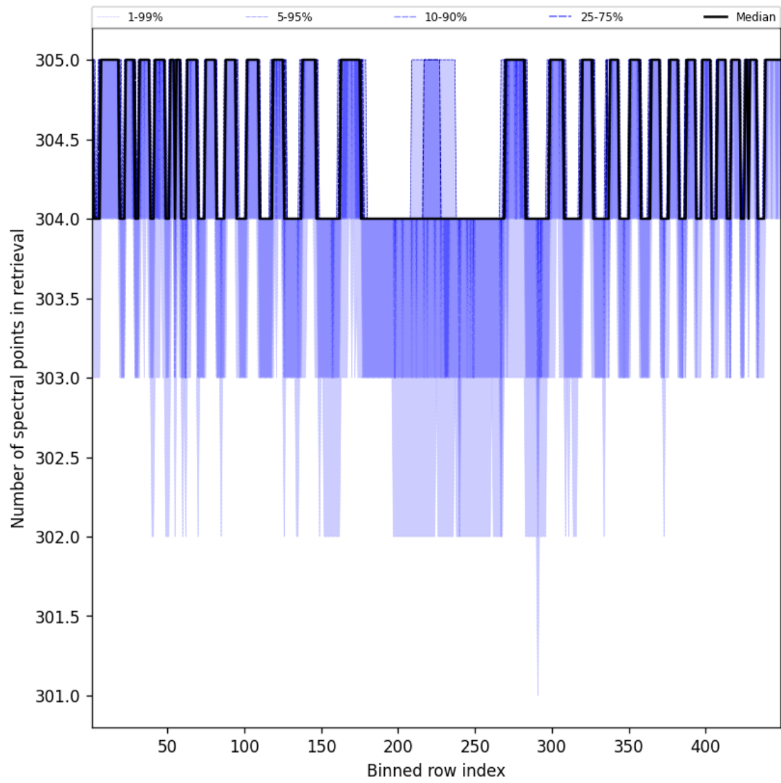
Figure 48: Along track statistics of “Number of spectral points in retrieval” for 2025-11-03 to 2025-11-04
