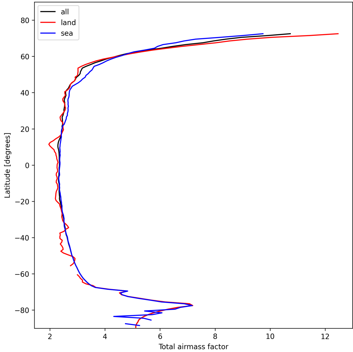
Figure 13: Zonal average of “Total airmass factor” for 2025-11-03 to 2025-11-04.
