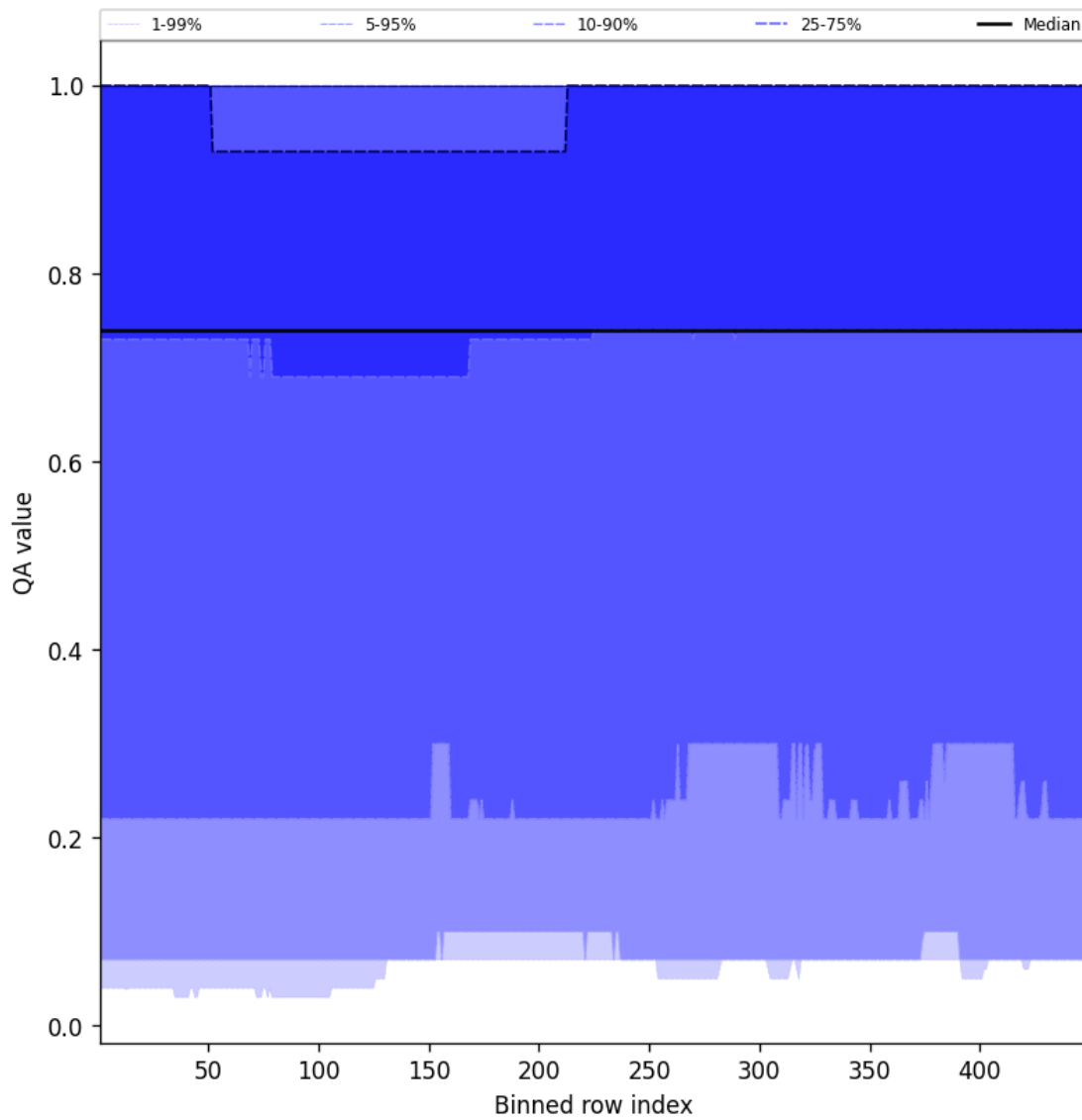
Figure 43: Along track statistics of “QA value” for 2025-11-03 to 2025-11-04
