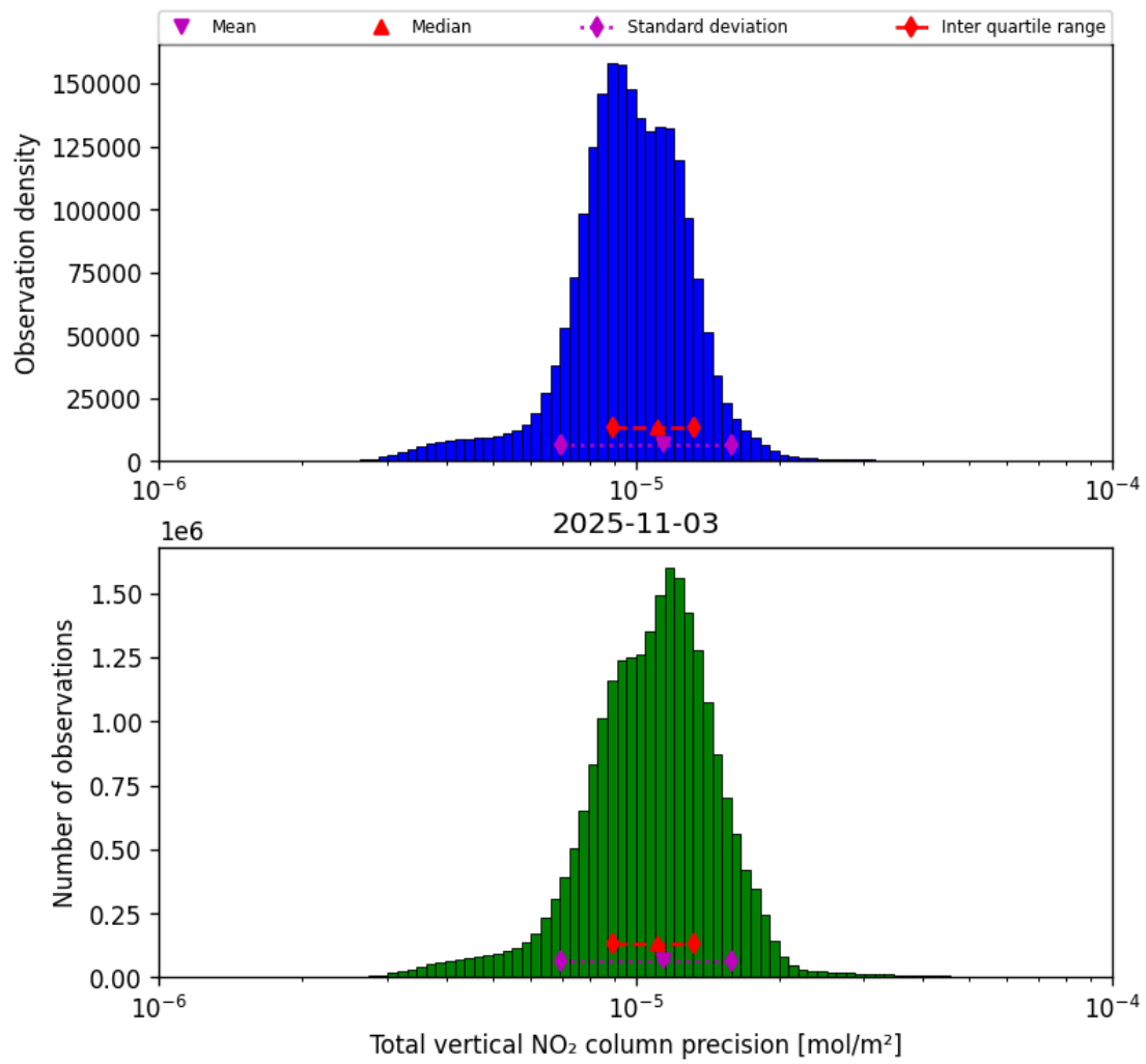
Figure 37: Histogram of “Total vertical NO 2 column precision” for 2025-11-03 to 2025-11-04
