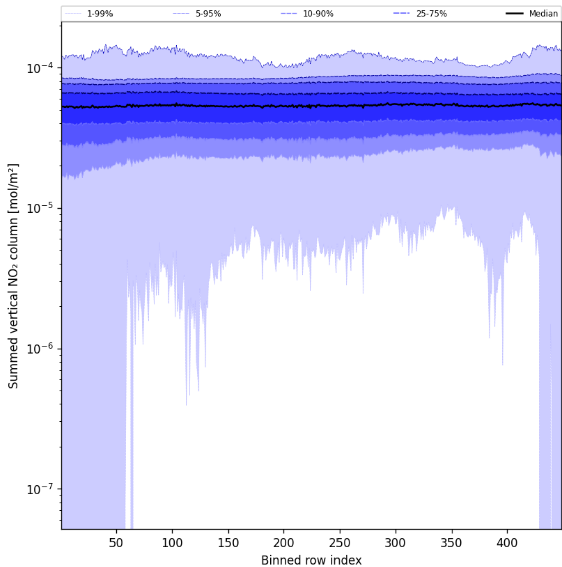
Figure 55: Along track statistics of “Summed vertical NO 2 column” for 2025-11-03 to 2025-11-04
