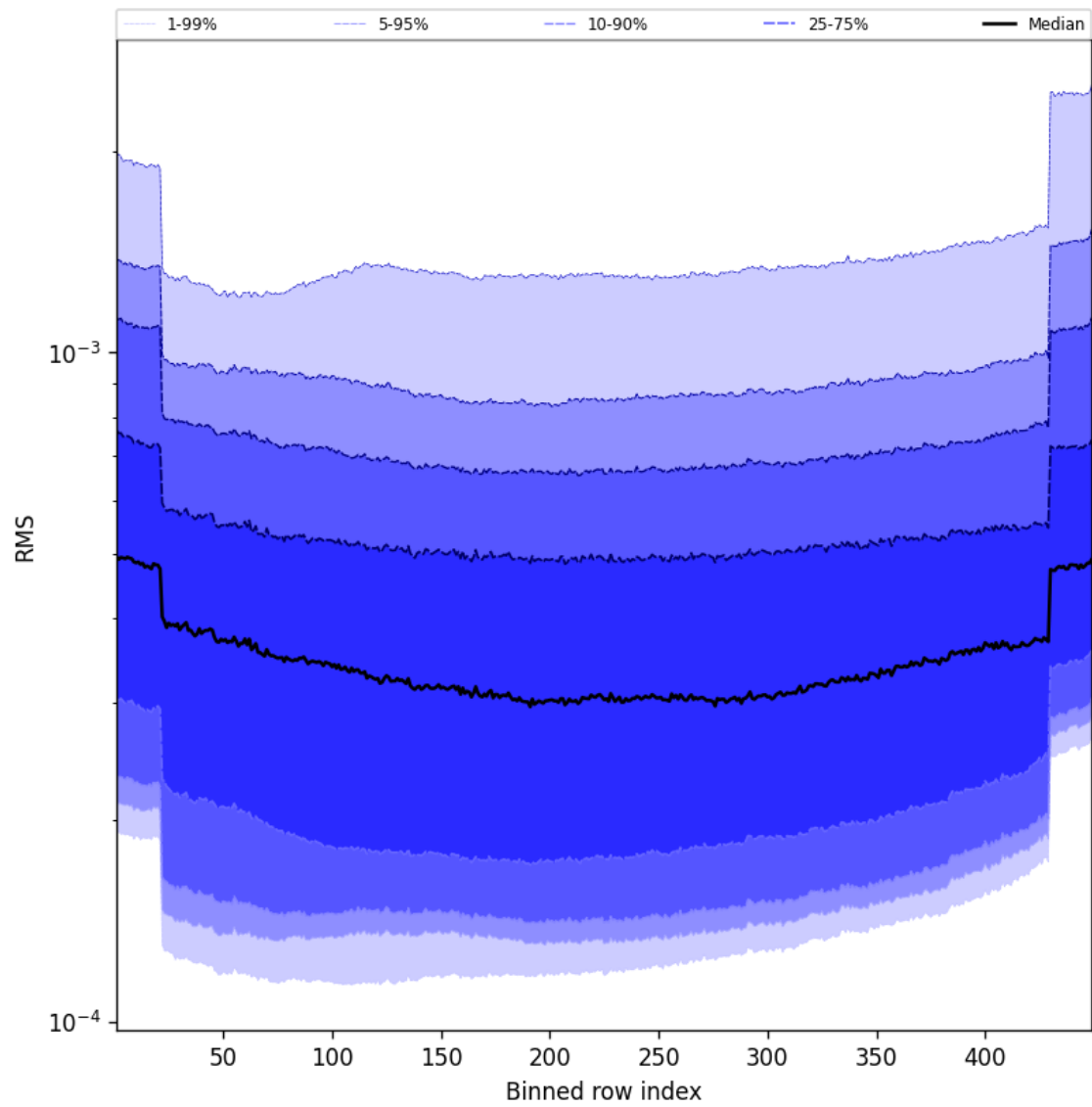
Figure 58: Along track statistics of “RMS” for 2025-11-03 to 2025-11-04
