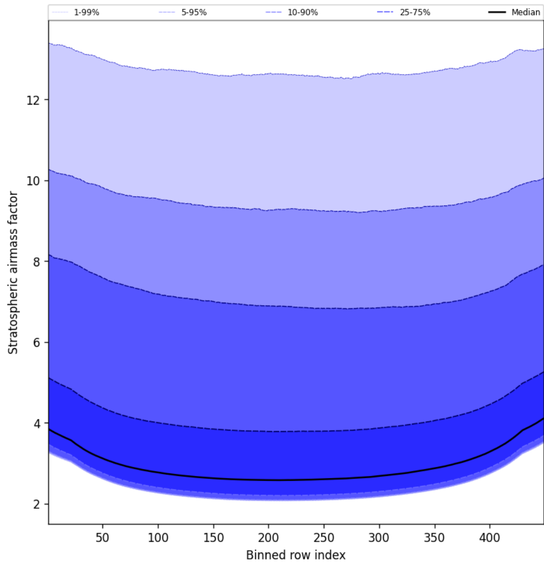
Figure 59: Along track statistics of “Stratospheric airmass factor” for 2025-11-03 to 2025-11-04
