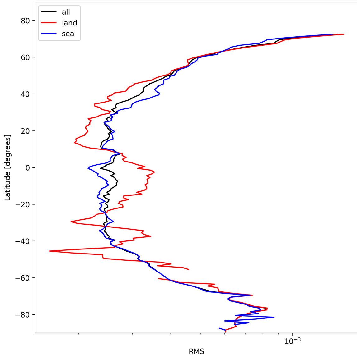
Figure 24: Zonal average of “RMS” for 2025-11-03 to 2025-11-04.
