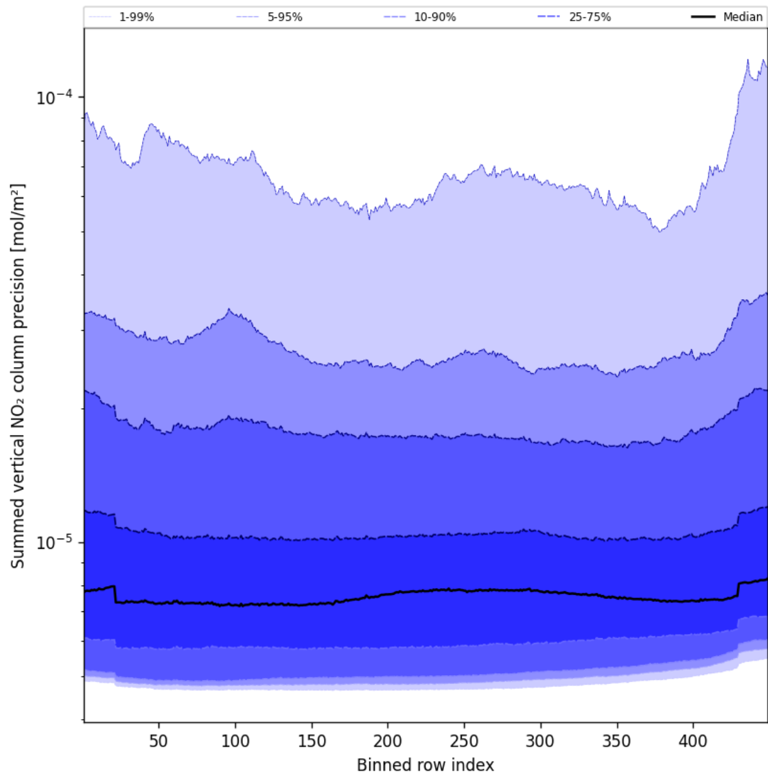
Figure 56: Along track statistics of “Summed vertical NO 2 column precision” for 2025-11-03 to 2025-11-04
