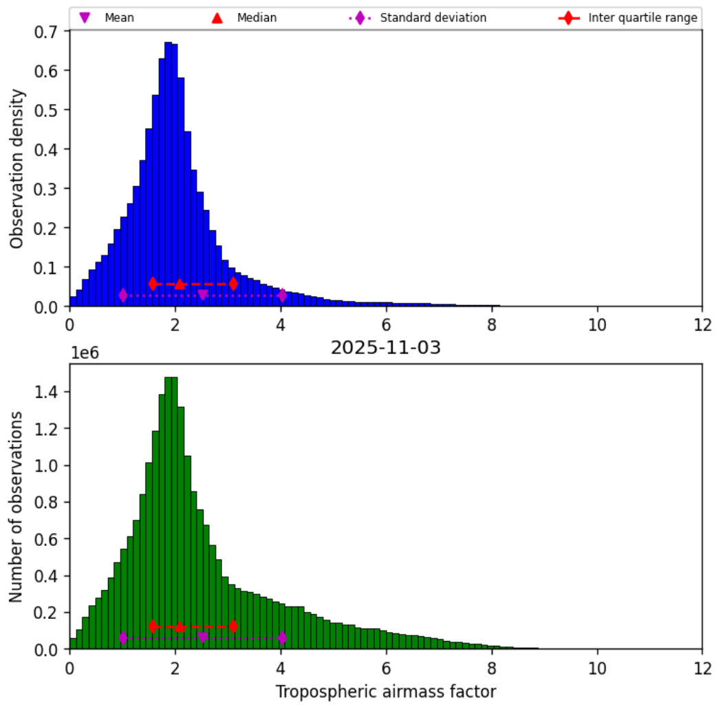
Figure 29: Histogram of “Tropospheric airmass factor” for 2025-11-03 to 2025-11-04
