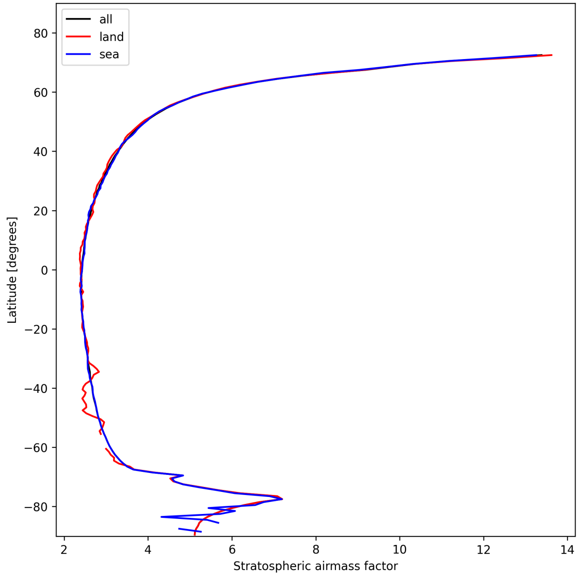
Figure 25: Zonal average of “Stratospheric air mass factor” for 2025-11-03 to 2025-11-04.
