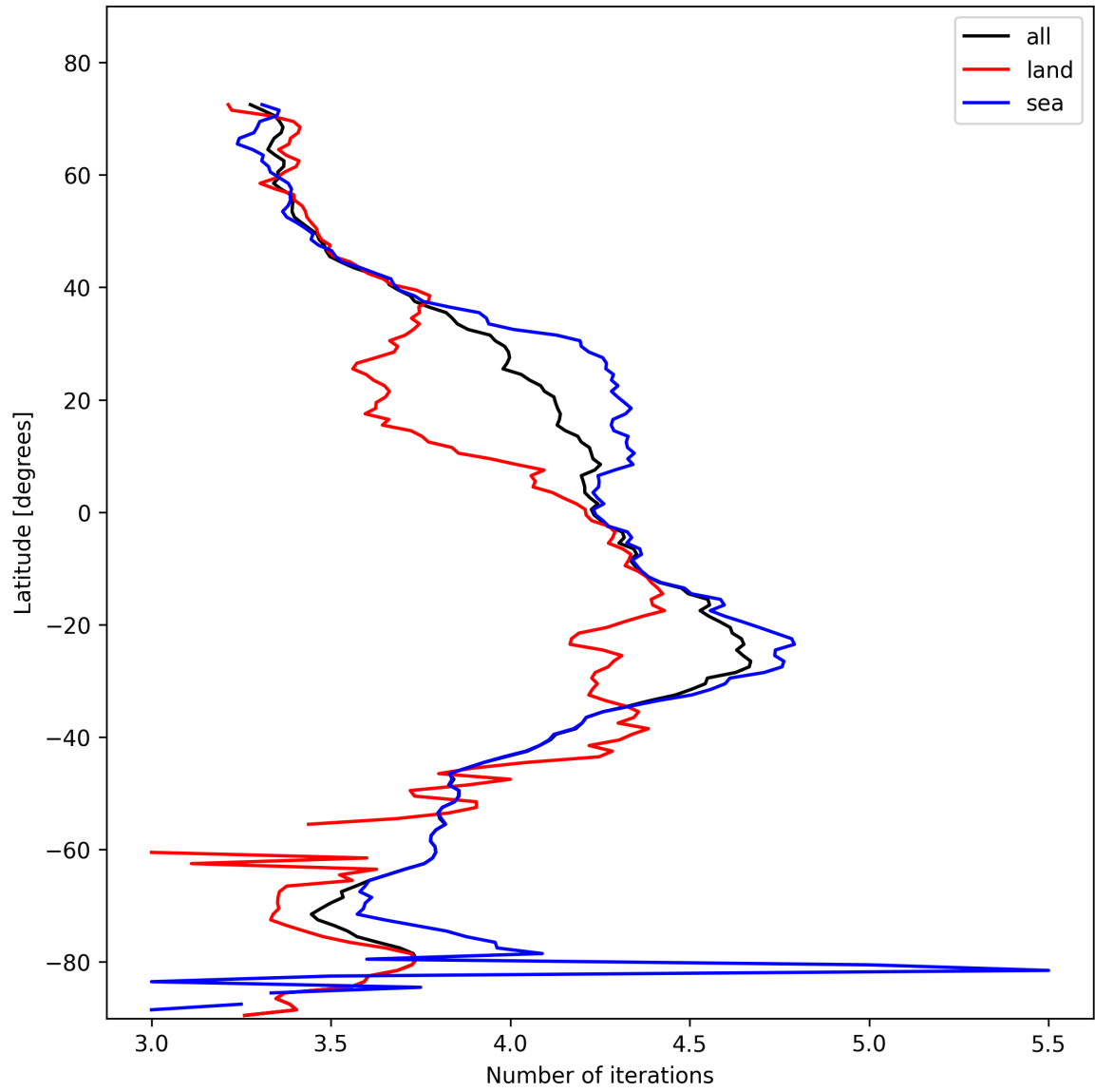
Figure 15: Zonal average of “Number of iterations” for 2025-11-03 to 2025-11-04.
