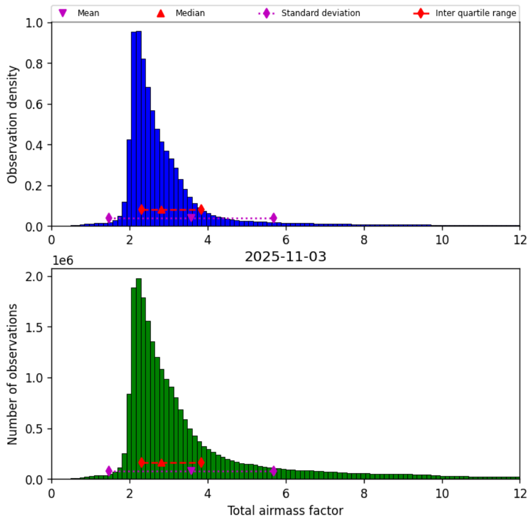
Figure 30: Histogram of “Total airmass factor” for 2025-11-03 to 2025-11-04
