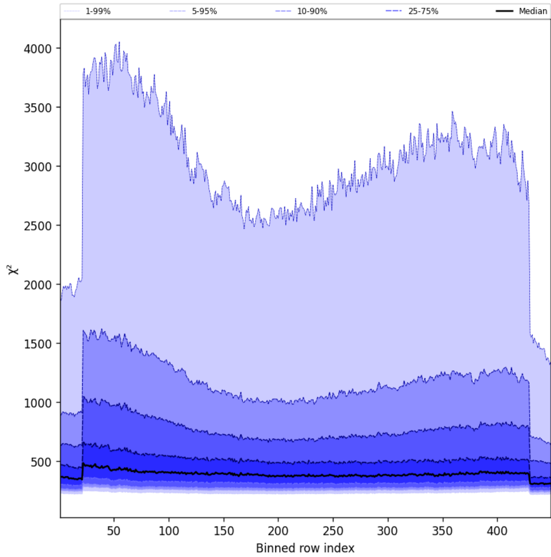
Figure 57: Along track statistics of “ \chi^2 ” for 2025-11-03 to 2025-11-04
