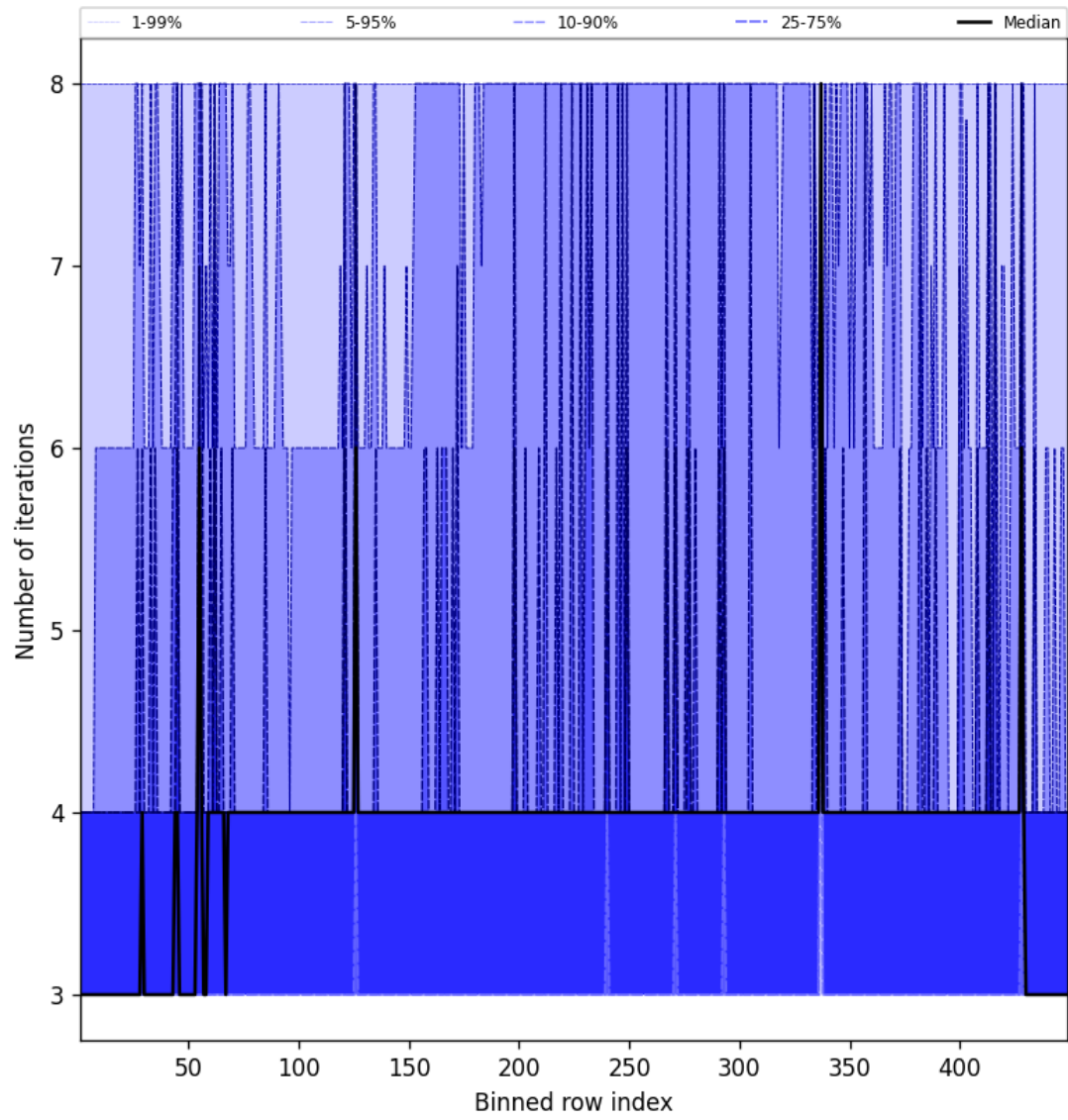
Figure 49: Along track statistics of “Number of iterations” for 2025-11-03 to 2025-11-04
