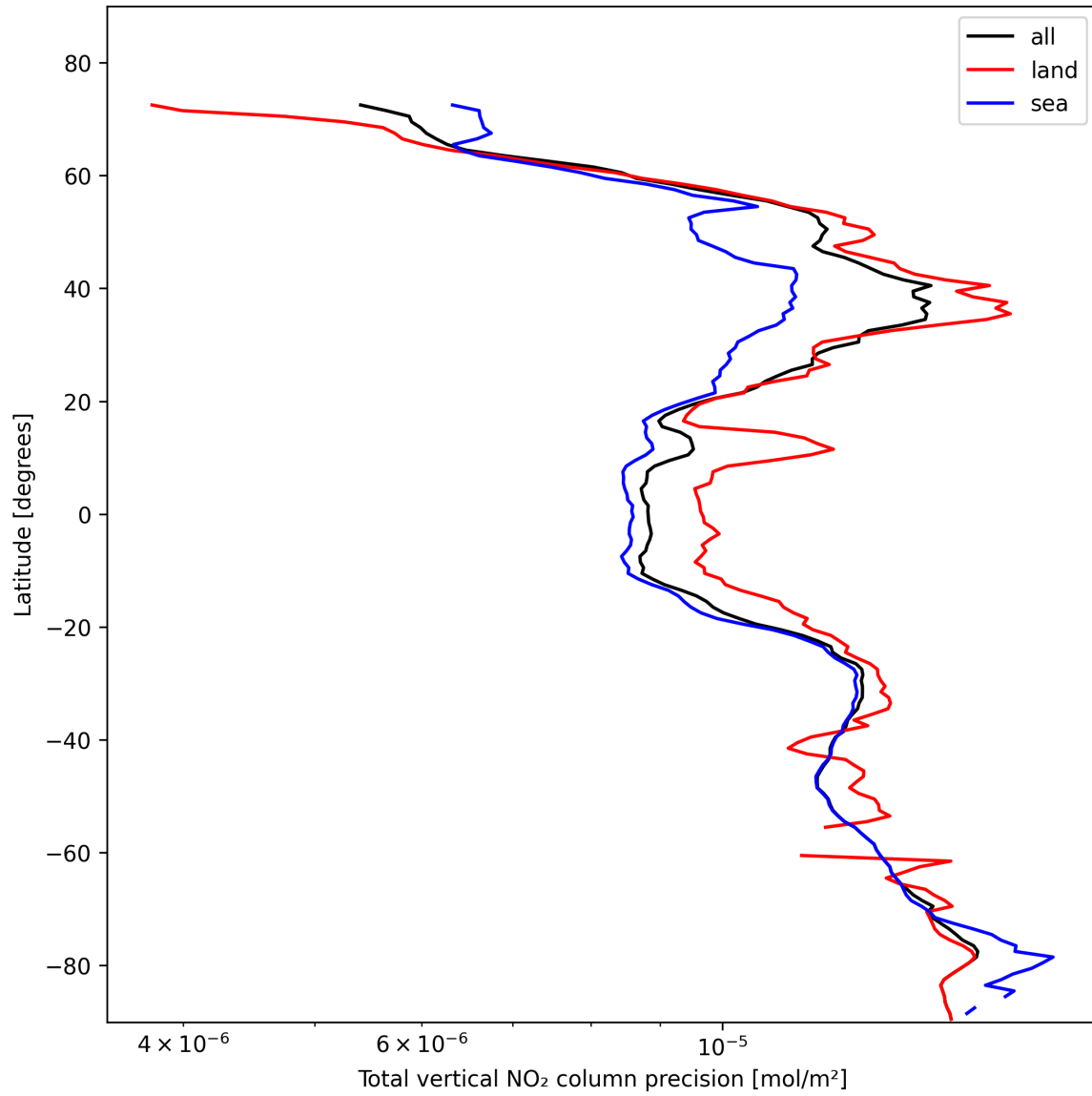
Figure 20: Zonal average of “Total vertical NO 2 column precision” for 2025-11-03 to 2025-11-04.
