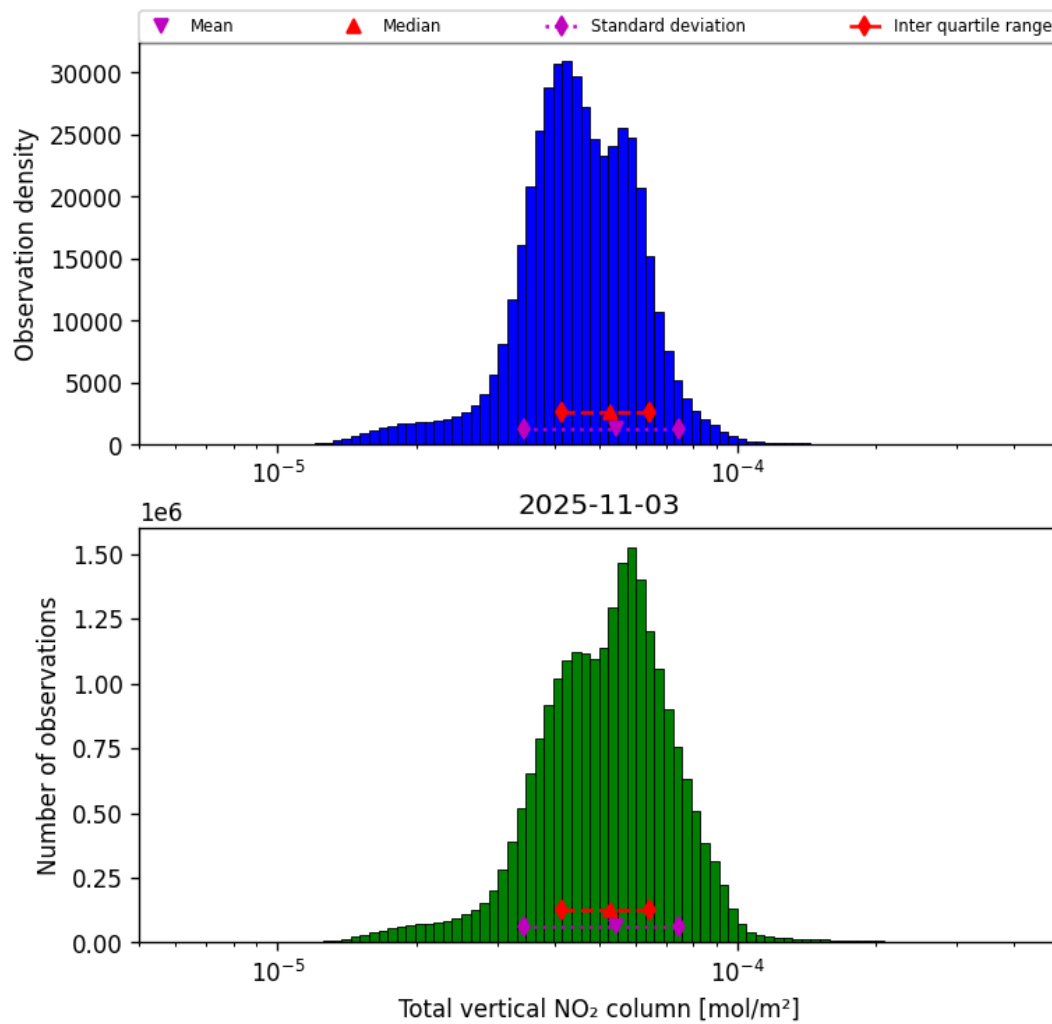
Figure 36: Histogram of "Total vertical NO 2 column" for 2025-11-03 to 2025-11-04
