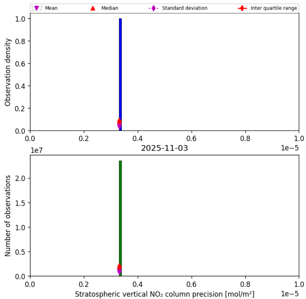
Figure 35: Histogram of “Stratospheric vertical NO 2 column precision” for 2025-11-03 to 2025-11-04
