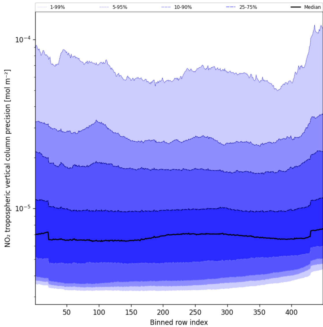
Figure 45: Along track statistics of “NO 2 tropospheric vertical column precision” for 2025-11-03 to 2025-11-04
