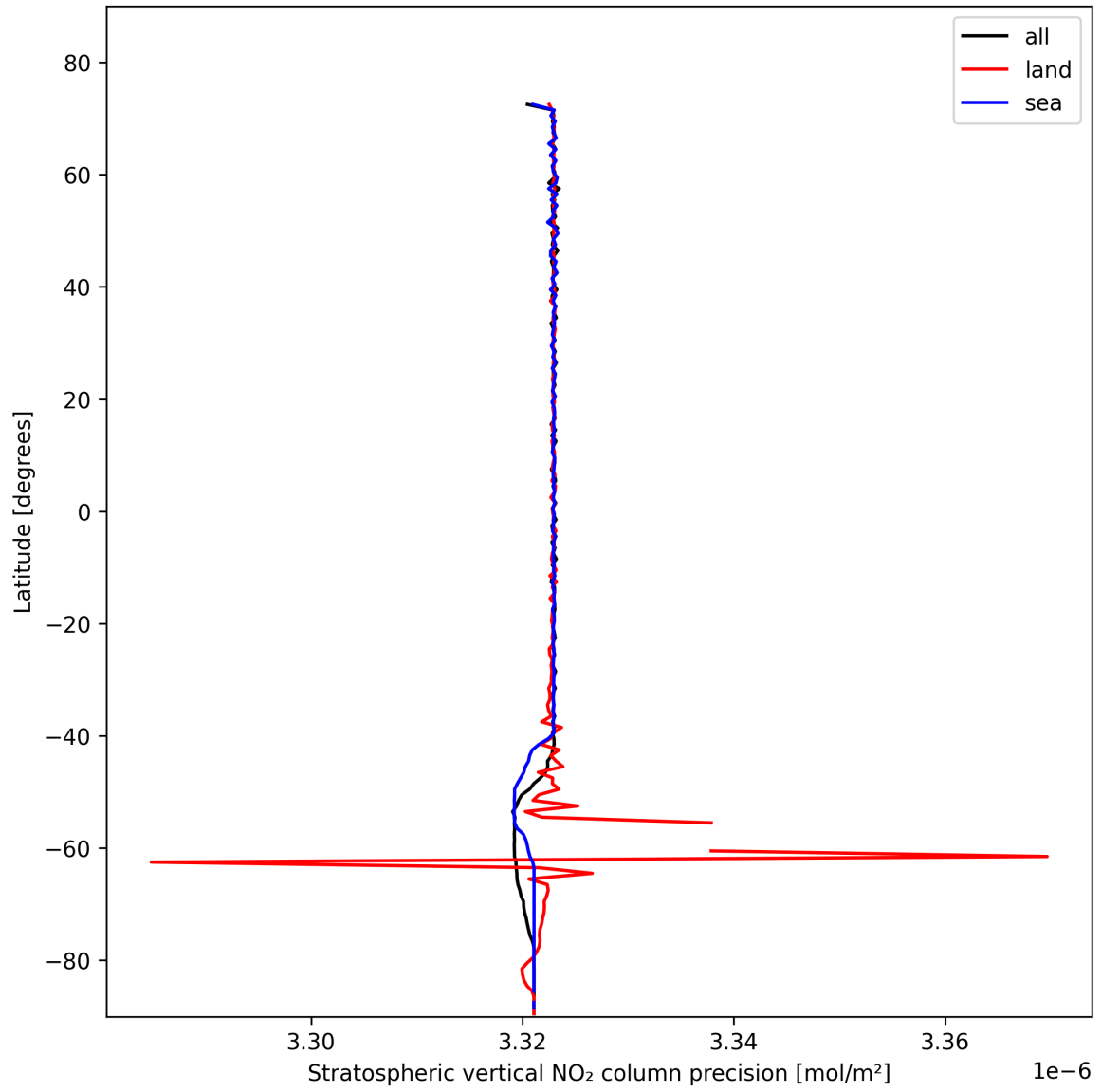
Figure 18: Zonal average of “Stratospheric vertical NO 2 column precision” for 2025-11-03 to 2025-11-04.
