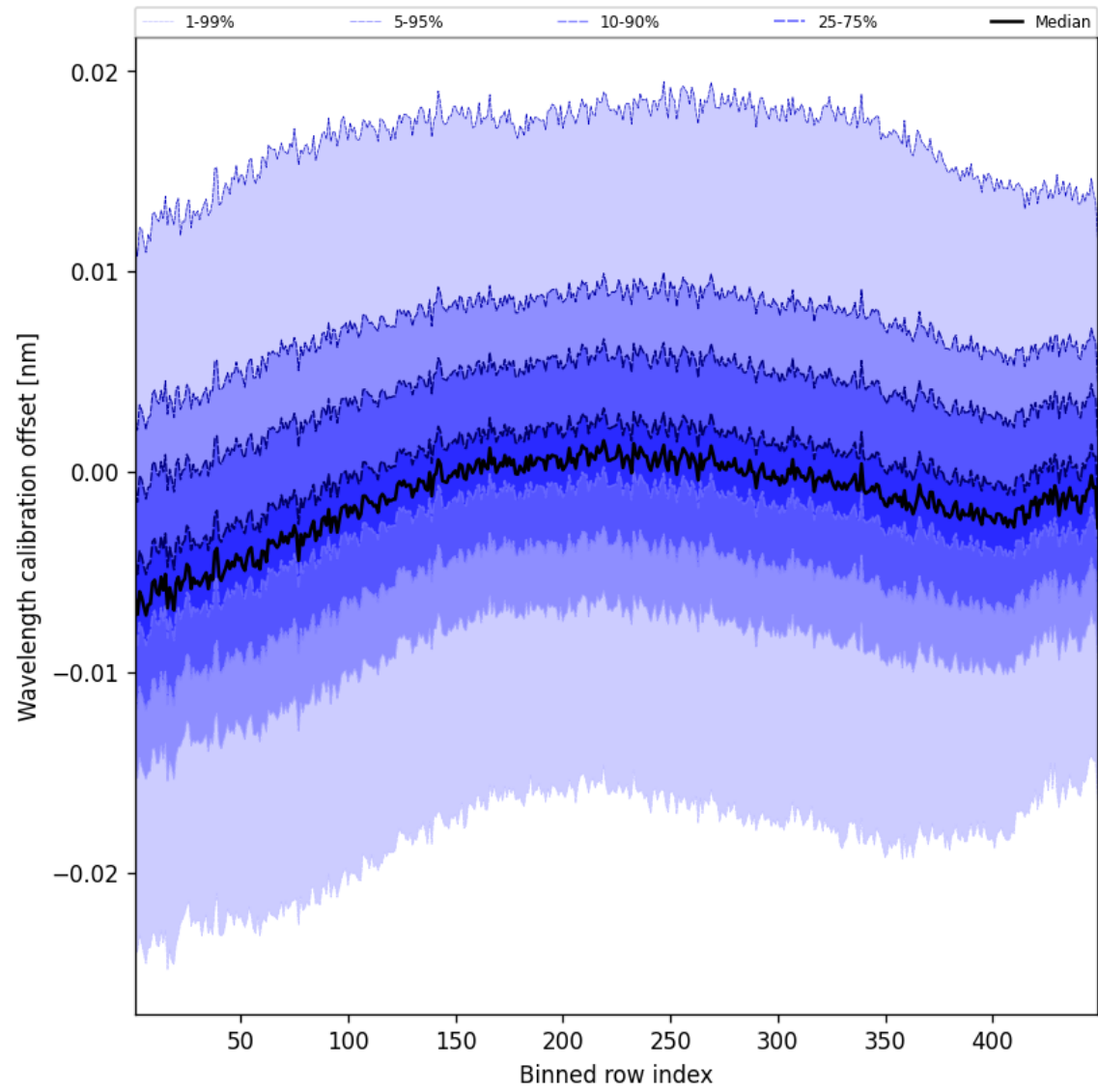
Figure 50: Along track statistics of “Wavelength calibration offset” for 2025-11-03 to 2025-11-04
