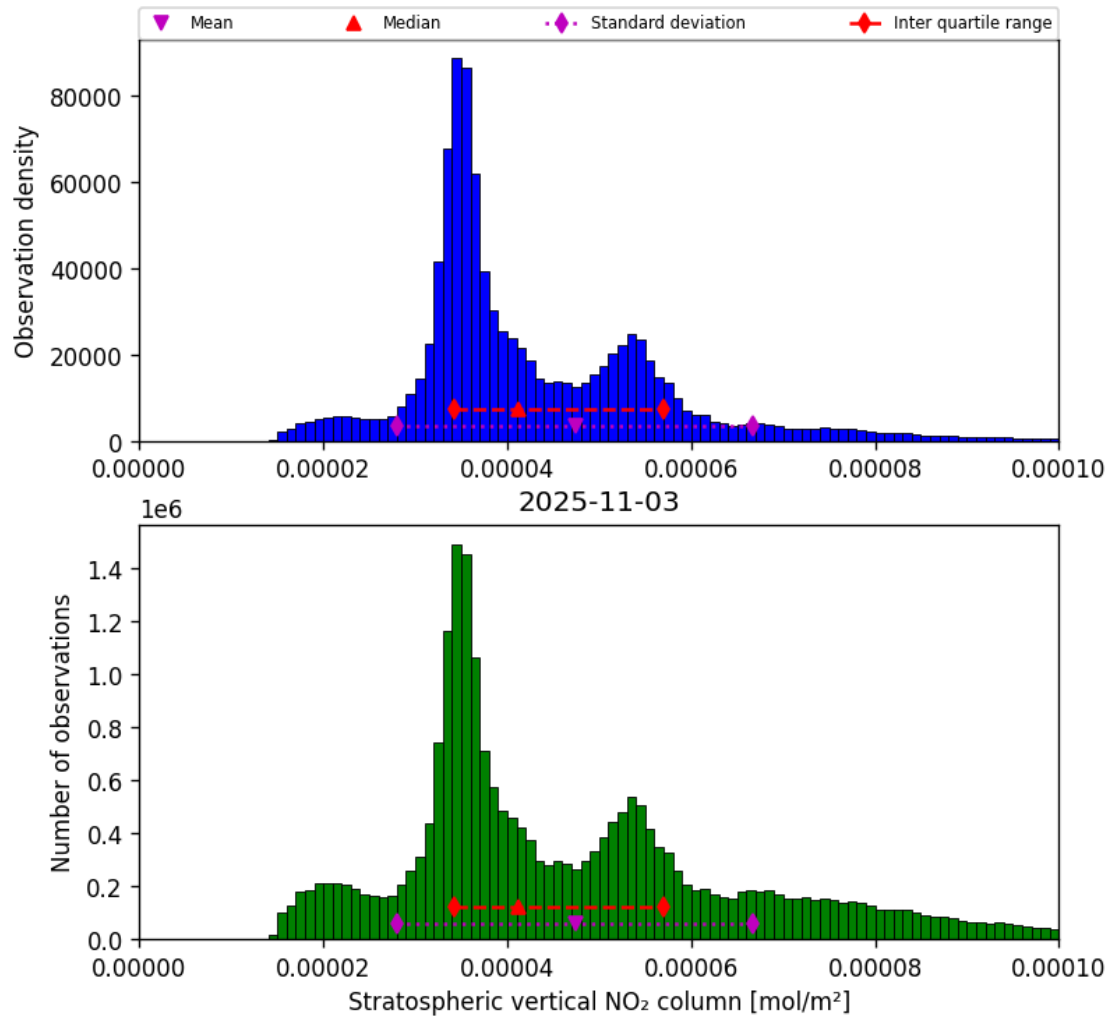
Figure 34: Histogram of “Stratospheric vertical NO 2 column” for 2025-11-03 to 2025-11-04
