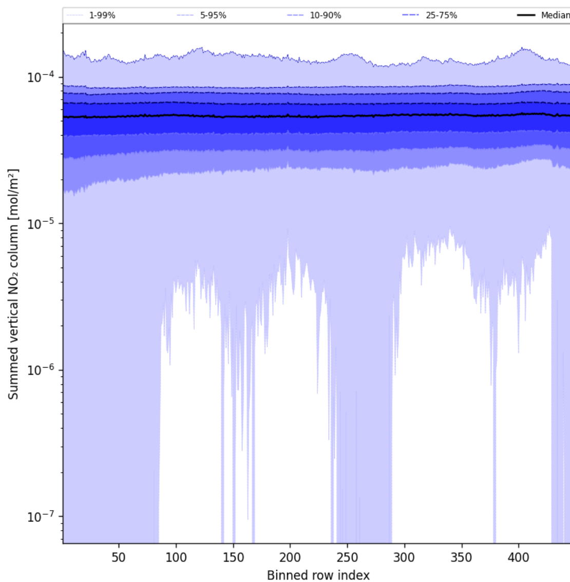
Figure 55: Along track statistics of “Summed vertical NO 2 column” for 2025-11-04 to 2025-11-05
