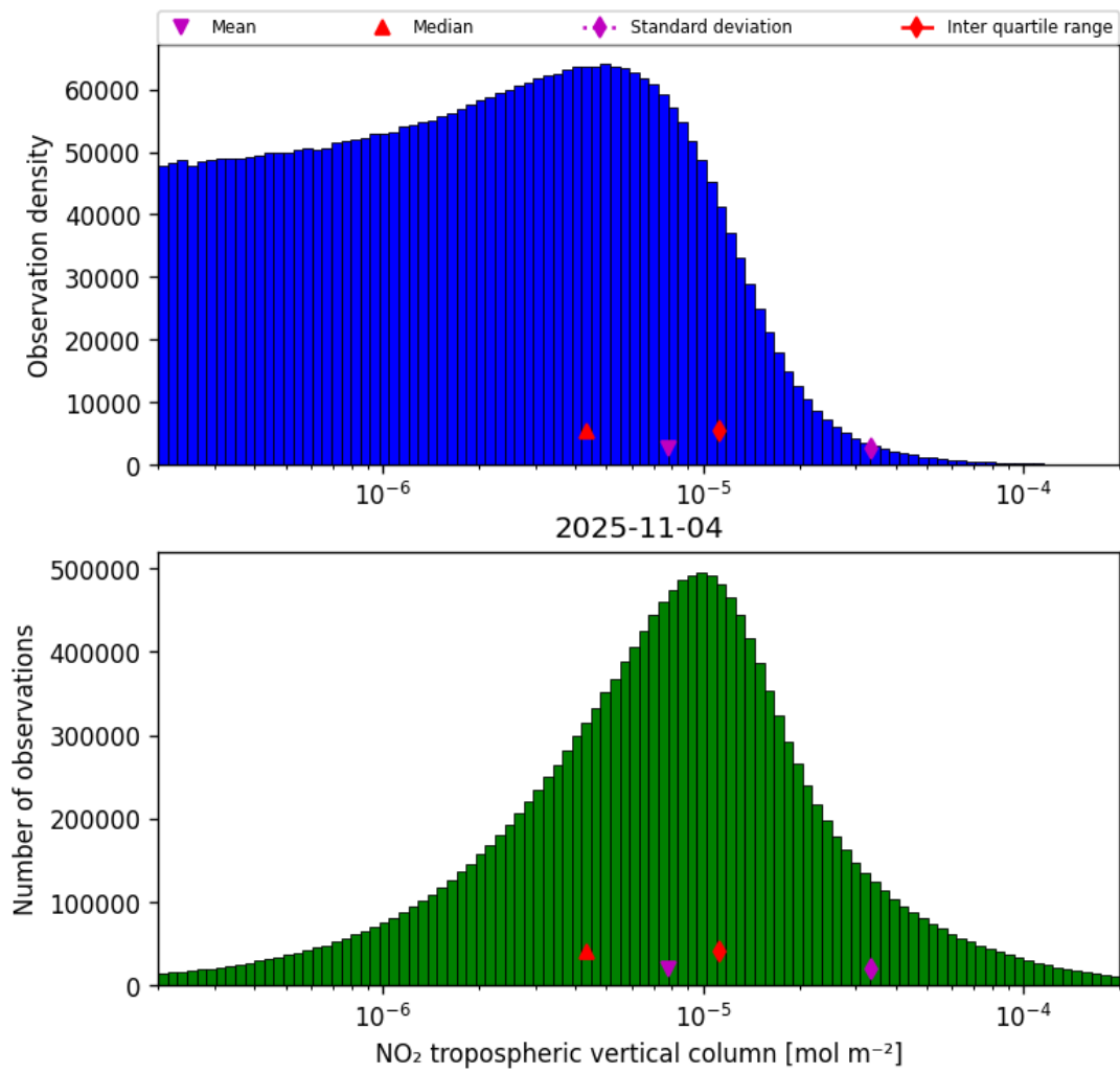
Figure 27: Histogram of “NO 2 tropospheric vertical column” for 2025-11-04 to 2025-11-05
