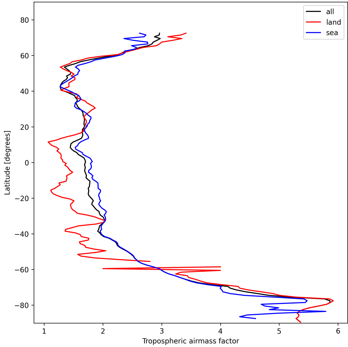
Figure 12: Zonal average of “Tropospheric airmass factor” for 2025-11-04 to 2025-11-05.
