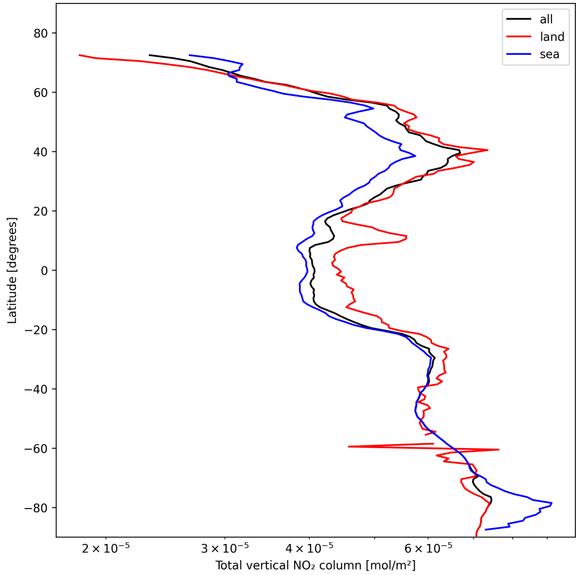
Figure 19: Zonal average of “Total vertical NO 2 column” for 2025-11-04 to 2025-11-05.
