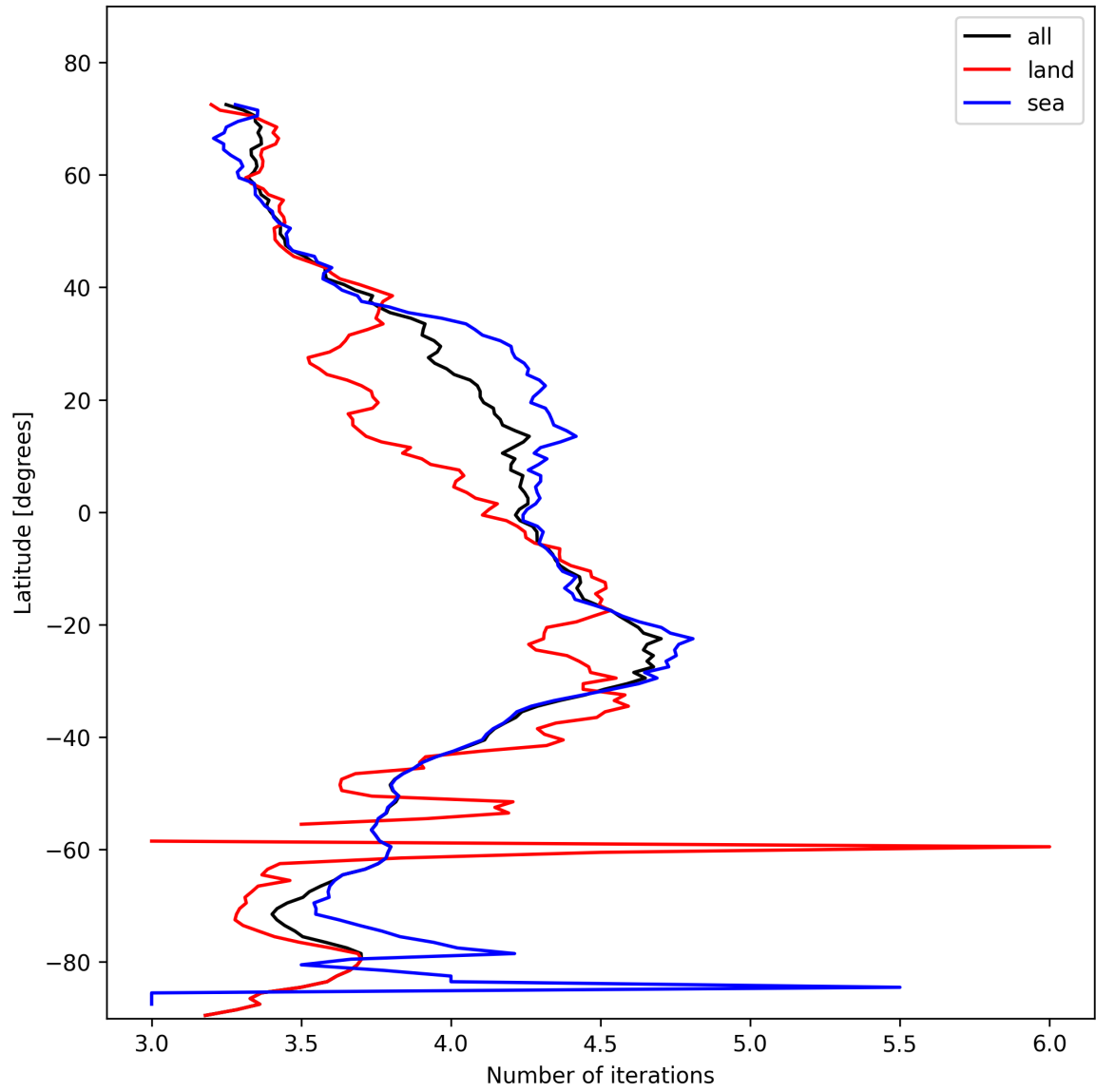
Figure 15: Zonal average of “Number of iterations” for 2025-11-04 to 2025-11-05.
