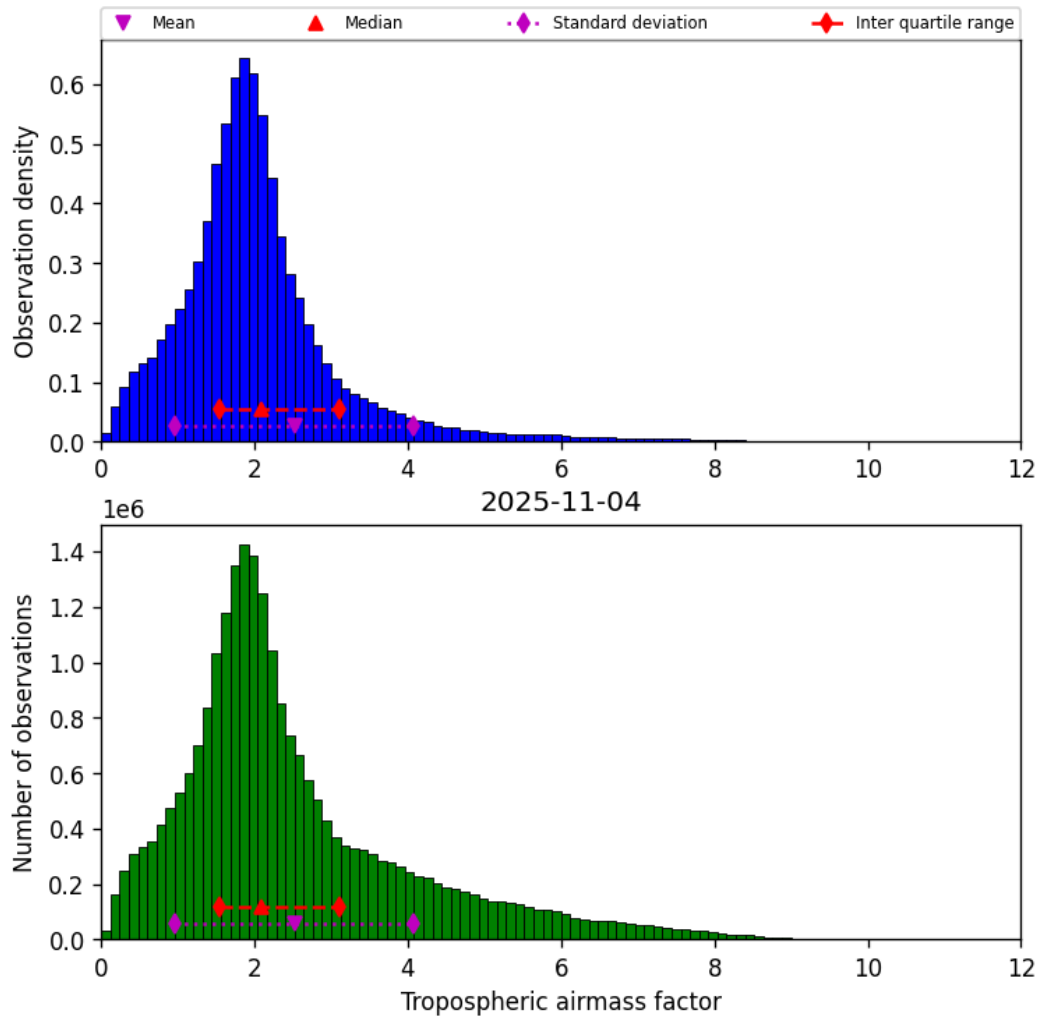
Figure 29: Histogram of “Tropospheric air mass factor” for 2025-11-04 to 2025-11-05
