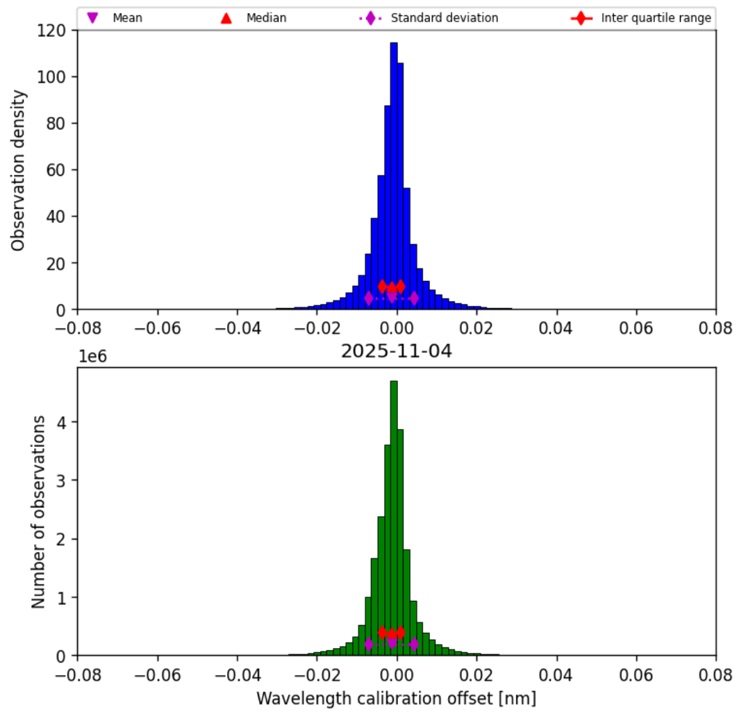
Figure 33: Histogram of “Wavelength calibration offset” for 2025-11-04 to 2025-11-05
