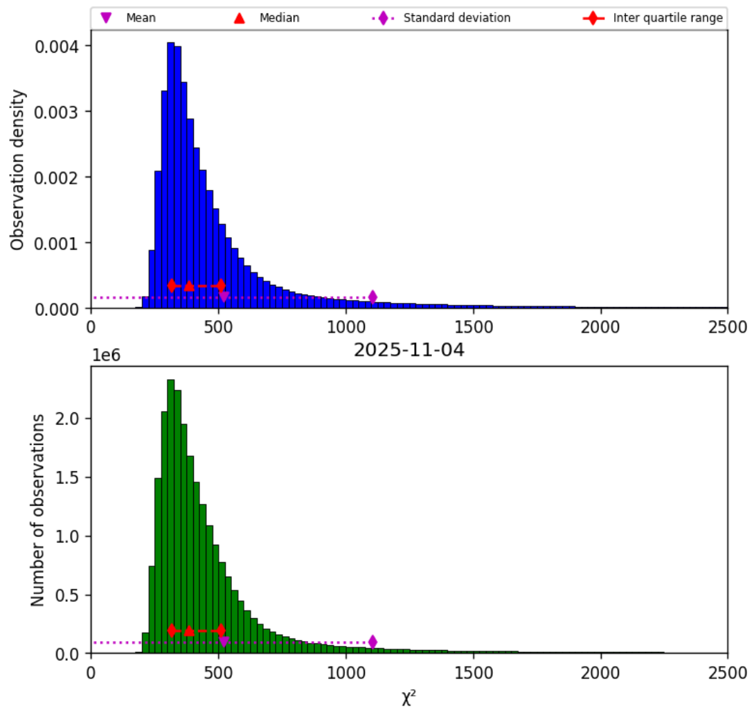
Figure 40: Histogram of “ \chi^2 ” for 2025-11-04 to 2025-11-05
