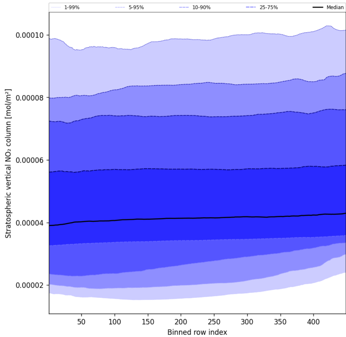
Figure 51: Along track statistics of “Stratospheric vertical NO 2 column” for 2025-11-04 to 2025-11-05
