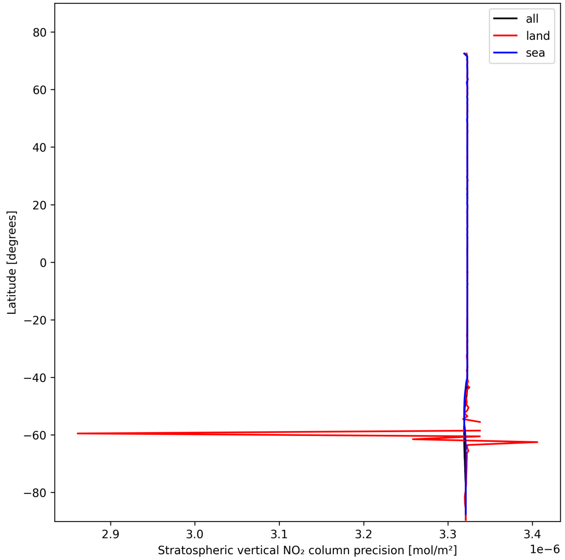
Figure 18: Zonal average of “Stratospheric vertical NO 2 column precision” for 2025-11-04 to 2025-11-05.
