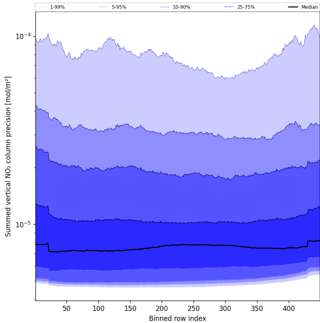
Figure 56: Along track statistics of “Summed vertical NO 2 column precision” for 2025-11-04 to 2025-11-05
