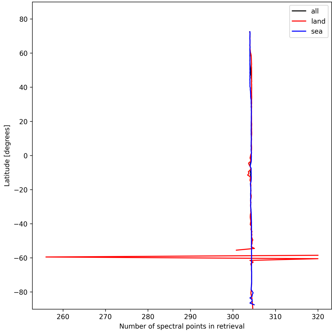
Figure 14: Zonal average of “Number of spectral points in retrieval” for 2025-11-04 to 2025-11-05.
