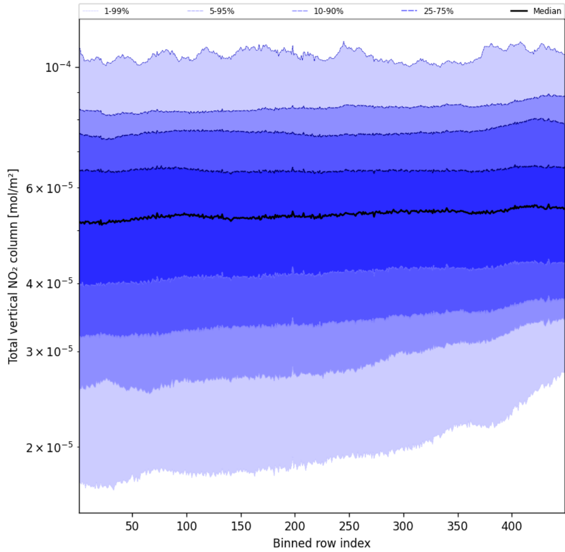
Figure 53: Along track statistics of “Total vertical NO 2 column” for 2025-11-04 to 2025-11-05
