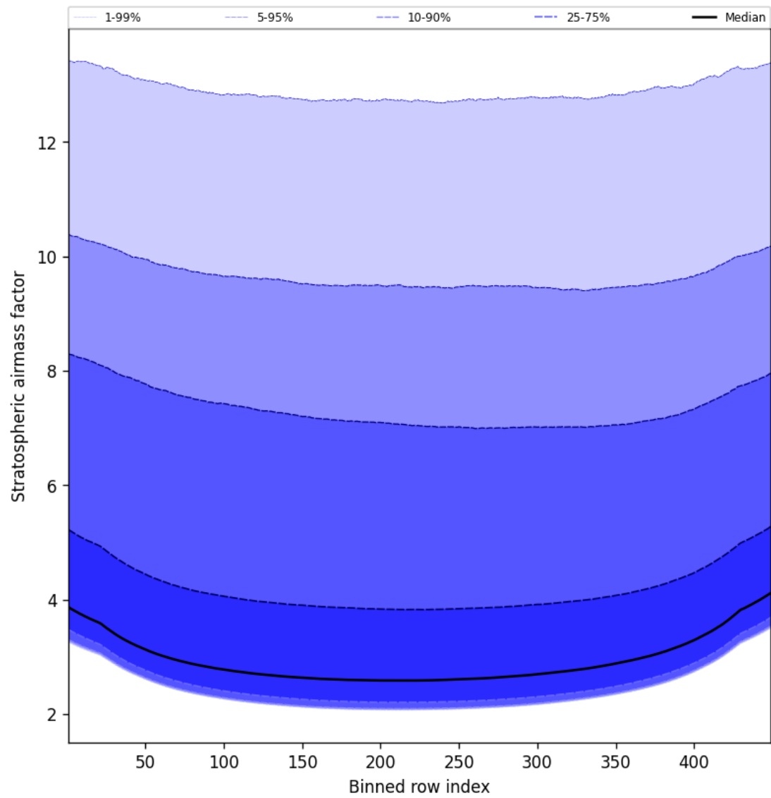
Figure 59: Along track statistics of “Stratospheric air mass factor” for 2025-11-04 to 2025-11-05
