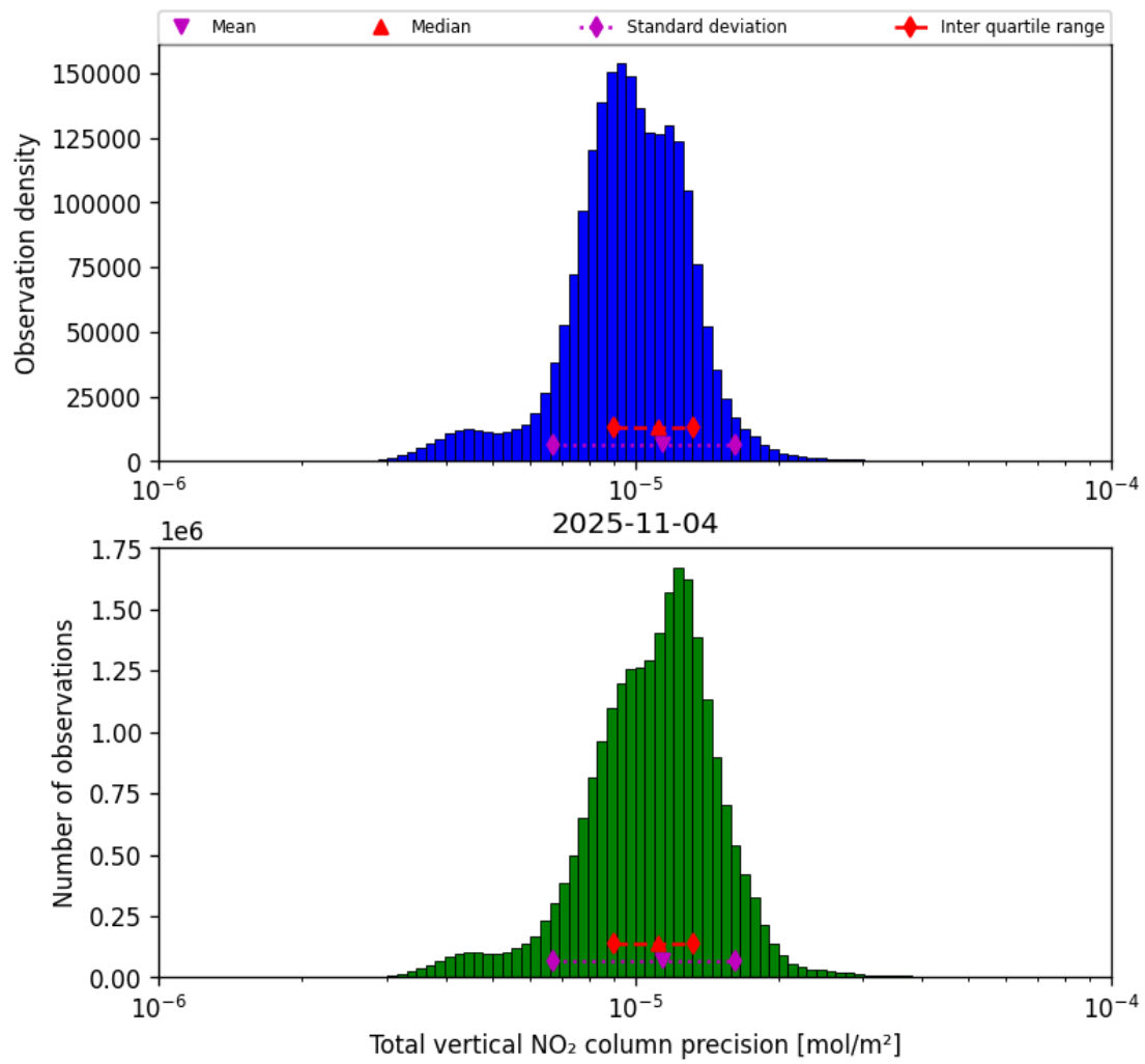
Figure 37: Histogram of “Total vertical NO 2 column precision” for 2025-11-04 to 2025-11-05
