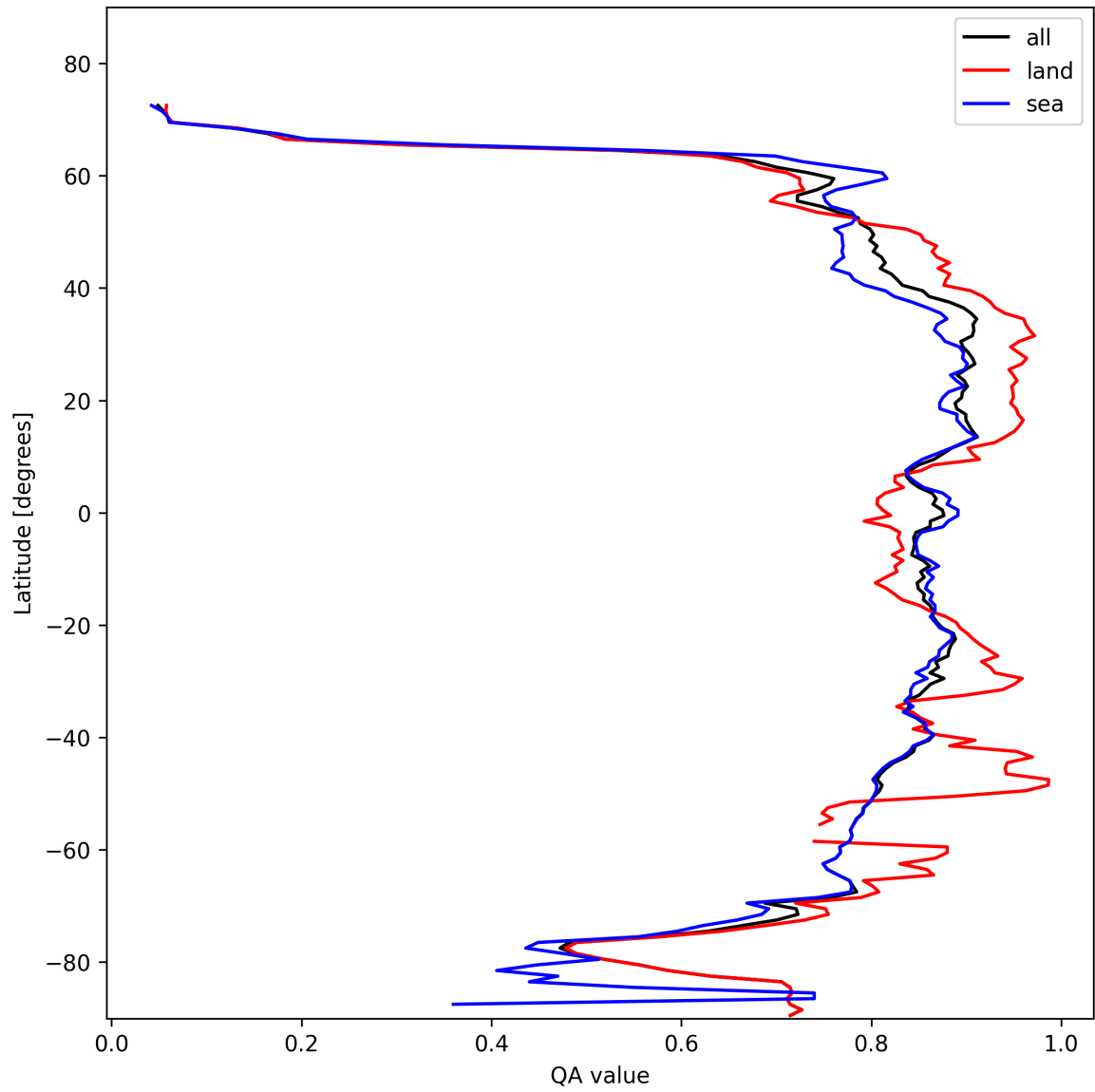
Figure 9: Zonal average of “QA value” for 2025-11-04 to 2025-11-05.
