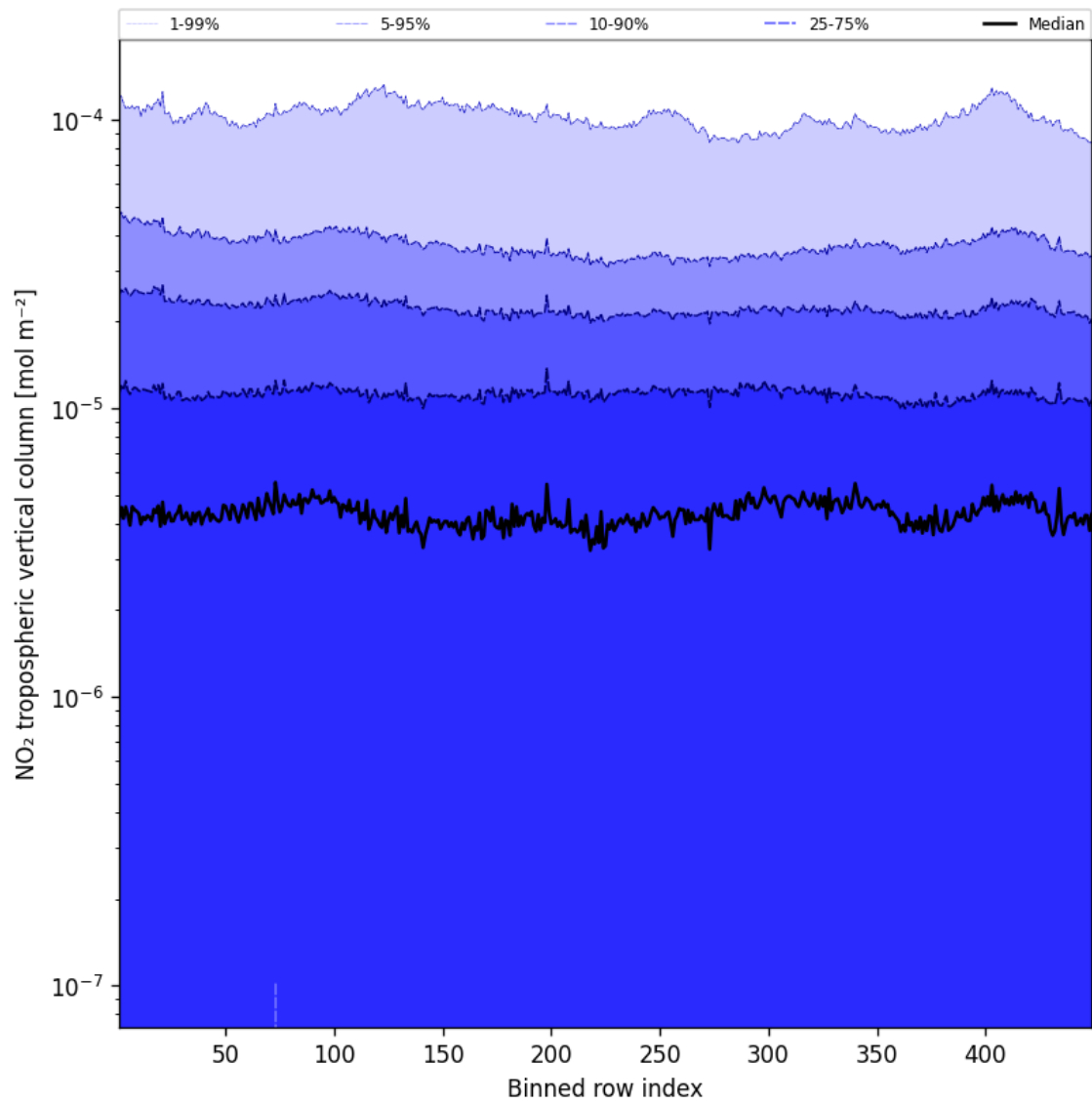
Figure 44: Along track statistics of “NO 2 tropospheric vertical column” for 2025-11-04 to 2025-11-05
