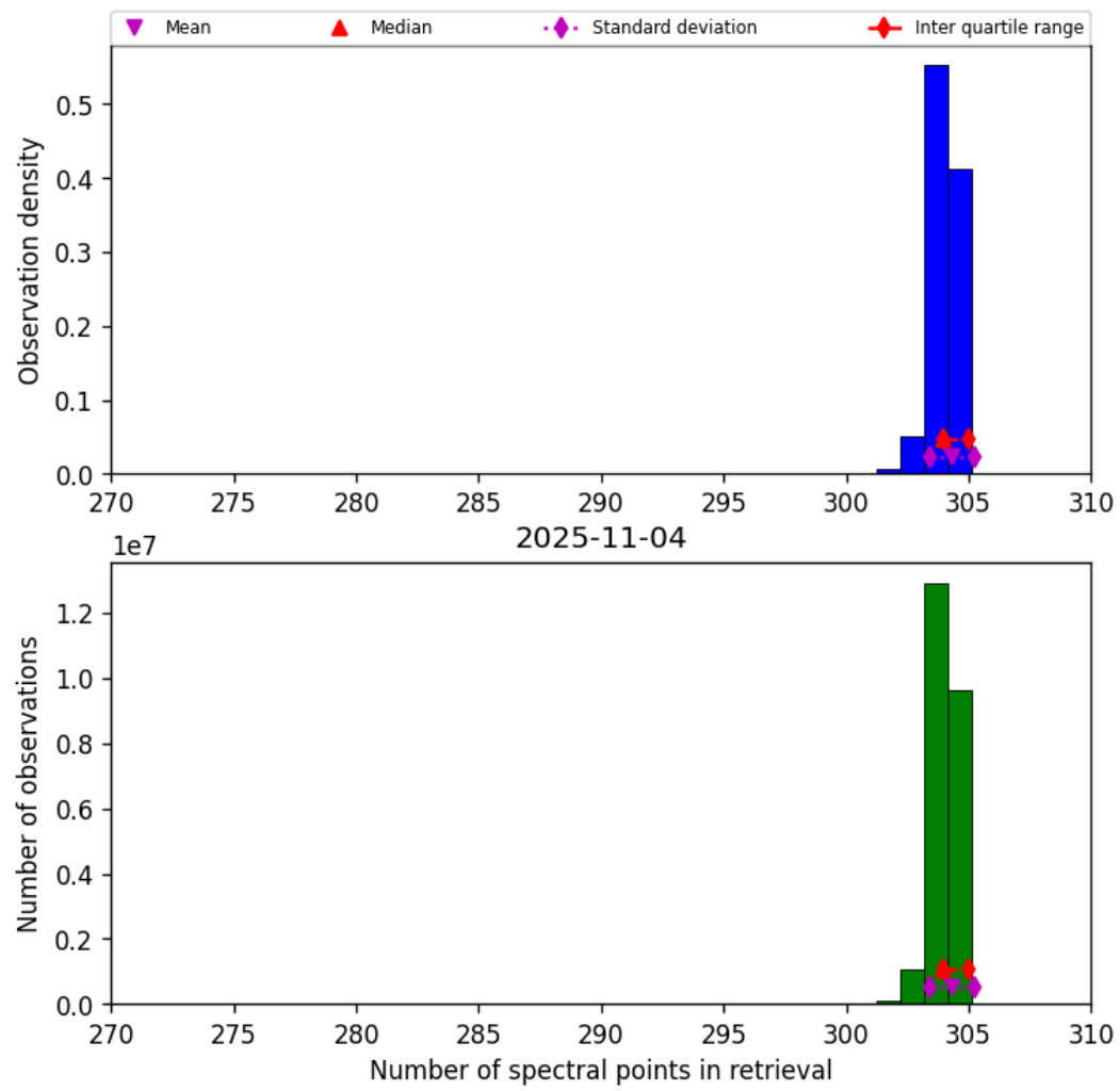
Figure 31: Histogram of “Number of spectral points in retrieval” for 2025-11-04 to 2025-11-05
