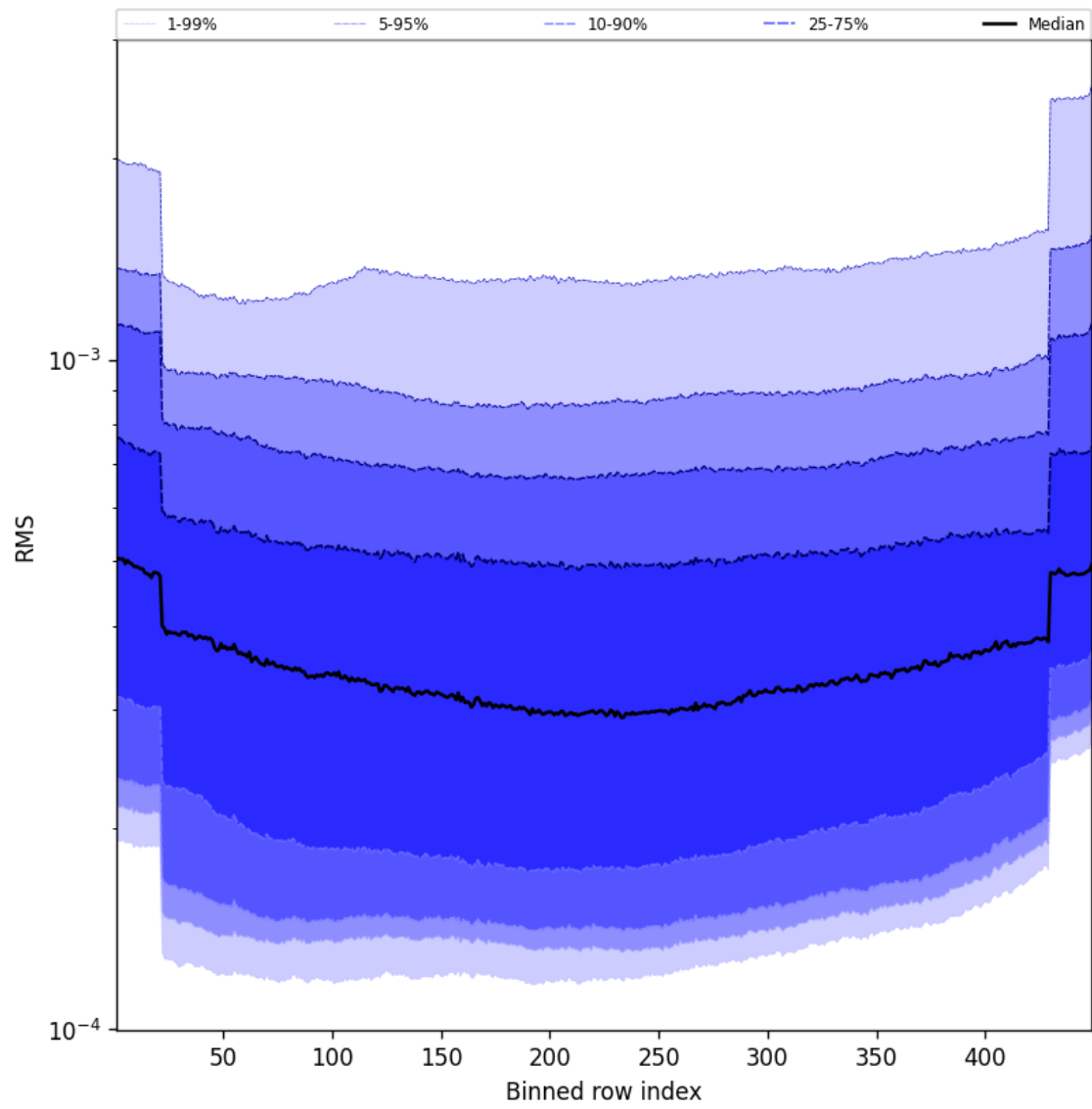
Figure 58: Along track statistics of “RMS” for 2025-11-04 to 2025-11-05
