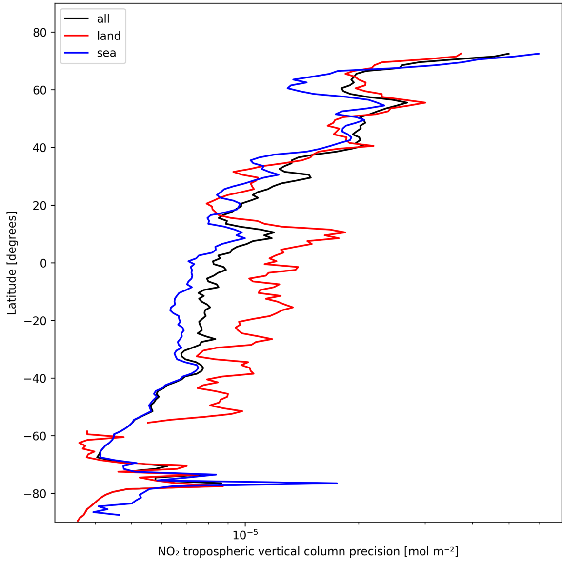
Figure 11: Zonal average of “NO 2 tropospheric vertical column precision” for 2025-11-04 to 2025-11-05.
