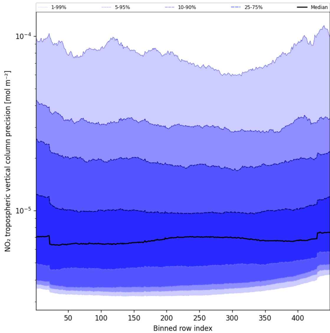
Figure 45: Along track statistics of “NO 2 tropospheric vertical column precision” for 2025-11-04 to 2025-11-05
