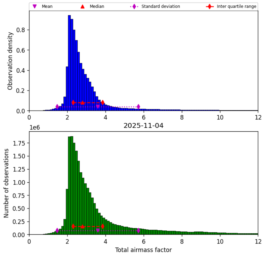
Figure 30: Histogram of “Total airmass factor” for 2025-11-04 to 2025-11-05
