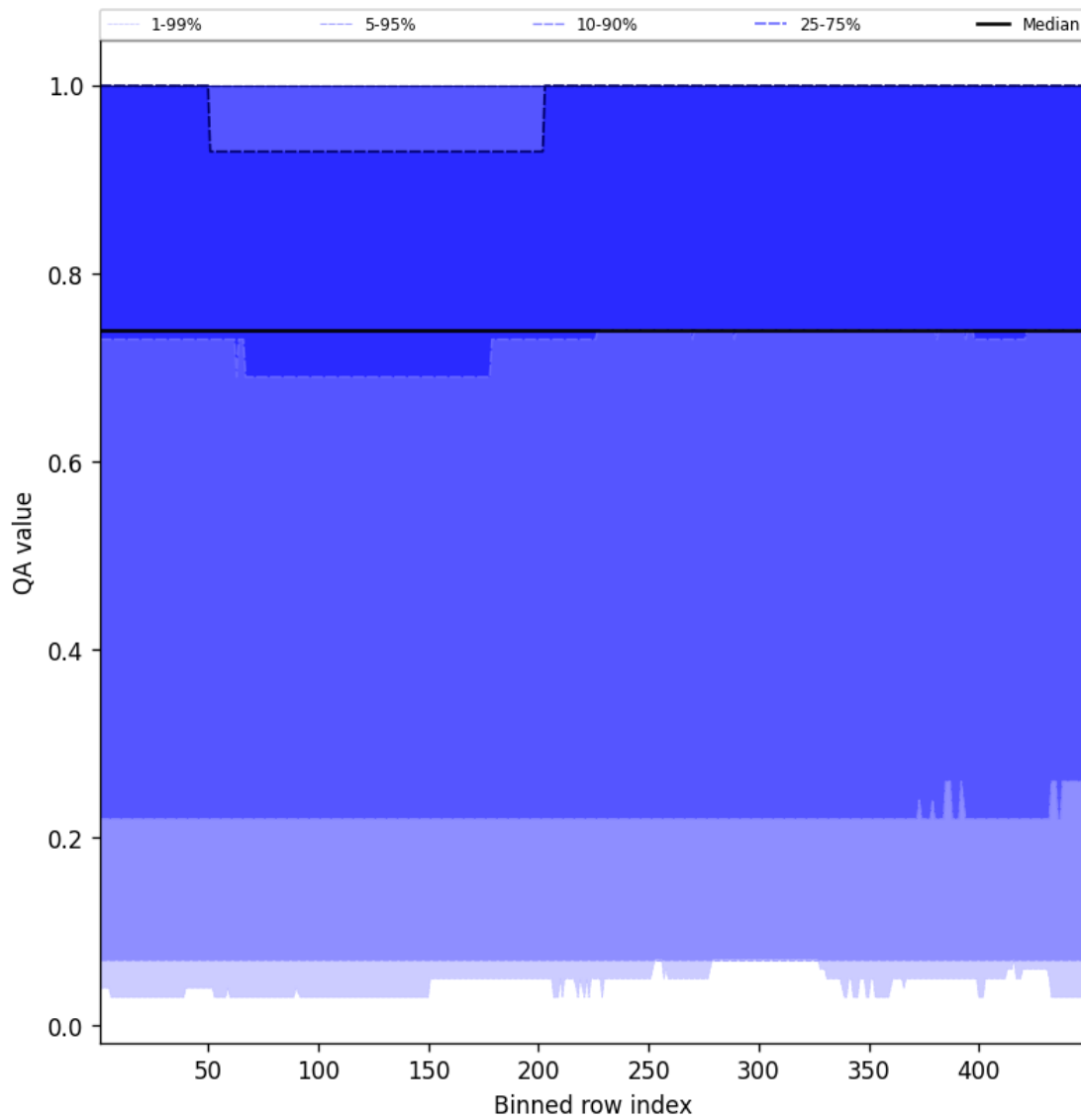
Figure 43: Along track statistics of “QA value” for 2025-11-04 to 2025-11-05
