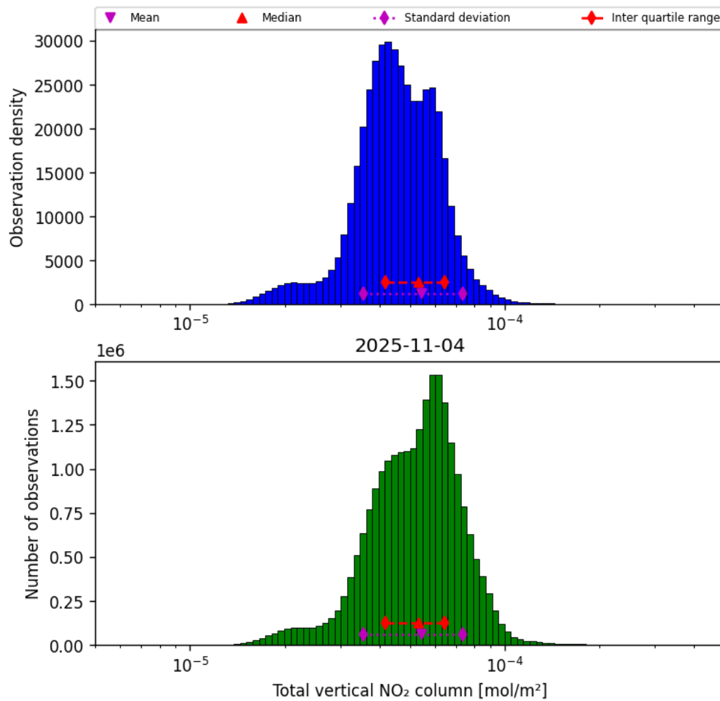
Figure 36: Histogram of “Total vertical NO 2 column” for 2025-11-04 to 2025-11-05
