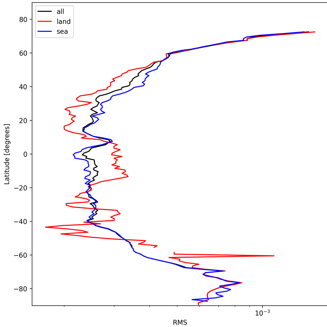
Figure 24: Zonal average of “RMS” for 2025-11-04 to 2025-11-05.
