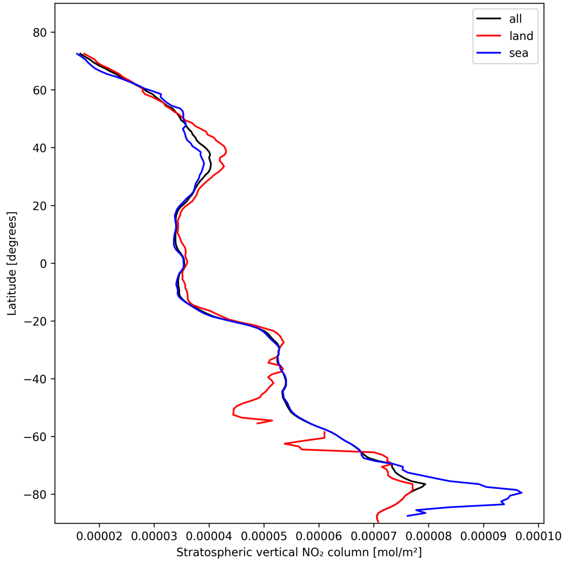
Figure 17: Zonal average of “Stratospheric vertical NO 2 column” for 2025-11-04 to 2025-11-05.
