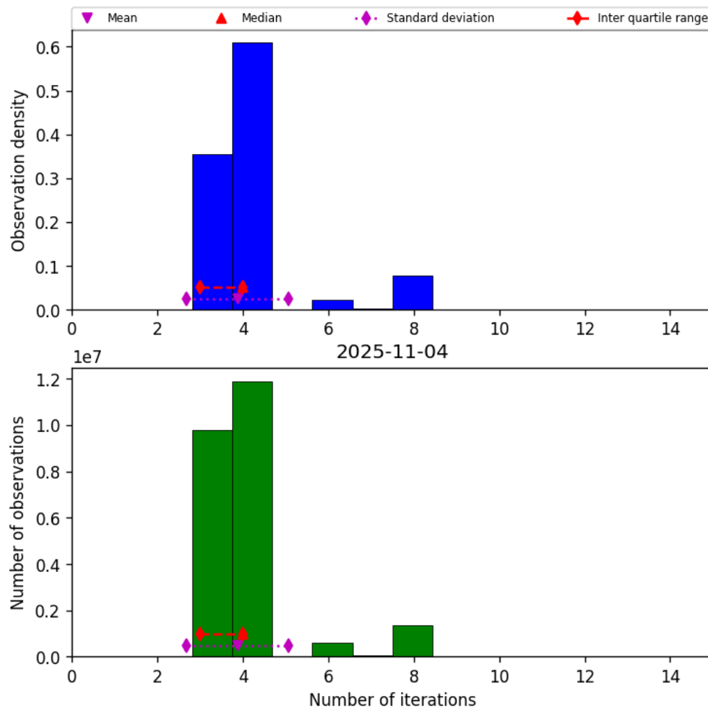
Figure 32: Histogram of “Number of iterations” for 2025-11-04 to 2025-11-05
