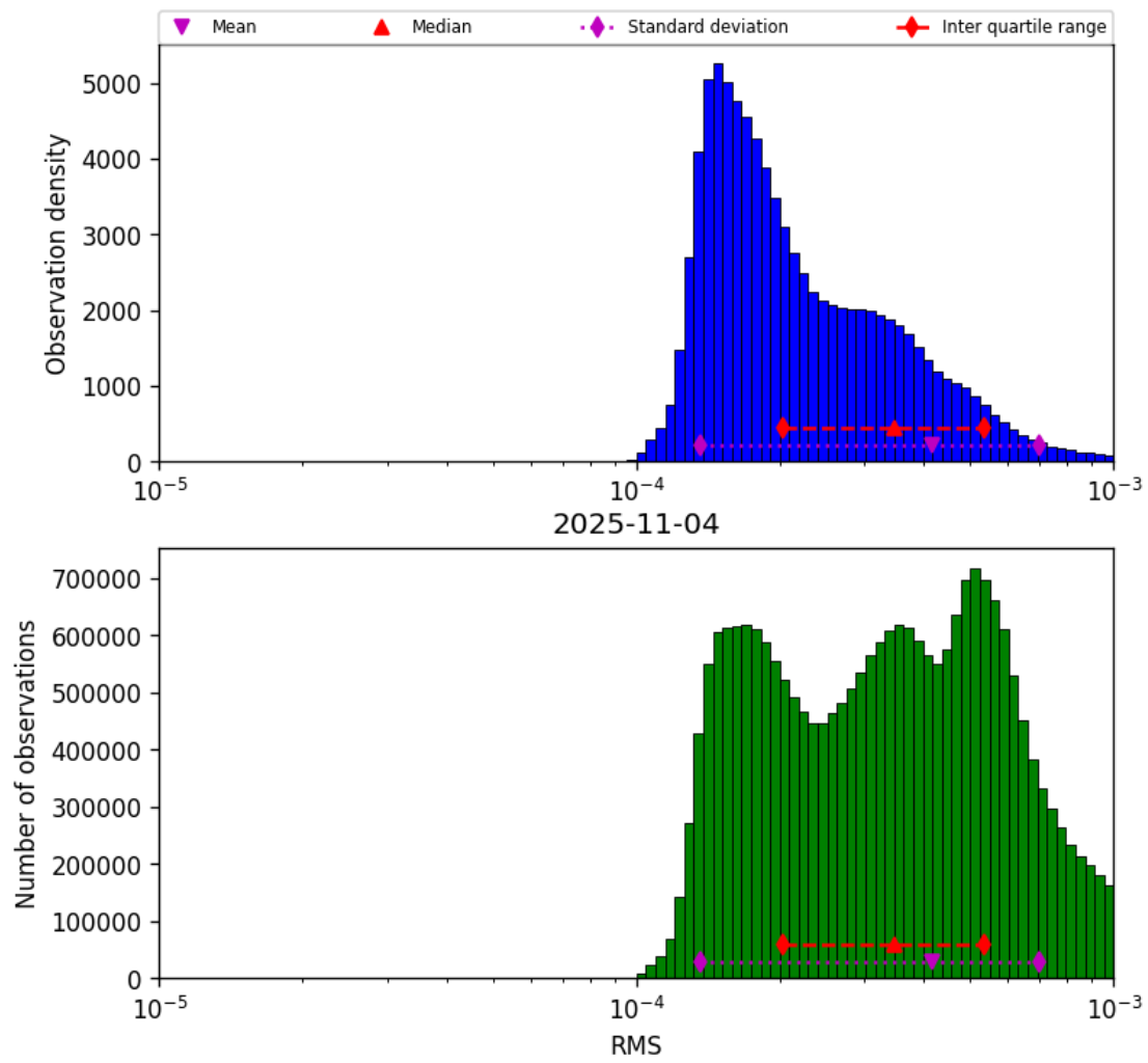
Figure 41: Histogram of “RMS” for 2025-11-04 to 2025-11-05
