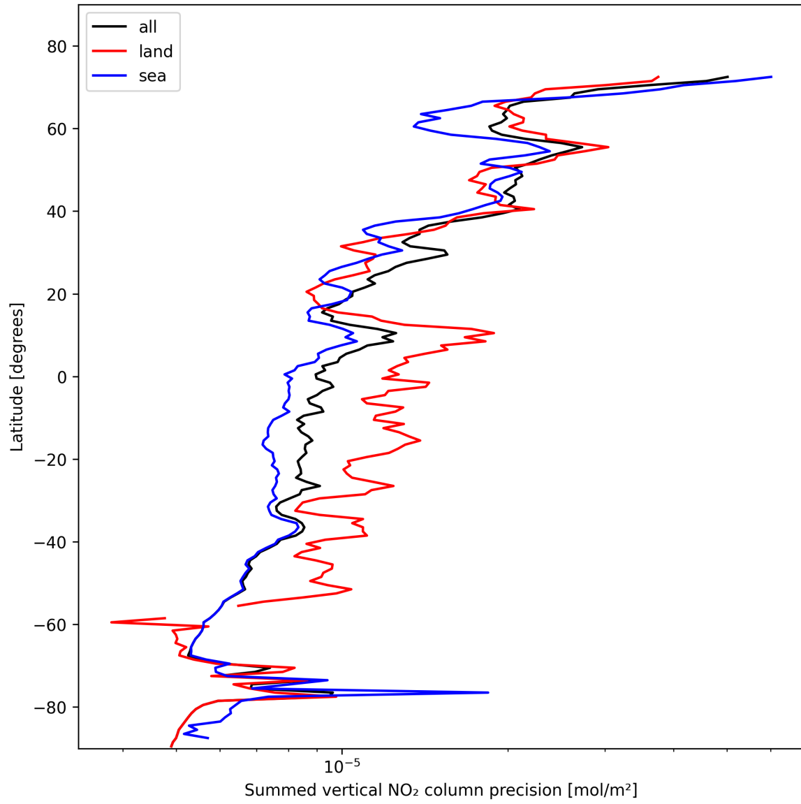
Figure 22: Zonal average of “Summed vertical NO 2 column precision” for 2025-11-04 to 2025-11-05.
