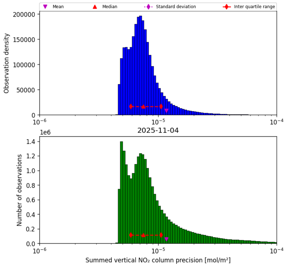
Figure 39: Histogram of "Summed vertical NO 2 column precision" for 2025-11-04 to 2025-11-05
