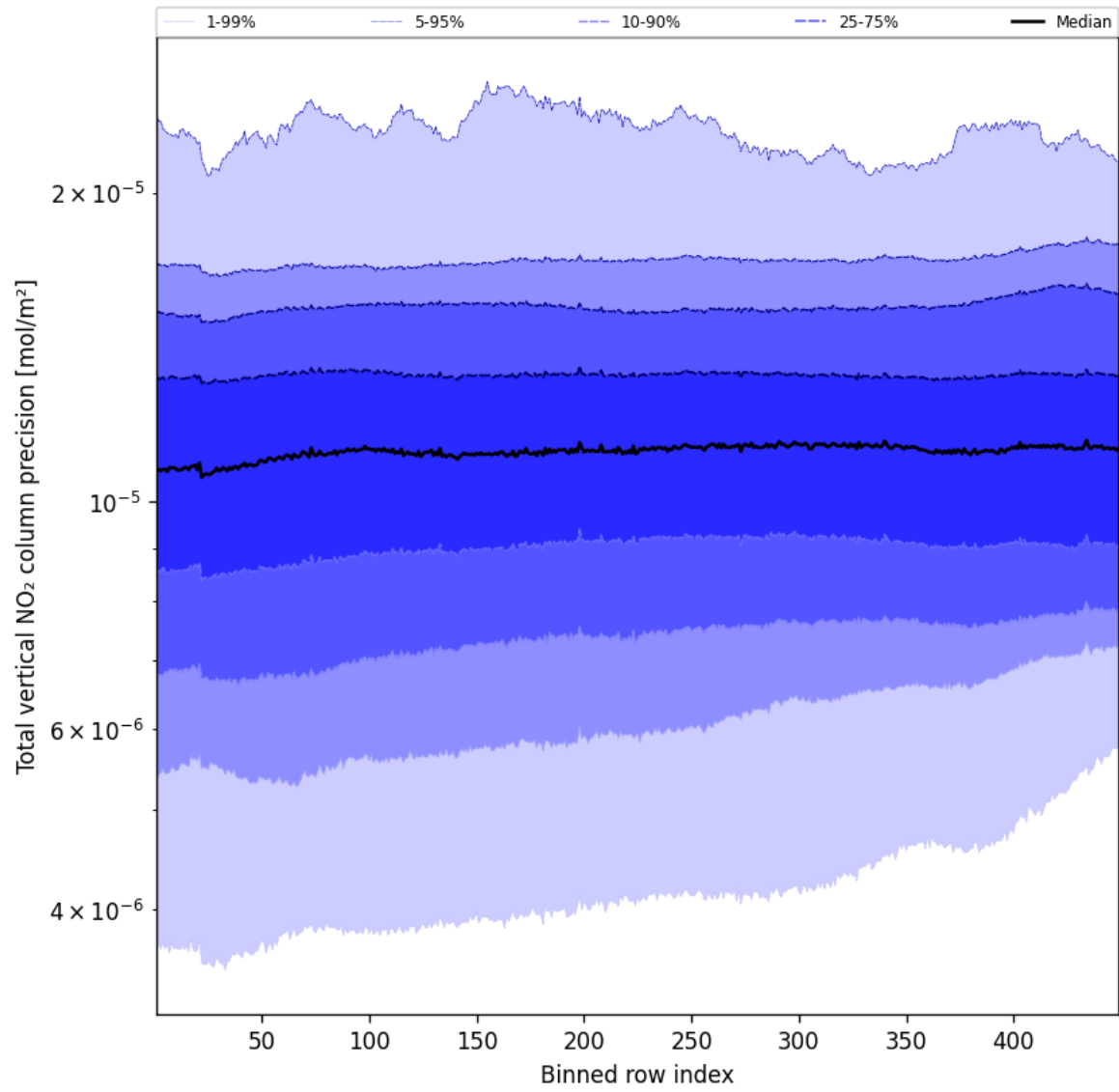
Figure 54: Along track statistics of “Total vertical NO 2 column precision” for 2025-11-04 to 2025-11-05
