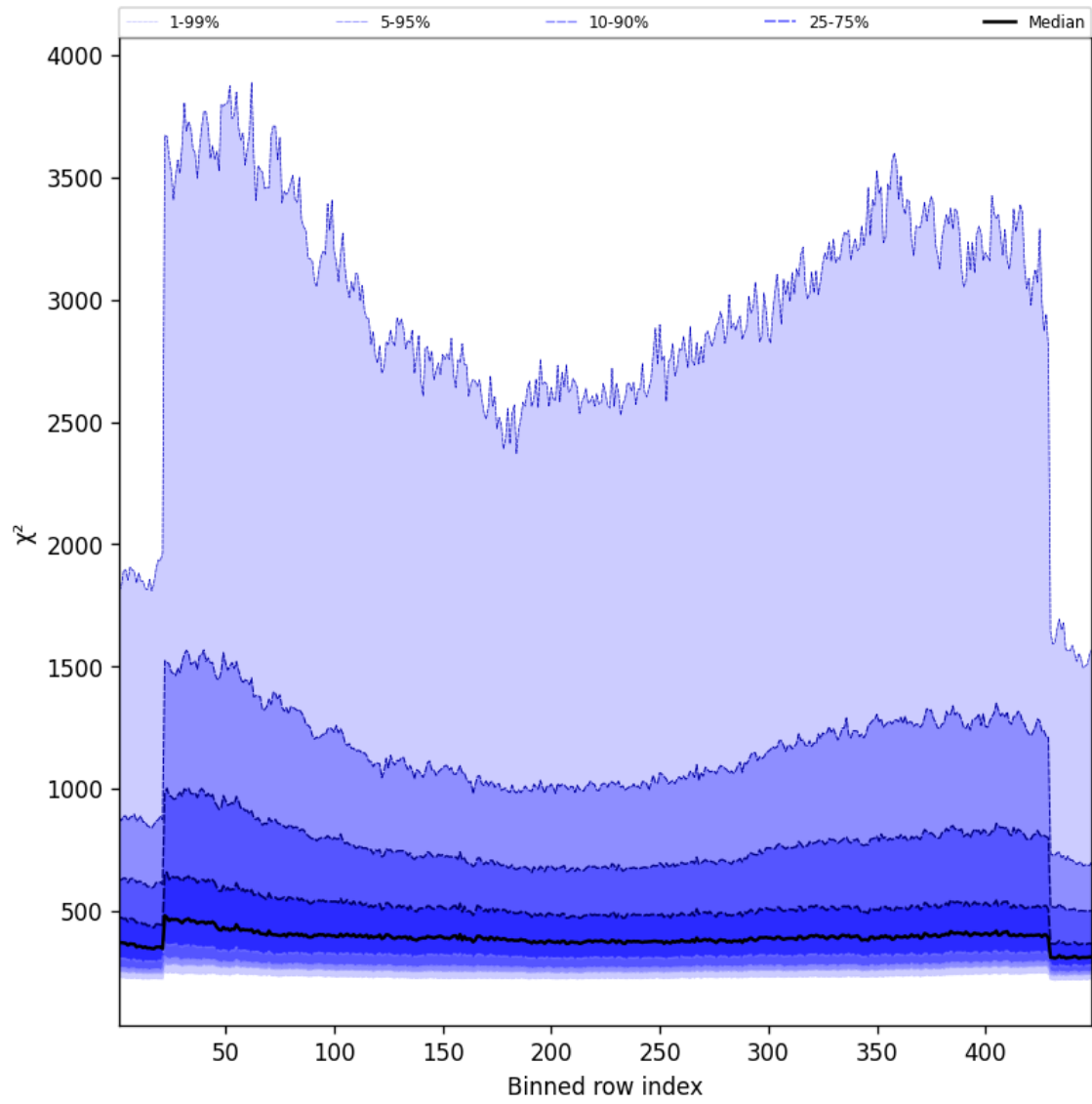
Figure 57: Along track statistics of “ \chi^2 ” for 2025-11-04 to 2025-11-05
