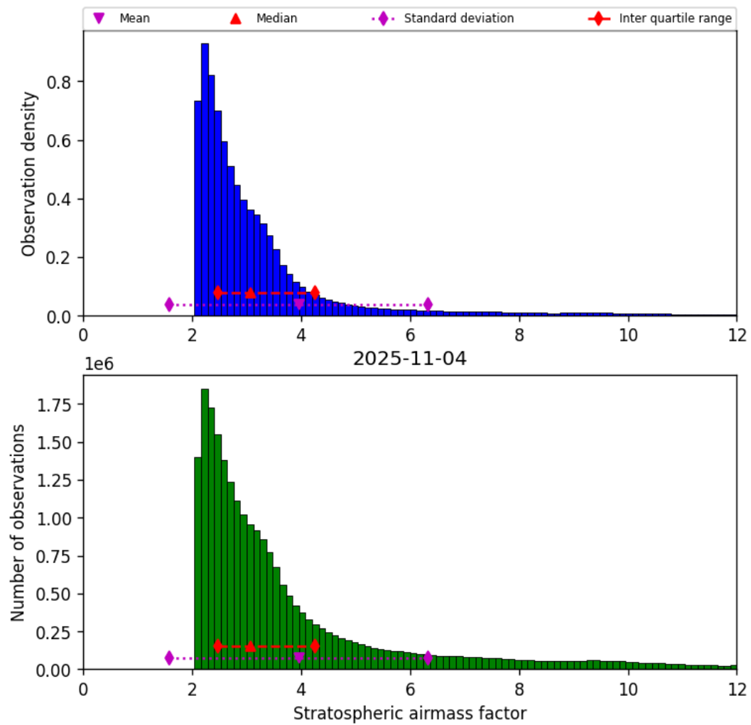
Figure 42: Histogram of “Stratospheric airmass factor” for 2025-11-04 to 2025-11-05
