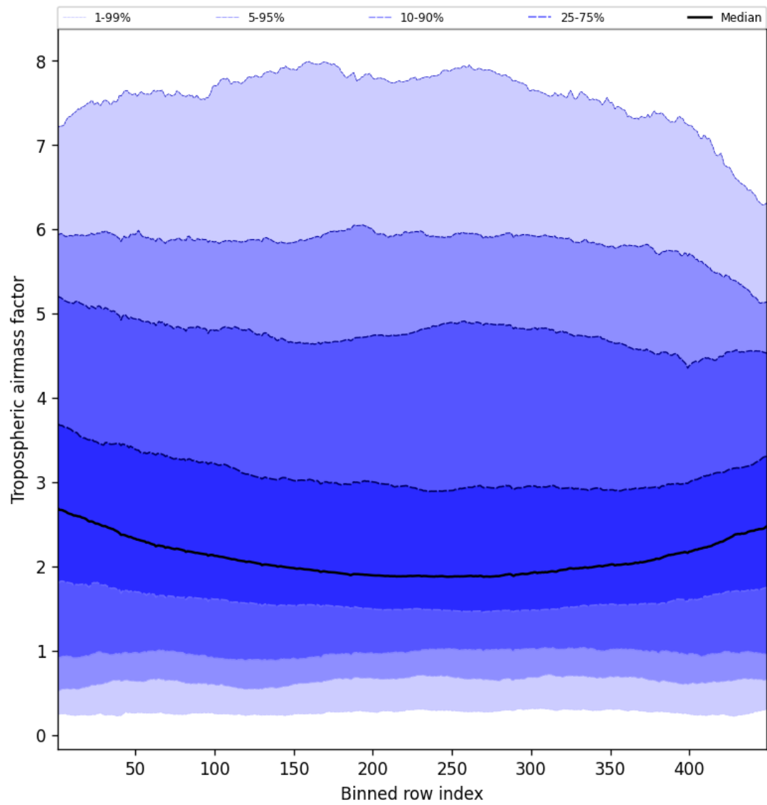
Figure 46: Along track statistics of “Tropospheric air mass factor” for 2025-11-04 to 2025-11-05
