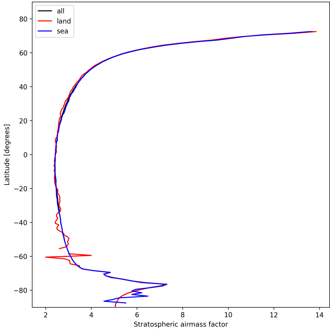
Figure 25: Zonal average of “Stratospheric air mass factor” for 2025-11-04 to 2025-11-05.
