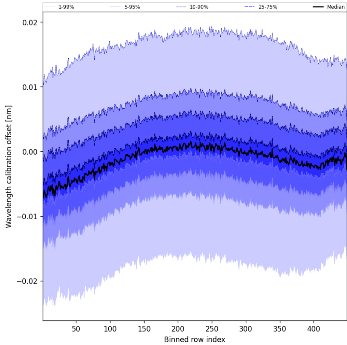
Figure 50: Along track statistics of “Wavelength calibration offset” for 2025-11-04 to 2025-11-05
