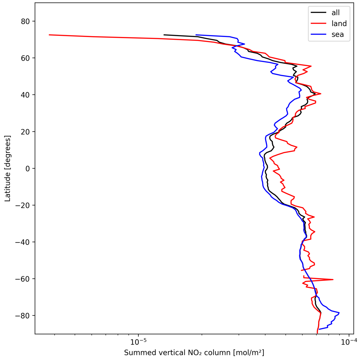
Figure 21: Zonal average of “Summed vertical NO 2 column” for 2025-11-04 to 2025-11-05.
