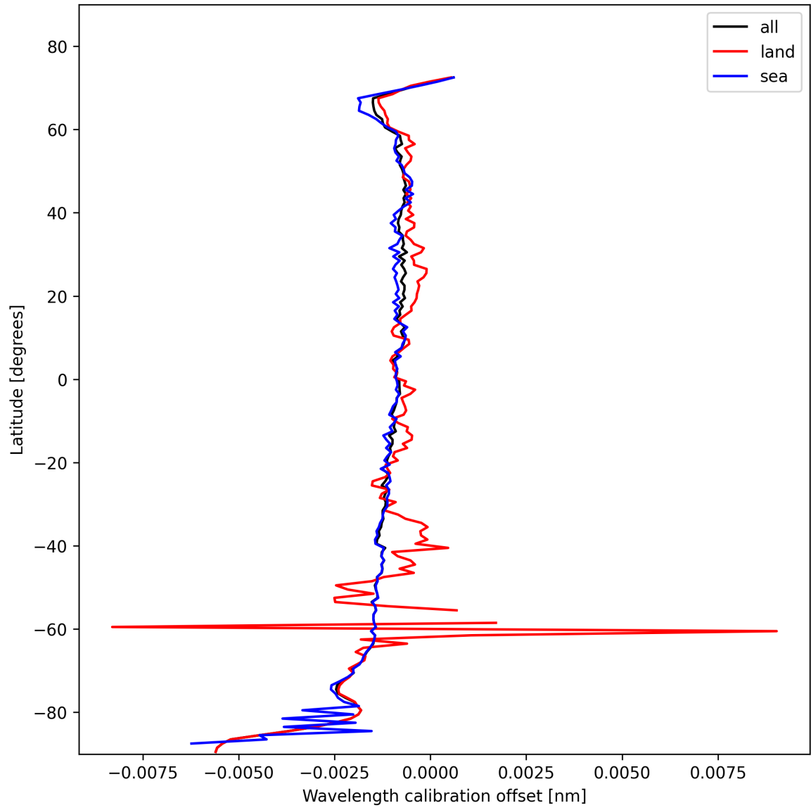
Figure 16: Zonal average of “Wavelength calibration offset” for 2025-11-04 to 2025-11-05.
