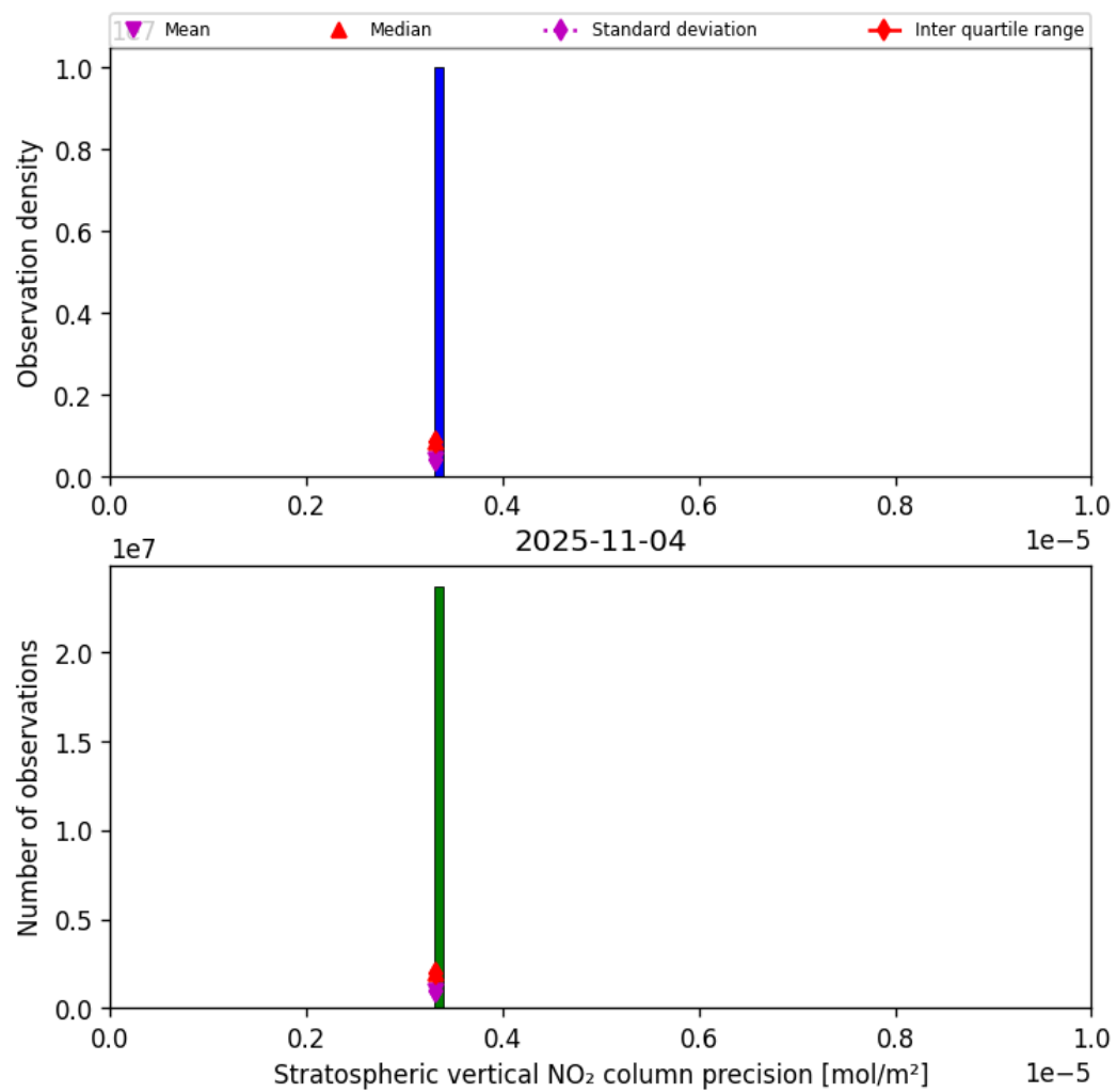
Figure 35: Histogram of “Stratospheric vertical NO 2 column precision” for 2025-11-04 to 2025-11-05
