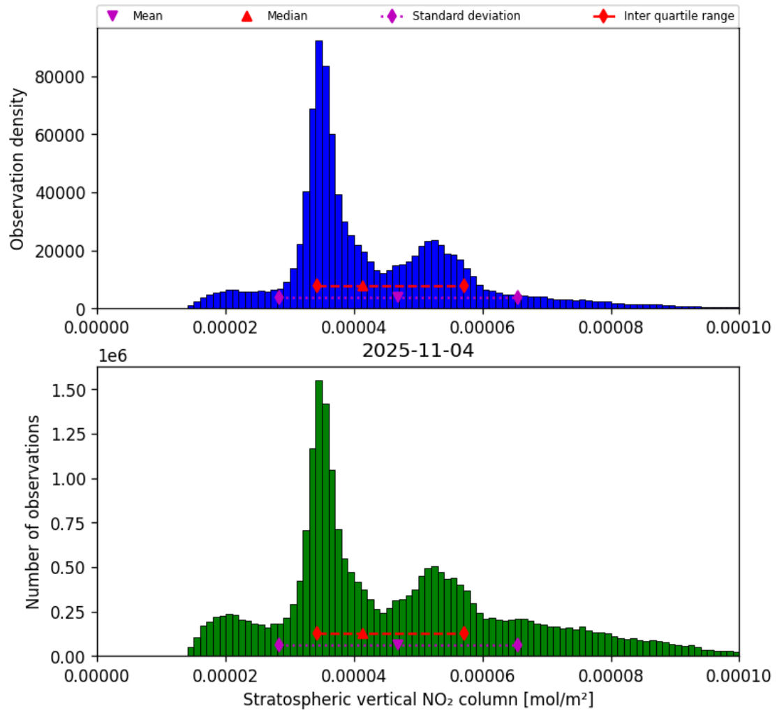
Figure 34: Histogram of “Stratospheric vertical NO 2 column” for 2025-11-04 to 2025-11-05
