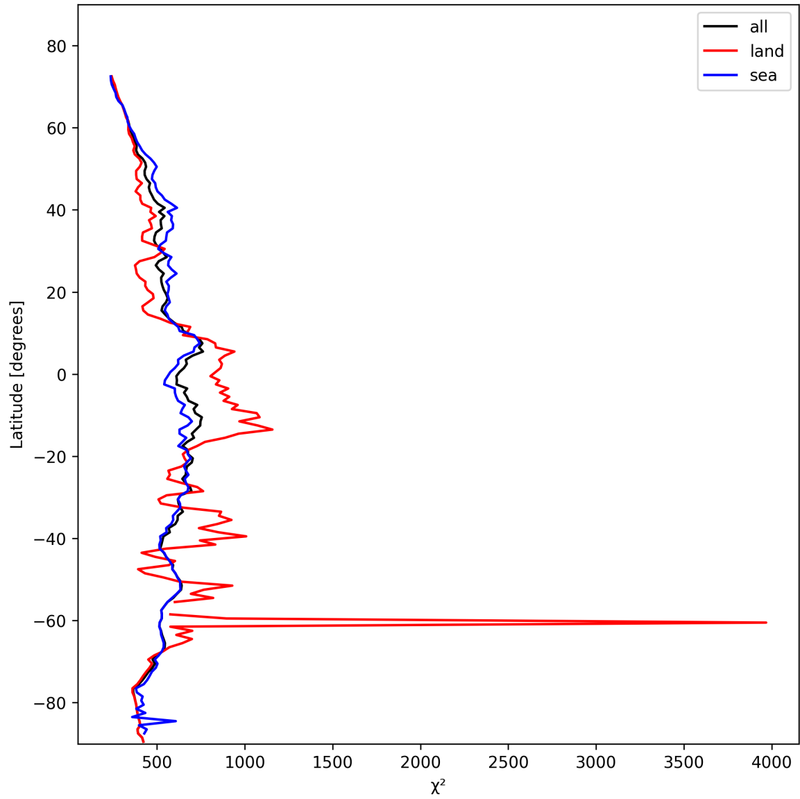
Figure 23: Zonal average of “ \chi^2 ” for 2025-11-04 to 2025-11-05.
