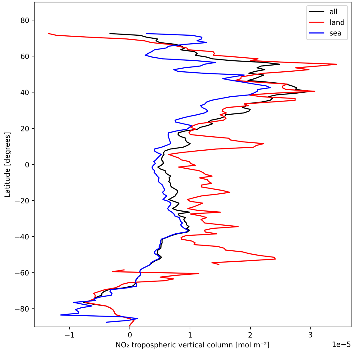
Figure 10: Zonal average of “NO 2 tropospheric vertical column” for 2025-11-04 to 2025-11-05.
