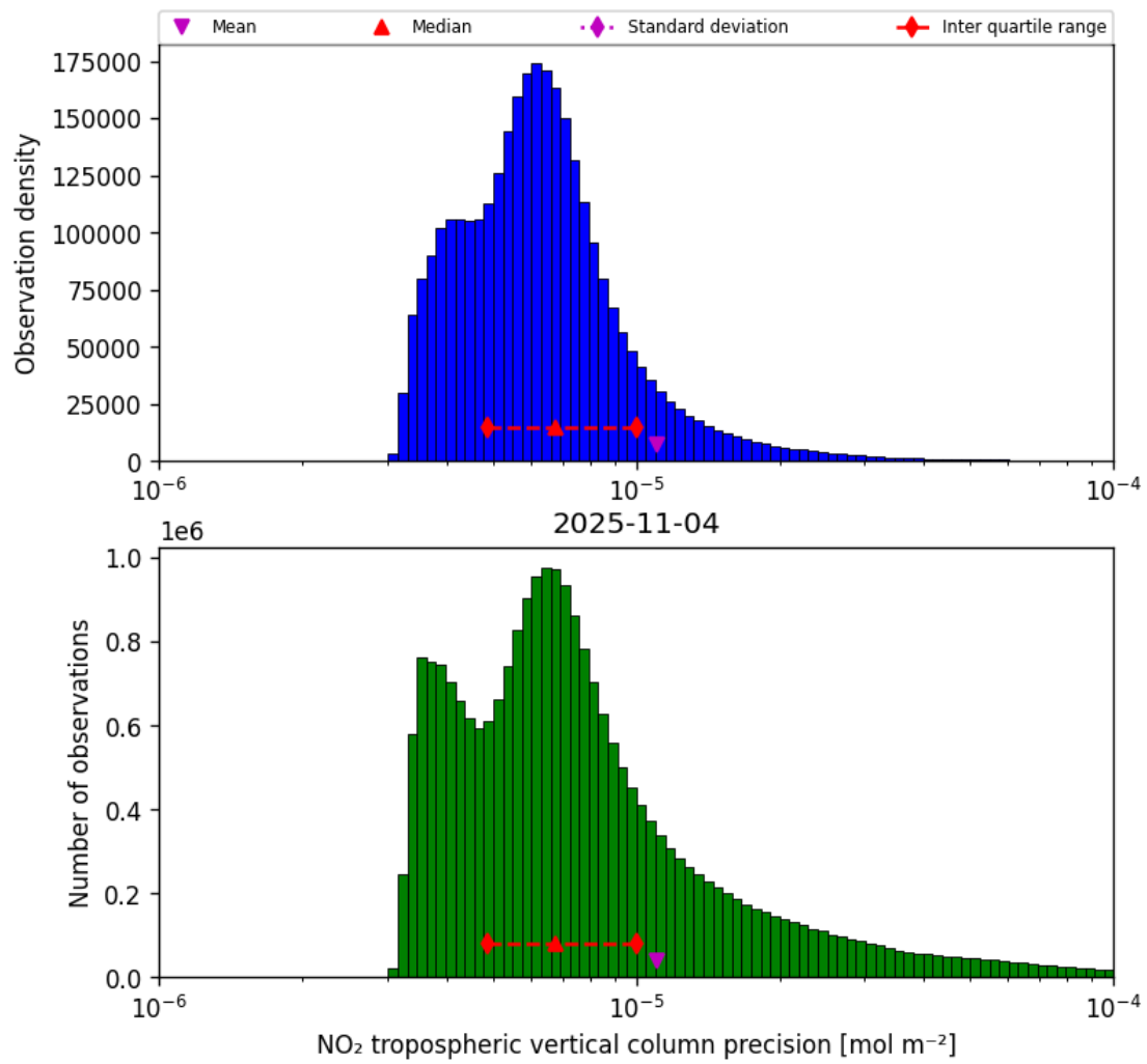
Figure 28: Histogram of "NO 2 tropospheric vertical column precision" for 2025-11-04 to 2025-11-05
