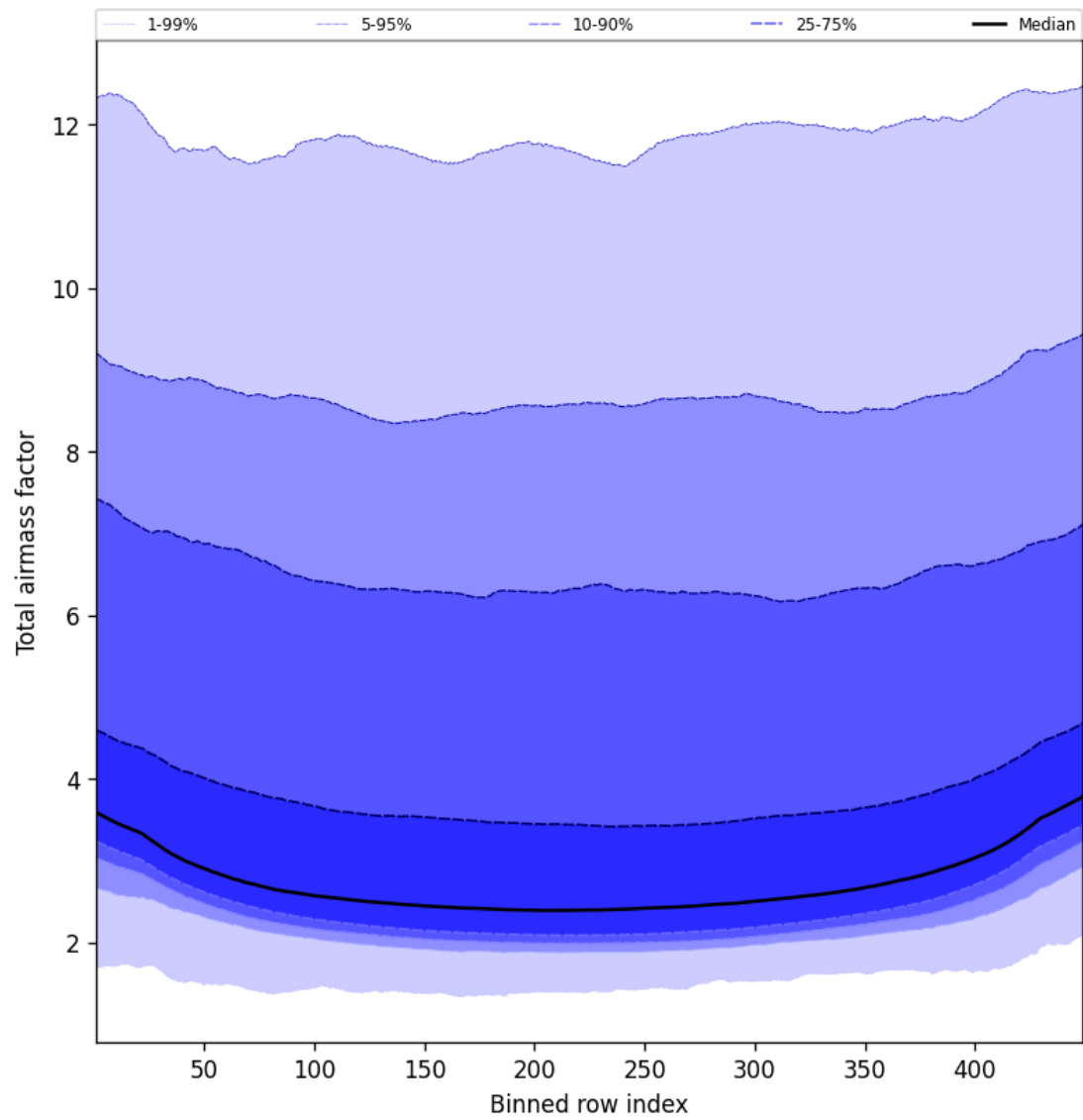
Figure 47: Along track statistics of “Total airmass factor” for 2025-11-04 to 2025-11-05
