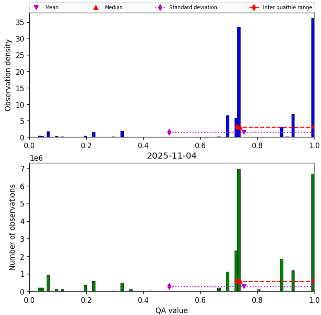
Figure 26: Histogram of “QA value” for 2025-11-04 to 2025-11-05
