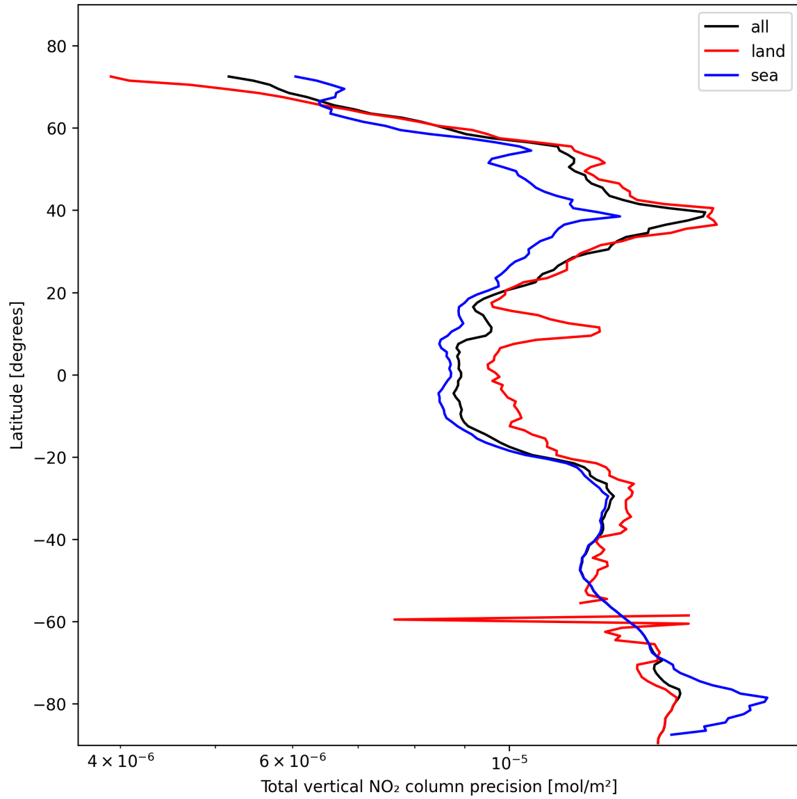
Figure 20: Zonal average of “Total vertical NO 2 column precision” for 2025-11-04 to 2025-11-05.
