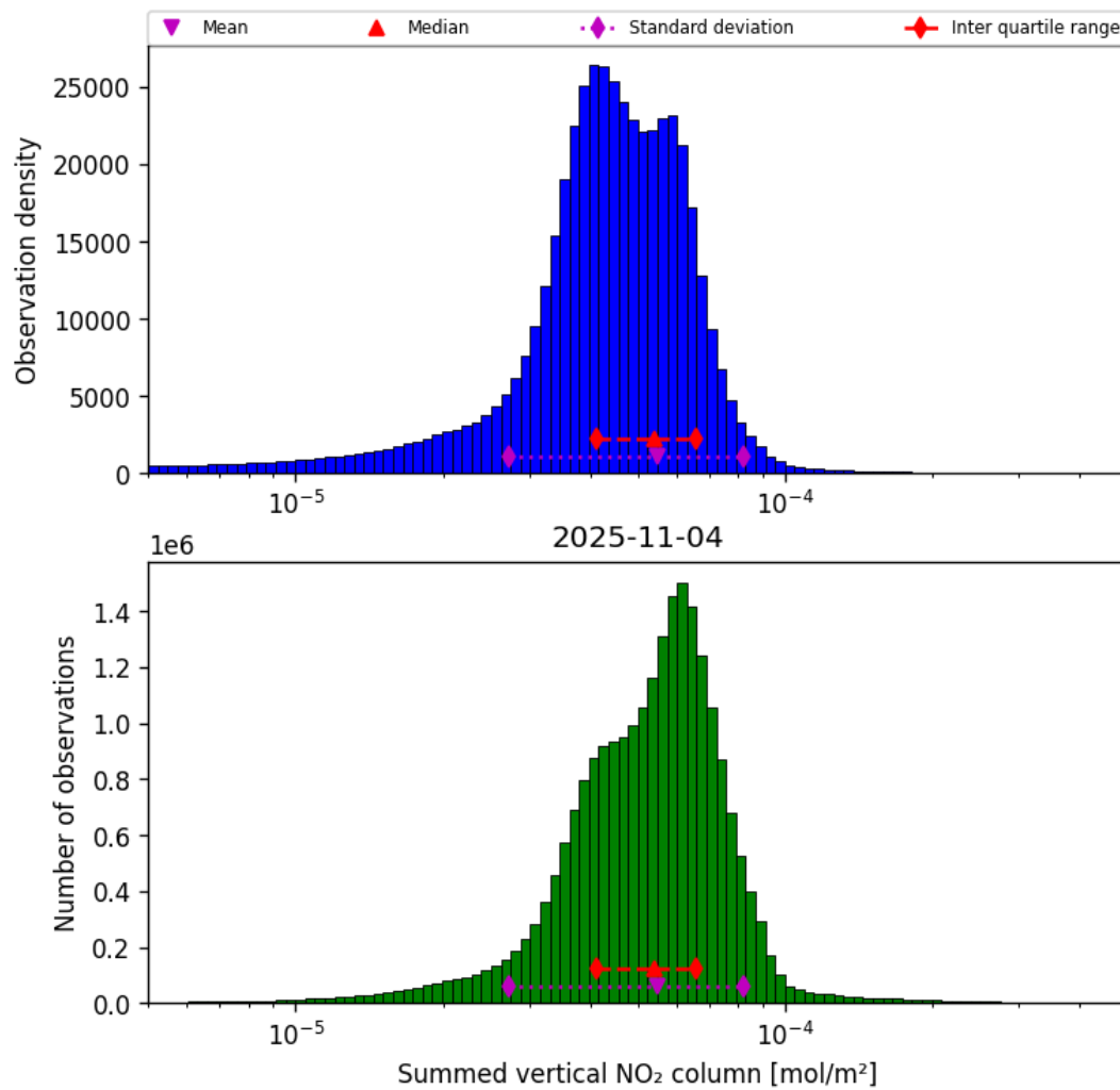
Figure 38: Histogram of “Summed vertical NO 2 column” for 2025-11-04 to 2025-11-05
