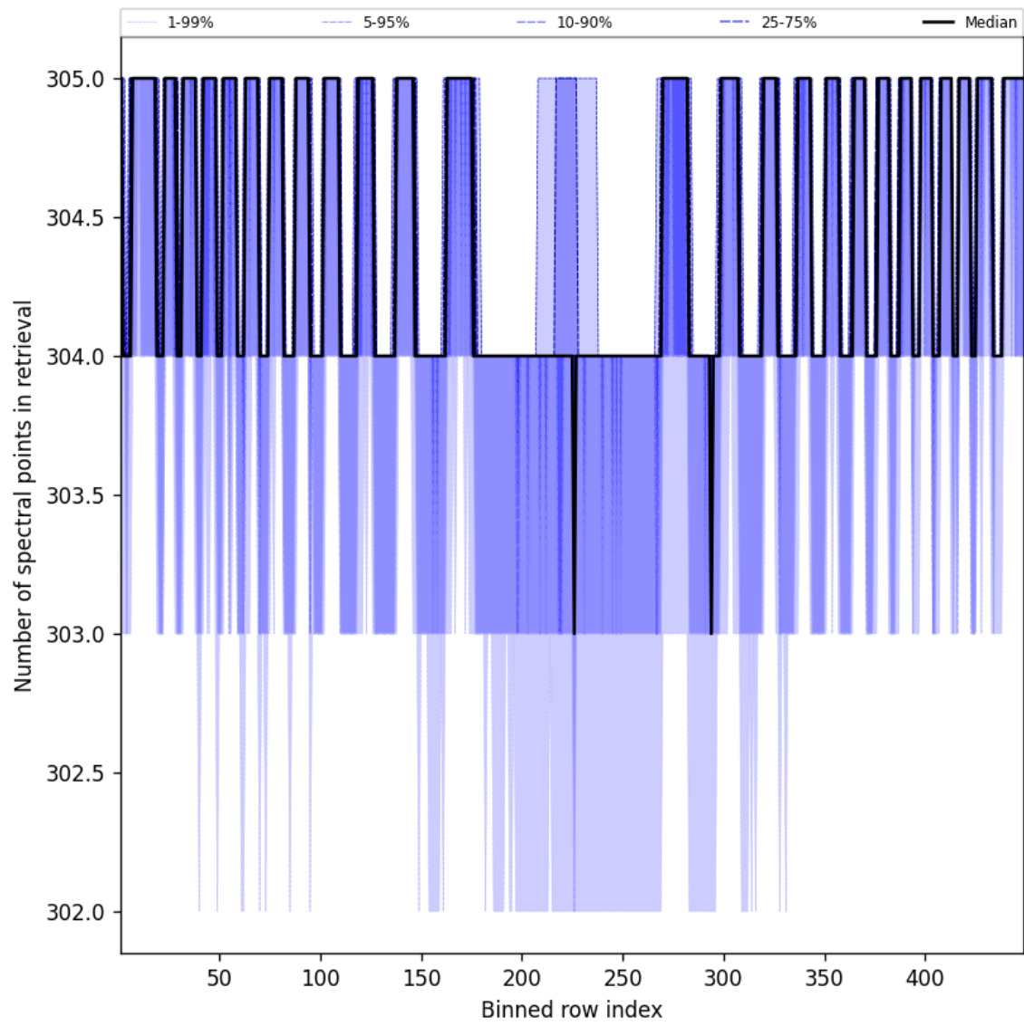
Figure 48: Along track statistics of “Number of spectral points in retrieval” for 2025-11-04 to 2025-11-05
