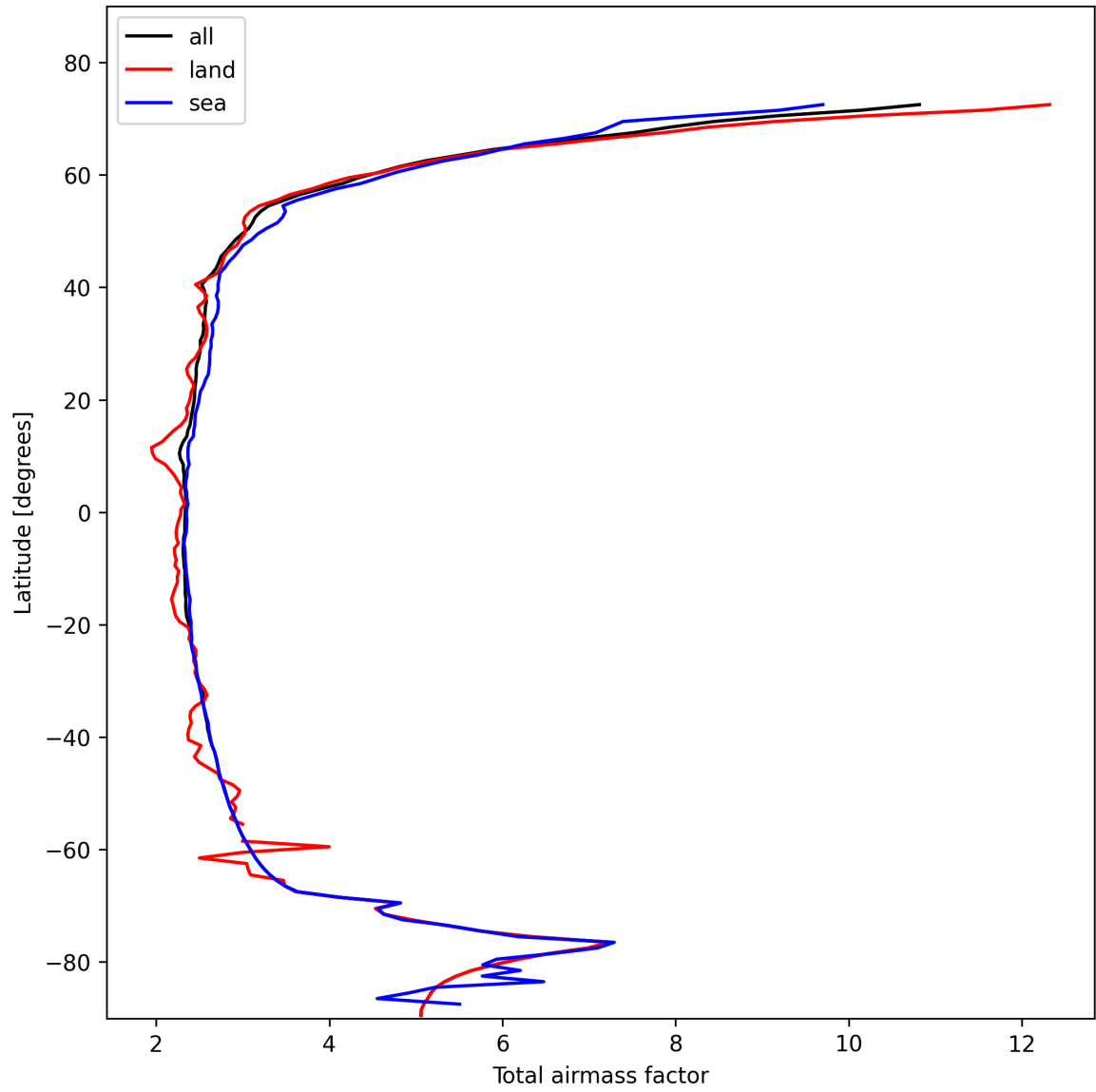
Figure 13: Zonal average of “Total airmass factor” for 2025-11-04 to 2025-11-05.
