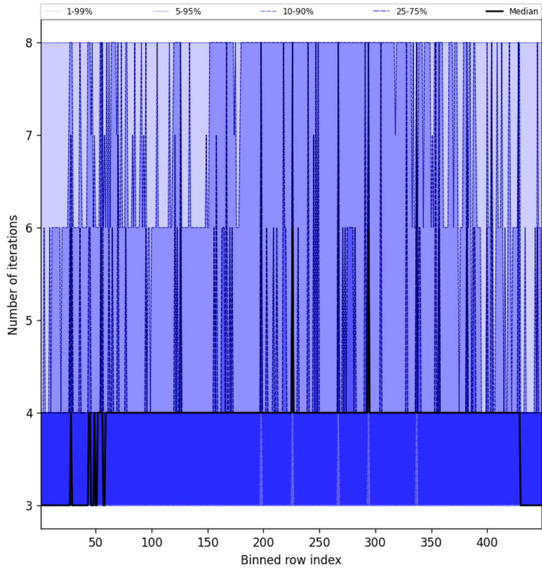
Figure 49: Along track statistics of “Number of iterations” for 2025-11-04 to 2025-11-05
