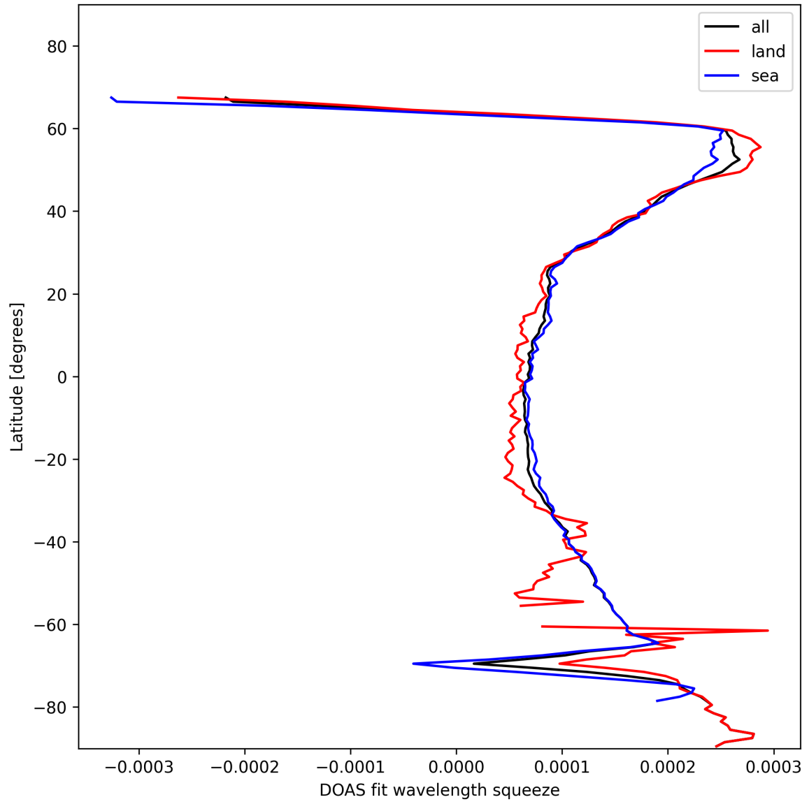
Figure 24: Zonal average of “DOAS fit wavelength squeeze” for 2024-12-01 to 2024-12-02.
