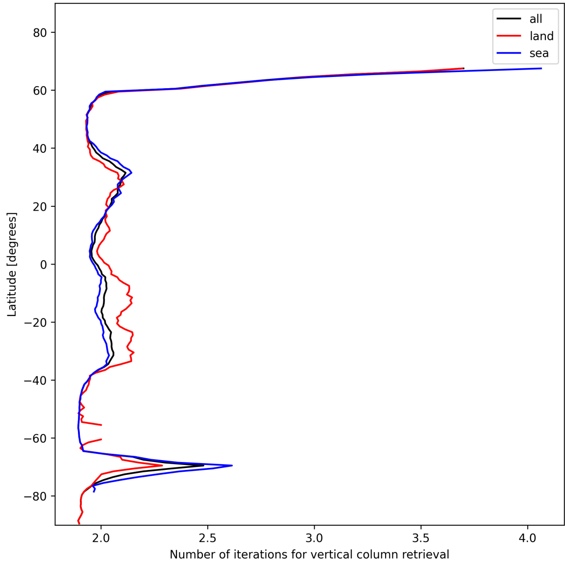
Figure 27: Zonal average of “Number of iterations for vertical column retrieval” for 2024-12-01 to 2024-12-02.
