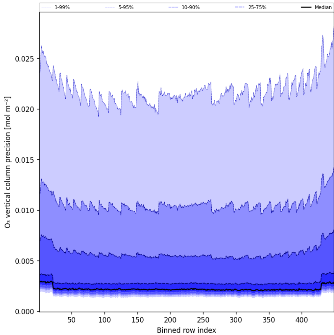
Figure 42: Along track statistics of “O 3 vertical column precision” for 2024-12-01 to 2024-12-02
