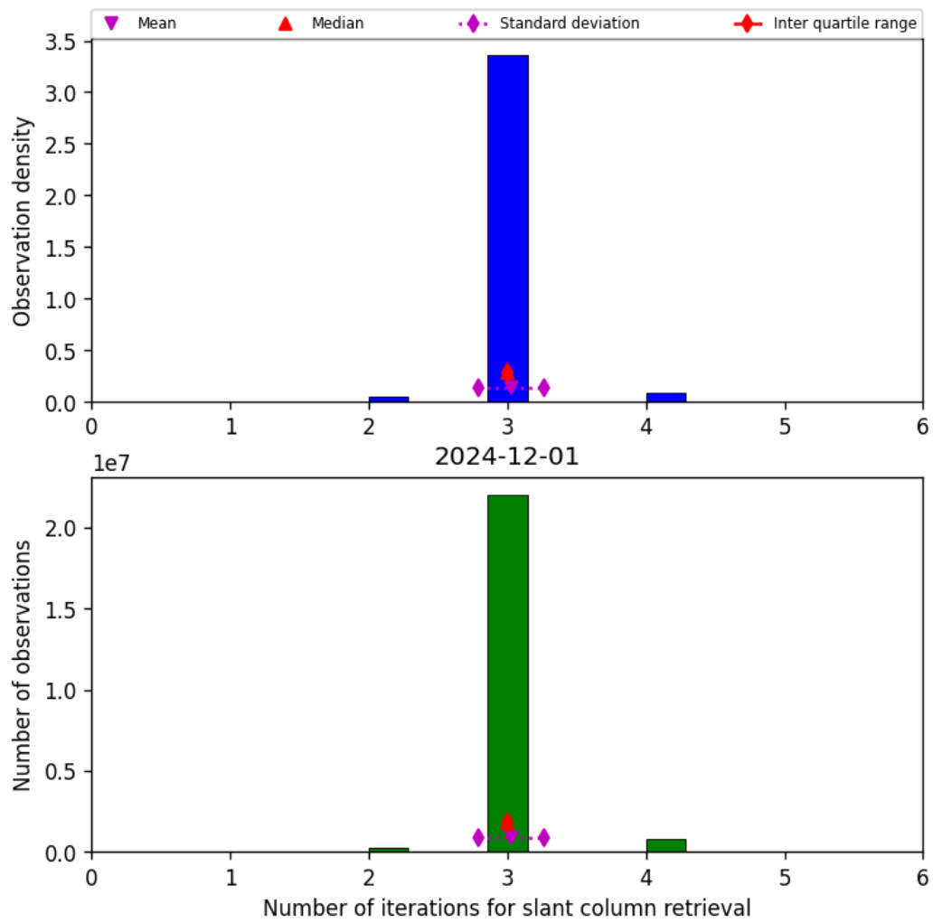
Figure 33: Histogram of “Number of iterations for slant column retrieval” for 2024-12-01 to 2024-12-02
