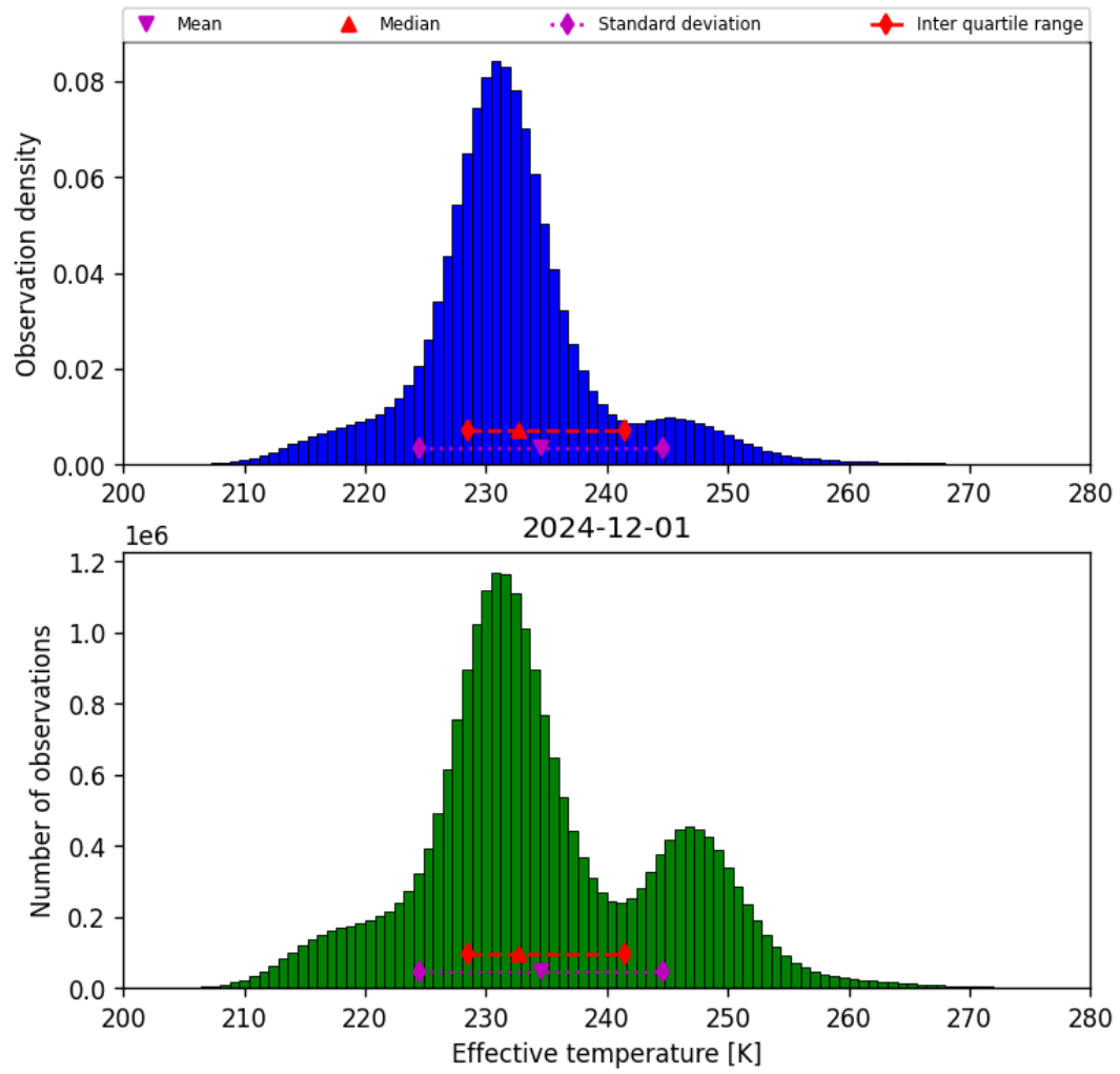
Figure 38: Histogram of “Effective temperature” for 2024-12-01 to 2024-12-02
