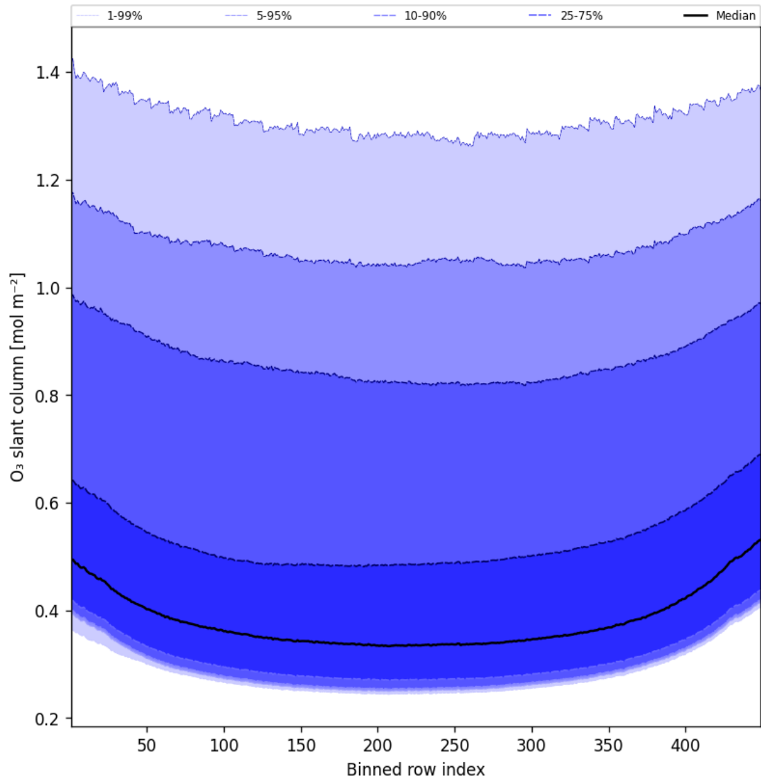
Figure 43: Along track statistics of “O 3 slant column” for 2024-12-01 to 2024-12-02
