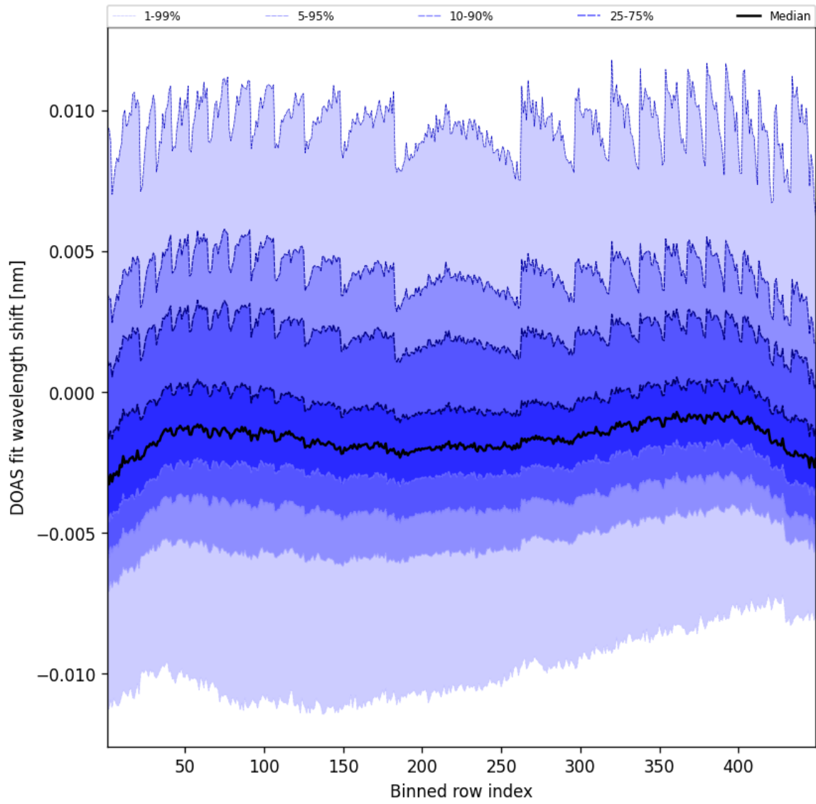
Figure 47: Along track statistics of “DOAS fit wavelength shift” for 2024-12-01 to 2024-12-02
