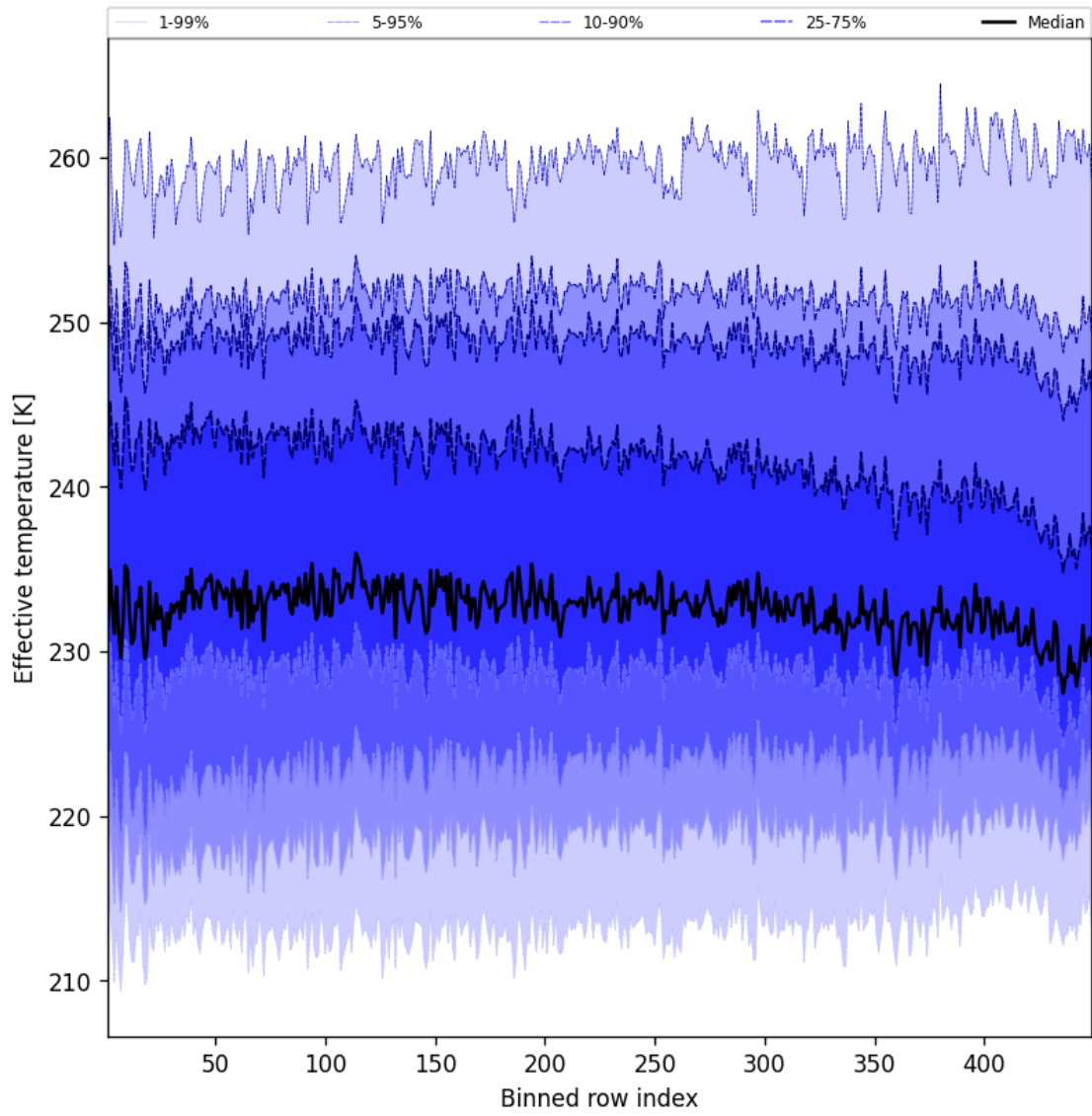
Figure 50: Along track statistics of “Effective temperature” for 2024-12-01 to 2024-12-02
