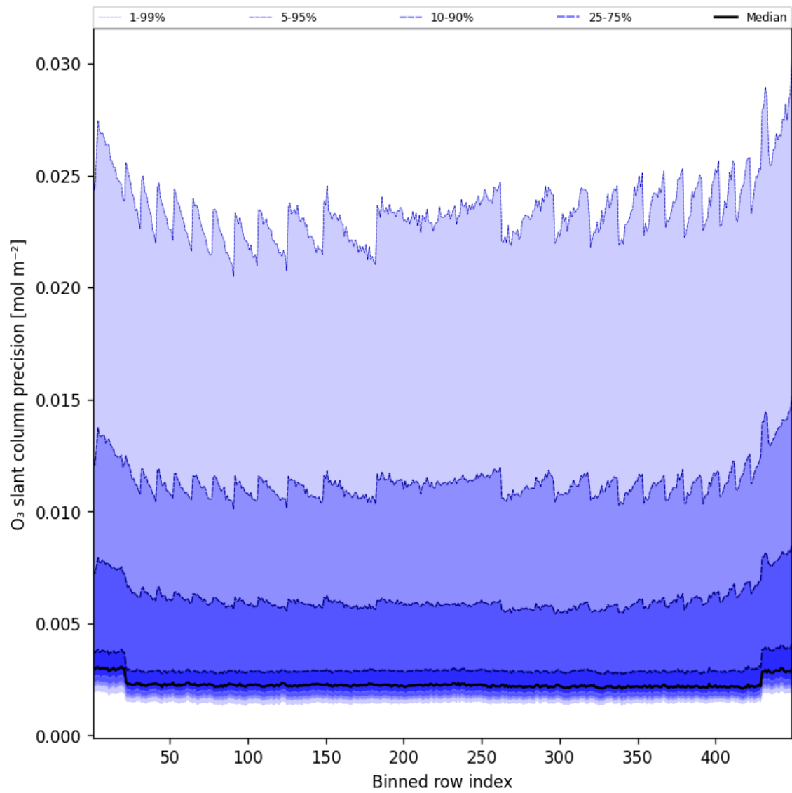
Figure 44: Along track statistics of “O 3 slant column precision” for 2024-12-01 to 2024-12-02
