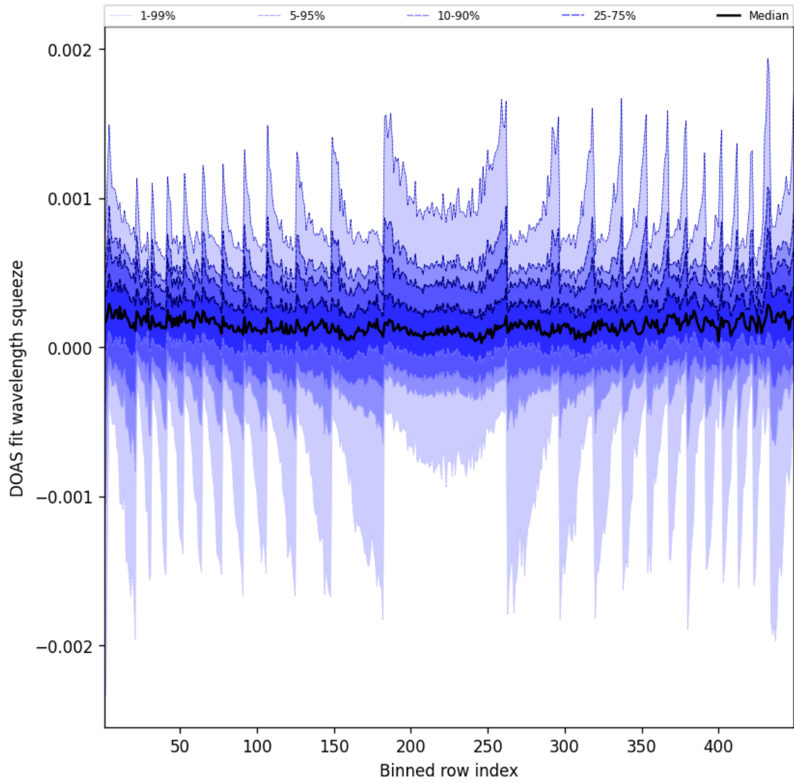
Figure 48: Along track statistics of “DOAS fit wavelength squeeze” for 2024-12-01 to 2024-12-02
