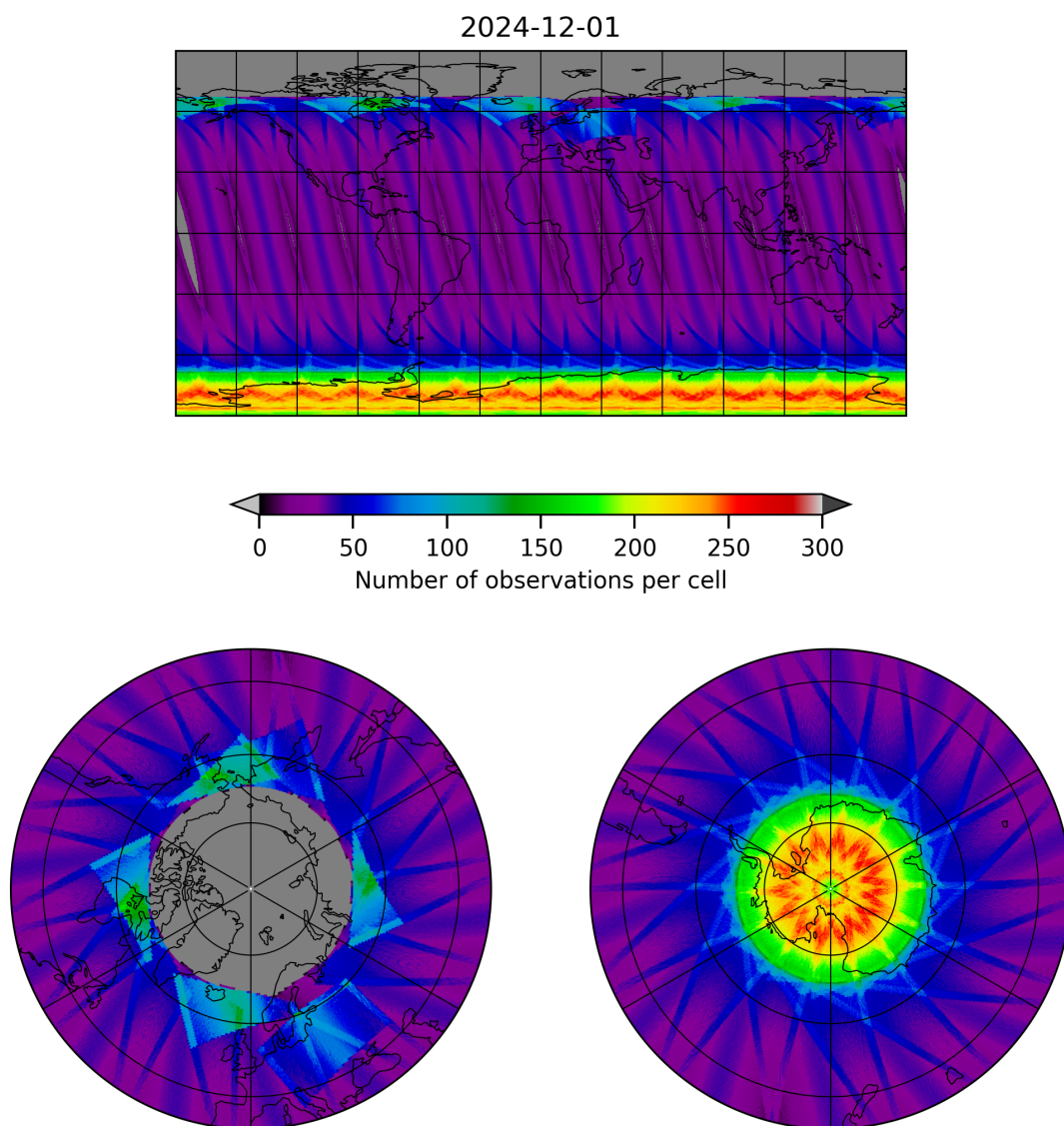
Figure 15: Map of the number of observations for 2024-12-01 to 2024-12-02
