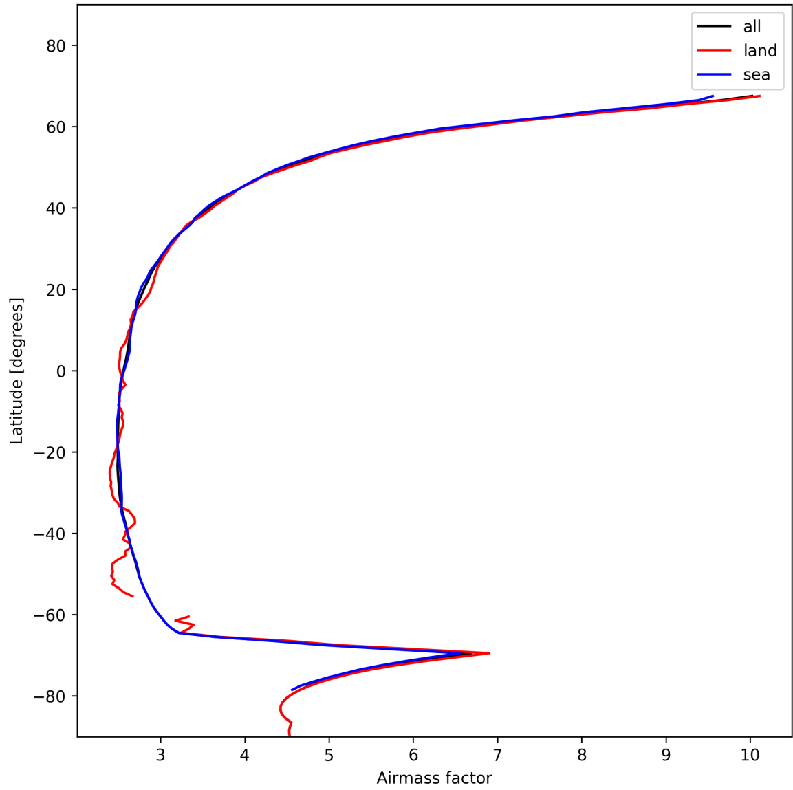
Figure 25: Zonal average of “Airmass factor” for 2024-12-01 to 2024-12-02.
