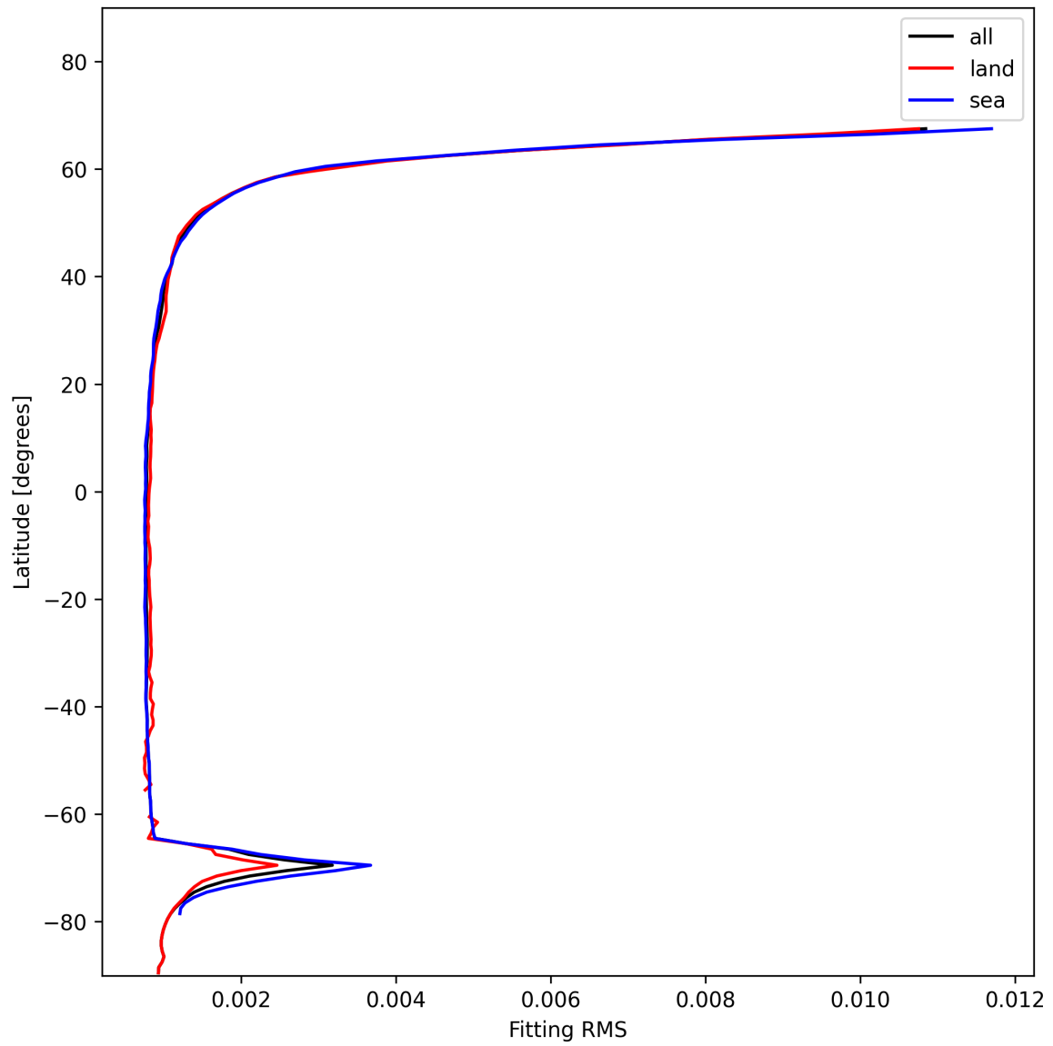
Figure 22: Zonal average of “Fitting RMS” for 2024-12-01 to 2024-12-02.
