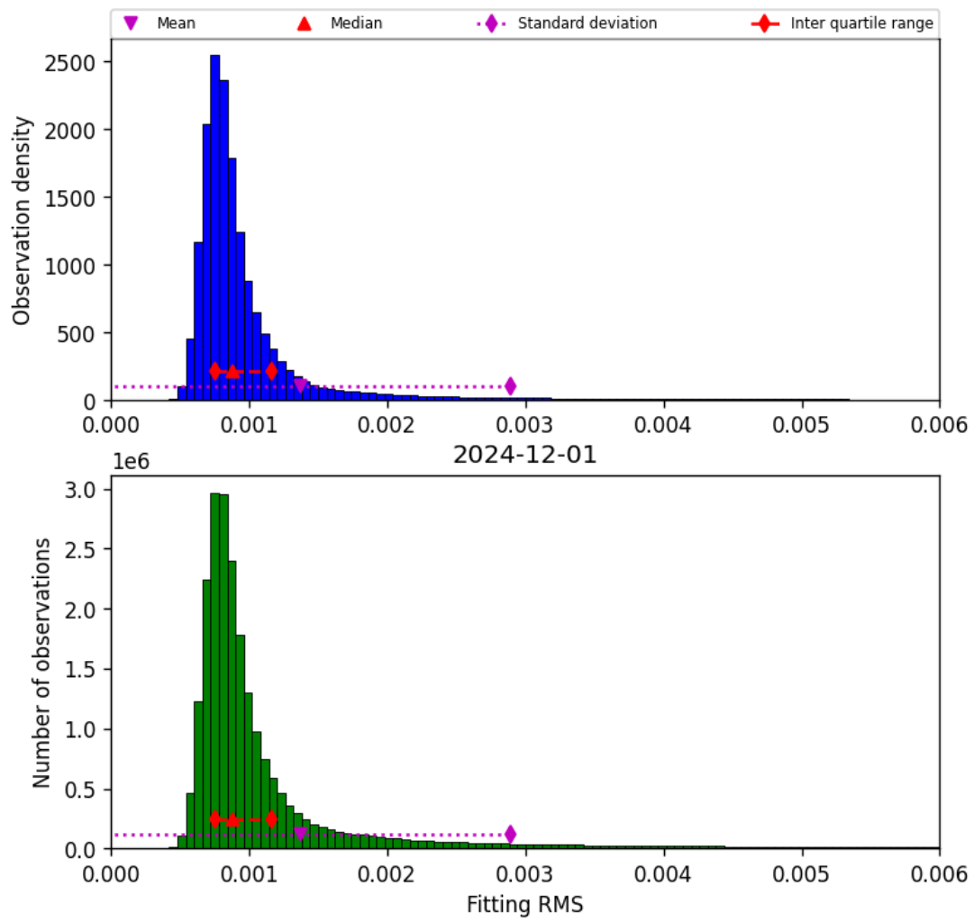
Figure 34: Histogram of “Fitting RMS” for 2024-12-01 to 2024-12-02
