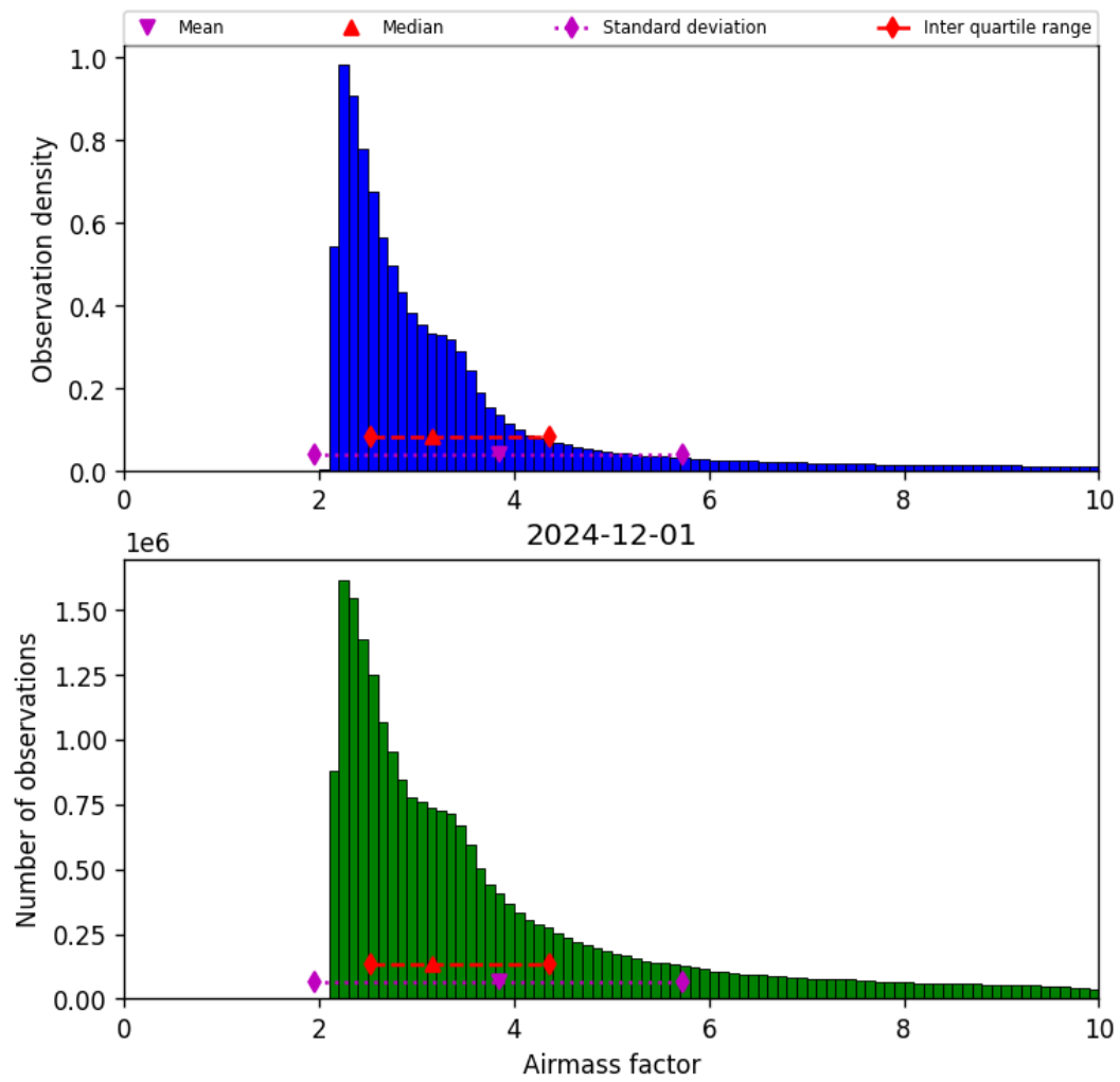
Figure 37: Histogram of “Airmass factor” for 2024-12-01 to 2024-12-02
