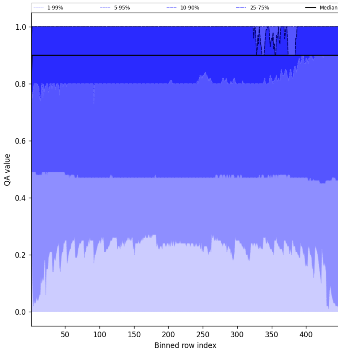
Figure 40: Along track statistics of “QA value” for 2024-12-01 to 2024-12-02
