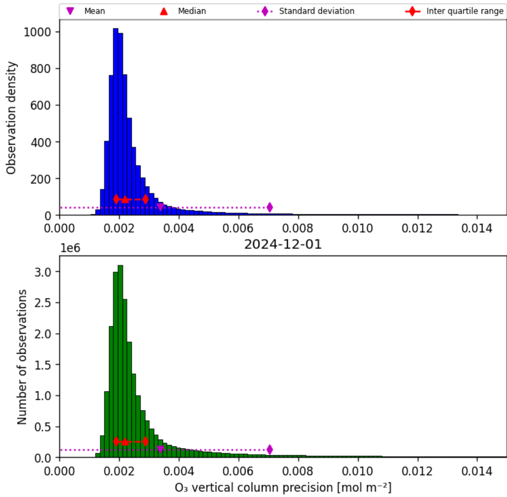
Figure 30: Histogram of "O 3 vertical column precision" for 2024-12-01 to 2024-12-02
