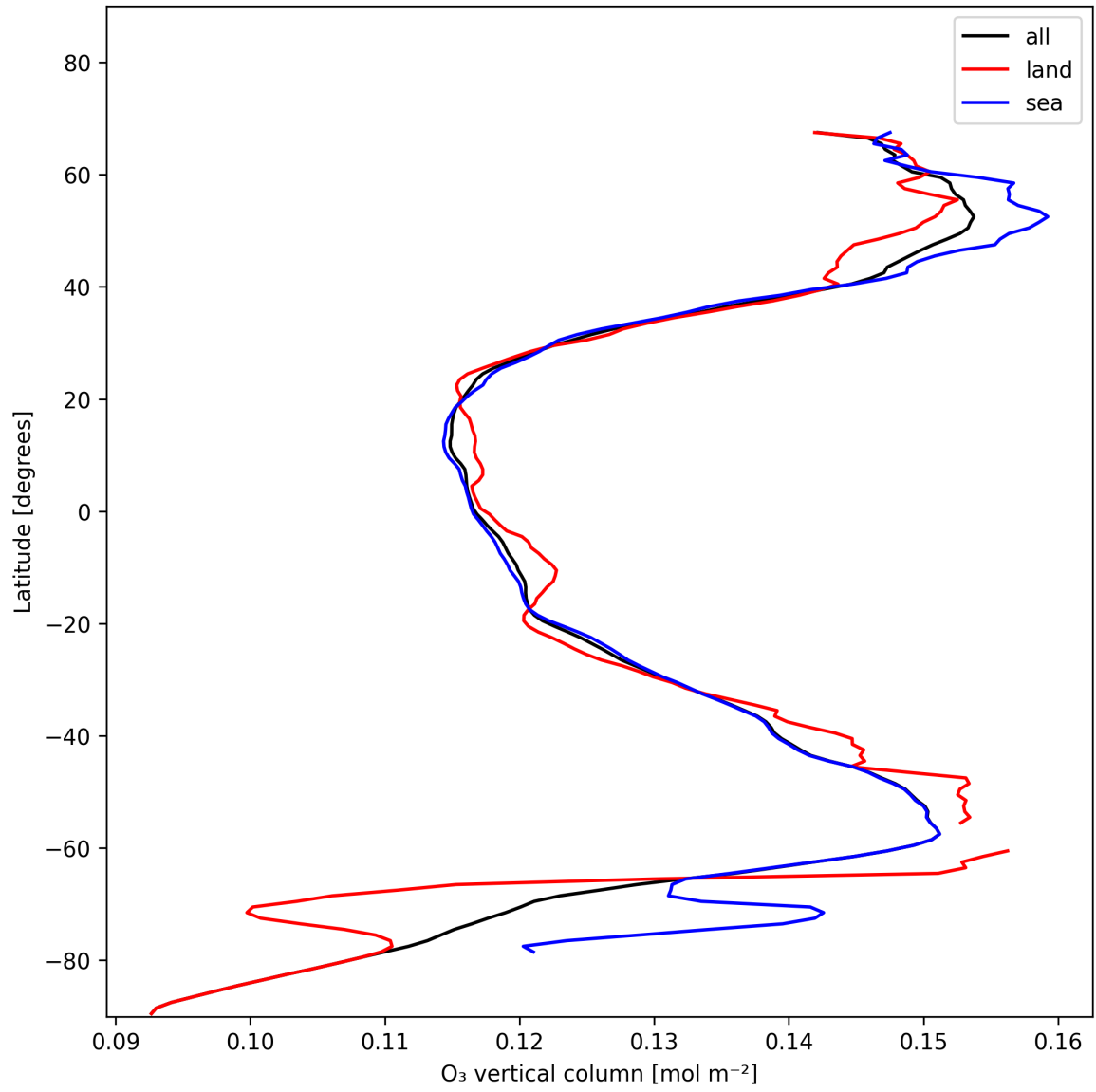
Figure 17: Zonal average of “O 3 vertical column” for 2024-12-01 to 2024-12-02.
