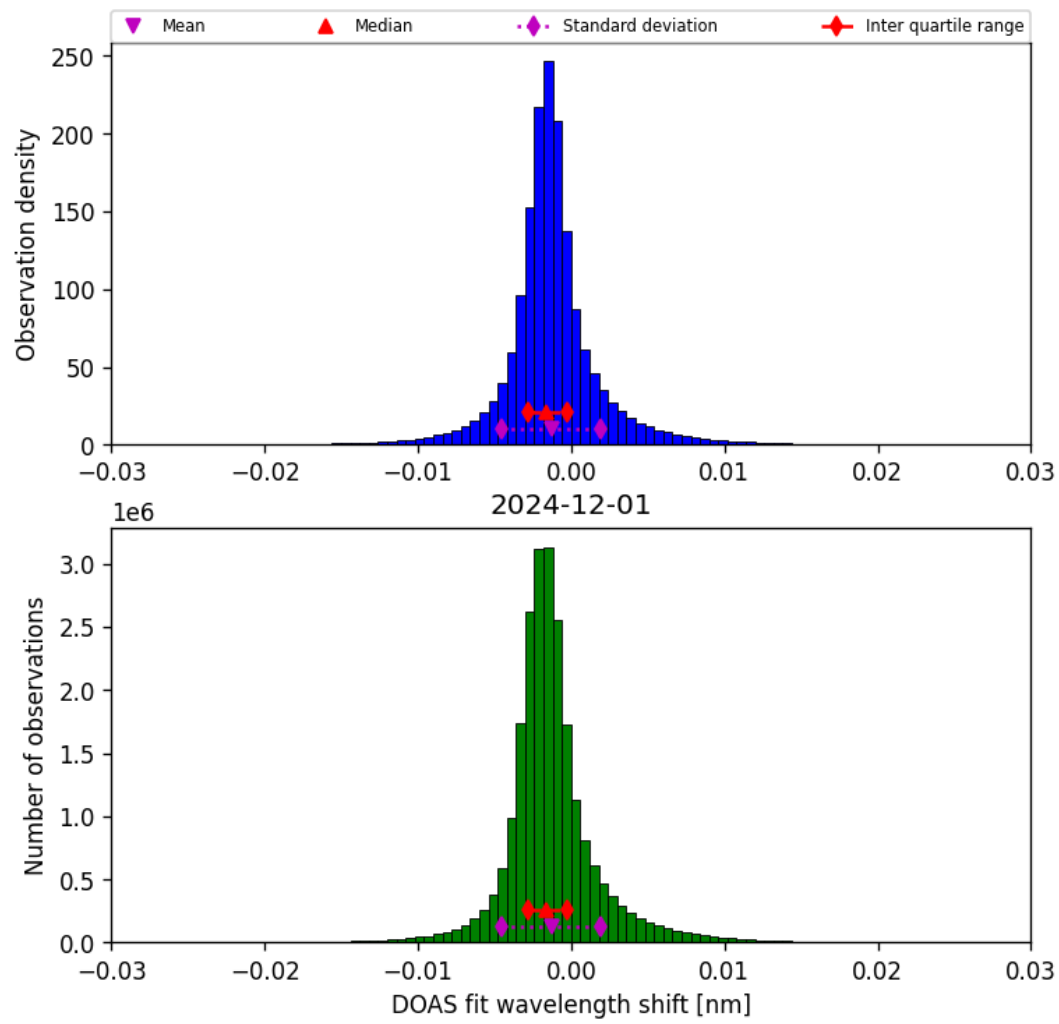
Figure 35: Histogram of “DOAS fit wavelength shift” for 2024-12-01 to 2024-12-02
