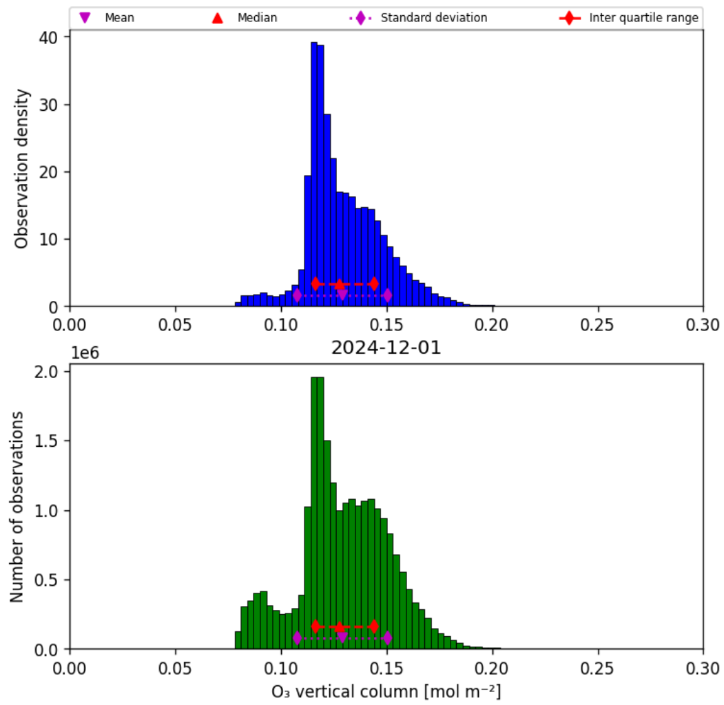
Figure 29: Histogram of “O 3 vertical column” for 2024-12-01 to 2024-12-02
