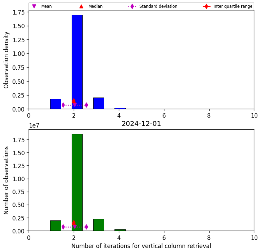
Figure 39: Histogram of “Number of iterations for vertical column retrieval” for 2024-12-01 to 2024-12-02
