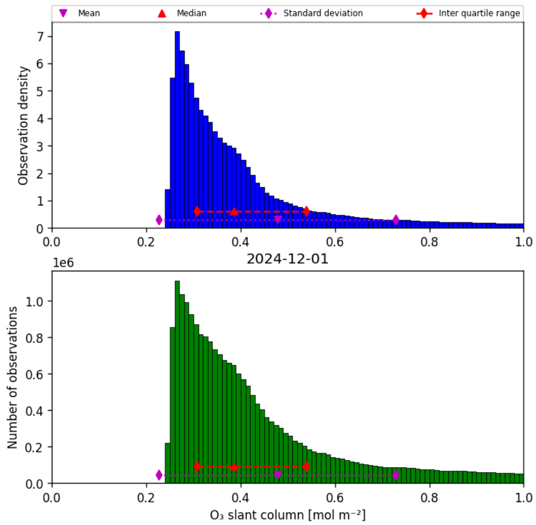
Figure 31: Histogram of “O 3 slant column” for 2024-12-01 to 2024-12-02
