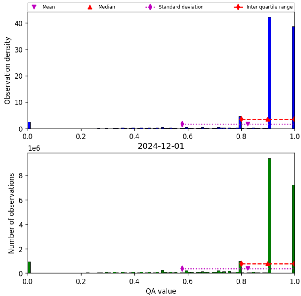
Figure 28: Histogram of “QA value” for 2024-12-01 to 2024-12-02
