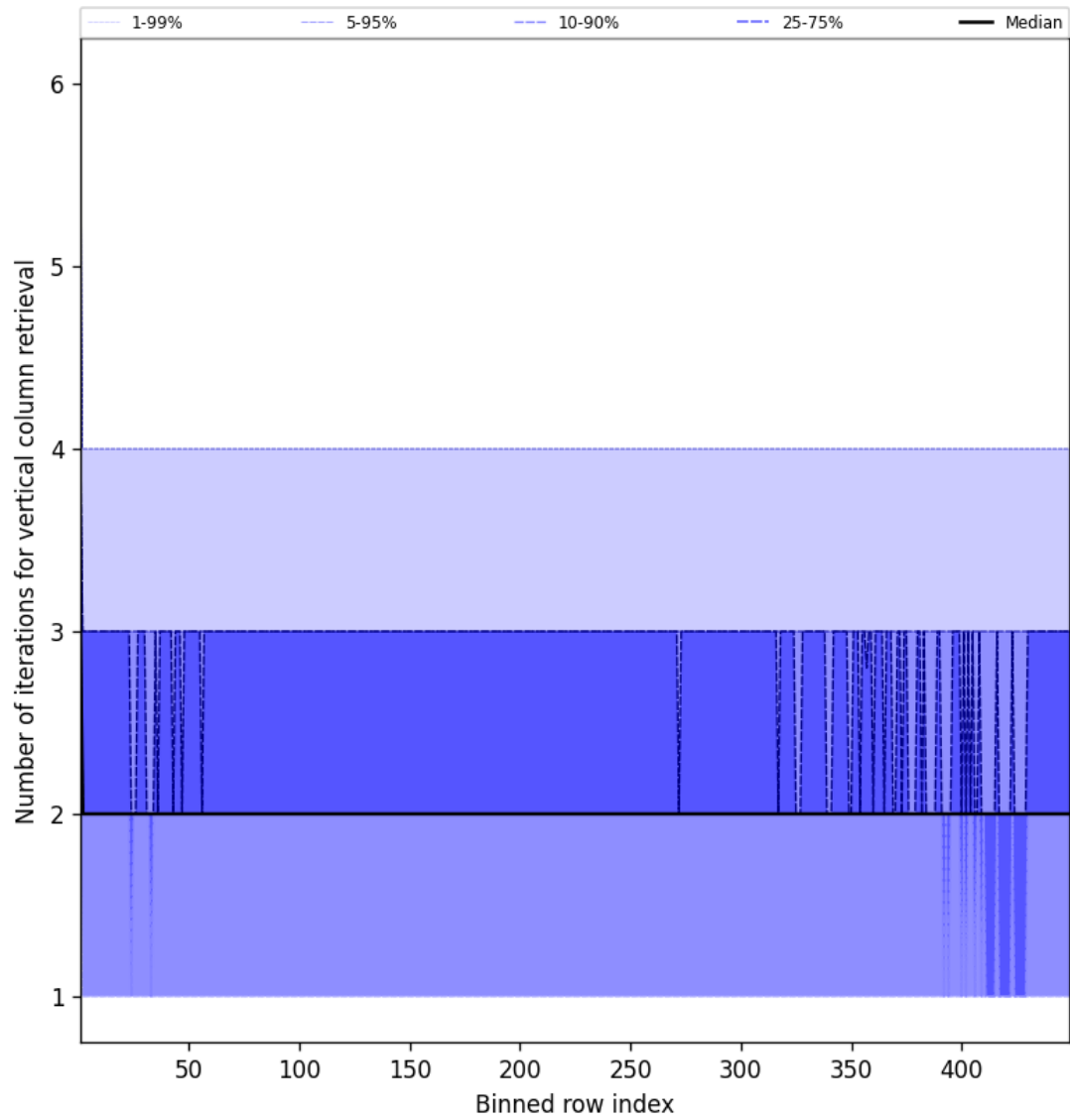
Figure 51: Along track statistics of “Number of iterations for vertical column retrieval” for 2024-12-01 to 2024-12-02
