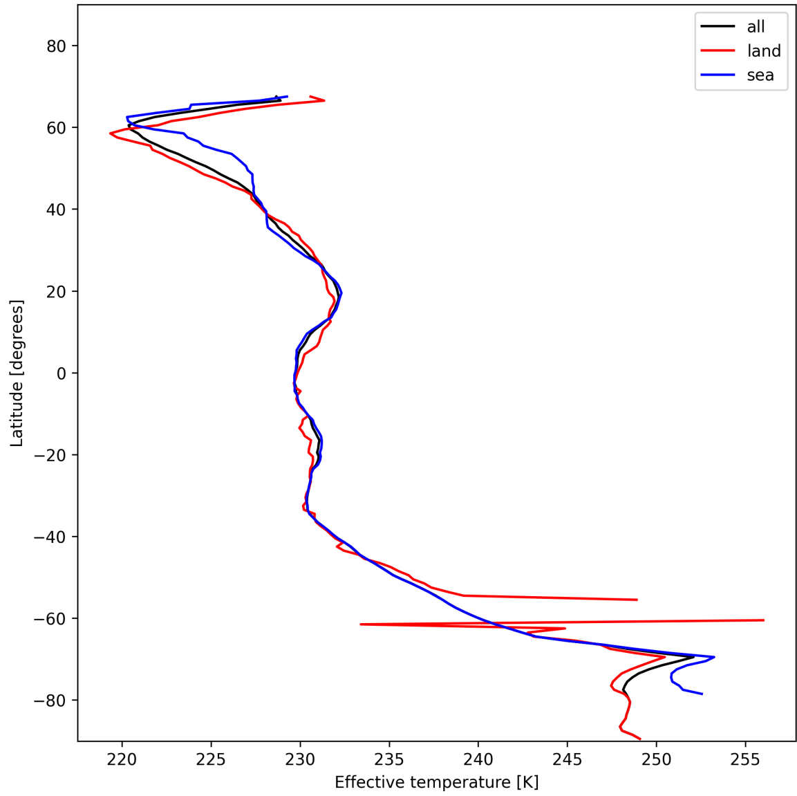
Figure 26: Zonal average of “Effective temperature” for 2024-12-01 to 2024-12-02.
