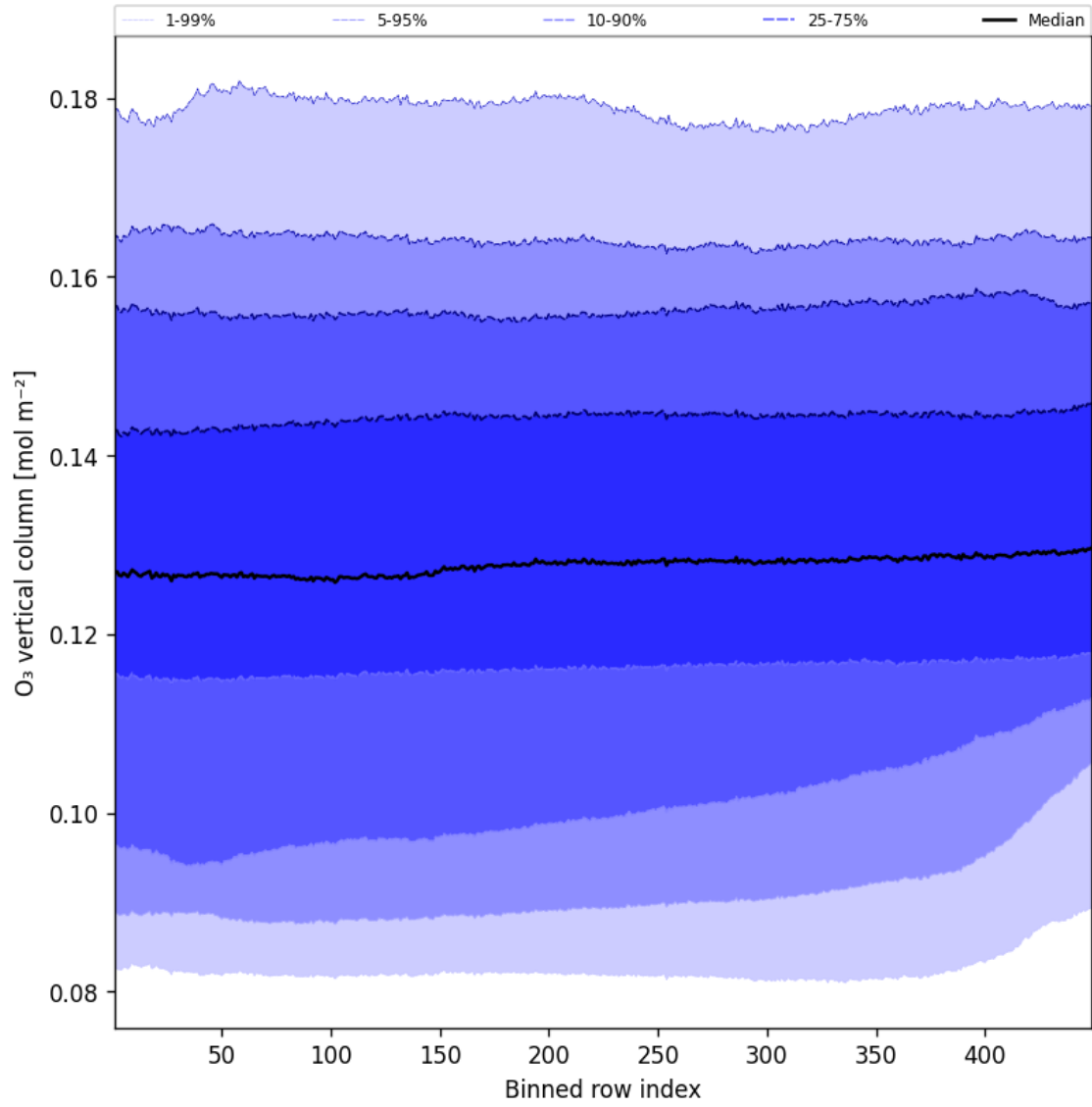
Figure 41: Along track statistics of “O 3 vertical column” for 2024-12-01 to 2024-12-02
