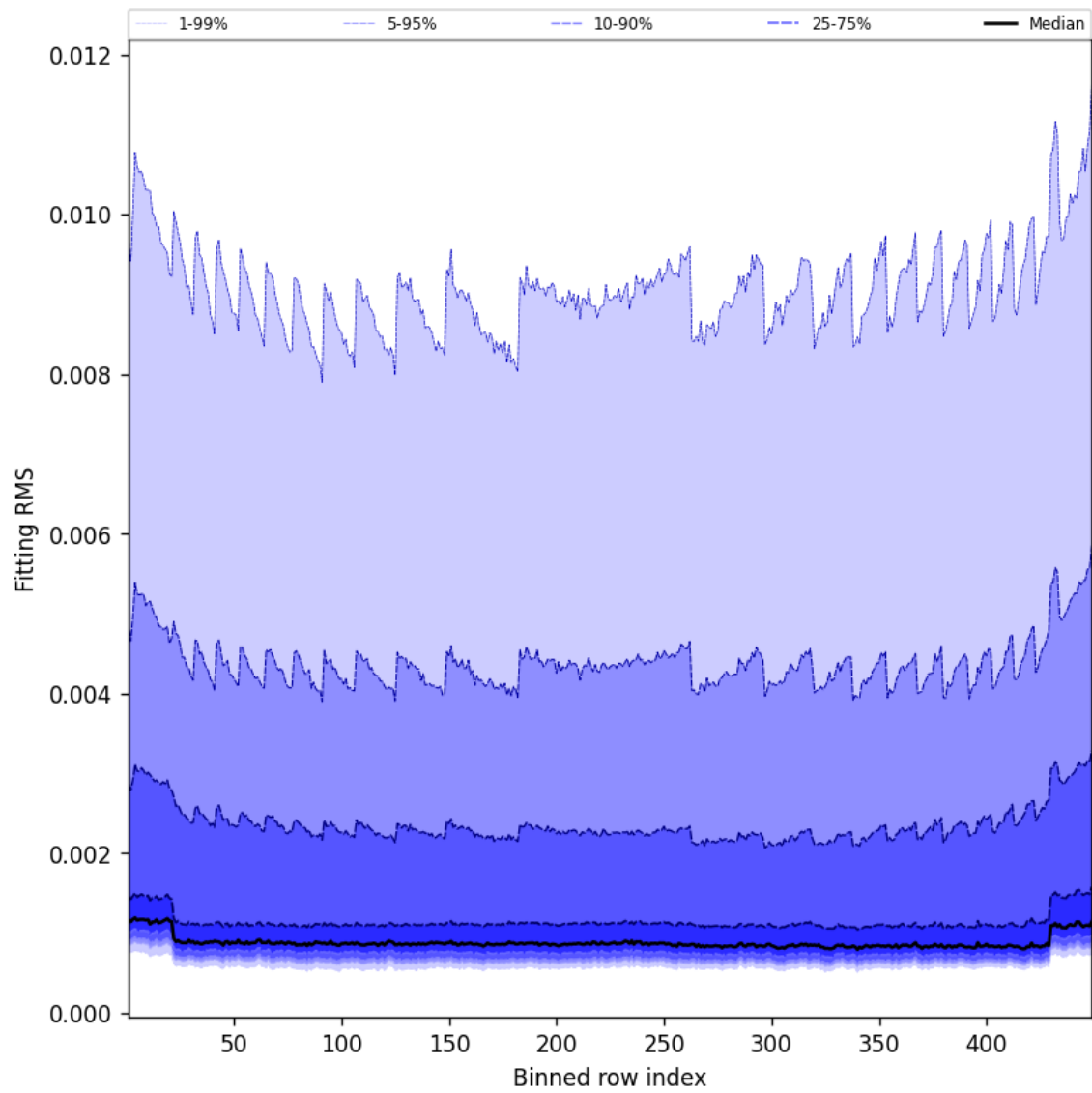
Figure 46: Along track statistics of “Fitting RMS” for 2024-12-01 to 2024-12-02
