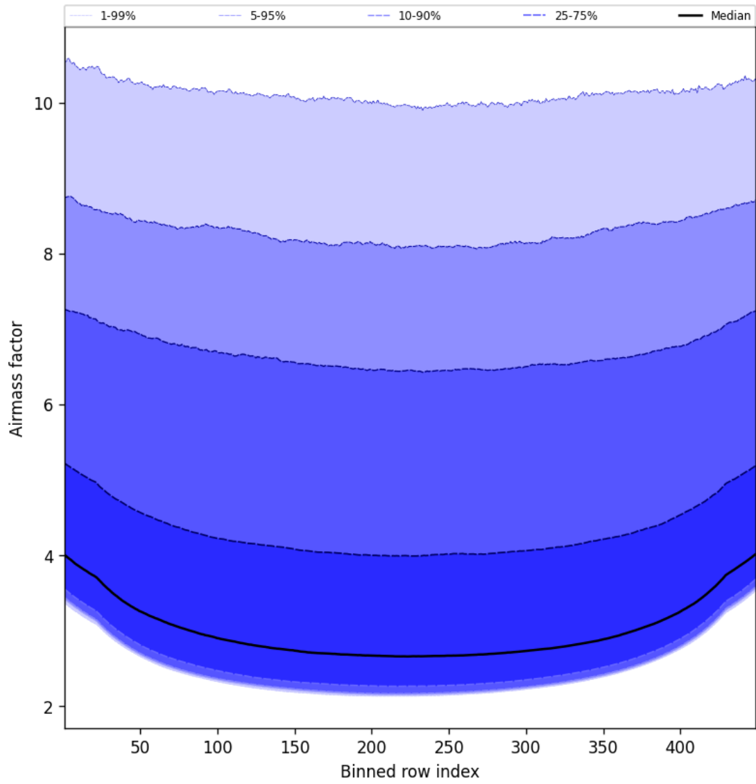
Figure 49: Along track statistics of “Airmass factor” for 2024-12-01 to 2024-12-02
