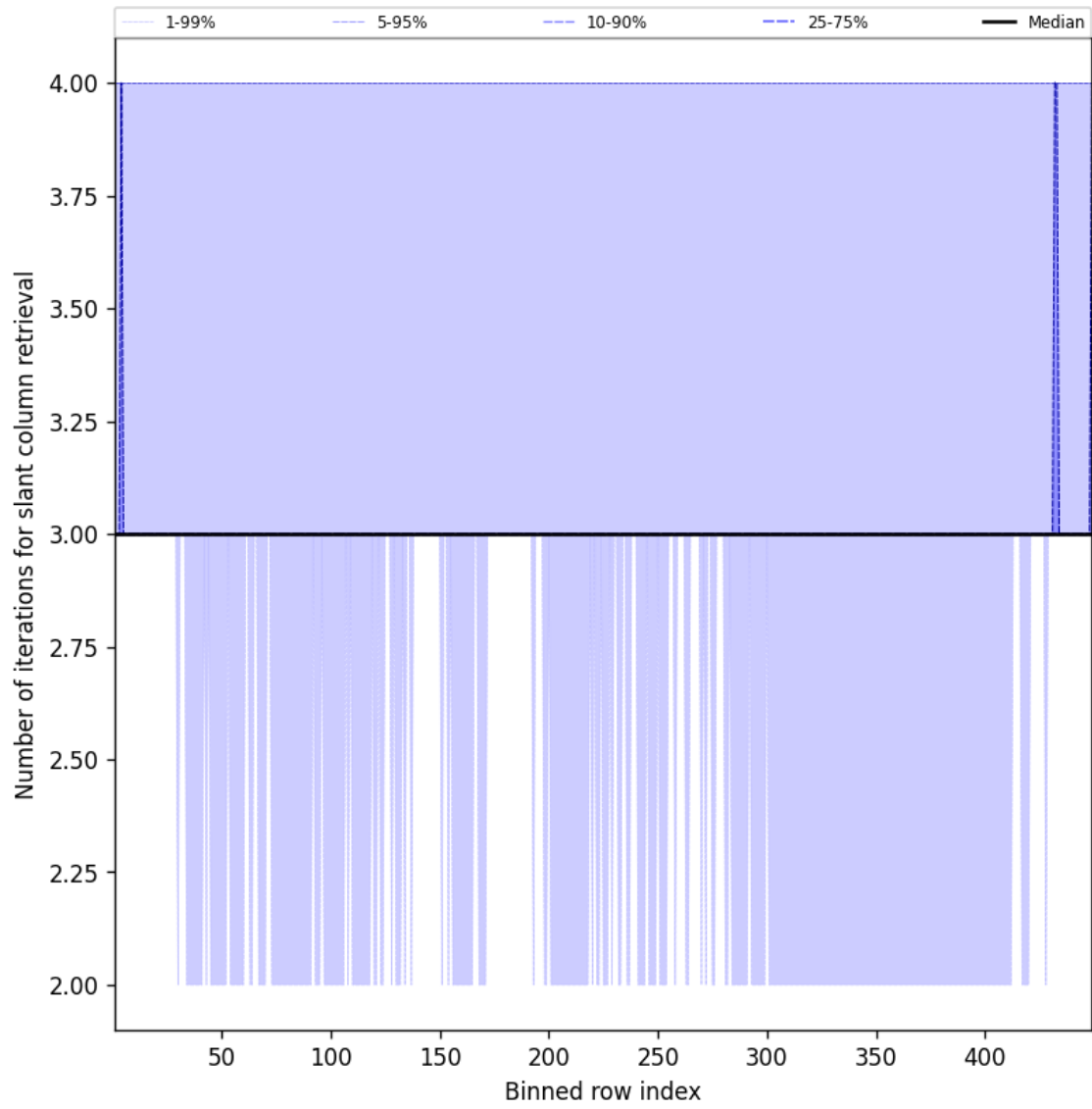
Figure 45: Along track statistics of “Number of iterations for slant column retrieval” for 2024-12-01 to 2024-12-02
