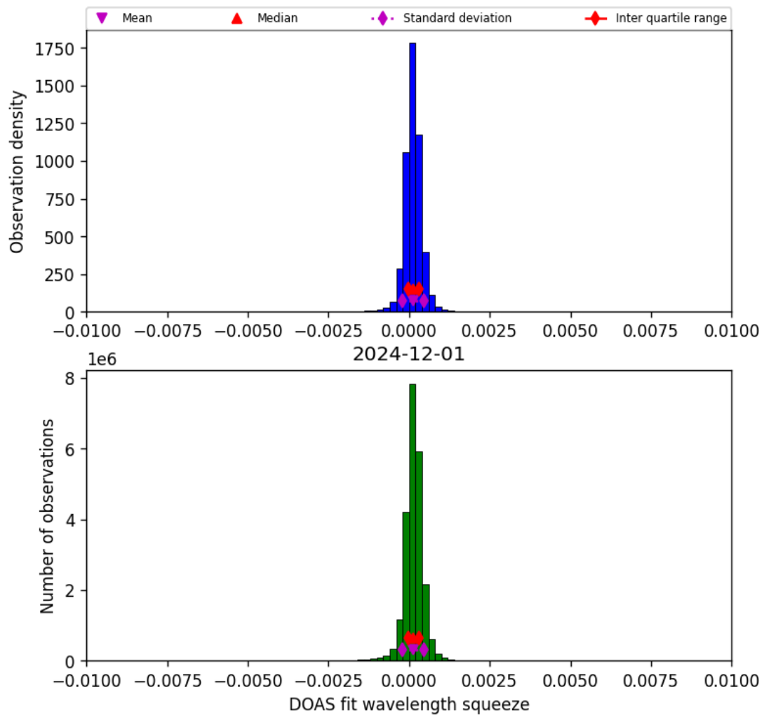
Figure 36: Histogram of “DOAS fit wavelength squeeze” for 2024-12-01 to 2024-12-02
