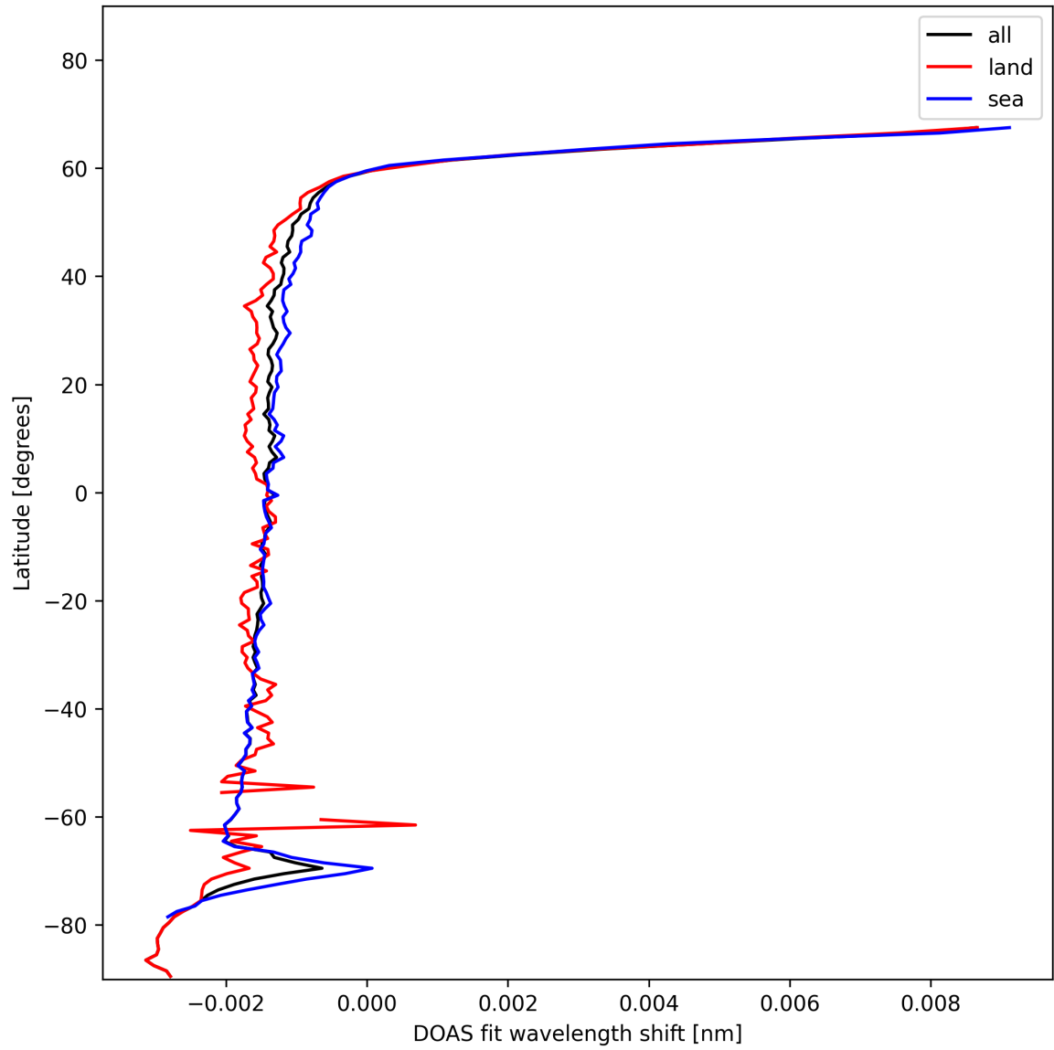
Figure 23: Zonal average of “DOAS fit wavelength shift” for 2024-12-01 to 2024-12-02.
