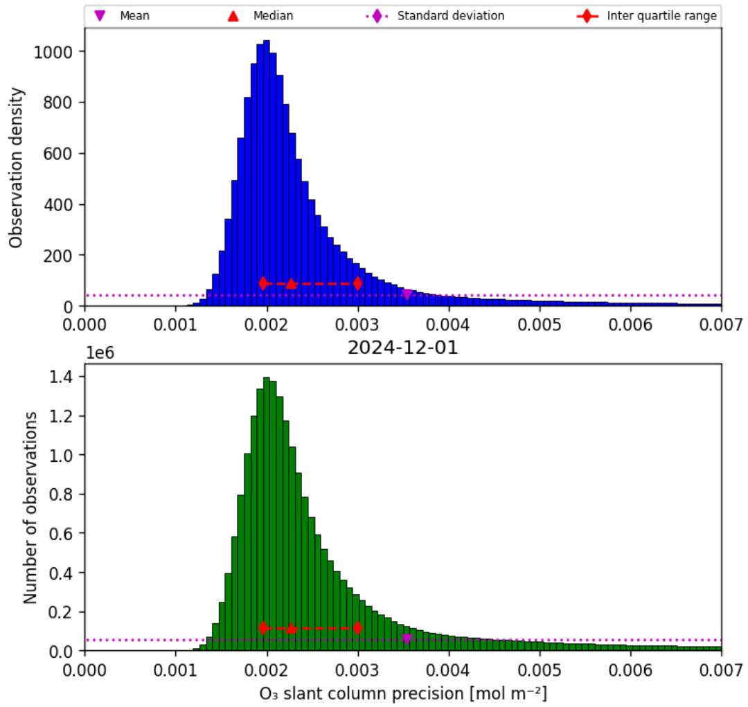
Figure 32: Histogram of “O 3 slant column precision” for 2024-12-01 to 2024-12-02
