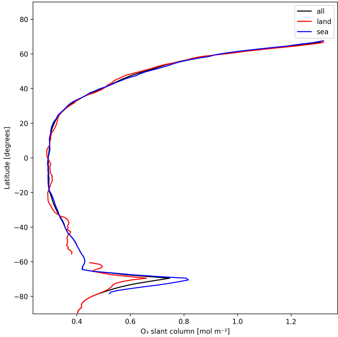
Figure 19: Zonal average of “O 3 slant column” for 2024-12-01 to 2024-12-02.
