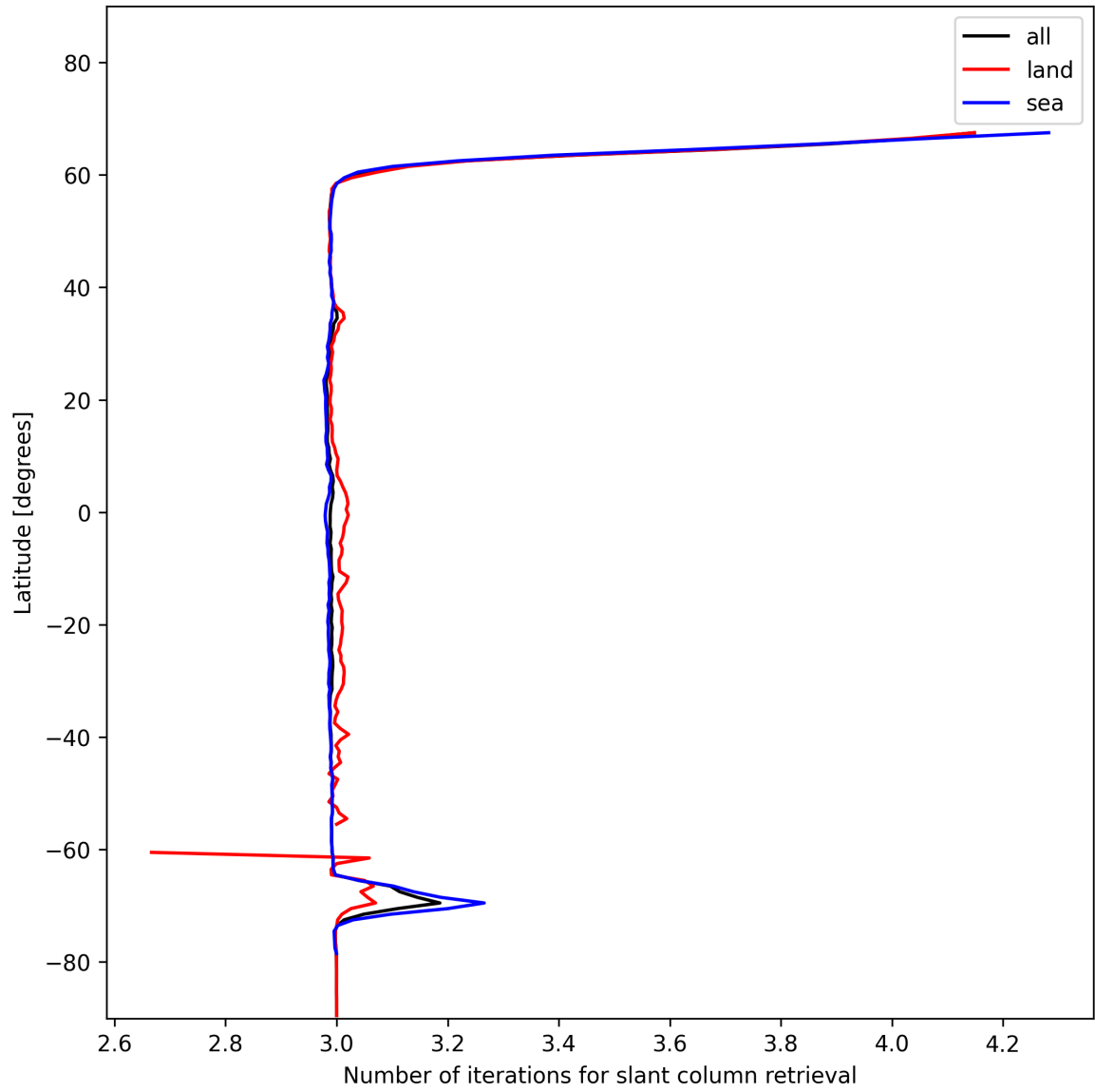
Figure 21: Zonal average of “Number of iterations for slant column retrieval” for 2024-12-01 to 2024-12-02.
