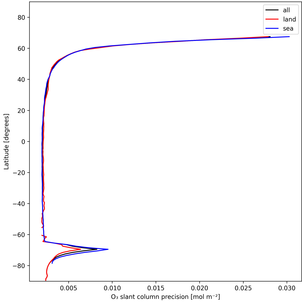
Figure 20: Zonal average of “O 3 slant column precision” for 2024-12-01 to 2024-12-02.
