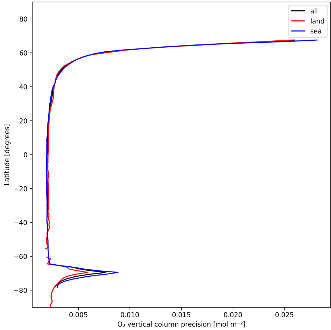
Figure 18: Zonal average of “O 3 vertical column precision” for 2024-12-01 to 2024-12-02.
