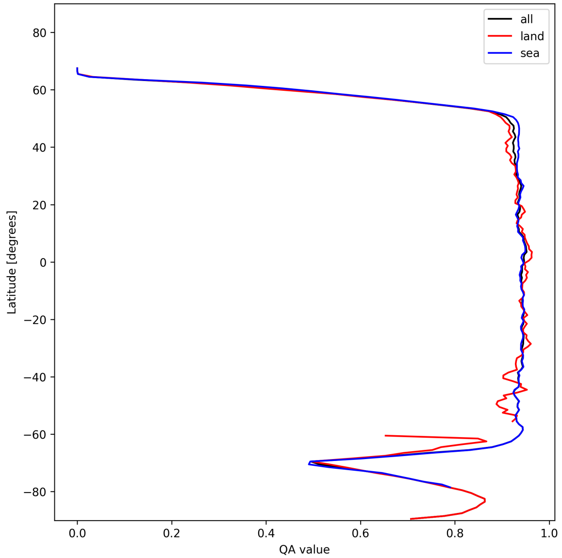
Figure 16: Zonal average of “QA value” for 2024-12-01 to 2024-12-02.
