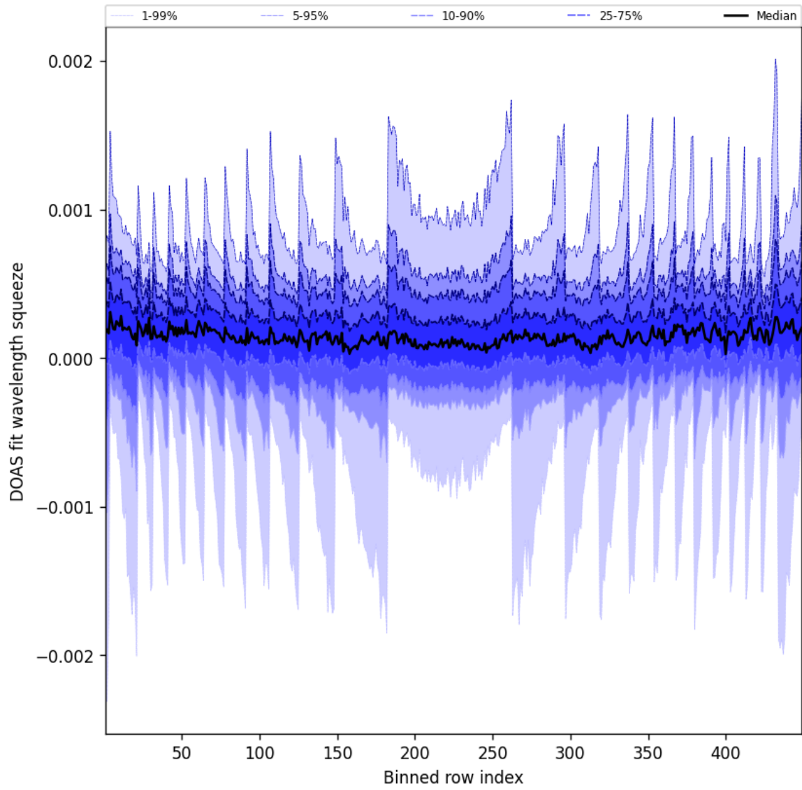
Figure 48: Along track statistics of “DOAS fit wavelength squeeze” for 2024-12-02 to 2024-12-03
