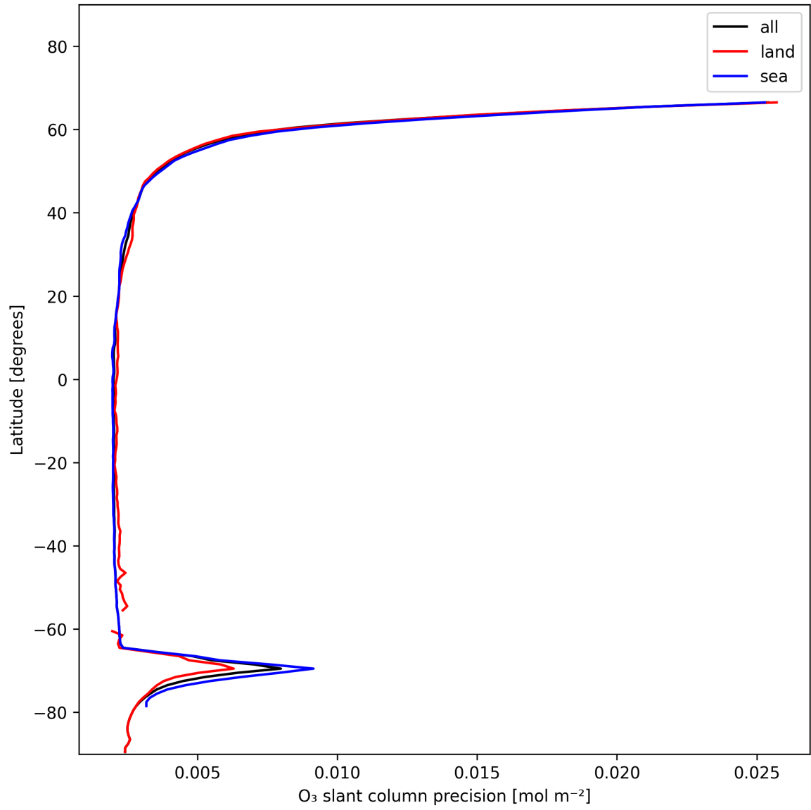
Figure 20: Zonal average of “O 3 slant column precision” for 2024-12-02 to 2024-12-03.
