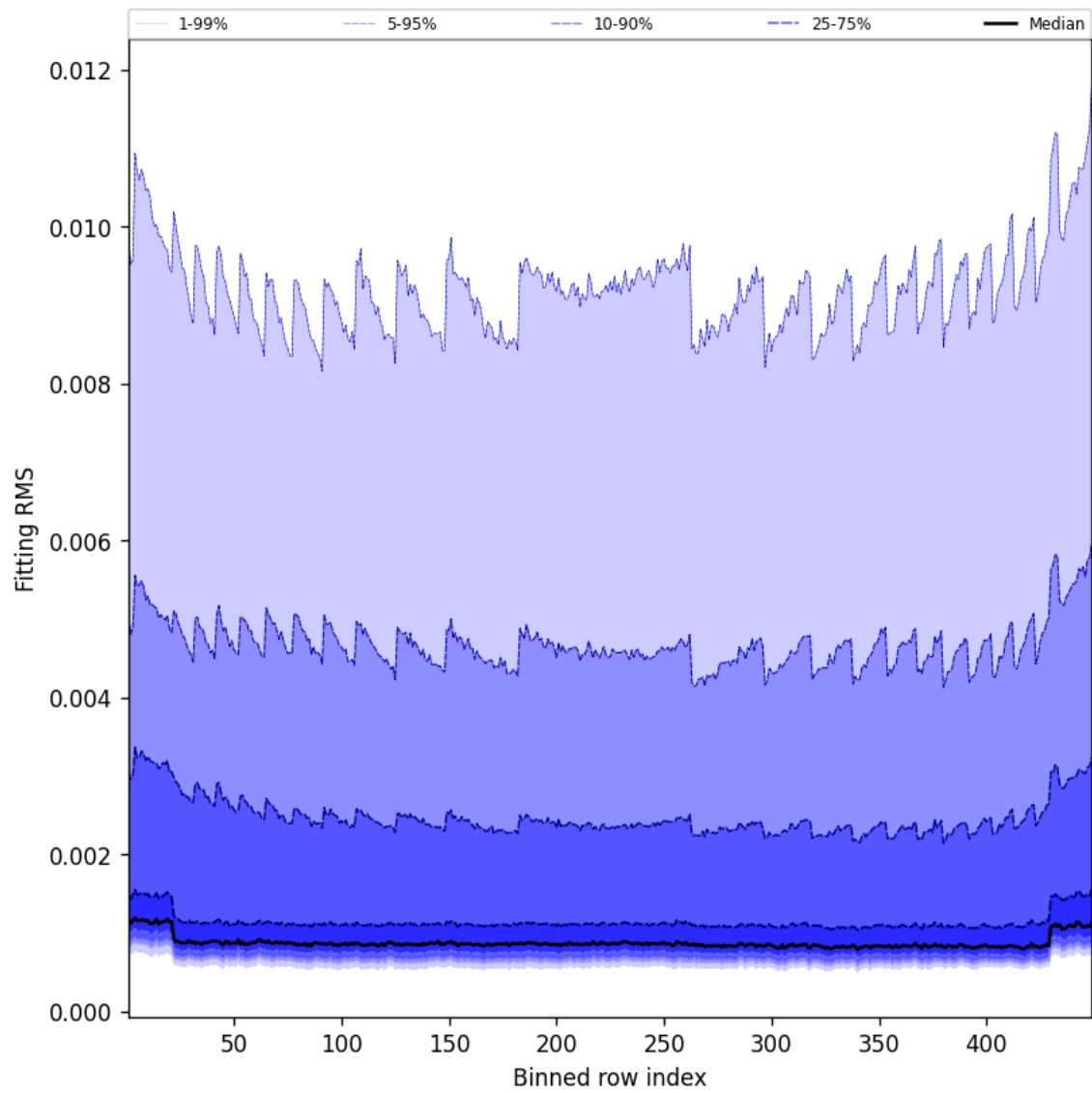
Figure 46: Along track statistics of “Fitting RMS” for 2024-12-02 to 2024-12-03
