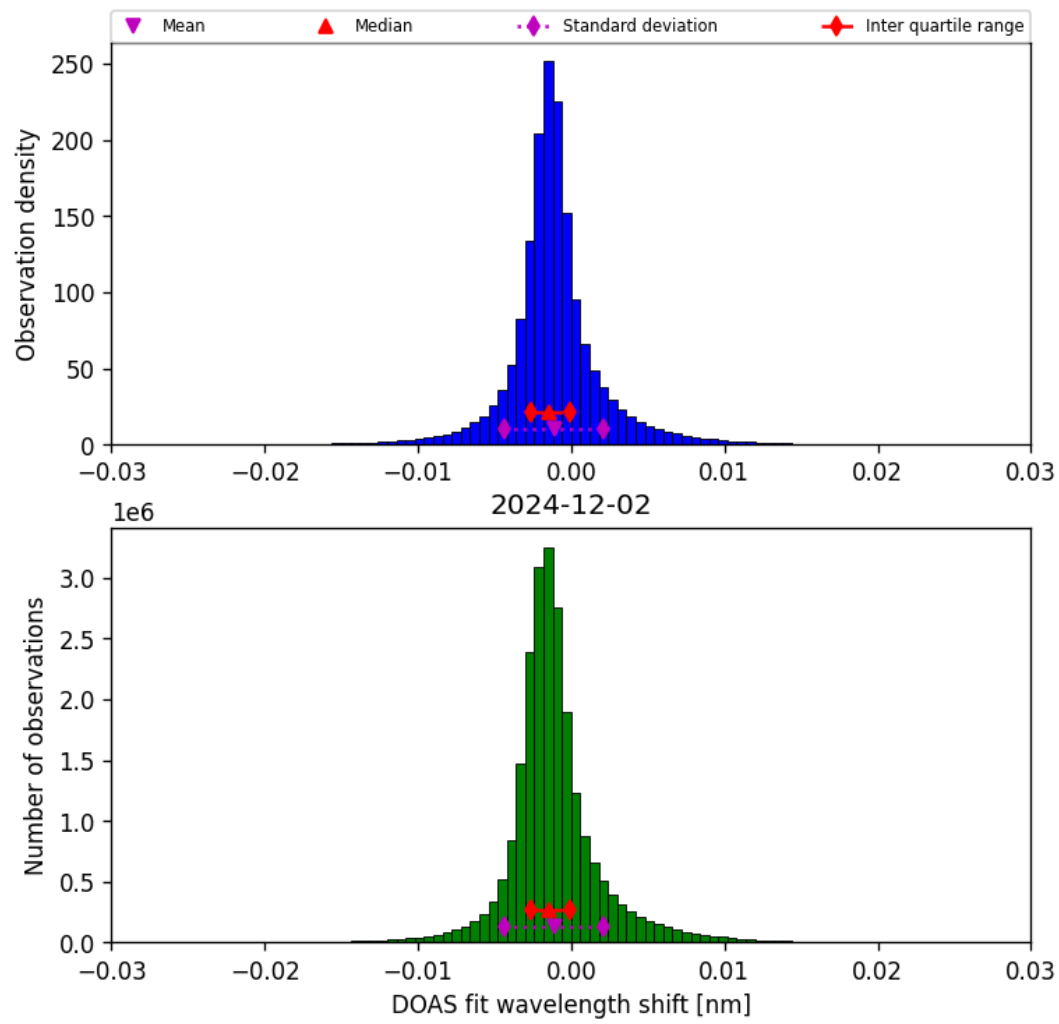
Figure 35: Histogram of “DOAS fit wavelength shift” for 2024-12-02 to 2024-12-03
