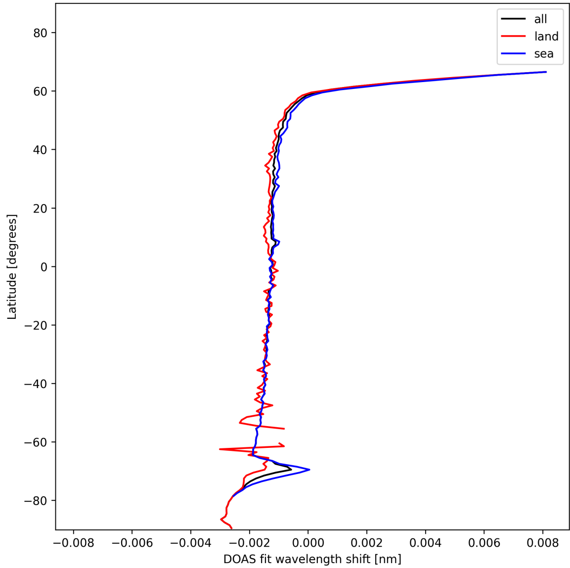
Figure 23: Zonal average of “DOAS fit wavelength shift” for 2024-12-02 to 2024-12-03.
