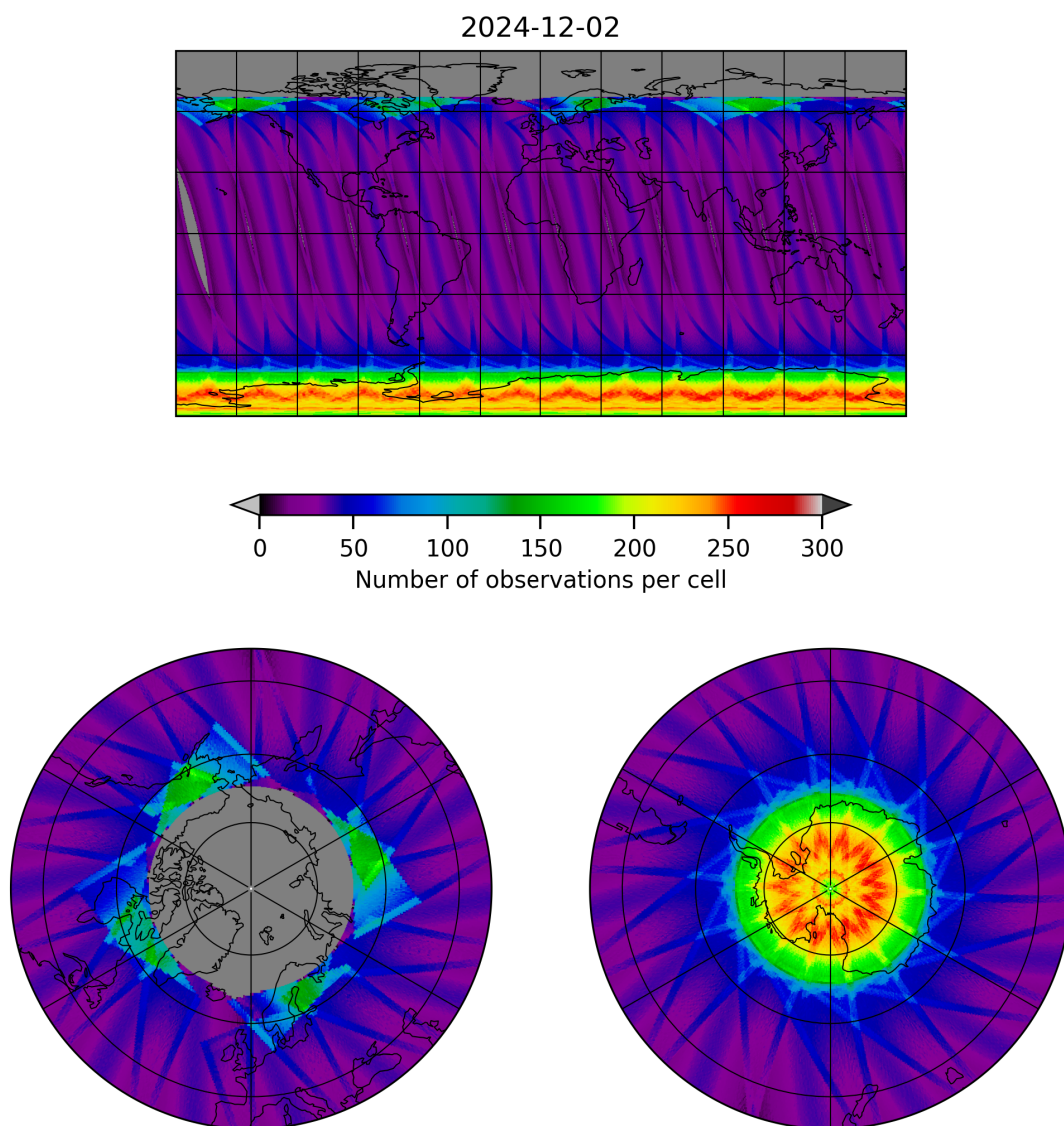
Figure 15: Map of the number of observations for 2024-12-02 to 2024-12-03
