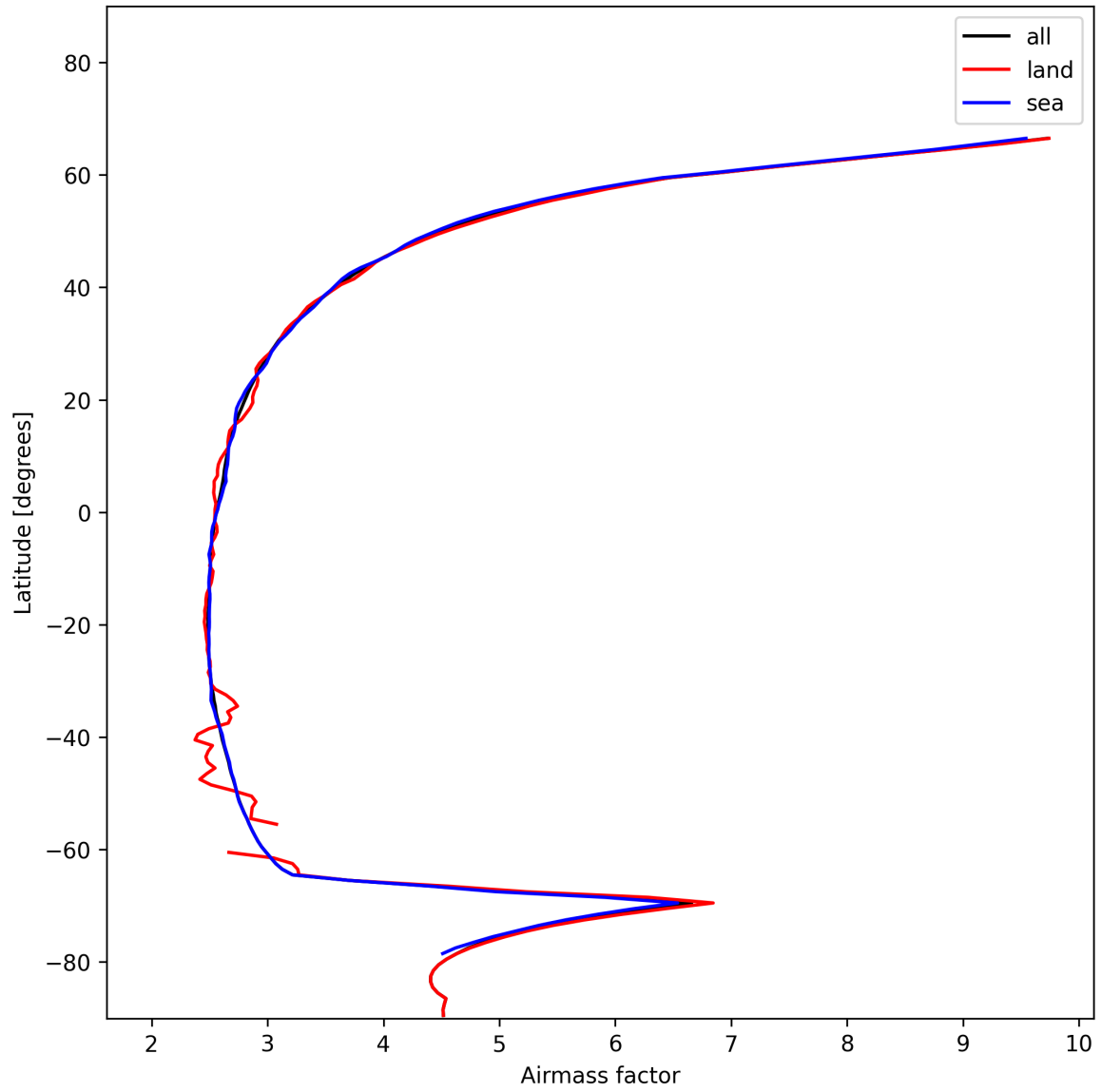
Figure 25: Zonal average of “Airmass factor” for 2024-12-02 to 2024-12-03.
