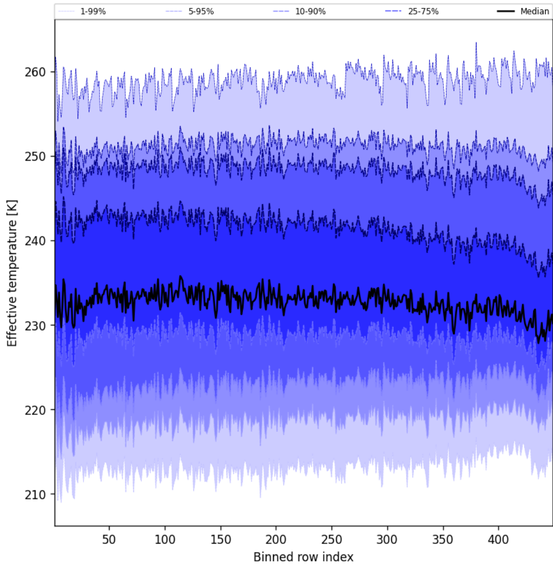
Figure 50: Along track statistics of “Effective temperature” for 2024-12-02 to 2024-12-03
