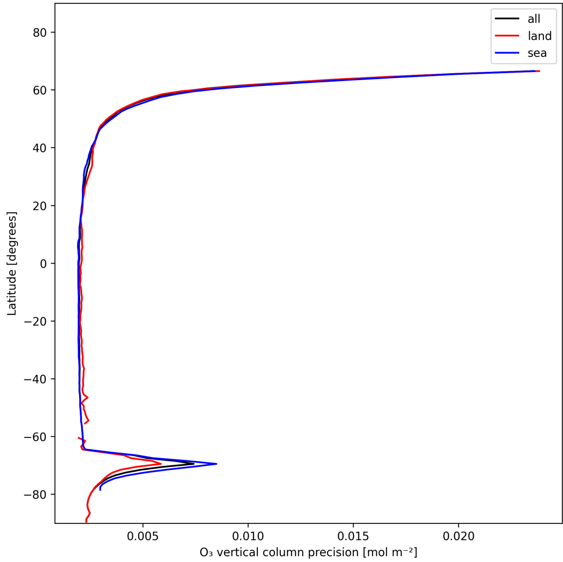
Figure 18: Zonal average of “O 3 vertical column precision” for 2024-12-02 to 2024-12-03.
