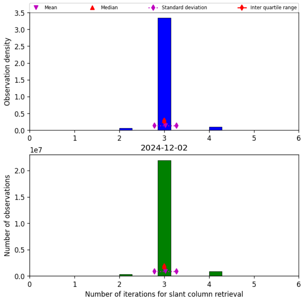
Figure 33: Histogram of “Number of iterations for slant column retrieval” for 2024-12-02 to 2024-12-03
