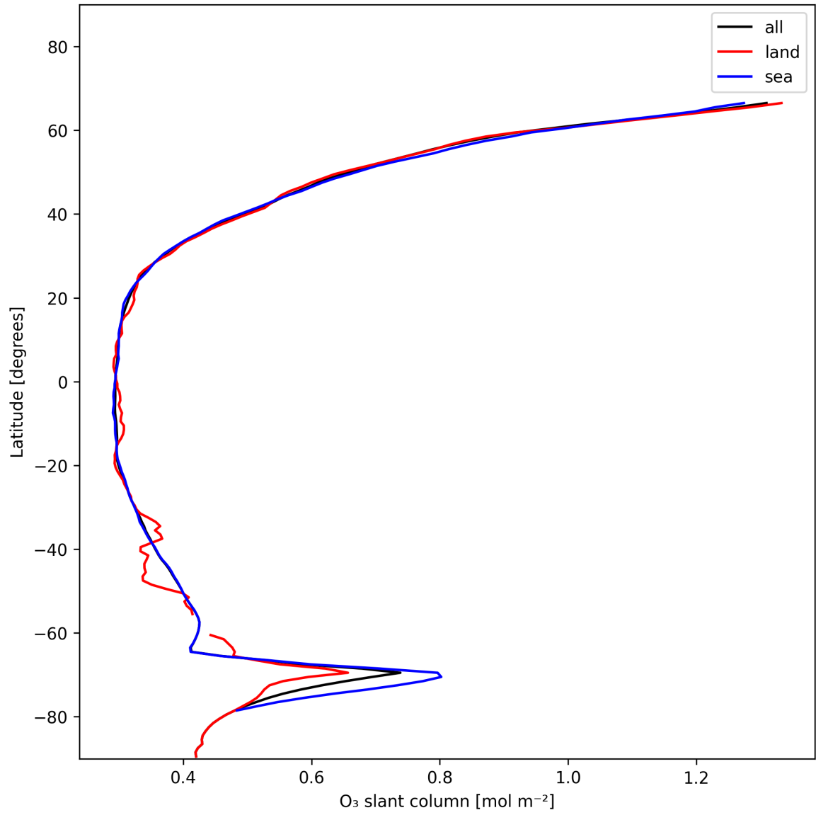
Figure 19: Zonal average of “O 3 slant column” for 2024-12-02 to 2024-12-03.
