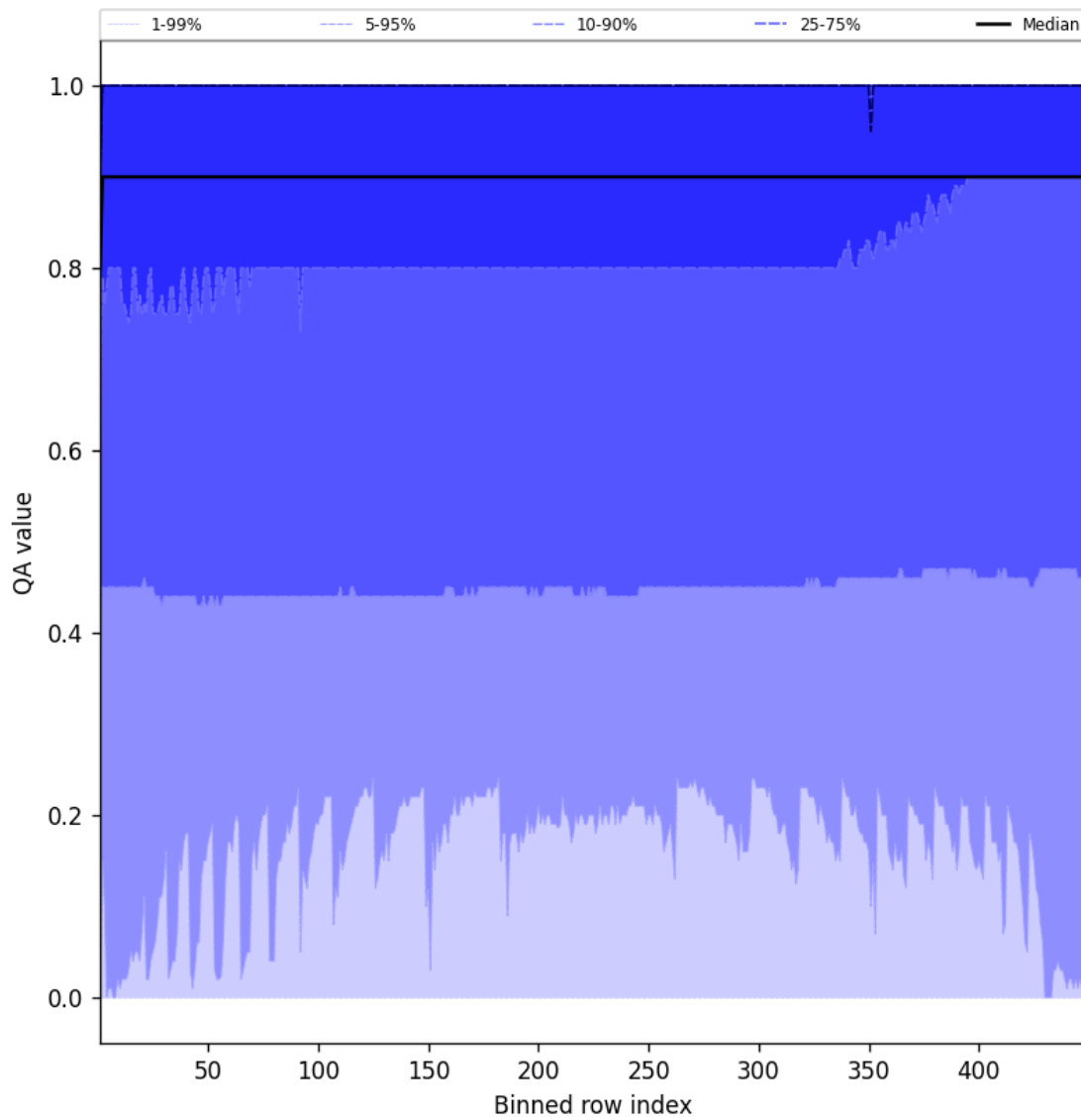
Figure 40: Along track statistics of “QA value” for 2024-12-02 to 2024-12-03
