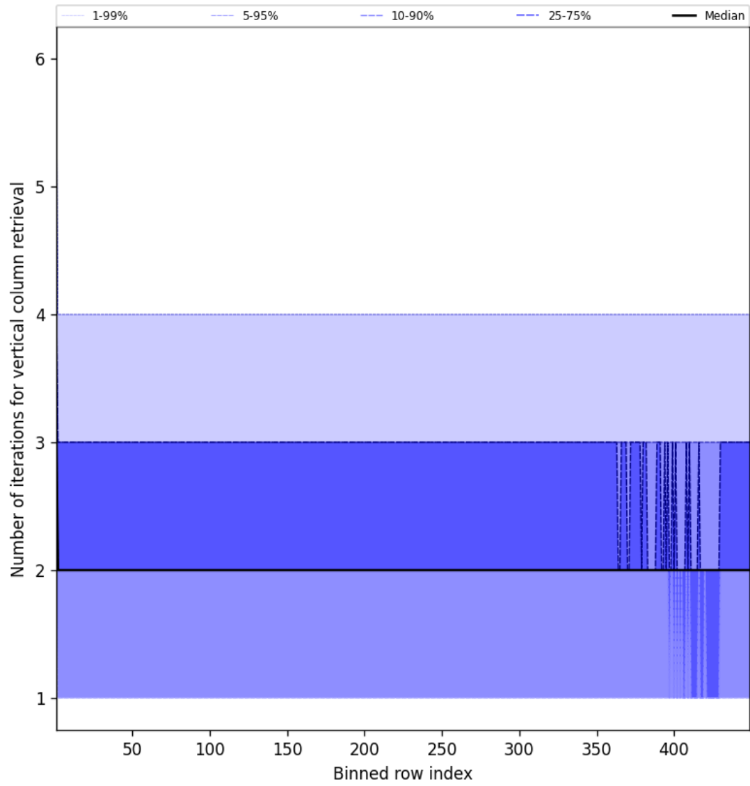
Figure 51: Along track statistics of “Number of iterations for vertical column retrieval” for 2024-12-02 to 2024-12-03
