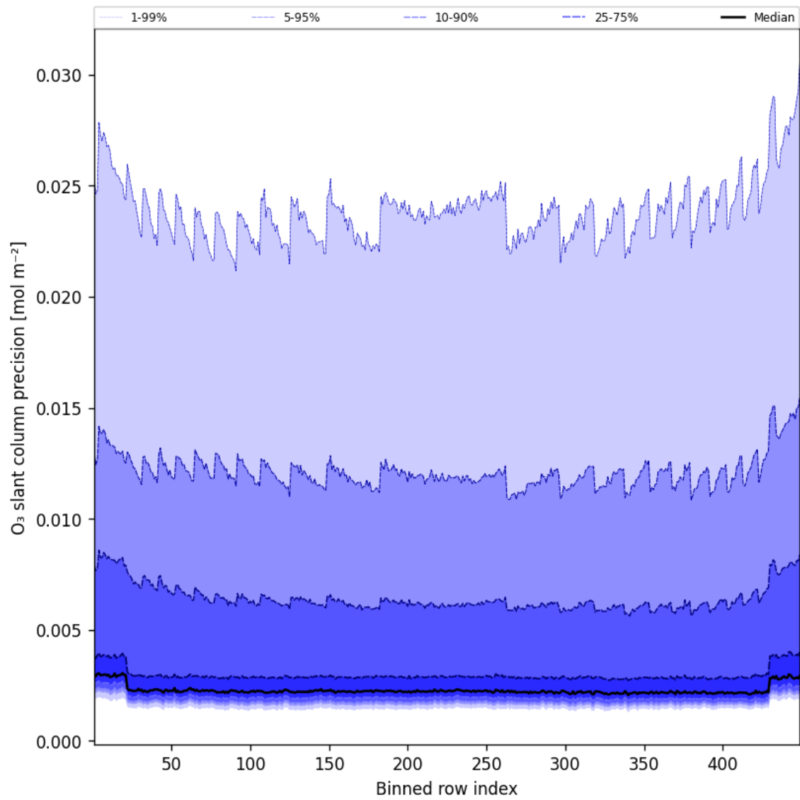
Figure 44: Along track statistics of “O 3 slant column precision” for 2024-12-02 to 2024-12-03
