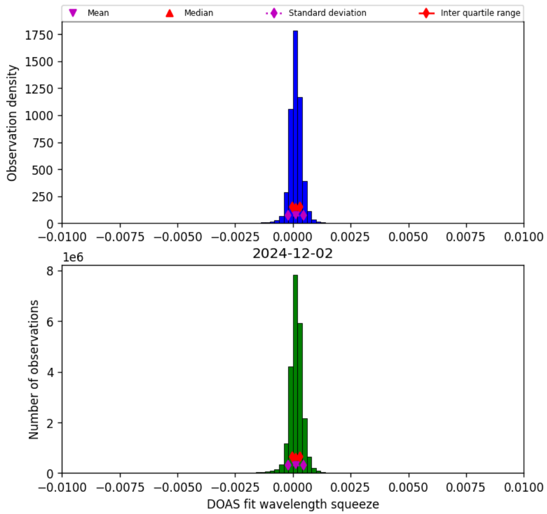
Figure 36: Histogram of “DOAS fit wavelength squeeze” for 2024-12-02 to 2024-12-03
