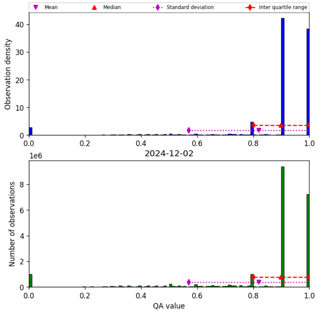
Figure 28: Histogram of “QA value” for 2024-12-02 to 2024-12-03
