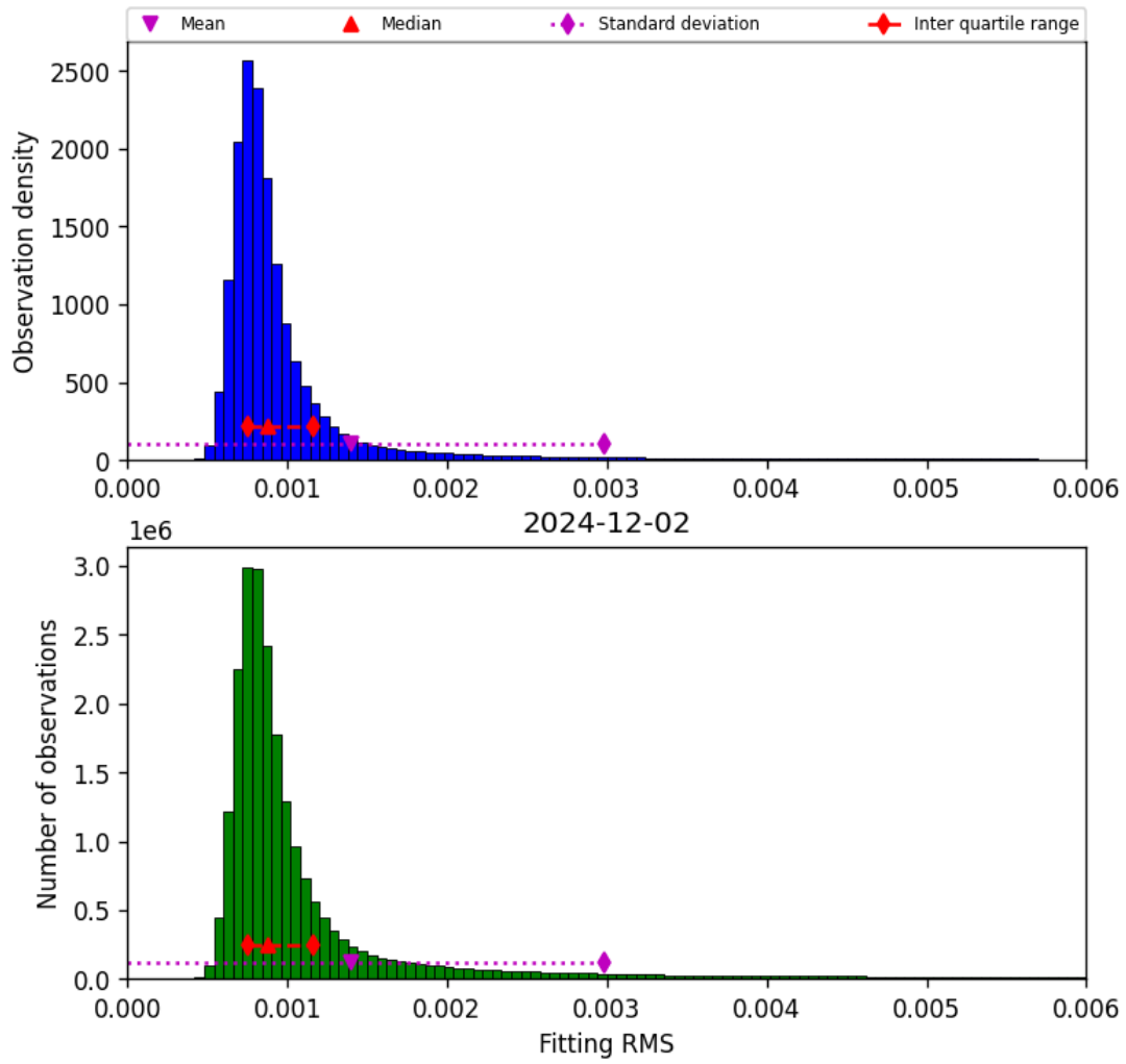
Figure 34: Histogram of “Fitting RMS” for 2024-12-02 to 2024-12-03
