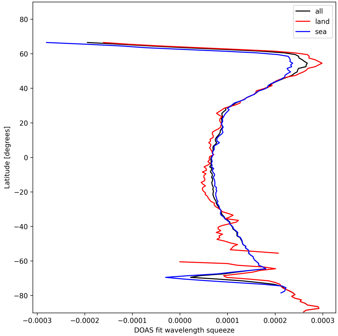
Figure 24: Zonal average of “DOAS fit wavelength squeeze” for 2024-12-02 to 2024-12-03.
