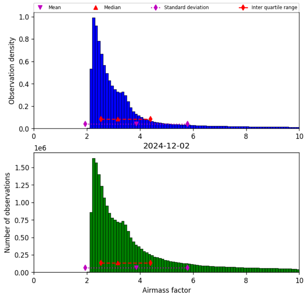
Figure 37: Histogram of "Airmass factor" for 2024-12-02 to 2024-12-03
