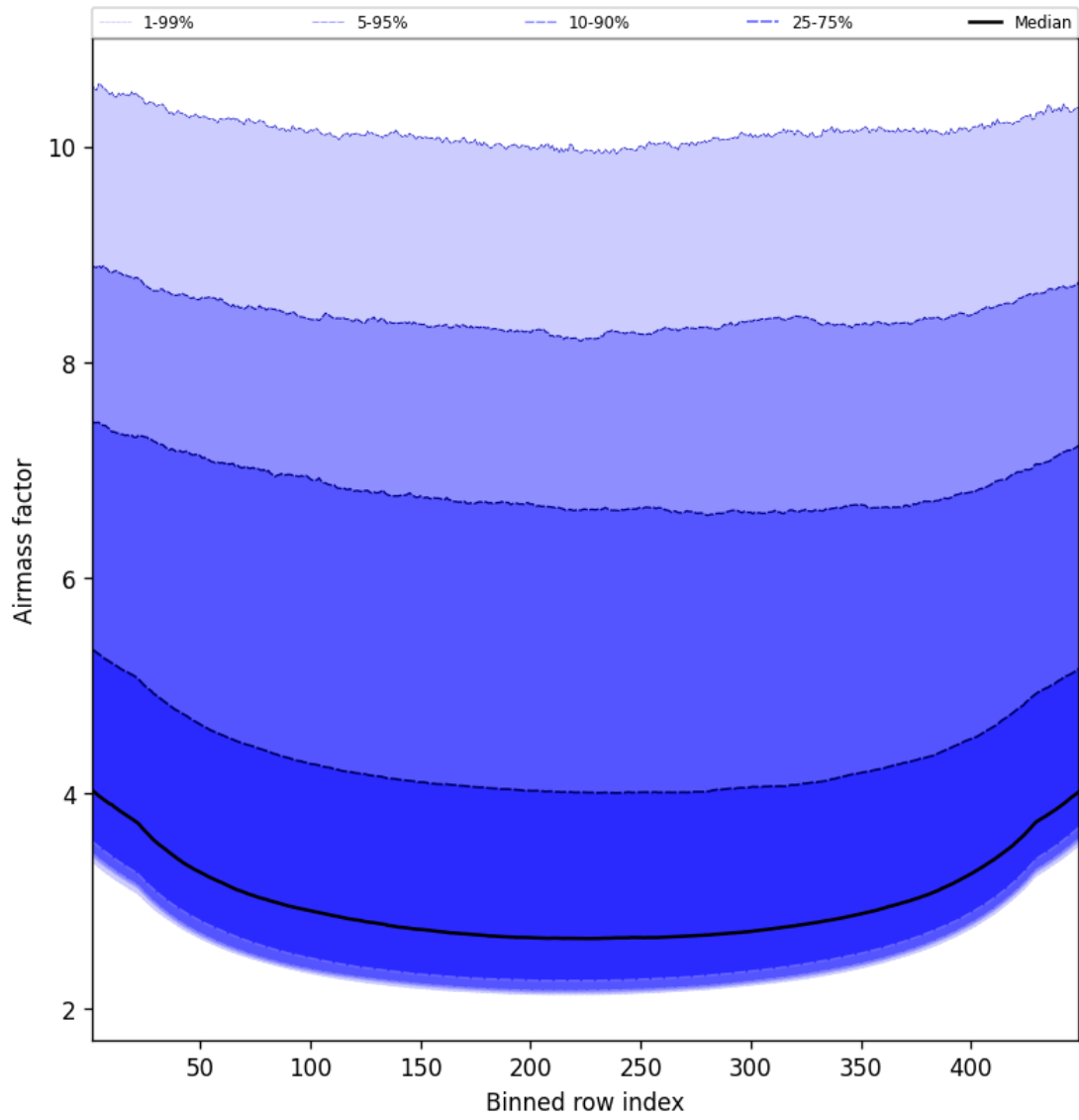
Figure 49: Along track statistics of “Airmass factor” for 2024-12-02 to 2024-12-03
