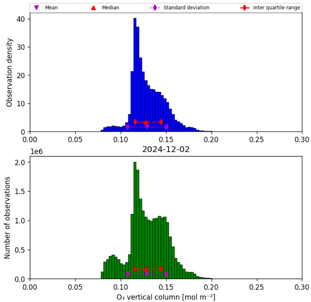
Figure 29: Histogram of “O 3 vertical column” for 2024-12-02 to 2024-12-03
