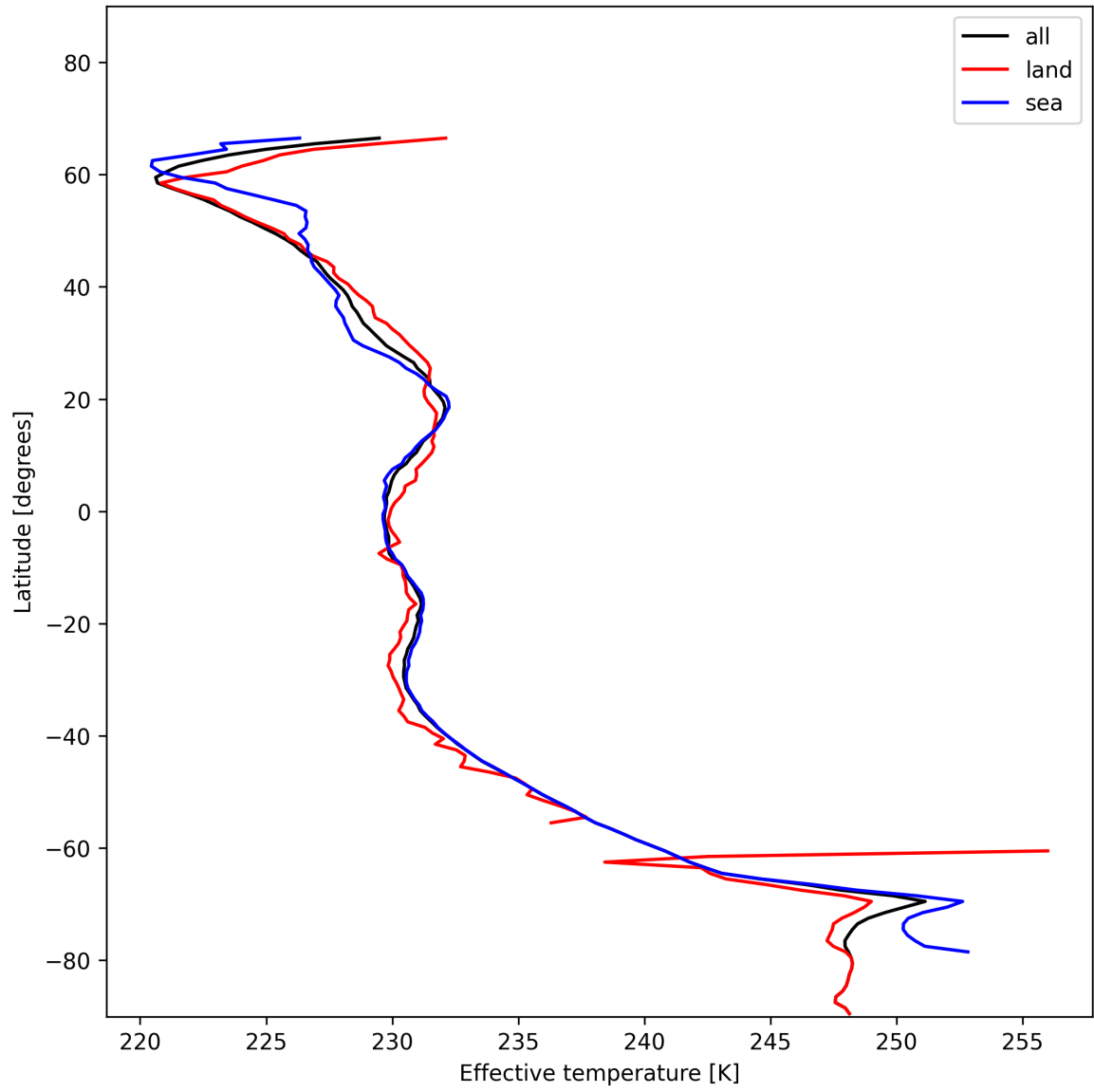
Figure 26: Zonal average of “Effective temperature” for 2024-12-02 to 2024-12-03.
