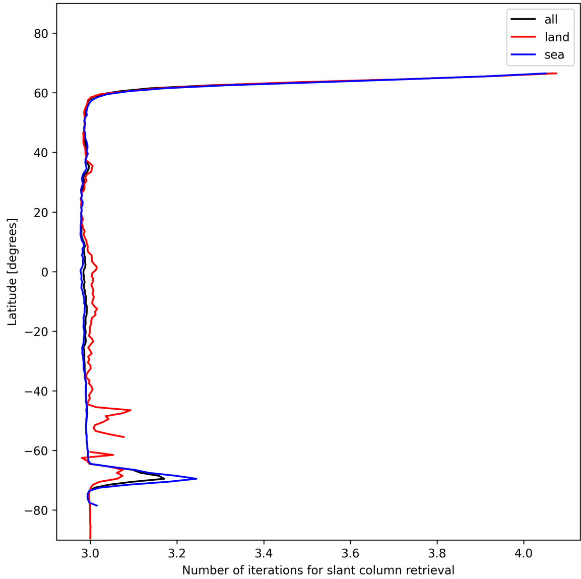
Figure 21: Zonal average of “Number of iterations for slant column retrieval” for 2024-12-02 to 2024-12-03.
