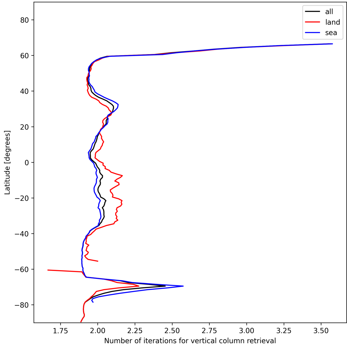
Figure 27: Zonal average of “Number of iterations for vertical column retrieval” for 2024-12-02 to 2024-12-03.
