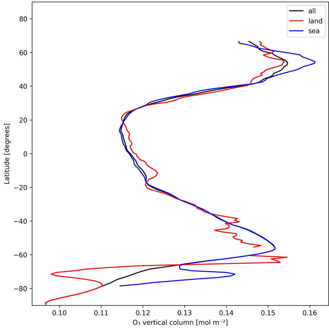
Figure 17: Zonal average of “O 3 vertical column” for 2024-12-02 to 2024-12-03.
