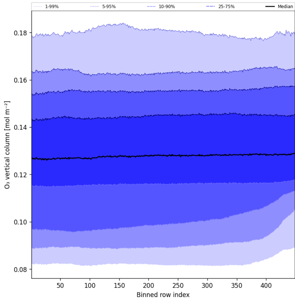
Figure 41: Along track statistics of “O 3 vertical column” for 2024-12-02 to 2024-12-03
