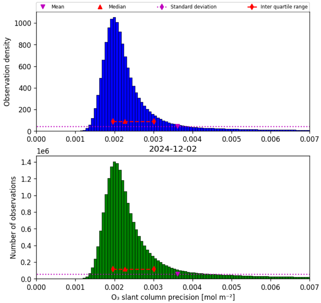
Figure 32: Histogram of “O 3 slant column precision” for 2024-12-02 to 2024-12-03
