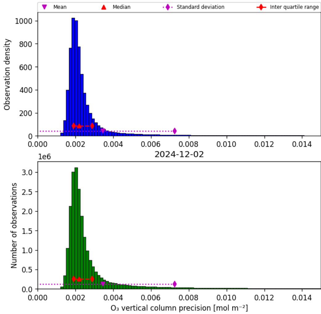
Figure 30: Histogram of “O 3 vertical column precision” for 2024-12-02 to 2024-12-03
