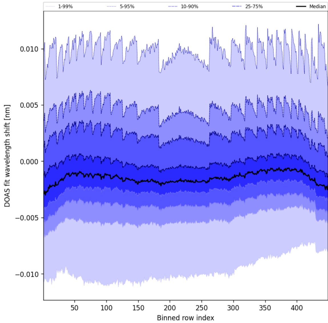
Figure 47: Along track statistics of “DOAS fit wavelength shift” for 2024-12-02 to 2024-12-03
