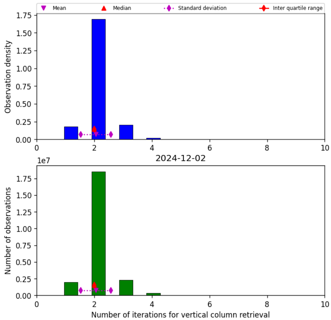
Figure 39: Histogram of “Number of iterations for vertical column retrieval” for 2024-12-02 to 2024-12-03
