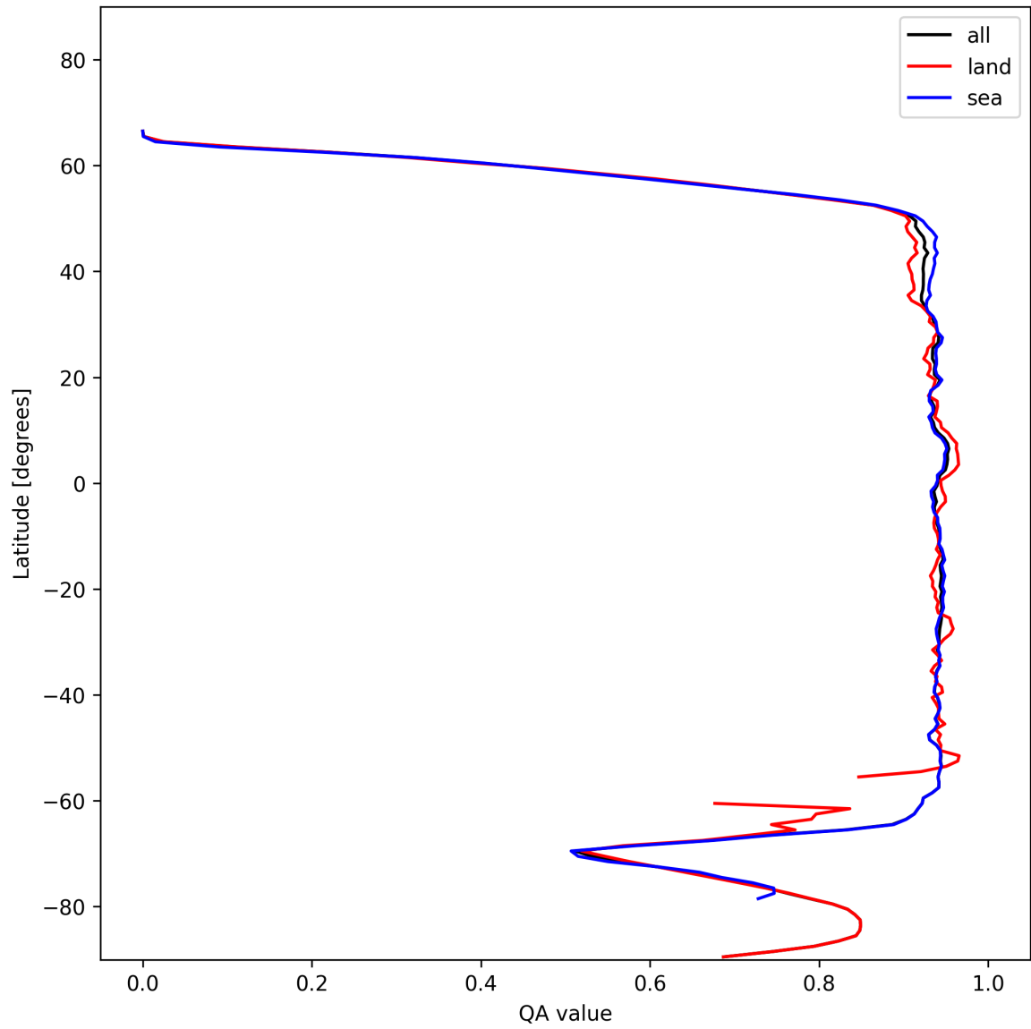
Figure 16: Zonal average of “QA value” for 2024-12-02 to 2024-12-03.
