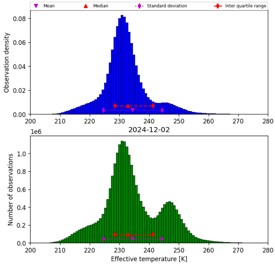
Figure 38: Histogram of “Effective temperature” for 2024-12-02 to 2024-12-03
