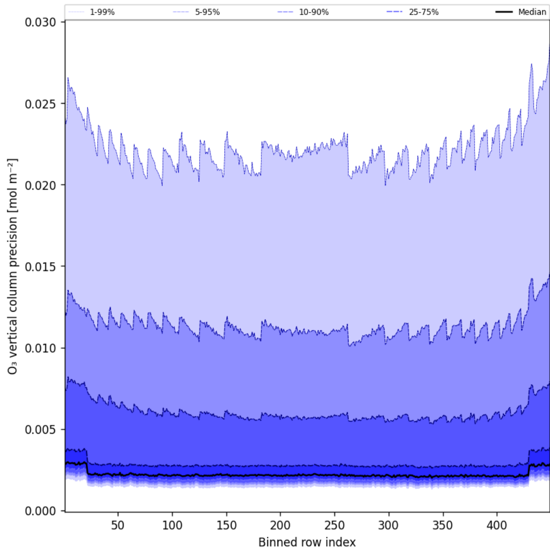
Figure 42: Along track statistics of “O 3 vertical column precision” for 2024-12-02 to 2024-12-03
