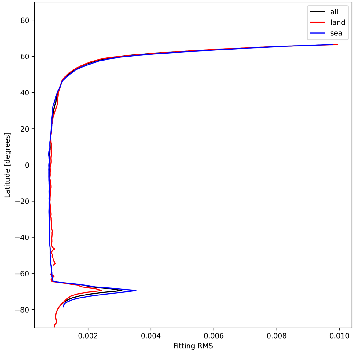
Figure 22: Zonal average of “Fitting RMS” for 2024-12-02 to 2024-12-03.
