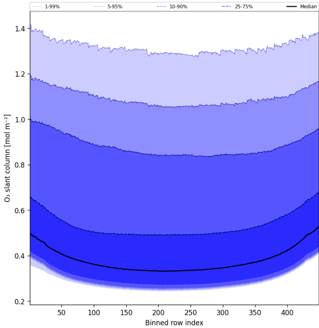
Figure 43: Along track statistics of “O 3 slant column” for 2024-12-02 to 2024-12-03
