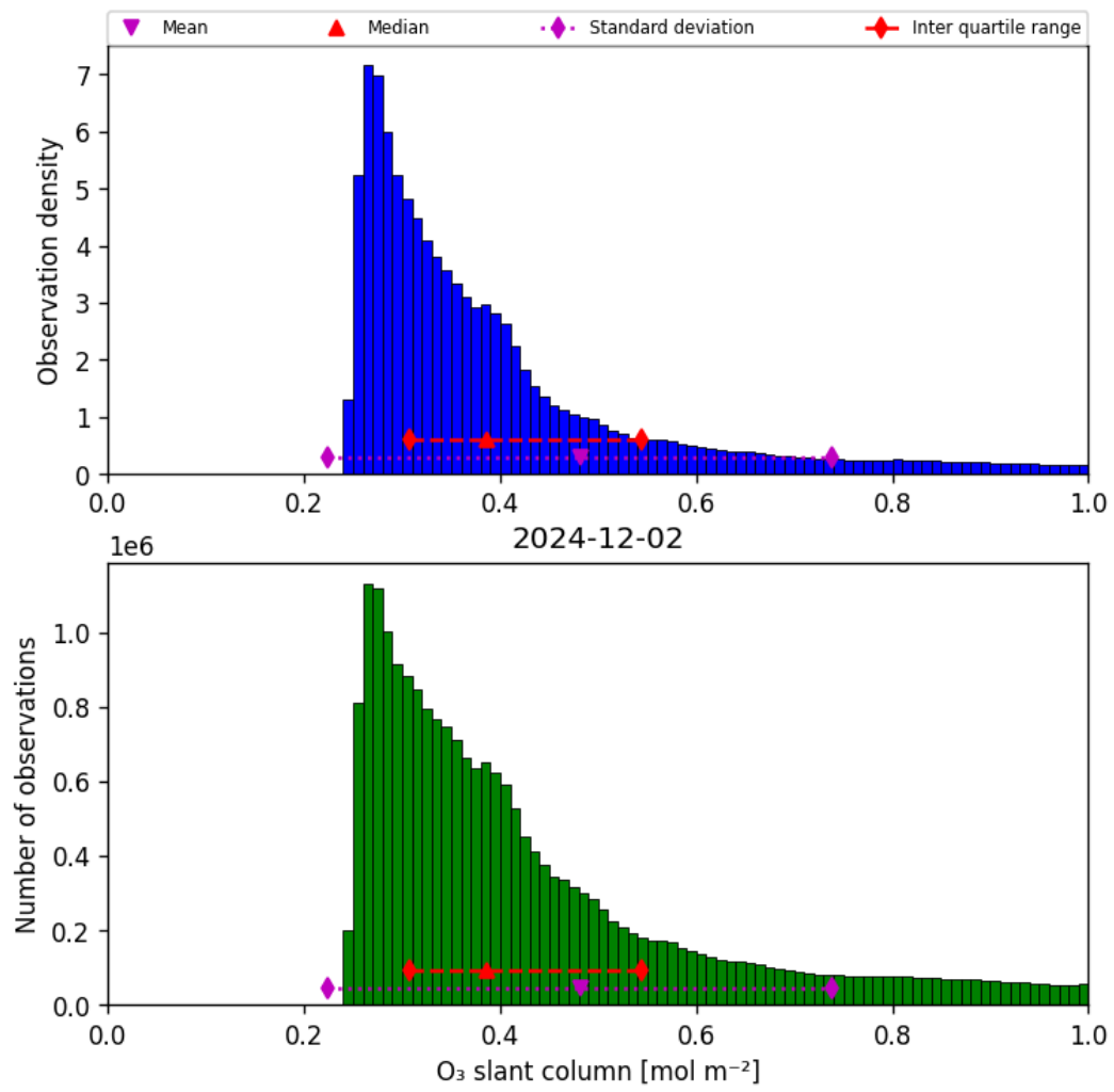
Figure 31: Histogram of “O 3 slant column” for 2024-12-02 to 2024-12-03
