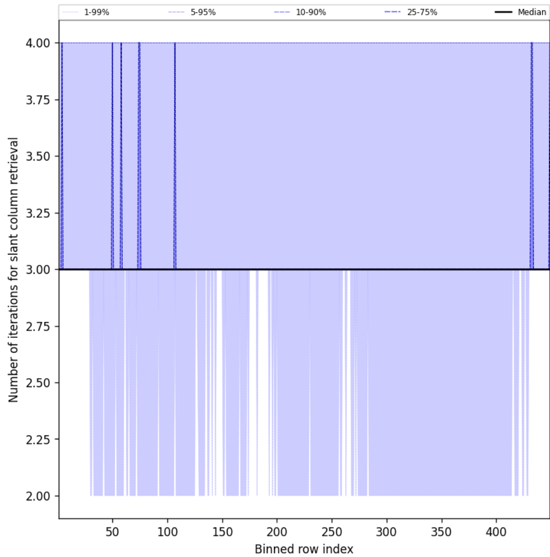
Figure 45: Along track statistics of “Number of iterations for slant column retrieval” for 2024-12-02 to 2024-12-03
