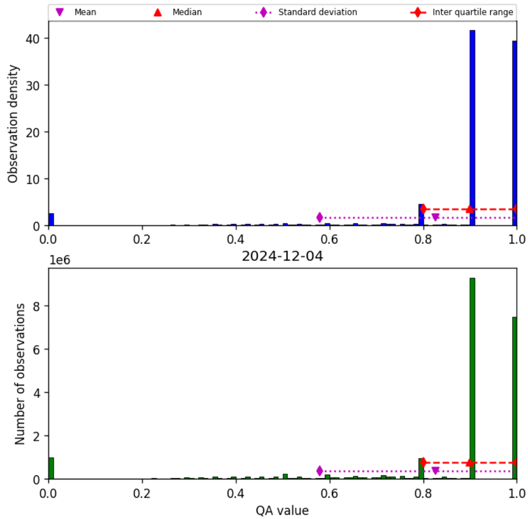
Figure 28: Histogram of “QA value” for 2024-12-04 to 2024-12-04
