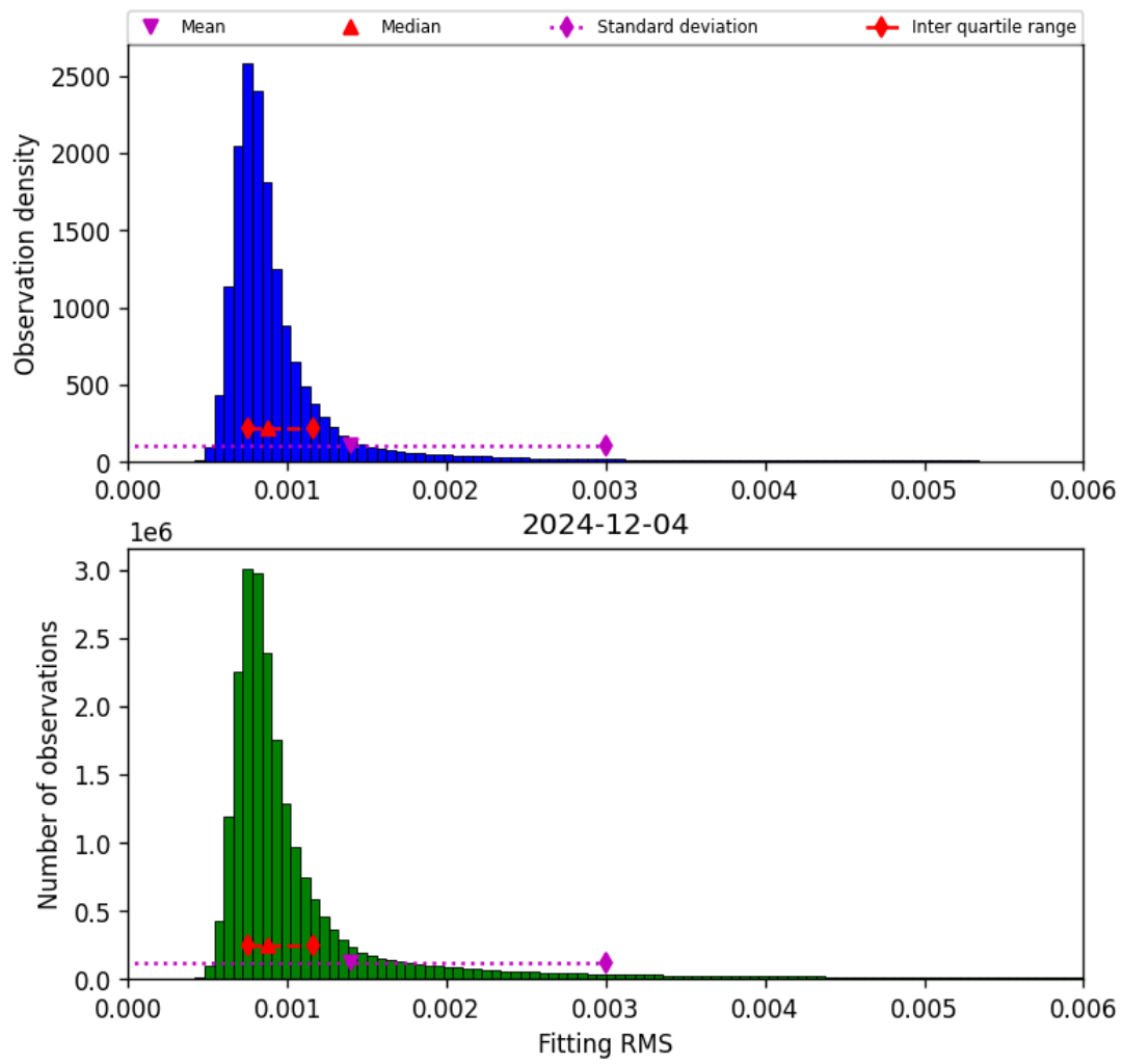
Figure 34: Histogram of “Fitting RMS” for 2024-12-04 to 2024-12-04
