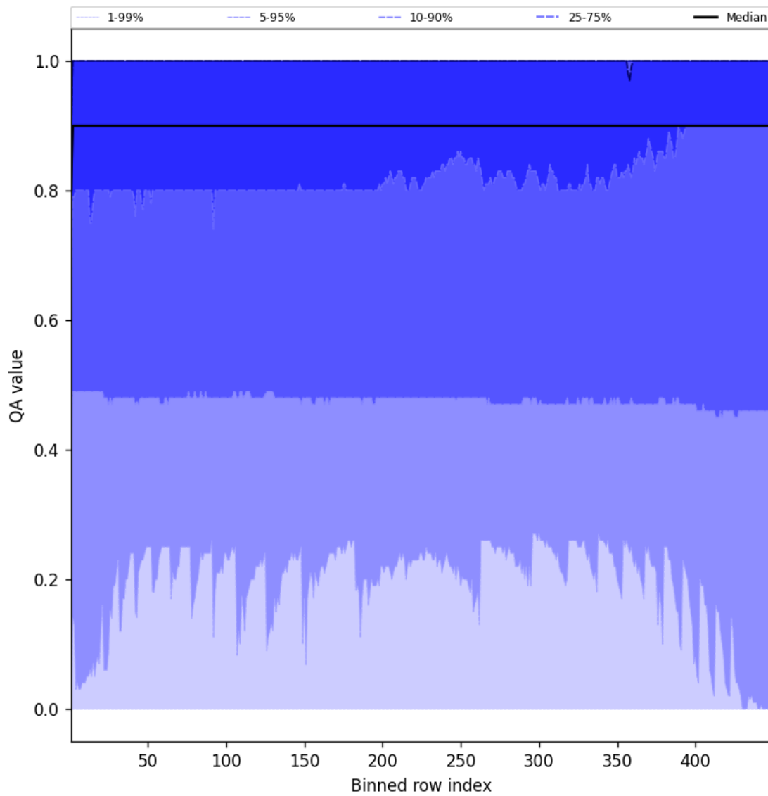
Figure 40: Along track statistics of “QA value” for 2024-12-04 to 2024-12-04
