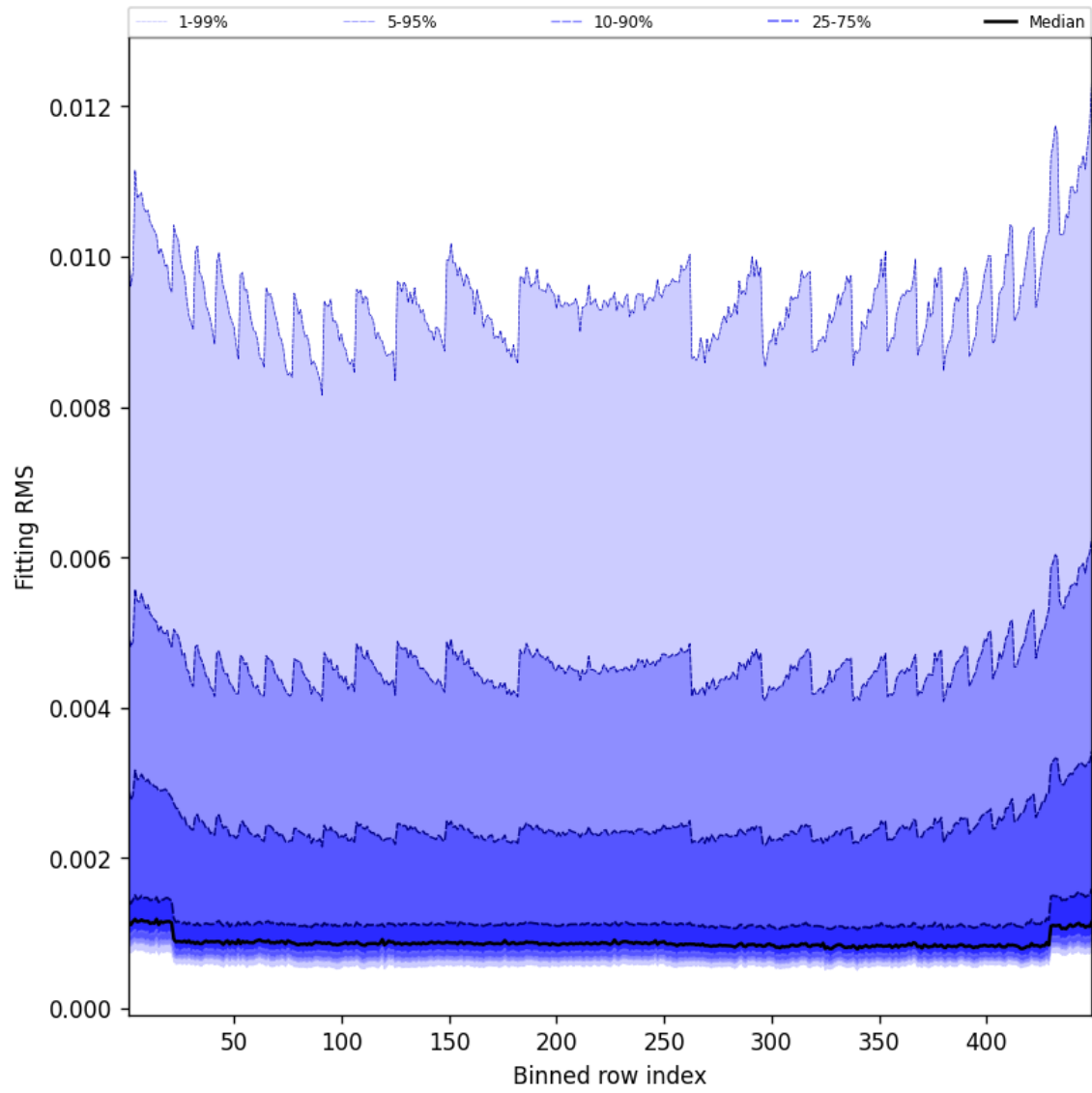
Figure 46: Along track statistics of “Fitting RMS” for 2024-12-04 to 2024-12-04
