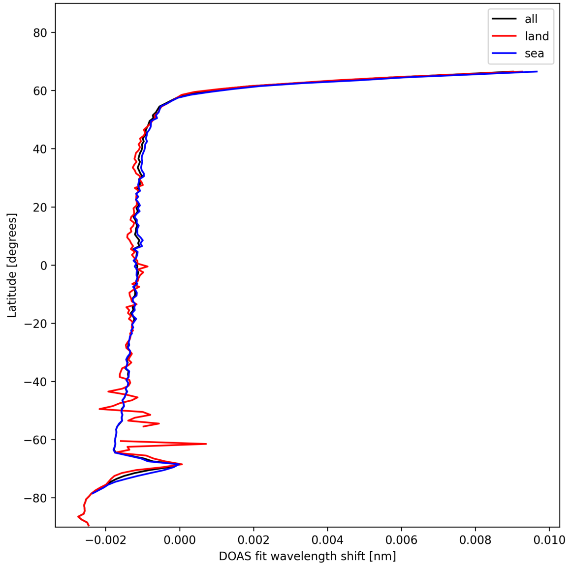
Figure 23: Zonal average of “DOAS fit wavelength shift” for 2024-12-04 to 2024-12-04.
