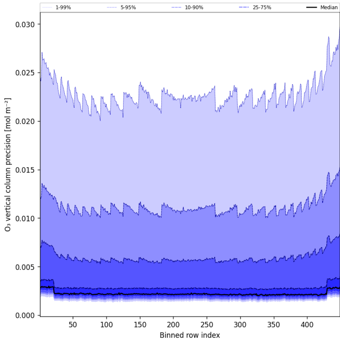
Figure 42: Along track statistics of “O 3 vertical column precision” for 2024-12-04 to 2024-12-04
