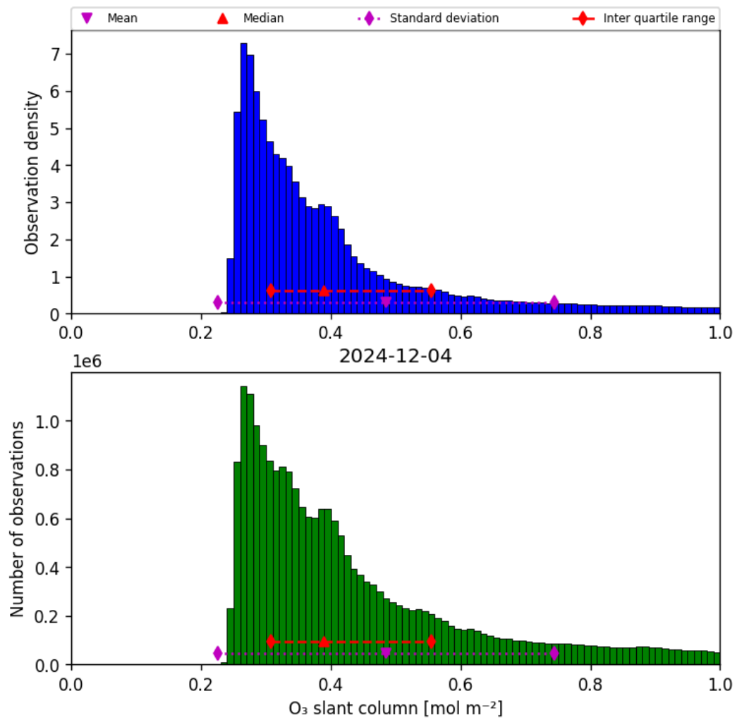
Figure 31: Histogram of “O 3 slant column” for 2024-12-04 to 2024-12-04
