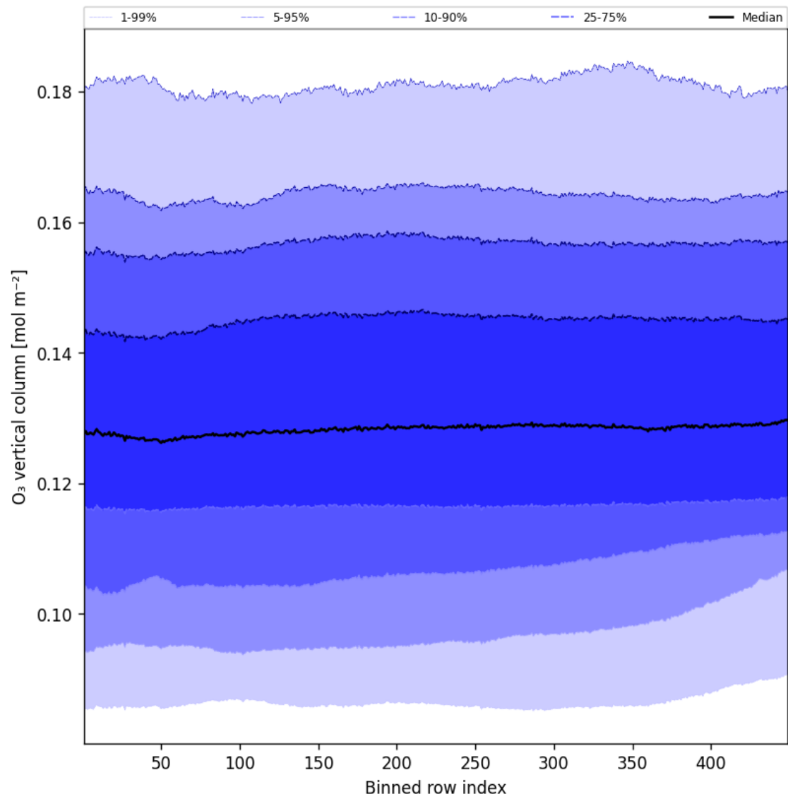
Figure 41: Along track statistics of “O 3 vertical column” for 2024-12-04 to 2024-12-04
