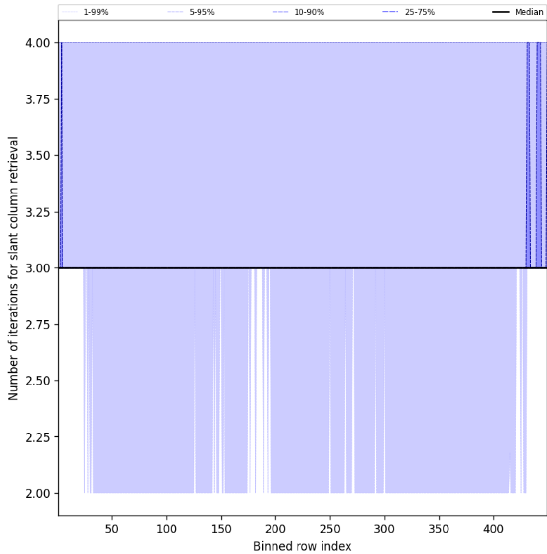
Figure 45: Along track statistics of “Number of iterations for slant column retrieval” for 2024-12-04 to 2024-12-04
