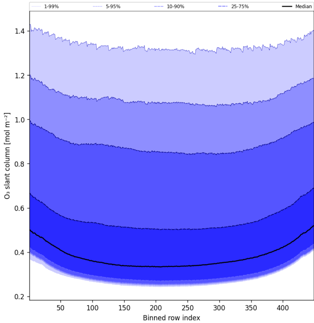
Figure 43: Along track statistics of “O 3 slant column” for 2024-12-04 to 2024-12-04
