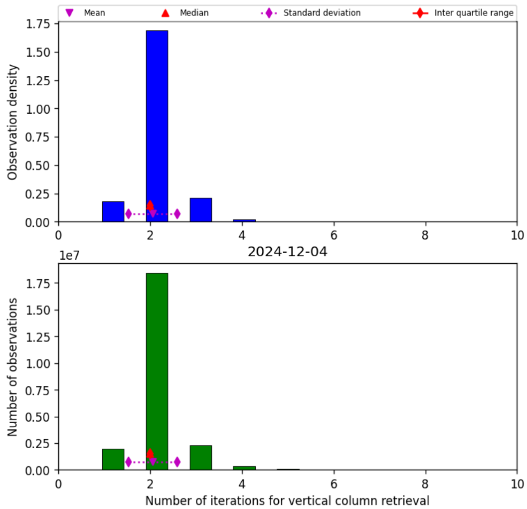
Figure 39: Histogram of “Number of iterations for vertical column retrieval” for 2024-12-04 to 2024-12-04
