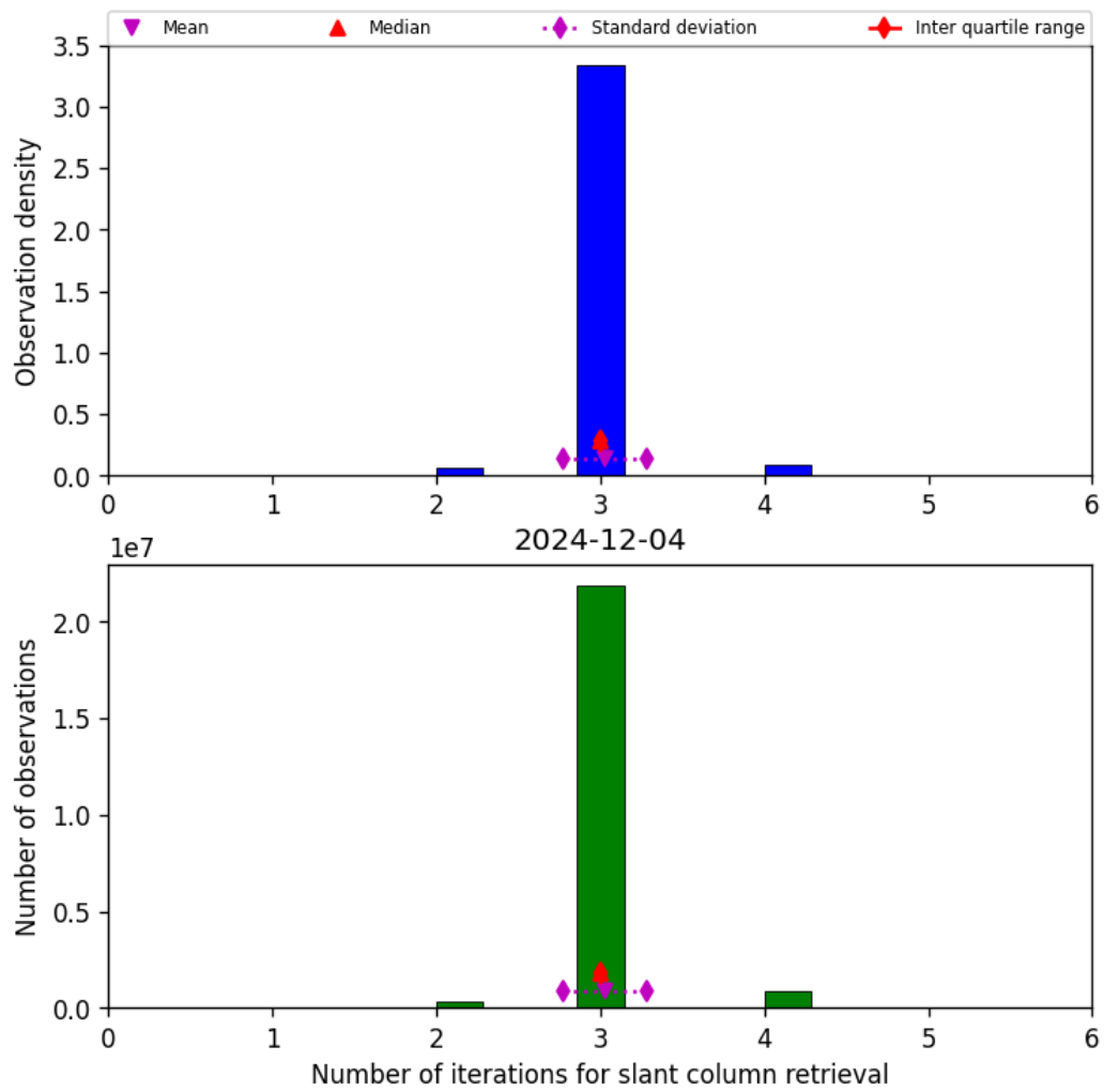
Figure 33: Histogram of “Number of iterations for slant column retrieval” for 2024-12-04 to 2024-12-04
