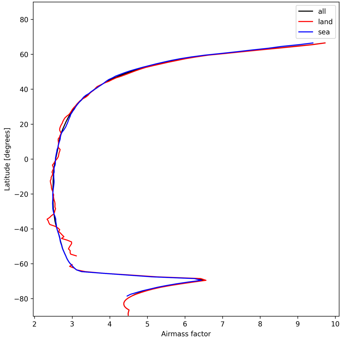
Figure 25: Zonal average of “Airmass factor” for 2024-12-04 to 2024-12-04.
