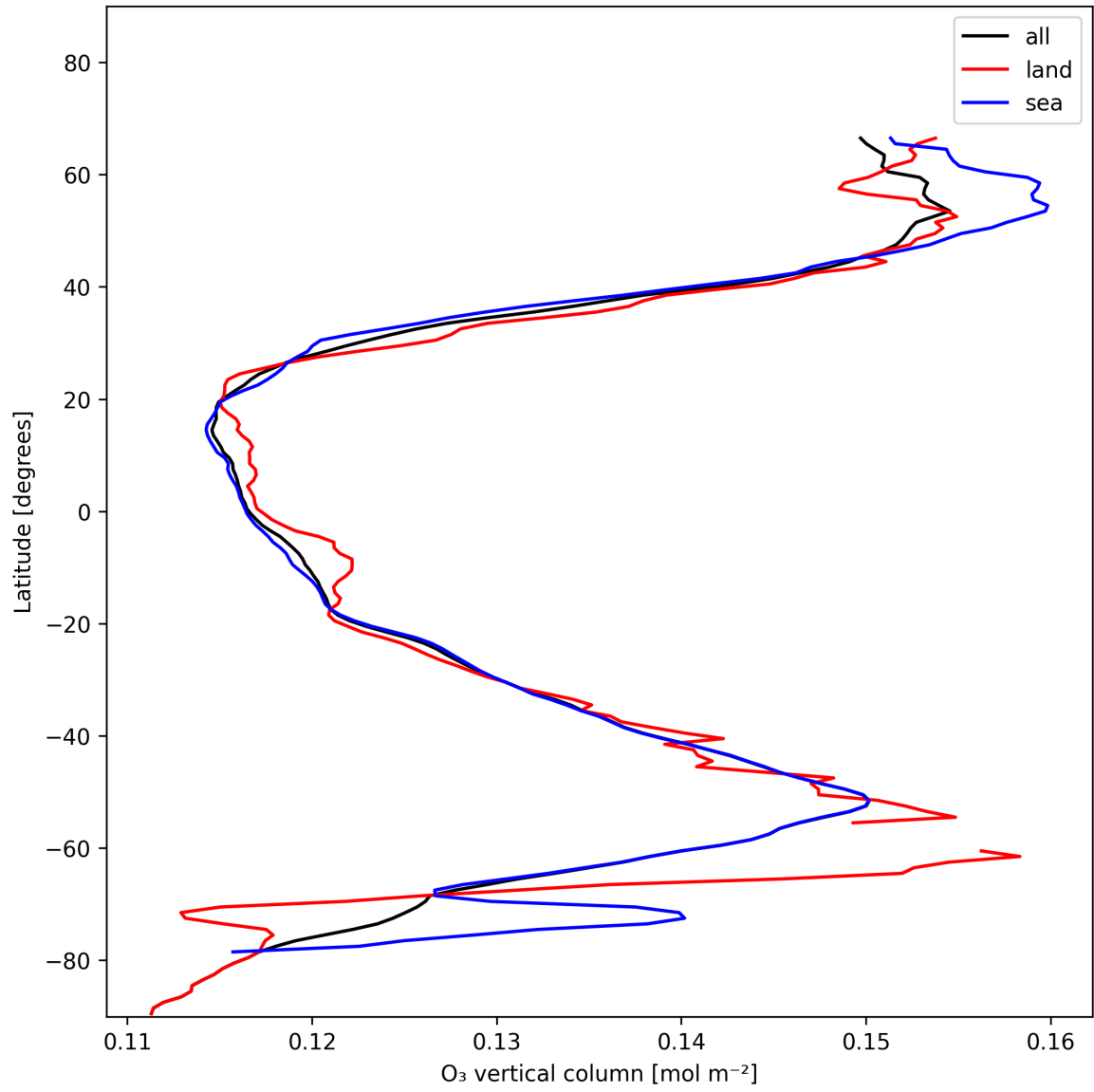
Figure 17: Zonal average of “O 3 vertical column” for 2024-12-04 to 2024-12-04.
