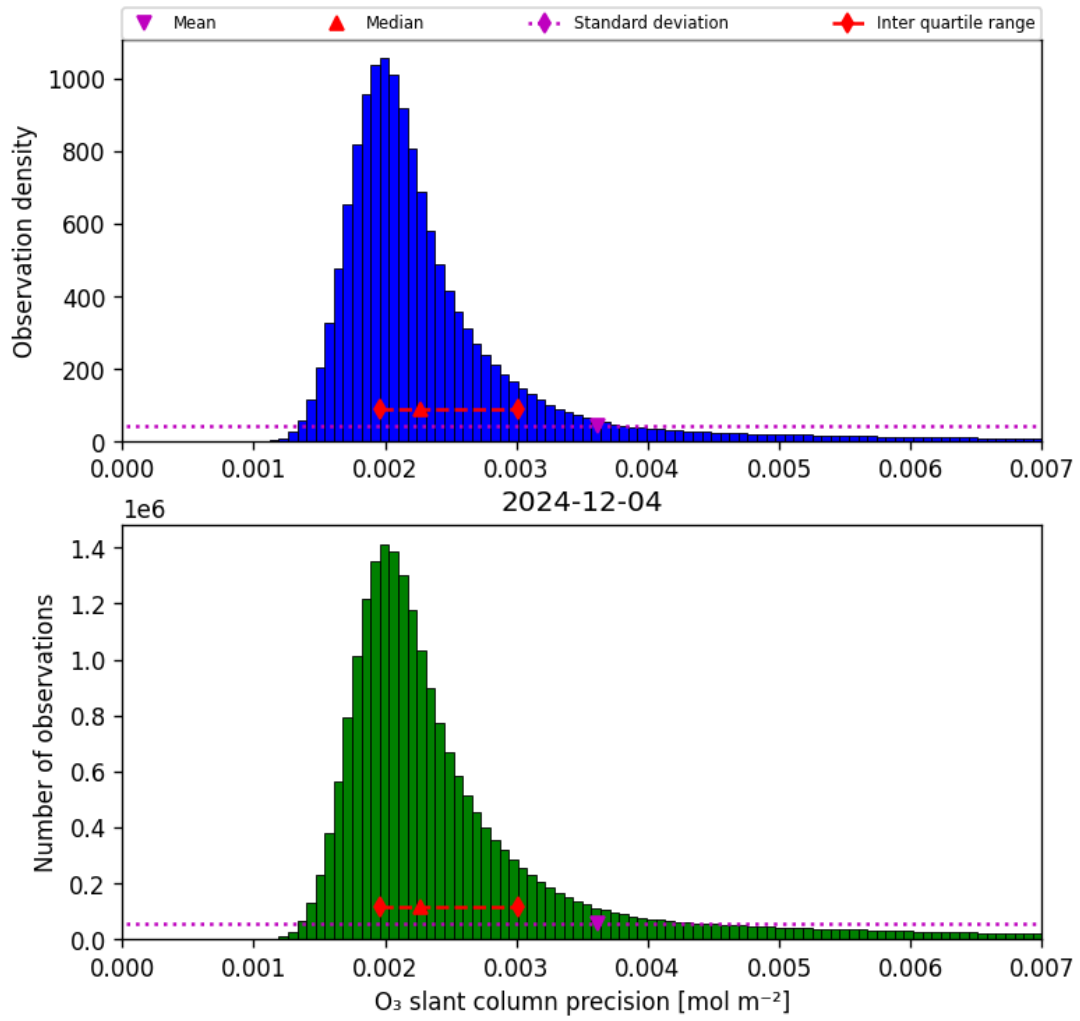
Figure 32: Histogram of “O 3 slant column precision” for 2024-12-04 to 2024-12-04
