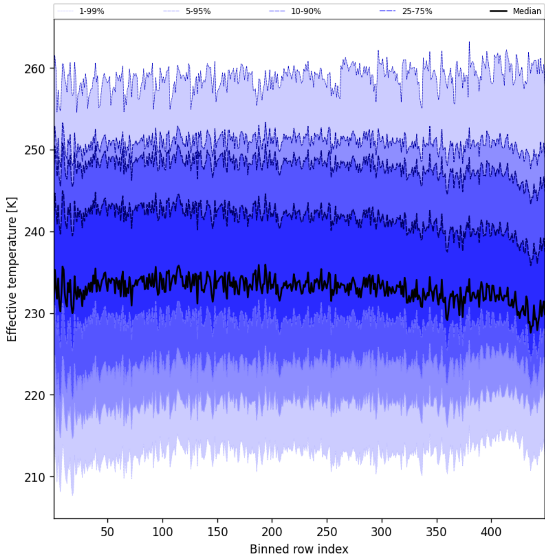
Figure 50: Along track statistics of “Effective temperature” for 2024-12-04 to 2024-12-04
