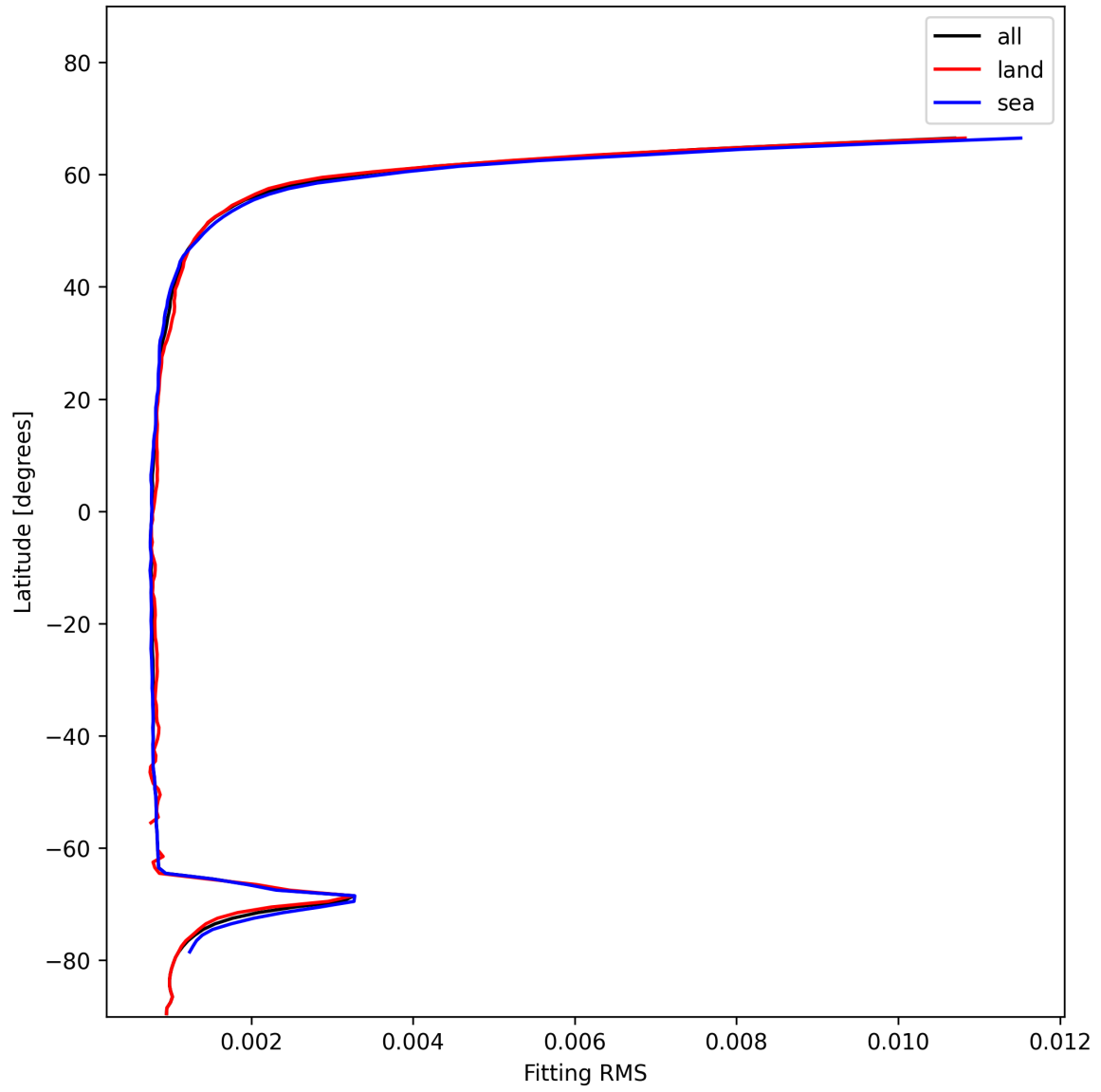
Figure 22: Zonal average of “Fitting RMS” for 2024-12-04 to 2024-12-04.
