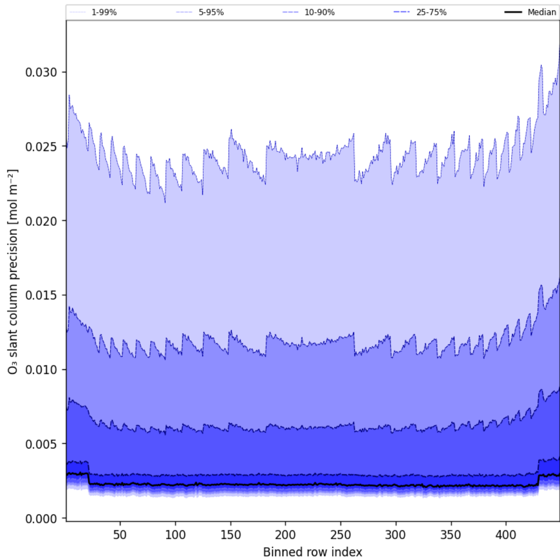
Figure 44: Along track statistics of “O 3 slant column precision” for 2024-12-04 to 2024-12-04
