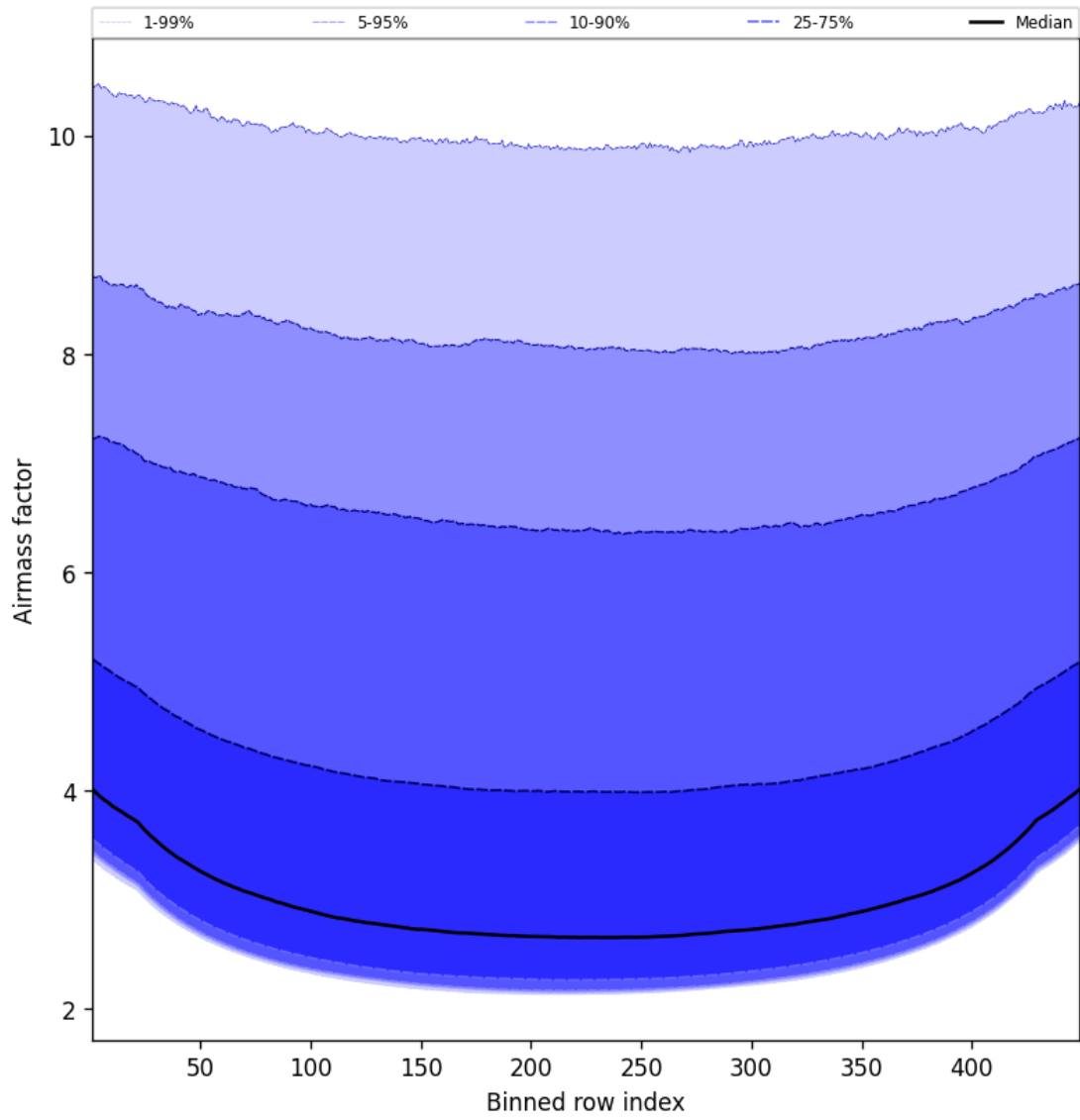
Figure 49: Along track statistics of “Airmass factor” for 2024-12-04 to 2024-12-04
