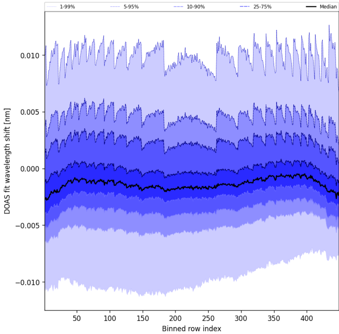
Figure 47: Along track statistics of “DOAS fit wavelength shift” for 2024-12-04 to 2024-12-04
