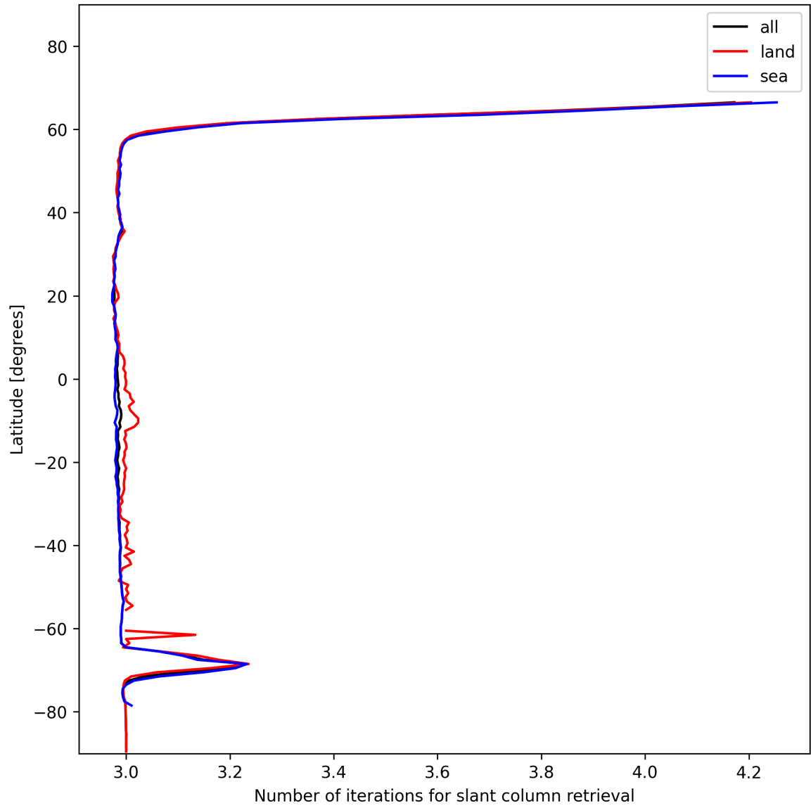
Figure 21: Zonal average of “Number of iterations for slant column retrieval” for 2024-12-04 to 2024-12-04.
