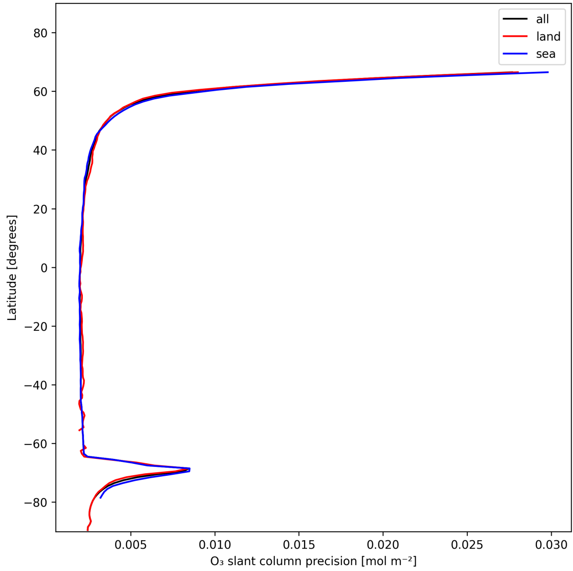
Figure 20: Zonal average of “O 3 slant column precision” for 2024-12-04 to 2024-12-04.
