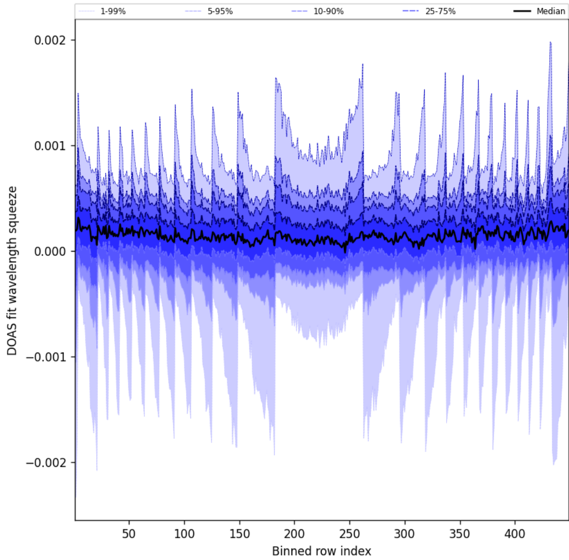
Figure 48: Along track statistics of “DOAS fit wavelength squeeze” for 2024-12-04 to 2024-12-04
