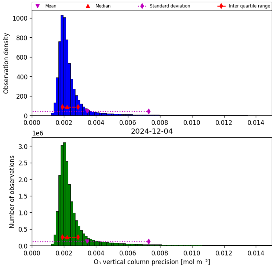
Figure 30: Histogram of “O 3 vertical column precision” for 2024-12-04 to 2024-12-04
