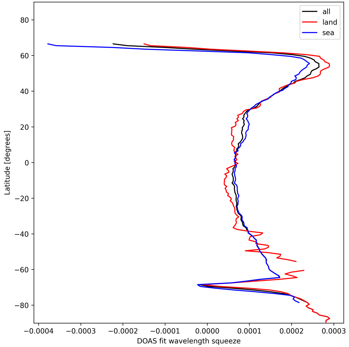
Figure 24: Zonal average of “DOAS fit wavelength squeeze” for 2024-12-04 to 2024-12-04.
