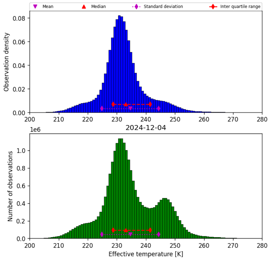
Figure 38: Histogram of “Effective temperature” for 2024-12-04 to 2024-12-04
