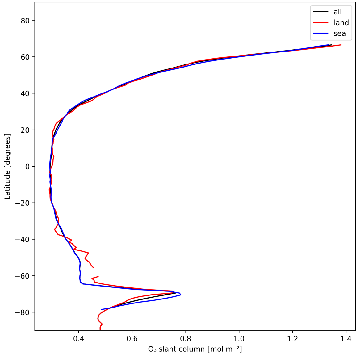
Figure 19: Zonal average of “O 3 slant column” for 2024-12-04 to 2024-12-04.
