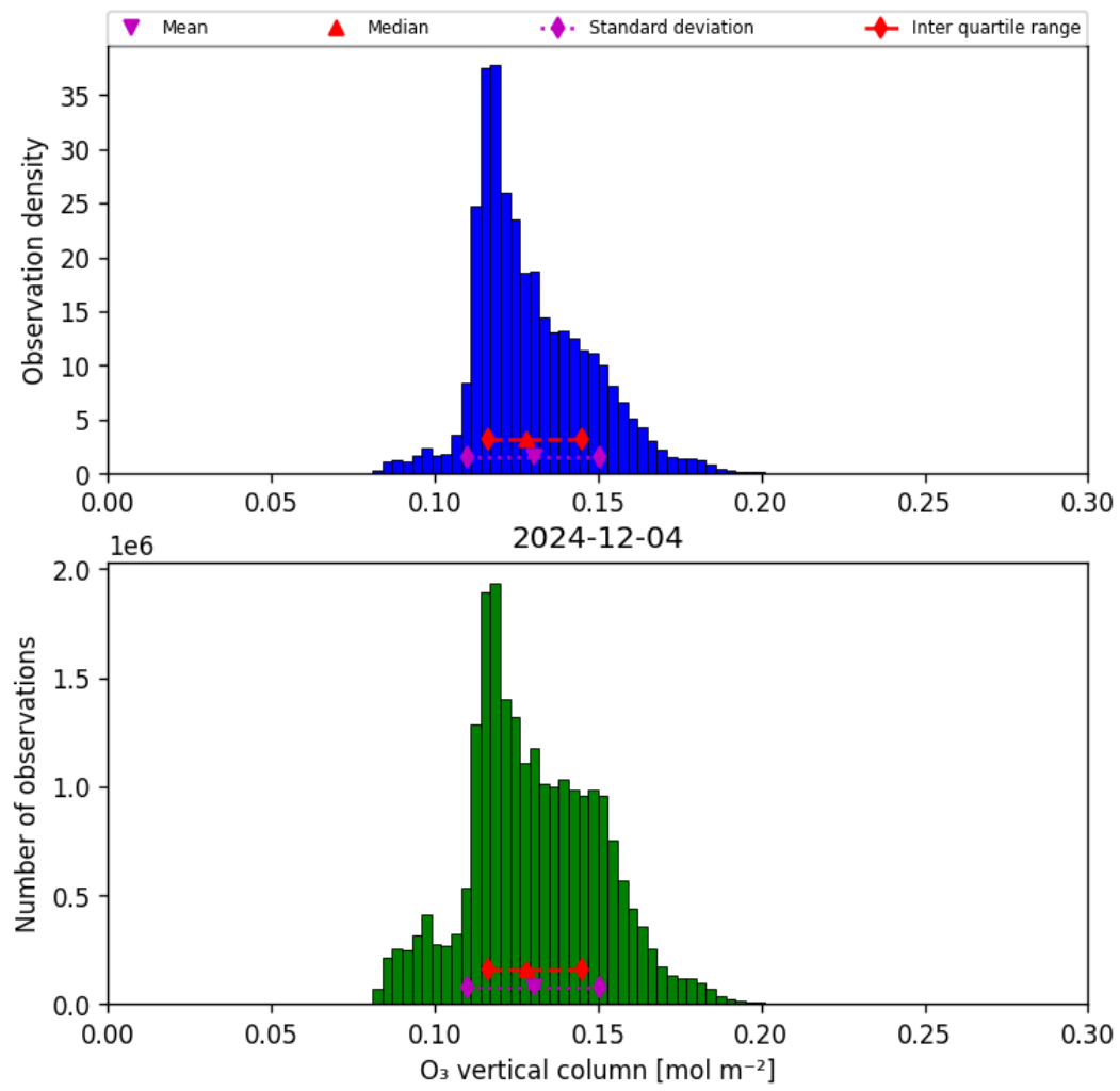
Figure 29: Histogram of “O 3 vertical column” for 2024-12-04 to 2024-12-04
