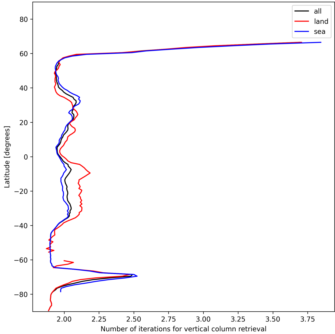
Figure 27: Zonal average of “Number of iterations for vertical column retrieval” for 2024-12-04 to 2024-12-04.
