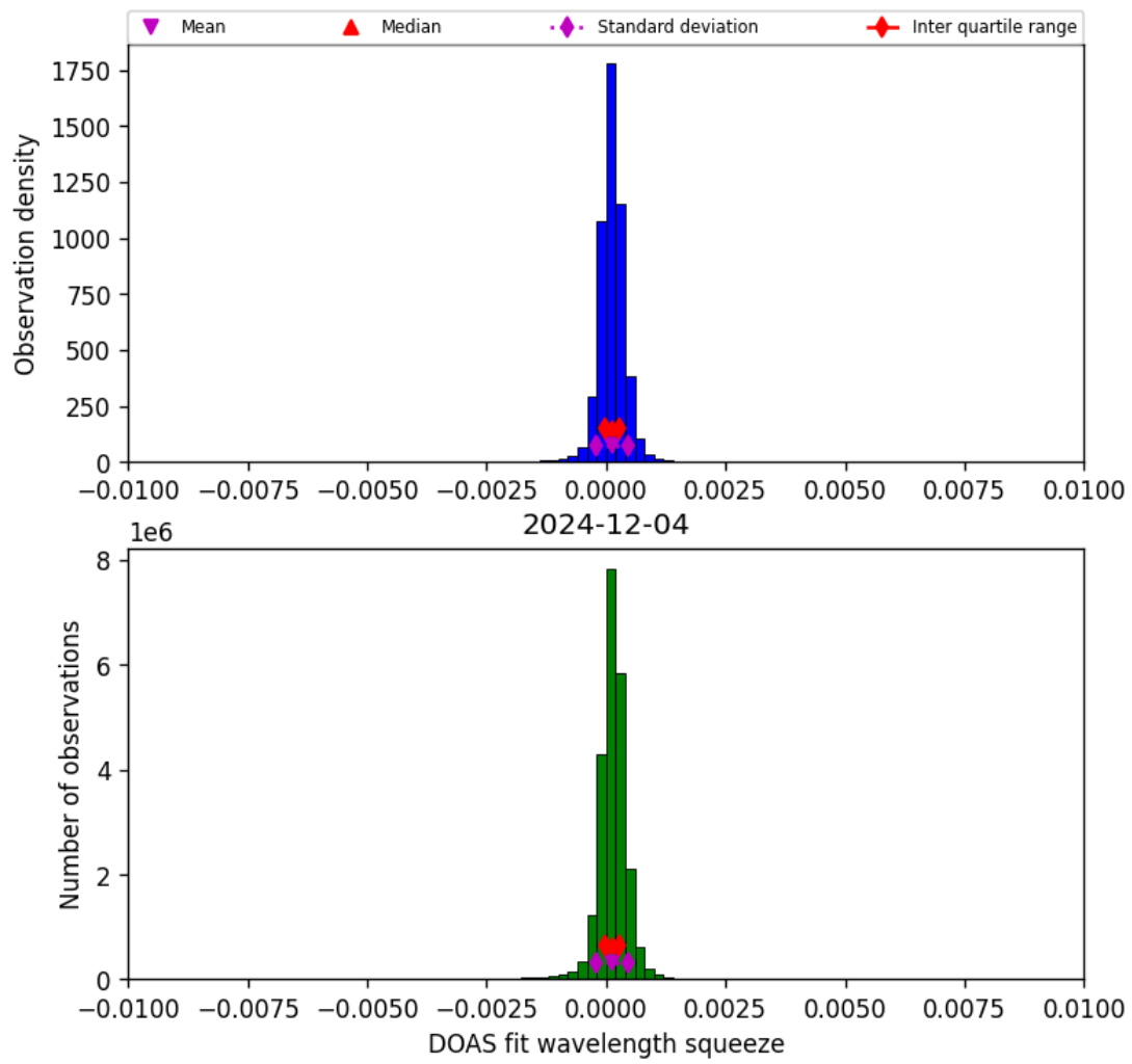
Figure 36: Histogram of “DOAS fit wavelength squeeze” for 2024-12-04 to 2024-12-04
