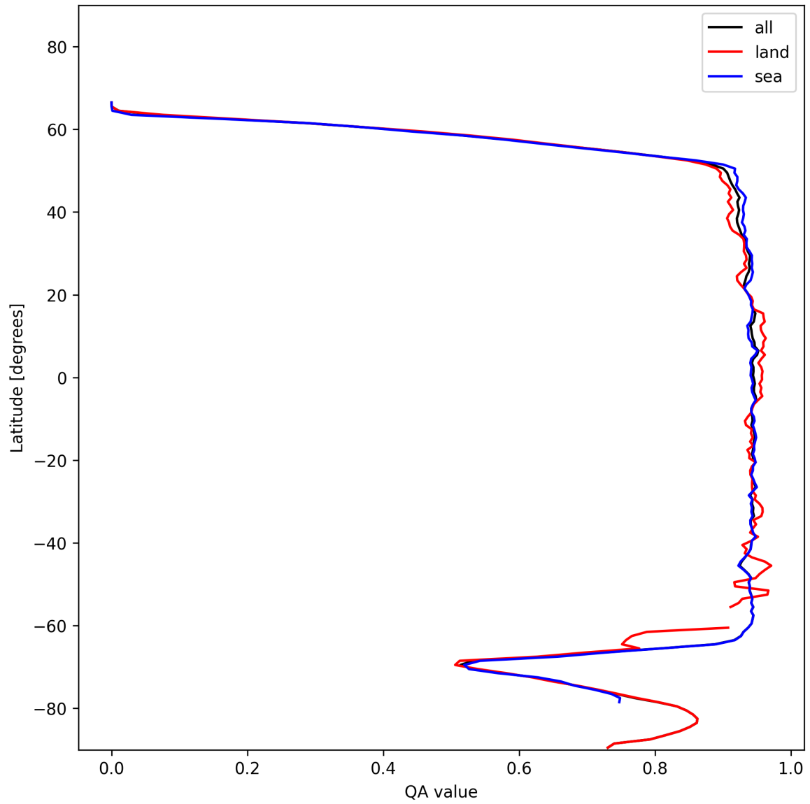
Figure 16: Zonal average of “QA value” for 2024-12-04 to 2024-12-04.
