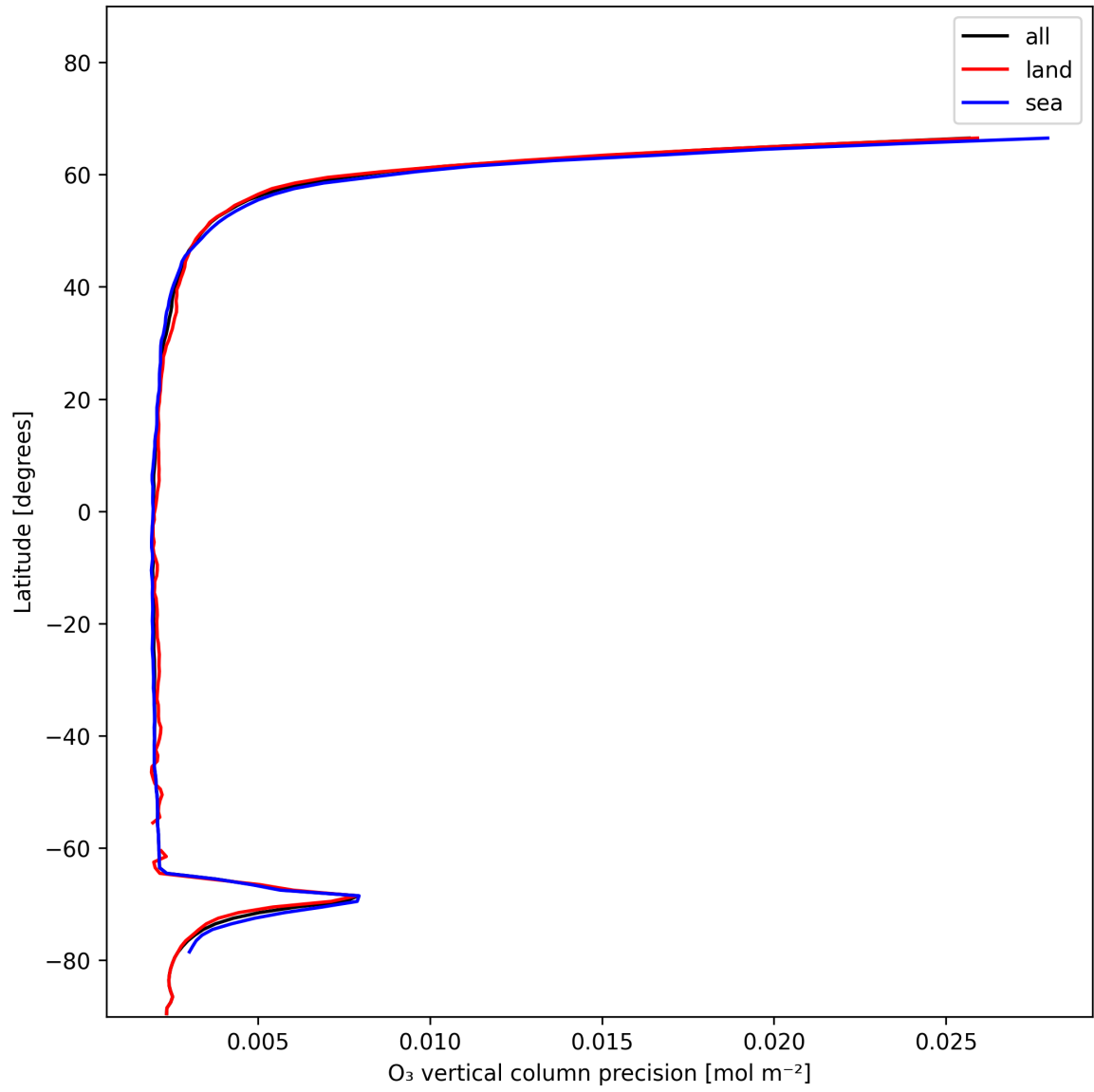
Figure 18: Zonal average of “O 3 vertical column precision” for 2024-12-04 to 2024-12-04.
