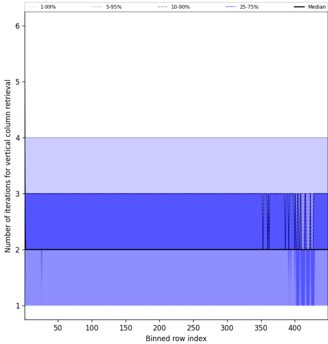
Figure 51: Along track statistics of “Number of iterations for vertical column retrieval” for 2024-12-04 to 2024-12-04
