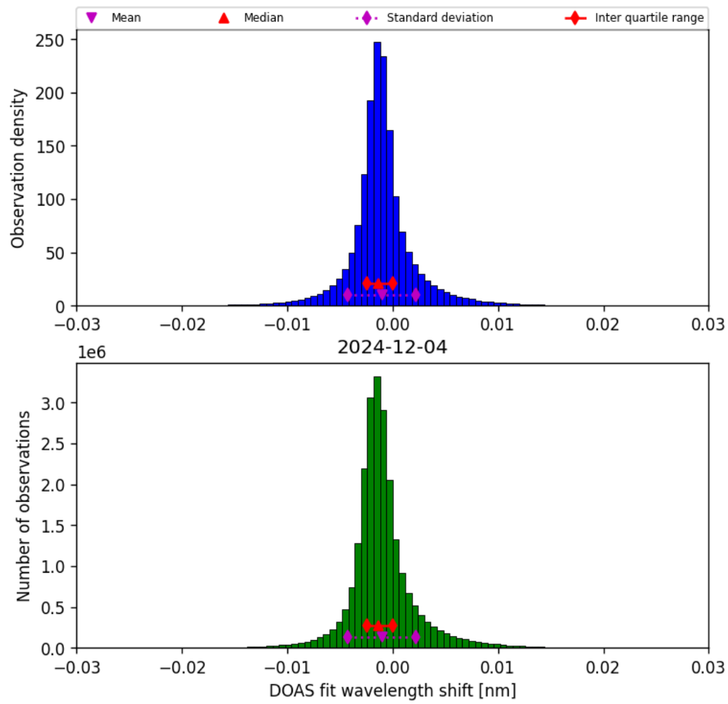
Figure 35: Histogram of “DOAS fit wavelength shift” for 2024-12-04 to 2024-12-04
