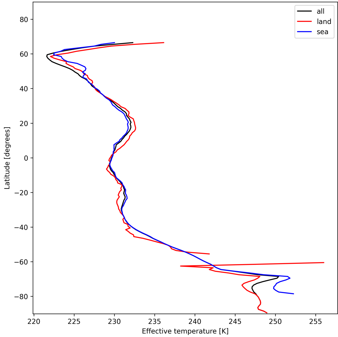
Figure 26: Zonal average of "Effective temperature" for 2024-12-04 to 2024-12-04.
