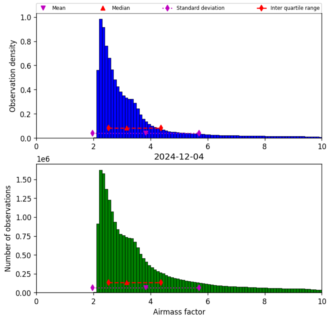
Figure 37: Histogram of “Airmass factor” for 2024-12-04 to 2024-12-04
