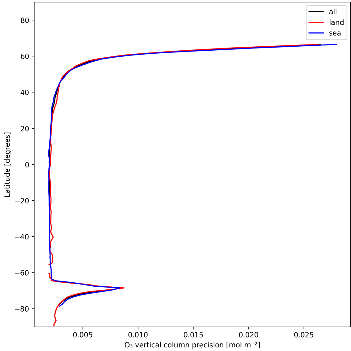
Figure 18: Zonal average of “O 3 vertical column precision” for 2024-12-05 to 2024-12-06.
