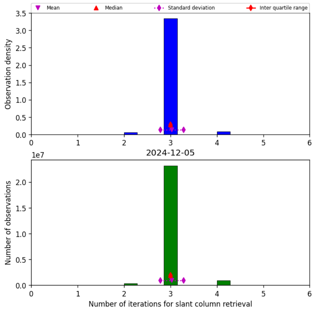
Figure 33: Histogram of “Number of iterations for slant column retrieval” for 2024-12-05 to 2024-12-06
