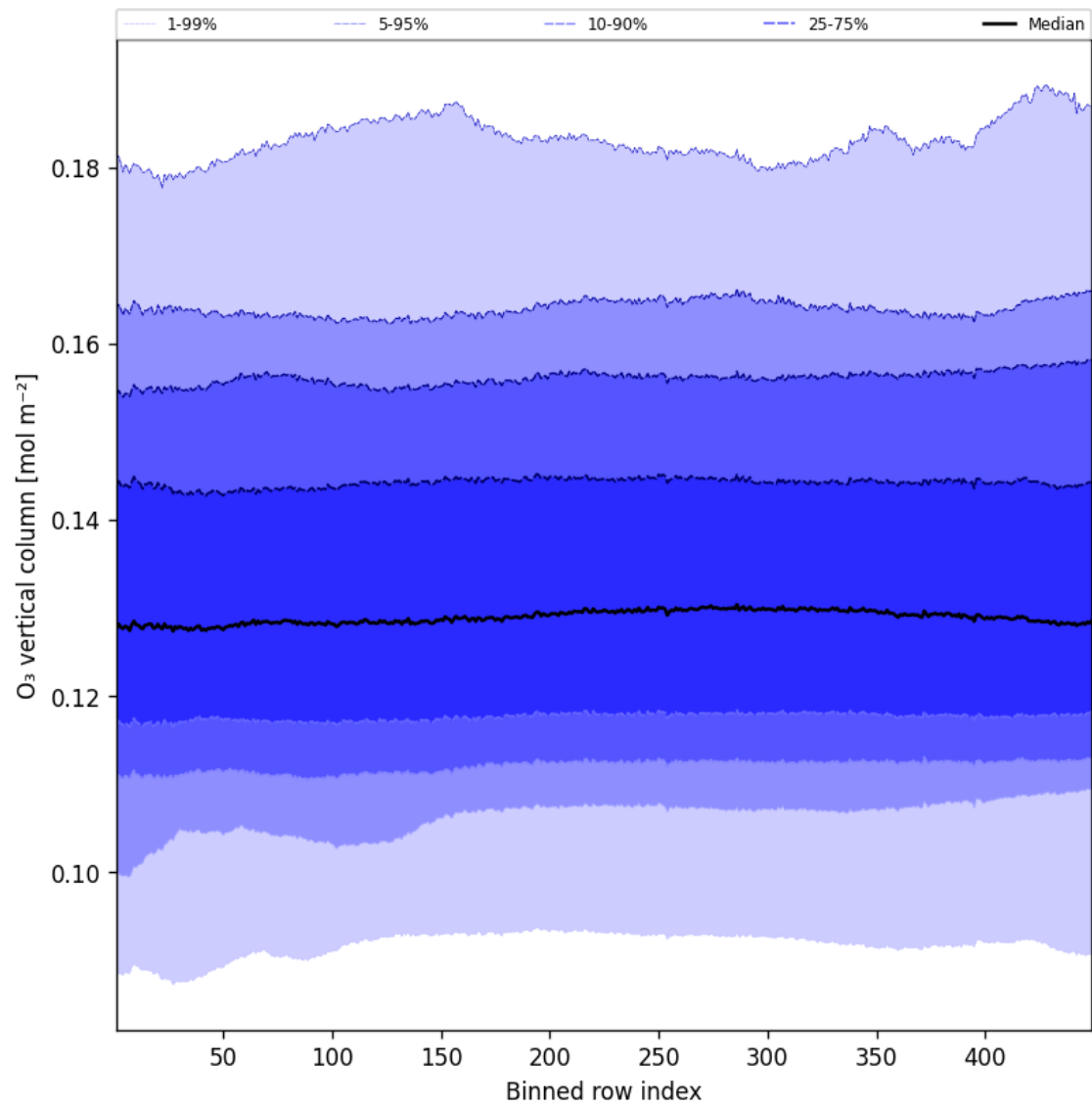
Figure 41: Along track statistics of “O 3 vertical column” for 2024-12-05 to 2024-12-06
