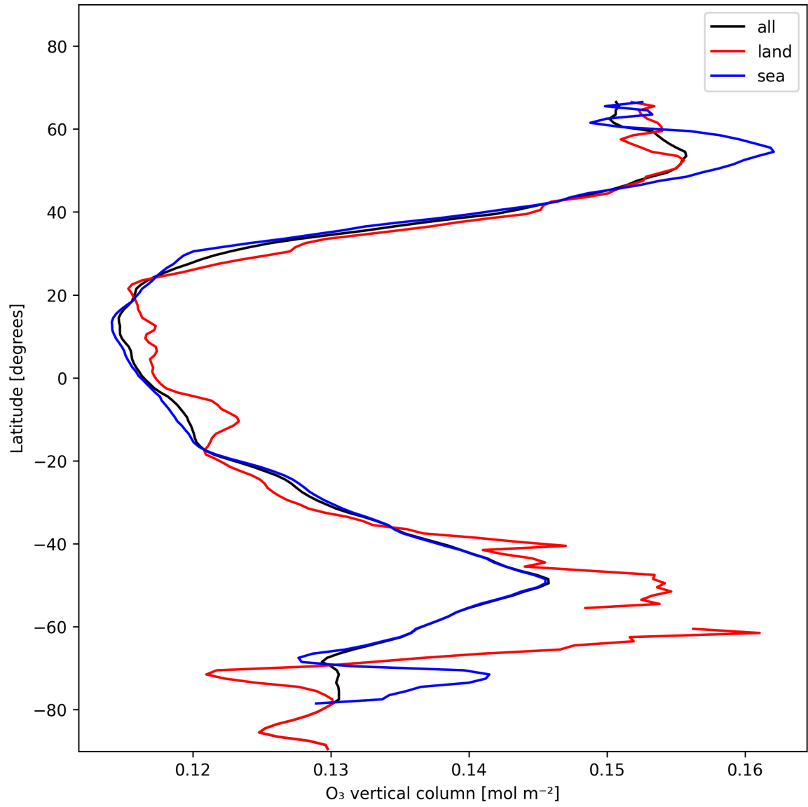
Figure 17: Zonal average of “O 3 vertical column” for 2024-12-05 to 2024-12-06.
