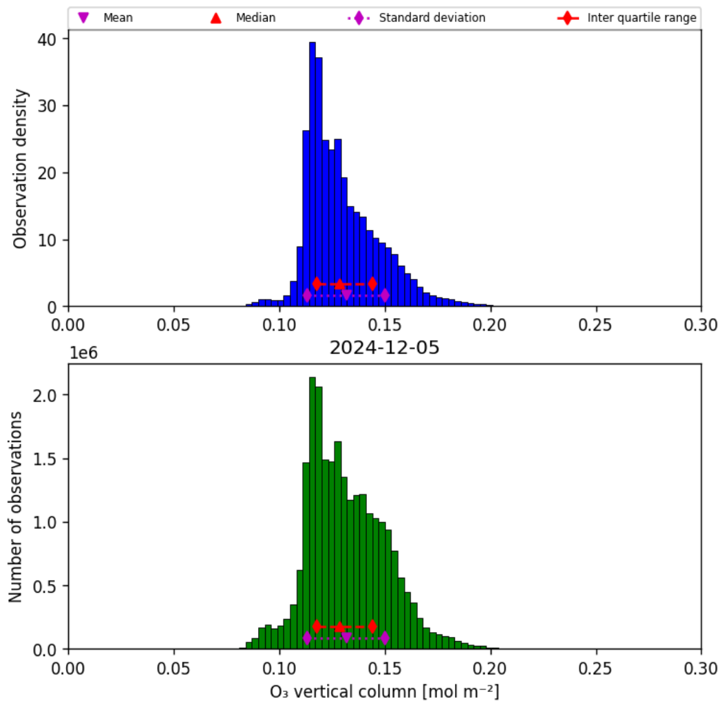
Figure 29: Histogram of “O 3 vertical column” for 2024-12-05 to 2024-12-06
