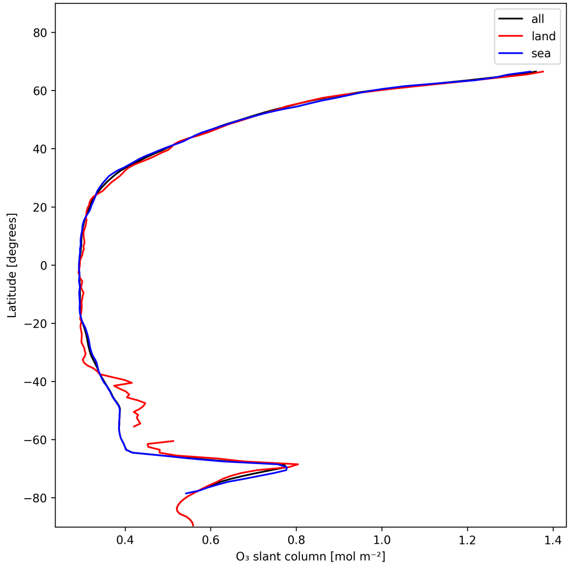
Figure 19: Zonal average of “O 3 slant column” for 2024-12-05 to 2024-12-06.
