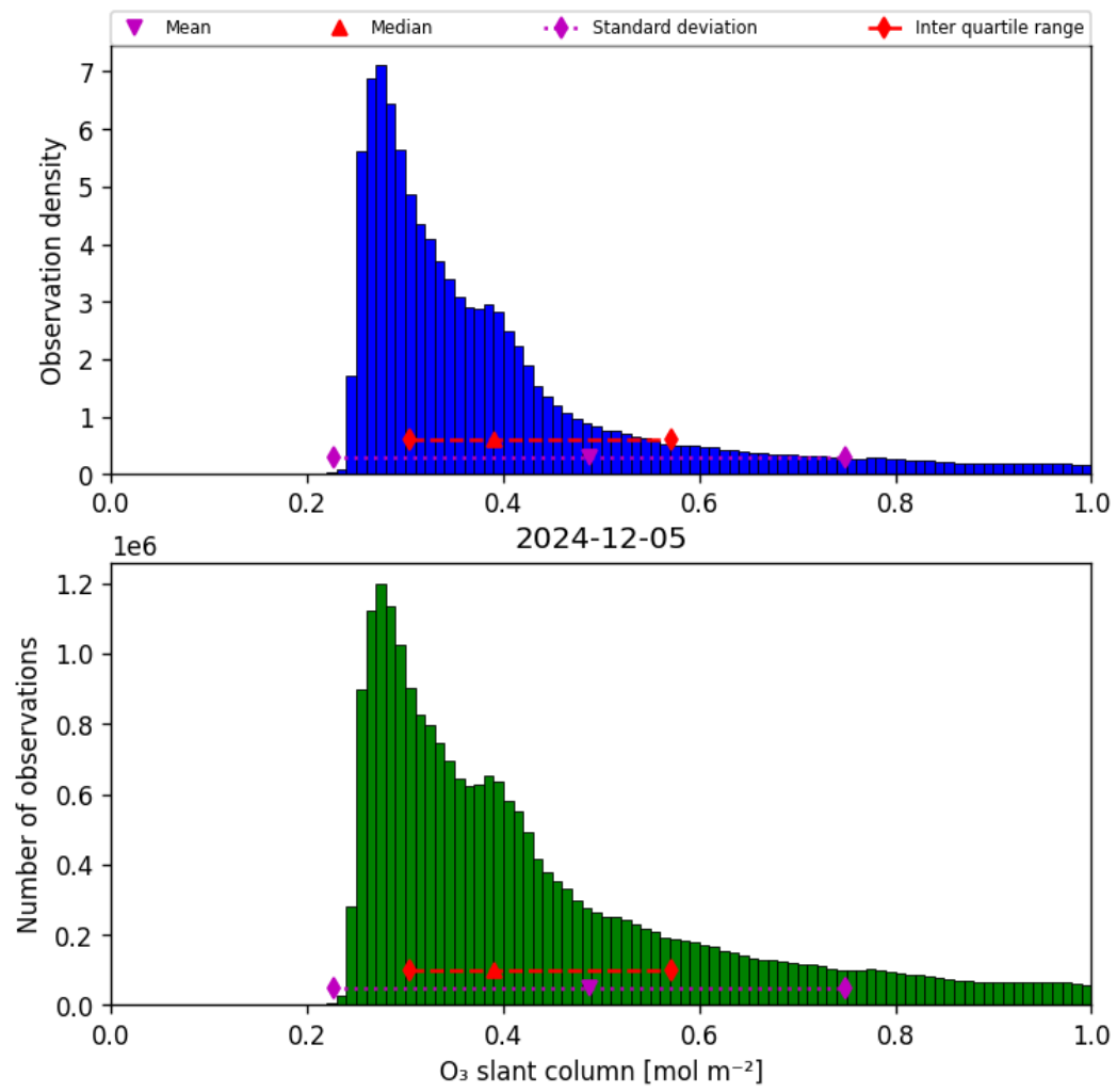
Figure 31: Histogram of “O 3 slant column” for 2024-12-05 to 2024-12-06
