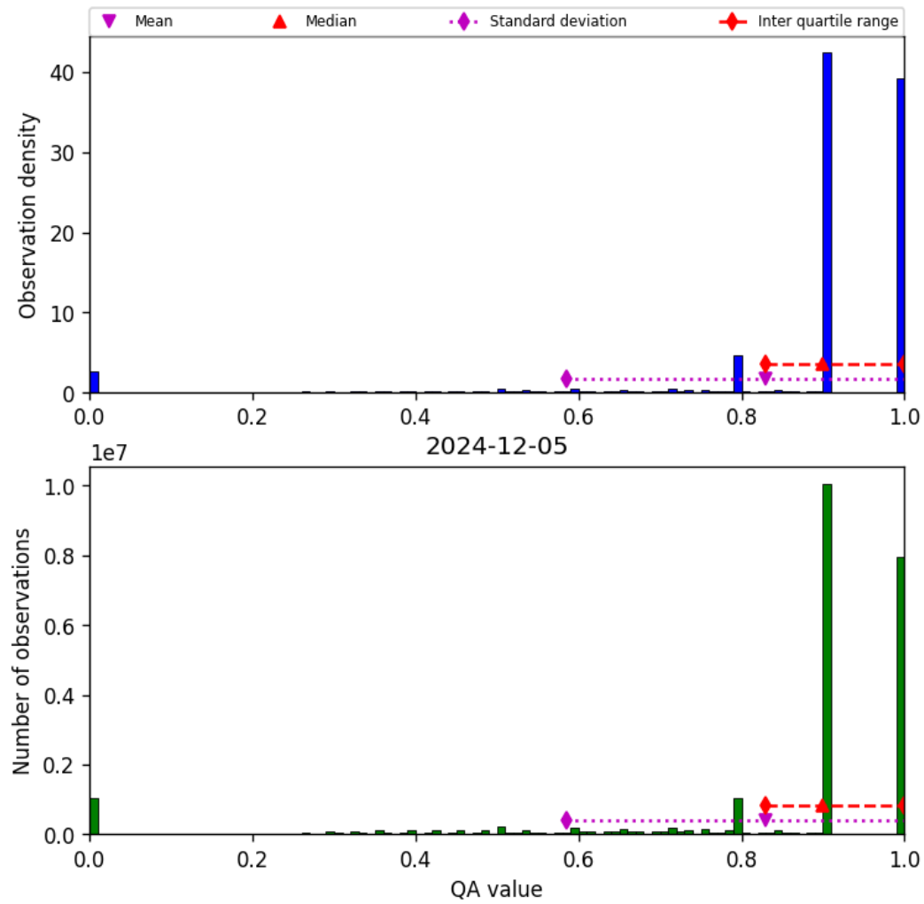
Figure 28: Histogram of “QA value” for 2024-12-05 to 2024-12-06
