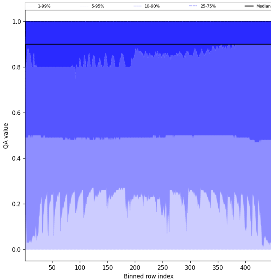
Figure 40: Along track statistics of “QA value” for 2024-12-05 to 2024-12-06
