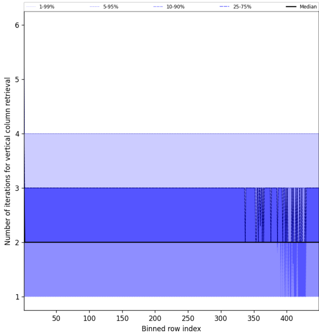
Figure 51: Along track statistics of “Number of iterations for vertical column retrieval” for 2024-12-05 to 2024-12-06
