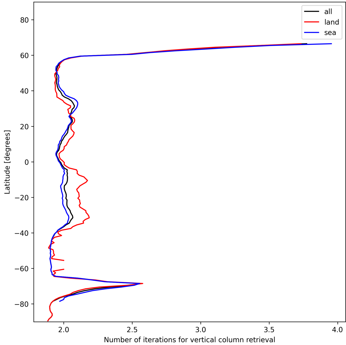
Figure 27: Zonal average of “Number of iterations for vertical column retrieval” for 2024-12-05 to 2024-12-06.
