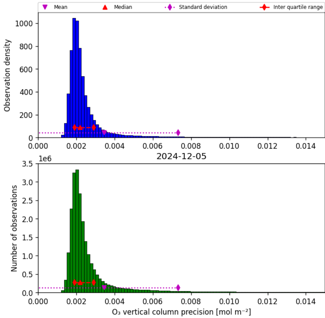
Figure 30: Histogram of “O 3 vertical column precision” for 2024-12-05 to 2024-12-06
