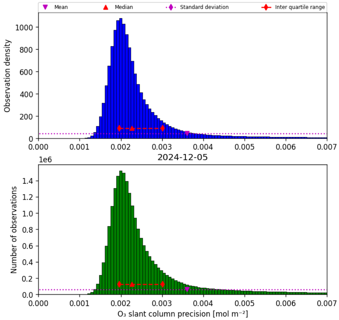
Figure 32: Histogram of “O 3 slant column precision” for 2024-12-05 to 2024-12-06
