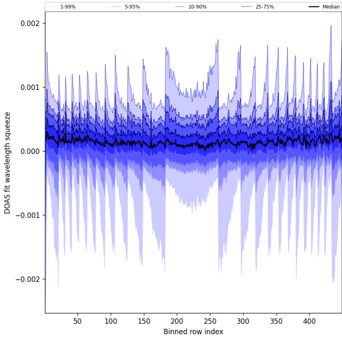
Figure 48: Along track statistics of “DOAS fit wavelength squeeze” for 2024-12-05 to 2024-12-06
