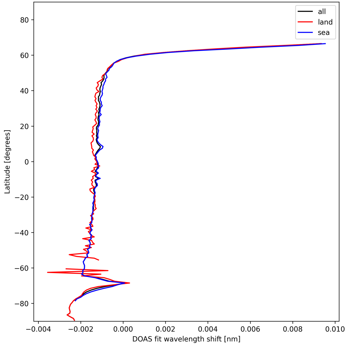
Figure 23: Zonal average of “DOAS fit wavelength shift” for 2024-12-05 to 2024-12-06.
