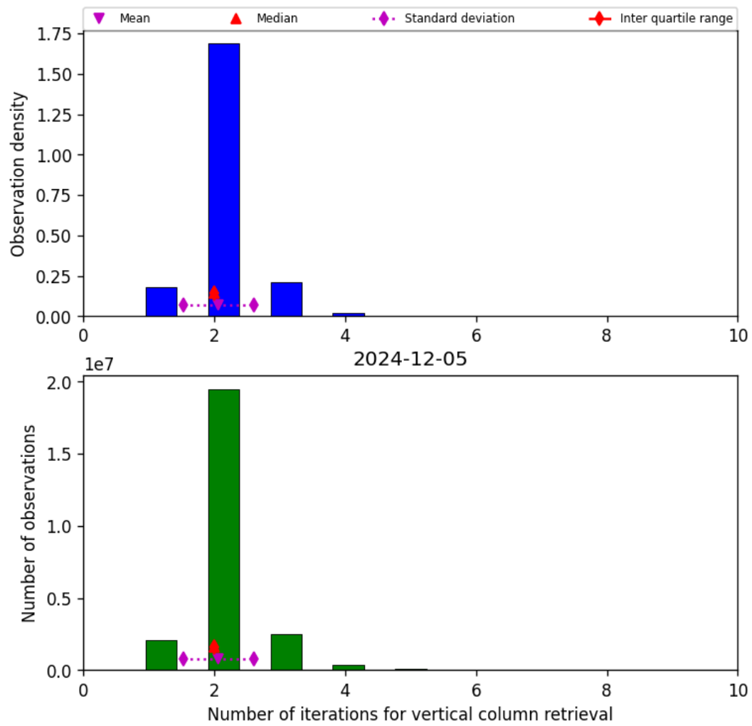
Figure 39: Histogram of “Number of iterations for vertical column retrieval” for 2024-12-05 to 2024-12-06
