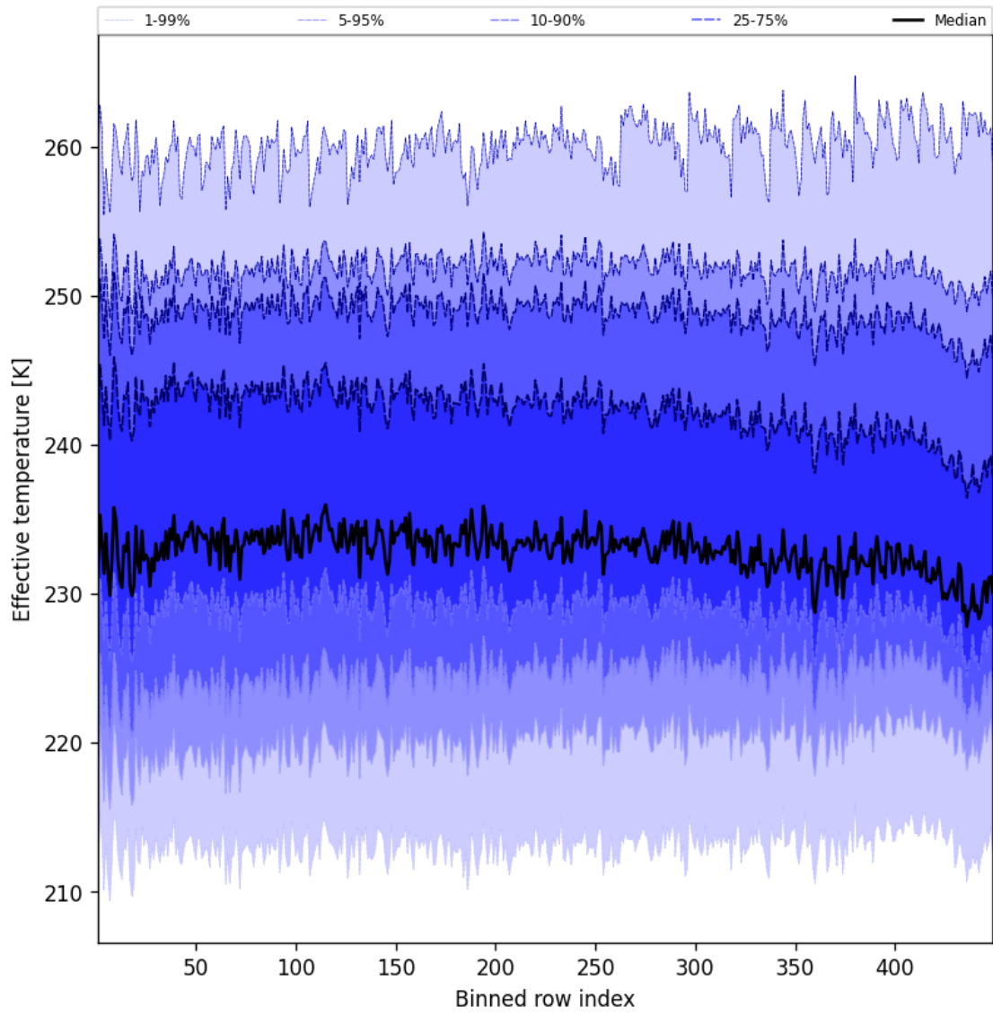
Figure 50: Along track statistics of “Effective temperature” for 2024-12-05 to 2024-12-06
