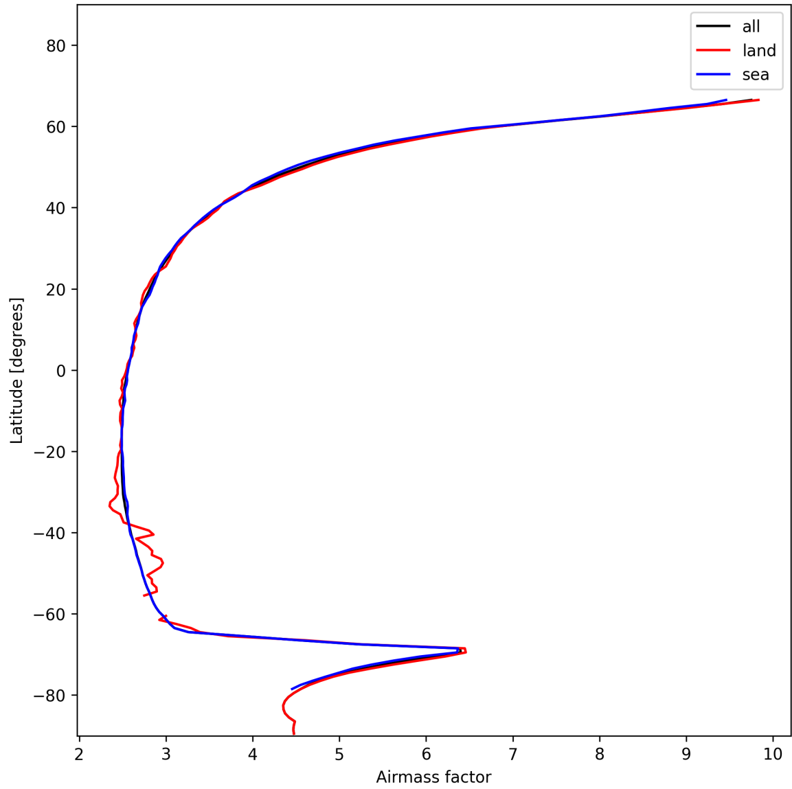
Figure 25: Zonal average of “Airmass factor” for 2024-12-05 to 2024-12-06.
