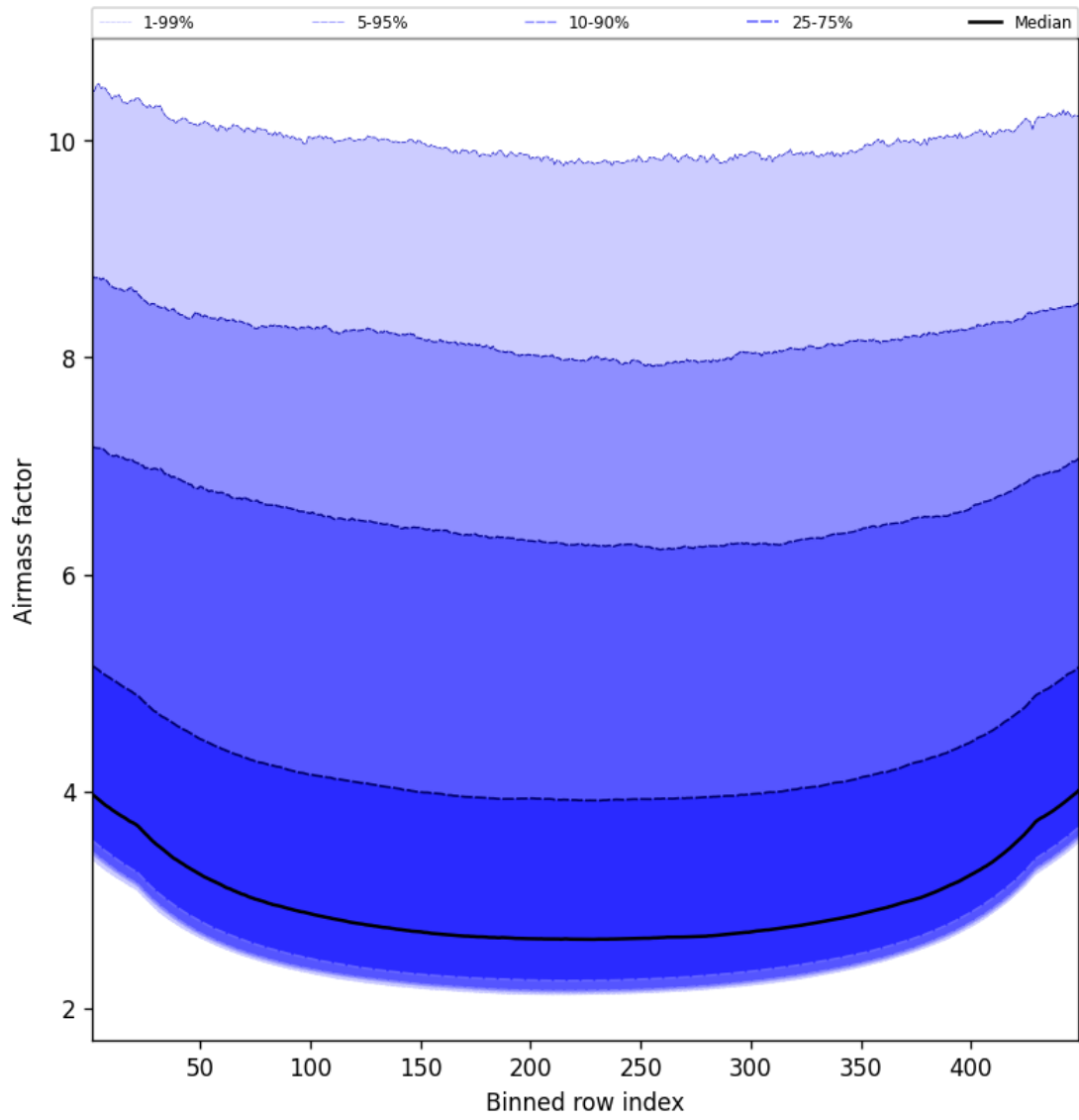
Figure 49: Along track statistics of “Airmass factor” for 2024-12-05 to 2024-12-06
