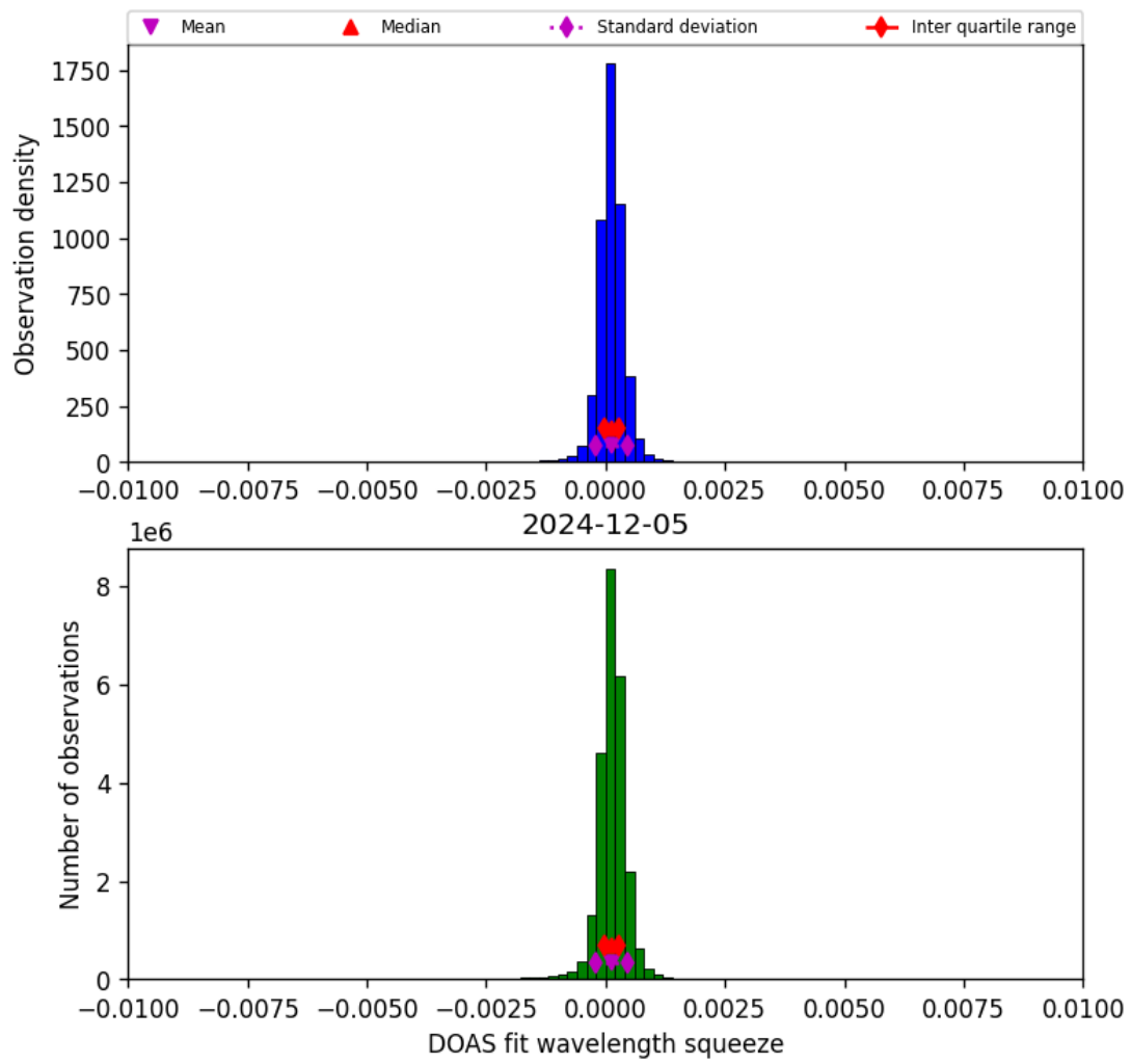
Figure 36: Histogram of “DOAS fit wavelength squeeze” for 2024-12-05 to 2024-12-06
