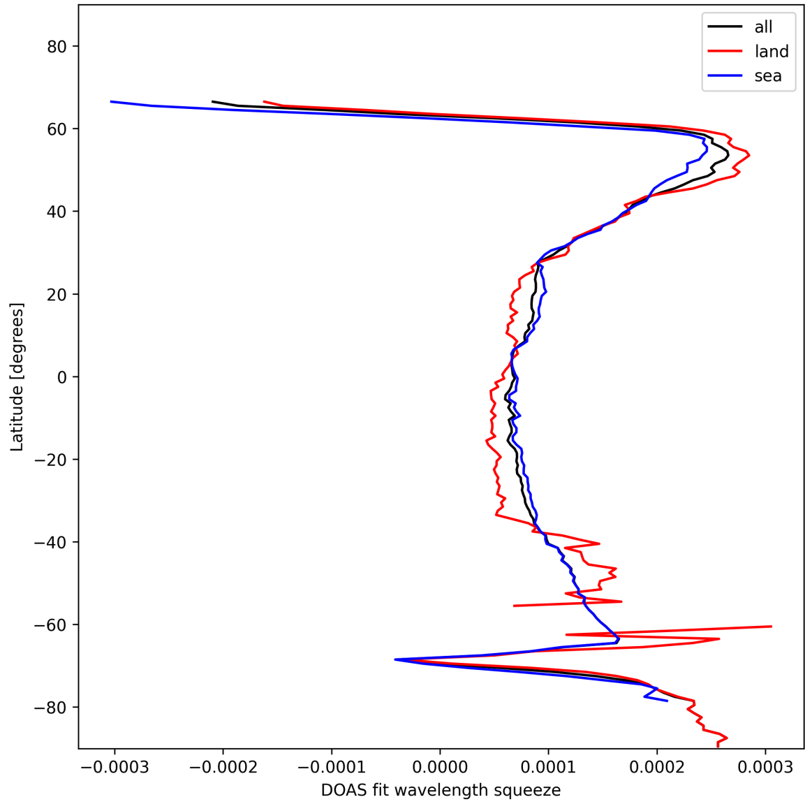
Figure 24: Zonal average of “DOAS fit wavelength squeeze” for 2024-12-05 to 2024-12-06.
