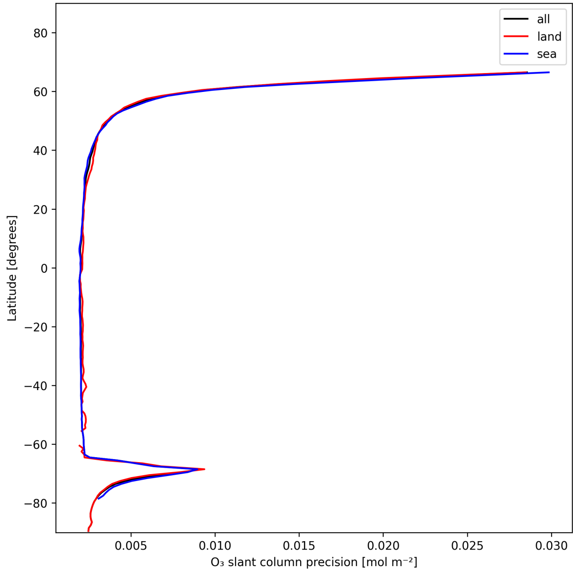
Figure 20: Zonal average of “O 3 slant column precision” for 2024-12-05 to 2024-12-06.
