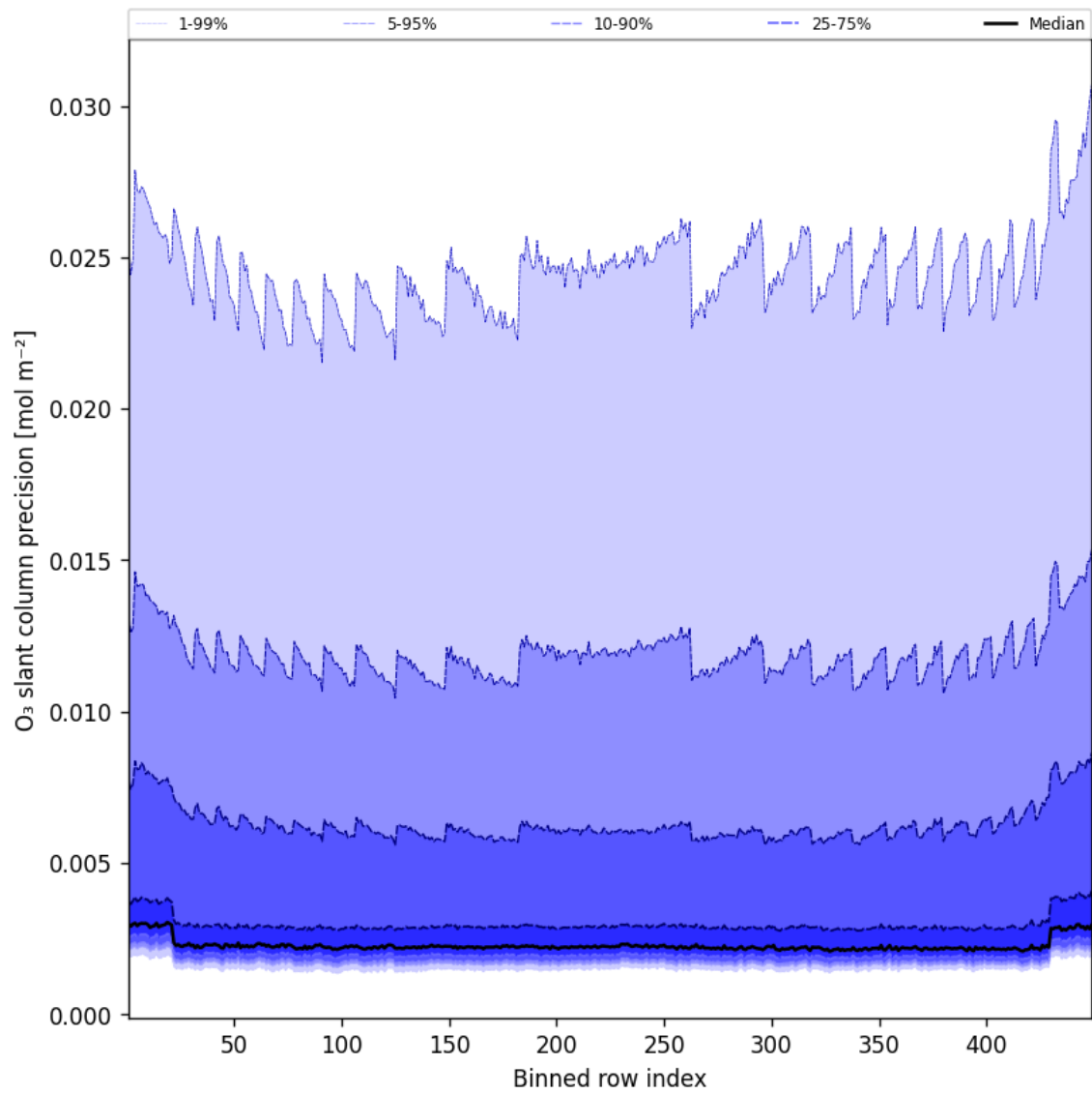
Figure 44: Along track statistics of “O 3 slant column precision” for 2024-12-05 to 2024-12-06
