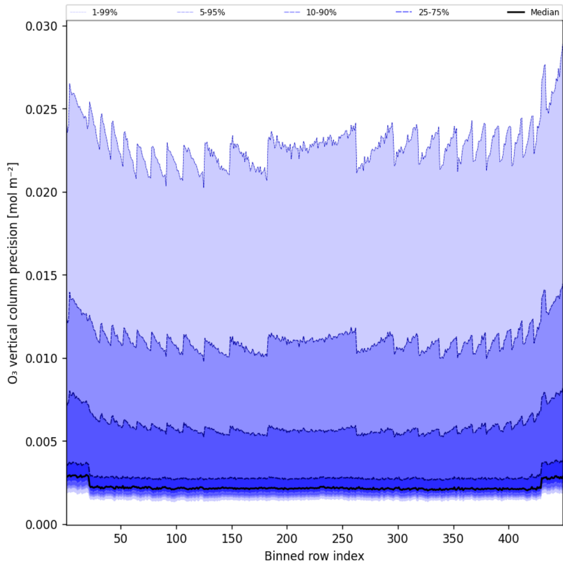
Figure 42: Along track statistics of “O 3 vertical column precision” for 2024-12-05 to 2024-12-06
