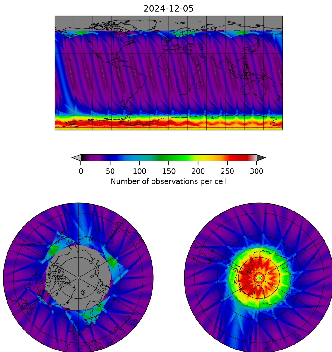
Figure 15: Map of the number of observations for 2024-12-05 to 2024-12-06
