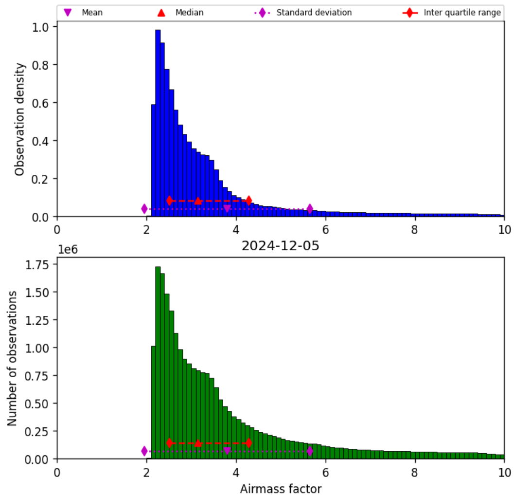
Figure 37: Histogram of “Airmass factor” for 2024-12-05 to 2024-12-06
