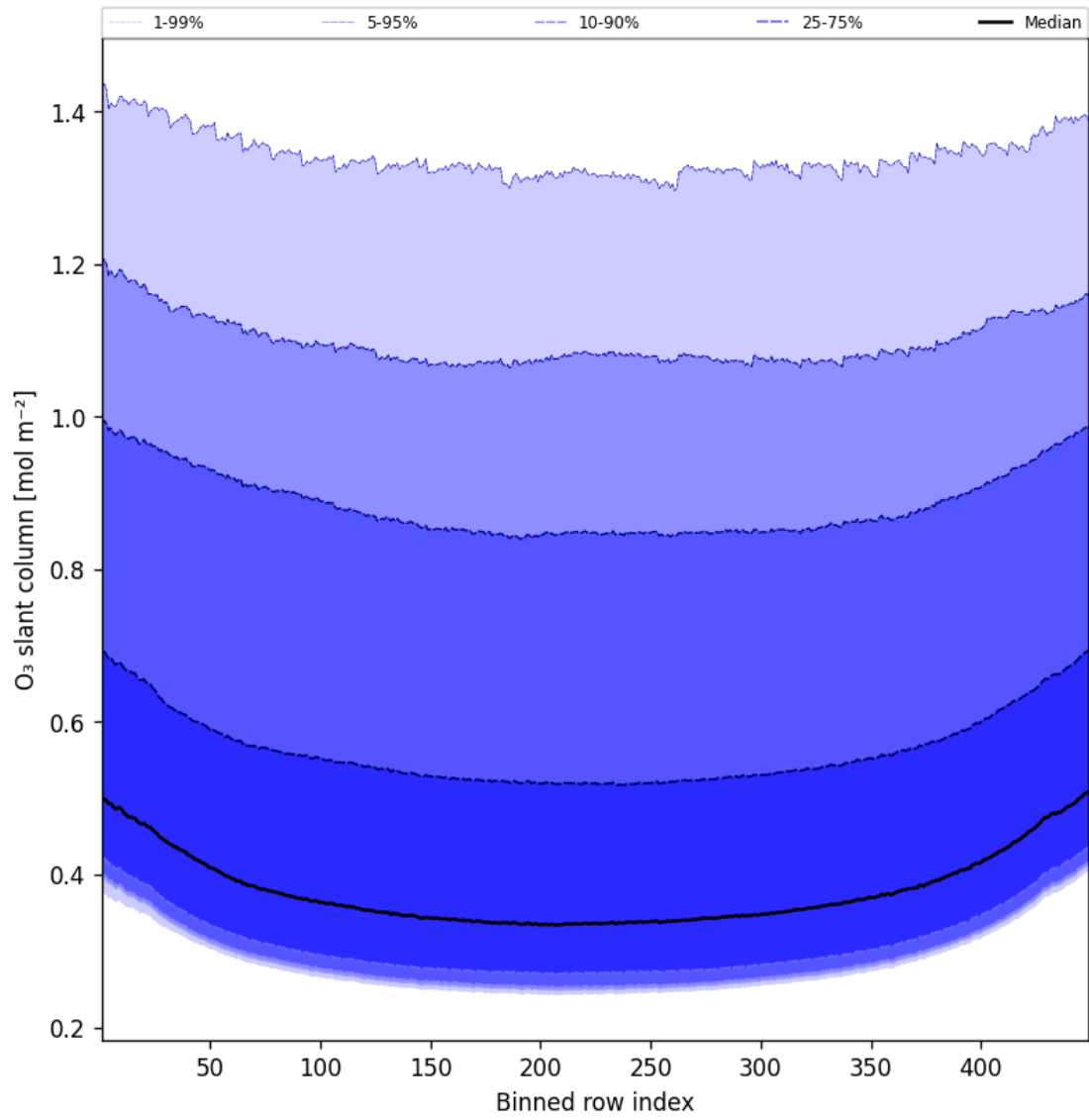
Figure 43: Along track statistics of “O 3 slant column” for 2024-12-05 to 2024-12-06
