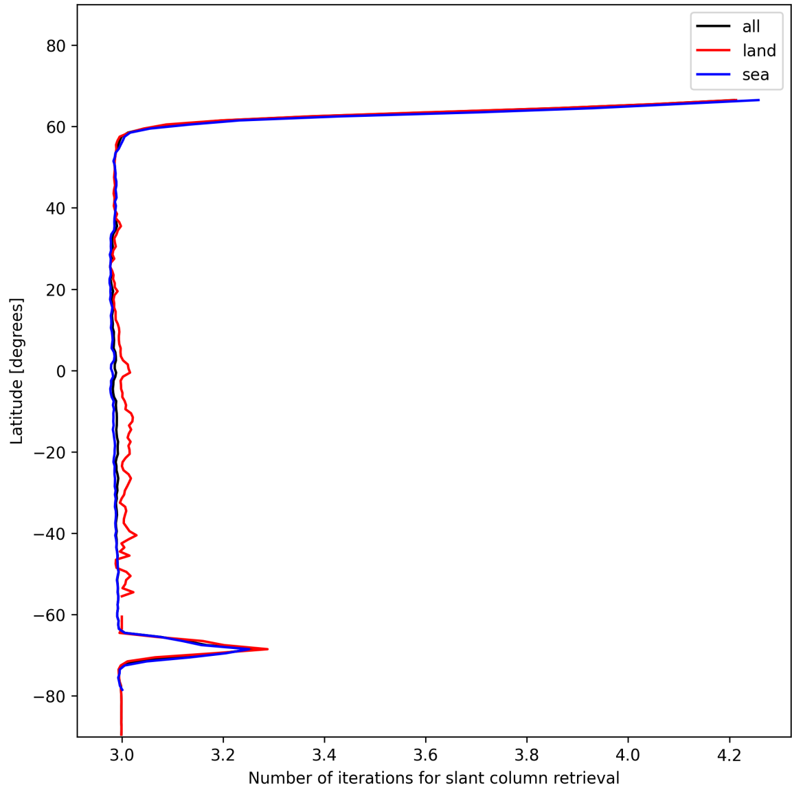
Figure 21: Zonal average of “Number of iterations for slant column retrieval” for 2024-12-05 to 2024-12-06.
