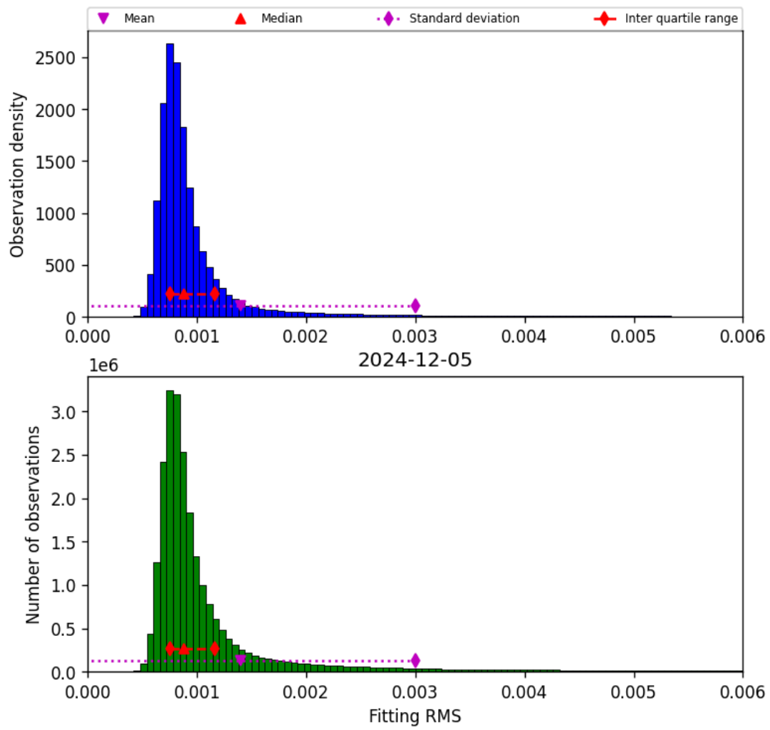
Figure 34: Histogram of "Fitting RMS" for 2024-12-05 to 2024-12-06
