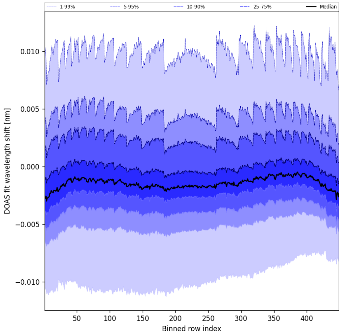
Figure 47: Along track statistics of "DOAS fit wavelength shift" for 2024-12-05 to 2024-12-06
