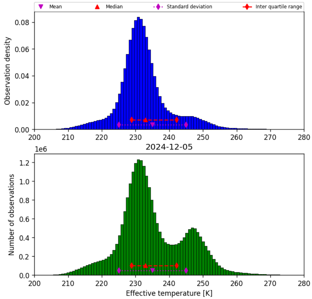
Figure 38: Histogram of “Effective temperature” for 2024-12-05 to 2024-12-06
