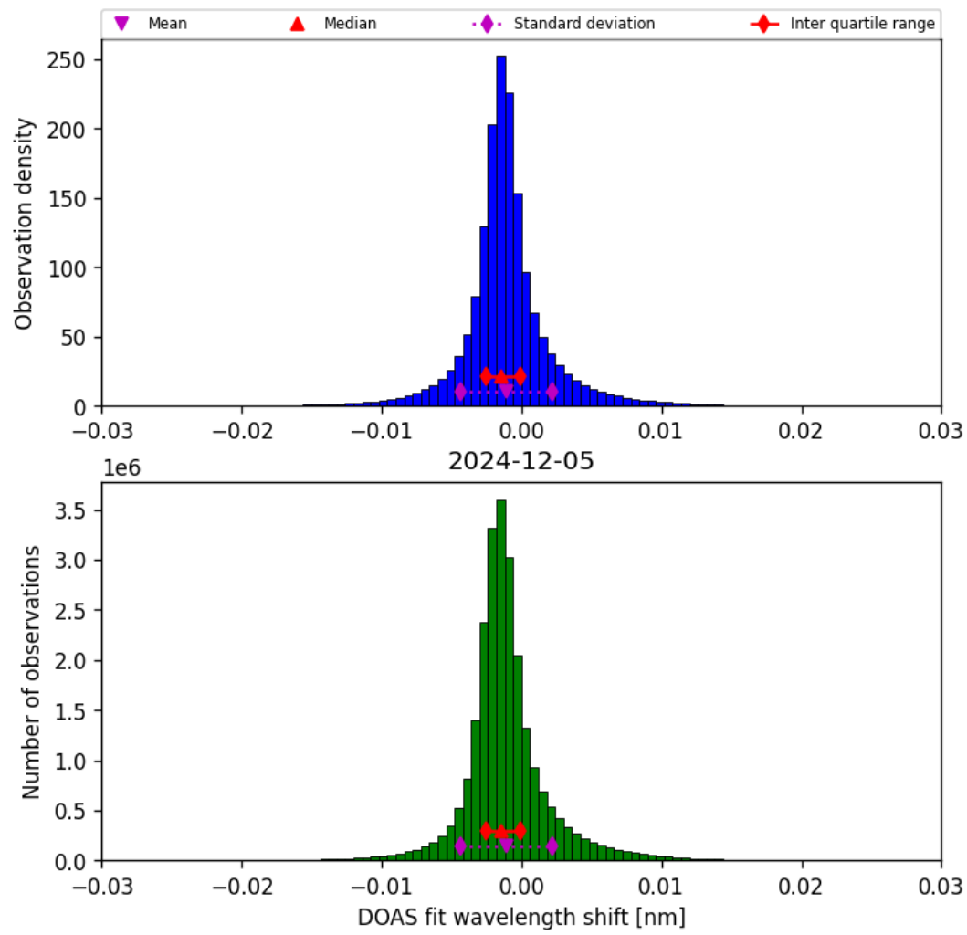
Figure 35: Histogram of “DOAS fit wavelength shift” for 2024-12-05 to 2024-12-06
