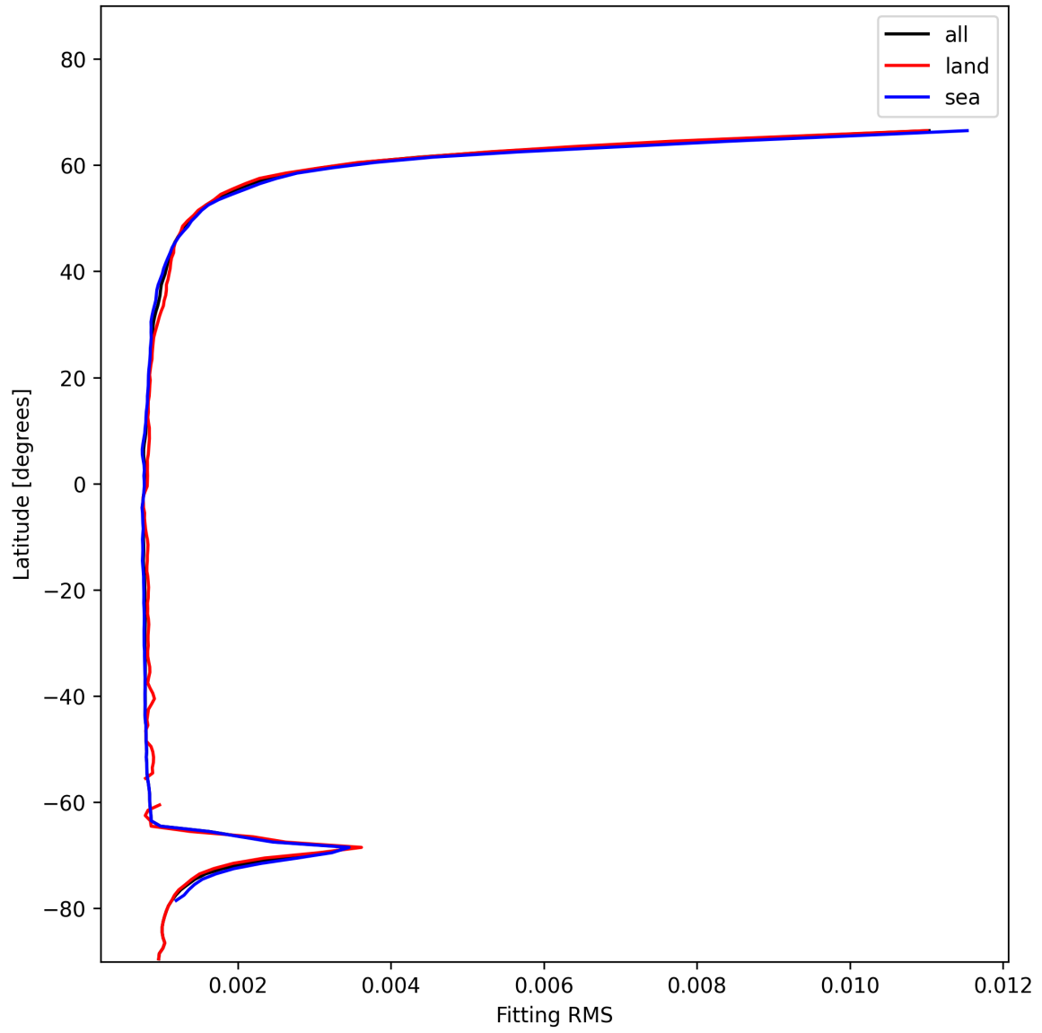
Figure 22: Zonal average of “Fitting RMS” for 2024-12-05 to 2024-12-06.
