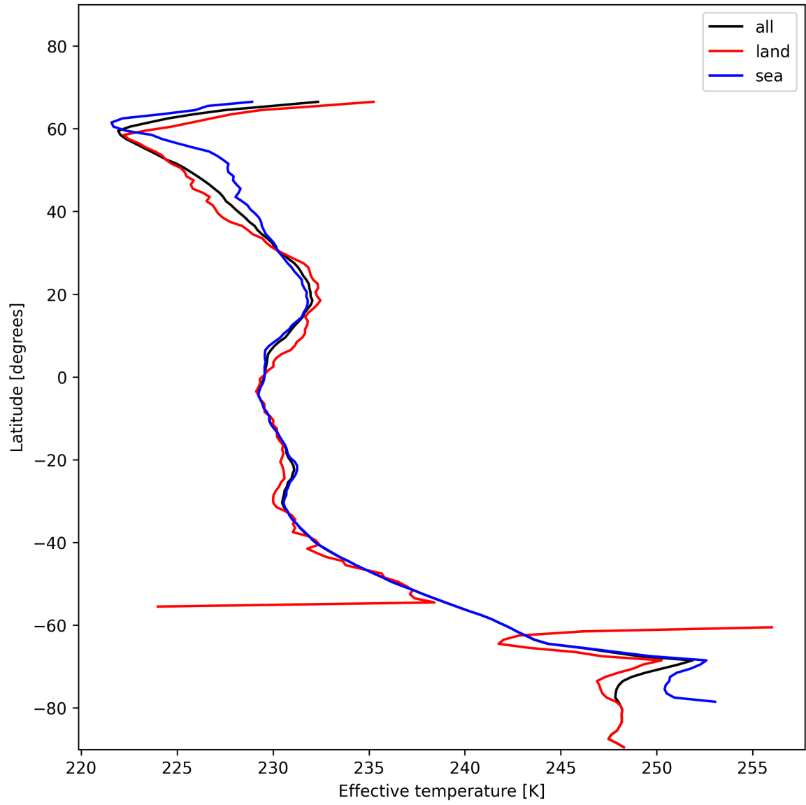
Figure 26: Zonal average of “Effective temperature” for 2024-12-05 to 2024-12-06.
