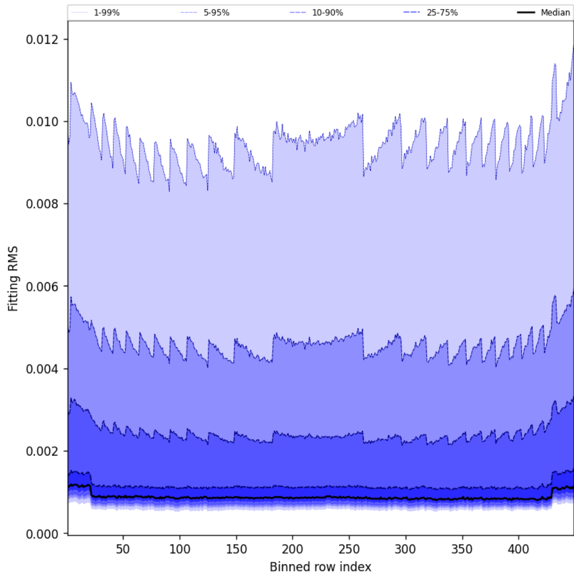
Figure 46: Along track statistics of “Fitting RMS” for 2024-12-05 to 2024-12-06
