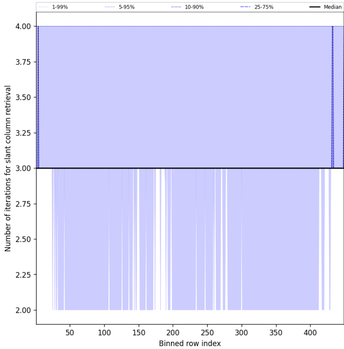
Figure 45: Along track statistics of “Number of iterations for slant column retrieval” for 2024-12-05 to 2024-12-06
