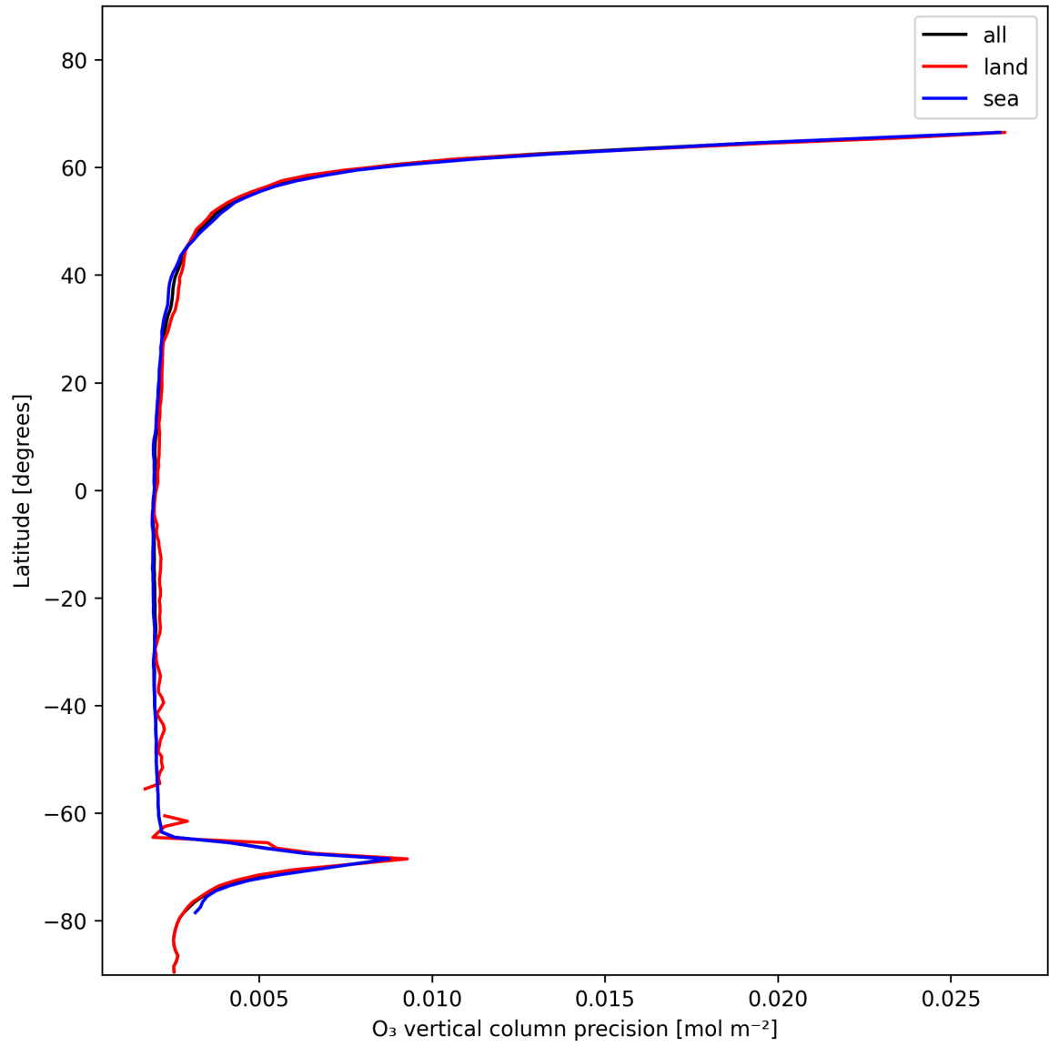
Figure 18: Zonal average of “O 3 vertical column precision” for 2024-12-06 to 2024-12-07.
