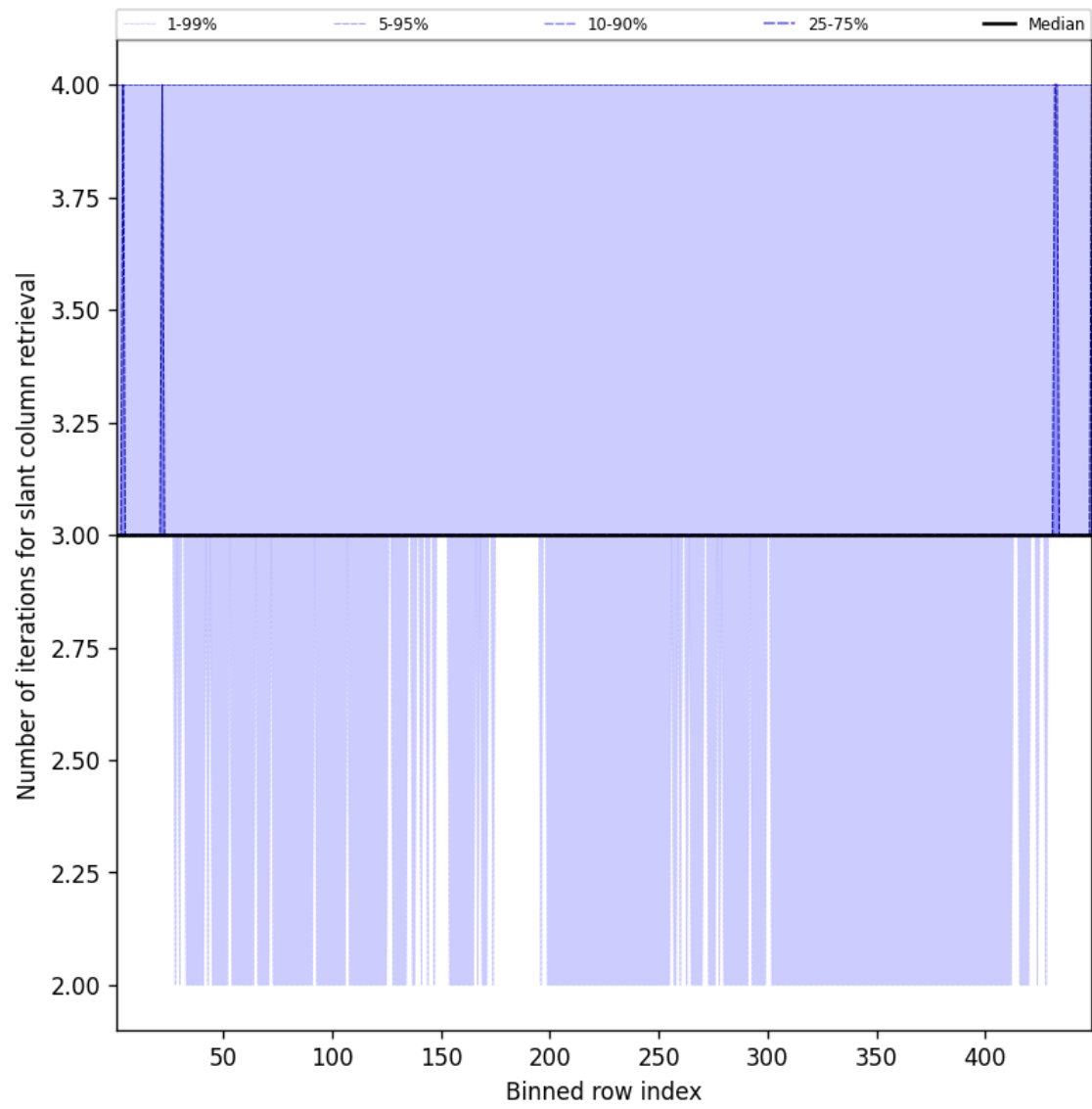
Figure 45: Along track statistics of “Number of iterations for slant column retrieval” for 2024-12-06 to 2024-12-07
