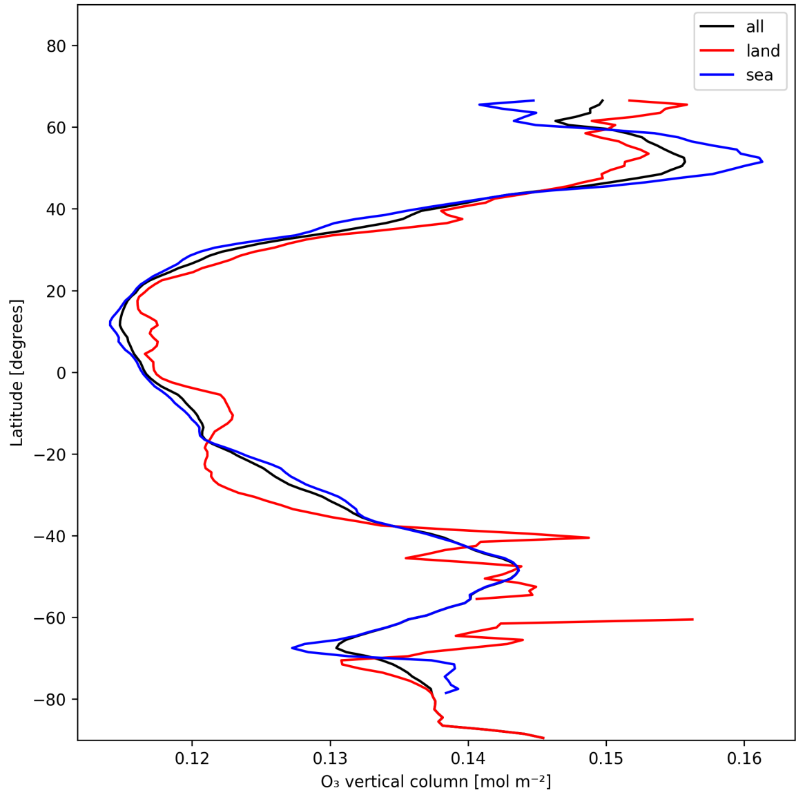
Figure 17: Zonal average of “O 3 vertical column” for 2024-12-06 to 2024-12-07.
