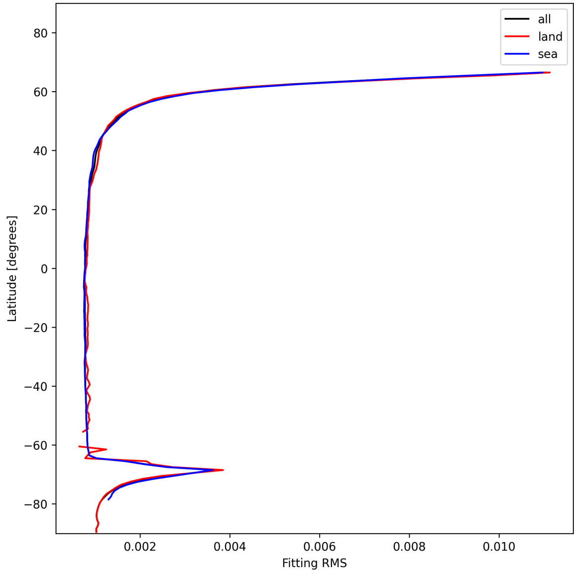
Figure 22: Zonal average of “Fitting RMS” for 2024-12-06 to 2024-12-07.
