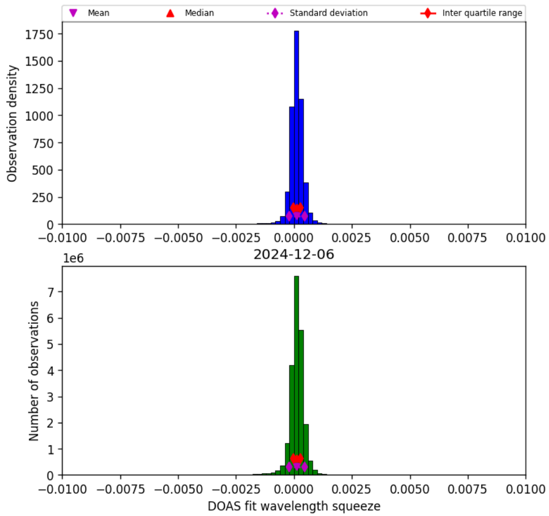
Figure 36: Histogram of “DOAS fit wavelength squeeze” for 2024-12-06 to 2024-12-07
