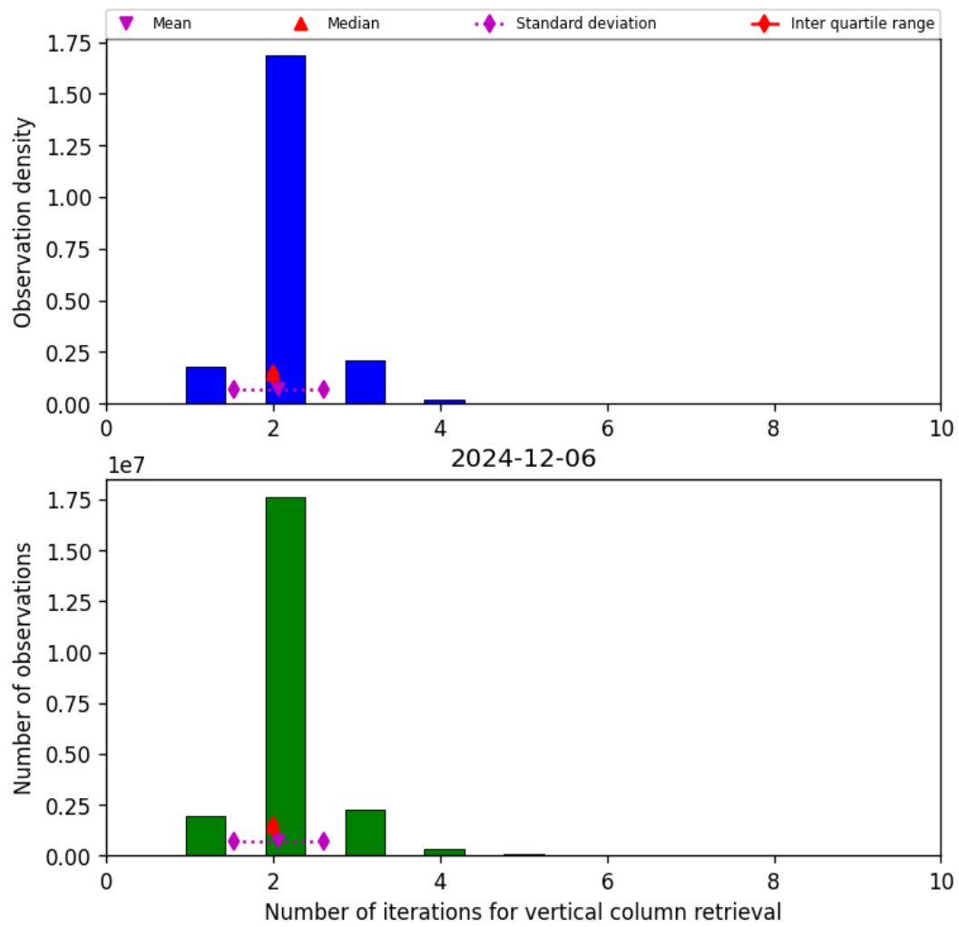
Figure 39: Histogram of “Number of iterations for vertical column retrieval” for 2024-12-06 to 2024-12-07
