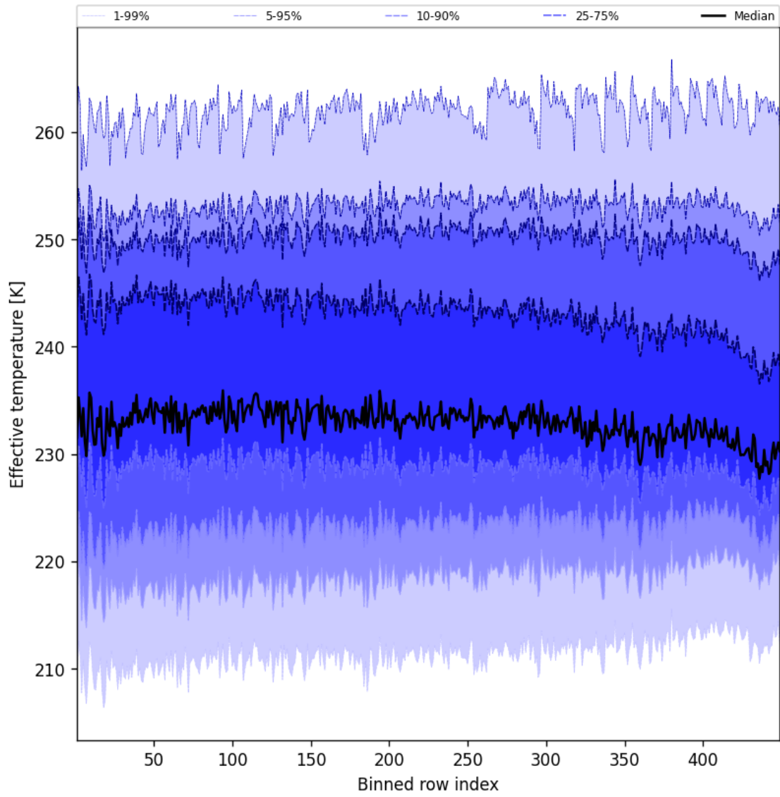
Figure 50: Along track statistics of “Effective temperature” for 2024-12-06 to 2024-12-07
