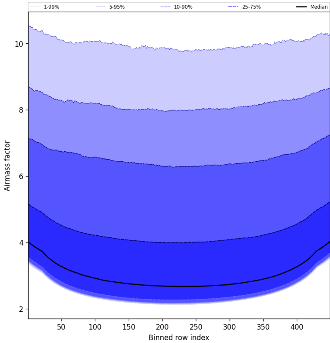
Figure 49: Along track statistics of “Airmass factor” for 2024-12-06 to 2024-12-07
