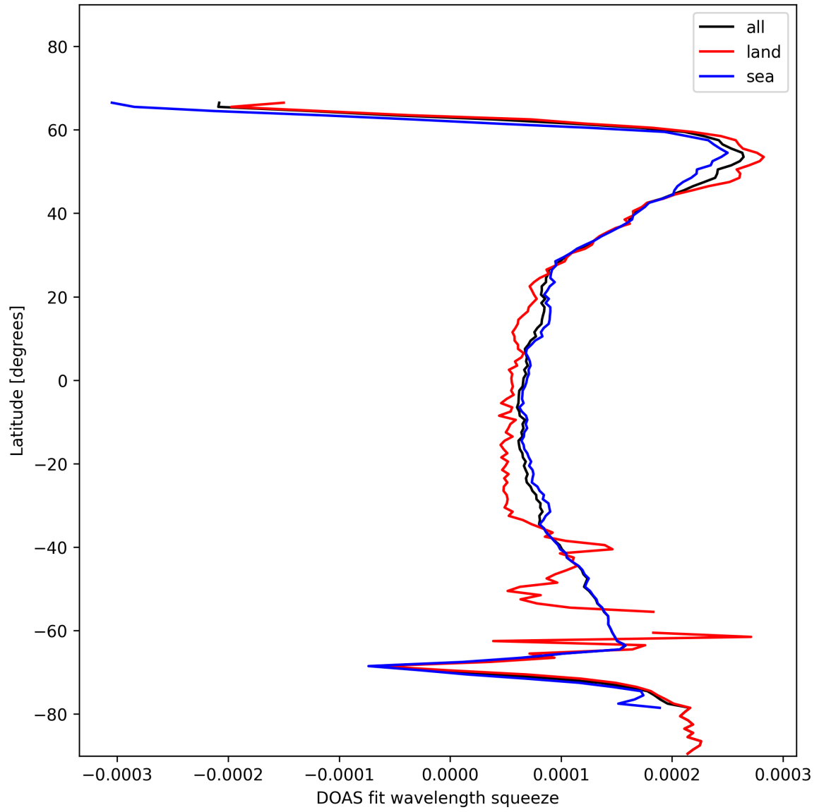
Figure 24: Zonal average of “DOAS fit wavelength squeeze” for 2024-12-06 to 2024-12-07.
