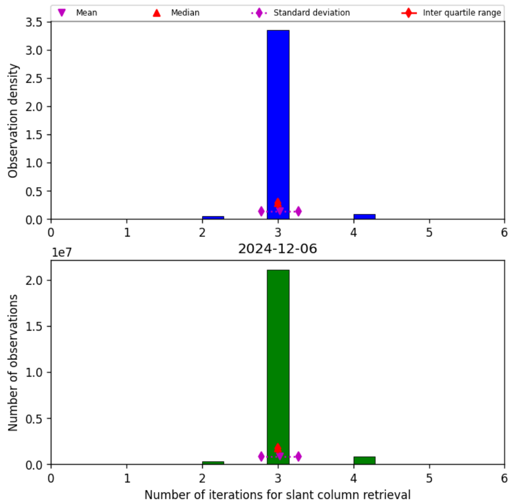
Figure 33: Histogram of “Number of iterations for slant column retrieval” for 2024-12-06 to 2024-12-07
