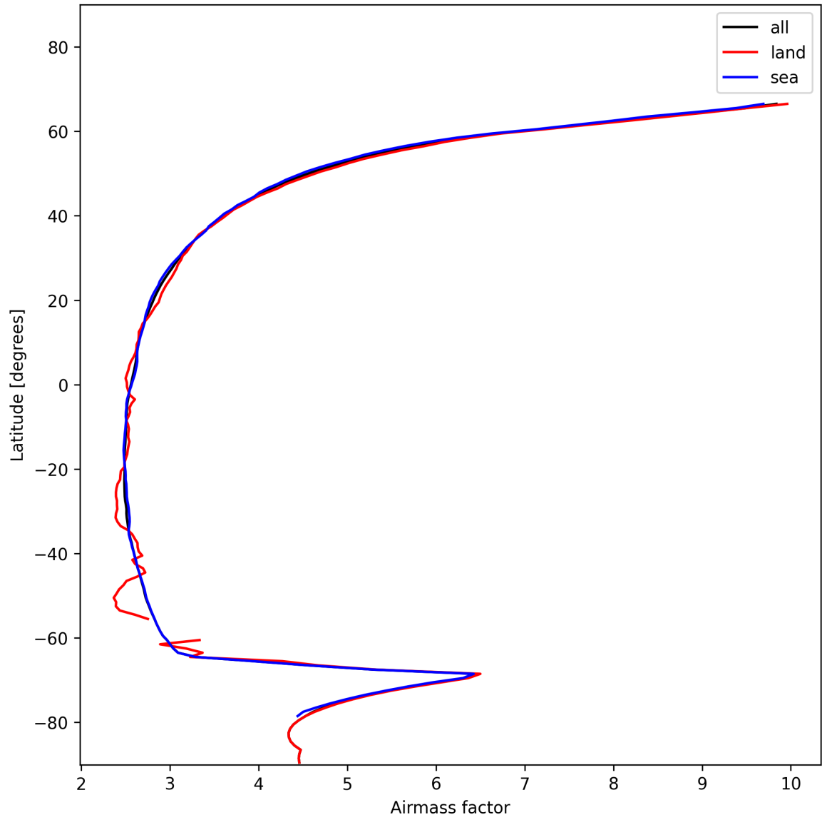
Figure 25: Zonal average of “Airmass factor” for 2024-12-06 to 2024-12-07.
