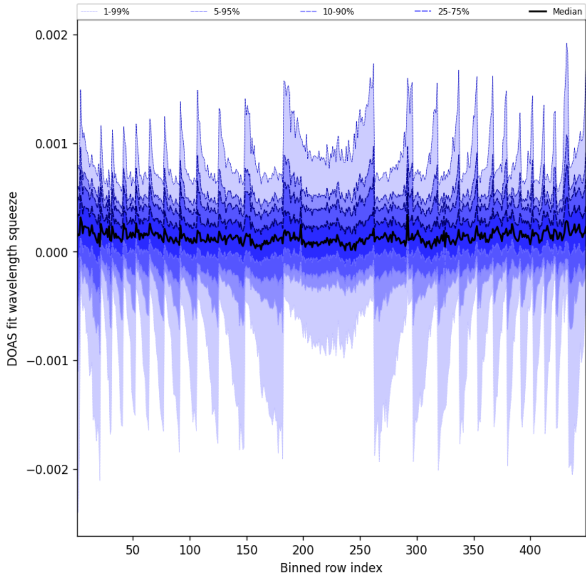
Figure 48: Along track statistics of “DOAS fit wavelength squeeze” for 2024-12-06 to 2024-12-07
