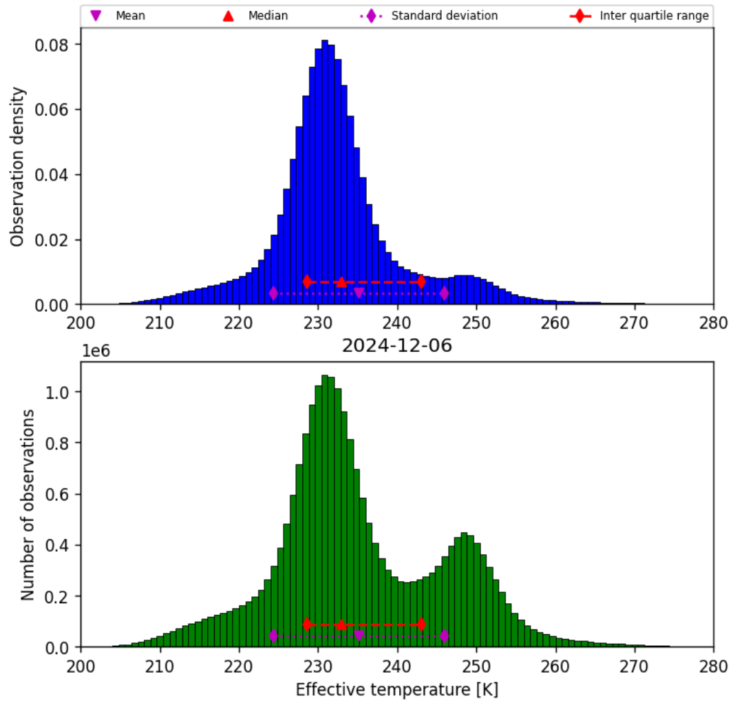
Figure 38: Histogram of “Effective temperature” for 2024-12-06 to 2024-12-07
