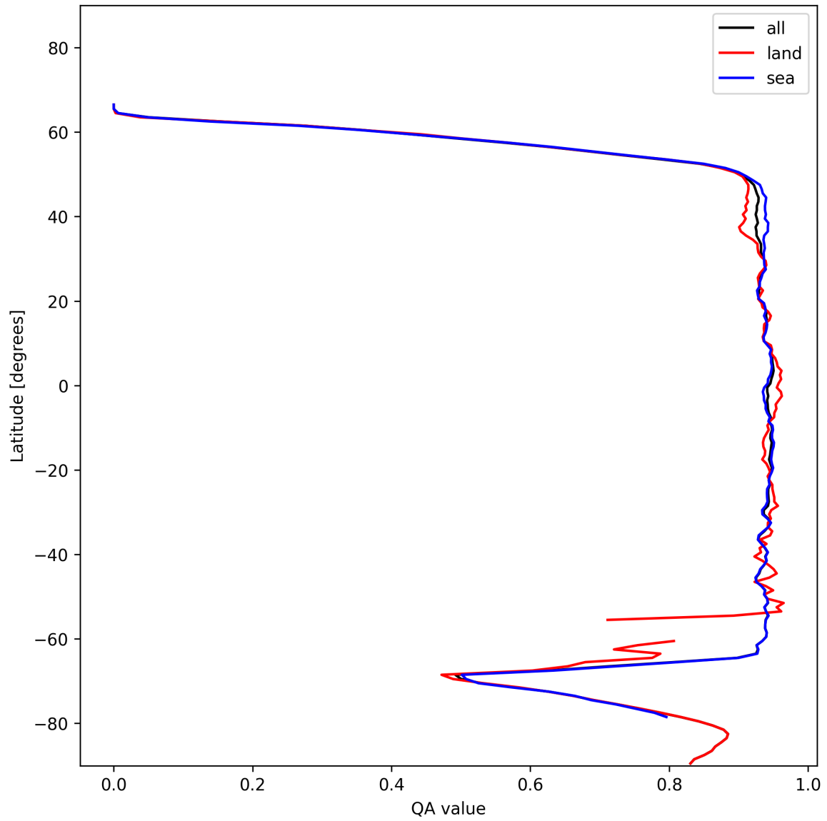
Figure 16: Zonal average of “QA value” for 2024-12-06 to 2024-12-07.
