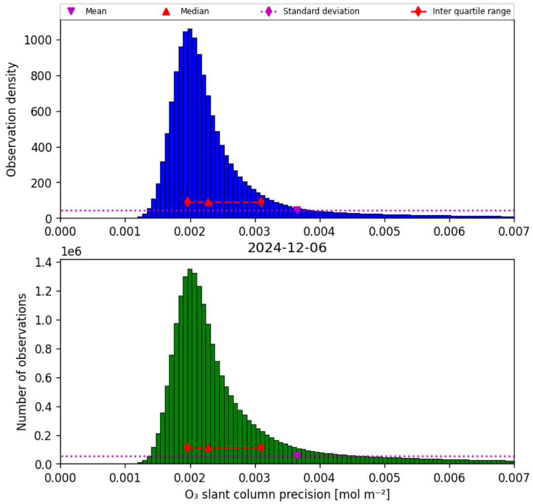
Figure 32: Histogram of “O 3 slant column precision” for 2024-12-06 to 2024-12-07
