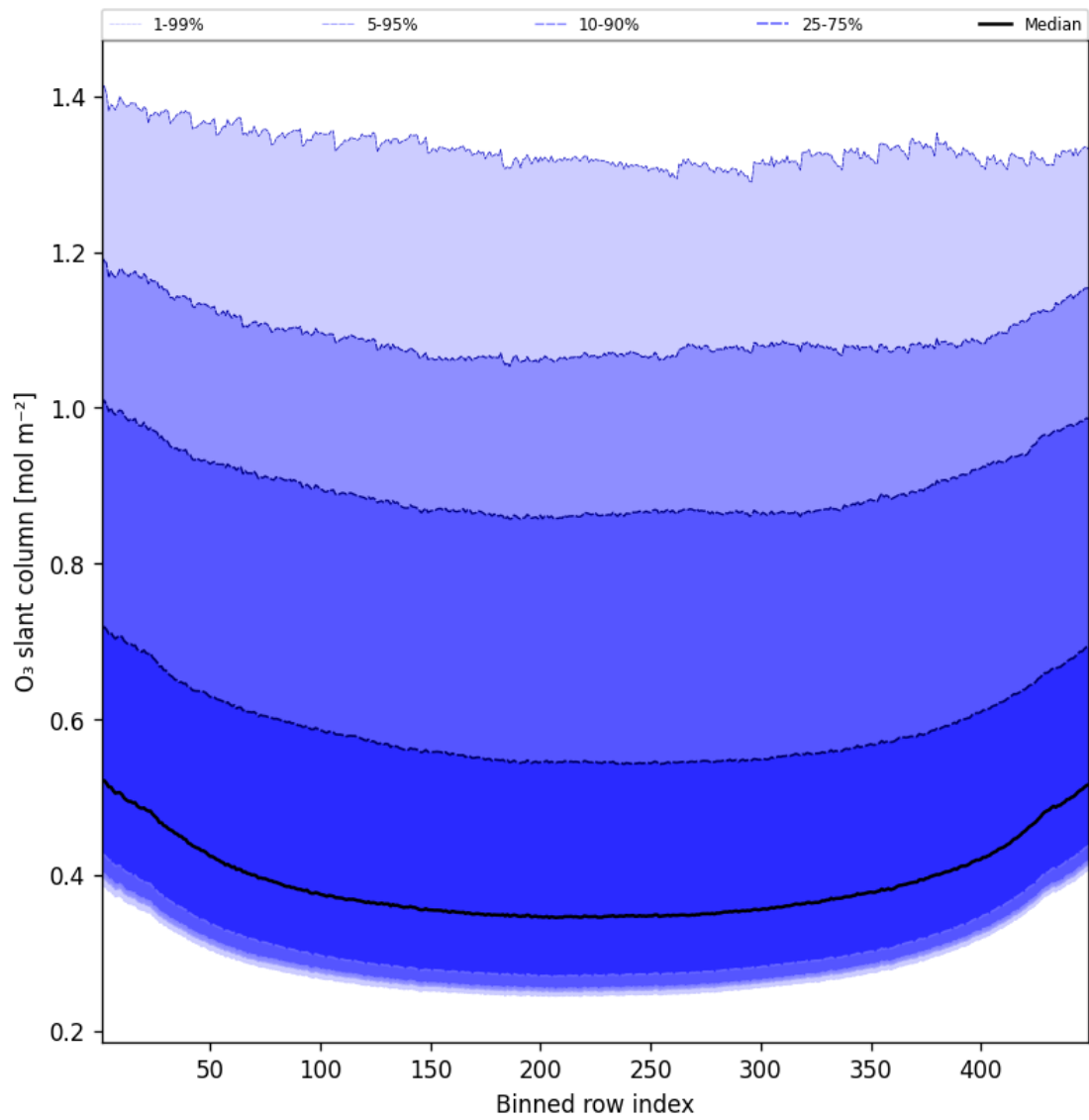
Figure 43: Along track statistics of “O 3 slant column” for 2024-12-06 to 2024-12-07
