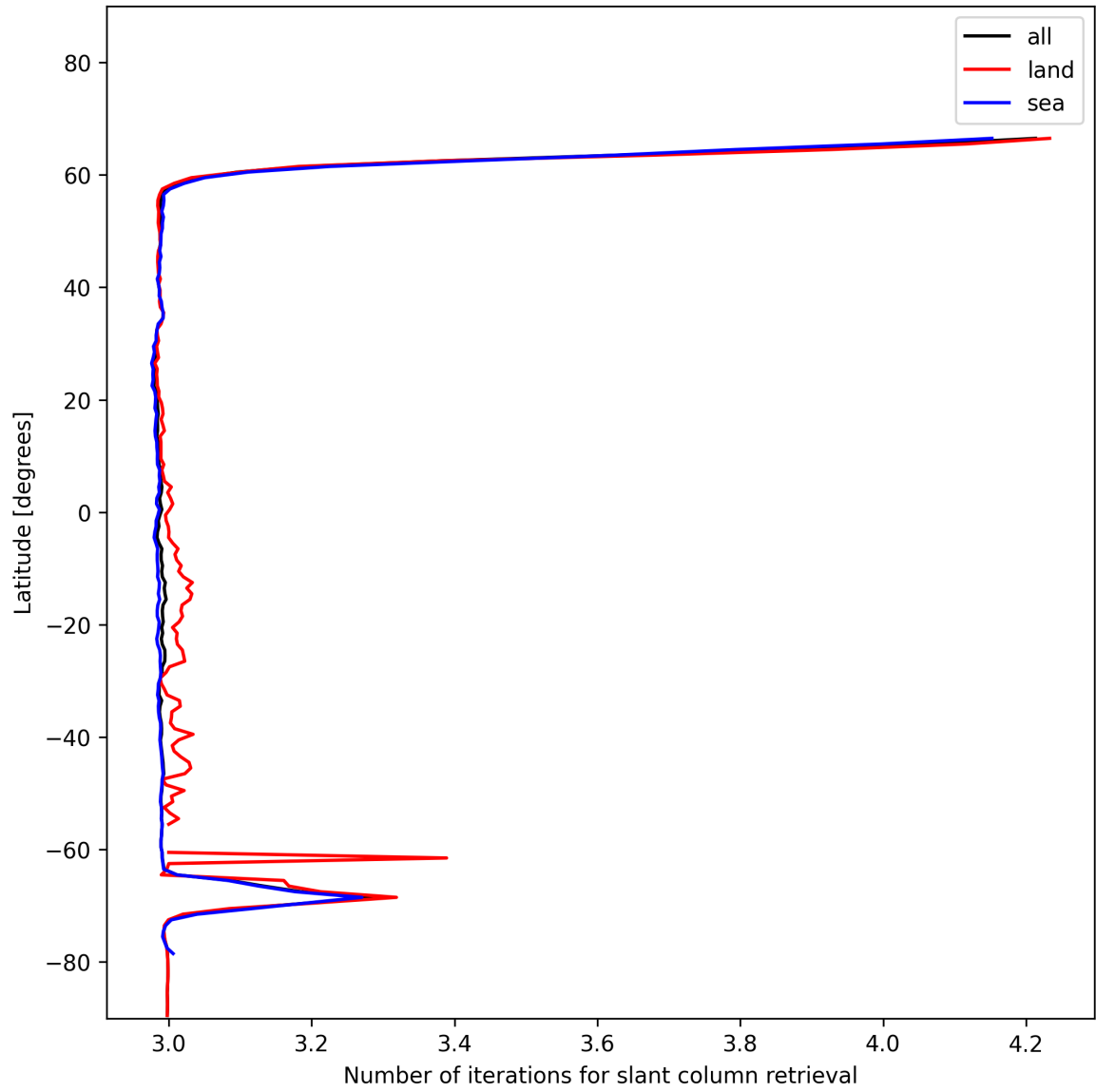
Figure 21: Zonal average of “Number of iterations for slant column retrieval” for 2024-12-06 to 2024-12-07.
