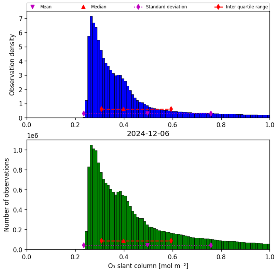
Figure 31: Histogram of “O 3 slant column” for 2024-12-06 to 2024-12-07
