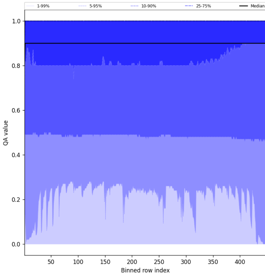
Figure 40: Along track statistics of “QA value” for 2024-12-06 to 2024-12-07
