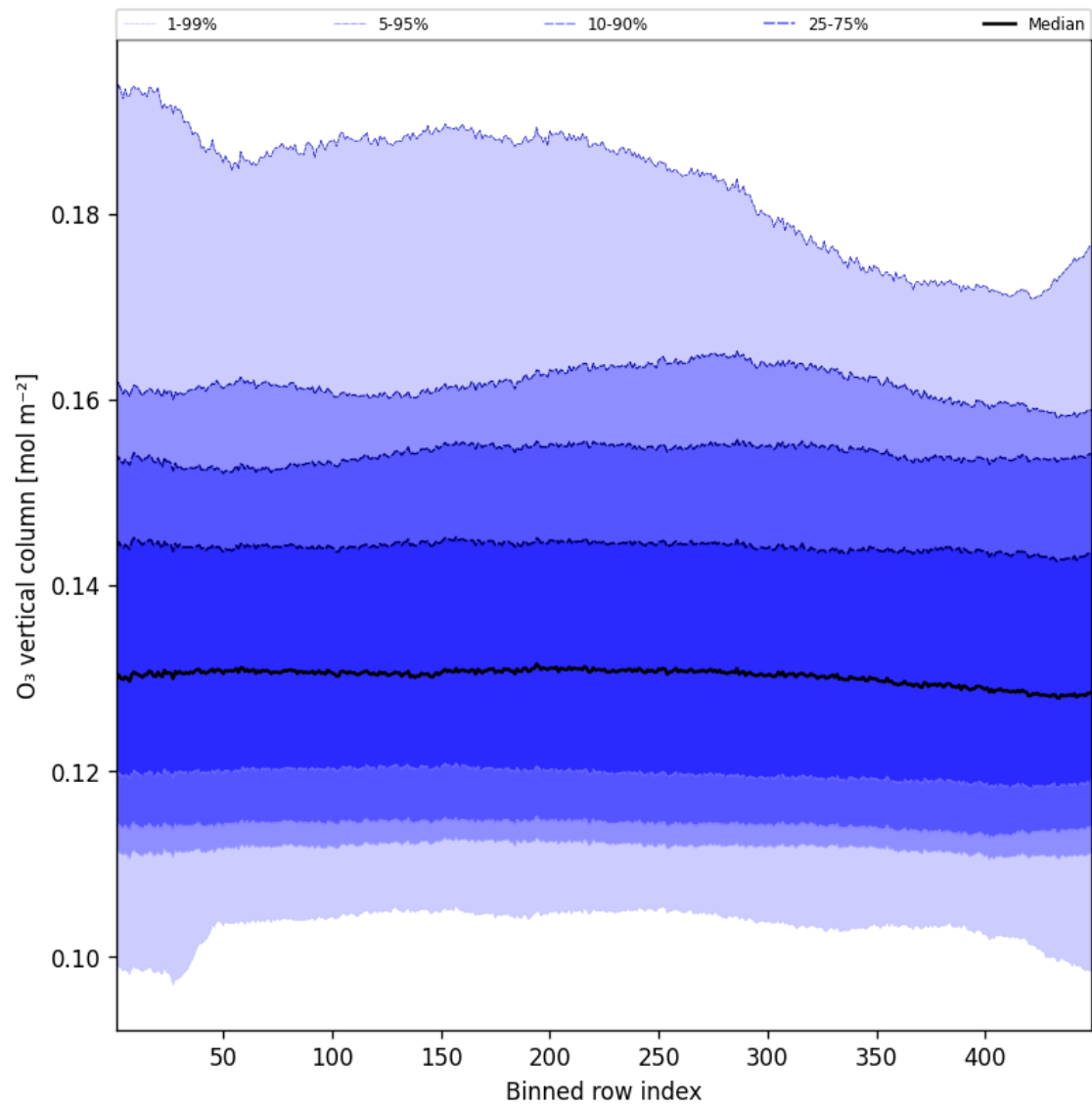
Figure 41: Along track statistics of “O 3 vertical column” for 2024-12-06 to 2024-12-07
