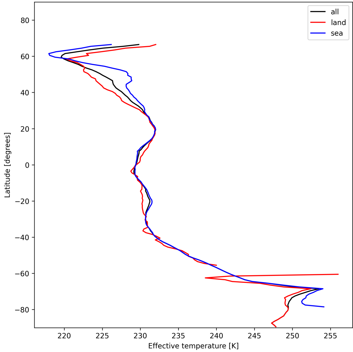
Figure 26: Zonal average of “Effective temperature” for 2024-12-06 to 2024-12-07.
