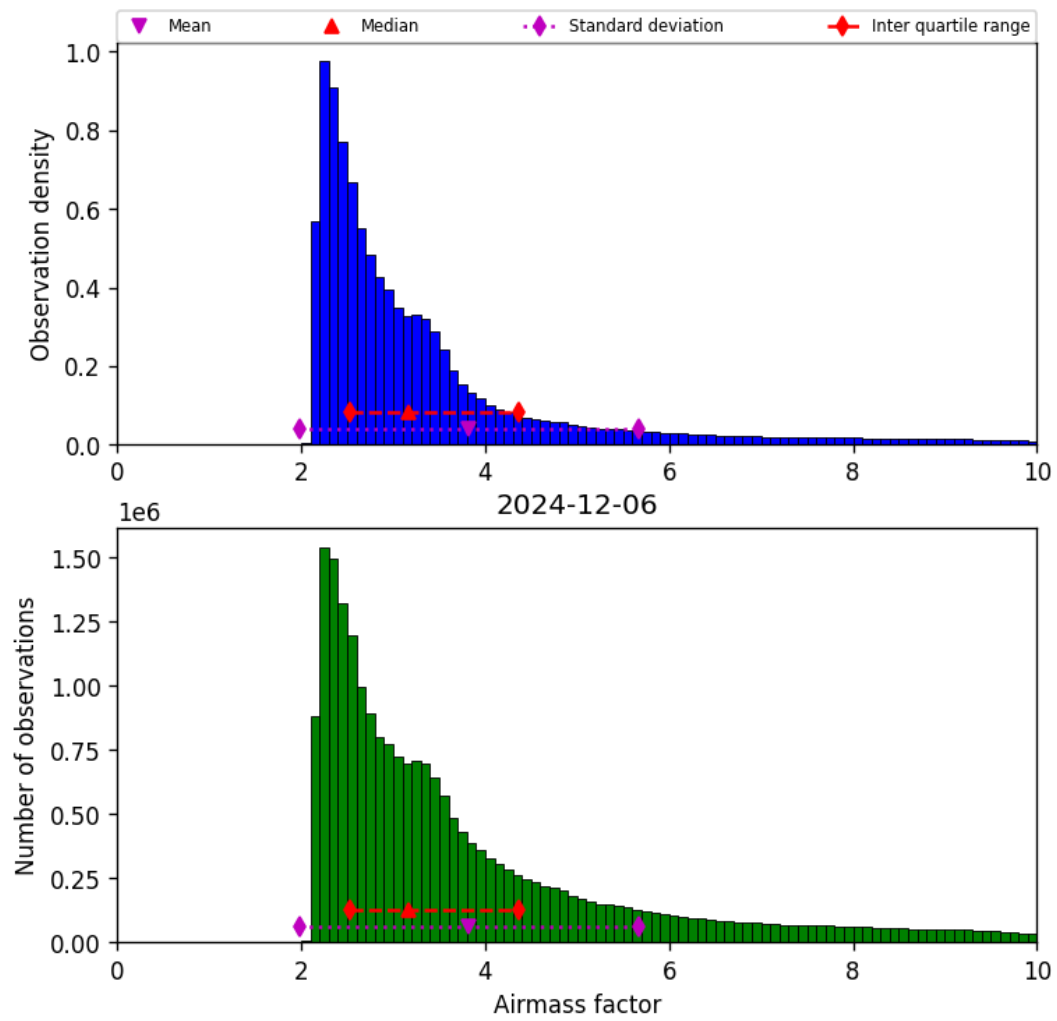
Figure 37: Histogram of “Airmass factor” for 2024-12-06 to 2024-12-07
