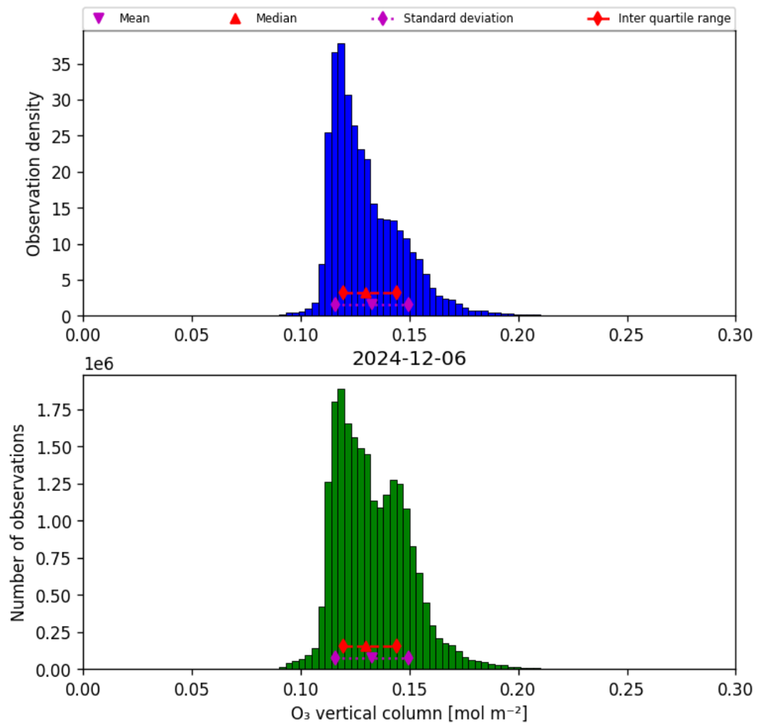
Figure 29: Histogram of “O 3 vertical column” for 2024-12-06 to 2024-12-07
