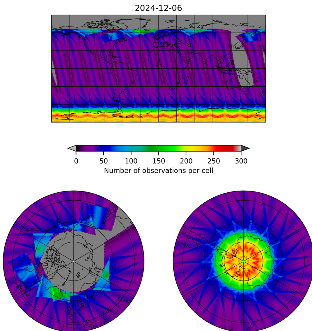
Figure 15: Map of the number of observations for 2024-12-06 to 2024-12-07
