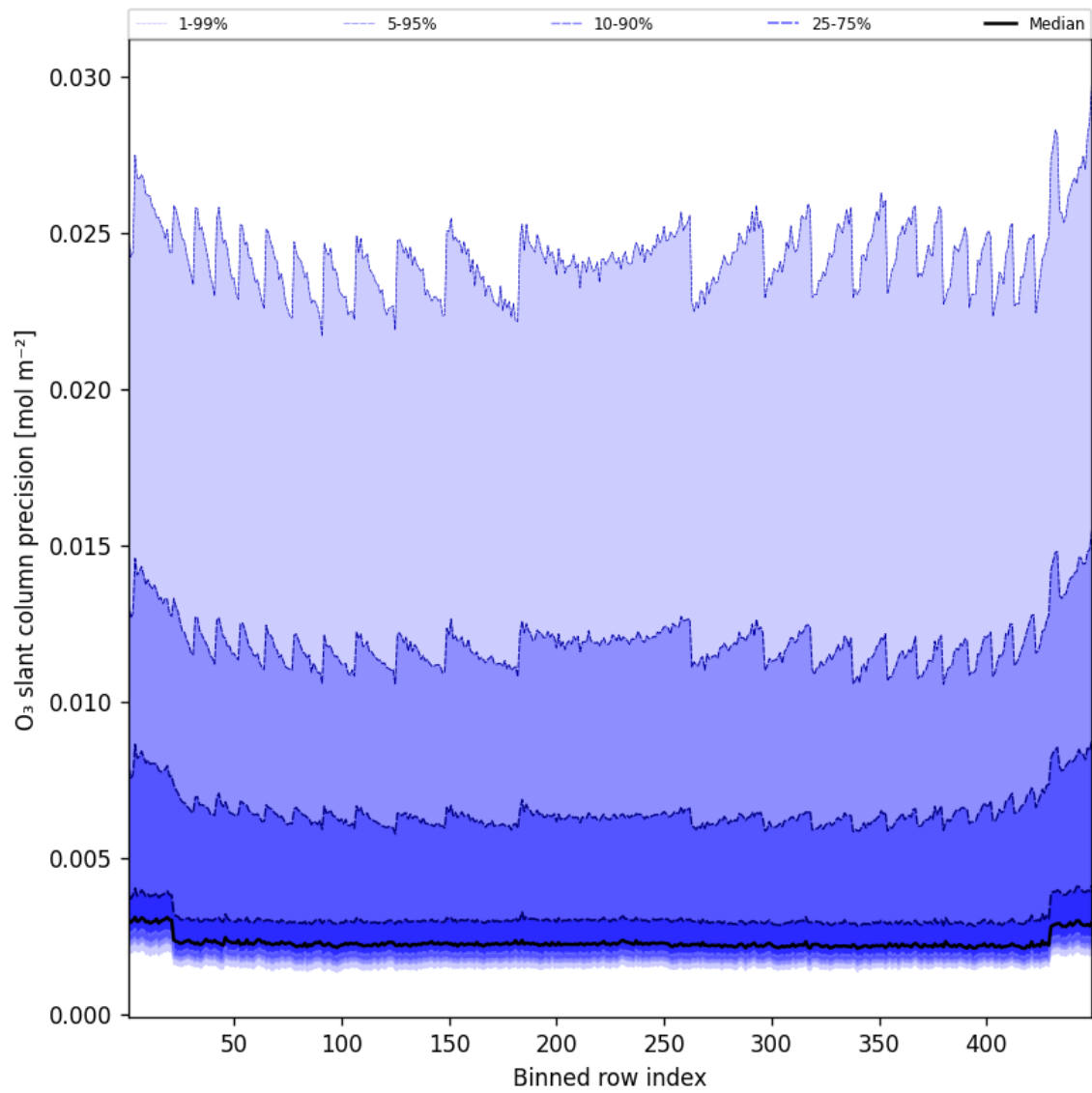
Figure 44: Along track statistics of “O 3 slant column precision” for 2024-12-06 to 2024-12-07
