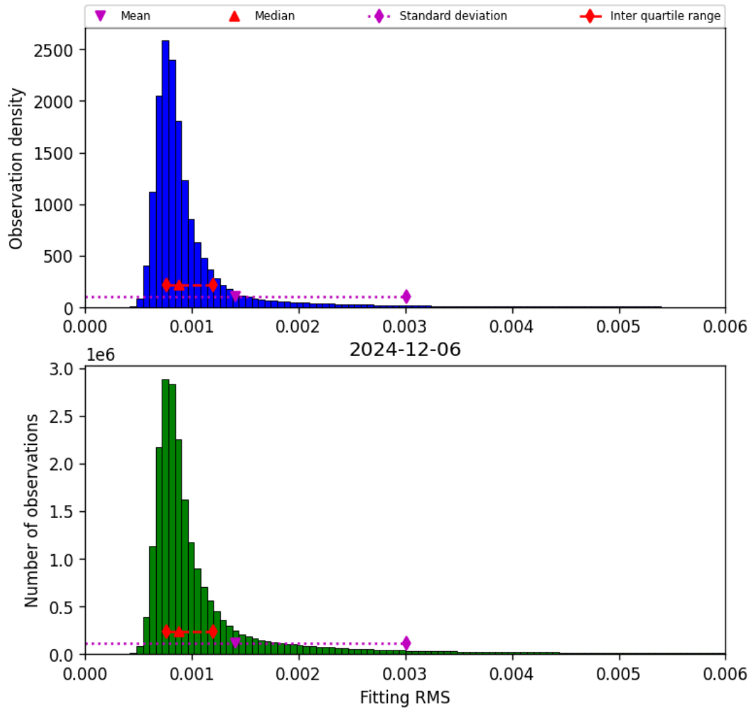
Figure 34: Histogram of “Fitting RMS” for 2024-12-06 to 2024-12-07
