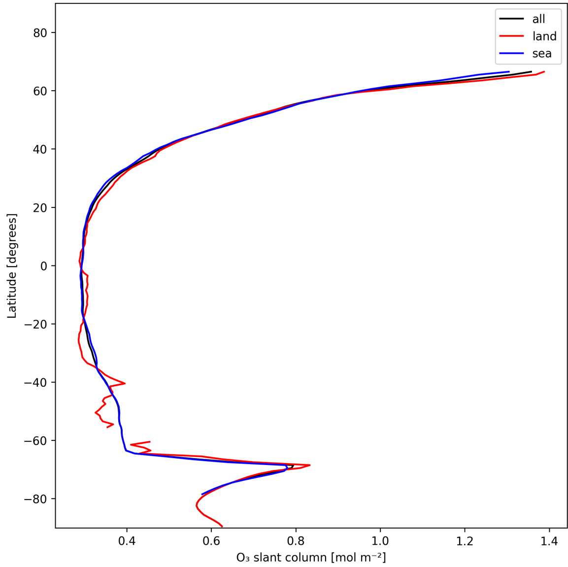
Figure 19: Zonal average of “O 3 slant column” for 2024-12-06 to 2024-12-07.
