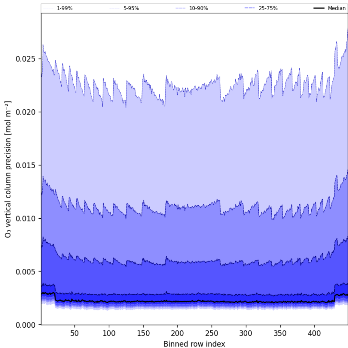
Figure 42: Along track statistics of “O 3 vertical column precision” for 2024-12-06 to 2024-12-07
