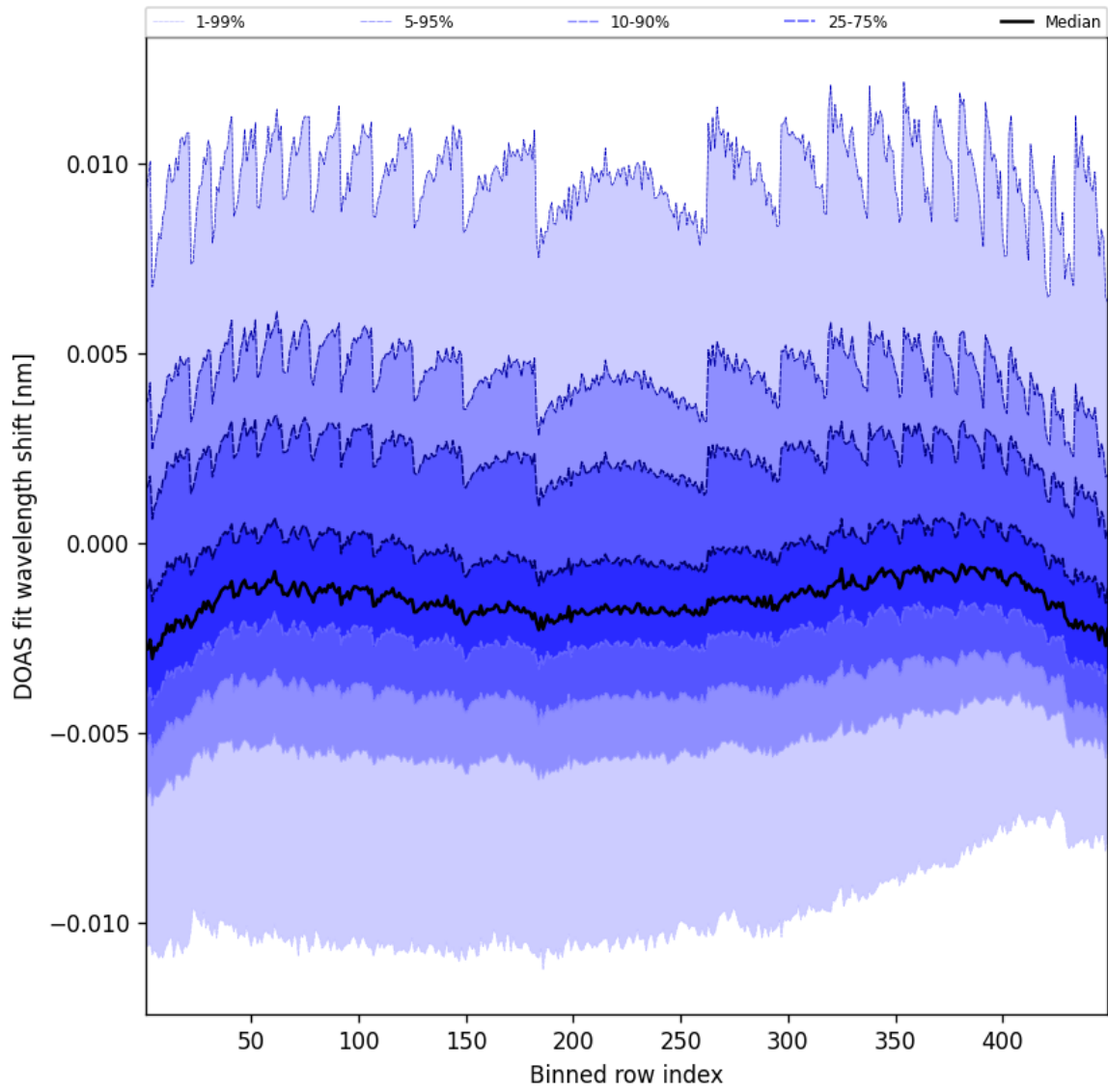
Figure 47: Along track statistics of “DOAS fit wavelength shift” for 2024-12-06 to 2024-12-07
