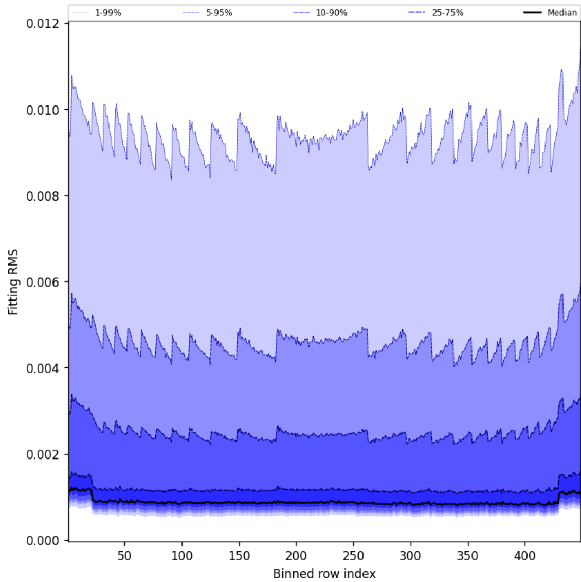
Figure 46: Along track statistics of “Fitting RMS” for 2024-12-06 to 2024-12-07
