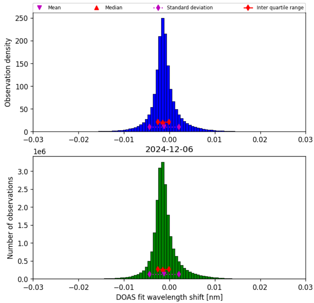
Figure 35: Histogram of “DOAS fit wavelength shift” for 2024-12-06 to 2024-12-07
