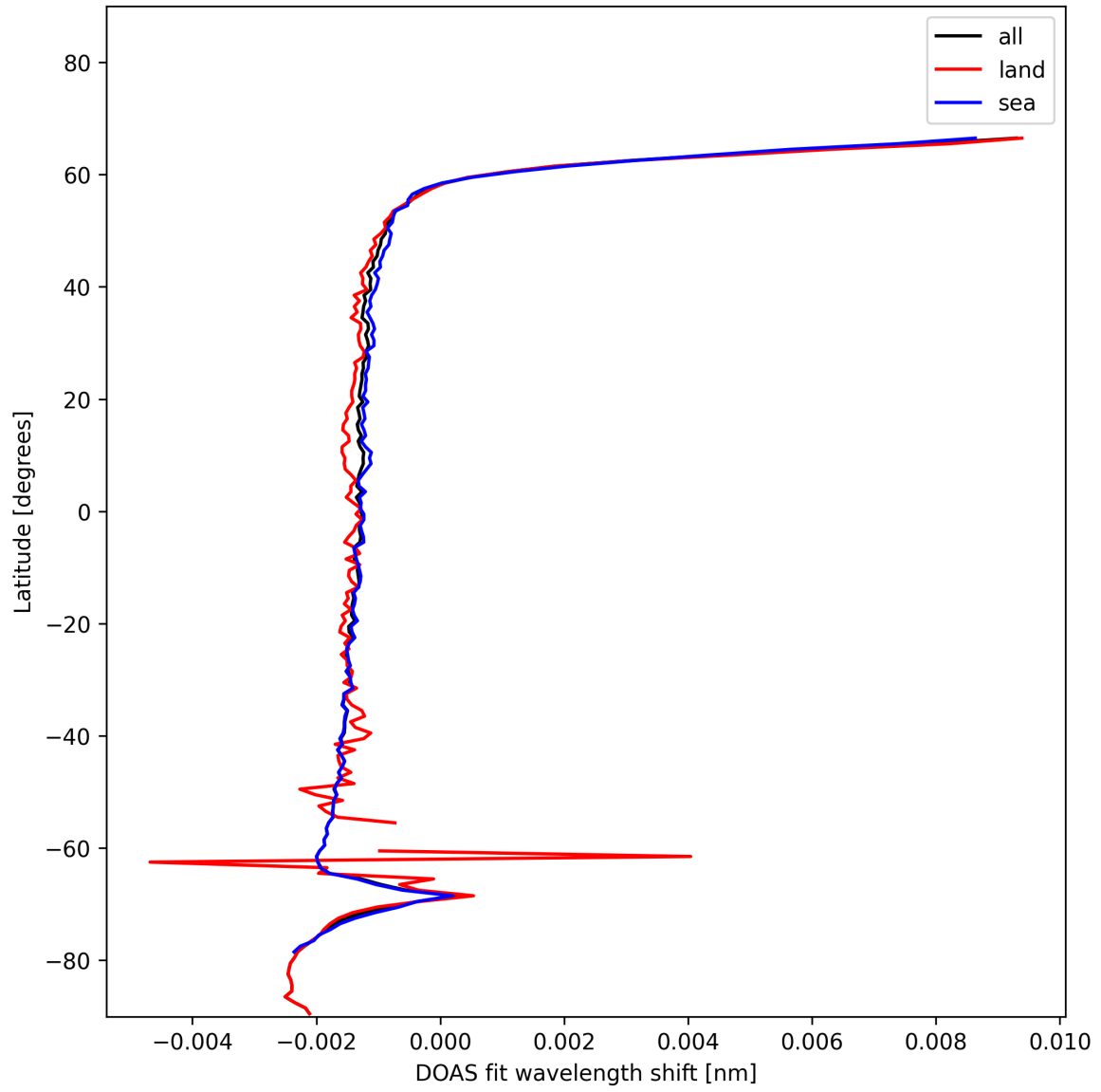
Figure 23: Zonal average of "DOAS fit wavelength shift" for 2024-12-06 to 2024-12-07.
