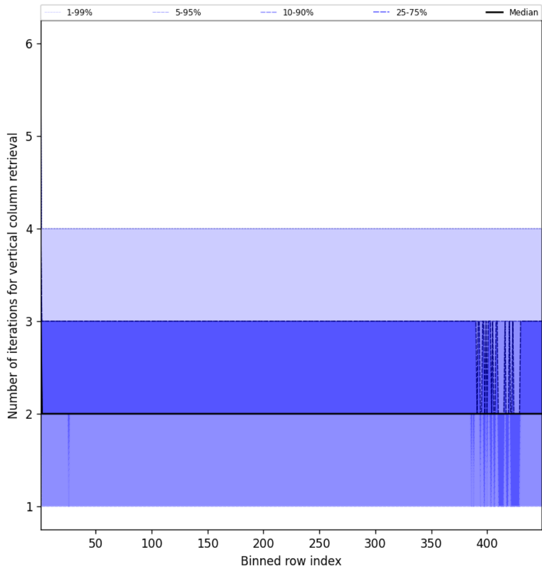
Figure 51: Along track statistics of “Number of iterations for vertical column retrieval” for 2024-12-06 to 2024-12-07
