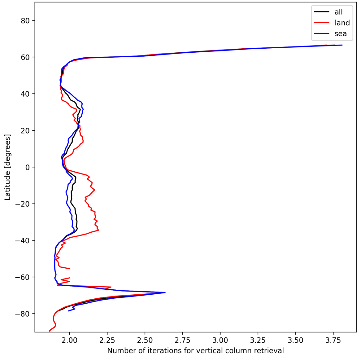
Figure 27: Zonal average of “Number of iterations for vertical column retrieval” for 2024-12-06 to 2024-12-07.
