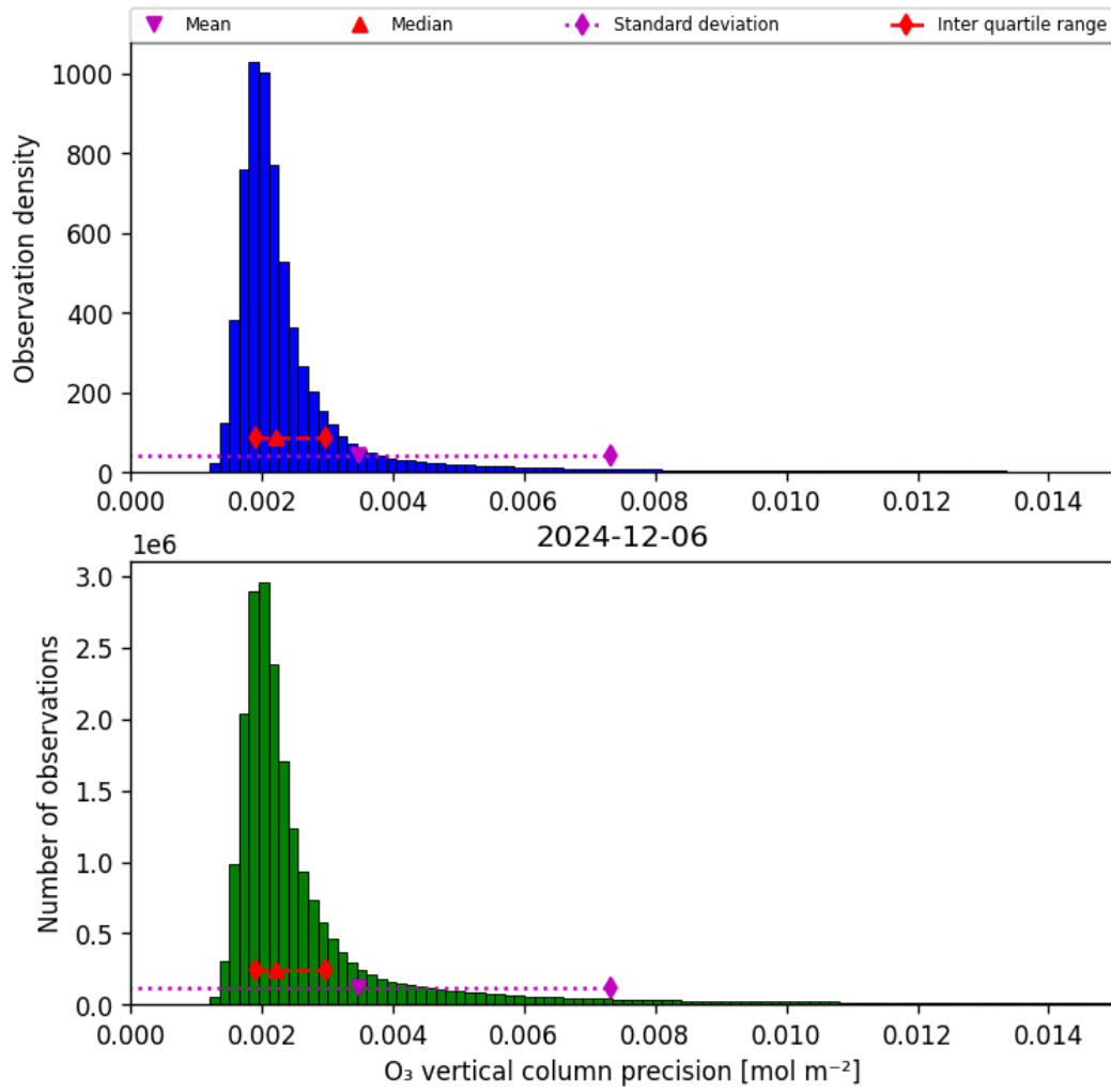
Figure 30: Histogram of “O 3 vertical column precision” for 2024-12-06 to 2024-12-07
