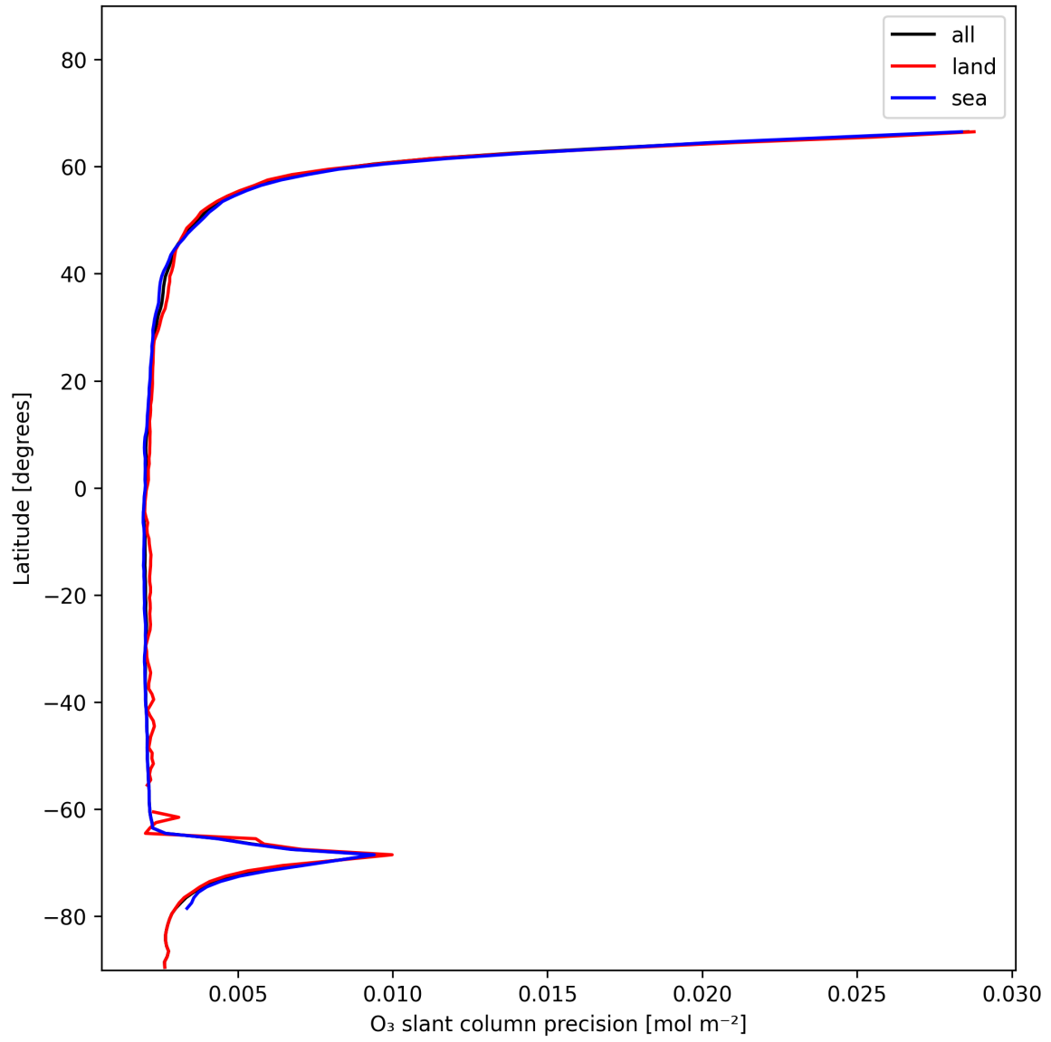
Figure 20: Zonal average of "O 3 slant column precision" for 2024-12-06 to 2024-12-07.
