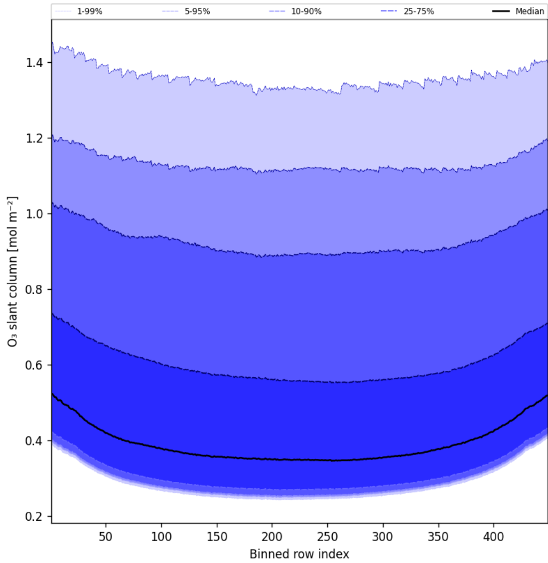
Figure 43: Along track statistics of “O 3 slant column” for 2024-12-07 to 2024-12-08
