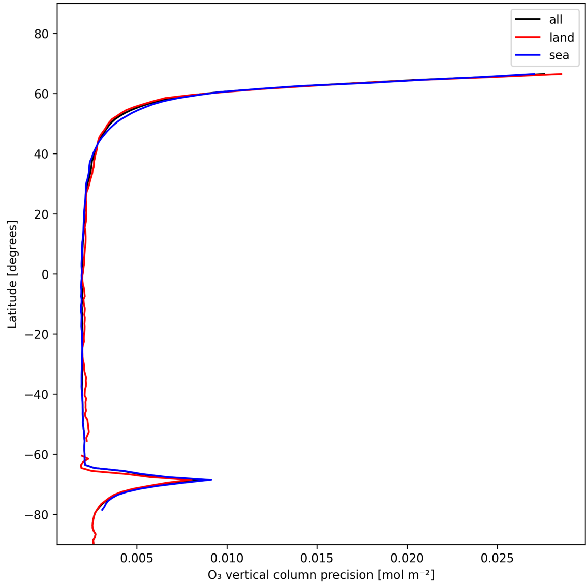
Figure 18: Zonal average of “O 3 vertical column precision” for 2024-12-07 to 2024-12-08.
