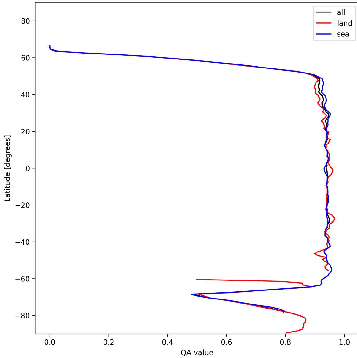
Figure 16: Zonal average of “QA value” for 2024-12-07 to 2024-12-08.
