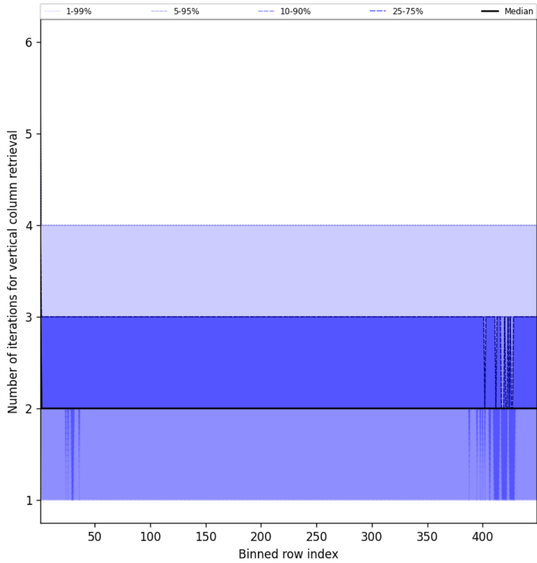
Figure 51: Along track statistics of “Number of iterations for vertical column retrieval” for 2024-12-07 to 2024-12-08
