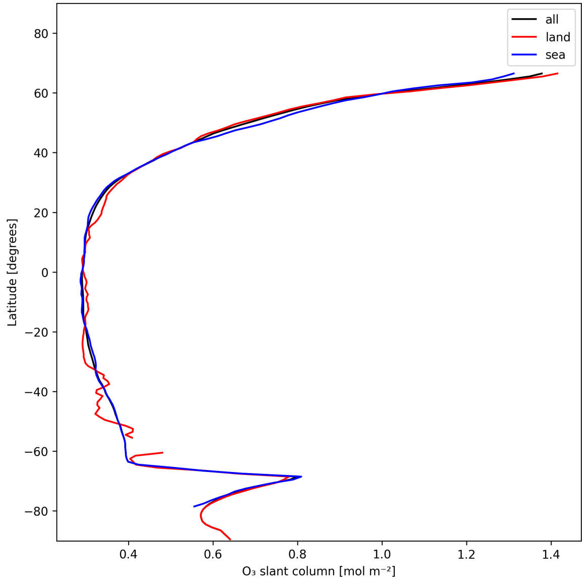
Figure 19: Zonal average of “O 3 slant column” for 2024-12-07 to 2024-12-08.
