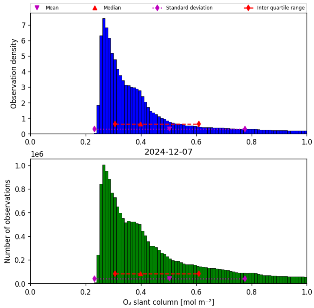
Figure 31: Histogram of “O 3 slant column” for 2024-12-07 to 2024-12-08
