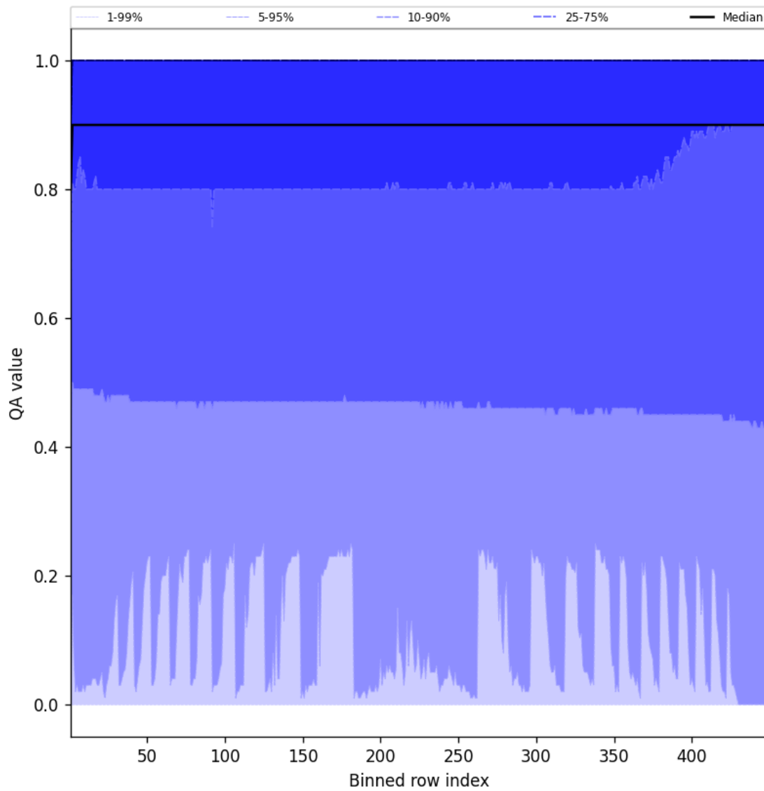
Figure 40: Along track statistics of “QA value” for 2024-12-07 to 2024-12-08
