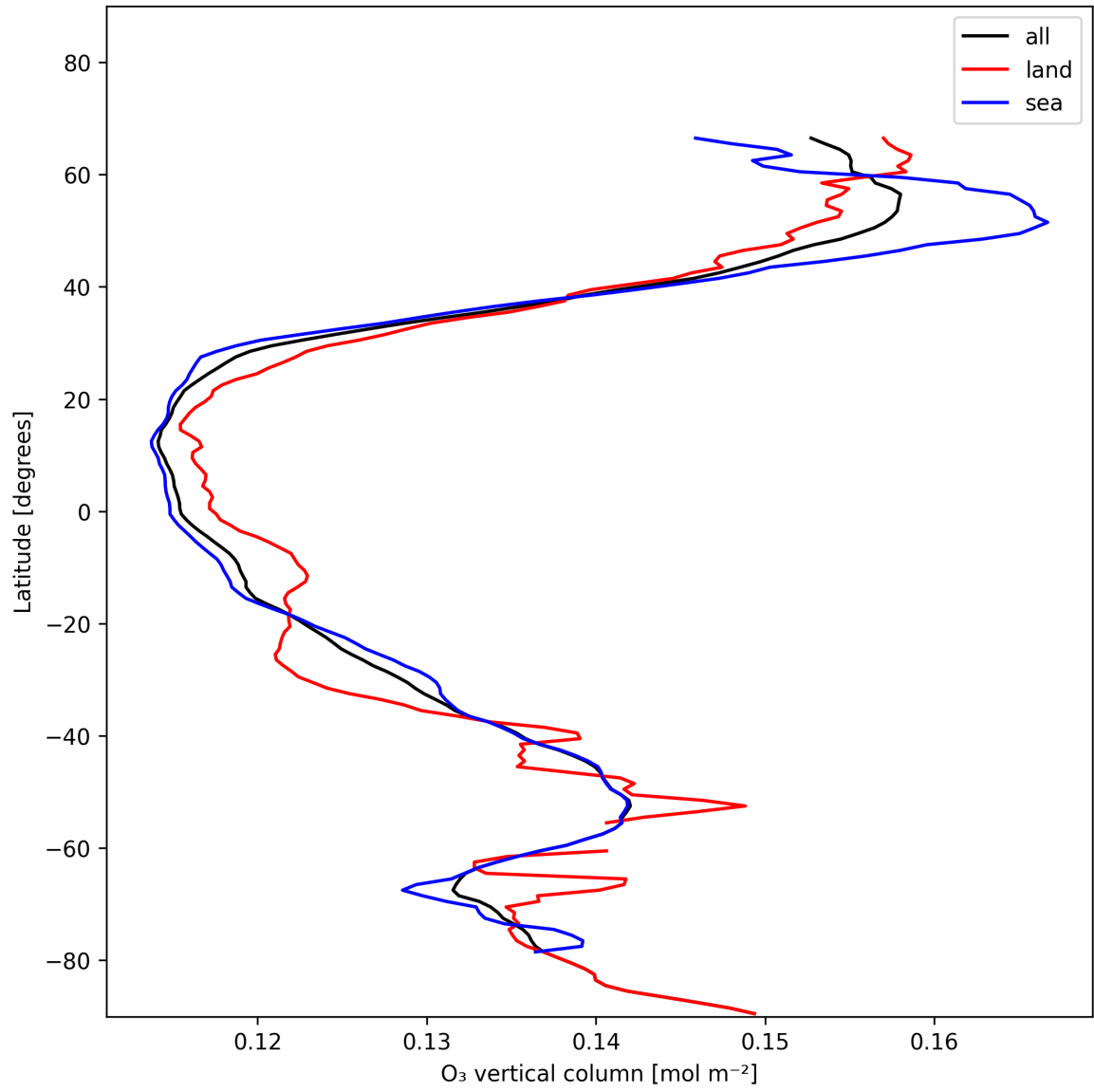
Figure 17: Zonal average of “O 3 vertical column” for 2024-12-07 to 2024-12-08.
