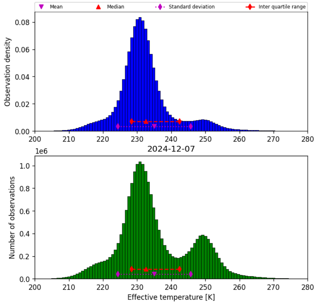
Figure 38: Histogram of “Effective temperature” for 2024-12-07 to 2024-12-08
