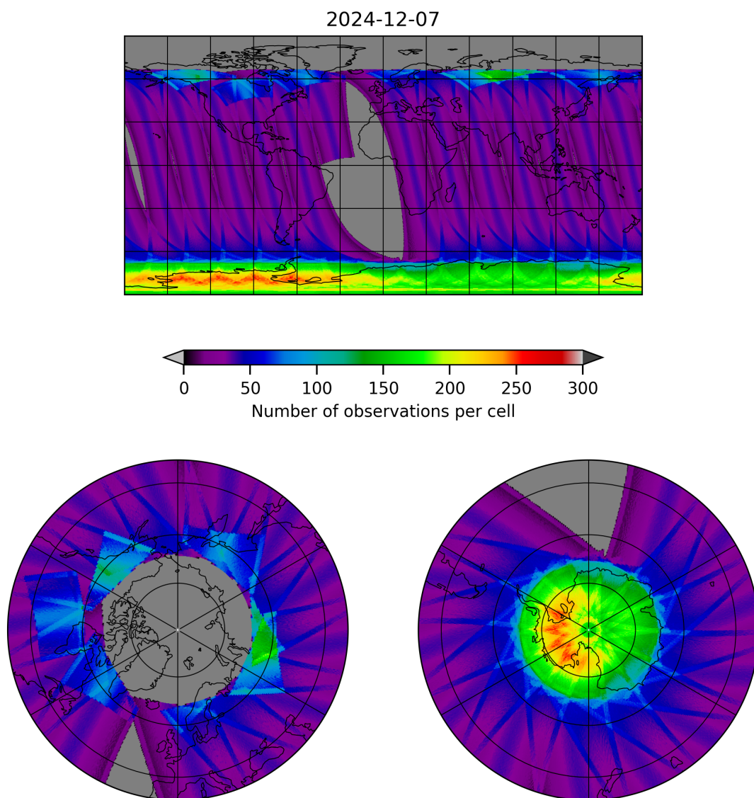
Figure 15: Map of the number of observations for 2024-12-07 to 2024-12-08
