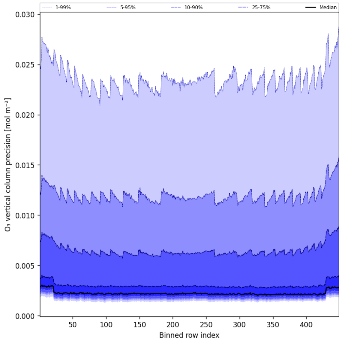
Figure 42: Along track statistics of “O 3 vertical column precision” for 2024-12-07 to 2024-12-08
