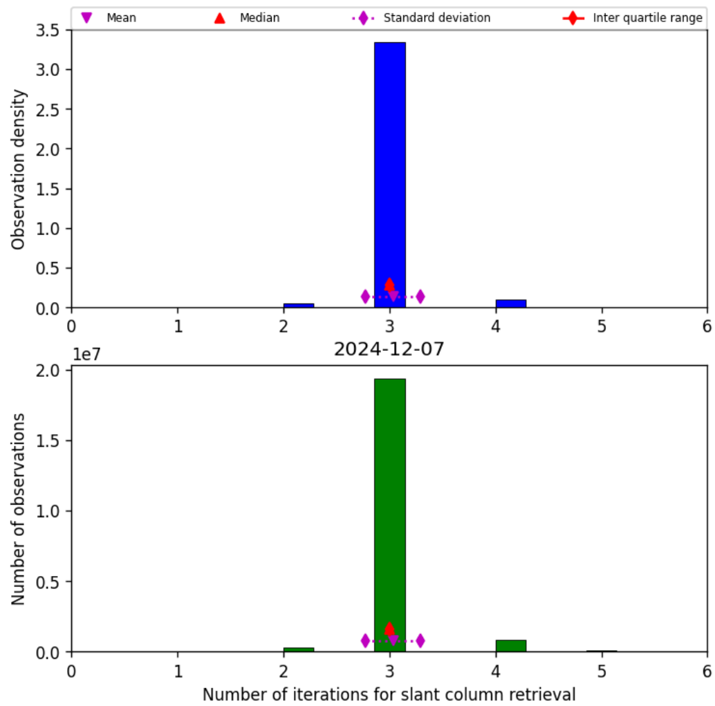
Figure 33: Histogram of “Number of iterations for slant column retrieval” for 2024-12-07 to 2024-12-08
