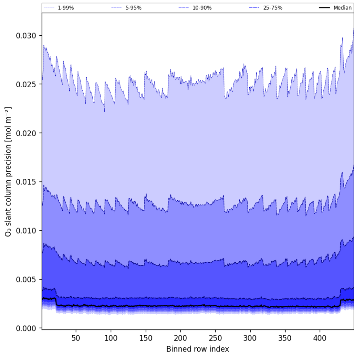
Figure 44: Along track statistics of “O 3 slant column precision” for 2024-12-07 to 2024-12-08
