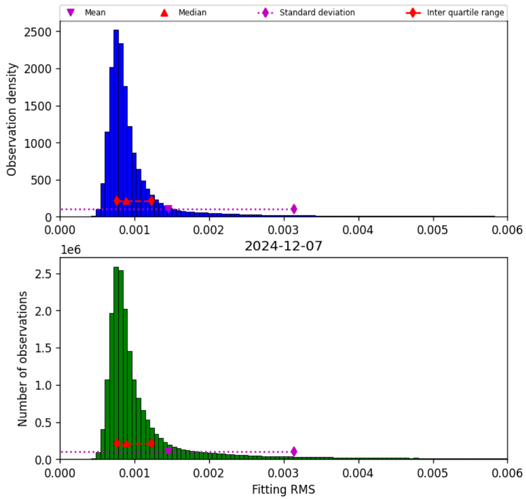
Figure 34: Histogram of "Fitting RMS" for 2024-12-07 to 2024-12-08
