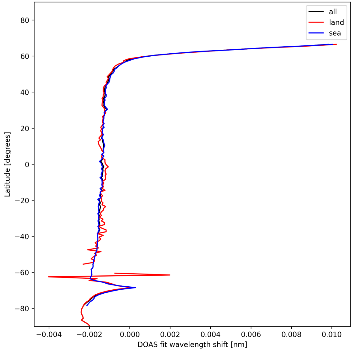
Figure 23: Zonal average of “DOAS fit wavelength shift” for 2024-12-07 to 2024-12-08.
