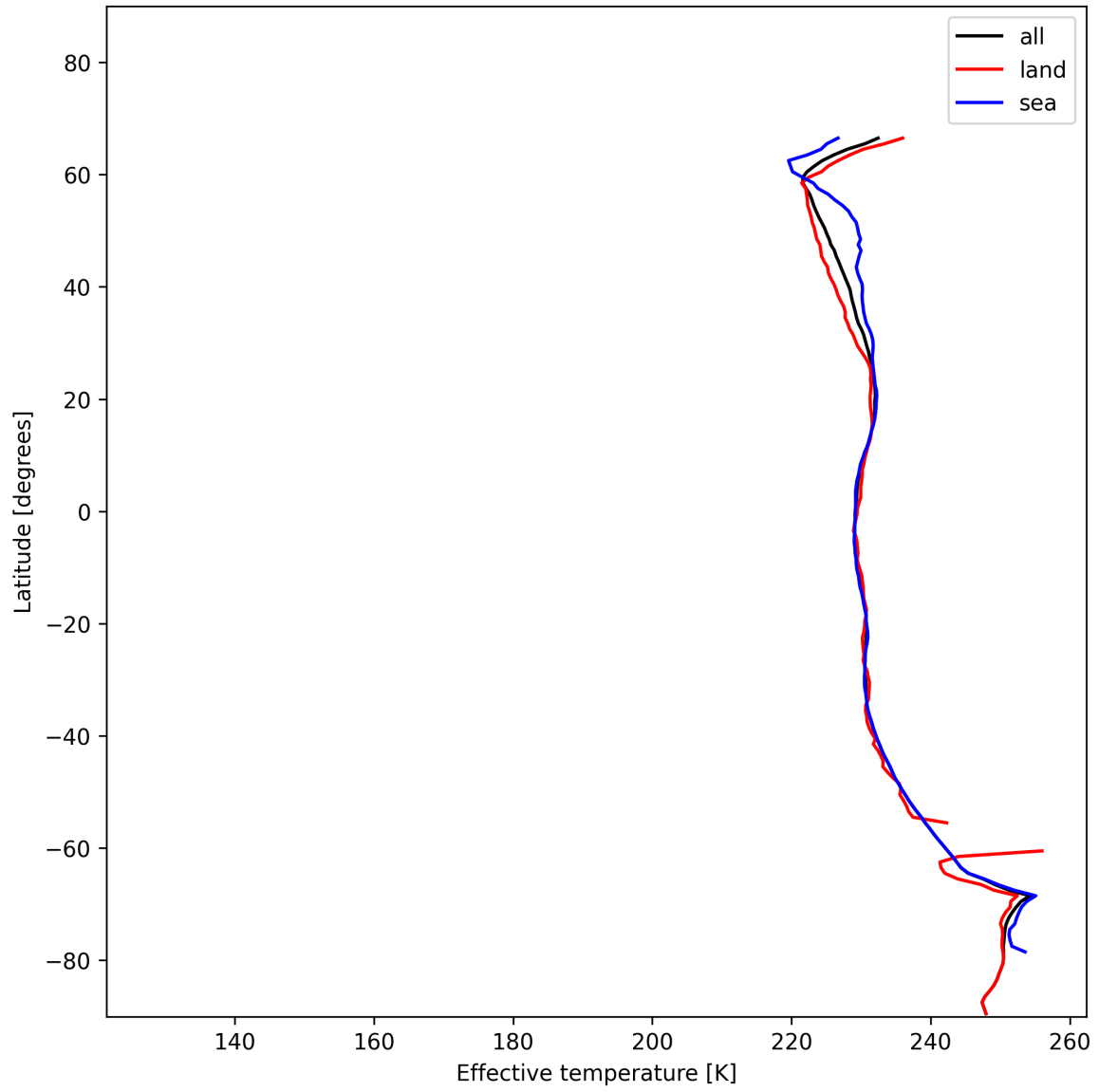
Figure 26: Zonal average of "Effective temperature" for 2024-12-07 to 2024-12-08.
