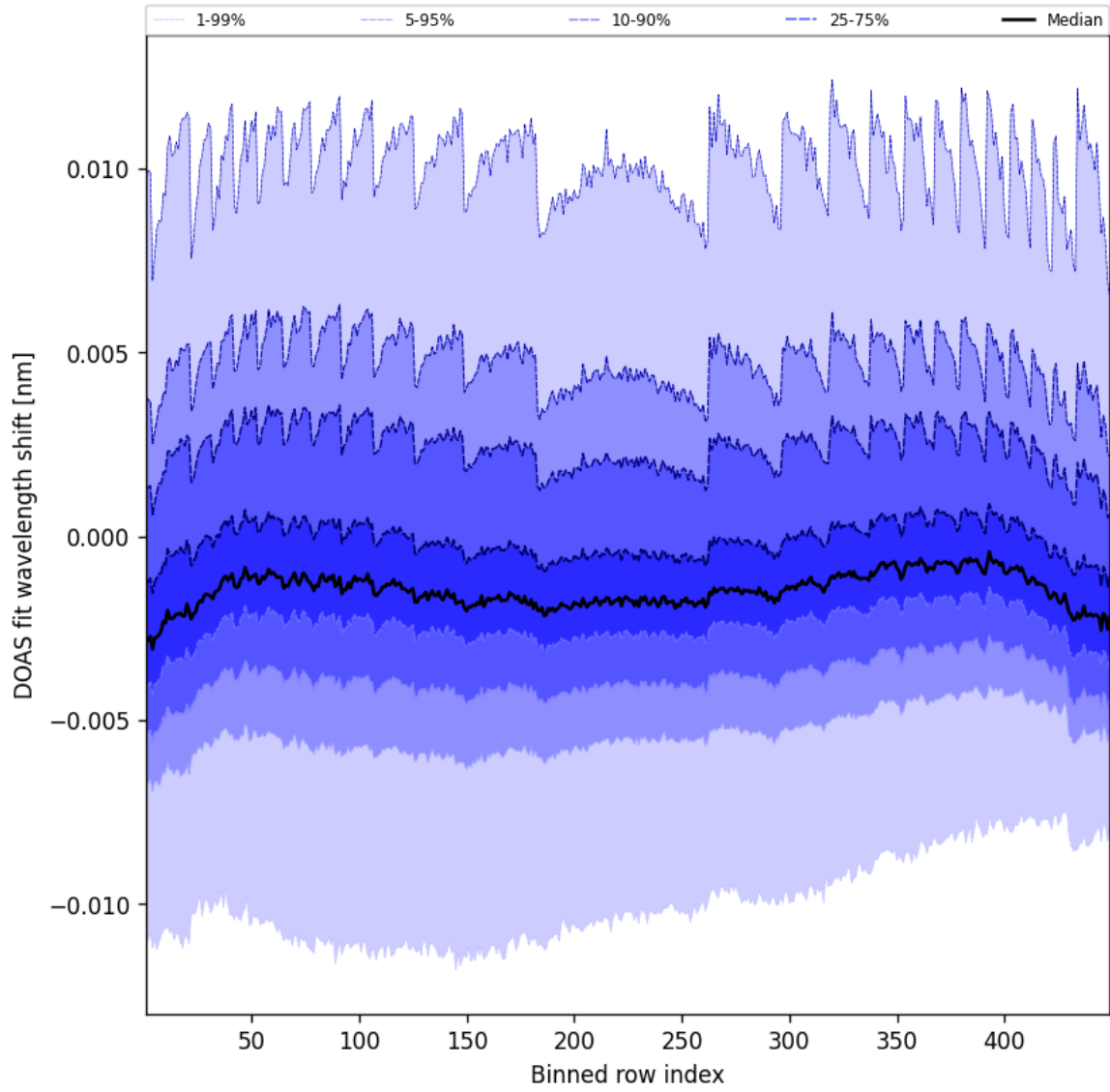
Figure 47: Along track statistics of “DOAS fit wavelength shift” for 2024-12-07 to 2024-12-08
