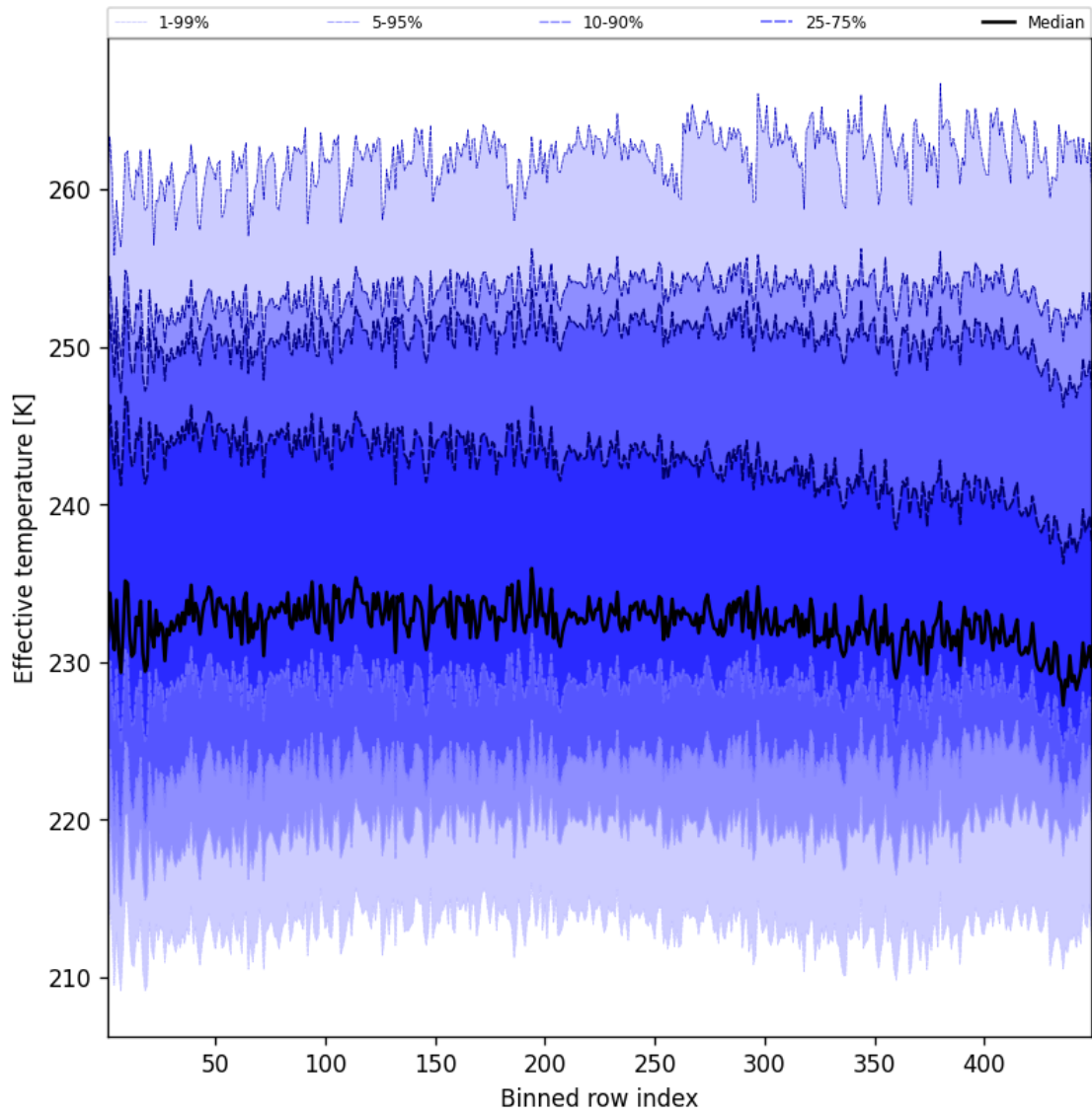
Figure 50: Along track statistics of “Effective temperature” for 2024-12-07 to 2024-12-08
