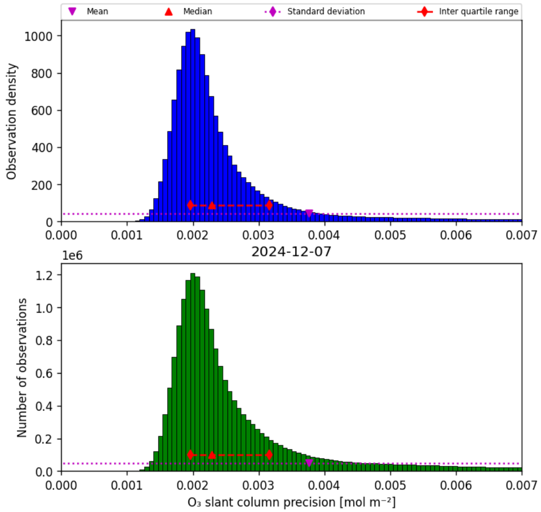
Figure 32: Histogram of “O 3 slant column precision” for 2024-12-07 to 2024-12-08
