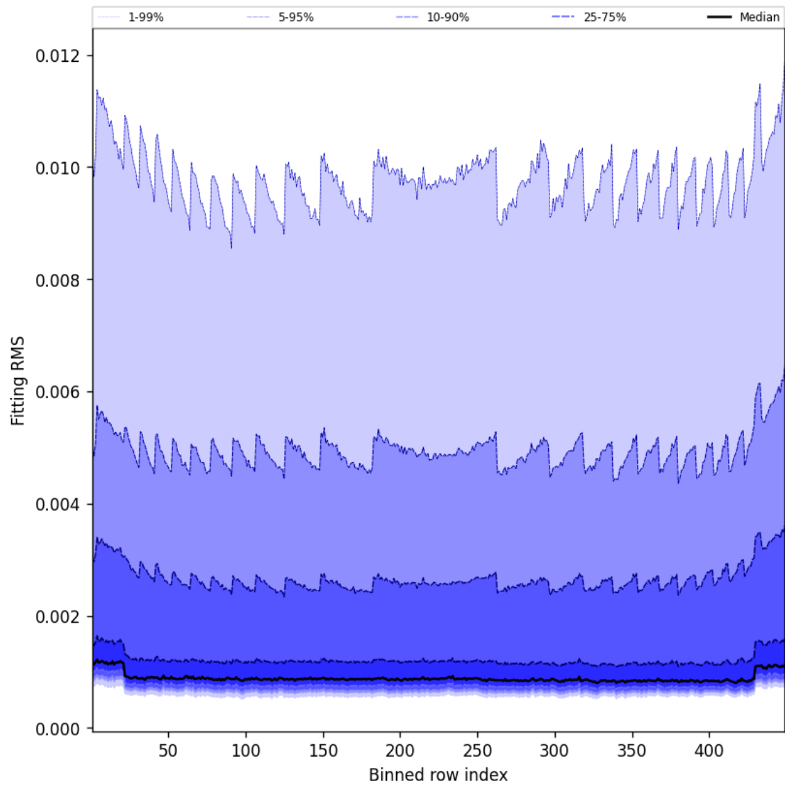
Figure 46: Along track statistics of “Fitting RMS” for 2024-12-07 to 2024-12-08
