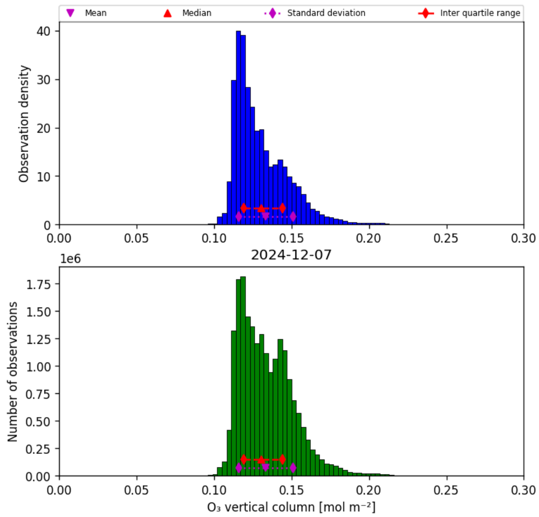
Figure 29: Histogram of “O 3 vertical column” for 2024-12-07 to 2024-12-08
