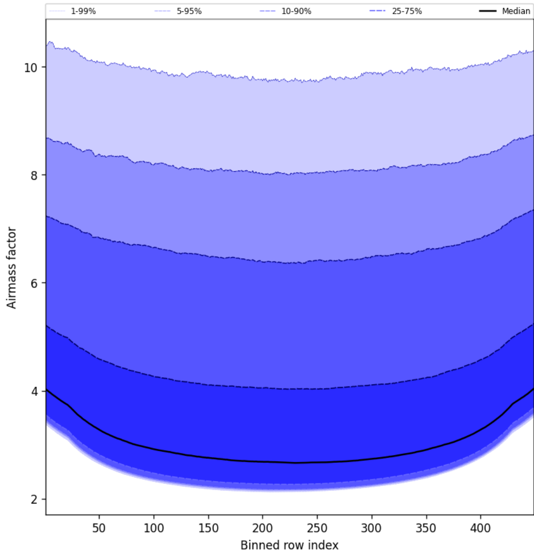
Figure 49: Along track statistics of “Airmass factor” for 2024-12-07 to 2024-12-08
