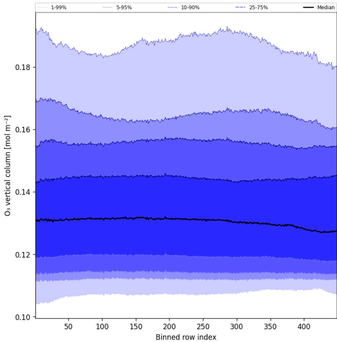
Figure 41: Along track statistics of “O 3 vertical column” for 2024-12-07 to 2024-12-08
