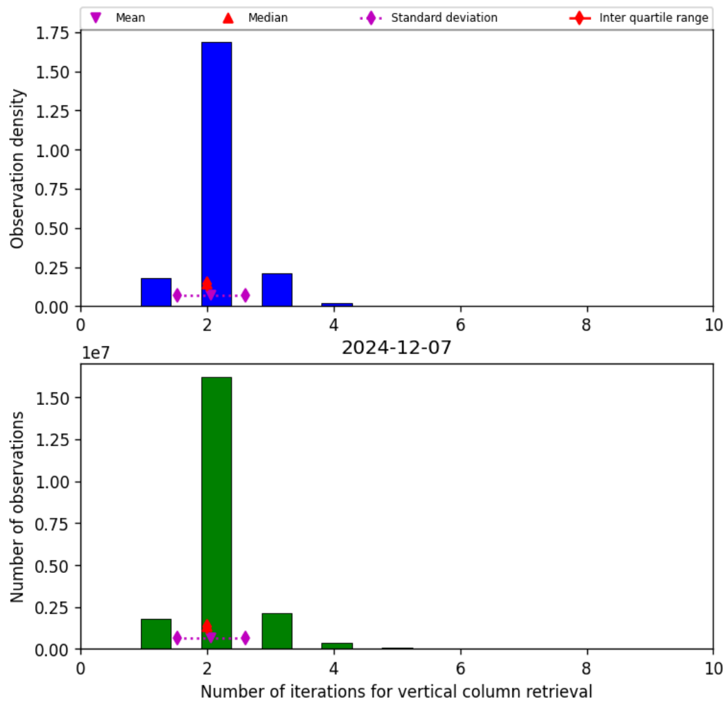
Figure 39: Histogram of “Number of iterations for vertical column retrieval” for 2024-12-07 to 2024-12-08
