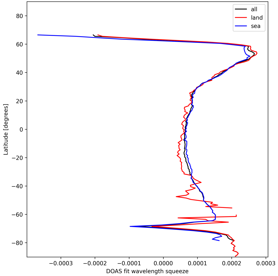
Figure 24: Zonal average of “DOAS fit wavelength squeeze” for 2024-12-07 to 2024-12-08.
