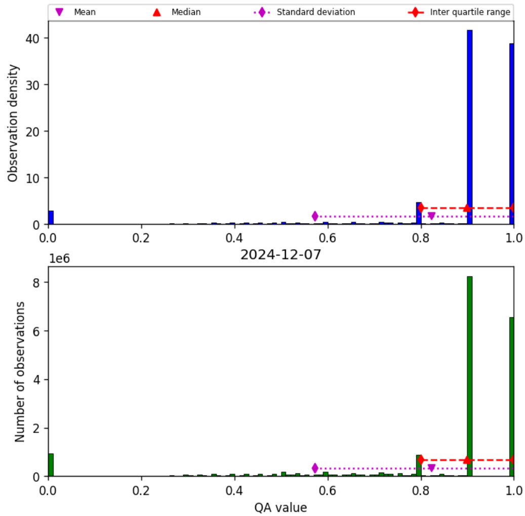
Figure 28: Histogram of “QA value” for 2024-12-07 to 2024-12-08
