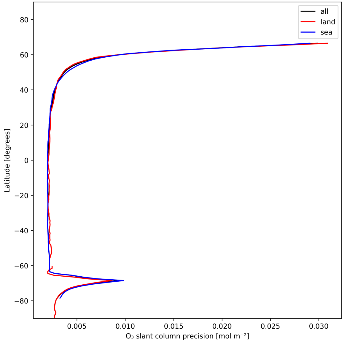
Figure 20: Zonal average of "O 3 slant column precision" for 2024-12-07 to 2024-12-08.
