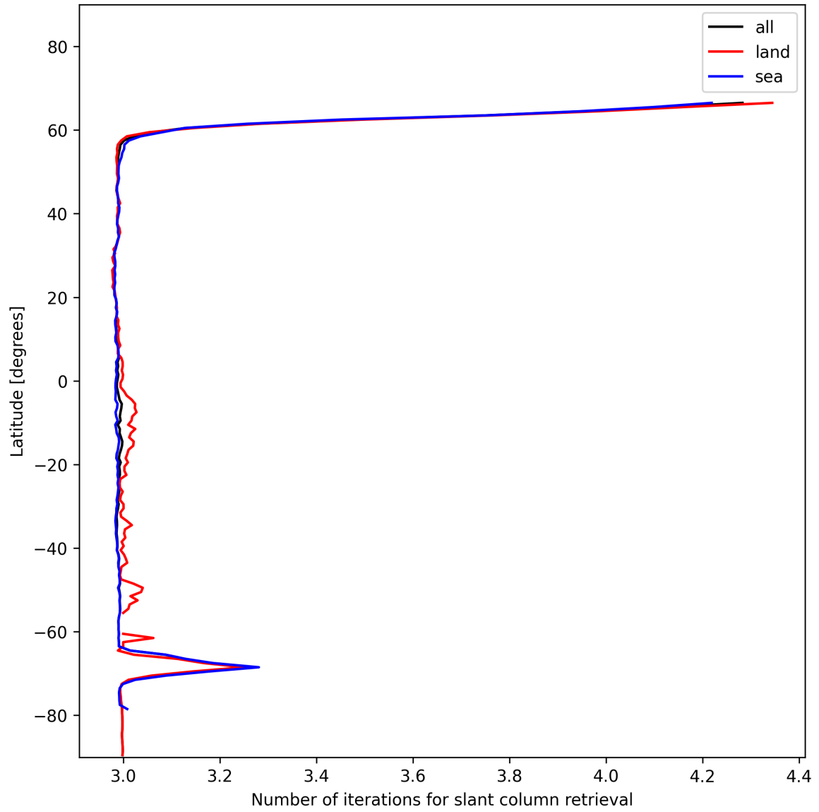
Figure 21: Zonal average of “Number of iterations for slant column retrieval” for 2024-12-07 to 2024-12-08.
