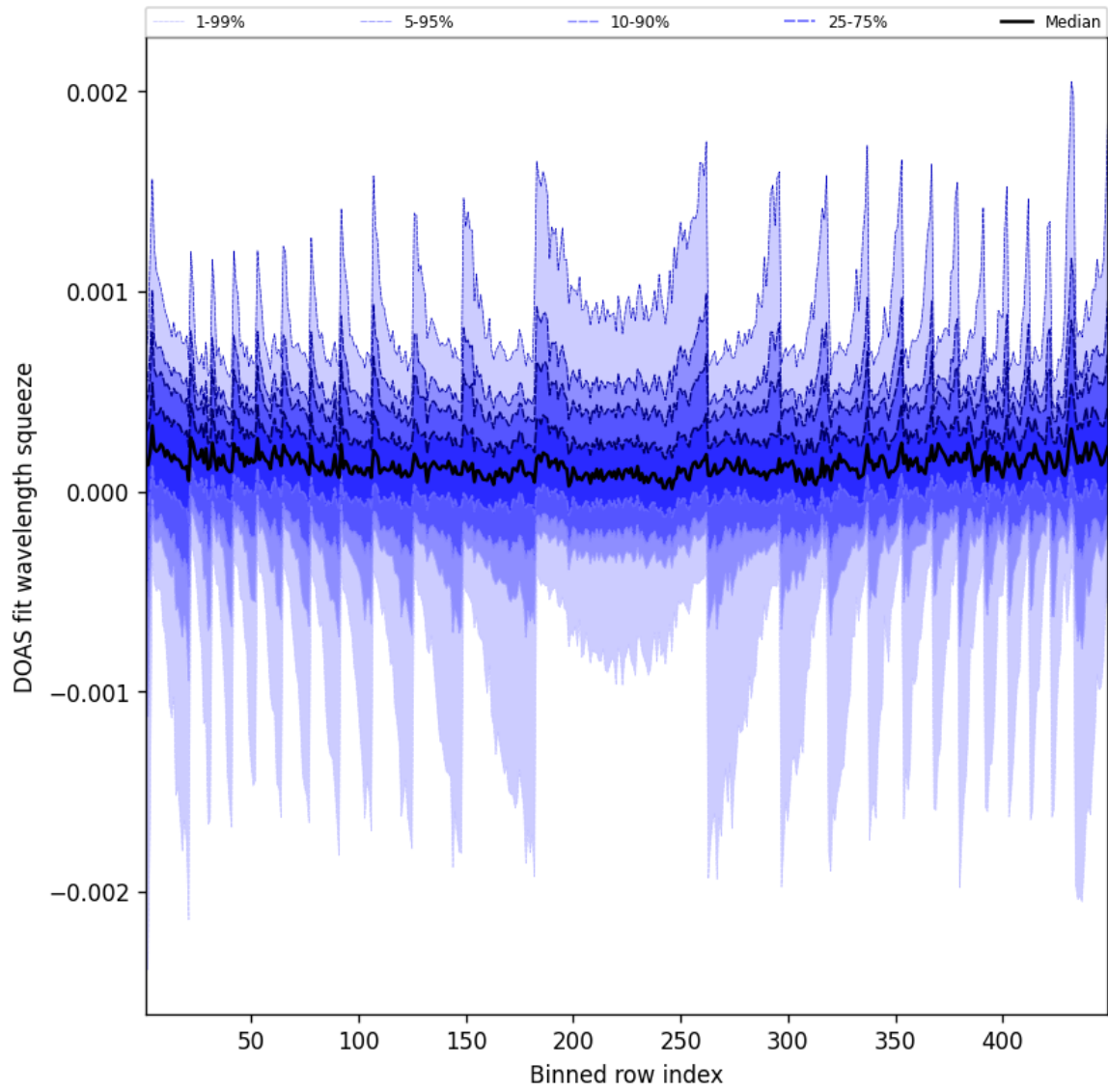
Figure 48: Along track statistics of “DOAS fit wavelength squeeze” for 2024-12-07 to 2024-12-08
