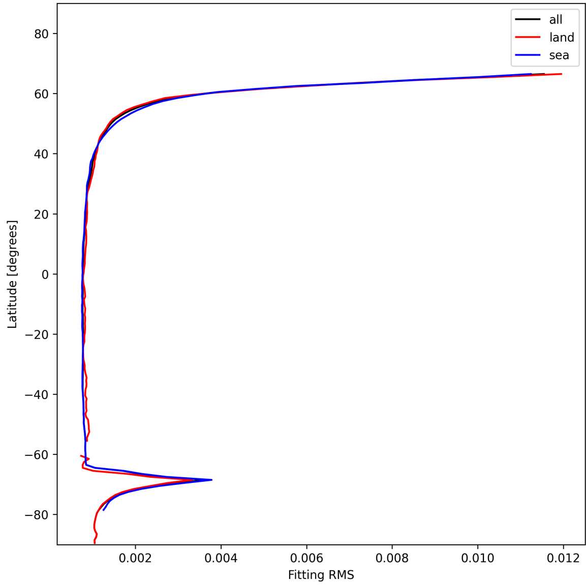
Figure 22: Zonal average of “Fitting RMS” for 2024-12-07 to 2024-12-08.
