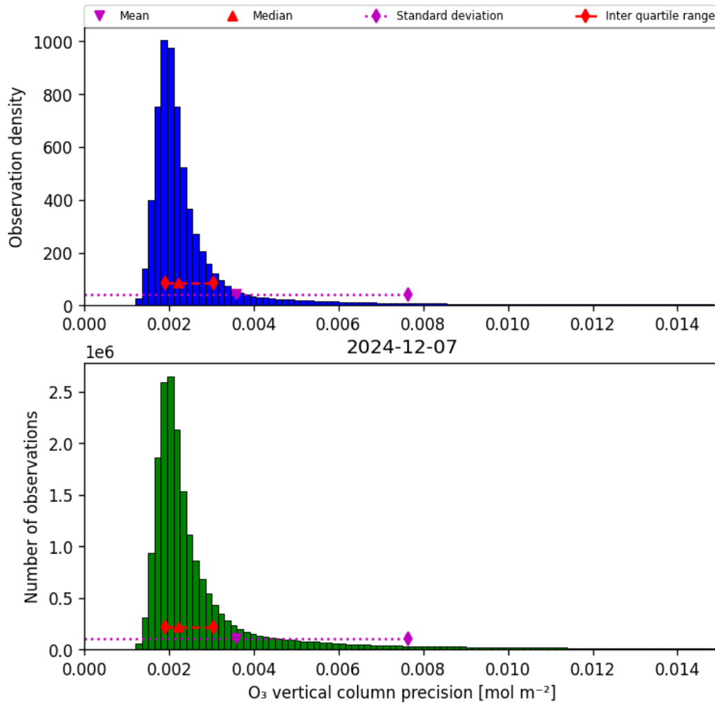
Figure 30: Histogram of “O 3 vertical column precision” for 2024-12-07 to 2024-12-08
