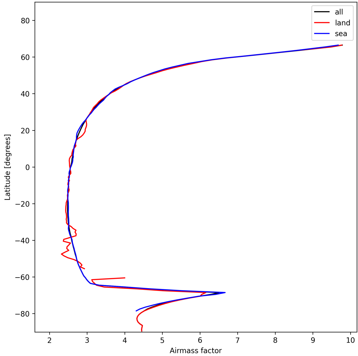
Figure 25: Zonal average of “Airmass factor” for 2024-12-07 to 2024-12-08.
