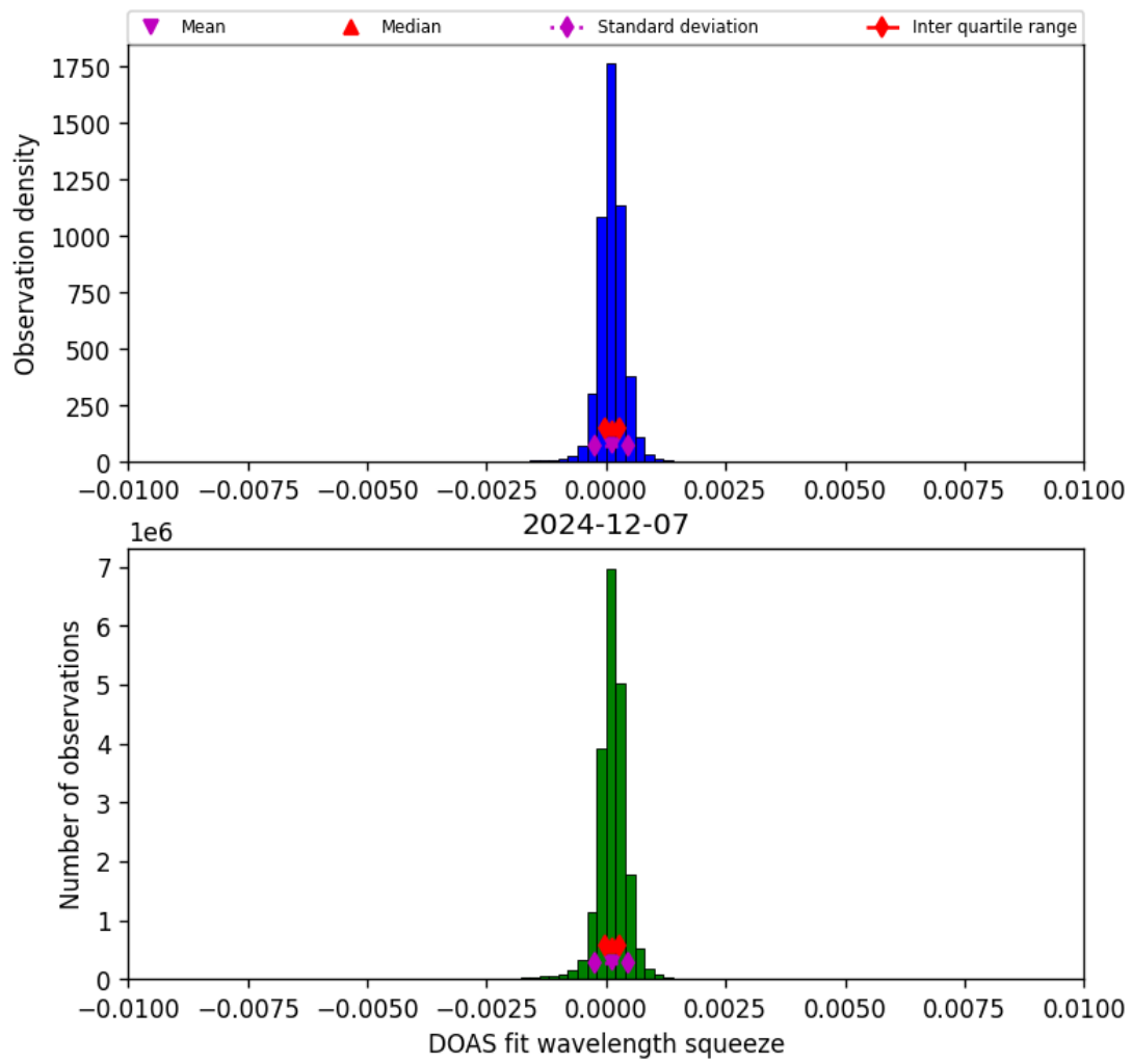
Figure 36: Histogram of “DOAS fit wavelength squeeze” for 2024-12-07 to 2024-12-08
