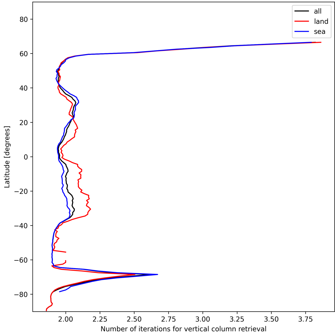
Figure 27: Zonal average of “Number of iterations for vertical column retrieval” for 2024-12-07 to 2024-12-08.
