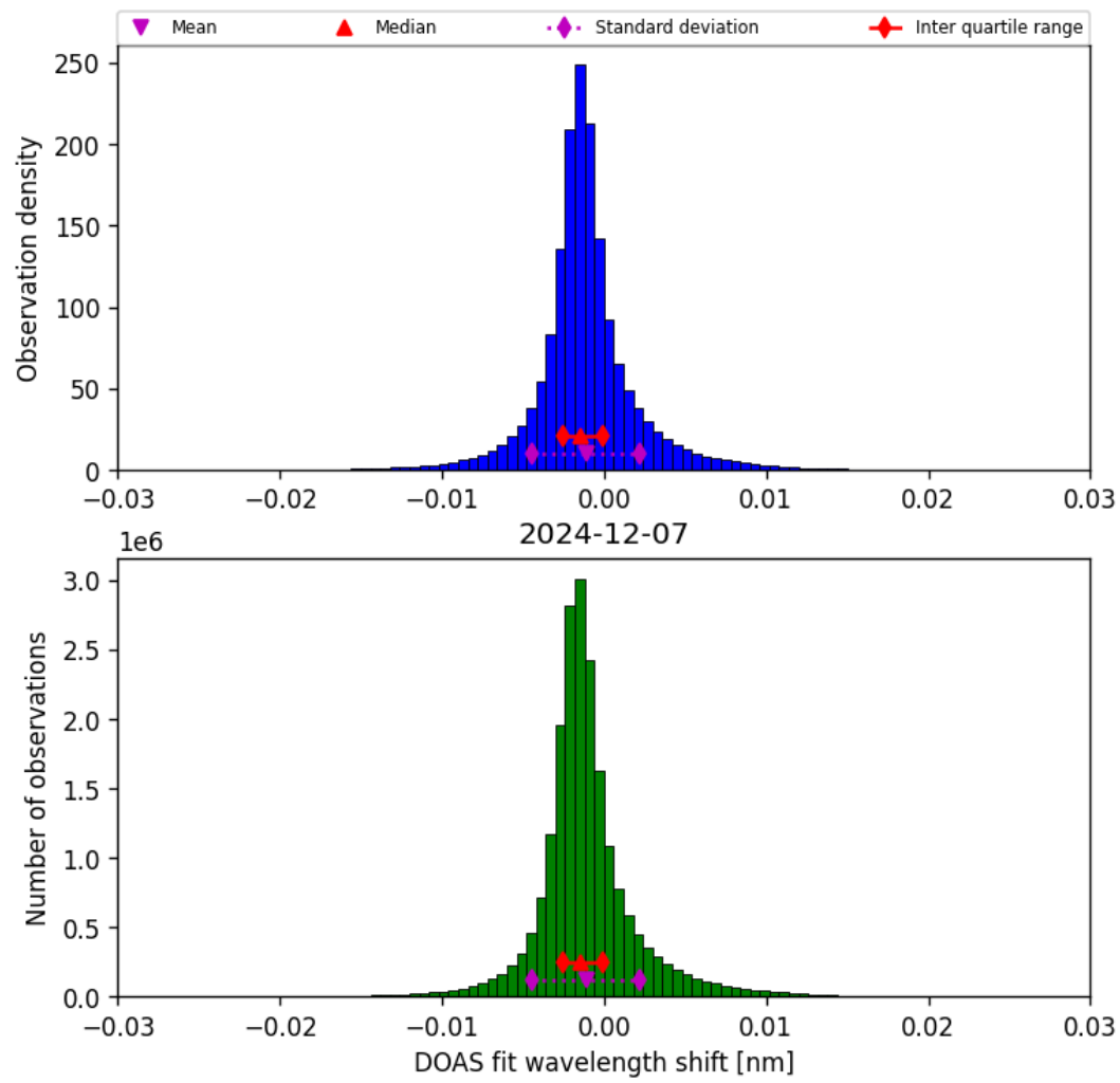
Figure 35: Histogram of “DOAS fit wavelength shift” for 2024-12-07 to 2024-12-08
