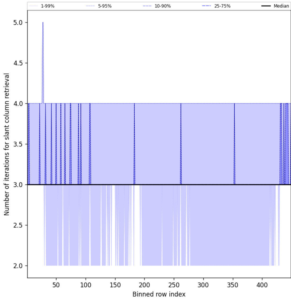
Figure 45: Along track statistics of “Number of iterations for slant column retrieval” for 2024-12-07 to 2024-12-08
