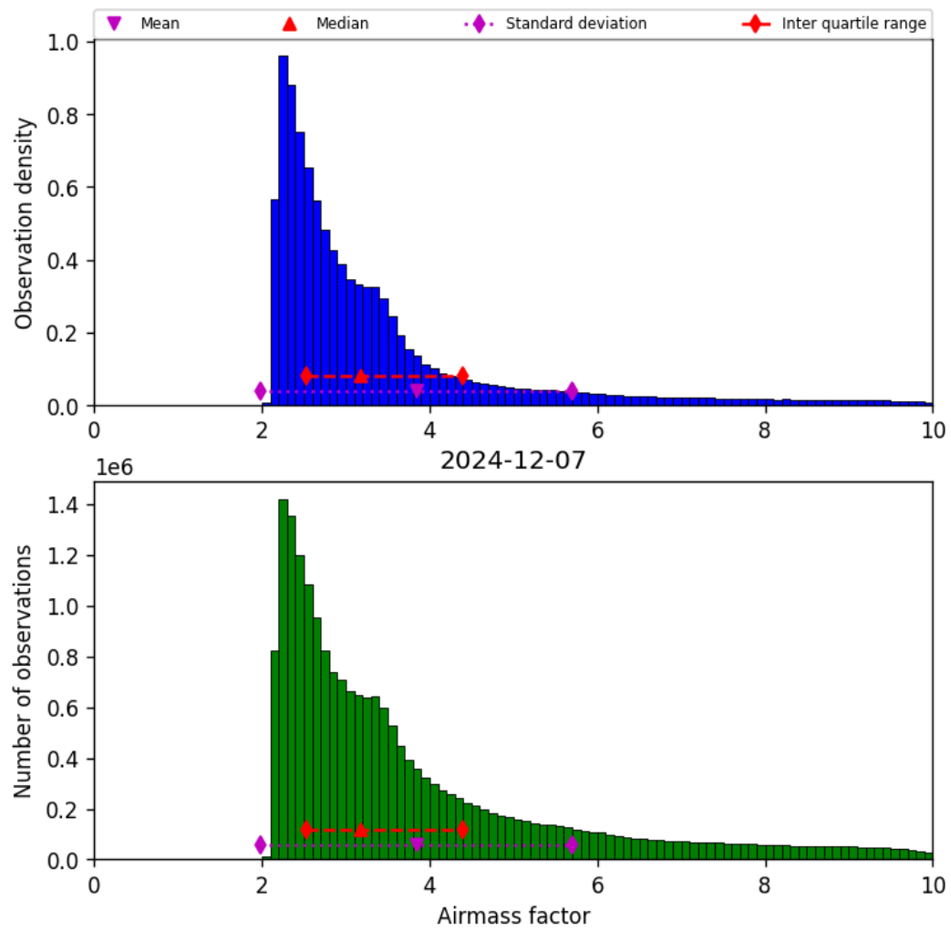
Figure 37: Histogram of “Airmass factor” for 2024-12-07 to 2024-12-08
