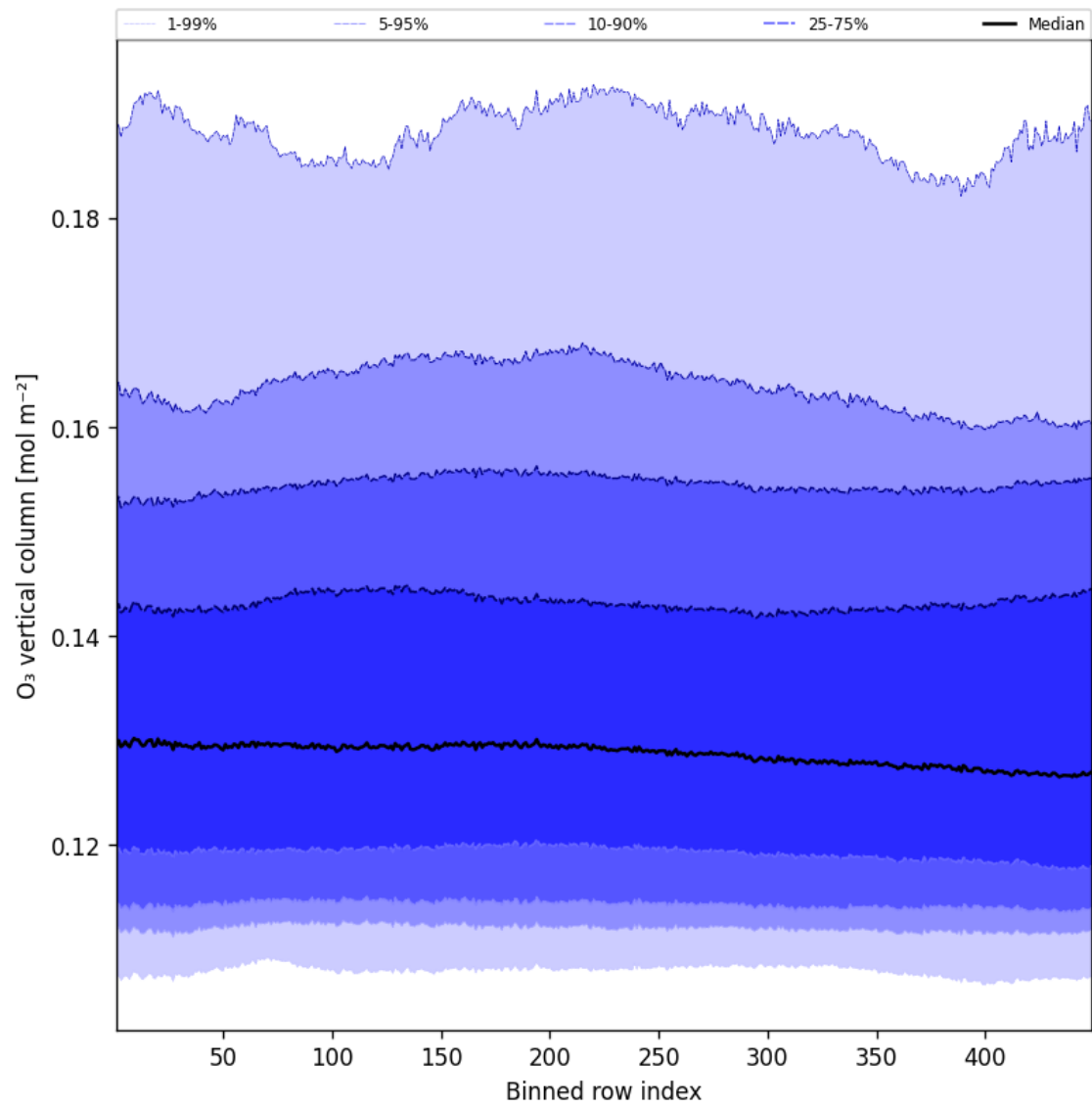
Figure 41: Along track statistics of “O 3 vertical column” for 2024-12-08 to 2024-12-09
