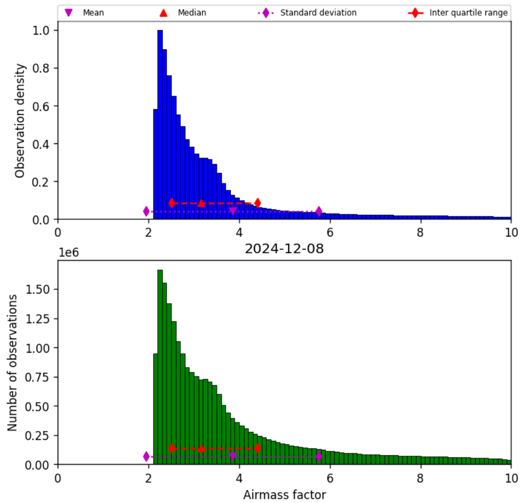
Figure 37: Histogram of “Airmass factor” for 2024-12-08 to 2024-12-09
