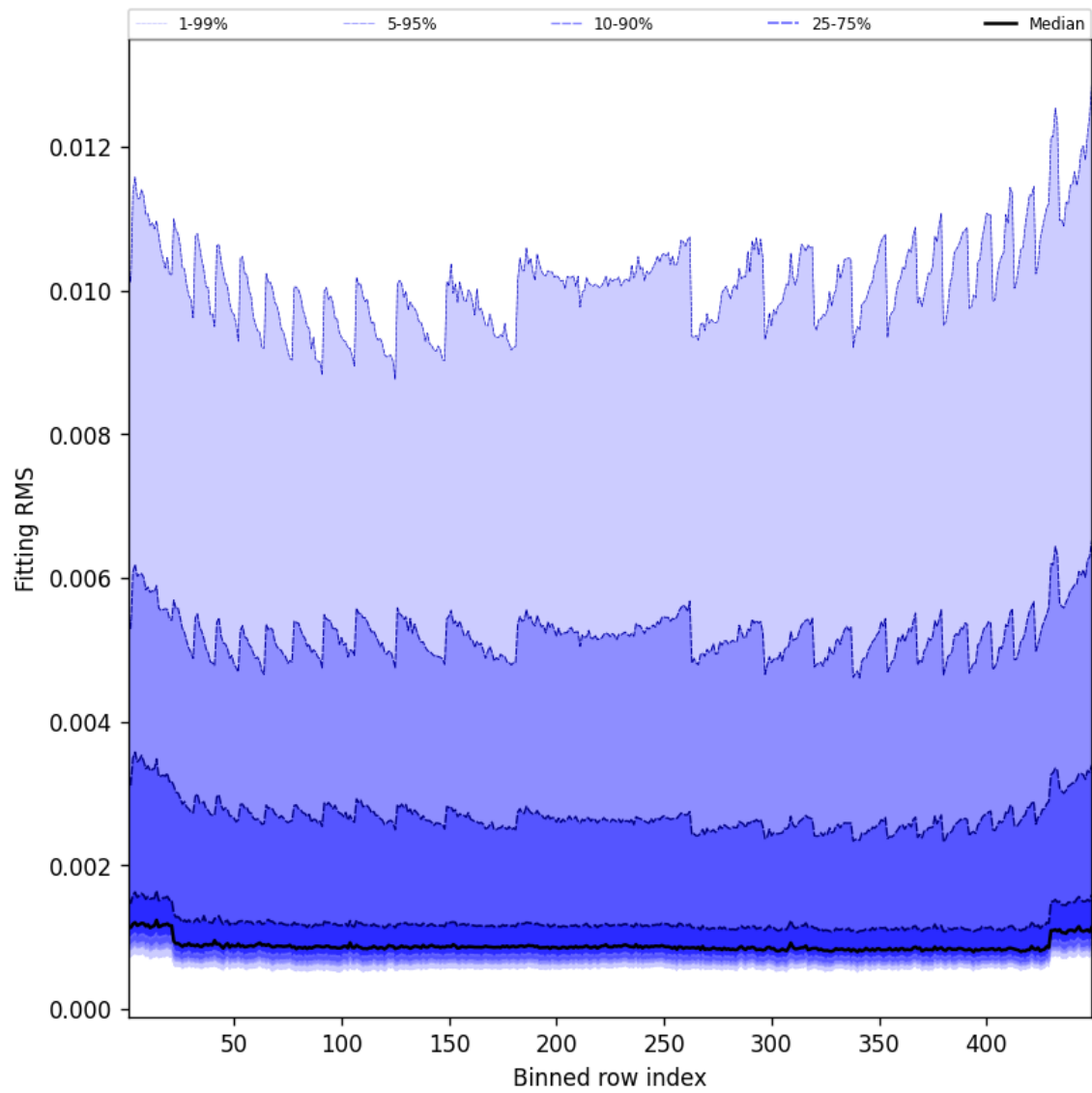
Figure 46: Along track statistics of “Fitting RMS” for 2024-12-08 to 2024-12-09
