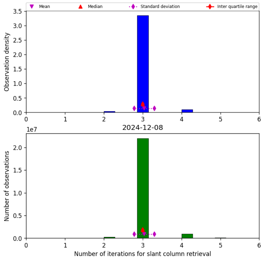
Figure 33: Histogram of “Number of iterations for slant column retrieval” for 2024-12-08 to 2024-12-09
