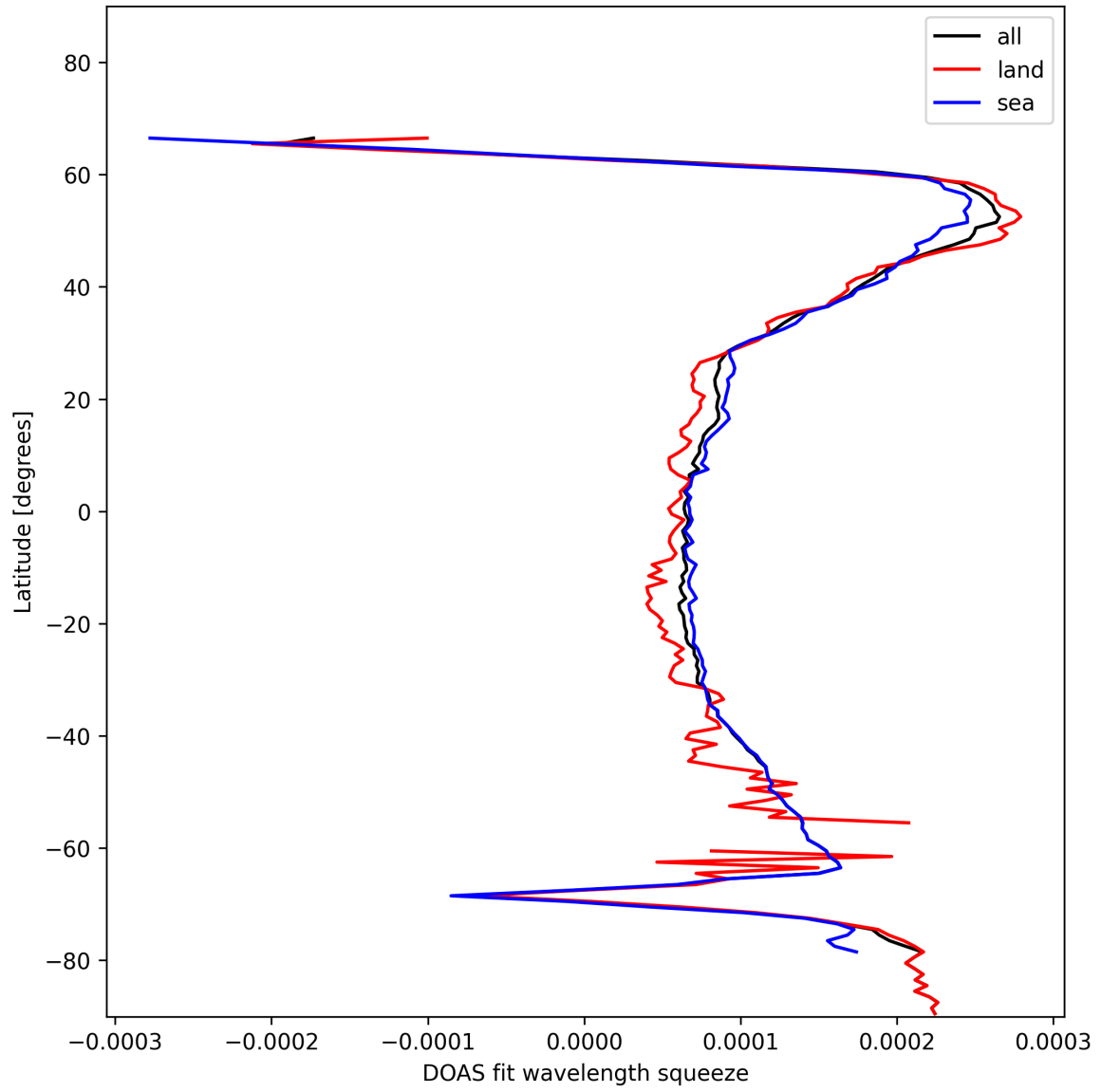
Figure 24: Zonal average of “DOAS fit wavelength squeeze” for 2024-12-08 to 2024-12-09.
