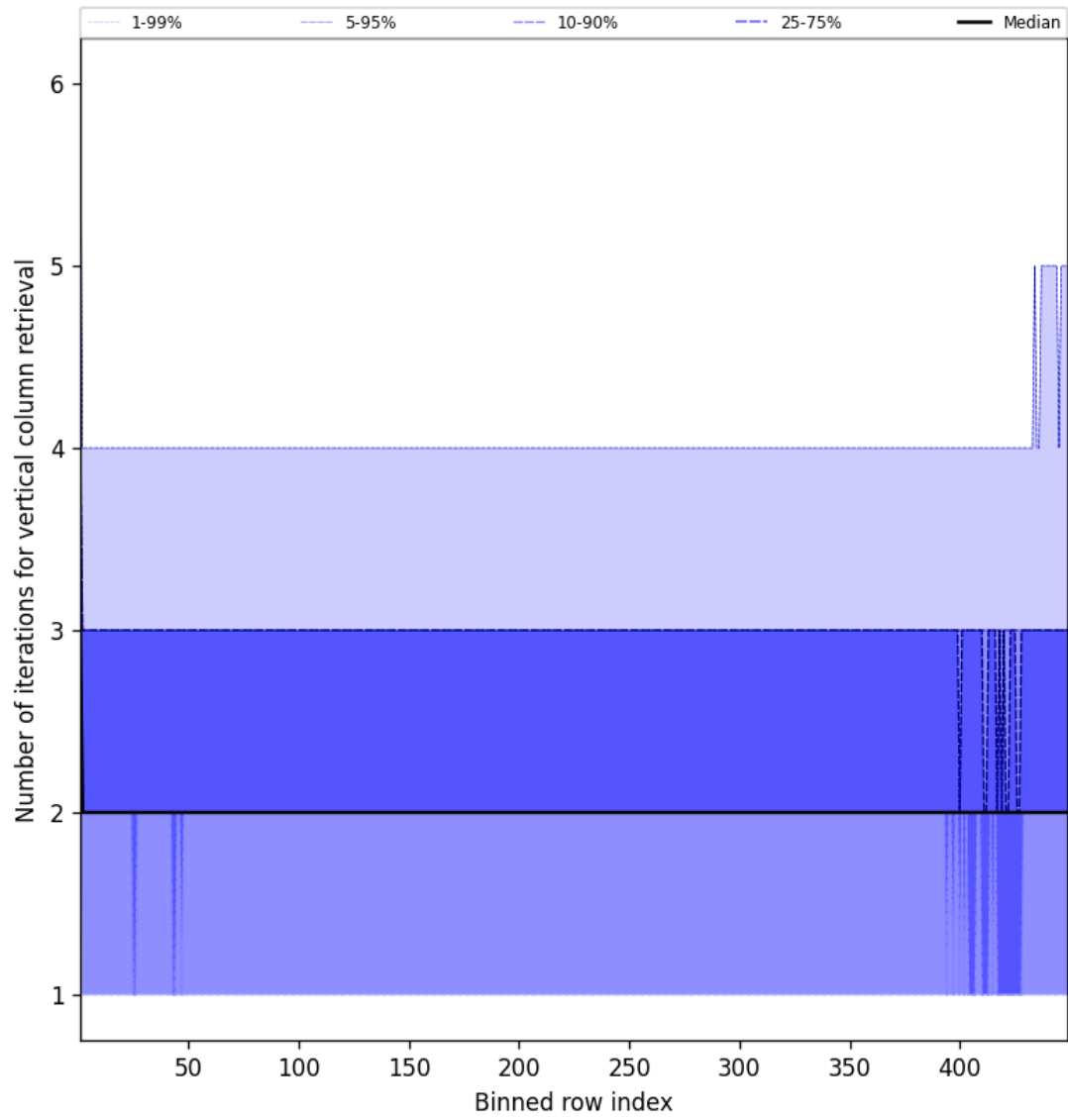
Figure 51: Along track statistics of “Number of iterations for vertical column retrieval” for 2024-12-08 to 2024-12-09
