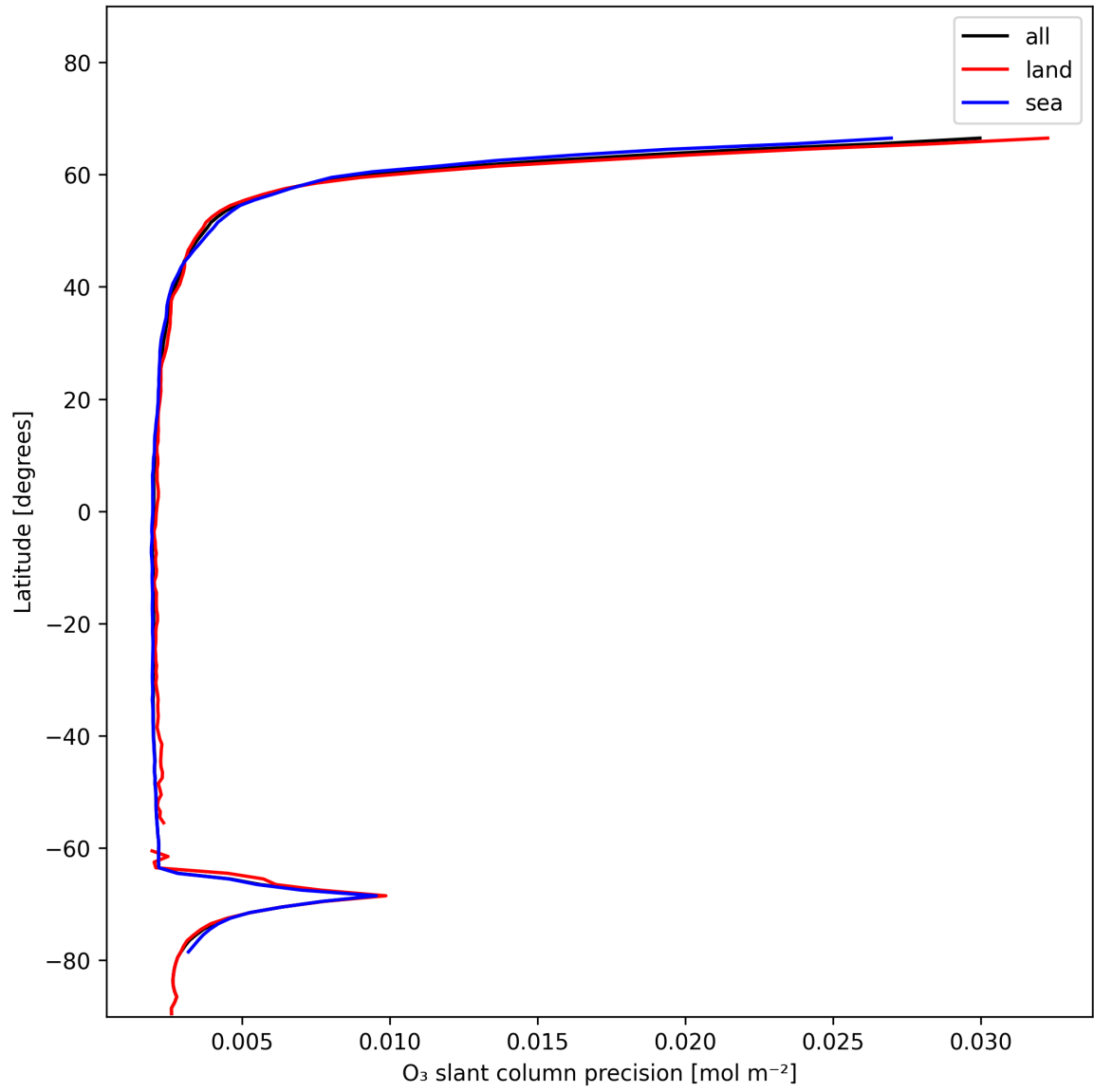
Figure 20: Zonal average of “O 3 slant column precision” for 2024-12-08 to 2024-12-09.
