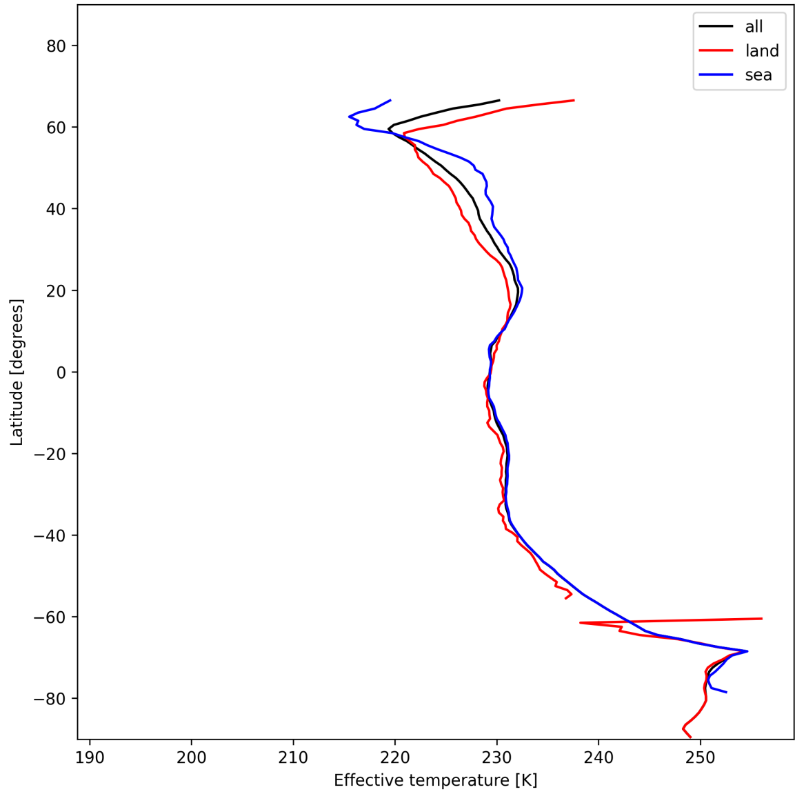
Figure 26: Zonal average of "Effective temperature" for 2024-12-08 to 2024-12-09.
