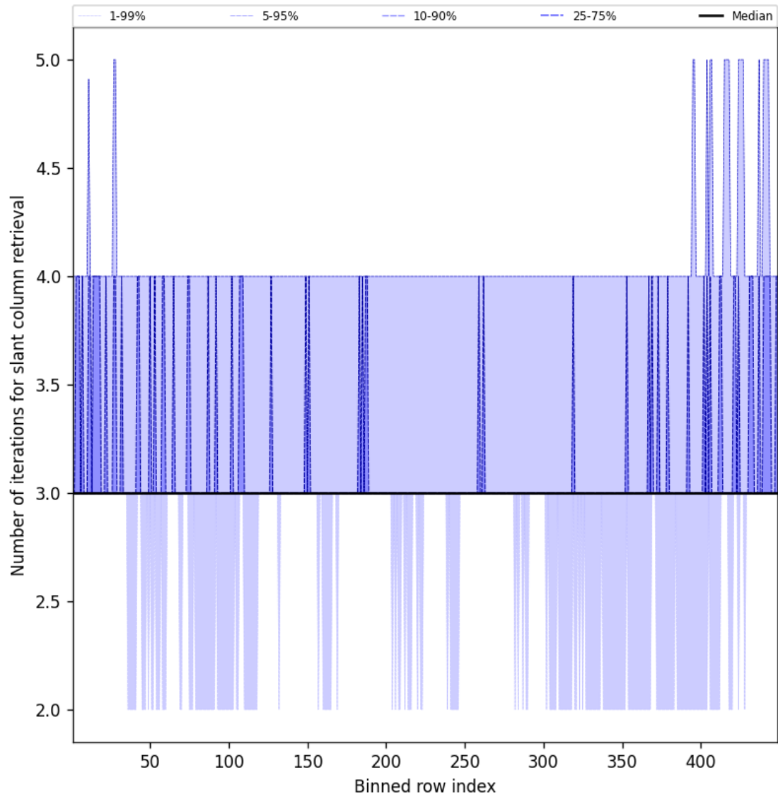
Figure 45: Along track statistics of “Number of iterations for slant column retrieval” for 2024-12-08 to 2024-12-09
