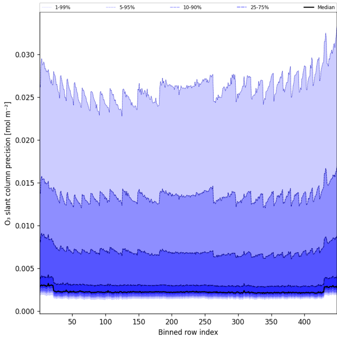
Figure 44: Along track statistics of “O 3 slant column precision” for 2024-12-08 to 2024-12-09
