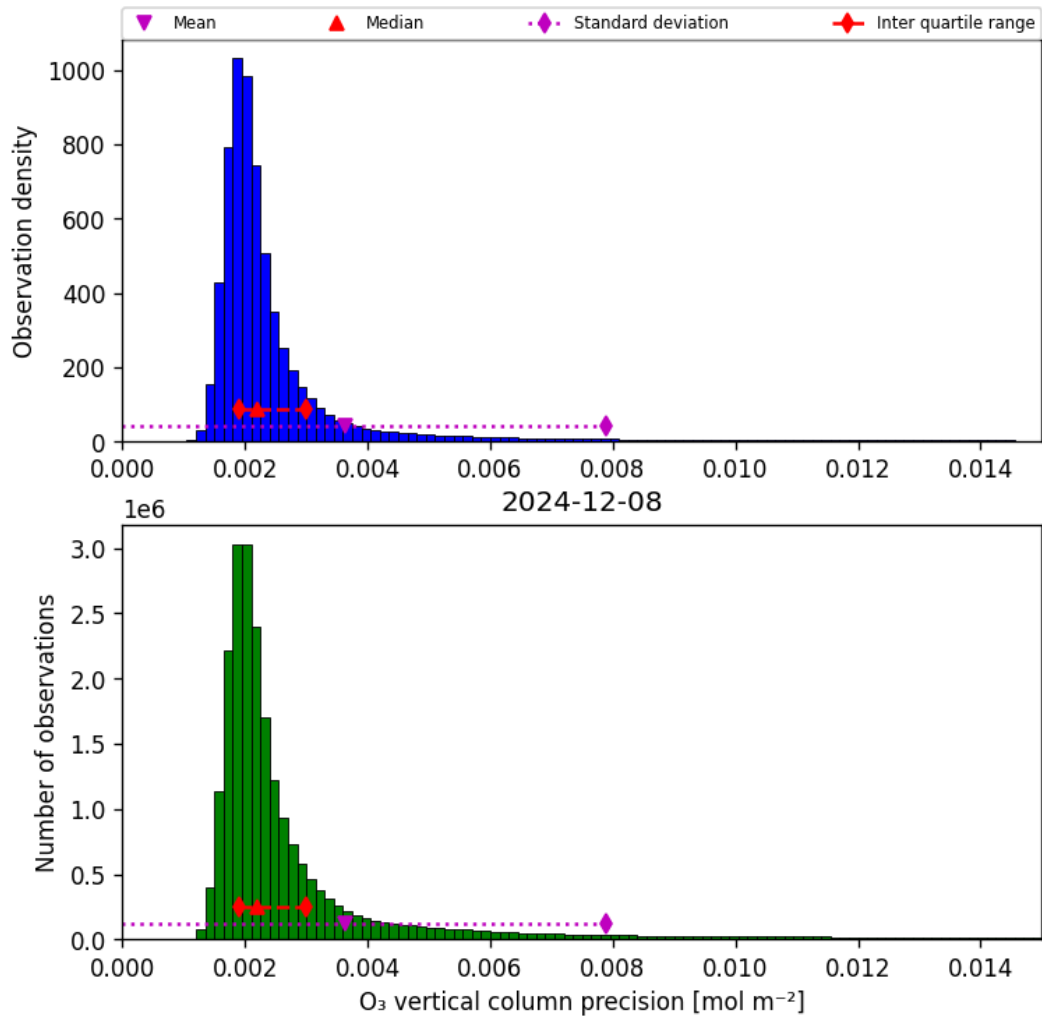
Figure 30: Histogram of “O 3 vertical column precision” for 2024-12-08 to 2024-12-09
