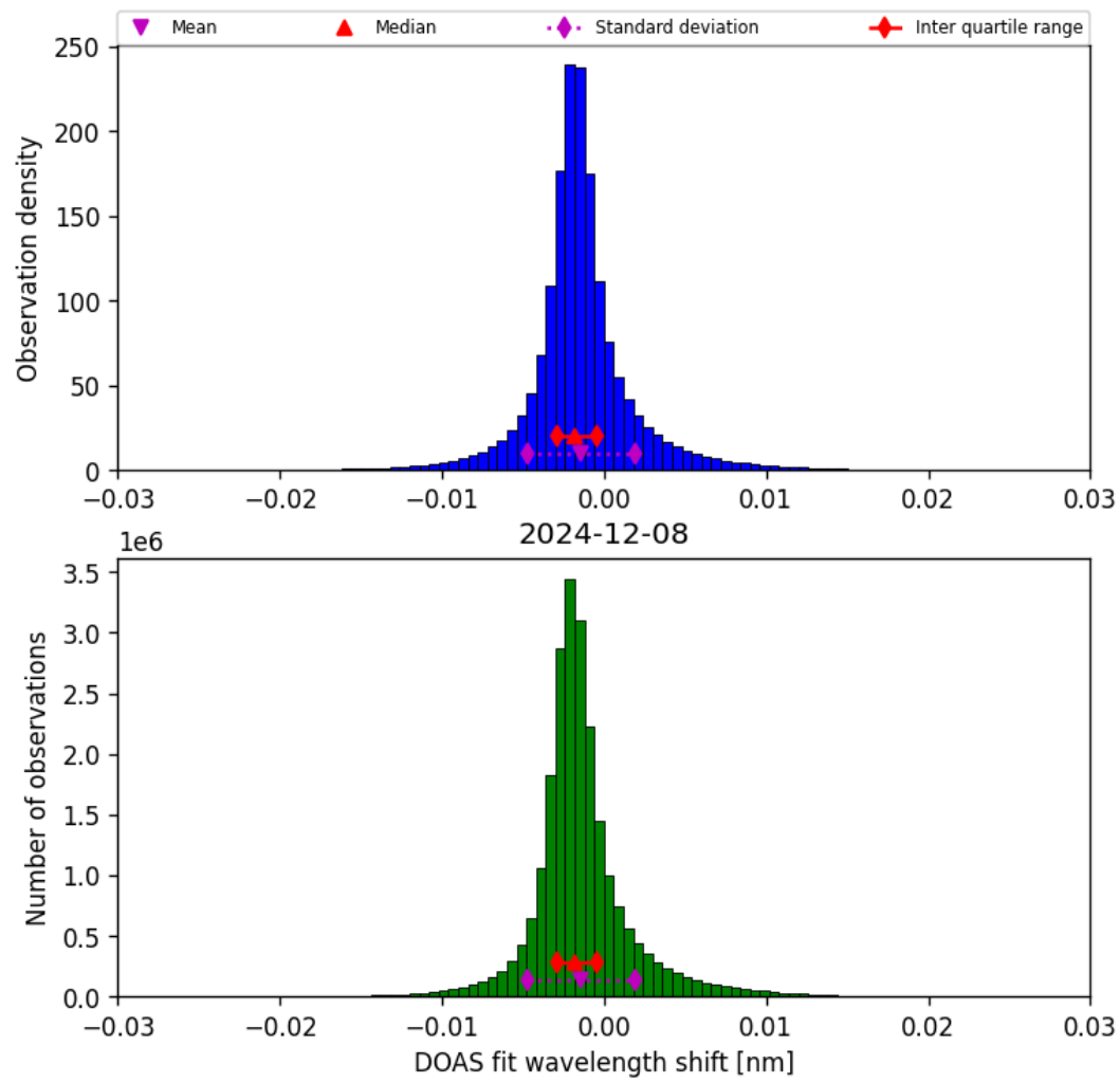
Figure 35: Histogram of “DOAS fit wavelength shift” for 2024-12-08 to 2024-12-09
