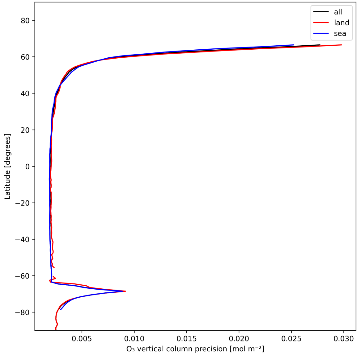
Figure 18: Zonal average of "O 3 vertical column precision" for 2024-12-08 to 2024-12-09.
