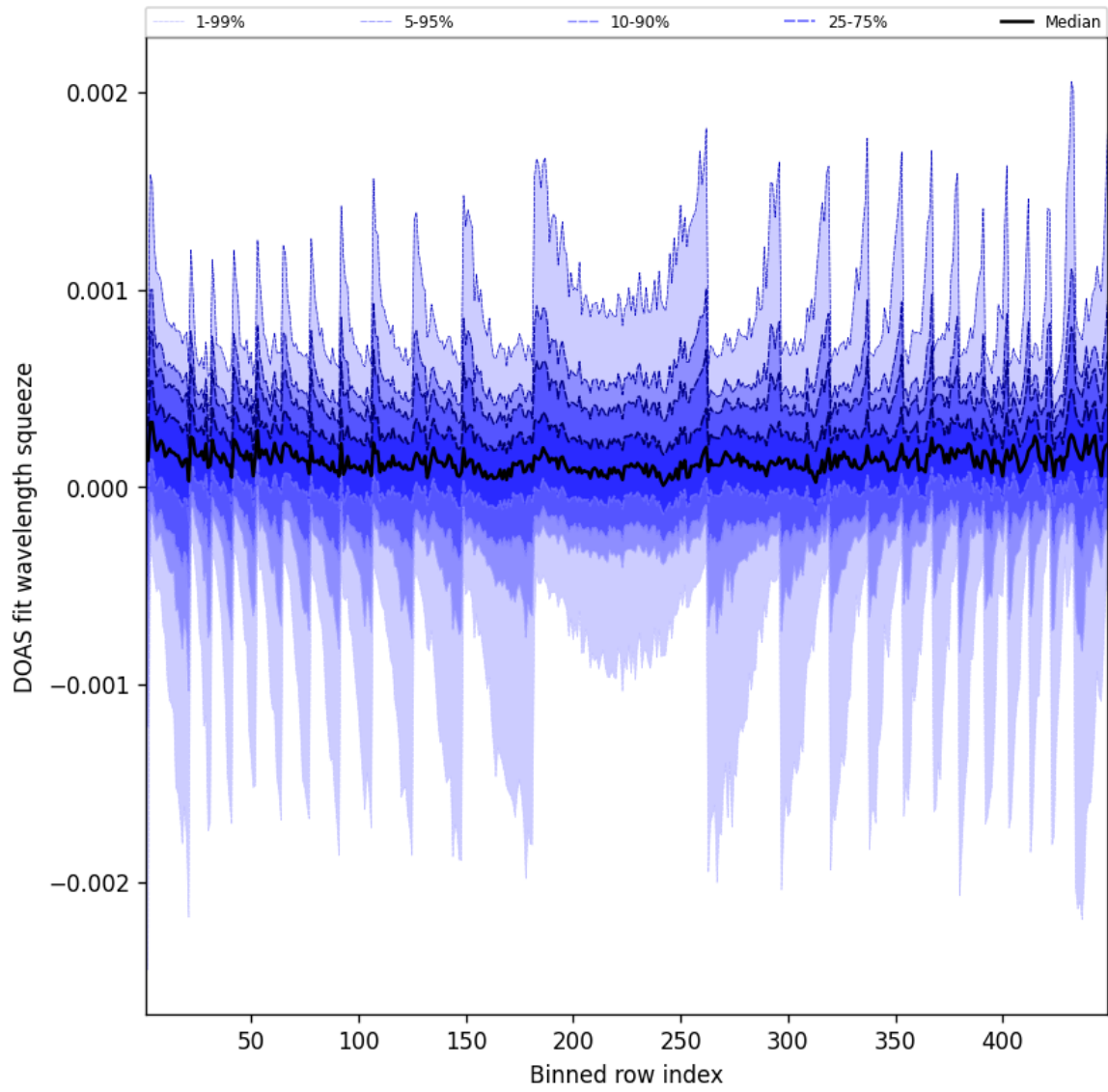
Figure 48: Along track statistics of “DOAS fit wavelength squeeze” for 2024-12-08 to 2024-12-09
