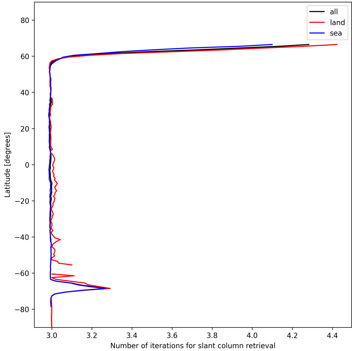
Figure 21: Zonal average of “Number of iterations for slant column retrieval” for 2024-12-08 to 2024-12-09.
