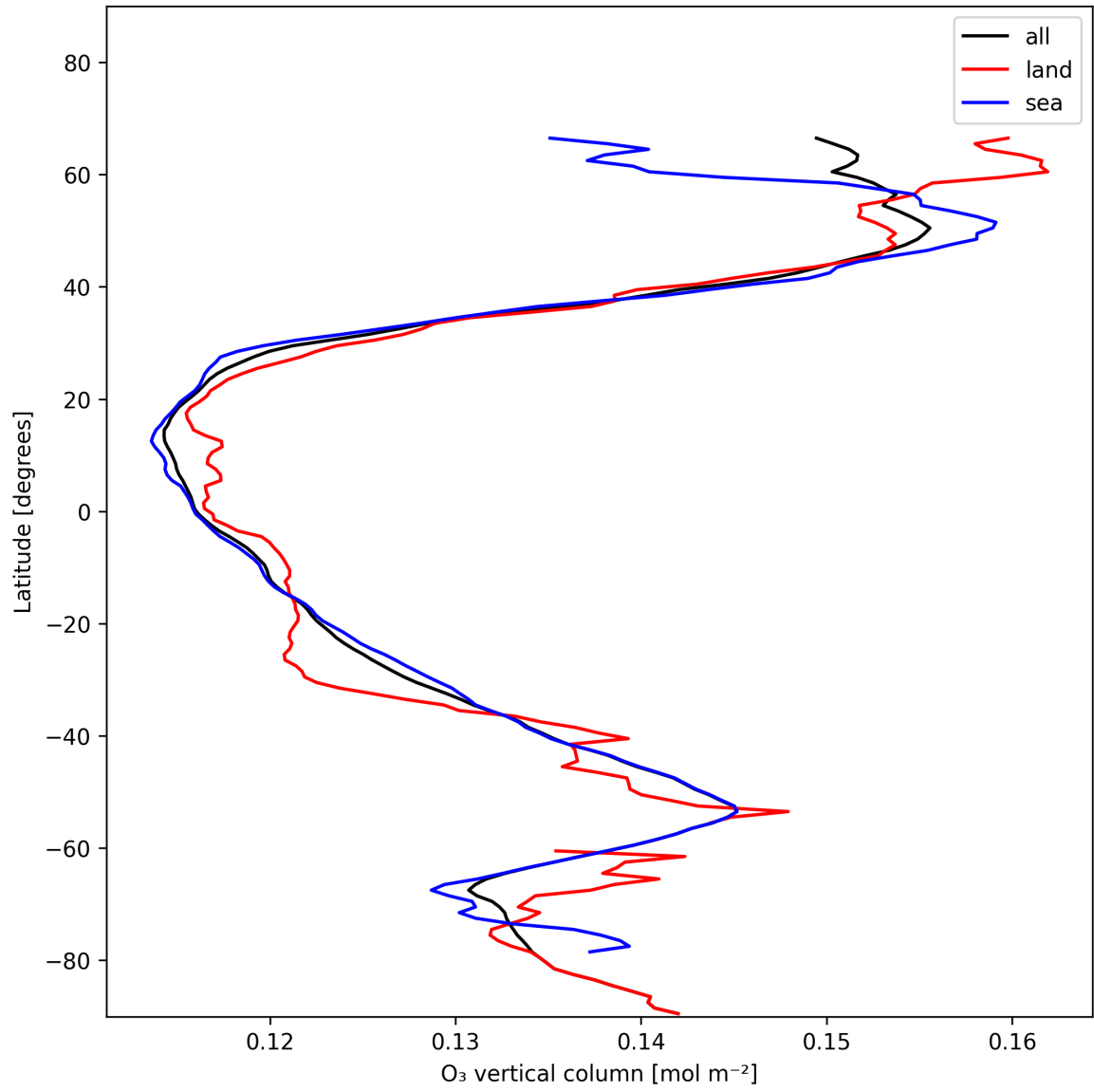
Figure 17: Zonal average of “O 3 vertical column” for 2024-12-08 to 2024-12-09.
