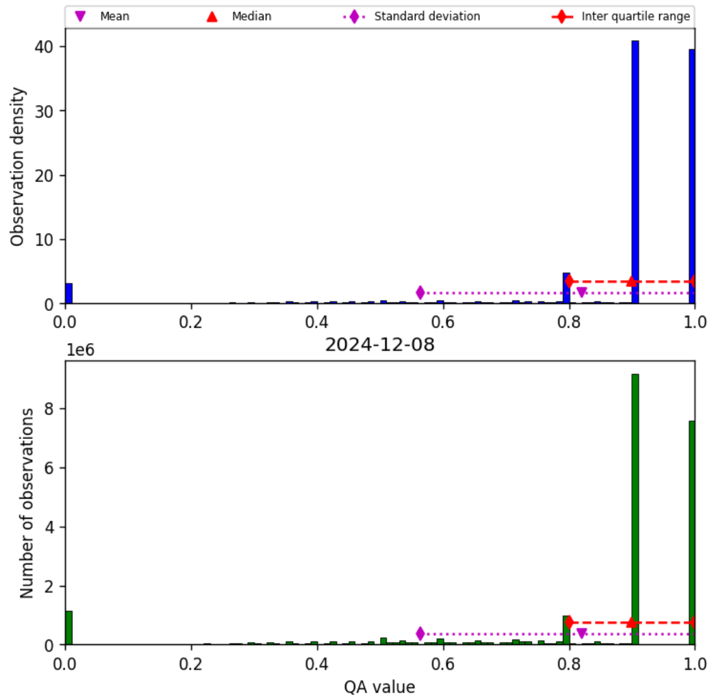
Figure 28: Histogram of “QA value” for 2024-12-08 to 2024-12-09
