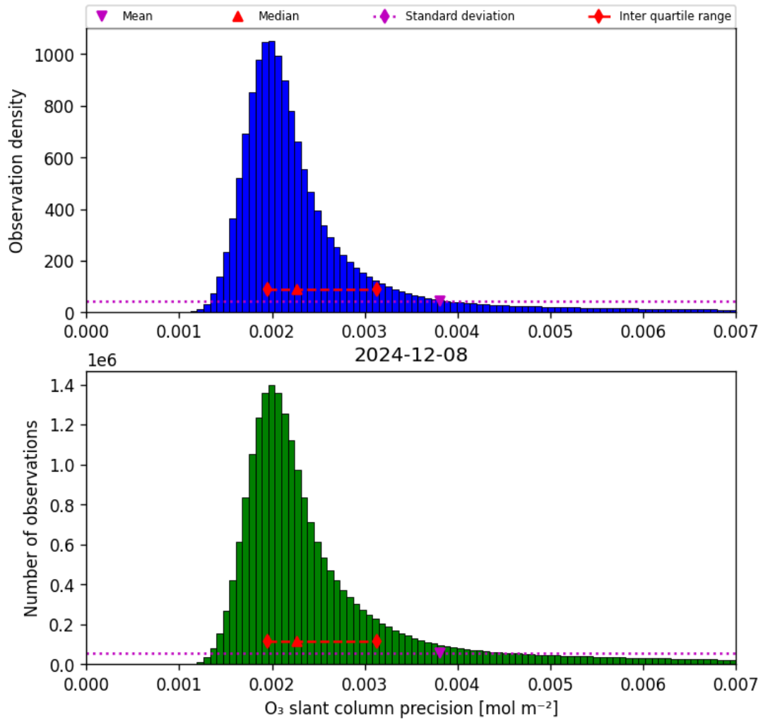
Figure 32: Histogram of “O 3 slant column precision” for 2024-12-08 to 2024-12-09
