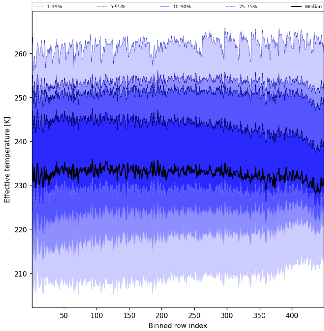
Figure 50: Along track statistics of “Effective temperature” for 2024-12-08 to 2024-12-09
