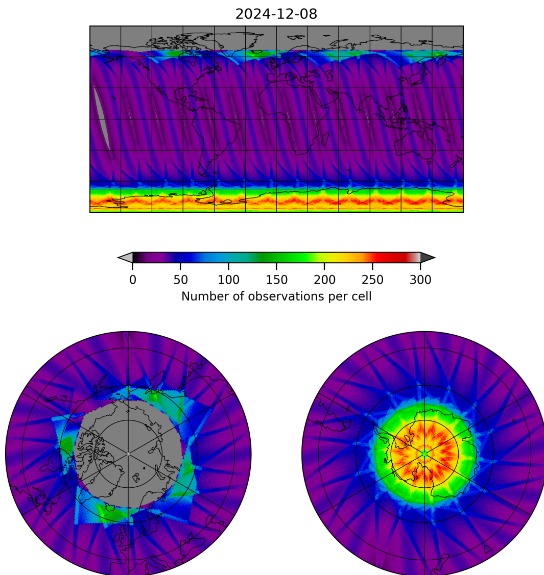
Figure 15: Map of the number of observations for 2024-12-08 to 2024-12-09
