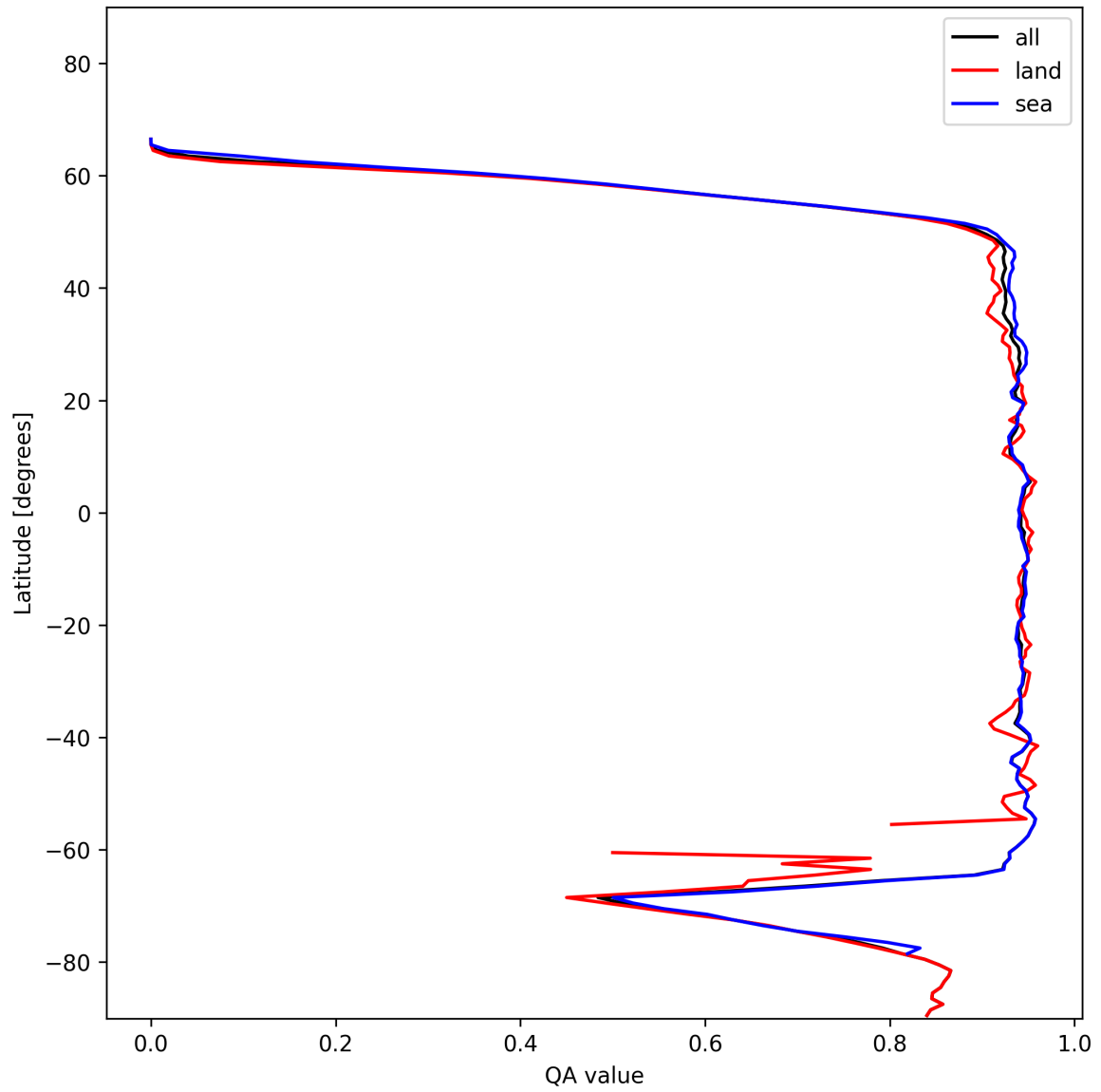
Figure 16: Zonal average of “QA value” for 2024-12-08 to 2024-12-09.
