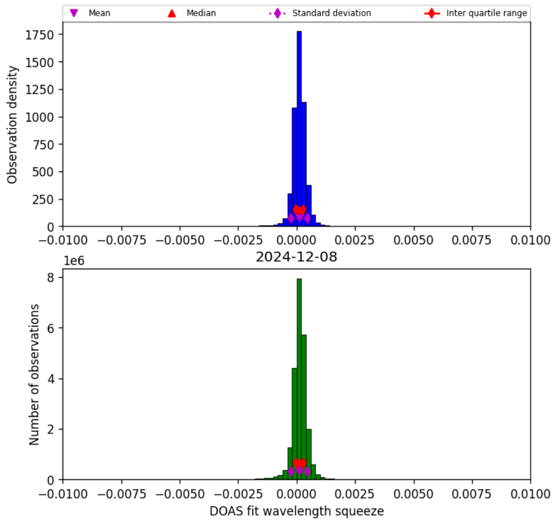
Figure 36: Histogram of “DOAS fit wavelength squeeze” for 2024-12-08 to 2024-12-09
