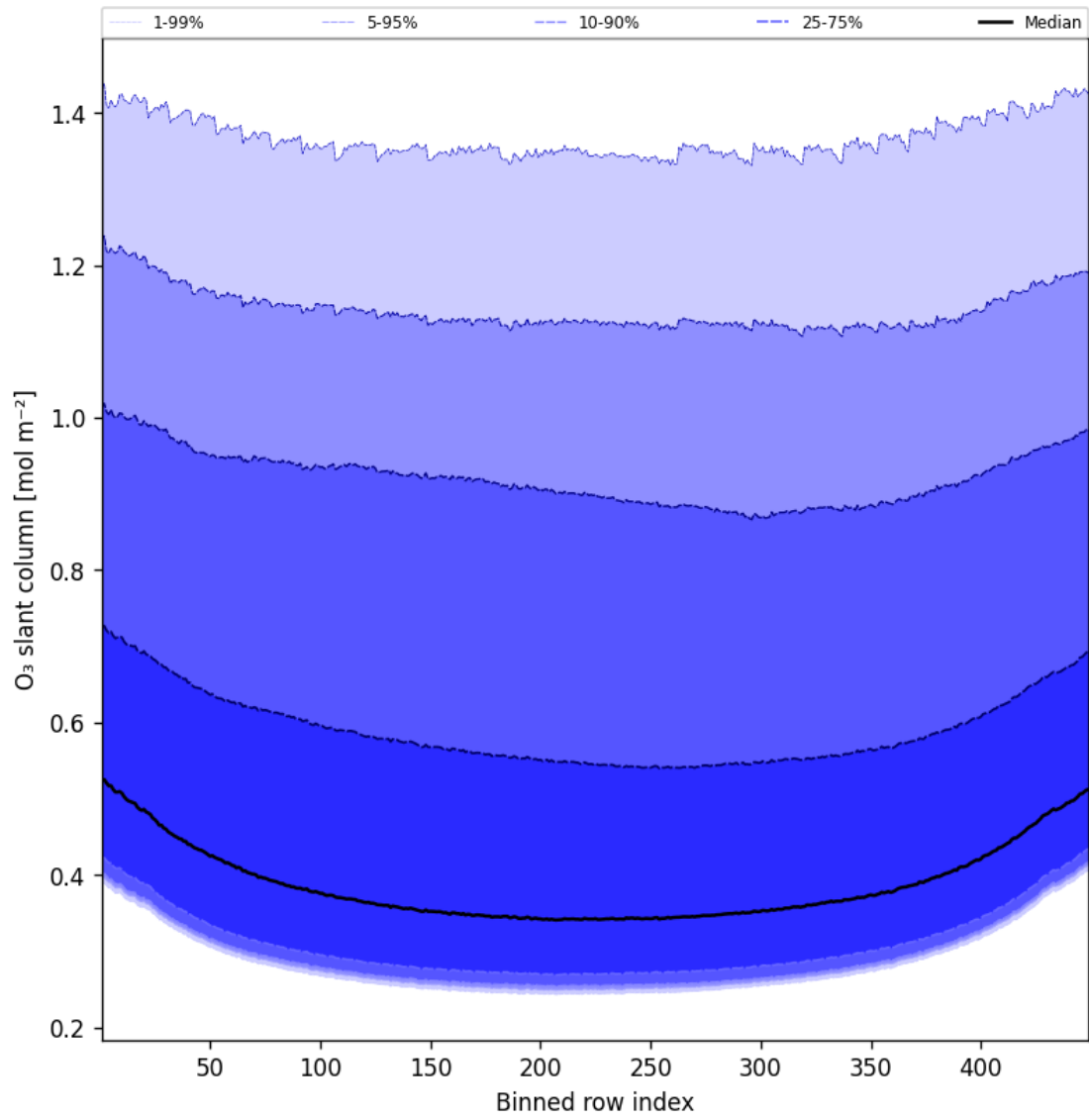
Figure 43: Along track statistics of “O 3 slant column” for 2024-12-08 to 2024-12-09
