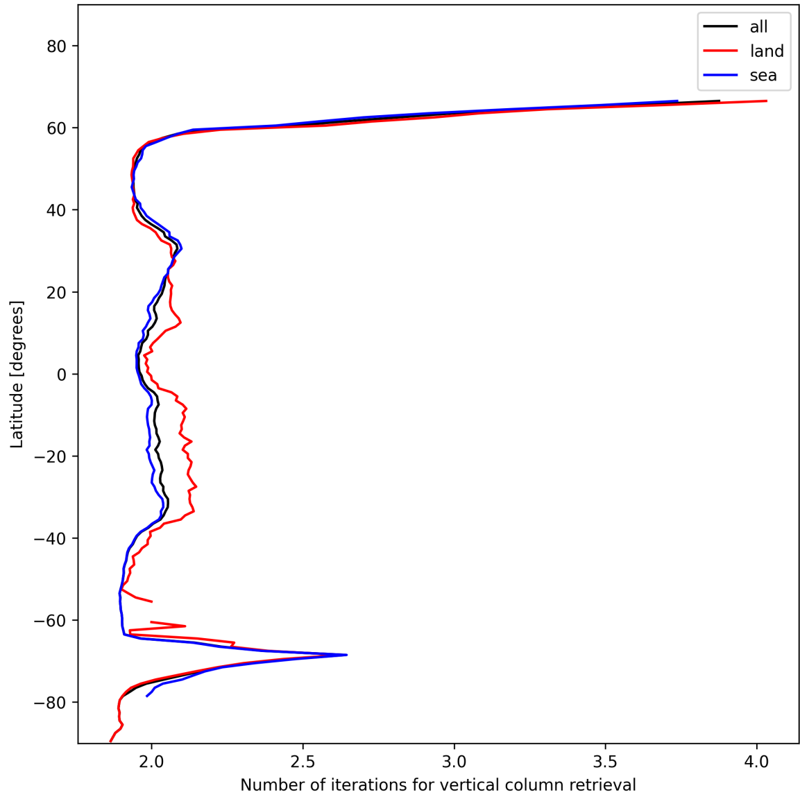
Figure 27: Zonal average of “Number of iterations for vertical column retrieval” for 2024-12-08 to 2024-12-09.
