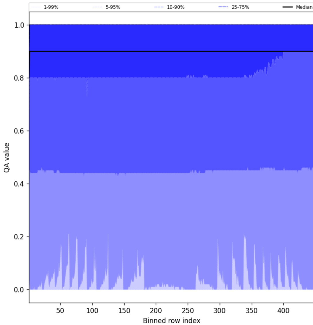
Figure 40: Along track statistics of “QA value” for 2024-12-08 to 2024-12-09
