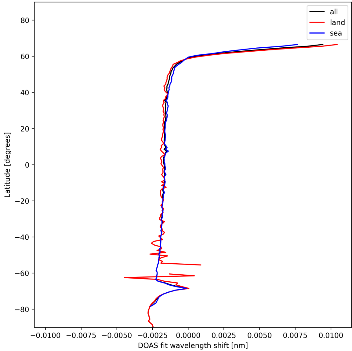
Figure 23: Zonal average of “DOAS fit wavelength shift” for 2024-12-08 to 2024-12-09.
