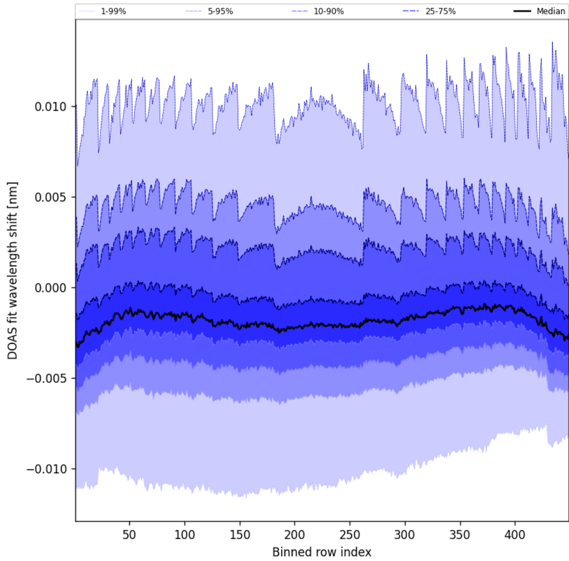
Figure 47: Along track statistics of “DOAS fit wavelength shift” for 2024-12-08 to 2024-12-09
