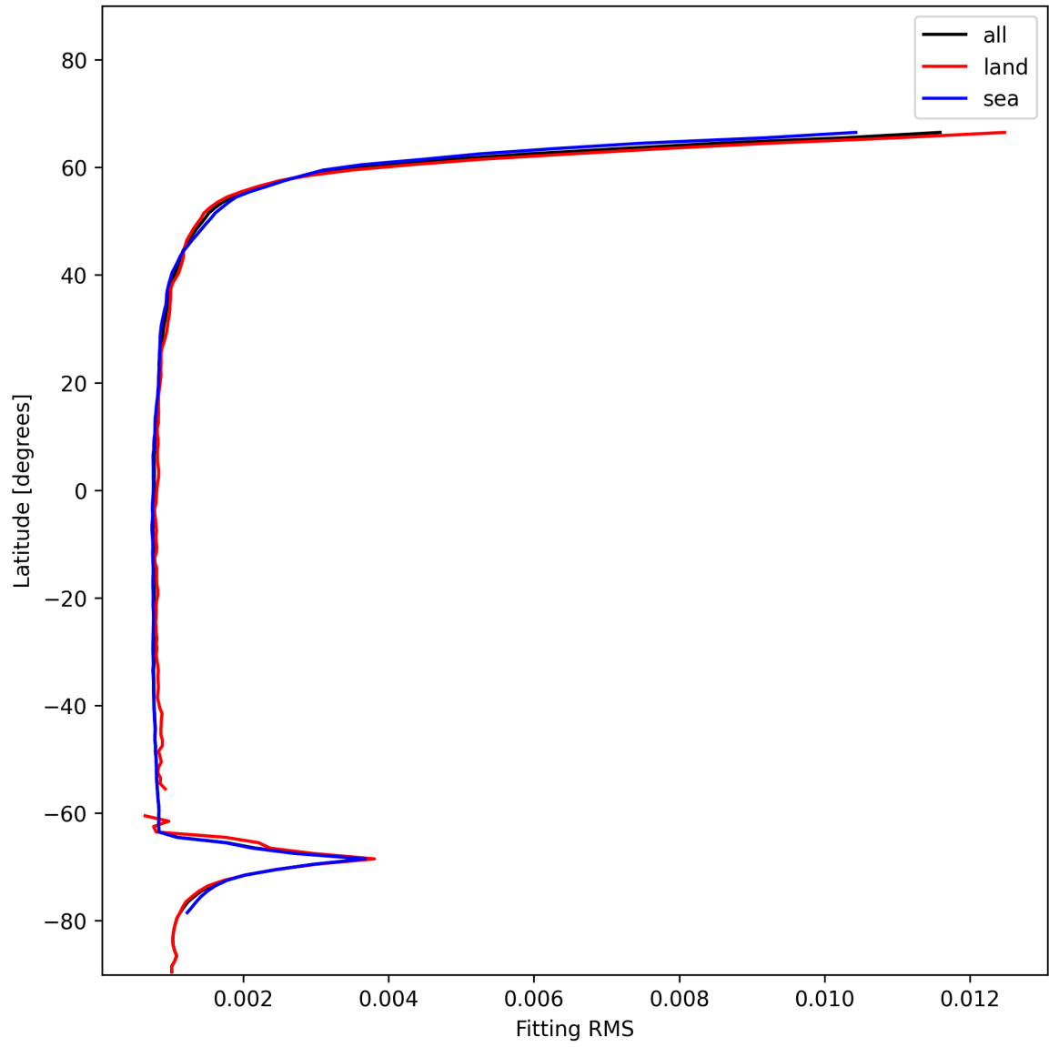
Figure 22: Zonal average of “Fitting RMS” for 2024-12-08 to 2024-12-09.
