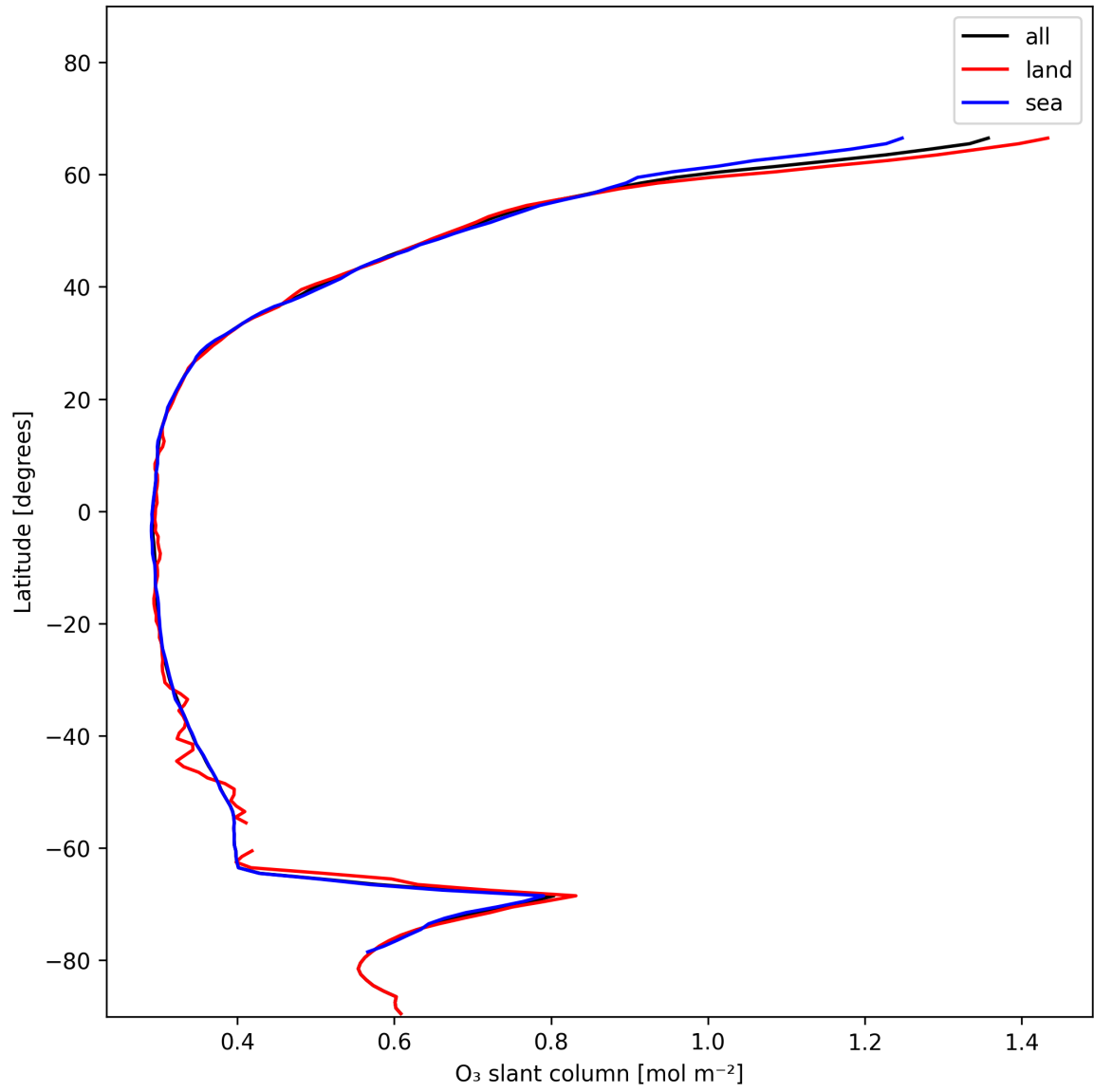
Figure 19: Zonal average of “O 3 slant column” for 2024-12-08 to 2024-12-09.
