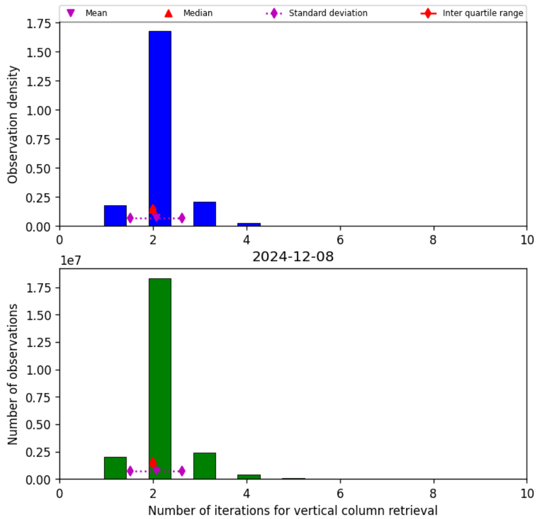
Figure 39: Histogram of “Number of iterations for vertical column retrieval” for 2024-12-08 to 2024-12-09
