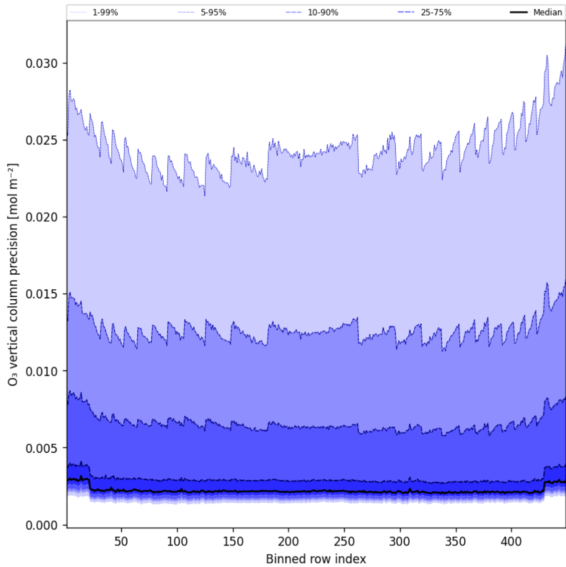
Figure 42: Along track statistics of “O 3 vertical column precision” for 2024-12-08 to 2024-12-09
