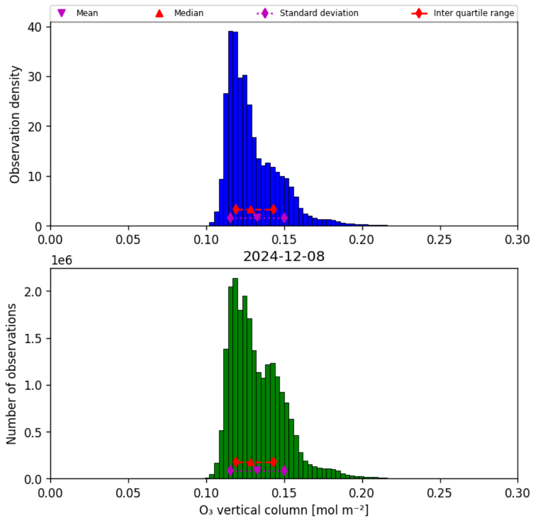
Figure 29: Histogram of “O 3 vertical column” for 2024-12-08 to 2024-12-09
