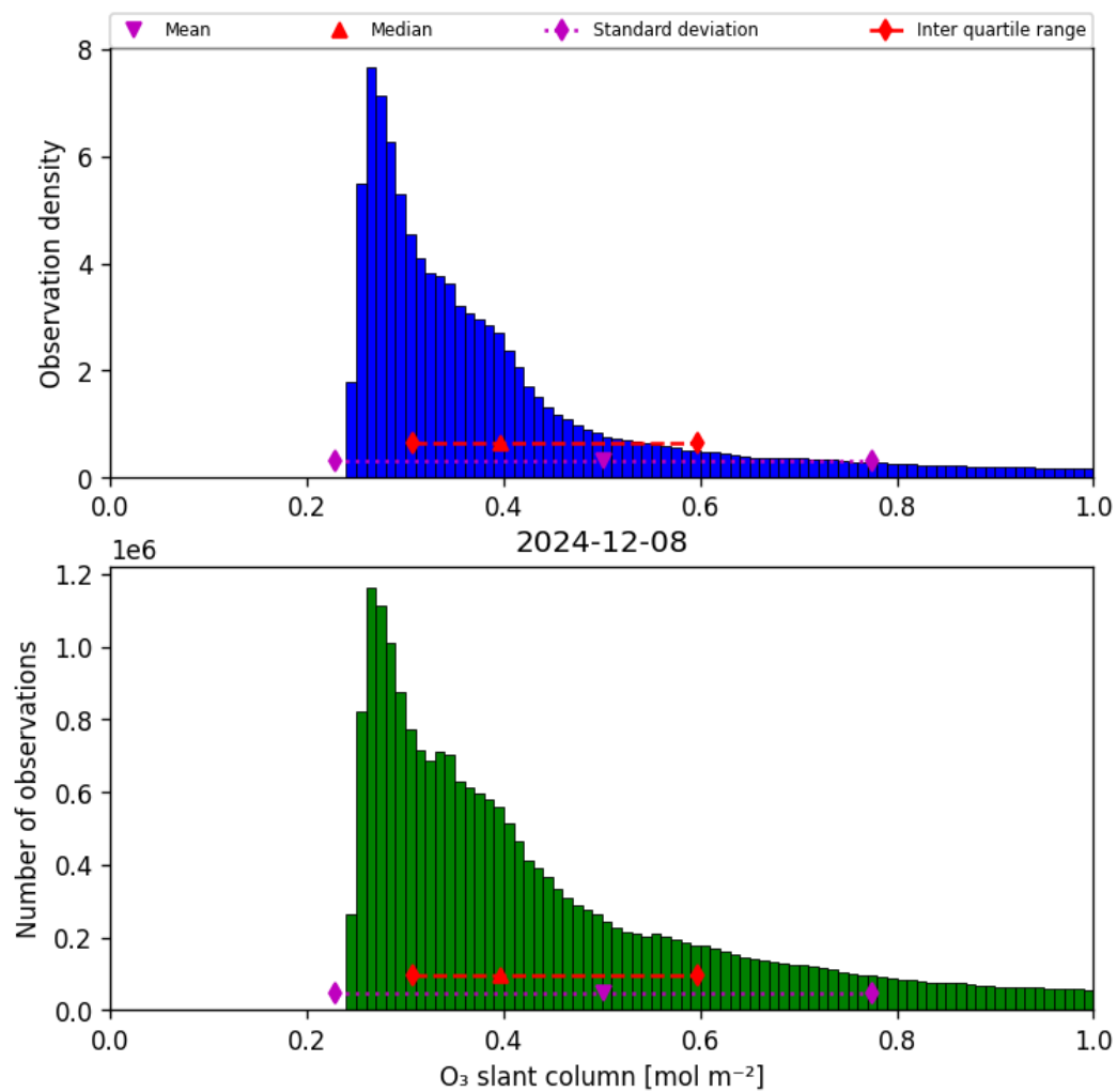
Figure 31: Histogram of “O 3 slant column” for 2024-12-08 to 2024-12-09
