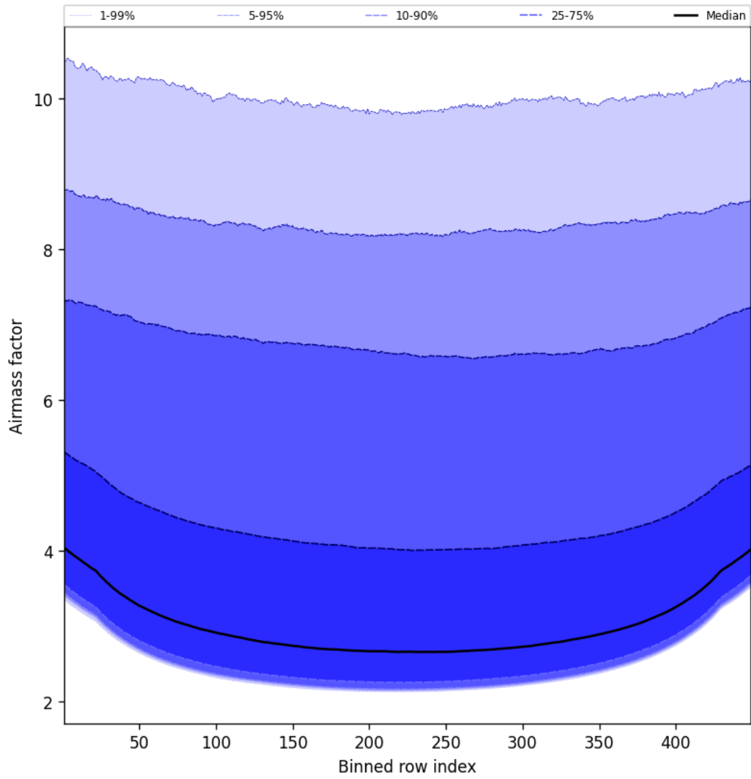
Figure 49: Along track statistics of “Airmass factor” for 2024-12-08 to 2024-12-09
