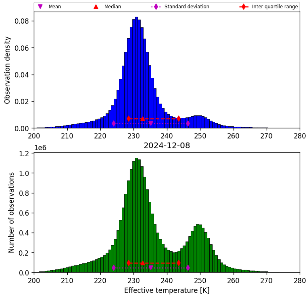
Figure 38: Histogram of “Effective temperature” for 2024-12-08 to 2024-12-09
