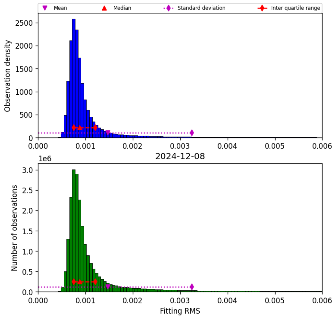
Figure 34: Histogram of “Fitting RMS” for 2024-12-08 to 2024-12-09
