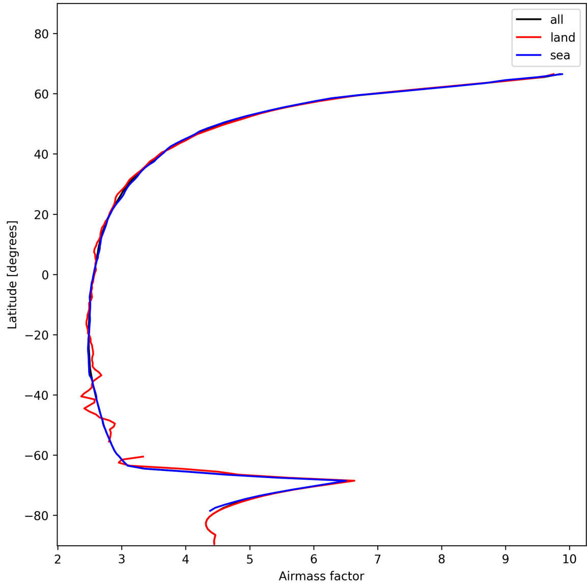
Figure 25: Zonal average of “Airmass factor” for 2024-12-08 to 2024-12-09.
