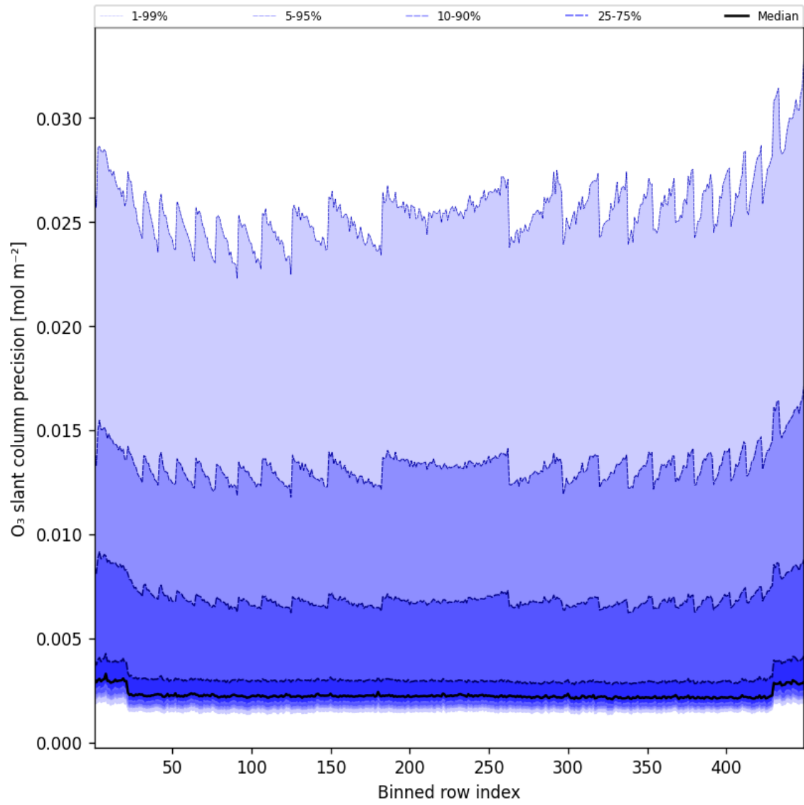
Figure 44: Along track statistics of “O 3 slant column precision” for 2024-12-09 to 2024-12-09
