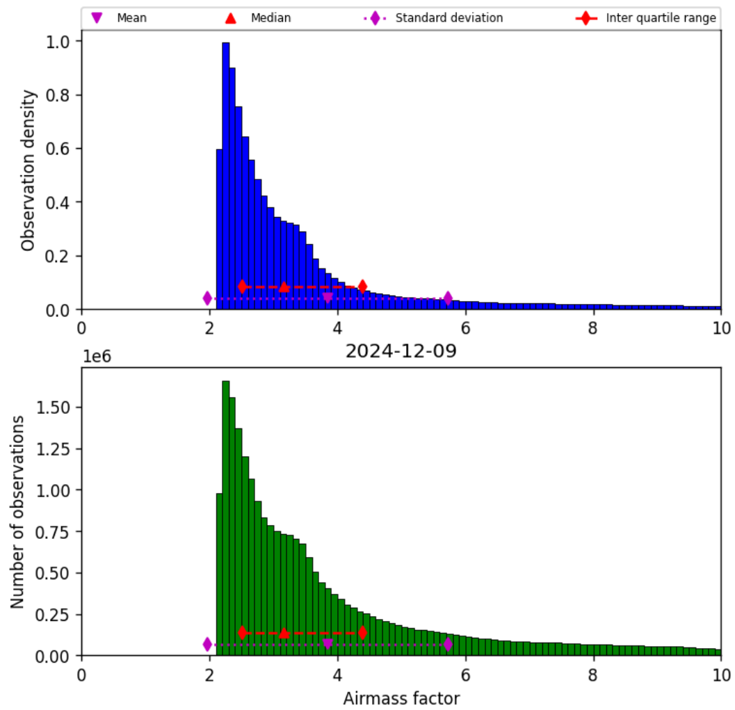
Figure 37: Histogram of “Airmass factor” for 2024-12-09 to 2024-12-09
