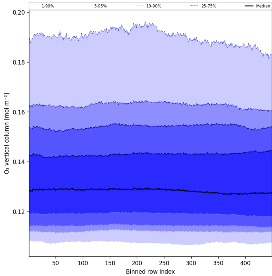
Figure 41: Along track statistics of “O 3 vertical column” for 2024-12-09 to 2024-12-09
