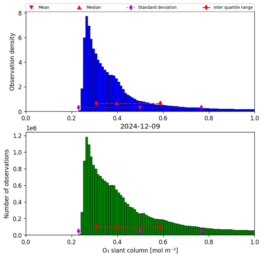
Figure 31: Histogram of “O 3 slant column” for 2024-12-09 to 2024-12-09
