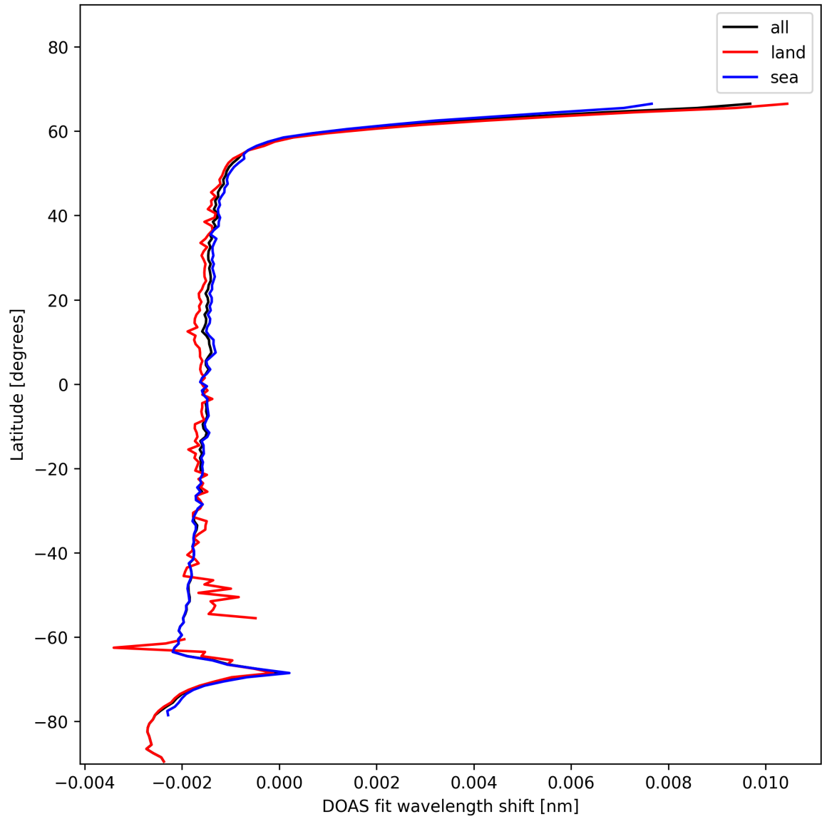
Figure 23: Zonal average of “DOAS fit wavelength shift” for 2024-12-09 to 2024-12-09.
