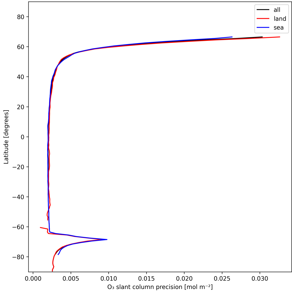
Figure 20: Zonal average of “O 3 slant column precision” for 2024-12-09 to 2024-12-09.
