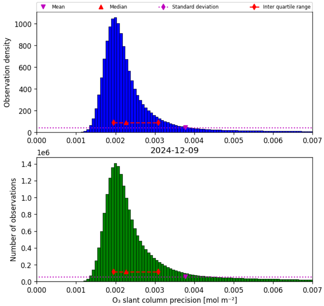
Figure 32: Histogram of “O 3 slant column precision” for 2024-12-09 to 2024-12-09
