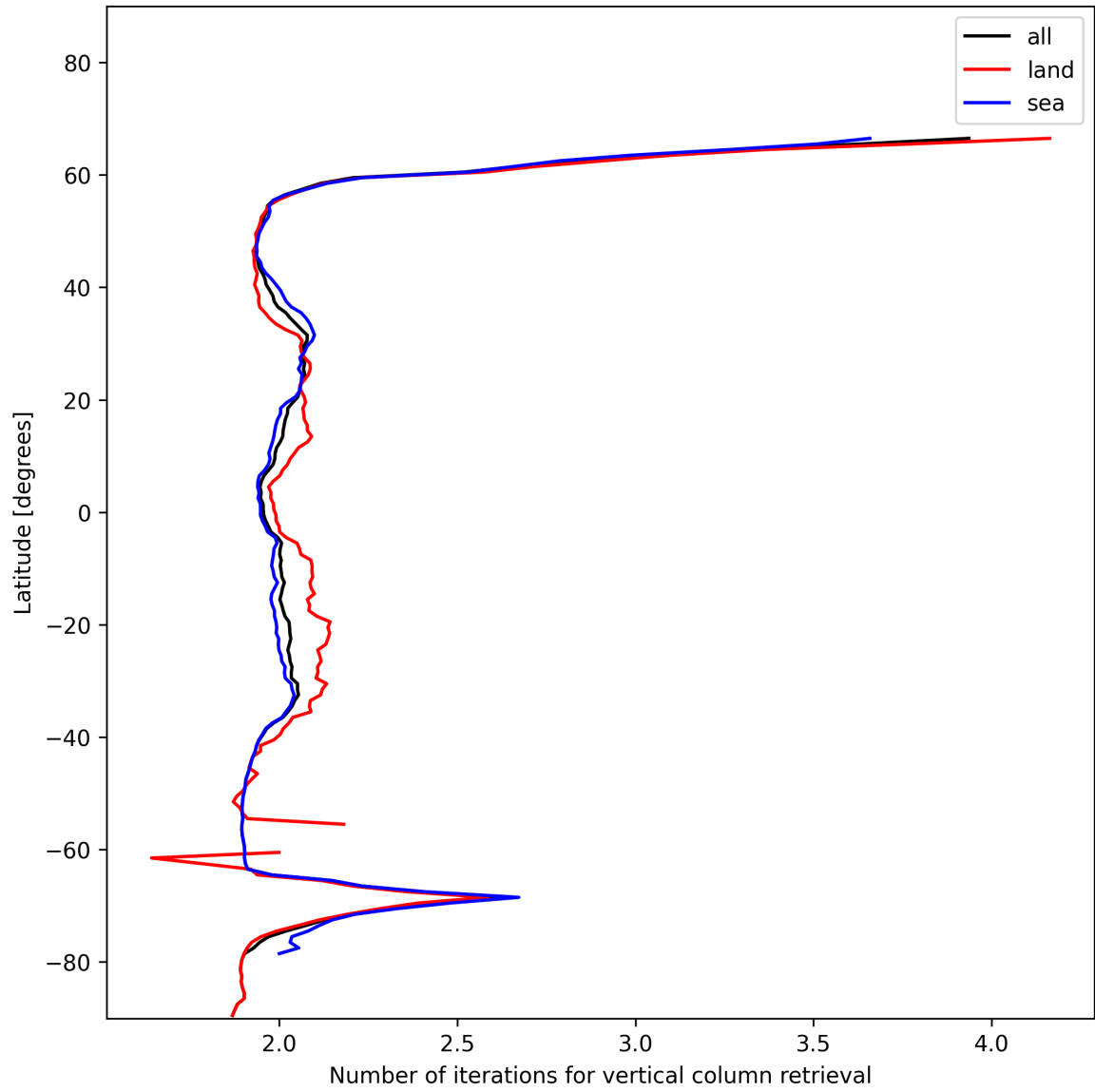
Figure 27: Zonal average of “Number of iterations for vertical column retrieval” for 2024-12-09 to 2024-12-09.
