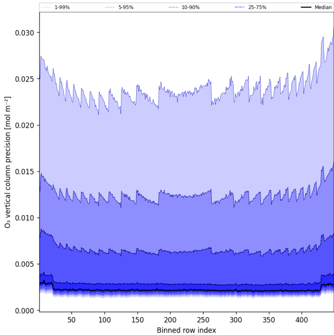
Figure 42: Along track statistics of “O 3 vertical column precision” for 2024-12-09 to 2024-12-09
