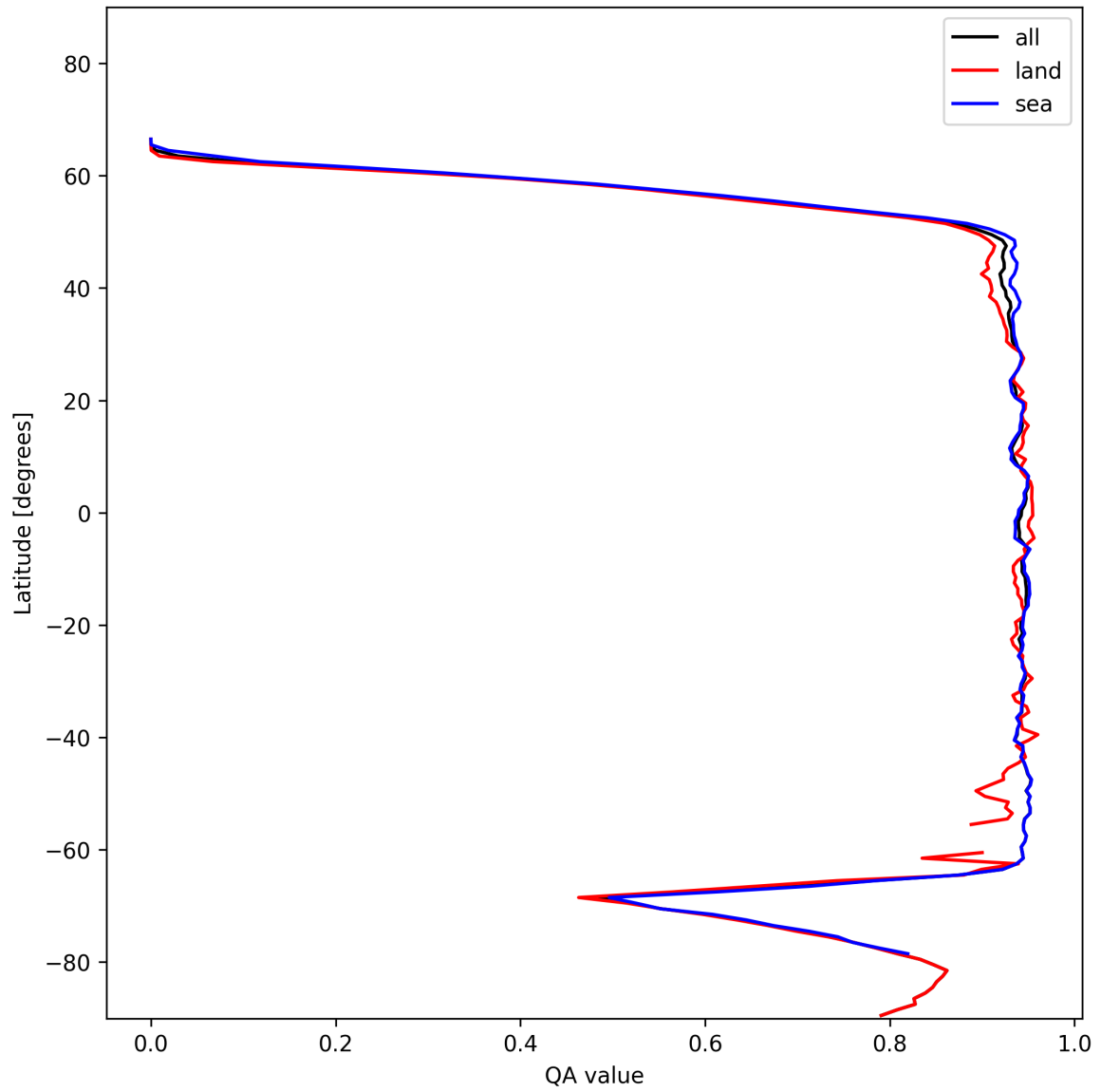
Figure 16: Zonal average of “QA value” for 2024-12-09 to 2024-12-09.
