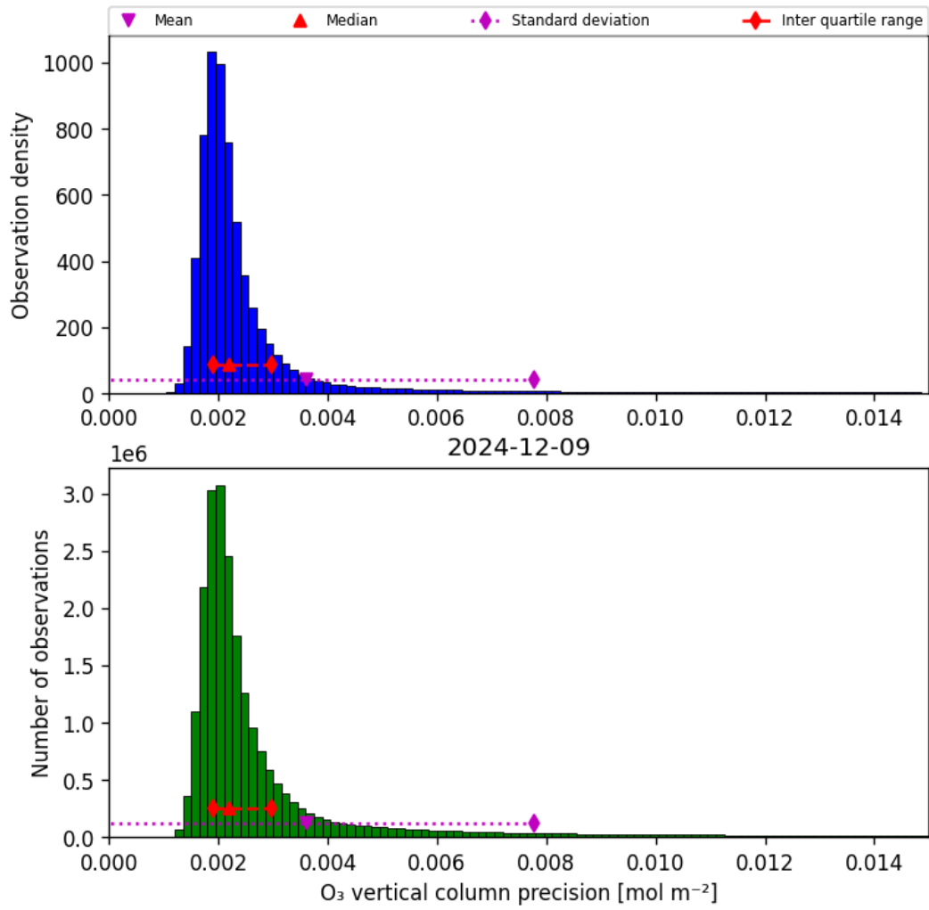
Figure 30: Histogram of “O 3 vertical column precision” for 2024-12-09 to 2024-12-09
