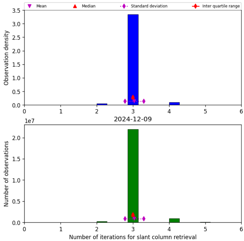
Figure 33: Histogram of "Number of iterations for slant column retrieval" for 2024-12-09 to 2024-12-09
