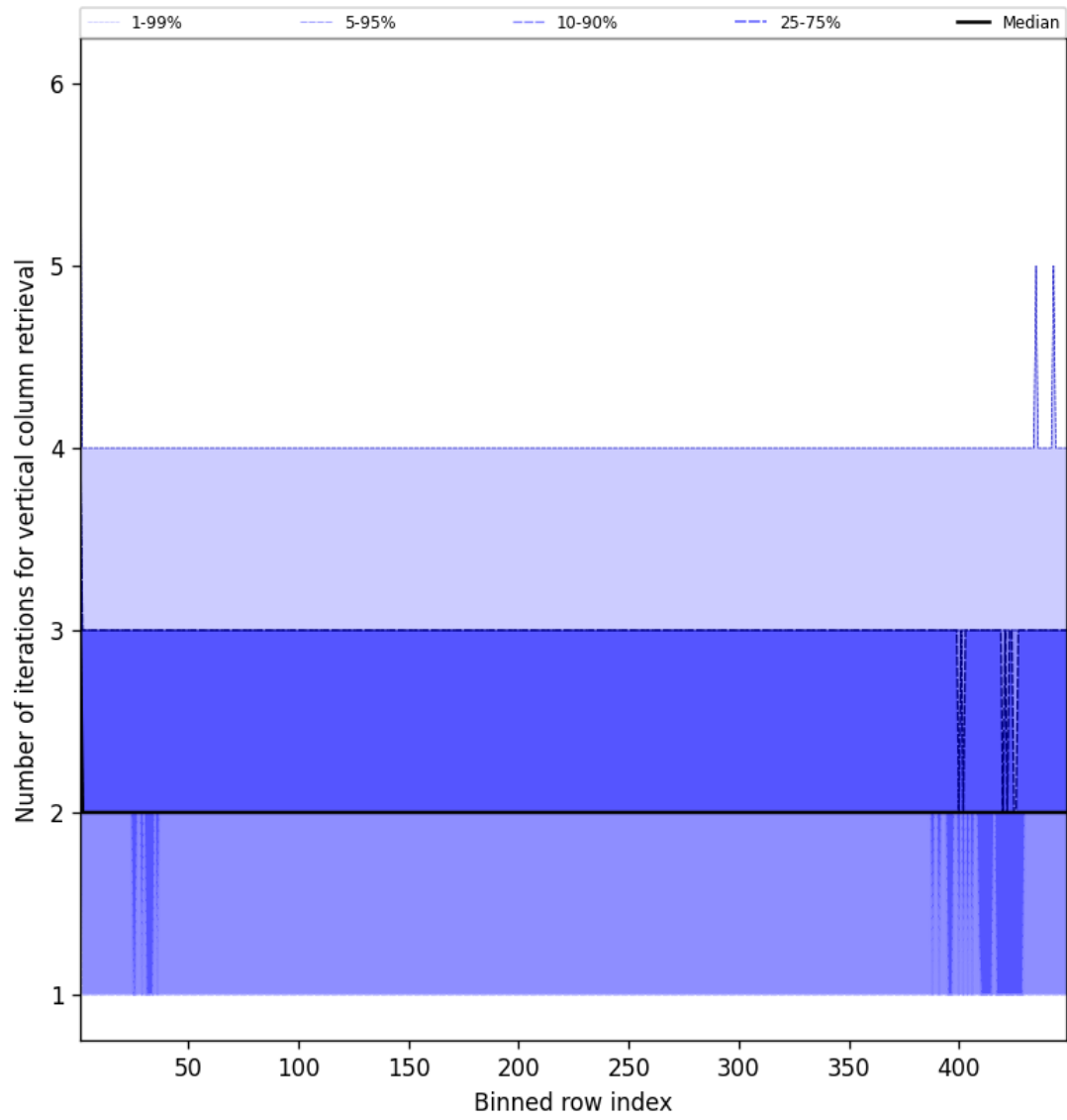
Figure 51: Along track statistics of “Number of iterations for vertical column retrieval” for 2024-12-09 to 2024-12-09
