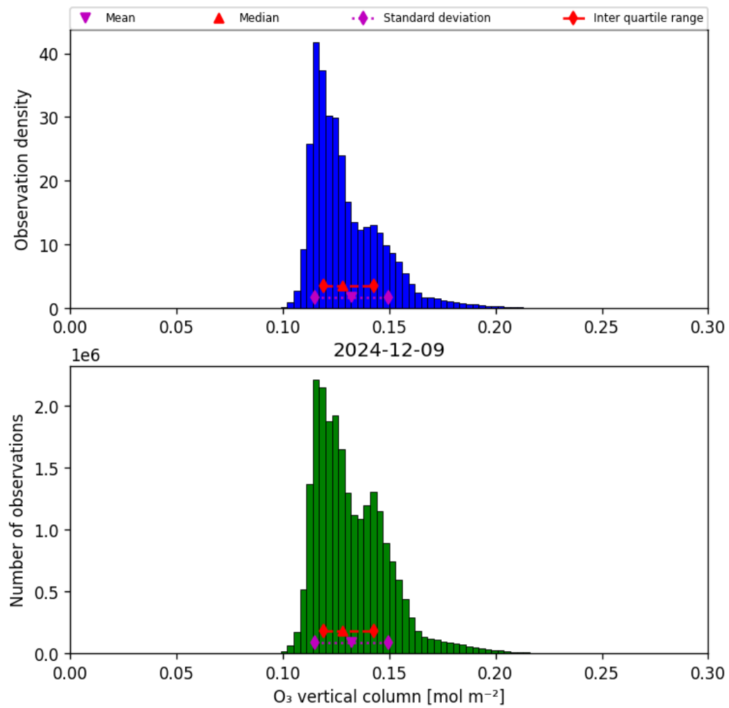
Figure 29: Histogram of “O 3 vertical column” for 2024-12-09 to 2024-12-09
