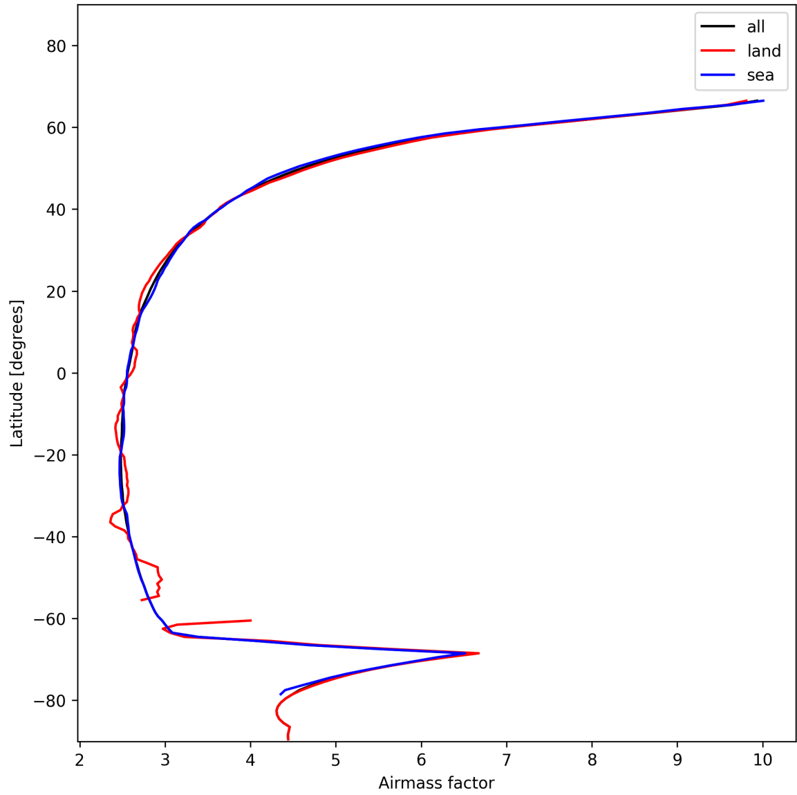
Figure 25: Zonal average of “Airmass factor” for 2024-12-09 to 2024-12-09.
