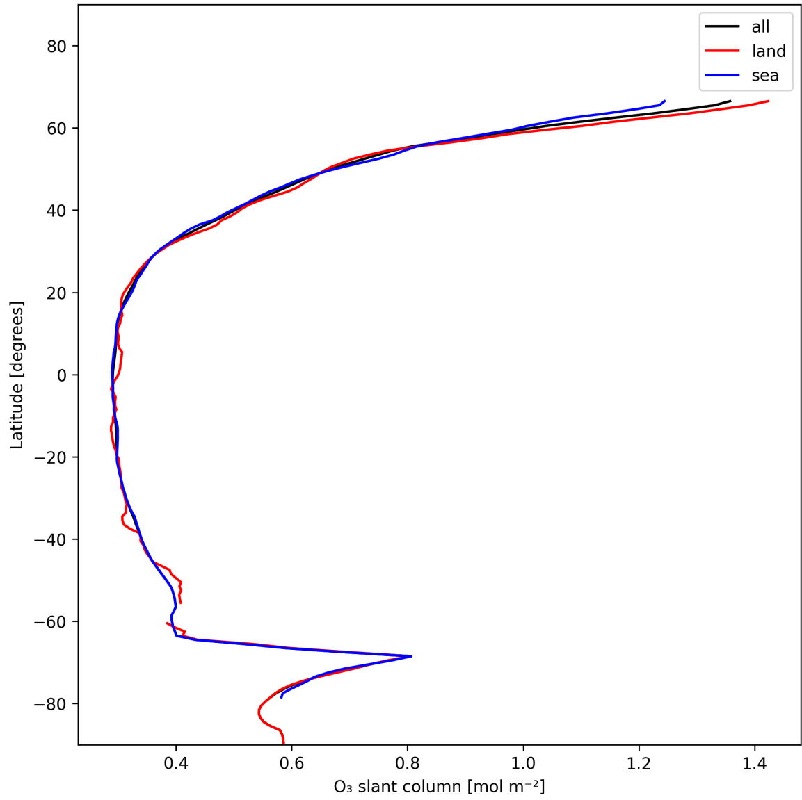
Figure 19: Zonal average of “O 3 slant column” for 2024-12-09 to 2024-12-09.
