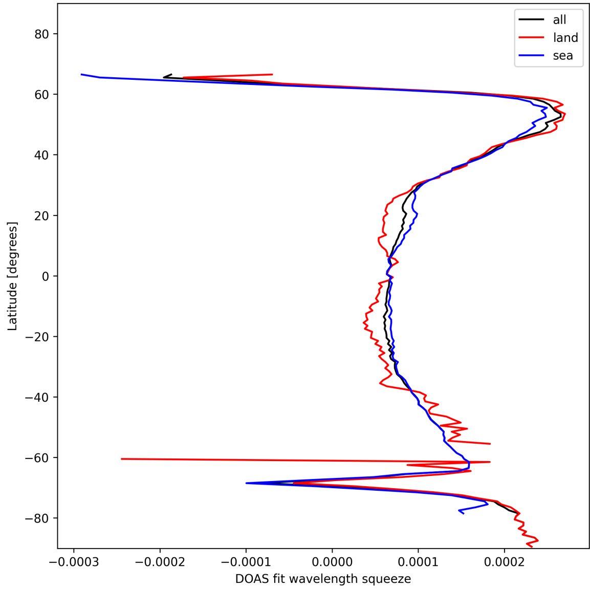
Figure 24: Zonal average of “DOAS fit wavelength squeeze” for 2024-12-09 to 2024-12-09.
