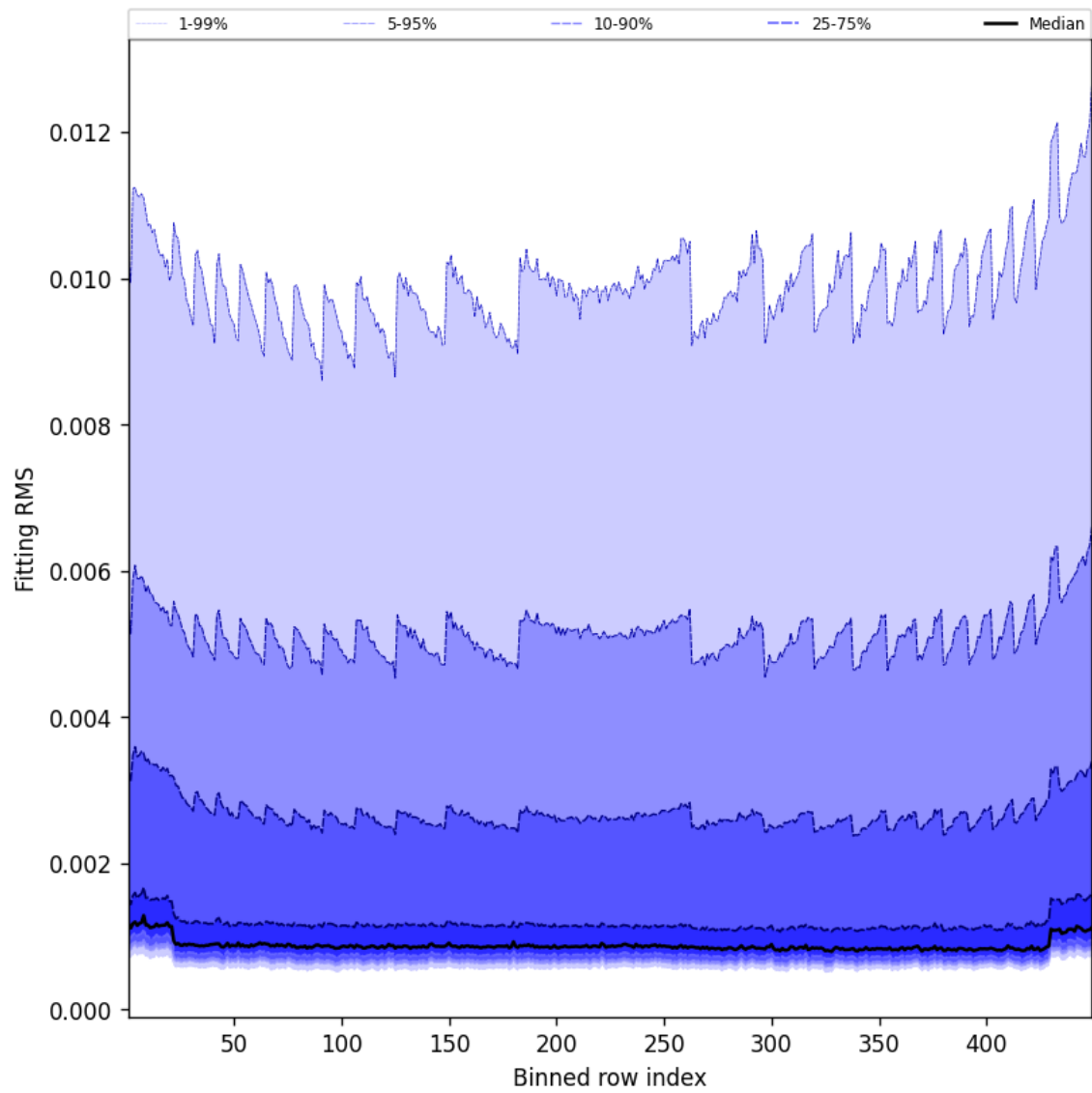
Figure 46: Along track statistics of “Fitting RMS” for 2024-12-09 to 2024-12-09
