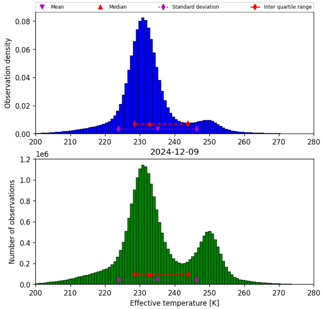
Figure 38: Histogram of “Effective temperature” for 2024-12-09 to 2024-12-09
