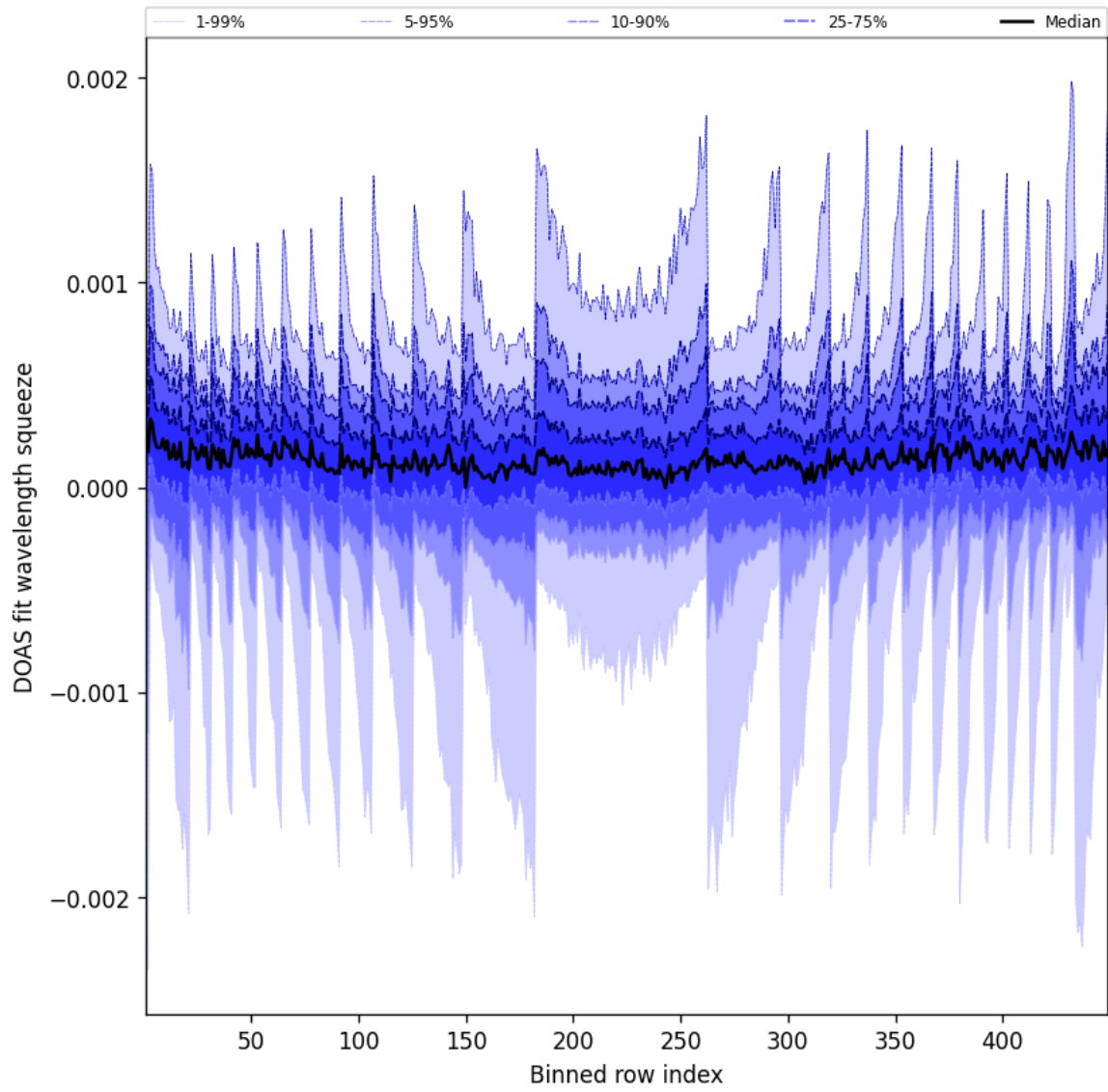
Figure 48: Along track statistics of “DOAS fit wavelength squeeze” for 2024-12-09 to 2024-12-09
