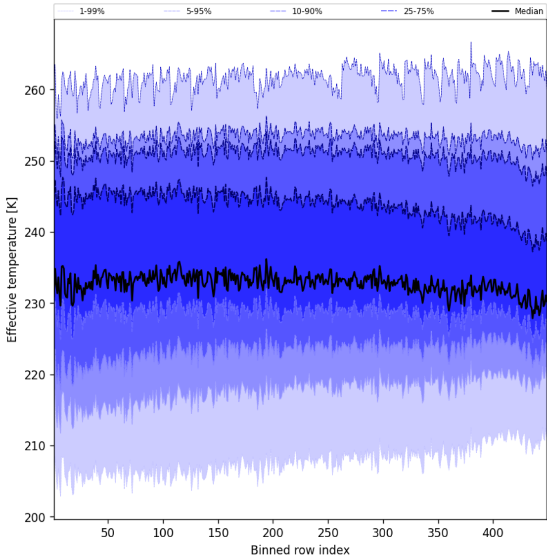
Figure 50: Along track statistics of “Effective temperature” for 2024-12-09 to 2024-12-09
