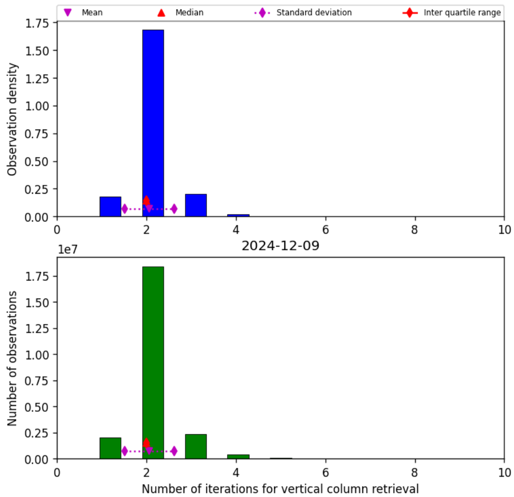
Figure 39: Histogram of “Number of iterations for vertical column retrieval” for 2024-12-09 to 2024-12-09
