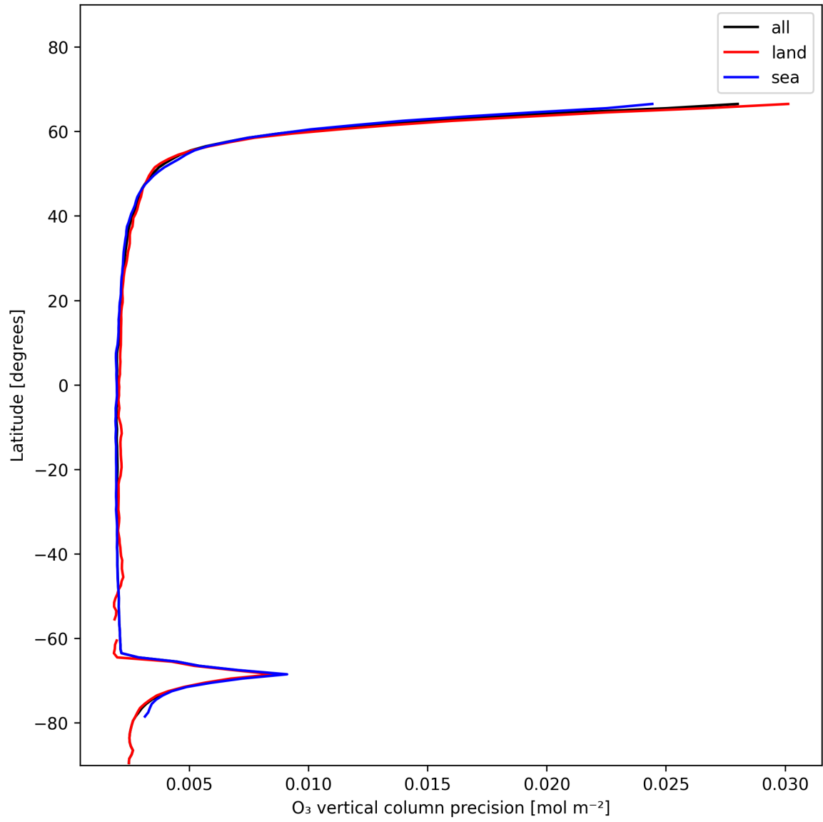
Figure 18: Zonal average of “O 3 vertical column precision” for 2024-12-09 to 2024-12-09.
