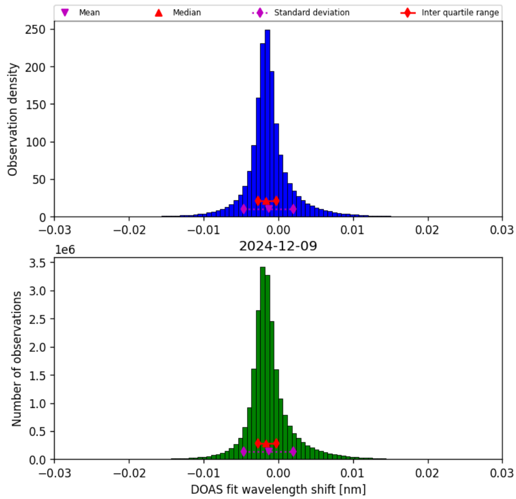
Figure 35: Histogram of “DOAS fit wavelength shift” for 2024-12-09 to 2024-12-09
