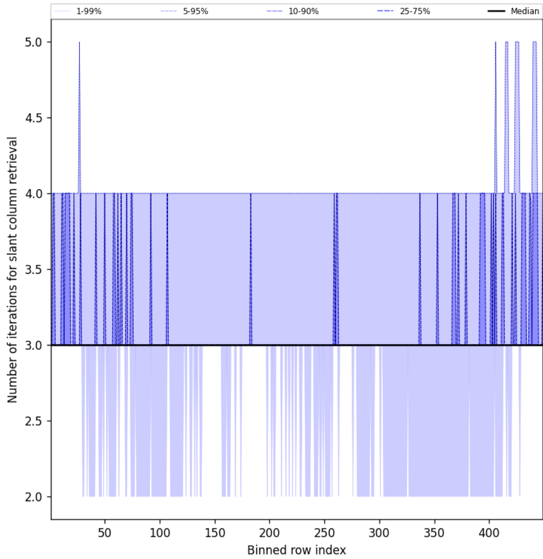
Figure 45: Along track statistics of “Number of iterations for slant column retrieval” for 2024-12-09 to 2024-12-09
