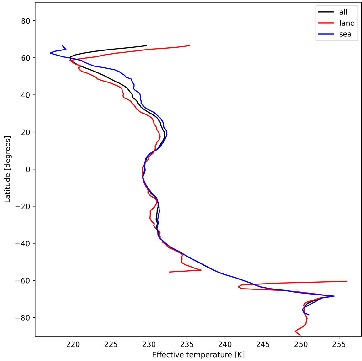
Figure 26: Zonal average of “Effective temperature” for 2024-12-09 to 2024-12-09.
