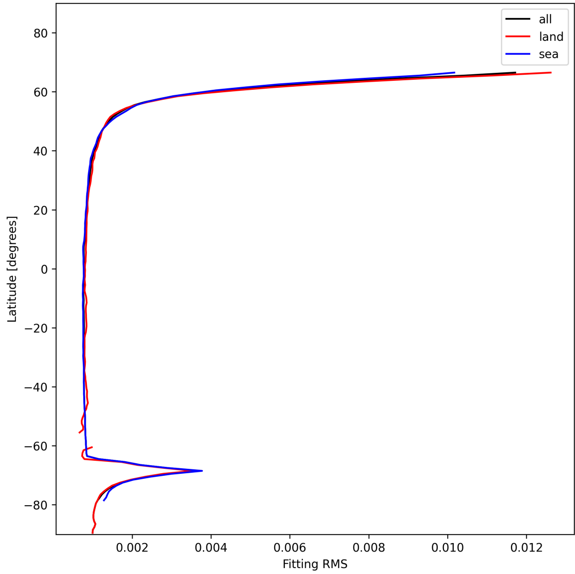
Figure 22: Zonal average of “Fitting RMS” for 2024-12-09 to 2024-12-09.
