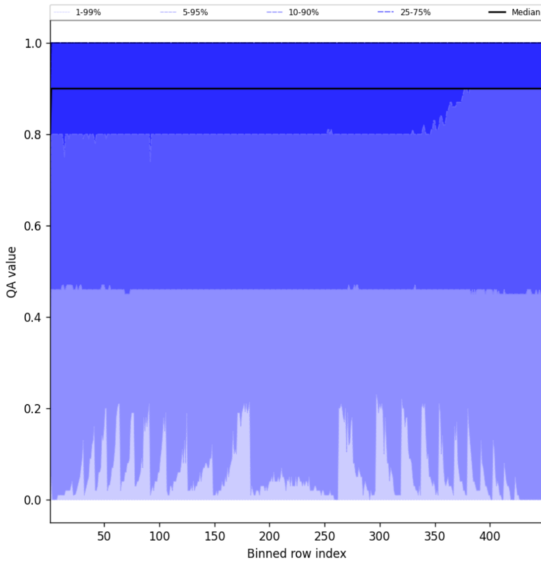
Figure 40: Along track statistics of “QA value” for 2024-12-09 to 2024-12-09
