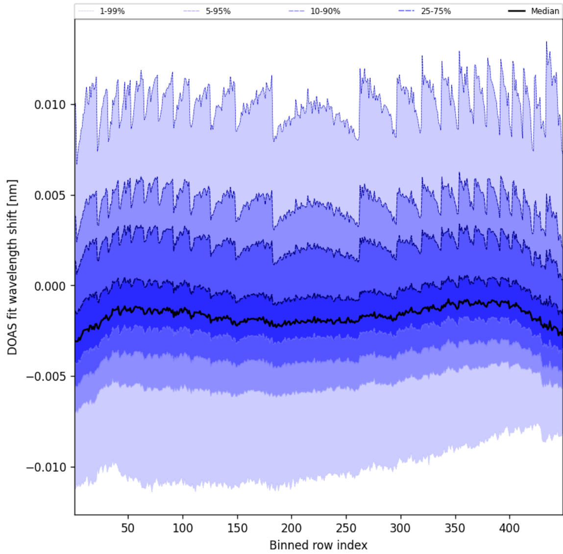
Figure 47: Along track statistics of “DOAS fit wavelength shift” for 2024-12-09 to 2024-12-09
