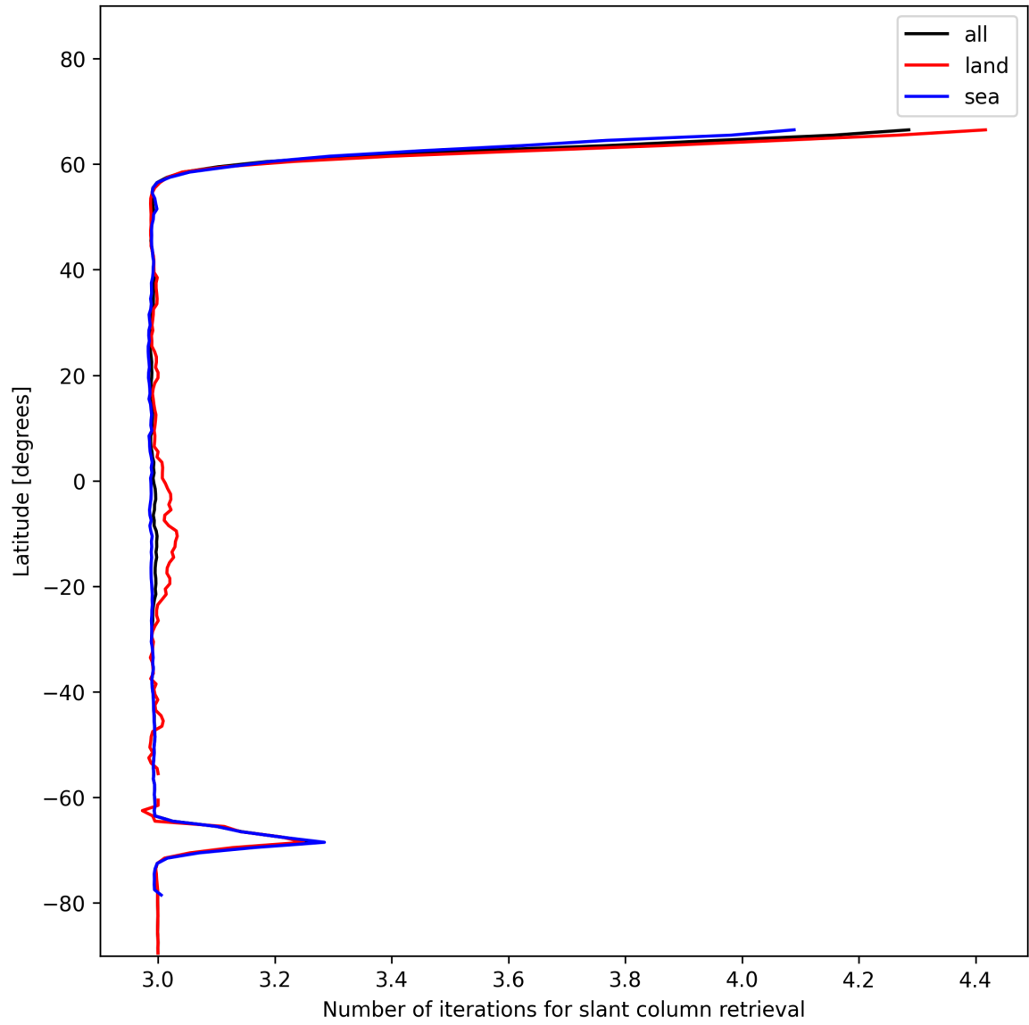
Figure 21: Zonal average of “Number of iterations for slant column retrieval” for 2024-12-09 to 2024-12-09.
