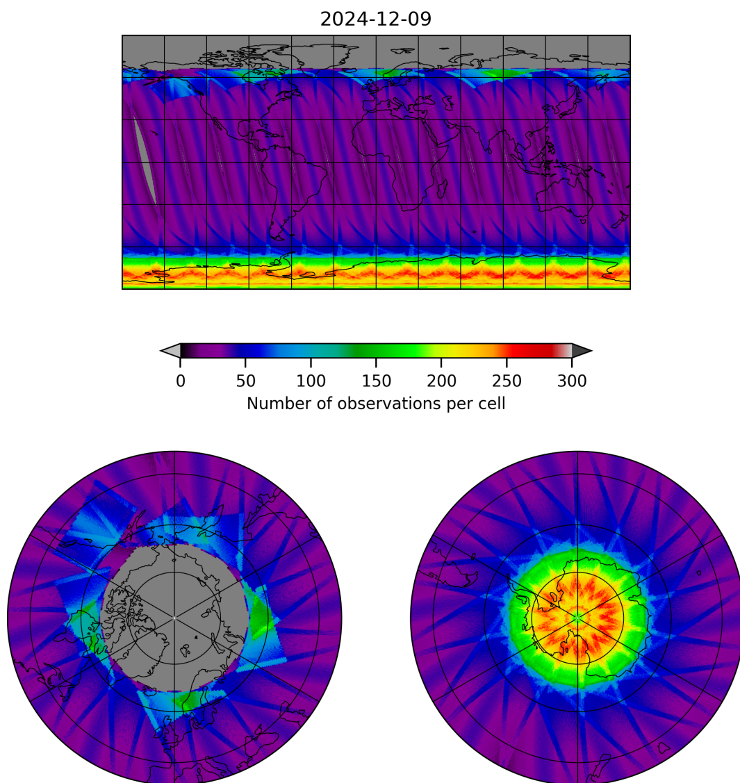
Figure 15: Map of the number of observations for 2024-12-09 to 2024-12-09
