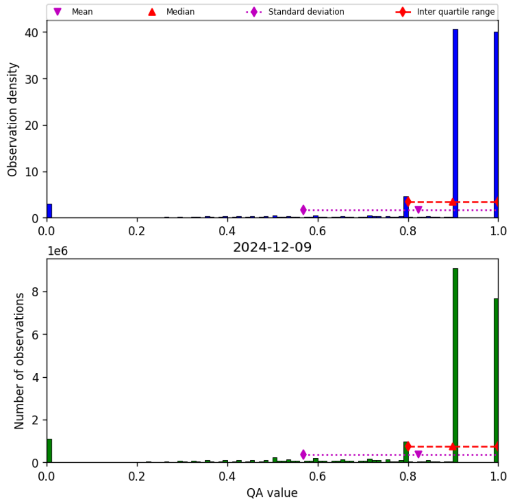
Figure 28: Histogram of “QA value” for 2024-12-09 to 2024-12-09
