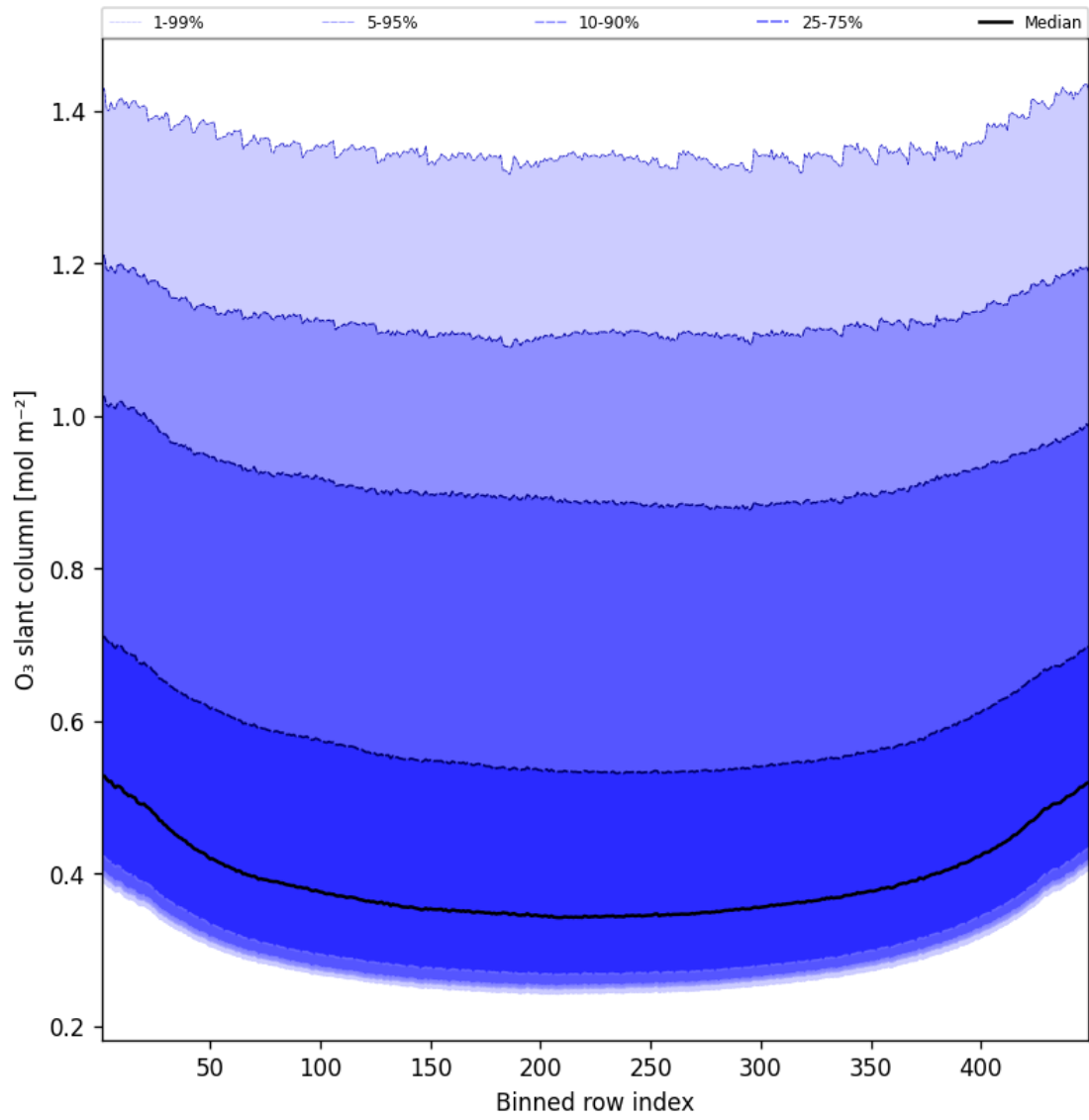
Figure 43: Along track statistics of “O 3 slant column” for 2024-12-09 to 2024-12-09
