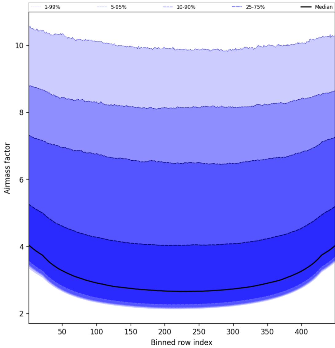
Figure 49: Along track statistics of “Airmass factor” for 2024-12-09 to 2024-12-09
