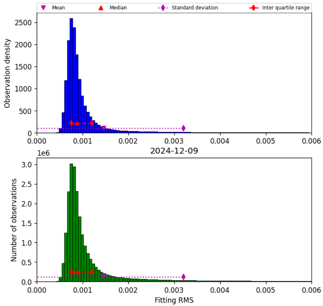
Figure 34: Histogram of “Fitting RMS” for 2024-12-09 to 2024-12-09
