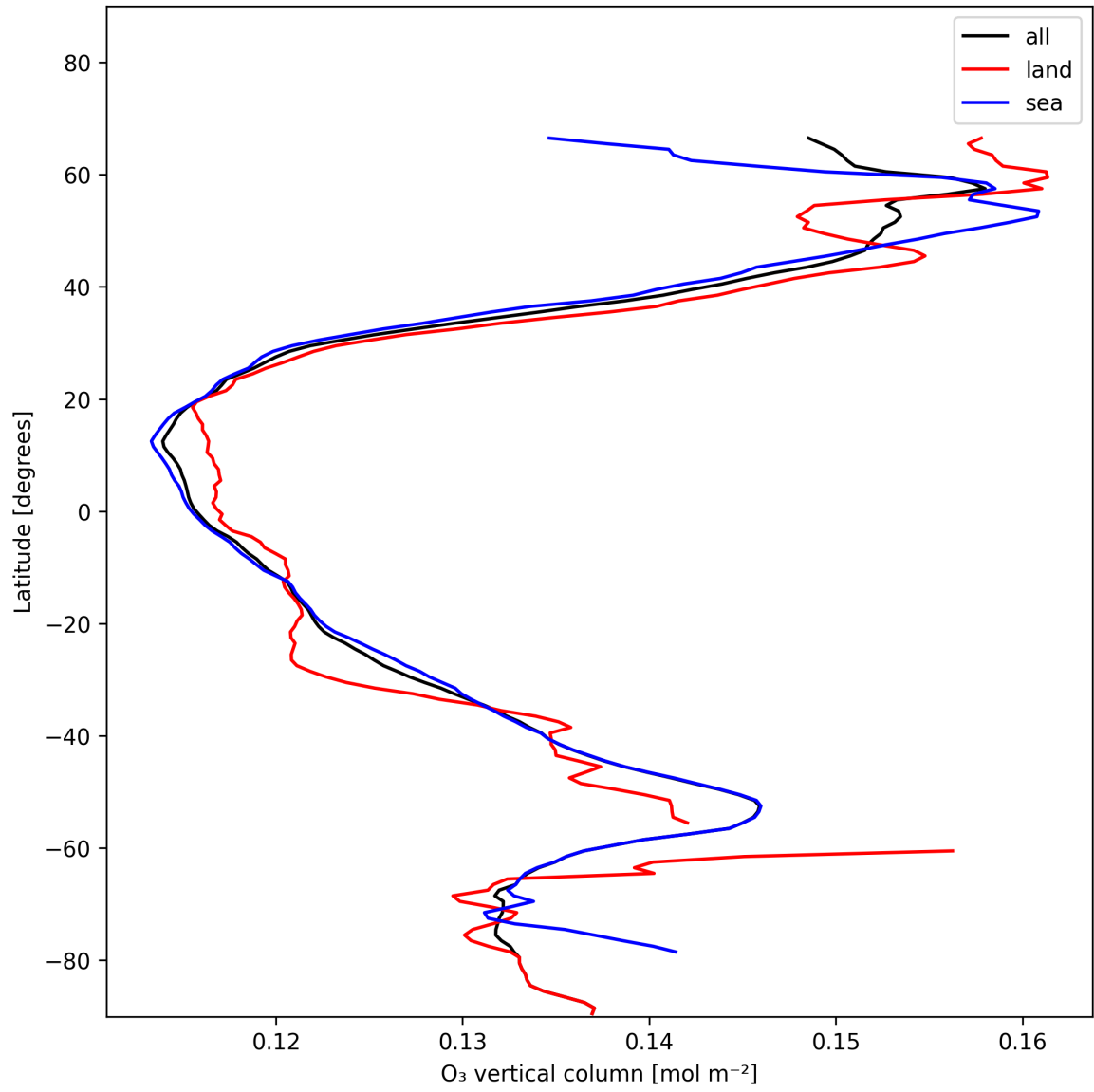
Figure 17: Zonal average of “O 3 vertical column” for 2024-12-09 to 2024-12-09.
