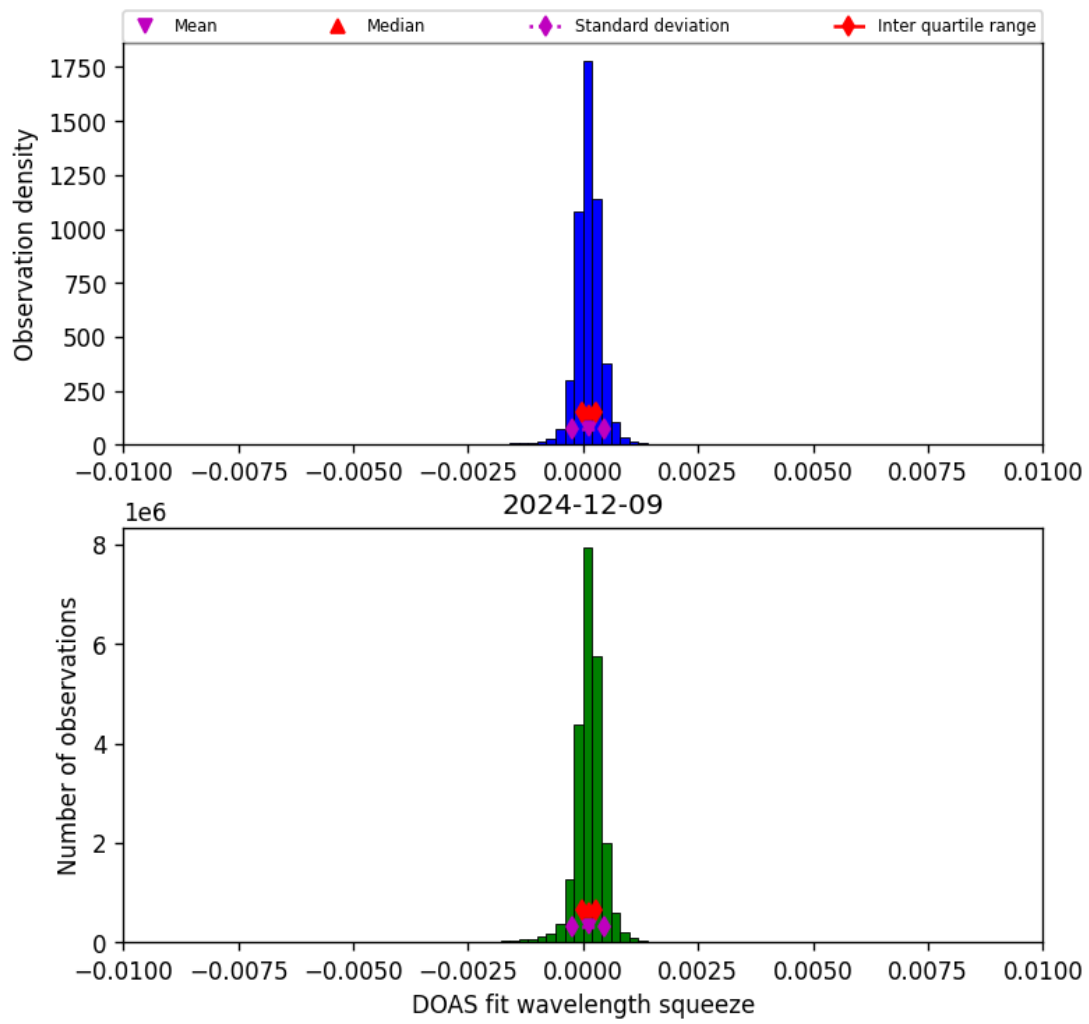
Figure 36: Histogram of “DOAS fit wavelength squeeze” for 2024-12-09 to 2024-12-09
